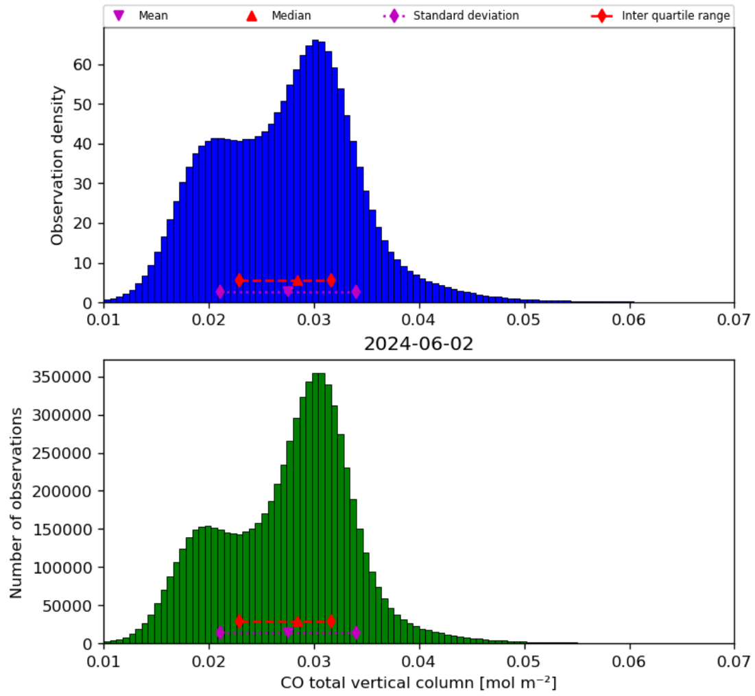
Figure 18: Histogram of “CO total vertical column” for 2024-06-01 to 2024-06-03
