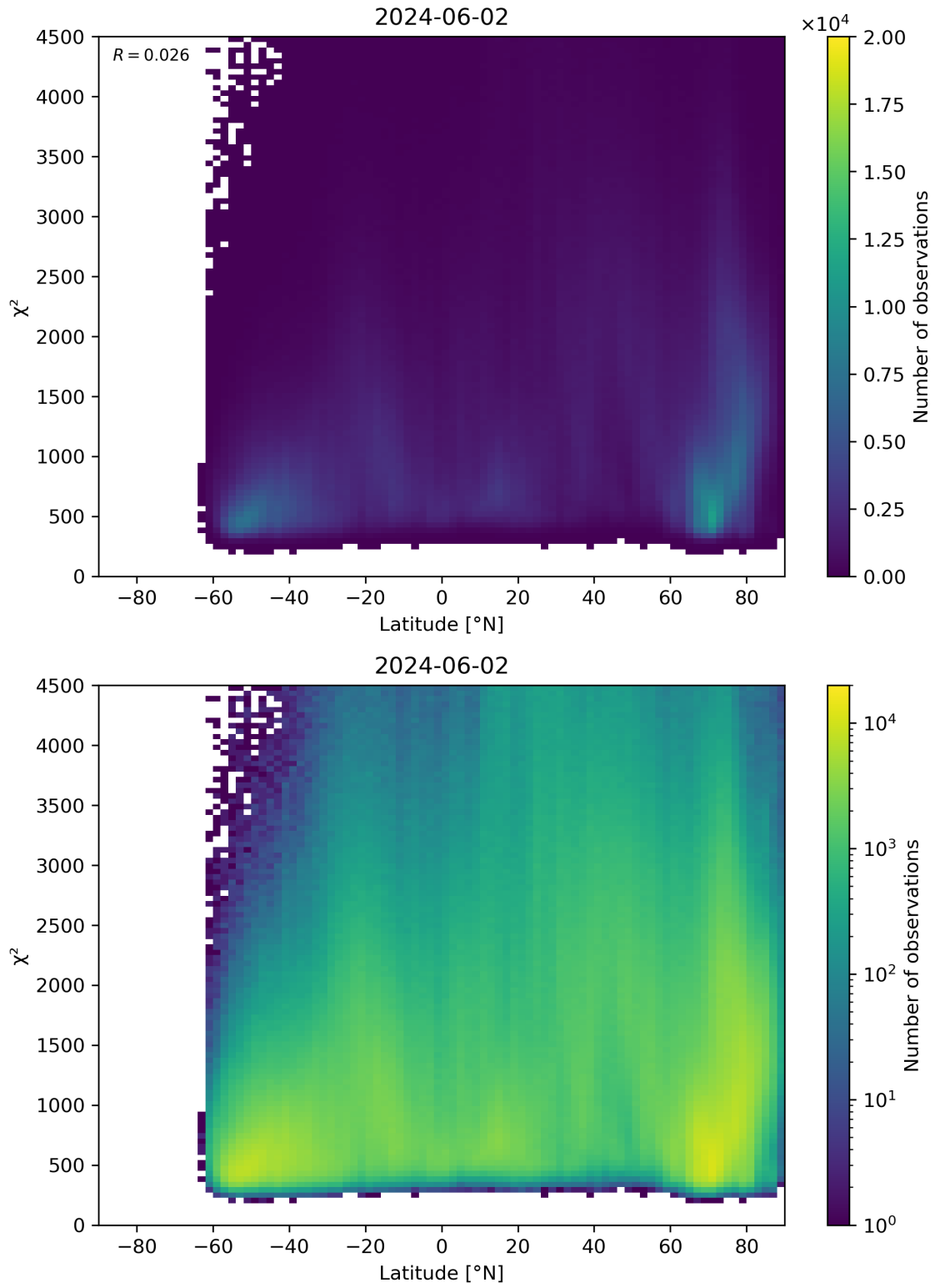
Figure 54: Scatter density plot of “Latitude” against “ \chi^2 ” for 2024-06-01 to 2024-06-03.
