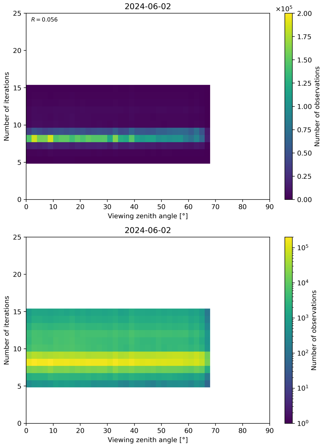
Figure 75: Scatter density plot of “Viewing zenith angle” against “Number of iterations” for 2024-06-01 to 2024-06-03.
