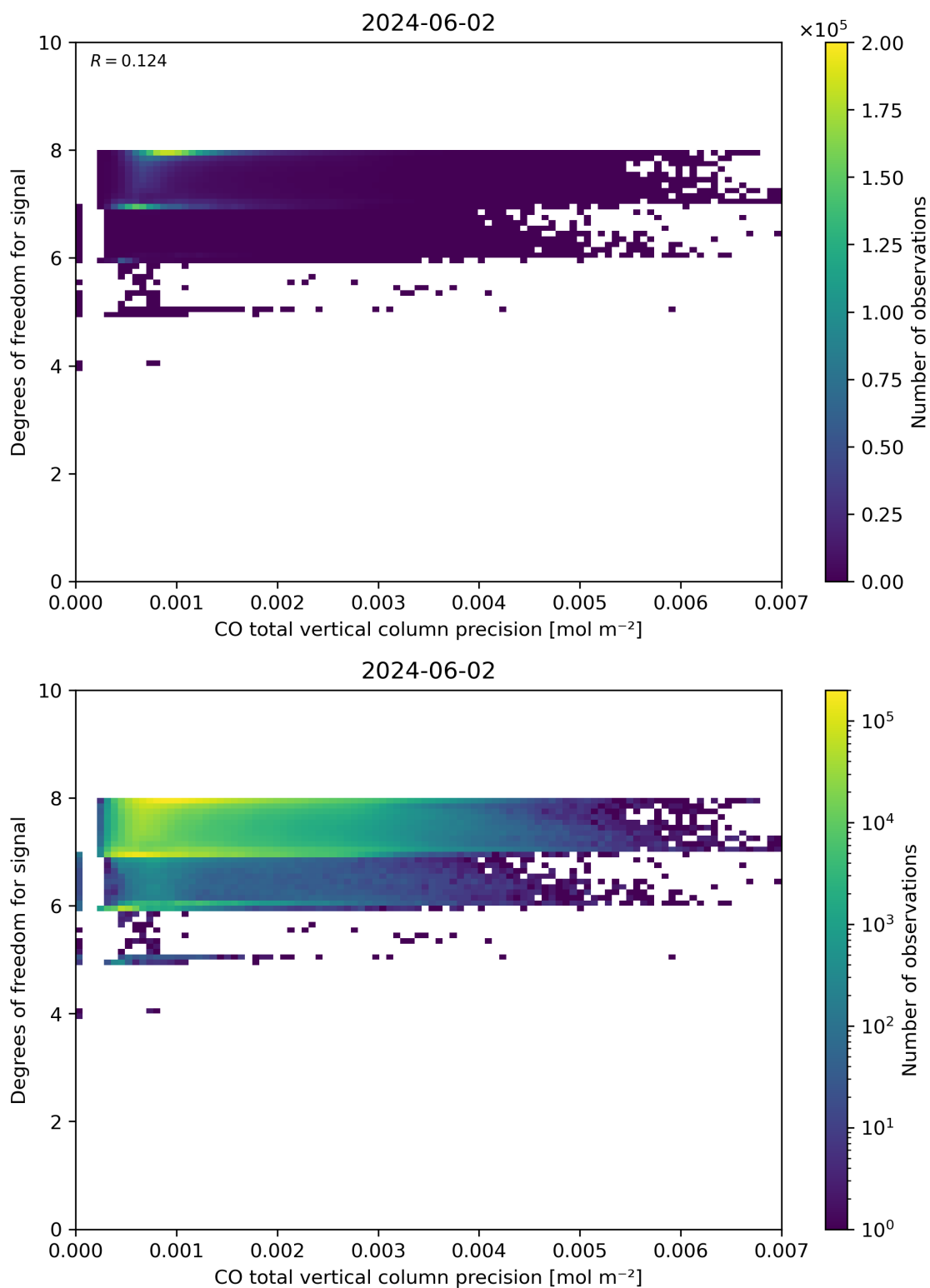
Figure 45: Scatter density plot of “CO total vertical column precision” against “Degrees of freedom for signal” for 2024-06-01 to 2024-06-03.
