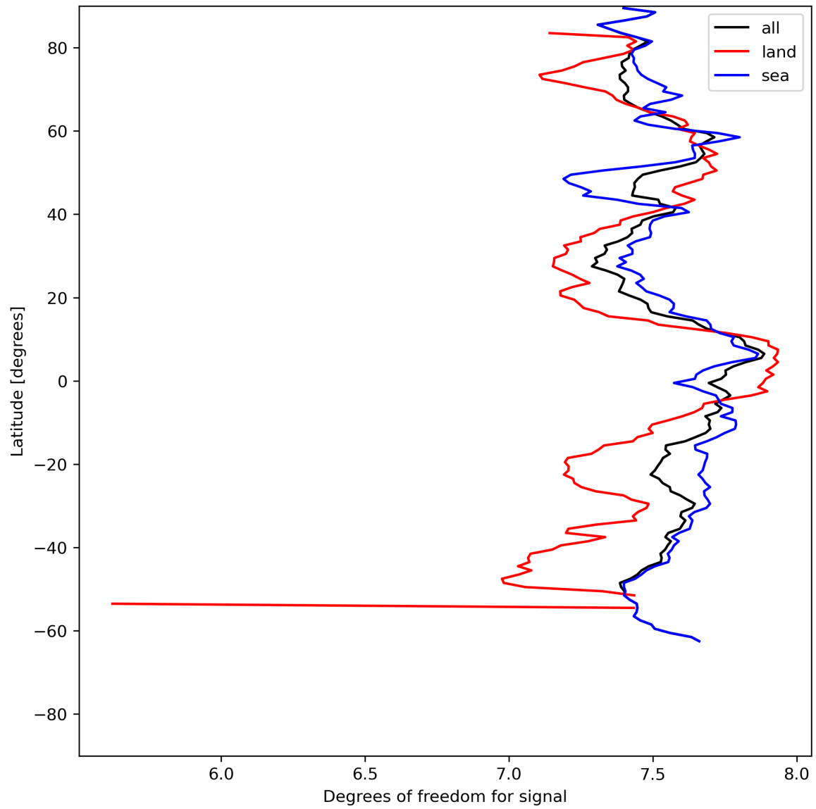
Figure 15: Zonal average of “Degrees of freedom for signal” for 2024-06-01 to 2024-06-03.
