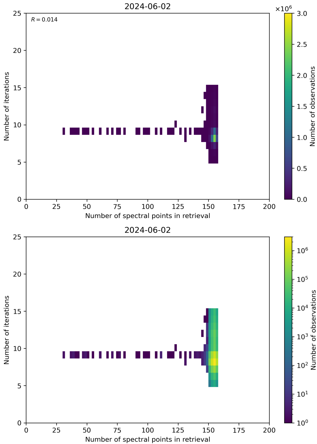
Figure 60: Scatter density plot of “Number of spectral points in retrieval” against “Number of iterations” for 2024-06-01 to 2024-06-03.
