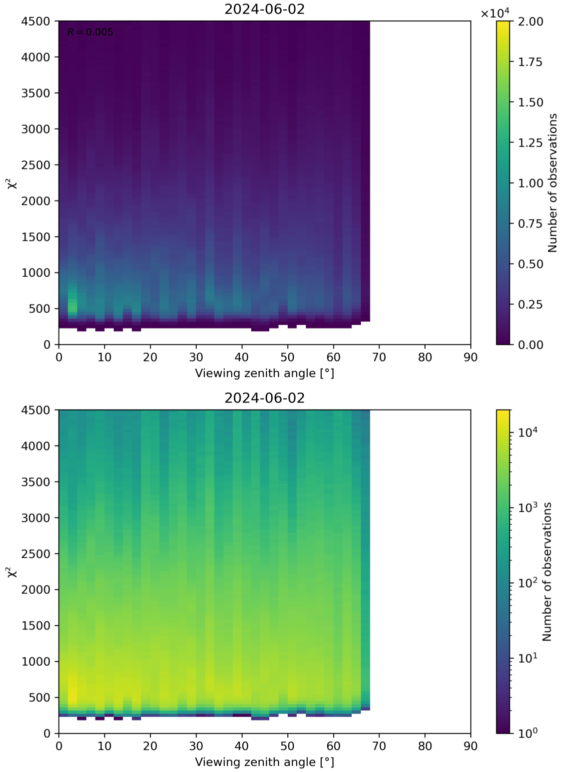
Figure 72: Scatter density plot of “Viewing zenith angle” against “ \chi^2 ” for 2024-06-01 to 2024-06-03.
