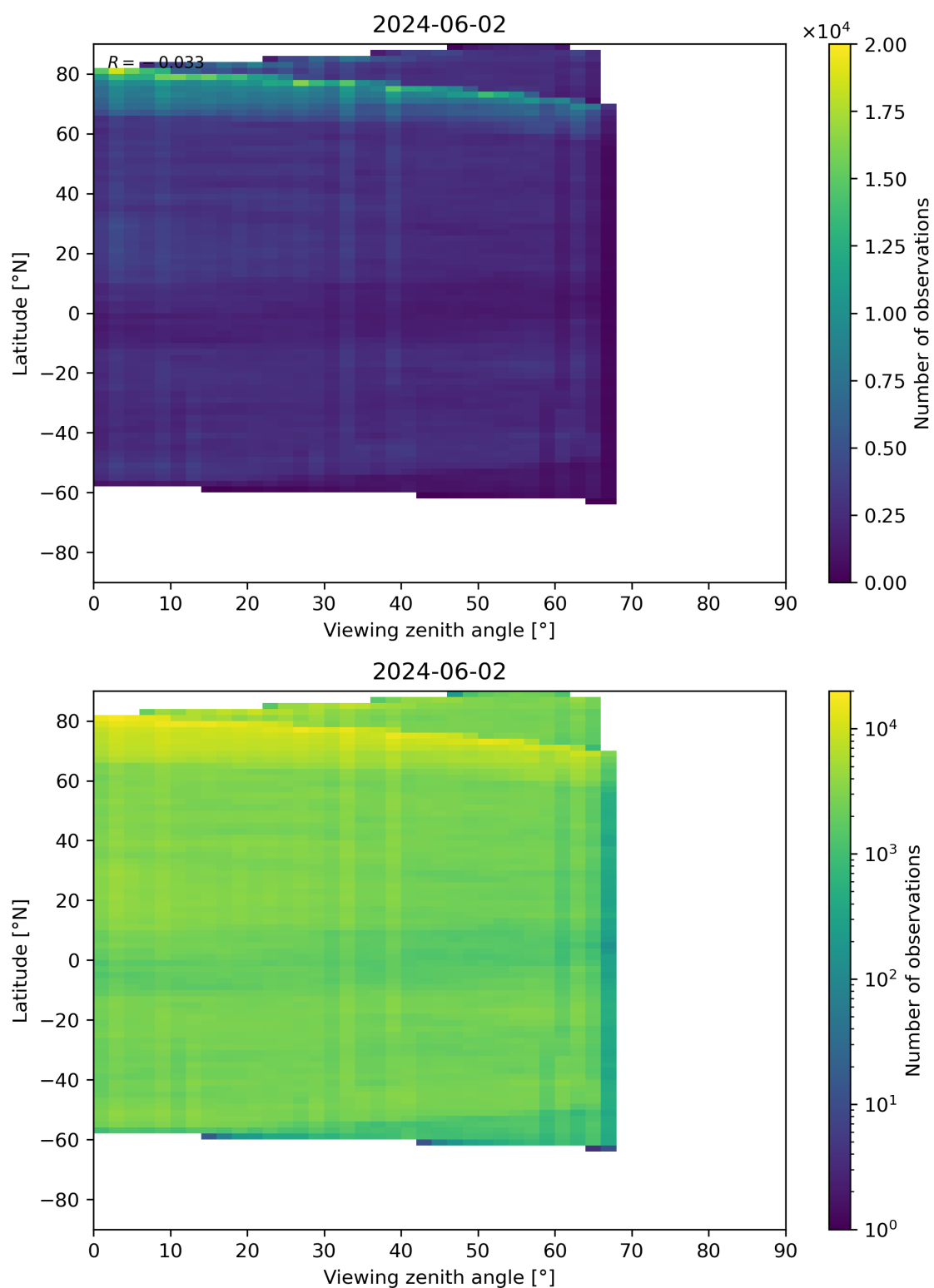
Figure 74: Scatter density plot of “Viewing zenith angle” against “Latitude” for 2024-06-01 to 2024-06-03.
