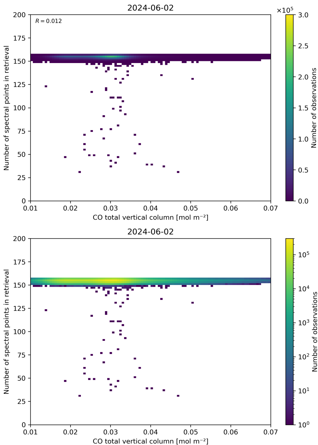
Figure 43: Scatter density plot of “CO total vertical column” against “Number of spectral points in retrieval” for 2024-06-01 to 2024-06-03.
