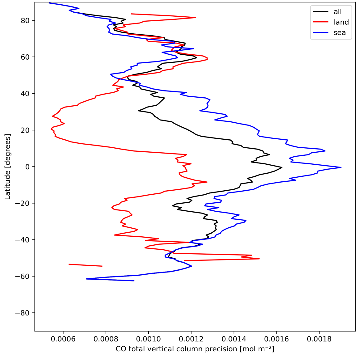
Figure 12: Zonal average of “CO total vertical column precision” for 2024-06-01 to 2024-06-03.
