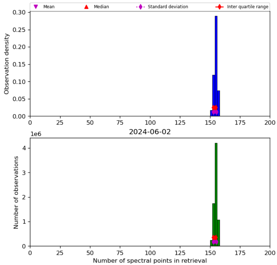
Figure 21: Histogram of “Number of spectral points in retrieval” for 2024-06-01 to 2024-06-03
