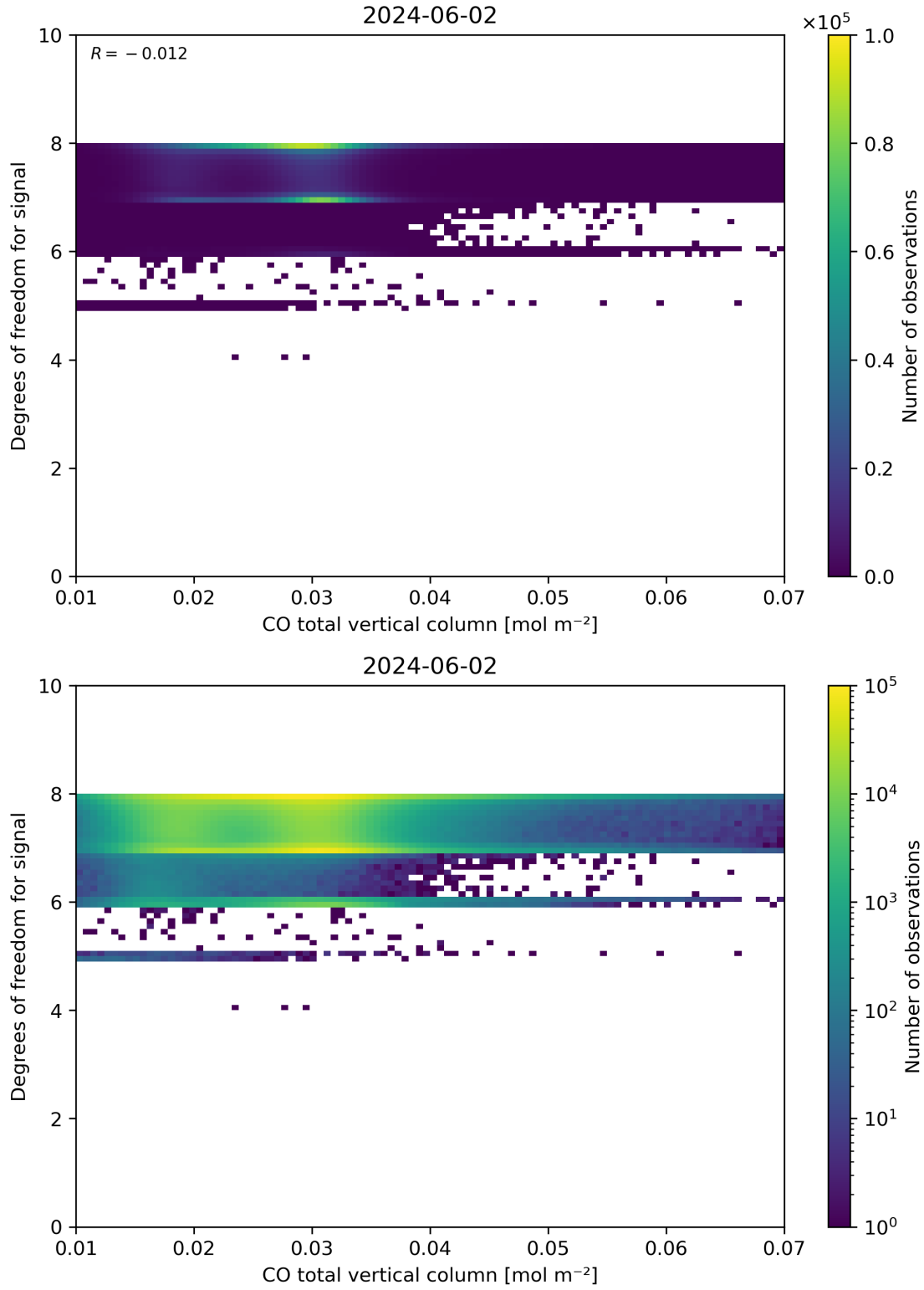
Figure 41: Scatter density plot of “CO total vertical column” against “Degrees of freedom for signal” for 2024-06-01 to 2024-06-03.
