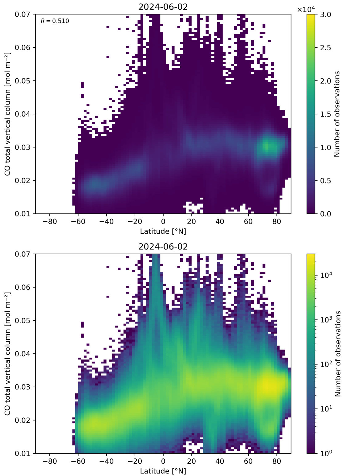
Figure 51: Scatter density plot of “Latitude” against “CO total vertical column” for 2024-06-01 to 2024-06-03.
