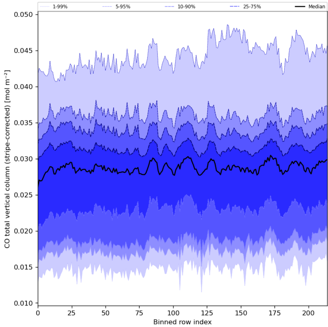
Figure 27: Along track statistics of “CO total vertical column (stripe-corrected)” for 2024-06-01 to 2024-06-03
