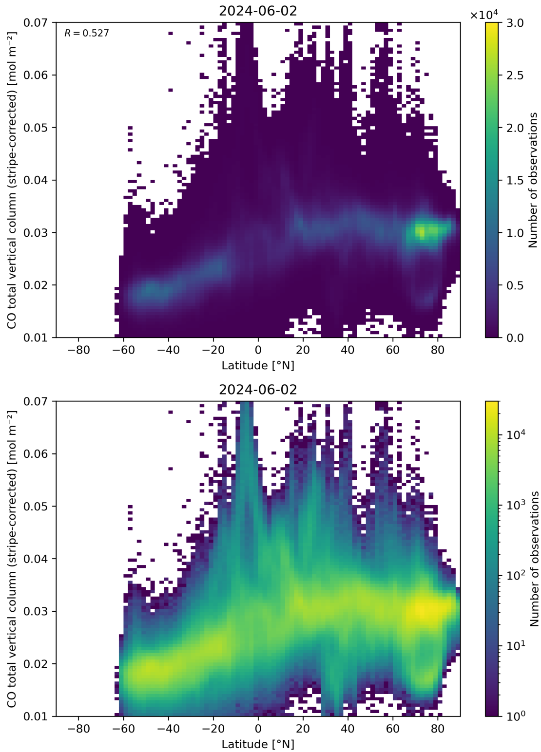
Figure 52: Scatter density plot of “Latitude” against “CO total vertical column (stripe-corrected)” for 2024-06-01 to 2024-06-03.
