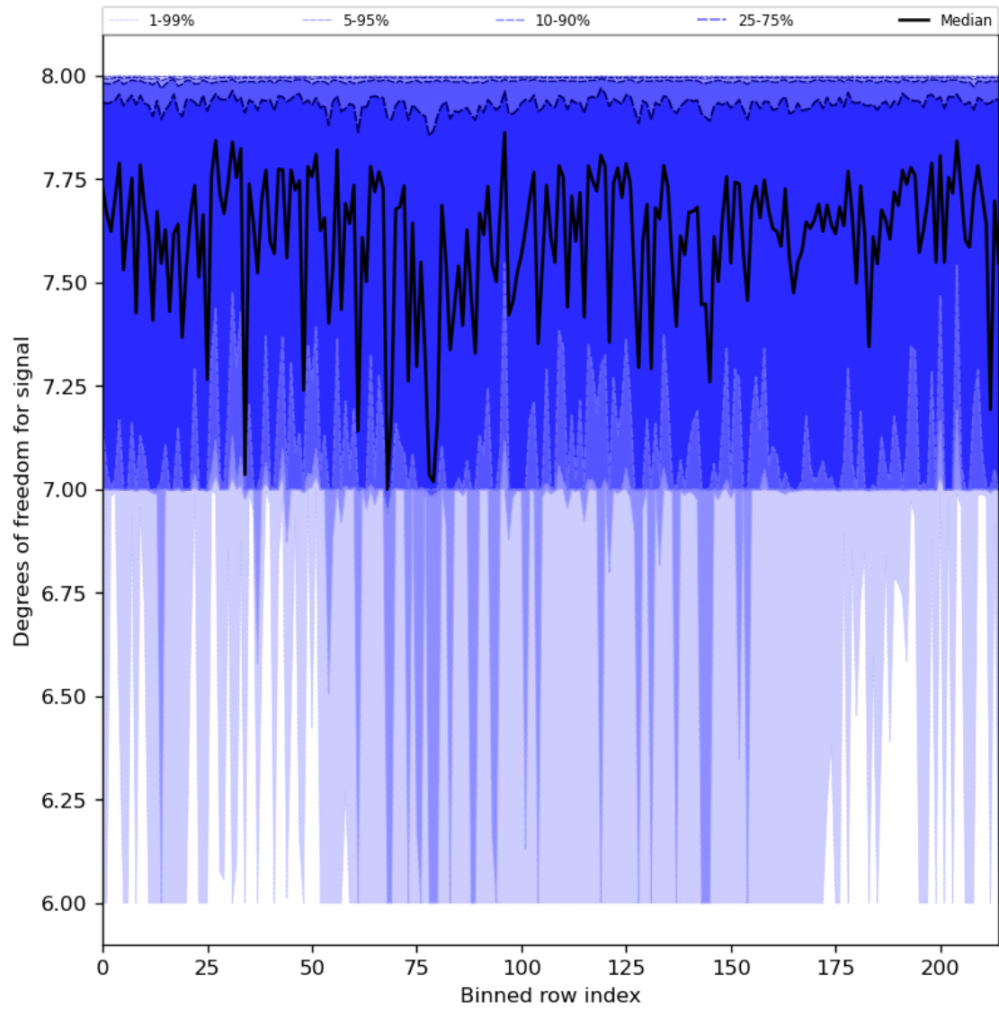
Figure 31: Along track statistics of “Degrees of freedom for signal” for 2024-06-01 to 2024-06-03
