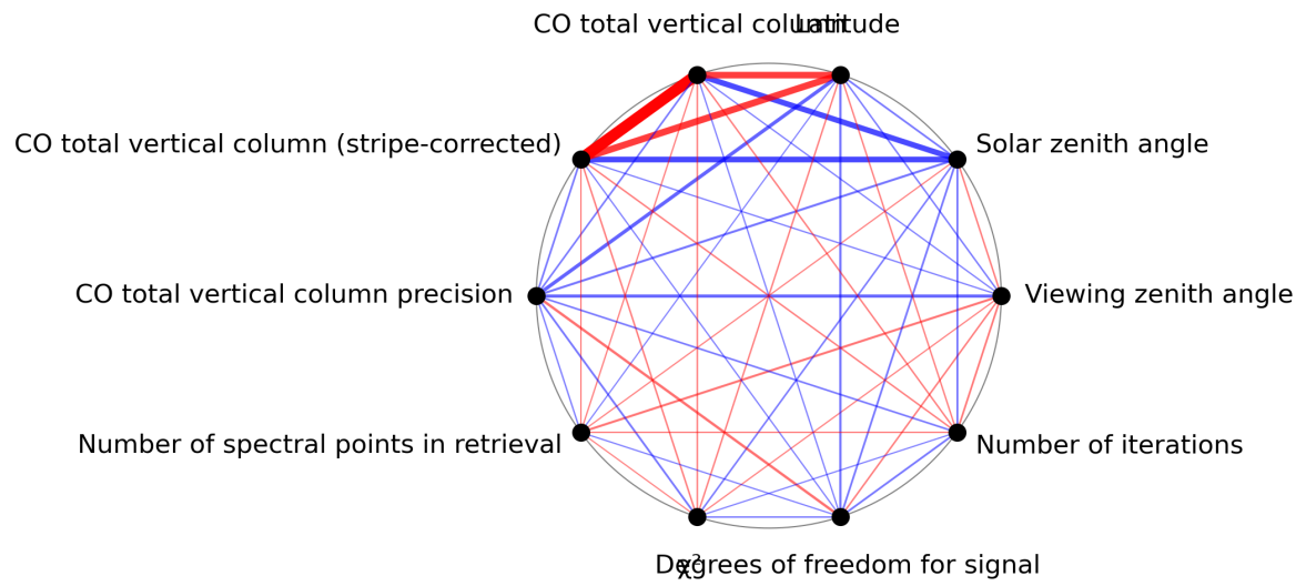
Figure 1: Map of correlation graph for 2024-06-01 to 2024-06-03.
