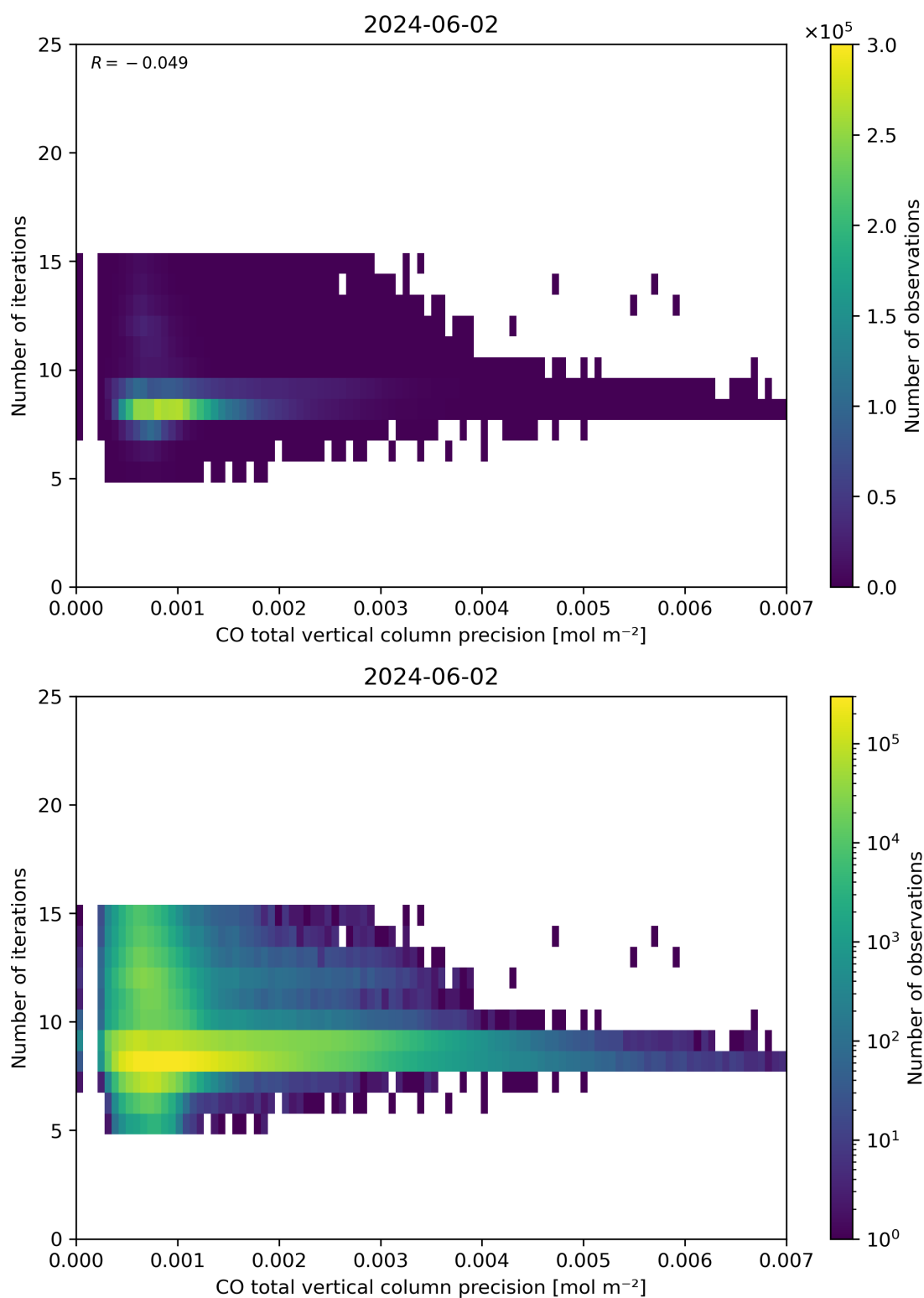
Figure 46: Scatter density plot of “CO total vertical column precision” against “Number of iterations” for 2024-06-01 to 2024-06-03.
