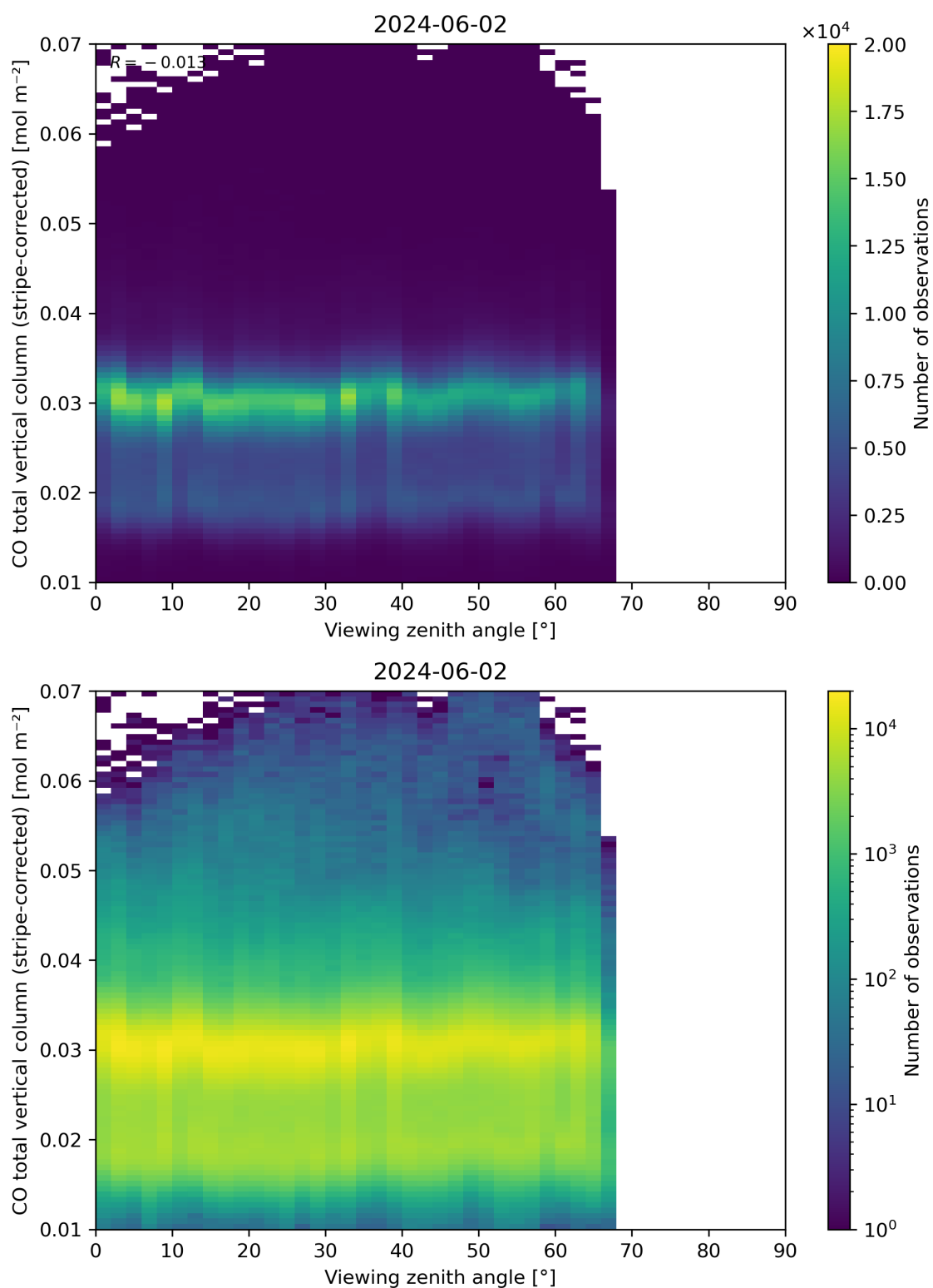
Figure 70: Scatter density plot of “Viewing zenith angle” against “CO total vertical column (stripe-corrected)” for 2024-06-01 to 2024-06-03.
