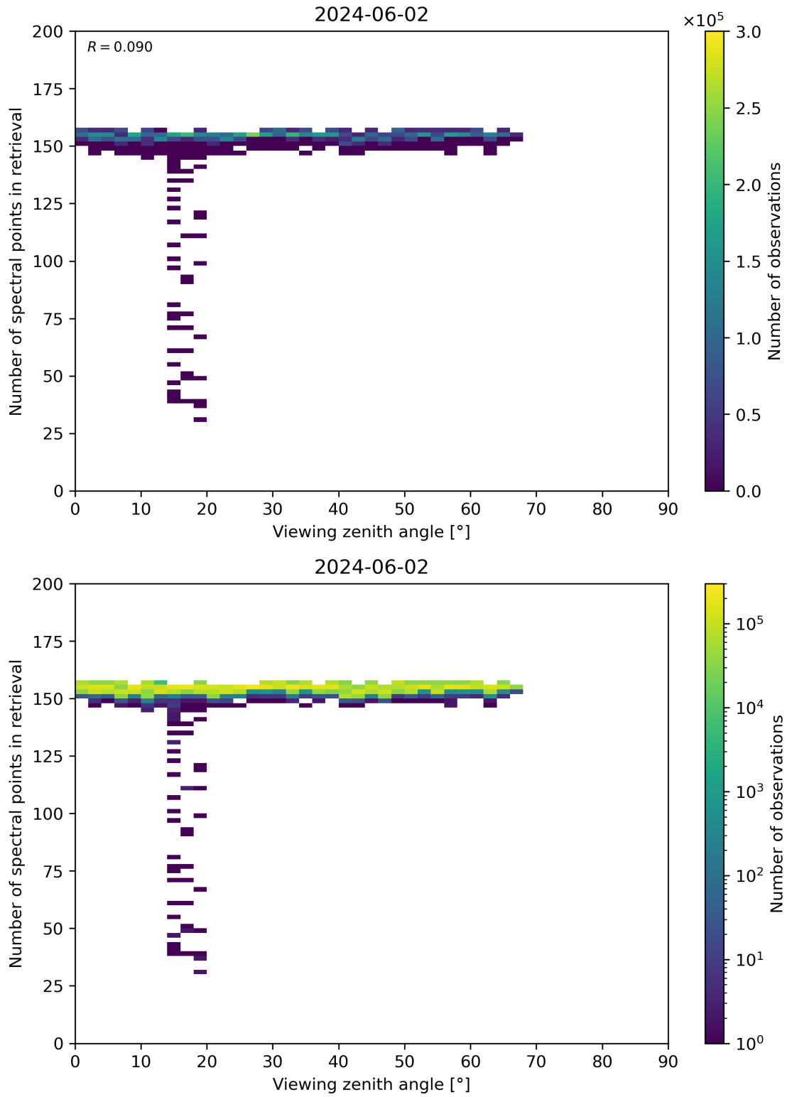
Figure 76: Scatter density plot of “Viewing zenith angle” against “Number of spectral points in retrieval” for 2024-06-01 to 2024-06-03.
