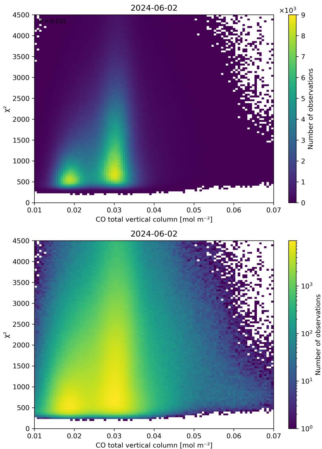
Figure 35: Scatter density plot of “CO total vertical column” against “ \chi^2 ” for 2024-06-01 to 2024-06-03.
