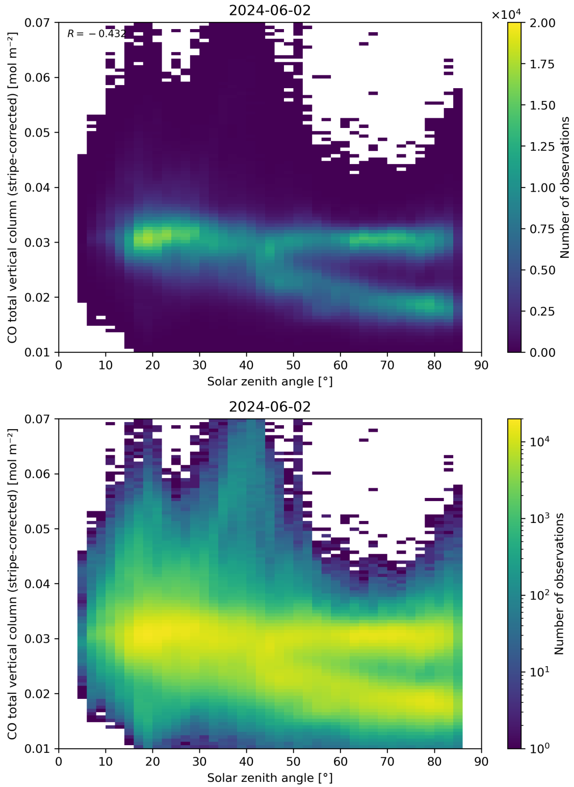
Figure 62: Scatter density plot of “Solar zenith angle” against “CO total vertical column (stripe-corrected)” for 2024-06-01 to 2024-06-03.
