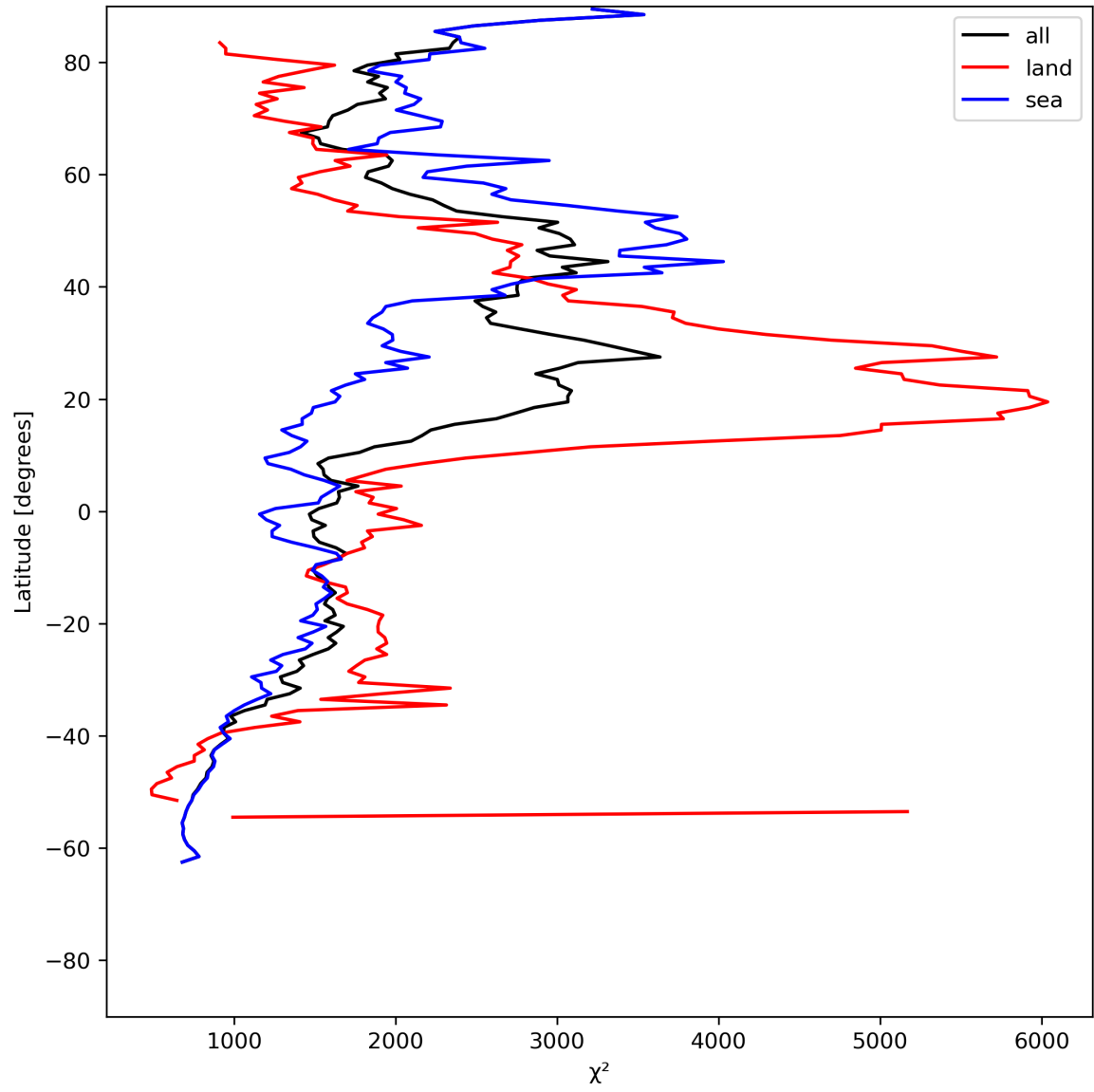
Figure 14: Zonal average of “ \chi^2 ” for 2024-06-01 to 2024-06-03.
