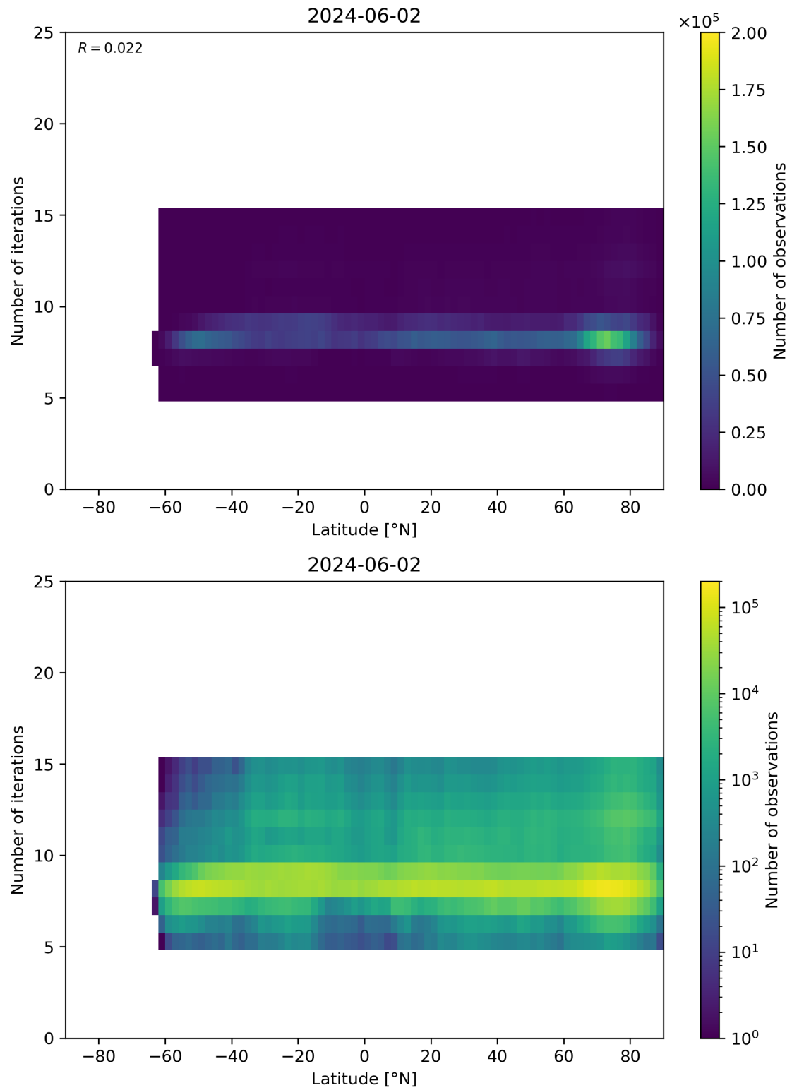
Figure 56: Scatter density plot of “Latitude” against “Number of iterations” for 2024-06-01 to 2024-06-03.
