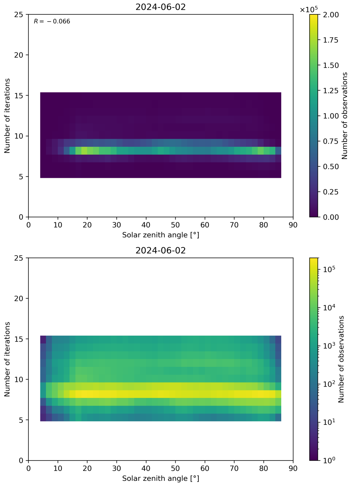
Figure 67: Scatter density plot of “Solar zenith angle” against “Number of iterations” for 2024-06-01 to 2024-06-03.
