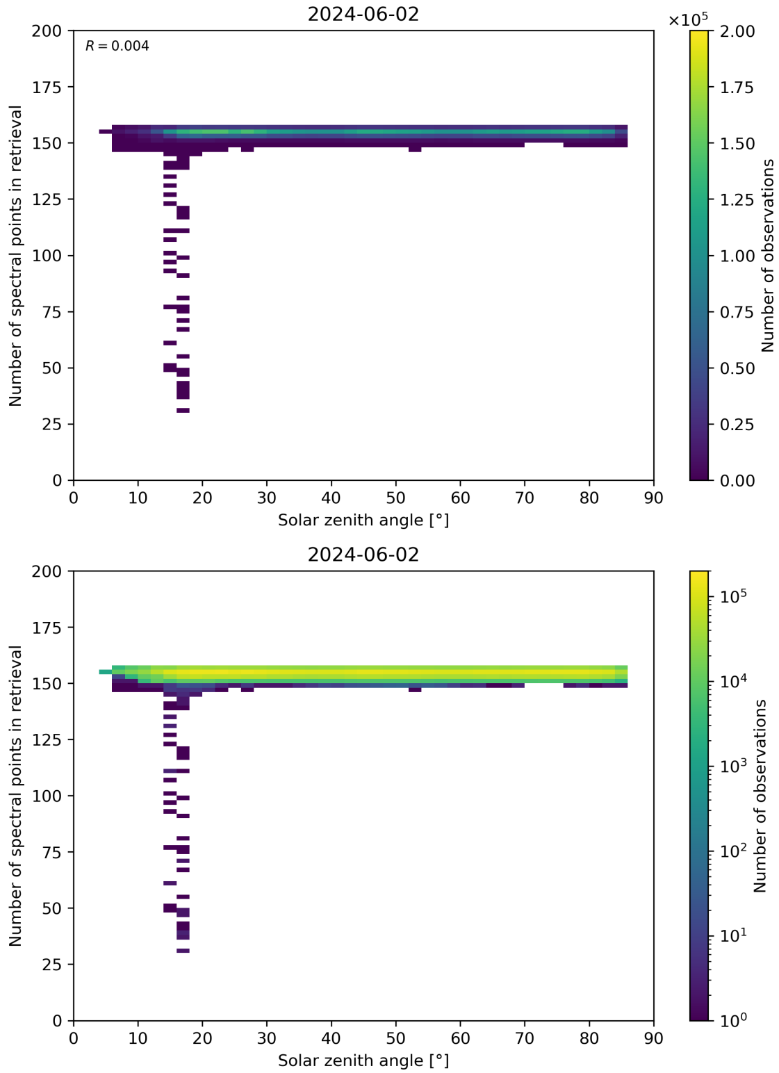
Figure 68: Scatter density plot of “Solar zenith angle” against “Number of spectral points in retrieval” for 2024-06-01 to 2024-06-03.
