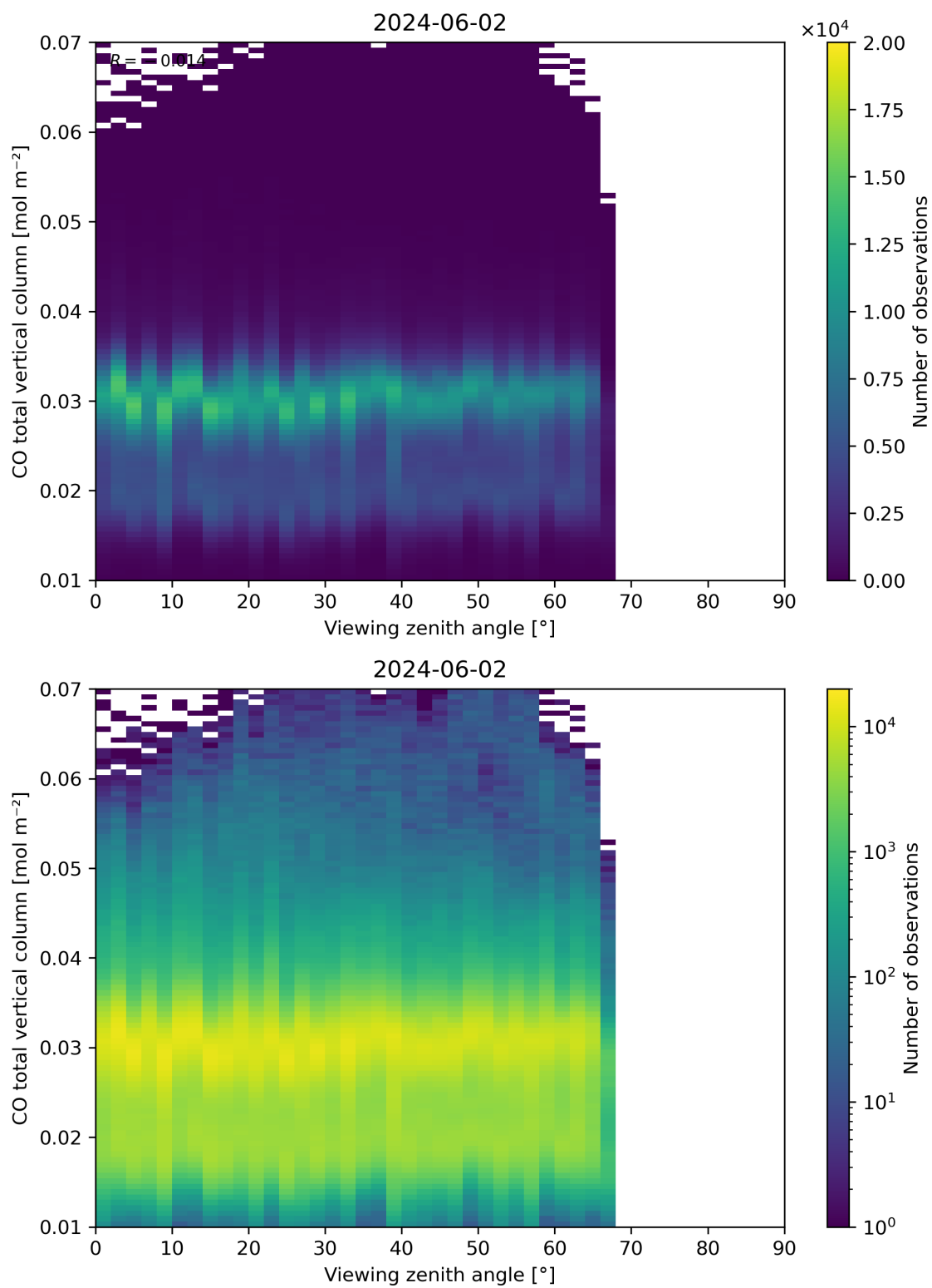
Figure 69: Scatter density plot of “Viewing zenith angle” against “CO total vertical column” for 2024-06-01 to 2024-06-03.
