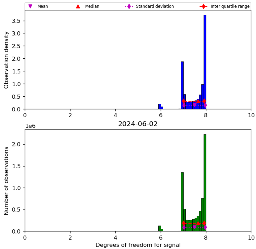
Figure 23: Histogram of “Degrees of freedom for signal” for 2024-06-01 to 2024-06-03
