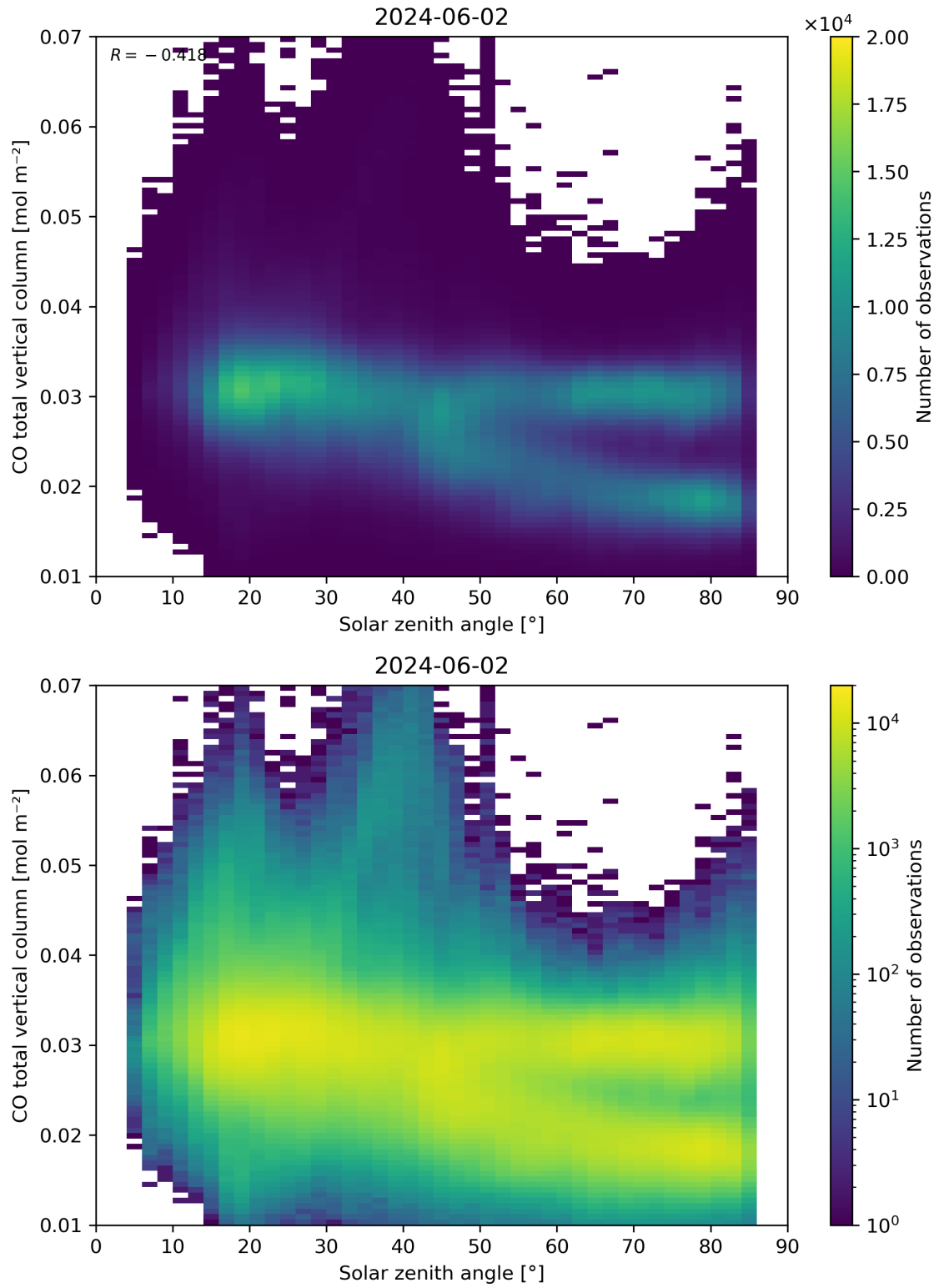
Figure 61: Scatter density plot of “Solar zenith angle” against “CO total vertical column” for 2024-06-01 to 2024-06-03.
