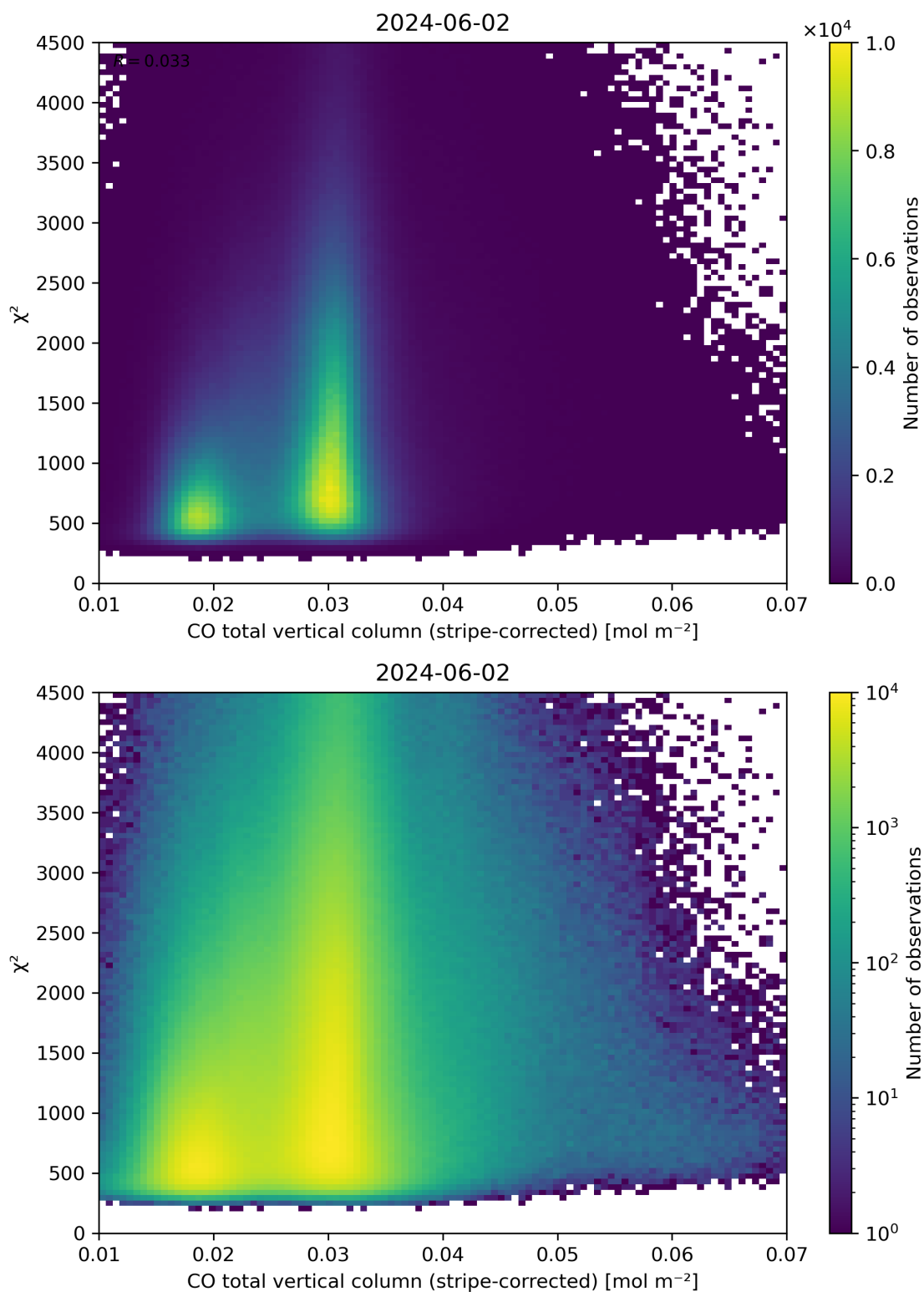
Figure 37: Scatter density plot of “CO total vertical column (stripe-corrected)” against “ \chi^2 ” for 2024-06-01 to 2024-06-03.
