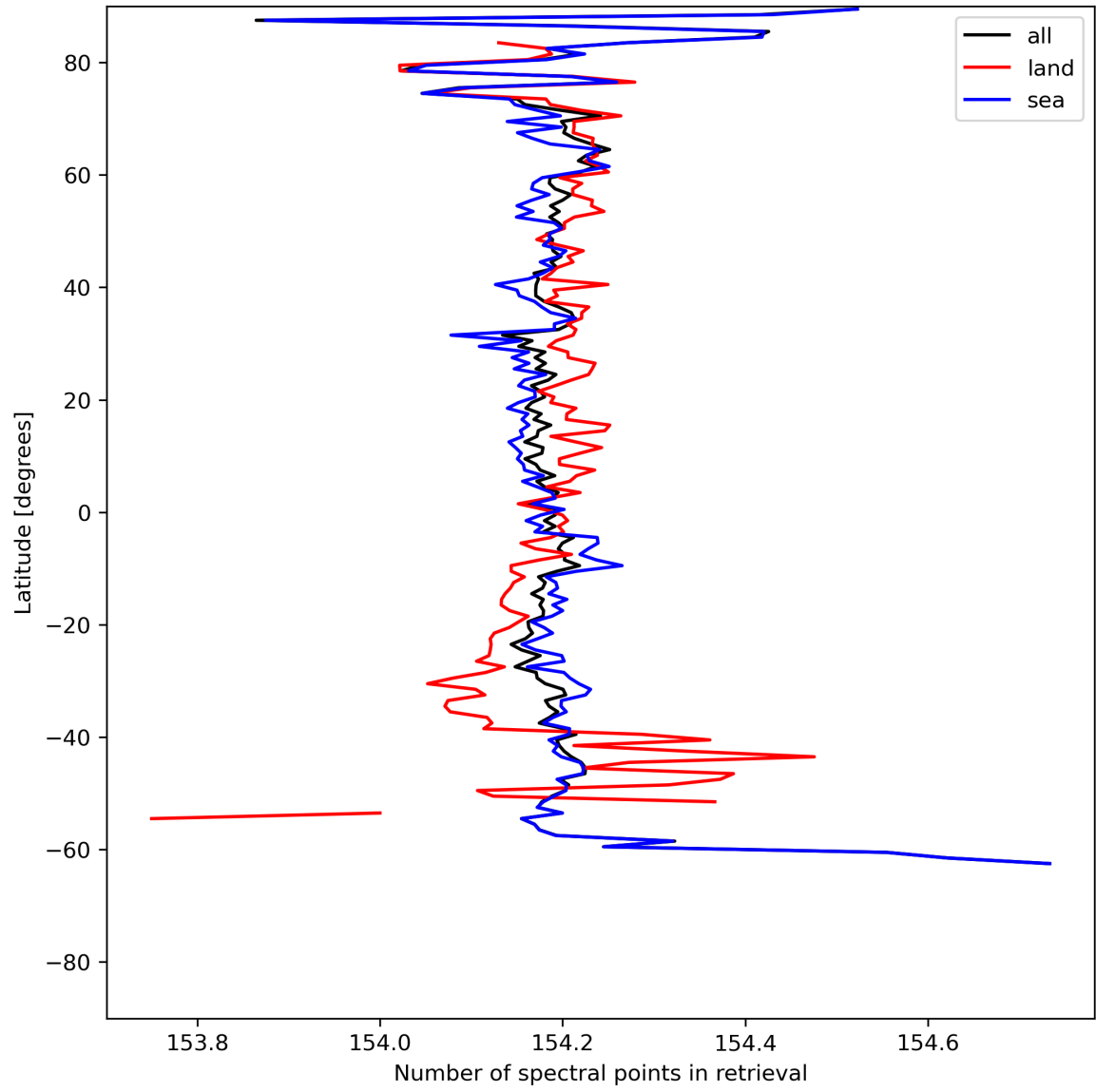
Figure 13: Zonal average of “Number of spectral points in retrieval” for 2024-06-01 to 2024-06-03.
