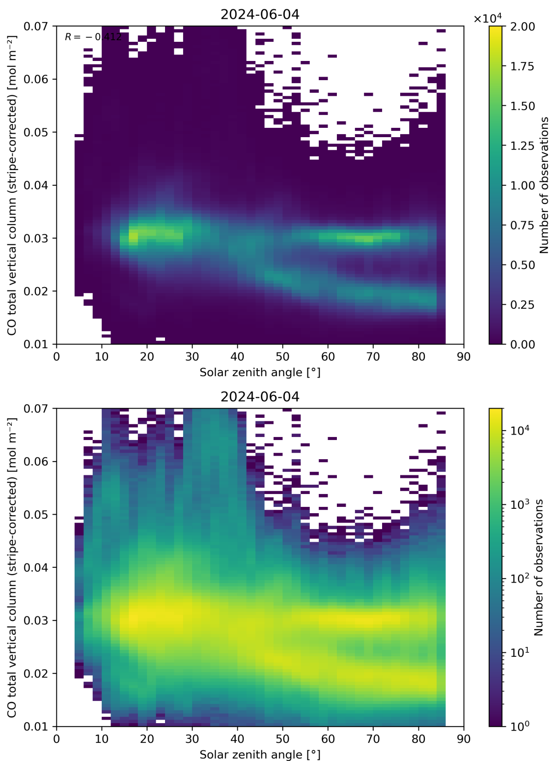
Figure 62: Scatter density plot of “Solar zenith angle” against “CO total vertical column (stripe-corrected)” for 2024-06-03 to 2024-06-05.
