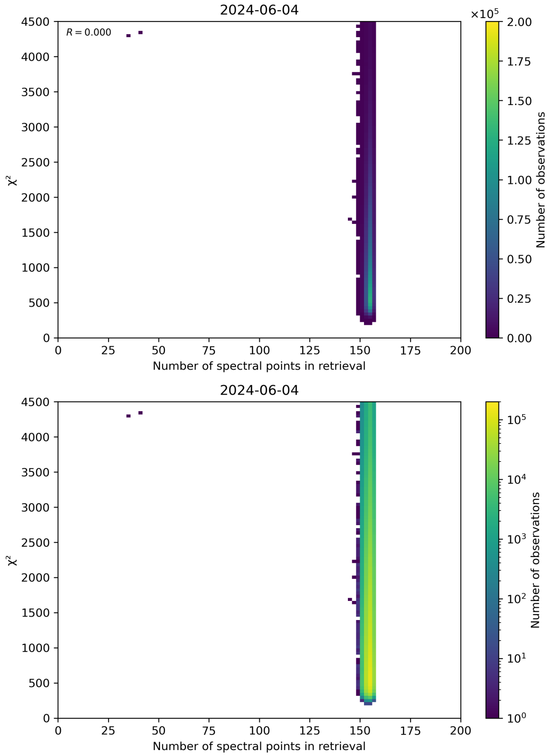
Figure 58: Scatter density plot of “Number of spectral points in retrieval” against “ \chi^2 ” for 2024-06-03 to 2024-06-05.
