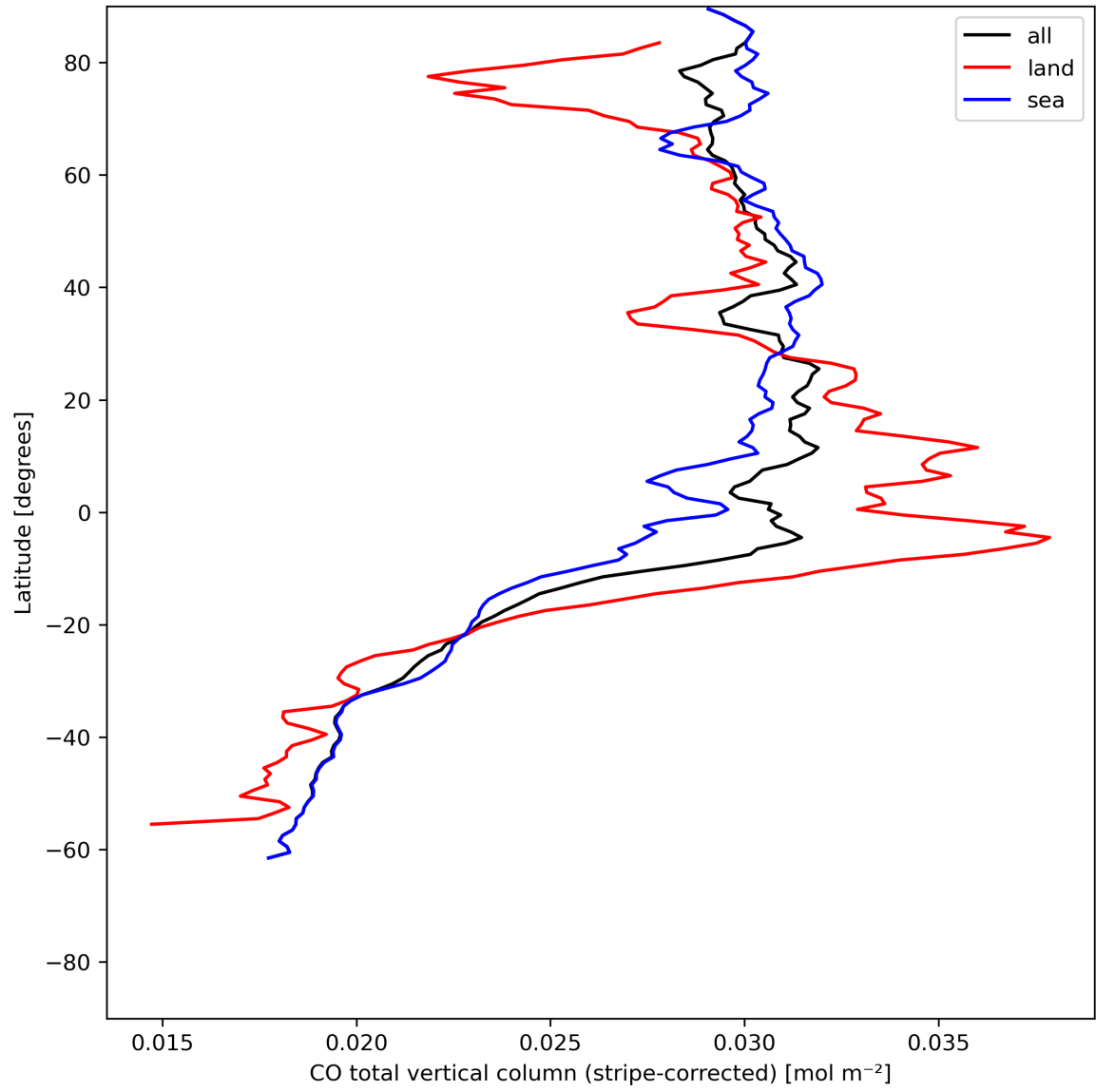
Figure 11: Zonal average of “CO total vertical column (stripe-corrected)” for 2024-06-03 to 2024-06-05.
