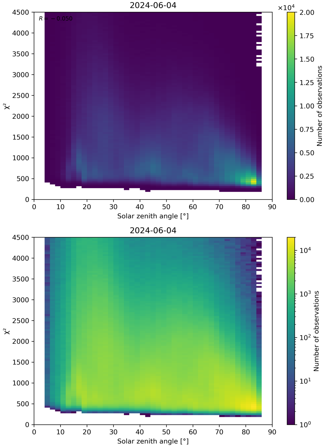
Figure 64: Scatter density plot of “Solar zenith angle” against “ \chi^2 ” for 2024-06-03 to 2024-06-05.
