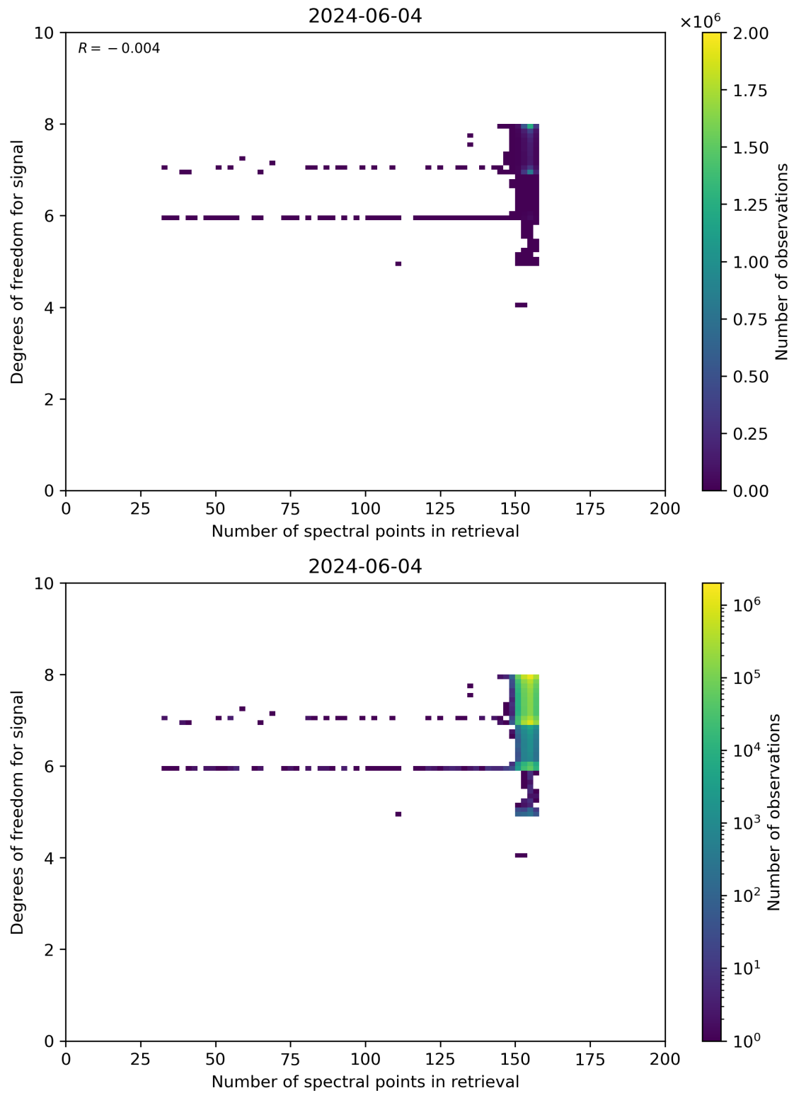
Figure 59: Scatter density plot of “Number of spectral points in retrieval” against “Degrees of freedom for signal” for 2024-06-03 to 2024-06-05.
