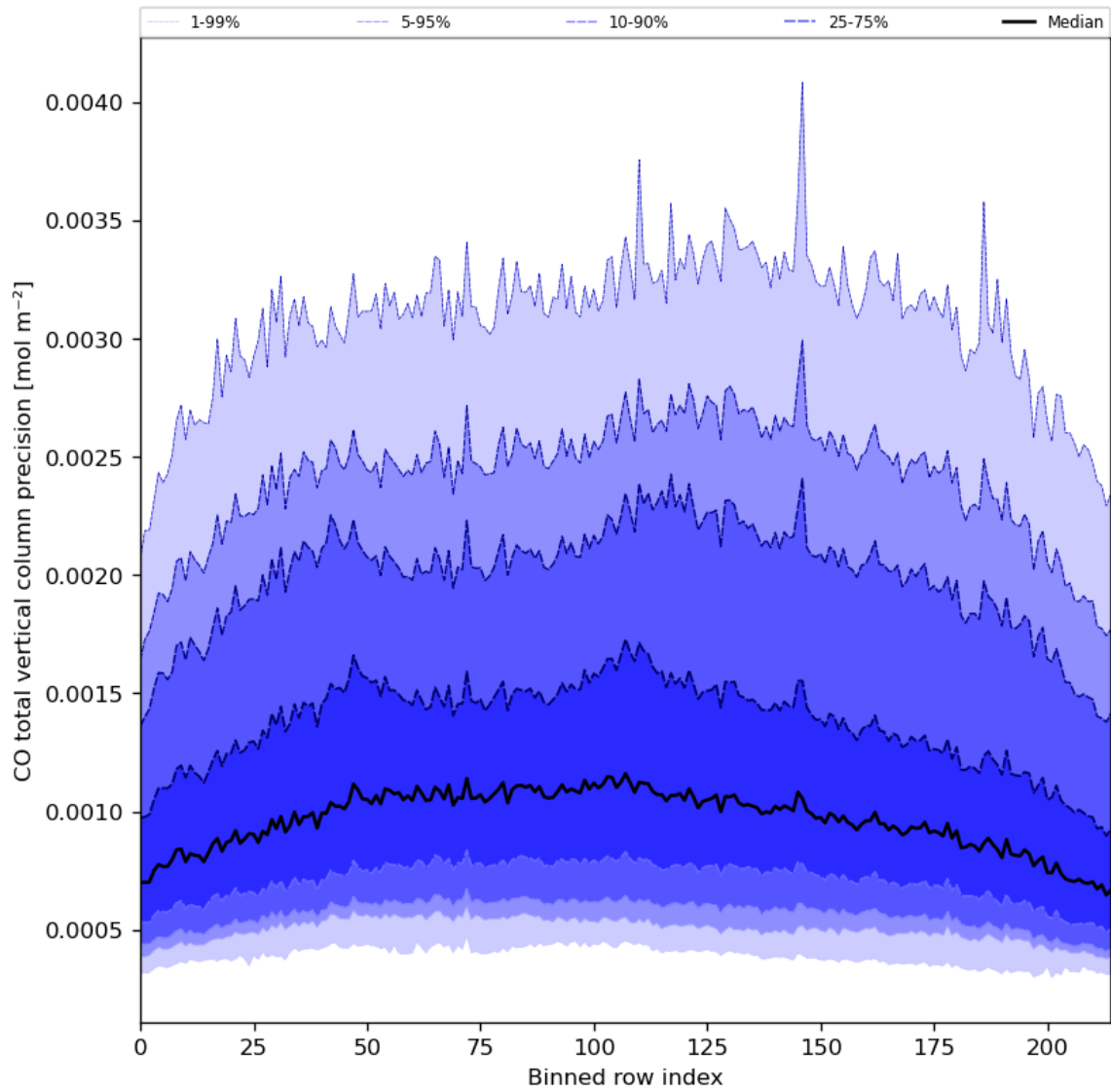
Figure 28: Along track statistics of “CO total vertical column precision” for 2024-06-03 to 2024-06-05
