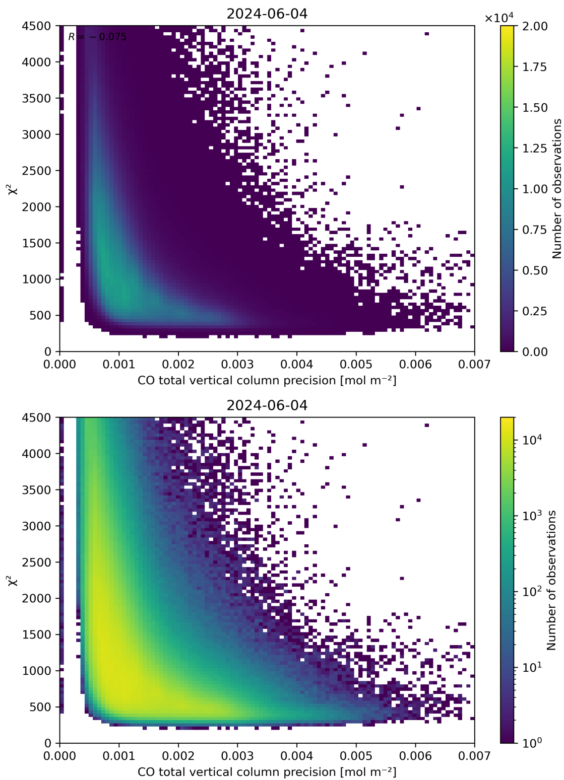
Figure 44: Scatter density plot of “CO total vertical column precision” against “ \chi^2 ” for 2024-06-03 to 2024-06-05.
