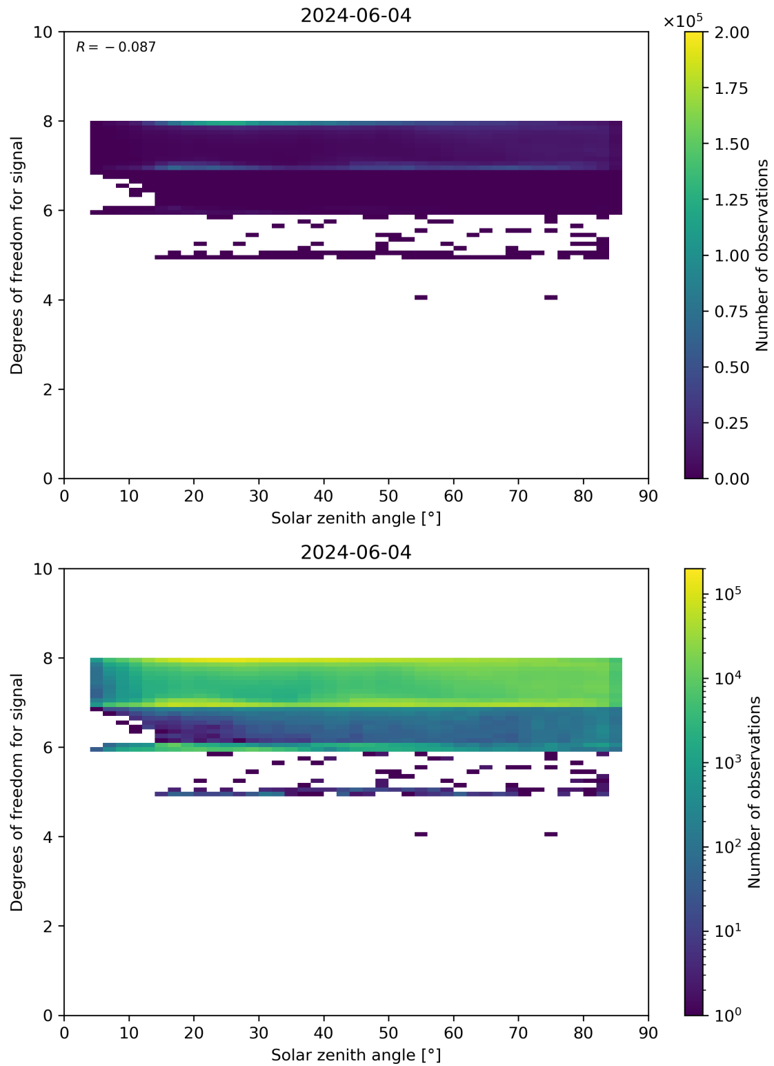
Figure 65: Scatter density plot of “Solar zenith angle” against “Degrees of freedom for signal” for 2024-06-03 to 2024-06-05.
