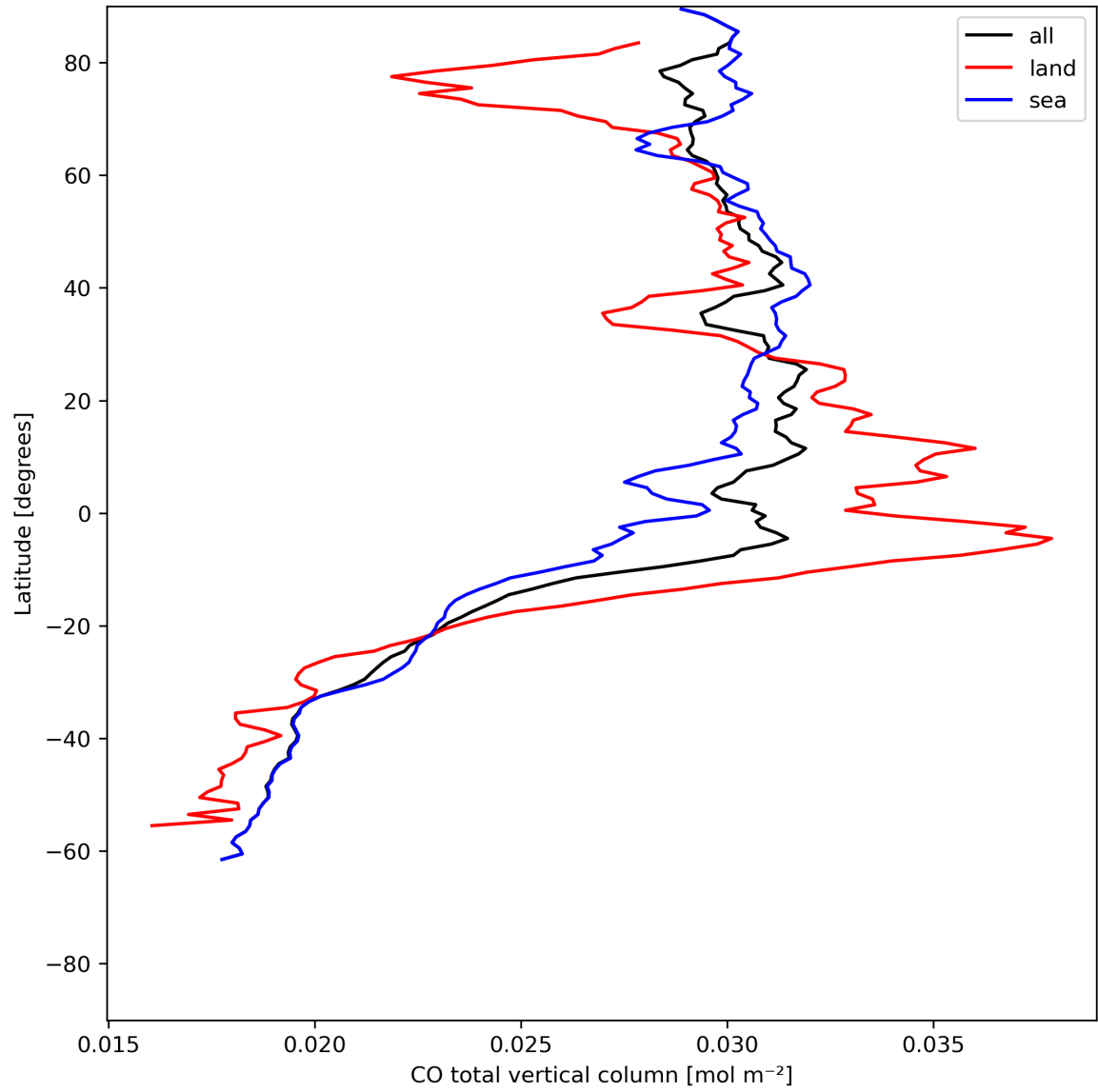
Figure 10: Zonal average of “CO total vertical column” for 2024-06-03 to 2024-06-05.
