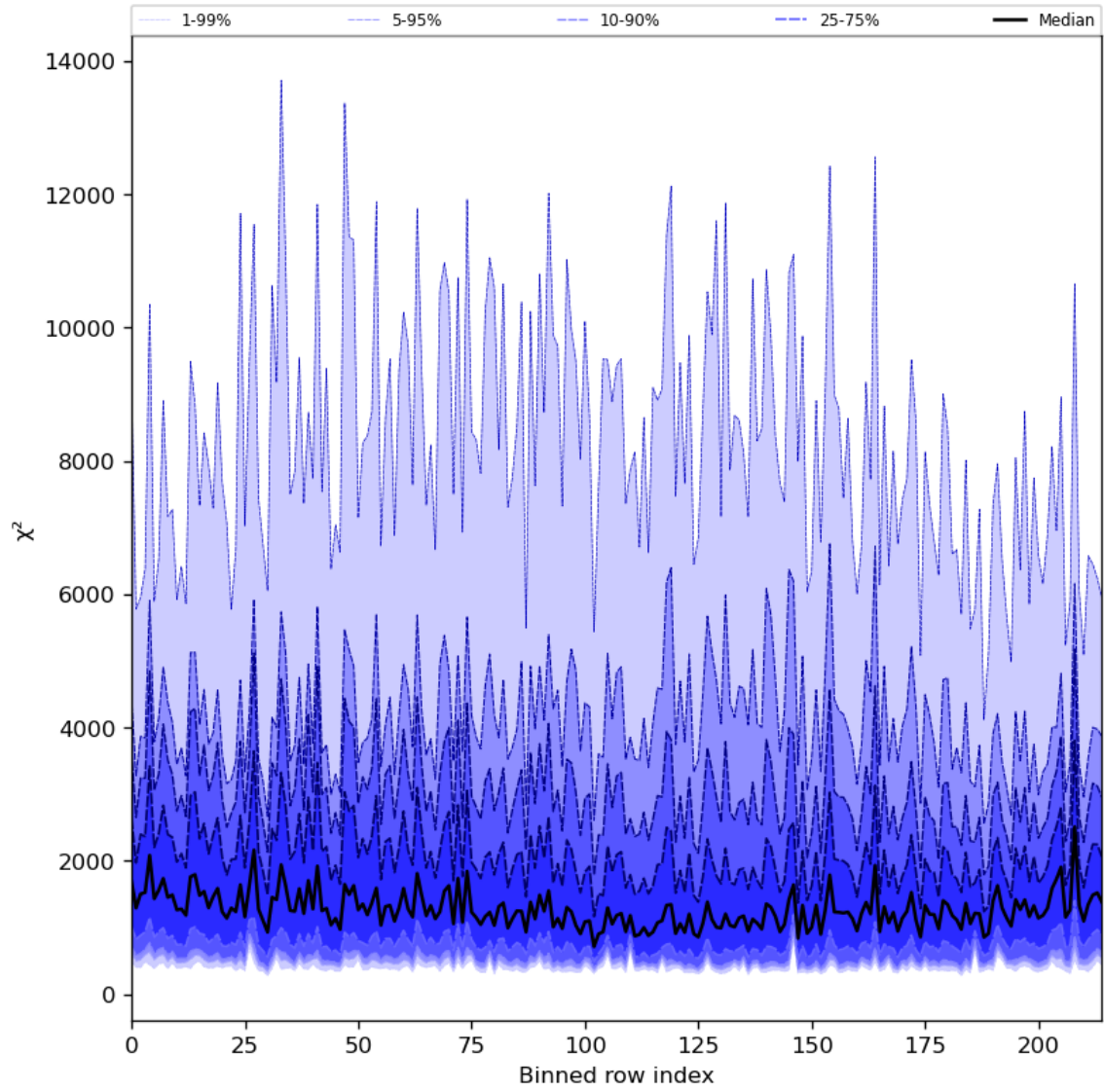
Figure 30: Along track statistics of “ \chi^2 ” for 2024-06-03 to 2024-06-05
