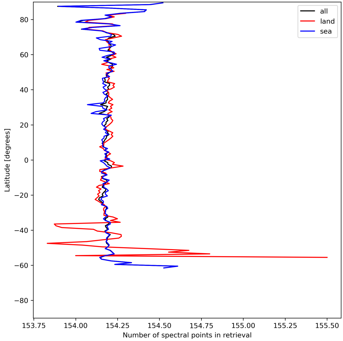
Figure 13: Zonal average of “Number of spectral points in retrieval” for 2024-06-03 to 2024-06-05.
