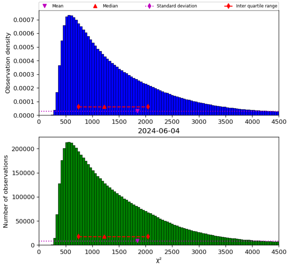
Figure 22: Histogram of “ \chi^2 ” for 2024-06-03 to 2024-06-05
