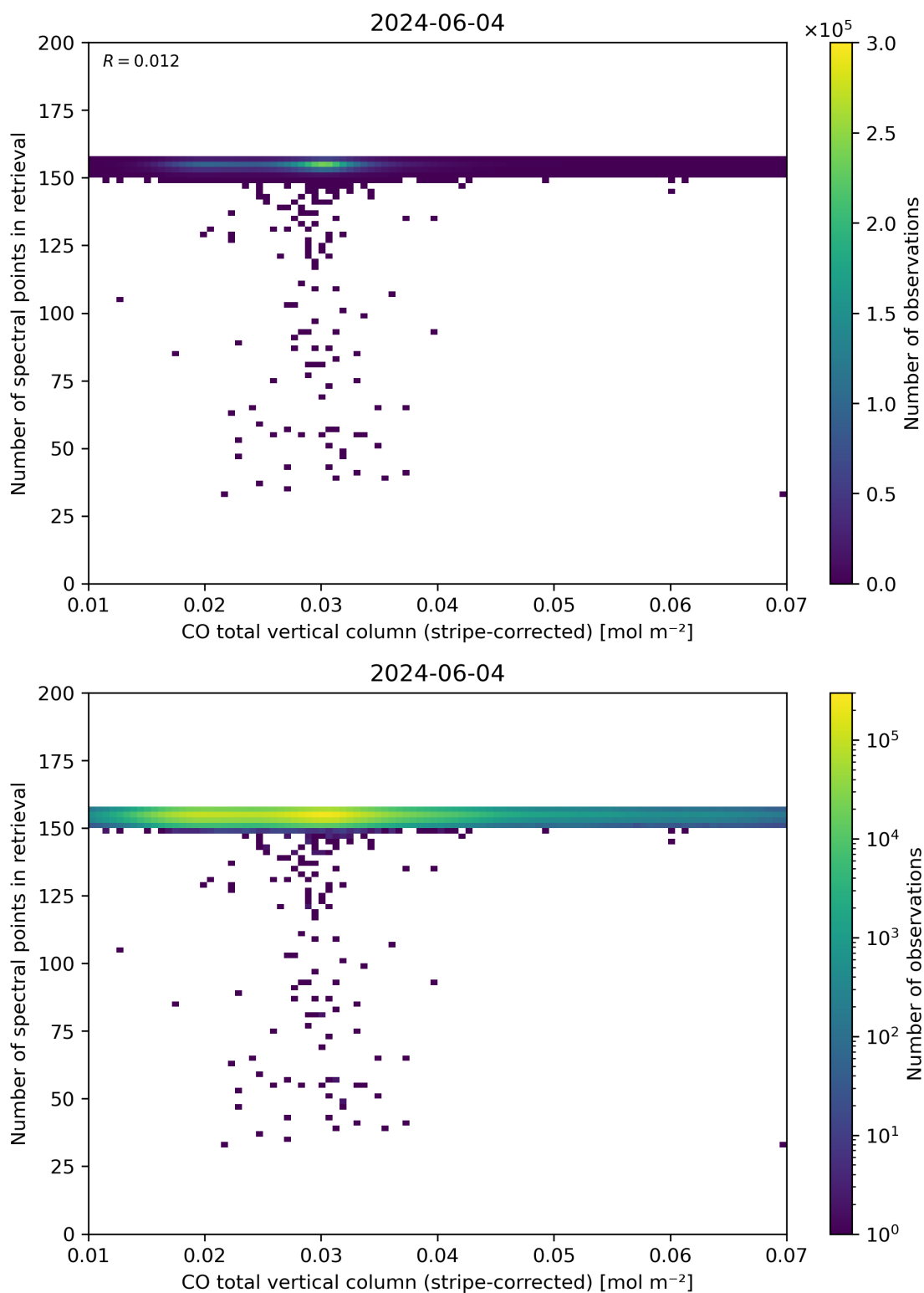
Figure 40: Scatter density plot of “CO total vertical column (stripe-corrected)” against “Number of spectral points in retrieval” for 2024-06-03 to 2024-06-05.
