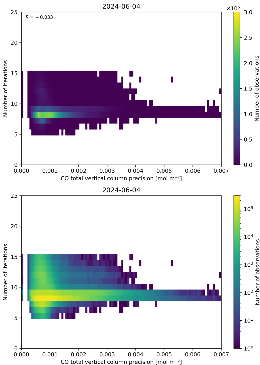
Figure 46: Scatter density plot of “CO total vertical column precision” against “Number of iterations” for 2024-06-03 to 2024-06-05.
