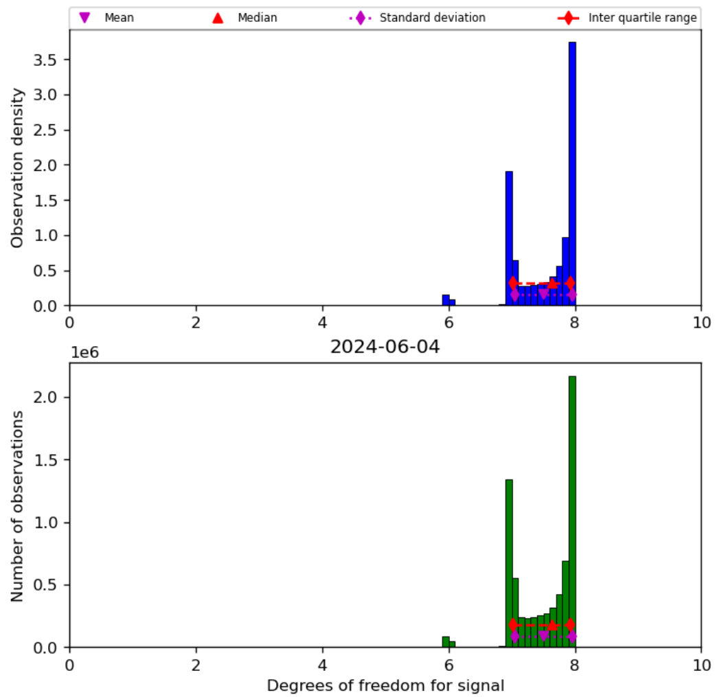
Figure 23: Histogram of “Degrees of freedom for signal” for 2024-06-03 to 2024-06-05
