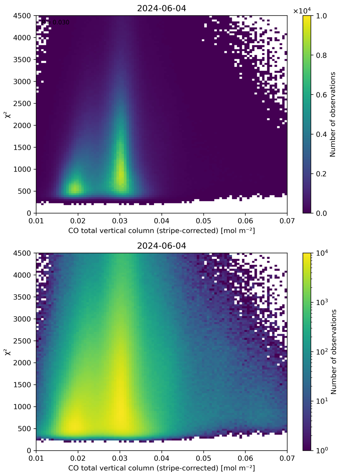
Figure 37: Scatter density plot of “CO total vertical column (stripe-corrected)” against “ \chi^2 ” for 2024-06-03 to 2024-06-05.
