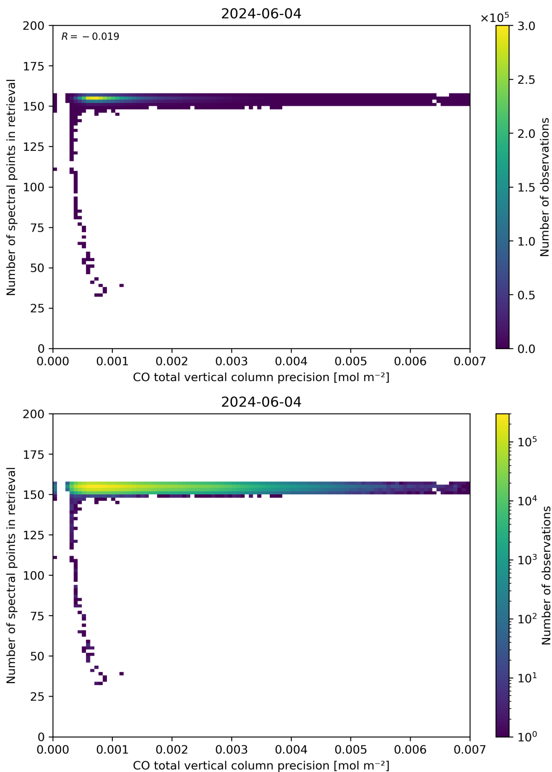
Figure 47: Scatter density plot of “CO total vertical column precision” against “Number of spectral points in retrieval” for 2024-06-03 to 2024-06-05.
