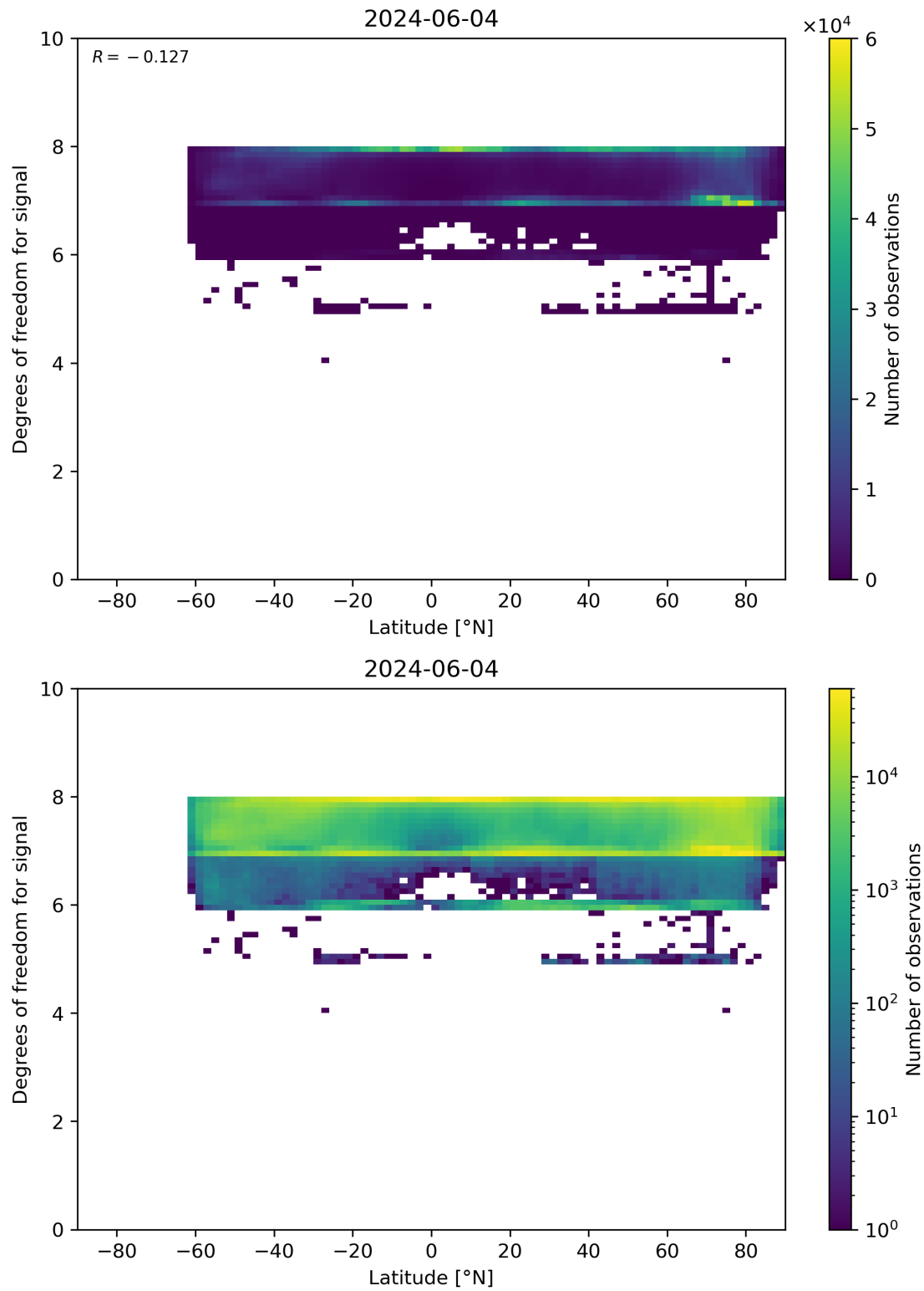
Figure 55: Scatter density plot of “Latitude” against “Degrees of freedom for signal” for 2024-06-03 to 2024-06-05.
