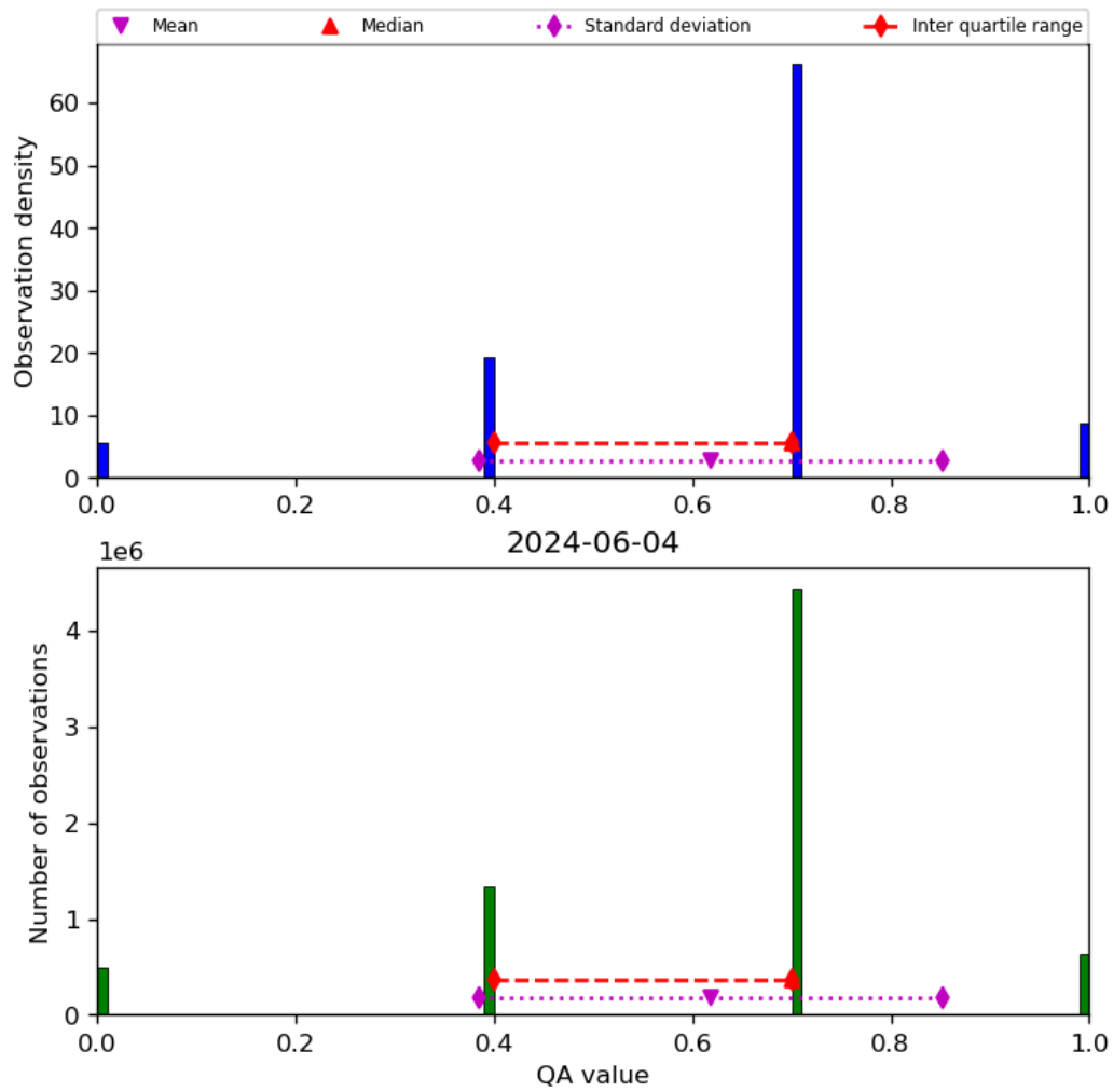
Figure 17: Histogram of “QA value” for 2024-06-03 to 2024-06-05
