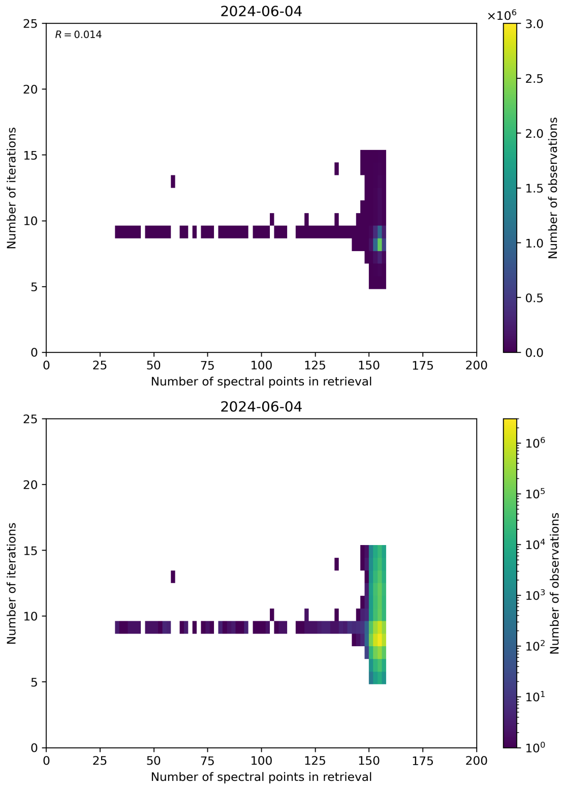
Figure 60: Scatter density plot of “Number of spectral points in retrieval” against “Number of iterations” for 2024-06-03 to 2024-06-05.
