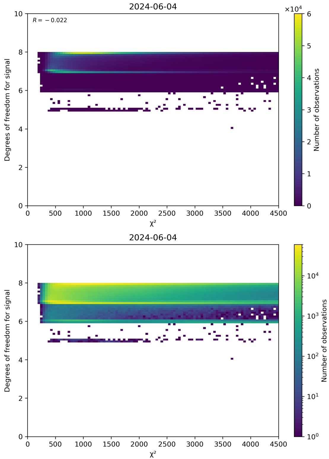
Figure 48: Scatter density plot of " \chi^2 " against "Degrees of freedom for signal" for 2024-06-03 to 2024-06-05.
