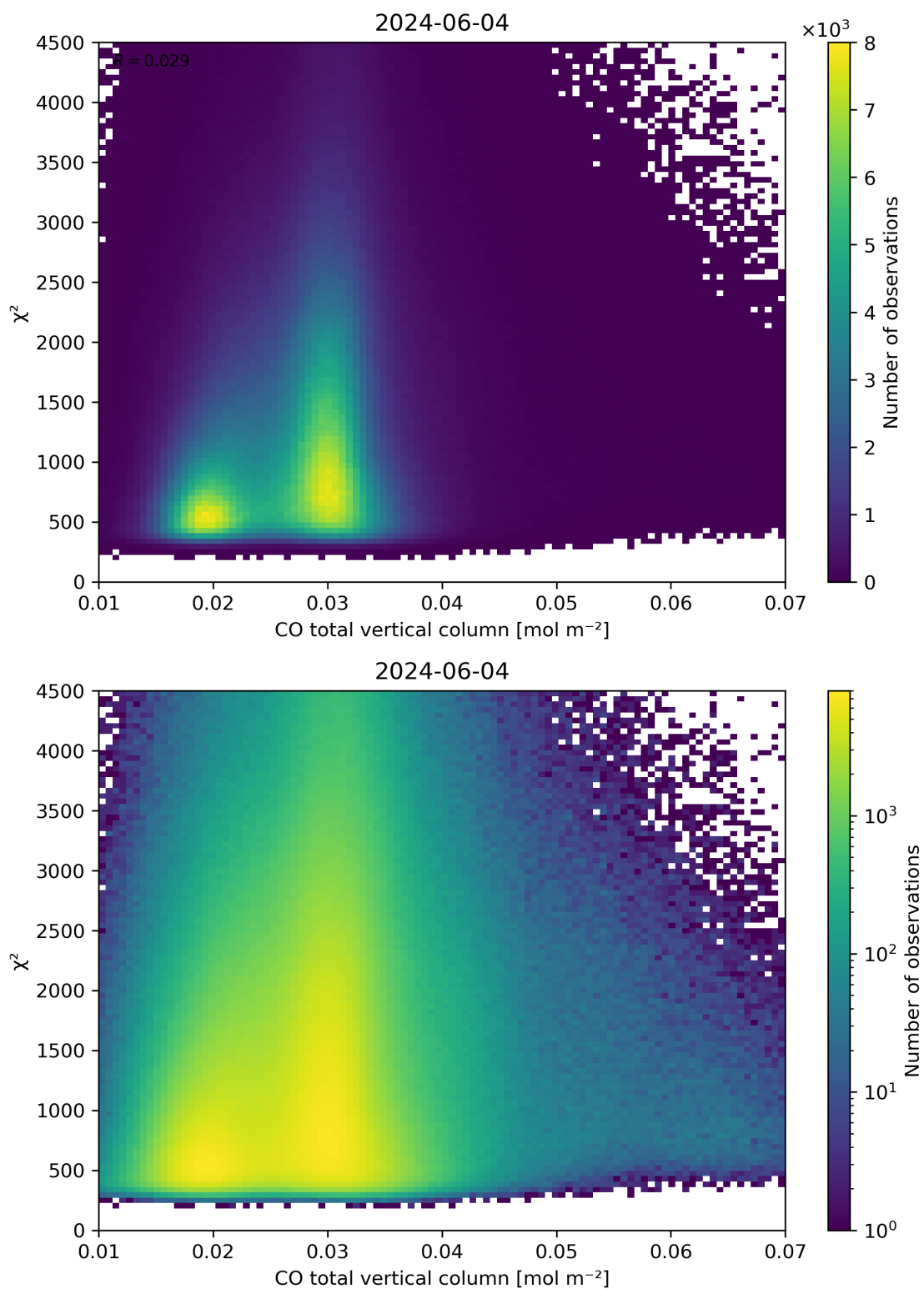
Figure 35: Scatter density plot of “CO total vertical column” against “ \chi^2 ” for 2024-06-03 to 2024-06-05.
