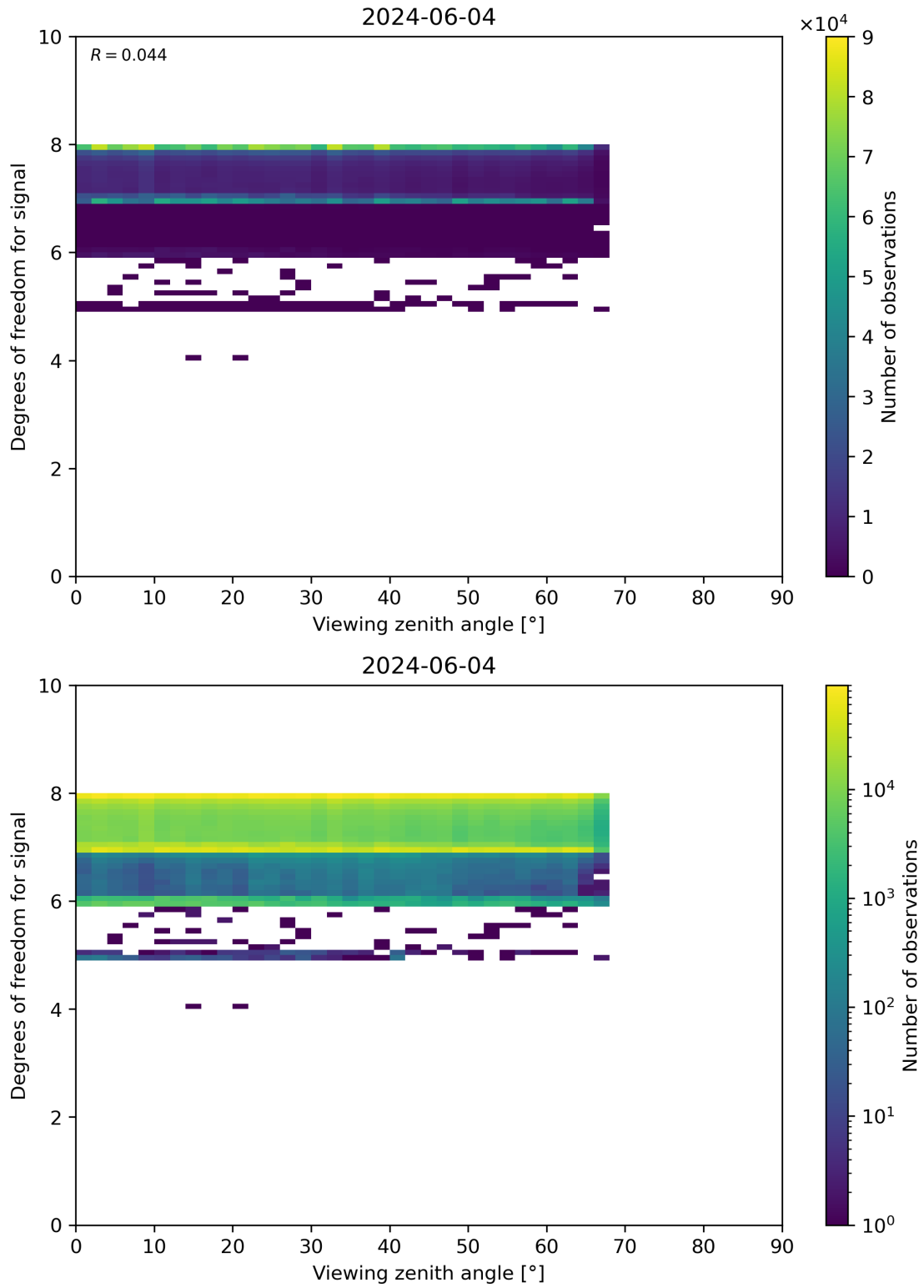
Figure 73: Scatter density plot of “Viewing zenith angle” against “Degrees of freedom for signal” for 2024-06-03 to 2024-06-05.
