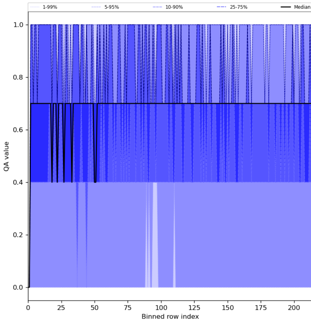
Figure 25: Along track statistics of “QA value” for 2024-06-03 to 2024-06-05
