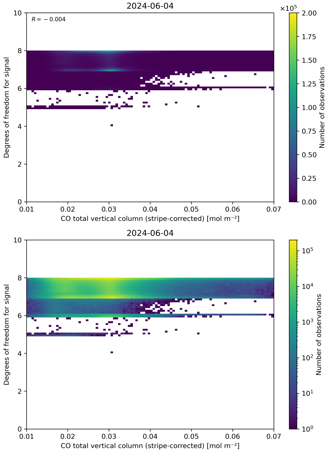
Figure 38: Scatter density plot of “CO total vertical column (stripe-corrected)” against “Degrees of freedom for signal” for 2024-06-03 to 2024-06-05.
