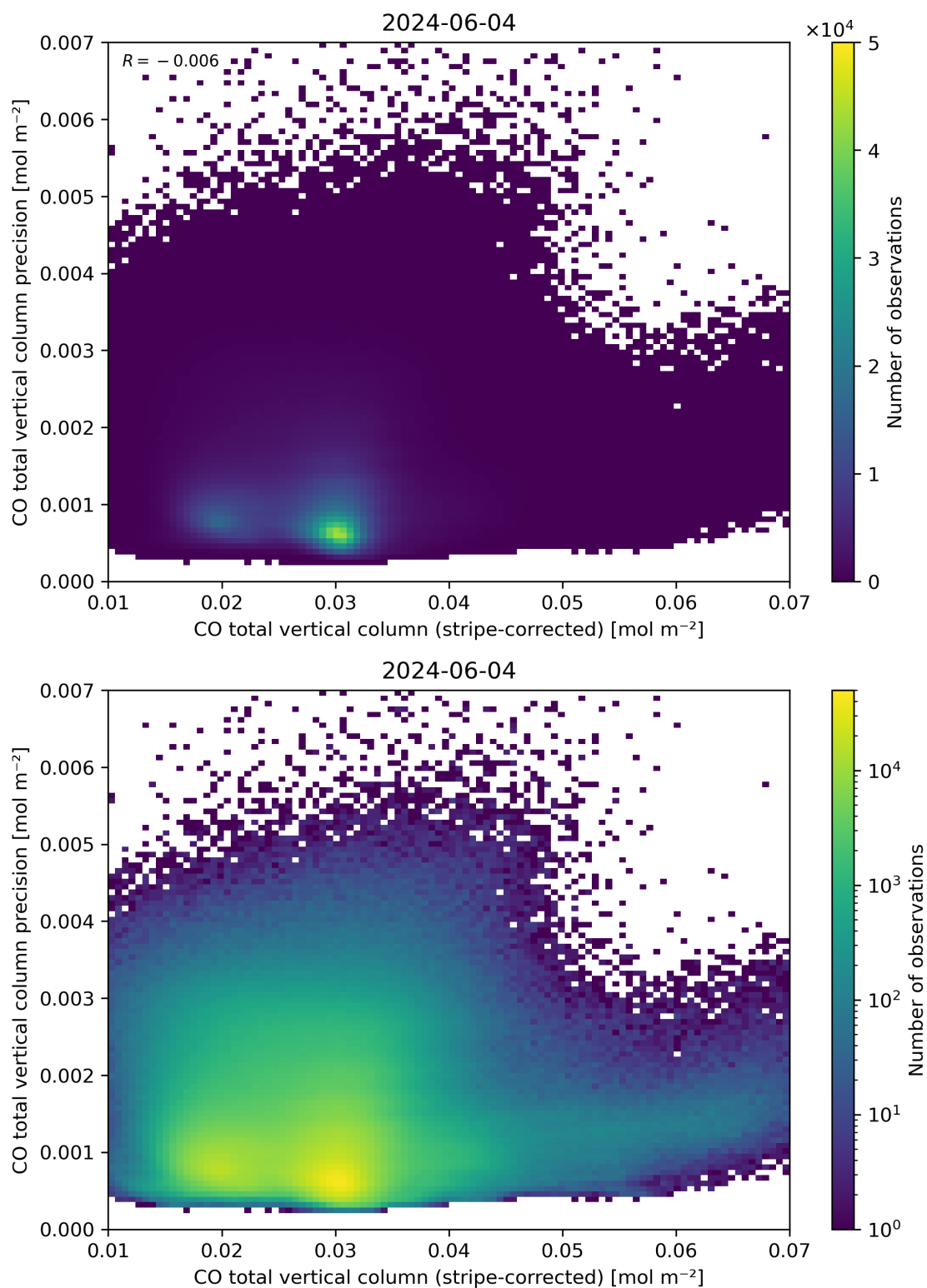
Figure 36: Scatter density plot of “CO total vertical column (stripe-corrected)” against “CO total vertical column precision” for 2024-06-03 to 2024-06-05.
