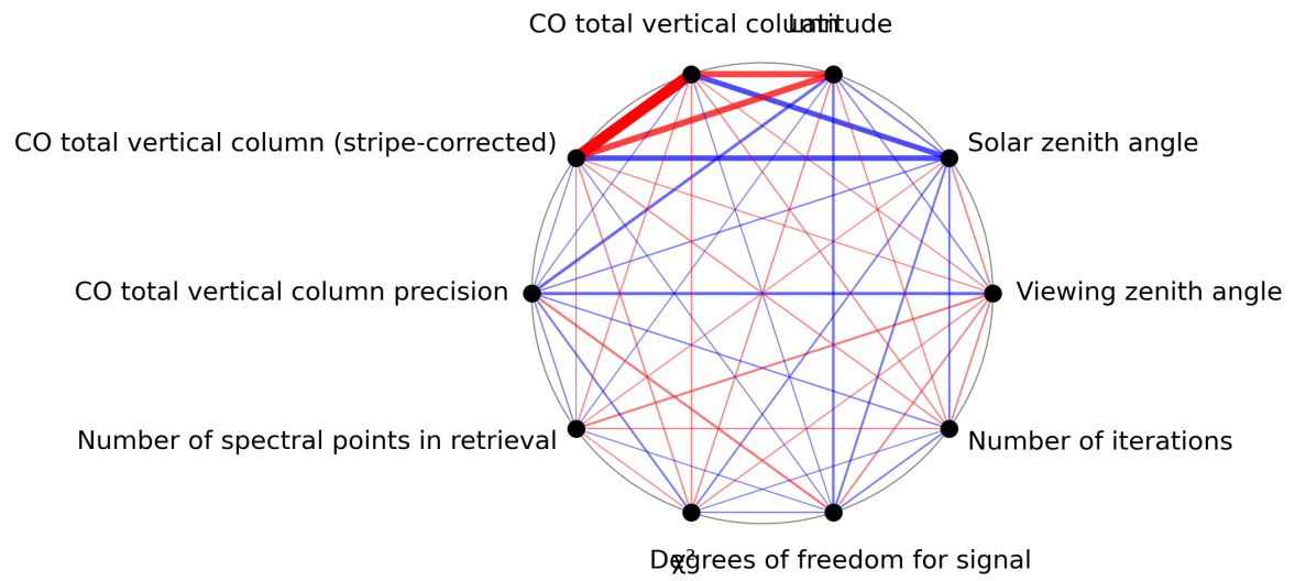
Figure 1: Map of correlation graph for 2024-06-03 to 2024-06-05.
