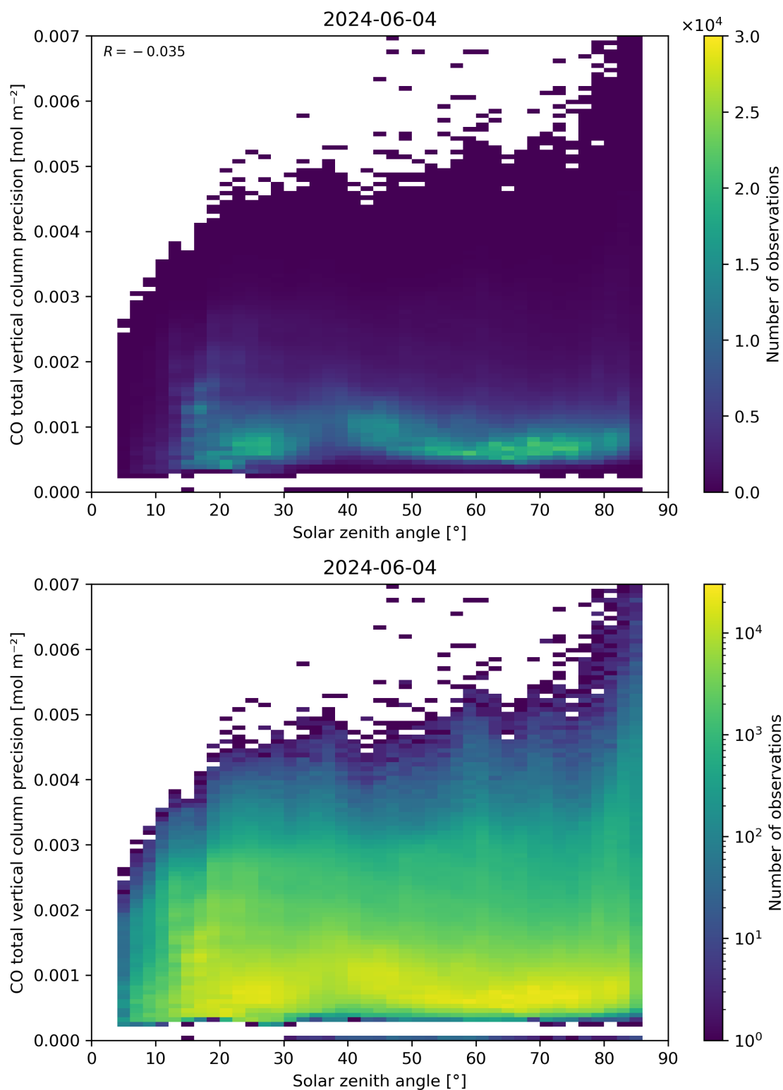
Figure 63: Scatter density plot of “Solar zenith angle” against “CO total vertical column precision” for 2024-06-03 to 2024-06-05.
