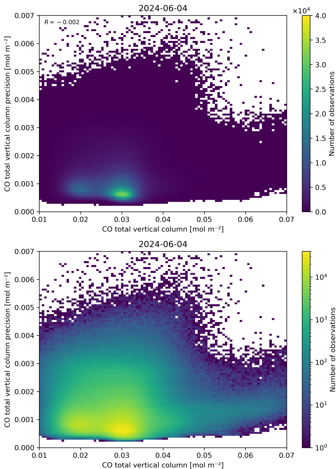
Figure 34: Scatter density plot of “CO total vertical column” against “CO total vertical column precision” for 2024-06-03 to 2024-06-05.
