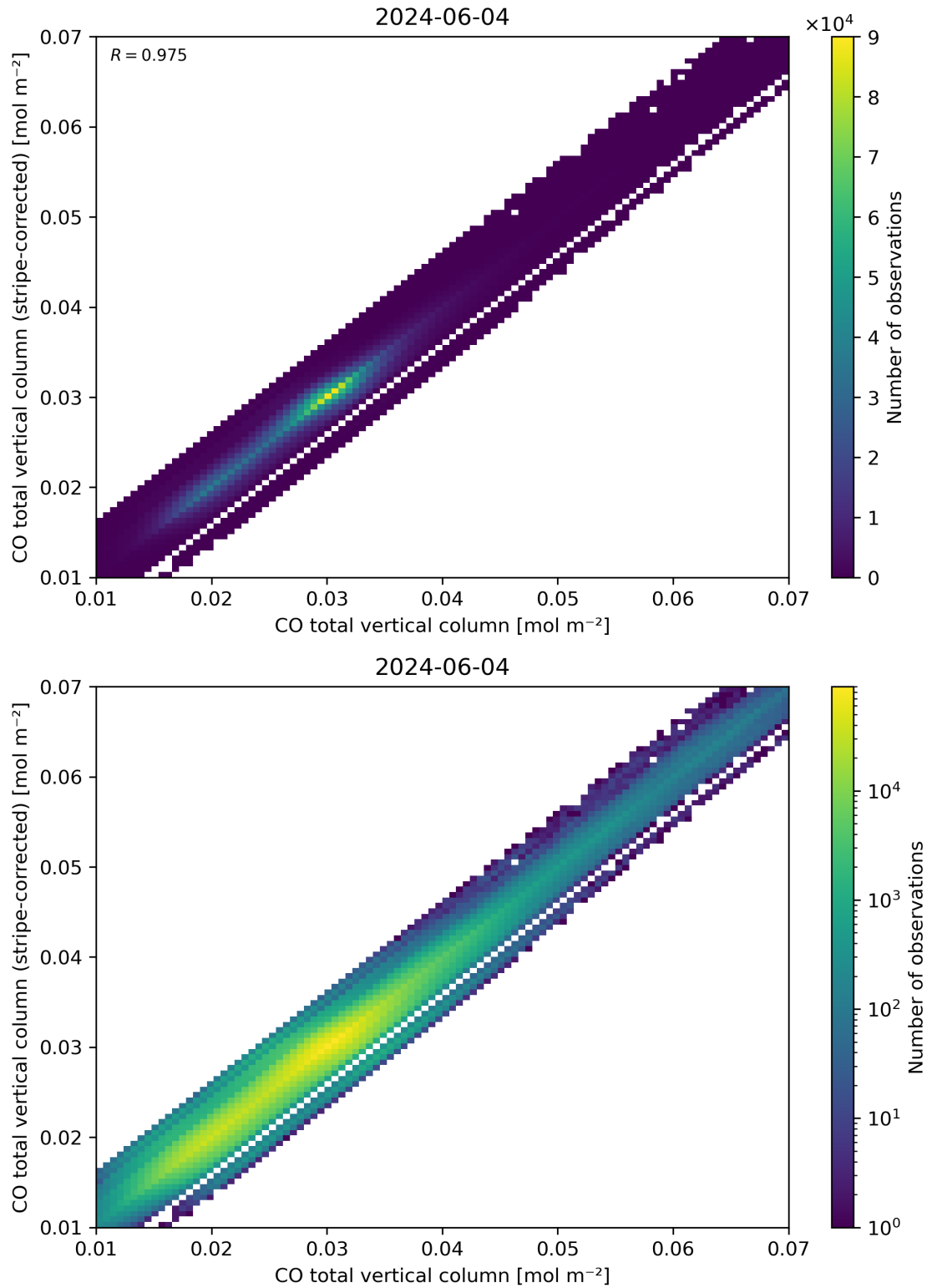
Figure 33: Scatter density plot of “CO total vertical column” against “CO total vertical column (stripe-corrected)” for 2024-06-03 to 2024-06-05.
