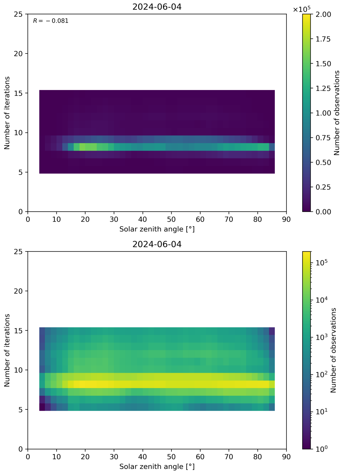
Figure 67: Scatter density plot of “Solar zenith angle” against “Number of iterations” for 2024-06-03 to 2024-06-05.
