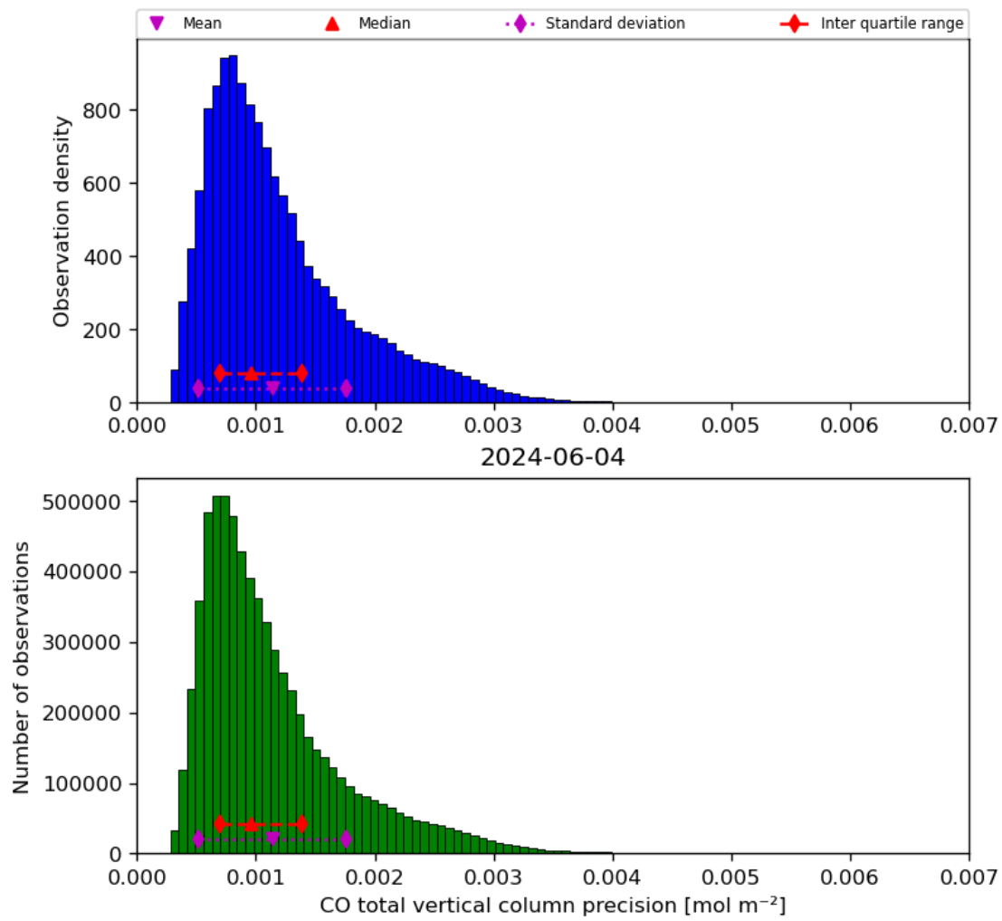
Figure 20: Histogram of “CO total vertical column precision” for 2024-06-03 to 2024-06-05
