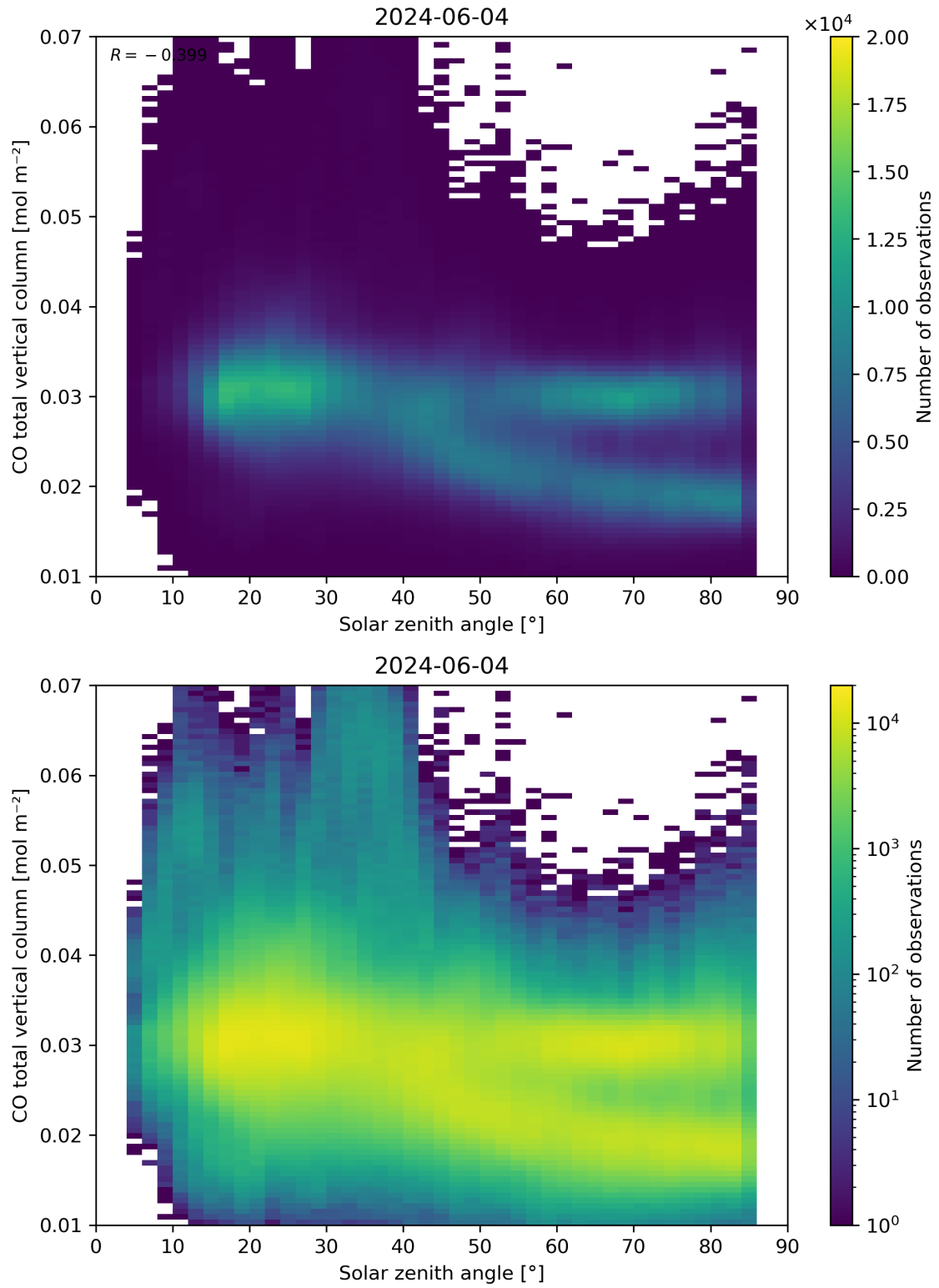
Figure 61: Scatter density plot of “Solar zenith angle” against “CO total vertical column” for 2024-06-03 to 2024-06-05.
