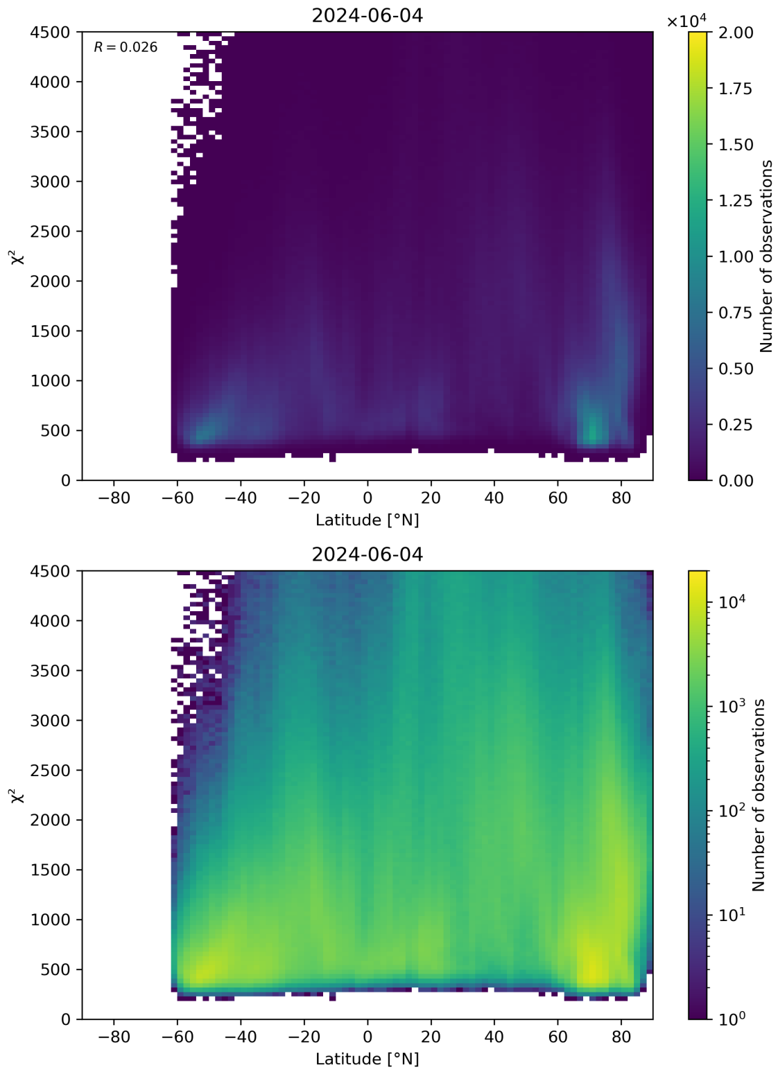
Figure 54: Scatter density plot of “Latitude” against “ \chi^2 ” for 2024-06-03 to 2024-06-05.
