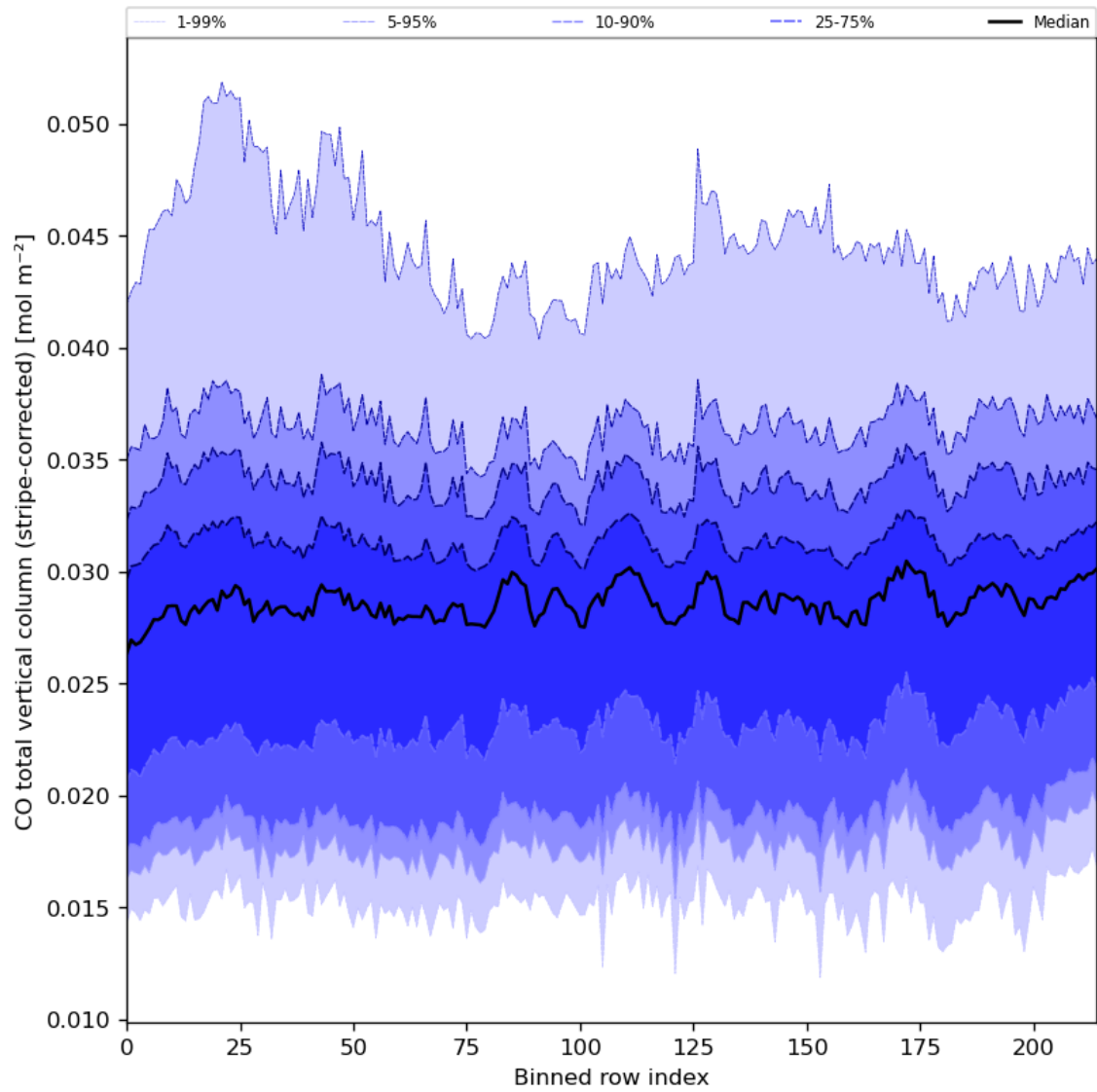
Figure 27: Along track statistics of “CO total vertical column (stripe-corrected)” for 2024-06-03 to 2024-06-05
