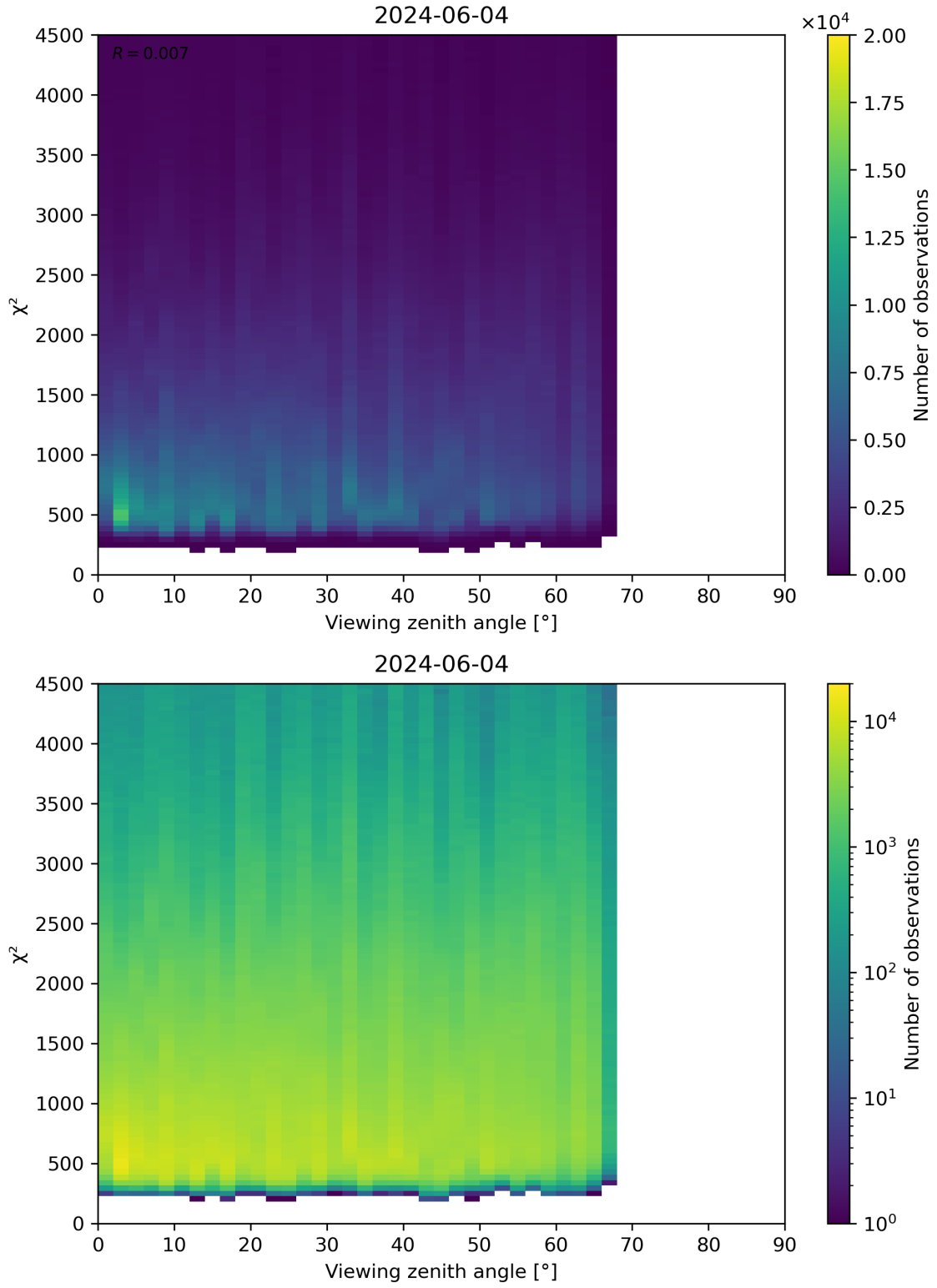
Figure 72: Scatter density plot of “Viewing zenith angle” against “ \chi^2 ” for 2024-06-03 to 2024-06-05.
