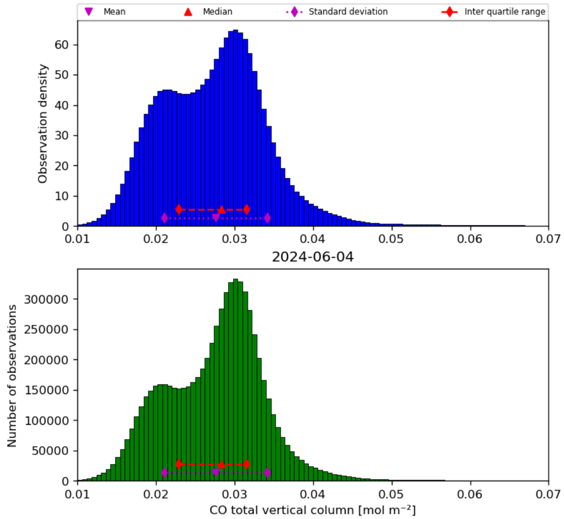
Figure 18: Histogram of “CO total vertical column” for 2024-06-03 to 2024-06-05
