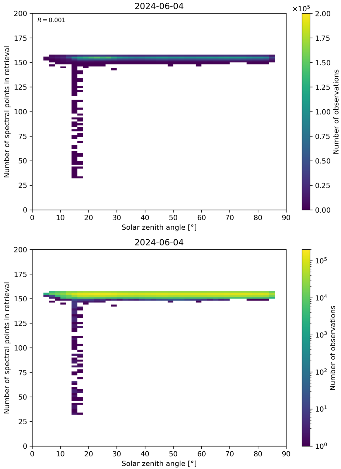
Figure 68: Scatter density plot of “Solar zenith angle” against “Number of spectral points in retrieval” for 2024-06-03 to 2024-06-05.
