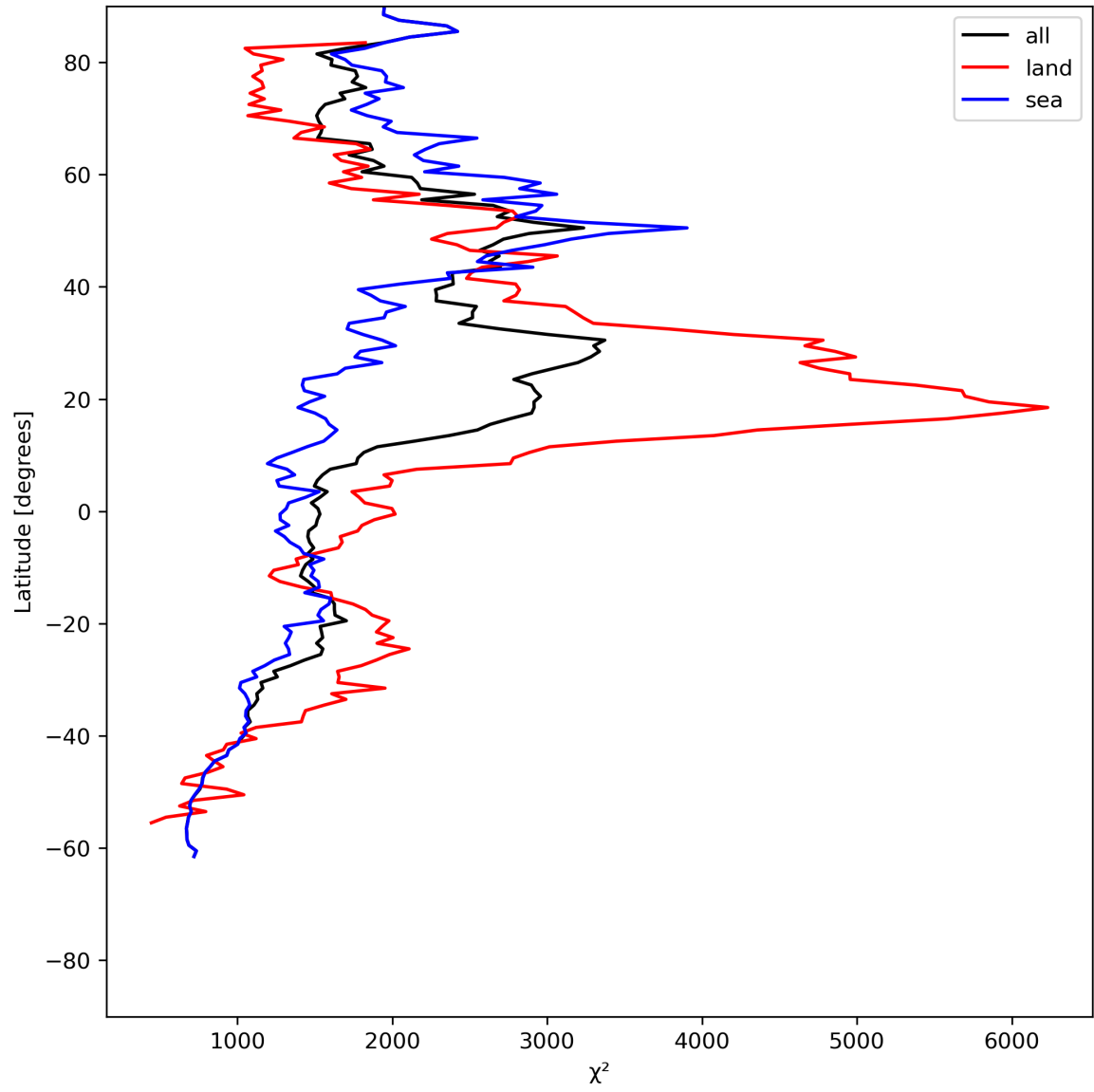
Figure 14: Zonal average of “ \chi^2 ” for 2024-06-03 to 2024-06-05.
