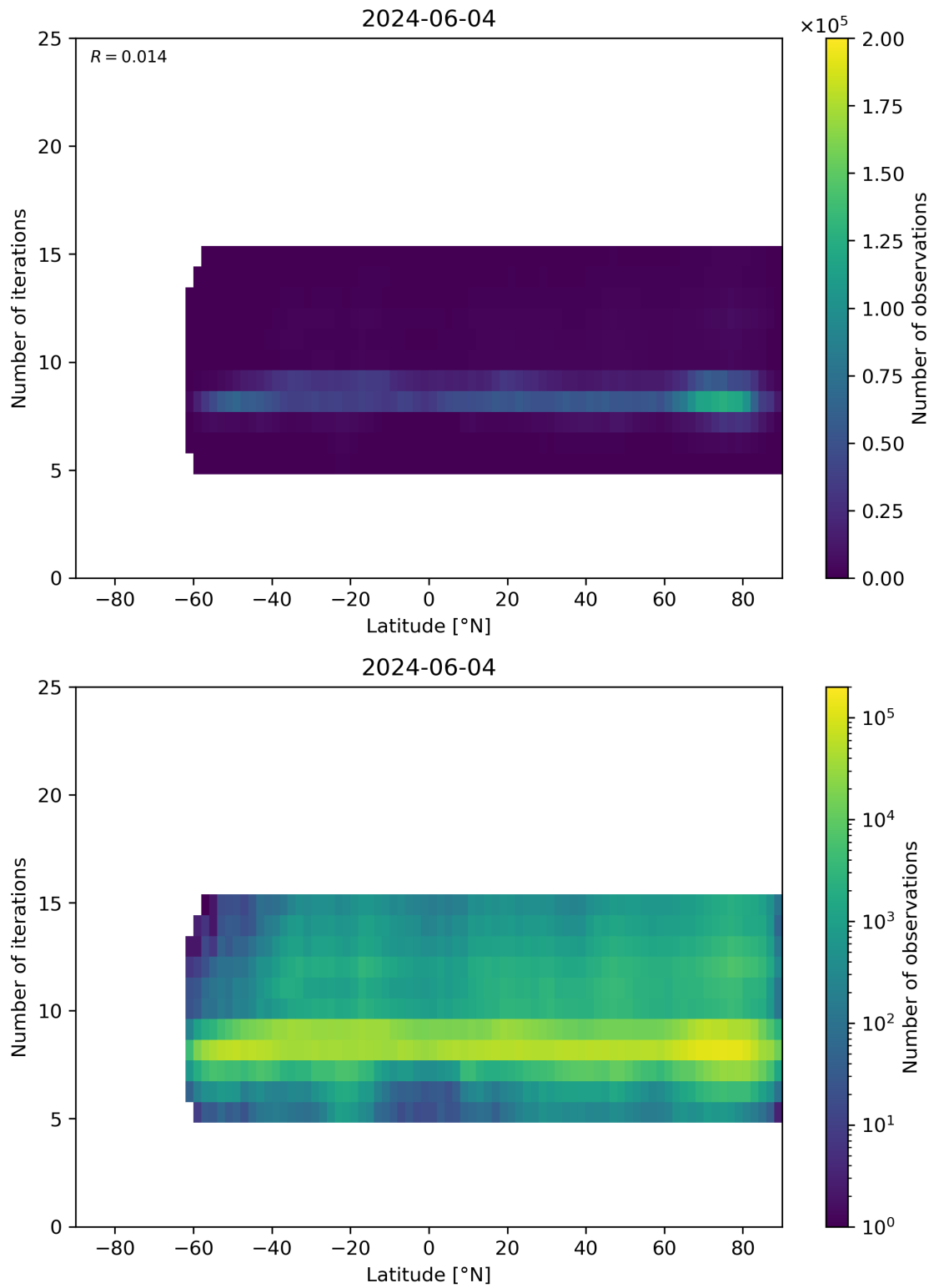
Figure 56: Scatter density plot of “Latitude” against “Number of iterations” for 2024-06-03 to 2024-06-05.
