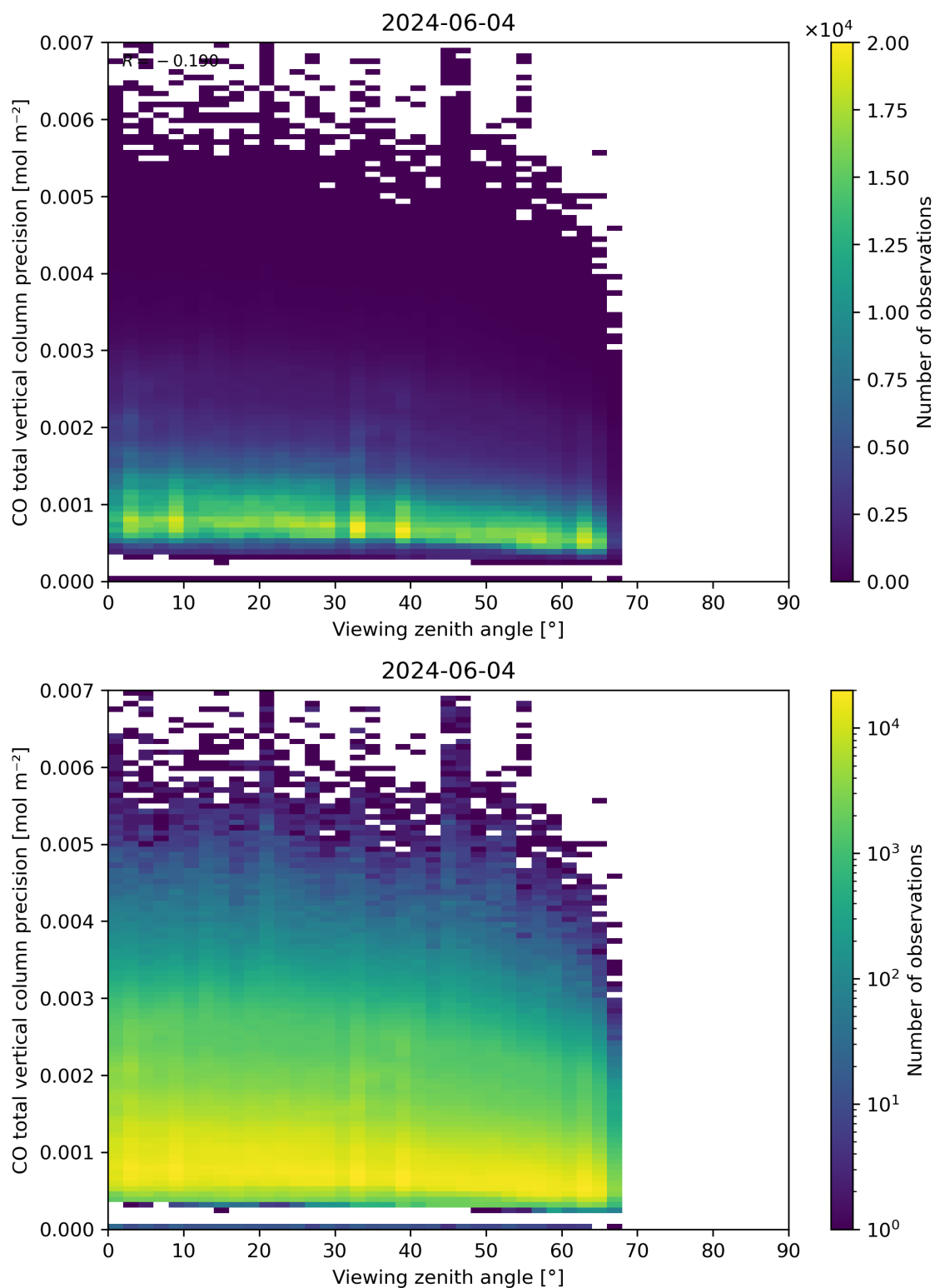
Figure 71: Scatter density plot of “Viewing zenith angle” against “CO total vertical column precision” for 2024-06-03 to 2024-06-05.
