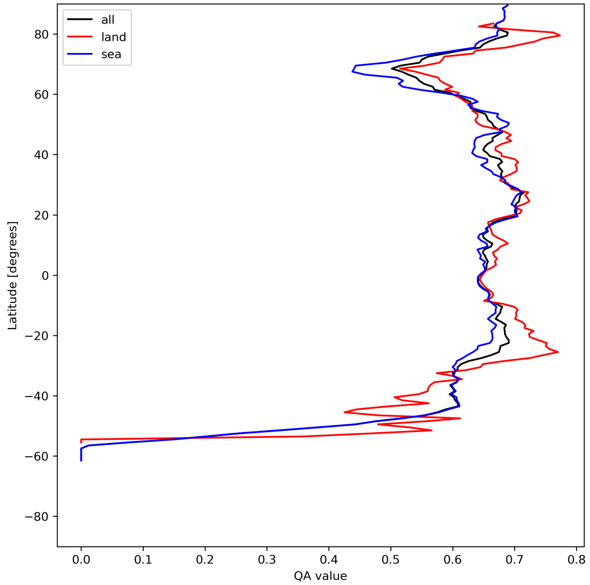
Figure 9: Zonal average of “QA value” for 2024-06-03 to 2024-06-05.
