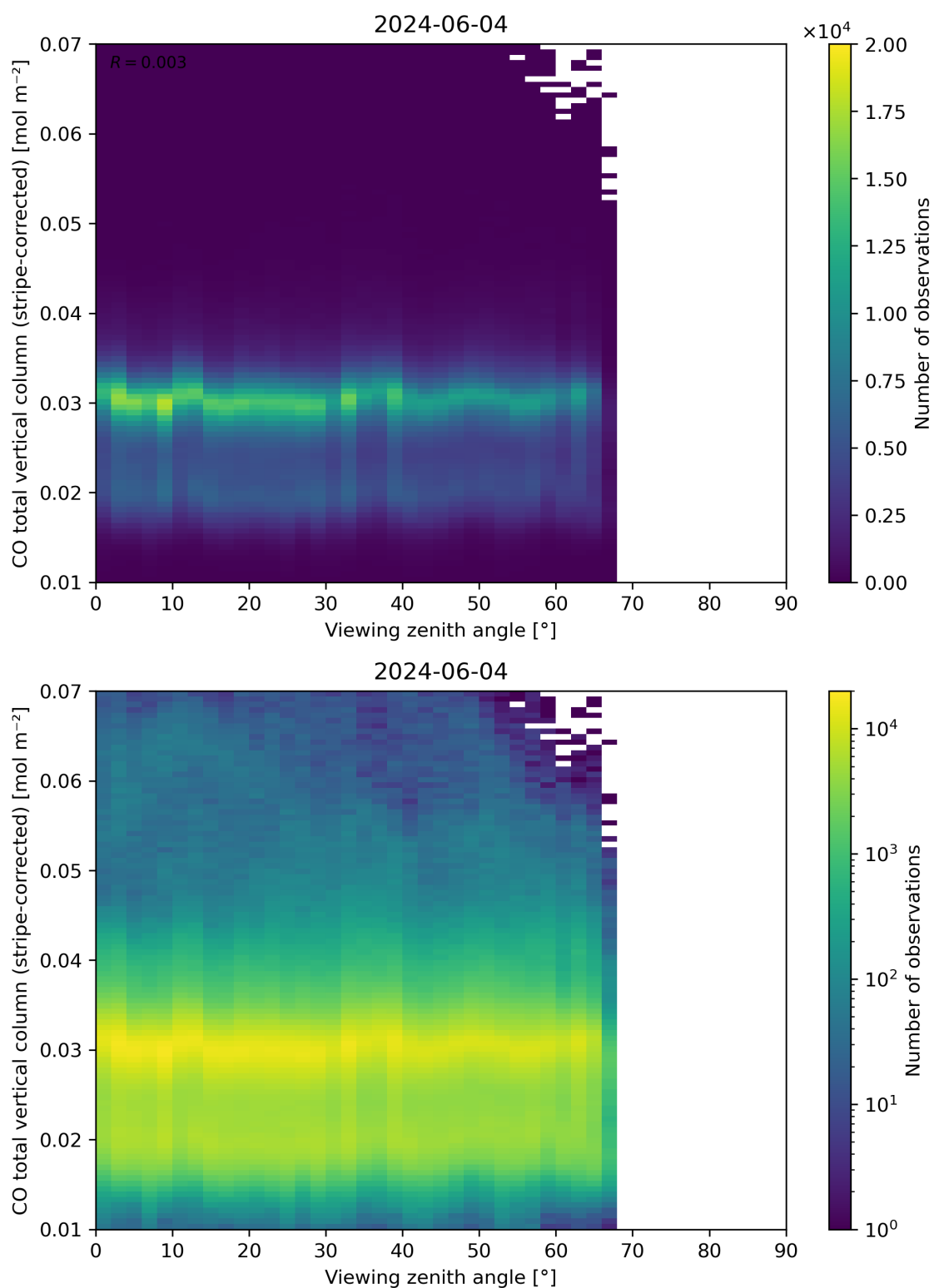
Figure 70: Scatter density plot of “Viewing zenith angle” against “CO total vertical column (stripe-corrected)” for 2024-06-03 to 2024-06-05.
