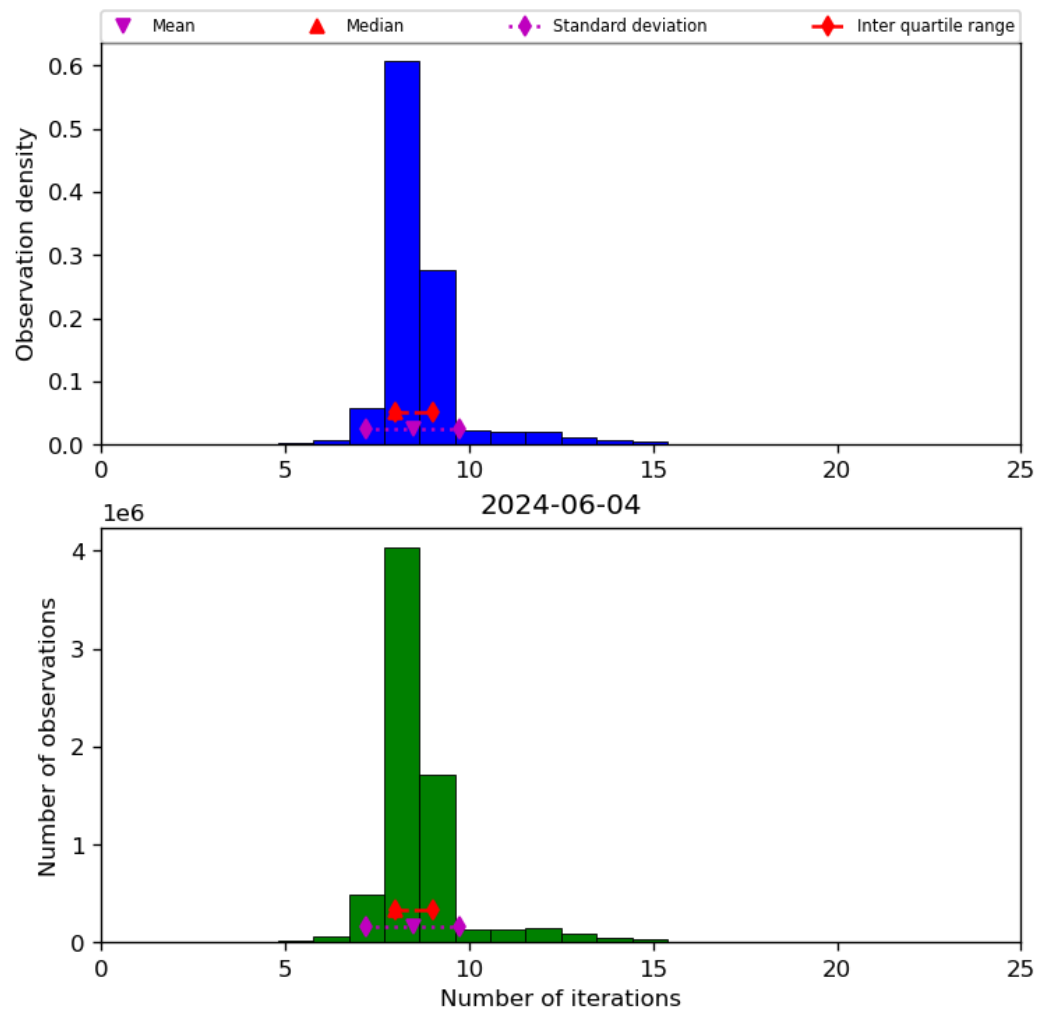
Figure 24: Histogram of “Number of iterations” for 2024-06-03 to 2024-06-05
