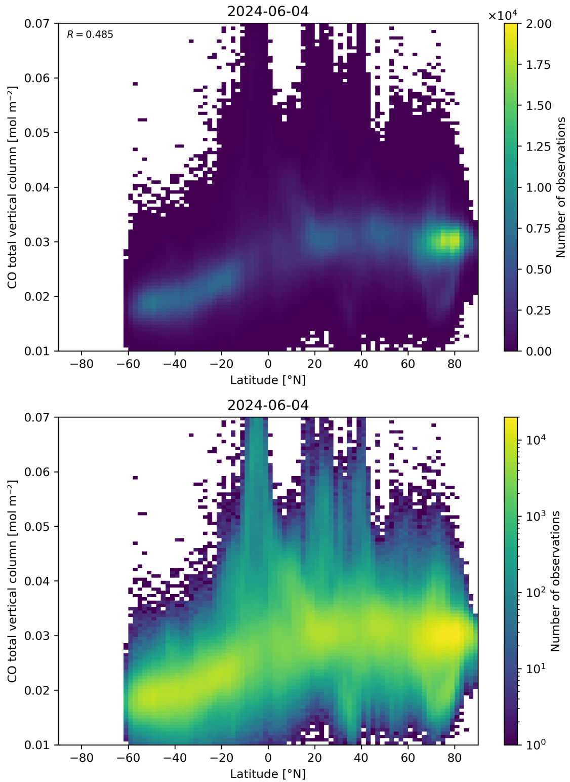
Figure 51: Scatter density plot of “Latitude” against “CO total vertical column” for 2024-06-03 to 2024-06-05.
