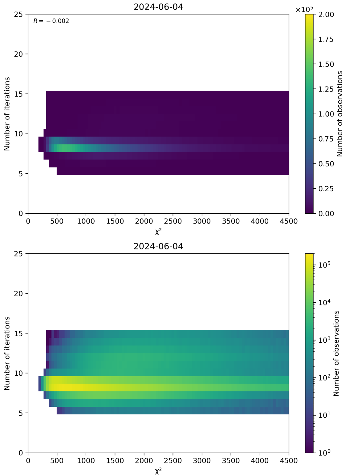
Figure 49: Scatter density plot of “ \chi^2 ” against “Number of iterations” for 2024-06-03 to 2024-06-05.
