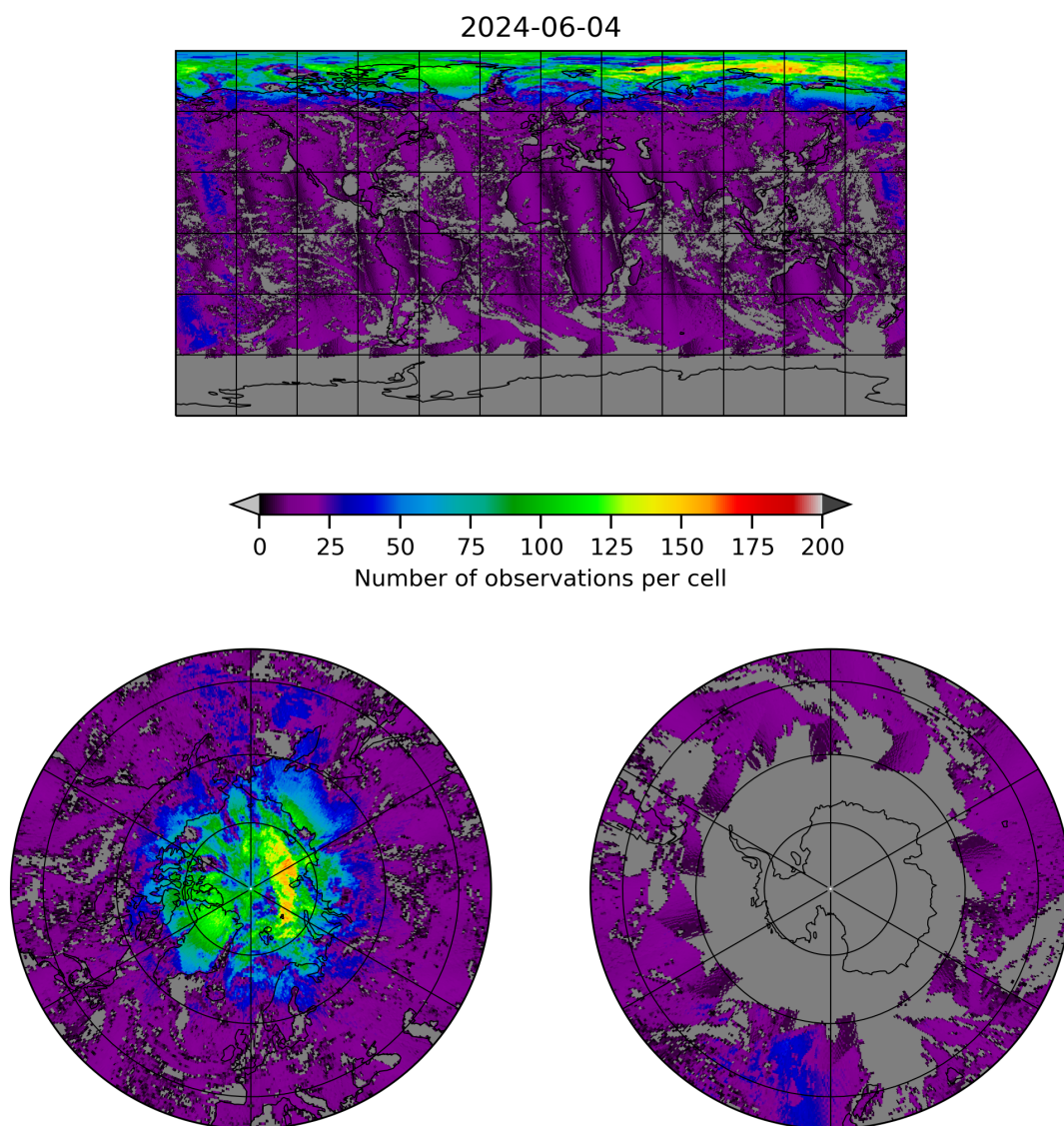
Figure 8: Map of the number of observations for 2024-06-03 to 2024-06-05
