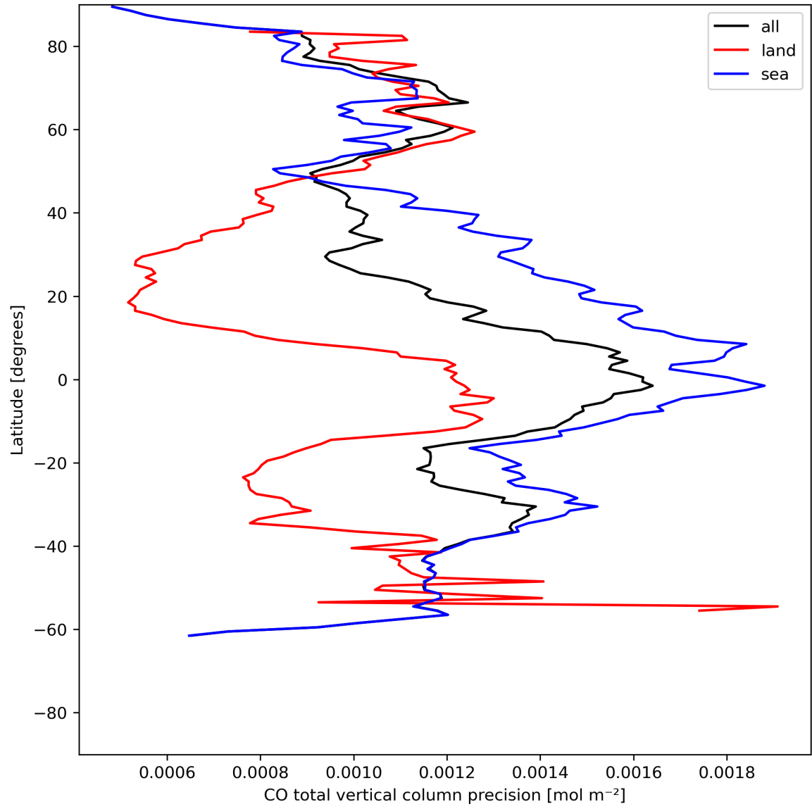
Figure 12: Zonal average of “CO total vertical column precision” for 2024-06-03 to 2024-06-05.
