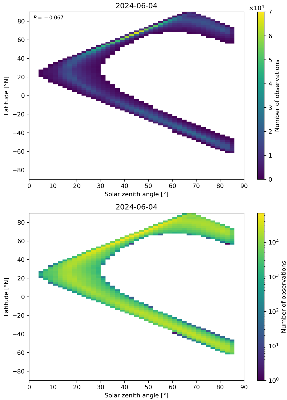
Figure 66: Scatter density plot of “Solar zenith angle” against “Latitude” for 2024-06-03 to 2024-06-05.
