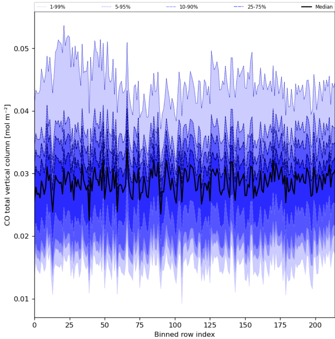
Figure 26: Along track statistics of “CO total vertical column” for 2024-06-03 to 2024-06-05
