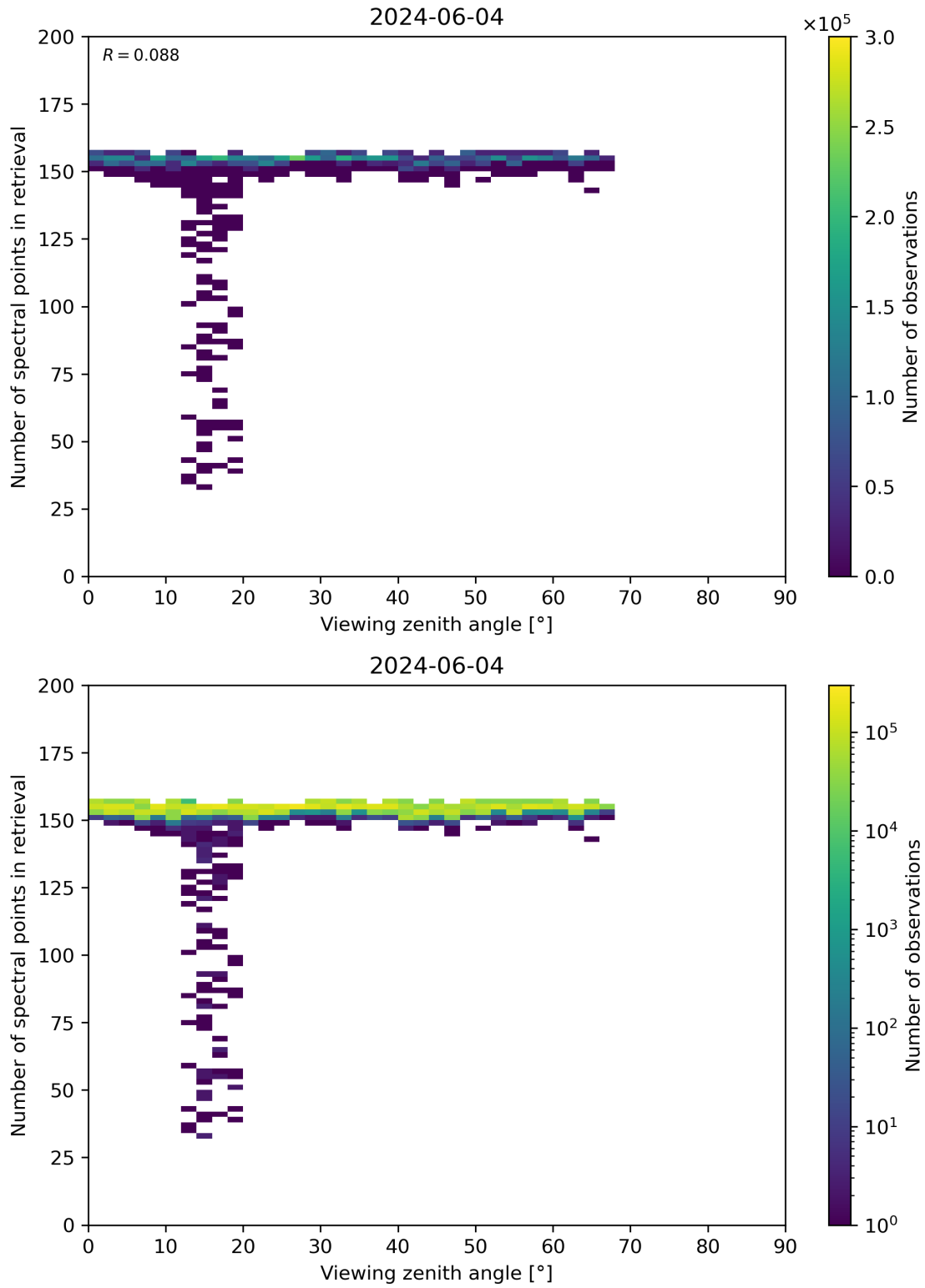
Figure 76: Scatter density plot of “Viewing zenith angle” against “Number of spectral points in retrieval” for 2024-06-03 to 2024-06-05.
