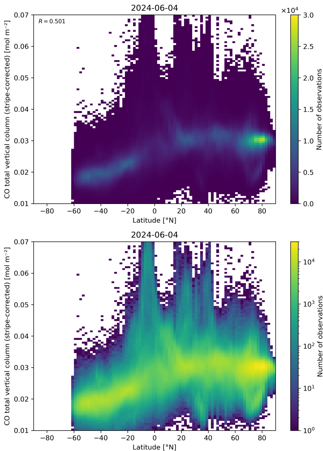
Figure 52: Scatter density plot of “Latitude” against “CO total vertical column (stripe-corrected)” for 2024-06-03 to 2024-06-05.
