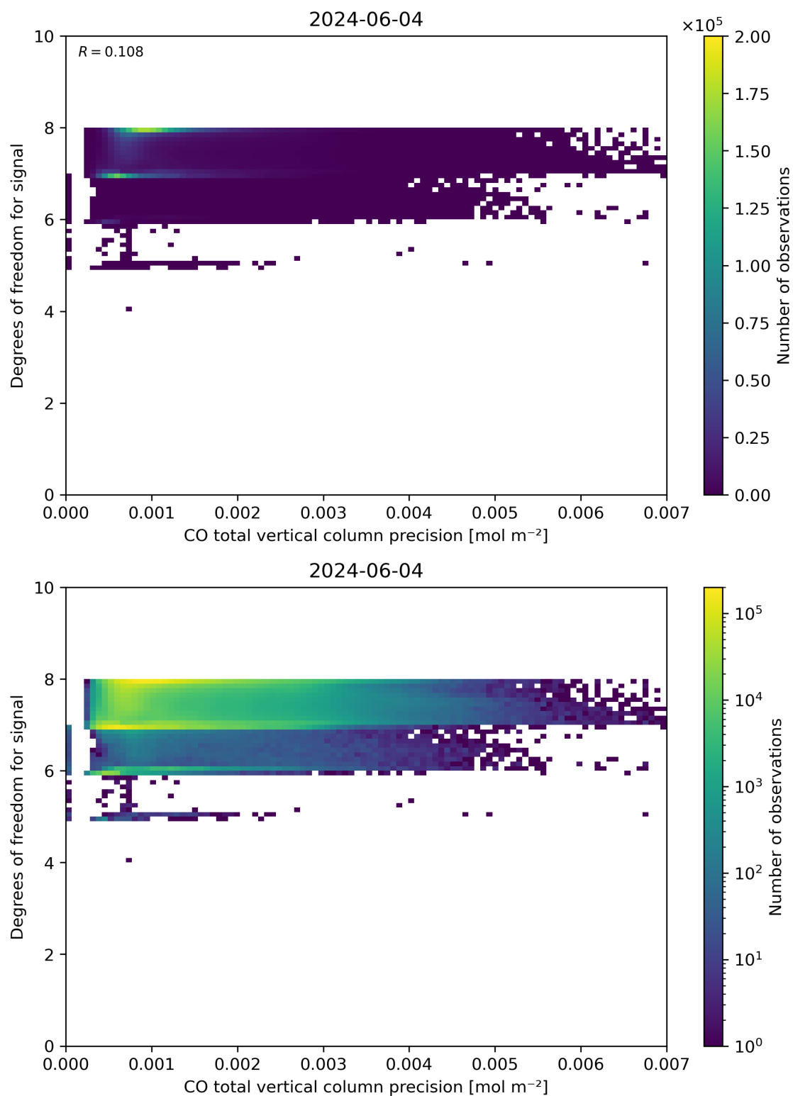
Figure 45: Scatter density plot of “CO total vertical column precision” against “Degrees of freedom for signal” for 2024-06-03 to 2024-06-05.
