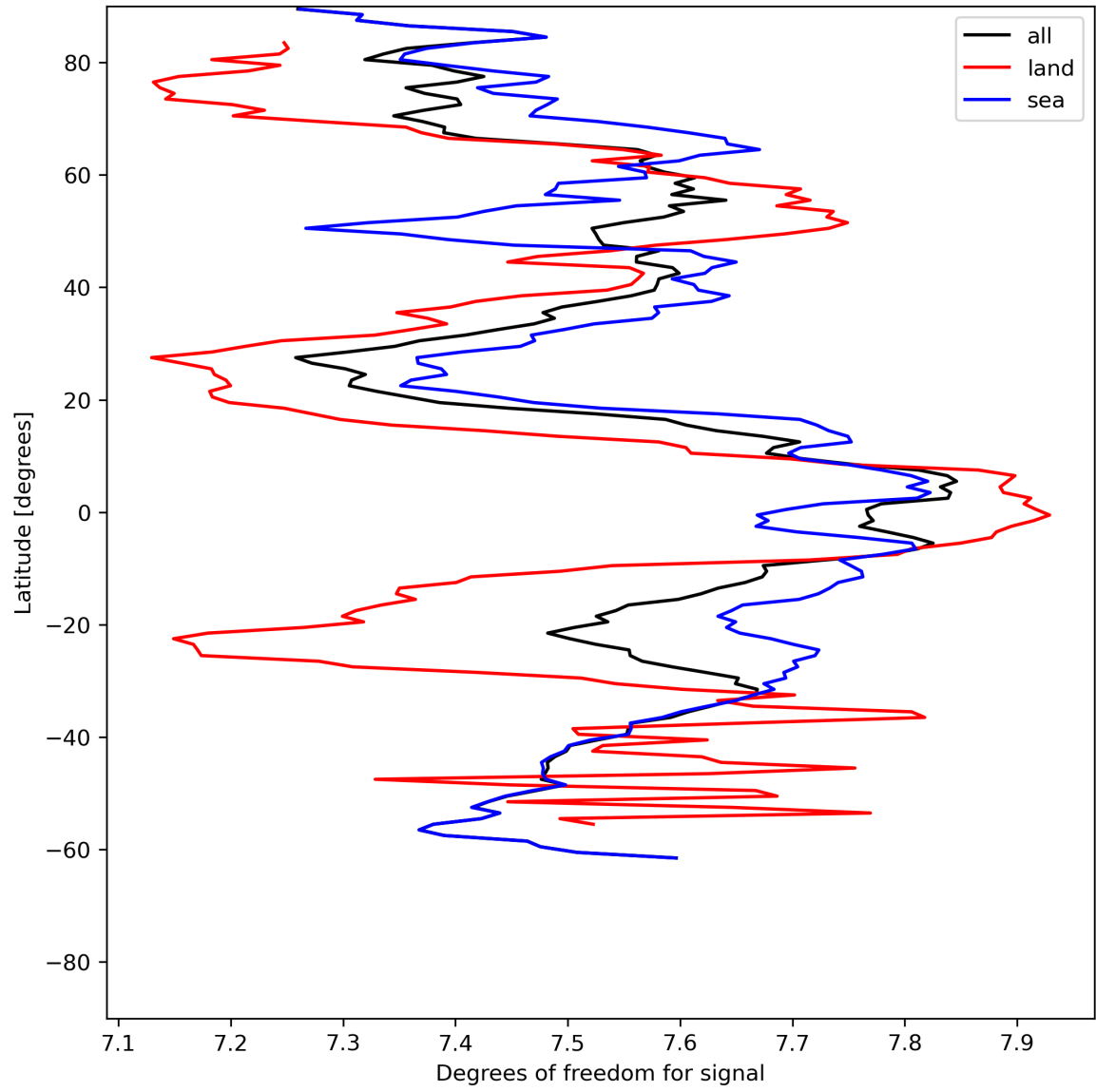
Figure 15: Zonal average of “Degrees of freedom for signal” for 2024-06-03 to 2024-06-05.
