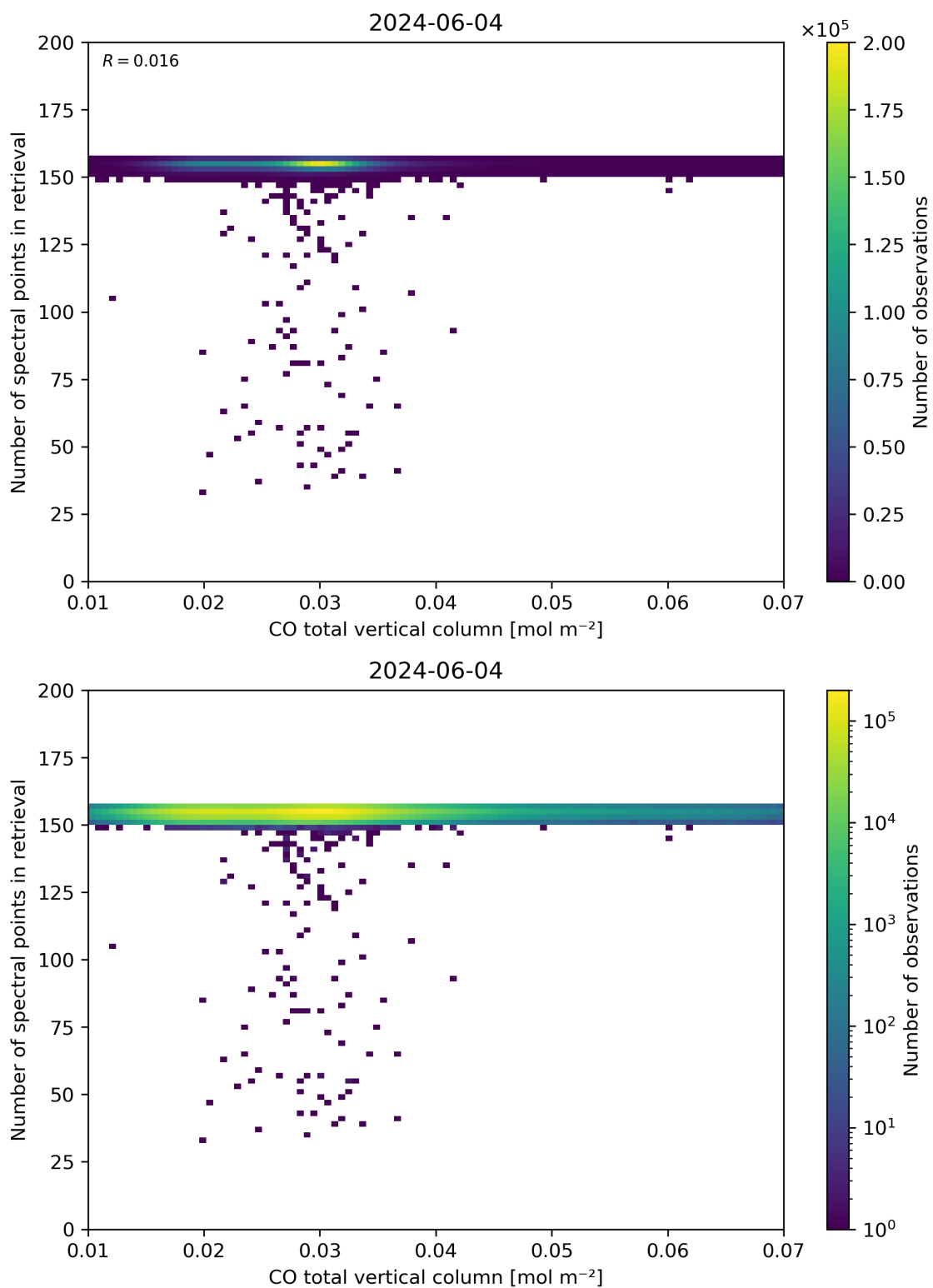
Figure 43: Scatter density plot of “CO total vertical column” against “Number of spectral points in retrieval” for 2024-06-03 to 2024-06-05.
