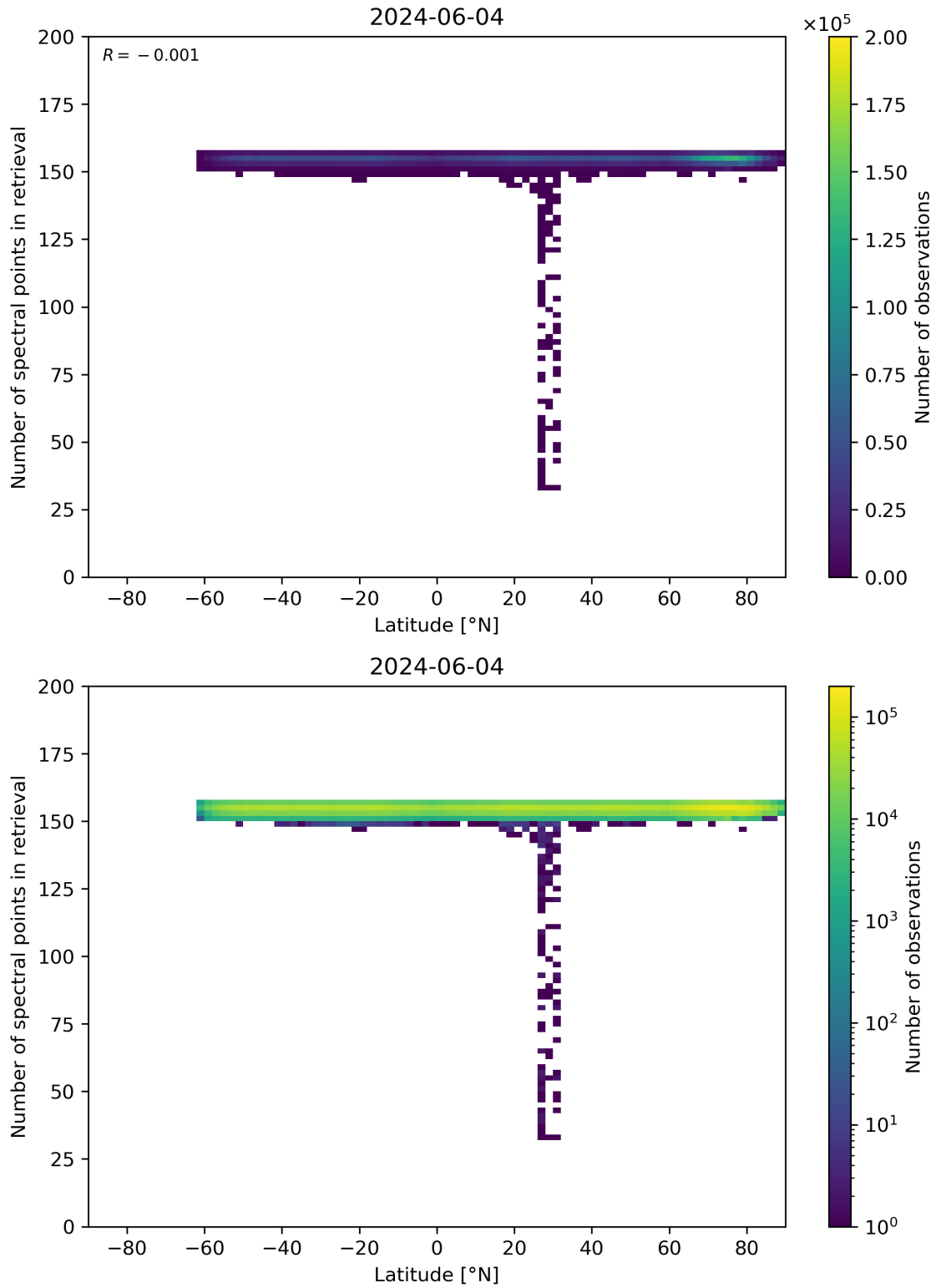
Figure 57: Scatter density plot of “Latitude” against “Number of spectral points in retrieval” for 2024-06-03 to 2024-06-05.
