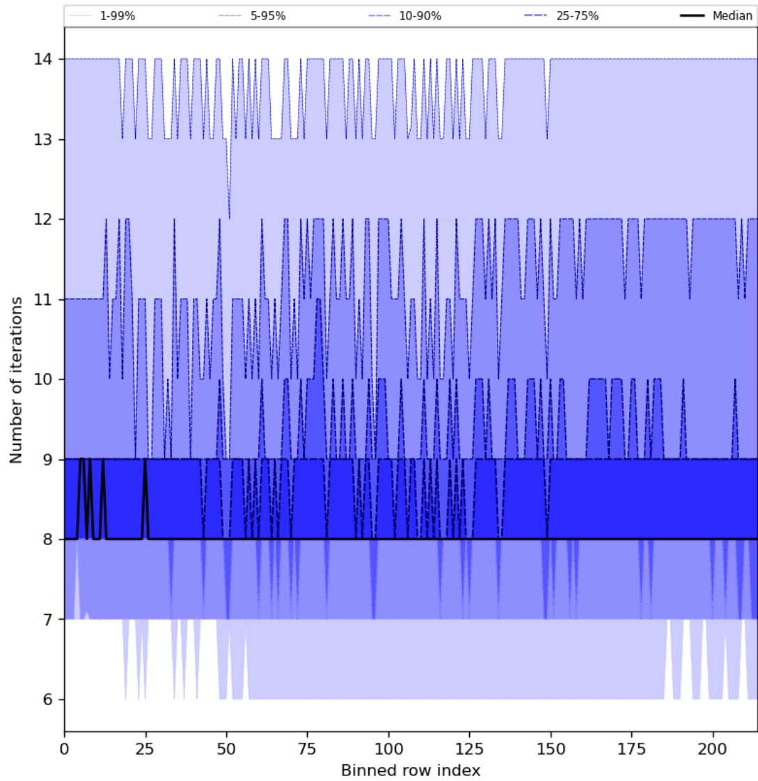
Figure 32: Along track statistics of “Number of iterations” for 2024-06-03 to 2024-06-05
