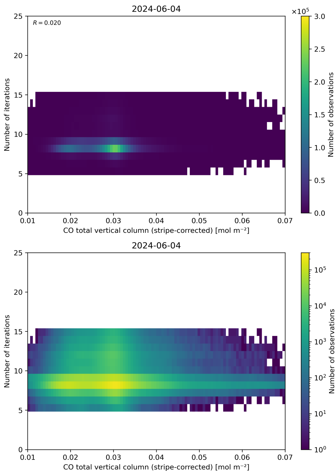
Figure 39: Scatter density plot of “CO total vertical column (stripe-corrected)” against “Number of iterations” for 2024-06-03 to 2024-06-05.
