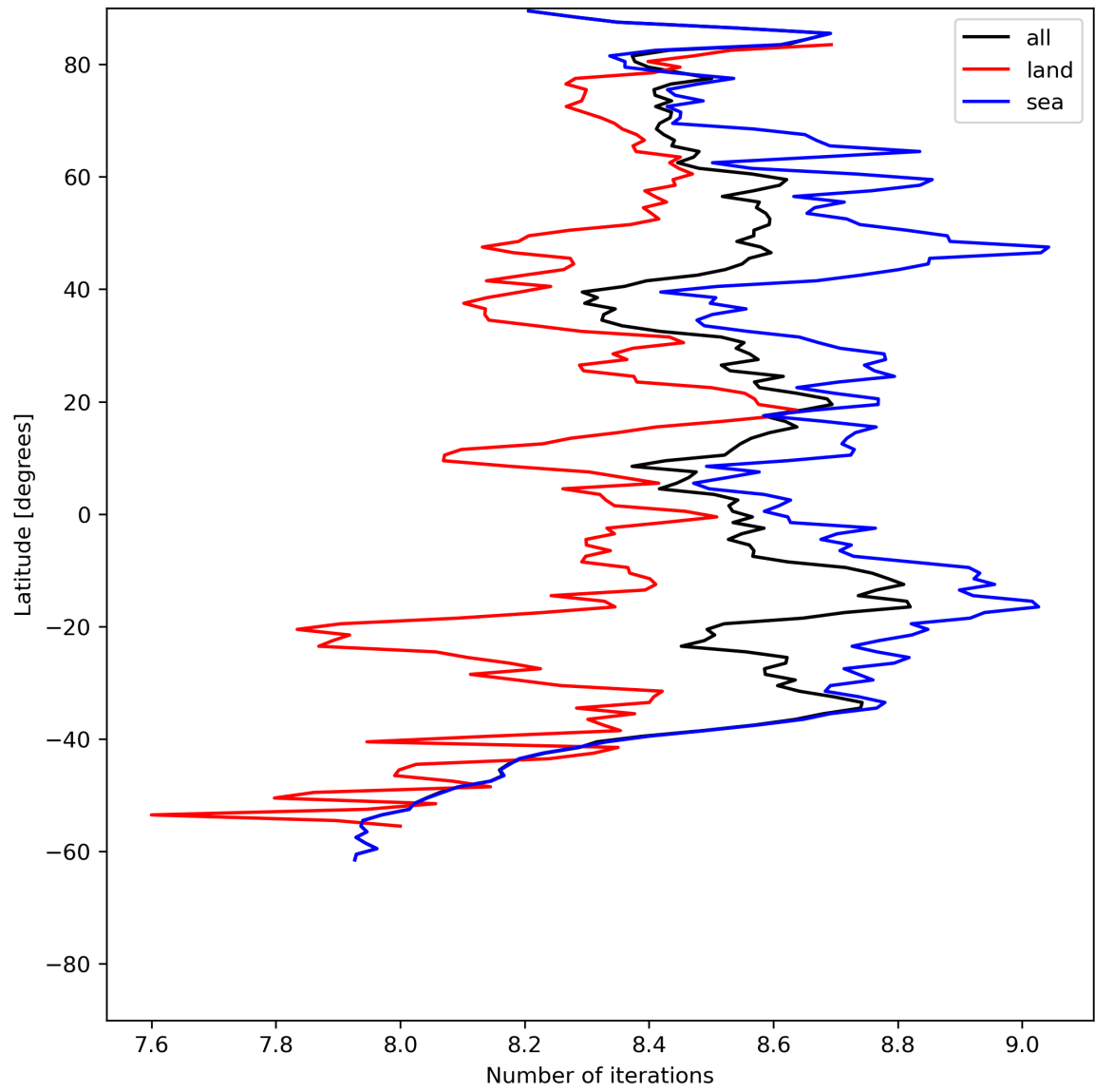
Figure 16: Zonal average of “Number of iterations” for 2024-06-03 to 2024-06-05.
