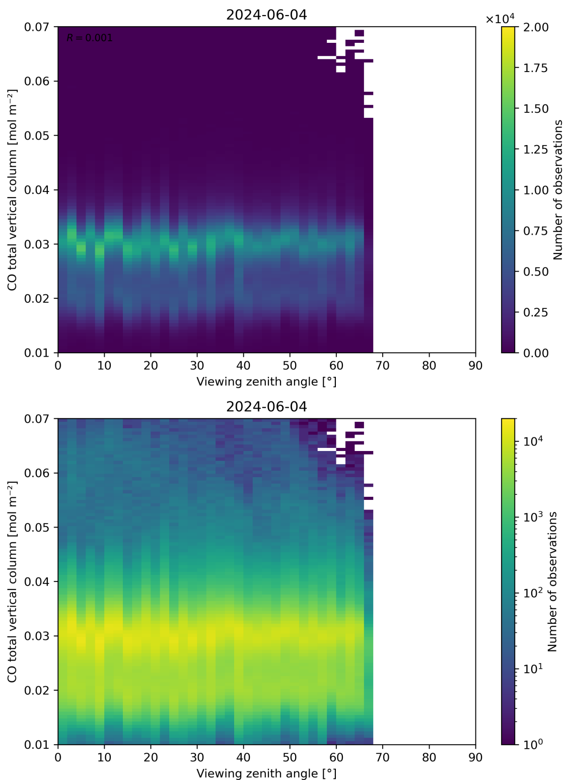
Figure 69: Scatter density plot of “Viewing zenith angle” against “CO total vertical column” for 2024-06-03 to 2024-06-05.
