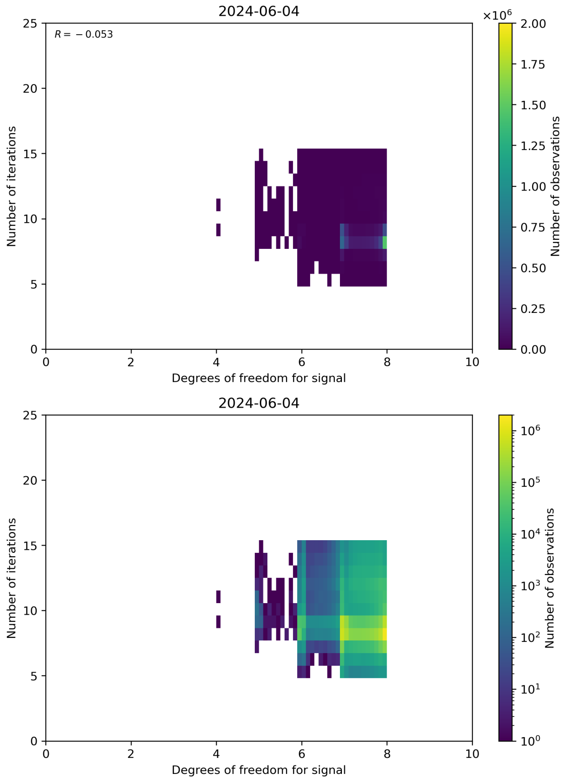
Figure 50: Scatter density plot of “Degrees of freedom for signal” against “Number of iterations” for 2024-06-03 to 2024-06-05.
