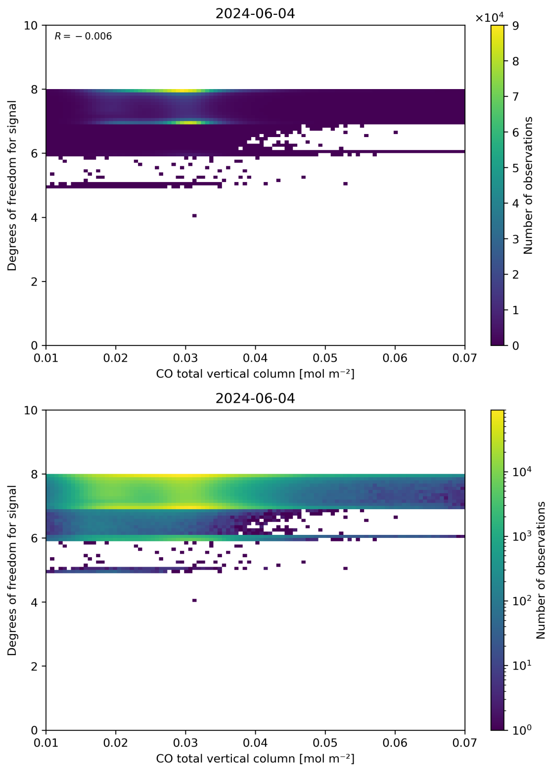
Figure 41: Scatter density plot of “CO total vertical column” against “Degrees of freedom for signal” for 2024-06-03 to 2024-06-05.
