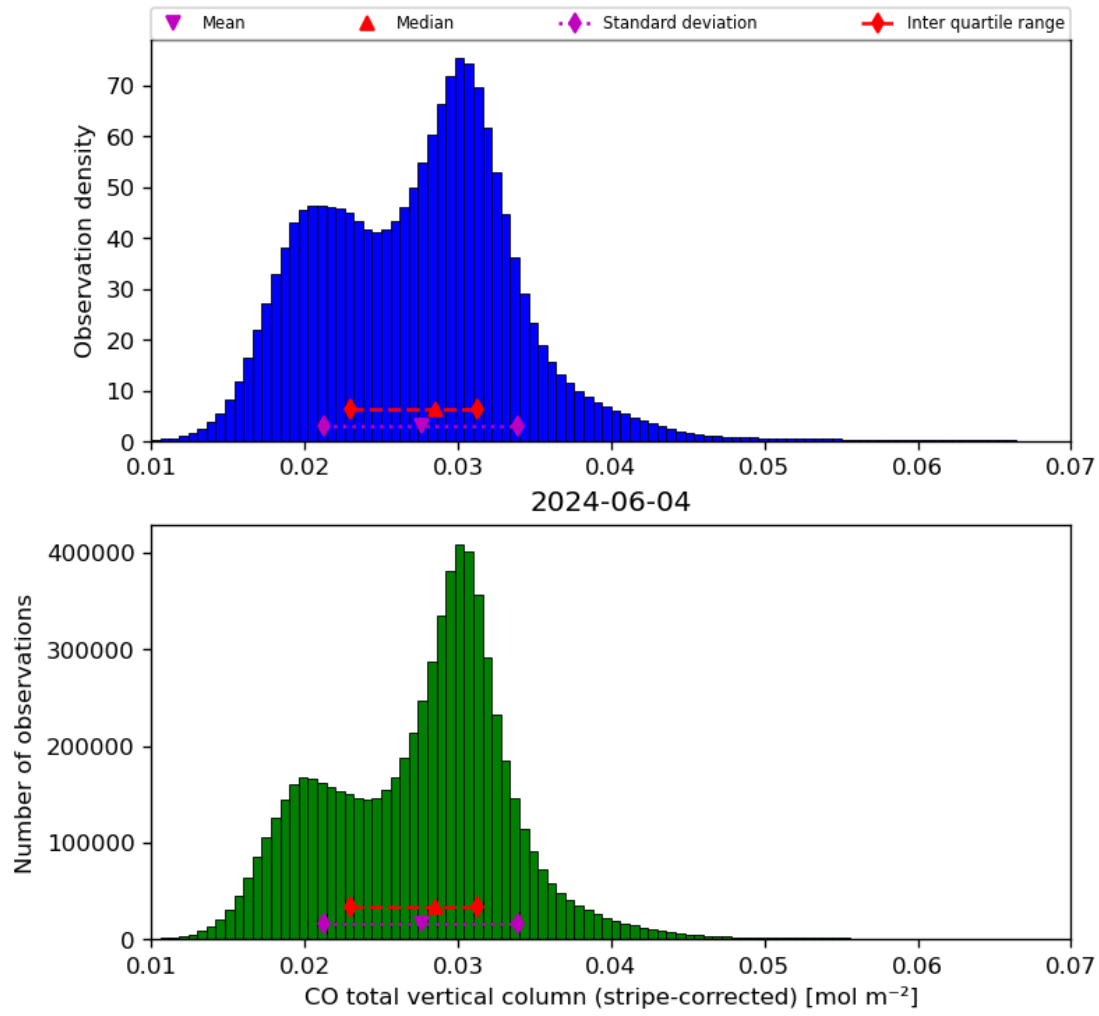
Figure 19: Histogram of “CO total vertical column (stripe-corrected)” for 2024-06-03 to 2024-06-05
