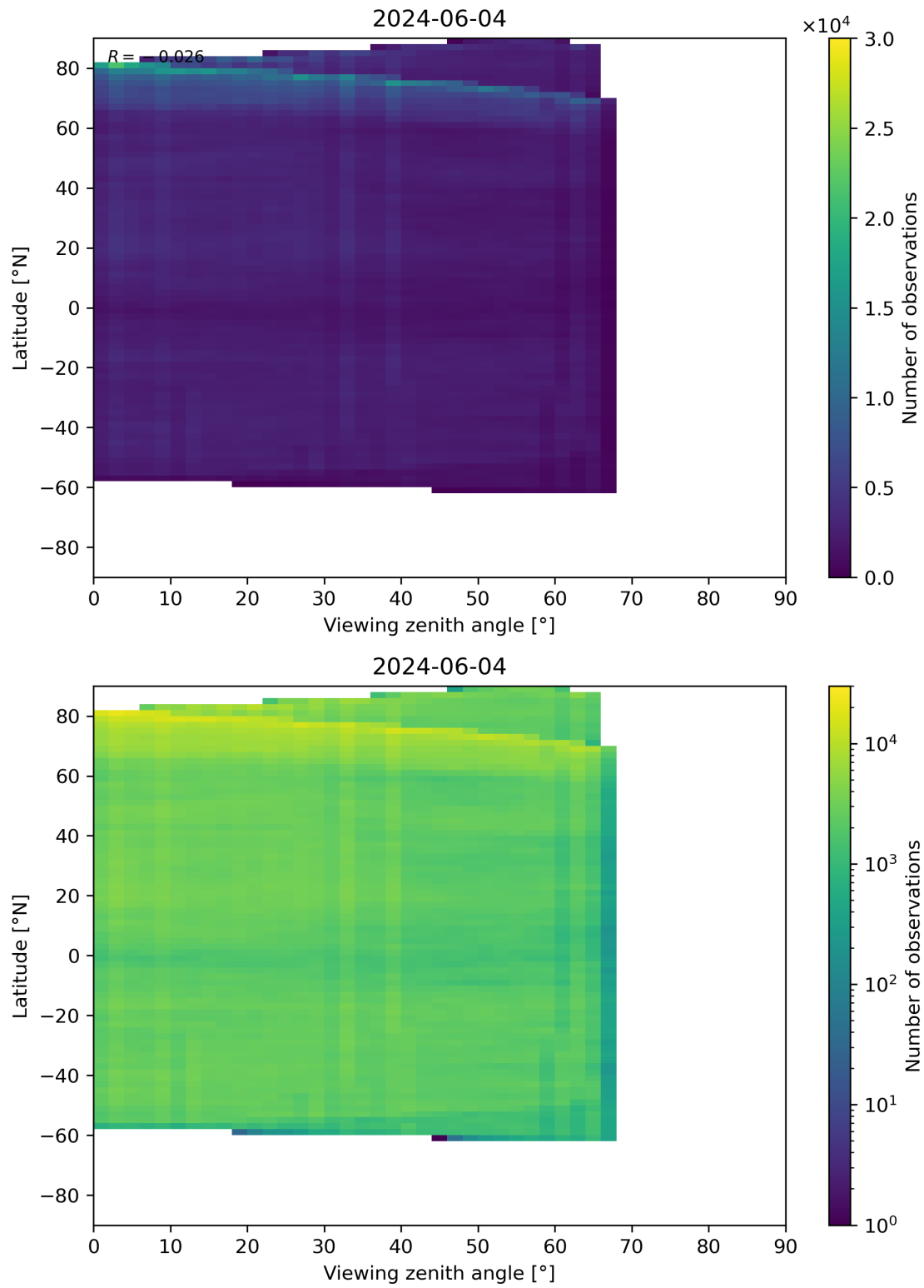
Figure 74: Scatter density plot of “Viewing zenith angle” against “Latitude” for 2024-06-03 to 2024-06-05.
