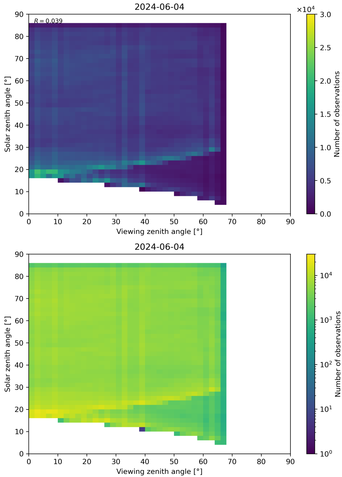
Figure 77: Scatter density plot of “Viewing zenith angle” against “Solar zenith angle” for 2024-06-03 to 2024-06-05.
