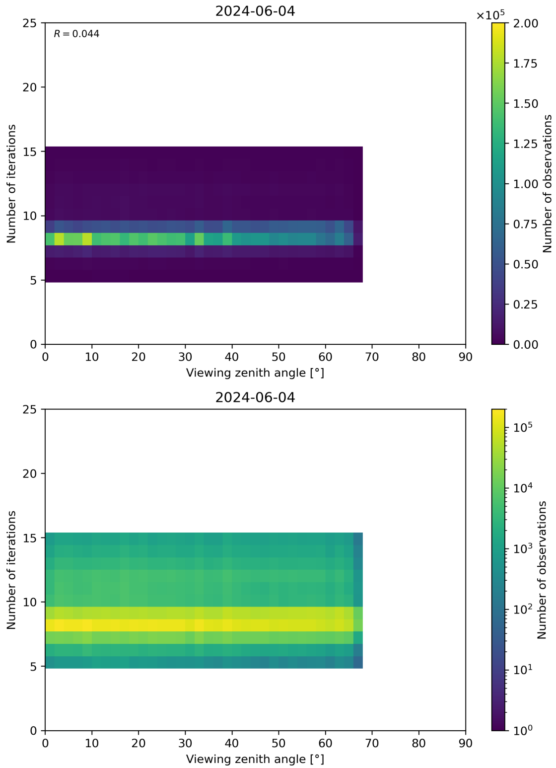
Figure 75: Scatter density plot of “Viewing zenith angle” against “Number of iterations” for 2024-06-03 to 2024-06-05.
