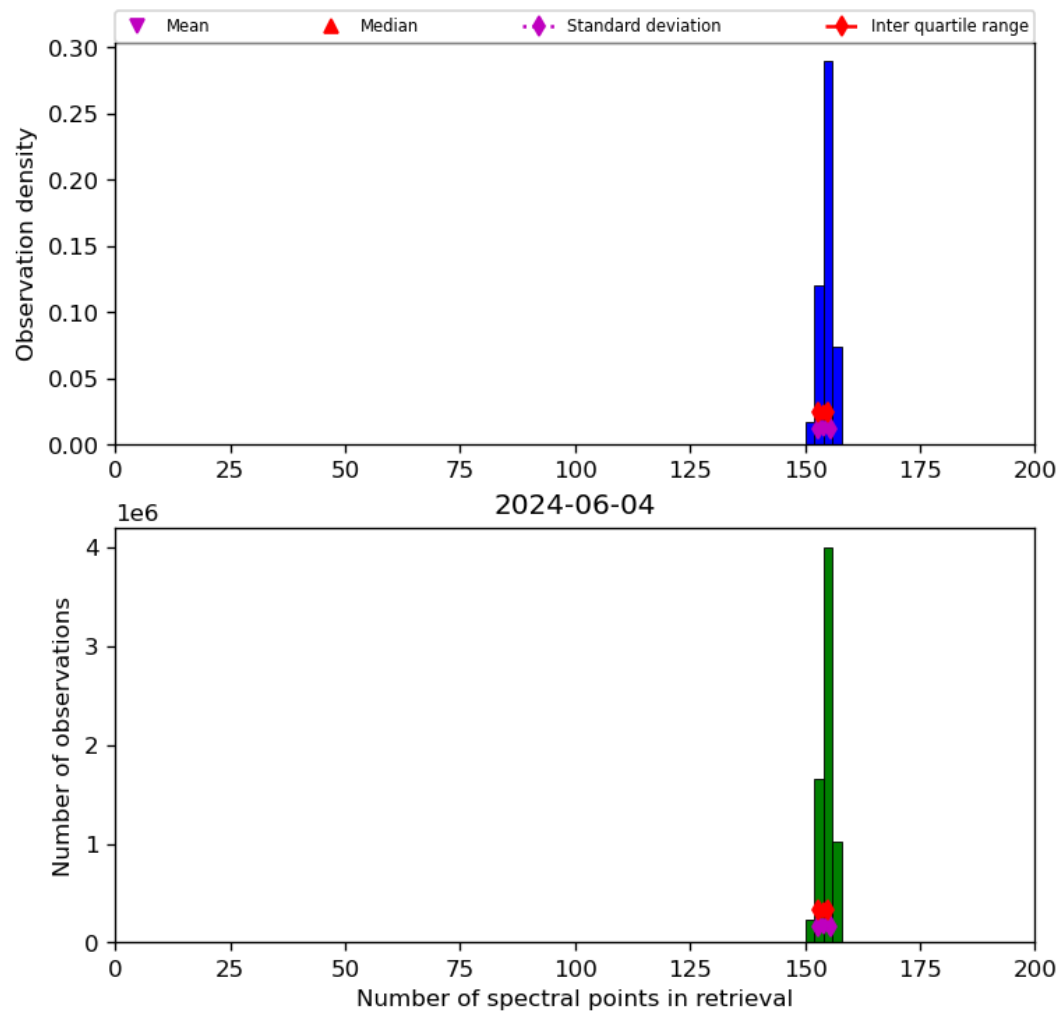
Figure 21: Histogram of “Number of spectral points in retrieval” for 2024-06-03 to 2024-06-05
