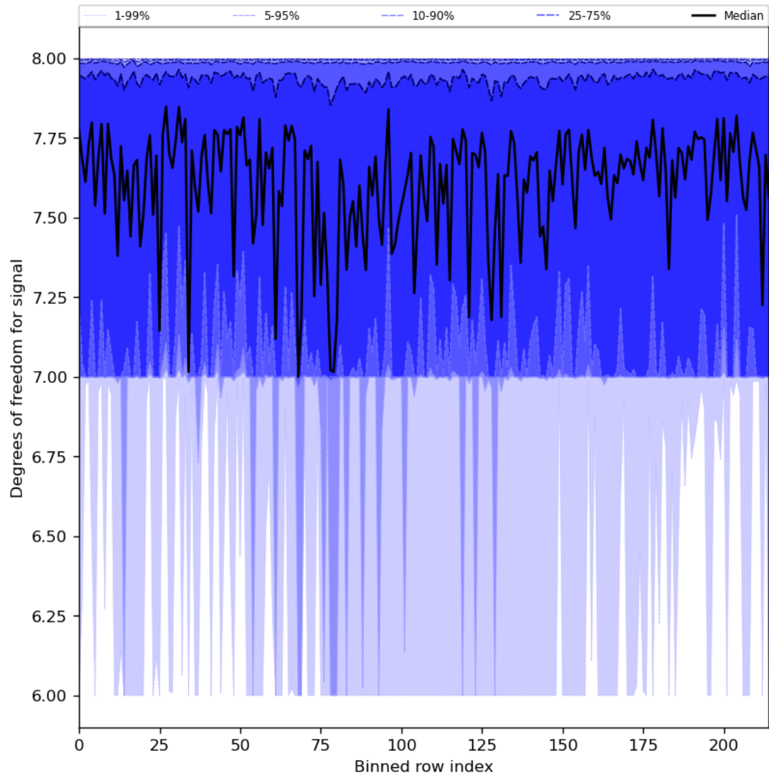
Figure 31: Along track statistics of “Degrees of freedom for signal” for 2024-06-03 to 2024-06-05
