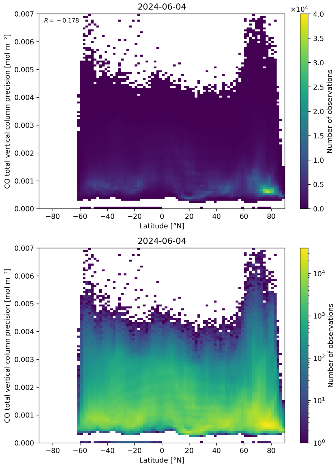
Figure 53: Scatter density plot of “Latitude” against “CO total vertical column precision” for 2024-06-03 to 2024-06-05.
