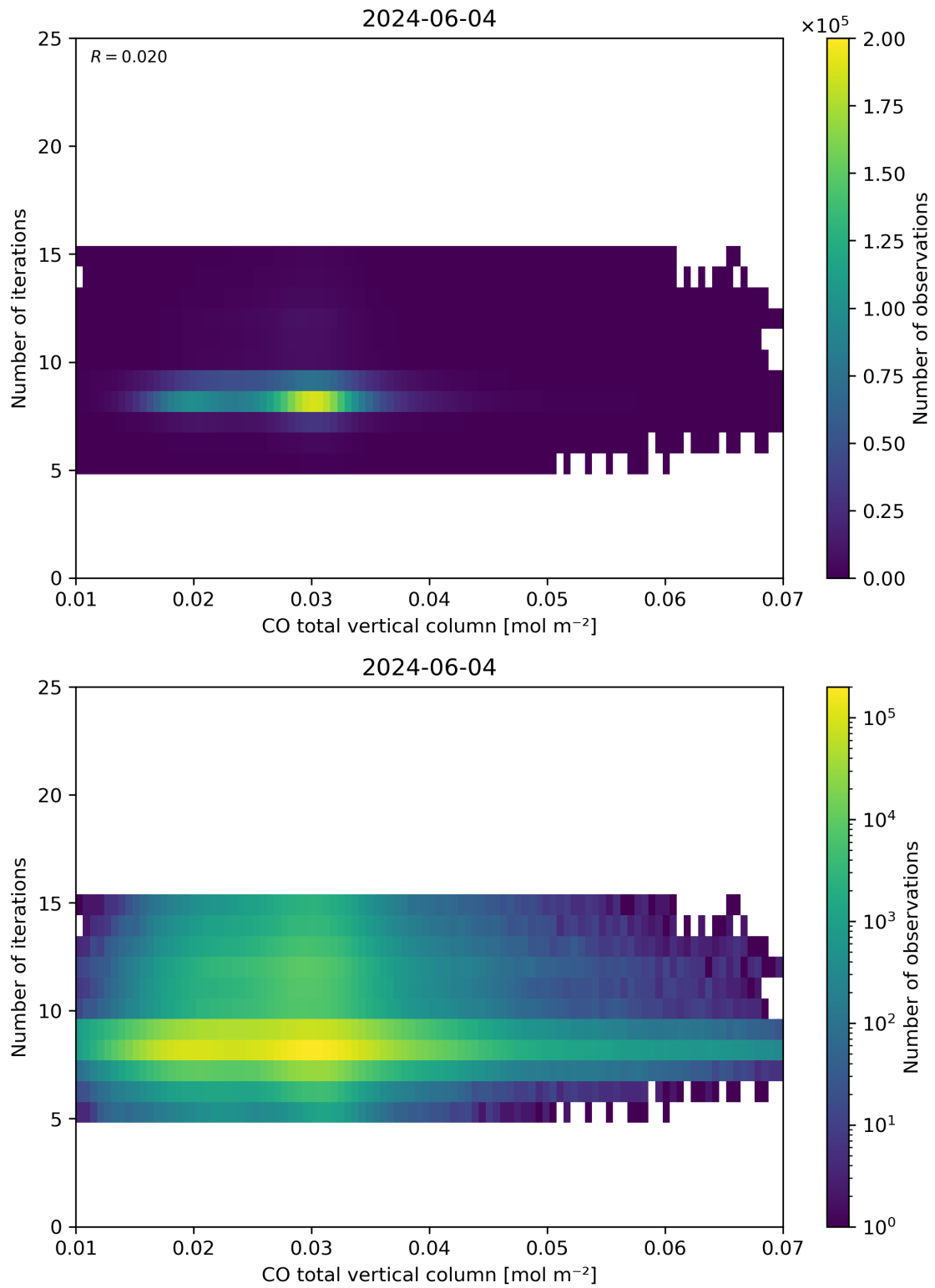
Figure 42: Scatter density plot of “CO total vertical column” against “Number of iterations” for 2024-06-03 to 2024-06-05.
