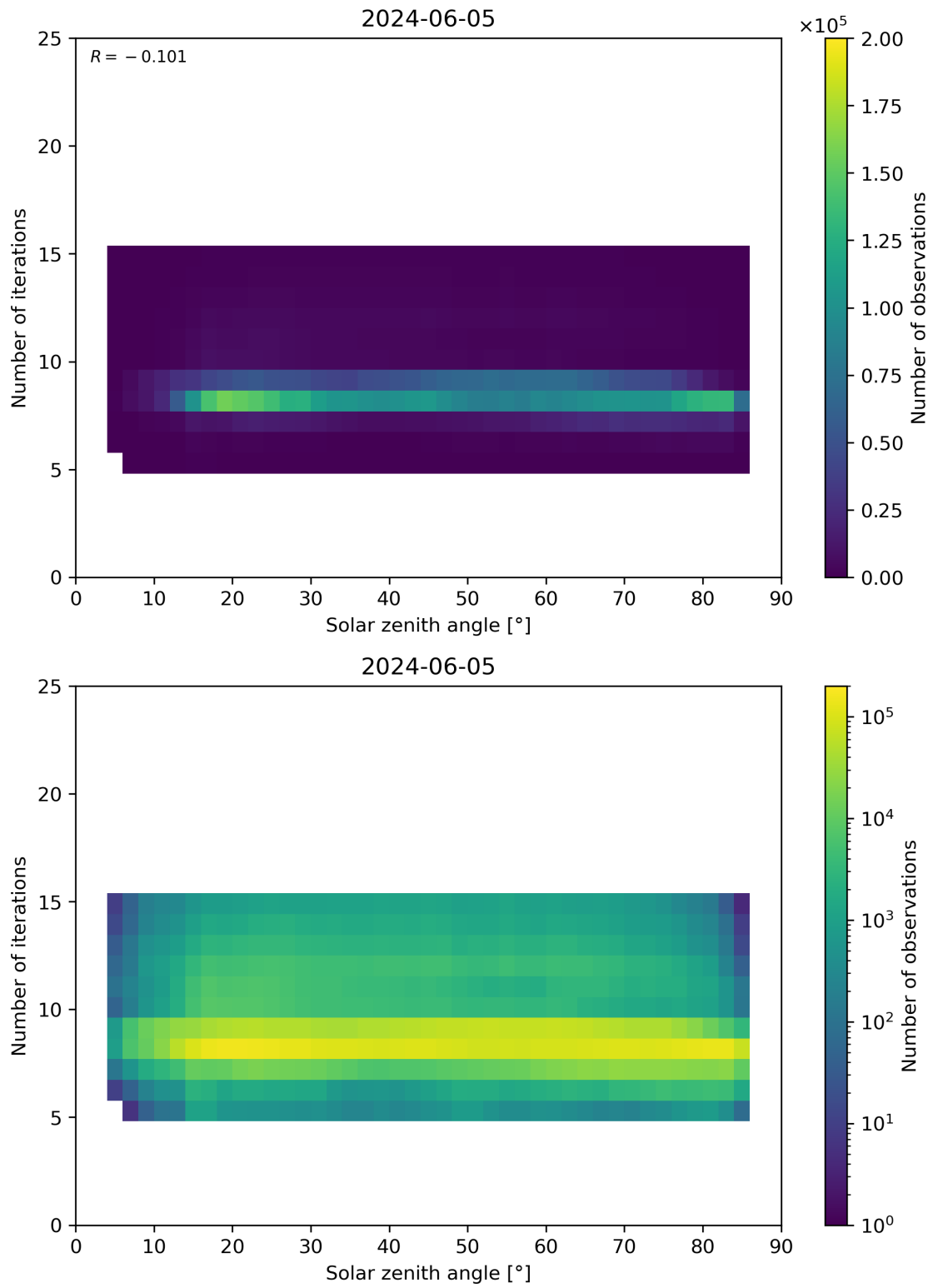
Figure 67: Scatter density plot of “Solar zenith angle” against “Number of iterations” for 2024-06-04 to 2024-06-06.
