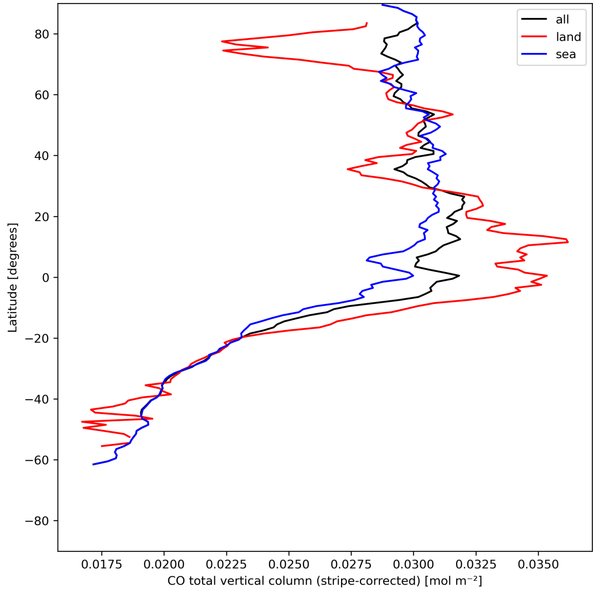
Figure 11: Zonal average of “CO total vertical column (stripe-corrected)” for 2024-06-04 to 2024-06-06.
