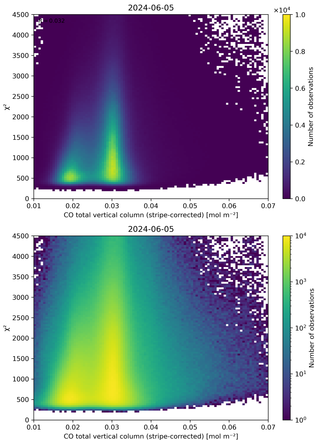
Figure 37: Scatter density plot of “CO total vertical column (stripe-corrected)” against “ \chi^2 ” for 2024-06-04 to 2024-06-06.
