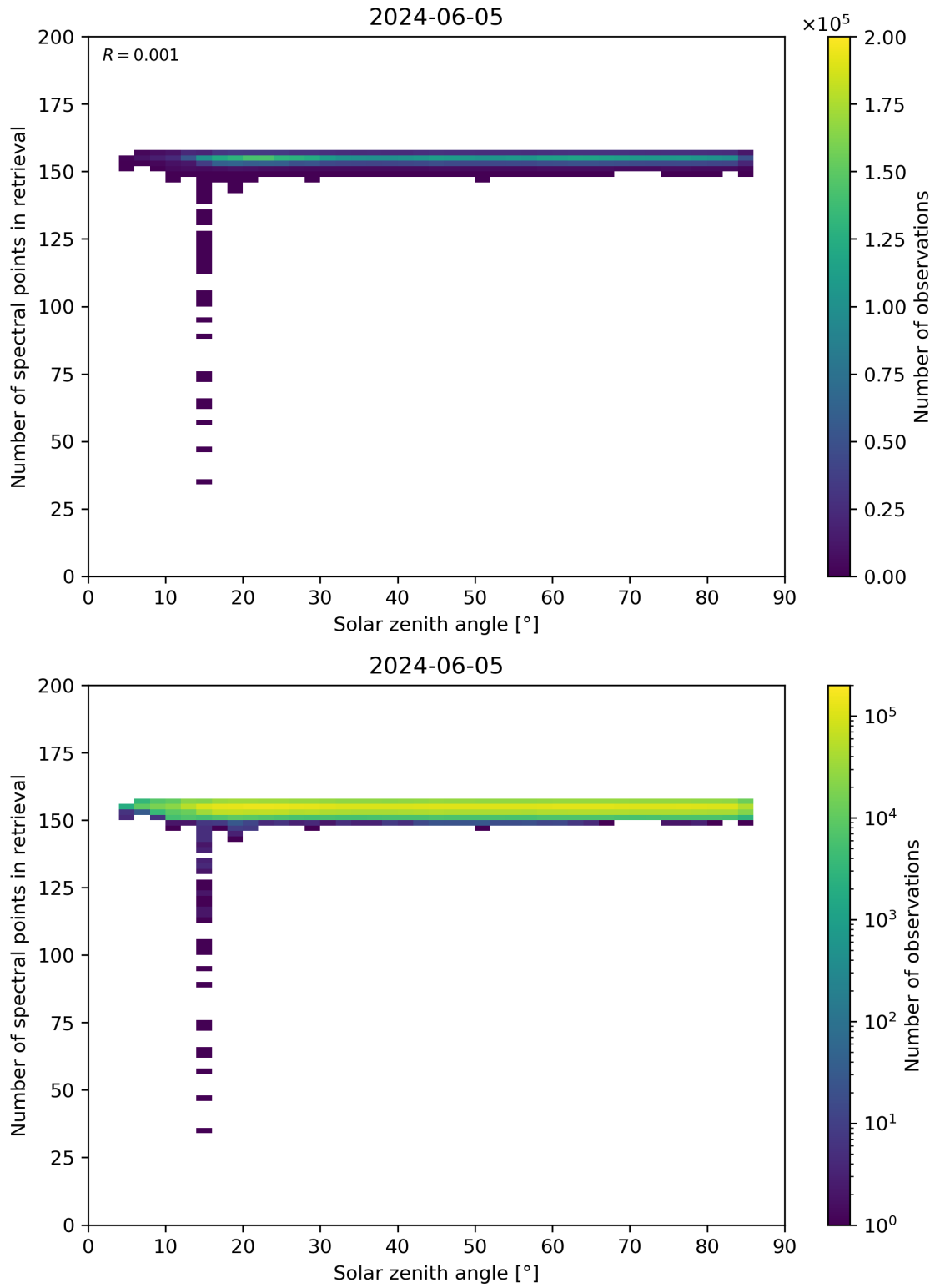
Figure 68: Scatter density plot of “Solar zenith angle” against “Number of spectral points in retrieval” for 2024-06-04 to 2024-06-06.
