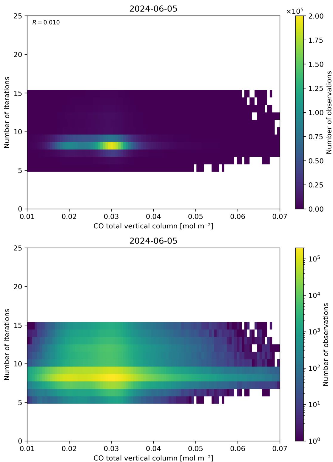
Figure 42: Scatter density plot of “CO total vertical column” against “Number of iterations” for 2024-06-04 to 2024-06-06.
