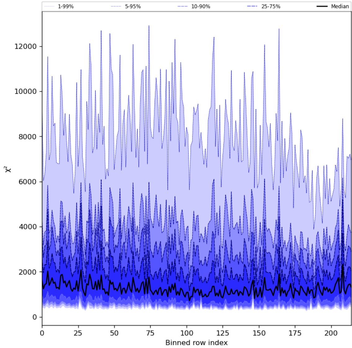
Figure 30: Along track statistics of “ \chi^2 ” for 2024-06-04 to 2024-06-06
