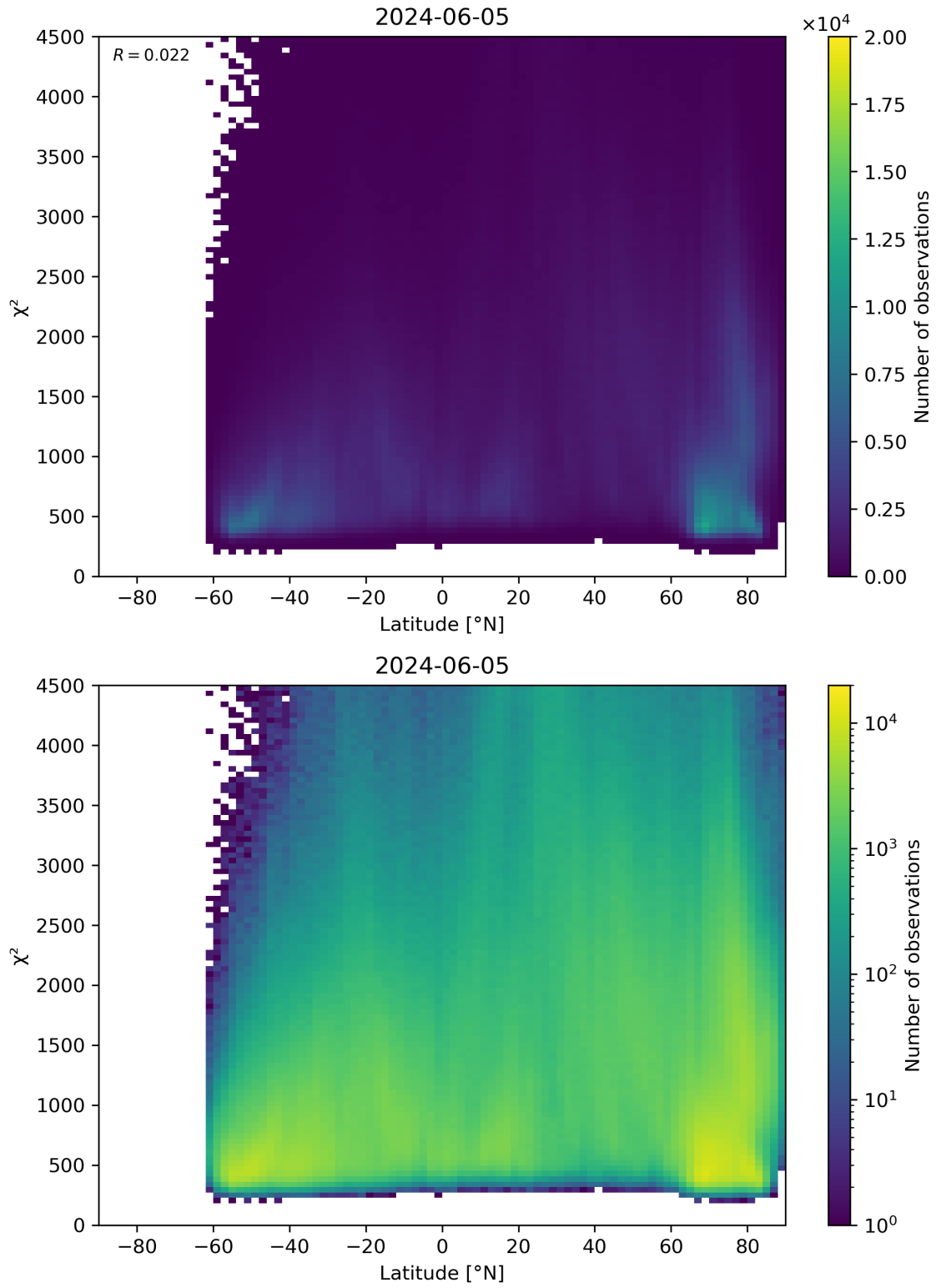
Figure 54: Scatter density plot of “Latitude” against “ \chi^2 ” for 2024-06-04 to 2024-06-06.
