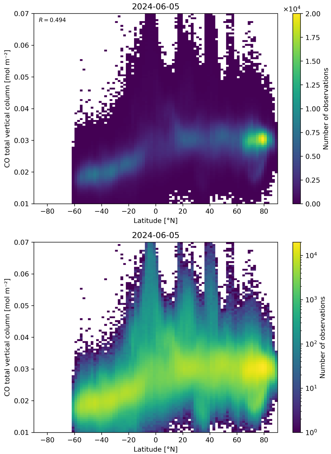
Figure 51: Scatter density plot of “Latitude” against “CO total vertical column” for 2024-06-04 to 2024-06-06.
