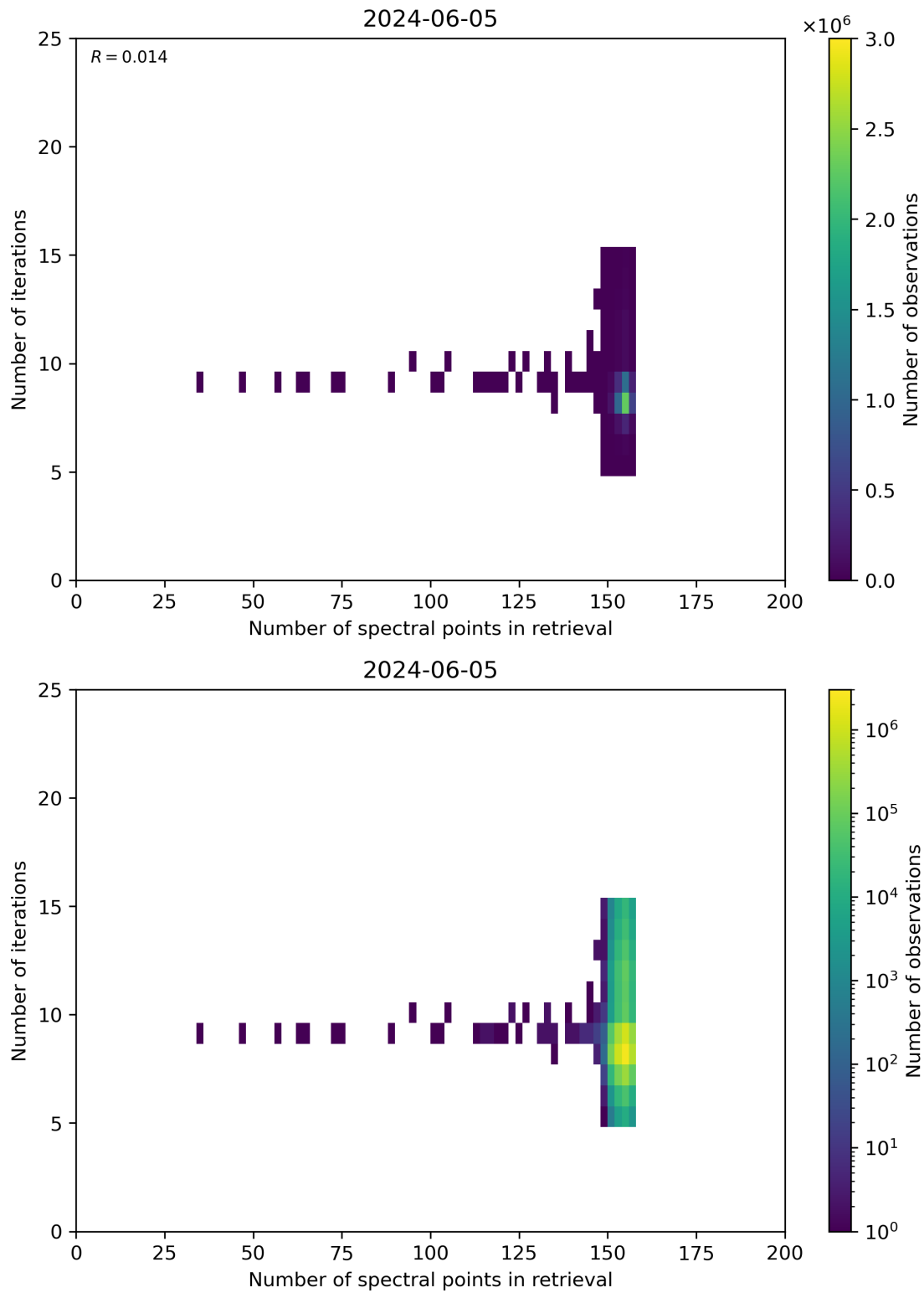
Figure 60: Scatter density plot of “Number of spectral points in retrieval” against “Number of iterations” for 2024-06-04 to 2024-06-06.
