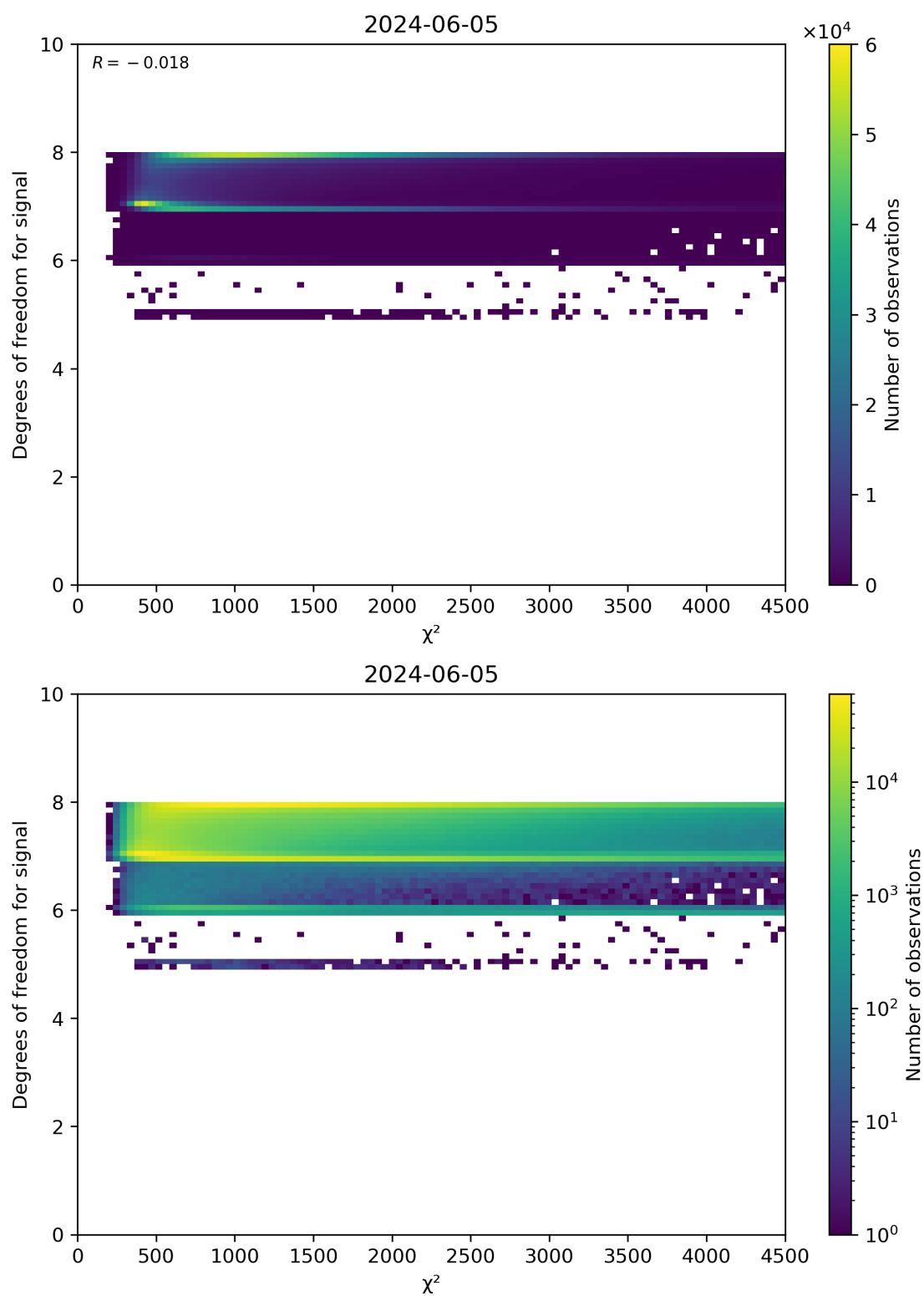
Figure 48: Scatter density plot of “ \chi^2 ” against “Degrees of freedom for signal” for 2024-06-04 to 2024-06-06.
