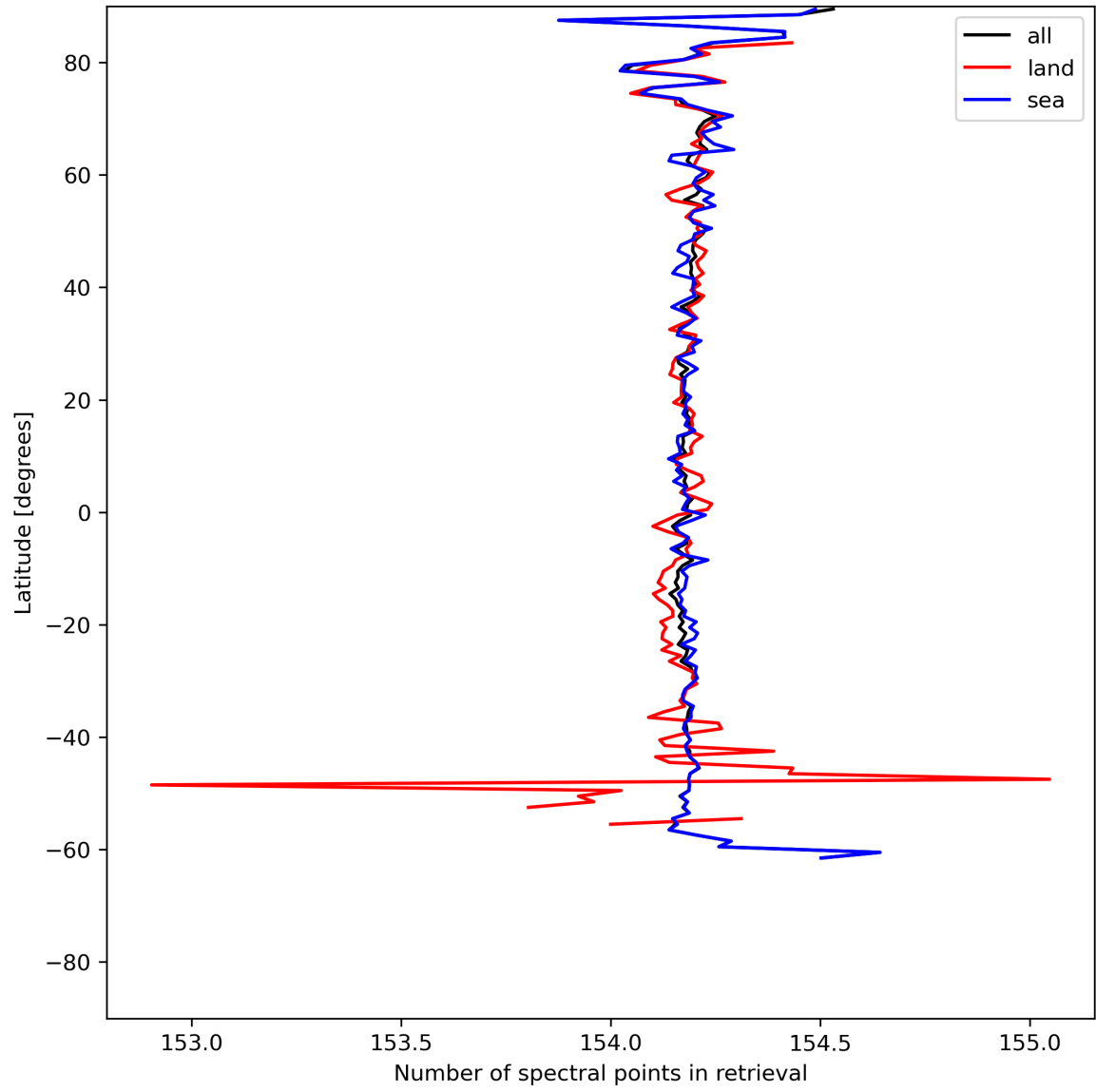
Figure 13: Zonal average of “Number of spectral points in retrieval” for 2024-06-04 to 2024-06-06.
