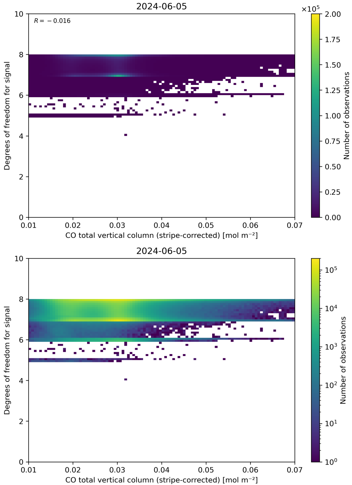
Figure 38: Scatter density plot of “CO total vertical column (stripe-corrected)” against “Degrees of freedom for signal” for 2024-06-04 to 2024-06-06.
