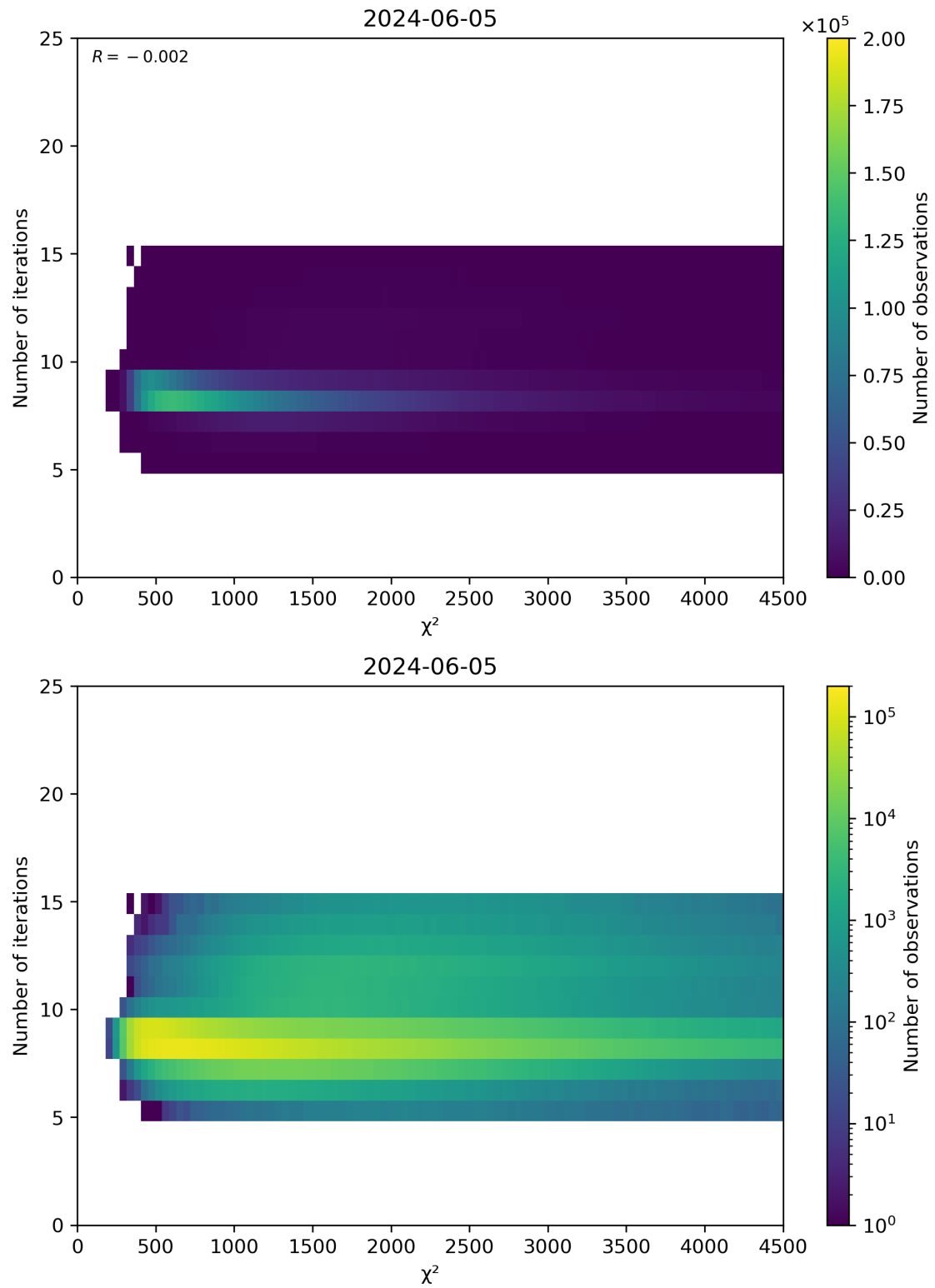
Figure 49: Scatter density plot of “ \chi^2 ” against “Number of iterations” for 2024-06-04 to 2024-06-06.
