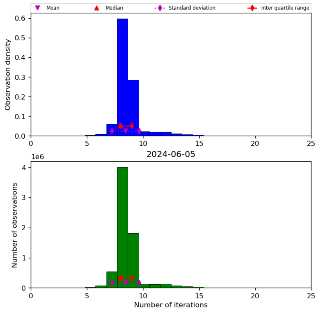
Figure 24: Histogram of "Number of iterations" for 2024-06-04 to 2024-06-06
