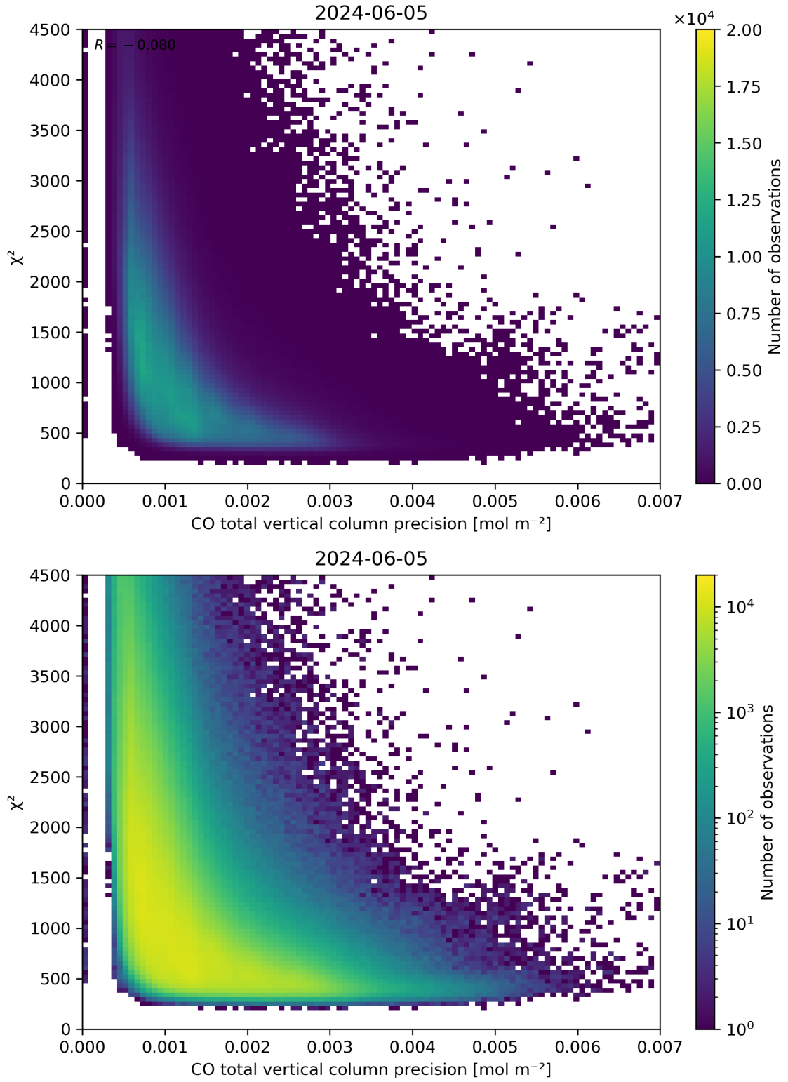
Figure 44: Scatter density plot of “CO total vertical column precision” against “ \chi^2 ” for 2024-06-04 to 2024-06-06.
