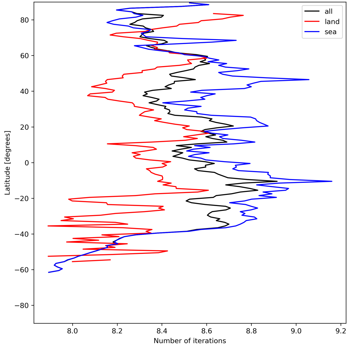
Figure 16: Zonal average of “Number of iterations” for 2024-06-04 to 2024-06-06.
