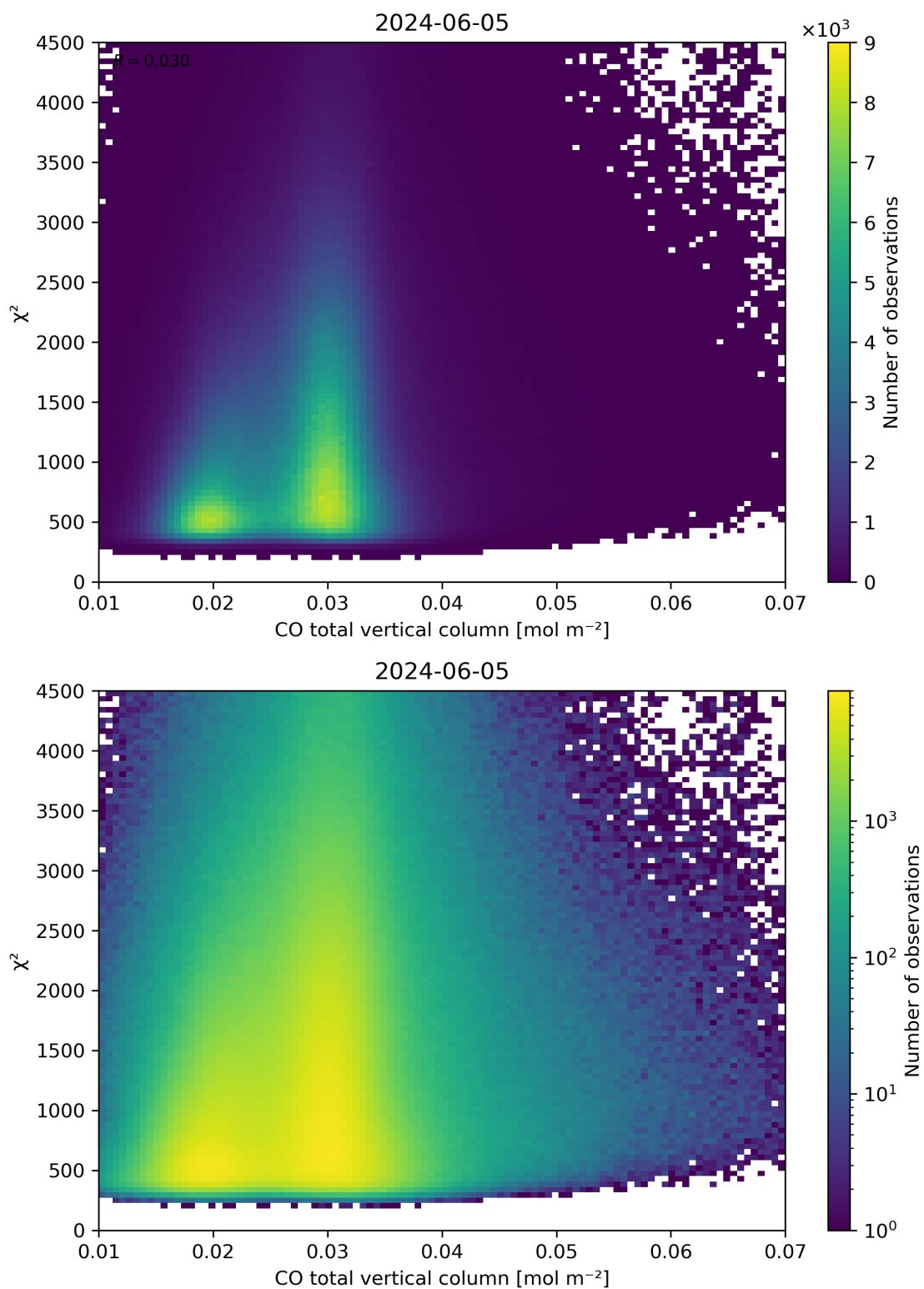
Figure 35: Scatter density plot of “CO total vertical column” against “ \chi^2 ” for 2024-06-04 to 2024-06-06.
