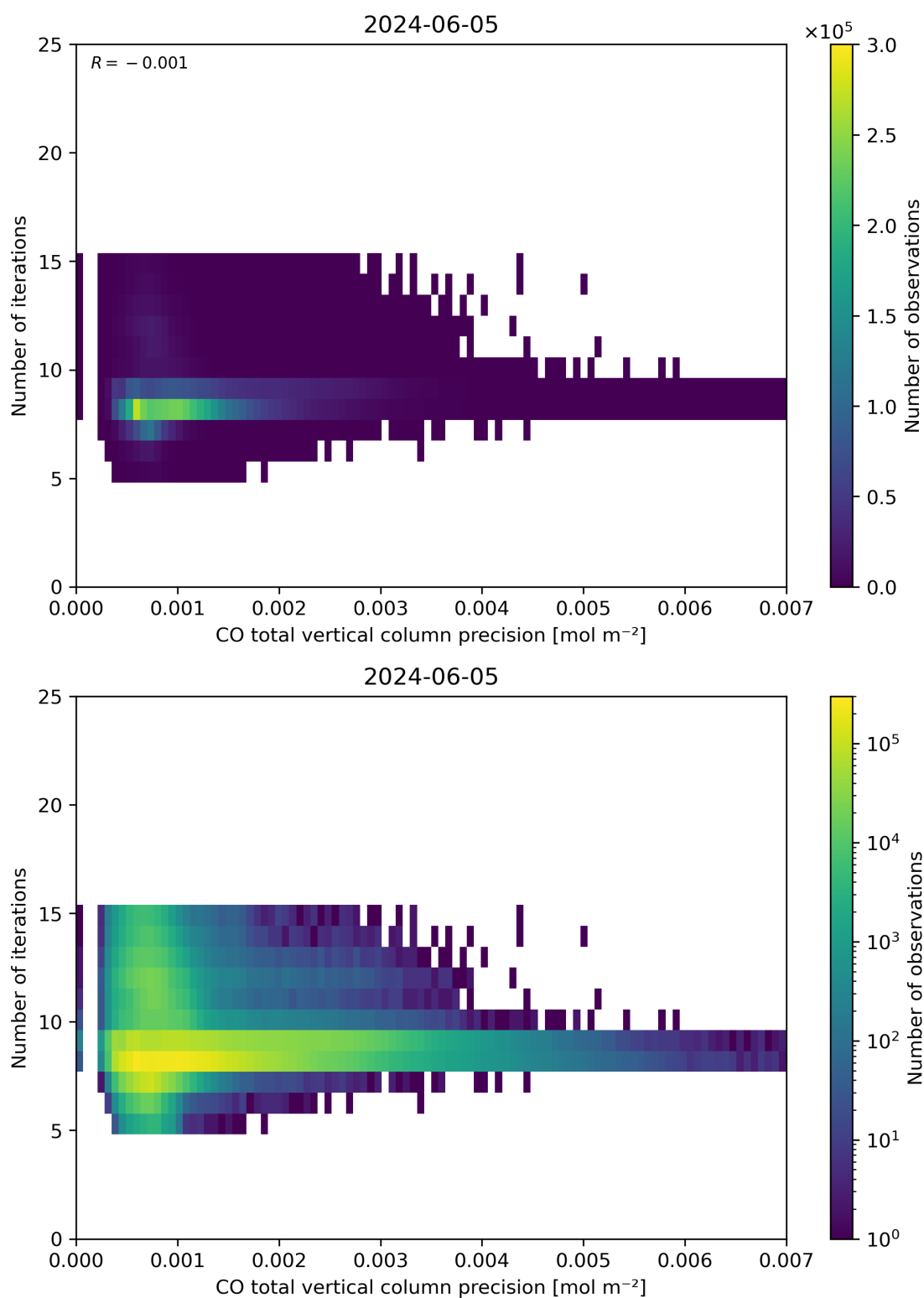
Figure 46: Scatter density plot of “CO total vertical column precision” against “Number of iterations” for 2024-06-04 to 2024-06-06.
