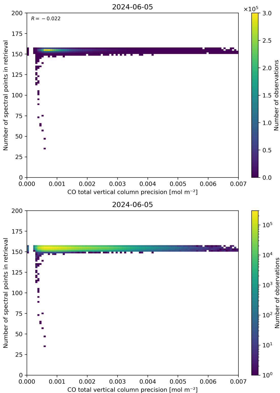
Figure 47: Scatter density plot of “CO total vertical column precision” against “Number of spectral points in retrieval” for 2024-06-04 to 2024-06-06.
