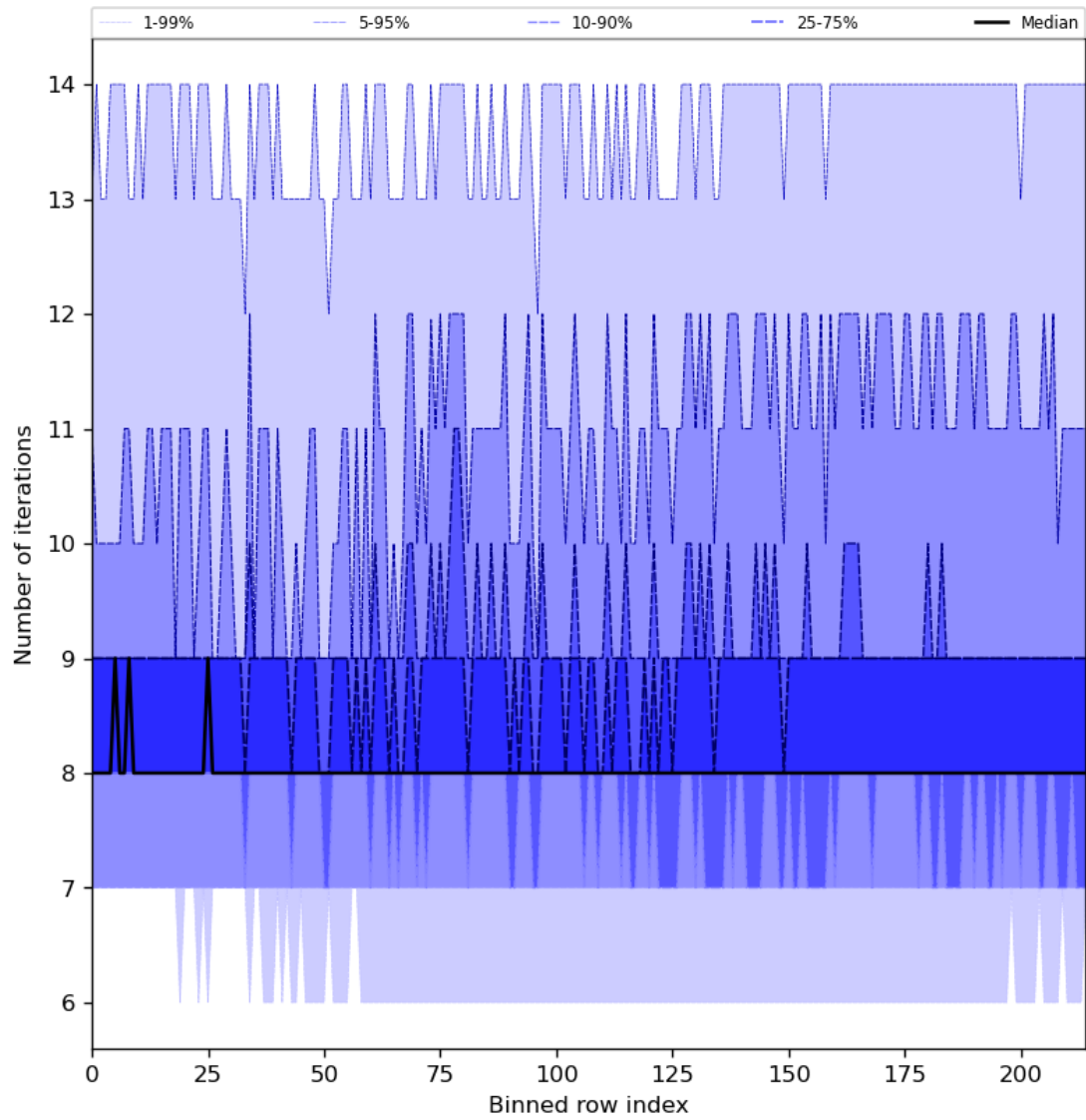
Figure 32: Along track statistics of “Number of iterations” for 2024-06-04 to 2024-06-06
