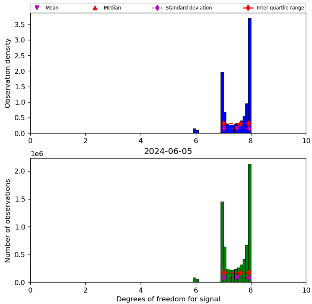
Figure 23: Histogram of “Degrees of freedom for signal” for 2024-06-04 to 2024-06-06
