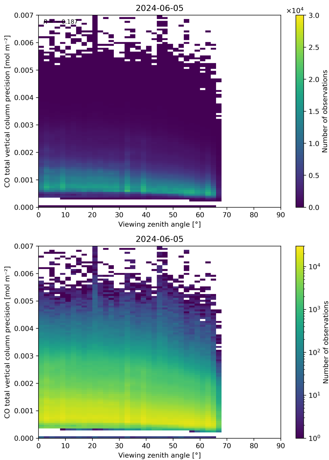
Figure 71: Scatter density plot of “Viewing zenith angle” against “CO total vertical column precision” for 2024-06-04 to 2024-06-06.
