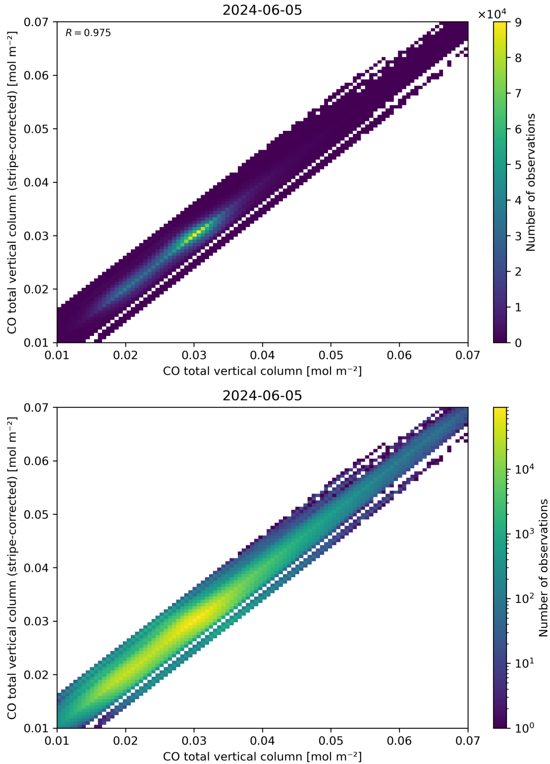
Figure 33: Scatter density plot of “CO total vertical column” against “CO total vertical column (stripe-corrected)” for 2024-06-04 to 2024-06-06.
