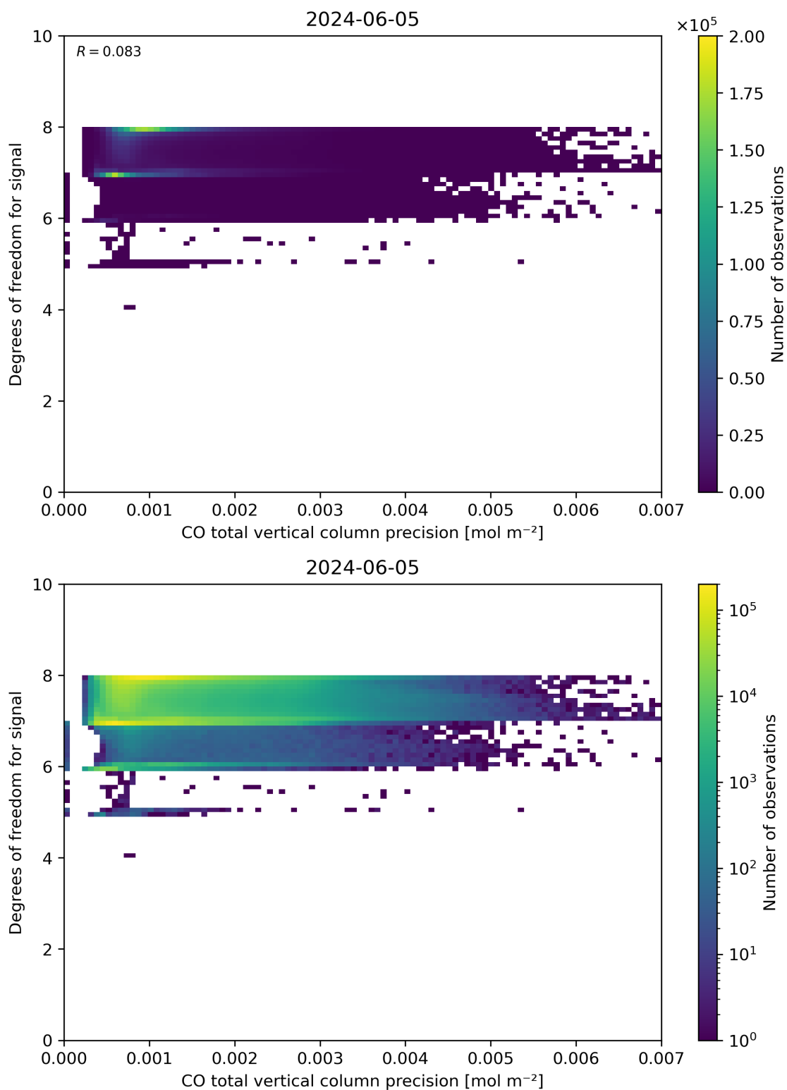
Figure 45: Scatter density plot of “CO total vertical column precision” against “Degrees of freedom for signal” for 2024-06-04 to 2024-06-06.
