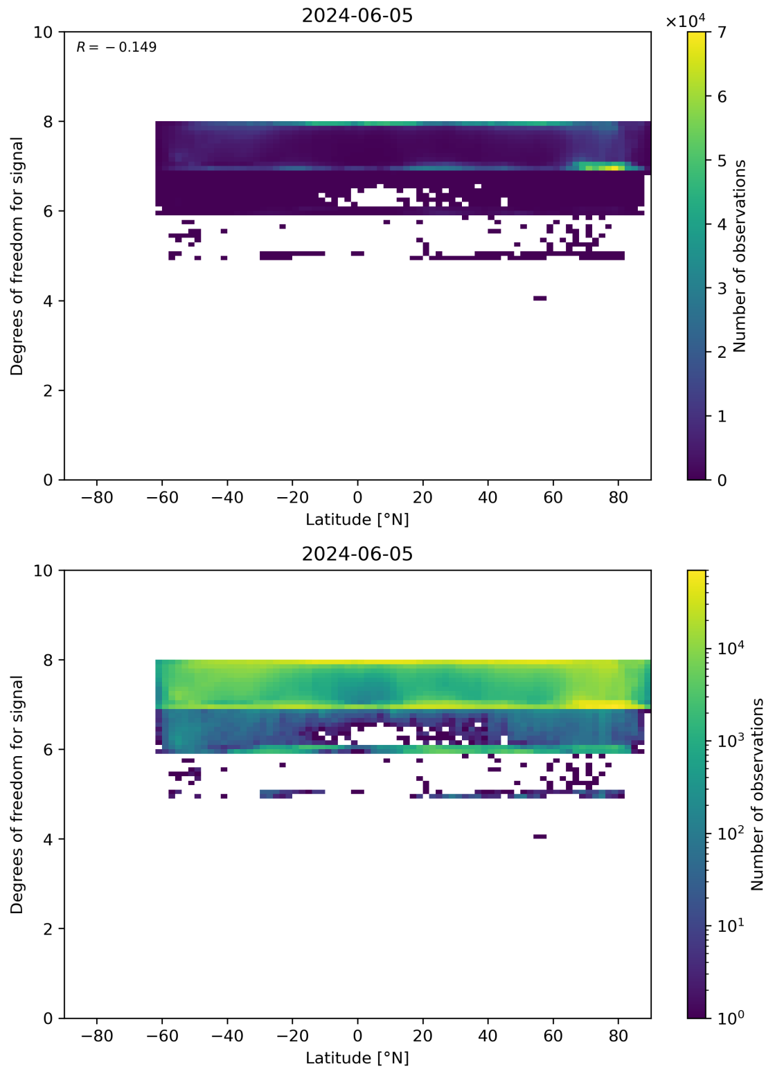
Figure 55: Scatter density plot of “Latitude” against “Degrees of freedom for signal” for 2024-06-04 to 2024-06-06.
