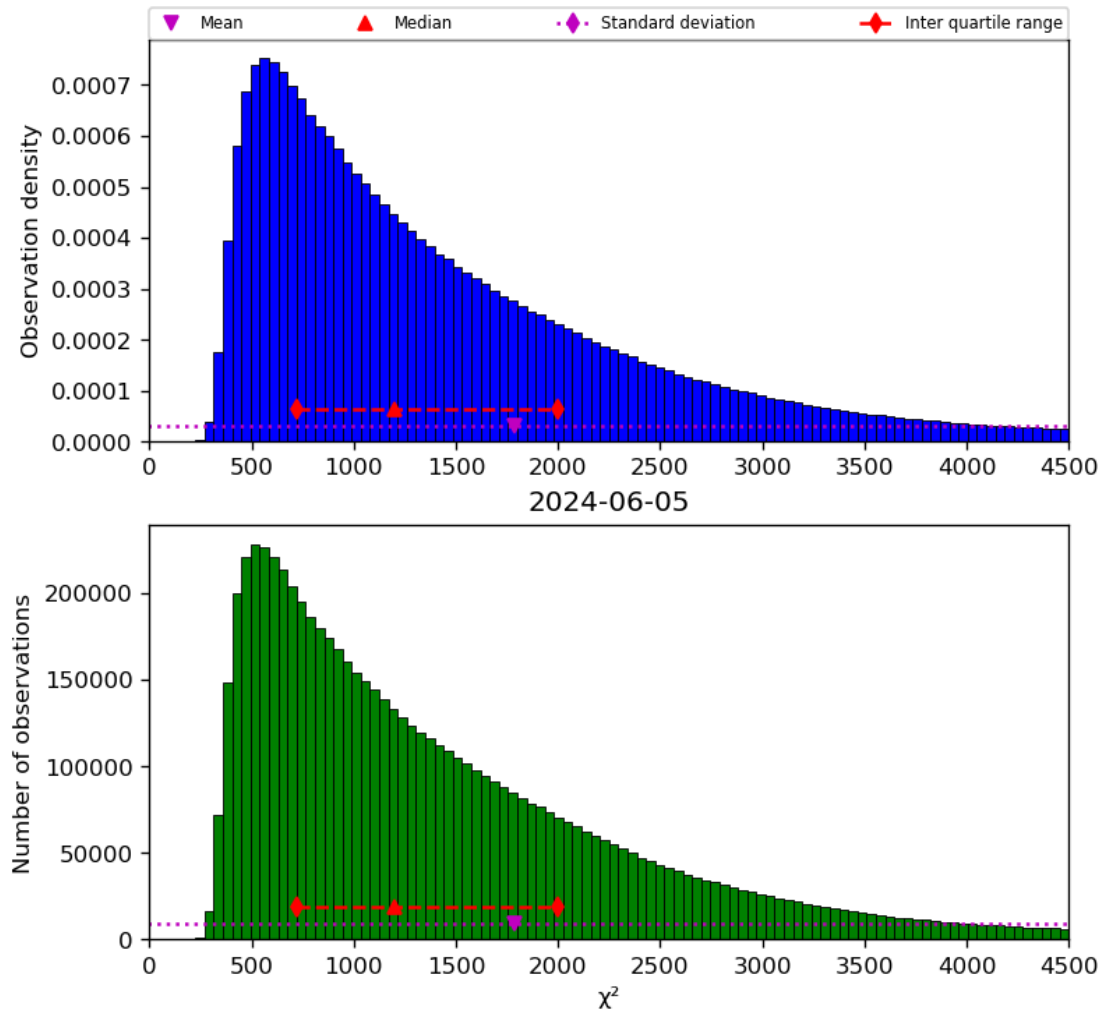
Figure 22: Histogram of “ \chi^2 ” for 2024-06-04 to 2024-06-06
