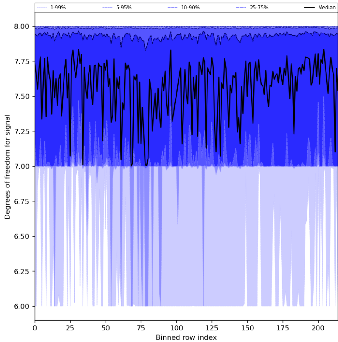
Figure 31: Along track statistics of “Degrees of freedom for signal” for 2024-06-04 to 2024-06-06
