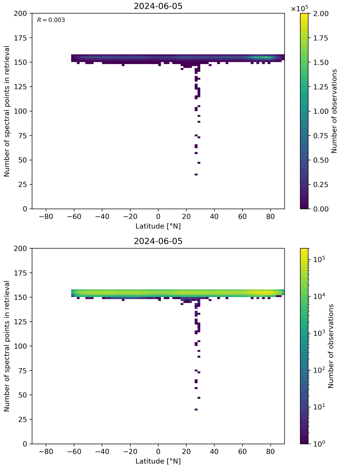
Figure 57: Scatter density plot of “Latitude” against “Number of spectral points in retrieval” for 2024-06-04 to 2024-06-06.
