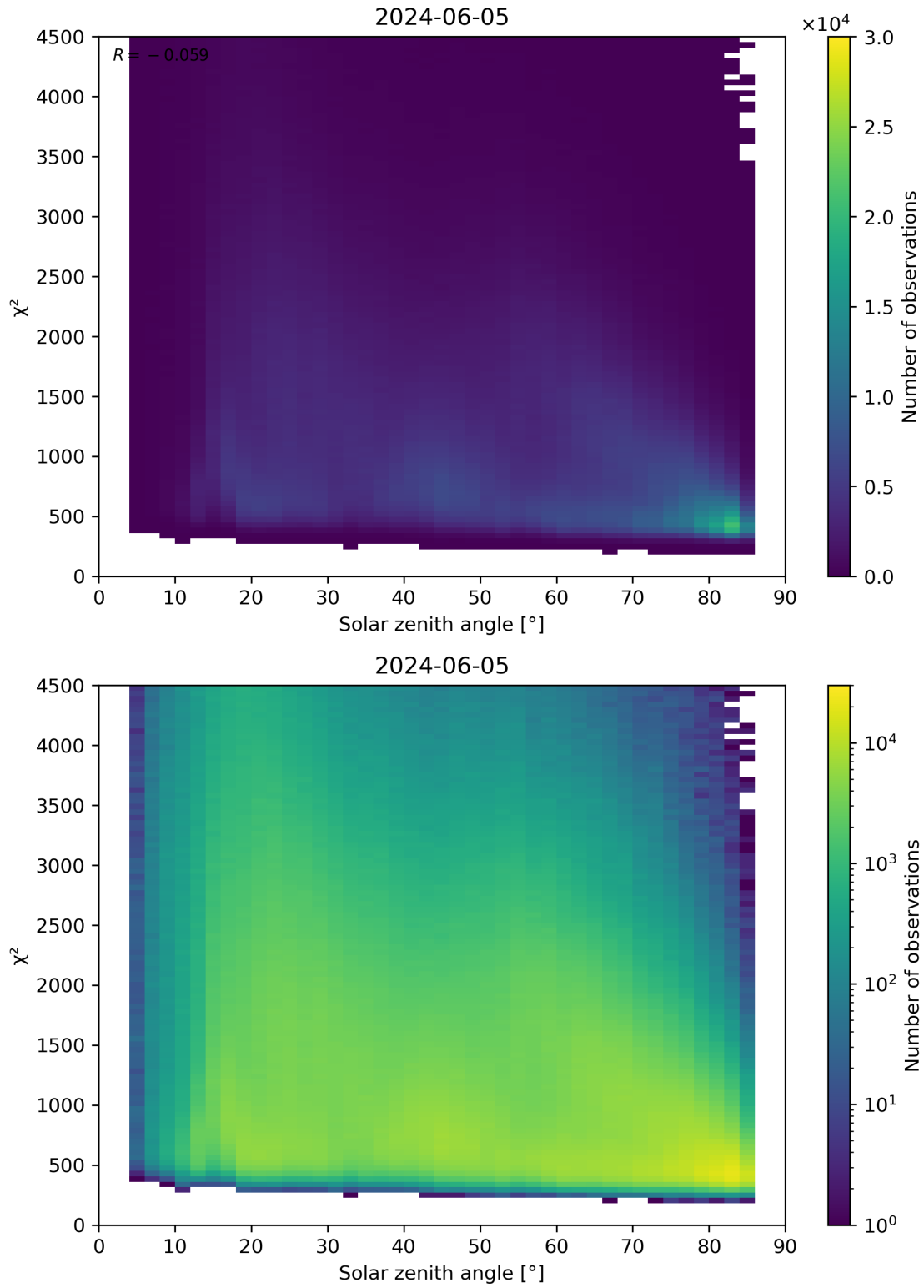
Figure 64: Scatter density plot of “Solar zenith angle” against “ \chi^2 ” for 2024-06-04 to 2024-06-06.
