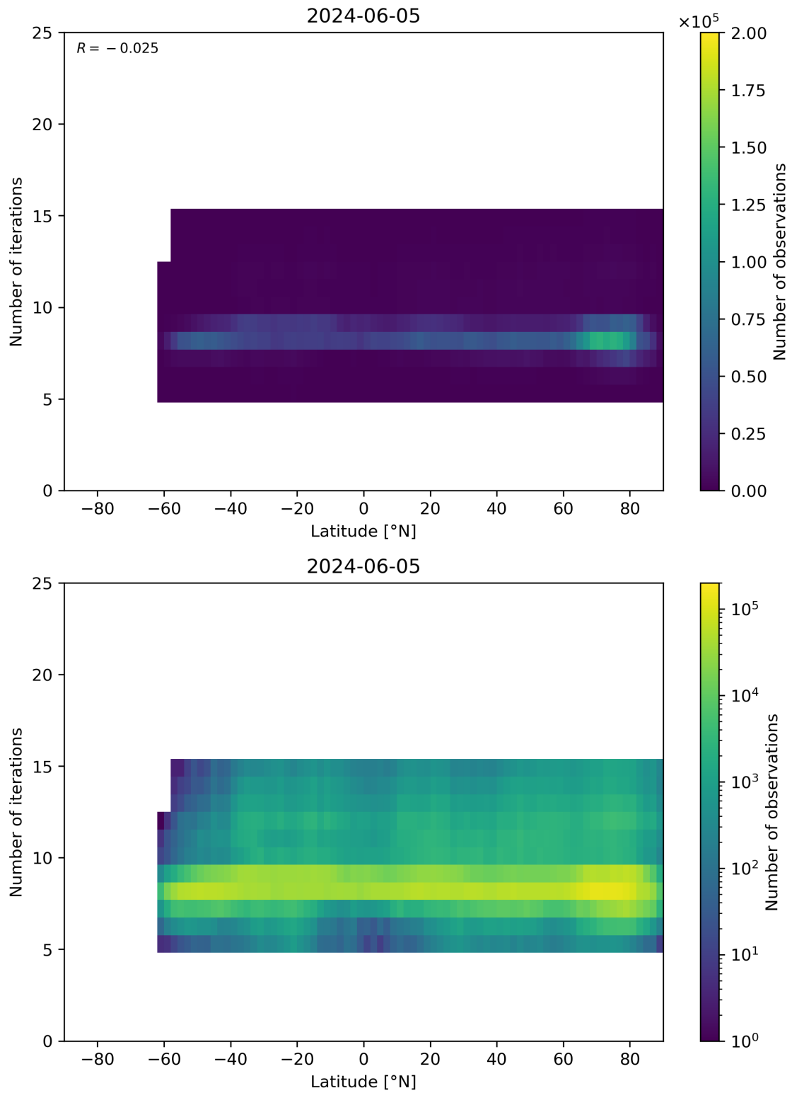
Figure 56: Scatter density plot of “Latitude” against “Number of iterations” for 2024-06-04 to 2024-06-06.
