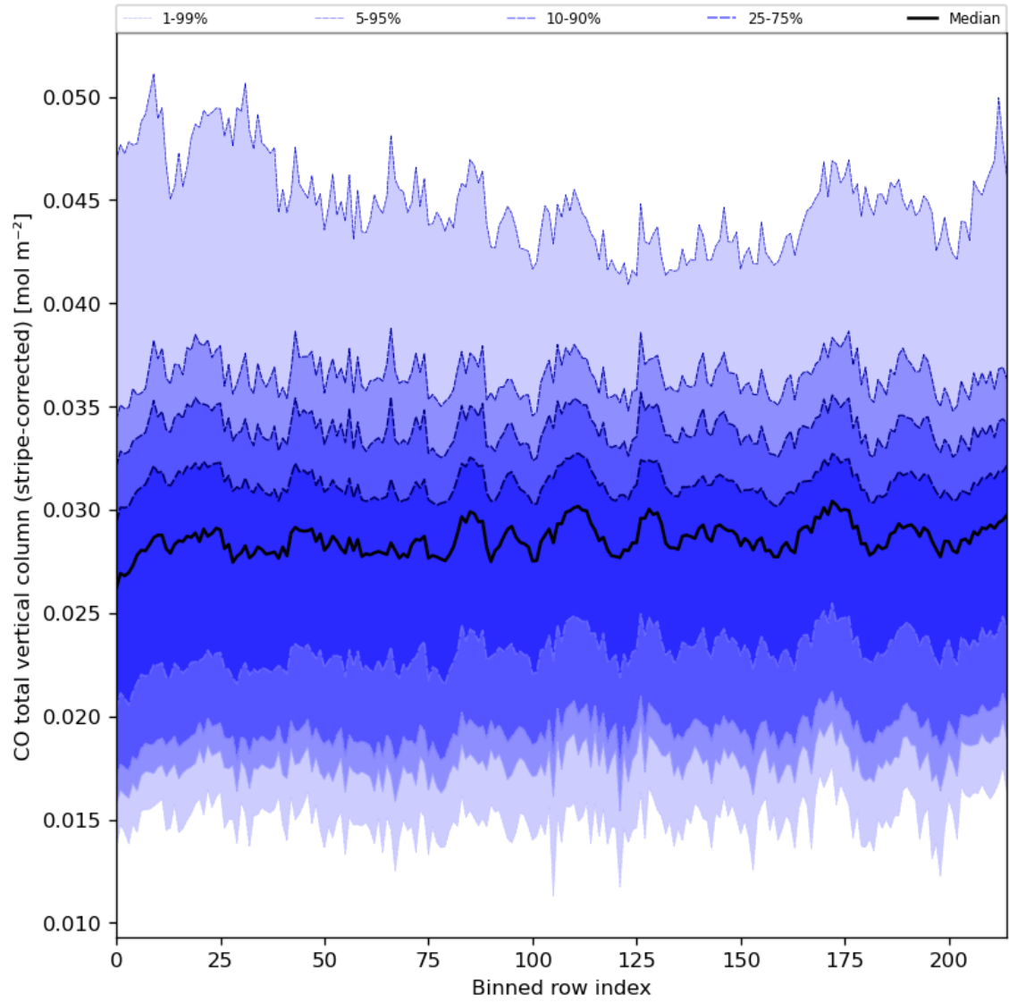
Figure 27: Along track statistics of “CO total vertical column (stripe-corrected)” for 2024-06-04 to 2024-06-06
