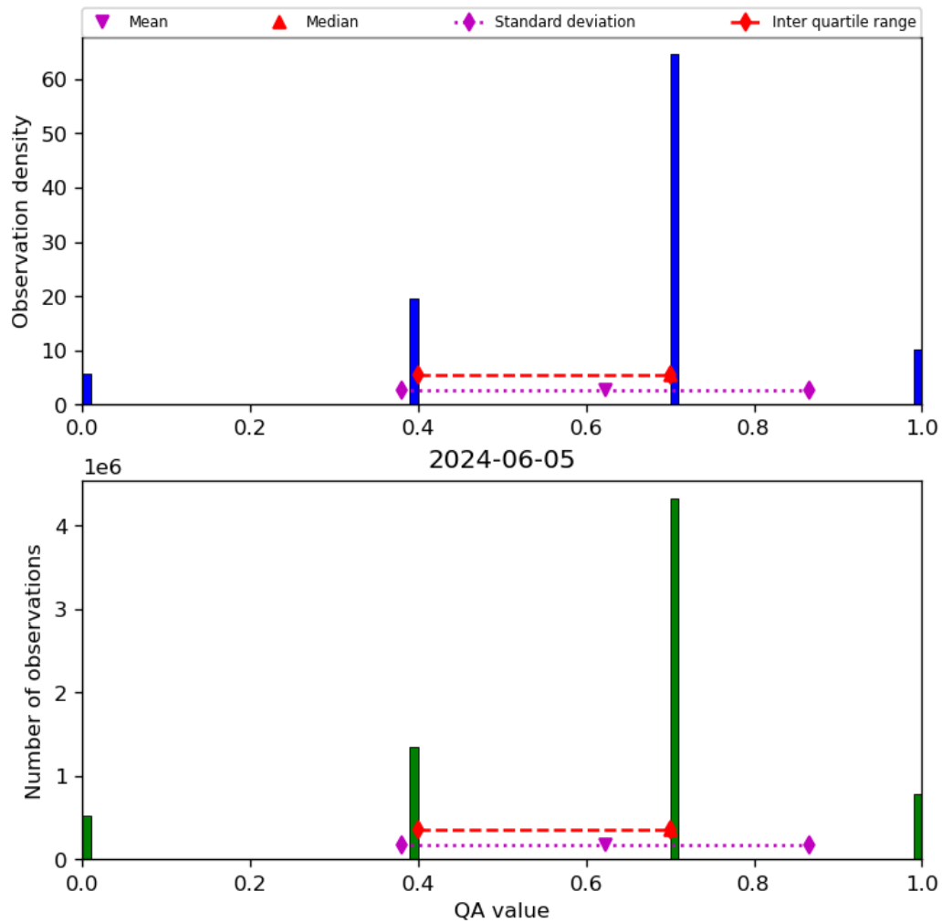
Figure 17: Histogram of “QA value” for 2024-06-04 to 2024-06-06
