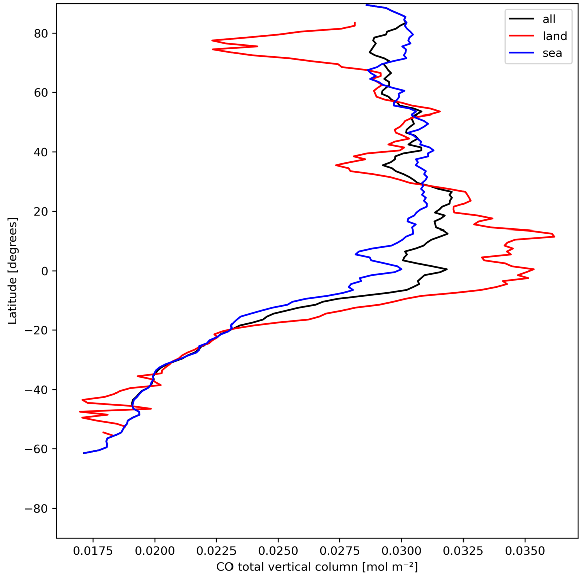
Figure 10: Zonal average of “CO total vertical column” for 2024-06-04 to 2024-06-06.
