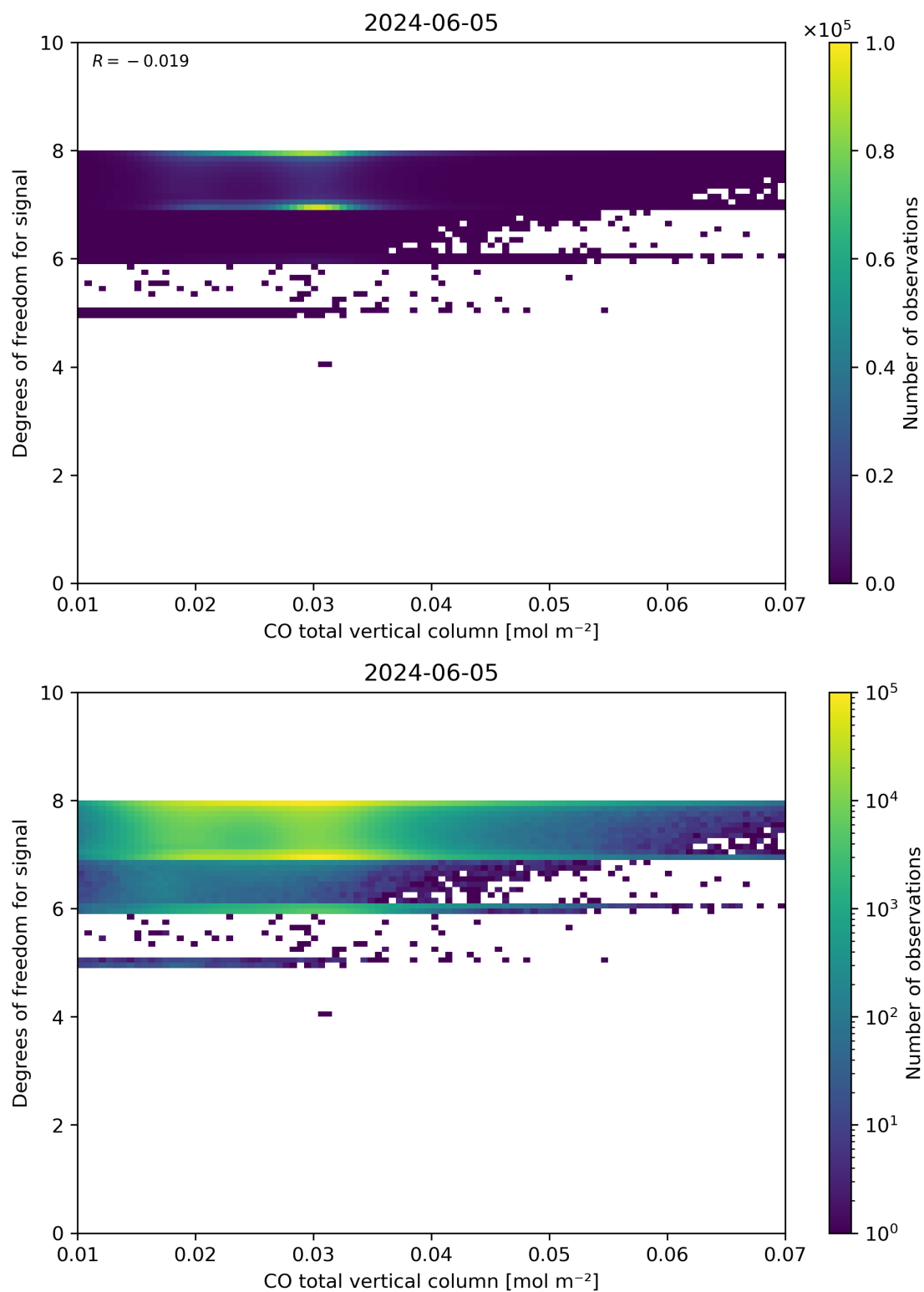
Figure 41: Scatter density plot of “CO total vertical column” against “Degrees of freedom for signal” for 2024-06-04 to 2024-06-06.
