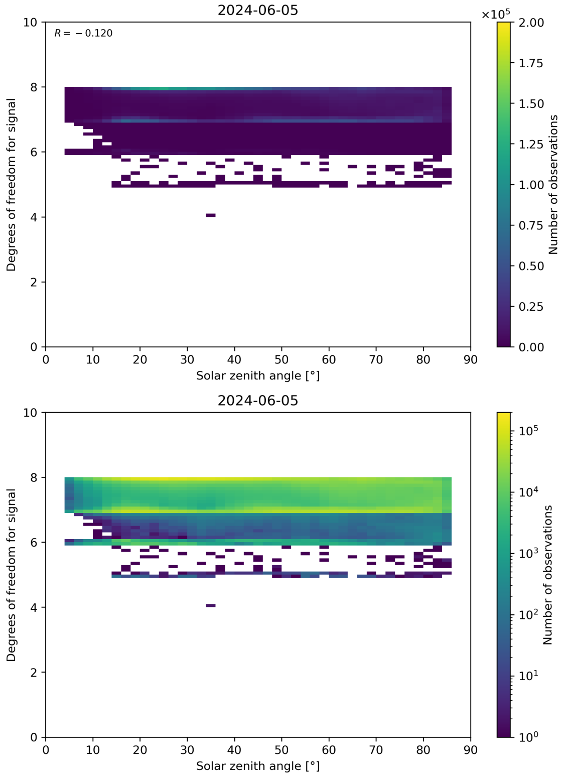
Figure 65: Scatter density plot of “Solar zenith angle” against “Degrees of freedom for signal” for 2024-06-04 to 2024-06-06.
