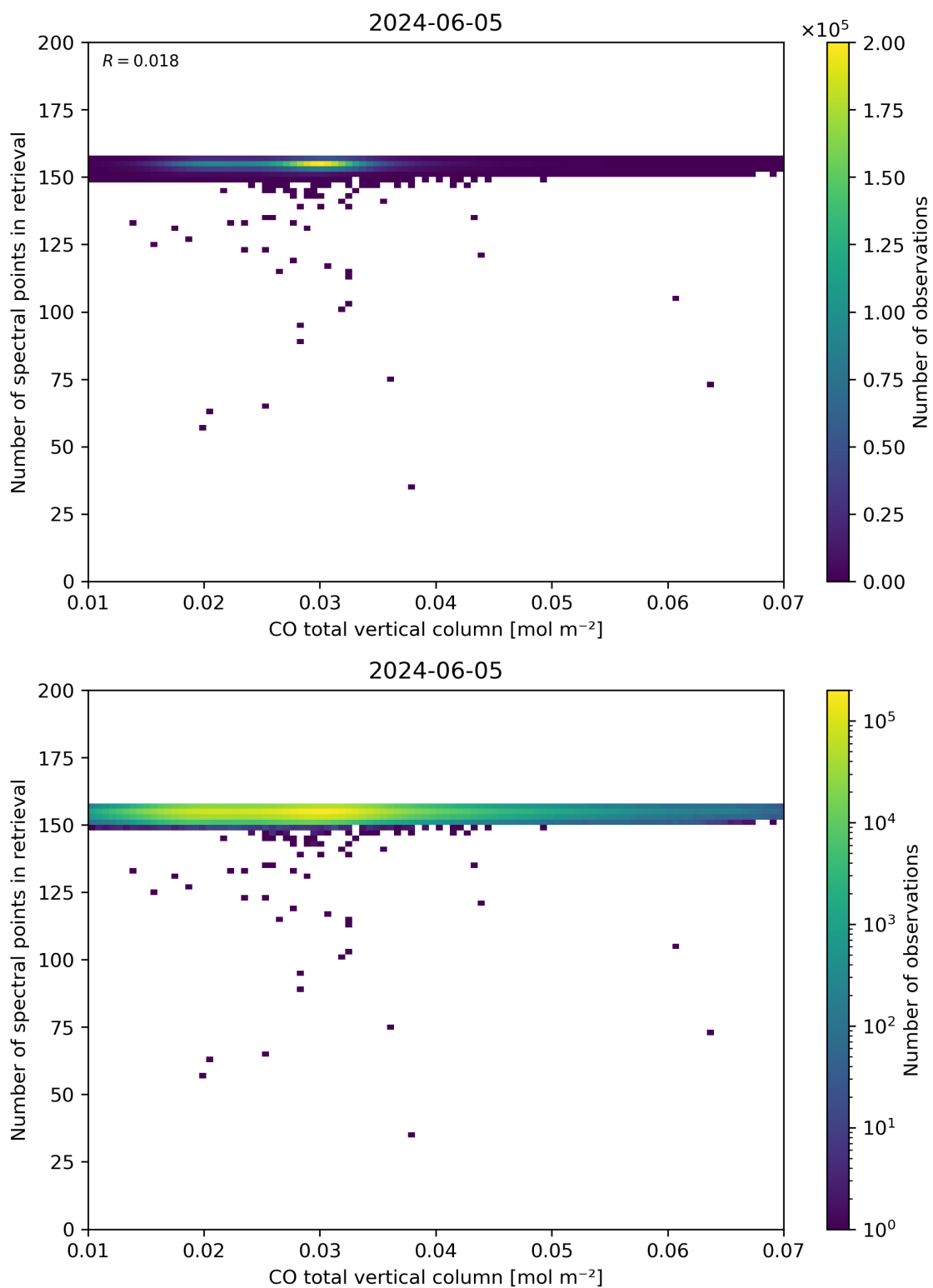
Figure 43: Scatter density plot of “CO total vertical column” against “Number of spectral points in retrieval” for 2024-06-04 to 2024-06-06.
