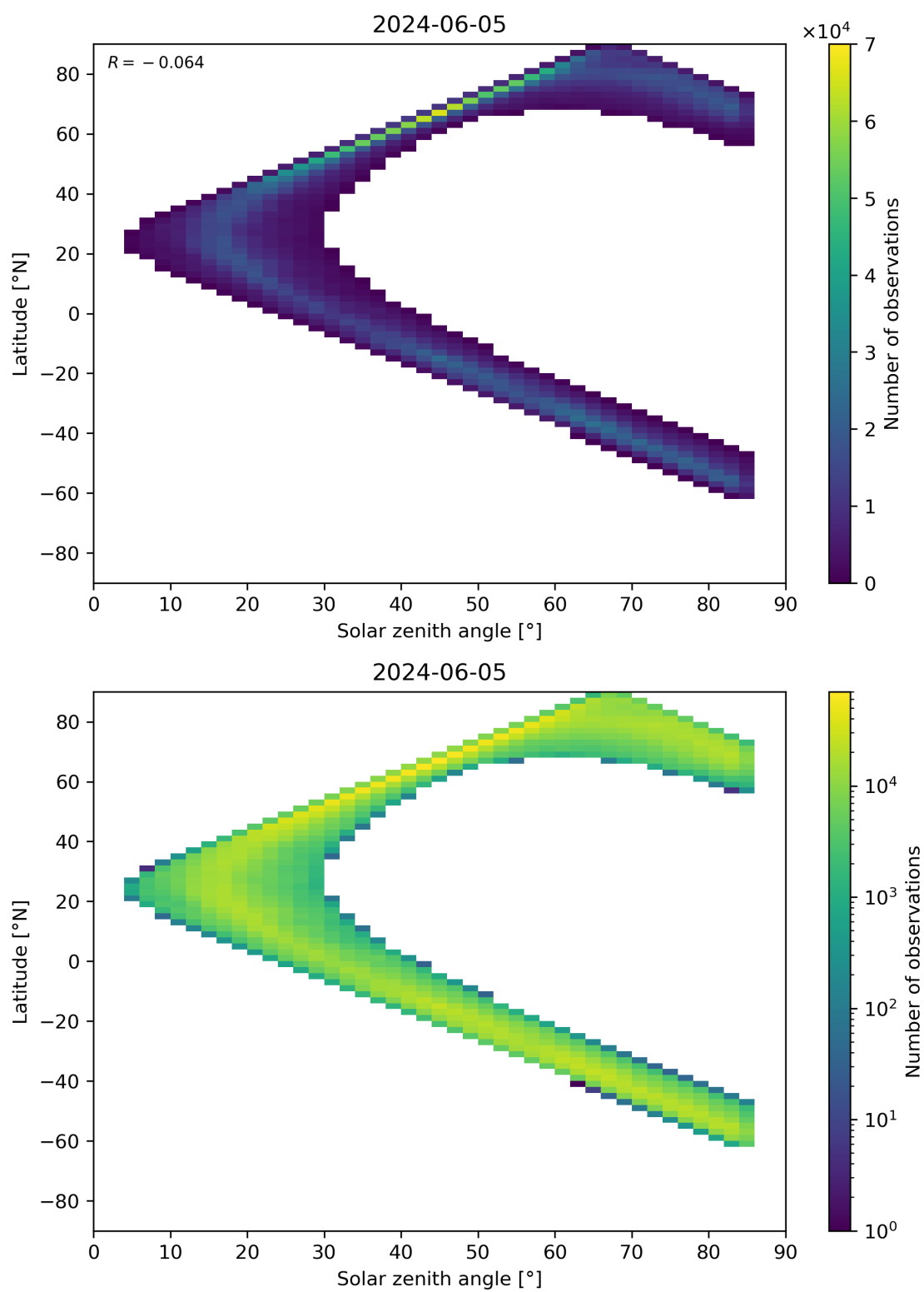
Figure 66: Scatter density plot of “Solar zenith angle” against “Latitude” for 2024-06-04 to 2024-06-06.
