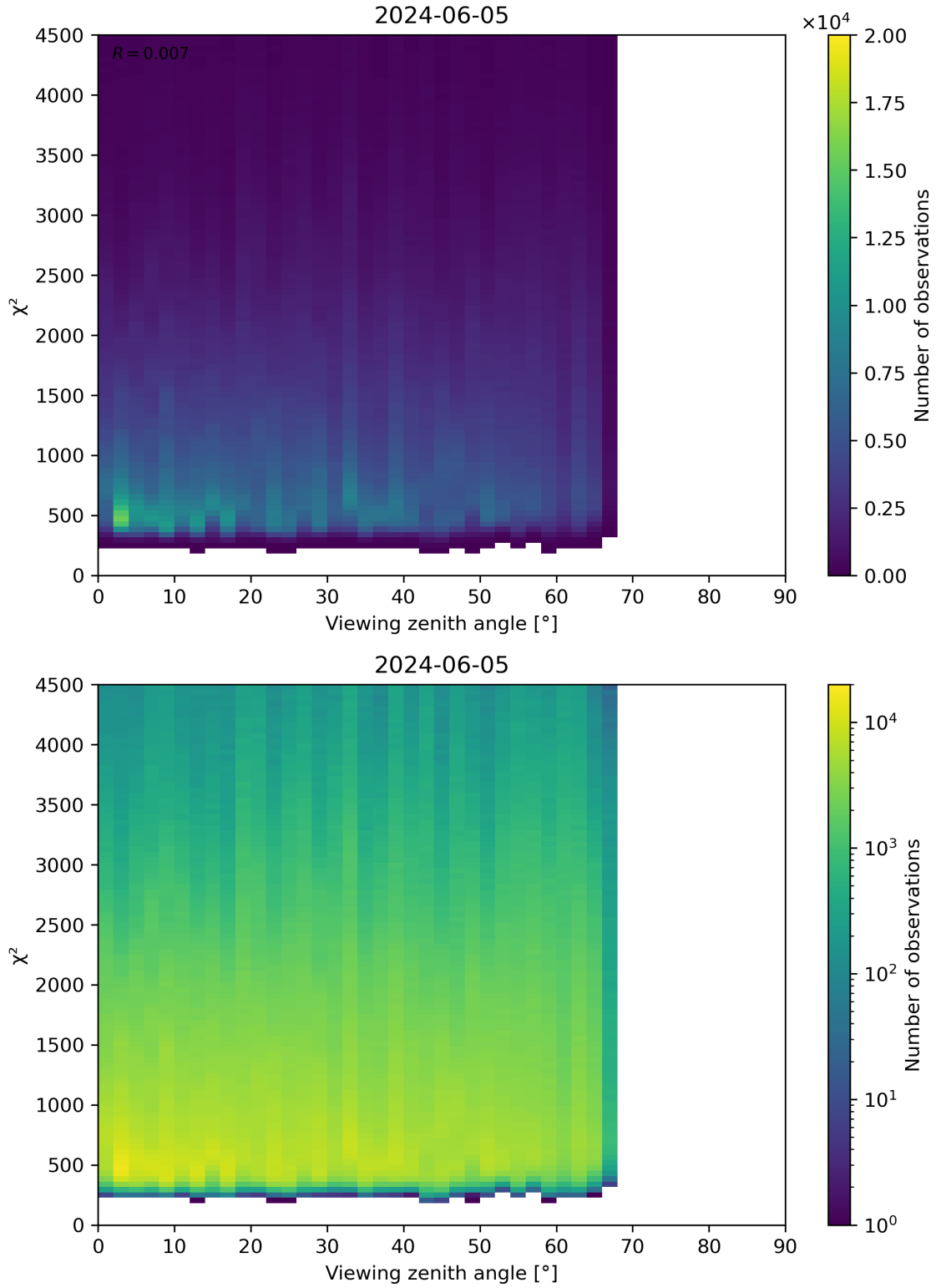
Figure 72: Scatter density plot of “Viewing zenith angle” against “ \chi^2 ” for 2024-06-04 to 2024-06-06.
