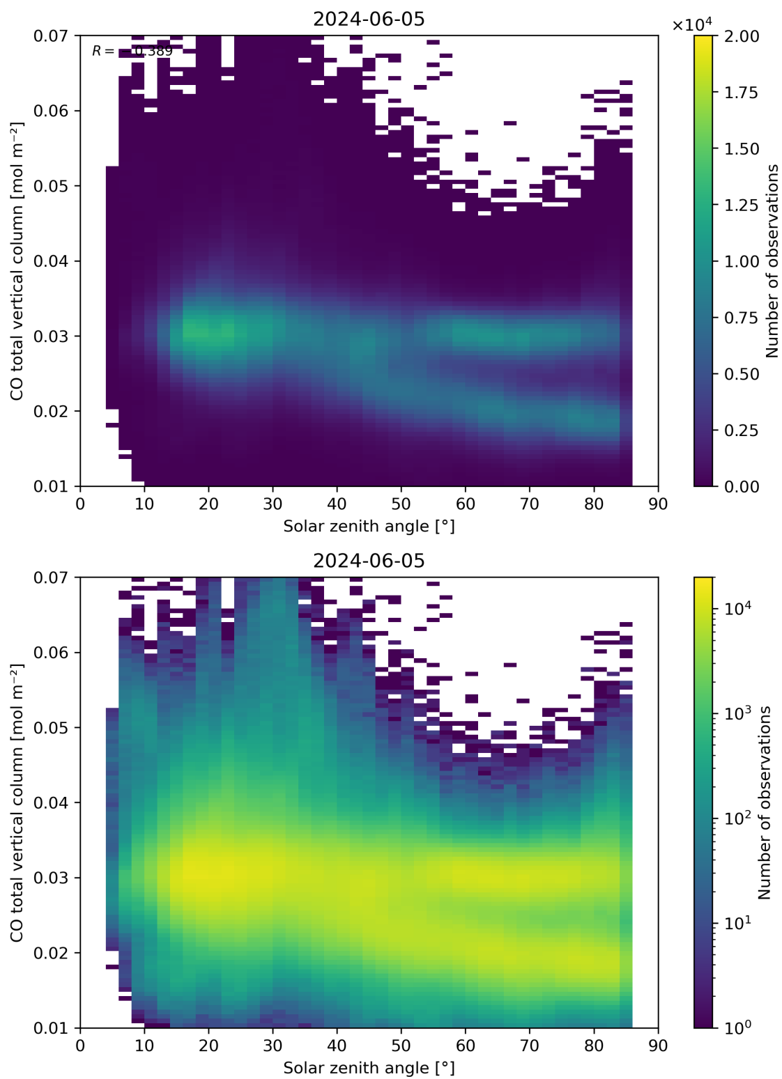
Figure 61: Scatter density plot of “Solar zenith angle” against “CO total vertical column” for 2024-06-04 to 2024-06-06.
