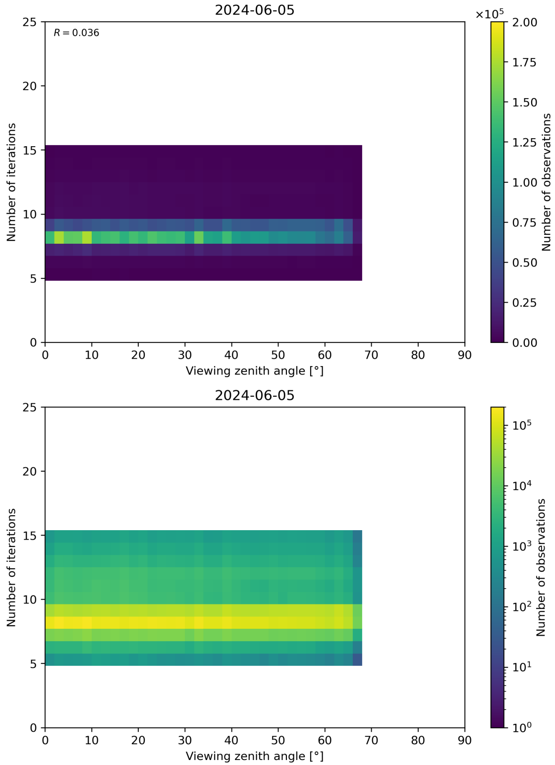
Figure 75: Scatter density plot of “Viewing zenith angle” against “Number of iterations” for 2024-06-04 to 2024-06-06.
