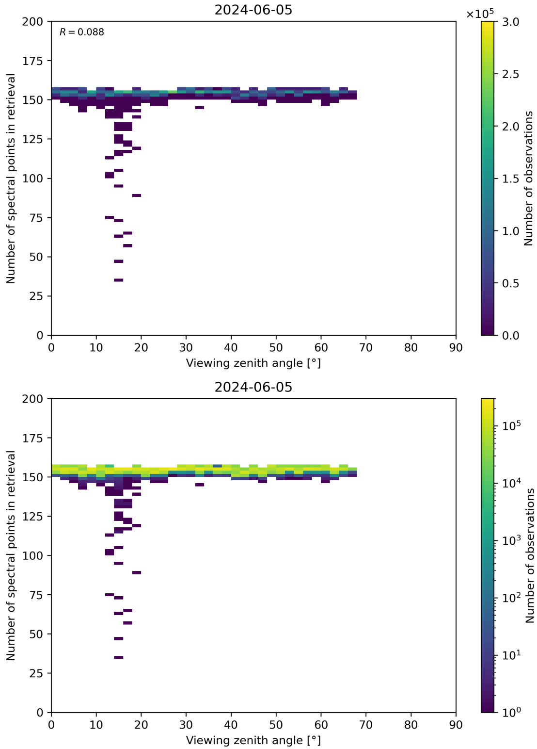
Figure 76: Scatter density plot of “Viewing zenith angle” against “Number of spectral points in retrieval” for 2024-06-04 to 2024-06-06.
