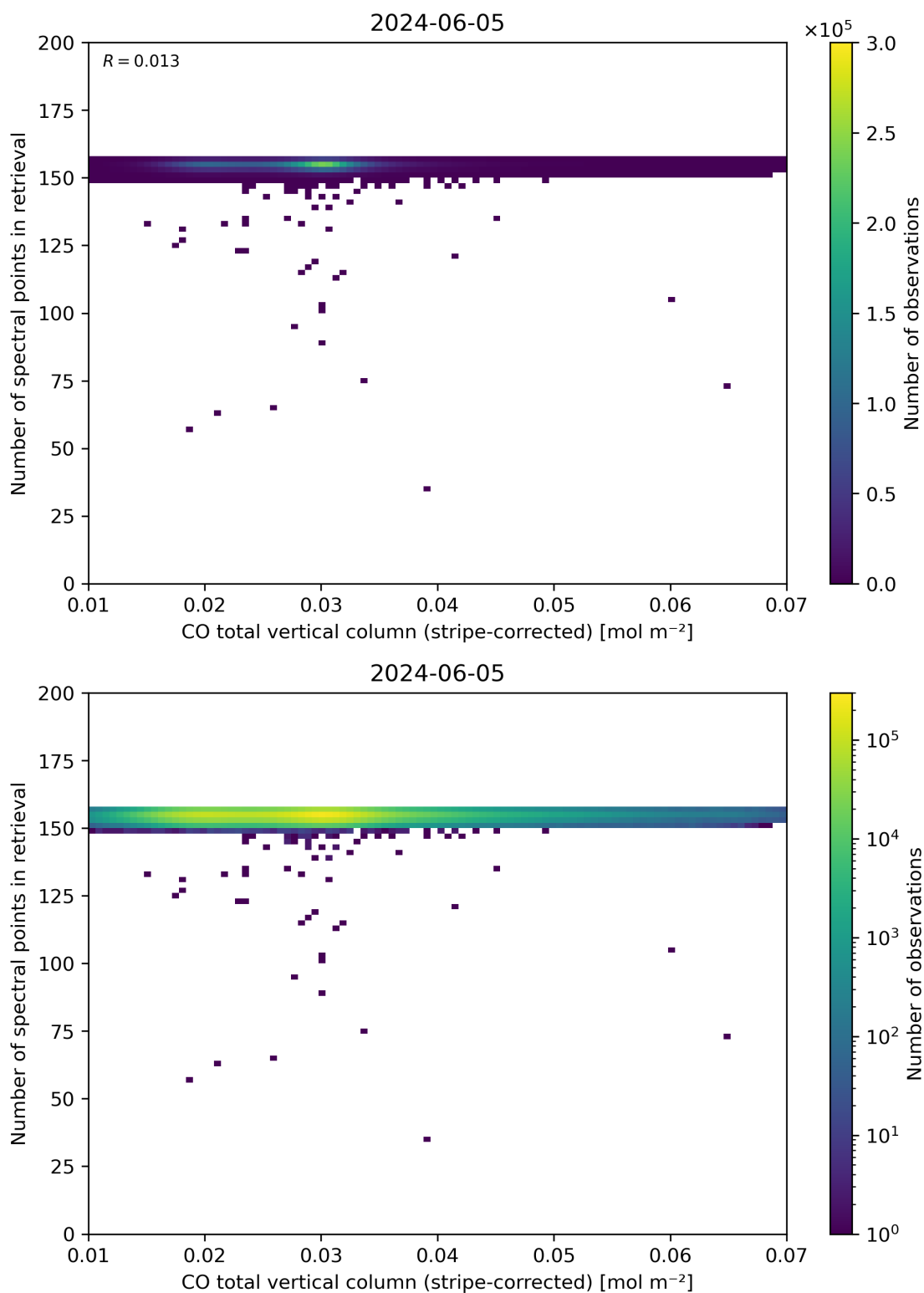
Figure 40: Scatter density plot of “CO total vertical column (stripe-corrected)” against “Number of spectral points in retrieval” for 2024-06-04 to 2024-06-06.
