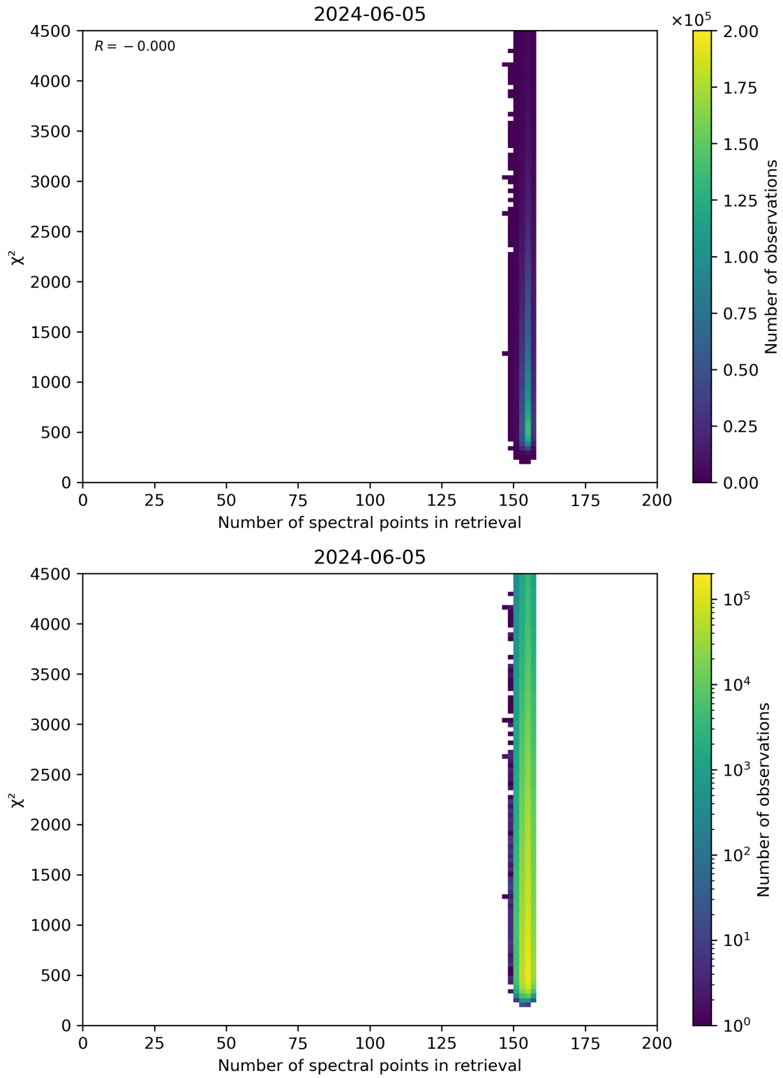
Figure 58: Scatter density plot of “Number of spectral points in retrieval” against “ \chi^2 ” for 2024-06-04 to 2024-06-06.
