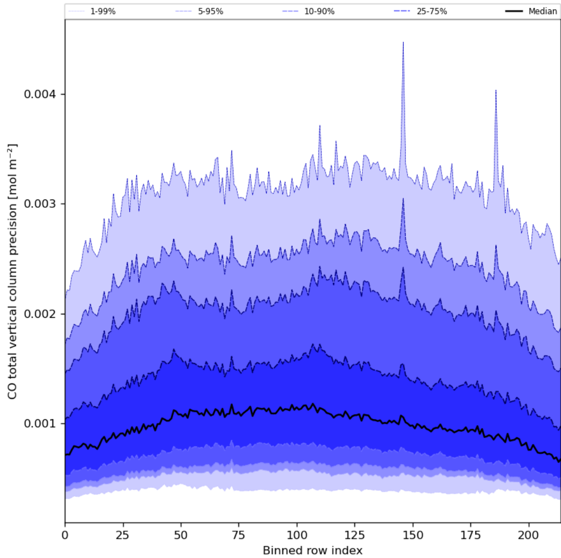
Figure 28: Along track statistics of “CO total vertical column precision” for 2024-06-04 to 2024-06-06
