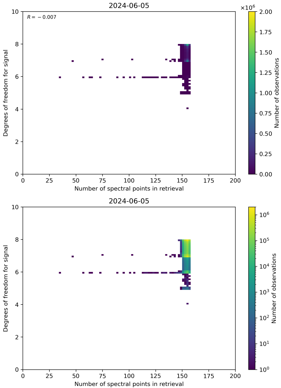
Figure 59: Scatter density plot of “Number of spectral points in retrieval” against “Degrees of freedom for signal” for 2024-06-04 to 2024-06-06.
