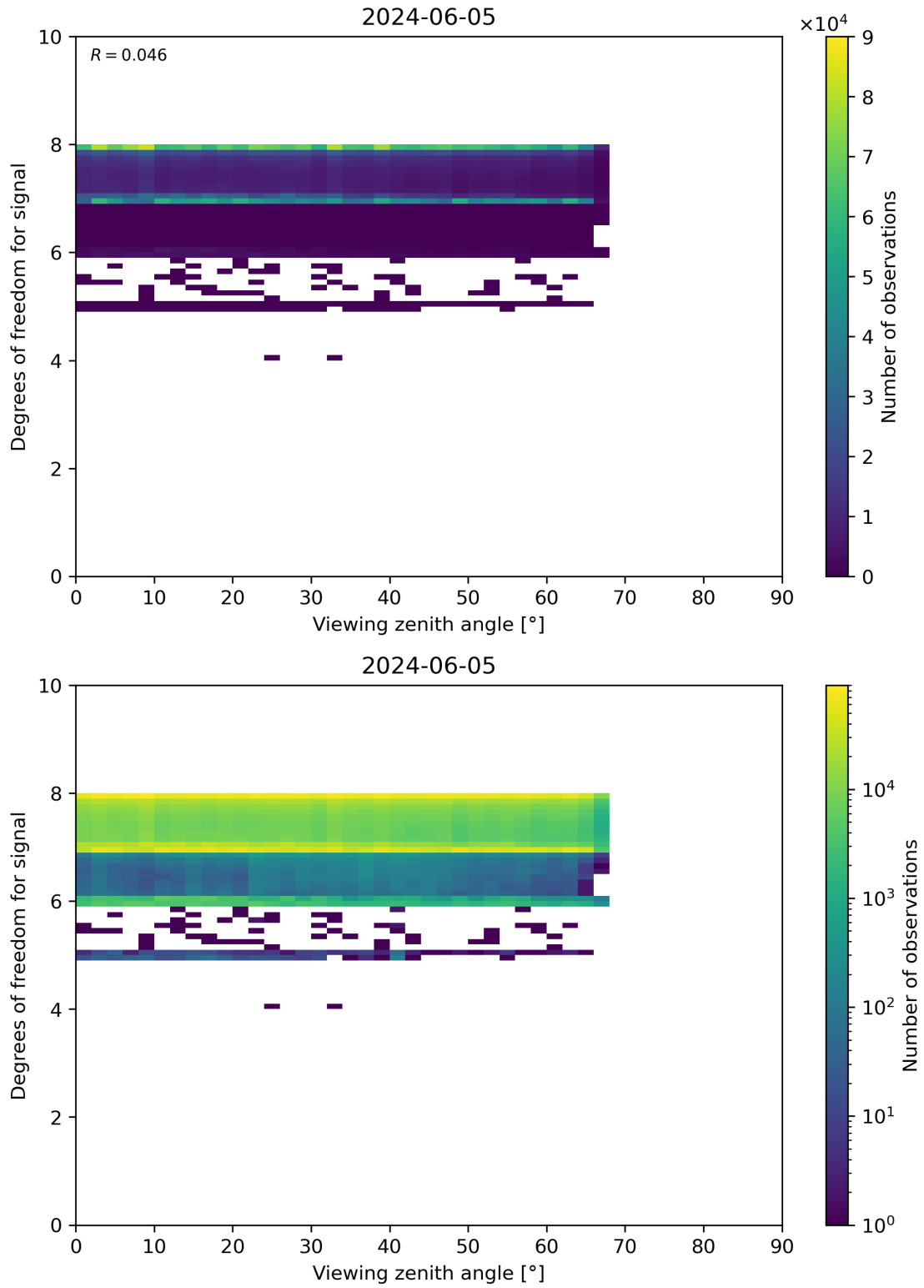
Figure 73: Scatter density plot of “Viewing zenith angle” against “Degrees of freedom for signal” for 2024-06-04 to 2024-06-06.
