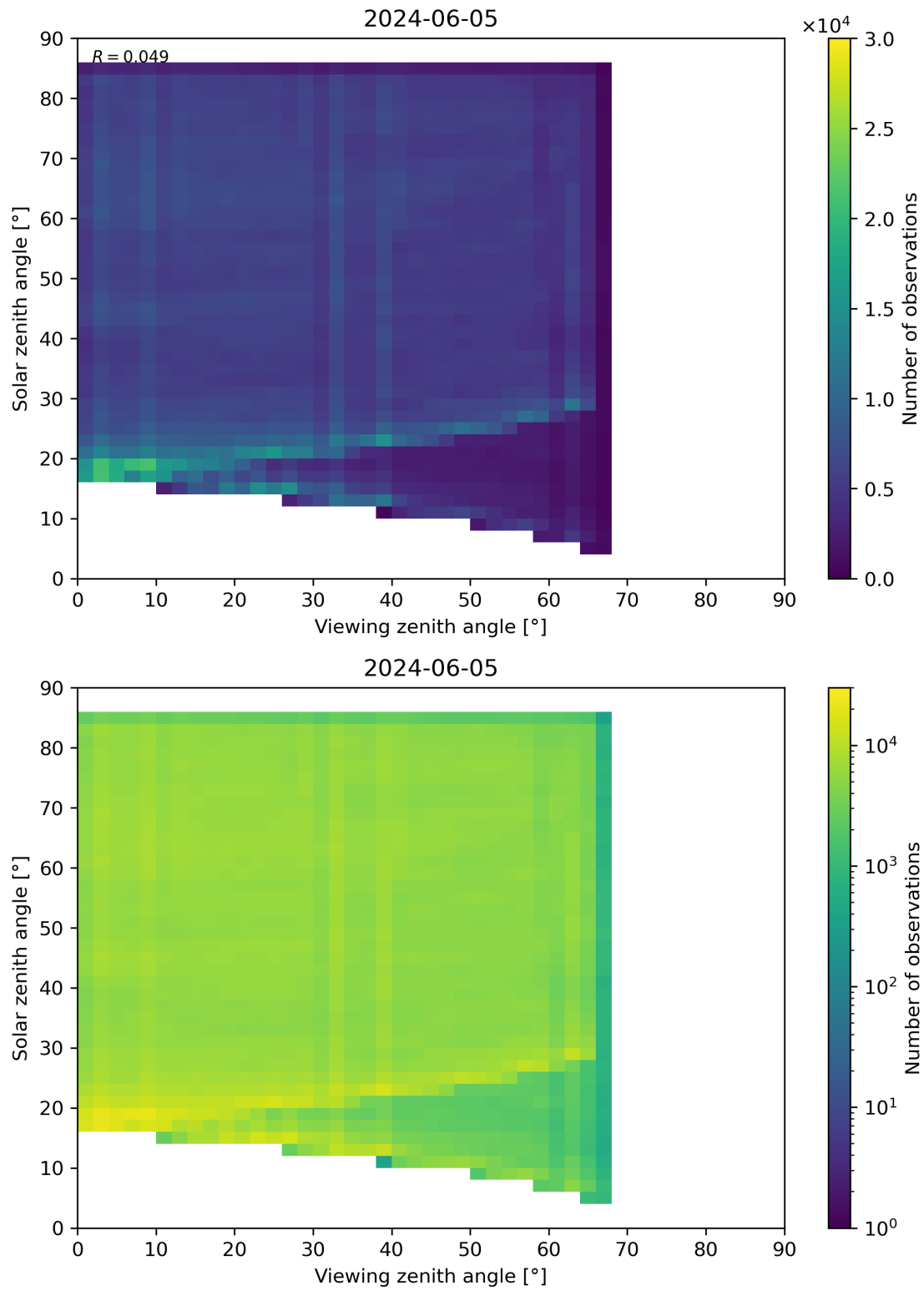
Figure 77: Scatter density plot of “Viewing zenith angle” against “Solar zenith angle” for 2024-06-04 to 2024-06-06.
