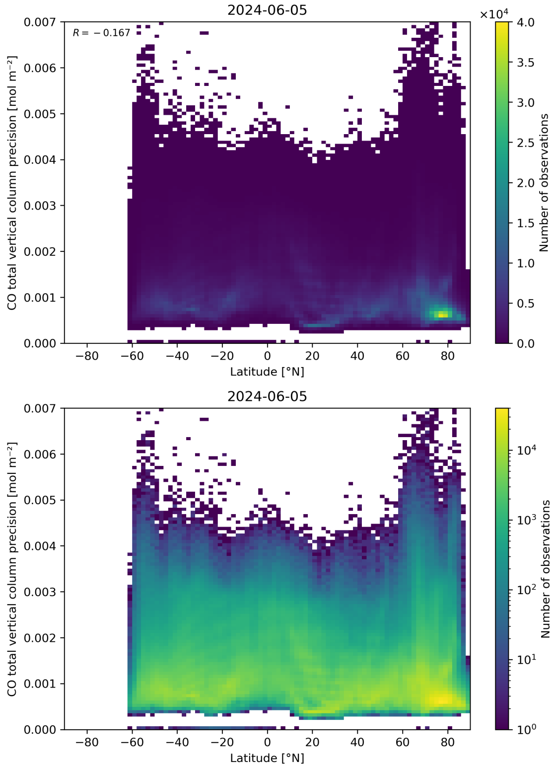
Figure 53: Scatter density plot of “Latitude” against “CO total vertical column precision” for 2024-06-04 to 2024-06-06.
