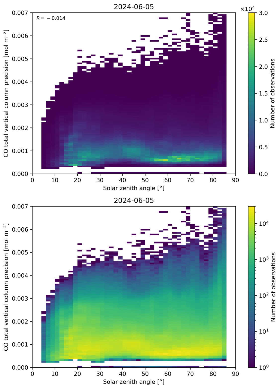
Figure 63: Scatter density plot of “Solar zenith angle” against “CO total vertical column precision” for 2024-06-04 to 2024-06-06.
