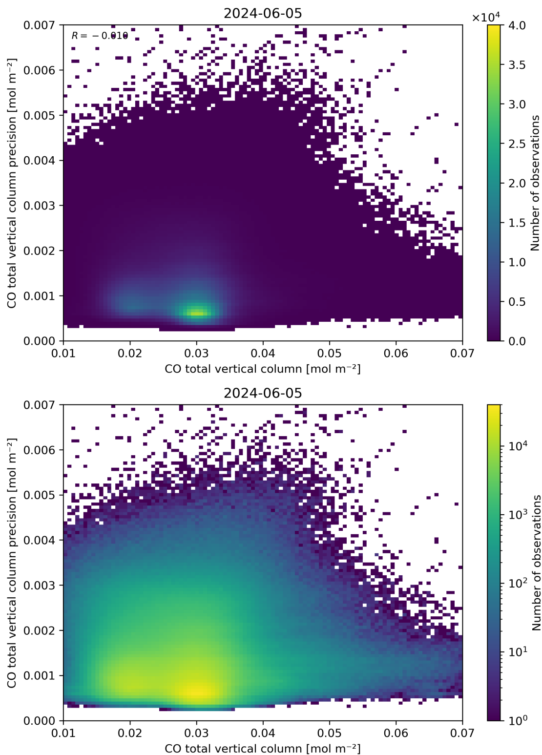
Figure 34: Scatter density plot of “CO total vertical column” against “CO total vertical column precision” for 2024-06-04 to 2024-06-06.
