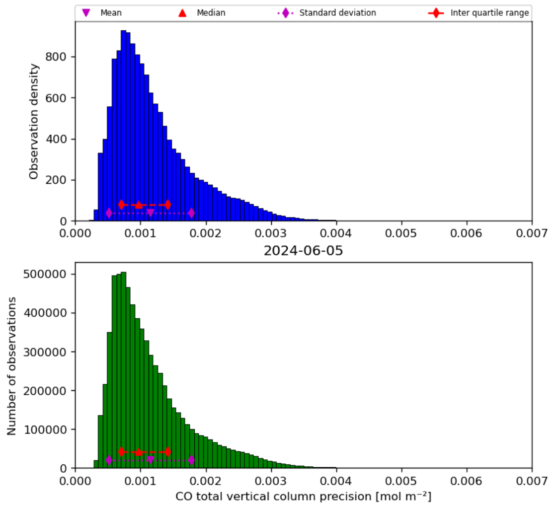
Figure 20: Histogram of “CO total vertical column precision” for 2024-06-04 to 2024-06-06
