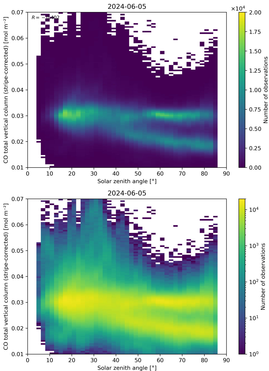
Figure 62: Scatter density plot of “Solar zenith angle” against “CO total vertical column (stripe-corrected)” for 2024-06-04 to 2024-06-06.
