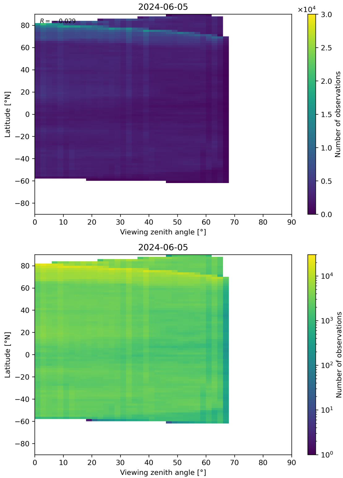
Figure 74: Scatter density plot of “Viewing zenith angle” against “Latitude” for 2024-06-04 to 2024-06-06.
