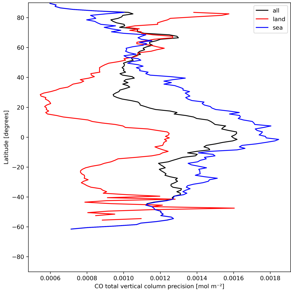
Figure 12: Zonal average of “CO total vertical column precision” for 2024-06-04 to 2024-06-06.
