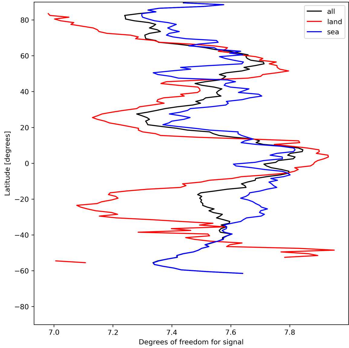
Figure 15: Zonal average of “Degrees of freedom for signal” for 2024-06-04 to 2024-06-06.
