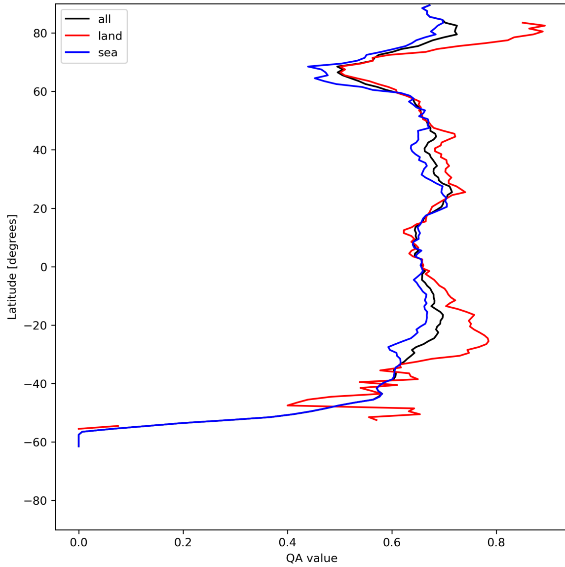
Figure 9: Zonal average of “QA value” for 2024-06-04 to 2024-06-06.
