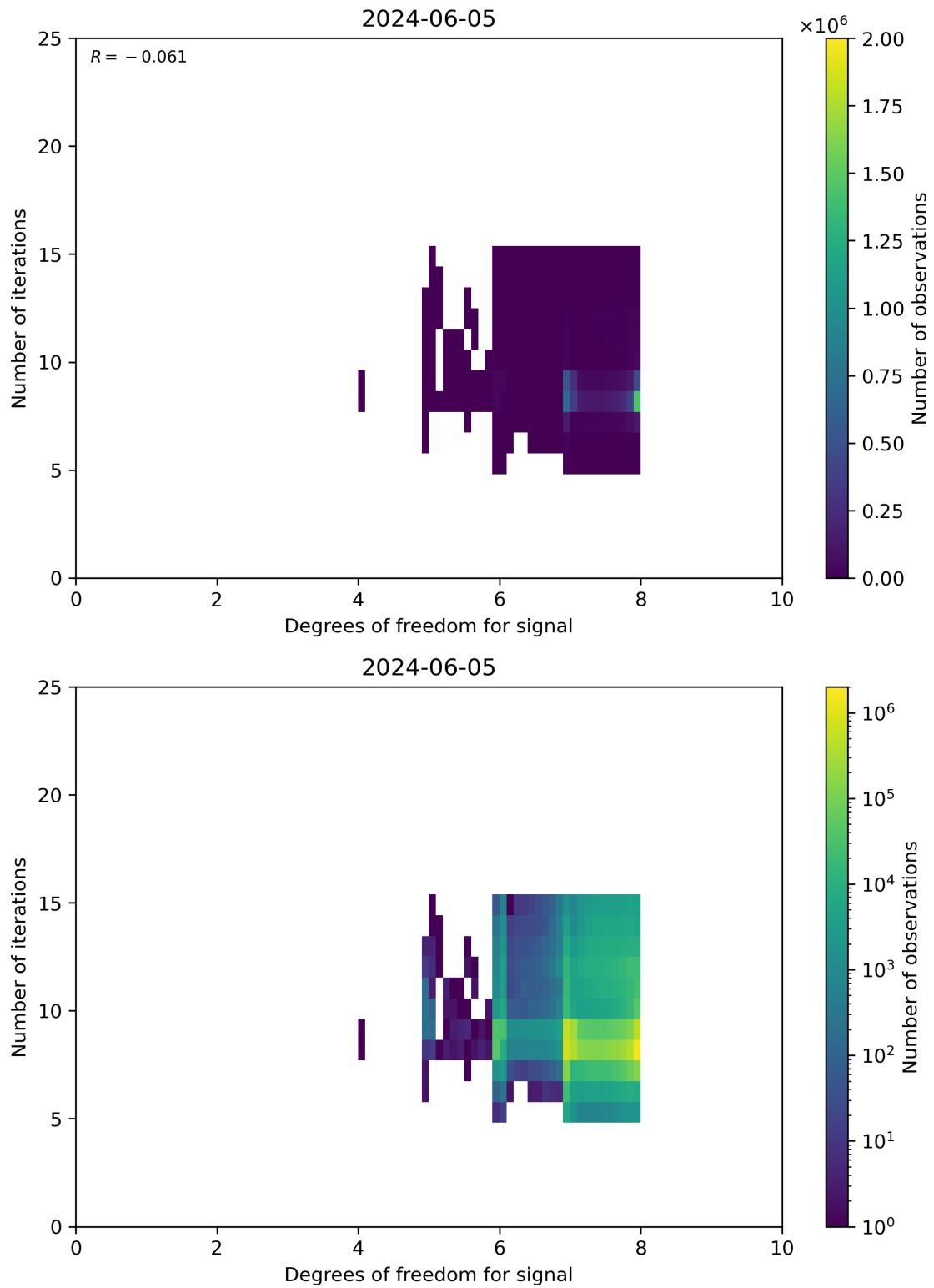
Figure 50: Scatter density plot of “Degrees of freedom for signal” against “Number of iterations” for 2024-06-04 to 2024-06-06.
