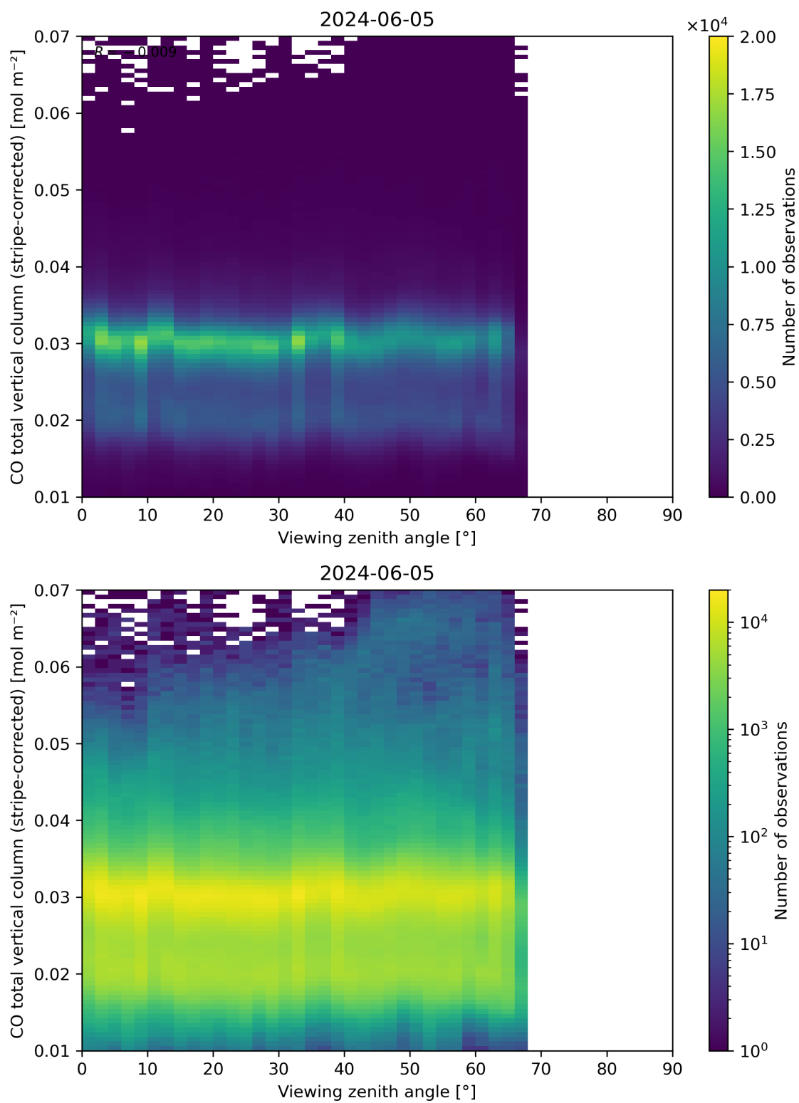
Figure 70: Scatter density plot of “Viewing zenith angle” against “CO total vertical column (stripe-corrected)” for 2024-06-04 to 2024-06-06.
