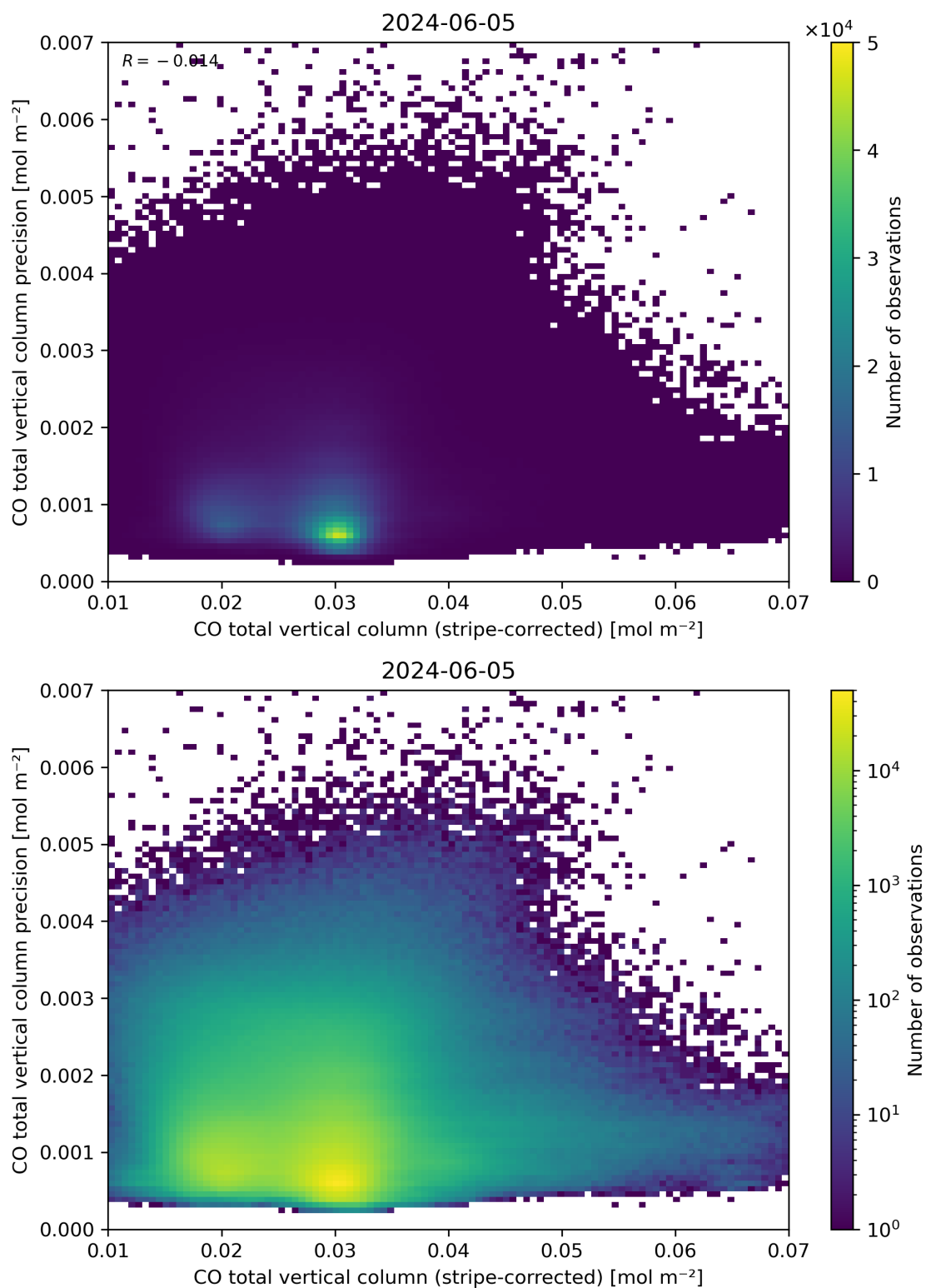
Figure 36: Scatter density plot of “CO total vertical column (stripe-corrected)” against “CO total vertical column precision” for 2024-06-04 to 2024-06-06.
