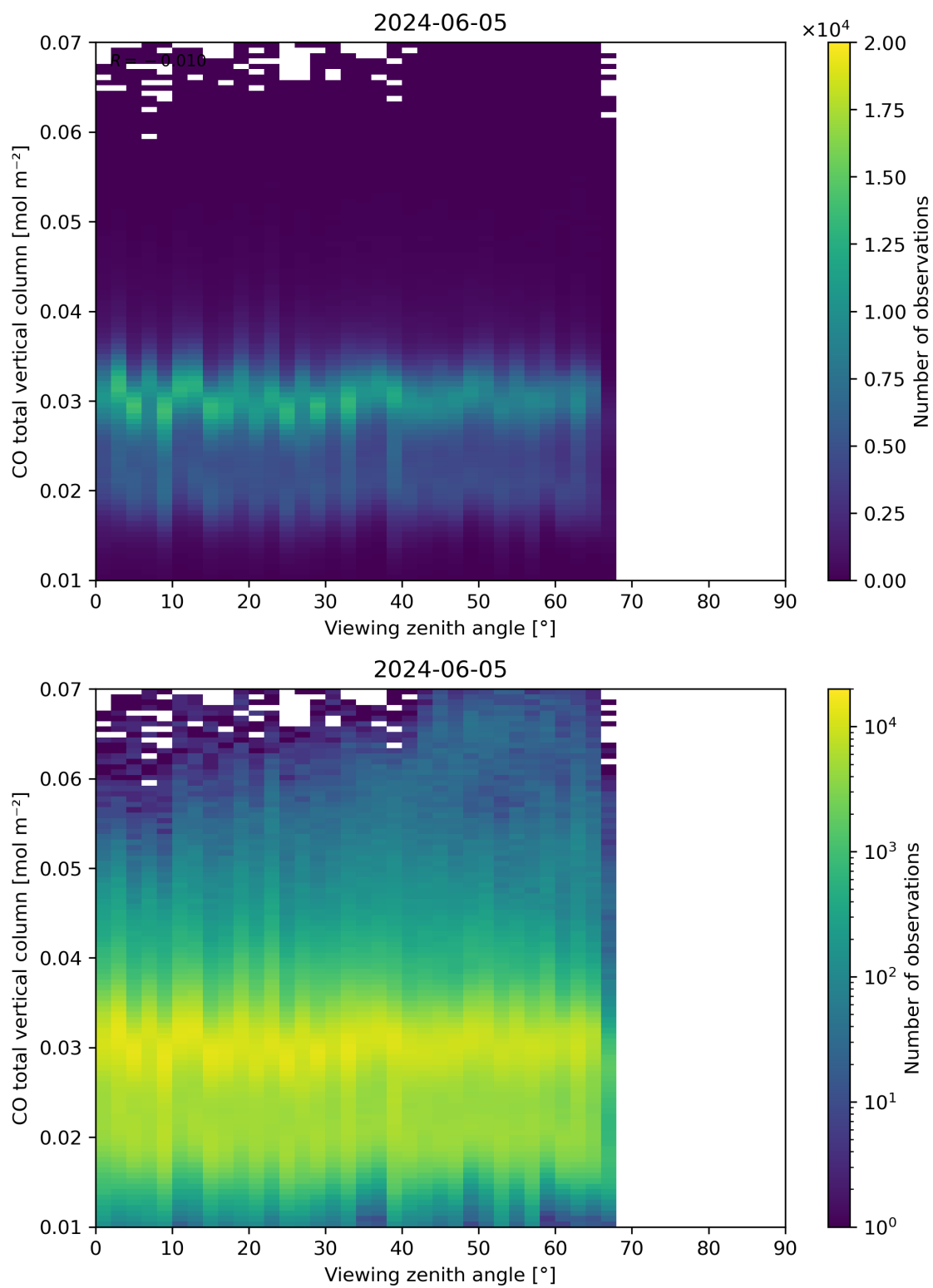
Figure 69: Scatter density plot of “Viewing zenith angle” against “CO total vertical column” for 2024-06-04 to 2024-06-06.
