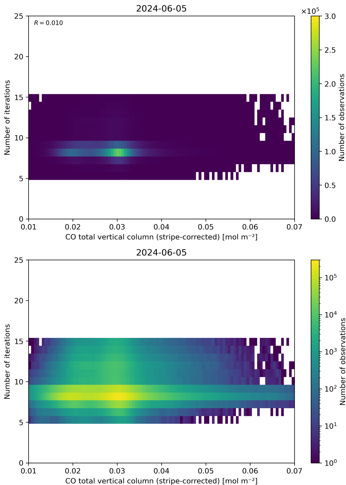
Figure 39: Scatter density plot of “CO total vertical column (stripe-corrected)” against “Number of iterations” for 2024-06-04 to 2024-06-06.
