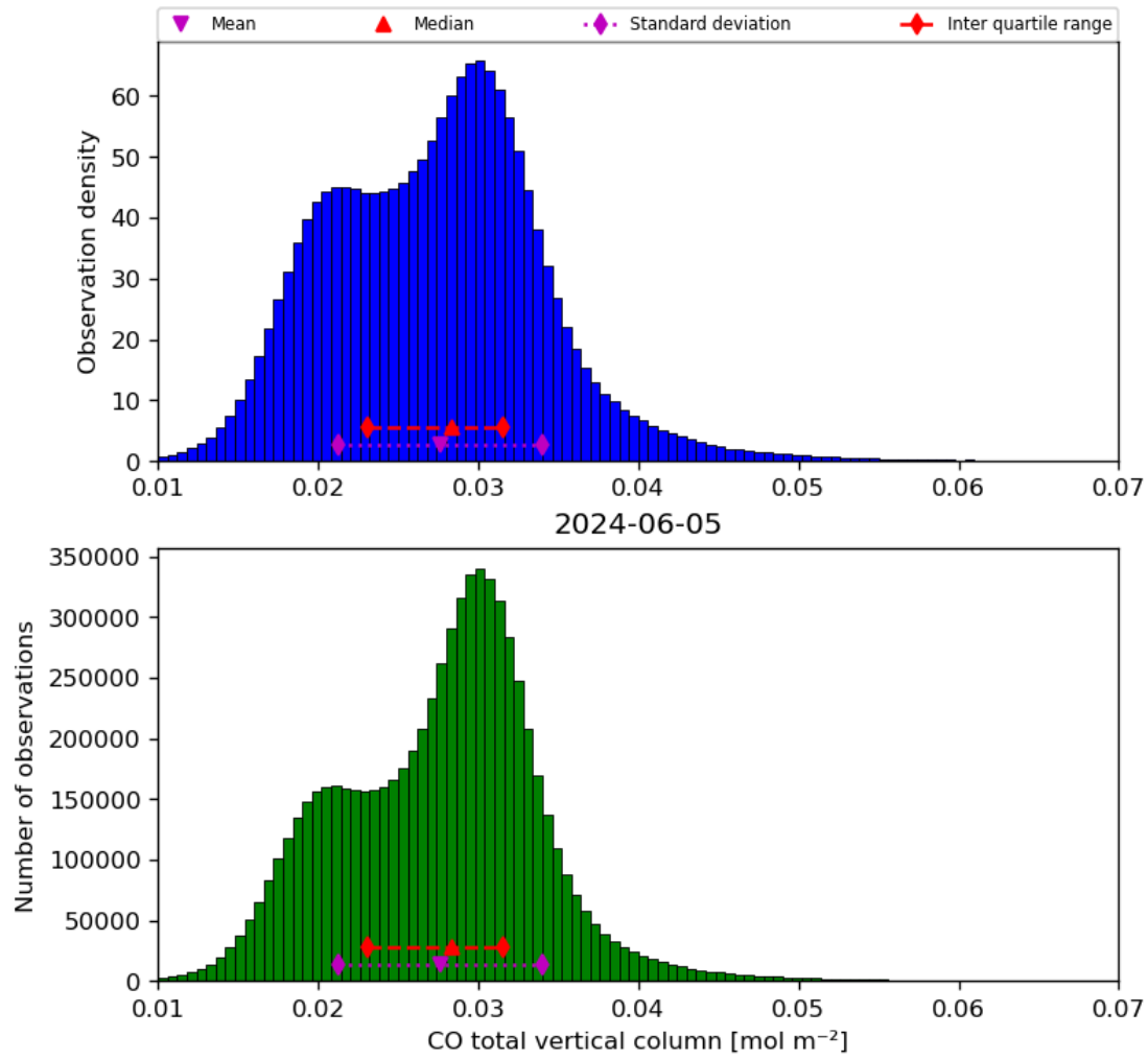
Figure 18: Histogram of “CO total vertical column” for 2024-06-04 to 2024-06-06
