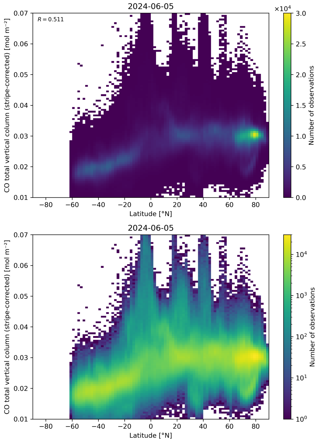
Figure 52: Scatter density plot of “Latitude” against “CO total vertical column (stripe-corrected)” for 2024-06-04 to 2024-06-06.
