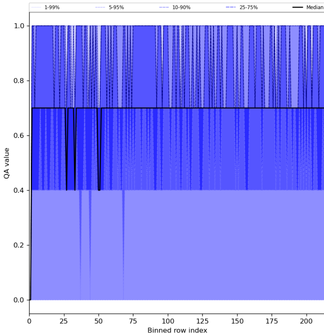
Figure 25: Along track statistics of “QA value” for 2024-06-04 to 2024-06-06
