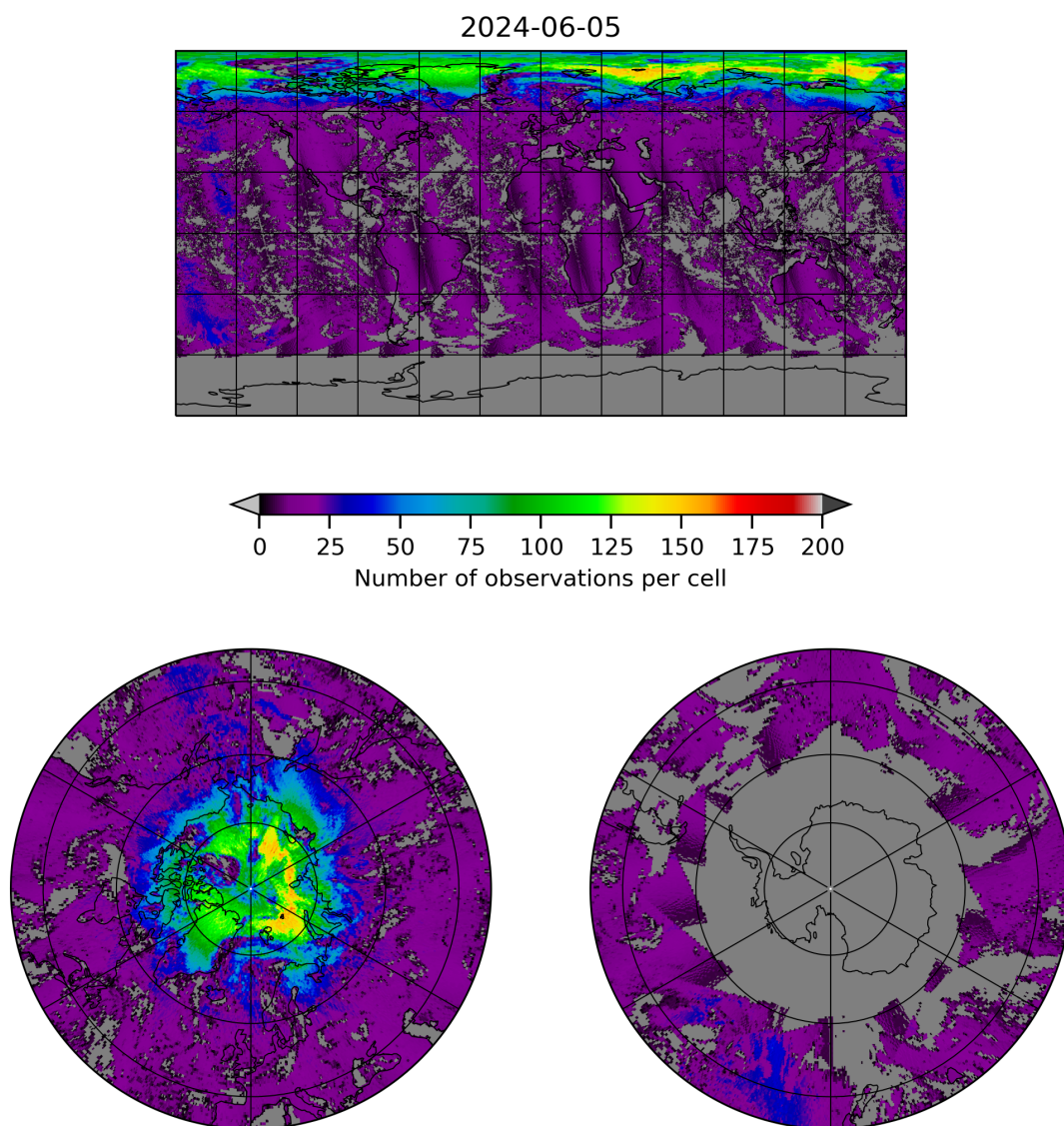
Figure 8: Map of the number of observations for 2024-06-04 to 2024-06-06
