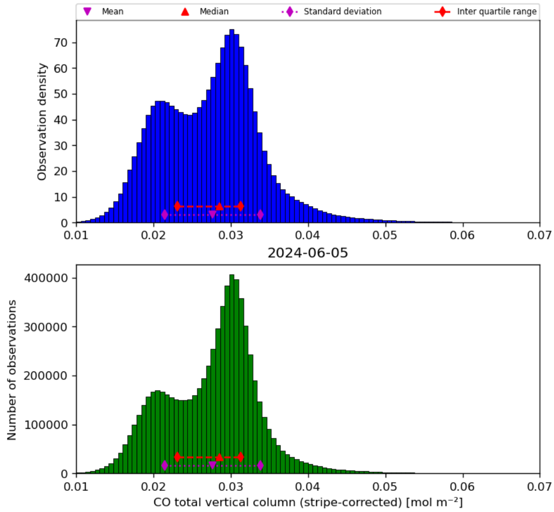
Figure 19: Histogram of “CO total vertical column (stripe-corrected)” for 2024-06-04 to 2024-06-06
