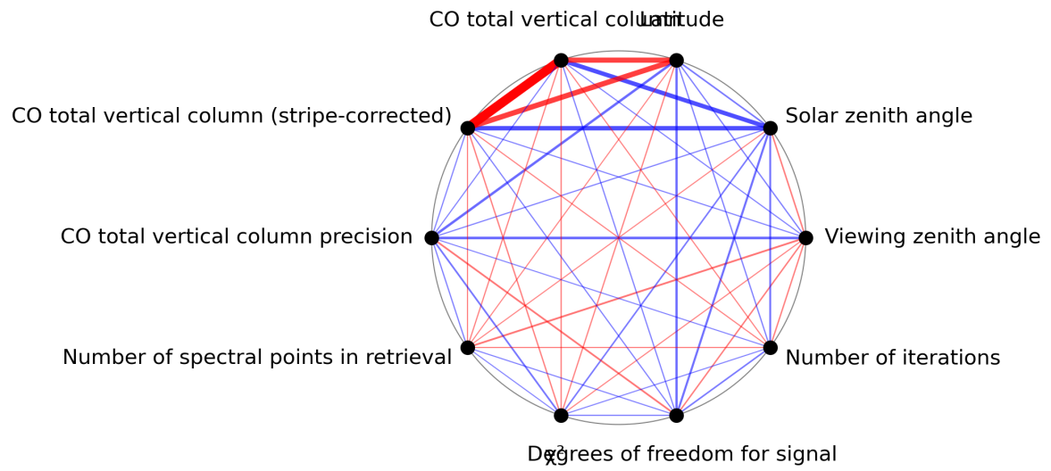
Figure 1: Map of correlation graph for 2024-06-04 to 2024-06-06.
