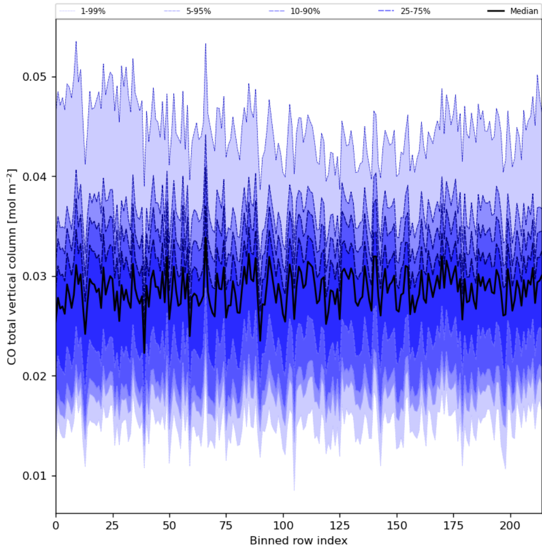
Figure 26: Along track statistics of “CO total vertical column” for 2024-06-04 to 2024-06-06
