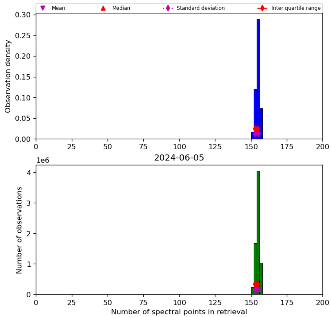
Figure 21: Histogram of “Number of spectral points in retrieval” for 2024-06-04 to 2024-06-06
