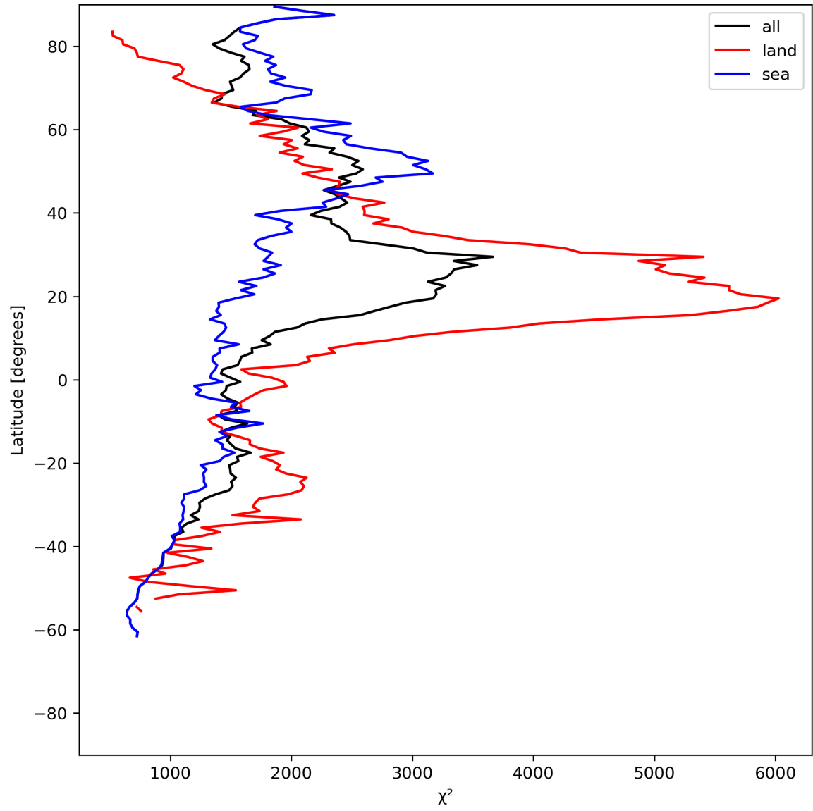
Figure 14: Zonal average of “ \chi^2 ” for 2024-06-04 to 2024-06-06.
