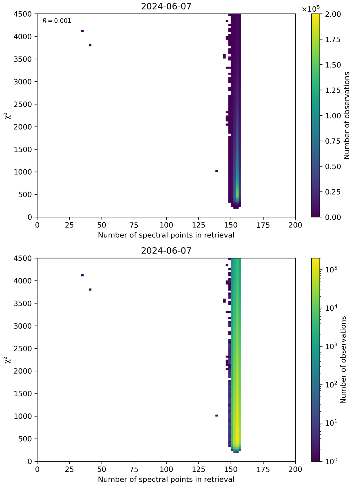
Figure 58: Scatter density plot of “Number of spectral points in retrieval” against “ \chi^2 ” for 2024-06-06 to 2024-06-08.
