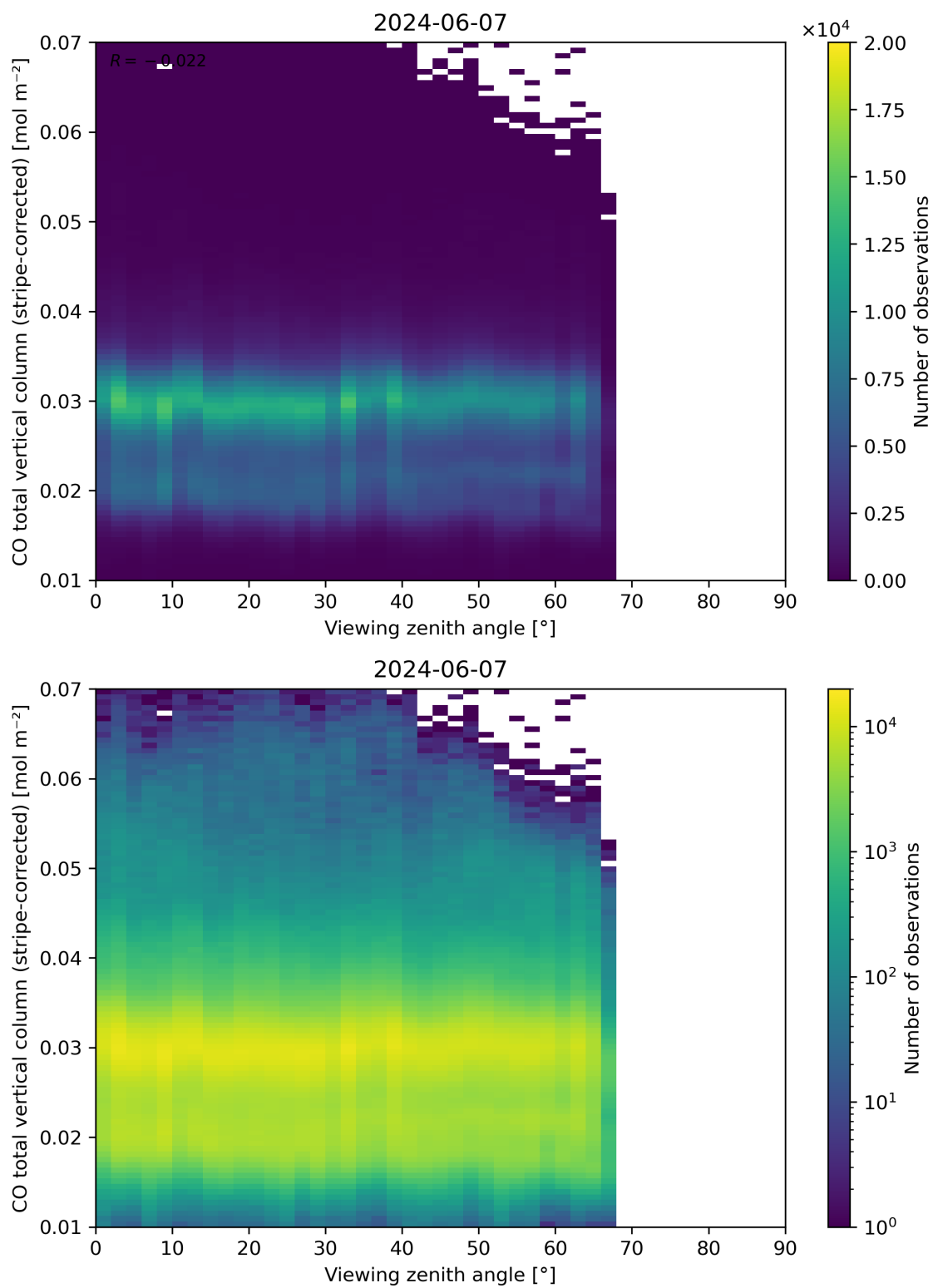
Figure 70: Scatter density plot of “Viewing zenith angle” against “CO total vertical column (stripe-corrected)” for 2024-06-06 to 2024-06-08.
