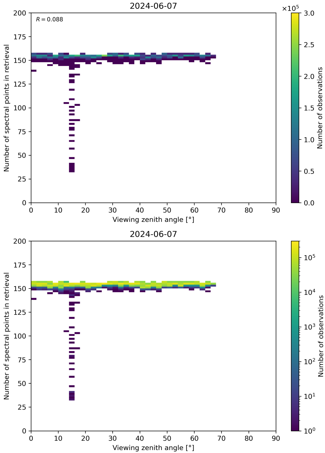
Figure 76: Scatter density plot of “Viewing zenith angle” against “Number of spectral points in retrieval” for 2024-06-06 to 2024-06-08.
