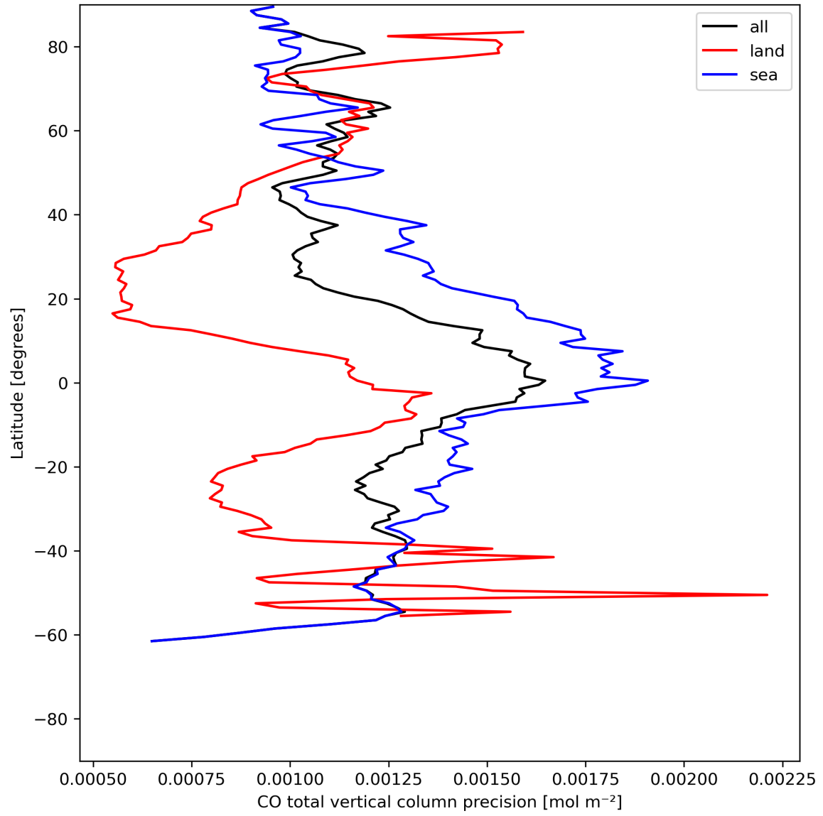
Figure 12: Zonal average of “CO total vertical column precision” for 2024-06-06 to 2024-06-08.
