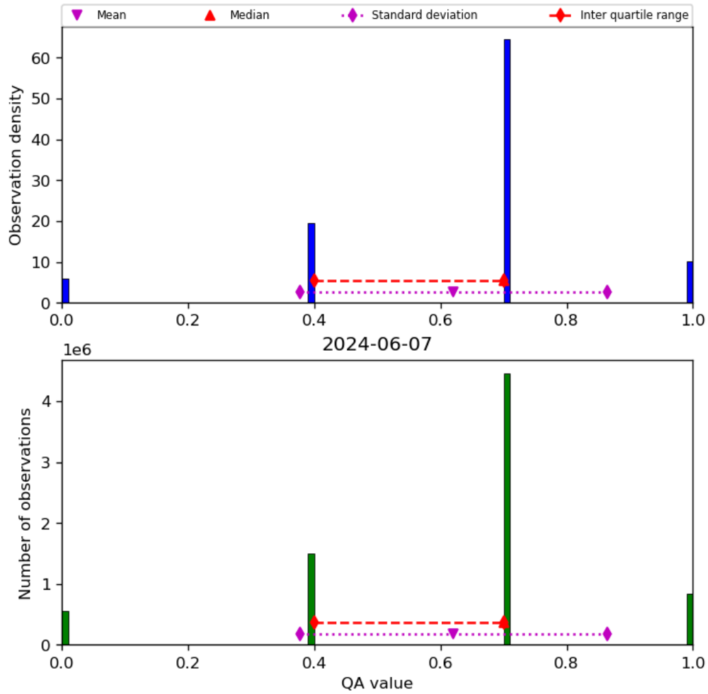
Figure 17: Histogram of “QA value” for 2024-06-06 to 2024-06-08
