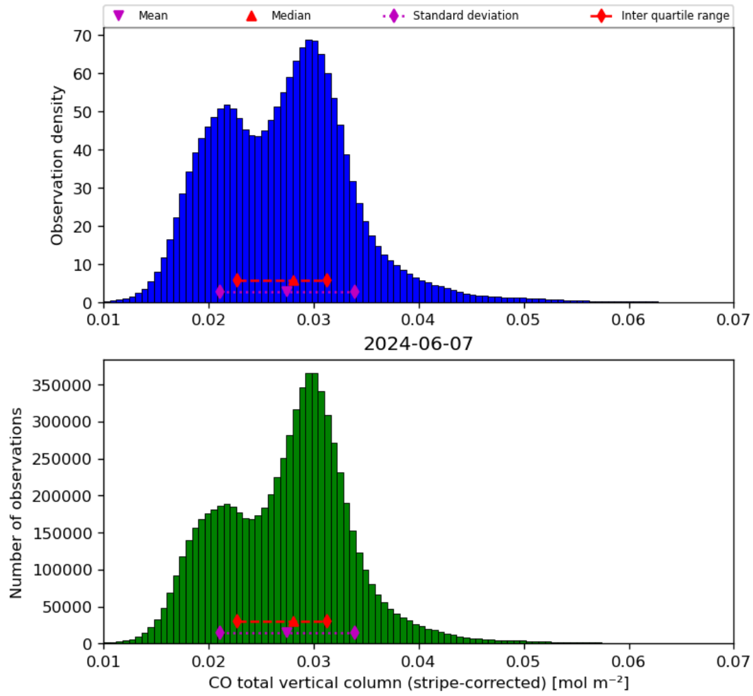
Figure 19: Histogram of “CO total vertical column (stripe-corrected)” for 2024-06-06 to 2024-06-08
