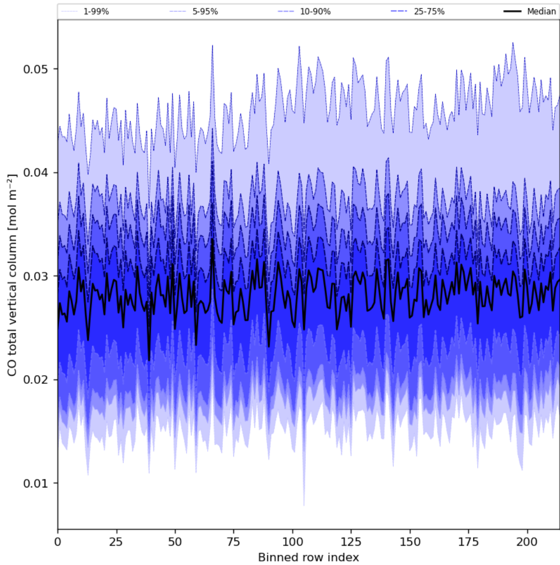
Figure 26: Along track statistics of “CO total vertical column” for 2024-06-06 to 2024-06-08
