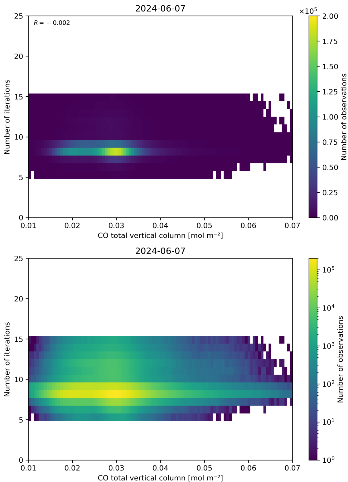
Figure 42: Scatter density plot of “CO total vertical column” against “Number of iterations” for 2024-06-06 to 2024-06-08.
