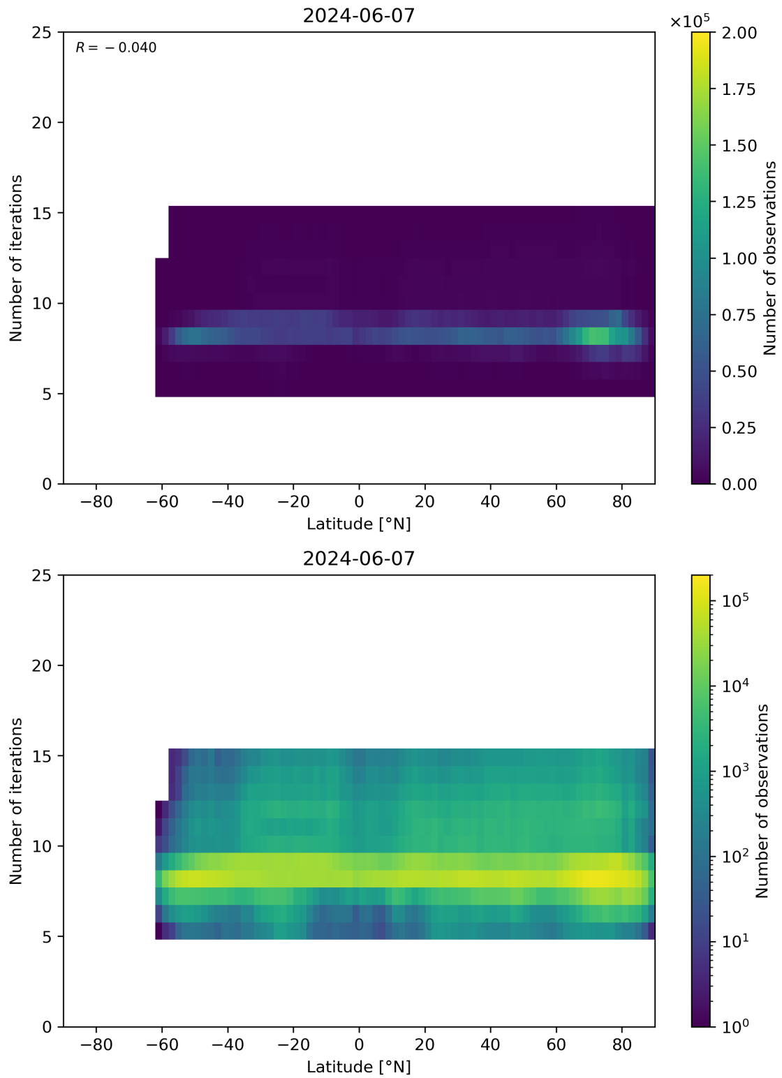
Figure 56: Scatter density plot of “Latitude” against “Number of iterations” for 2024-06-06 to 2024-06-08.
