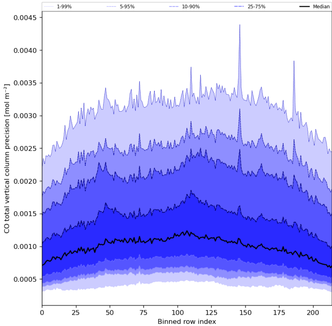
Figure 28: Along track statistics of “CO total vertical column precision” for 2024-06-06 to 2024-06-08
