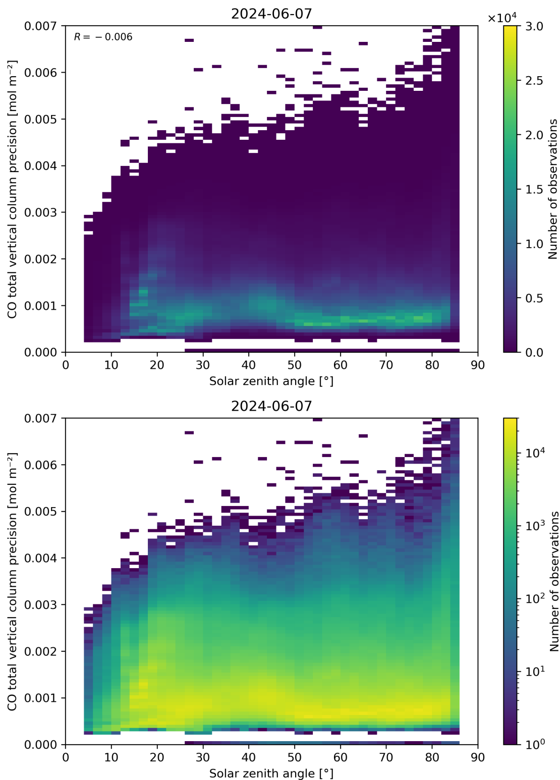
Figure 63: Scatter density plot of “Solar zenith angle” against “CO total vertical column precision” for 2024-06-06 to 2024-06-08.
