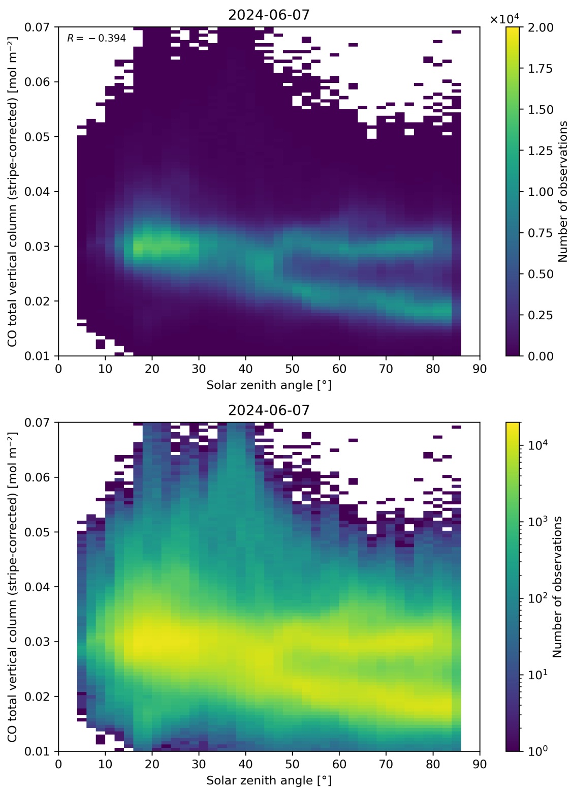
Figure 62: Scatter density plot of “Solar zenith angle” against “CO total vertical column (stripe-corrected)” for 2024-06-06 to 2024-06-08.
