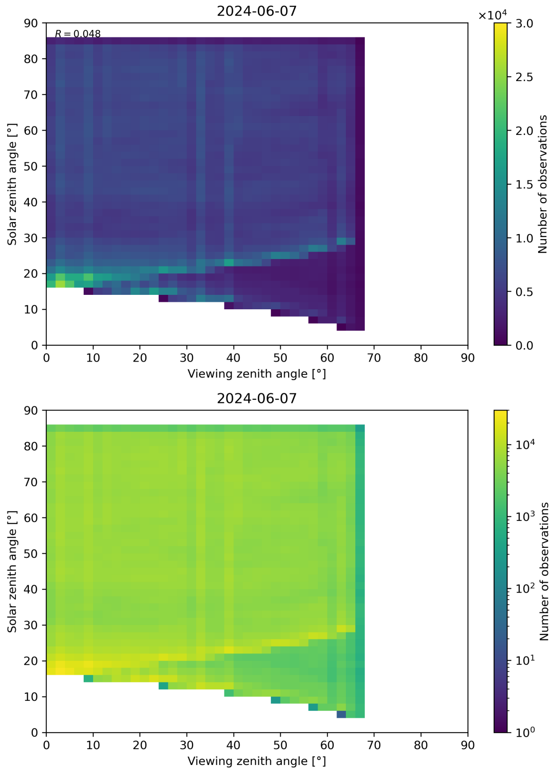
Figure 77: Scatter density plot of “Viewing zenith angle” against “Solar zenith angle” for 2024-06-06 to 2024-06-08.
