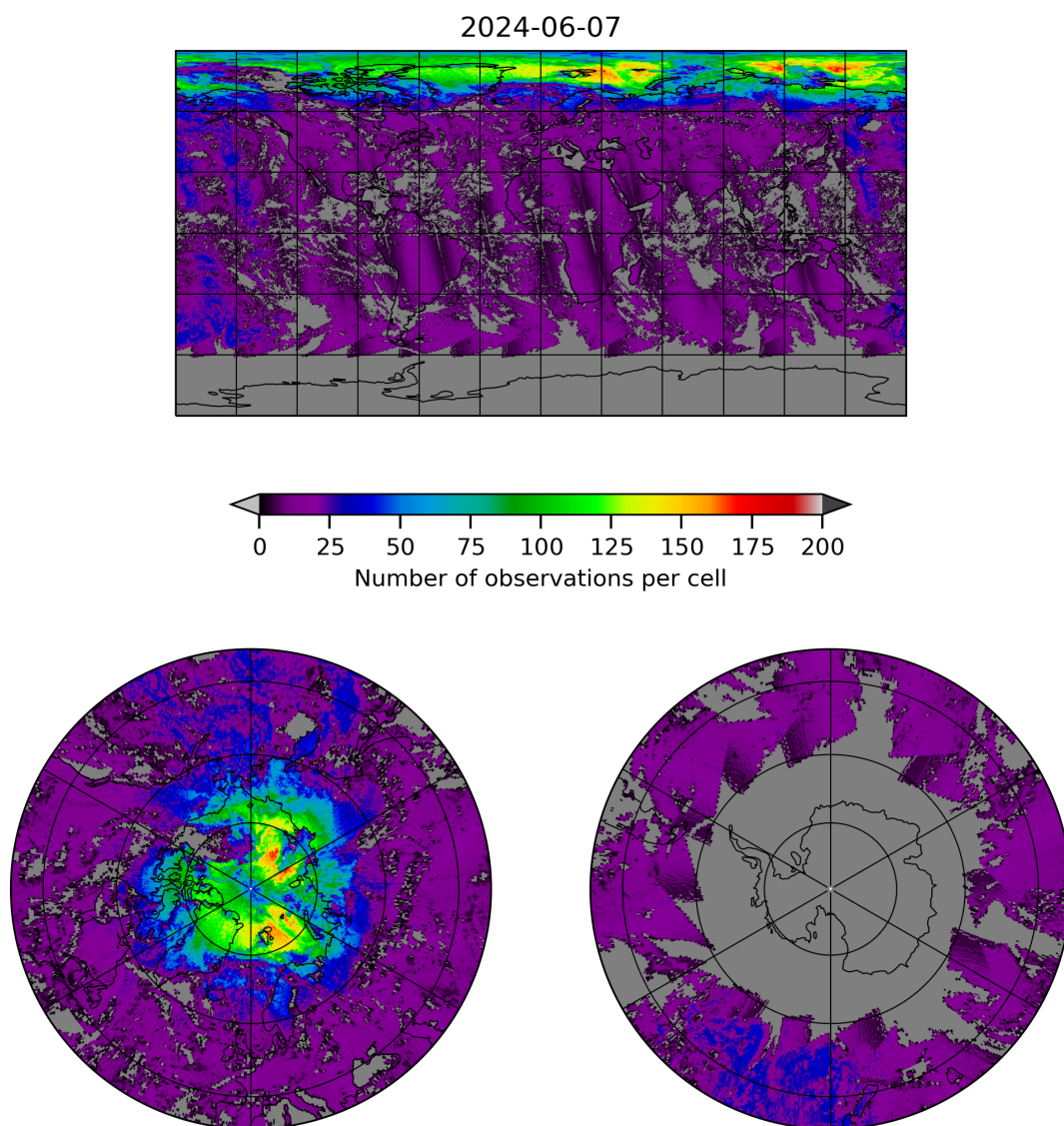
Figure 8: Map of the number of observations for 2024-06-06 to 2024-06-08
