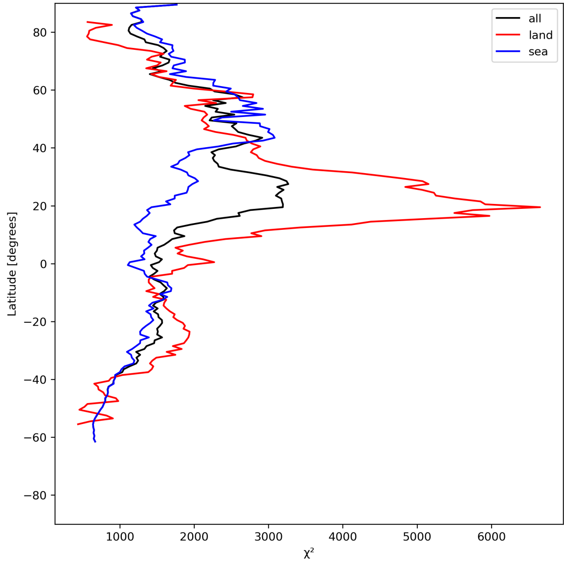
Figure 14: Zonal average of “ \chi^2 ” for 2024-06-06 to 2024-06-08.
