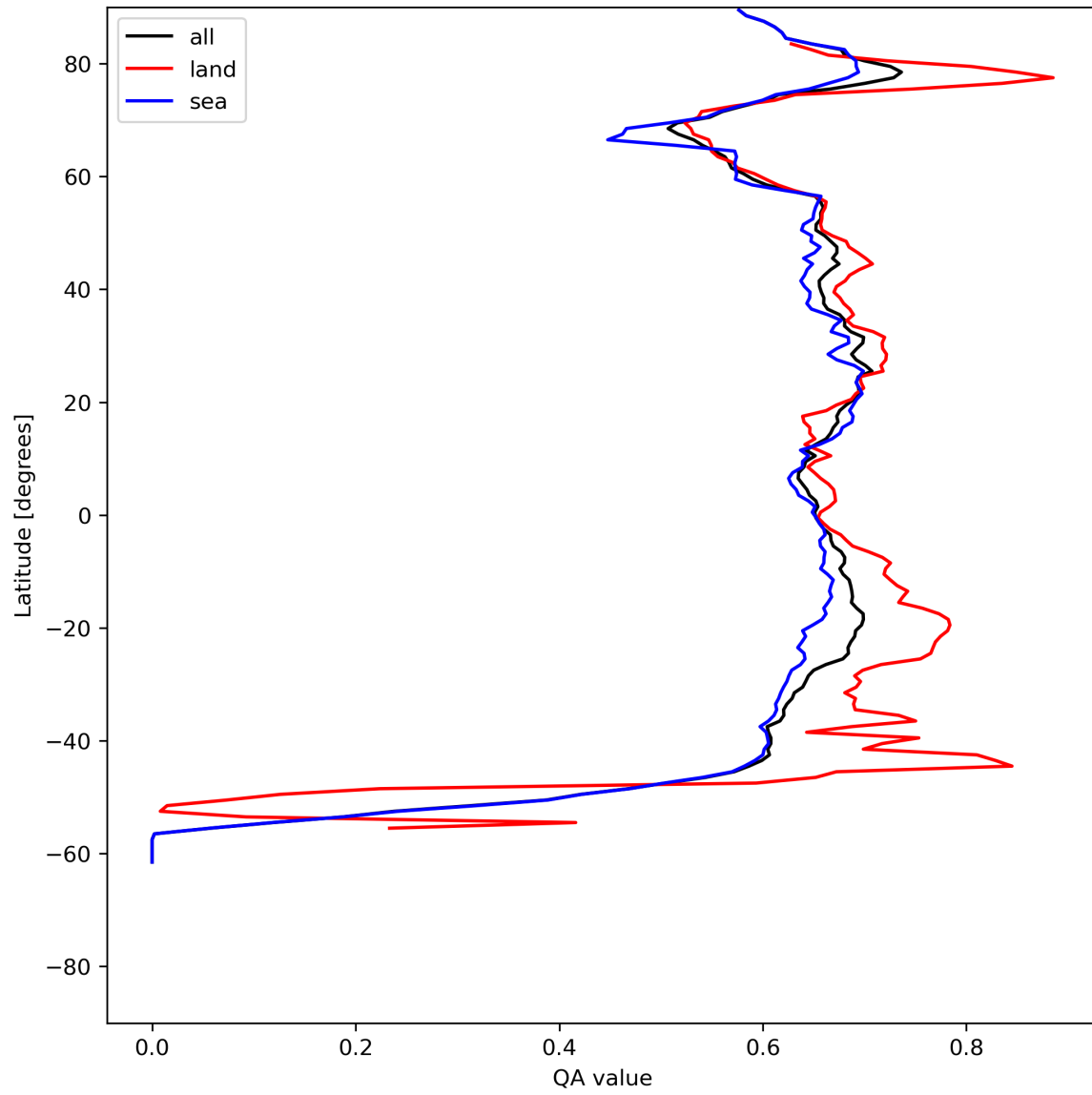
Figure 9: Zonal average of “QA value” for 2024-06-06 to 2024-06-08.
