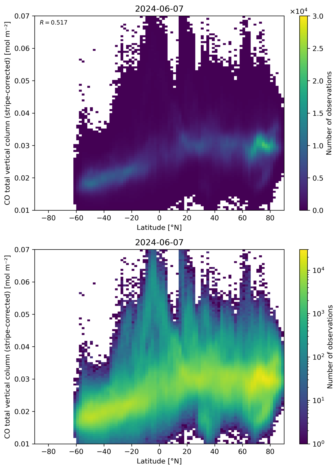
Figure 52: Scatter density plot of “Latitude” against “CO total vertical column (stripe-corrected)” for 2024-06-06 to 2024-06-08.
