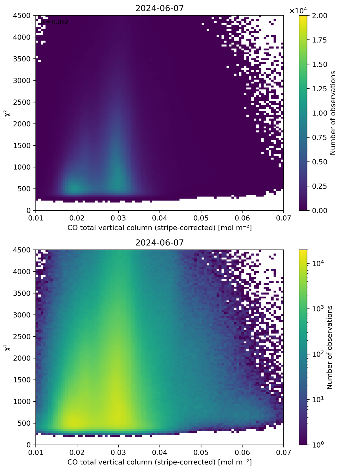
Figure 37: Scatter density plot of “CO total vertical column (stripe-corrected)” against “ \chi^2 ” for 2024-06-06 to 2024-06-08.
