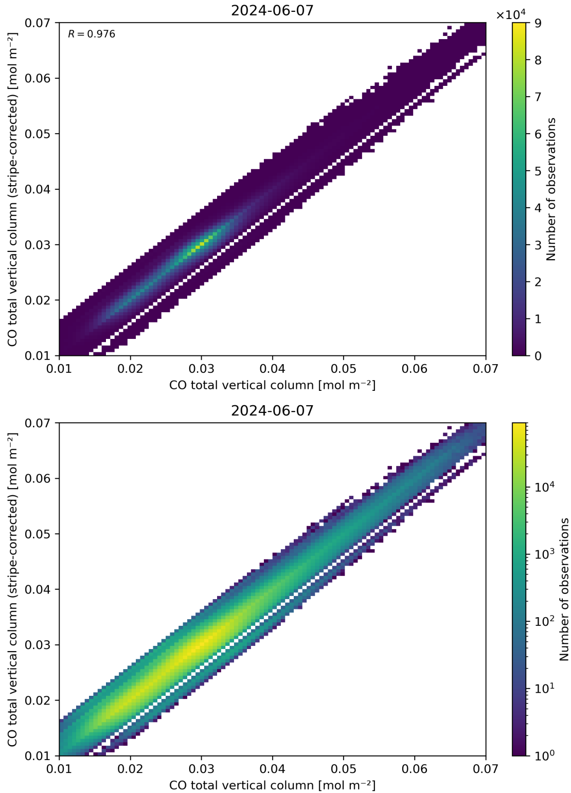
Figure 33: Scatter density plot of “CO total vertical column” against “CO total vertical column (stripe-corrected)” for 2024-06-06 to 2024-06-08.
