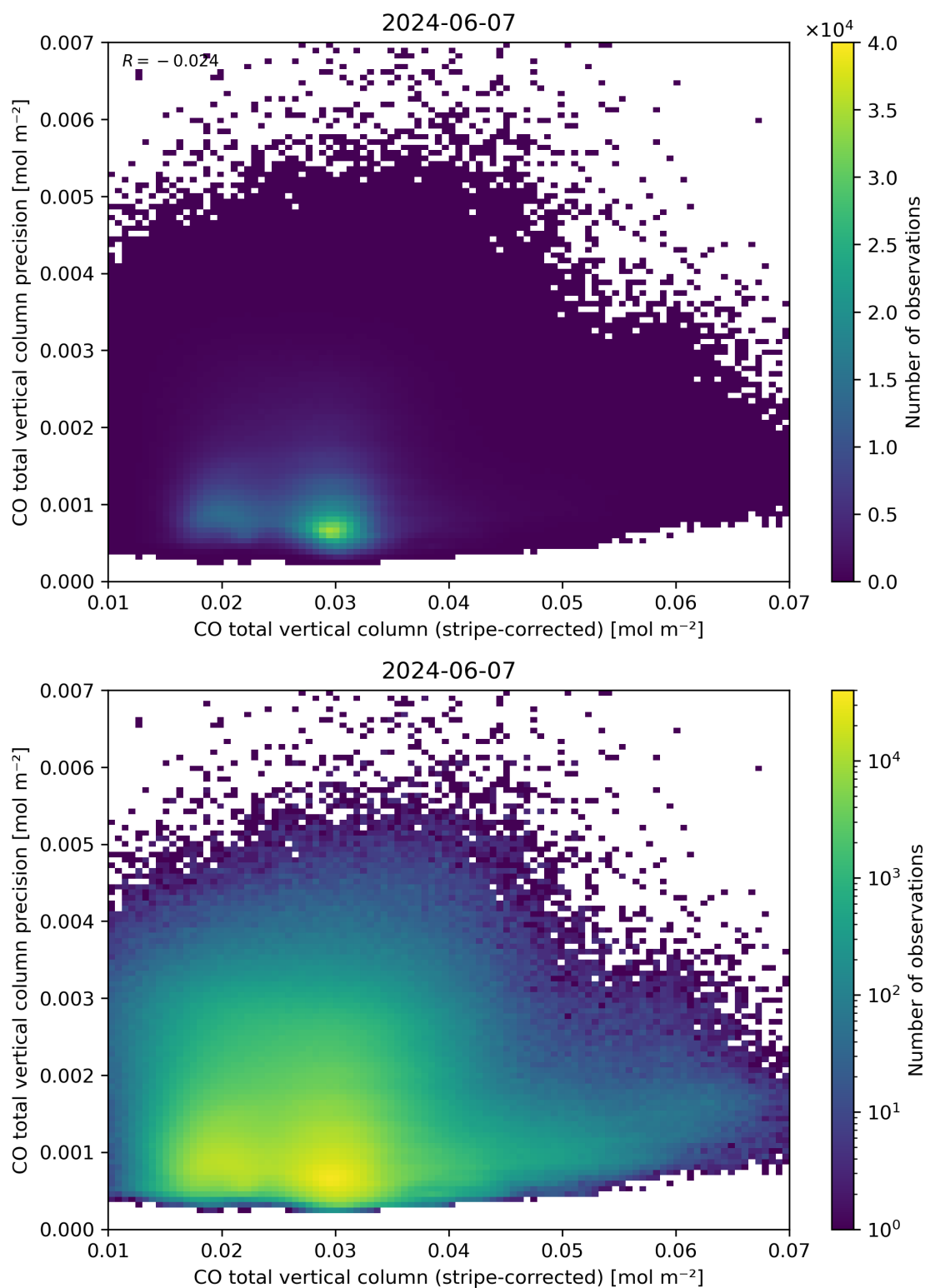
Figure 36: Scatter density plot of “CO total vertical column (stripe-corrected)” against “CO total vertical column precision” for 2024-06-06 to 2024-06-08.
