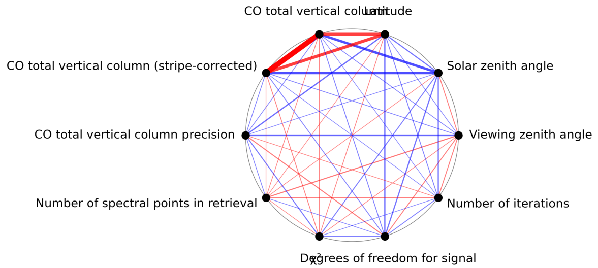
Figure 1: Map of correlation graph for 2024-06-06 to 2024-06-08.
