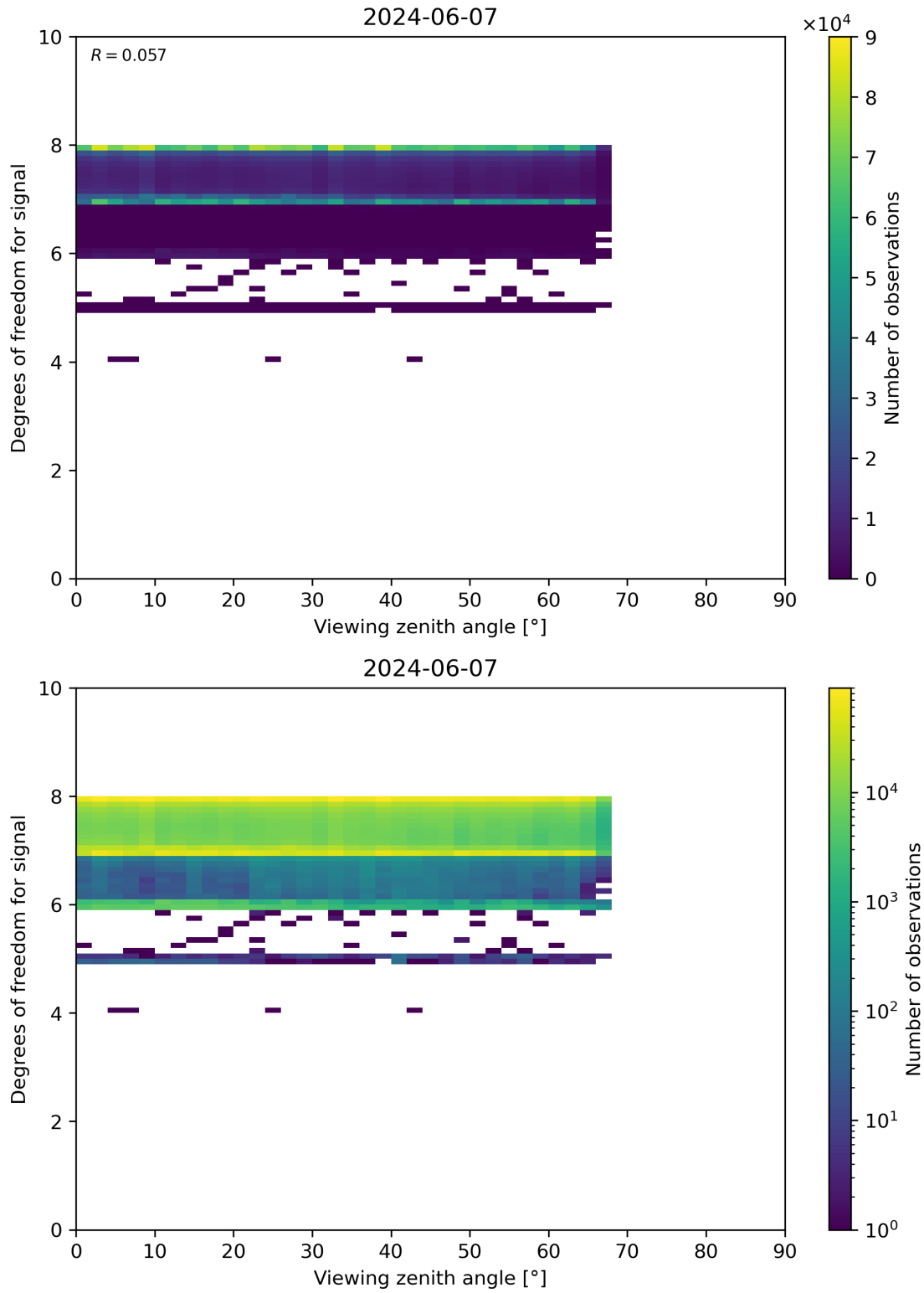
Figure 73: Scatter density plot of “Viewing zenith angle” against “Degrees of freedom for signal” for 2024-06-06 to 2024-06-08.
