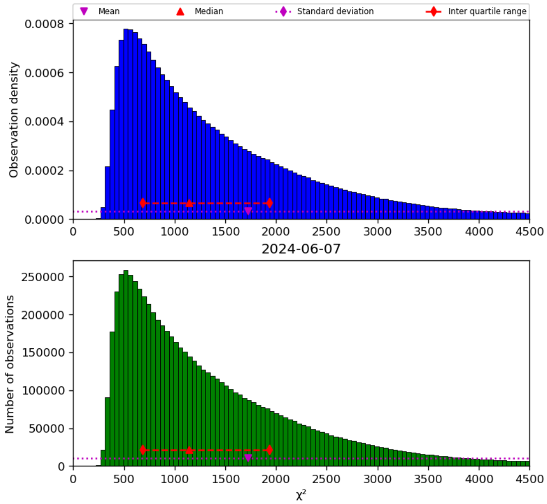
Figure 22: Histogram of “ \chi^2 ” for 2024-06-06 to 2024-06-08
