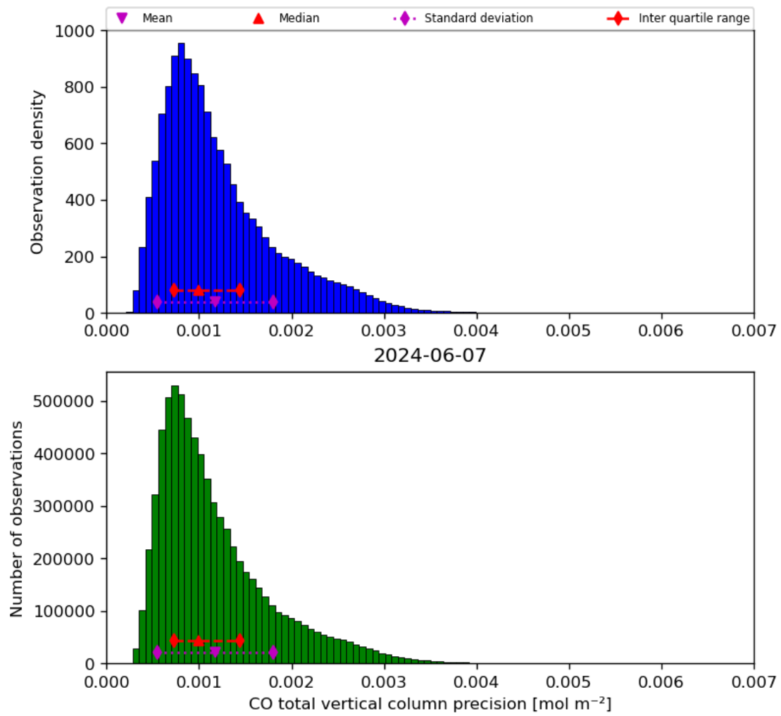
Figure 20: Histogram of “CO total vertical column precision” for 2024-06-06 to 2024-06-08
