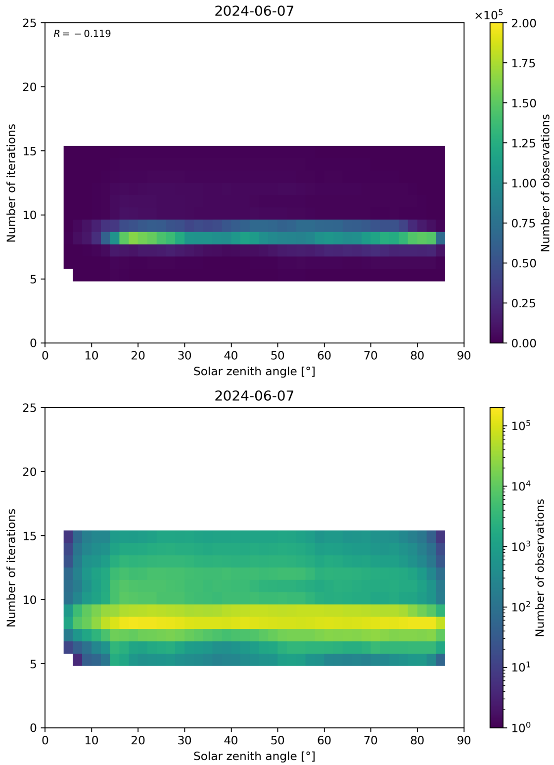
Figure 67: Scatter density plot of “Solar zenith angle” against “Number of iterations” for 2024-06-06 to 2024-06-08.
