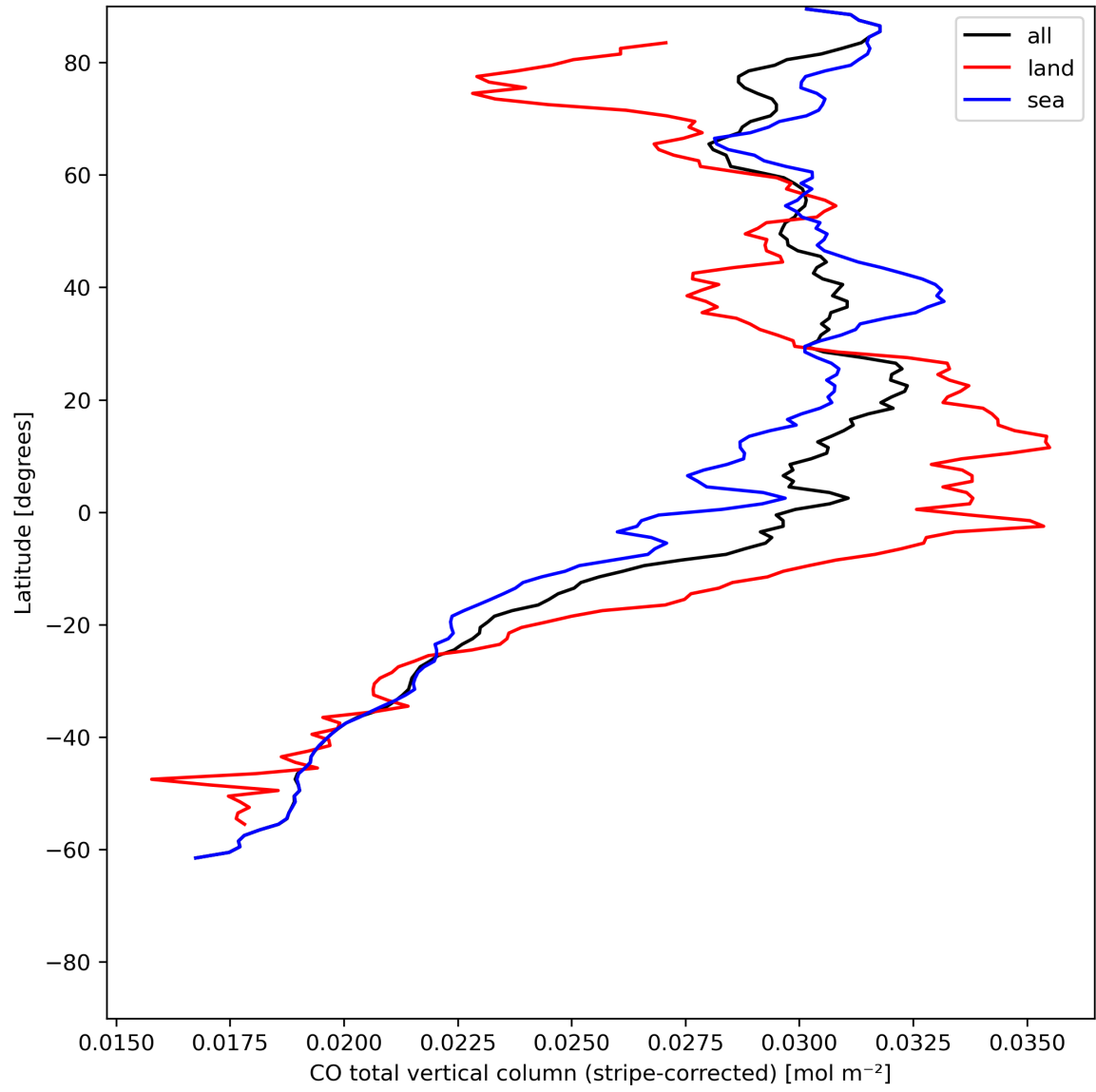
Figure 11: Zonal average of “CO total vertical column (stripe-corrected)” for 2024-06-06 to 2024-06-08.
