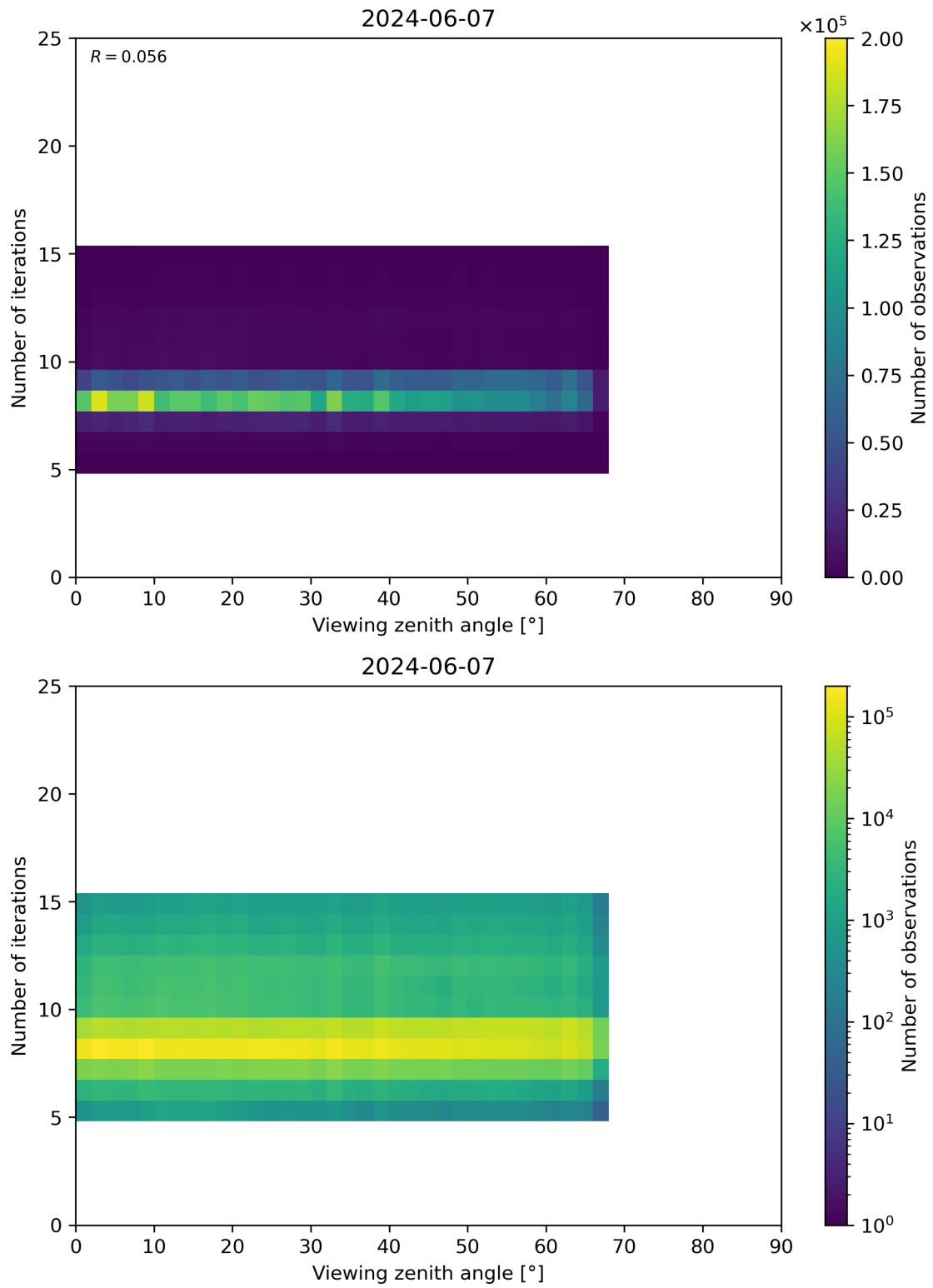
Figure 75: Scatter density plot of “Viewing zenith angle” against “Number of iterations” for 2024-06-06 to 2024-06-08.
