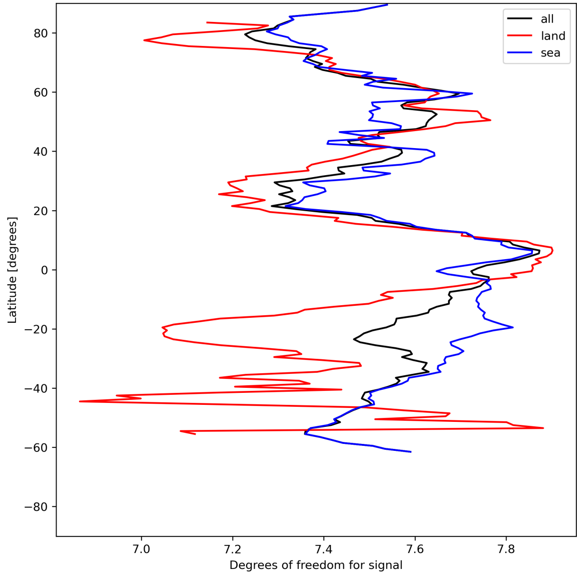
Figure 15: Zonal average of “Degrees of freedom for signal” for 2024-06-06 to 2024-06-08.
