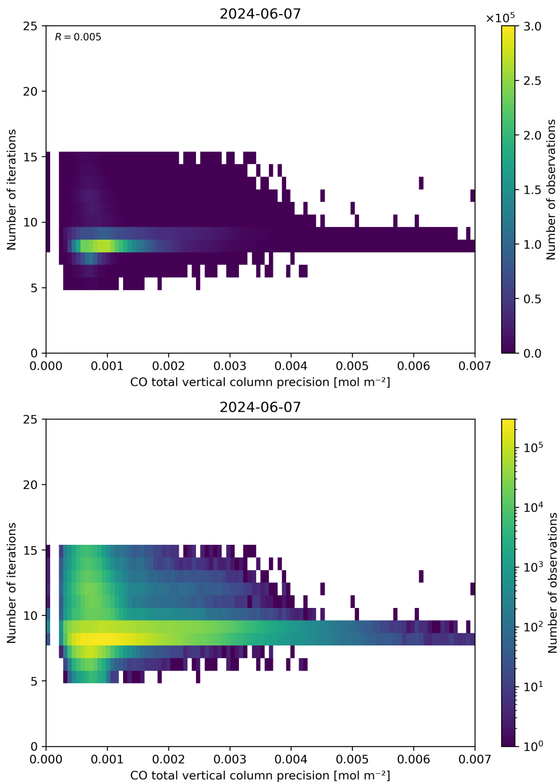
Figure 46: Scatter density plot of “CO total vertical column precision” against “Number of iterations” for 2024-06-06 to 2024-06-08.
