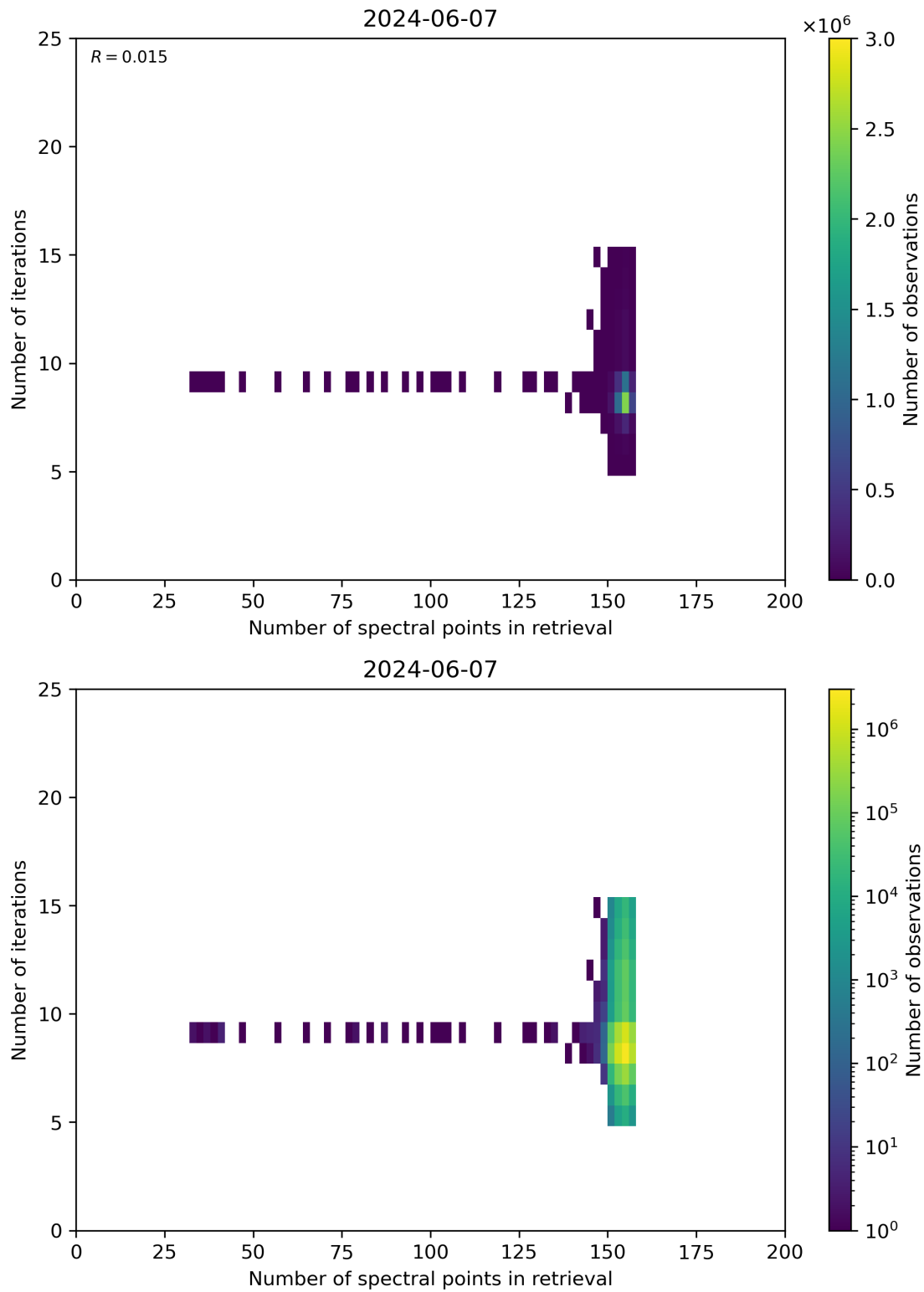
Figure 60: Scatter density plot of “Number of spectral points in retrieval” against “Number of iterations” for 2024-06-06 to 2024-06-08.
