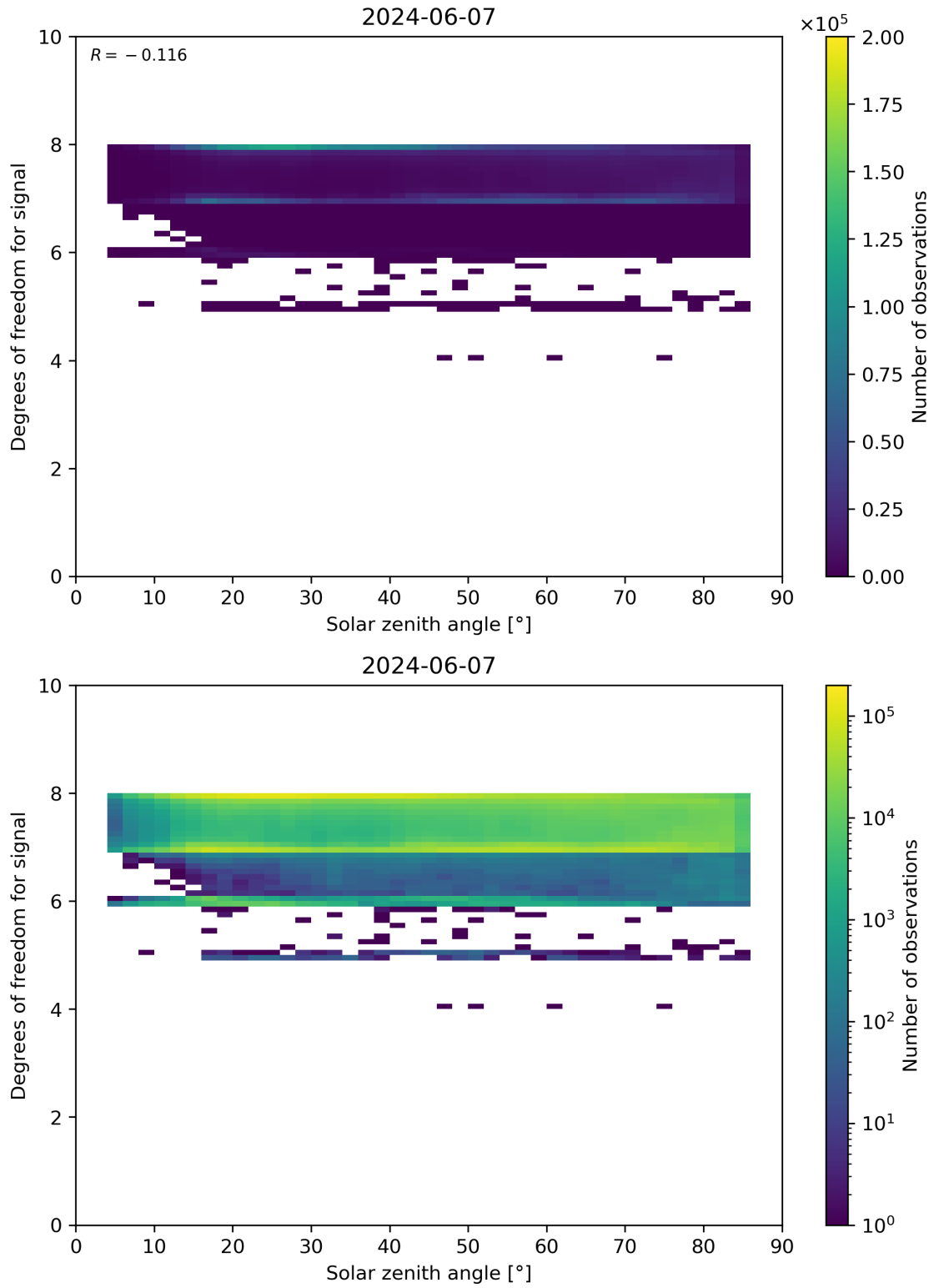
Figure 65: Scatter density plot of “Solar zenith angle” against “Degrees of freedom for signal” for 2024-06-06 to 2024-06-08.
