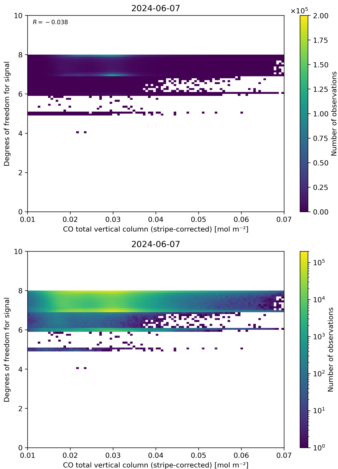
Figure 38: Scatter density plot of “CO total vertical column (stripe-corrected)” against “Degrees of freedom for signal” for 2024-06-06 to 2024-06-08.
