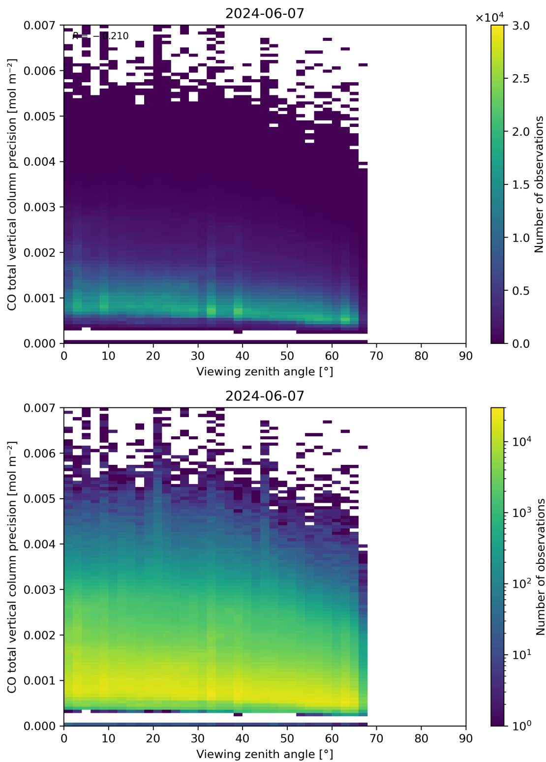
Figure 71: Scatter density plot of “Viewing zenith angle” against “CO total vertical column precision” for 2024-06-06 to 2024-06-08.
