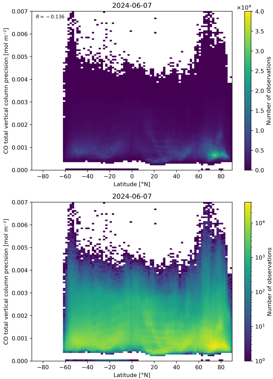
Figure 53: Scatter density plot of “Latitude” against “CO total vertical column precision” for 2024-06-06 to 2024-06-08.
