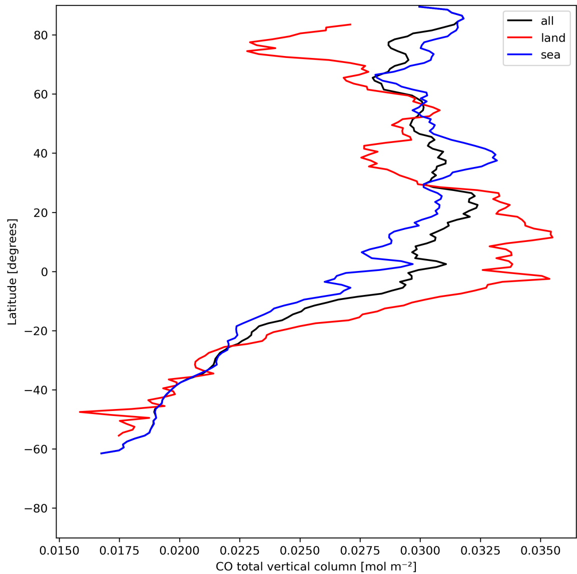
Figure 10: Zonal average of “CO total vertical column” for 2024-06-06 to 2024-06-08.
