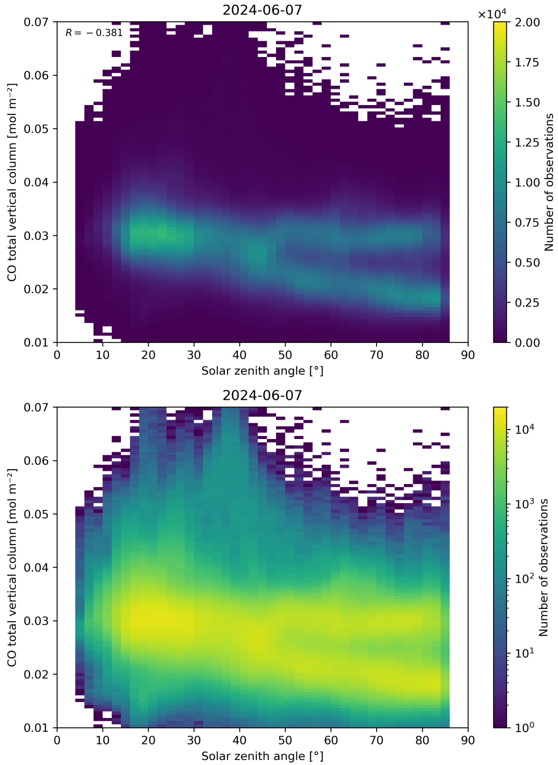
Figure 61: Scatter density plot of “Solar zenith angle” against “CO total vertical column” for 2024-06-06 to 2024-06-08.
