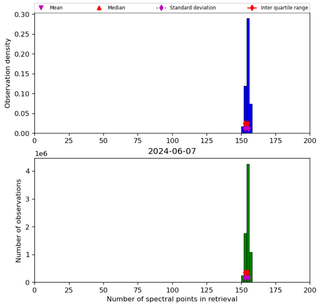
Figure 21: Histogram of “Number of spectral points in retrieval” for 2024-06-06 to 2024-06-08
