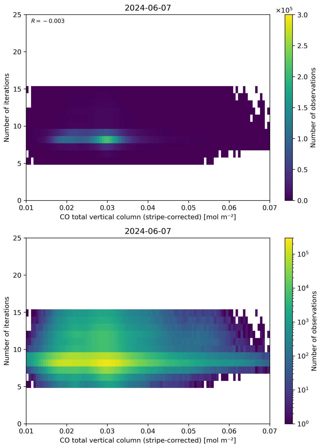
Figure 39: Scatter density plot of “CO total vertical column (stripe-corrected)” against “Number of iterations” for 2024-06-06 to 2024-06-08.
