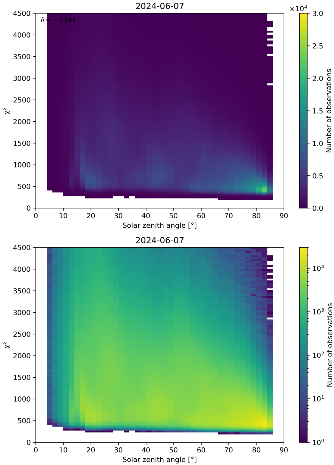
Figure 64: Scatter density plot of “Solar zenith angle” against “ \chi^2 ” for 2024-06-06 to 2024-06-08.
