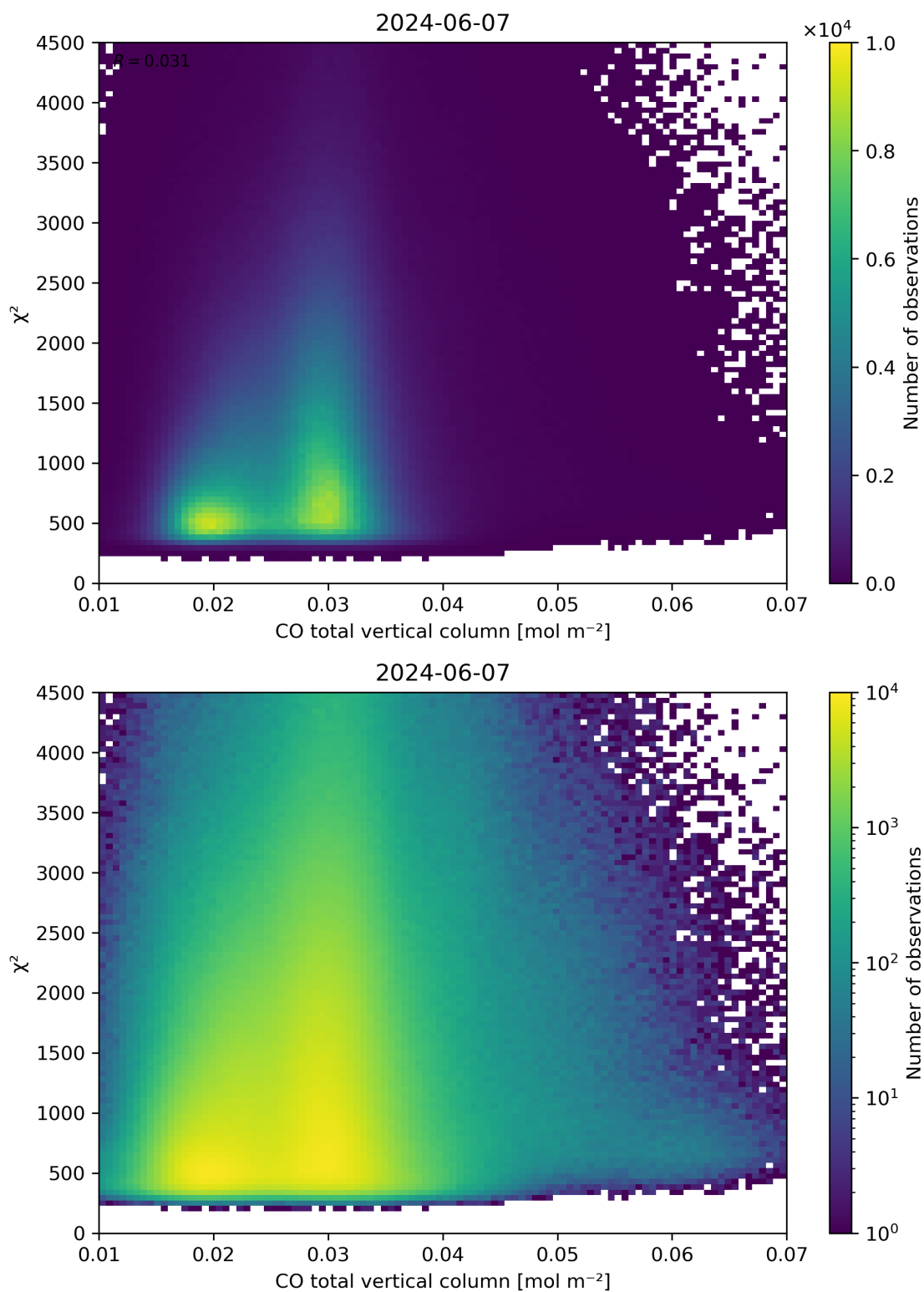
Figure 35: Scatter density plot of “CO total vertical column” against “ \chi^2 ” for 2024-06-06 to 2024-06-08.
