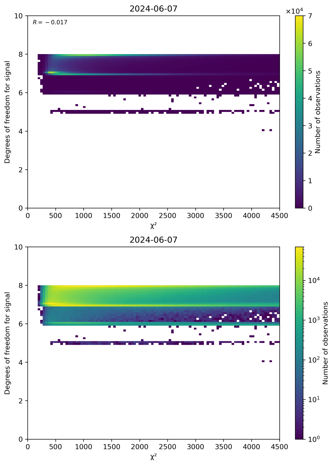
Figure 48: Scatter density plot of " \chi^2 " against "Degrees of freedom for signal" for 2024-06-06 to 2024-06-08.
