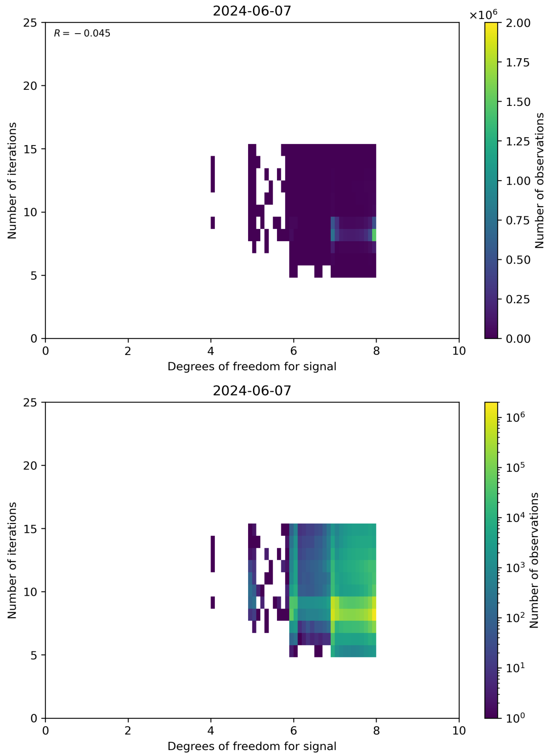
Figure 50: Scatter density plot of “Degrees of freedom for signal” against “Number of iterations” for 2024-06-06 to 2024-06-08.
