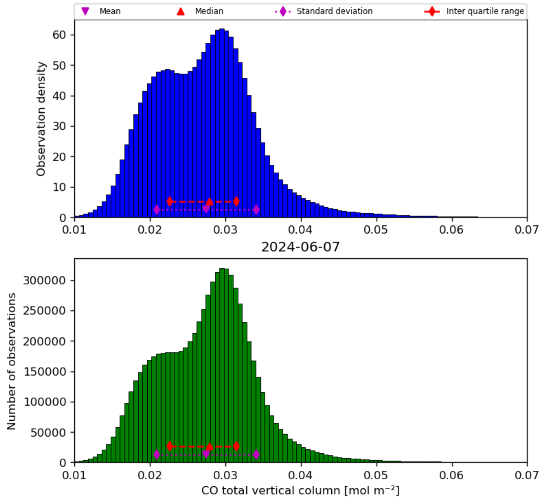
Figure 18: Histogram of “CO total vertical column” for 2024-06-06 to 2024-06-08
