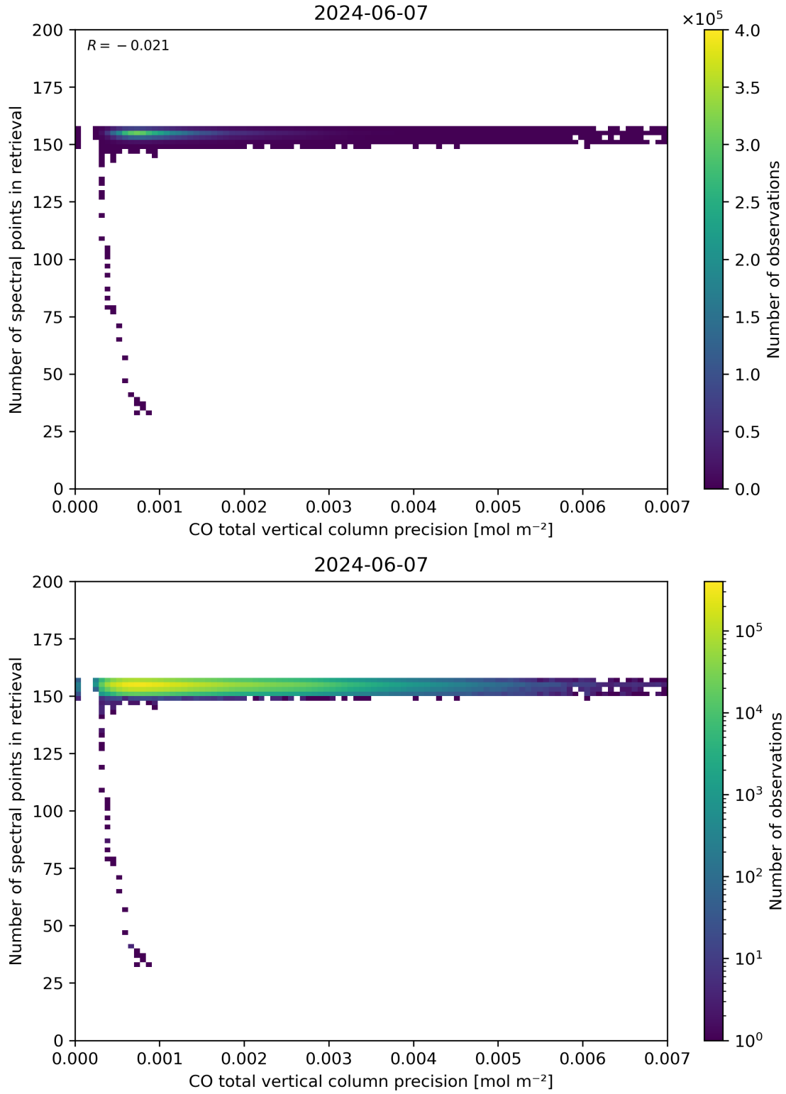
Figure 47: Scatter density plot of “CO total vertical column precision” against “Number of spectral points in retrieval” for 2024-06-06 to 2024-06-08.
