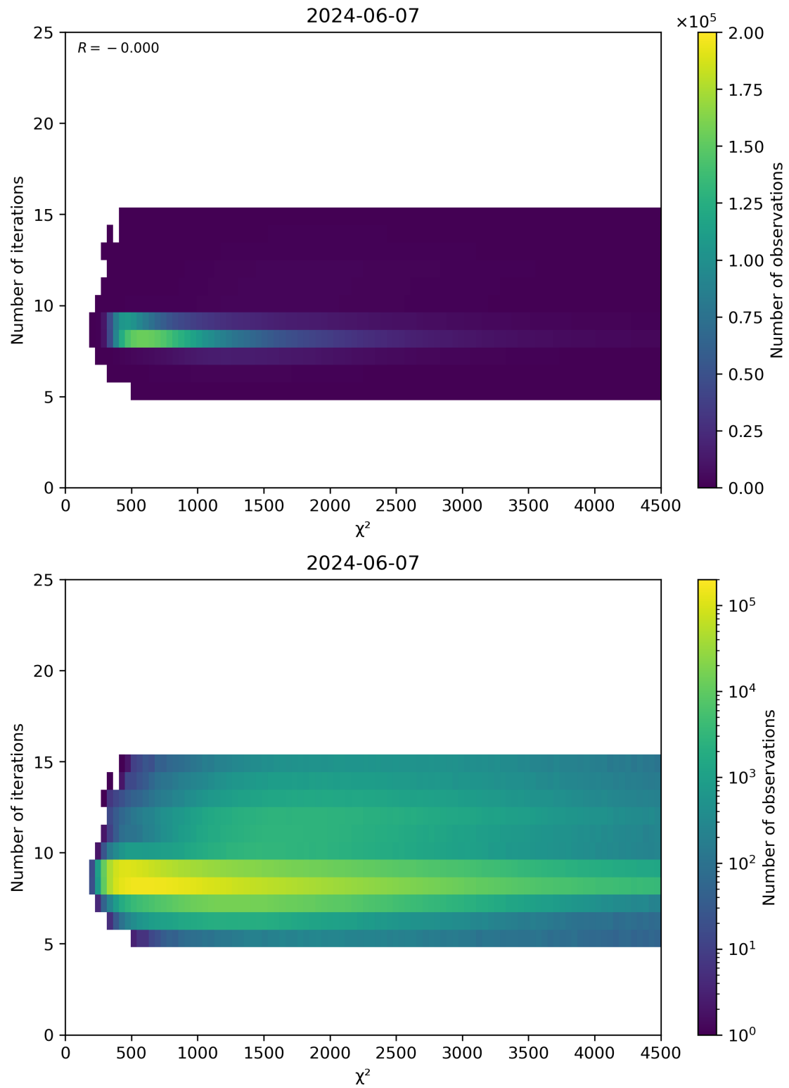
Figure 49: Scatter density plot of “ \chi^2 ” against “Number of iterations” for 2024-06-06 to 2024-06-08.
