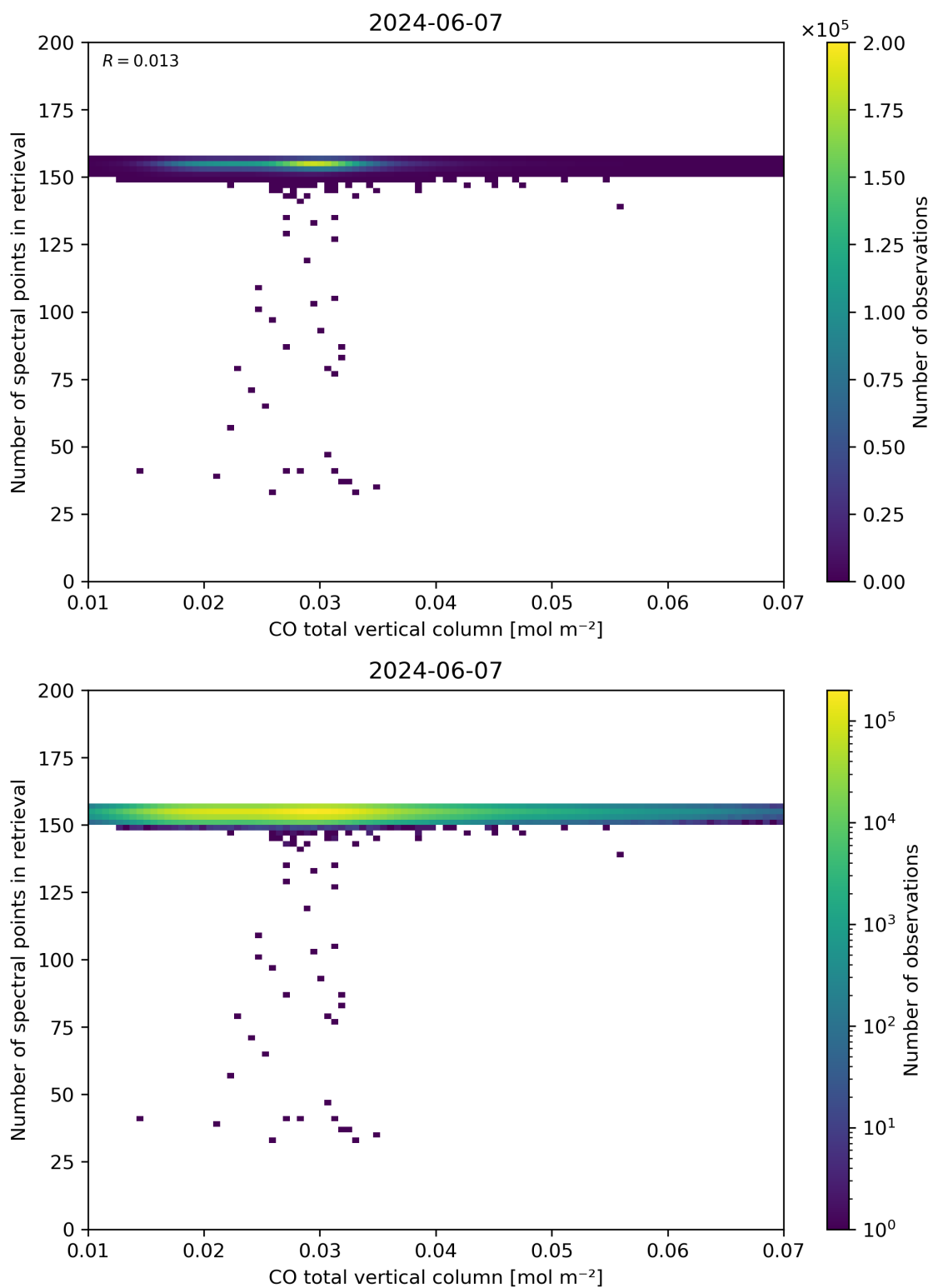
Figure 43: Scatter density plot of “CO total vertical column” against “Number of spectral points in retrieval” for 2024-06-06 to 2024-06-08.
