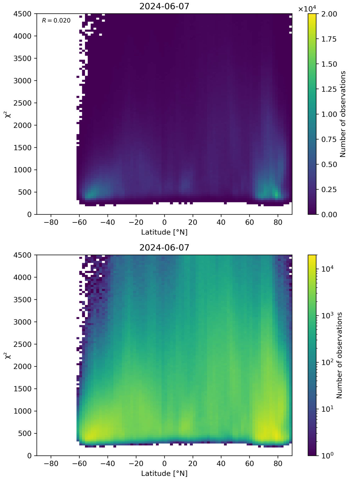
Figure 54: Scatter density plot of “Latitude” against “ \chi^2 ” for 2024-06-06 to 2024-06-08.
