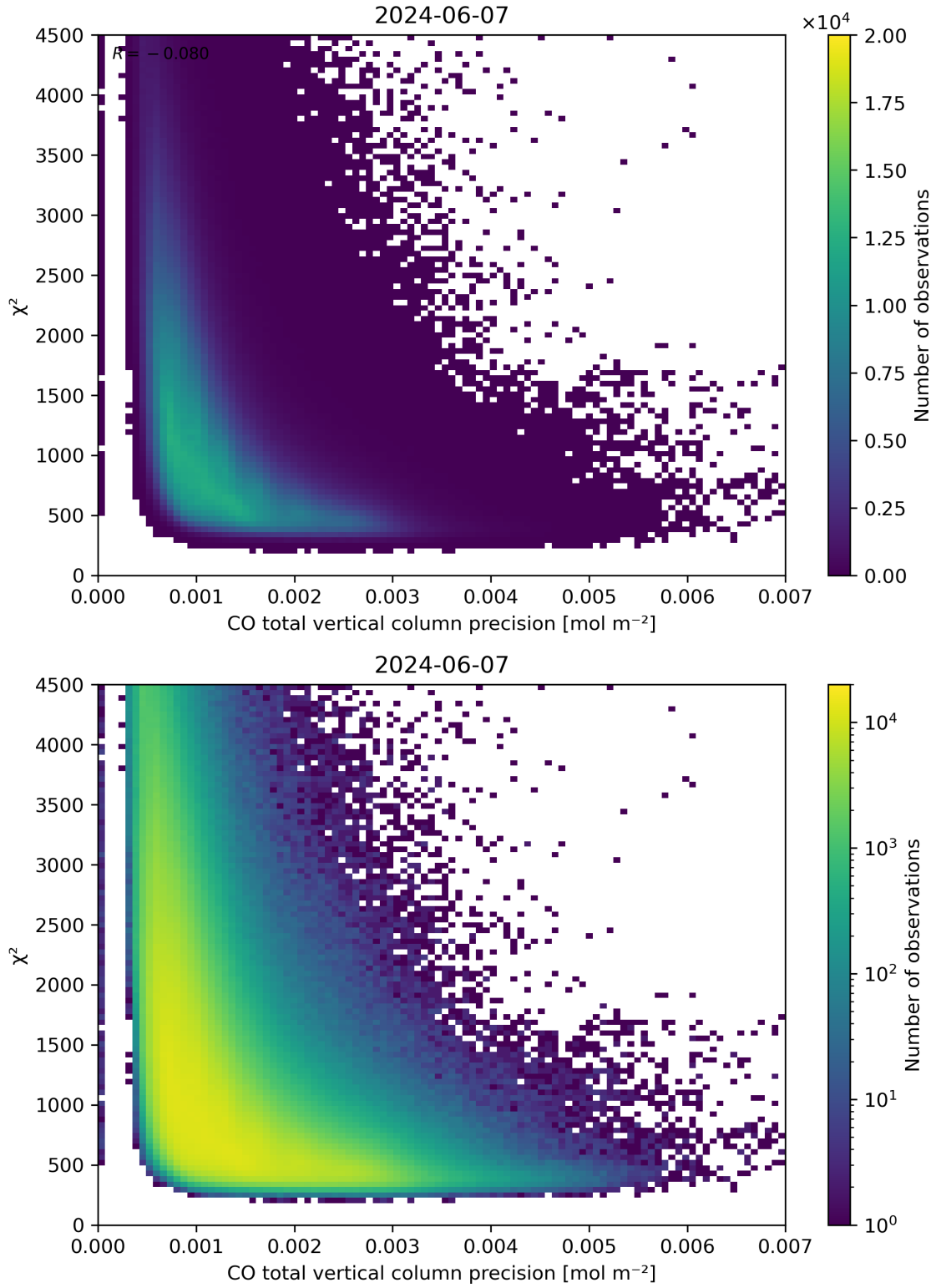
Figure 44: Scatter density plot of “CO total vertical column precision” against “ \chi^2 ” for 2024-06-06 to 2024-06-08.
