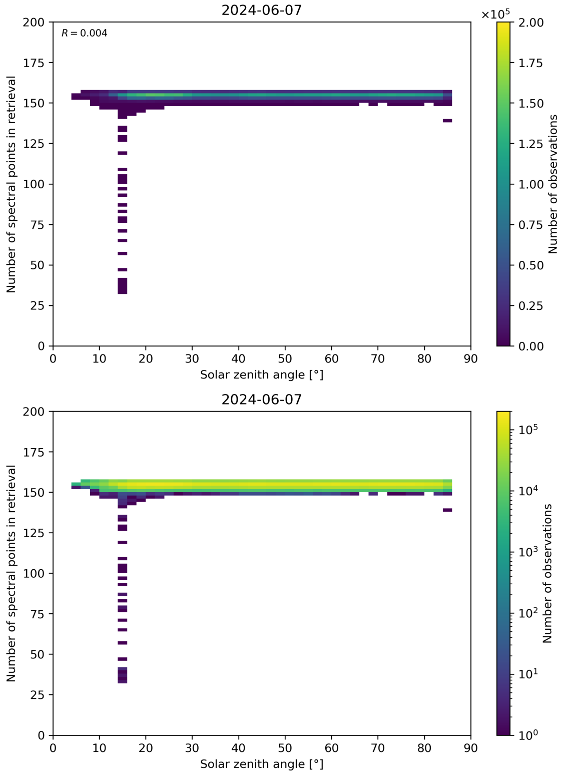
Figure 68: Scatter density plot of “Solar zenith angle” against “Number of spectral points in retrieval” for 2024-06-06 to 2024-06-08.
