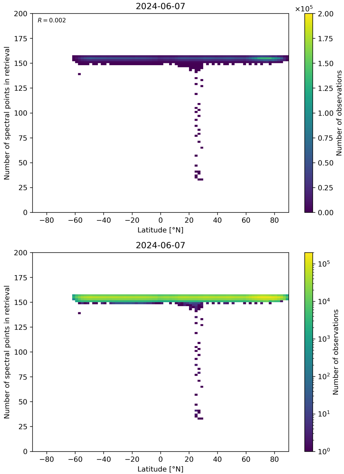
Figure 57: Scatter density plot of “Latitude” against “Number of spectral points in retrieval” for 2024-06-06 to 2024-06-08.
