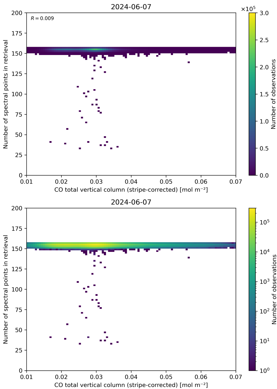
Figure 40: Scatter density plot of “CO total vertical column (stripe-corrected)” against “Number of spectral points in retrieval” for 2024-06-06 to 2024-06-08.
