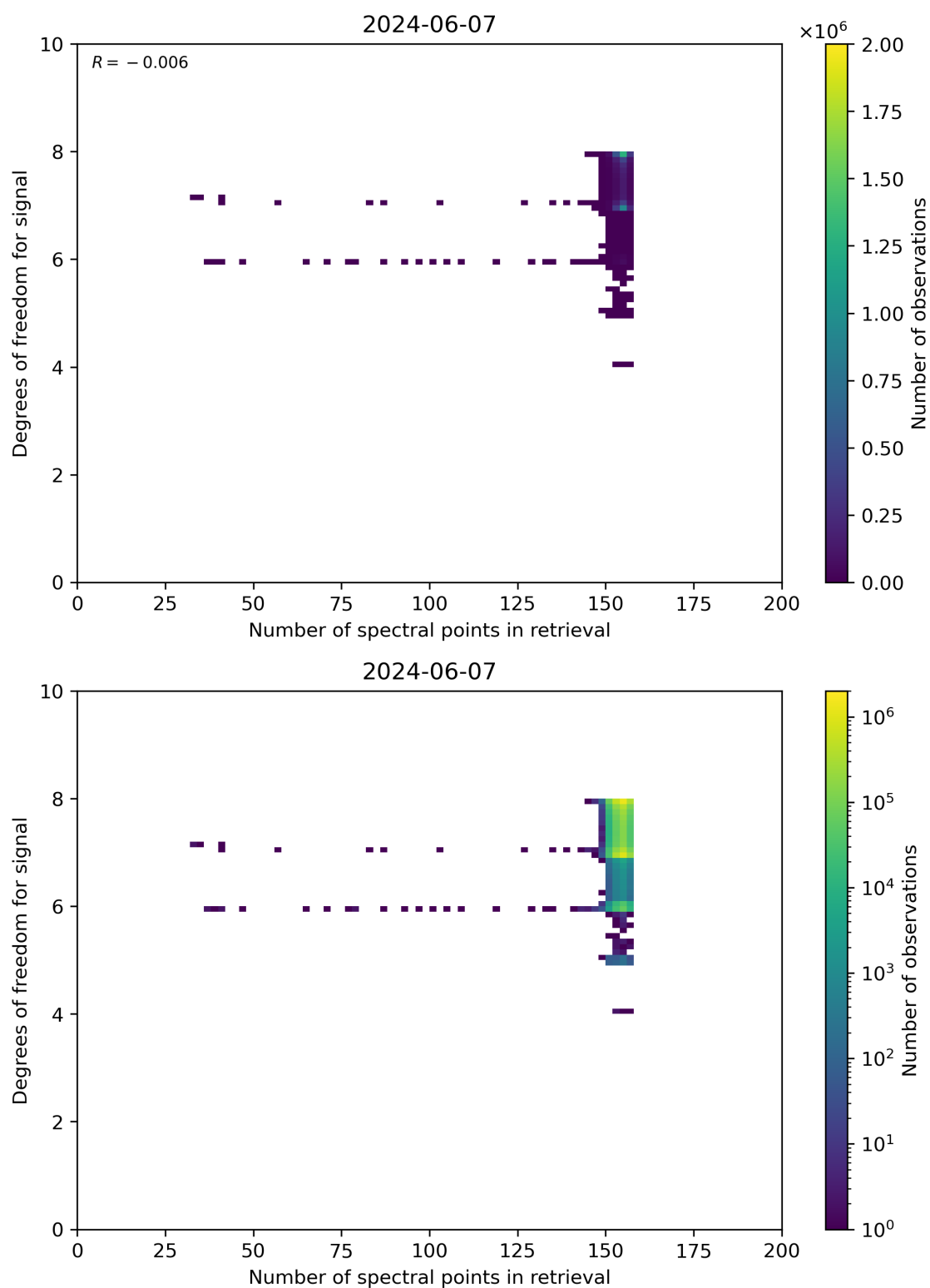
Figure 59: Scatter density plot of “Number of spectral points in retrieval” against “Degrees of freedom for signal” for 2024-06-06 to 2024-06-08.
