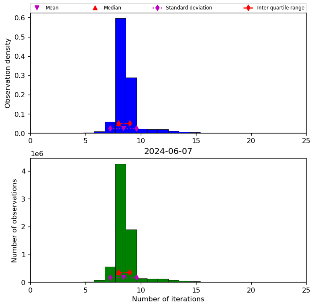
Figure 24: Histogram of “Number of iterations” for 2024-06-06 to 2024-06-08
