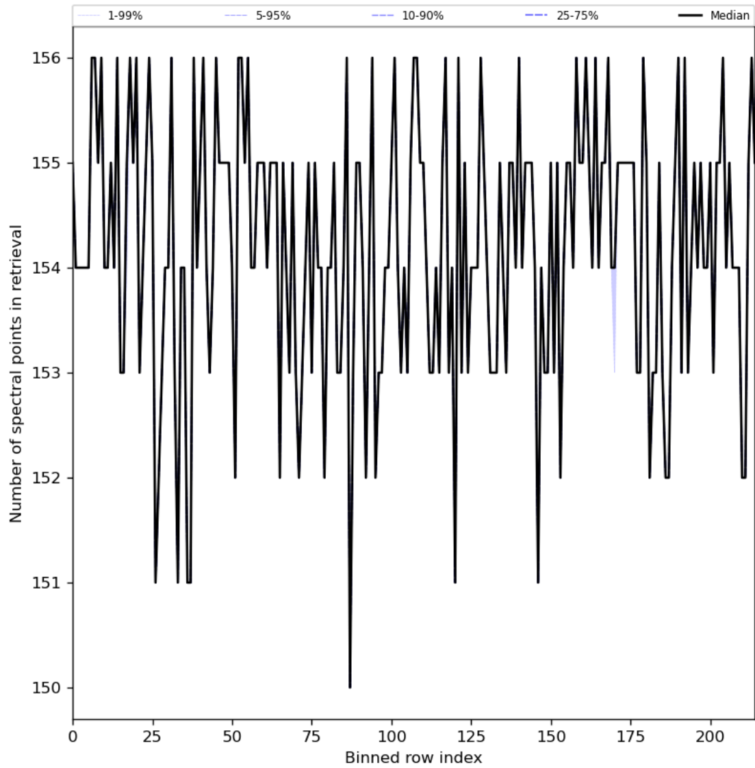
Figure 29: Along track statistics of “Number of spectral points in retrieval” for 2024-06-08 to 2024-06-10
