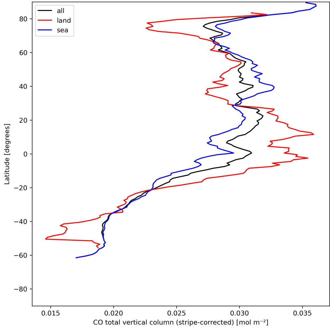
Figure 11: Zonal average of “CO total vertical column (stripe-corrected)” for 2024-06-08 to 2024-06-10.
