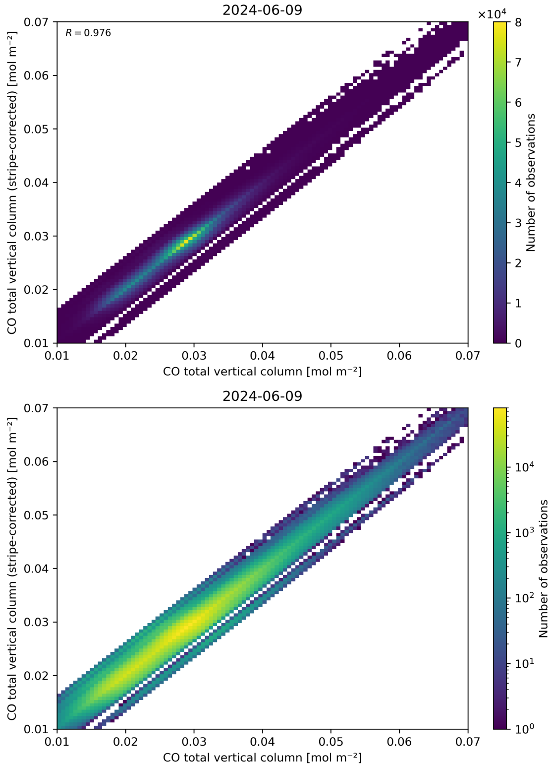
Figure 33: Scatter density plot of “CO total vertical column” against “CO total vertical column (stripe-corrected)” for 2024-06-08 to 2024-06-10.
