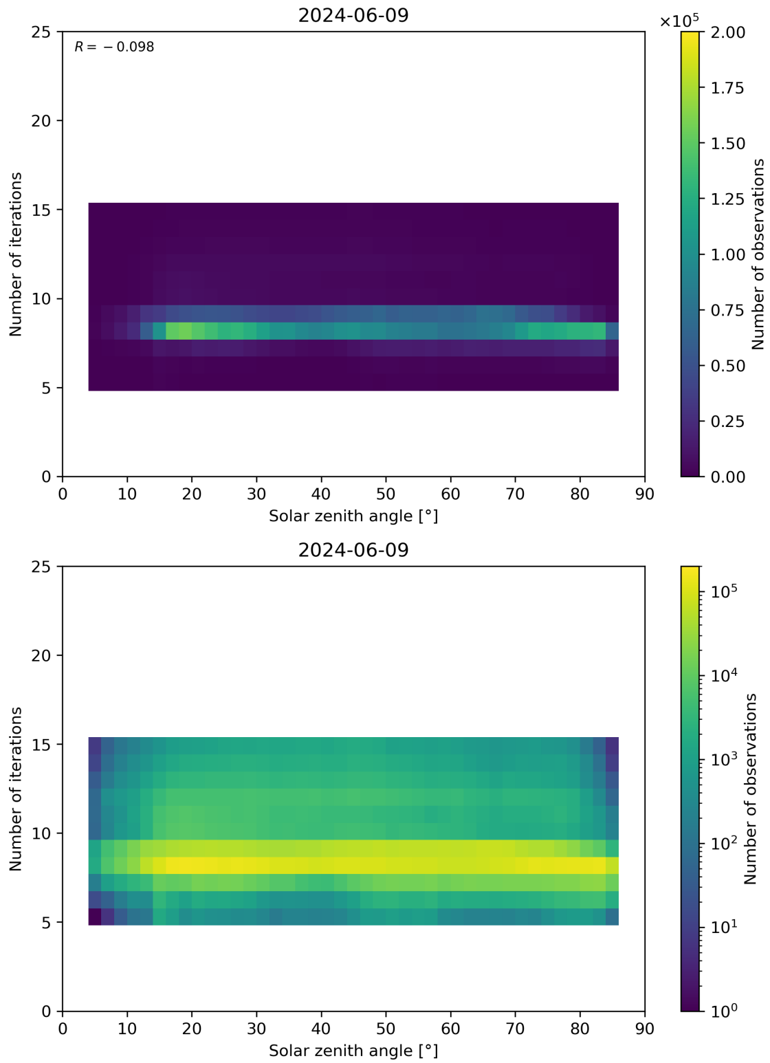
Figure 67: Scatter density plot of “Solar zenith angle” against “Number of iterations” for 2024-06-08 to 2024-06-10.
