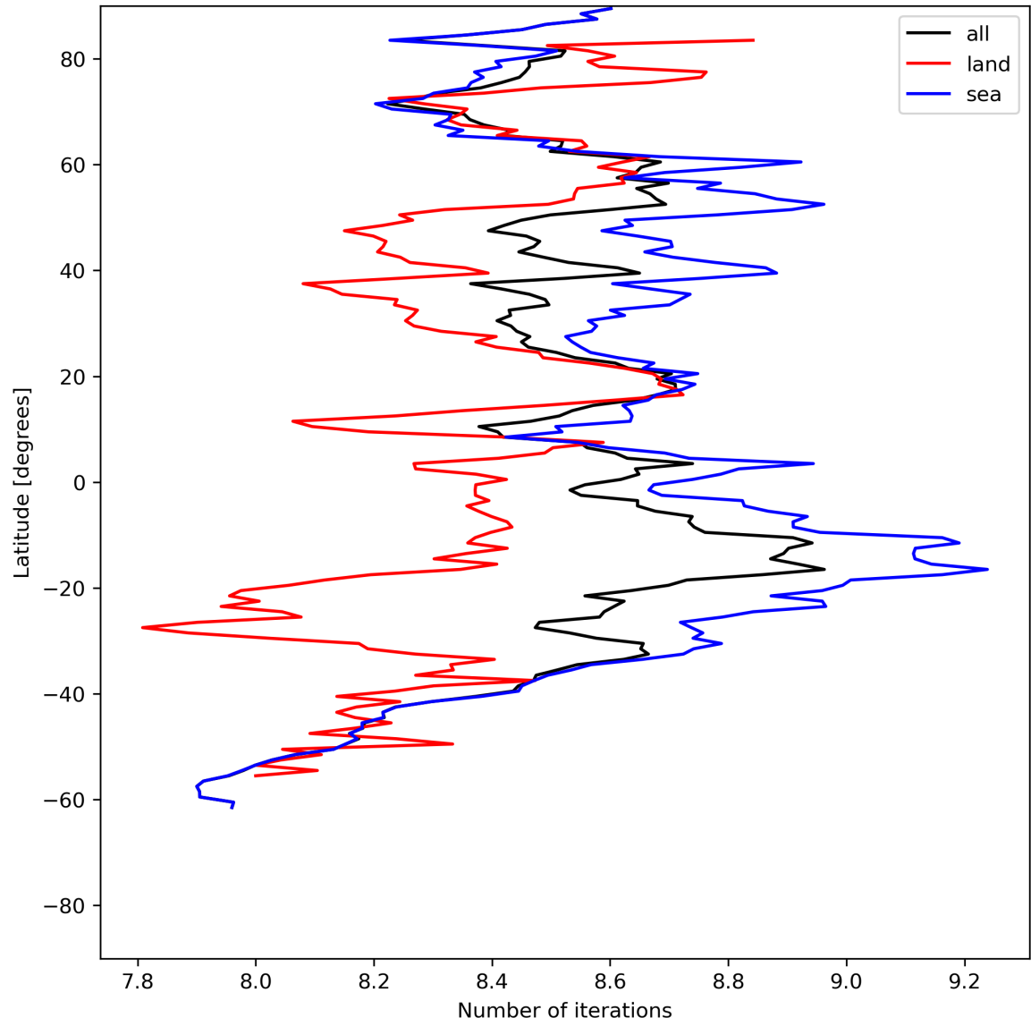
Figure 16: Zonal average of “Number of iterations” for 2024-06-08 to 2024-06-10.
