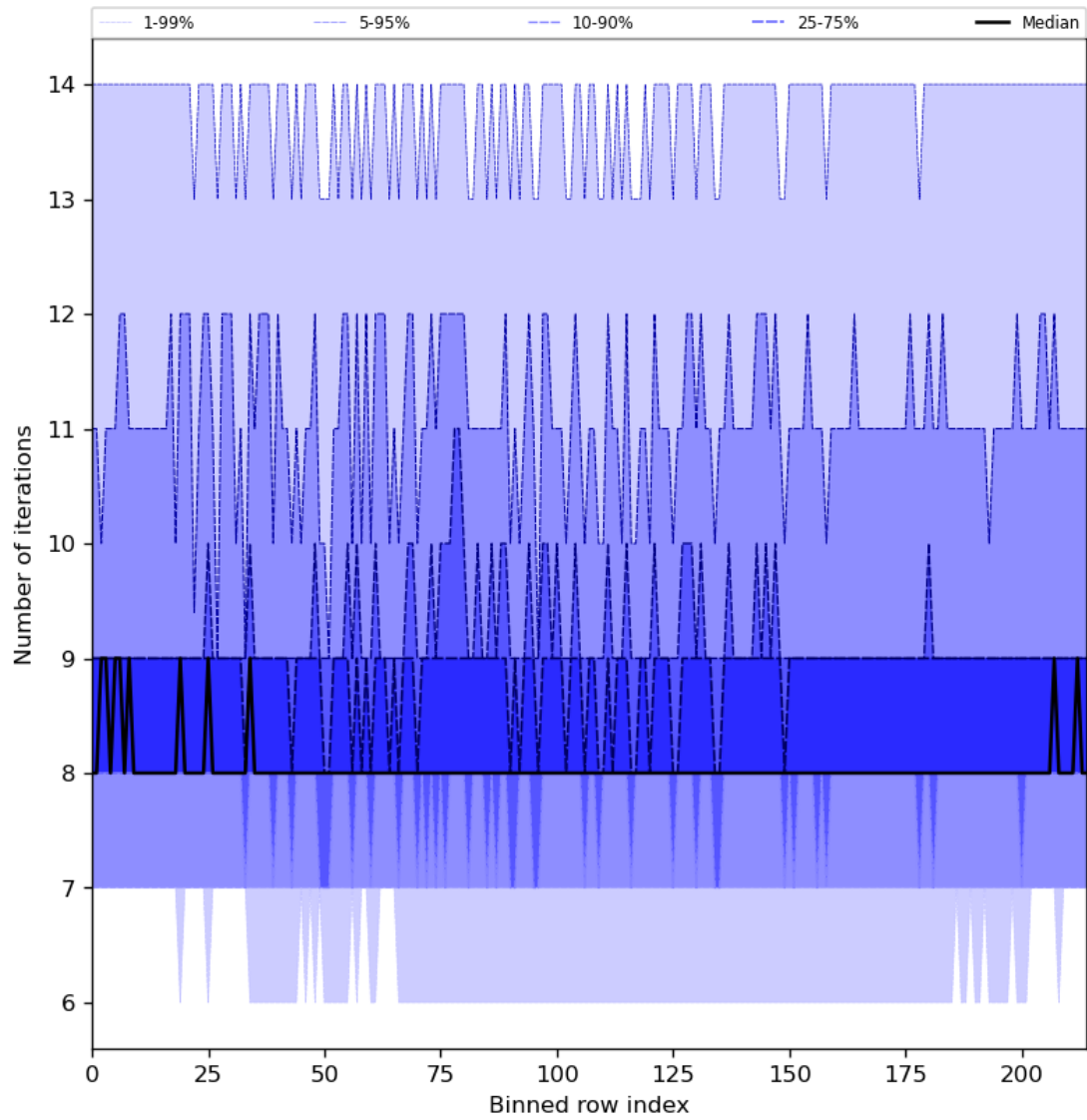
Figure 32: Along track statistics of “Number of iterations” for 2024-06-08 to 2024-06-10
