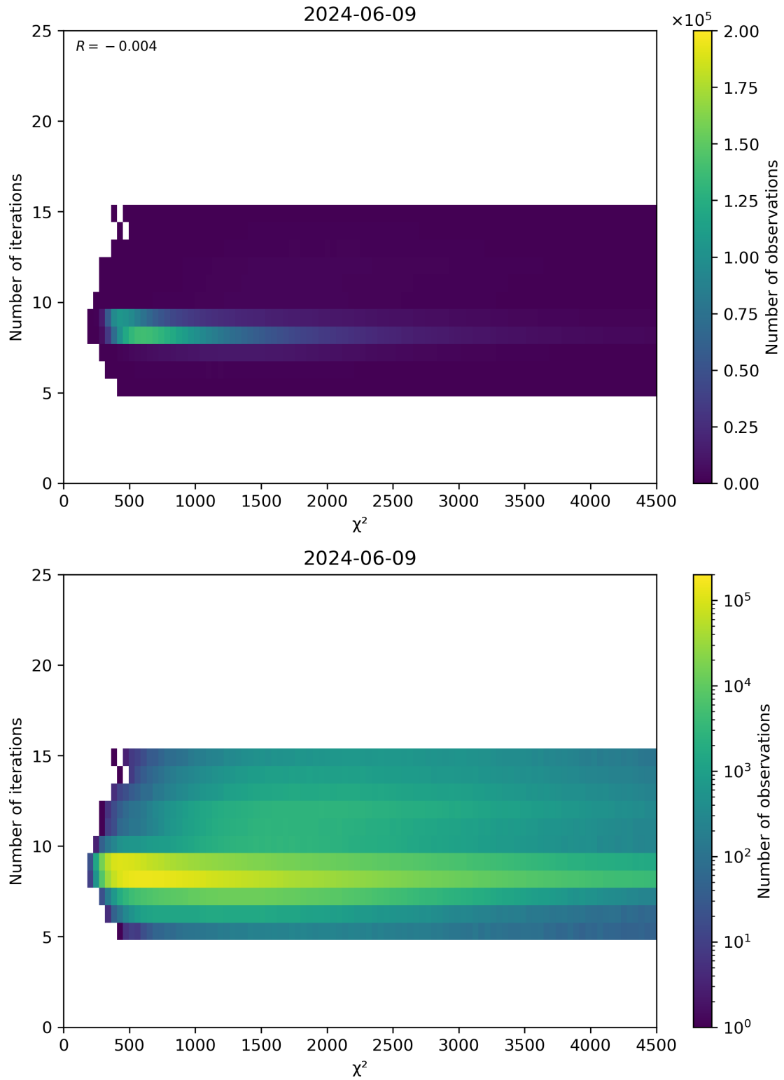
Figure 49: Scatter density plot of “ \chi^2 ” against “Number of iterations” for 2024-06-08 to 2024-06-10.
