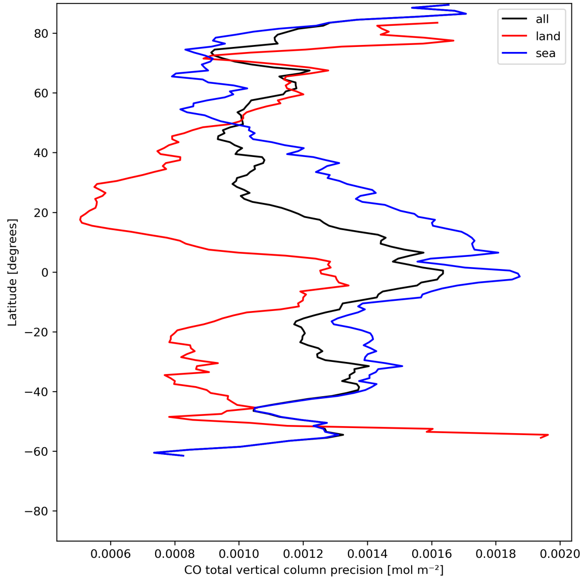
Figure 12: Zonal average of “CO total vertical column precision” for 2024-06-08 to 2024-06-10.
