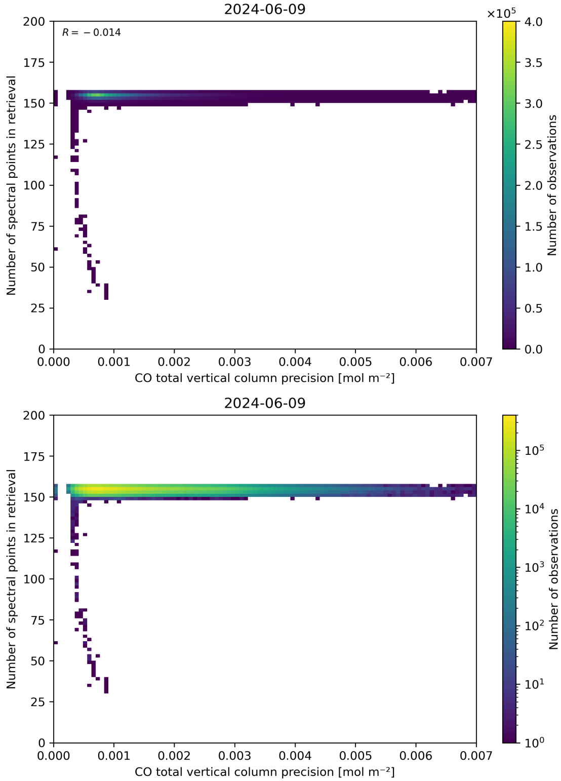
Figure 47: Scatter density plot of “CO total vertical column precision” against “Number of spectral points in retrieval” for 2024-06-08 to 2024-06-10.
