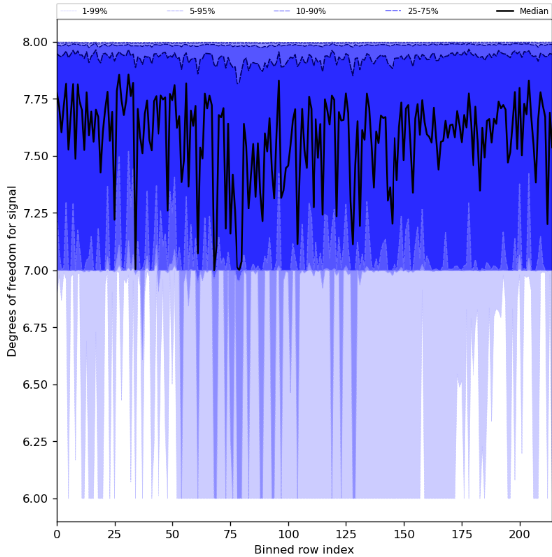
Figure 31: Along track statistics of “Degrees of freedom for signal” for 2024-06-08 to 2024-06-10
