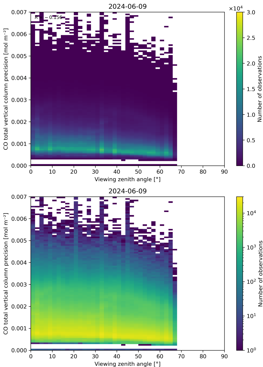
Figure 71: Scatter density plot of “Viewing zenith angle” against “CO total vertical column precision” for 2024-06-08 to 2024-06-10.
