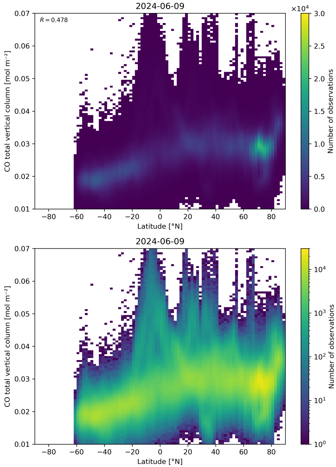
Figure 51: Scatter density plot of “Latitude” against “CO total vertical column” for 2024-06-08 to 2024-06-10.
