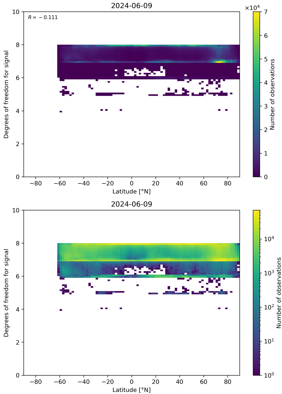
Figure 55: Scatter density plot of “Latitude” against “Degrees of freedom for signal” for 2024-06-08 to 2024-06-10.
