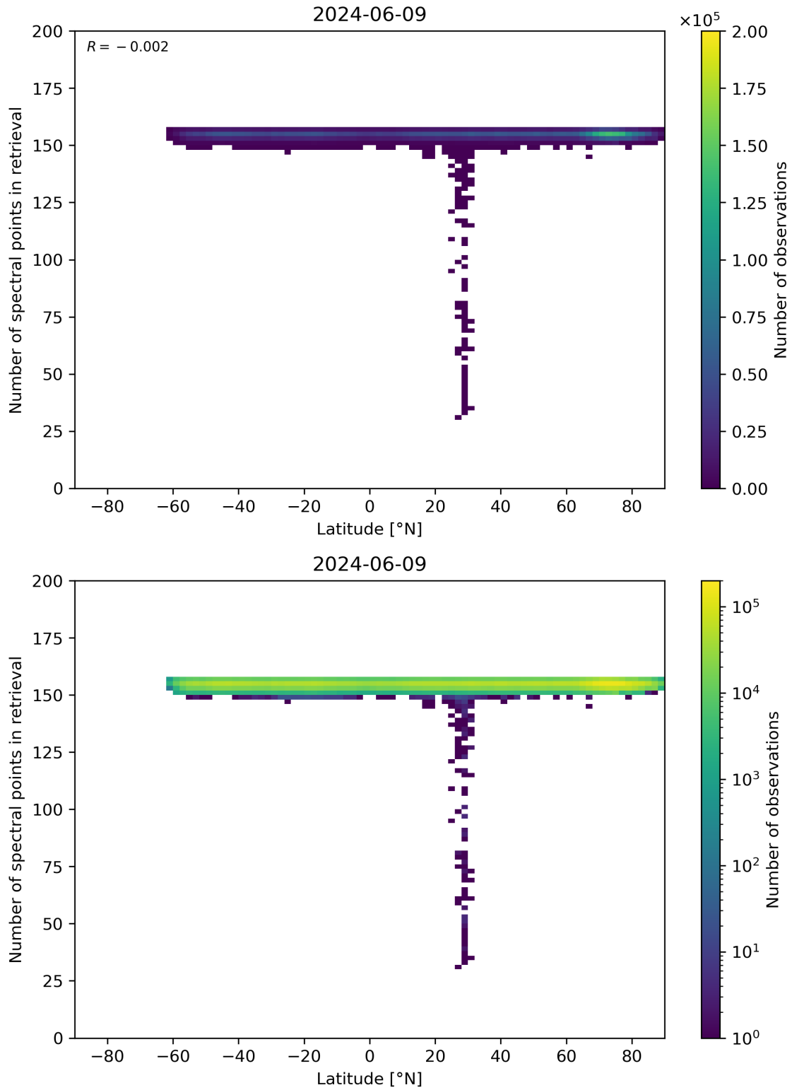
Figure 57: Scatter density plot of “Latitude” against “Number of spectral points in retrieval” for 2024-06-08 to 2024-06-10.
