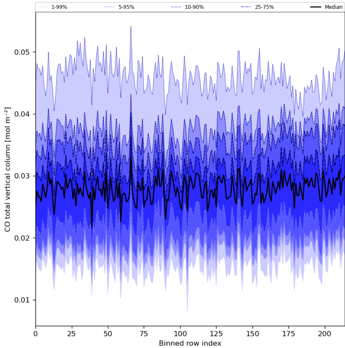
Figure 26: Along track statistics of “CO total vertical column” for 2024-06-08 to 2024-06-10
