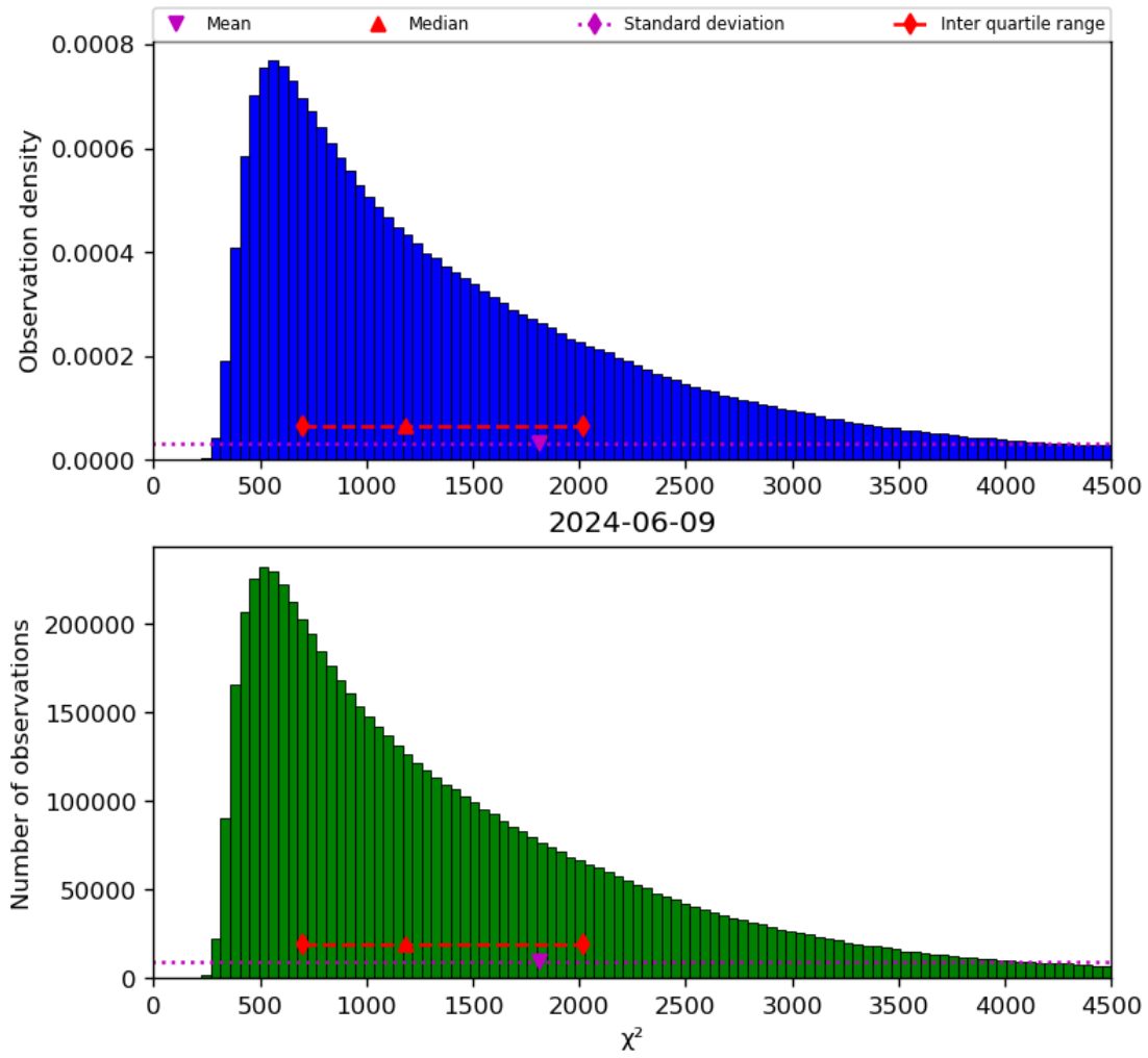
Figure 22: Histogram of “ \chi^2 ” for 2024-06-08 to 2024-06-10
