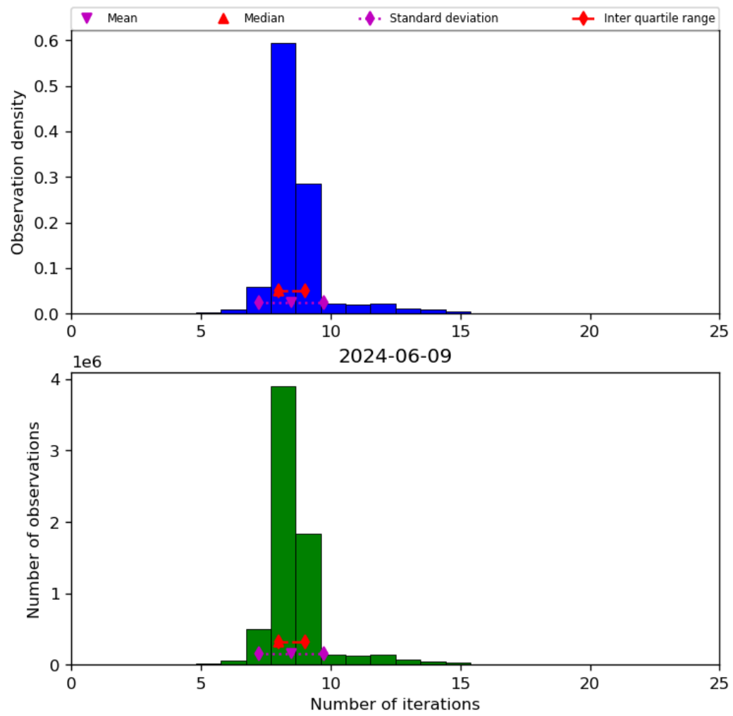
Figure 24: Histogram of “Number of iterations” for 2024-06-08 to 2024-06-10
