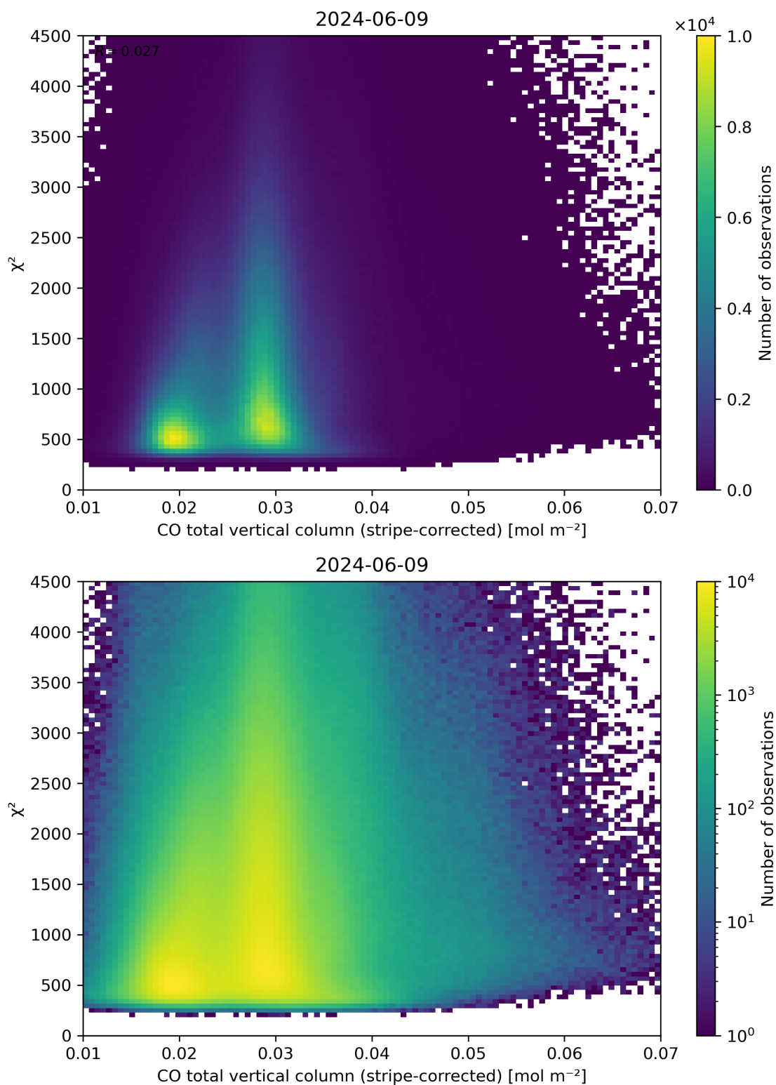
Figure 37: Scatter density plot of “CO total vertical column (stripe-corrected)” against “ \chi^2 ” for 2024-06-08 to 2024-06-10.
