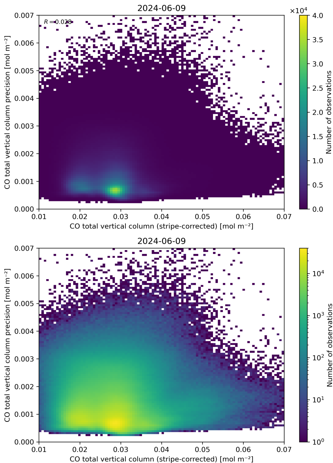
Figure 36: Scatter density plot of “CO total vertical column (stripe-corrected)” against “CO total vertical column precision” for 2024-06-08 to 2024-06-10.
