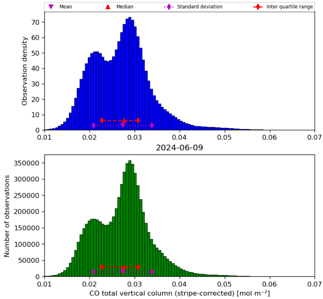
Figure 19: Histogram of “CO total vertical column (stripe-corrected)” for 2024-06-08 to 2024-06-10
