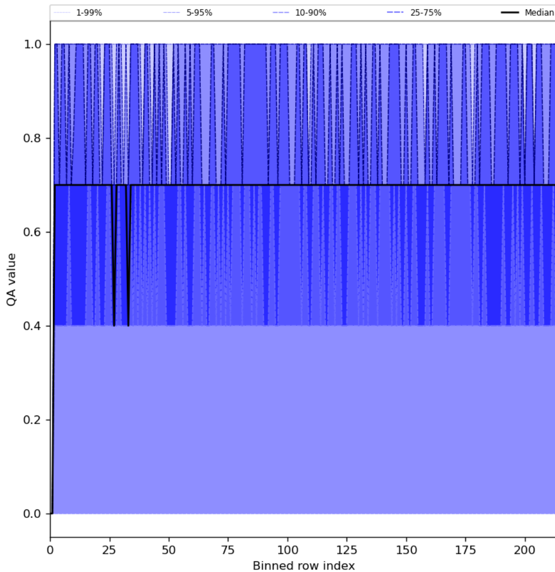
Figure 25: Along track statistics of “QA value” for 2024-06-08 to 2024-06-10
