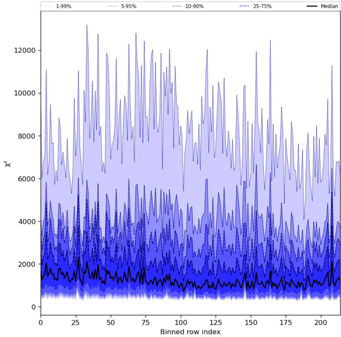
Figure 30: Along track statistics of “ \chi^2 ” for 2024-06-08 to 2024-06-10
