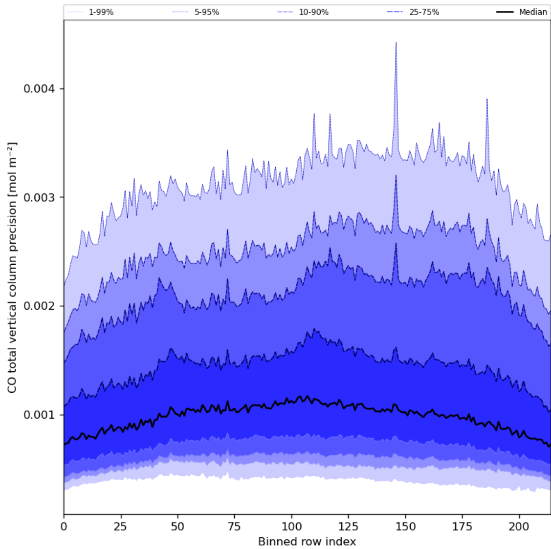
Figure 28: Along track statistics of “CO total vertical column precision” for 2024-06-08 to 2024-06-10
