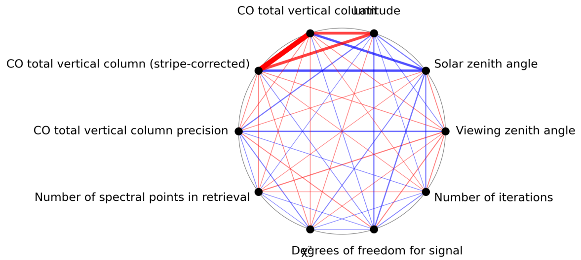
Figure 1: Map of correlation graph for 2024-06-08 to 2024-06-10.
