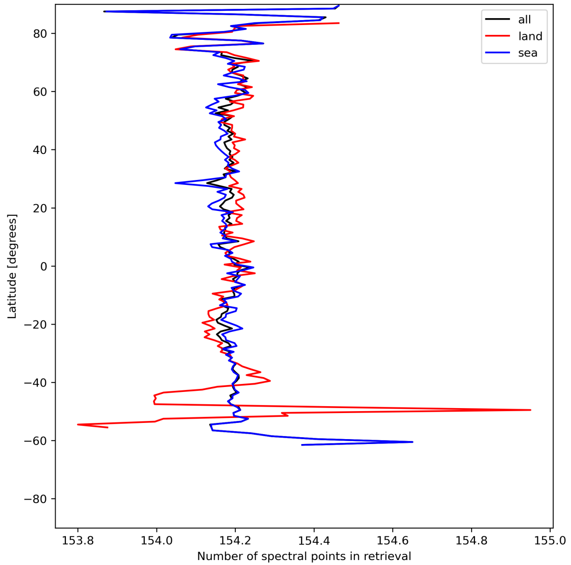
Figure 13: Zonal average of “Number of spectral points in retrieval” for 2024-06-08 to 2024-06-10.
