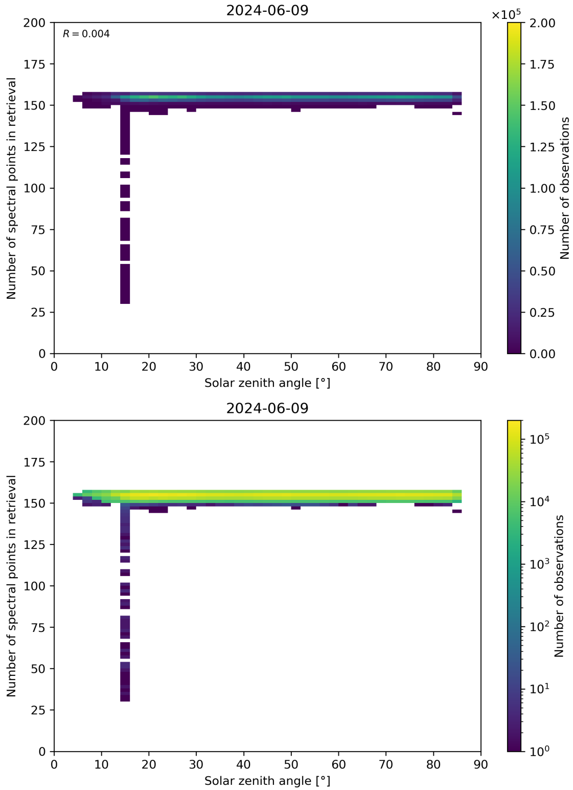
Figure 68: Scatter density plot of “Solar zenith angle” against “Number of spectral points in retrieval” for 2024-06-08 to 2024-06-10.
