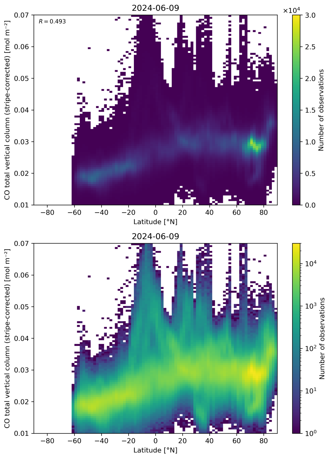
Figure 52: Scatter density plot of “Latitude” against “CO total vertical column (stripe-corrected)” for 2024-06-08 to 2024-06-10.
