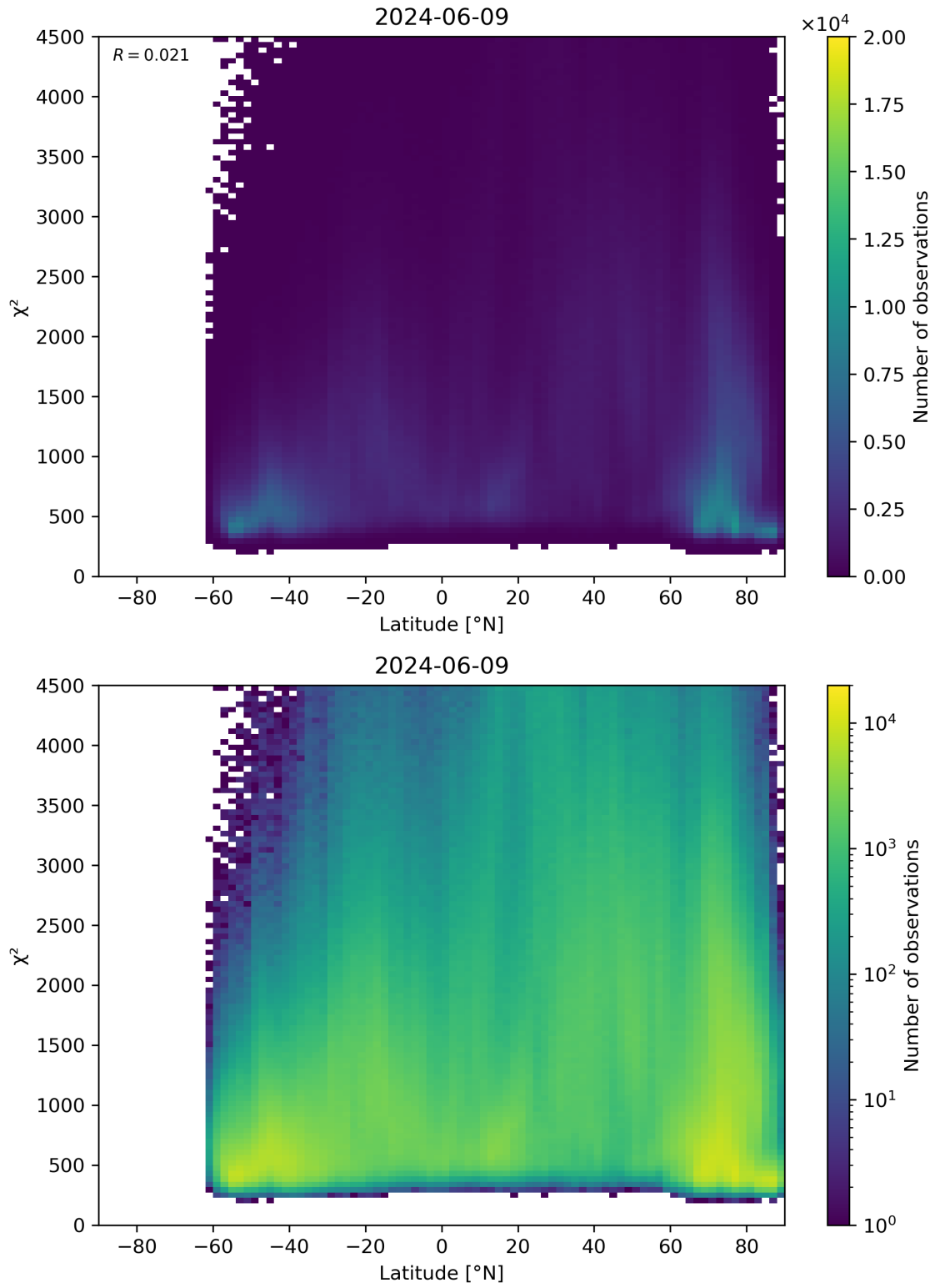
Figure 54: Scatter density plot of “Latitude” against “ \chi^2 ” for 2024-06-08 to 2024-06-10.
