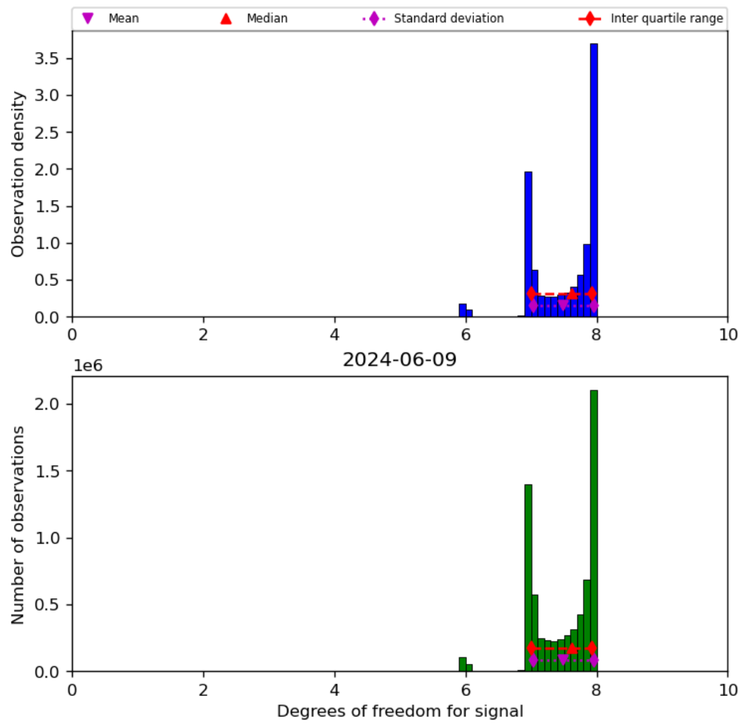
Figure 23: Histogram of “Degrees of freedom for signal” for 2024-06-08 to 2024-06-10
