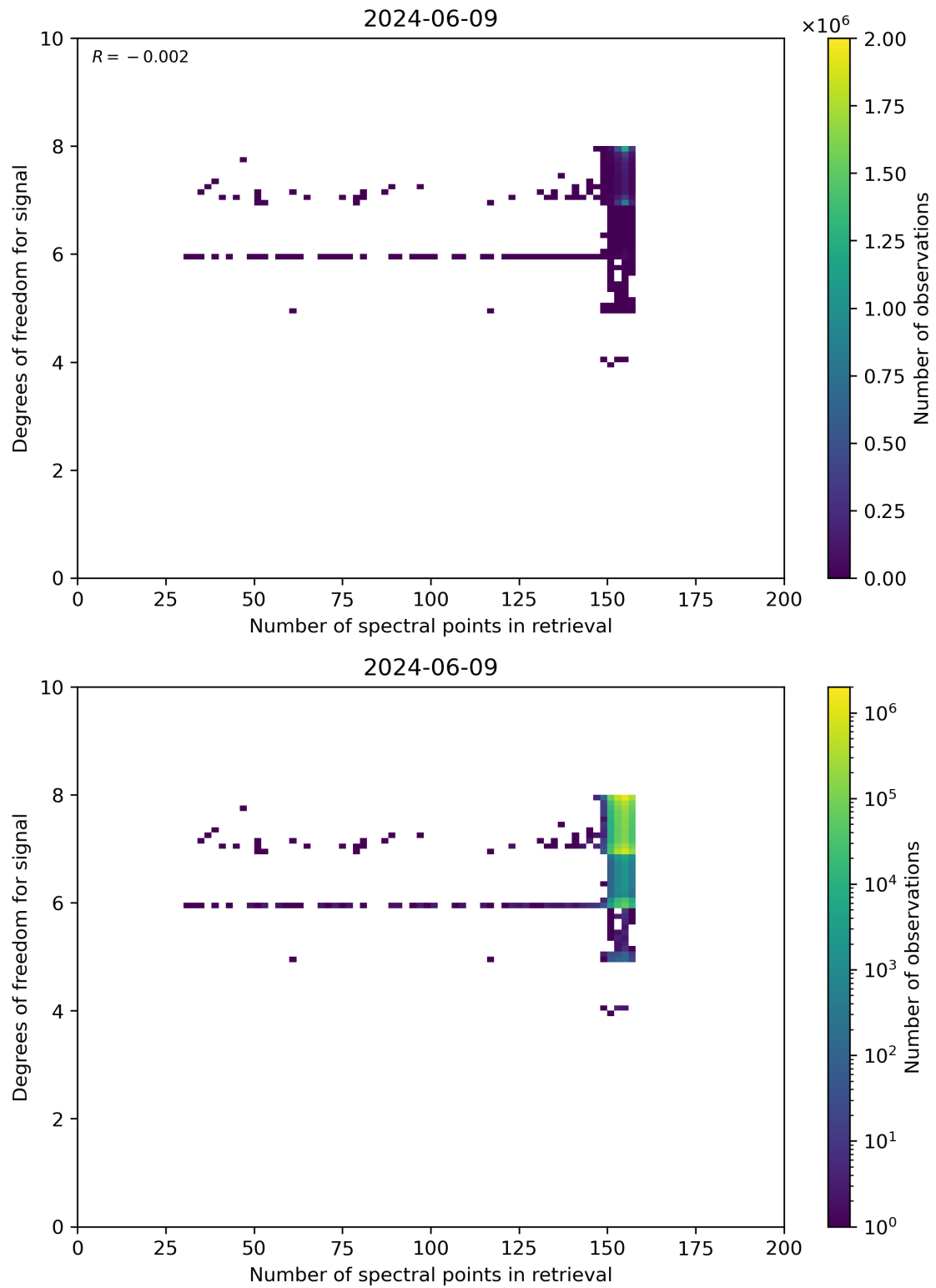
Figure 59: Scatter density plot of “Number of spectral points in retrieval” against “Degrees of freedom for signal” for 2024-06-08 to 2024-06-10.
