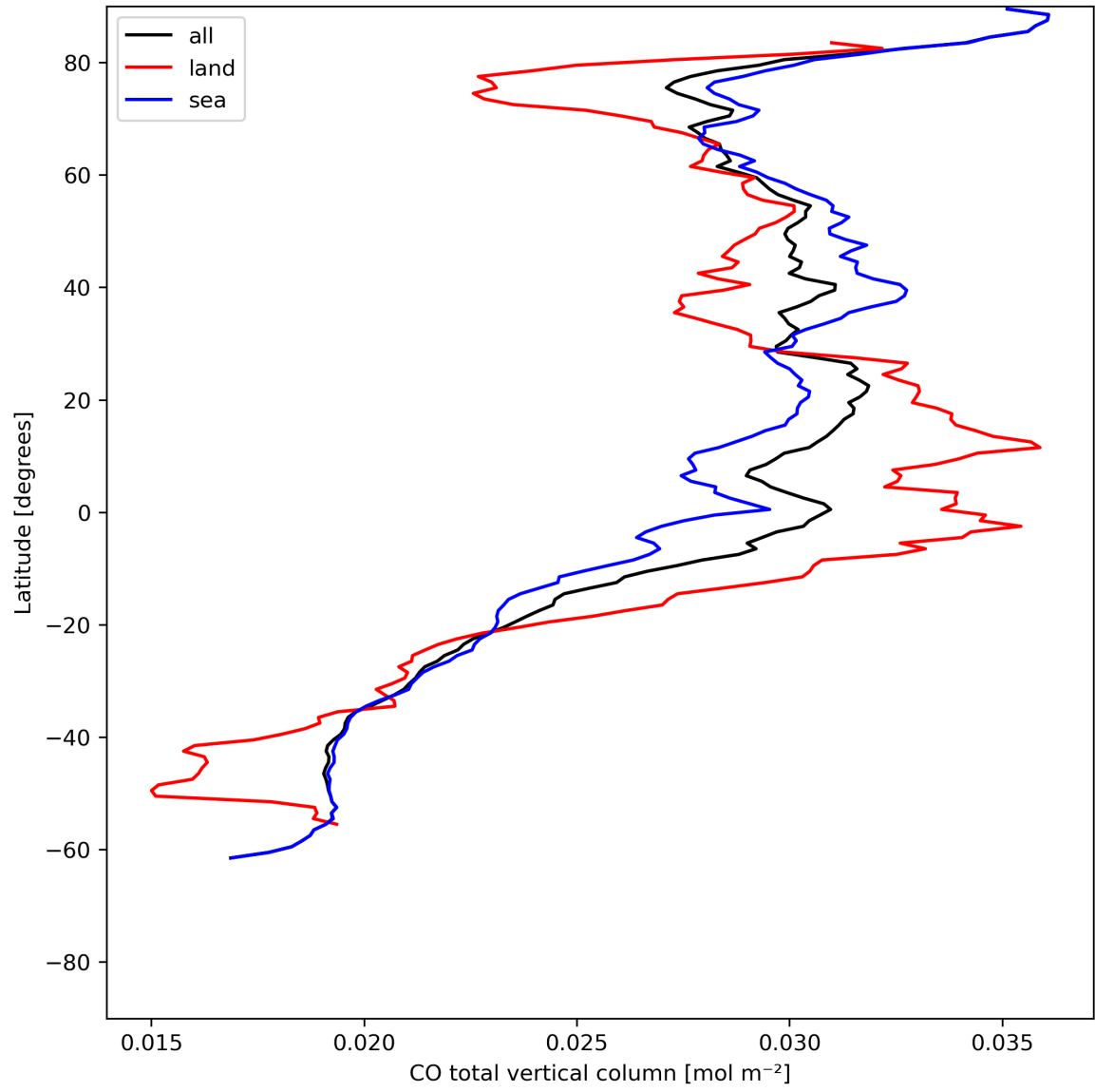
Figure 10: Zonal average of “CO total vertical column” for 2024-06-08 to 2024-06-10.
