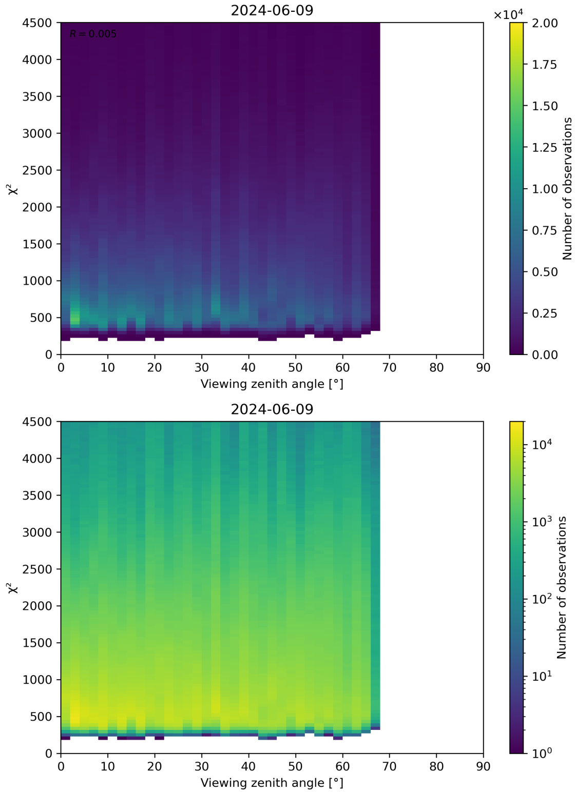
Figure 72: Scatter density plot of “Viewing zenith angle” against “ \chi^2 ” for 2024-06-08 to 2024-06-10.
