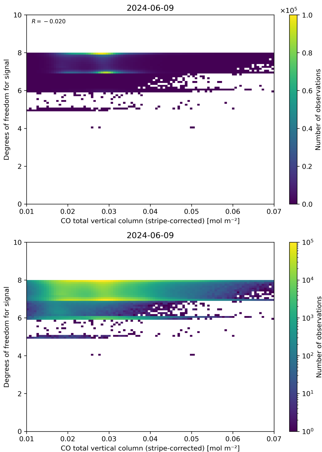
Figure 38: Scatter density plot of “CO total vertical column (stripe-corrected)” against “Degrees of freedom for signal” for 2024-06-08 to 2024-06-10.
