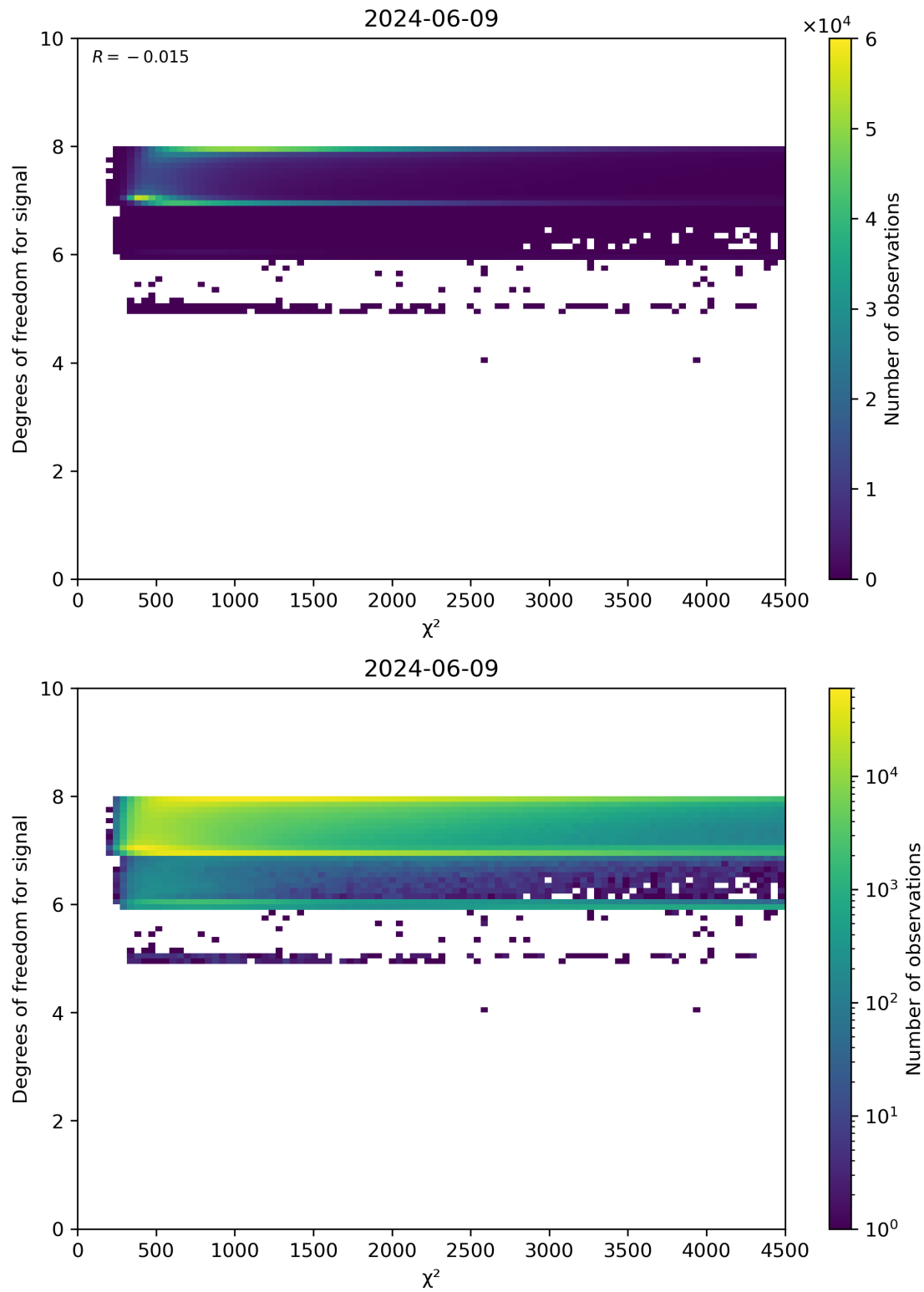
Figure 48: Scatter density plot of “ \chi^2 ” against “Degrees of freedom for signal” for 2024-06-08 to 2024-06-10.
