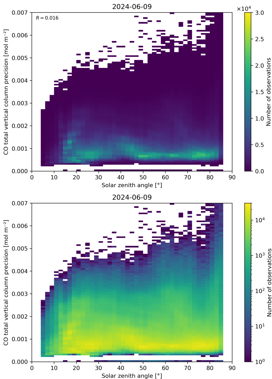
Figure 63: Scatter density plot of “Solar zenith angle” against “CO total vertical column precision” for 2024-06-08 to 2024-06-10.
