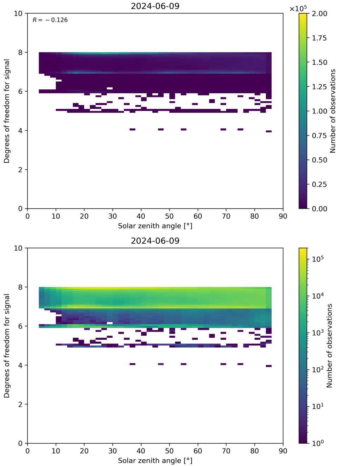
Figure 65: Scatter density plot of “Solar zenith angle” against “Degrees of freedom for signal” for 2024-06-08 to 2024-06-10.
