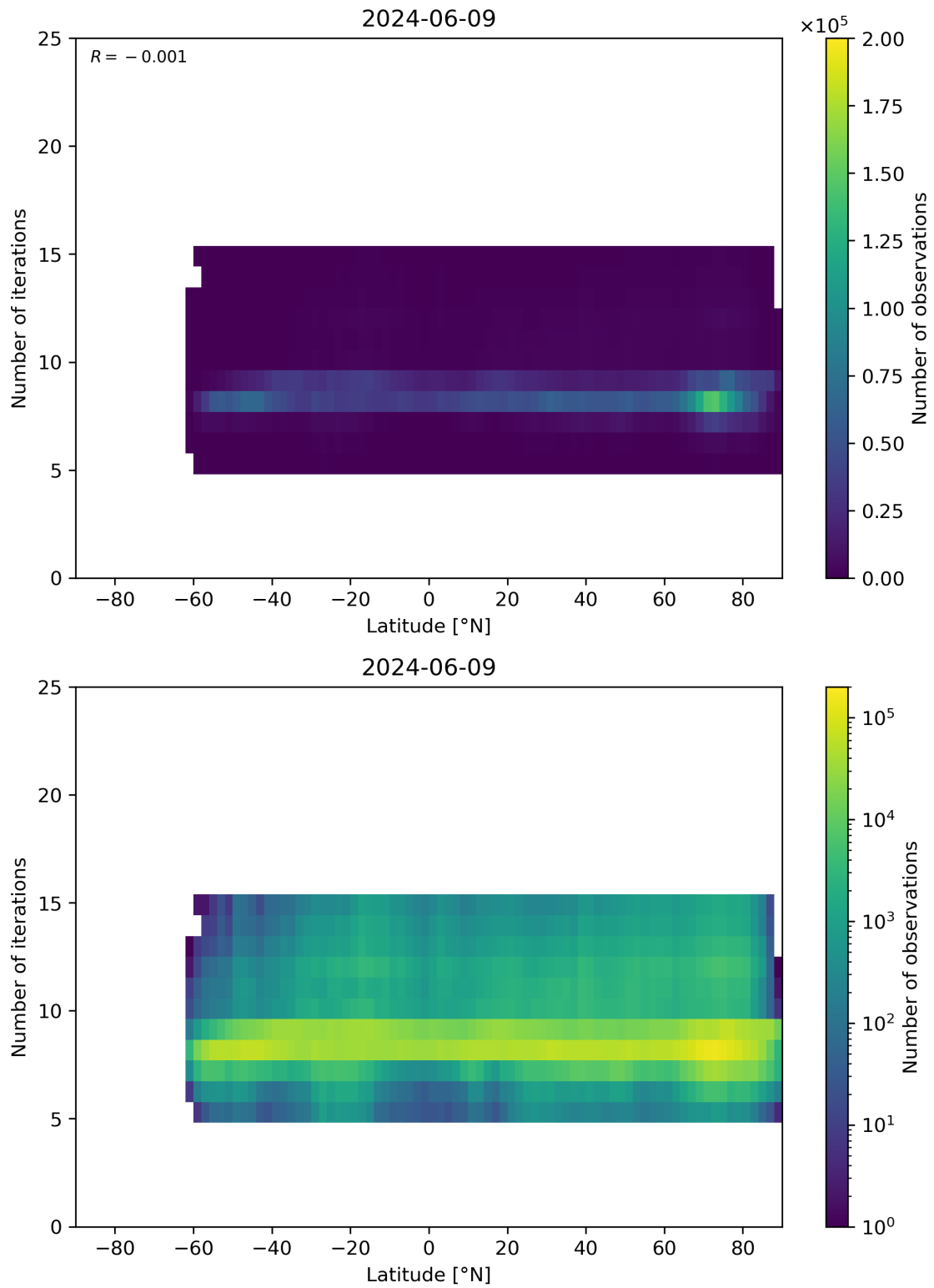
Figure 56: Scatter density plot of “Latitude” against “Number of iterations” for 2024-06-08 to 2024-06-10.
