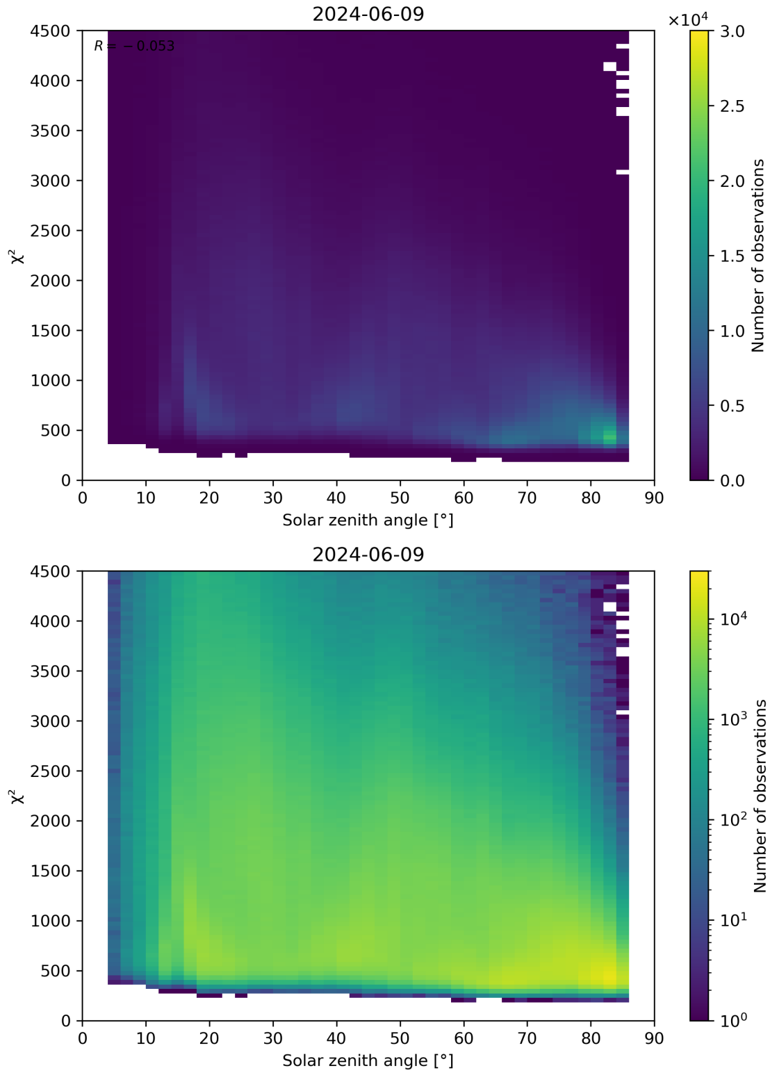
Figure 64: Scatter density plot of “Solar zenith angle” against “ \chi^2 ” for 2024-06-08 to 2024-06-10.
