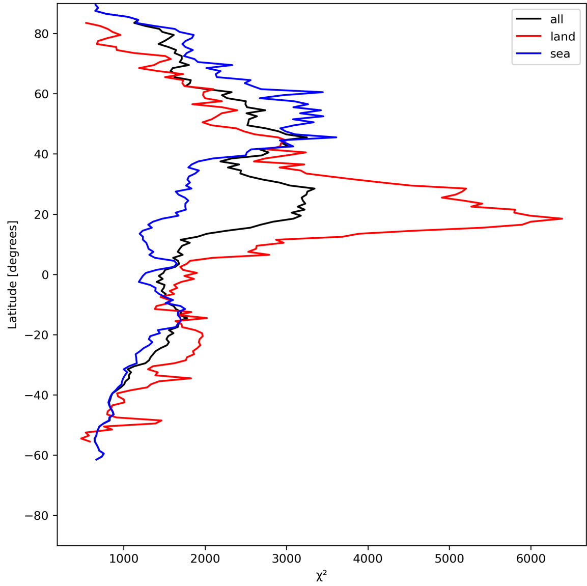
Figure 14: Zonal average of “ \chi^2 ” for 2024-06-08 to 2024-06-10.
