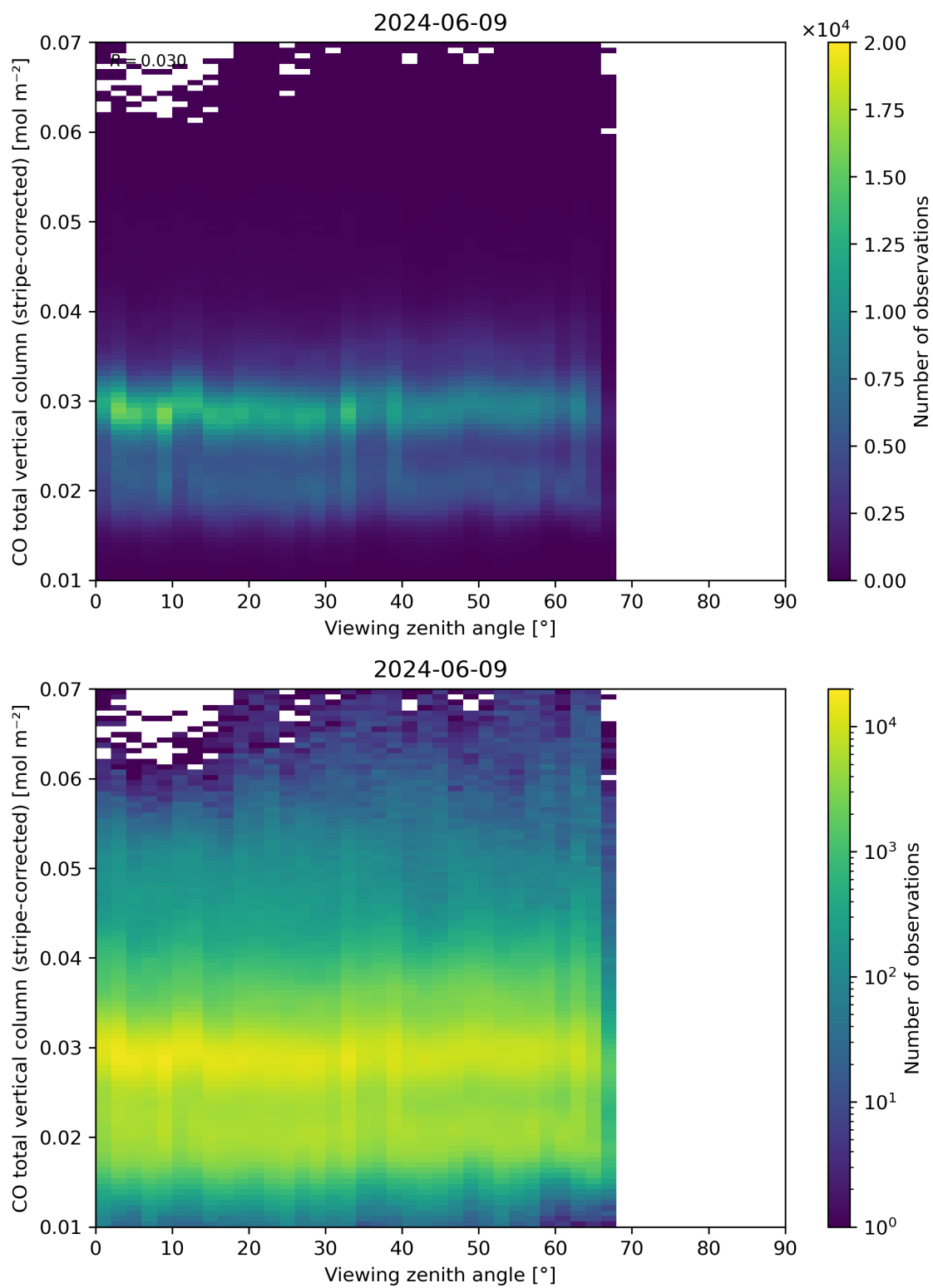
Figure 70: Scatter density plot of “Viewing zenith angle” against “CO total vertical column (stripe-corrected)” for 2024-06-08 to 2024-06-10.
