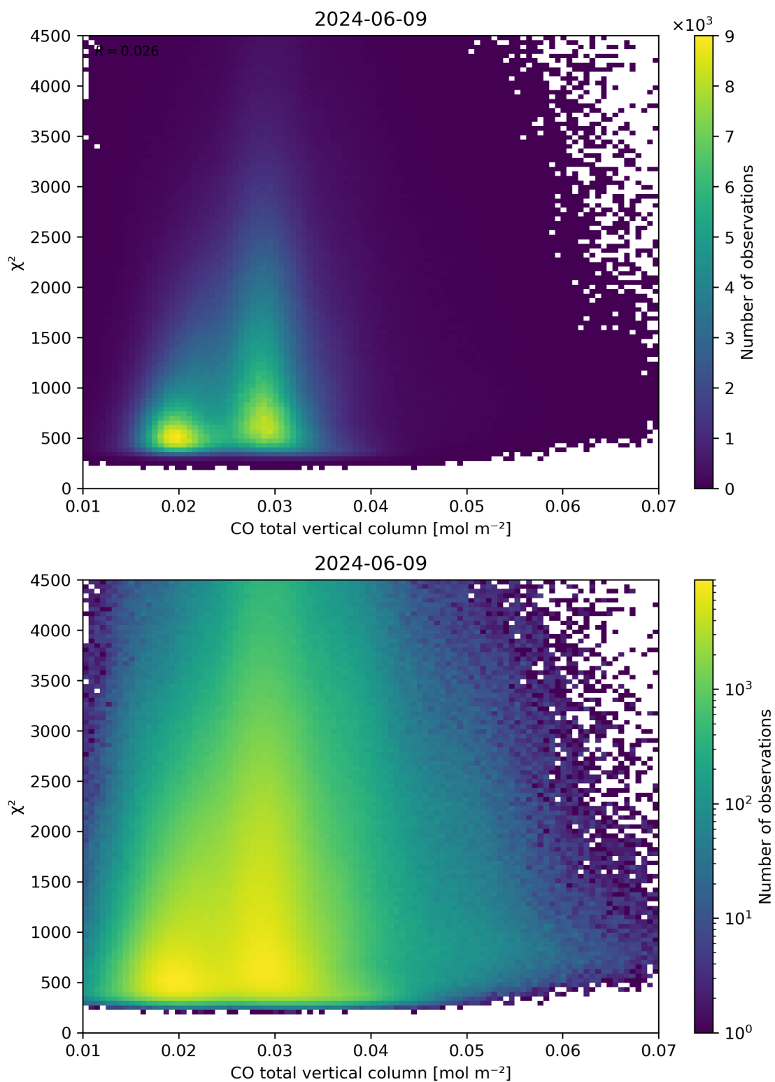
Figure 35: Scatter density plot of “CO total vertical column” against “ \chi^2 ” for 2024-06-08 to 2024-06-10.
