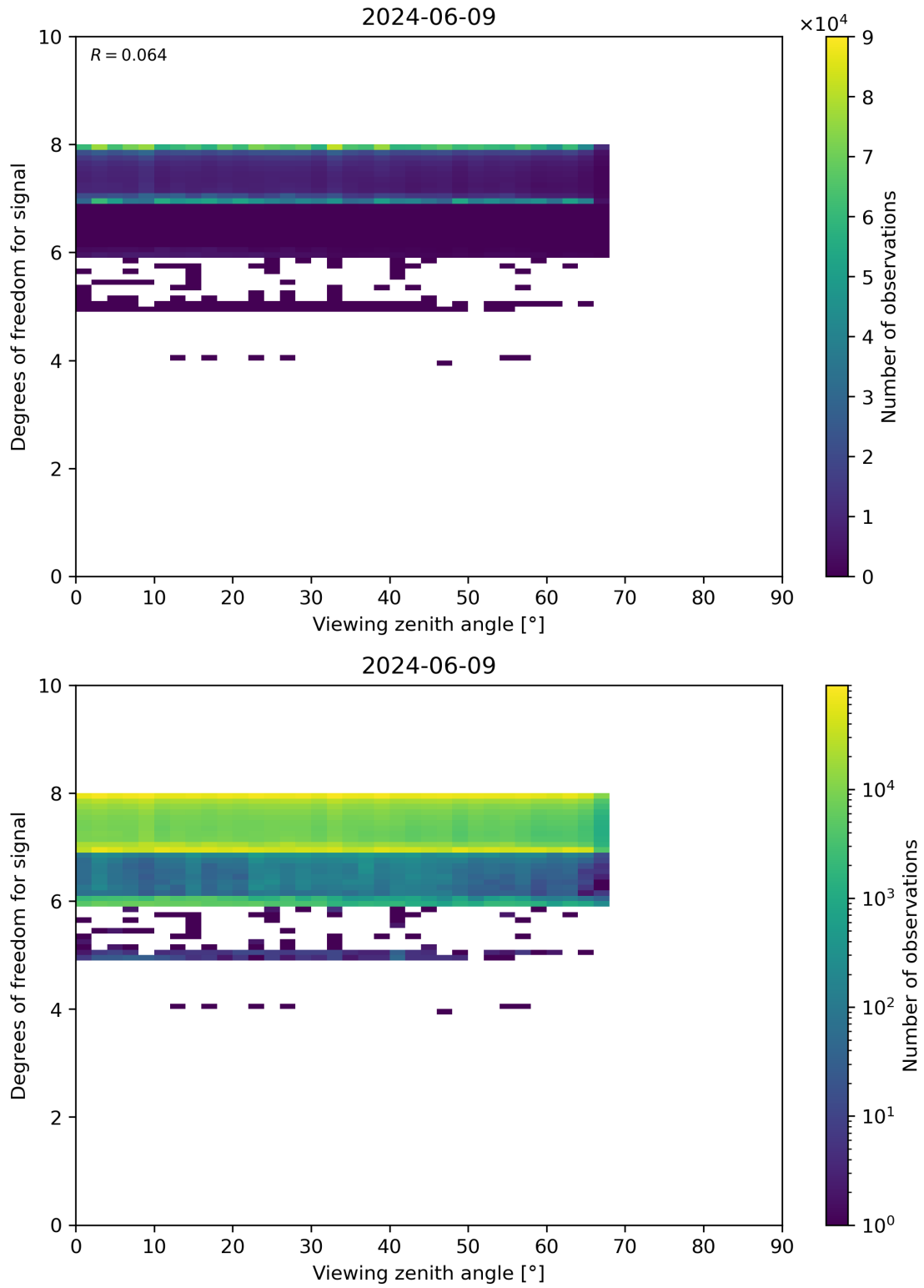
Figure 73: Scatter density plot of “Viewing zenith angle” against “Degrees of freedom for signal” for 2024-06-08 to 2024-06-10.
