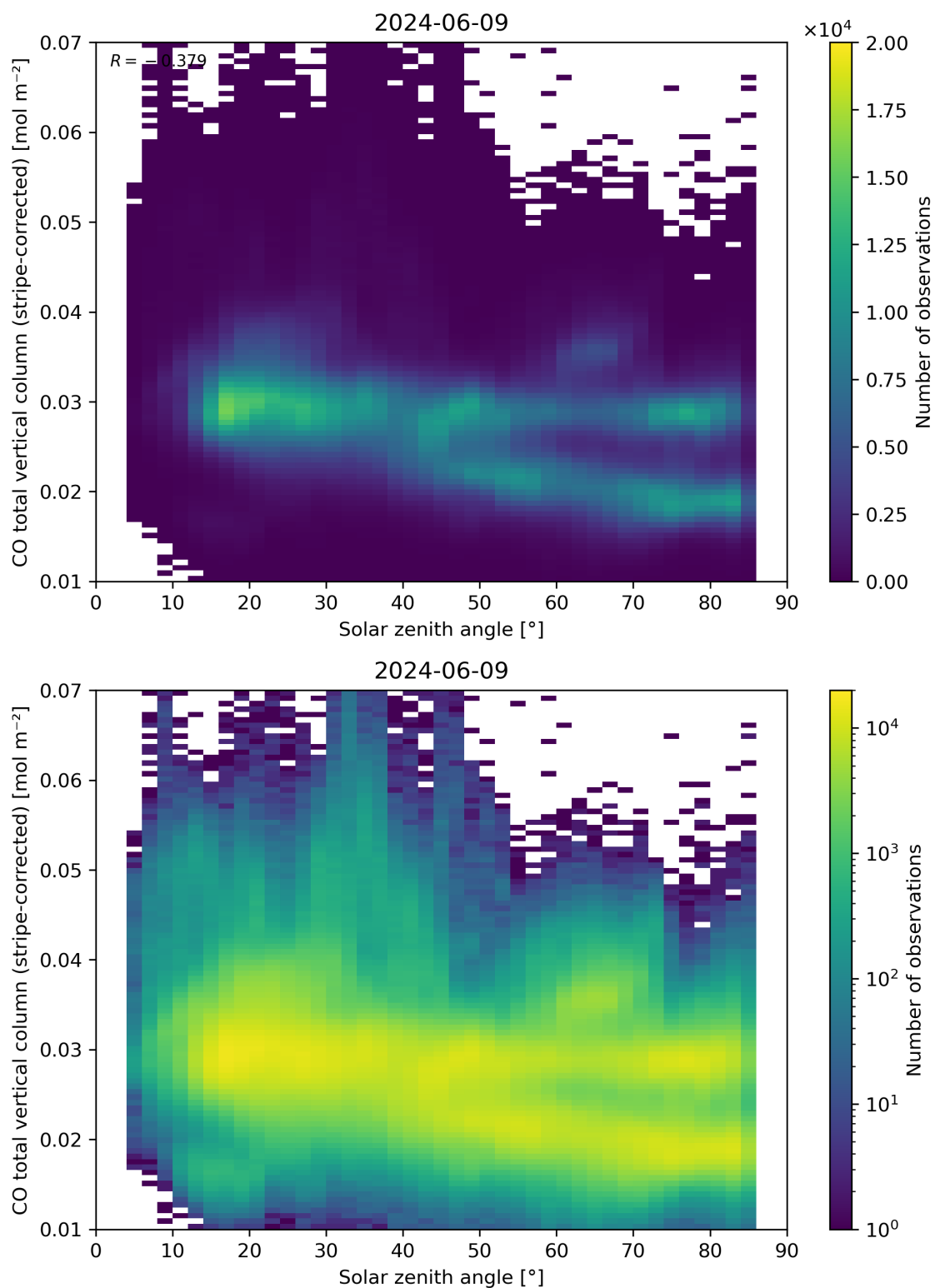
Figure 62: Scatter density plot of “Solar zenith angle” against “CO total vertical column (stripe-corrected)” for 2024-06-08 to 2024-06-10.
