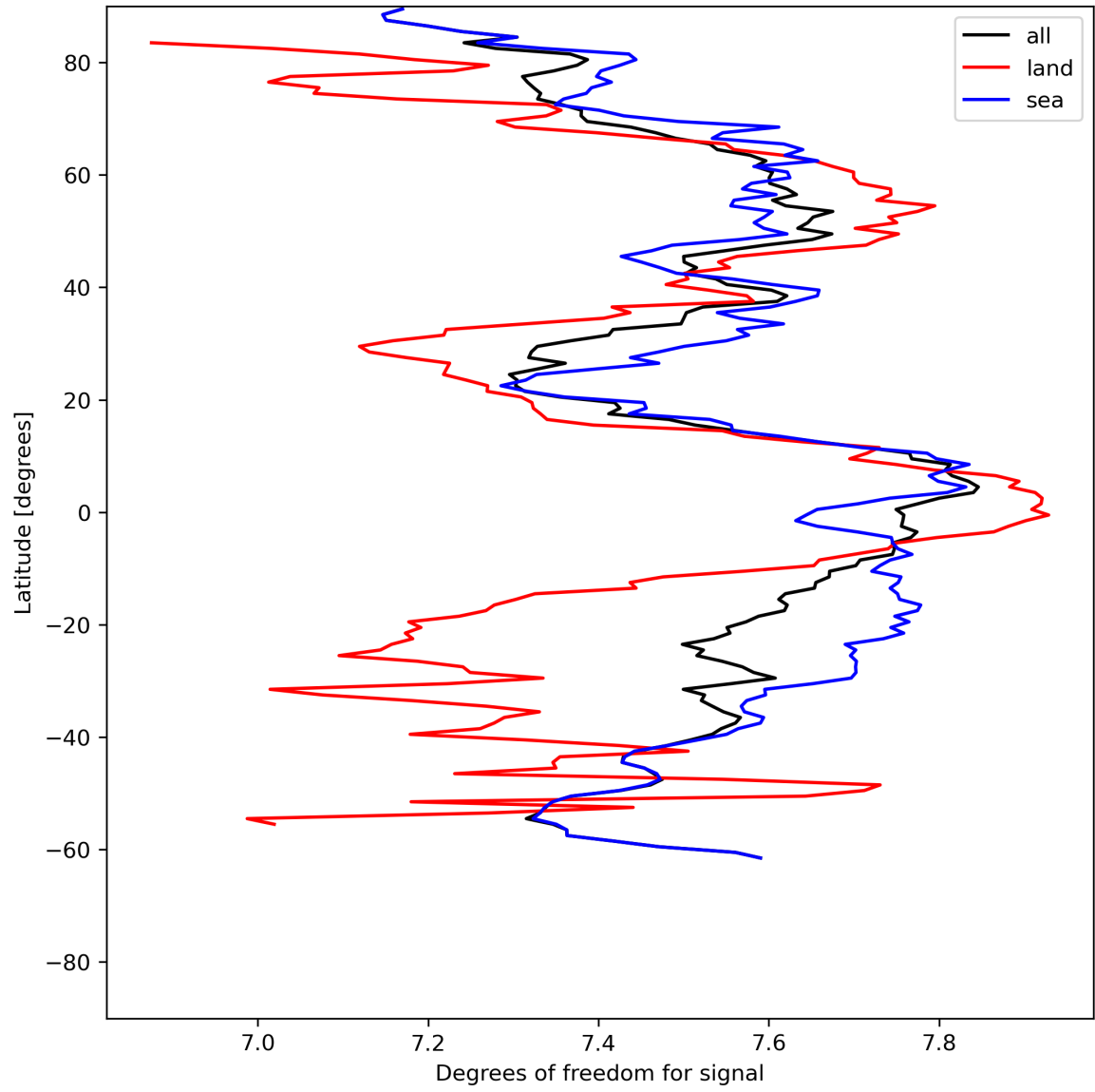
Figure 15: Zonal average of “Degrees of freedom for signal” for 2024-06-08 to 2024-06-10.
