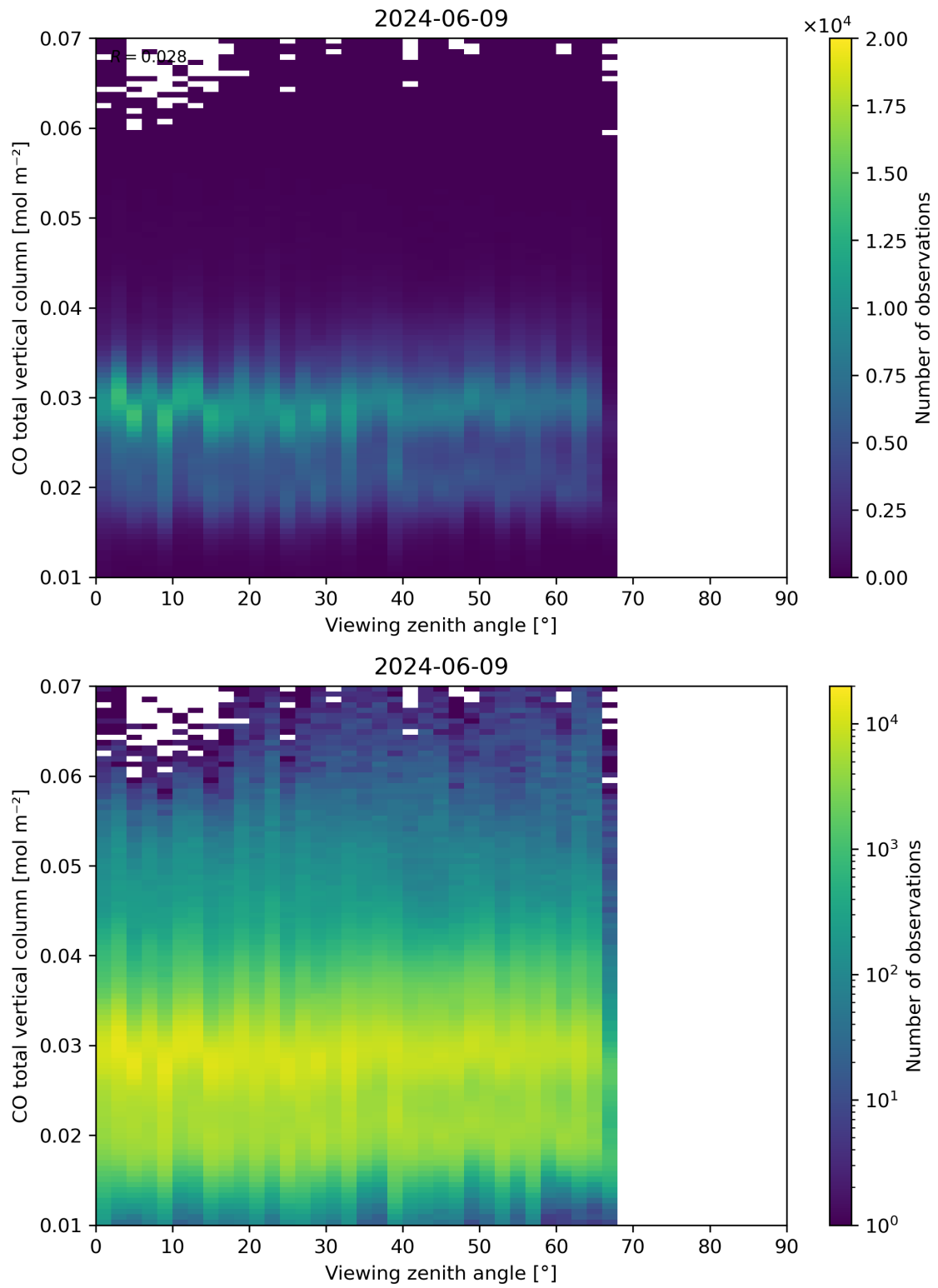
Figure 69: Scatter density plot of “Viewing zenith angle” against “CO total vertical column” for 2024-06-08 to 2024-06-10.
