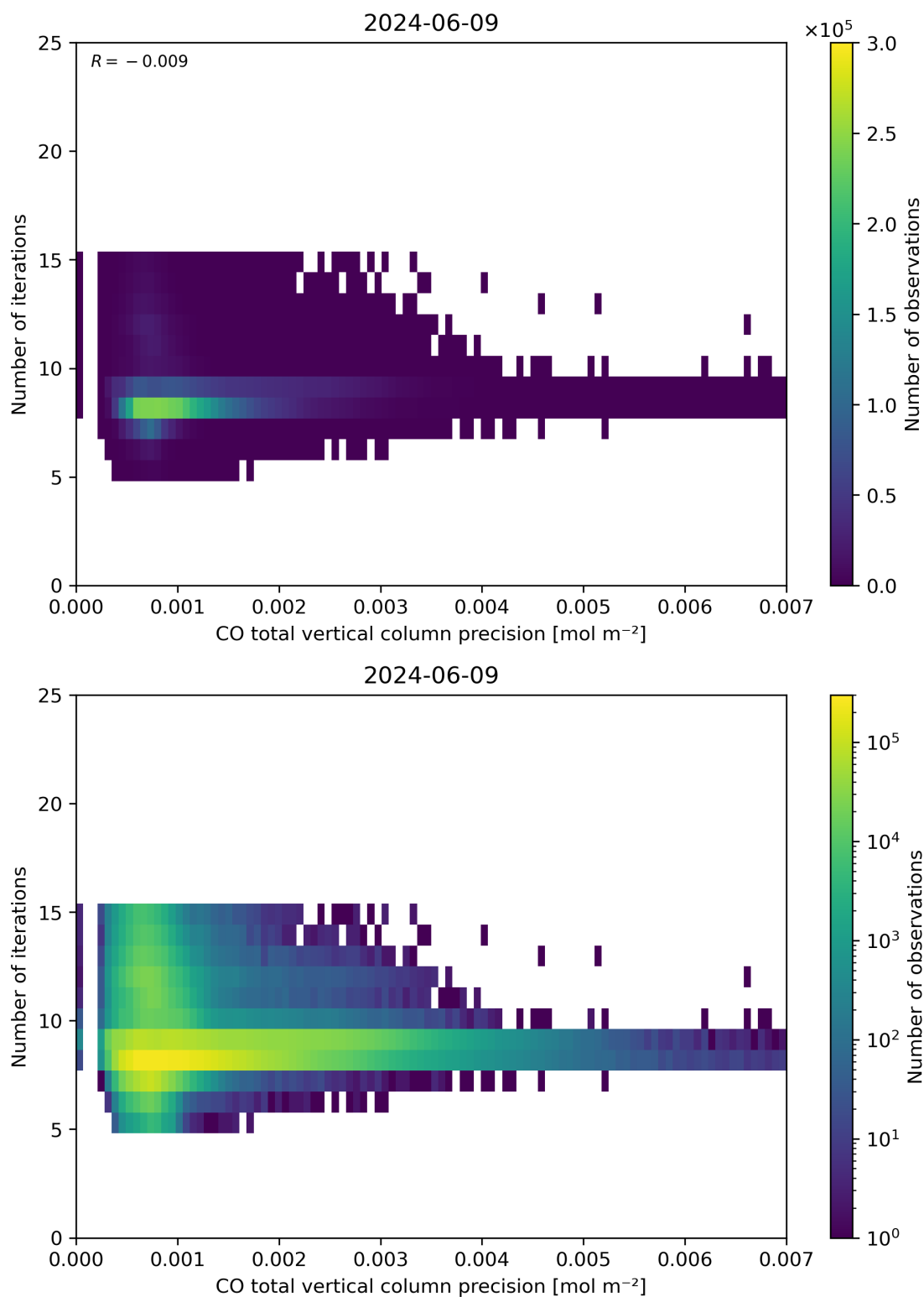
Figure 46: Scatter density plot of “CO total vertical column precision” against “Number of iterations” for 2024-06-08 to 2024-06-10.
