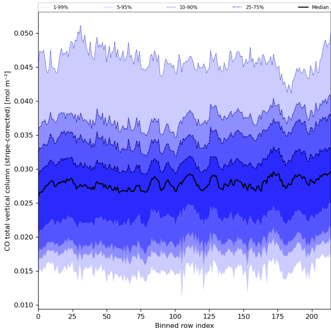
Figure 27: Along track statistics of “CO total vertical column (stripe-corrected)” for 2024-06-08 to 2024-06-10
