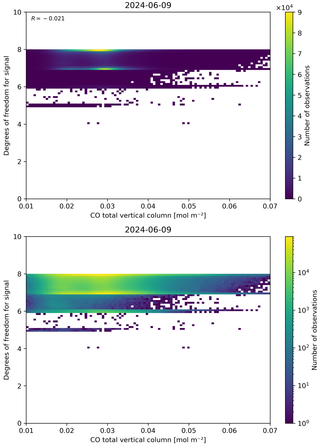
Figure 41: Scatter density plot of “CO total vertical column” against “Degrees of freedom for signal” for 2024-06-08 to 2024-06-10.
