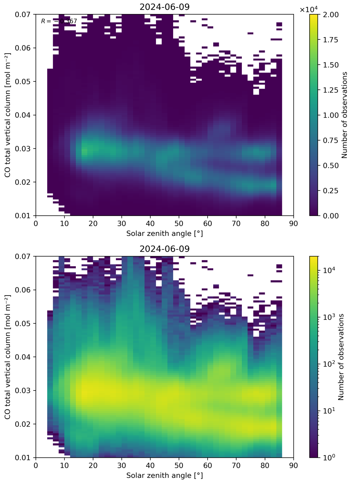
Figure 61: Scatter density plot of “Solar zenith angle” against “CO total vertical column” for 2024-06-08 to 2024-06-10.
