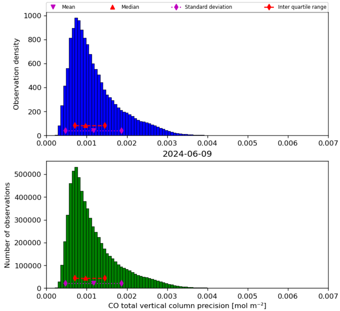
Figure 20: Histogram of “CO total vertical column precision” for 2024-06-08 to 2024-06-10
