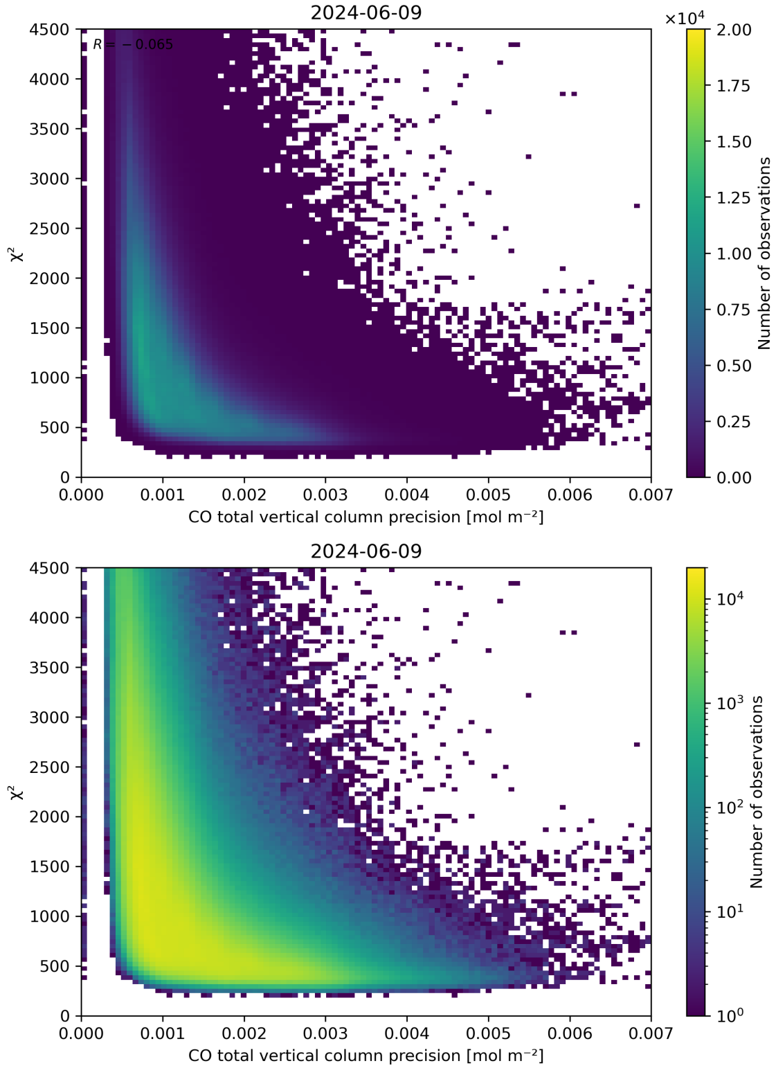
Figure 44: Scatter density plot of “CO total vertical column precision” against “ \chi^2 ” for 2024-06-08 to 2024-06-10.
