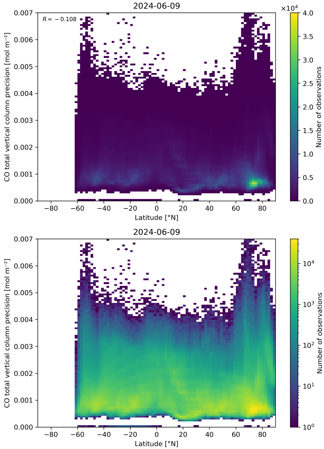
Figure 53: Scatter density plot of “Latitude” against “CO total vertical column precision” for 2024-06-08 to 2024-06-10.
