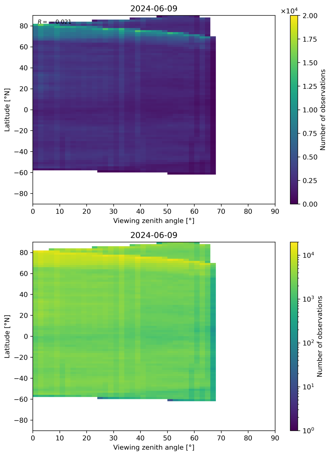
Figure 74: Scatter density plot of “Viewing zenith angle” against “Latitude” for 2024-06-08 to 2024-06-10.
