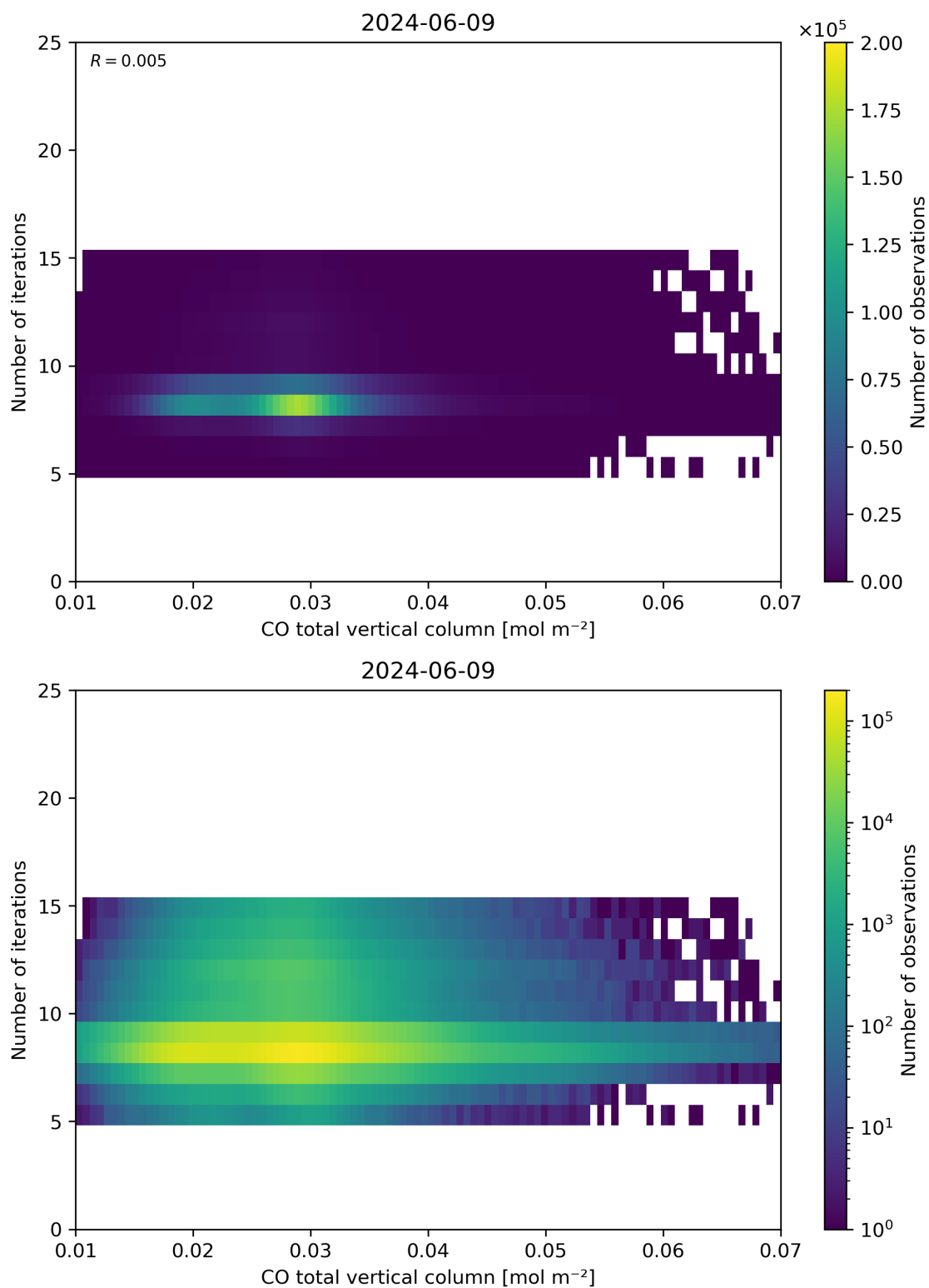
Figure 42: Scatter density plot of “CO total vertical column” against “Number of iterations” for 2024-06-08 to 2024-06-10.
