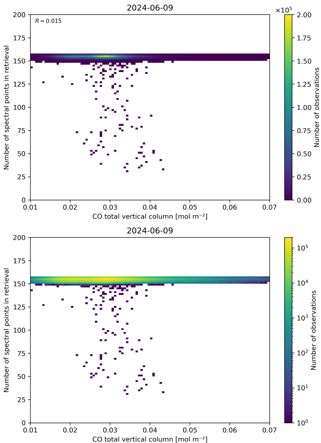
Figure 43: Scatter density plot of “CO total vertical column” against “Number of spectral points in retrieval” for 2024-06-08 to 2024-06-10.
