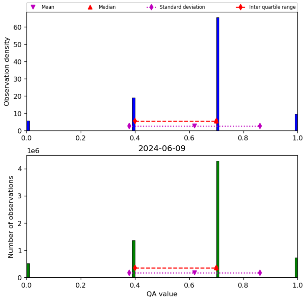
Figure 17: Histogram of “QA value” for 2024-06-08 to 2024-06-10
