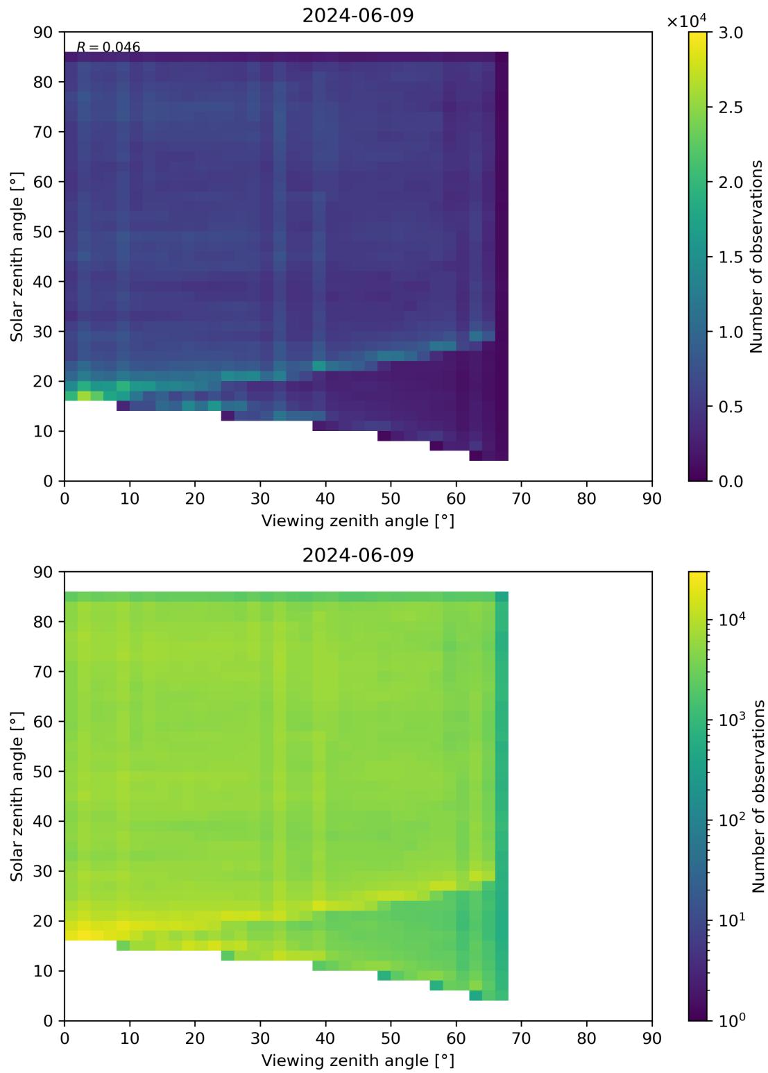
Figure 77: Scatter density plot of “Viewing zenith angle” against “Solar zenith angle” for 2024-06-08 to 2024-06-10.
