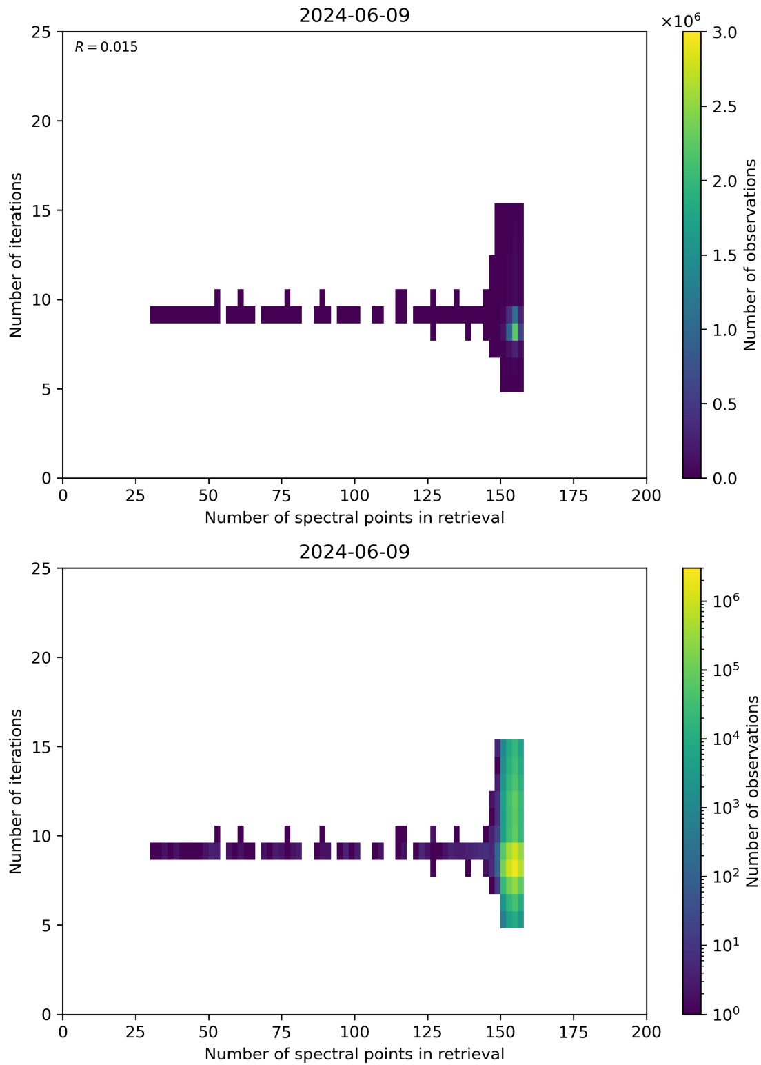
Figure 60: Scatter density plot of “Number of spectral points in retrieval” against “Number of iterations” for 2024-06-08 to 2024-06-10.
