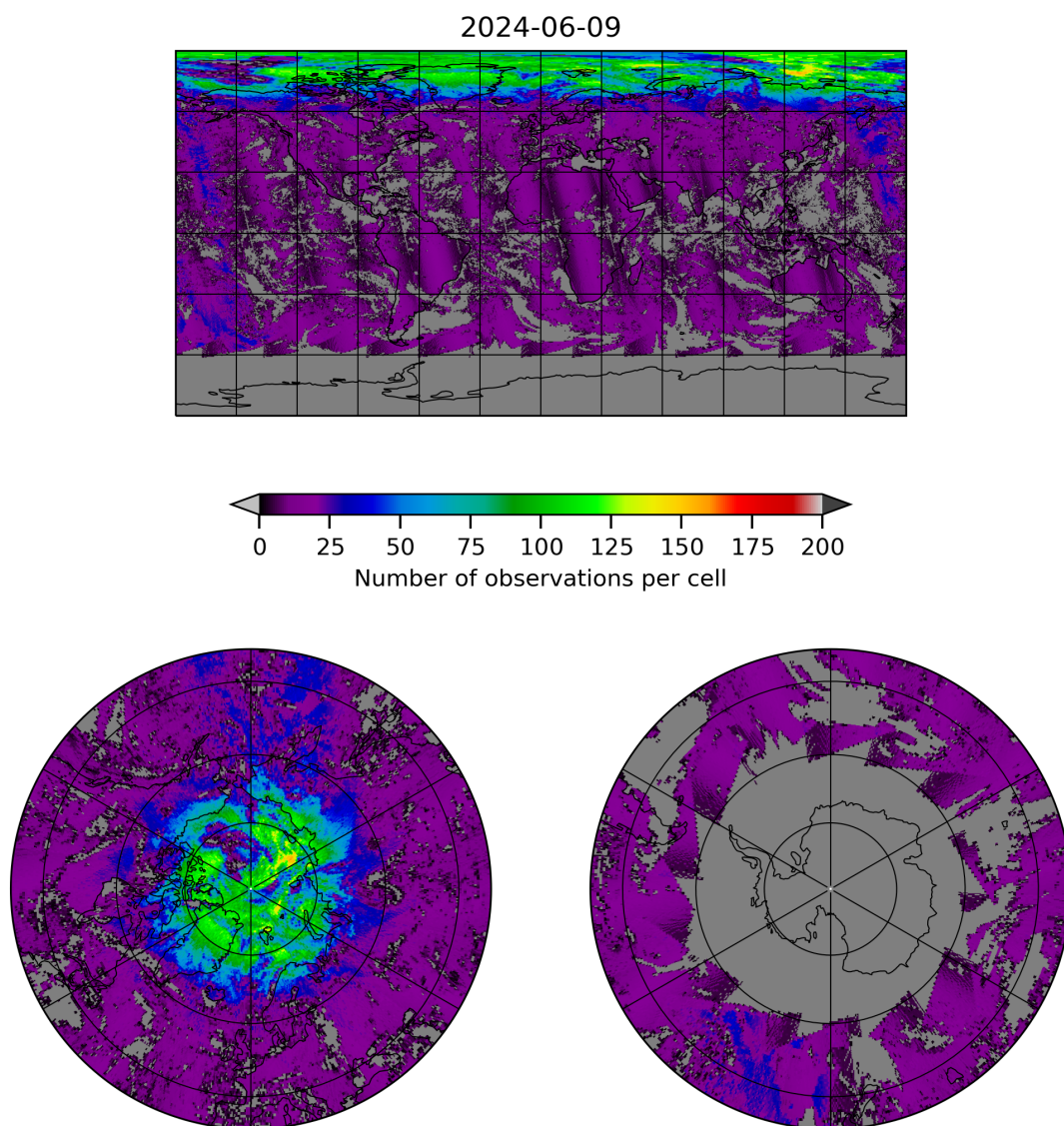
Figure 8: Map of the number of observations for 2024-06-08 to 2024-06-10
