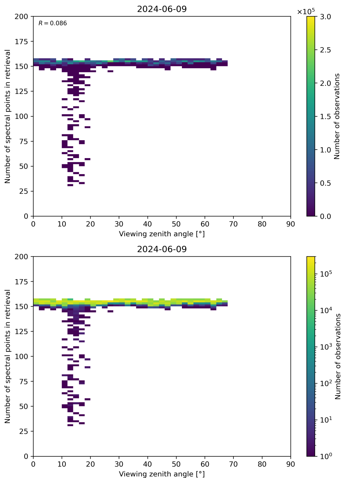
Figure 76: Scatter density plot of “Viewing zenith angle” against “Number of spectral points in retrieval” for 2024-06-08 to 2024-06-10.
