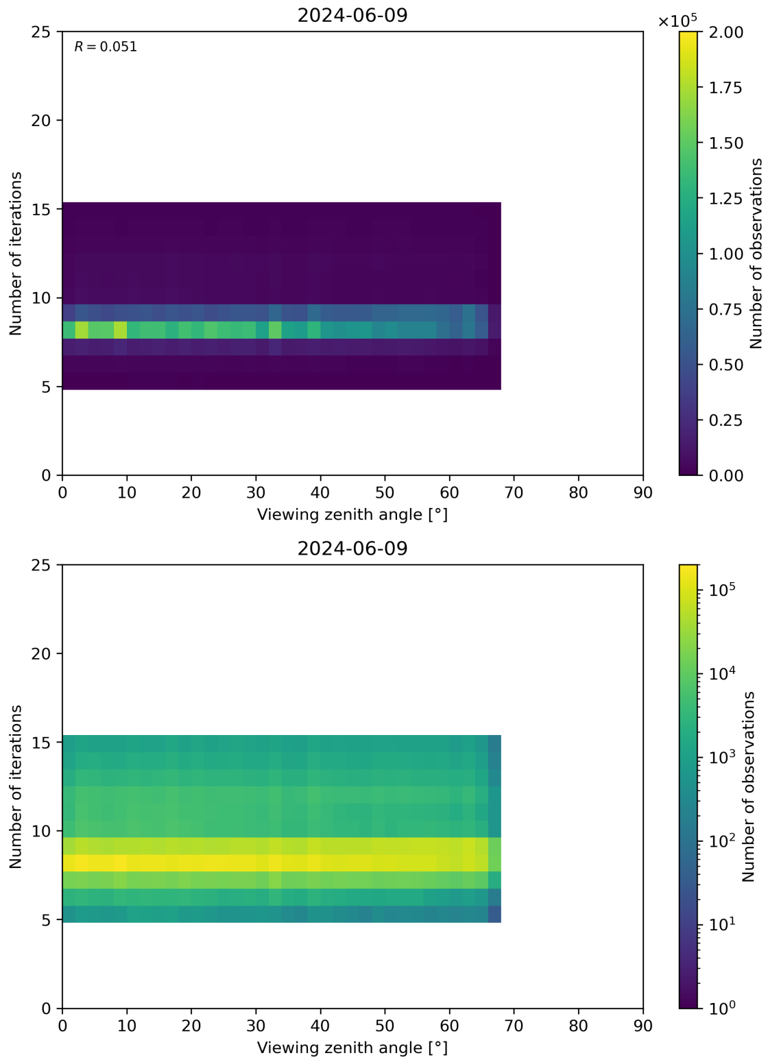
Figure 75: Scatter density plot of “Viewing zenith angle” against “Number of iterations” for 2024-06-08 to 2024-06-10.
