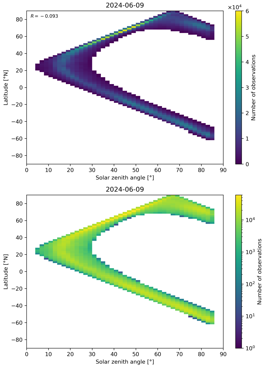
Figure 66: Scatter density plot of “Solar zenith angle” against “Latitude” for 2024-06-08 to 2024-06-10.
