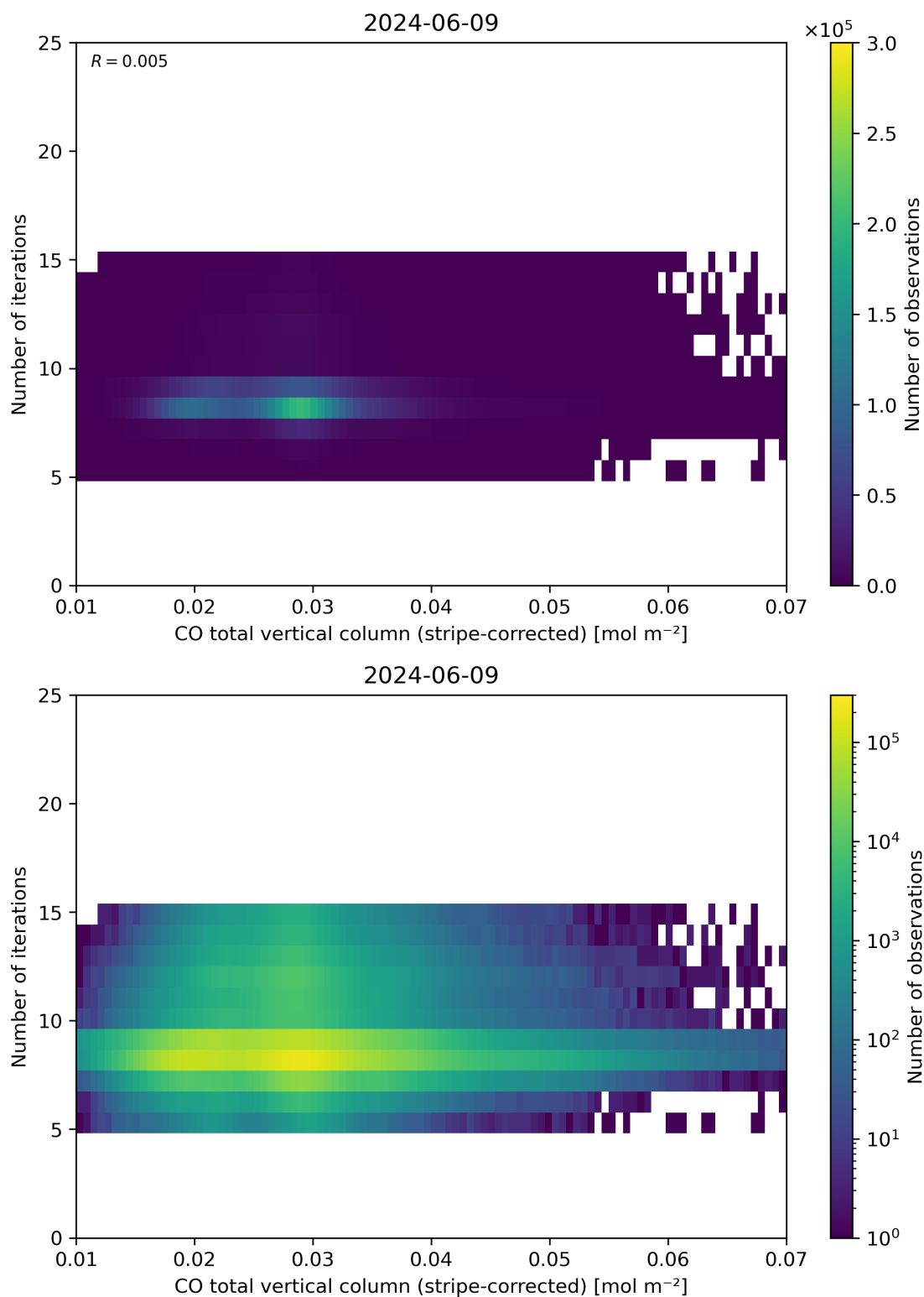
Figure 39: Scatter density plot of “CO total vertical column (stripe-corrected)” against “Number of iterations” for 2024-06-08 to 2024-06-10.
