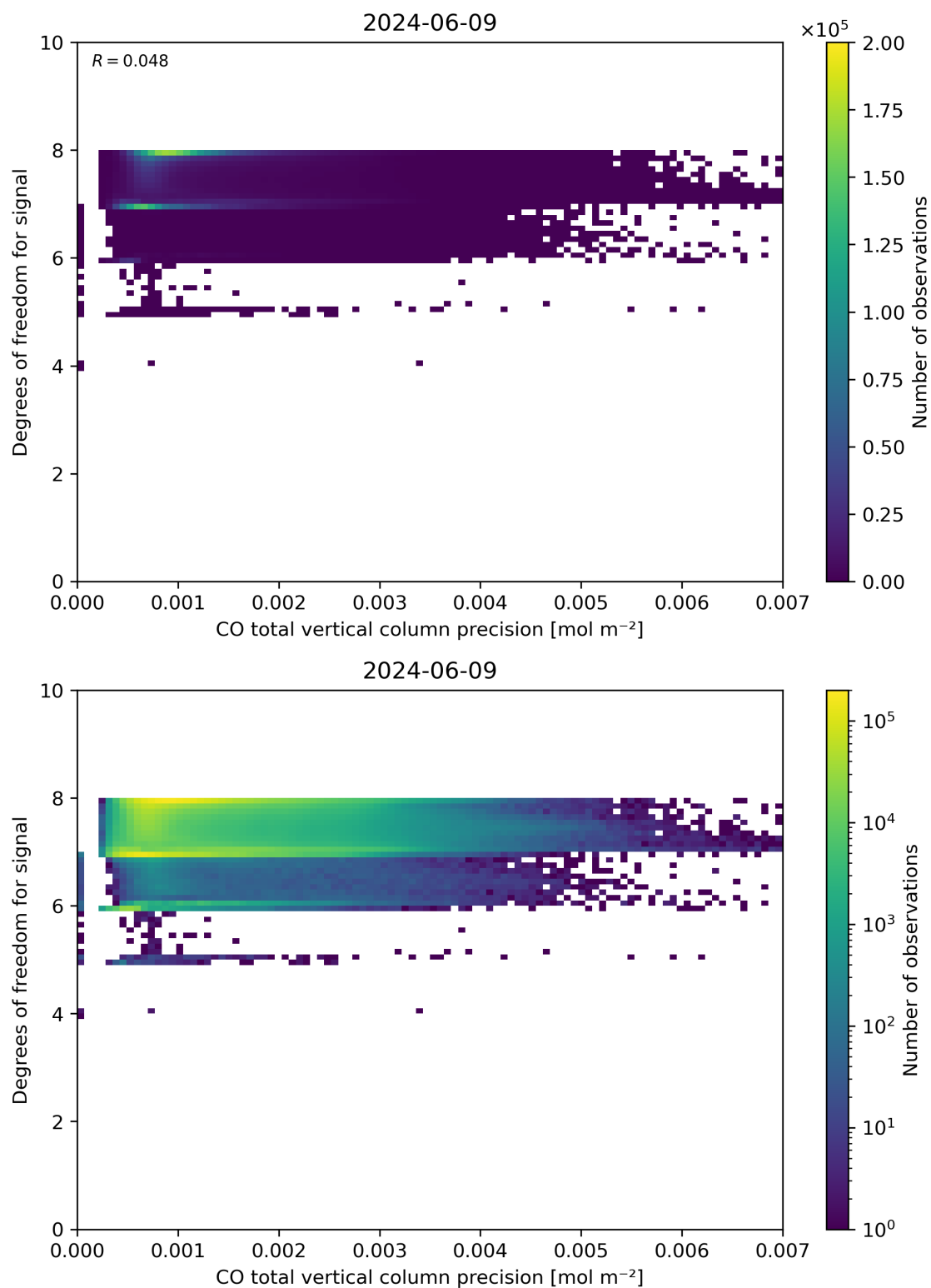
Figure 45: Scatter density plot of “CO total vertical column precision” against “Degrees of freedom for signal” for 2024-06-08 to 2024-06-10.
