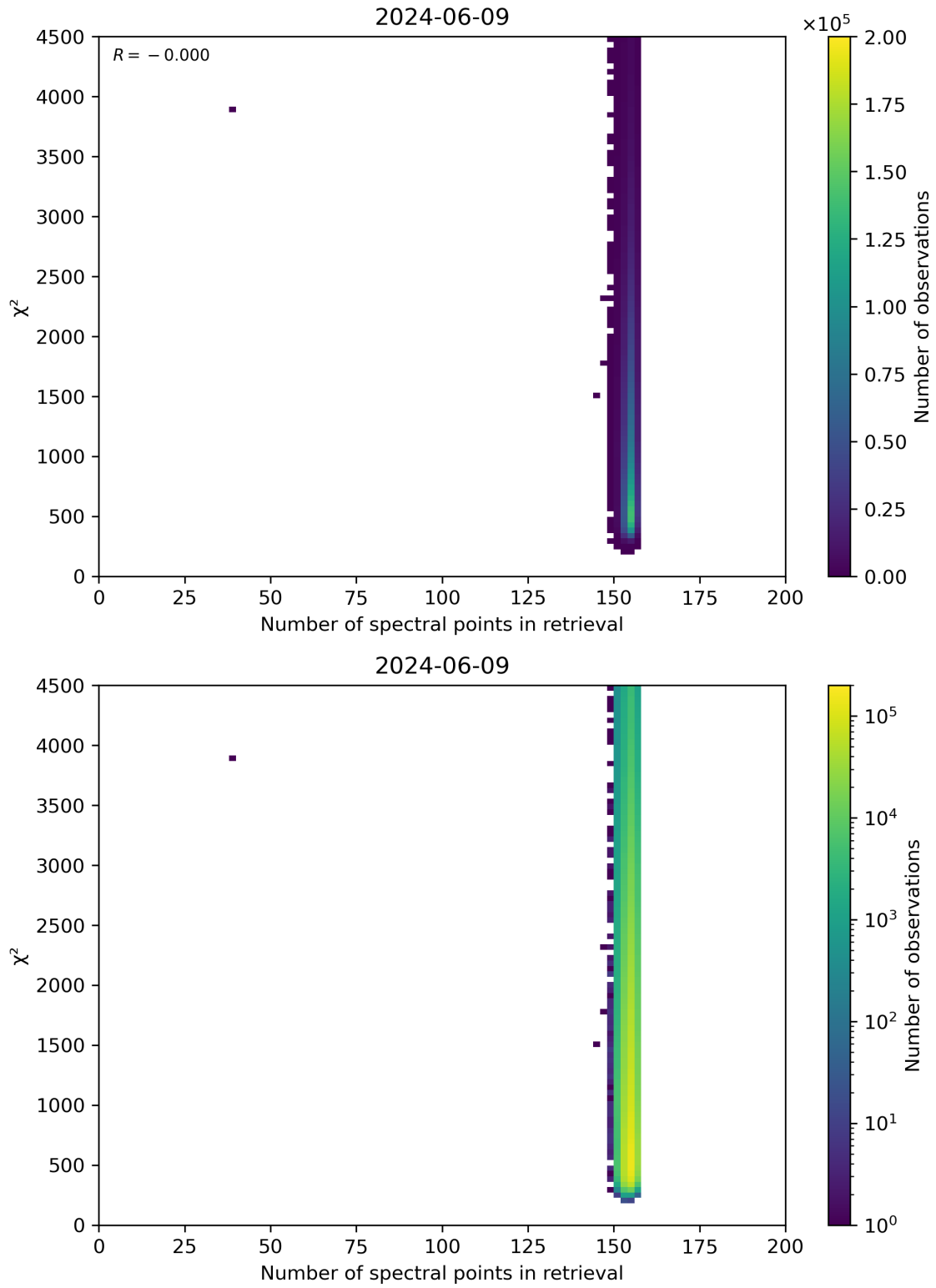
Figure 58: Scatter density plot of “Number of spectral points in retrieval” against “ \chi^2 ” for 2024-06-08 to 2024-06-10.
