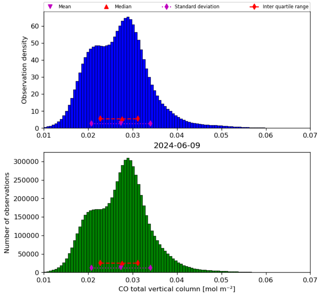
Figure 18: Histogram of “CO total vertical column” for 2024-06-08 to 2024-06-10
