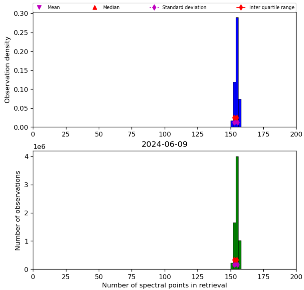
Figure 21: Histogram of “Number of spectral points in retrieval” for 2024-06-08 to 2024-06-10
