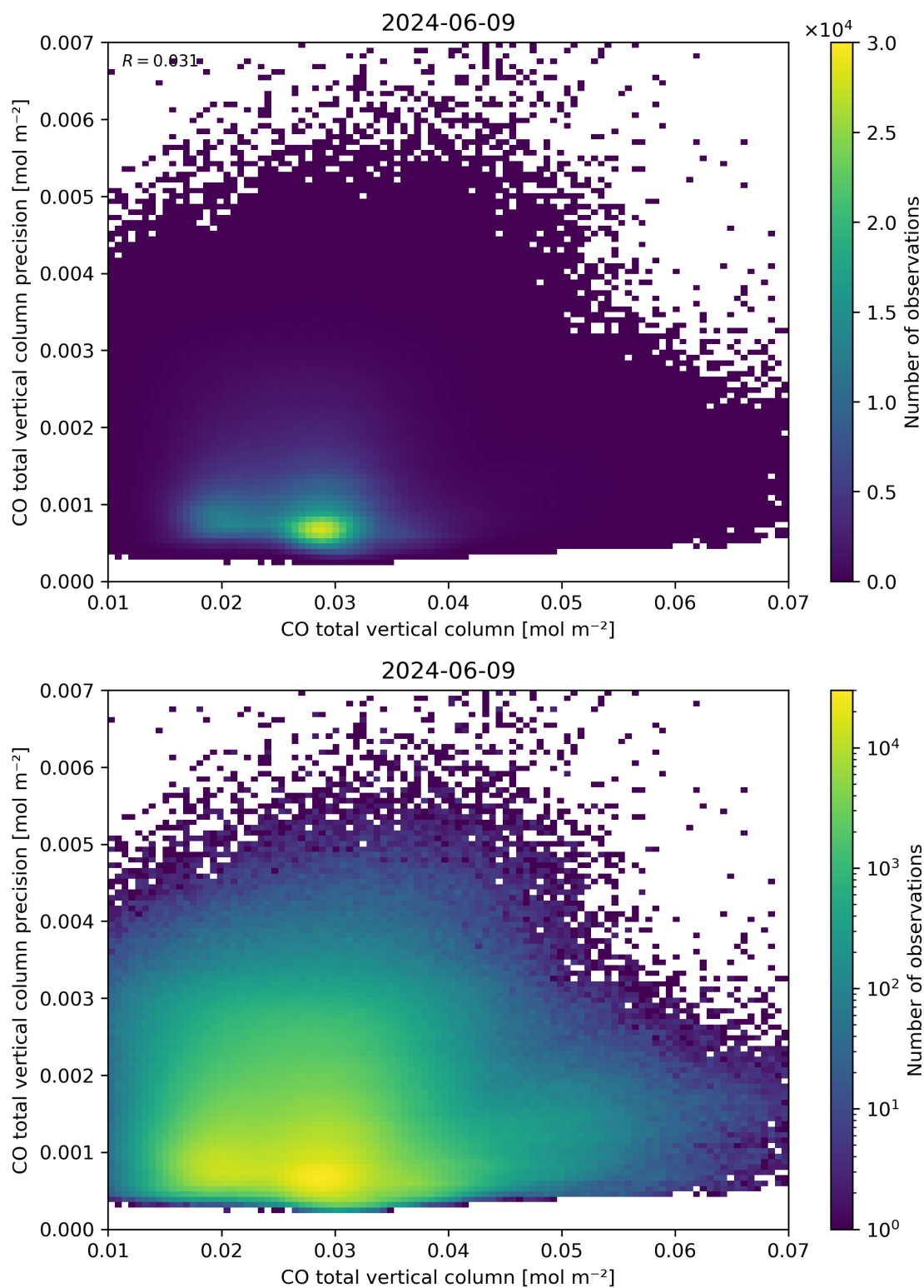
Figure 34: Scatter density plot of “CO total vertical column” against “CO total vertical column precision” for 2024-06-08 to 2024-06-10.
