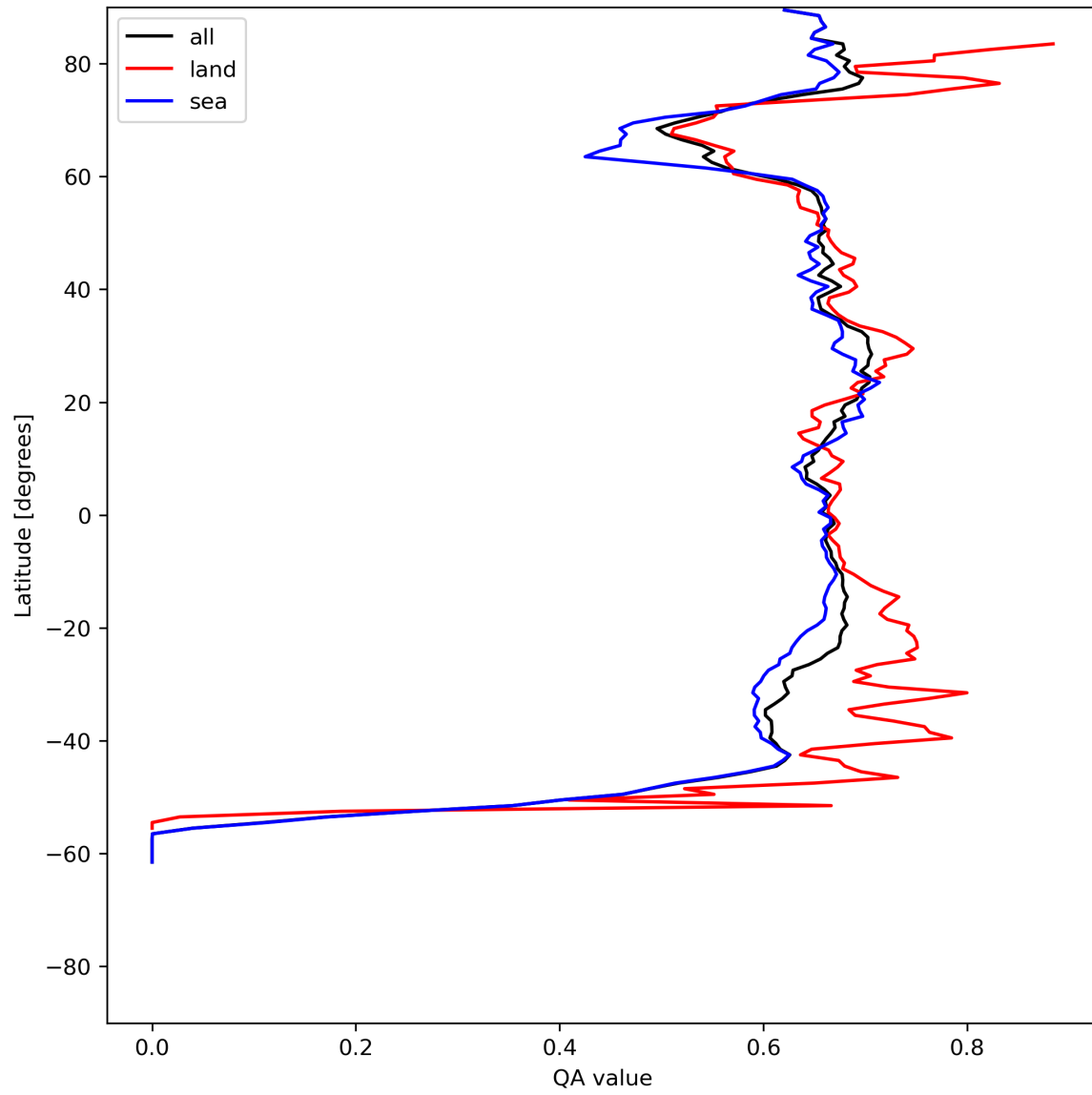
Figure 9: Zonal average of “QA value” for 2024-06-08 to 2024-06-10.
