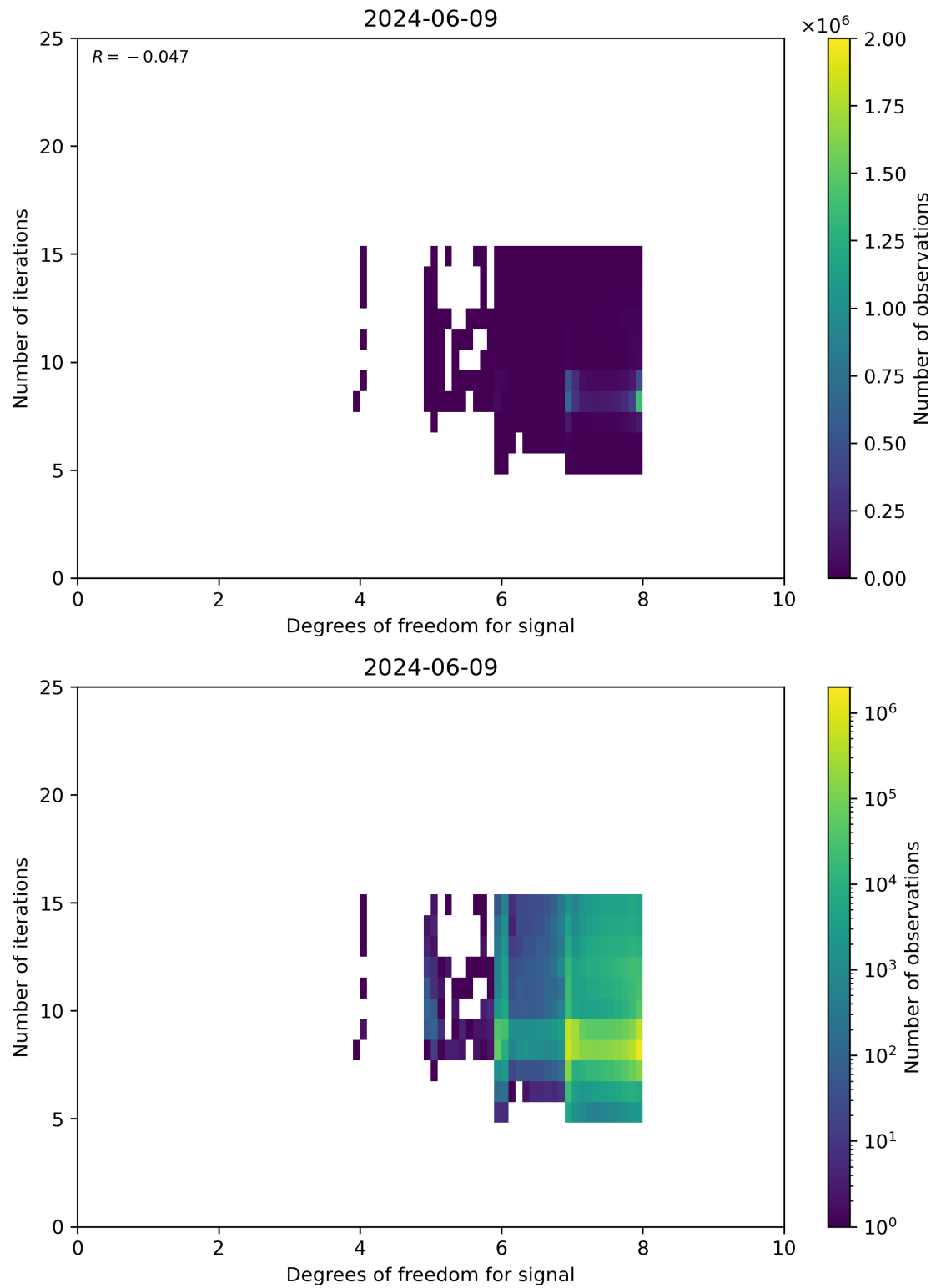
Figure 50: Scatter density plot of “Degrees of freedom for signal” against “Number of iterations” for 2024-06-08 to 2024-06-10.
