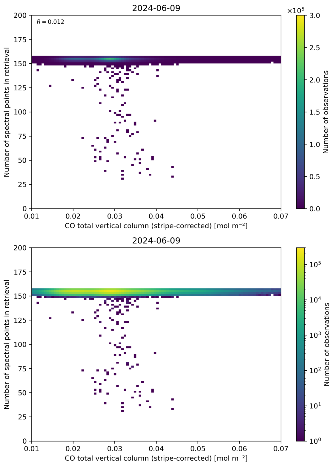
Figure 40: Scatter density plot of “CO total vertical column (stripe-corrected)” against “Number of spectral points in retrieval” for 2024-06-08 to 2024-06-10.
