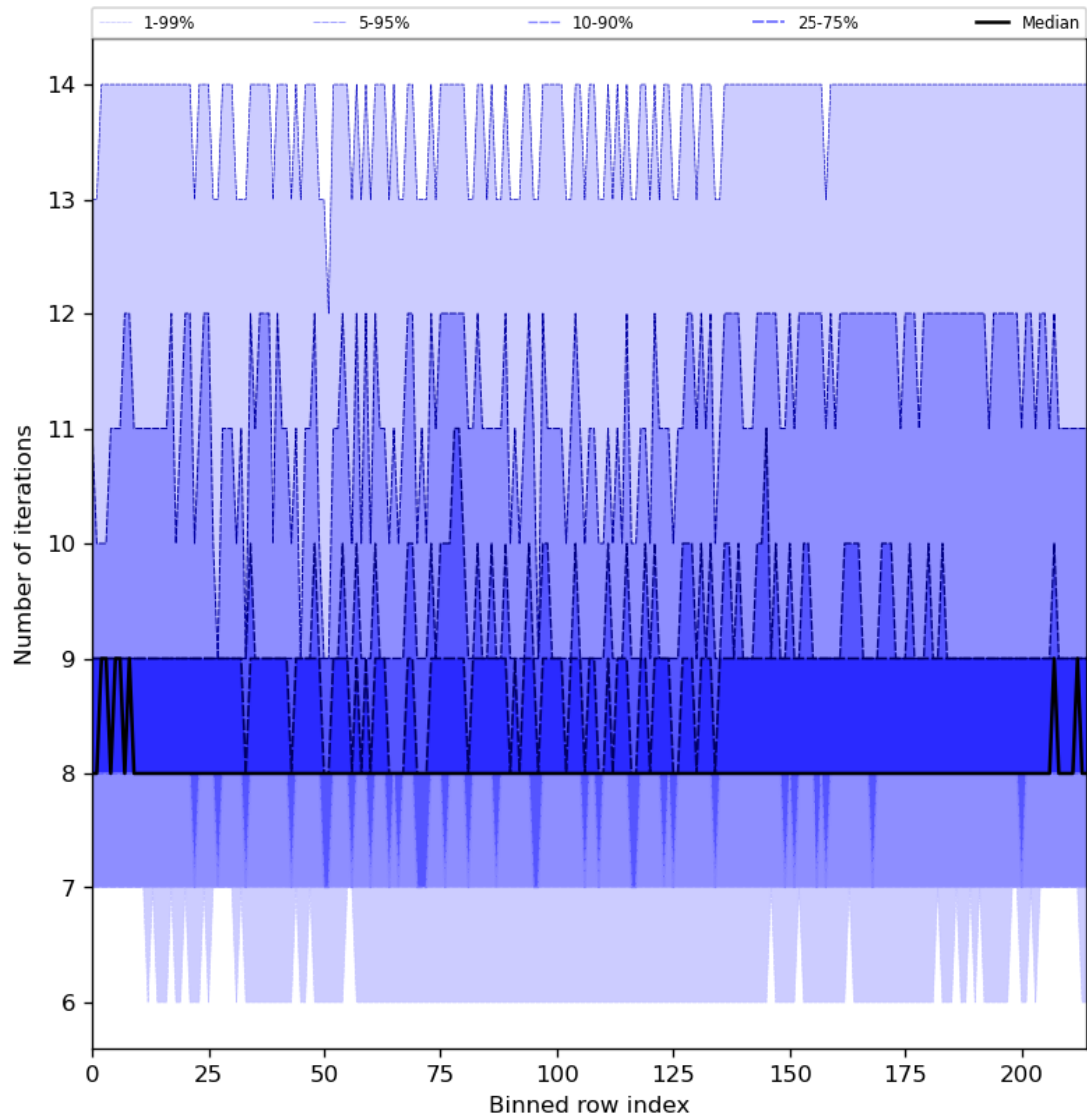
Figure 32: Along track statistics of “Number of iterations” for 2024-06-09 to 2024-06-11
