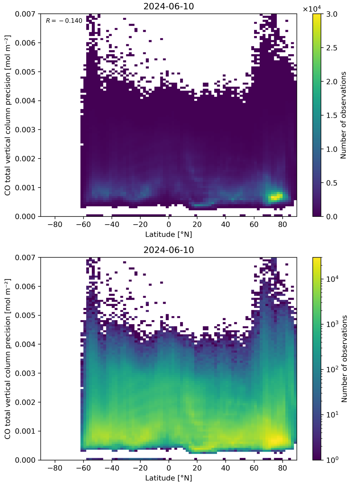
Figure 53: Scatter density plot of “Latitude” against “CO total vertical column precision” for 2024-06-09 to 2024-06-11.
