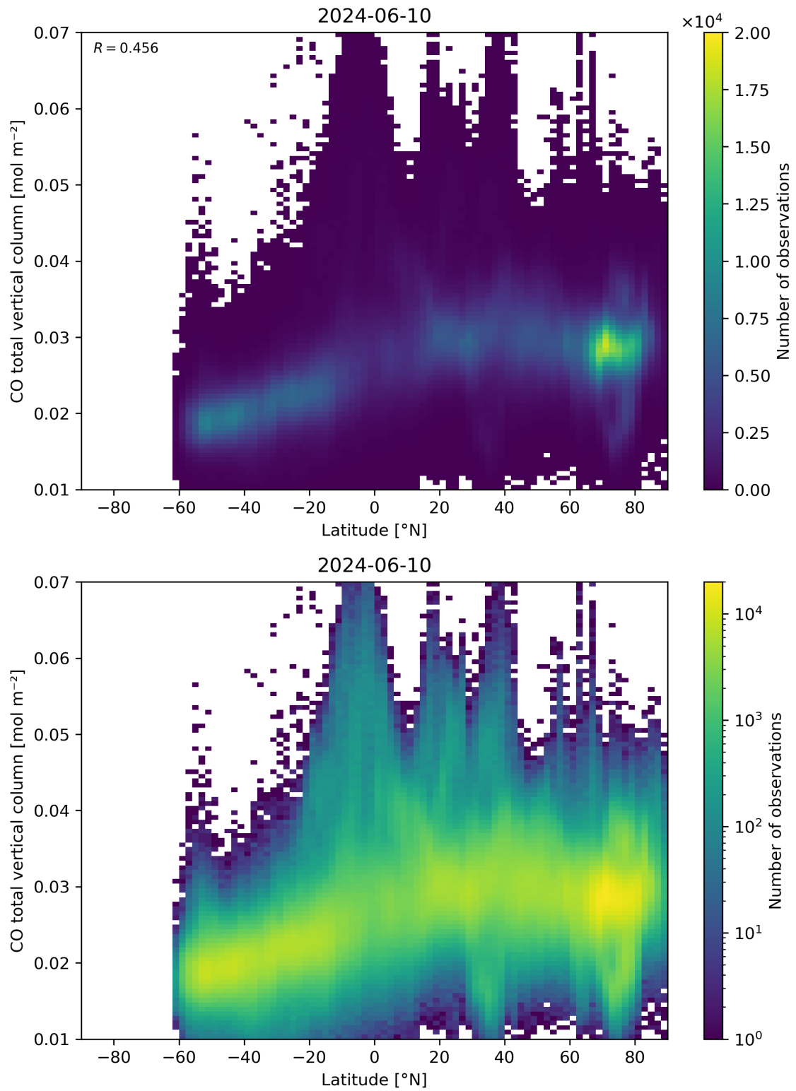
Figure 51: Scatter density plot of “Latitude” against “CO total vertical column” for 2024-06-09 to 2024-06-11.
