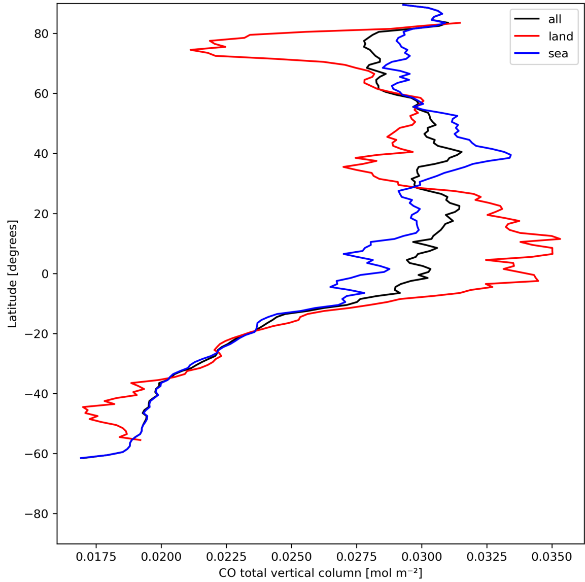
Figure 10: Zonal average of “CO total vertical column” for 2024-06-09 to 2024-06-11.
