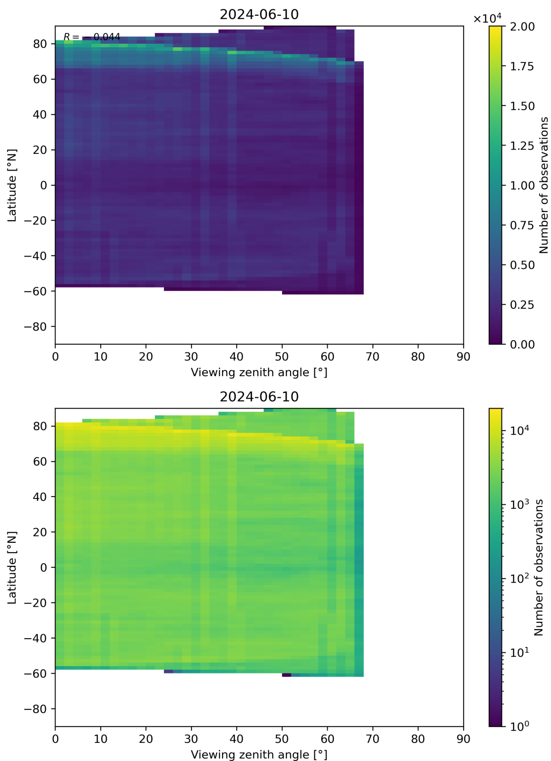
Figure 74: Scatter density plot of “Viewing zenith angle” against “Latitude” for 2024-06-09 to 2024-06-11.
