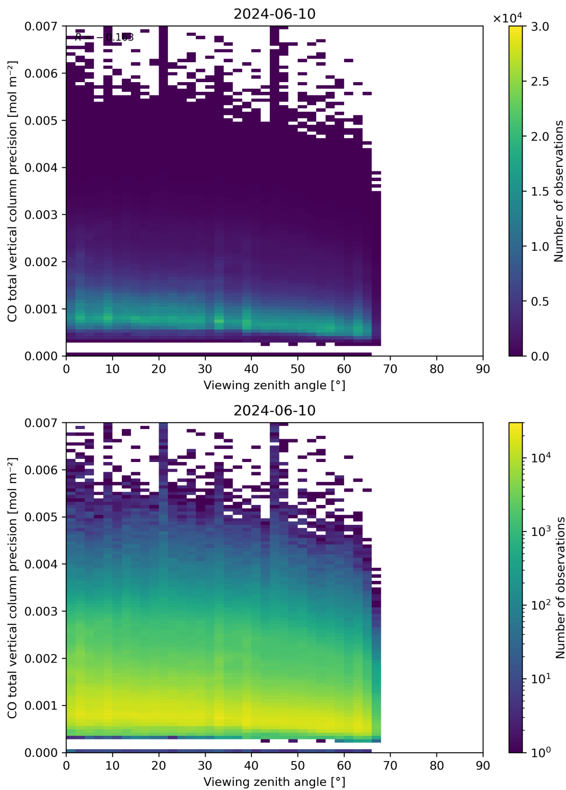
Figure 71: Scatter density plot of “Viewing zenith angle” against “CO total vertical column precision” for 2024-06-09 to 2024-06-11.
