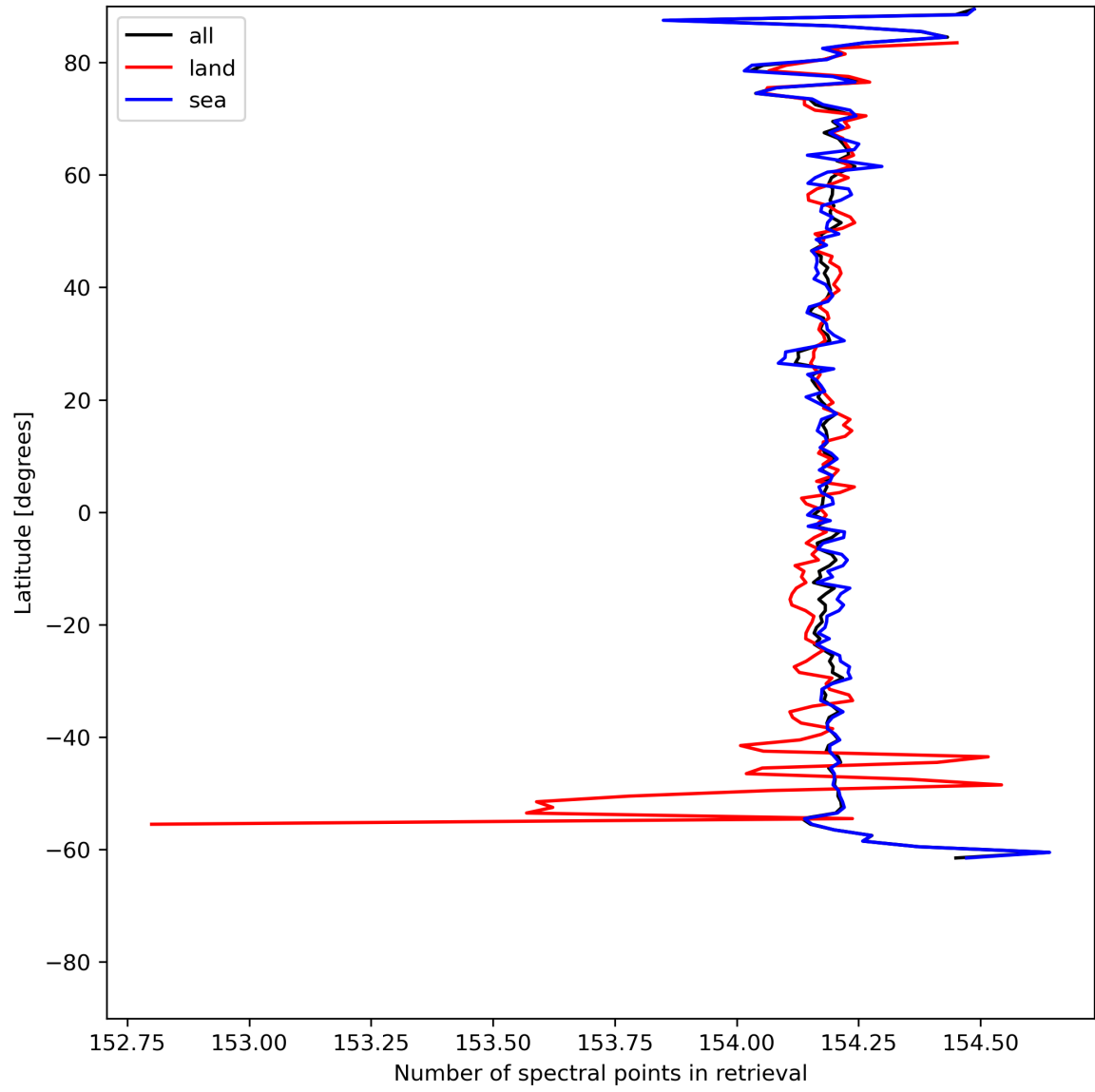
Figure 13: Zonal average of “Number of spectral points in retrieval” for 2024-06-09 to 2024-06-11.
