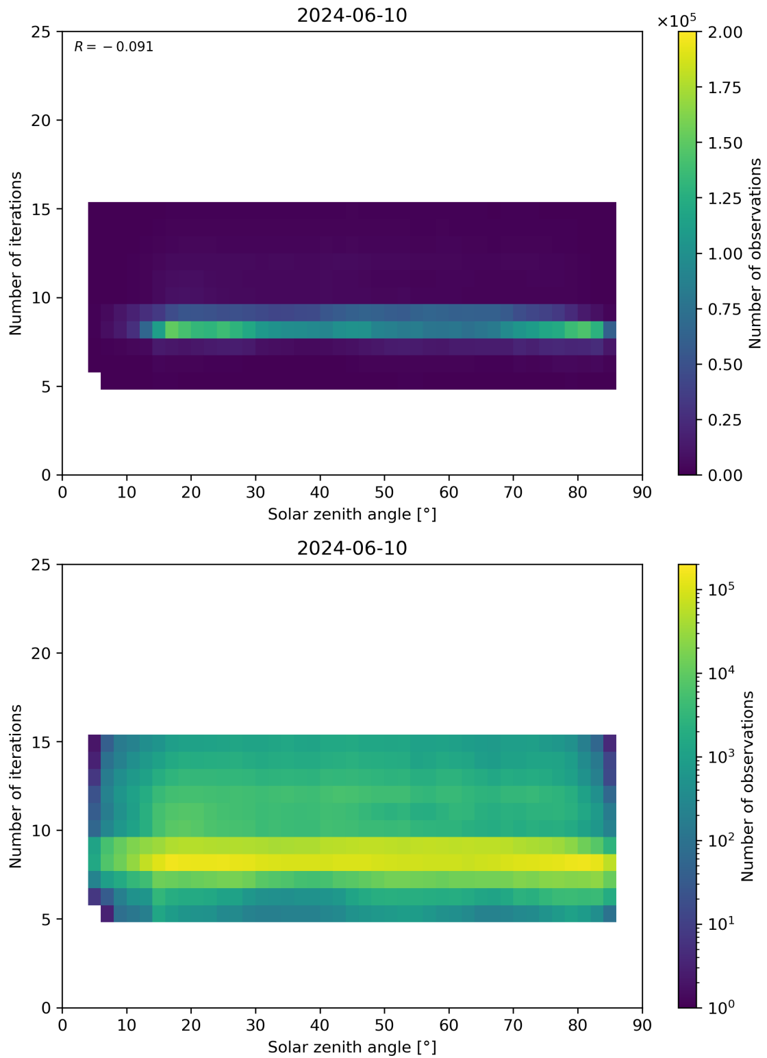
Figure 67: Scatter density plot of “Solar zenith angle” against “Number of iterations” for 2024-06-09 to 2024-06-11.
