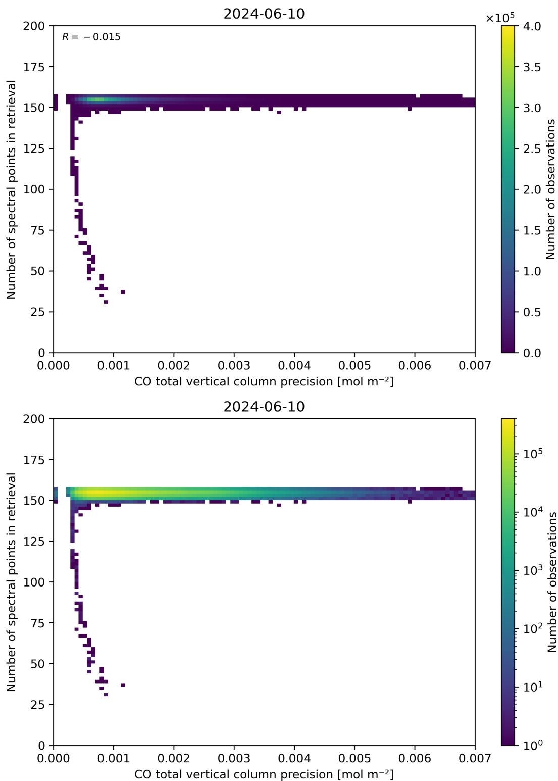
Figure 47: Scatter density plot of “CO total vertical column precision” against “Number of spectral points in retrieval” for 2024-06-09 to 2024-06-11.
