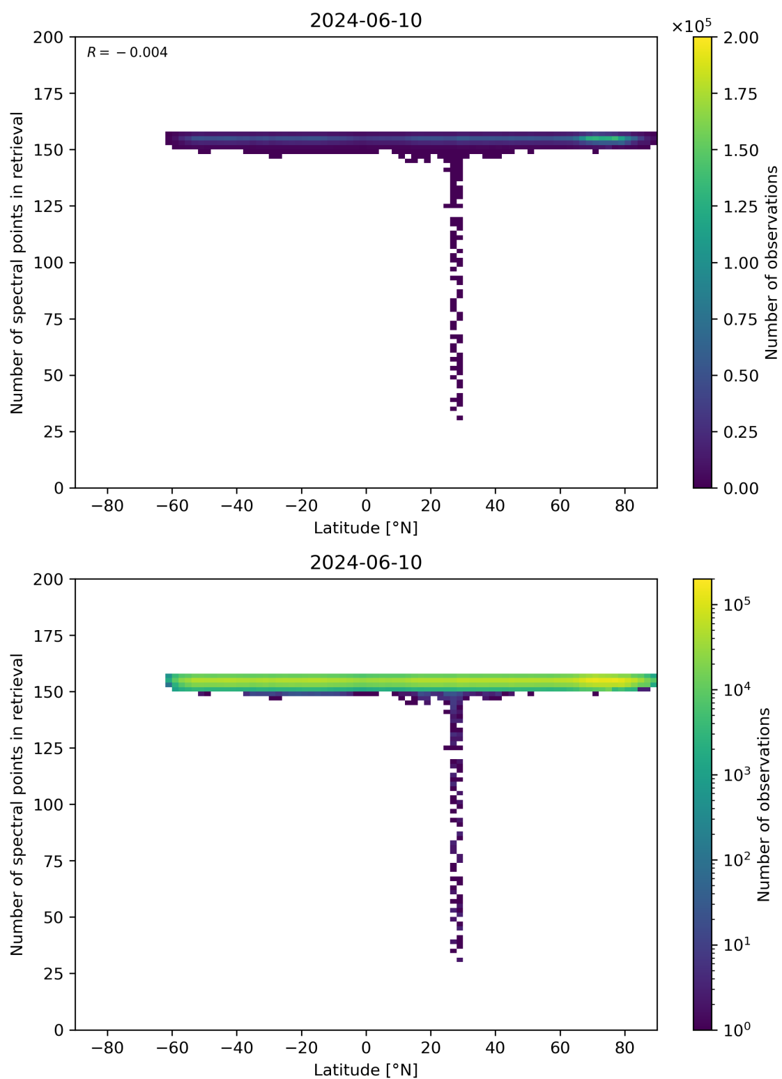
Figure 57: Scatter density plot of “Latitude” against “Number of spectral points in retrieval” for 2024-06-09 to 2024-06-11.
