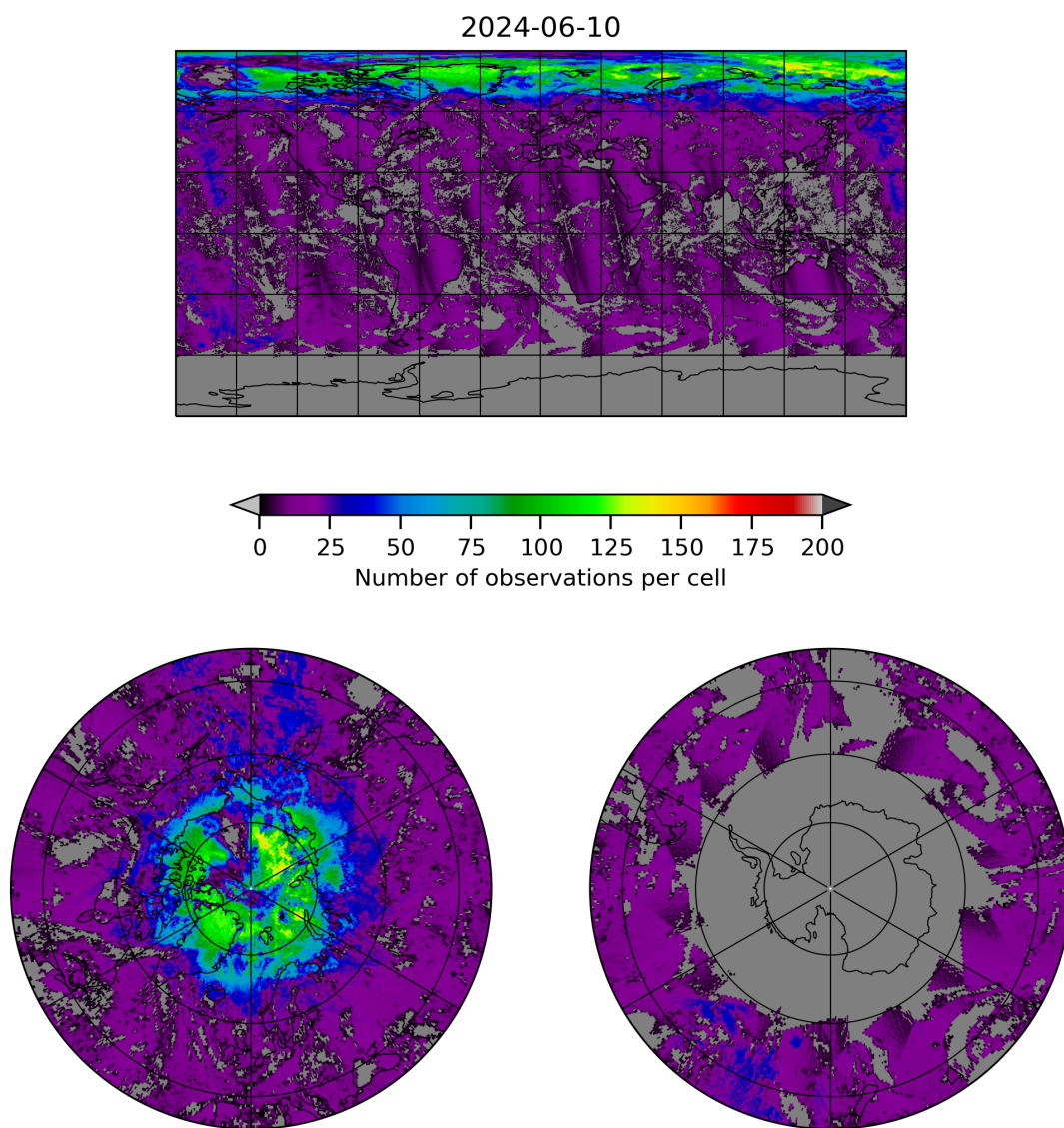
Figure 8: Map of the number of observations for 2024-06-09 to 2024-06-11
