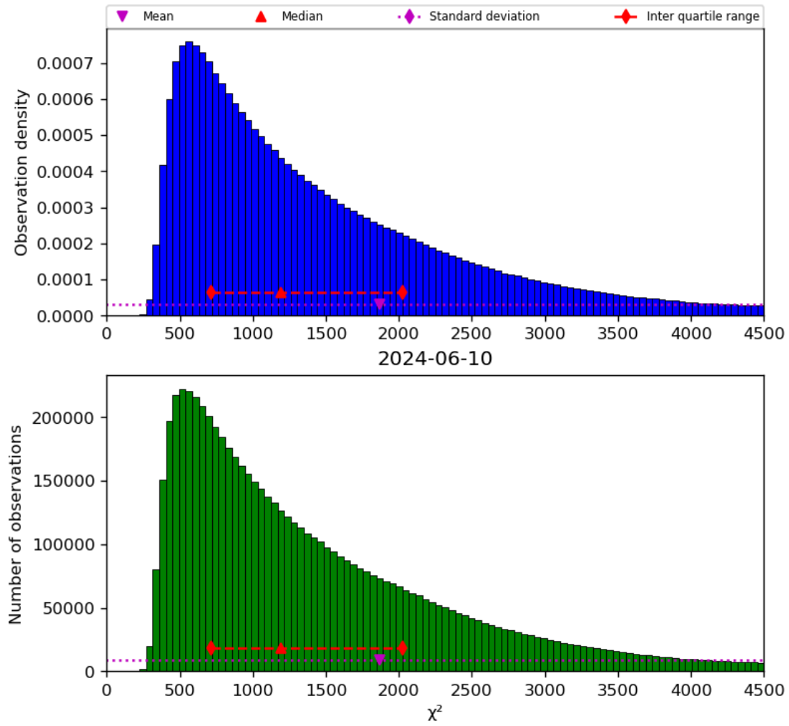
Figure 22: Histogram of “ \chi^2 ” for 2024-06-09 to 2024-06-11
