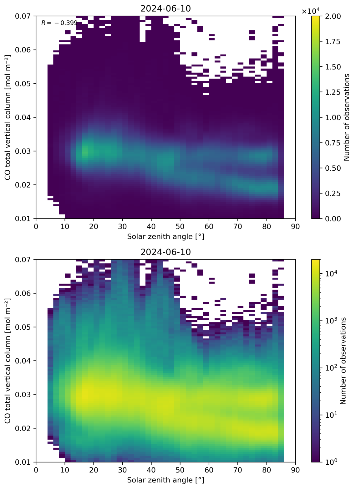
Figure 61: Scatter density plot of “Solar zenith angle” against “CO total vertical column” for 2024-06-09 to 2024-06-11.
