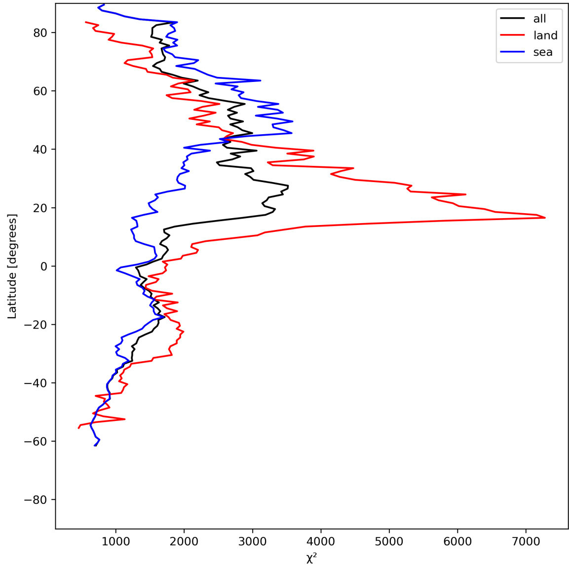
Figure 14: Zonal average of “ \chi^2 ” for 2024-06-09 to 2024-06-11.
