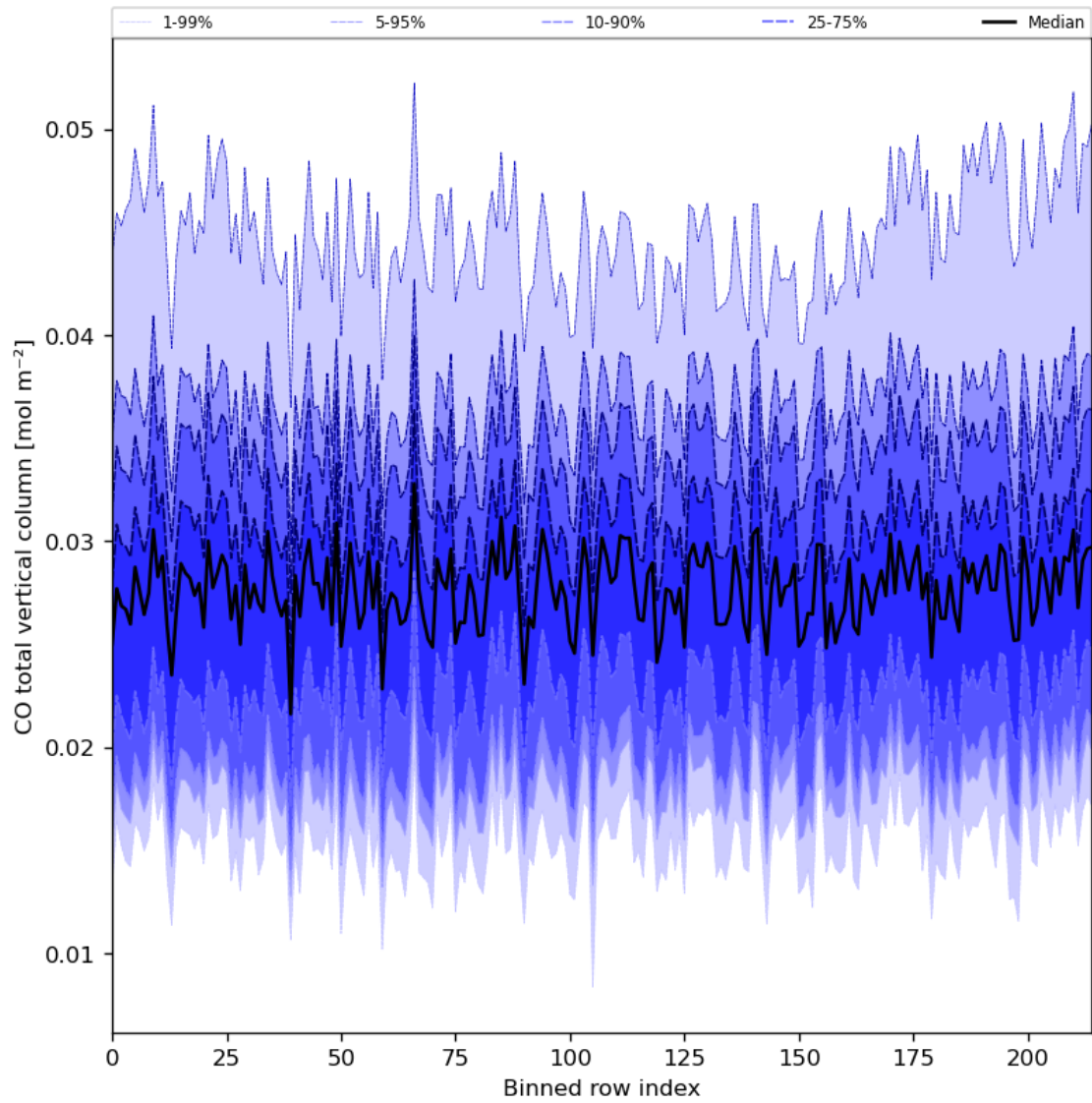
Figure 26: Along track statistics of “CO total vertical column” for 2024-06-09 to 2024-06-11
