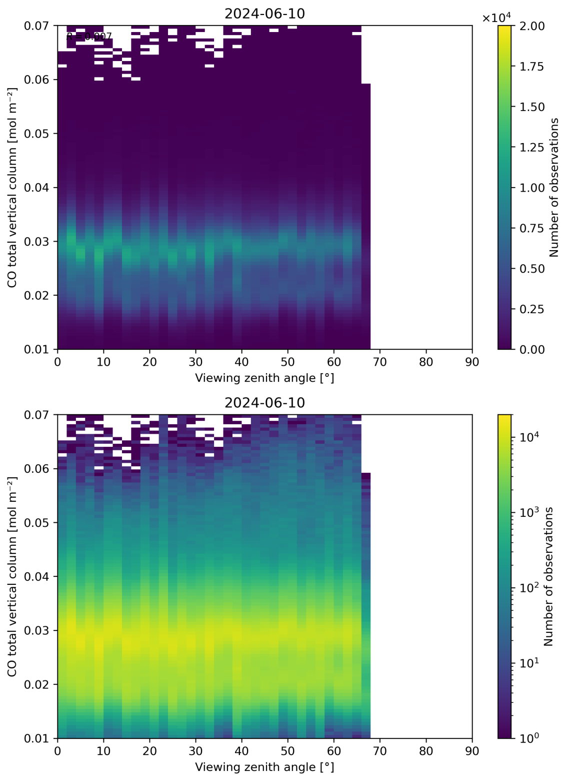
Figure 69: Scatter density plot of “Viewing zenith angle” against “CO total vertical column” for 2024-06-09 to 2024-06-11.
