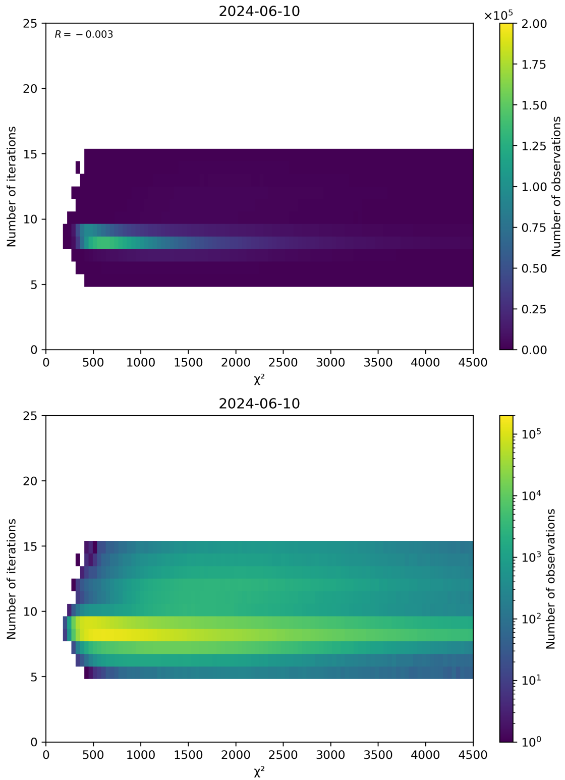
Figure 49: Scatter density plot of “ \chi^2 ” against “Number of iterations” for 2024-06-09 to 2024-06-11.
