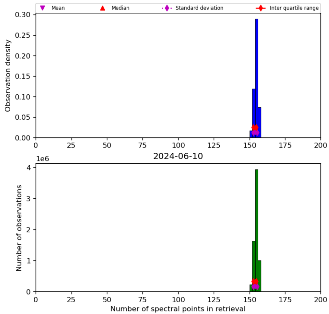
Figure 21: Histogram of “Number of spectral points in retrieval” for 2024-06-09 to 2024-06-11
