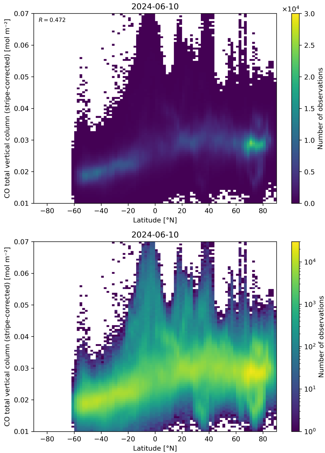
Figure 52: Scatter density plot of “Latitude” against “CO total vertical column (stripe-corrected)” for 2024-06-09 to 2024-06-11.
