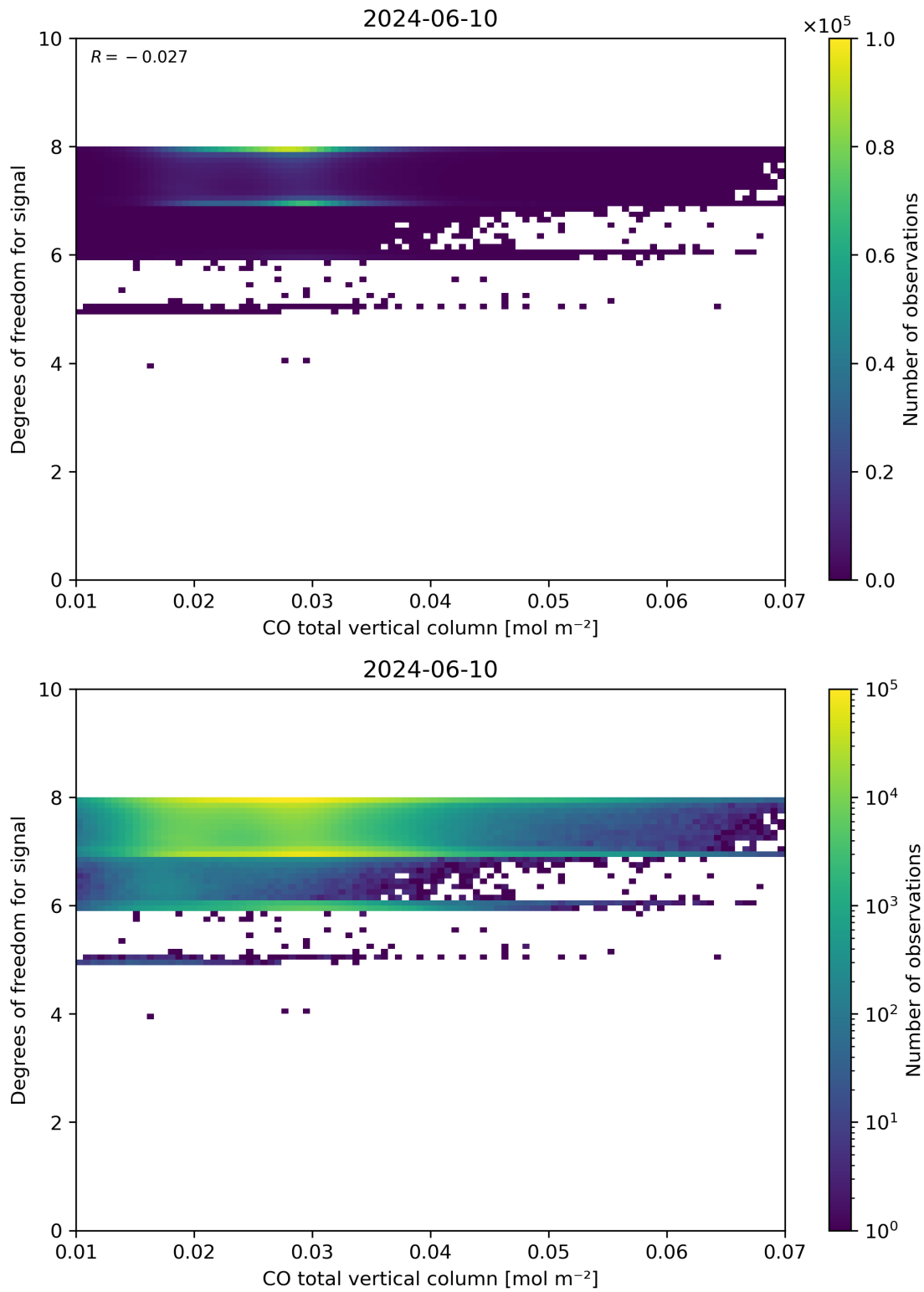
Figure 41: Scatter density plot of “CO total vertical column” against “Degrees of freedom for signal” for 2024-06-09 to 2024-06-11.
