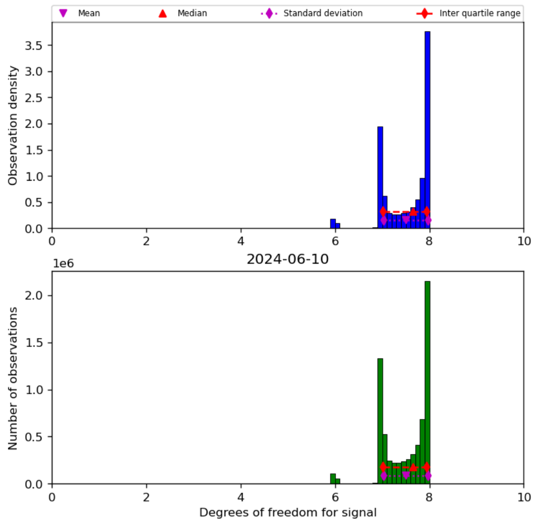
Figure 23: Histogram of “Degrees of freedom for signal” for 2024-06-09 to 2024-06-11
