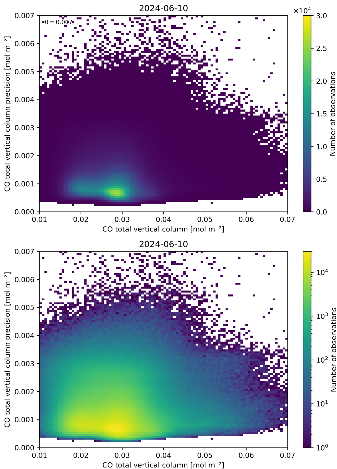
Figure 34: Scatter density plot of “CO total vertical column” against “CO total vertical column precision” for 2024-06-09 to 2024-06-11.
