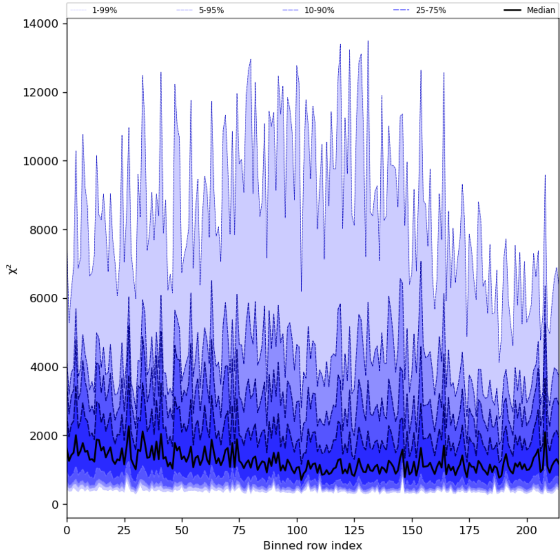
Figure 30: Along track statistics of “ \chi^2 ” for 2024-06-09 to 2024-06-11
