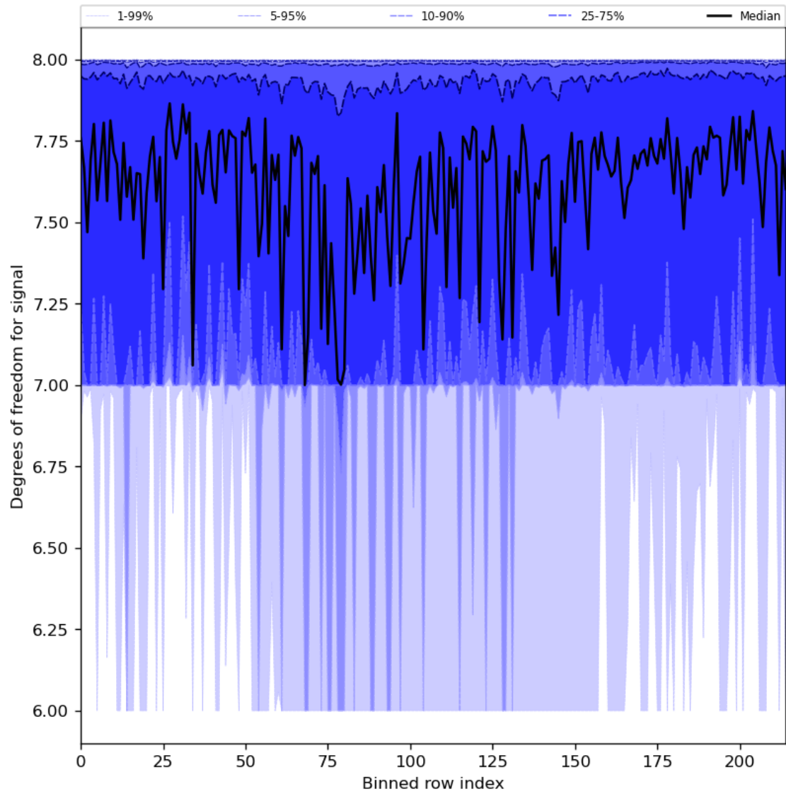
Figure 31: Along track statistics of “Degrees of freedom for signal” for 2024-06-09 to 2024-06-11
