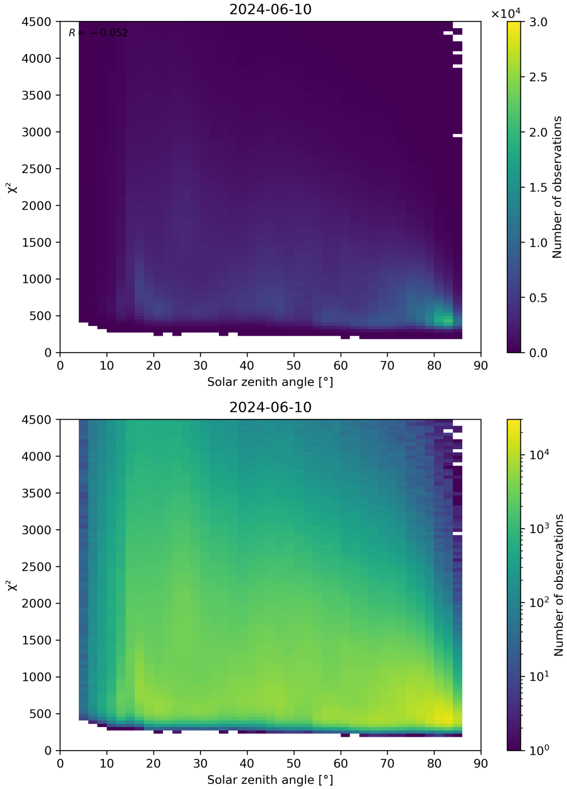
Figure 64: Scatter density plot of “Solar zenith angle” against “ \chi^2 ” for 2024-06-09 to 2024-06-11.
