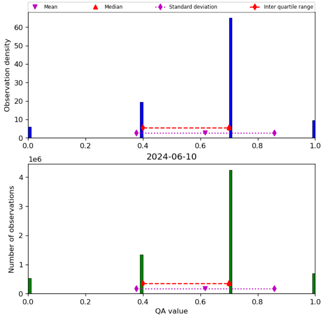
Figure 17: Histogram of “QA value” for 2024-06-09 to 2024-06-11
