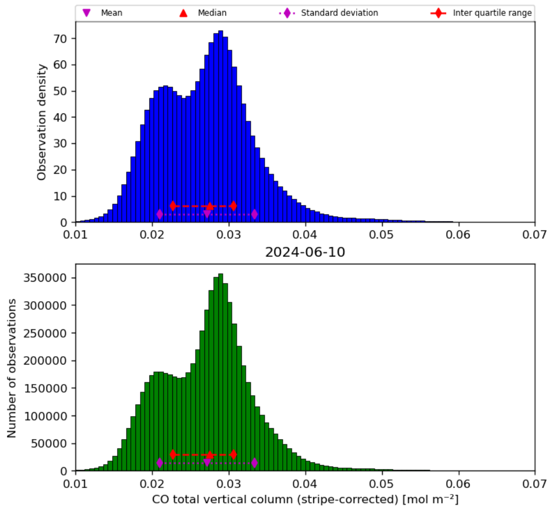
Figure 19: Histogram of “CO total vertical column (stripe-corrected)” for 2024-06-09 to 2024-06-11
