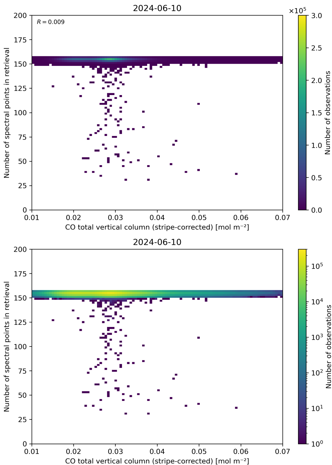
Figure 40: Scatter density plot of “CO total vertical column (stripe-corrected)” against “Number of spectral points in retrieval” for 2024-06-09 to 2024-06-11.
