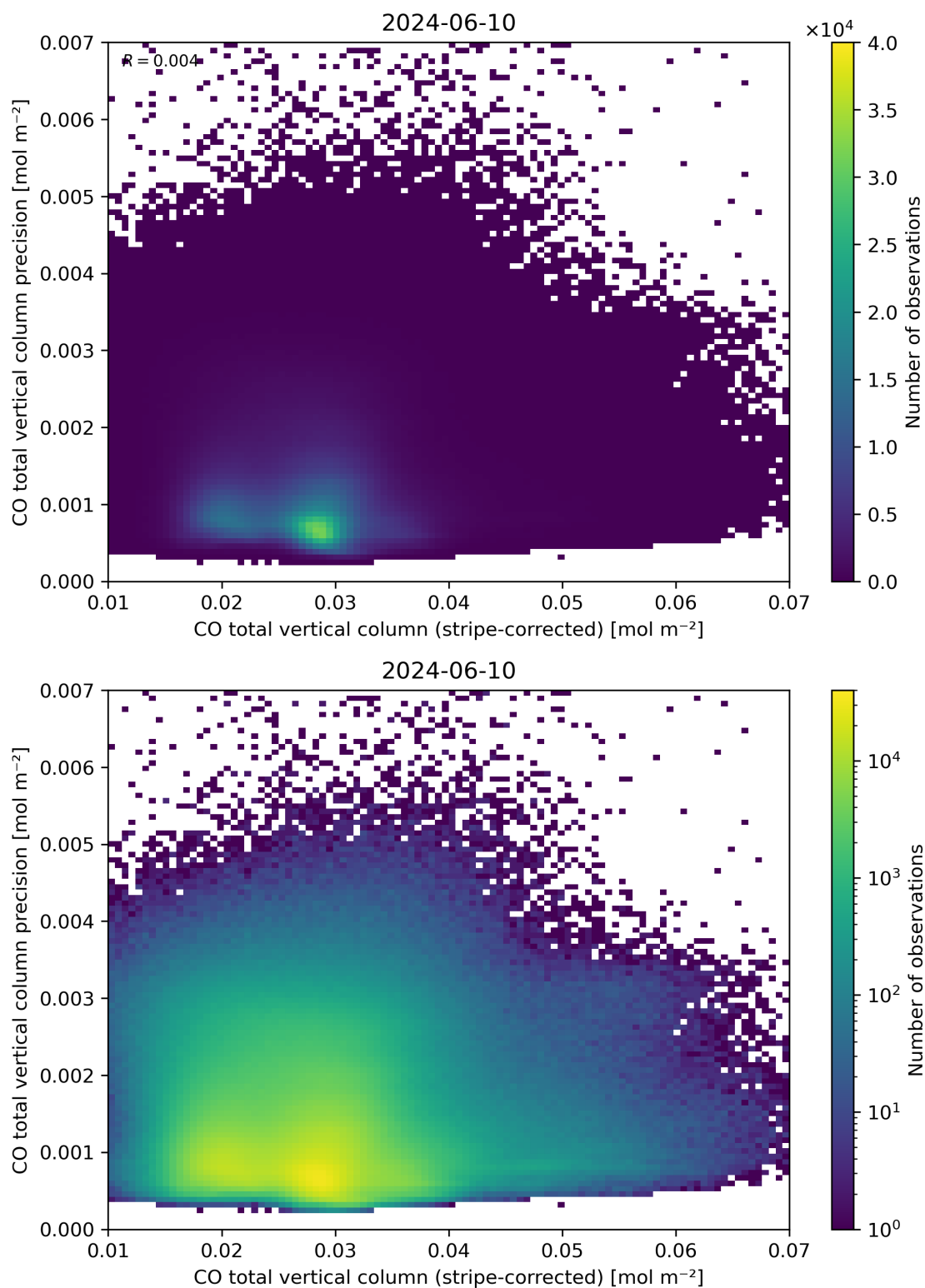
Figure 36: Scatter density plot of “CO total vertical column (stripe-corrected)” against “CO total vertical column precision” for 2024-06-09 to 2024-06-11.
