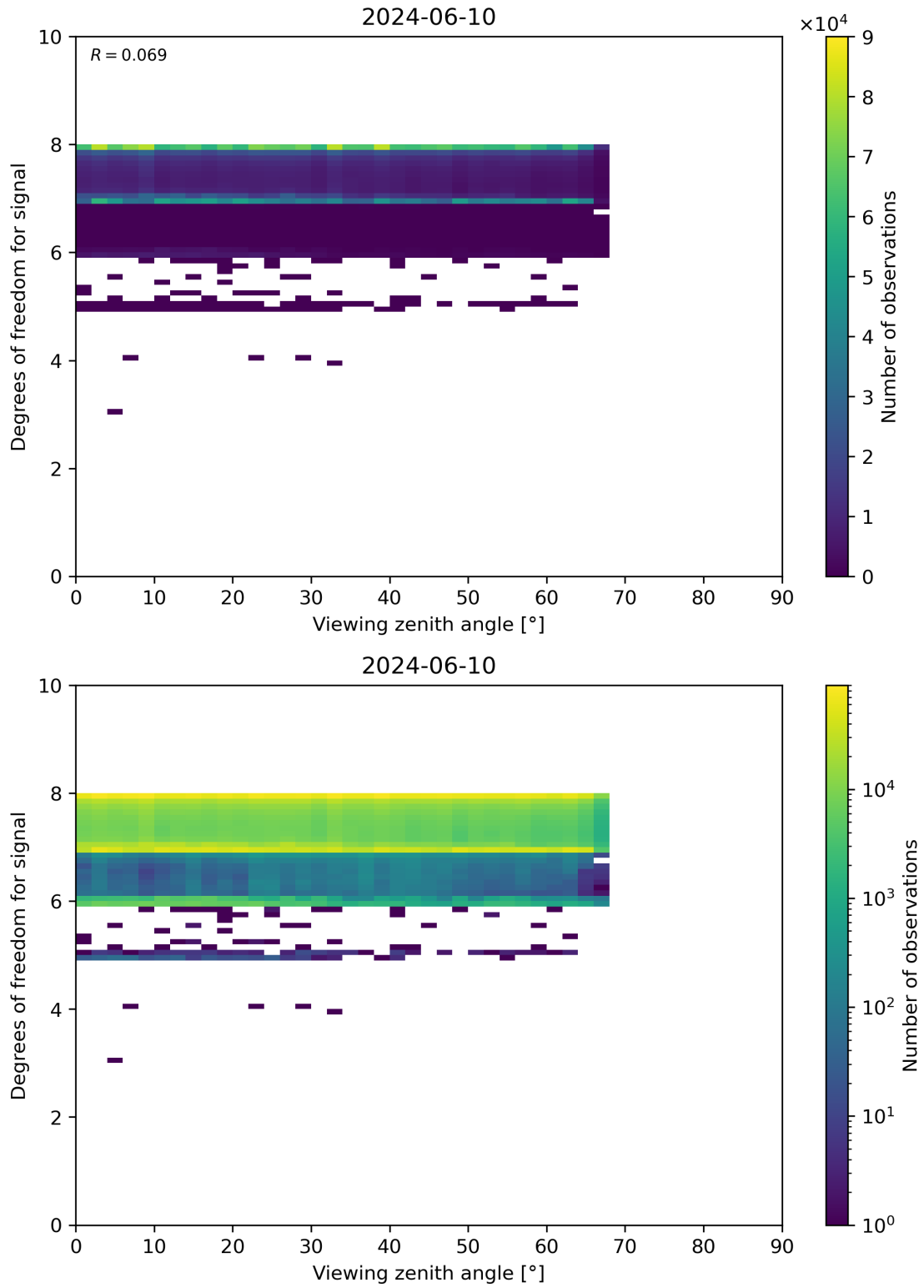
Figure 73: Scatter density plot of “Viewing zenith angle” against “Degrees of freedom for signal” for 2024-06-09 to 2024-06-11.
