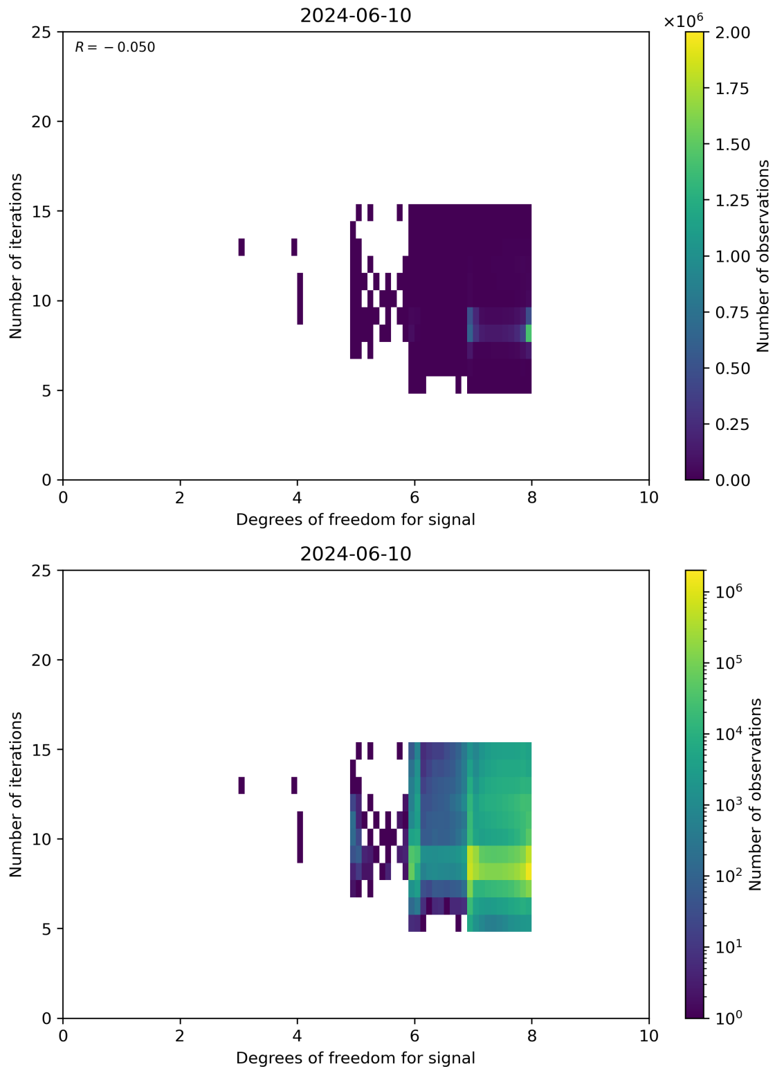
Figure 50: Scatter density plot of “Degrees of freedom for signal” against “Number of iterations” for 2024-06-09 to 2024-06-11.
