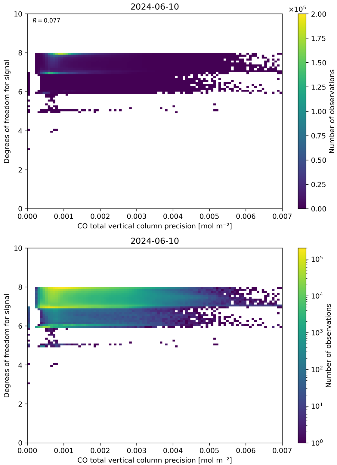
Figure 45: Scatter density plot of “CO total vertical column precision” against “Degrees of freedom for signal” for 2024-06-09 to 2024-06-11.
