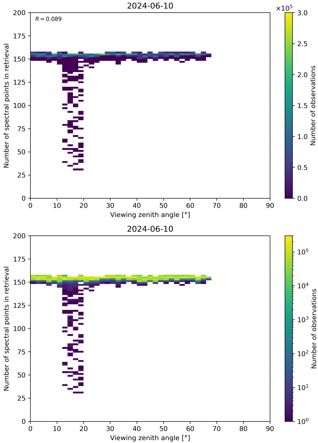
Figure 76: Scatter density plot of “Viewing zenith angle” against “Number of spectral points in retrieval” for 2024-06-09 to 2024-06-11.
