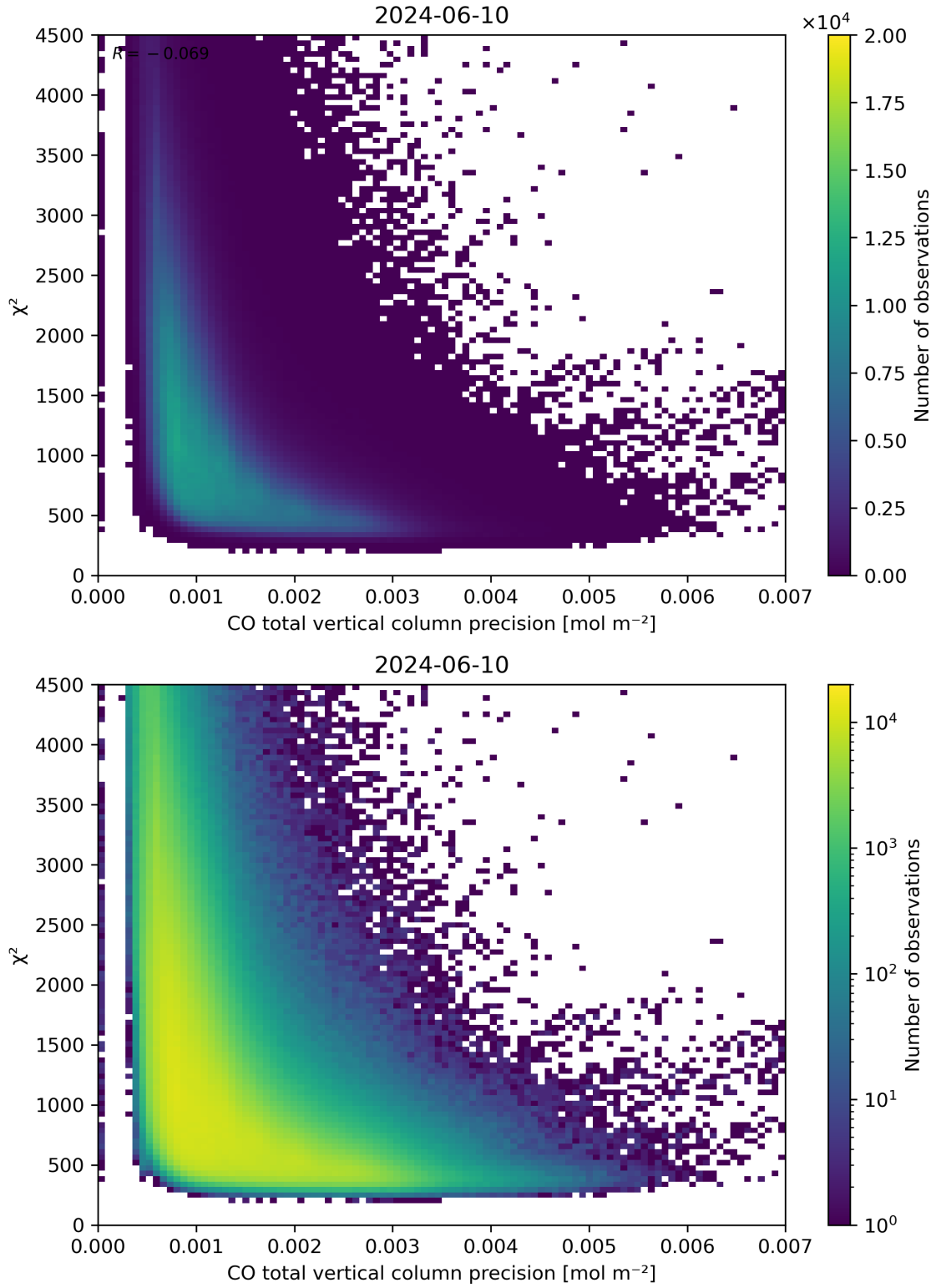
Figure 44: Scatter density plot of “CO total vertical column precision” against “ \chi^2 ” for 2024-06-09 to 2024-06-11.
