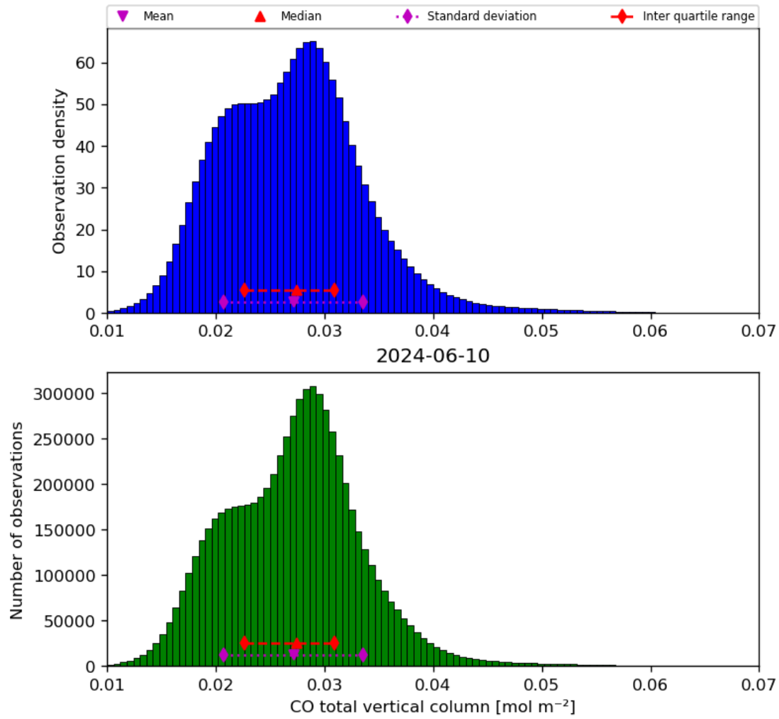
Figure 18: Histogram of “CO total vertical column” for 2024-06-09 to 2024-06-11
