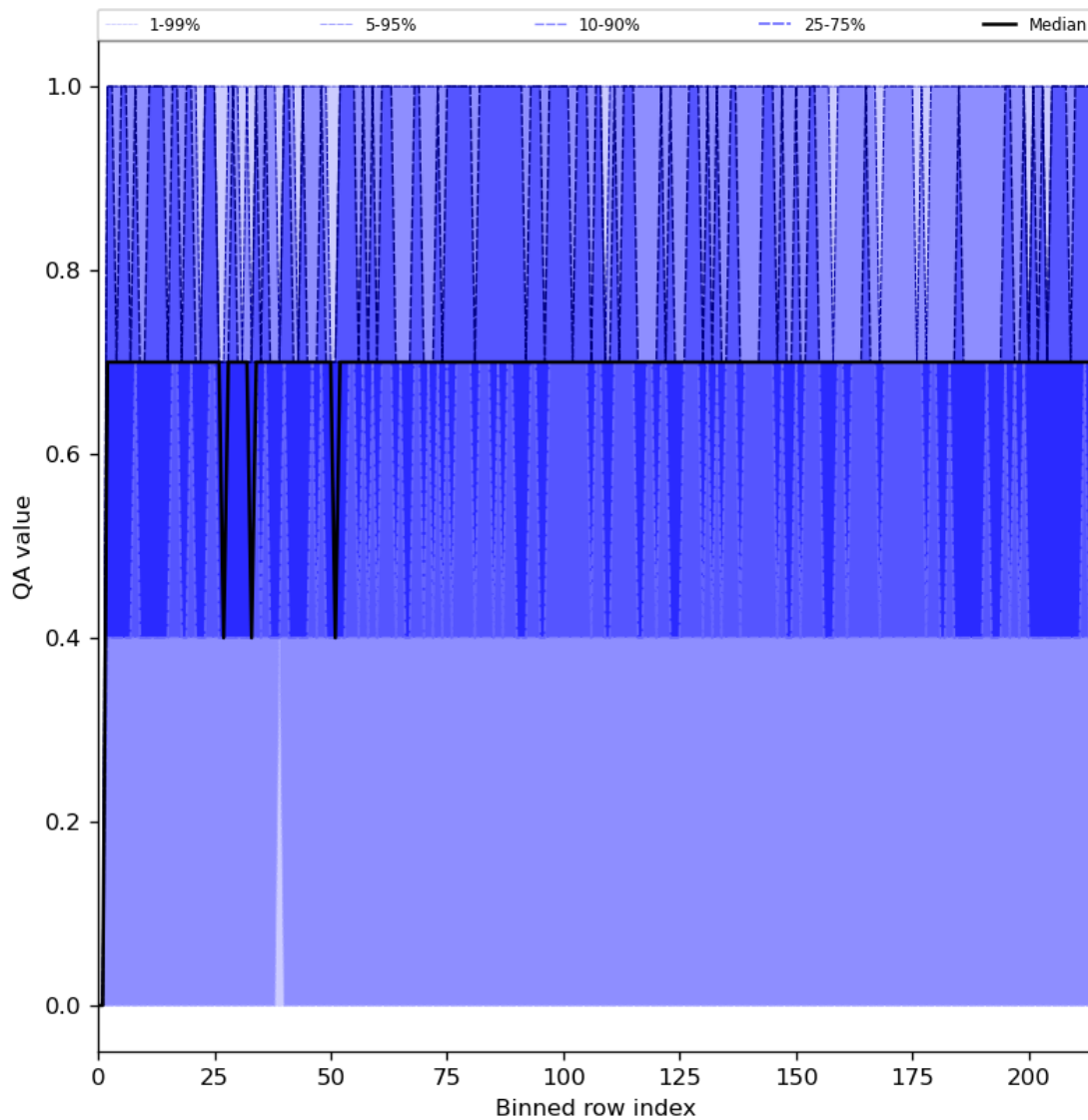
Figure 25: Along track statistics of “QA value” for 2024-06-09 to 2024-06-11
