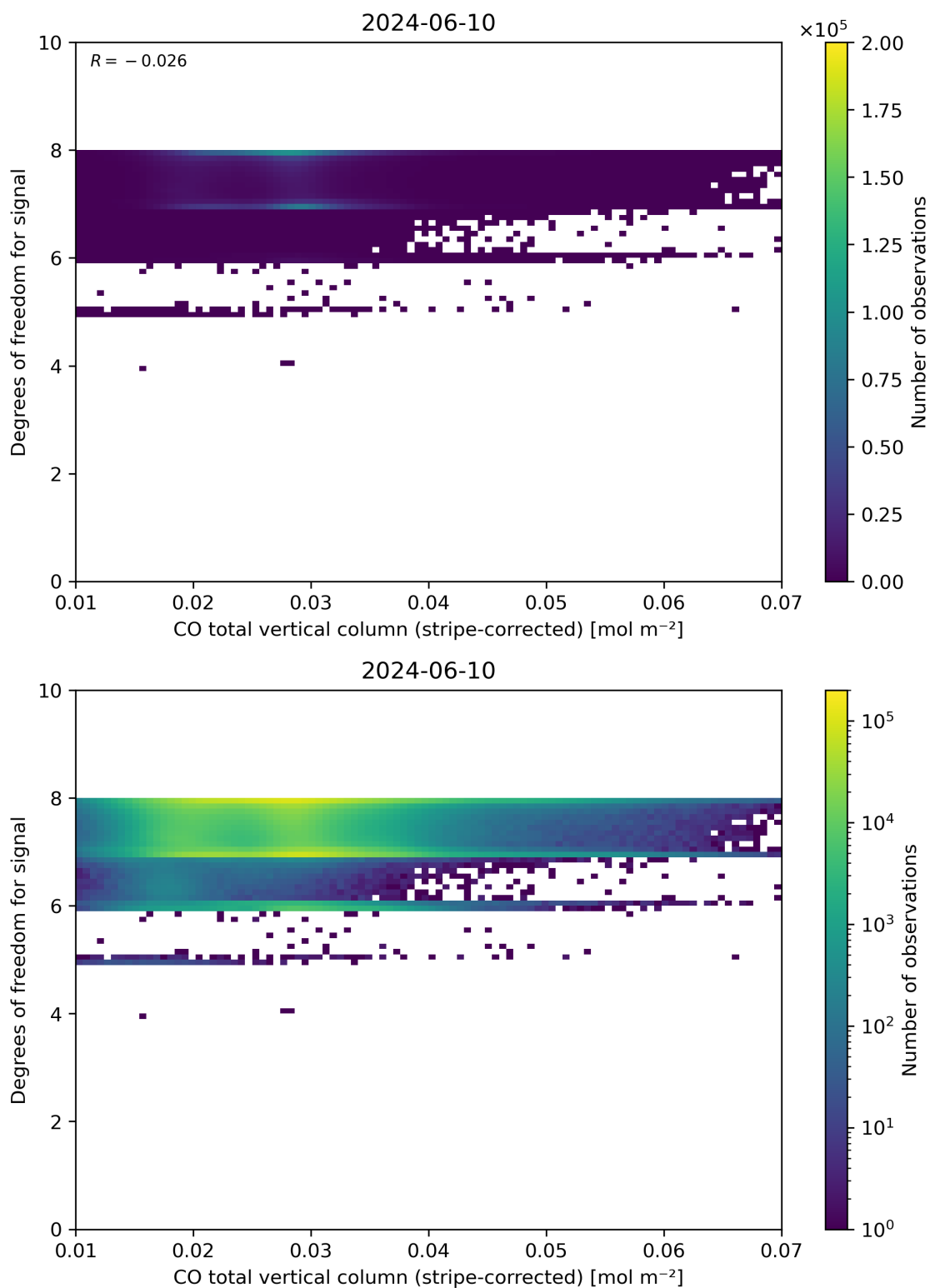
Figure 38: Scatter density plot of “CO total vertical column (stripe-corrected)” against “Degrees of freedom for signal” for 2024-06-09 to 2024-06-11.
