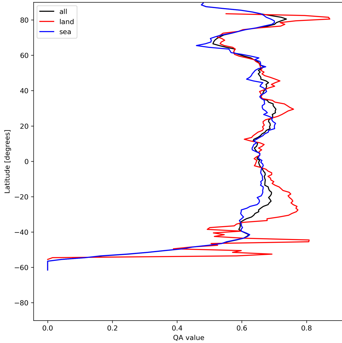
Figure 9: Zonal average of “QA value” for 2024-06-09 to 2024-06-11.
