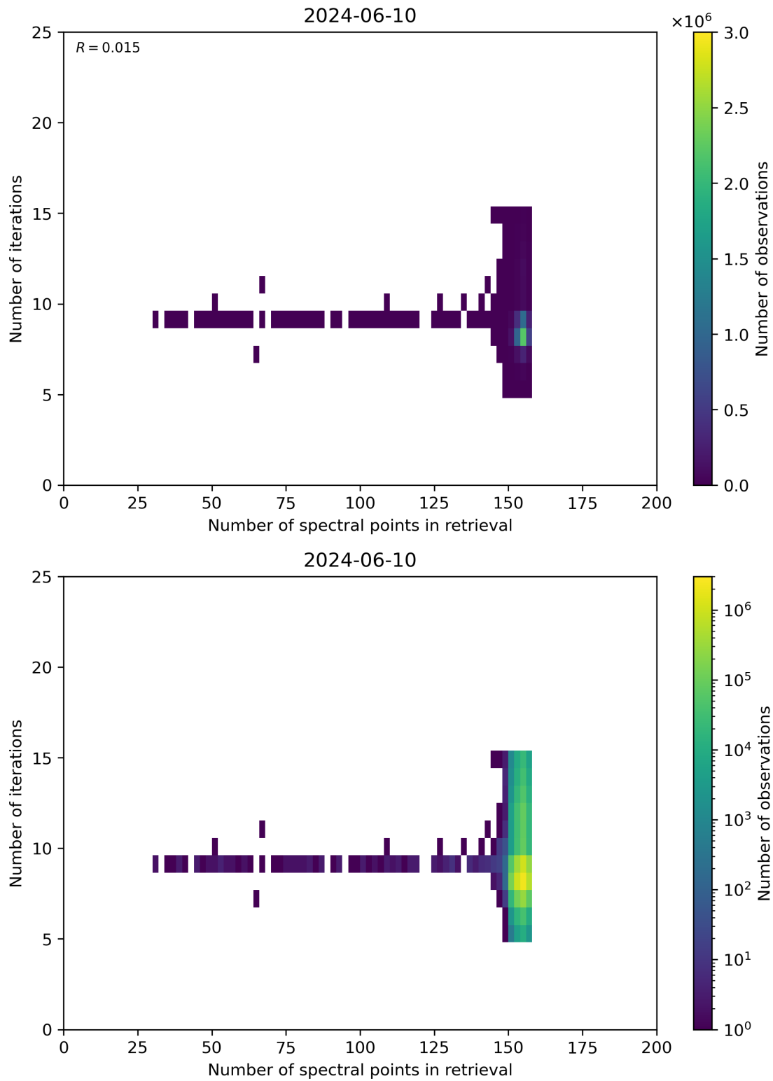
Figure 60: Scatter density plot of “Number of spectral points in retrieval” against “Number of iterations” for 2024-06-09 to 2024-06-11.
