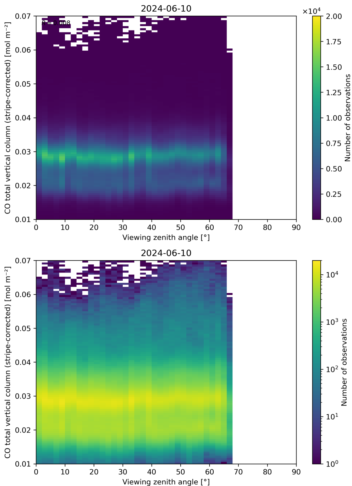
Figure 70: Scatter density plot of “Viewing zenith angle” against “CO total vertical column (stripe-corrected)” for 2024-06-09 to 2024-06-11.
