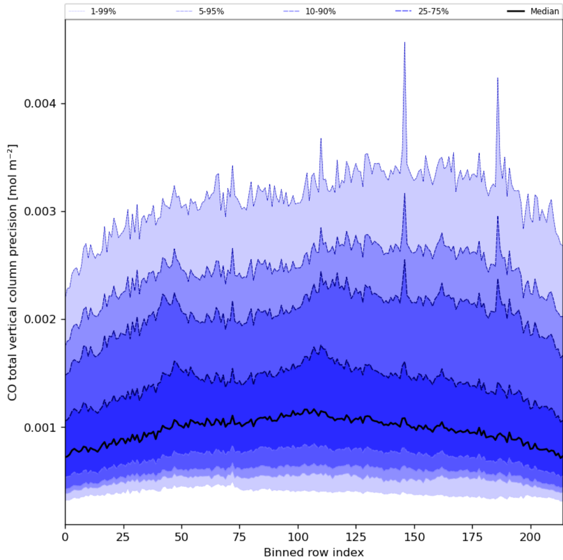
Figure 28: Along track statistics of “CO total vertical column precision” for 2024-06-09 to 2024-06-11
