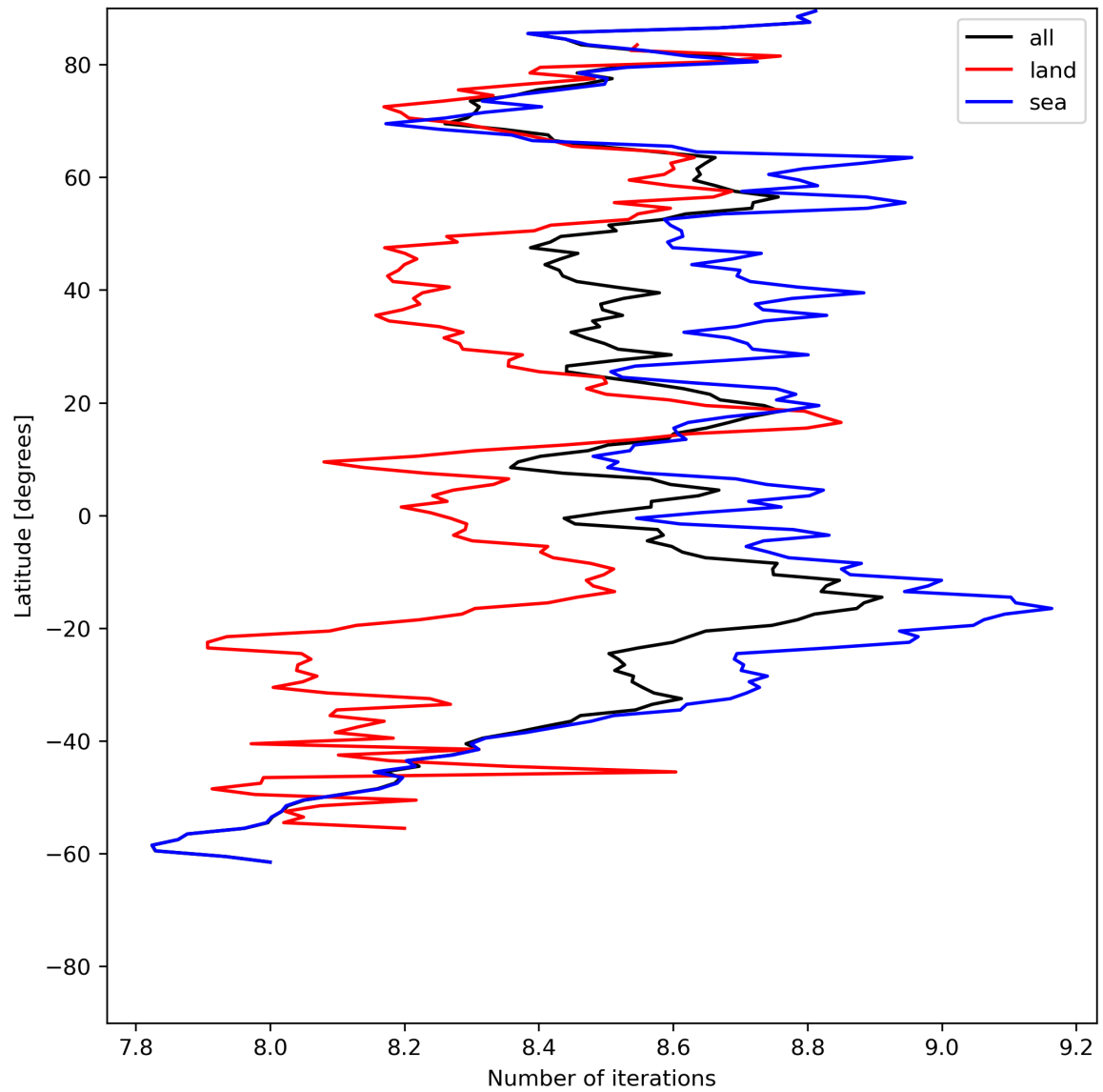
Figure 16: Zonal average of “Number of iterations” for 2024-06-09 to 2024-06-11.
