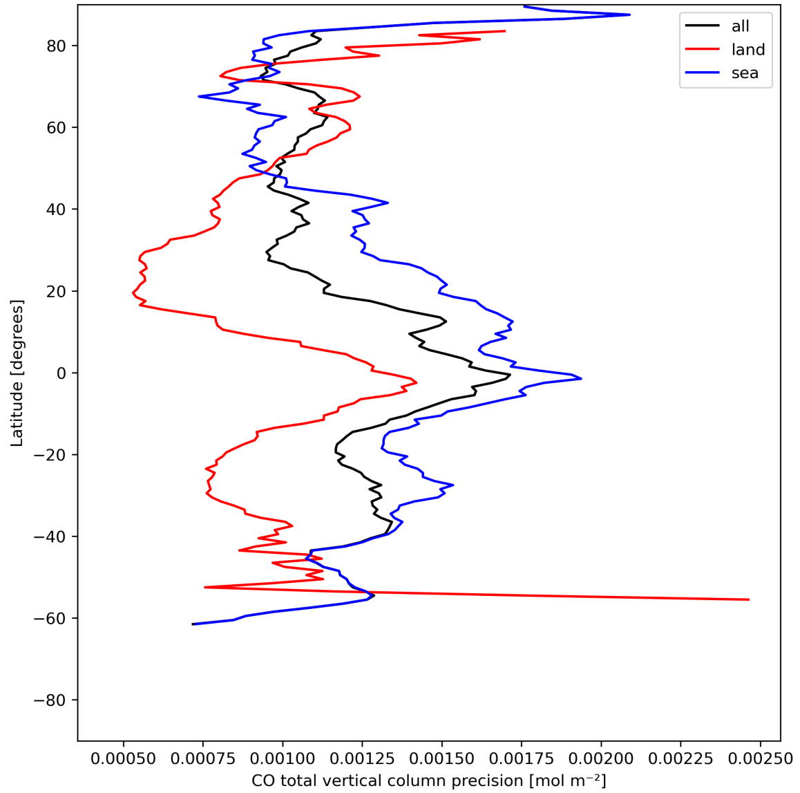
Figure 12: Zonal average of “CO total vertical column precision” for 2024-06-09 to 2024-06-11.
