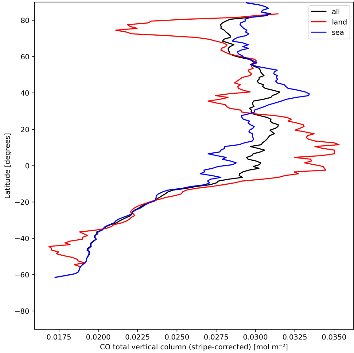
Figure 11: Zonal average of “CO total vertical column (stripe-corrected)” for 2024-06-09 to 2024-06-11.
