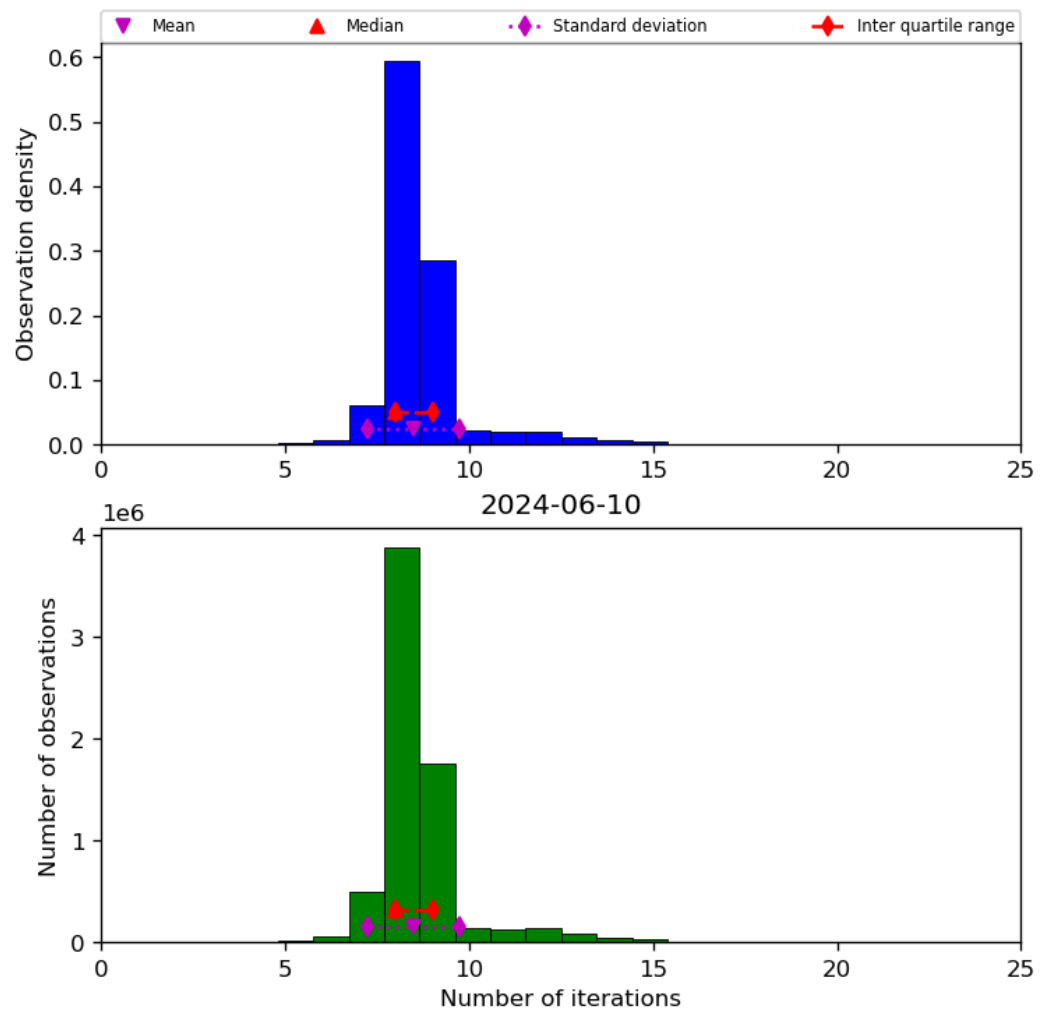
Figure 24: Histogram of “Number of iterations” for 2024-06-09 to 2024-06-11
