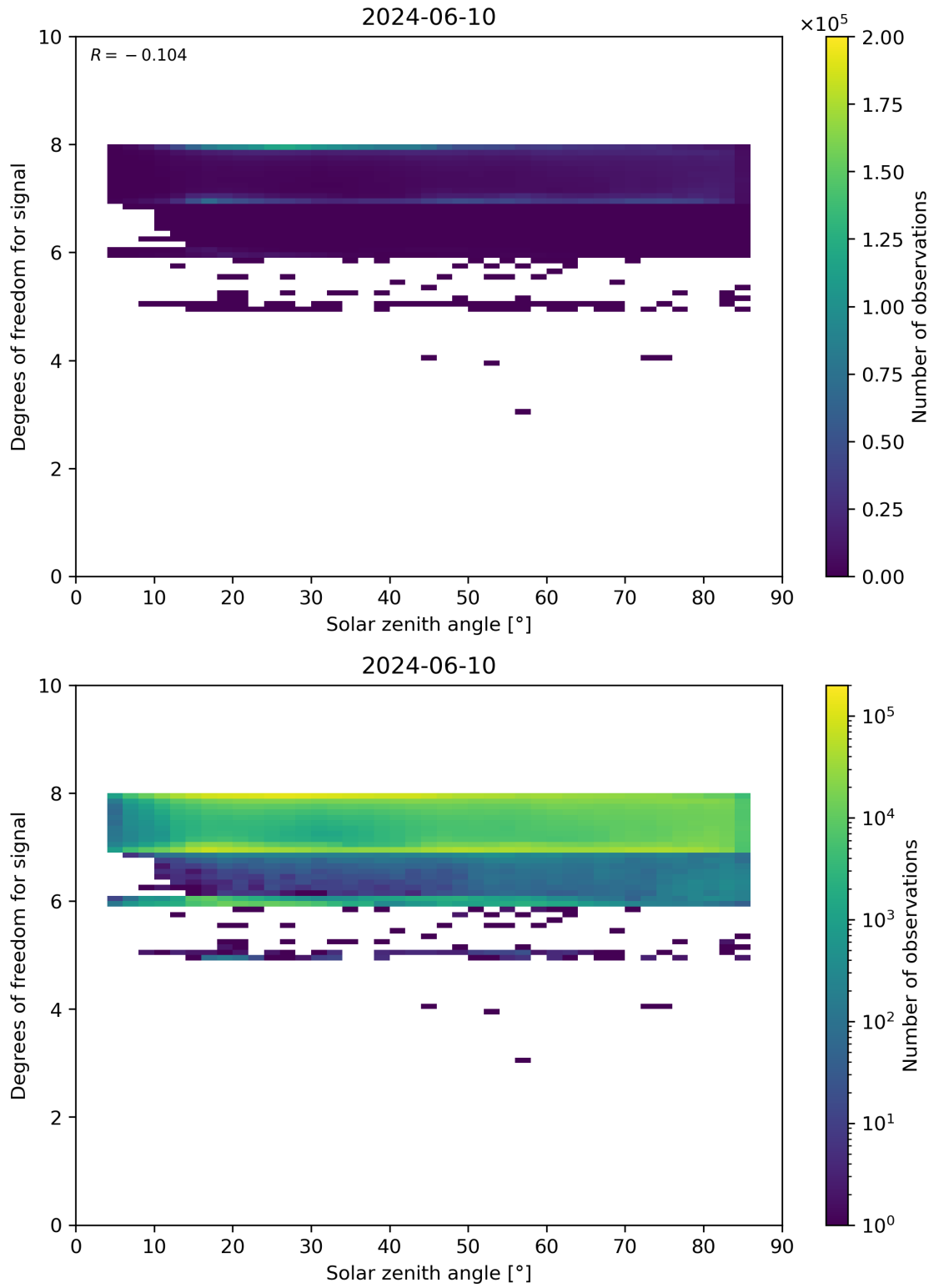
Figure 65: Scatter density plot of “Solar zenith angle” against “Degrees of freedom for signal” for 2024-06-09 to 2024-06-11.
