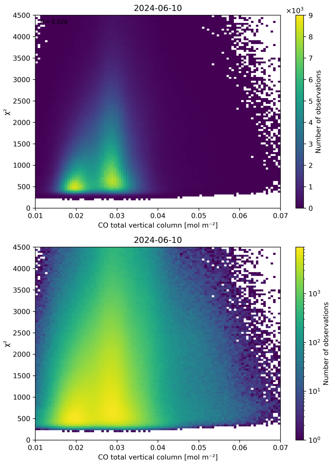
Figure 35: Scatter density plot of “CO total vertical column” against “ \chi^2 ” for 2024-06-09 to 2024-06-11.
