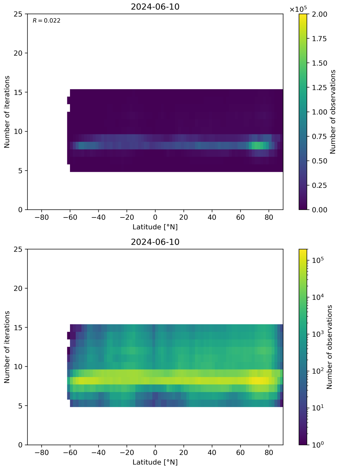
Figure 56: Scatter density plot of “Latitude” against “Number of iterations” for 2024-06-09 to 2024-06-11.
