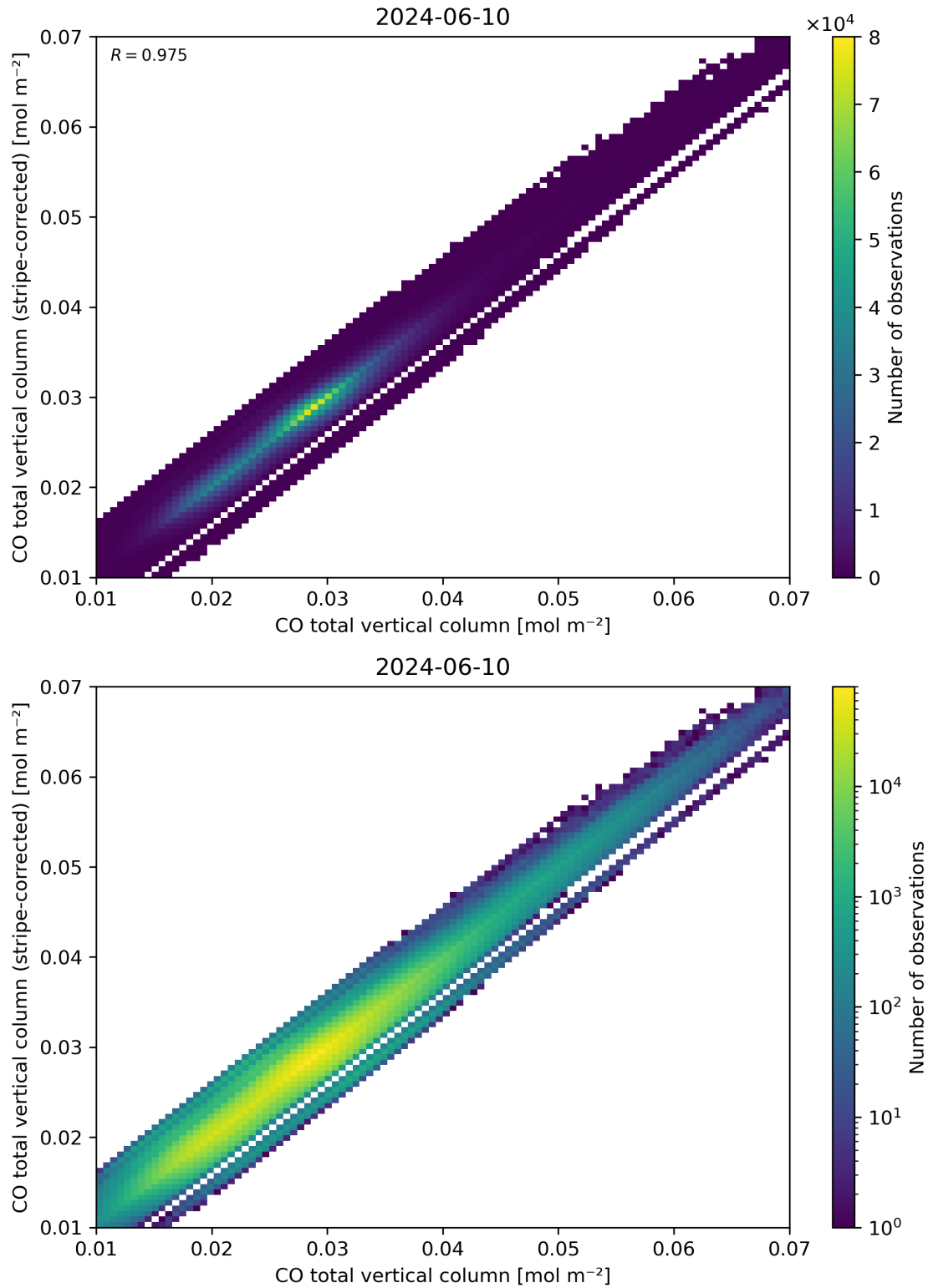
Figure 33: Scatter density plot of “CO total vertical column” against “CO total vertical column (stripe-corrected)” for 2024-06-09 to 2024-06-11.
