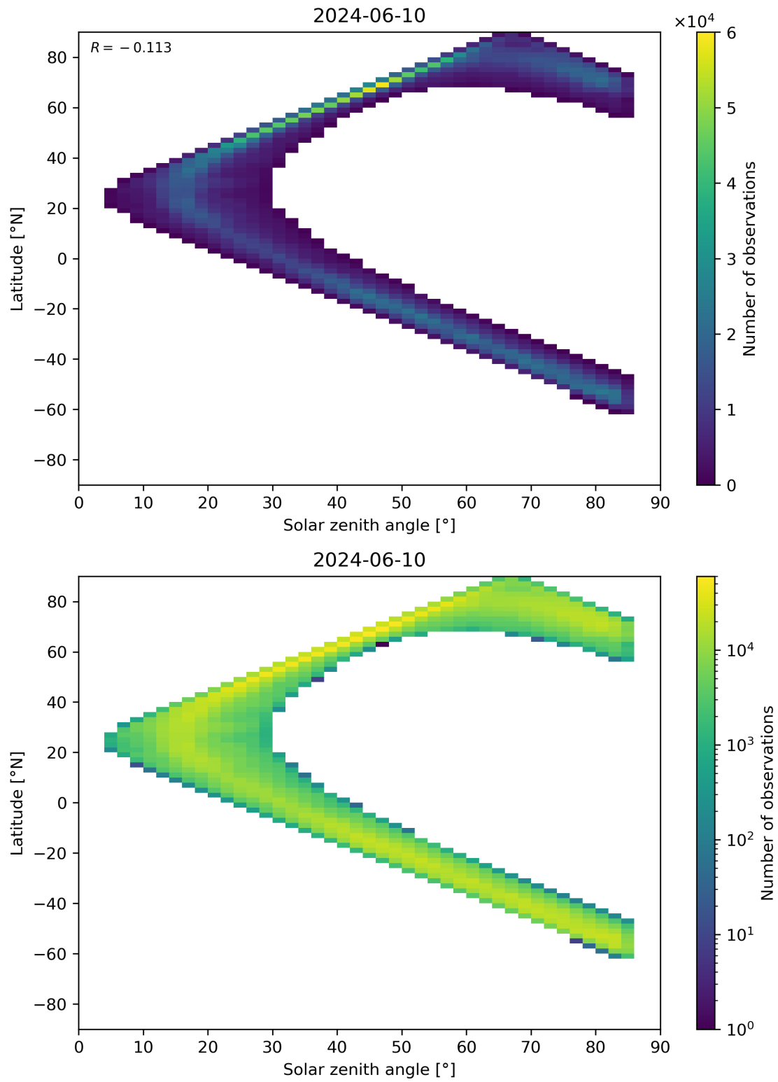
Figure 66: Scatter density plot of “Solar zenith angle” against “Latitude” for 2024-06-09 to 2024-06-11.
