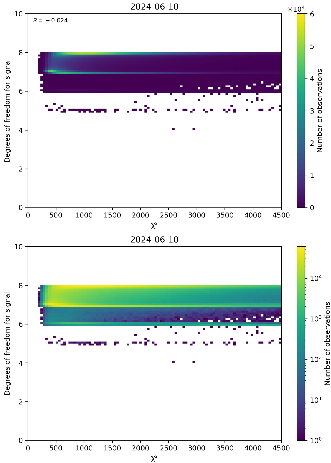
Figure 48: Scatter density plot of “ \chi^2 ” against “Degrees of freedom for signal” for 2024-06-09 to 2024-06-11.
