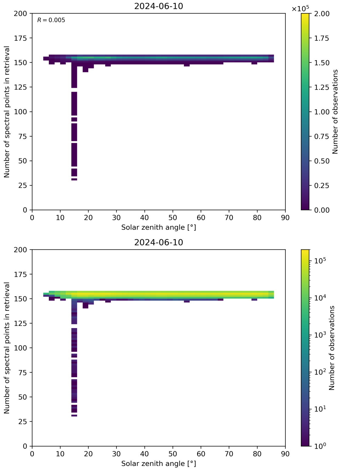
Figure 68: Scatter density plot of “Solar zenith angle” against “Number of spectral points in retrieval” for 2024-06-09 to 2024-06-11.
