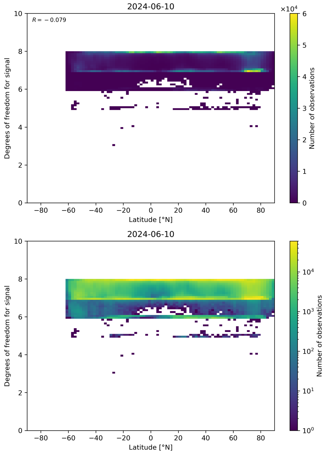
Figure 55: Scatter density plot of “Latitude” against “Degrees of freedom for signal” for 2024-06-09 to 2024-06-11.
