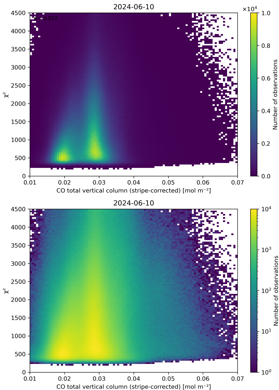
Figure 37: Scatter density plot of “CO total vertical column (stripe-corrected)” against “ \chi^2 ” for 2024-06-09 to 2024-06-11.
