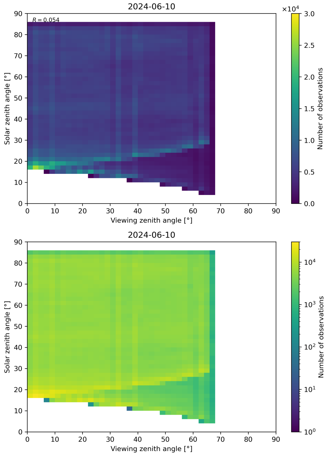
Figure 77: Scatter density plot of “Viewing zenith angle” against “Solar zenith angle” for 2024-06-09 to 2024-06-11.
