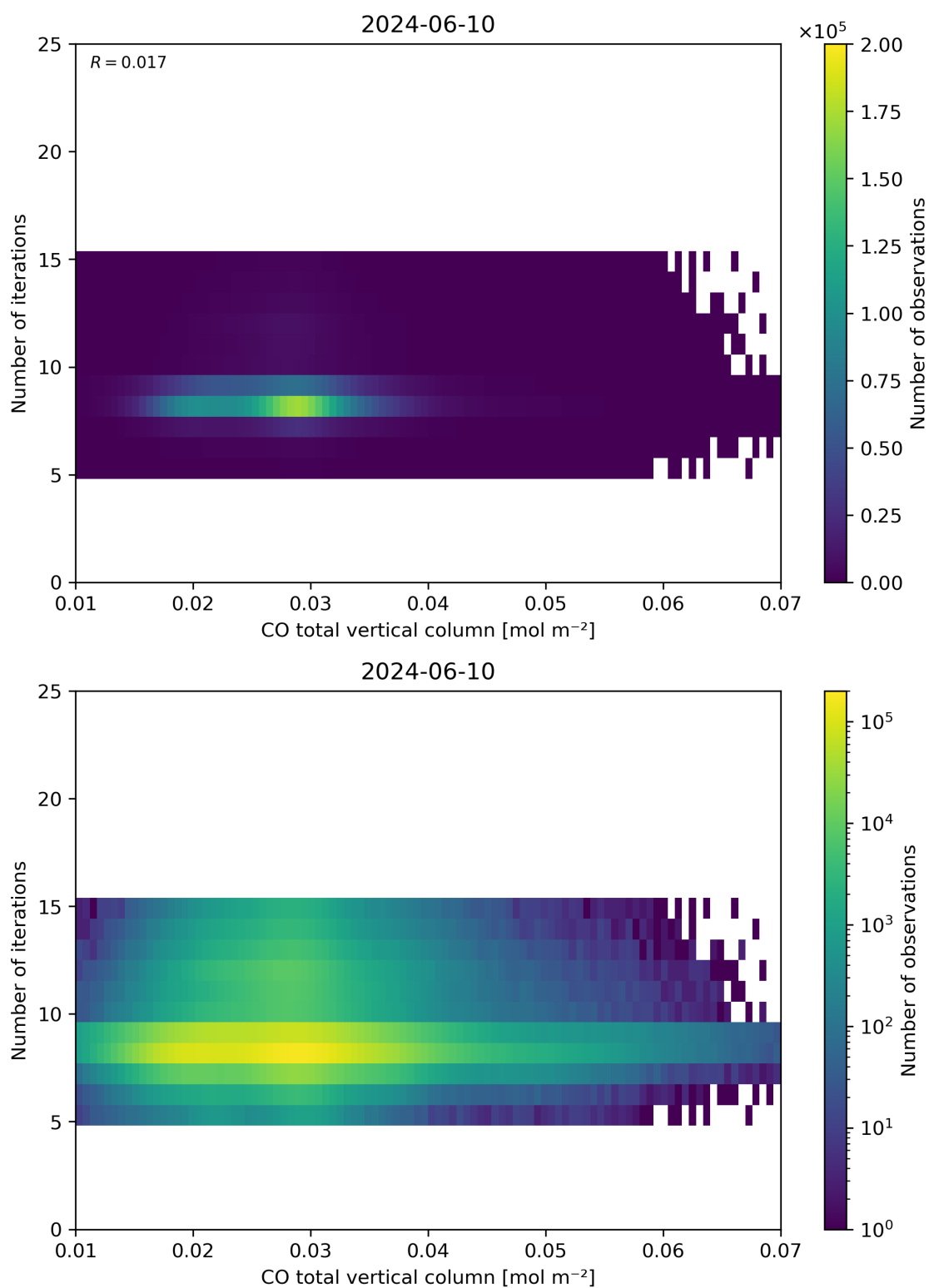
Figure 42: Scatter density plot of “CO total vertical column” against “Number of iterations” for 2024-06-09 to 2024-06-11.
