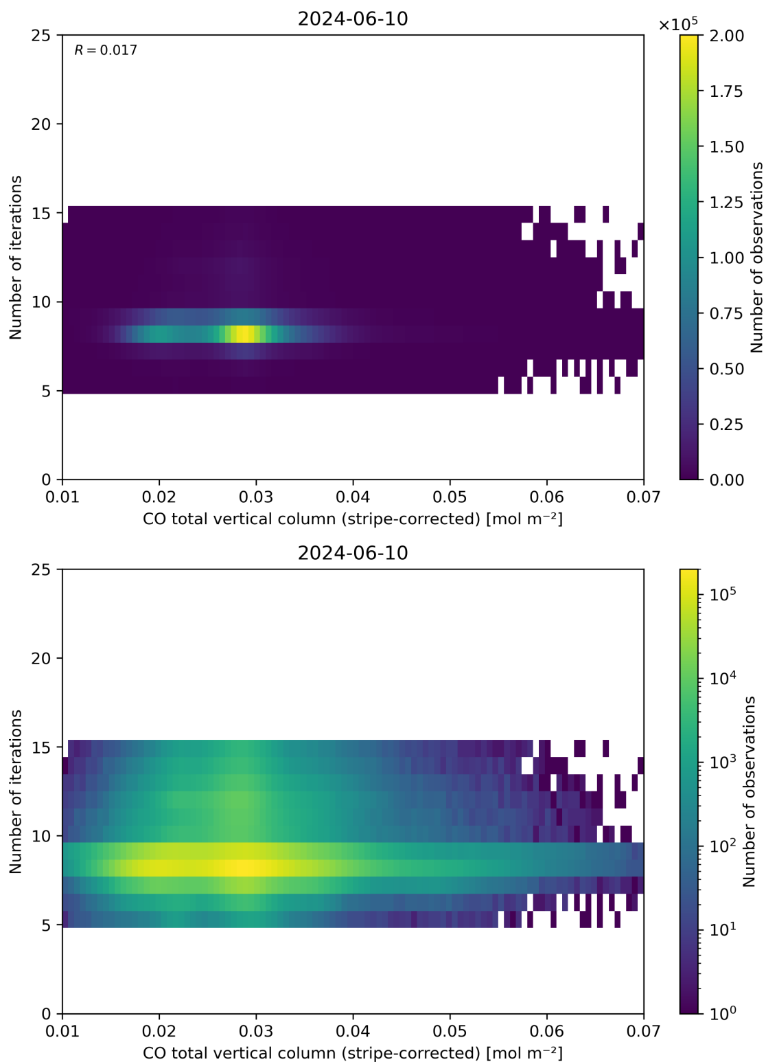
Figure 39: Scatter density plot of “CO total vertical column (stripe-corrected)” against “Number of iterations” for 2024-06-09 to 2024-06-11.
