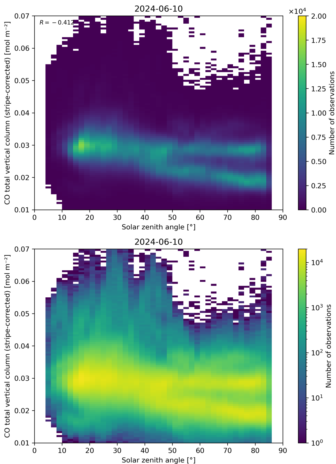
Figure 62: Scatter density plot of “Solar zenith angle” against “CO total vertical column (stripe-corrected)” for 2024-06-09 to 2024-06-11.
