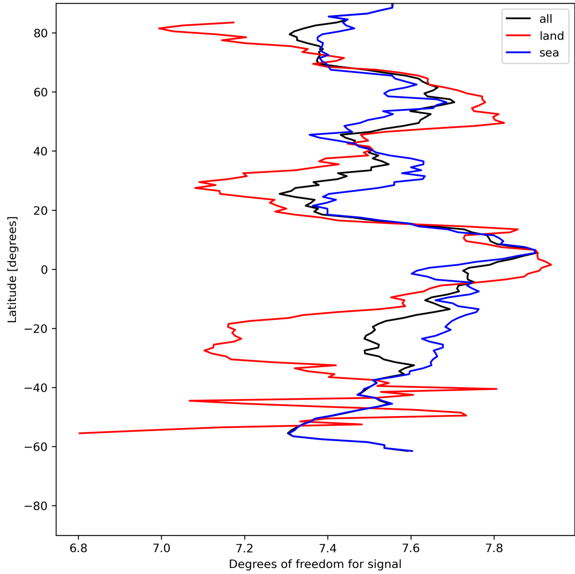
Figure 15: Zonal average of “Degrees of freedom for signal” for 2024-06-09 to 2024-06-11.
