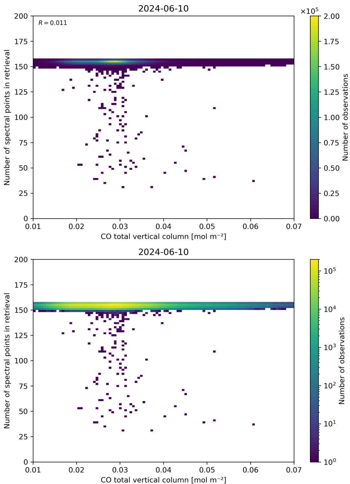
Figure 43: Scatter density plot of “CO total vertical column” against “Number of spectral points in retrieval” for 2024-06-09 to 2024-06-11.
