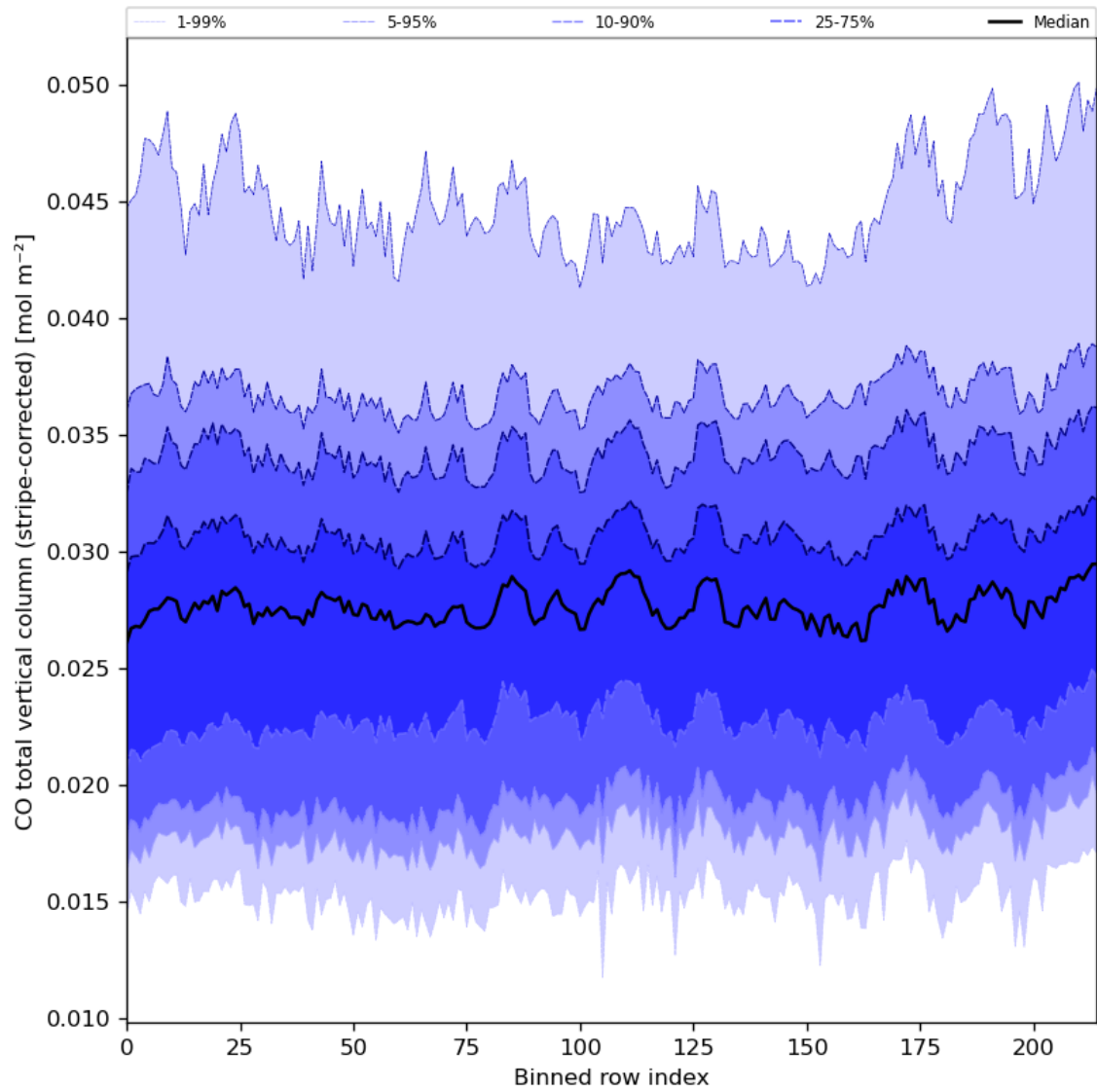
Figure 27: Along track statistics of “CO total vertical column (stripe-corrected)” for 2024-06-09 to 2024-06-11
