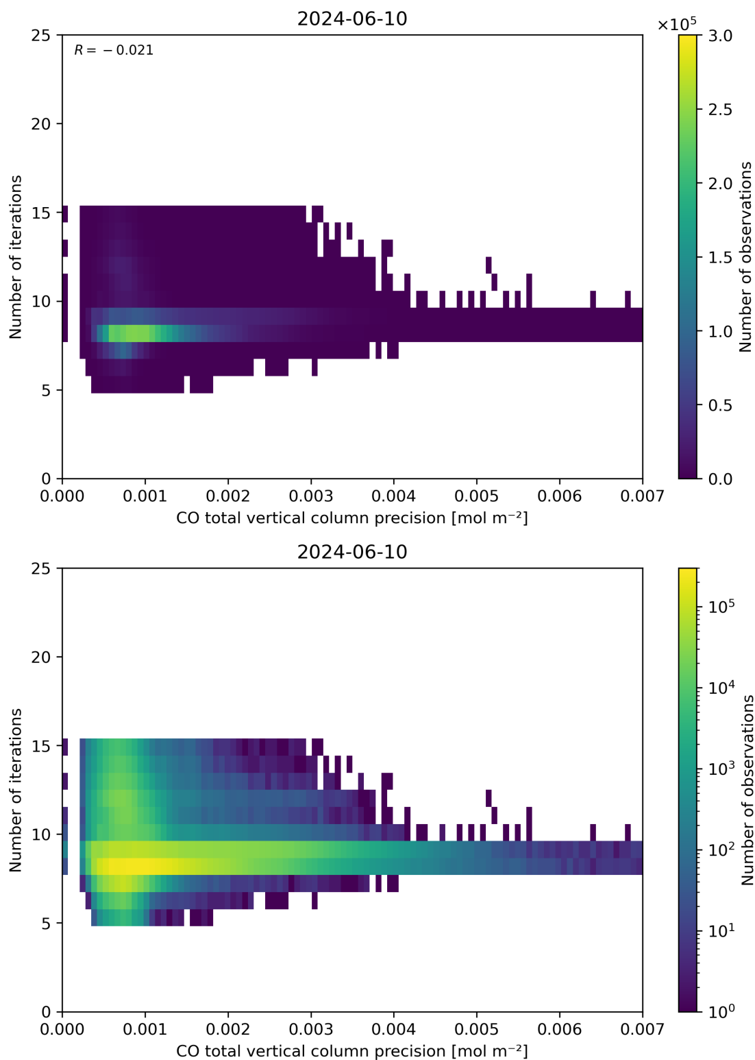
Figure 46: Scatter density plot of “CO total vertical column precision” against “Number of iterations” for 2024-06-09 to 2024-06-11.
