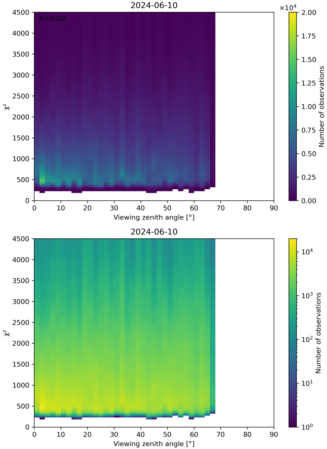
Figure 72: Scatter density plot of “Viewing zenith angle” against “ \chi^2 ” for 2024-06-09 to 2024-06-11.
