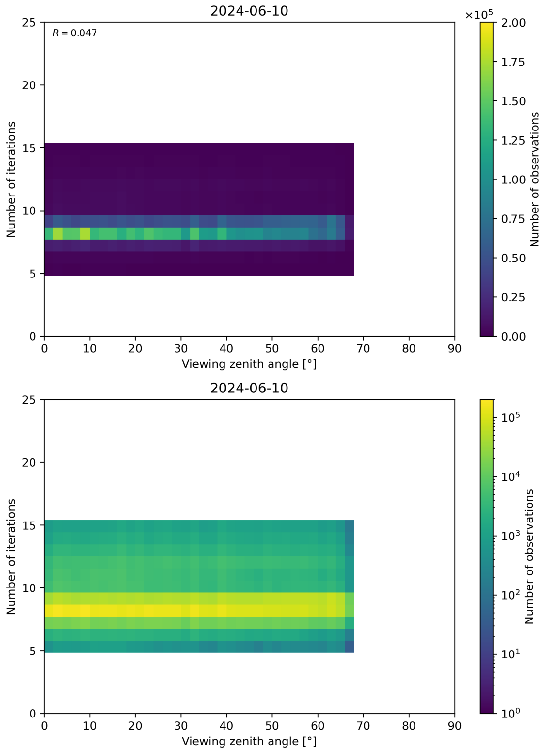
Figure 75: Scatter density plot of “Viewing zenith angle” against “Number of iterations” for 2024-06-09 to 2024-06-11.
