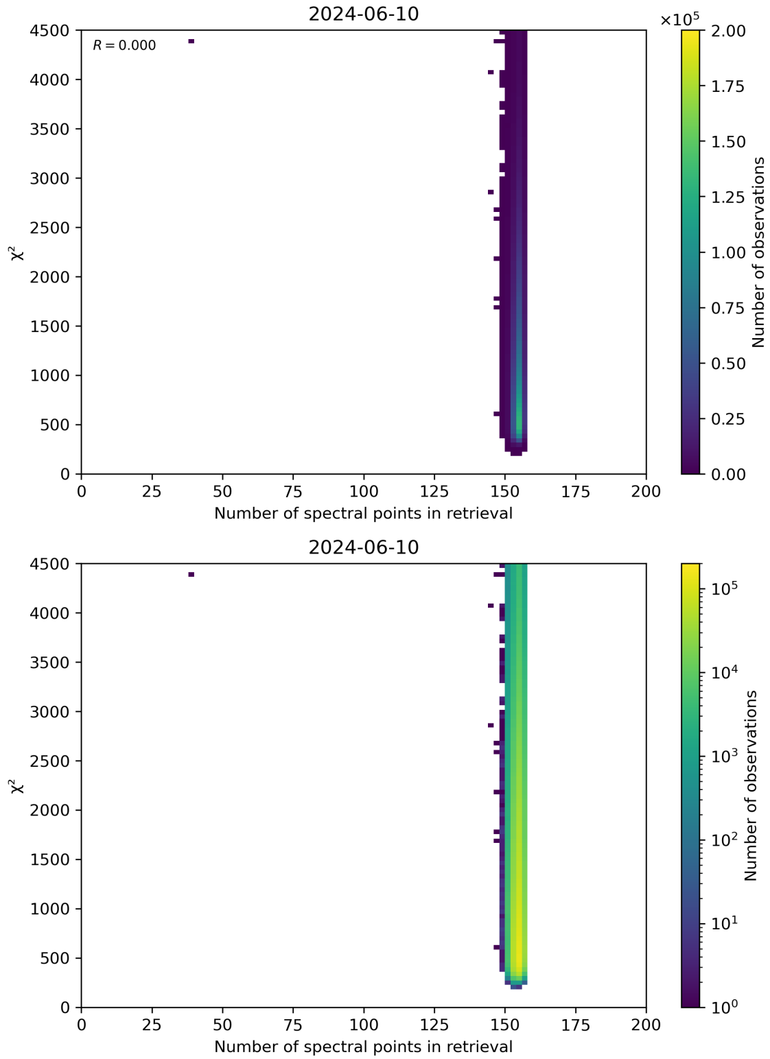
Figure 58: Scatter density plot of “Number of spectral points in retrieval” against “ \chi^2 ” for 2024-06-09 to 2024-06-11.
