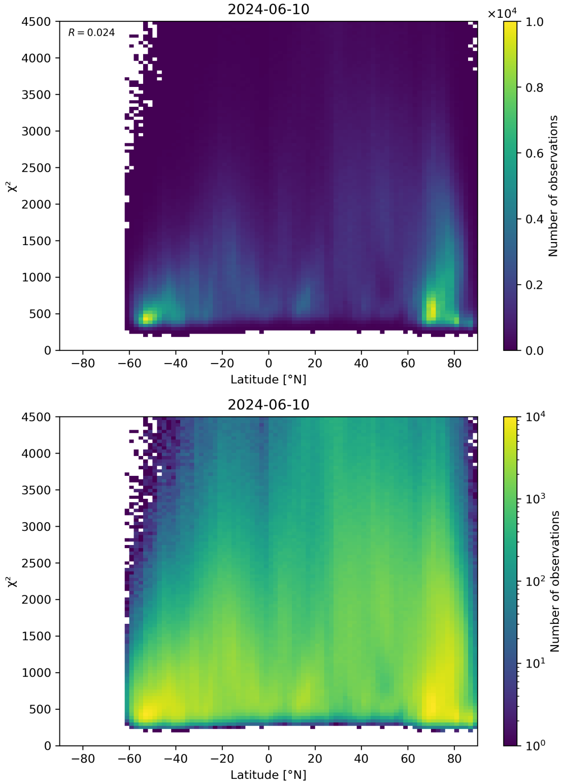
Figure 54: Scatter density plot of “Latitude” against “ \chi^2 ” for 2024-06-09 to 2024-06-11.
