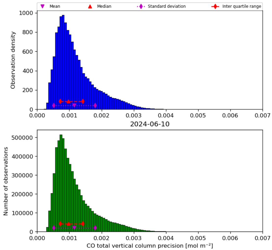
Figure 20: Histogram of “CO total vertical column precision” for 2024-06-09 to 2024-06-11
