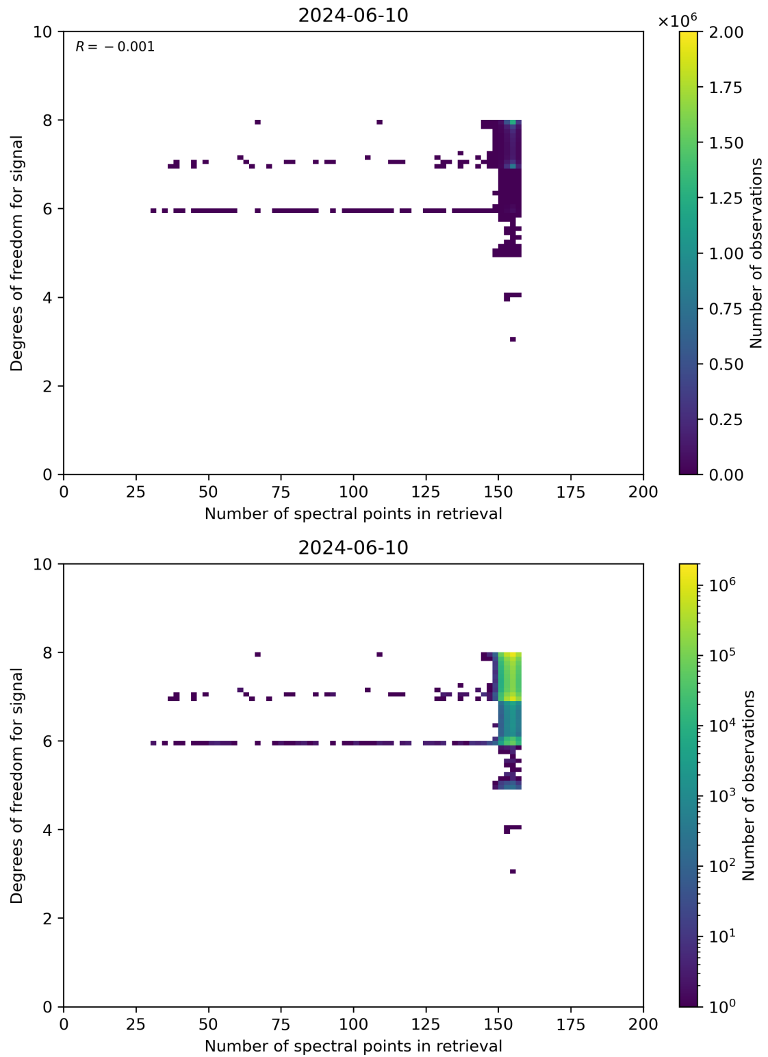
Figure 59: Scatter density plot of “Number of spectral points in retrieval” against “Degrees of freedom for signal” for 2024-06-09 to 2024-06-11.
