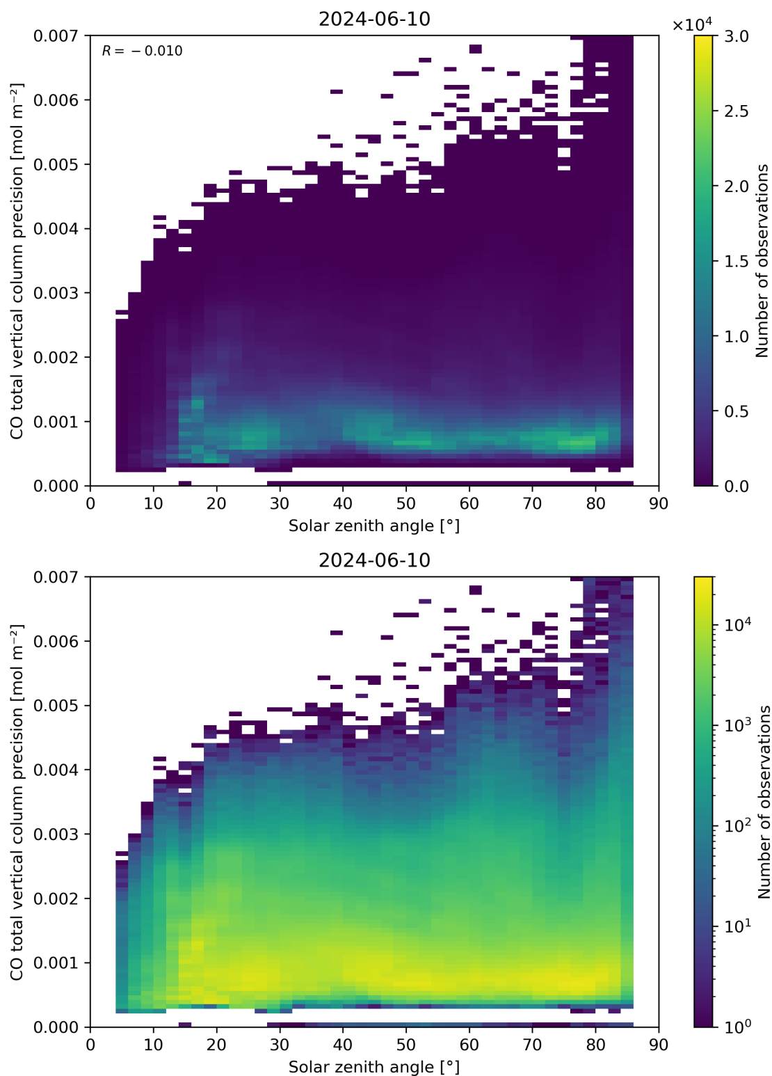
Figure 63: Scatter density plot of “Solar zenith angle” against “CO total vertical column precision” for 2024-06-09 to 2024-06-11.
