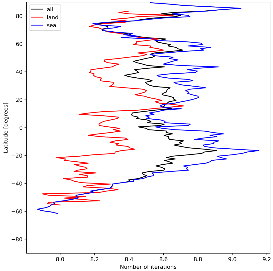
Figure 16: Zonal average of “Number of iterations” for 2024-06-10 to 2024-06-12.
