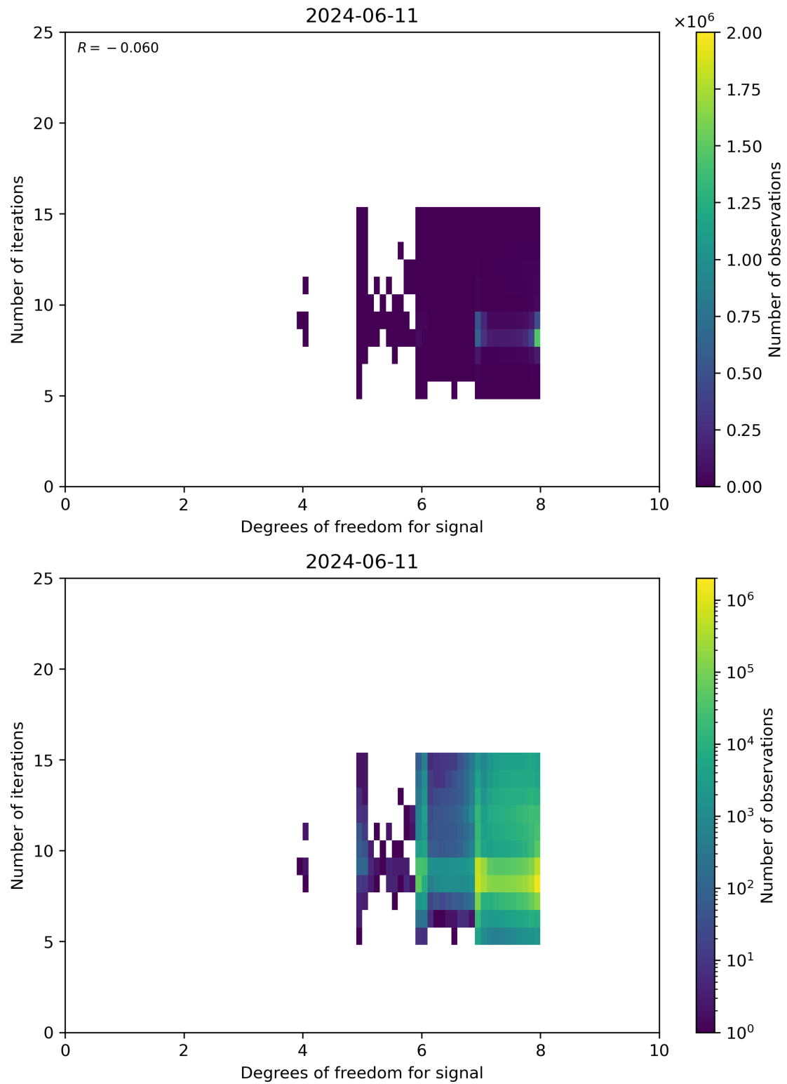
Figure 50: Scatter density plot of “Degrees of freedom for signal” against “Number of iterations” for 2024-06-10 to 2024-06-12.
