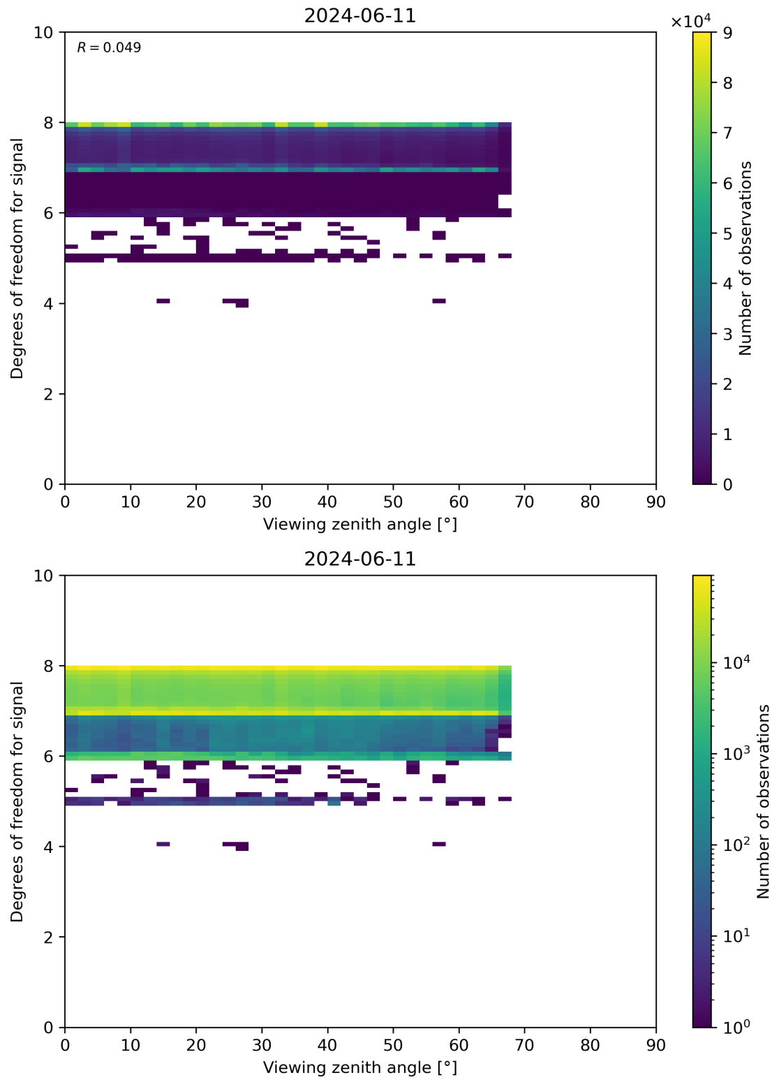
Figure 73: Scatter density plot of “Viewing zenith angle” against “Degrees of freedom for signal” for 2024-06-10 to 2024-06-12.
