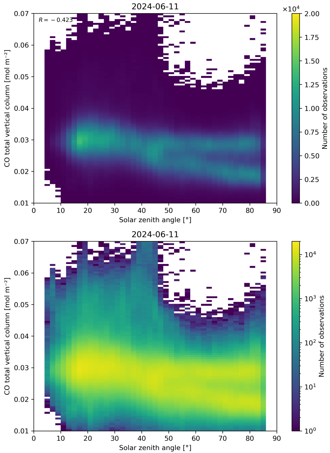
Figure 61: Scatter density plot of “Solar zenith angle” against “CO total vertical column” for 2024-06-10 to 2024-06-12.
