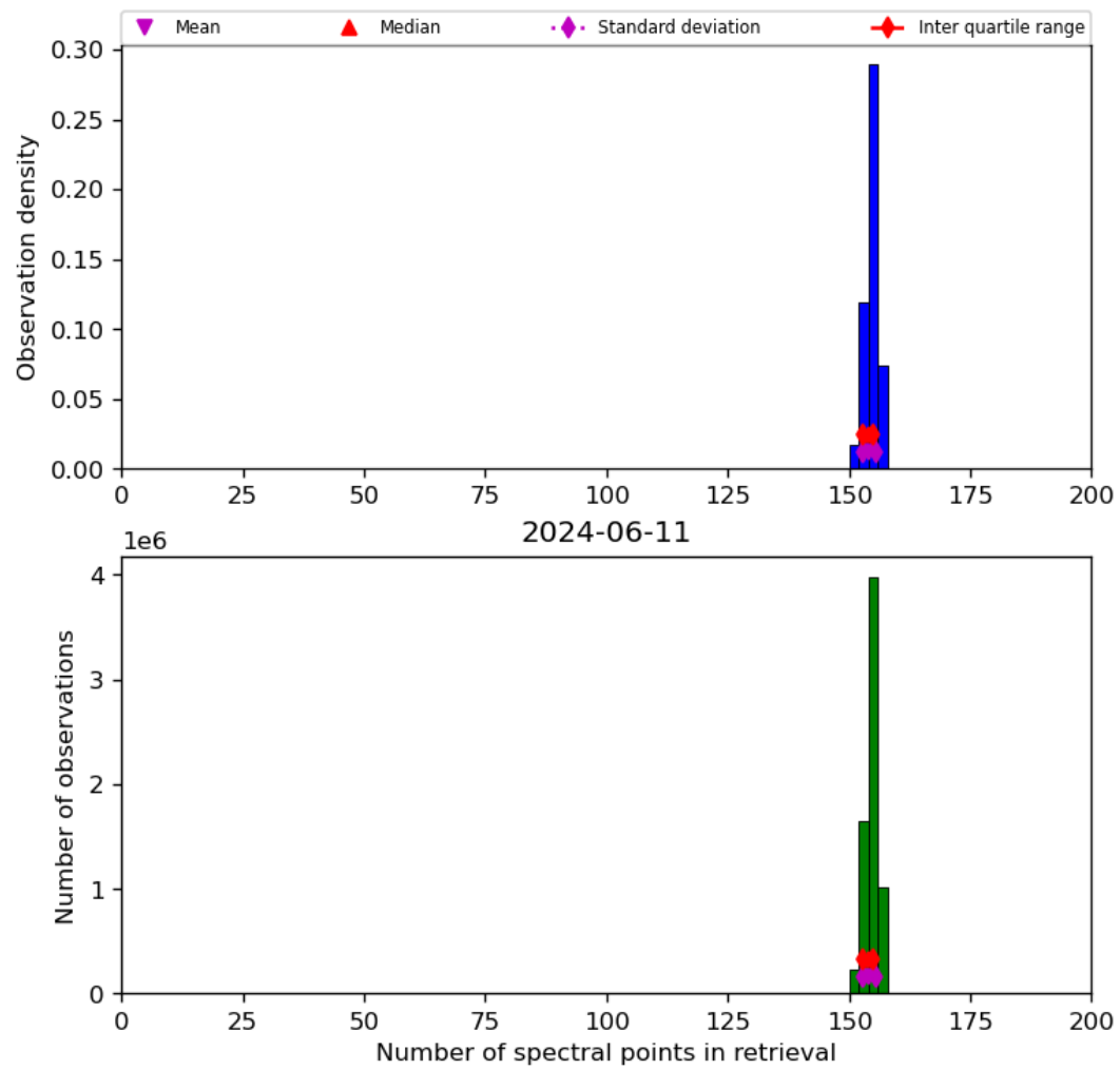
Figure 21: Histogram of “Number of spectral points in retrieval” for 2024-06-10 to 2024-06-12
