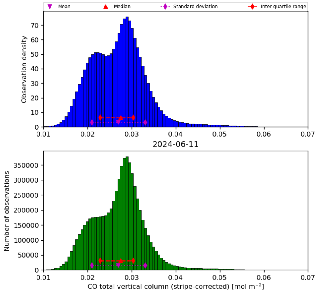
Figure 19: Histogram of “CO total vertical column (stripe-corrected)” for 2024-06-10 to 2024-06-12
