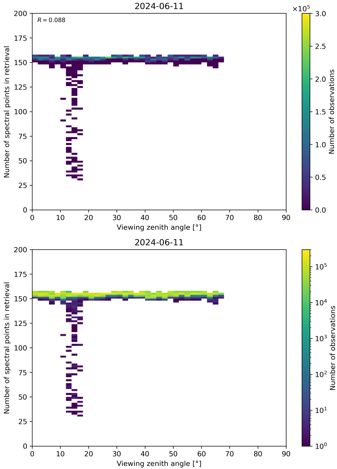
Figure 76: Scatter density plot of “Viewing zenith angle” against “Number of spectral points in retrieval” for 2024-06-10 to 2024-06-12.
