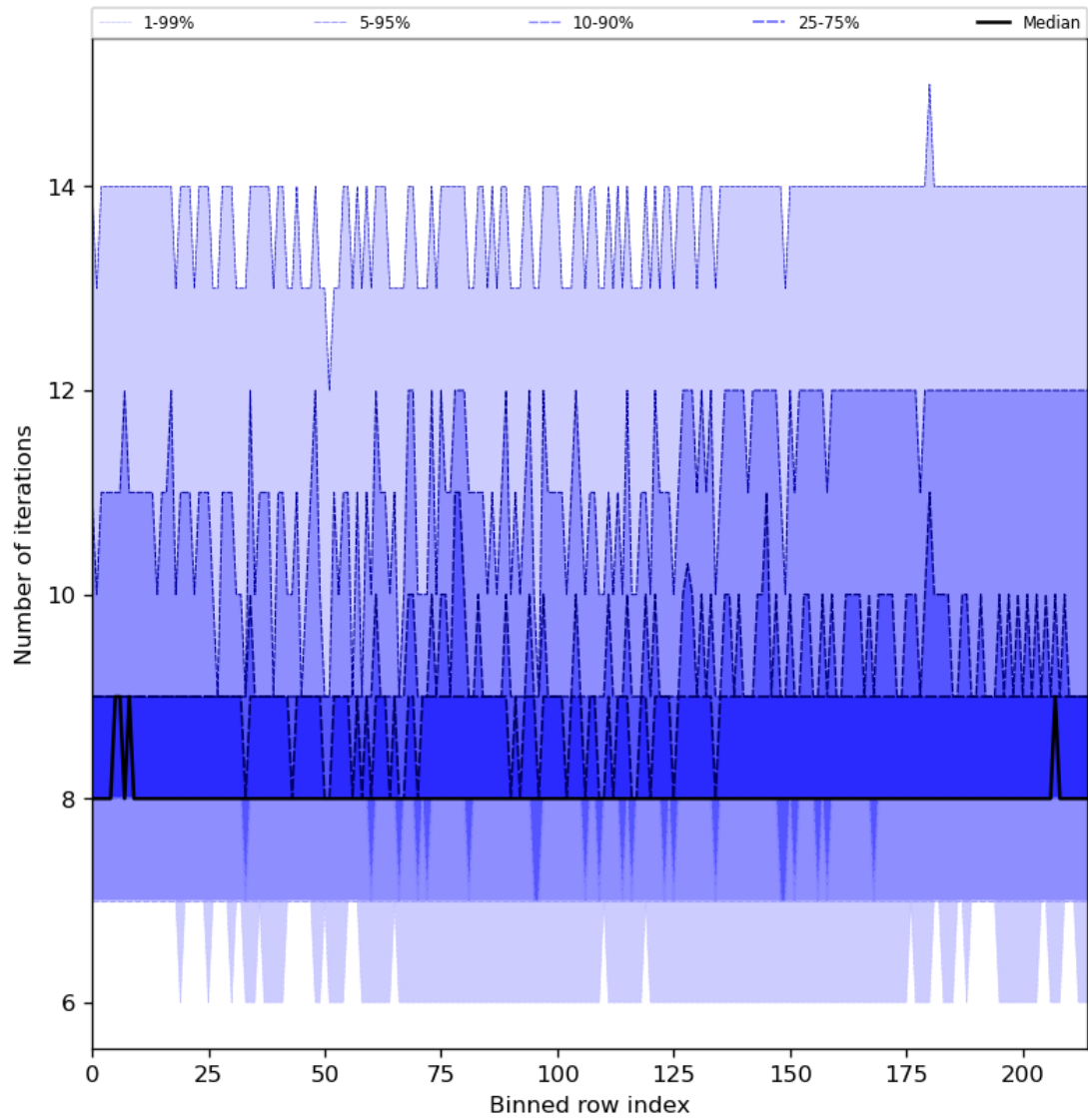
Figure 32: Along track statistics of “Number of iterations” for 2024-06-10 to 2024-06-12
