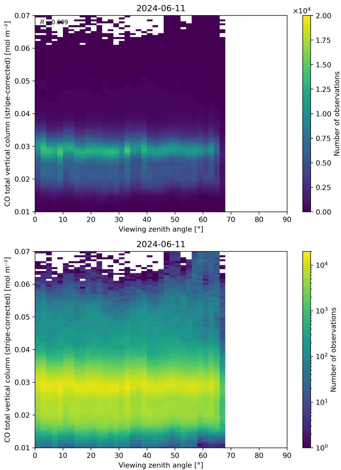
Figure 70: Scatter density plot of “Viewing zenith angle” against “CO total vertical column (stripe-corrected)” for 2024-06-10 to 2024-06-12.
