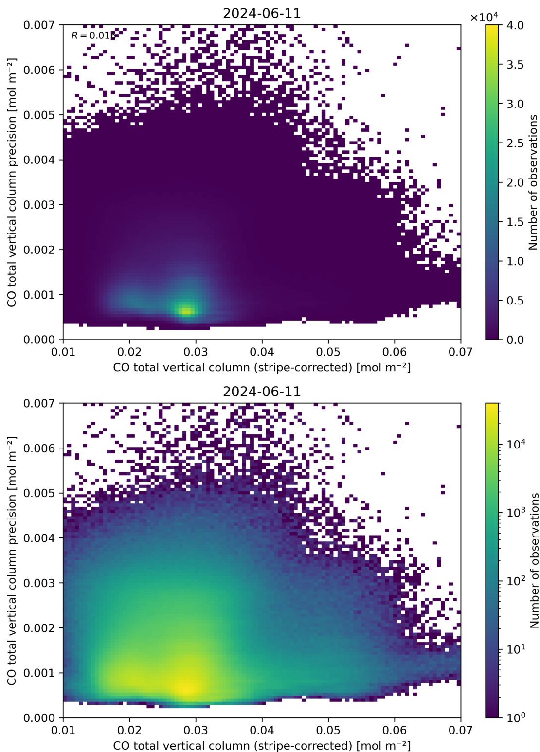
Figure 36: Scatter density plot of “CO total vertical column (stripe-corrected)” against “CO total vertical column precision” for 2024-06-10 to 2024-06-12.
