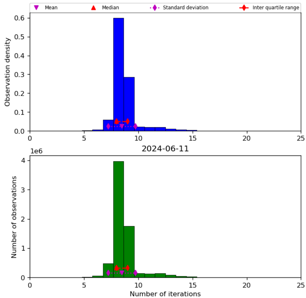
Figure 24: Histogram of “Number of iterations” for 2024-06-10 to 2024-06-12
