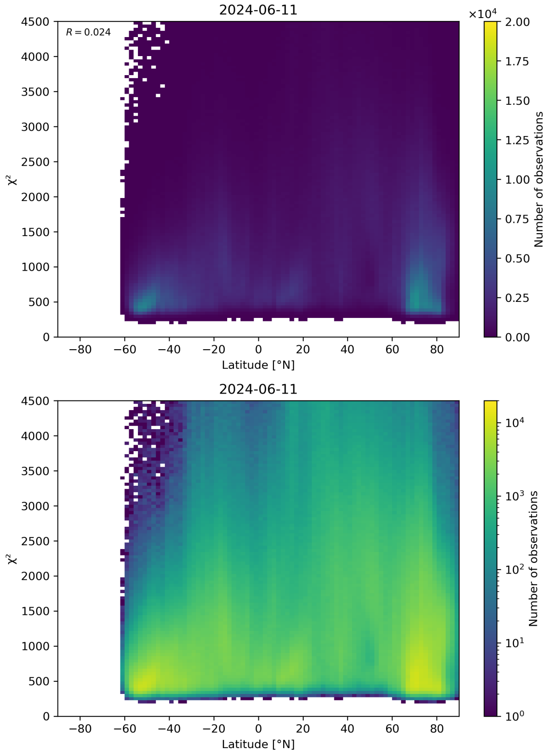
Figure 54: Scatter density plot of “Latitude” against “ \chi^2 ” for 2024-06-10 to 2024-06-12.
