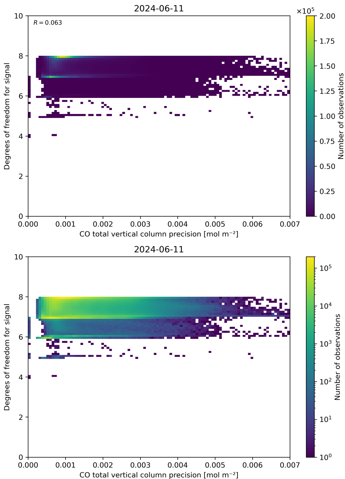
Figure 45: Scatter density plot of “CO total vertical column precision” against “Degrees of freedom for signal” for 2024-06-10 to 2024-06-12.
