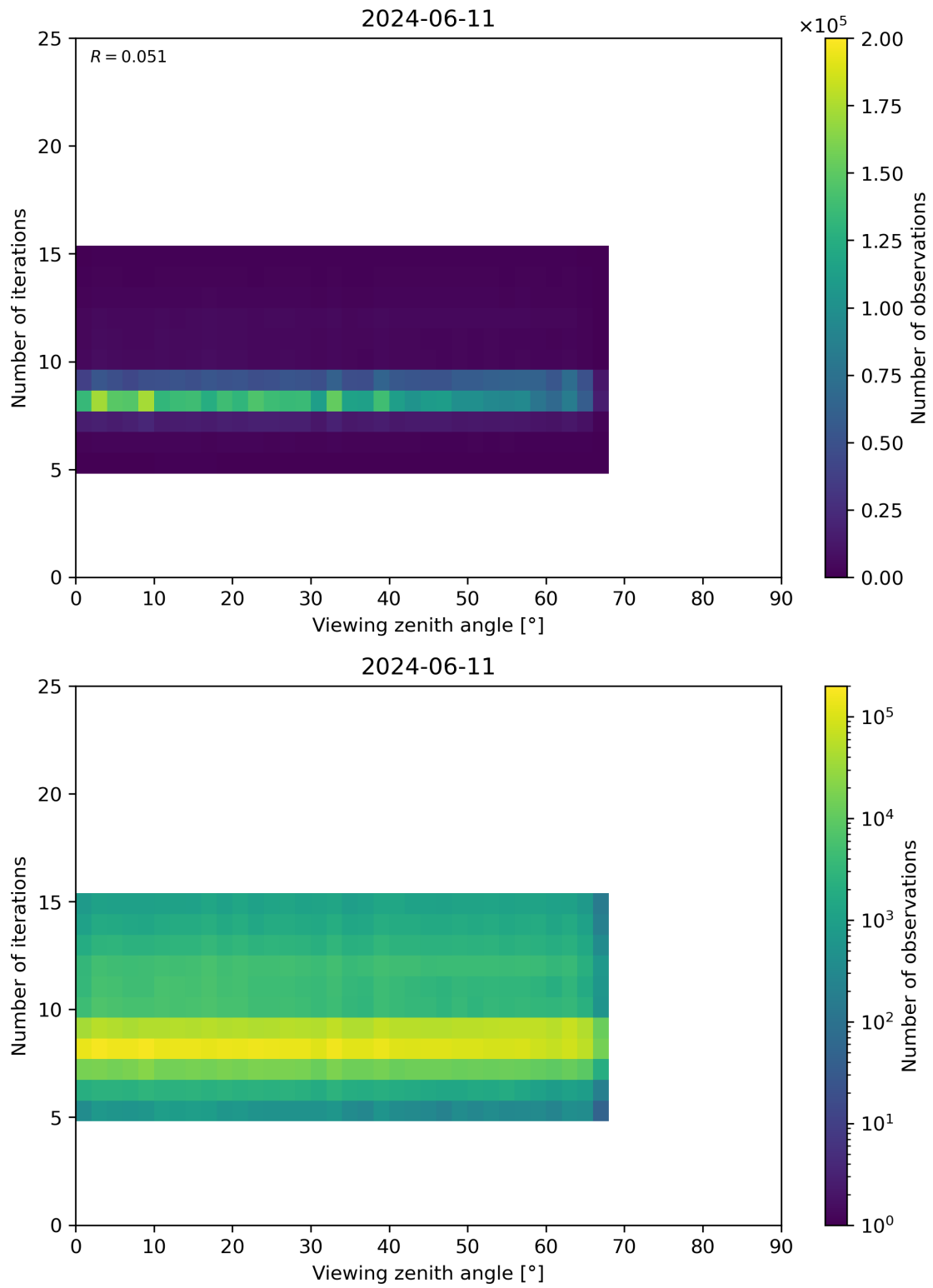
Figure 75: Scatter density plot of “Viewing zenith angle” against “Number of iterations” for 2024-06-10 to 2024-06-12.
