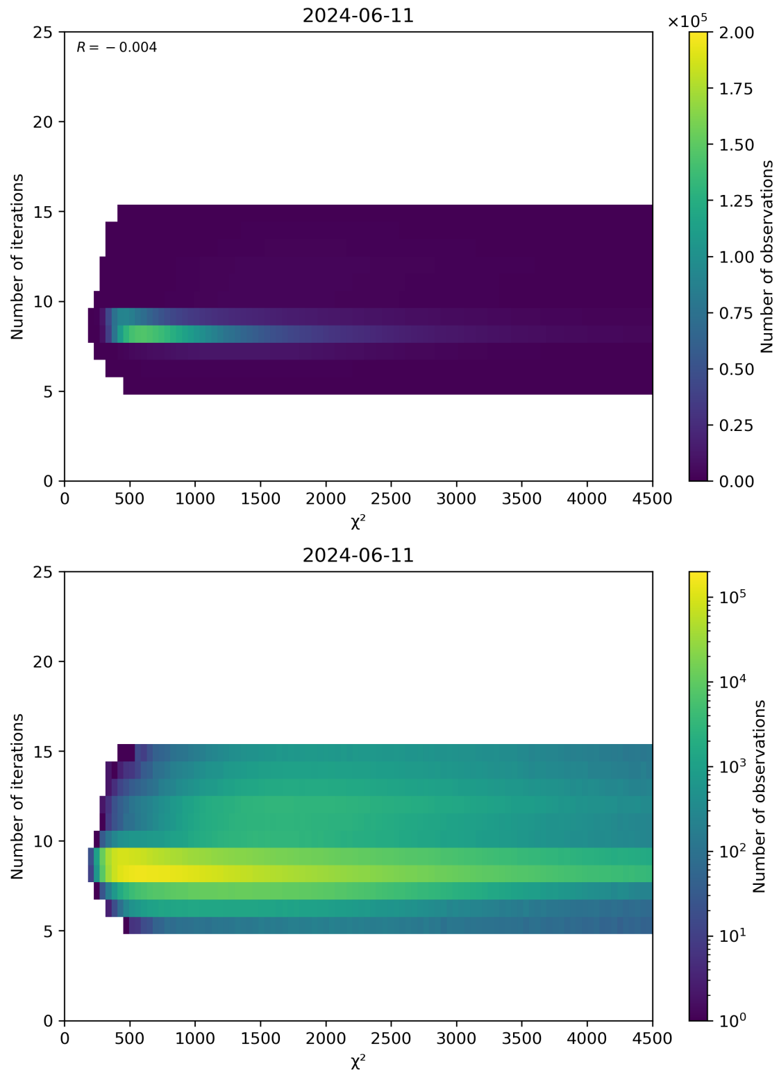
Figure 49: Scatter density plot of “ \chi^2 ” against “Number of iterations” for 2024-06-10 to 2024-06-12.
