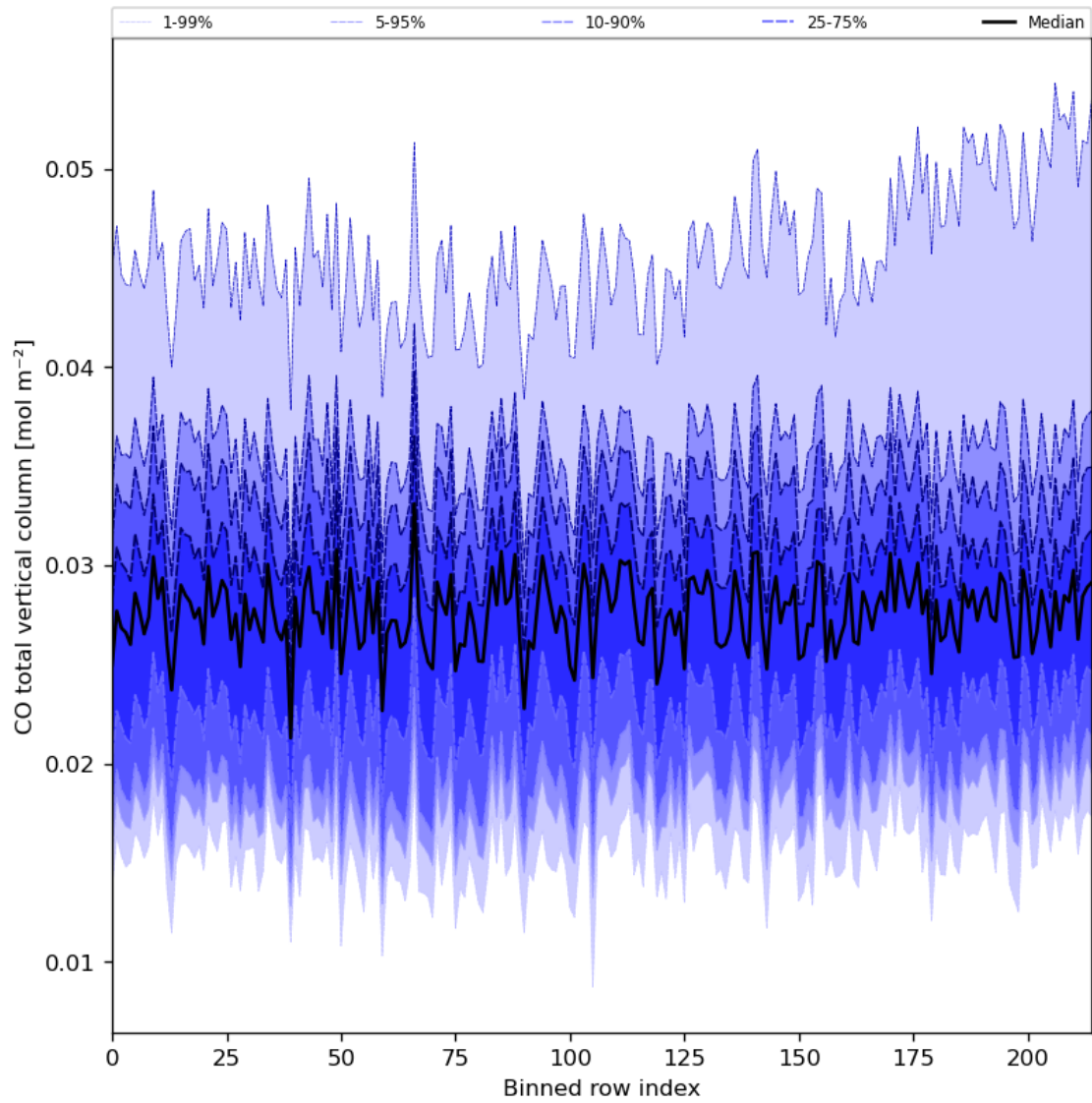
Figure 26: Along track statistics of “CO total vertical column” for 2024-06-10 to 2024-06-12
