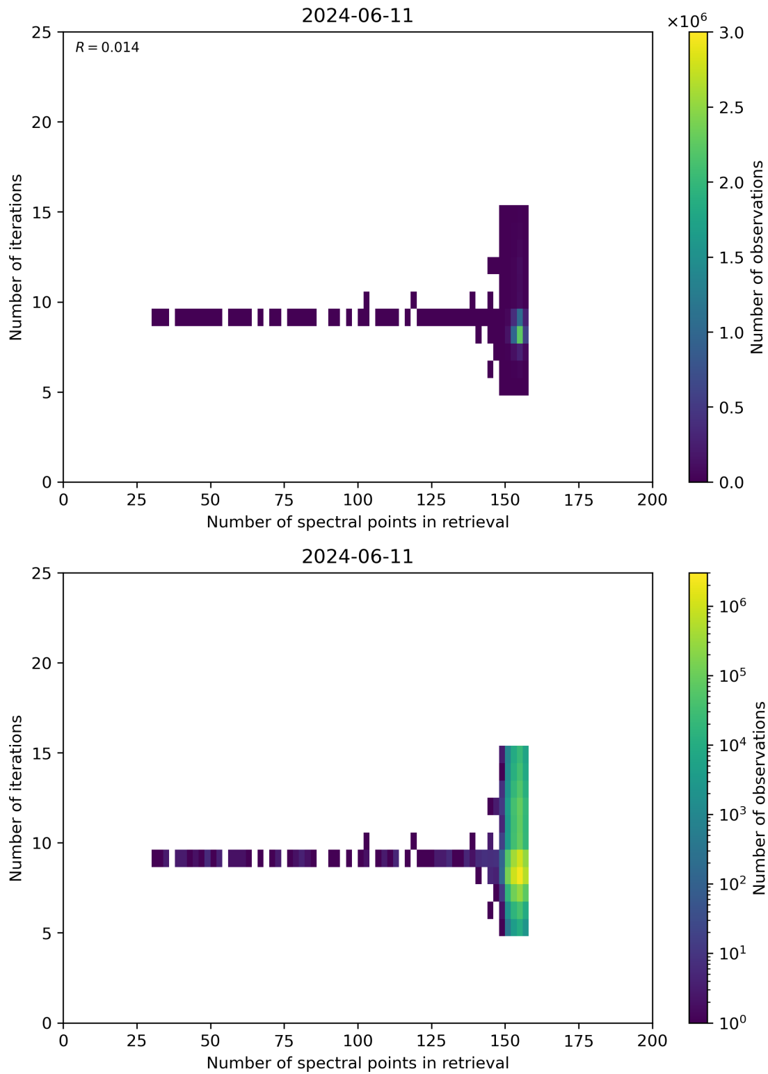
Figure 60: Scatter density plot of “Number of spectral points in retrieval” against “Number of iterations” for 2024-06-10 to 2024-06-12.
