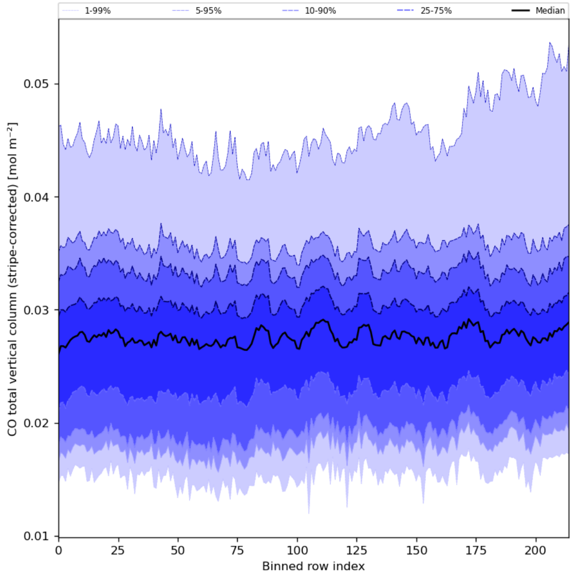
Figure 27: Along track statistics of “CO total vertical column (stripe-corrected)” for 2024-06-10 to 2024-06-12
