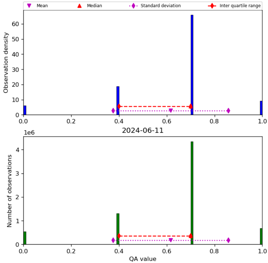
Figure 17: Histogram of “QA value” for 2024-06-10 to 2024-06-12
