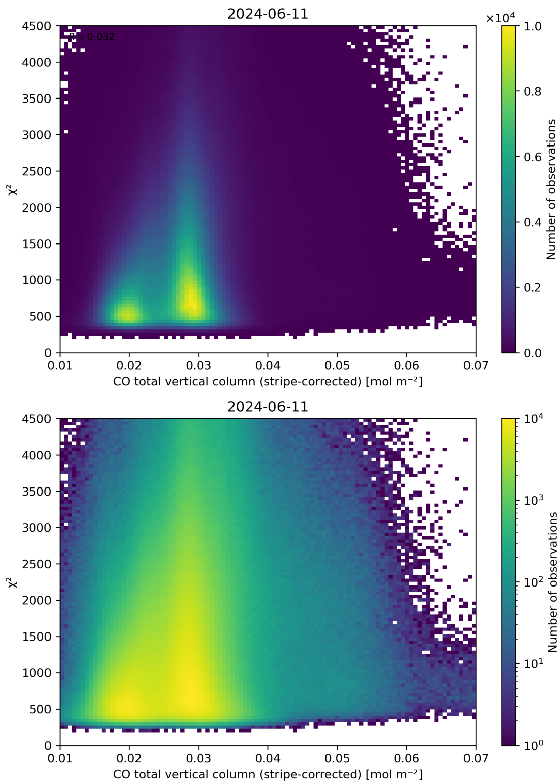
Figure 37: Scatter density plot of “CO total vertical column (stripe-corrected)” against “ \chi^2 ” for 2024-06-10 to 2024-06-12.
