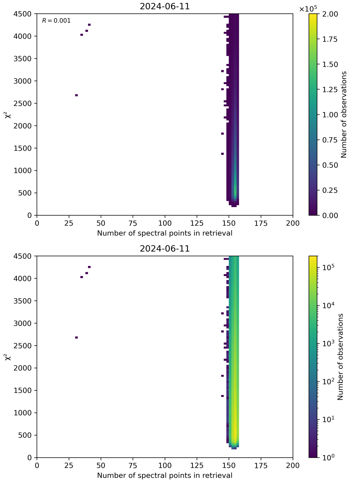
Figure 58: Scatter density plot of “Number of spectral points in retrieval” against “ \chi^2 ” for 2024-06-10 to 2024-06-12.
