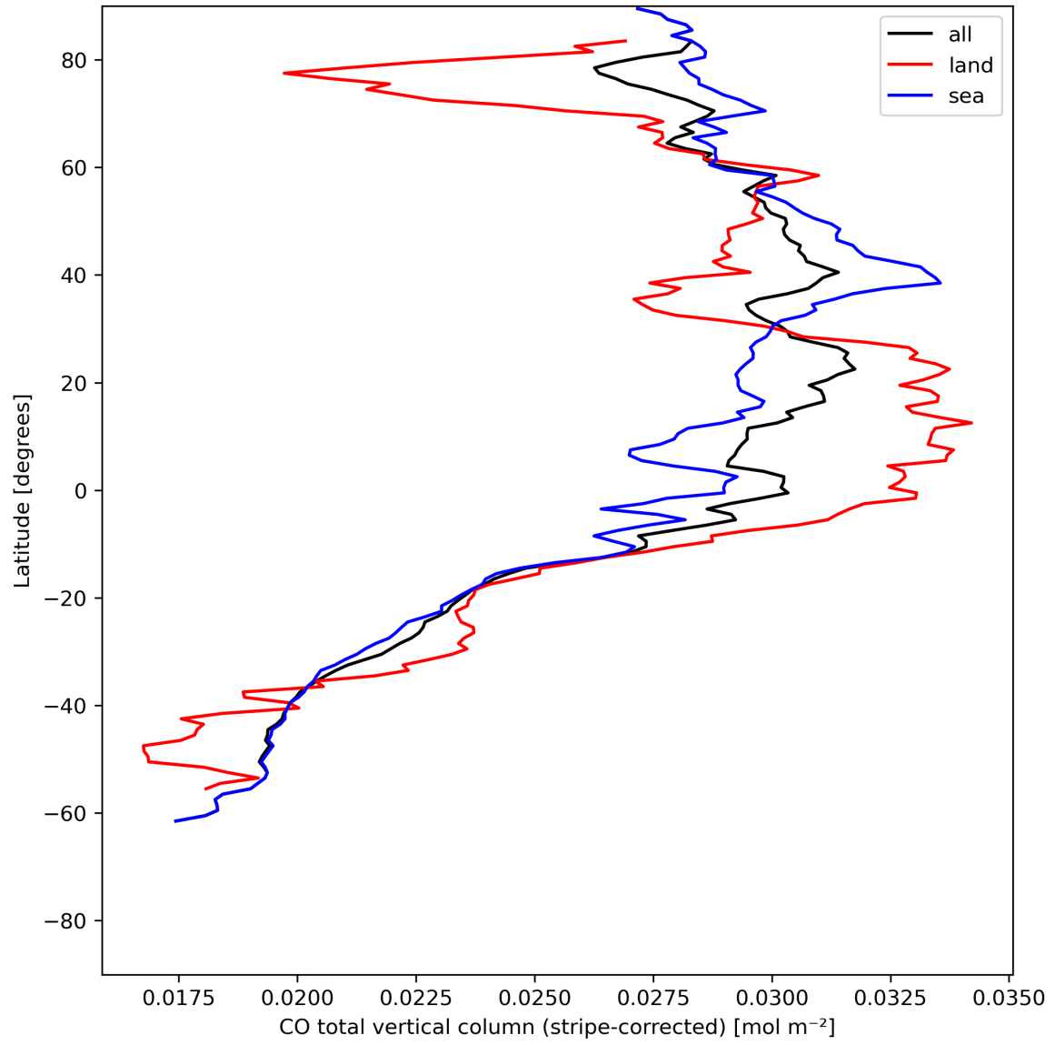
Figure 11: Zonal average of “CO total vertical column (stripe-corrected)” for 2024-06-10 to 2024-06-12.
