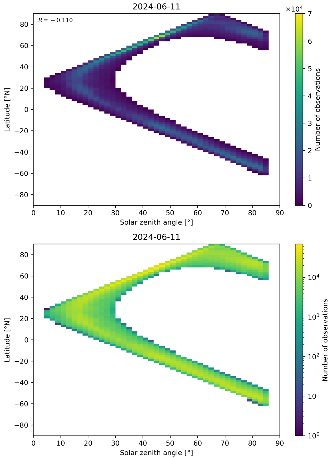
Figure 66: Scatter density plot of “Solar zenith angle” against “Latitude” for 2024-06-10 to 2024-06-12.
