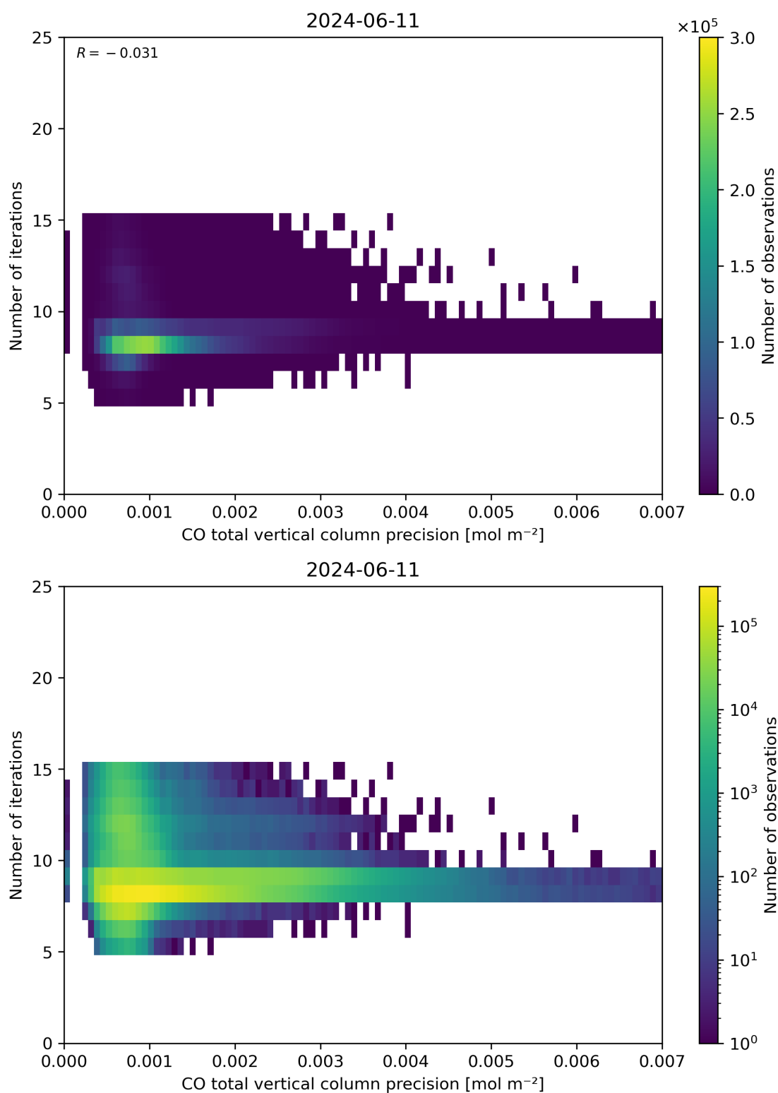
Figure 46: Scatter density plot of “CO total vertical column precision” against “Number of iterations” for 2024-06-10 to 2024-06-12.
