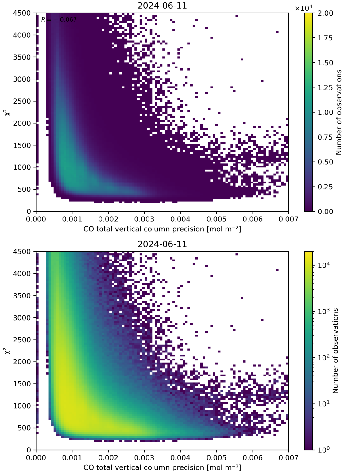
Figure 44: Scatter density plot of “CO total vertical column precision” against “ \chi^2 ” for 2024-06-10 to 2024-06-12.
