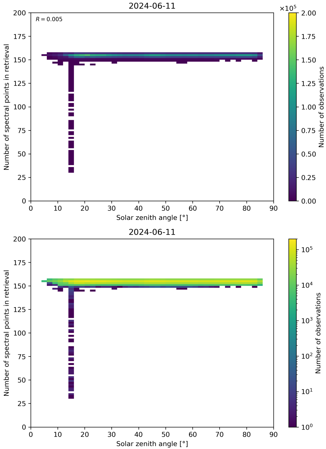
Figure 68: Scatter density plot of “Solar zenith angle” against “Number of spectral points in retrieval” for 2024-06-10 to 2024-06-12.
