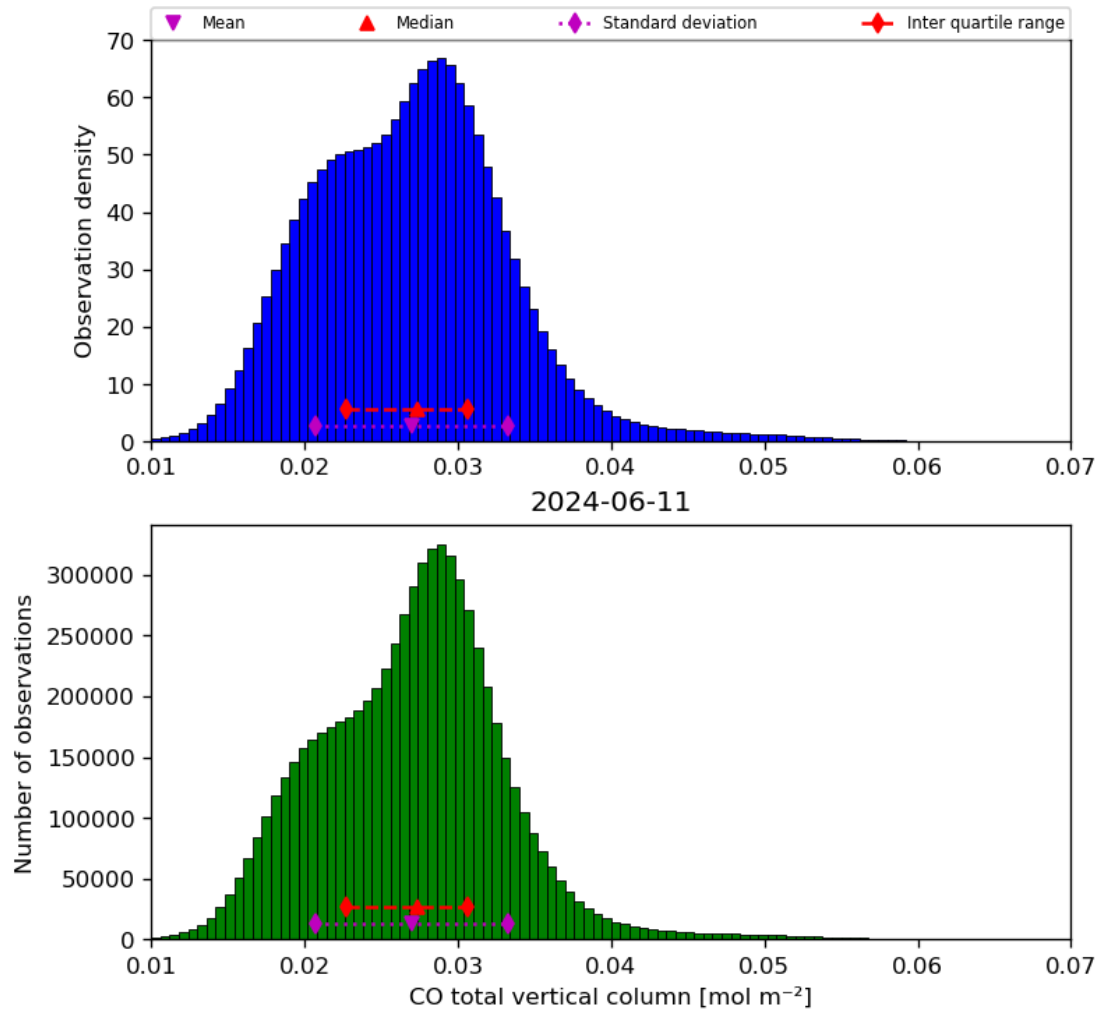
Figure 18: Histogram of “CO total vertical column” for 2024-06-10 to 2024-06-12
