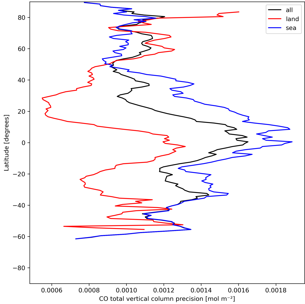
Figure 12: Zonal average of "CO total vertical column precision" for 2024-06-10 to 2024-06-12.
