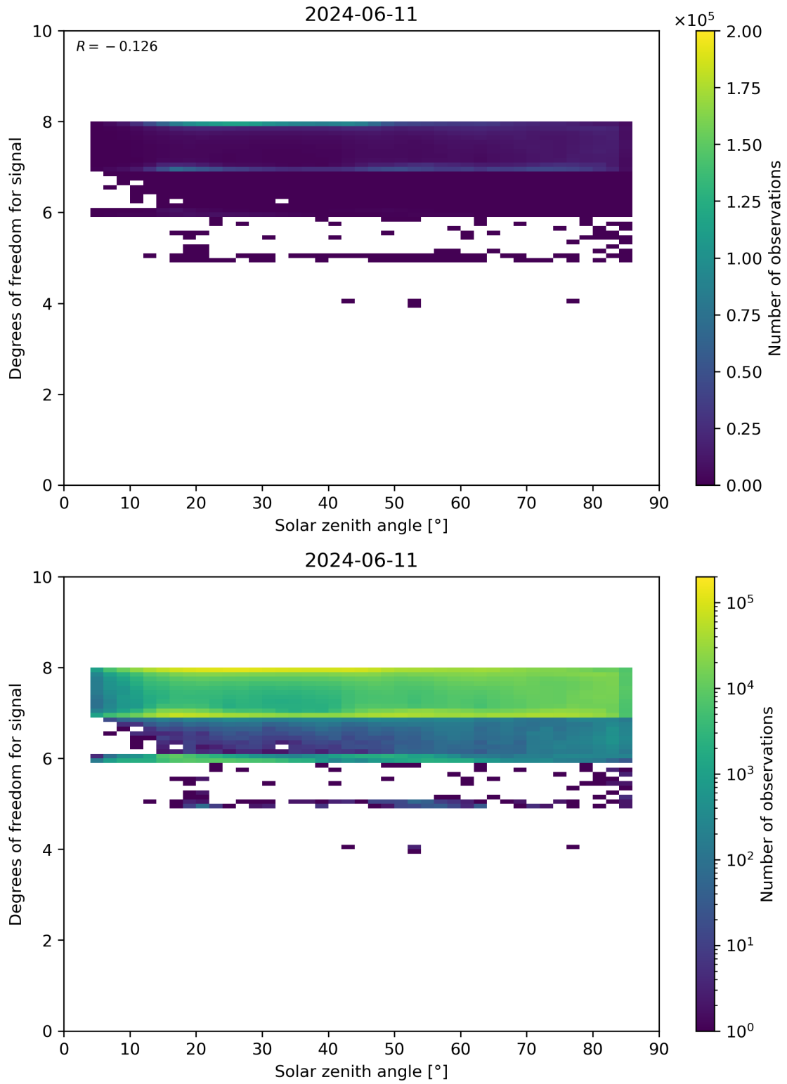
Figure 65: Scatter density plot of “Solar zenith angle” against “Degrees of freedom for signal” for 2024-06-10 to 2024-06-12.
