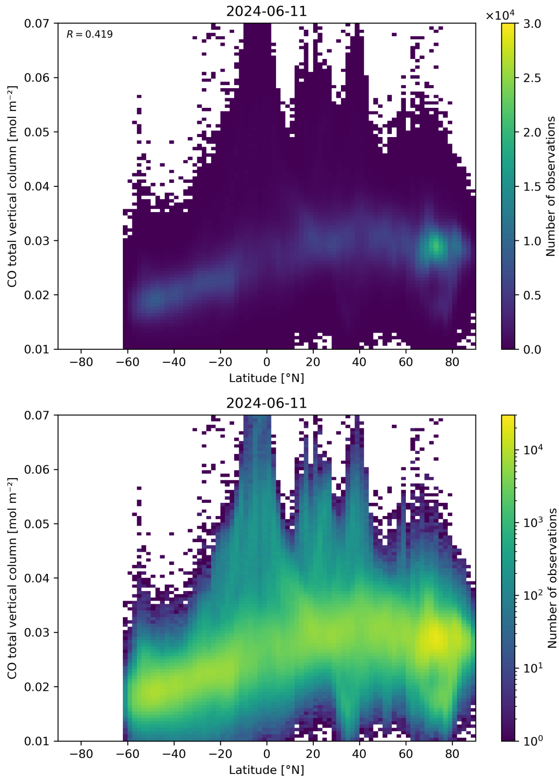
Figure 51: Scatter density plot of “Latitude” against “CO total vertical column” for 2024-06-10 to 2024-06-12.
