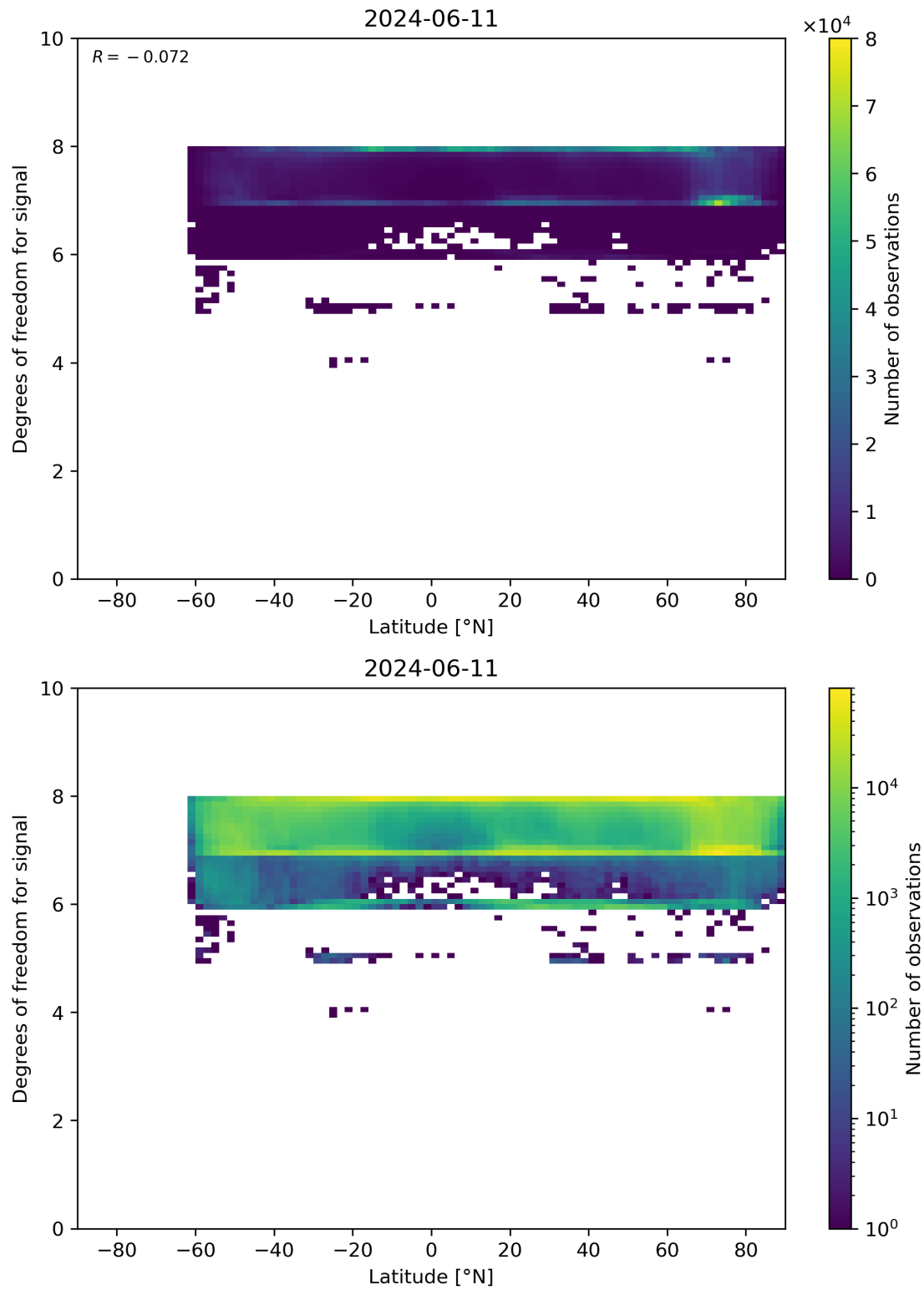
Figure 55: Scatter density plot of “Latitude” against “Degrees of freedom for signal” for 2024-06-10 to 2024-06-12.
