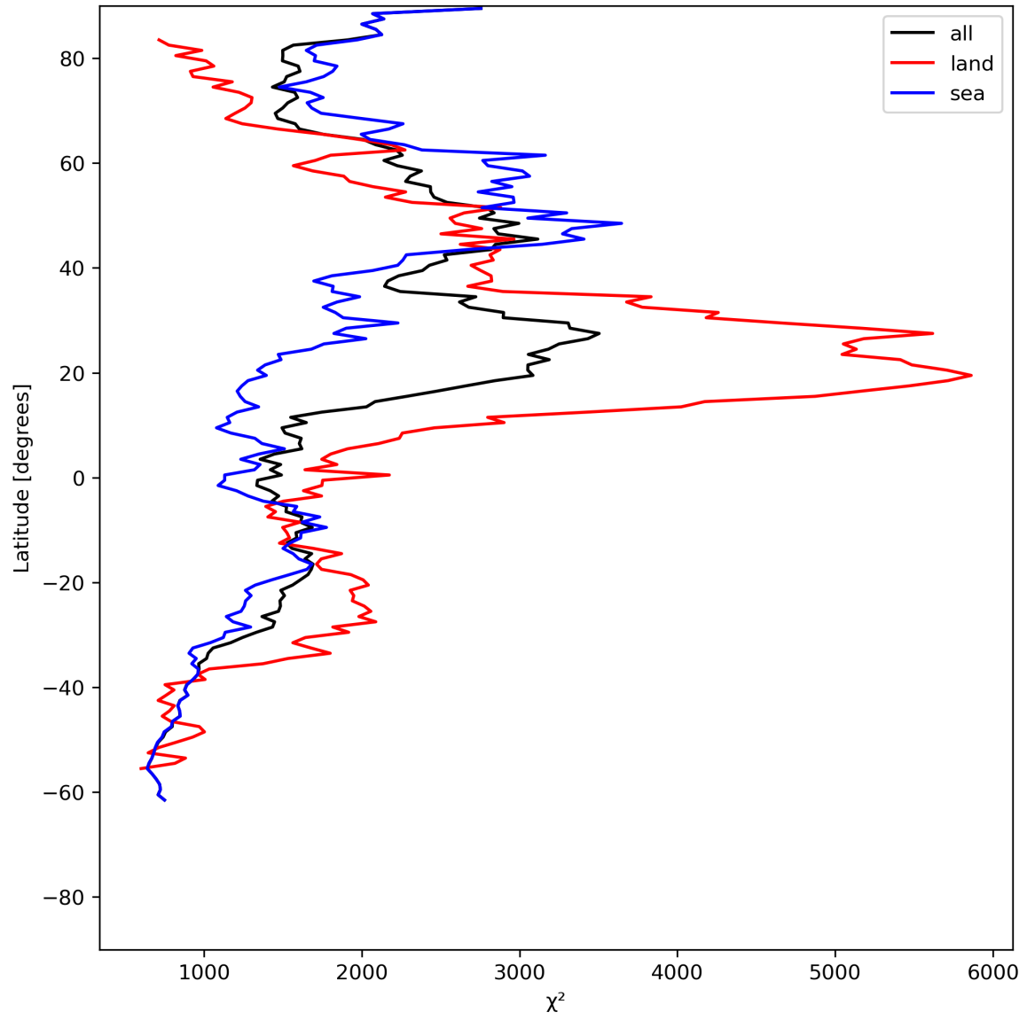
Figure 14: Zonal average of “ \chi^2 ” for 2024-06-10 to 2024-06-12.
