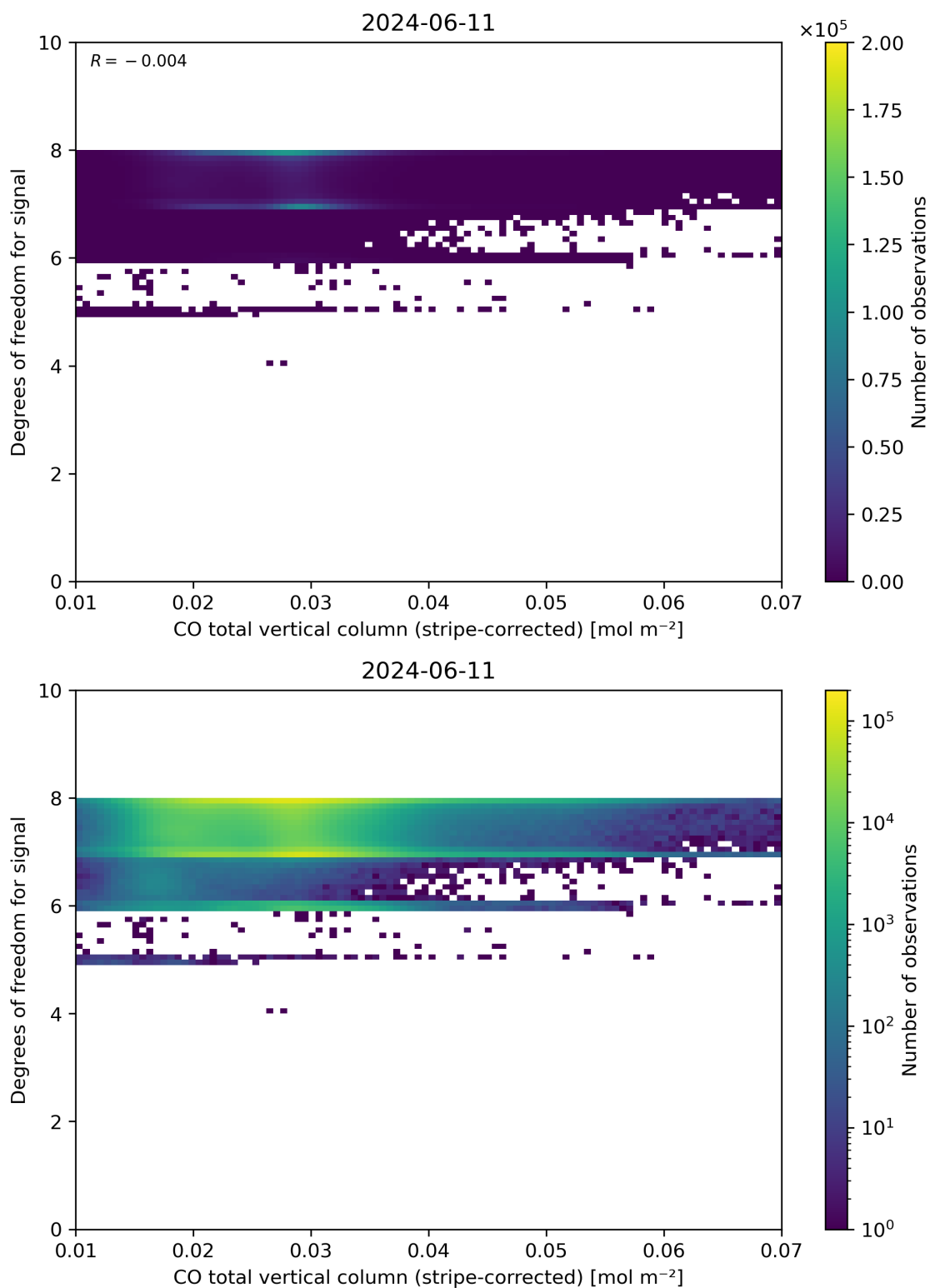
Figure 38: Scatter density plot of “CO total vertical column (stripe-corrected)” against “Degrees of freedom for signal” for 2024-06-10 to 2024-06-12.
