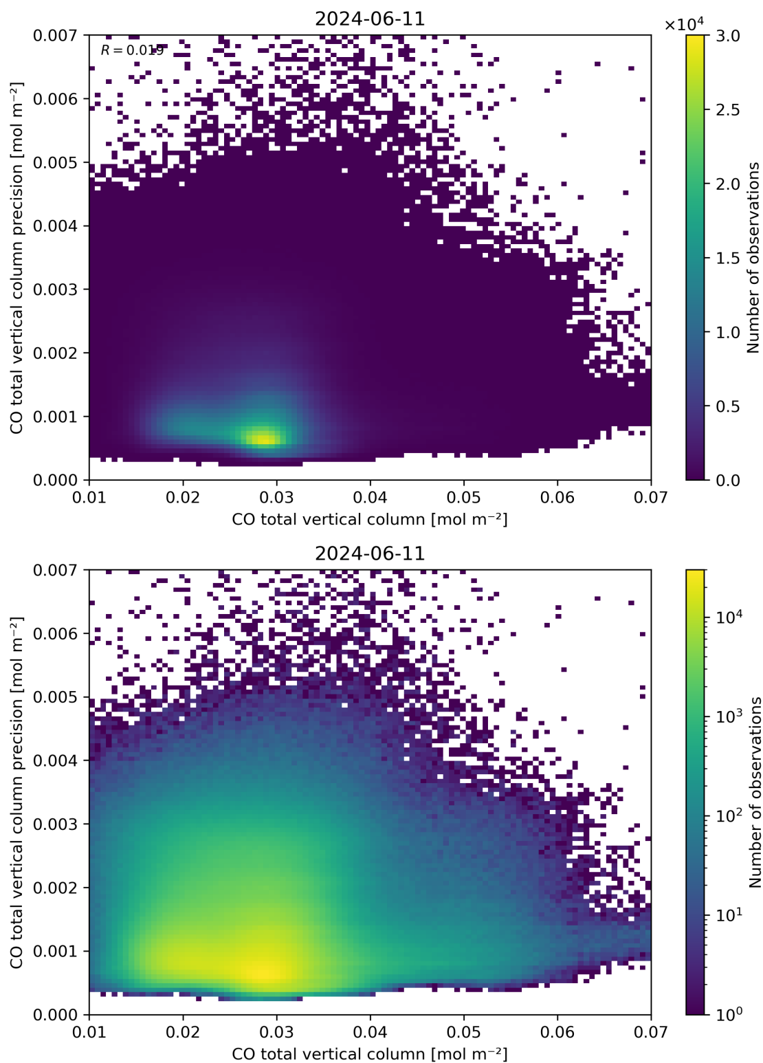
Figure 34: Scatter density plot of “CO total vertical column” against “CO total vertical column precision” for 2024-06-10 to 2024-06-12.
