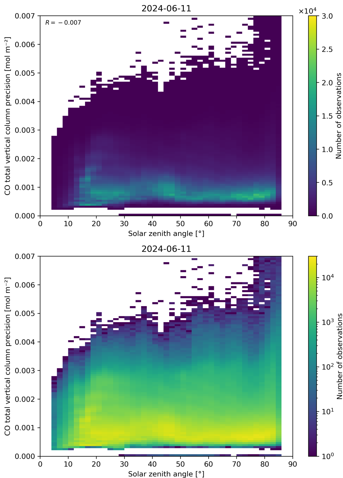
Figure 63: Scatter density plot of “Solar zenith angle” against “CO total vertical column precision” for 2024-06-10 to 2024-06-12.
