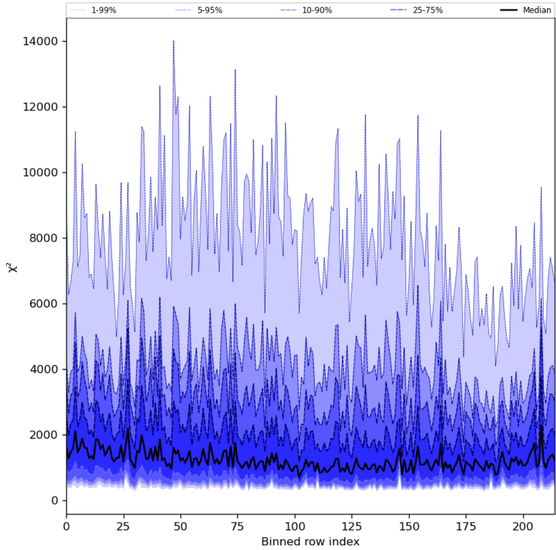
Figure 30: Along track statistics of “ \chi^2 ” for 2024-06-10 to 2024-06-12
