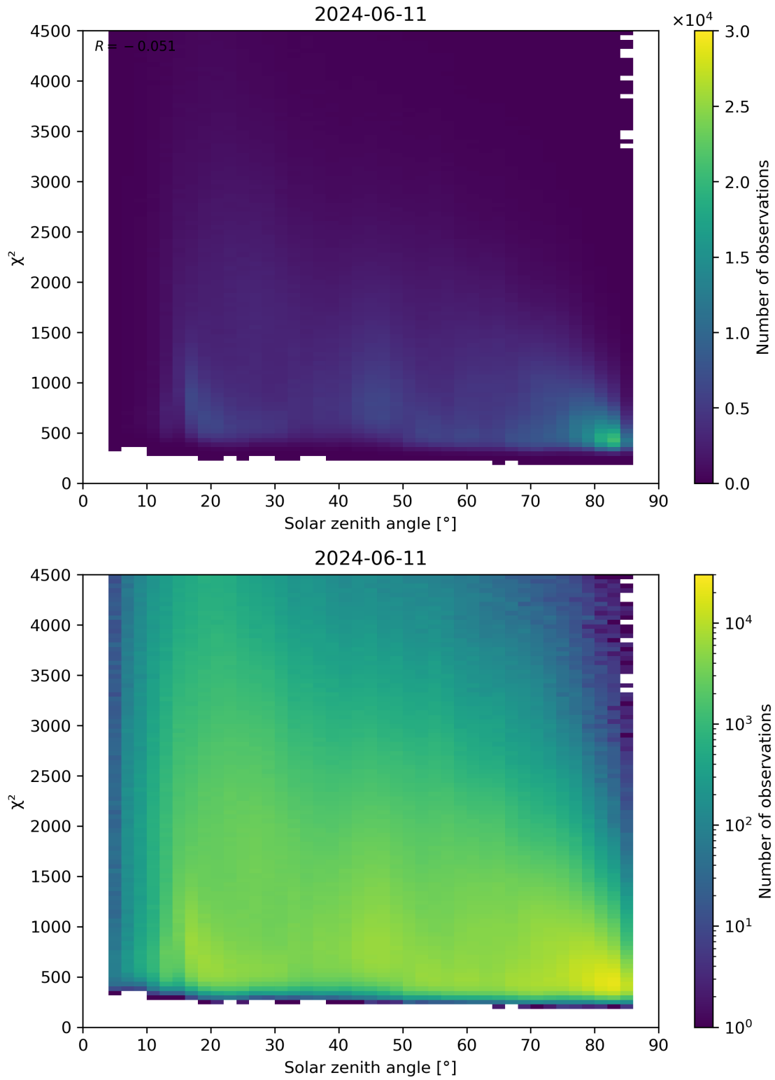
Figure 64: Scatter density plot of “Solar zenith angle” against “ \chi^2 ” for 2024-06-10 to 2024-06-12.
