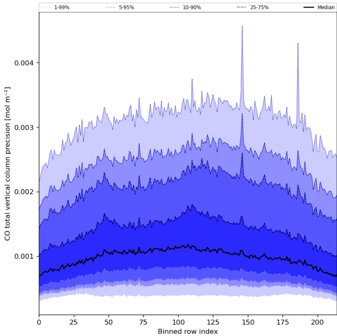
Figure 28: Along track statistics of “CO total vertical column precision” for 2024-06-10 to 2024-06-12
