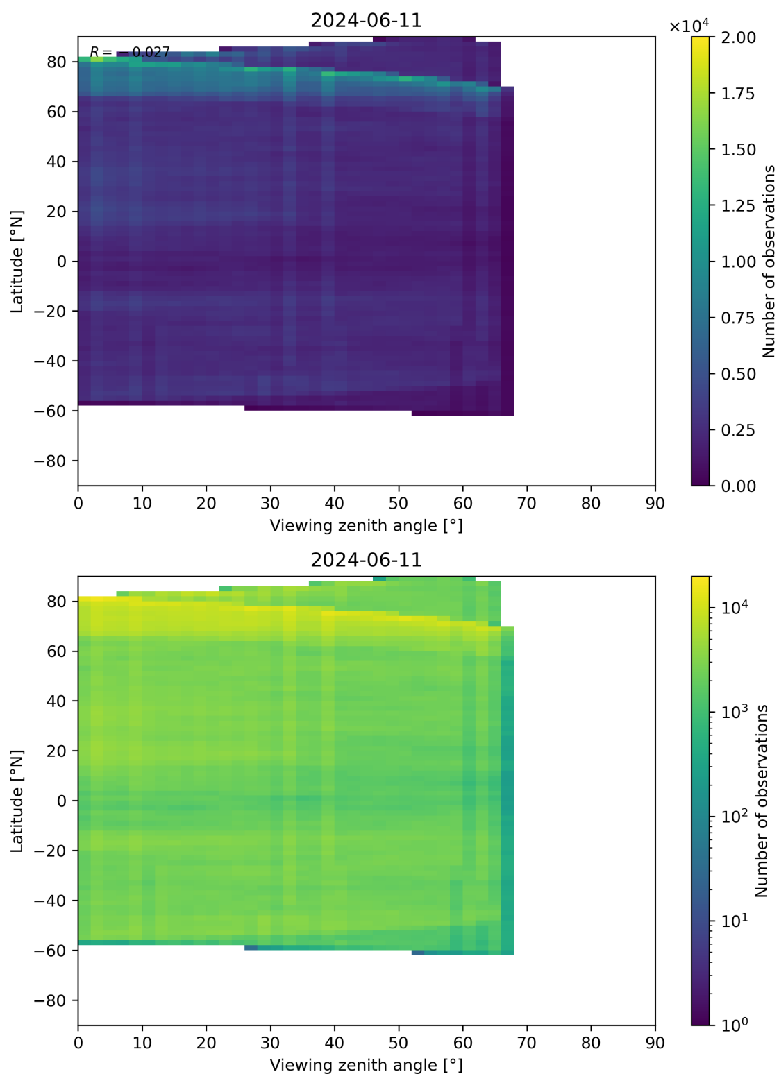
Figure 74: Scatter density plot of “Viewing zenith angle” against “Latitude” for 2024-06-10 to 2024-06-12.
