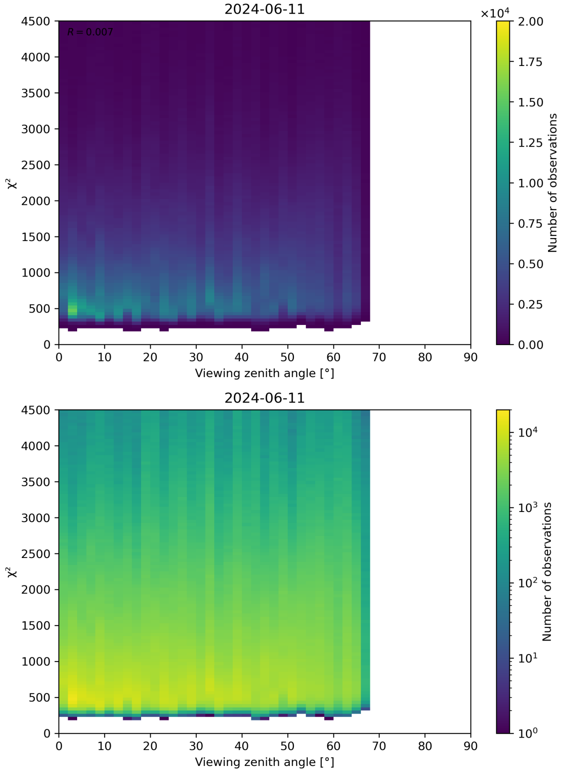
Figure 72: Scatter density plot of “Viewing zenith angle” against “ \chi^2 ” for 2024-06-10 to 2024-06-12.
