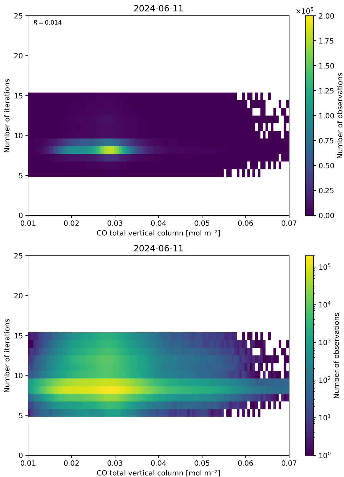
Figure 42: Scatter density plot of “CO total vertical column” against “Number of iterations” for 2024-06-10 to 2024-06-12.
