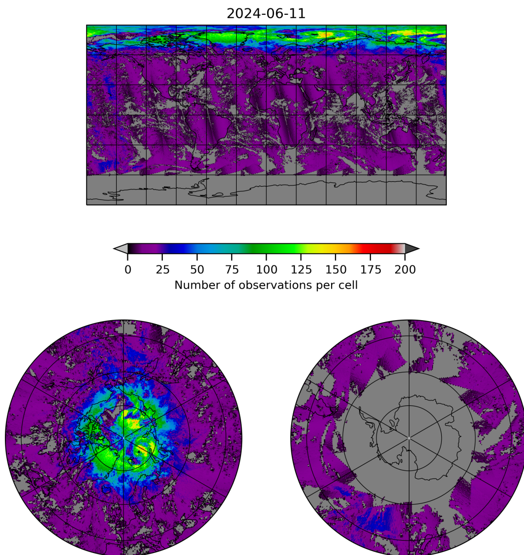
Figure 8: Map of the number of observations for 2024-06-10 to 2024-06-12
