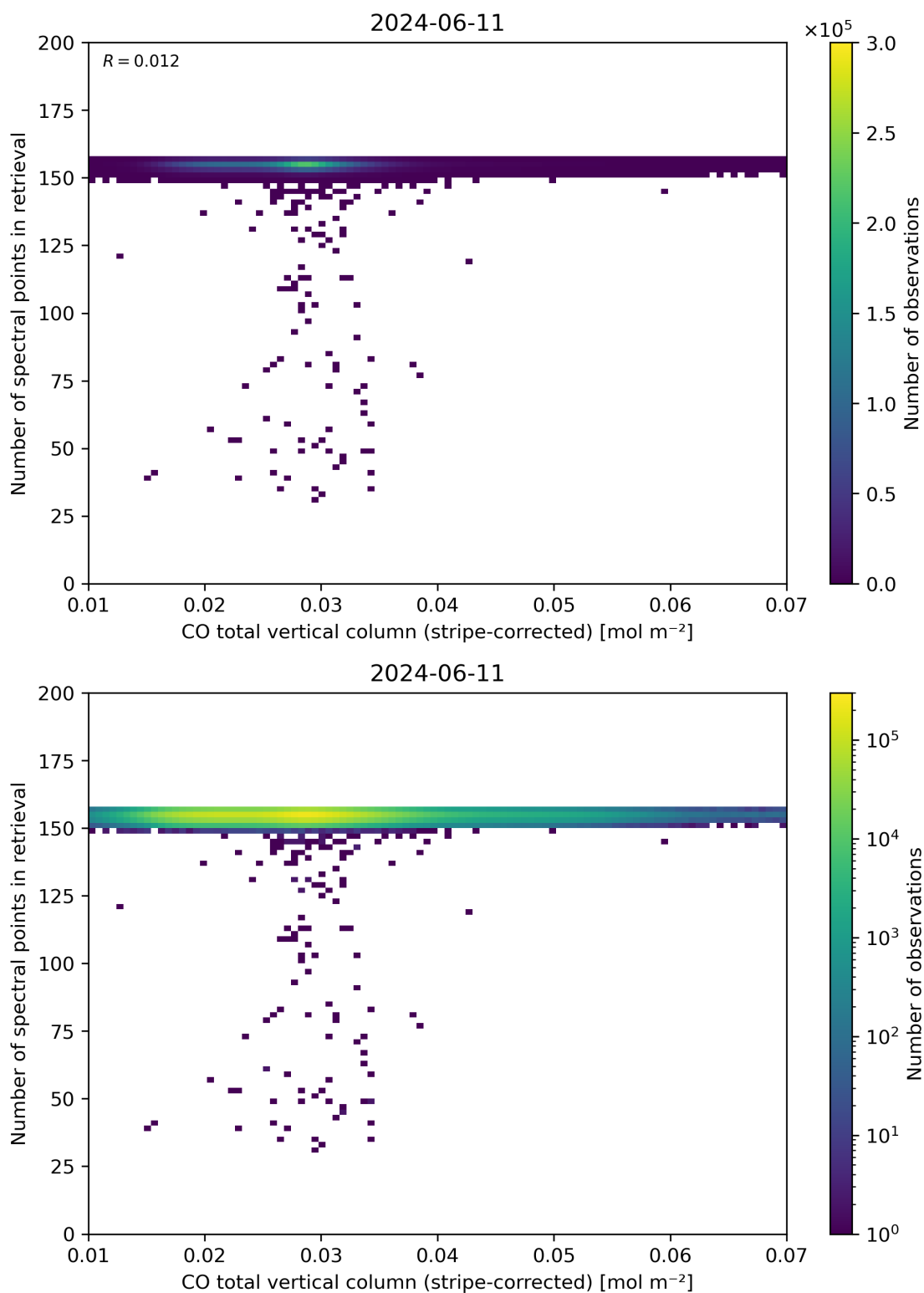
Figure 40: Scatter density plot of “CO total vertical column (stripe-corrected)” against “Number of spectral points in retrieval” for 2024-06-10 to 2024-06-12.
