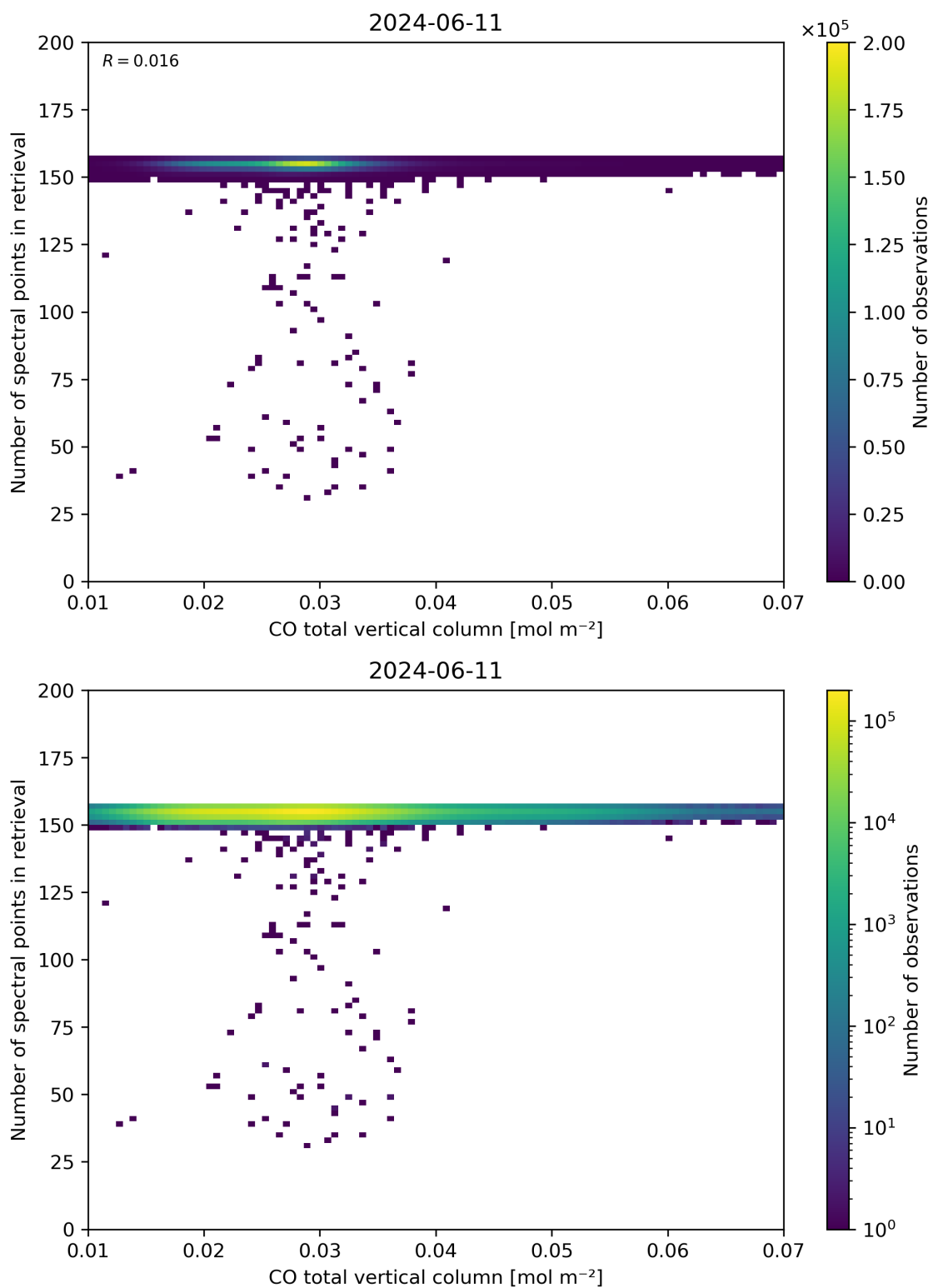
Figure 43: Scatter density plot of “CO total vertical column” against “Number of spectral points in retrieval” for 2024-06-10 to 2024-06-12.
