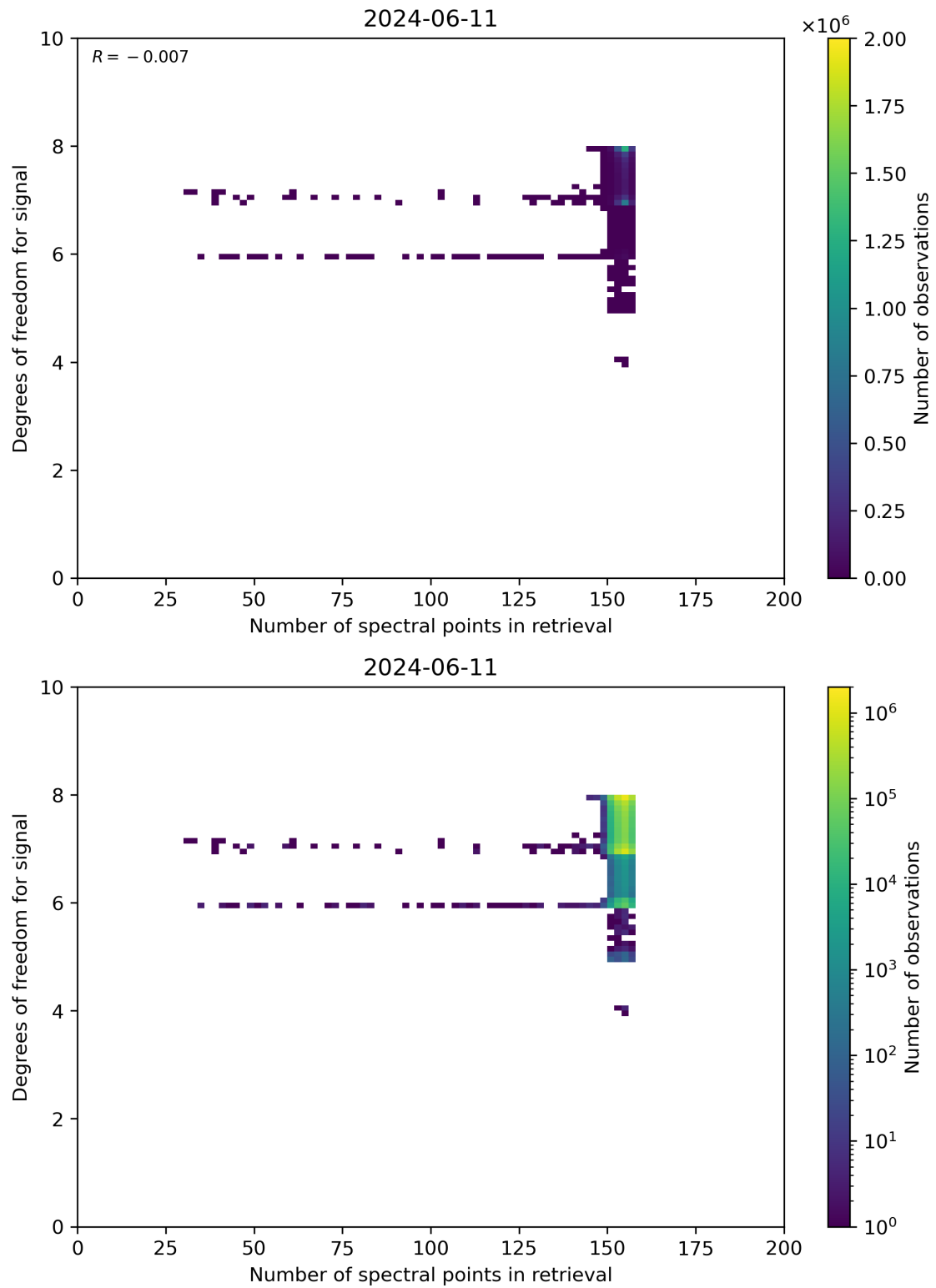
Figure 59: Scatter density plot of “Number of spectral points in retrieval” against “Degrees of freedom for signal” for 2024-06-10 to 2024-06-12.
