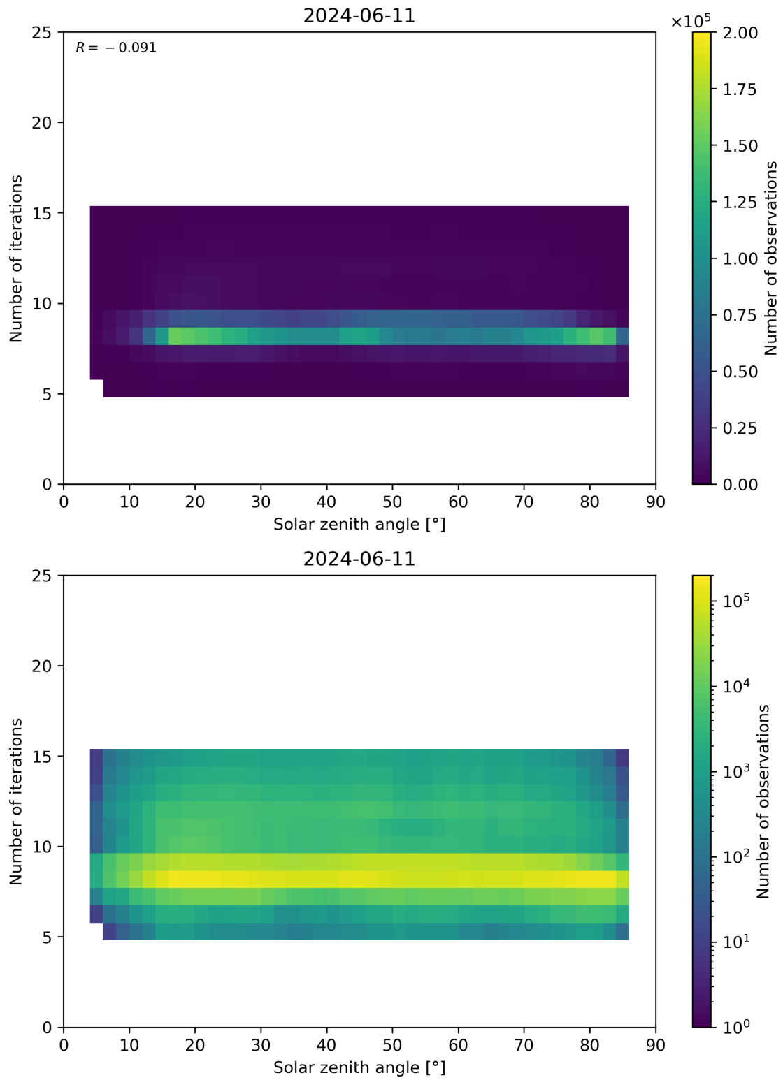
Figure 67: Scatter density plot of “Solar zenith angle” against “Number of iterations” for 2024-06-10 to 2024-06-12.
