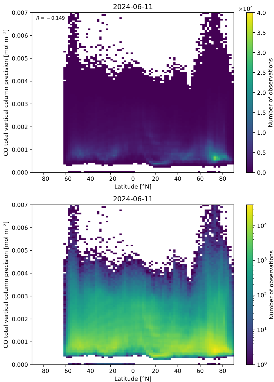
Figure 53: Scatter density plot of “Latitude” against “CO total vertical column precision” for 2024-06-10 to 2024-06-12.
