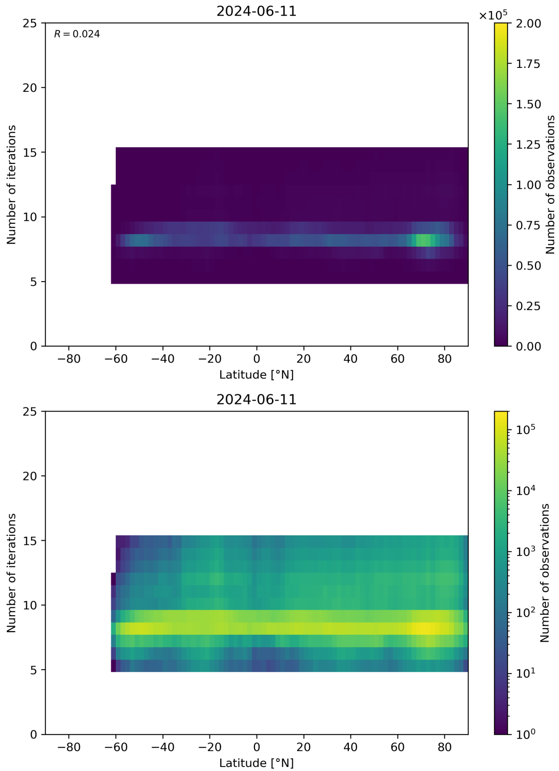
Figure 56: Scatter density plot of “Latitude” against “Number of iterations” for 2024-06-10 to 2024-06-12.
