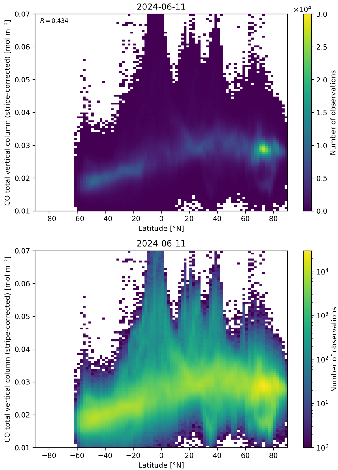
Figure 52: Scatter density plot of “Latitude” against “CO total vertical column (stripe-corrected)” for 2024-06-10 to 2024-06-12.
