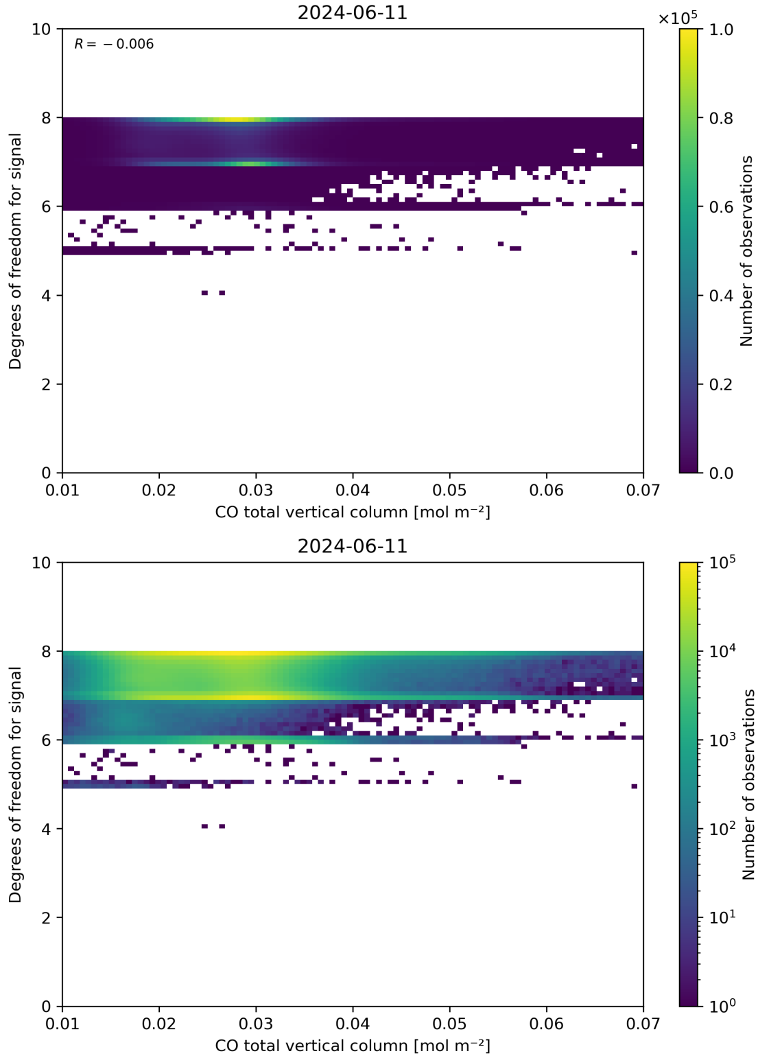
Figure 41: Scatter density plot of “CO total vertical column” against “Degrees of freedom for signal” for 2024-06-10 to 2024-06-12.
