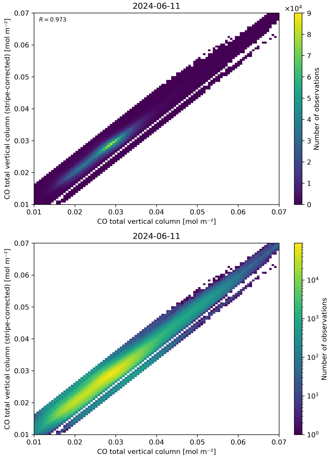
Figure 33: Scatter density plot of “CO total vertical column” against “CO total vertical column (stripe-corrected)” for 2024-06-10 to 2024-06-12.
