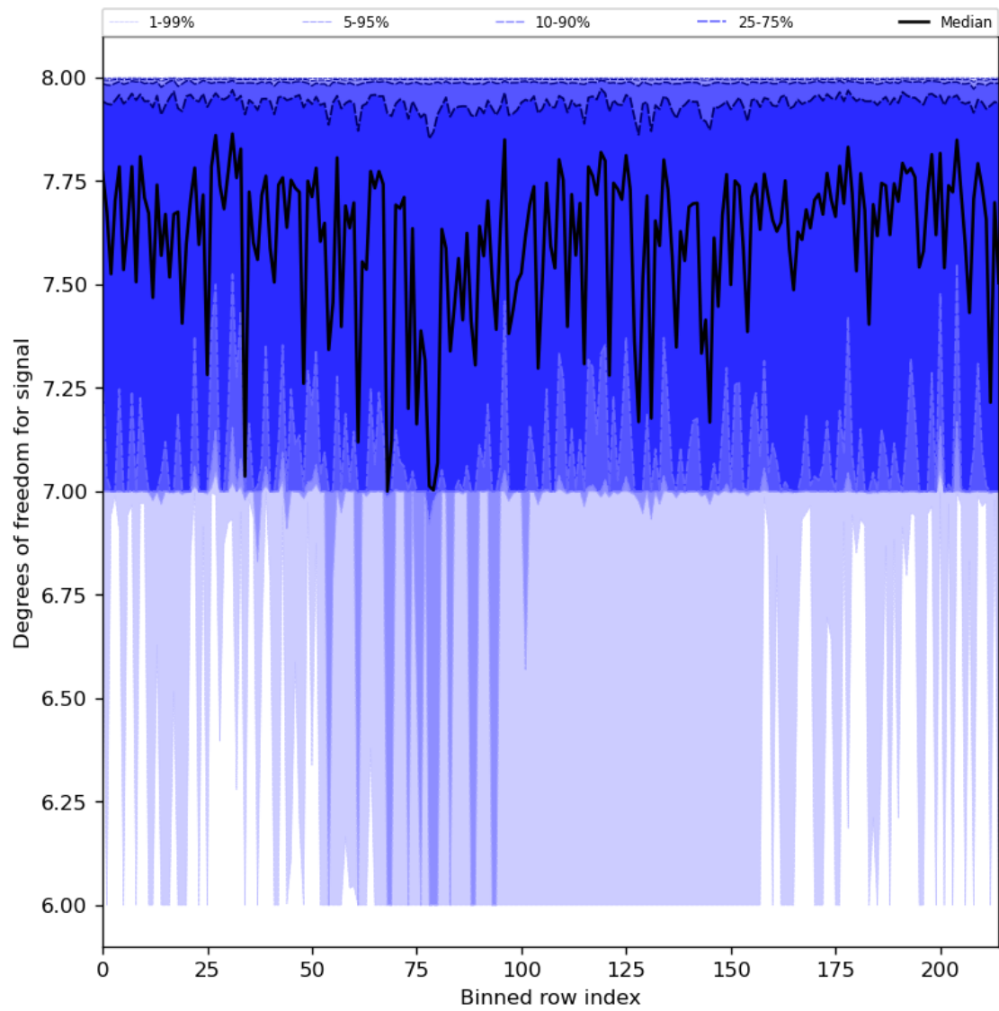
Figure 31: Along track statistics of “Degrees of freedom for signal” for 2024-06-10 to 2024-06-12
