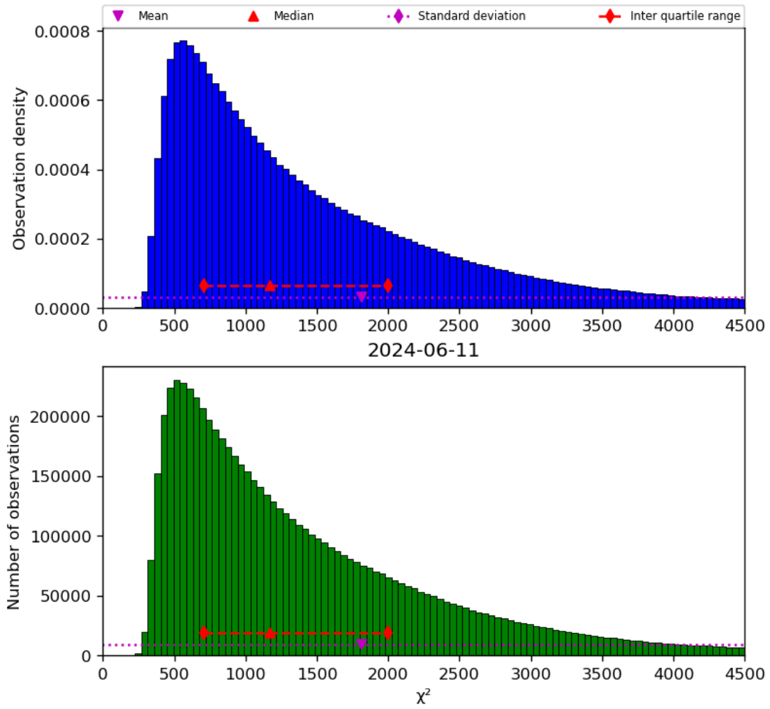
Figure 22: Histogram of “ \chi^2 ” for 2024-06-10 to 2024-06-12
