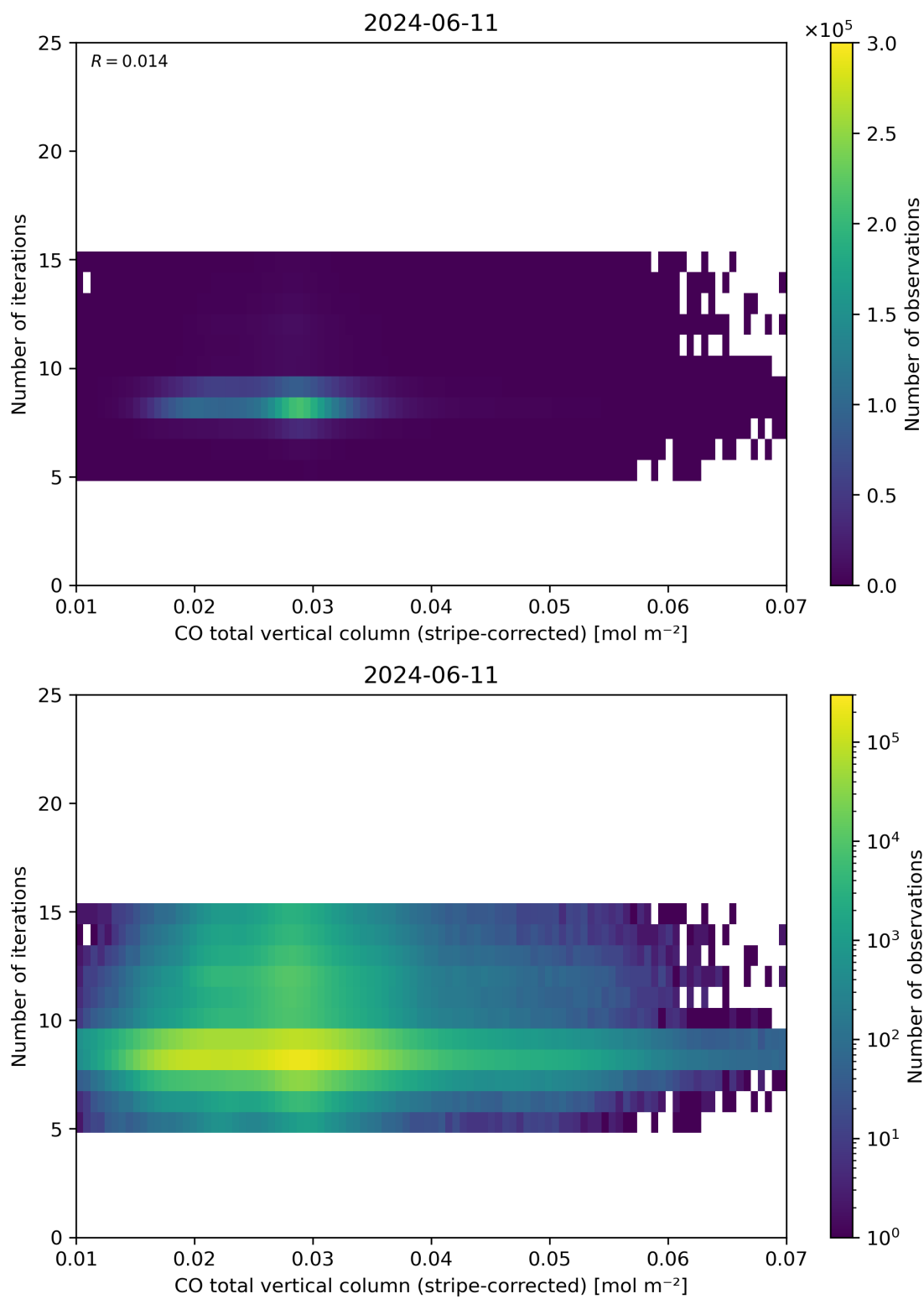
Figure 39: Scatter density plot of “CO total vertical column (stripe-corrected)” against “Number of iterations” for 2024-06-10 to 2024-06-12.
