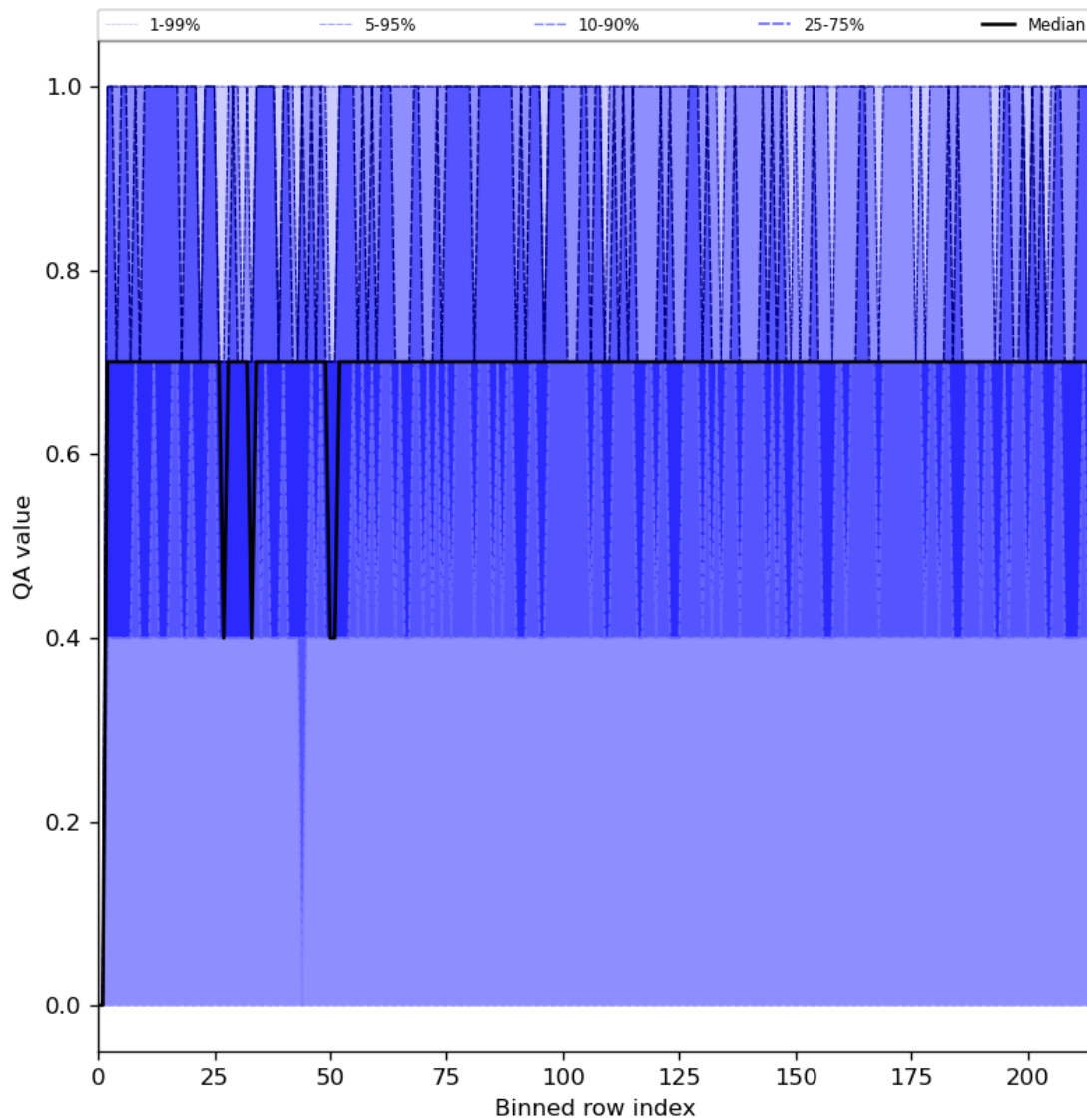
Figure 25: Along track statistics of “QA value” for 2024-06-10 to 2024-06-12
