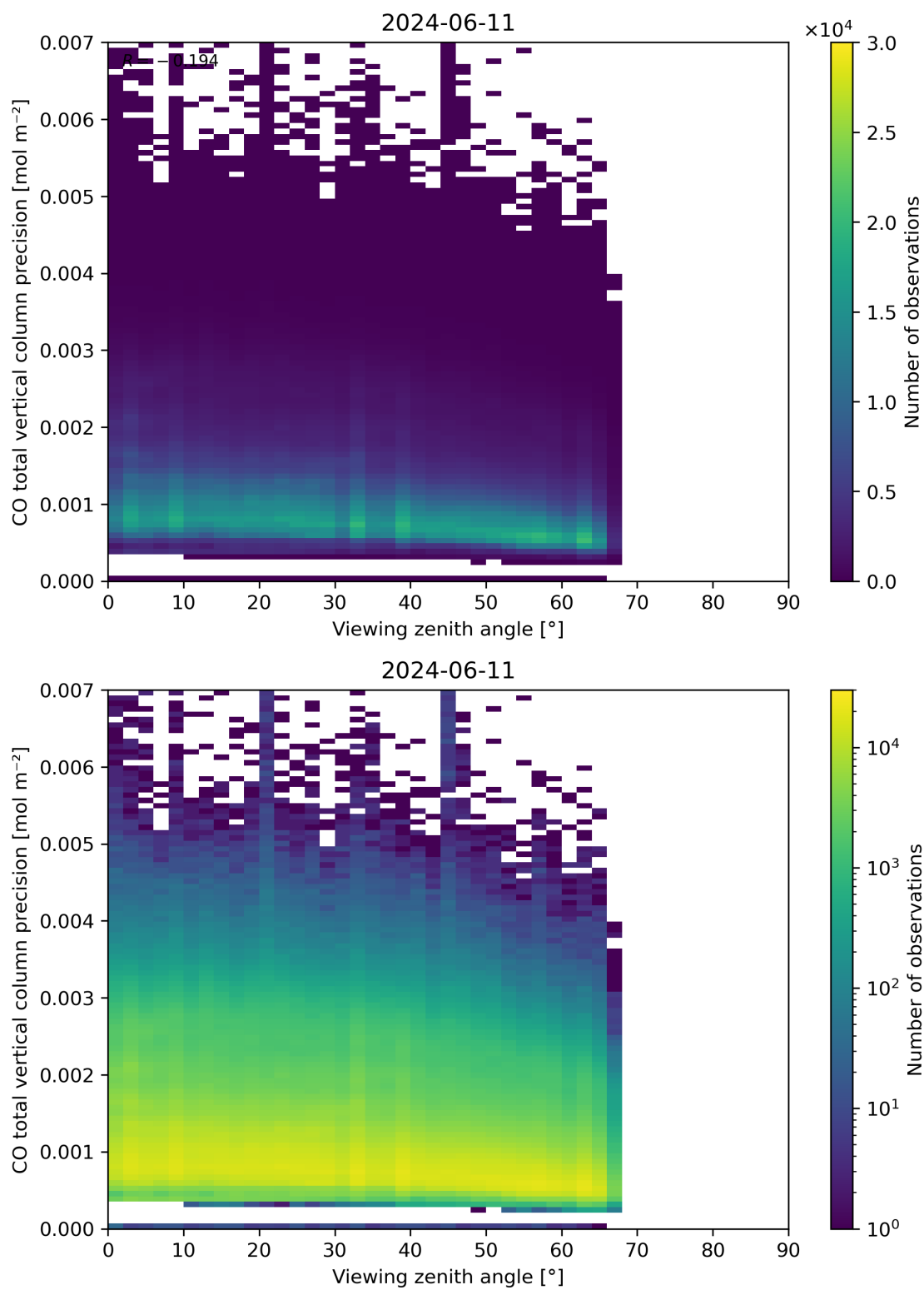
Figure 71: Scatter density plot of “Viewing zenith angle” against “CO total vertical column precision” for 2024-06-10 to 2024-06-12.
