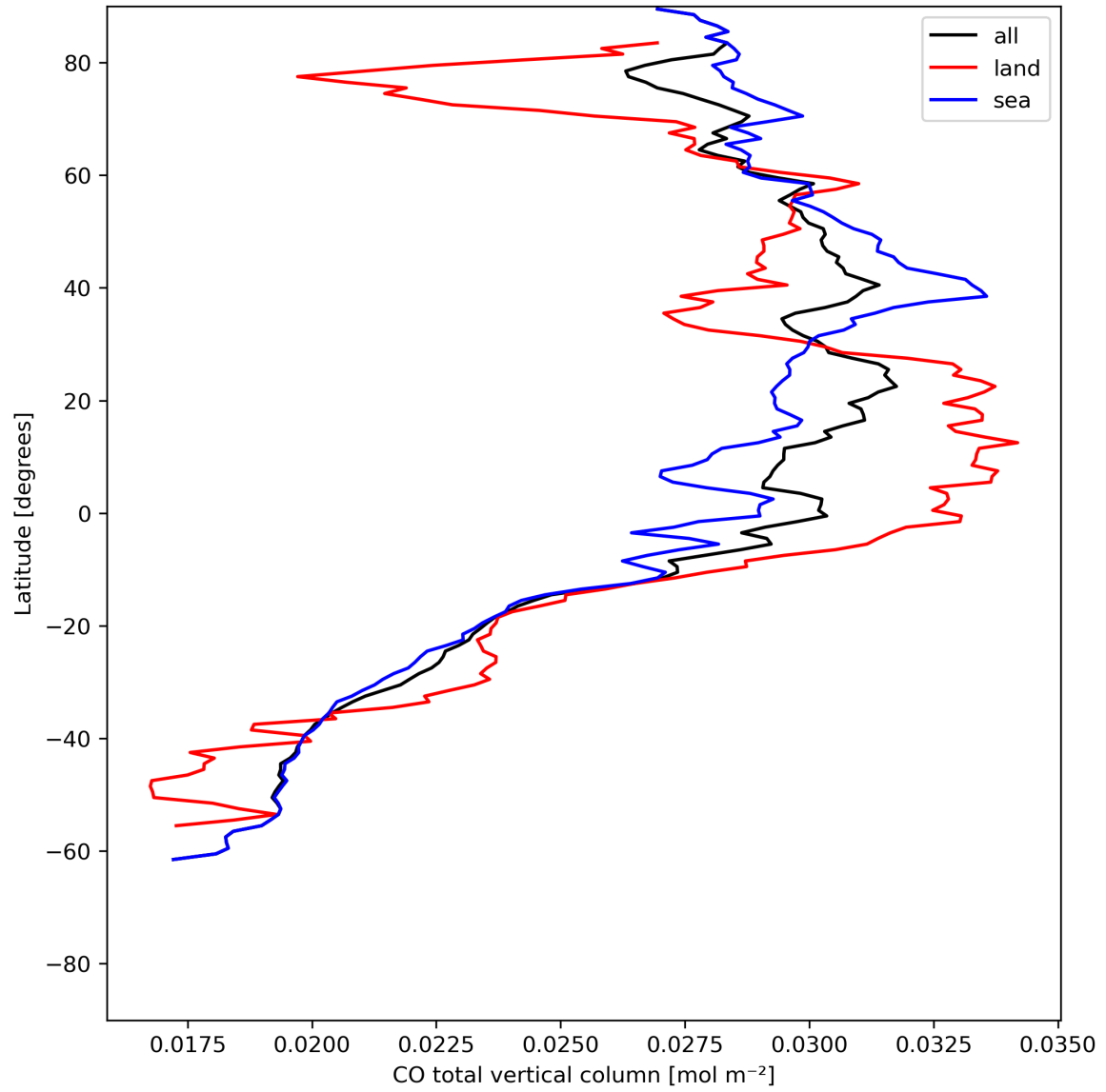
Figure 10: Zonal average of “CO total vertical column” for 2024-06-10 to 2024-06-12.
