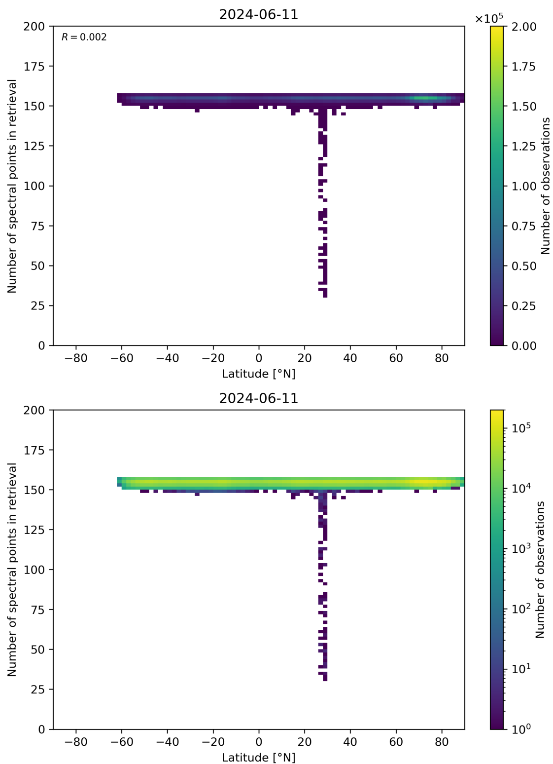
Figure 57: Scatter density plot of “Latitude” against “Number of spectral points in retrieval” for 2024-06-10 to 2024-06-12.
