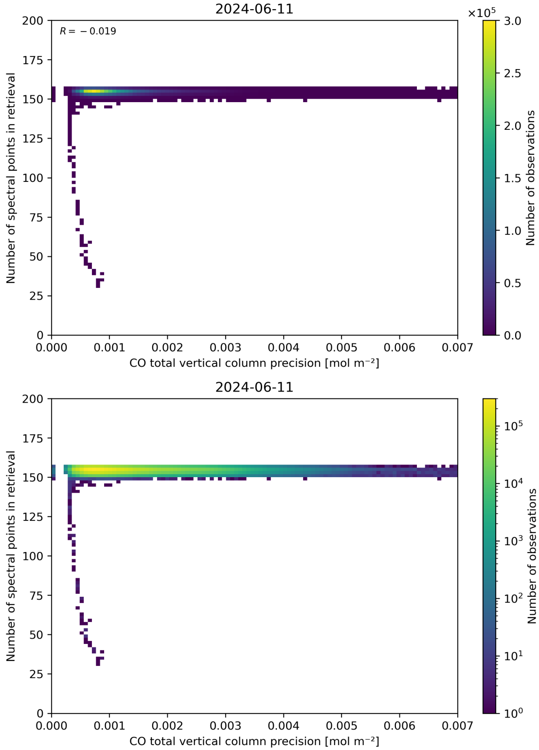
Figure 47: Scatter density plot of “CO total vertical column precision” against “Number of spectral points in retrieval” for 2024-06-10 to 2024-06-12.
