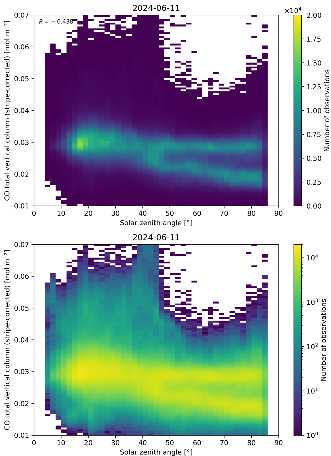
Figure 62: Scatter density plot of “Solar zenith angle” against “CO total vertical column (stripe-corrected)” for 2024-06-10 to 2024-06-12.
