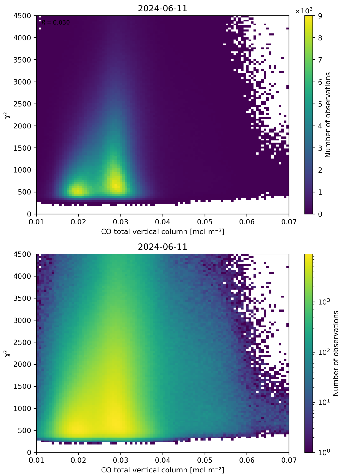
Figure 35: Scatter density plot of “CO total vertical column” against “ \chi^2 ” for 2024-06-10 to 2024-06-12.
