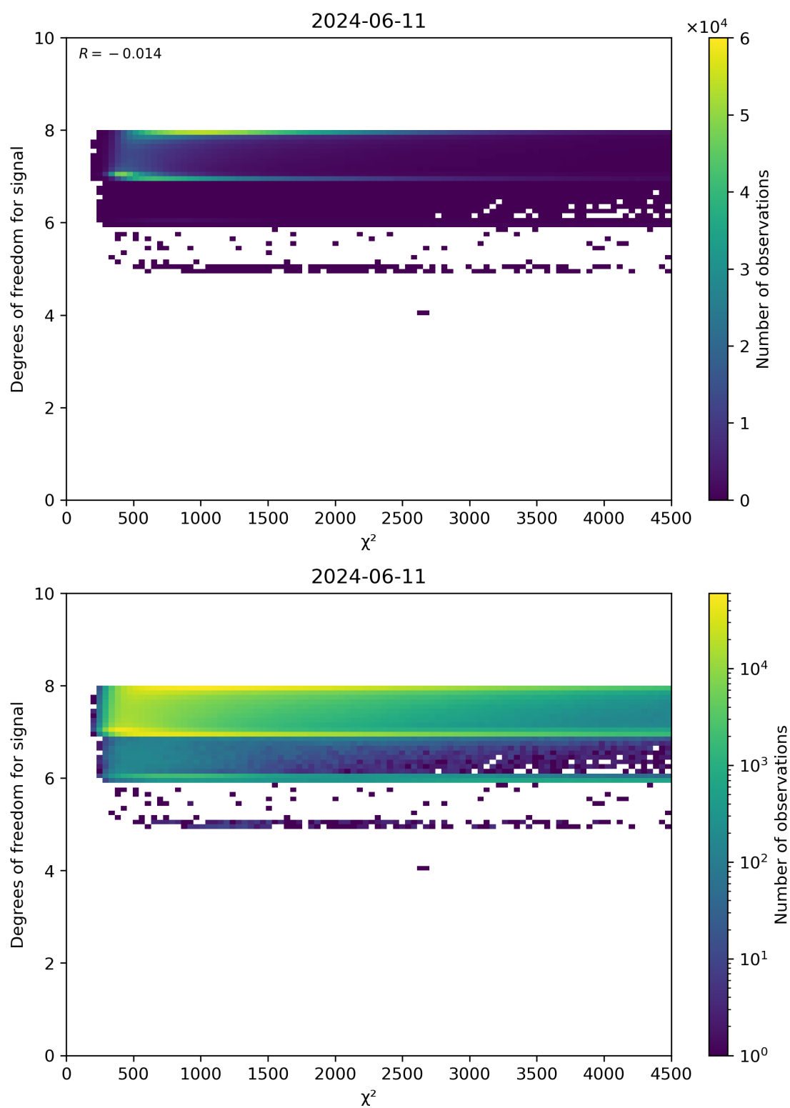
Figure 48: Scatter density plot of “ \chi^2 ” against “Degrees of freedom for signal” for 2024-06-10 to 2024-06-12.
