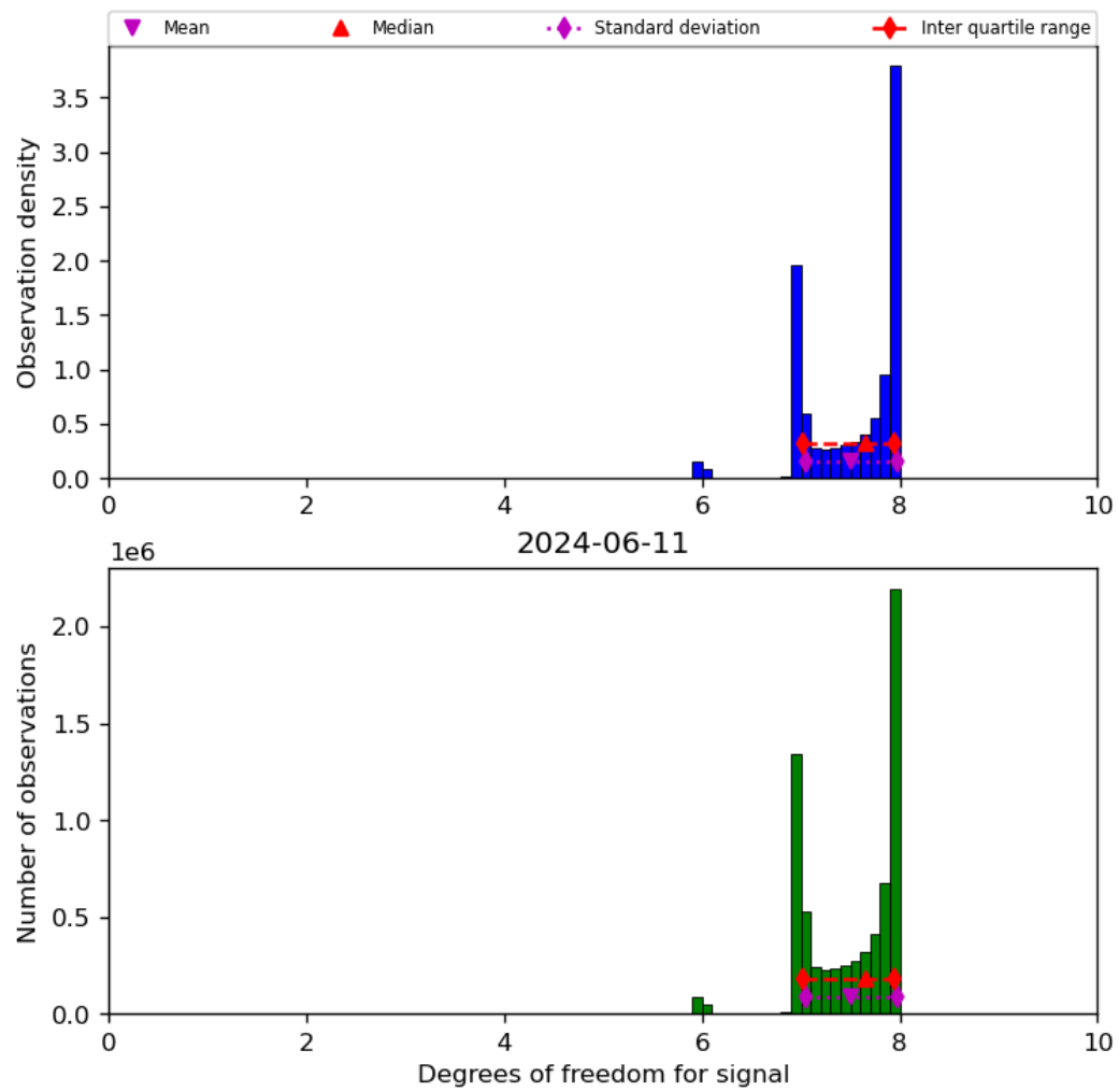
Figure 23: Histogram of “Degrees of freedom for signal” for 2024-06-10 to 2024-06-12
