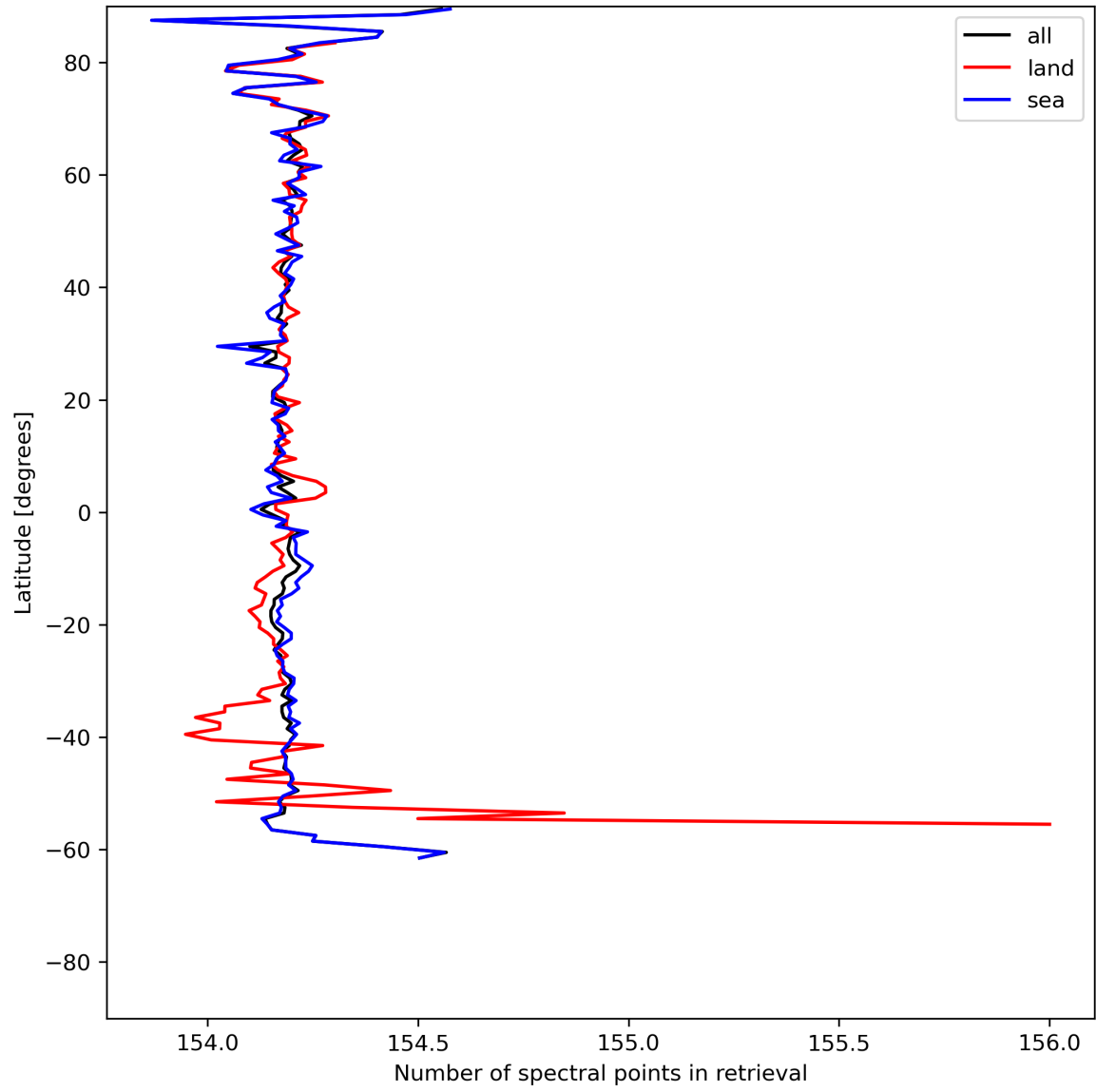
Figure 13: Zonal average of “Number of spectral points in retrieval” for 2024-06-10 to 2024-06-12.
