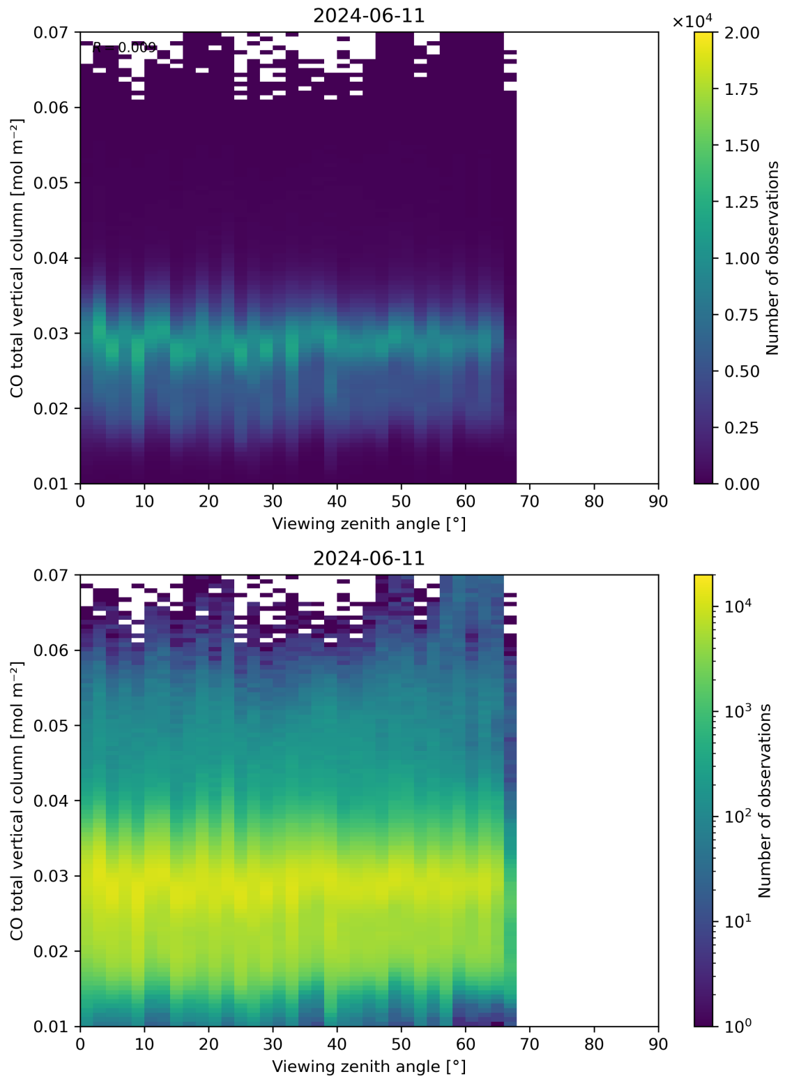
Figure 69: Scatter density plot of “Viewing zenith angle” against “CO total vertical column” for 2024-06-10 to 2024-06-12.
