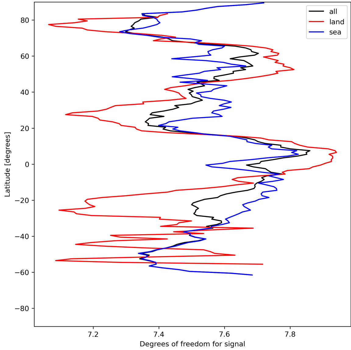
Figure 15: Zonal average of “Degrees of freedom for signal” for 2024-06-10 to 2024-06-12.
