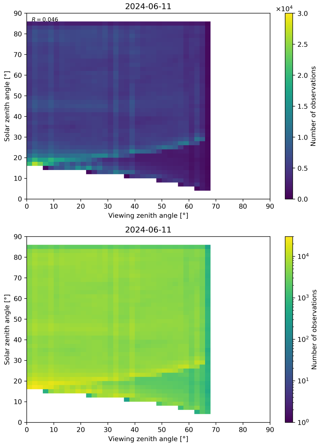
Figure 77: Scatter density plot of “Viewing zenith angle” against “Solar zenith angle” for 2024-06-10 to 2024-06-12.
