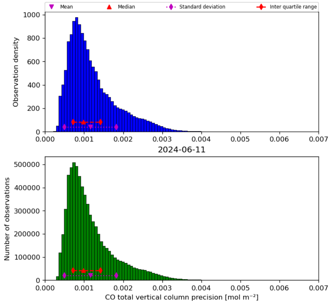
Figure 20: Histogram of “CO total vertical column precision” for 2024-06-10 to 2024-06-12
