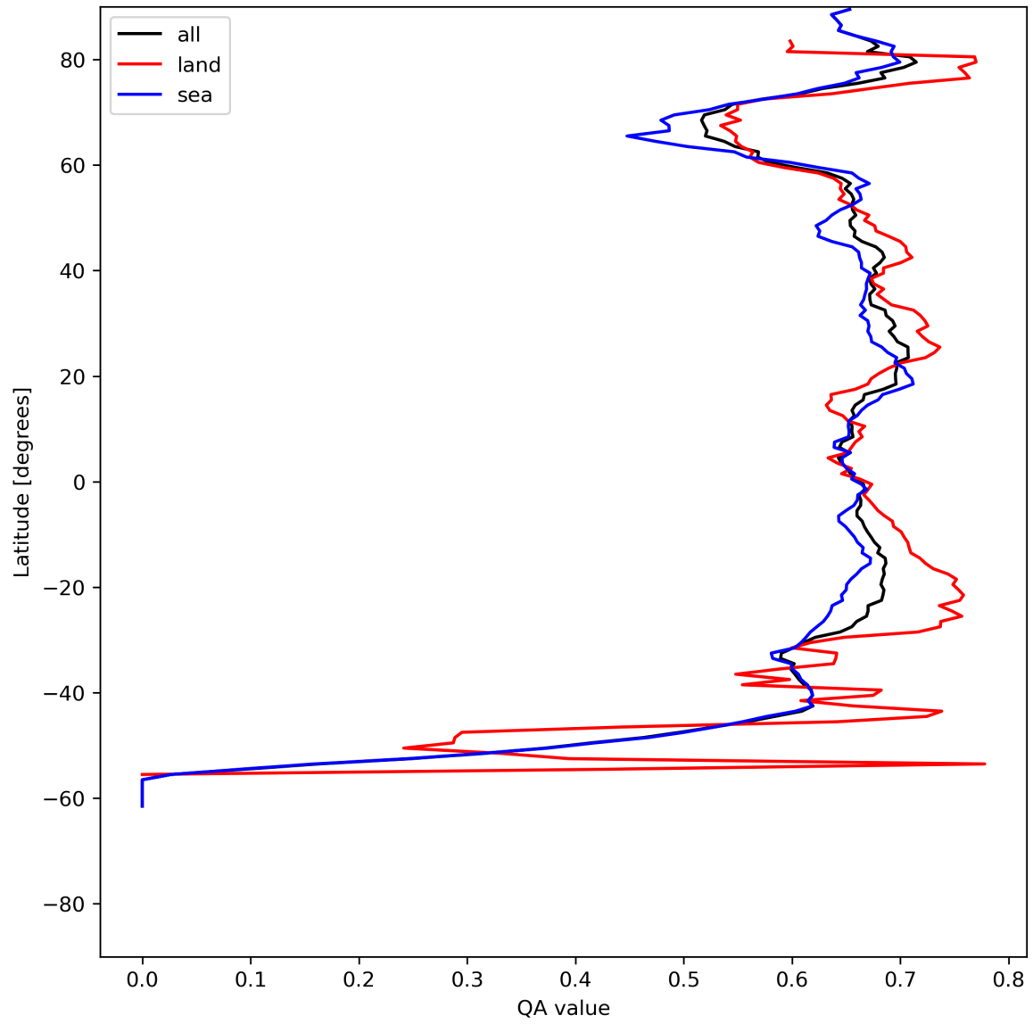
Figure 9: Zonal average of “QA value” for 2024-06-10 to 2024-06-12.
