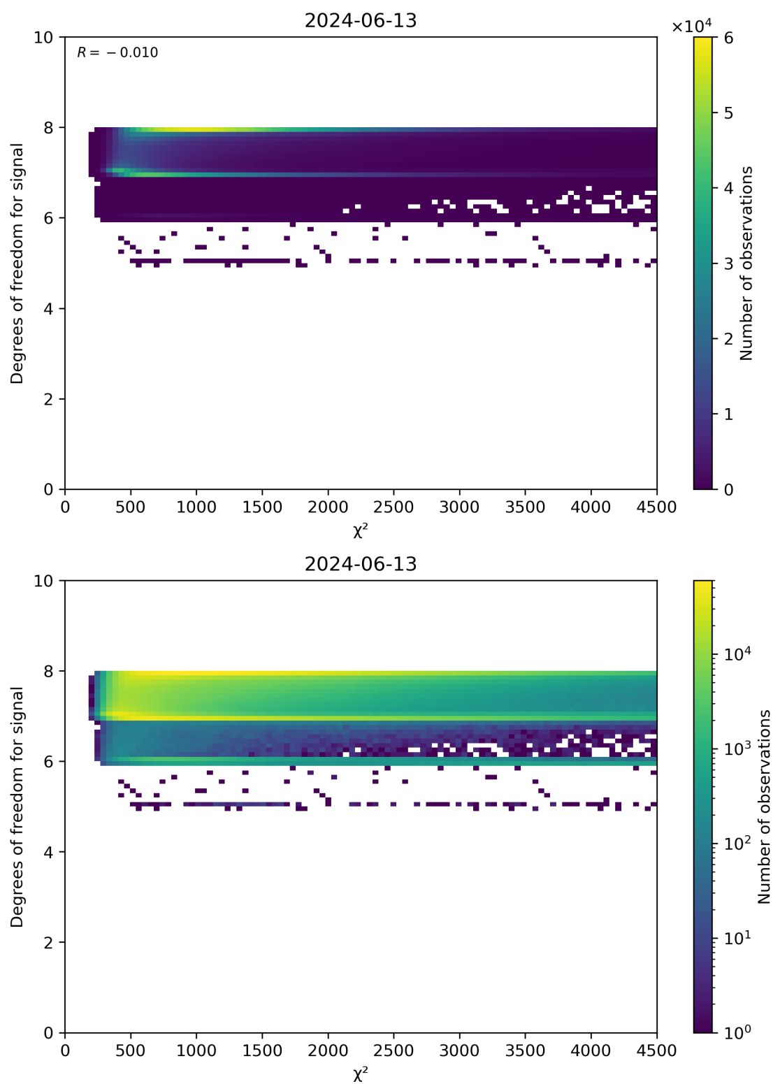
Figure 48: Scatter density plot of " \chi^2 " against "Degrees of freedom for signal" for 2024-06-13 to 2024-06-14.
