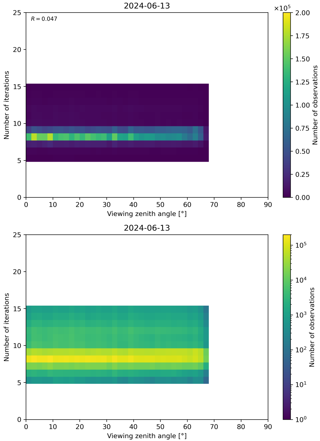
Figure 75: Scatter density plot of “Viewing zenith angle” against “Number of iterations” for 2024-06-13 to 2024-06-14.
