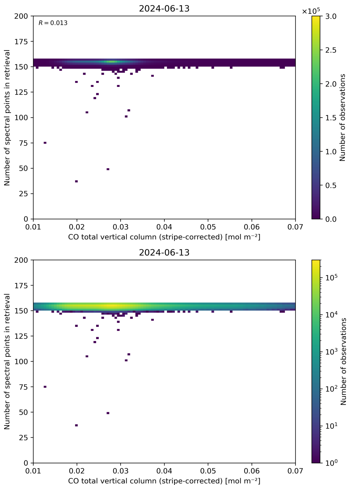
Figure 40: Scatter density plot of “CO total vertical column (stripe-corrected)” against “Number of spectral points in retrieval” for 2024-06-13 to 2024-06-14.
