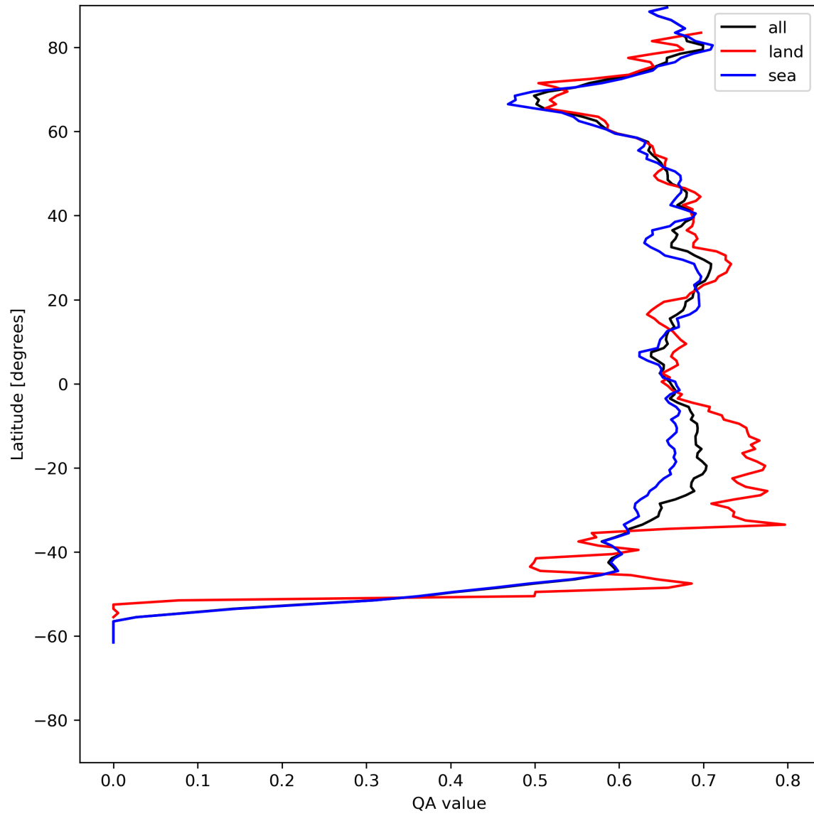
Figure 9: Zonal average of “QA value” for 2024-06-13 to 2024-06-14.
