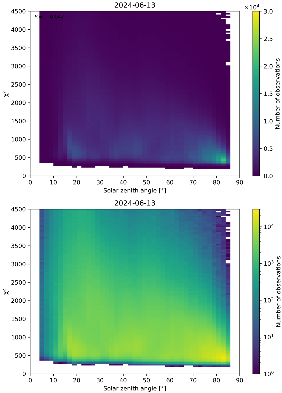
Figure 64: Scatter density plot of “Solar zenith angle” against “ \chi^2 ” for 2024-06-13 to 2024-06-14.
