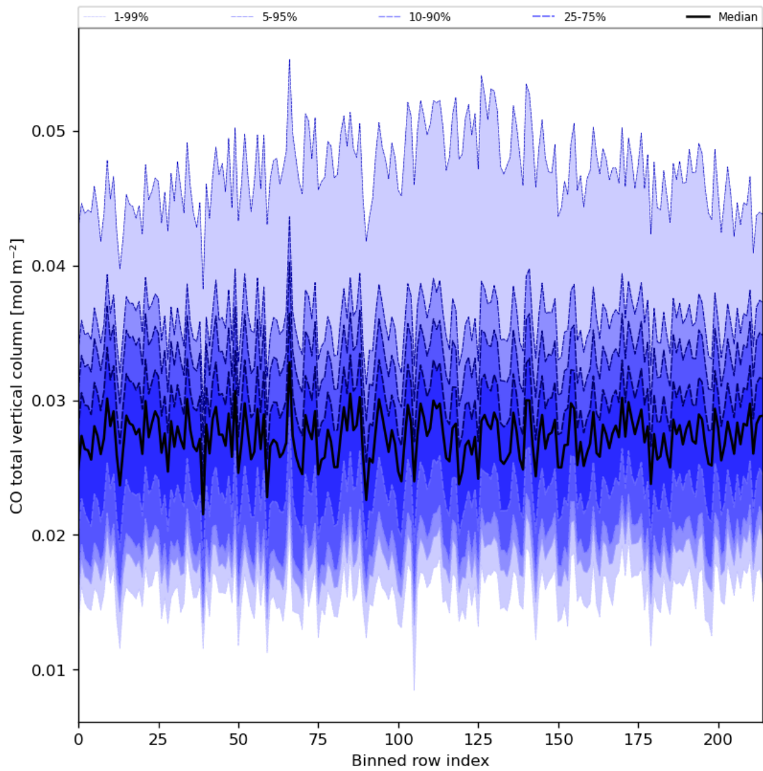
Figure 26: Along track statistics of “CO total vertical column” for 2024-06-13 to 2024-06-14
