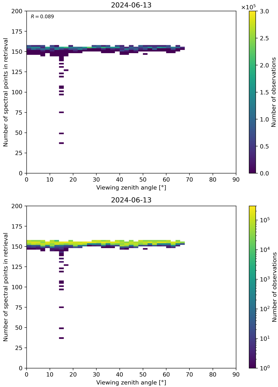
Figure 76: Scatter density plot of “Viewing zenith angle” against “Number of spectral points in retrieval” for 2024-06-13 to 2024-06-14.
