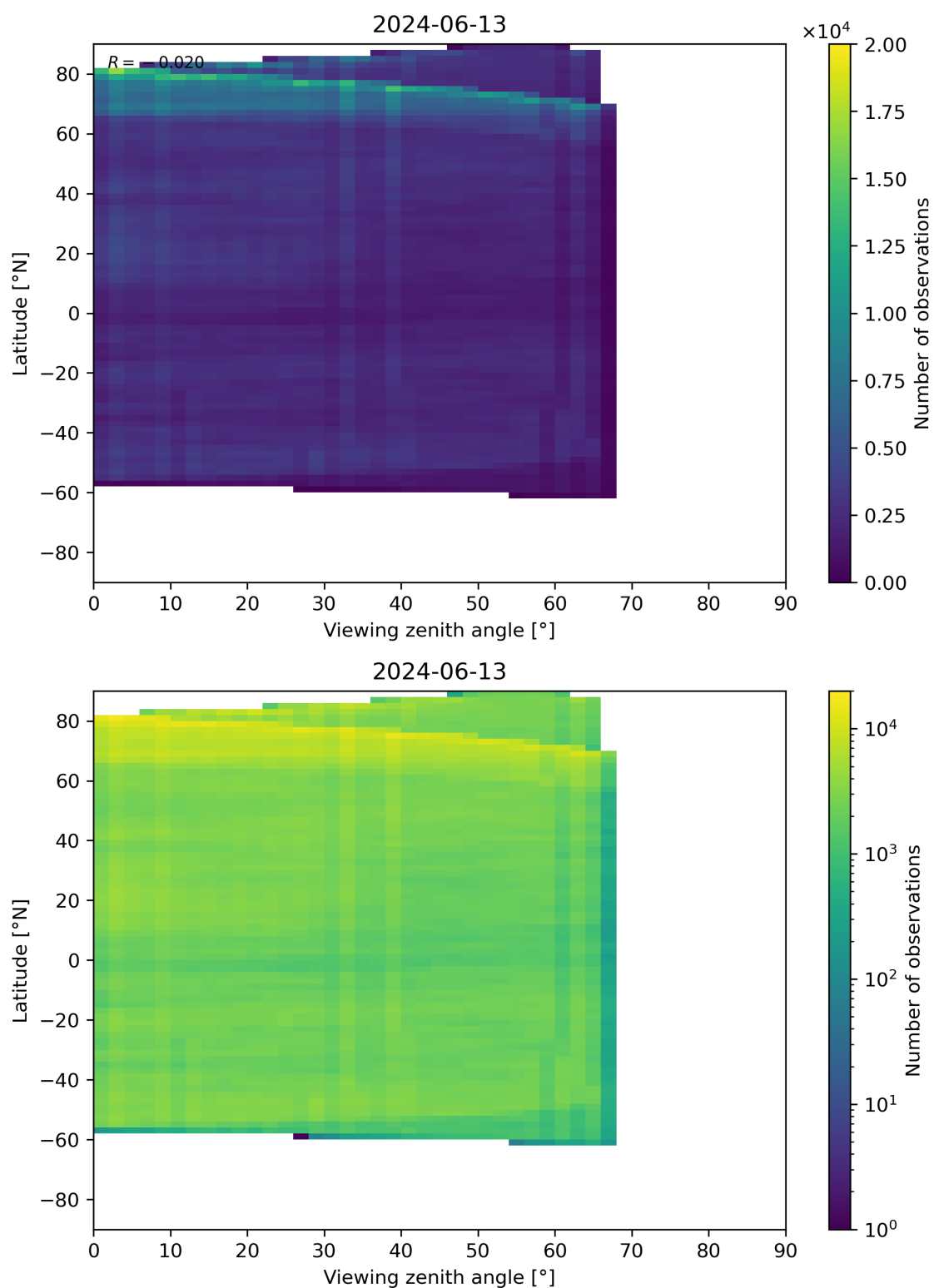
Figure 74: Scatter density plot of “Viewing zenith angle” against “Latitude” for 2024-06-13 to 2024-06-14.
