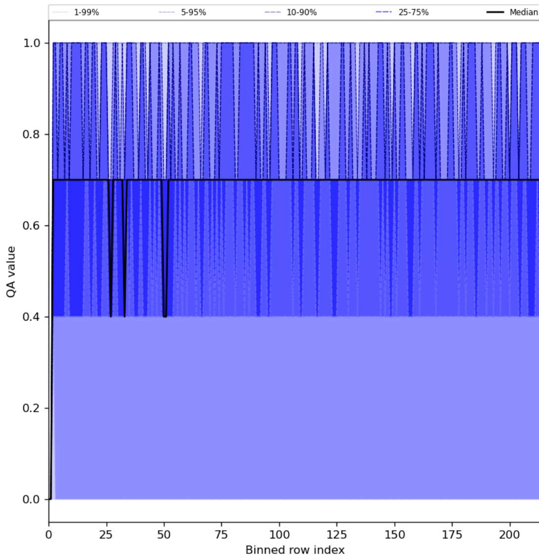
Figure 25: Along track statistics of "QA value" for 2024-06-13 to 2024-06-14
