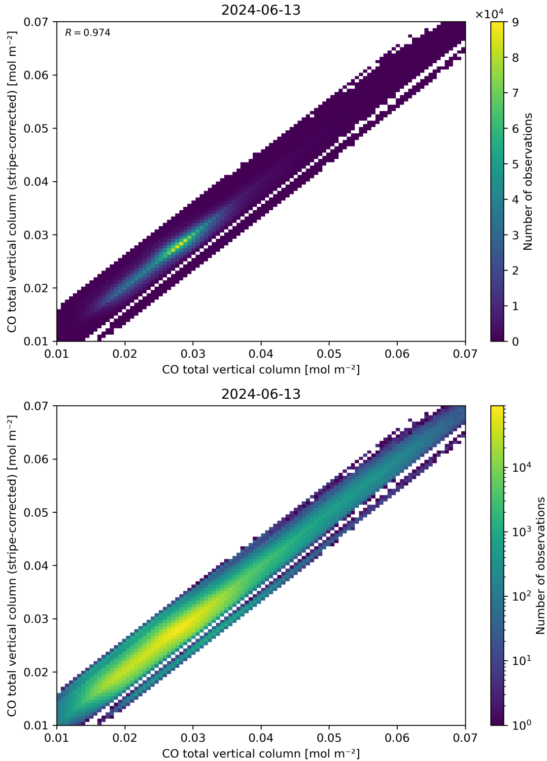
Figure 33: Scatter density plot of “CO total vertical column” against “CO total vertical column (stripe-corrected)” for 2024-06-13 to 2024-06-14.
