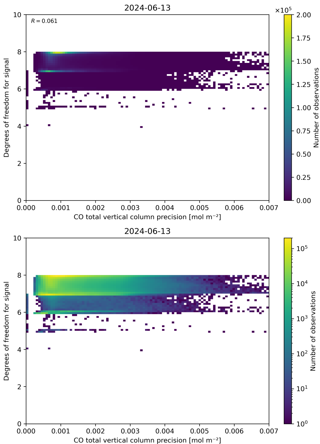
Figure 45: Scatter density plot of “CO total vertical column precision” against “Degrees of freedom for signal” for 2024-06-13 to 2024-06-14.
