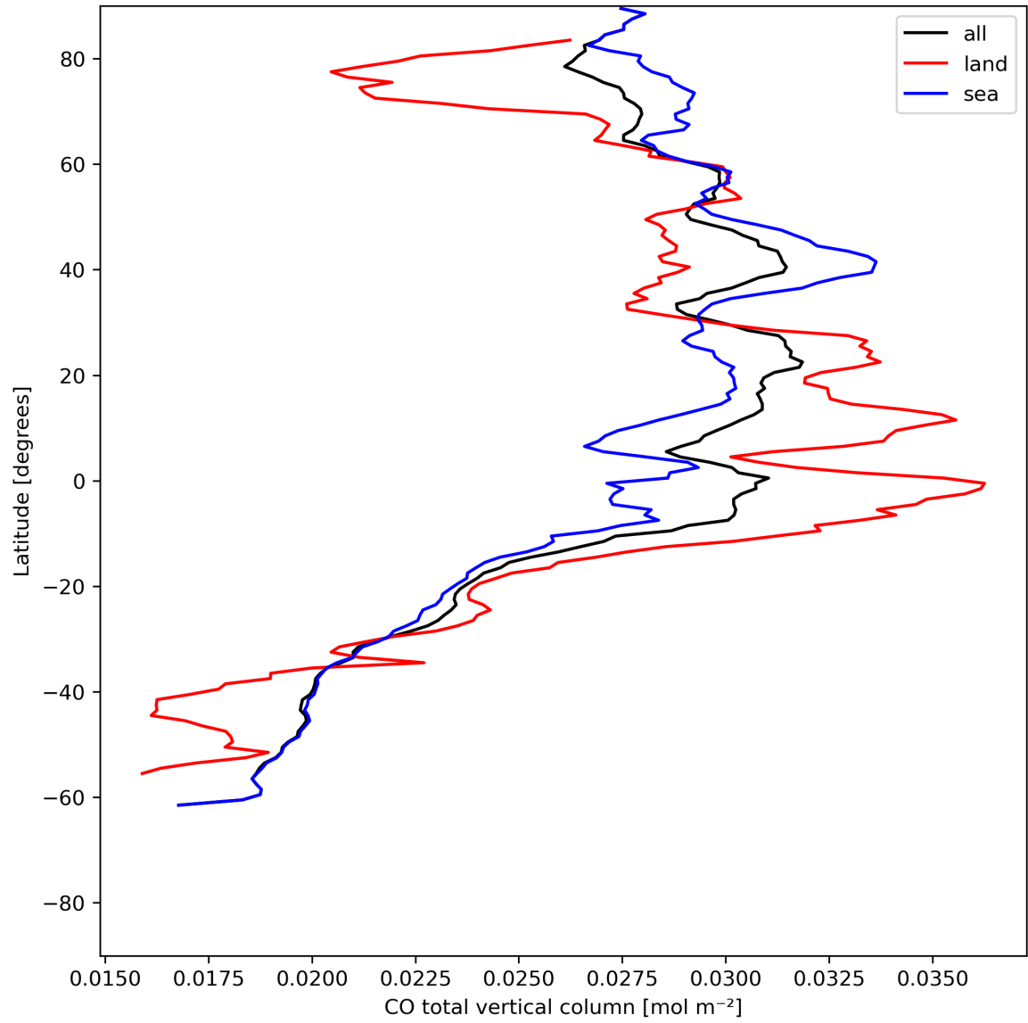
Figure 10: Zonal average of “CO total vertical column” for 2024-06-13 to 2024-06-14.
