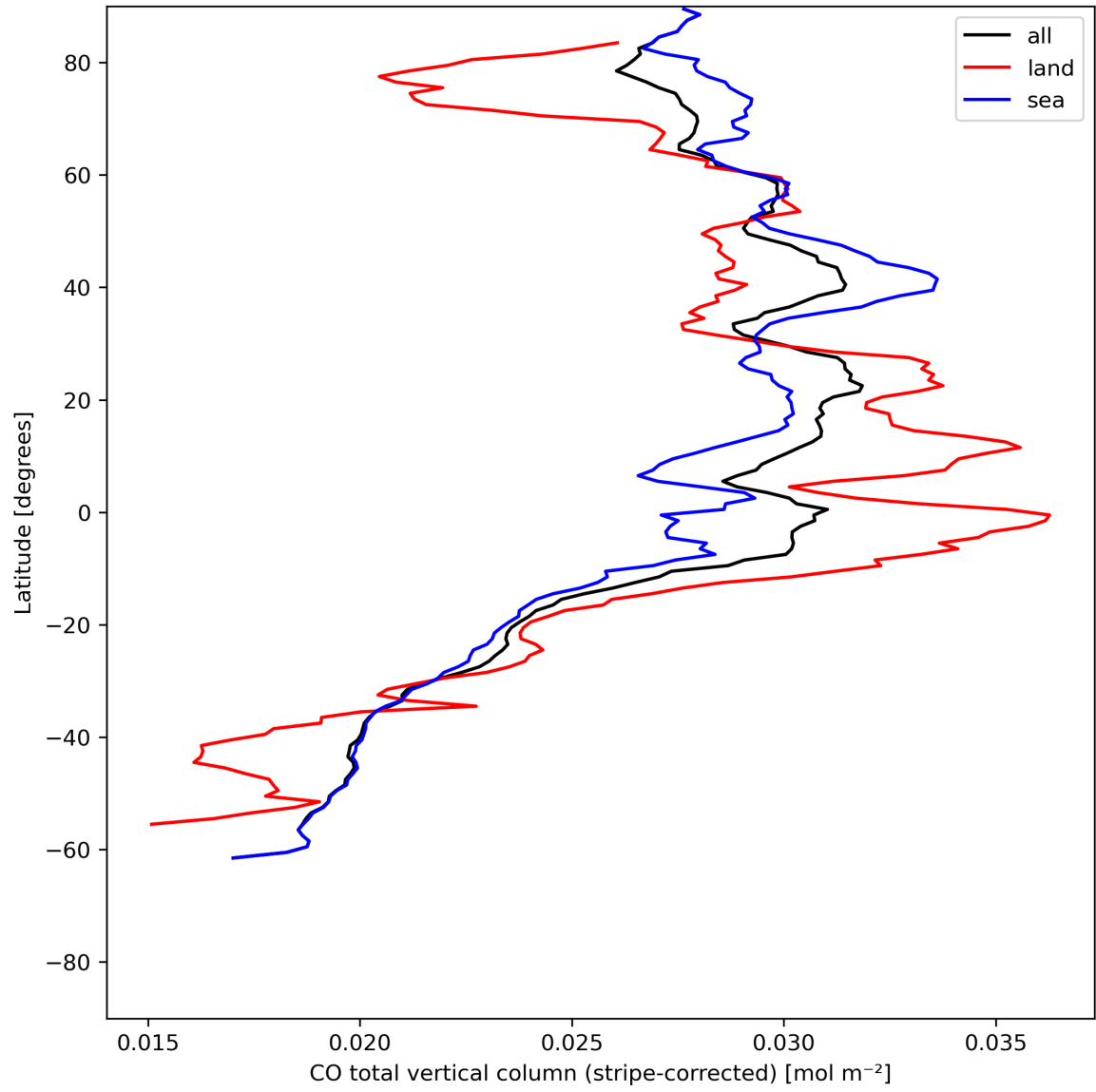
Figure 11: Zonal average of “CO total vertical column (stripe-corrected)” for 2024-06-13 to 2024-06-14.
