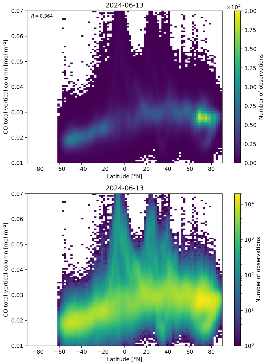
Figure 51: Scatter density plot of “Latitude” against “CO total vertical column” for 2024-06-13 to 2024-06-14.
