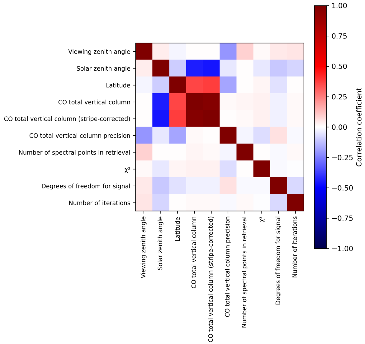
Figure 2: Map of correlation matrix for 2024-06-13 to 2024-06-14.
