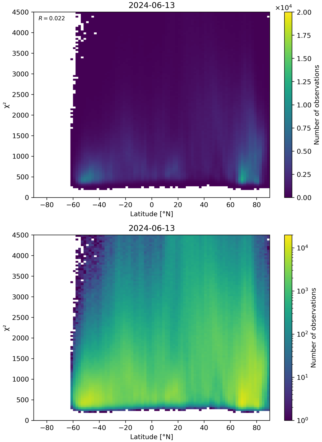
Figure 54: Scatter density plot of “Latitude” against “ \chi^2 ” for 2024-06-13 to 2024-06-14.
