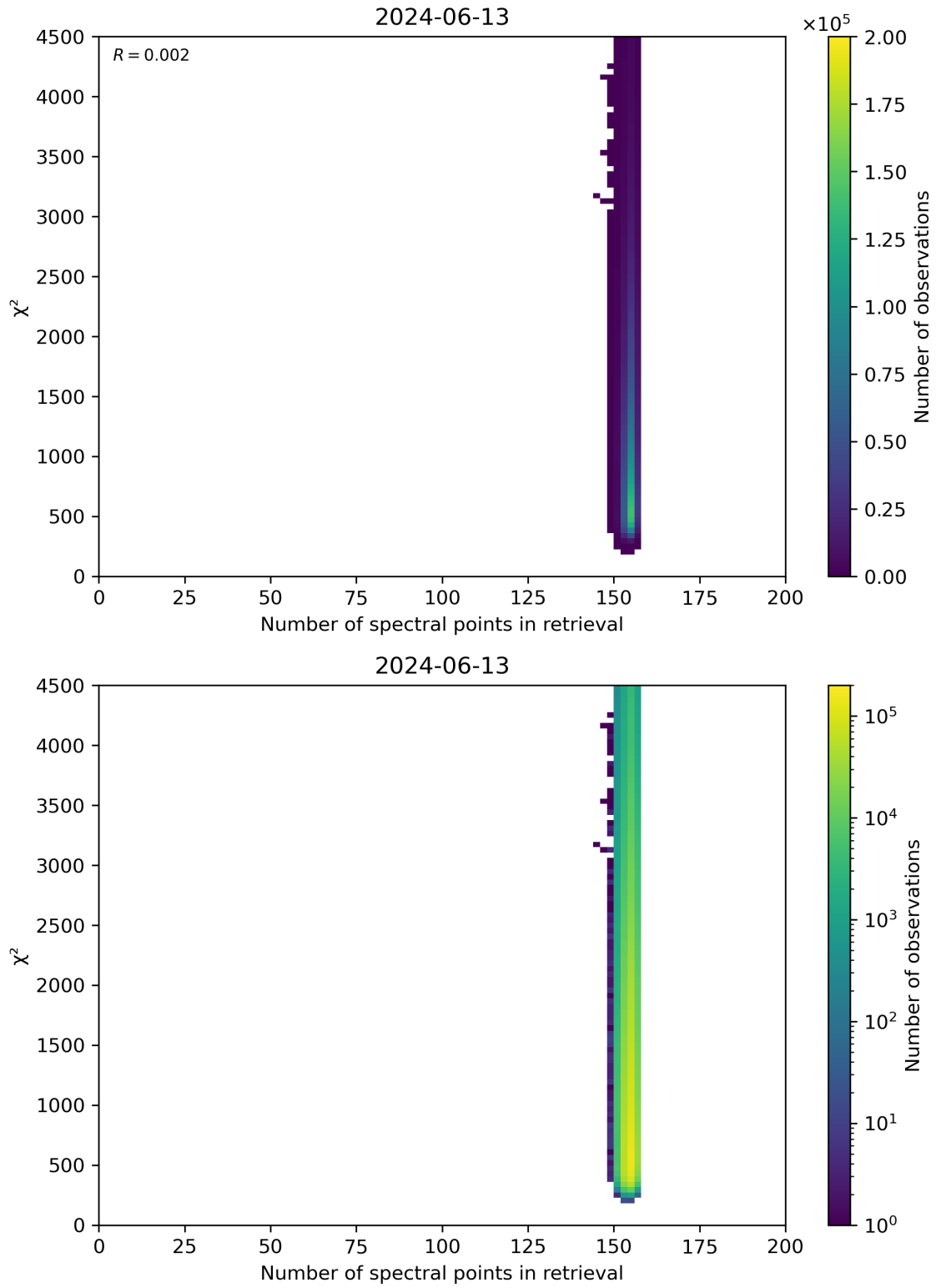
Figure 58: Scatter density plot of “Number of spectral points in retrieval” against “ \chi^2 ” for 2024-06-13 to 2024-06-14.
