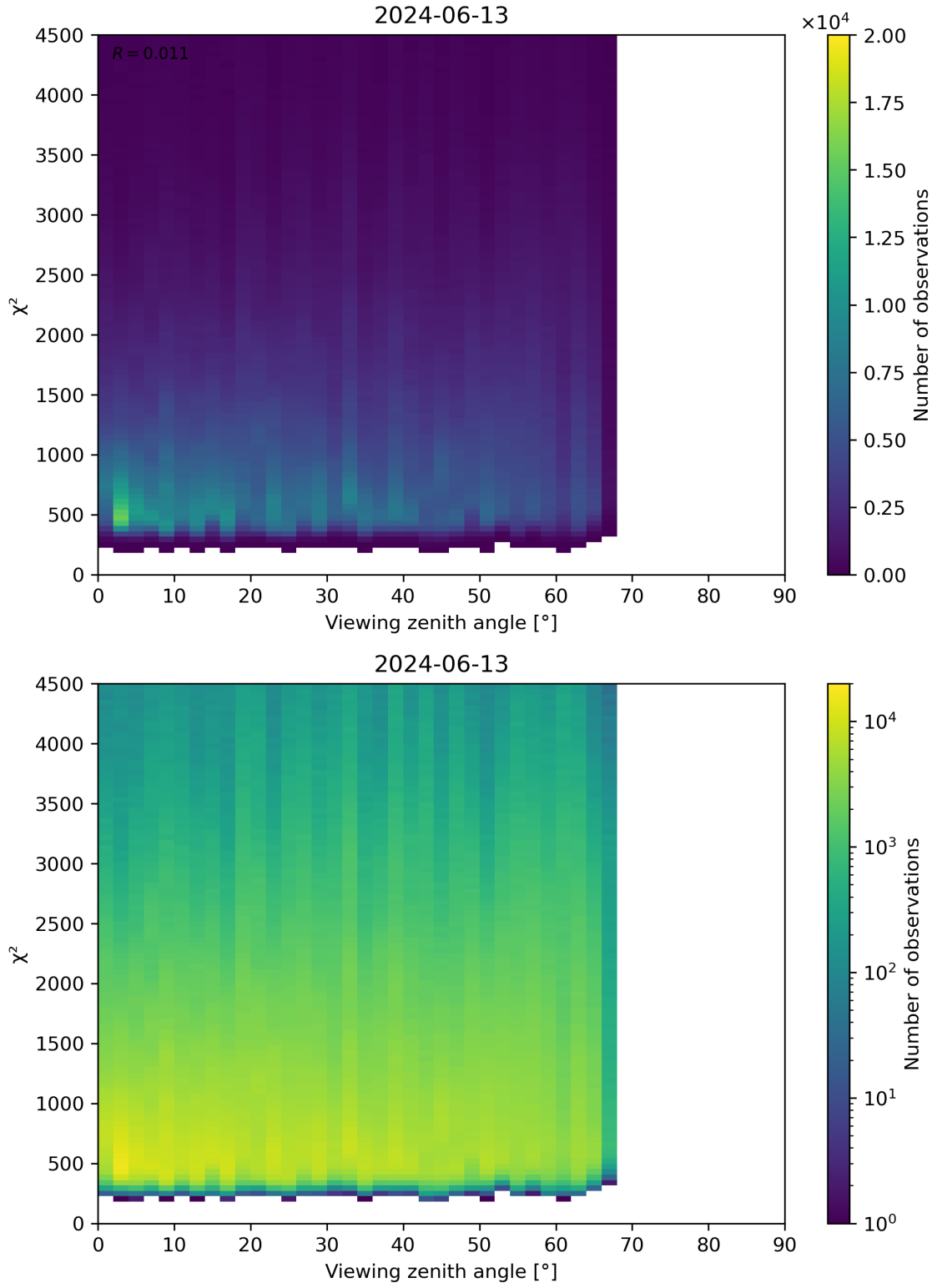
Figure 72: Scatter density plot of “Viewing zenith angle” against “ \chi^2 ” for 2024-06-13 to 2024-06-14.
