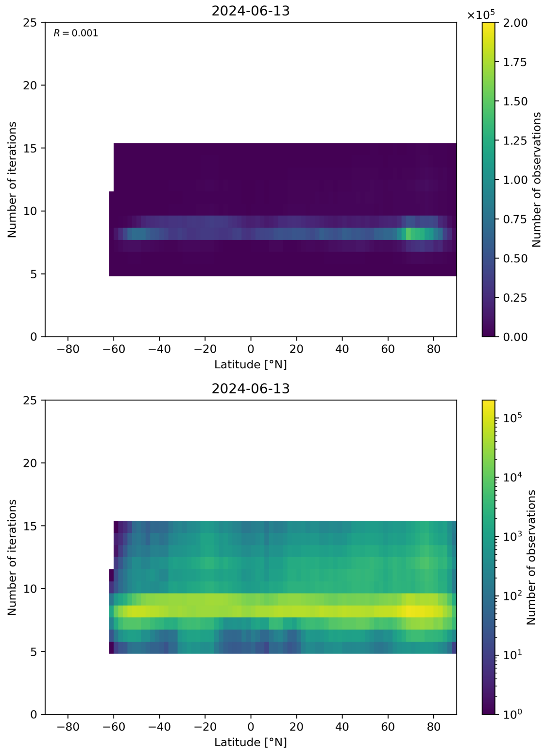
Figure 56: Scatter density plot of “Latitude” against “Number of iterations” for 2024-06-13 to 2024-06-14.
