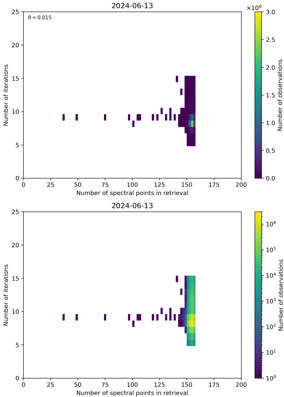
Figure 60: Scatter density plot of “Number of spectral points in retrieval” against “Number of iterations” for 2024-06-13 to 2024-06-14.
