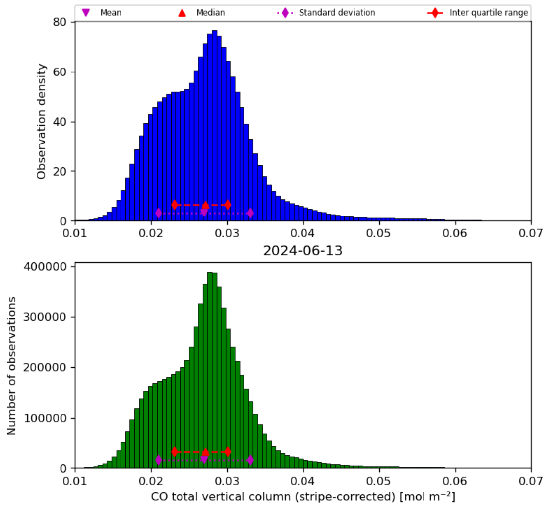
Figure 19: Histogram of “CO total vertical column (stripe-corrected)” for 2024-06-13 to 2024-06-14
