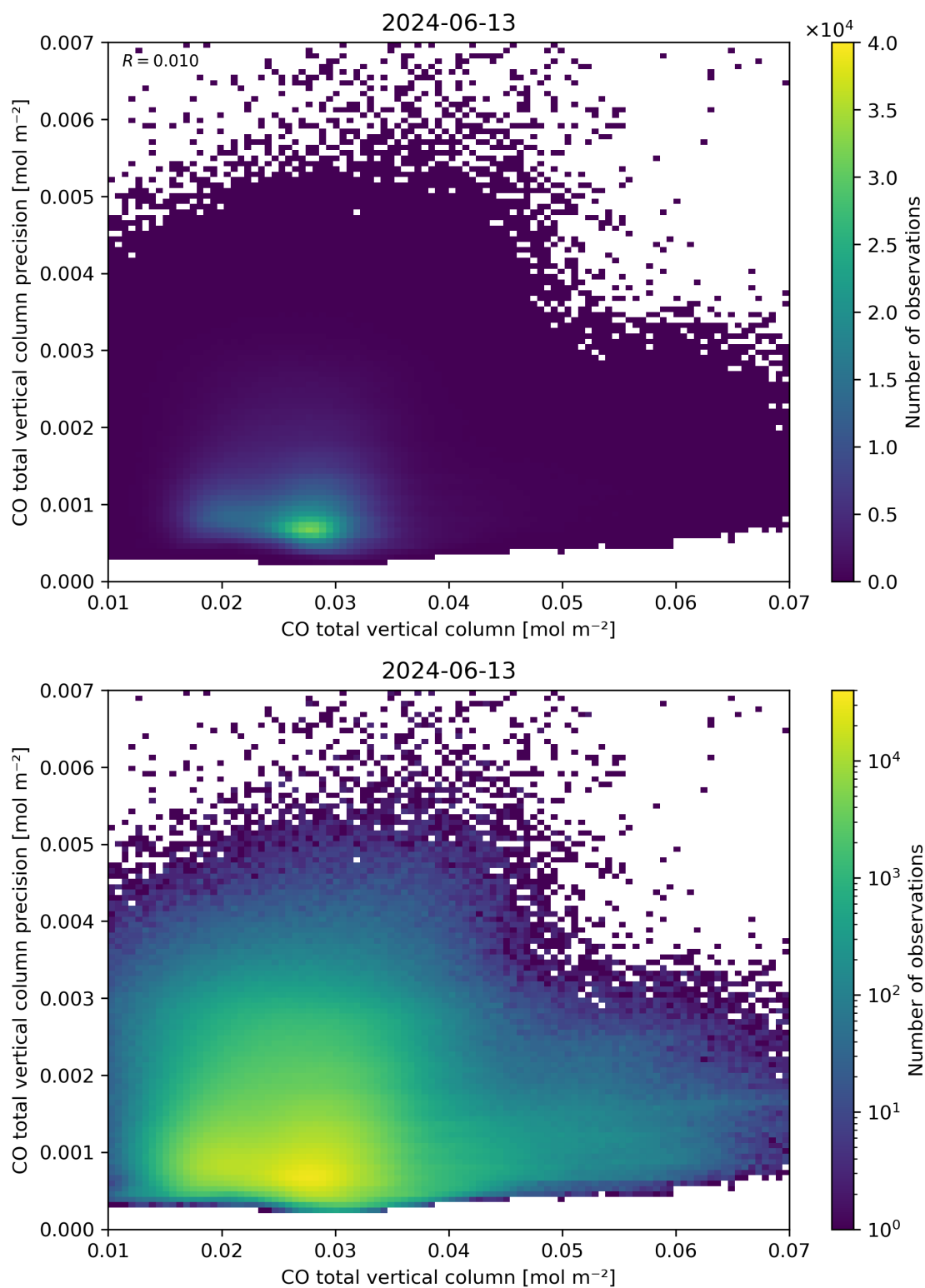
Figure 34: Scatter density plot of “CO total vertical column” against “CO total vertical column precision” for 2024-06-13 to 2024-06-14.
