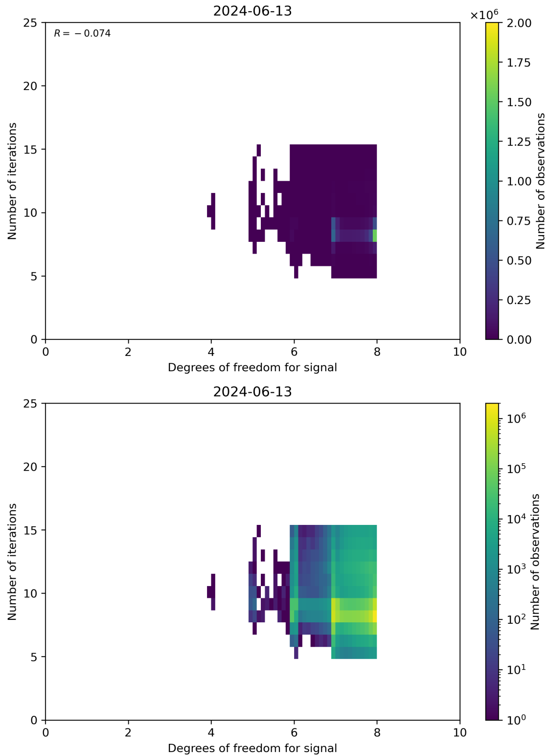
Figure 50: Scatter density plot of “Degrees of freedom for signal” against “Number of iterations” for 2024-06-13 to 2024-06-14.
