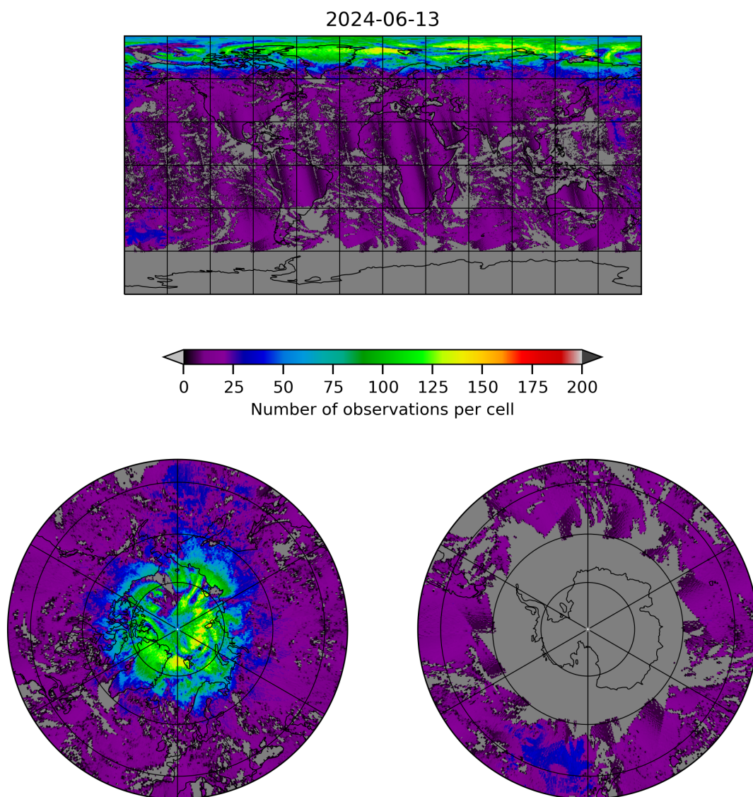
Figure 8: Map of the number of observations for 2024-06-13 to 2024-06-14
