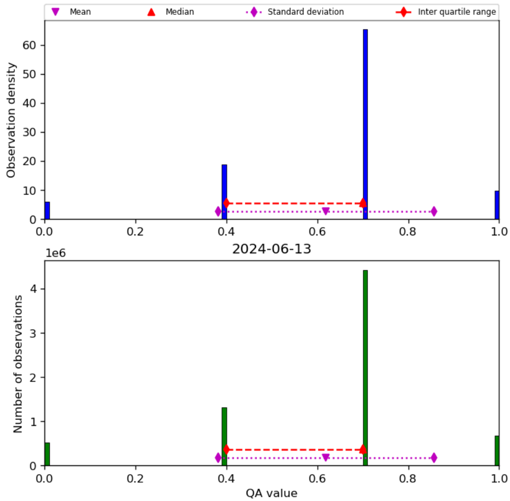
Figure 17: Histogram of “QA value” for 2024-06-13 to 2024-06-14
