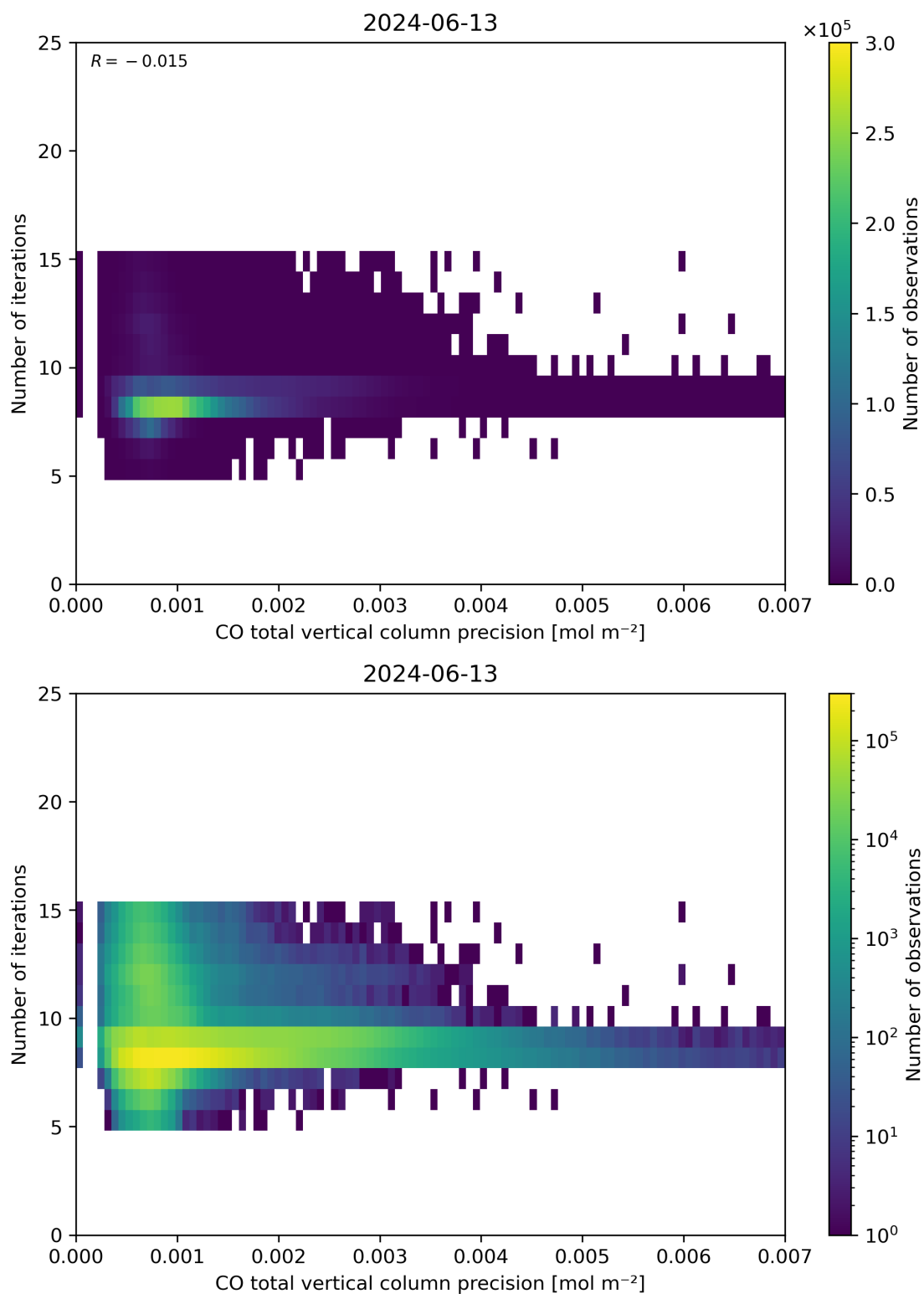
Figure 46: Scatter density plot of “CO total vertical column precision” against “Number of iterations” for 2024-06-13 to 2024-06-14.
