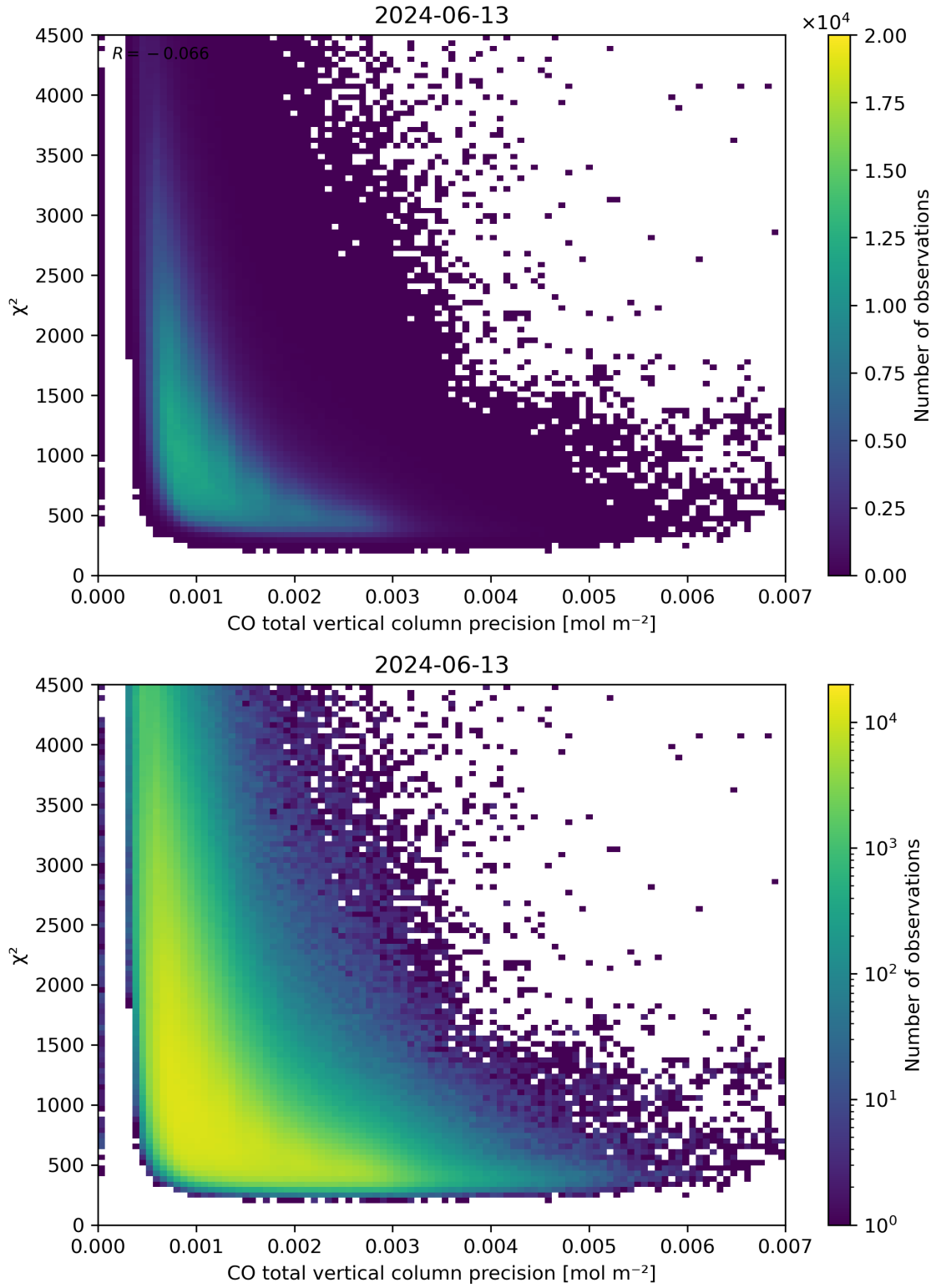
Figure 44: Scatter density plot of “CO total vertical column precision” against “ \chi^2 ” for 2024-06-13 to 2024-06-14.
