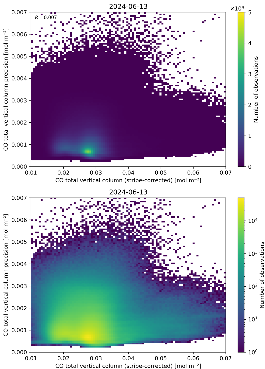
Figure 36: Scatter density plot of “CO total vertical column (stripe-corrected)” against “CO total vertical column precision” for 2024-06-13 to 2024-06-14.
