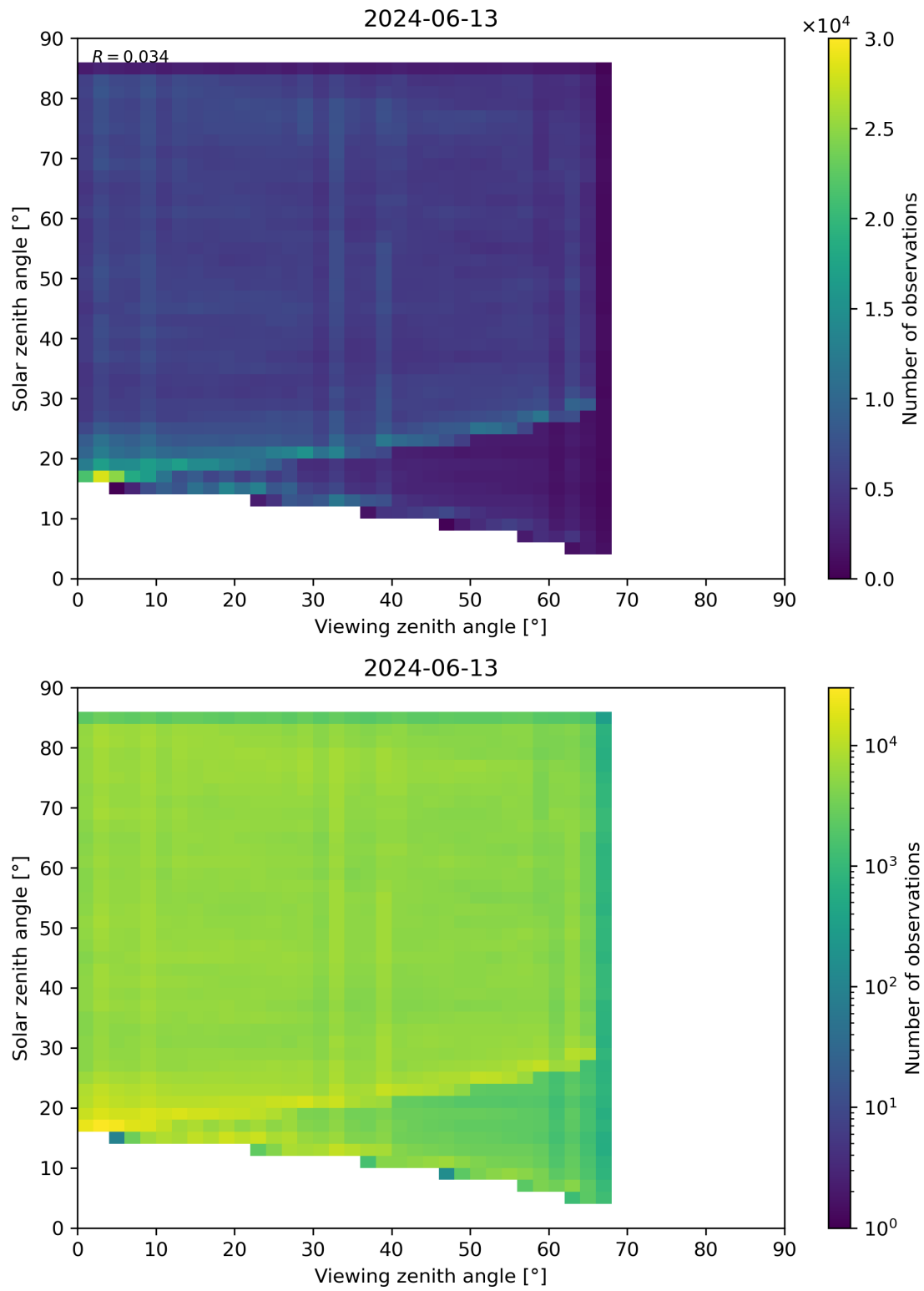
Figure 77: Scatter density plot of “Viewing zenith angle” against “Solar zenith angle” for 2024-06-13 to 2024-06-14.
