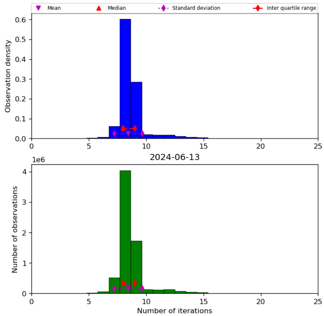
Figure 24: Histogram of “Number of iterations” for 2024-06-13 to 2024-06-14
