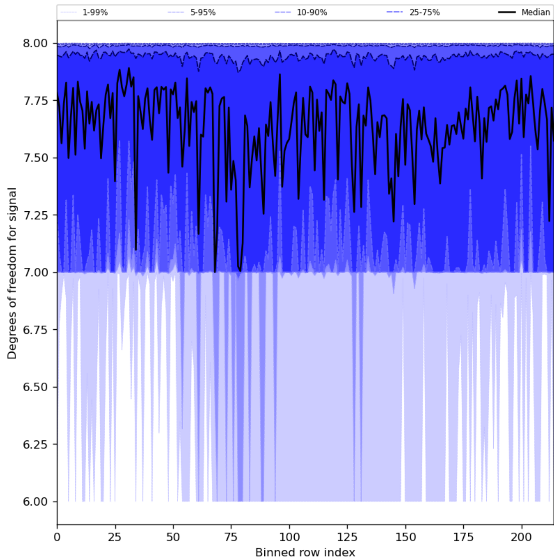
Figure 31: Along track statistics of “Degrees of freedom for signal” for 2024-06-13 to 2024-06-14
