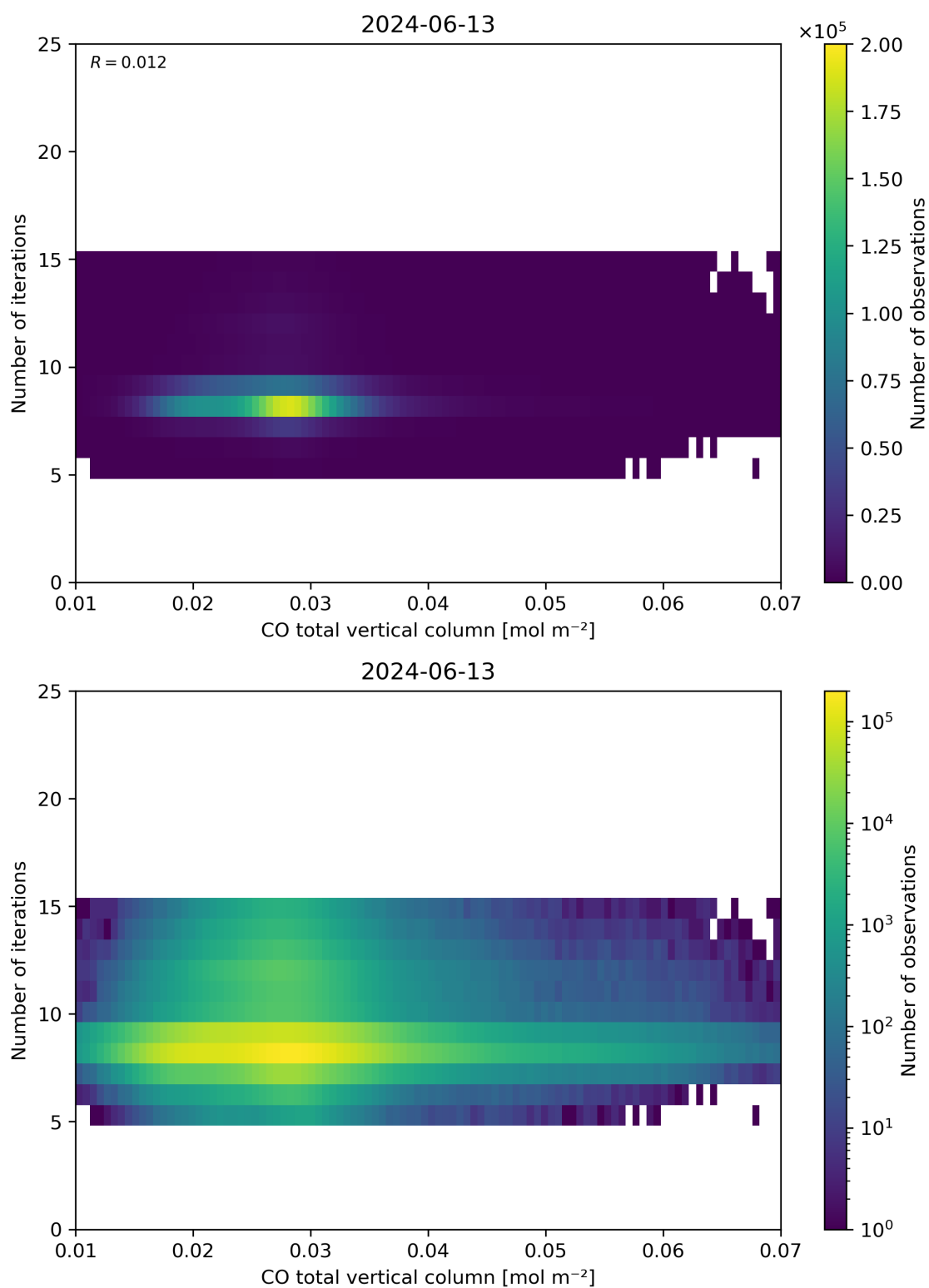
Figure 42: Scatter density plot of “CO total vertical column” against “Number of iterations” for 2024-06-13 to 2024-06-14.
