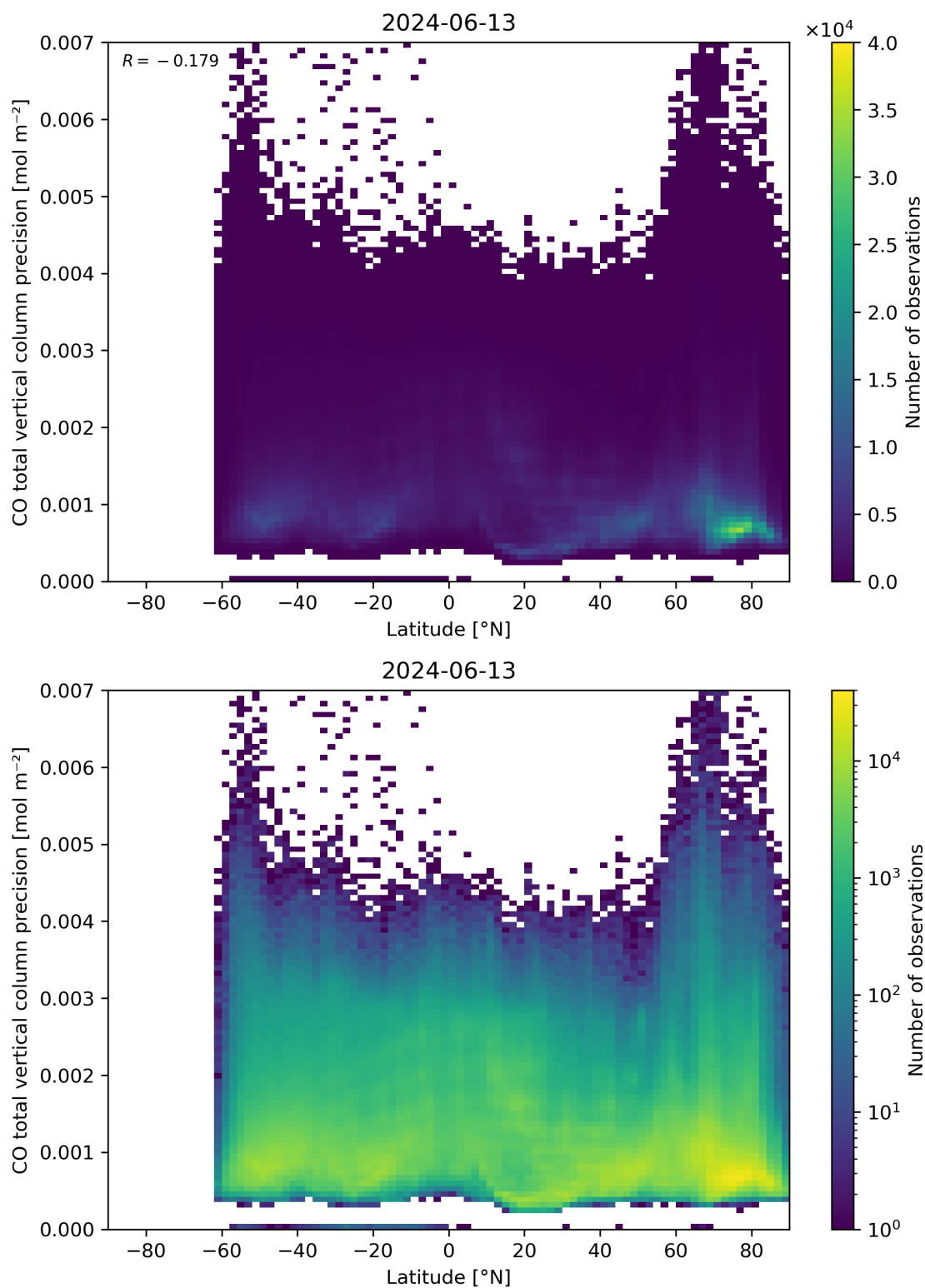
Figure 53: Scatter density plot of “Latitude” against “CO total vertical column precision” for 2024-06-13 to 2024-06-14.
