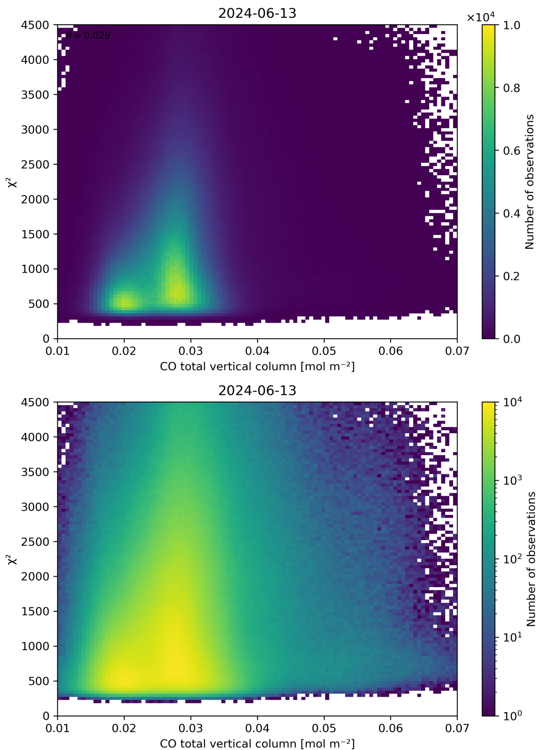
Figure 35: Scatter density plot of “CO total vertical column” against “ \chi^2 ” for 2024-06-13 to 2024-06-14.
