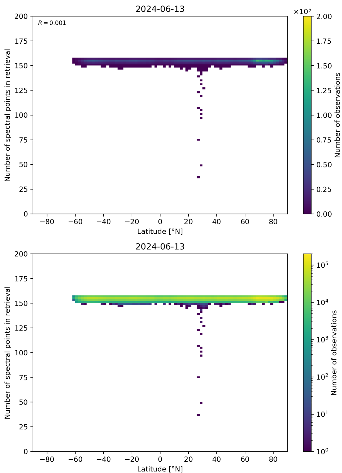
Figure 57: Scatter density plot of “Latitude” against “Number of spectral points in retrieval” for 2024-06-13 to 2024-06-14.
