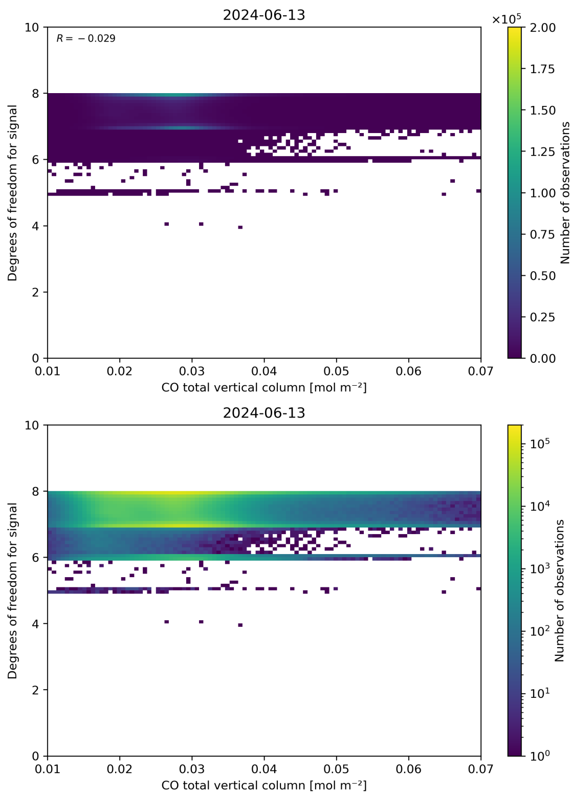
Figure 41: Scatter density plot of “CO total vertical column” against “Degrees of freedom for signal” for 2024-06-13 to 2024-06-14.
