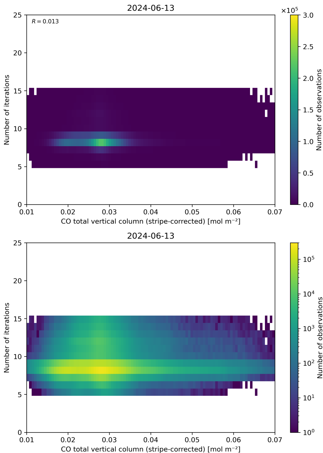
Figure 39: Scatter density plot of “CO total vertical column (stripe-corrected)” against “Number of iterations” for 2024-06-13 to 2024-06-14.
