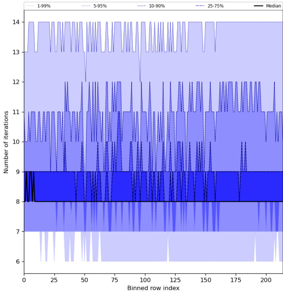
Figure 32: Along track statistics of “Number of iterations” for 2024-06-13 to 2024-06-14
