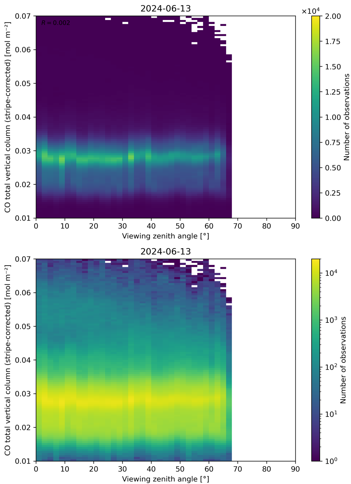
Figure 70: Scatter density plot of “Viewing zenith angle” against “CO total vertical column (stripe-corrected)” for 2024-06-13 to 2024-06-14.
