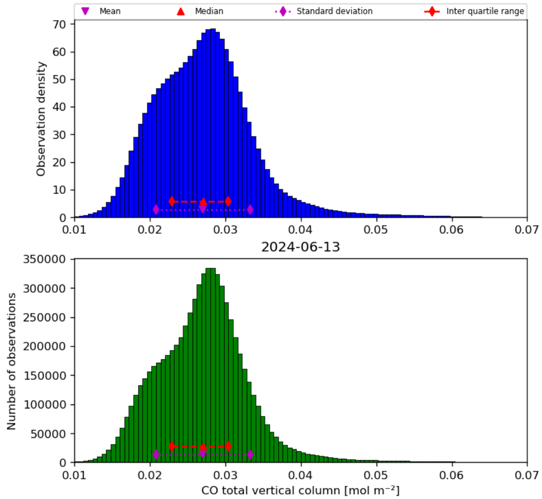
Figure 18: Histogram of “CO total vertical column” for 2024-06-13 to 2024-06-14
