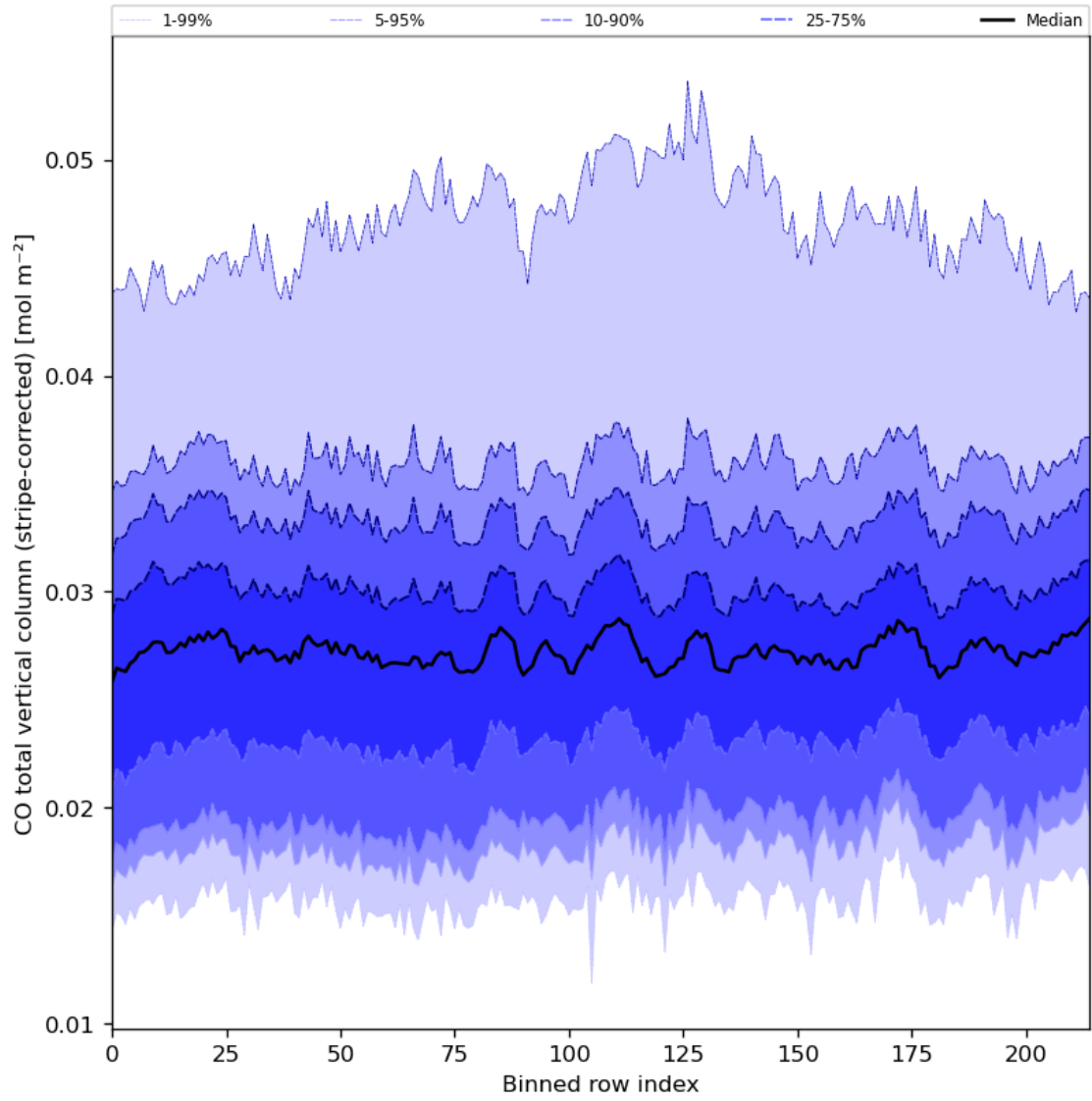
Figure 27: Along track statistics of “CO total vertical column (stripe-corrected)” for 2024-06-13 to 2024-06-14
