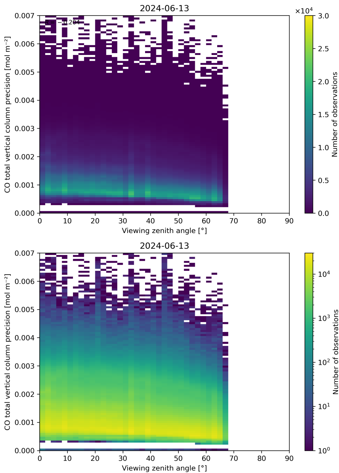
Figure 71: Scatter density plot of “Viewing zenith angle” against “CO total vertical column precision” for 2024-06-13 to 2024-06-14.
