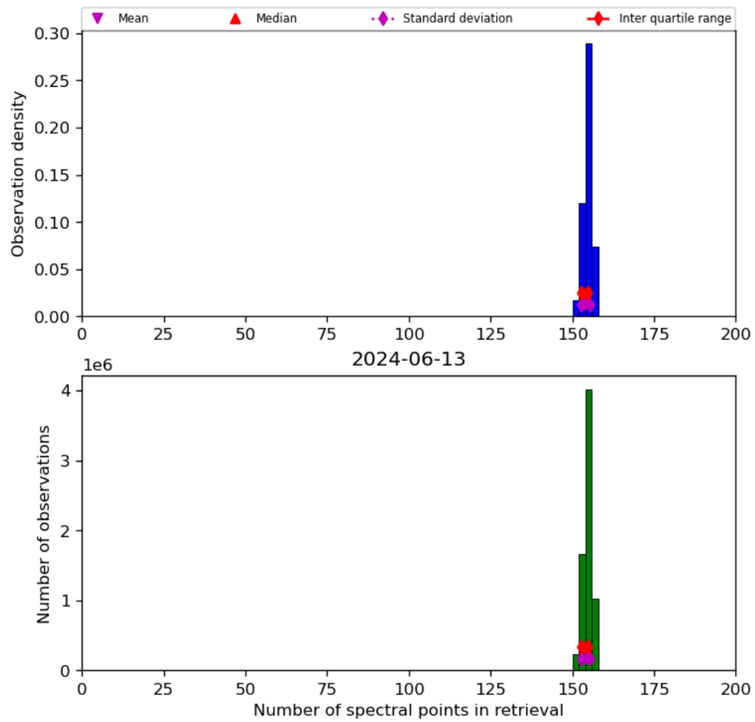
Figure 21: Histogram of “Number of spectral points in retrieval” for 2024-06-13 to 2024-06-14
