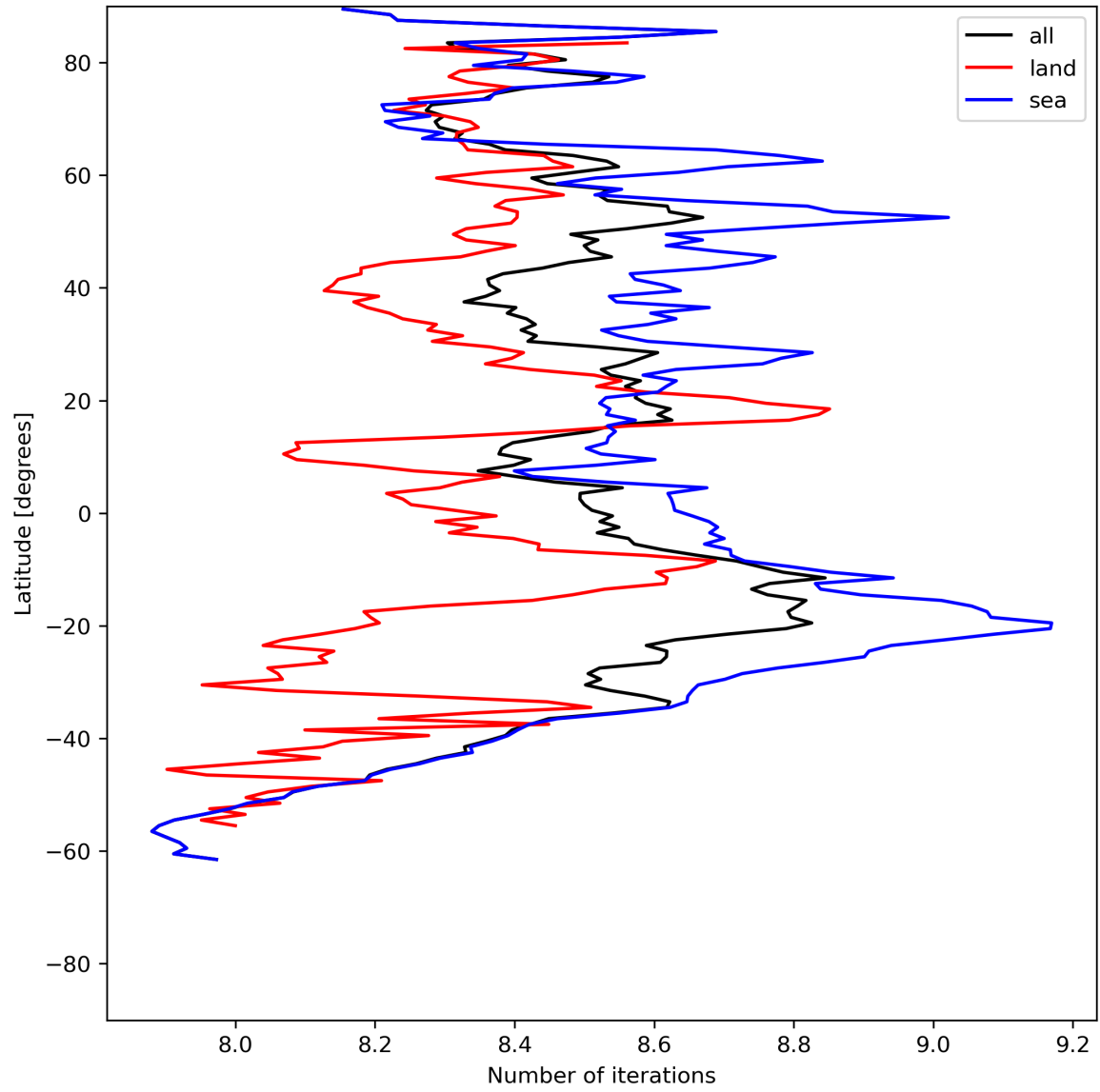
Figure 16: Zonal average of “Number of iterations” for 2024-06-13 to 2024-06-14.
