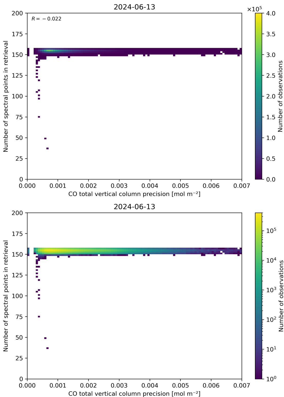
Figure 47: Scatter density plot of “CO total vertical column precision” against “Number of spectral points in retrieval” for 2024-06-13 to 2024-06-14.
