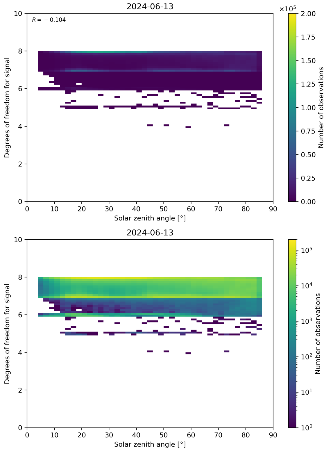
Figure 65: Scatter density plot of “Solar zenith angle” against “Degrees of freedom for signal” for 2024-06-13 to 2024-06-14.
