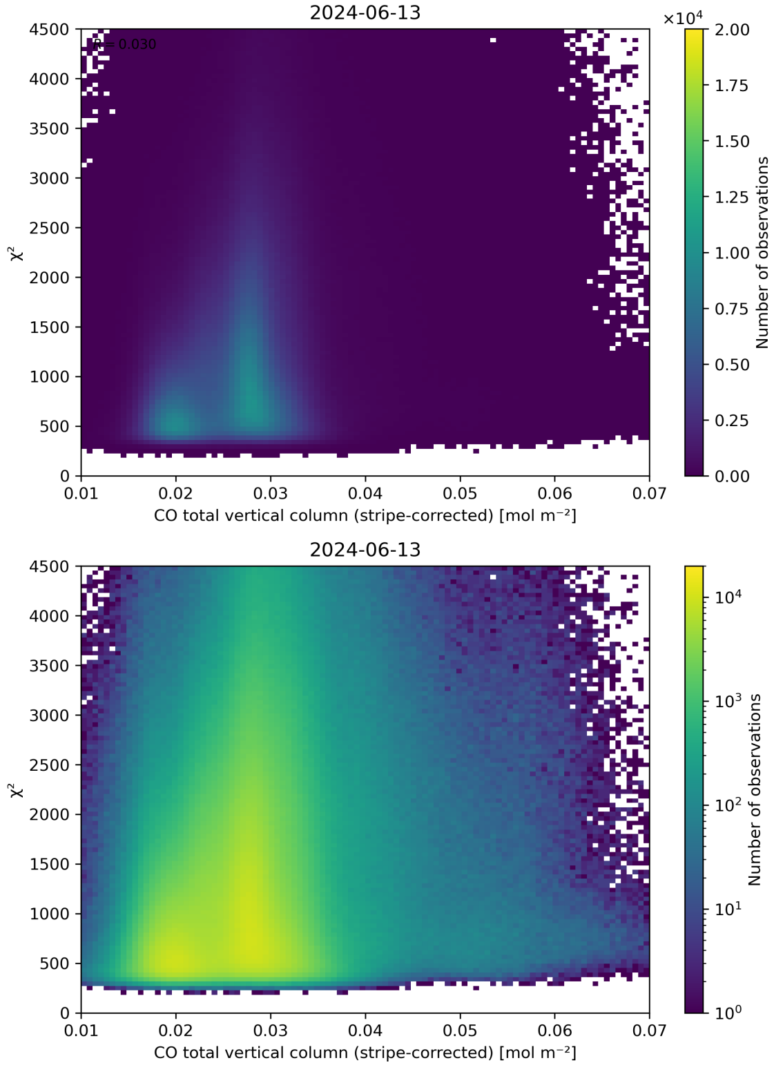
Figure 37: Scatter density plot of “CO total vertical column (stripe-corrected)” against “ \chi^2 ” for 2024-06-13 to 2024-06-14.
