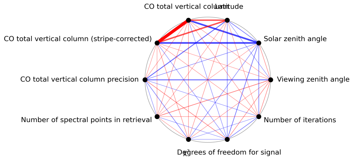
Figure 1: Map of correlation graph for 2024-06-13 to 2024-06-14.
