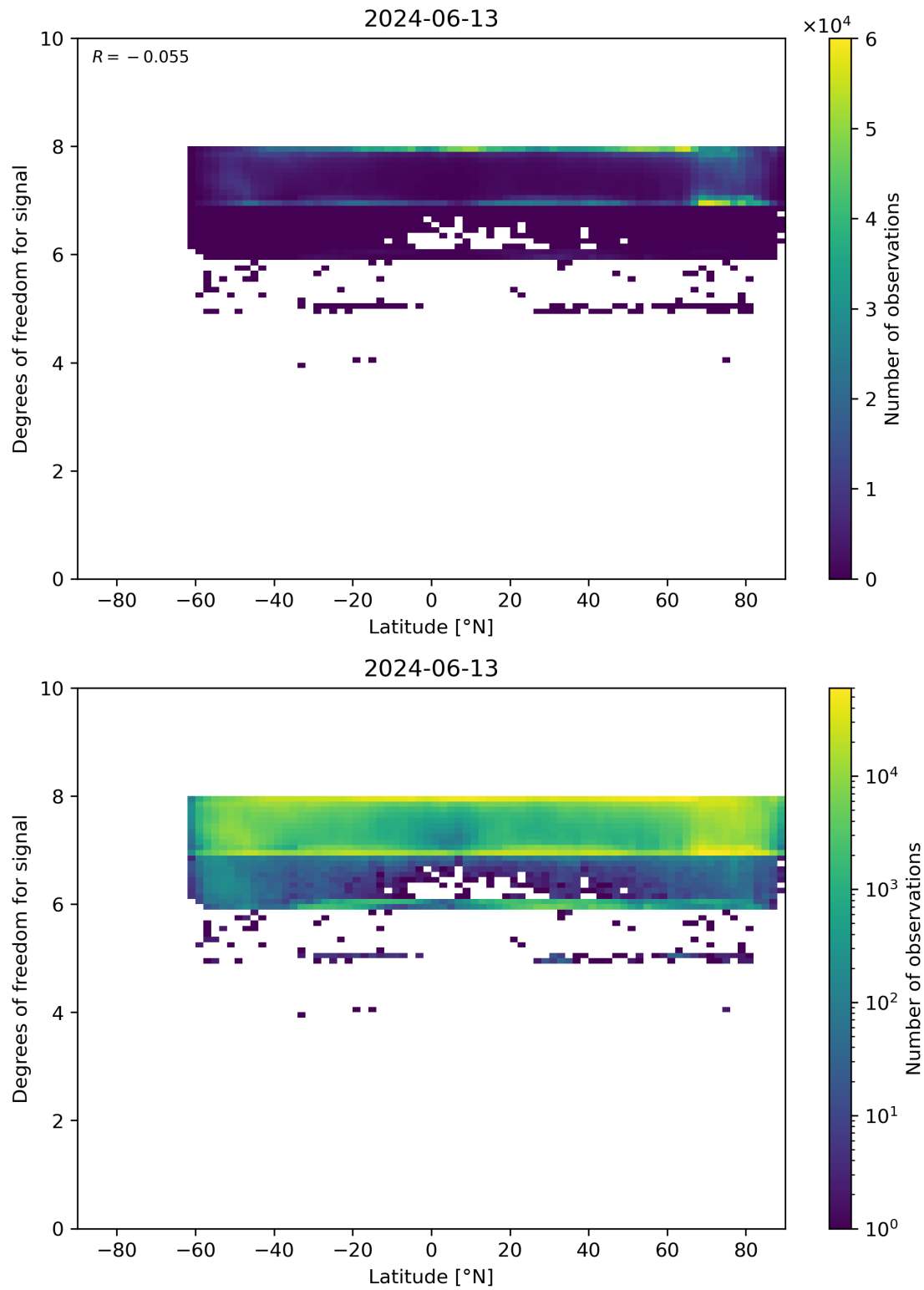
Figure 55: Scatter density plot of “Latitude” against “Degrees of freedom for signal” for 2024-06-13 to 2024-06-14.
