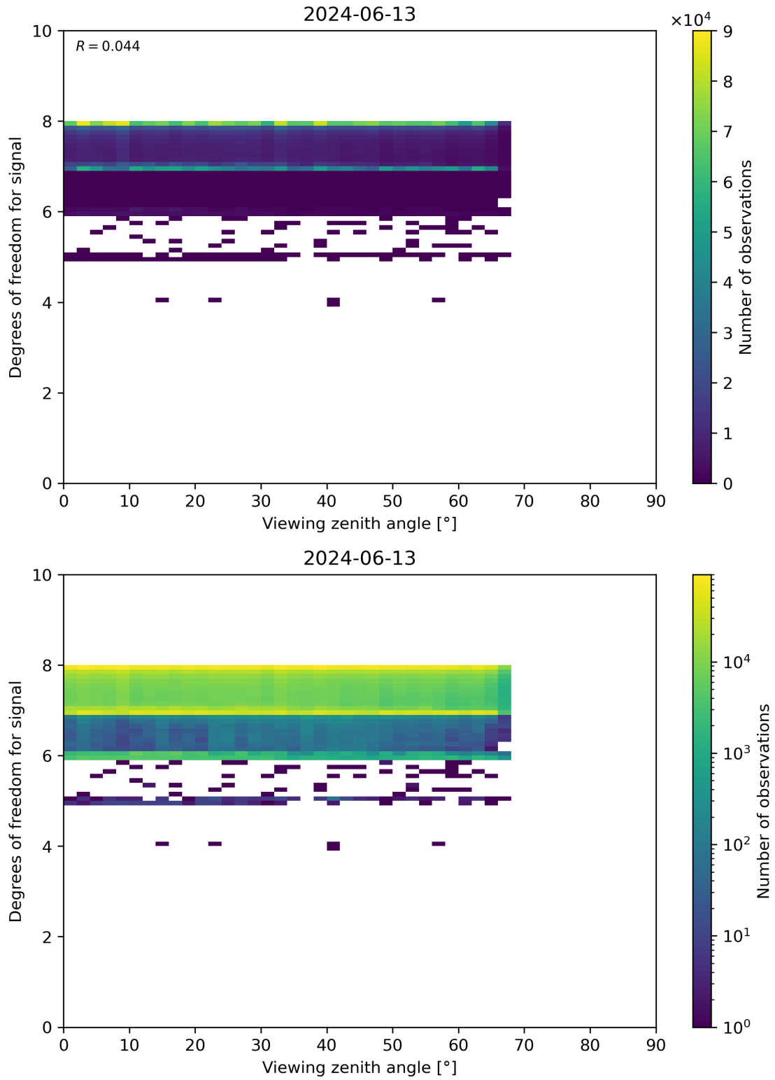
Figure 73: Scatter density plot of “Viewing zenith angle” against “Degrees of freedom for signal” for 2024-06-13 to 2024-06-14.
