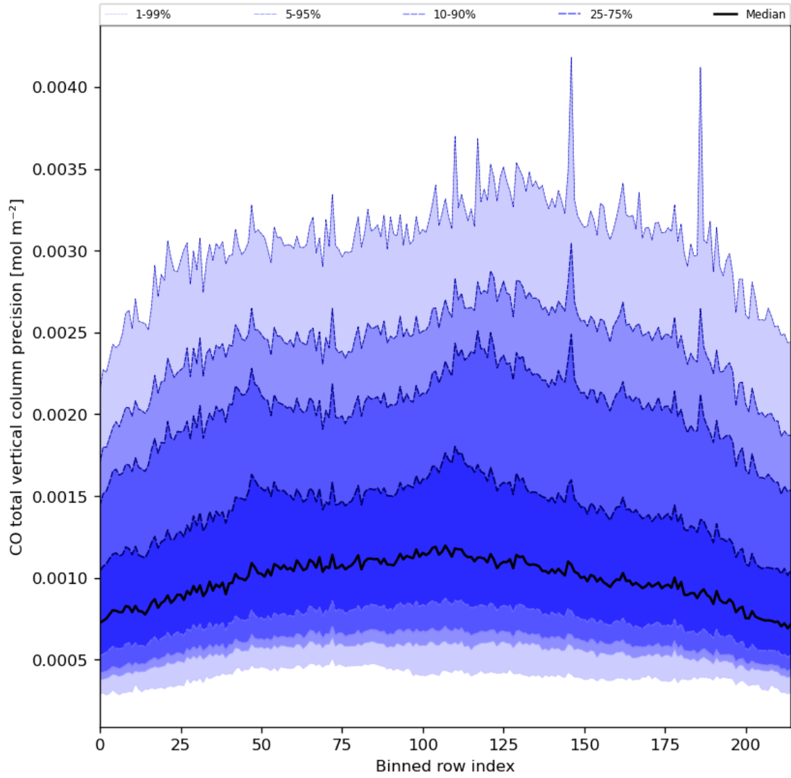
Figure 28: Along track statistics of “CO total vertical column precision” for 2024-06-13 to 2024-06-14
