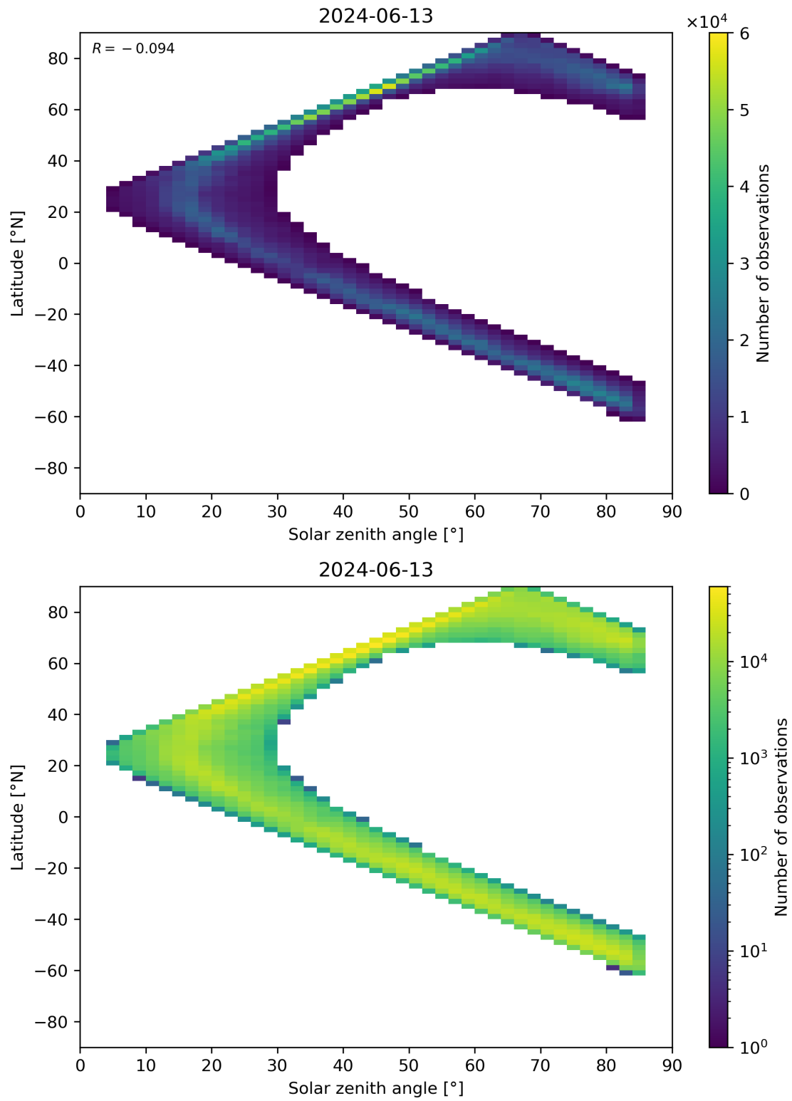
Figure 66: Scatter density plot of “Solar zenith angle” against “Latitude” for 2024-06-13 to 2024-06-14.
