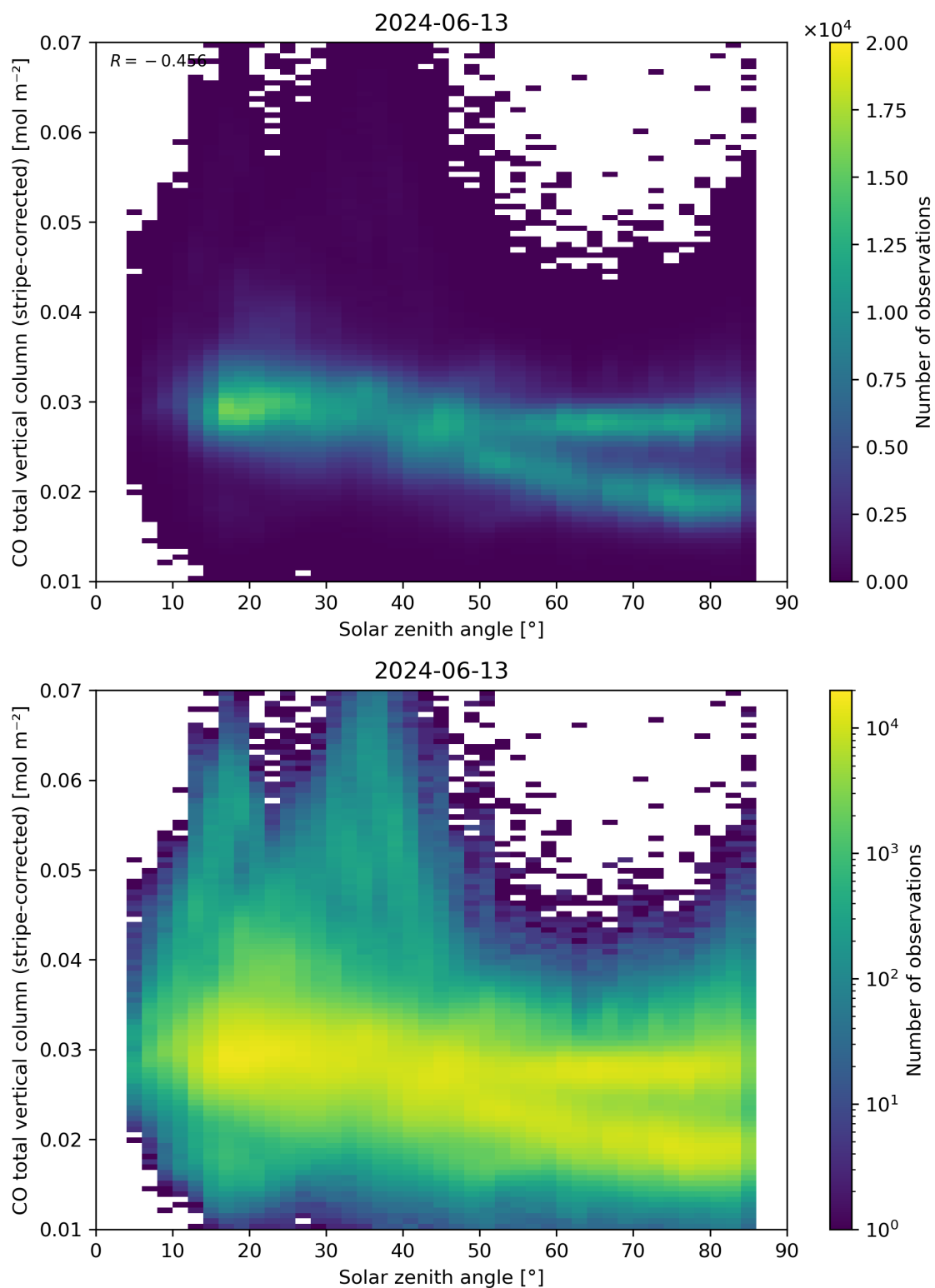
Figure 62: Scatter density plot of “Solar zenith angle” against “CO total vertical column (stripe-corrected)” for 2024-06-13 to 2024-06-14.
