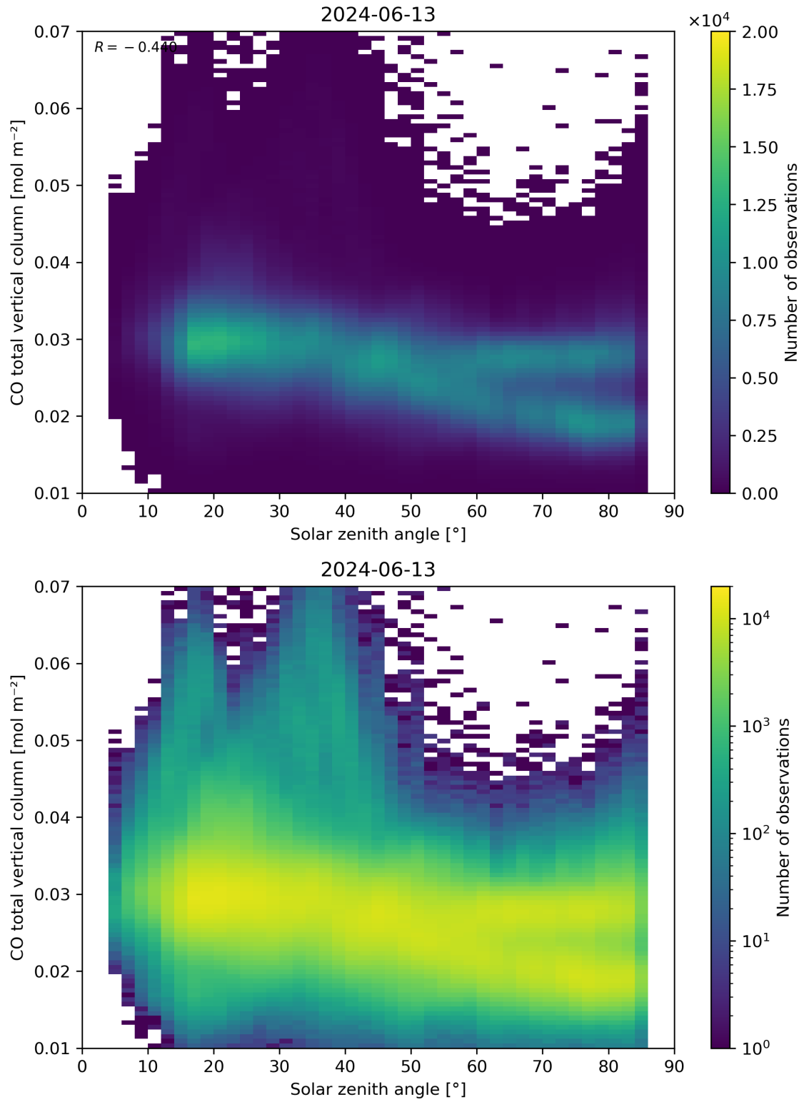
Figure 61: Scatter density plot of “Solar zenith angle” against “CO total vertical column” for 2024-06-13 to 2024-06-14.
