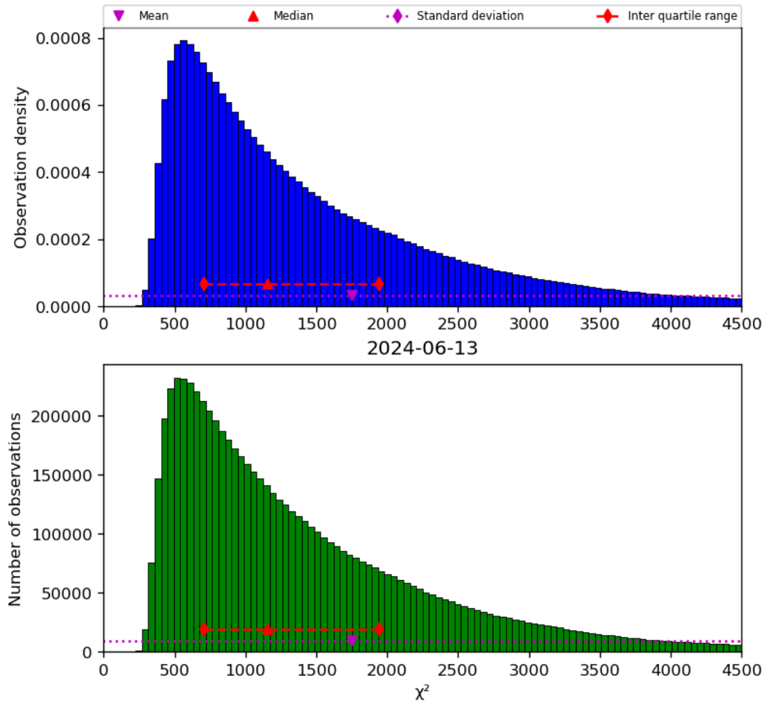
Figure 22: Histogram of “ \chi^2 ” for 2024-06-13 to 2024-06-14
