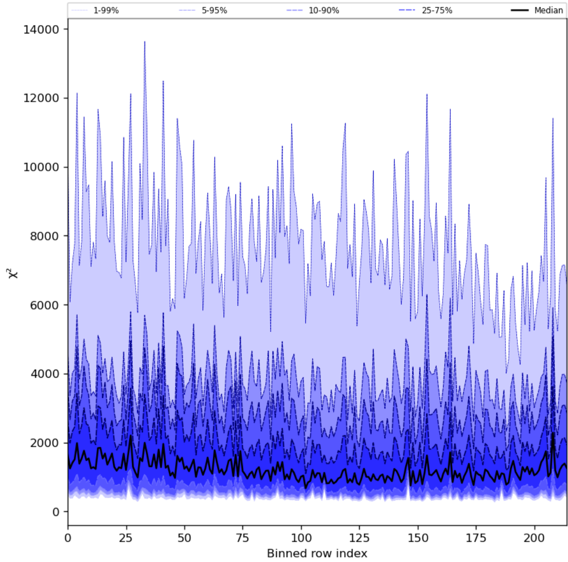
Figure 30: Along track statistics of “ \chi^2 ” for 2024-06-13 to 2024-06-14
