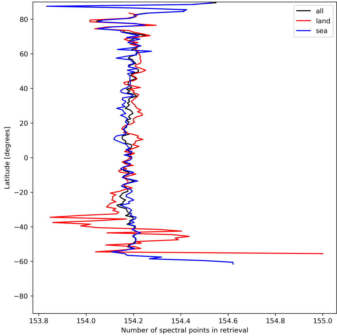
Figure 13: Zonal average of “Number of spectral points in retrieval” for 2024-06-13 to 2024-06-14.
