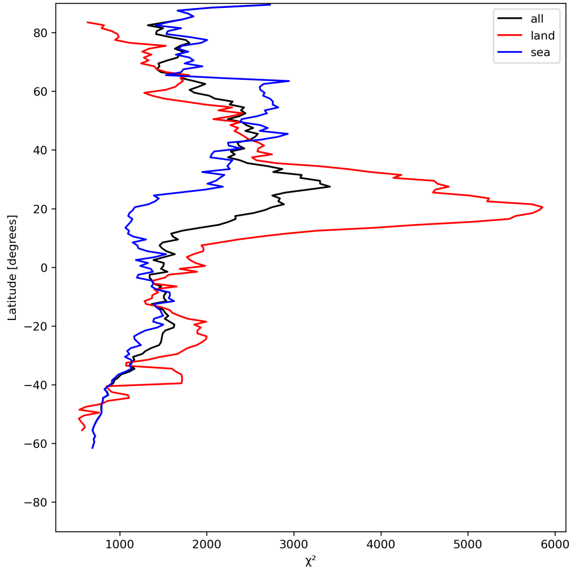
Figure 14: Zonal average of “ \chi^2 ” for 2024-06-13 to 2024-06-14.
