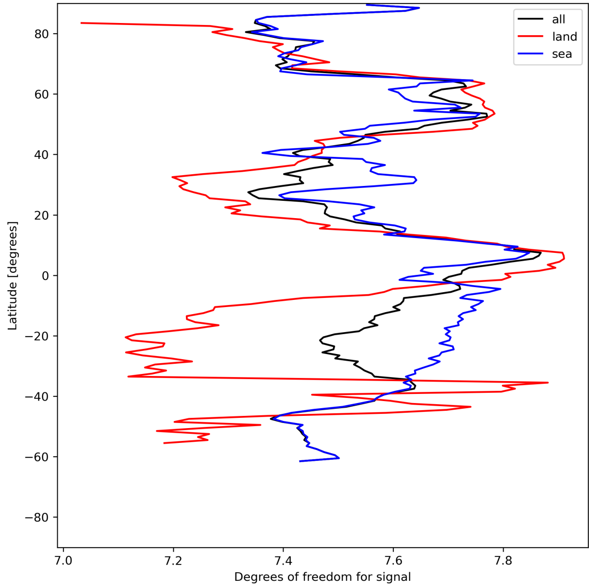
Figure 15: Zonal average of “Degrees of freedom for signal” for 2024-06-13 to 2024-06-14.
