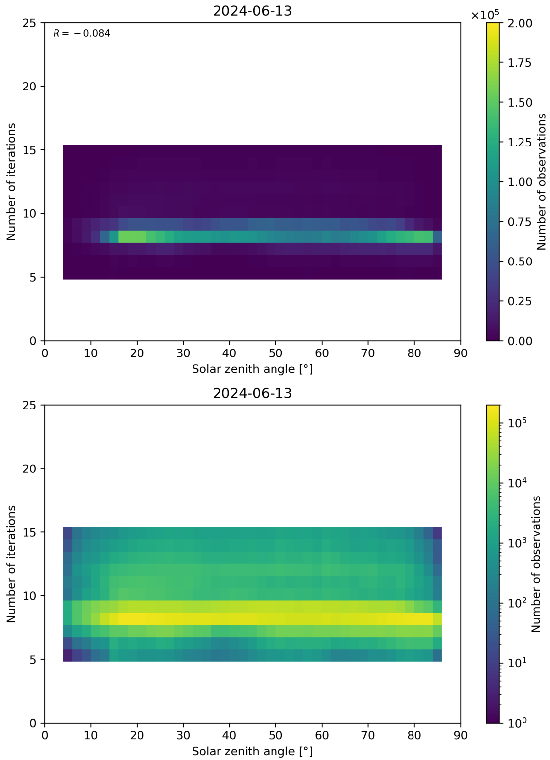
Figure 67: Scatter density plot of “Solar zenith angle” against “Number of iterations” for 2024-06-13 to 2024-06-14.
