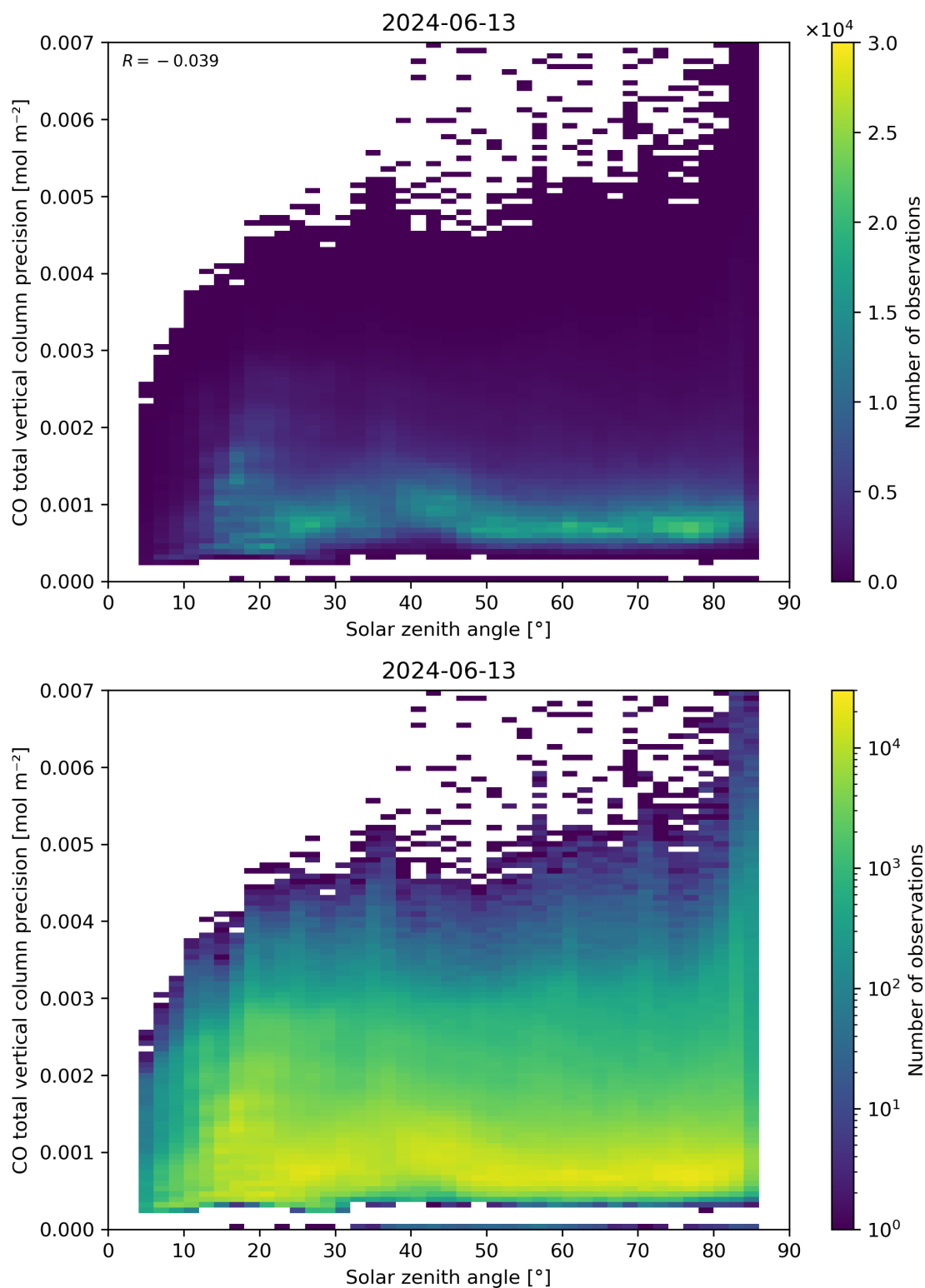
Figure 63: Scatter density plot of “Solar zenith angle” against “CO total vertical column precision” for 2024-06-13 to 2024-06-14.
