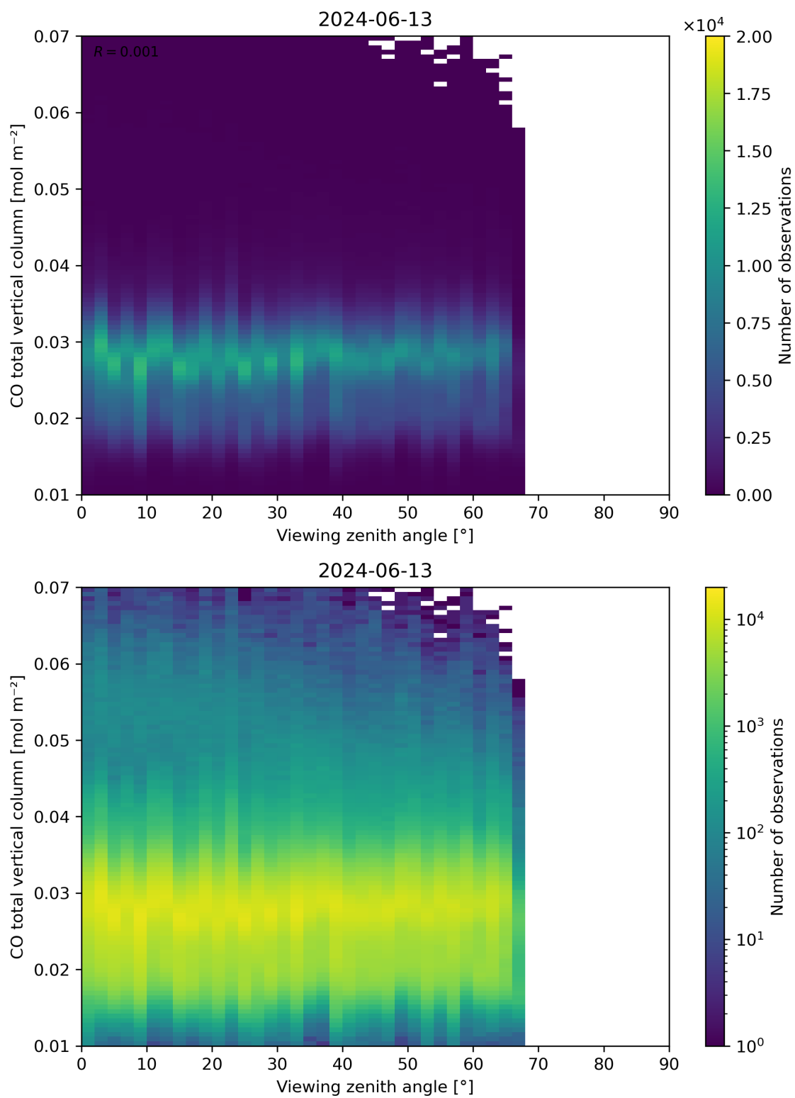
Figure 69: Scatter density plot of “Viewing zenith angle” against “CO total vertical column” for 2024-06-13 to 2024-06-14.
