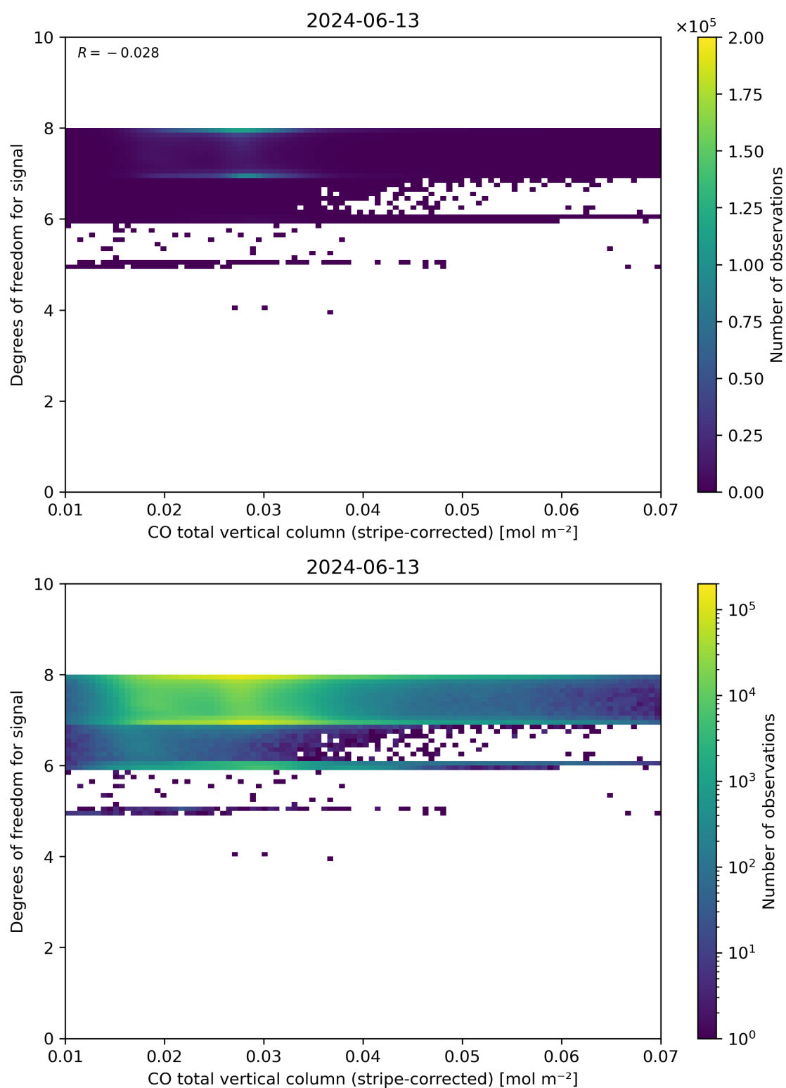
Figure 38: Scatter density plot of “CO total vertical column (stripe-corrected)” against “Degrees of freedom for signal” for 2024-06-13 to 2024-06-14.
