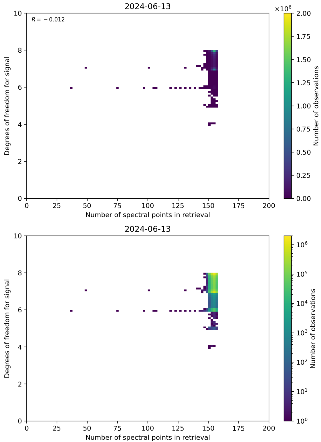
Figure 59: Scatter density plot of “Number of spectral points in retrieval” against “Degrees of freedom for signal” for 2024-06-13 to 2024-06-14.
