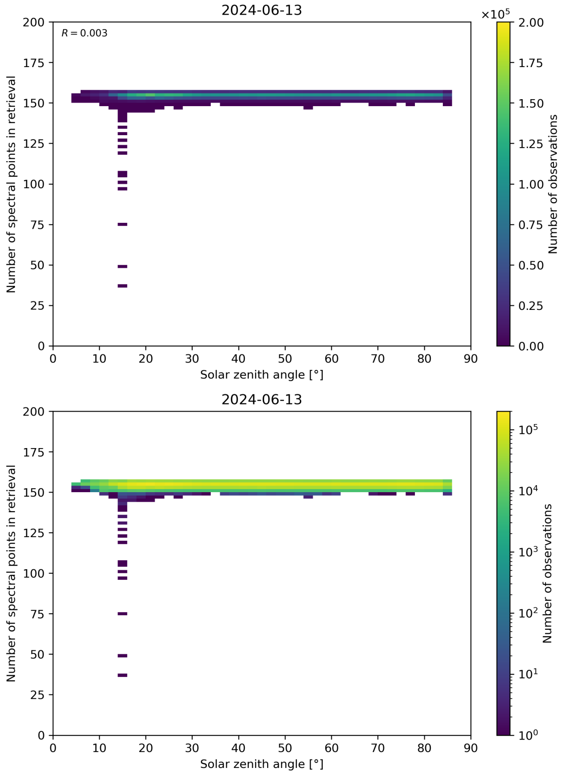
Figure 68: Scatter density plot of “Solar zenith angle” against “Number of spectral points in retrieval” for 2024-06-13 to 2024-06-14.
