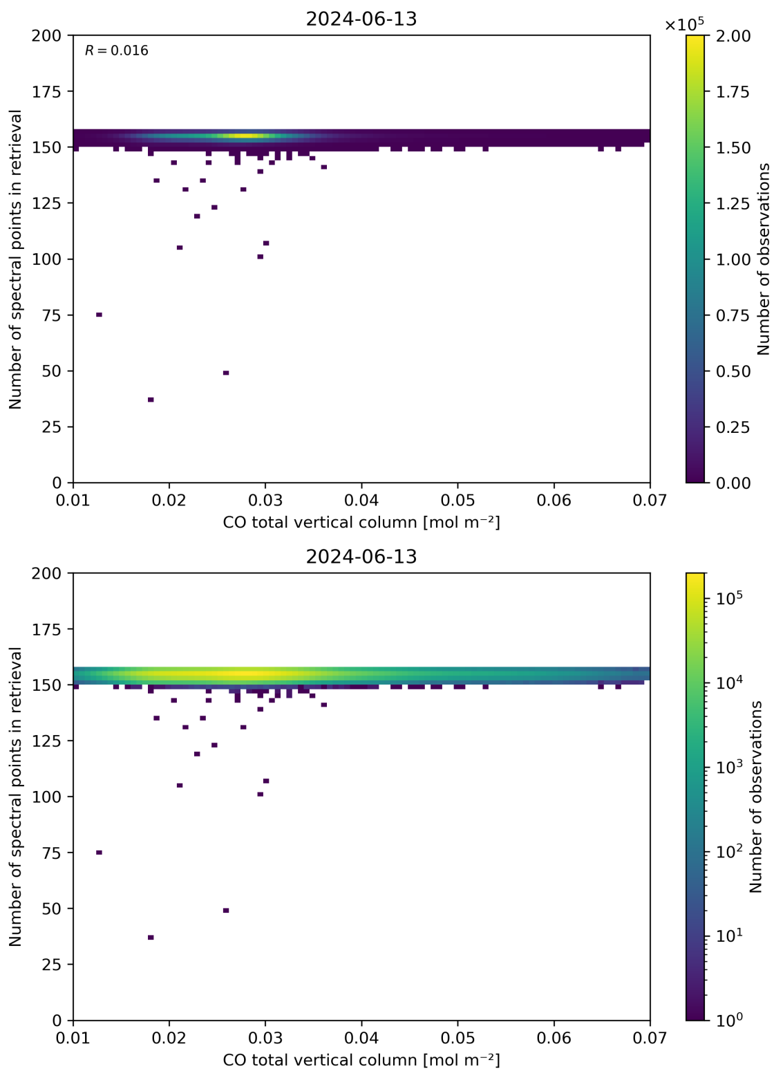
Figure 43: Scatter density plot of “CO total vertical column” against “Number of spectral points in retrieval” for 2024-06-13 to 2024-06-14.
