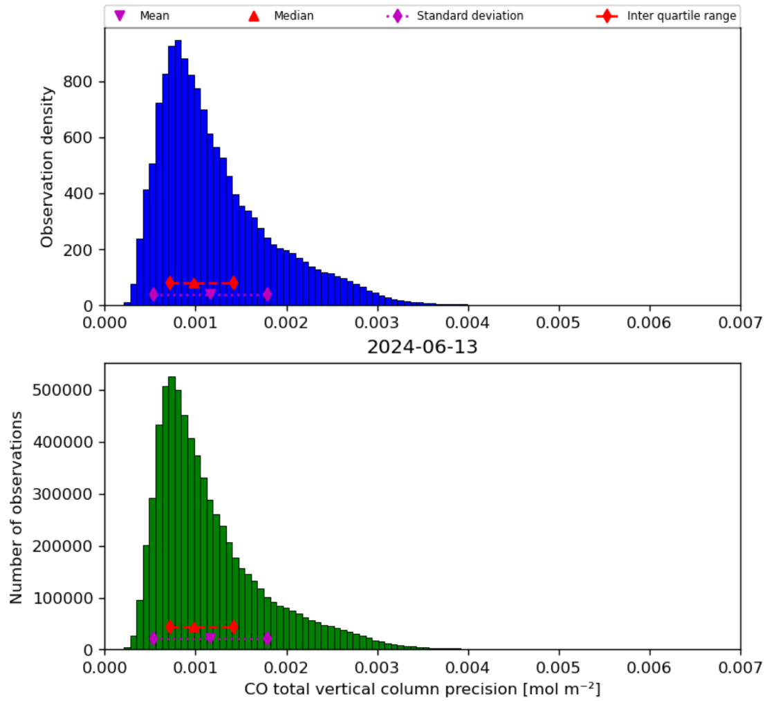
Figure 20: Histogram of “CO total vertical column precision” for 2024-06-13 to 2024-06-14
