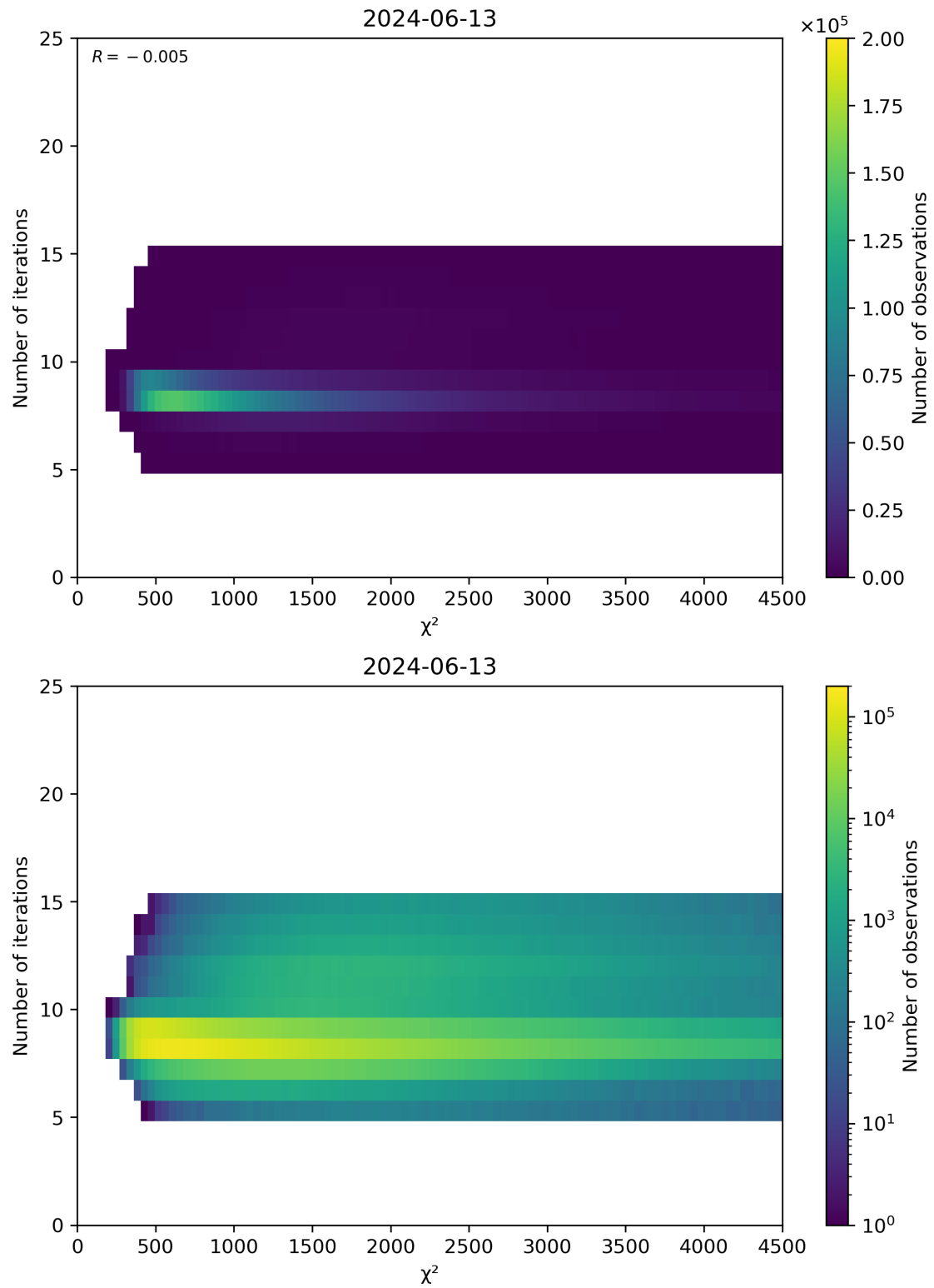
Figure 49: Scatter density plot of “ \chi^2 ” against “Number of iterations” for 2024-06-13 to 2024-06-14.
