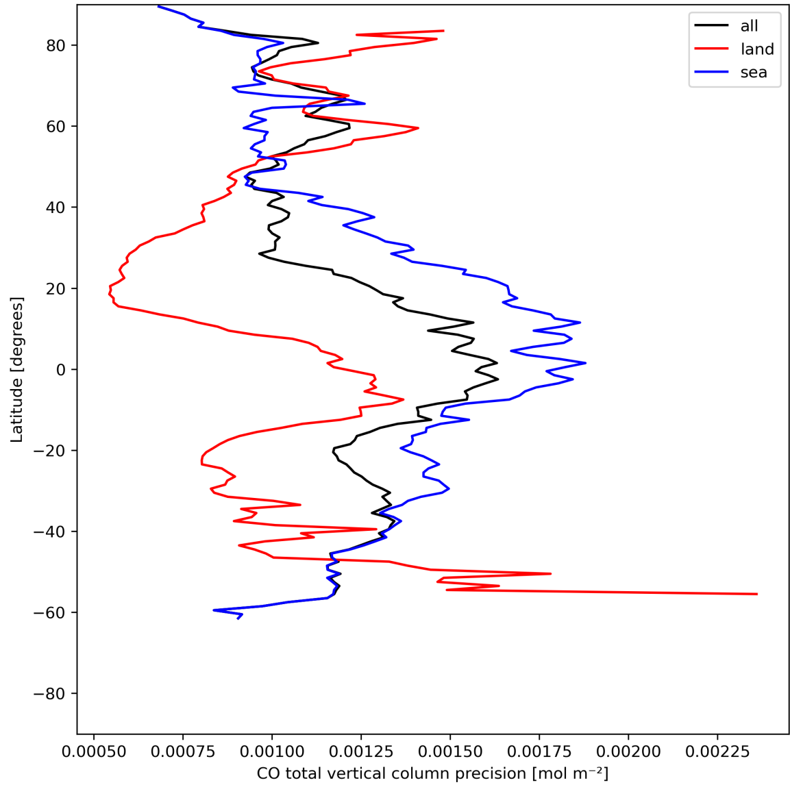
Figure 12: Zonal average of “CO total vertical column precision” for 2024-06-13 to 2024-06-14.
