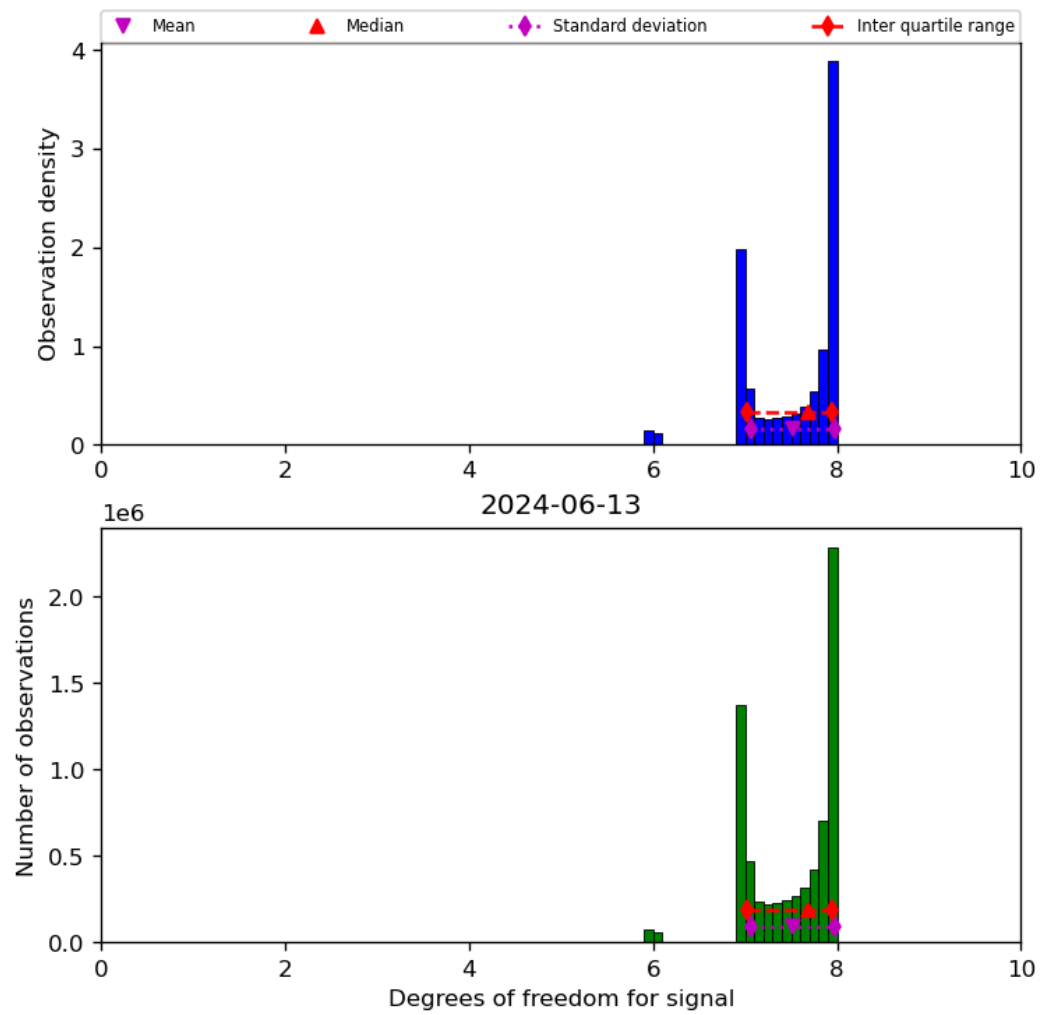
Figure 23: Histogram of “Degrees of freedom for signal” for 2024-06-13 to 2024-06-14
