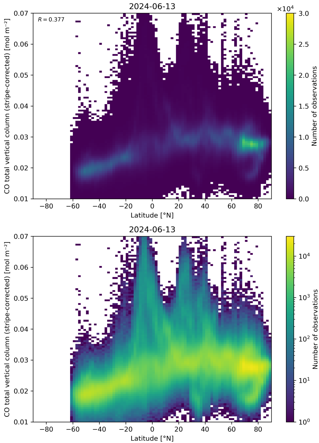
Figure 52: Scatter density plot of “Latitude” against “CO total vertical column (stripe-corrected)” for 2024-06-13 to 2024-06-14.
