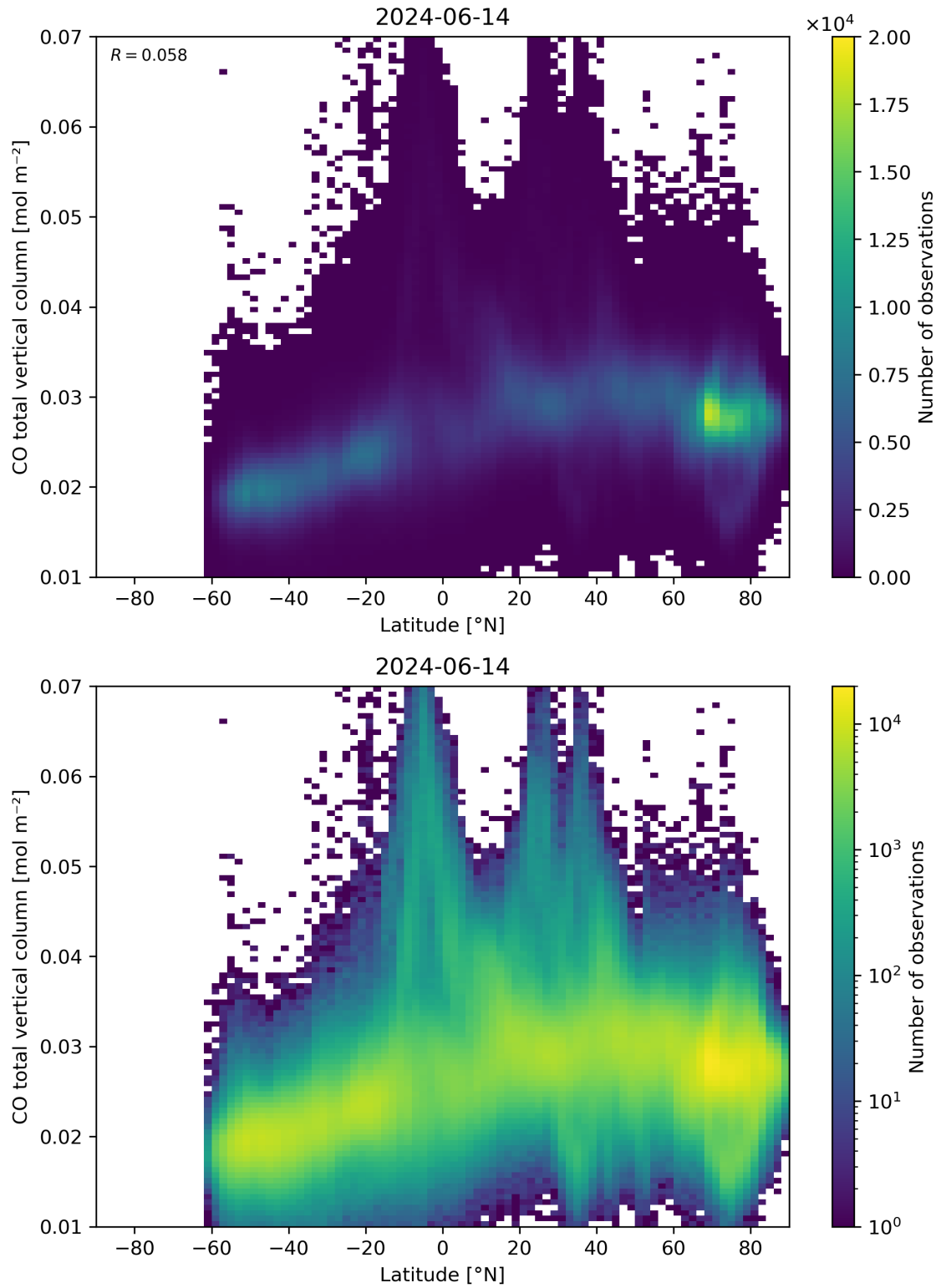
Figure 51: Scatter density plot of “Latitude” against “CO total vertical column” for 2024-06-13 to 2024-06-15.
