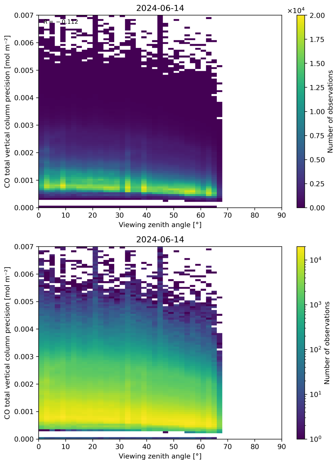
Figure 71: Scatter density plot of “Viewing zenith angle” against “CO total vertical column precision” for 2024-06-13 to 2024-06-15.
