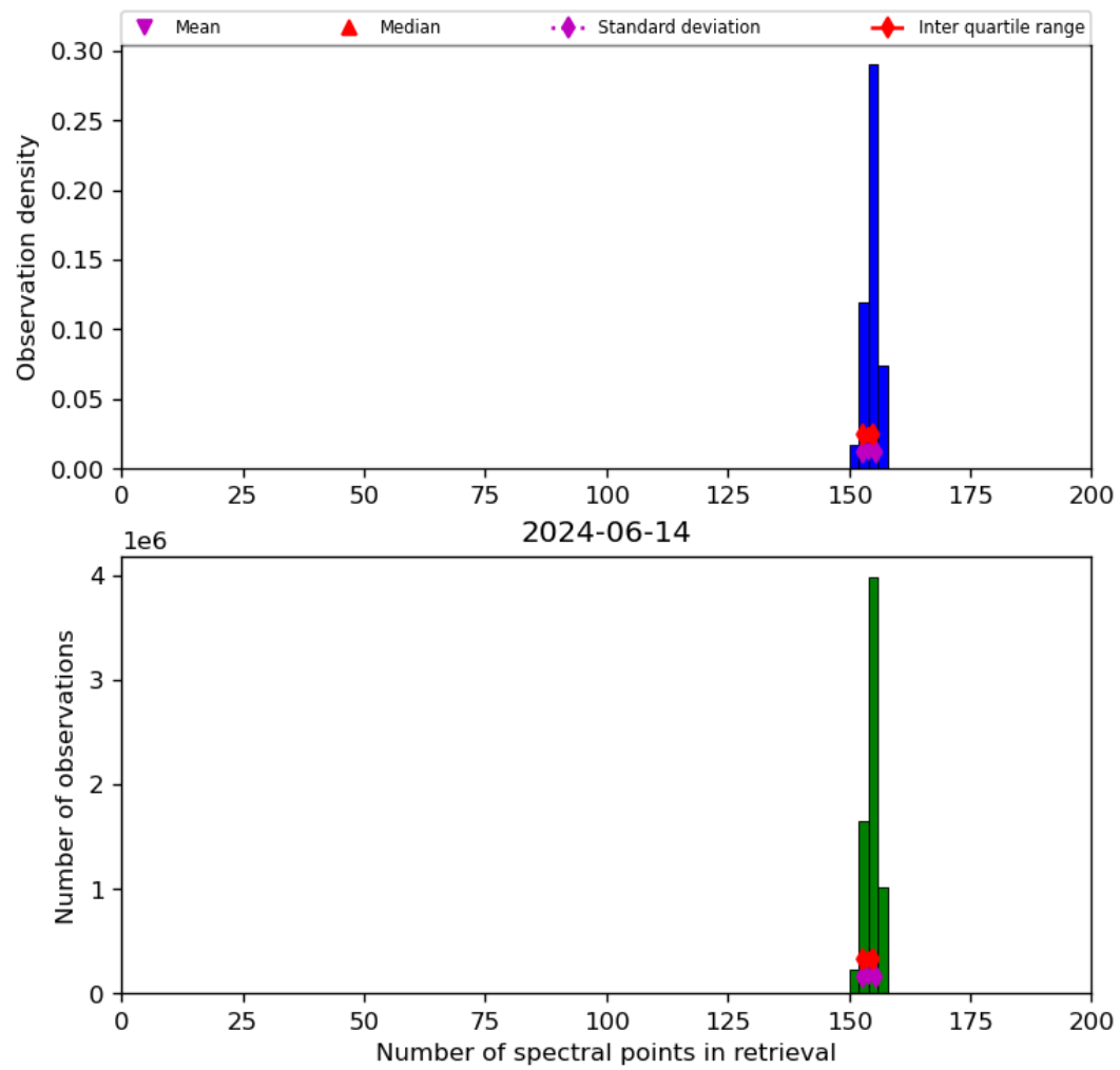
Figure 21: Histogram of “Number of spectral points in retrieval” for 2024-06-13 to 2024-06-15
