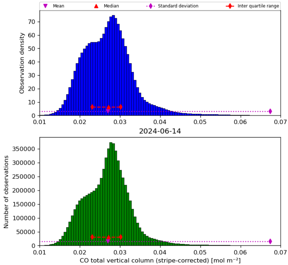
Figure 19: Histogram of “CO total vertical column (stripe-corrected)” for 2024-06-13 to 2024-06-15
