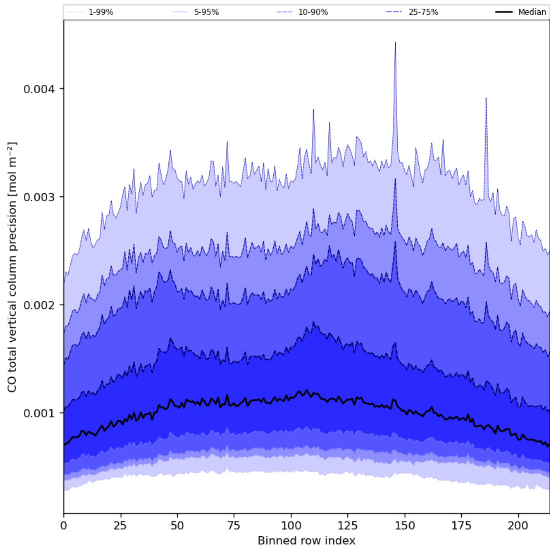
Figure 28: Along track statistics of “CO total vertical column precision” for 2024-06-13 to 2024-06-15
