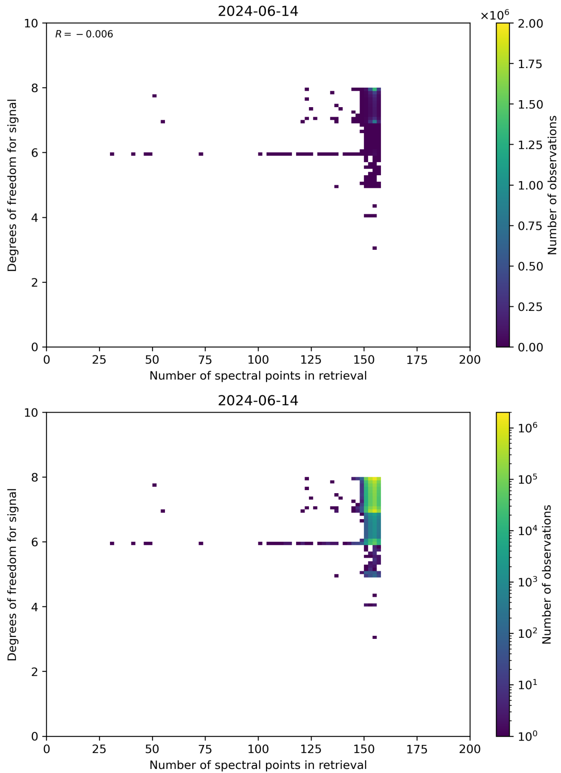
Figure 59: Scatter density plot of “Number of spectral points in retrieval” against “Degrees of freedom for signal” for 2024-06-13 to 2024-06-15.
