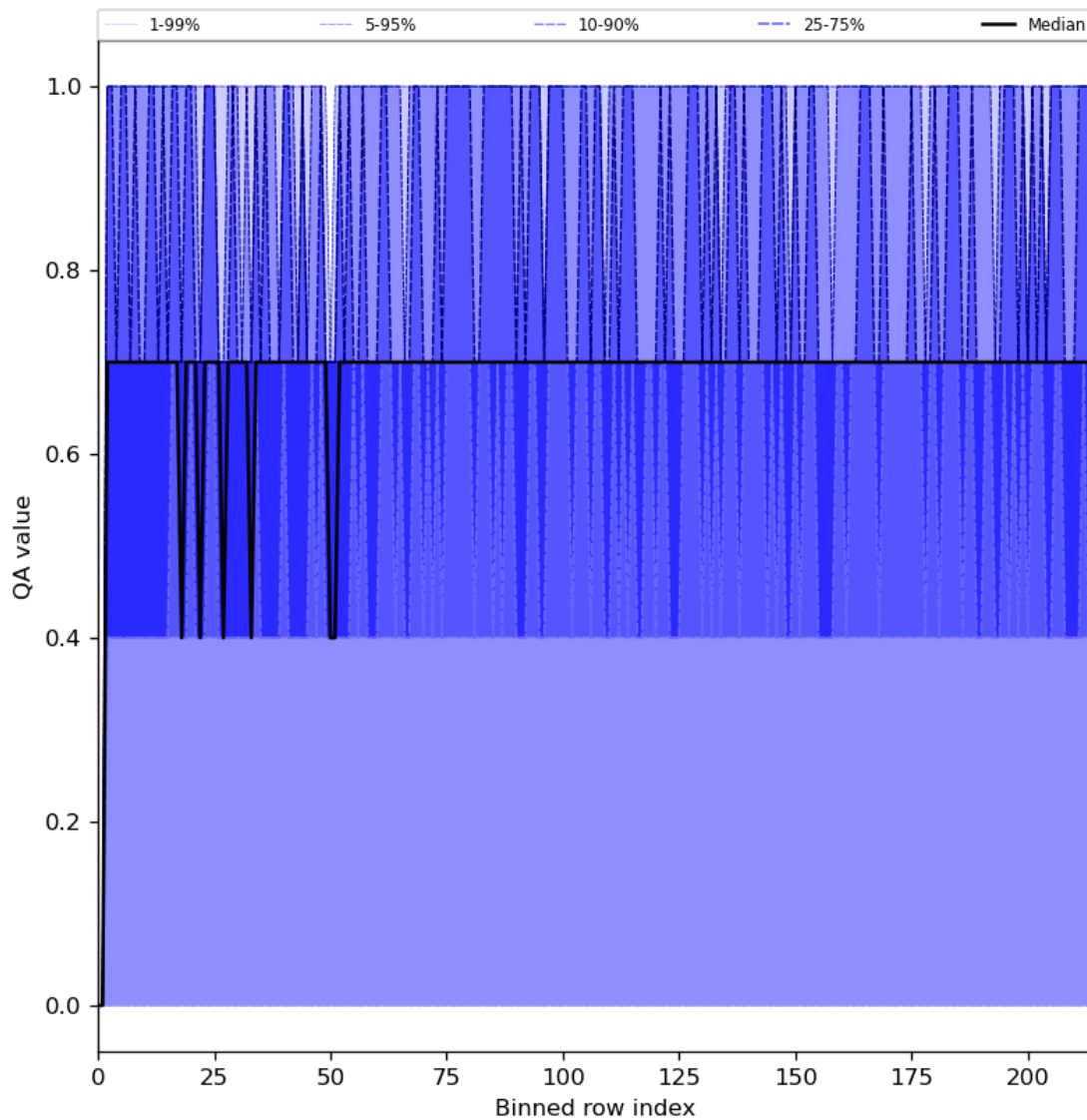
Figure 25: Along track statistics of “QA value” for 2024-06-13 to 2024-06-15
