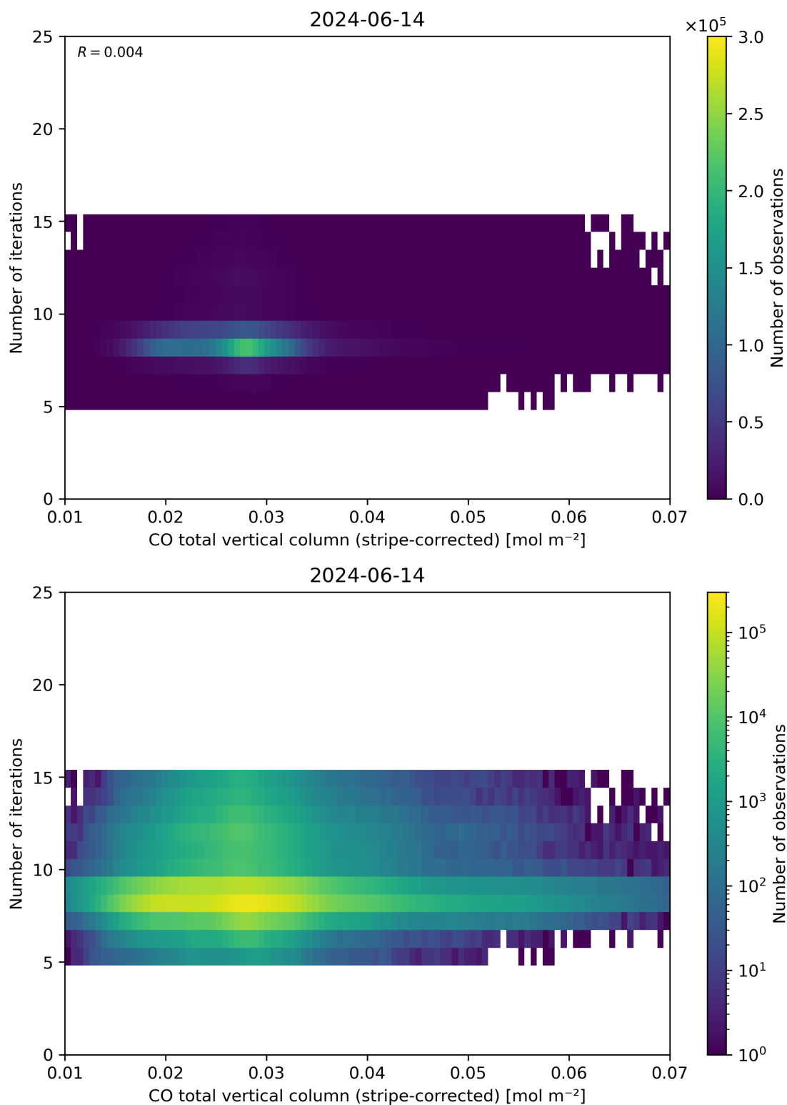
Figure 39: Scatter density plot of “CO total vertical column (stripe-corrected)” against “Number of iterations” for 2024-06-13 to 2024-06-15.
