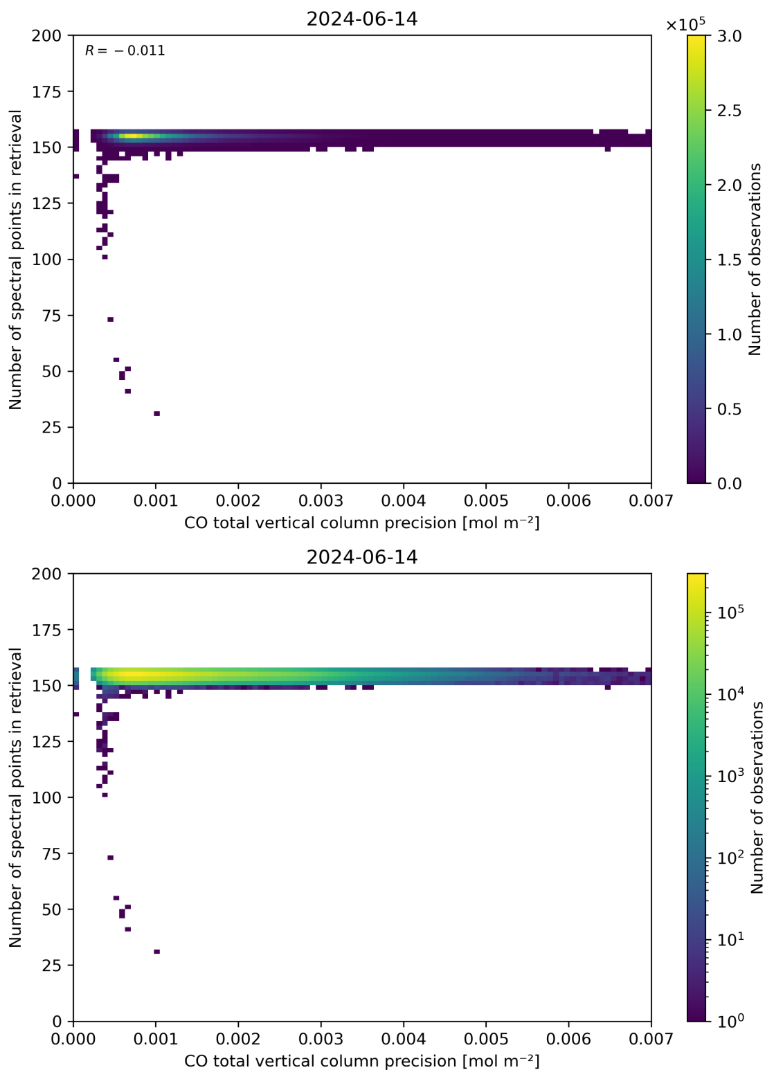
Figure 47: Scatter density plot of “CO total vertical column precision” against “Number of spectral points in retrieval” for 2024-06-13 to 2024-06-15.
