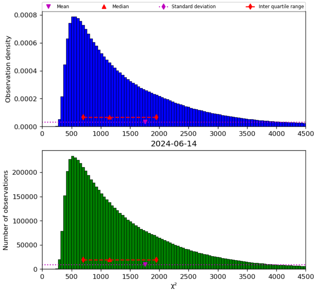
Figure 22: Histogram of “ \chi^2 ” for 2024-06-13 to 2024-06-15
