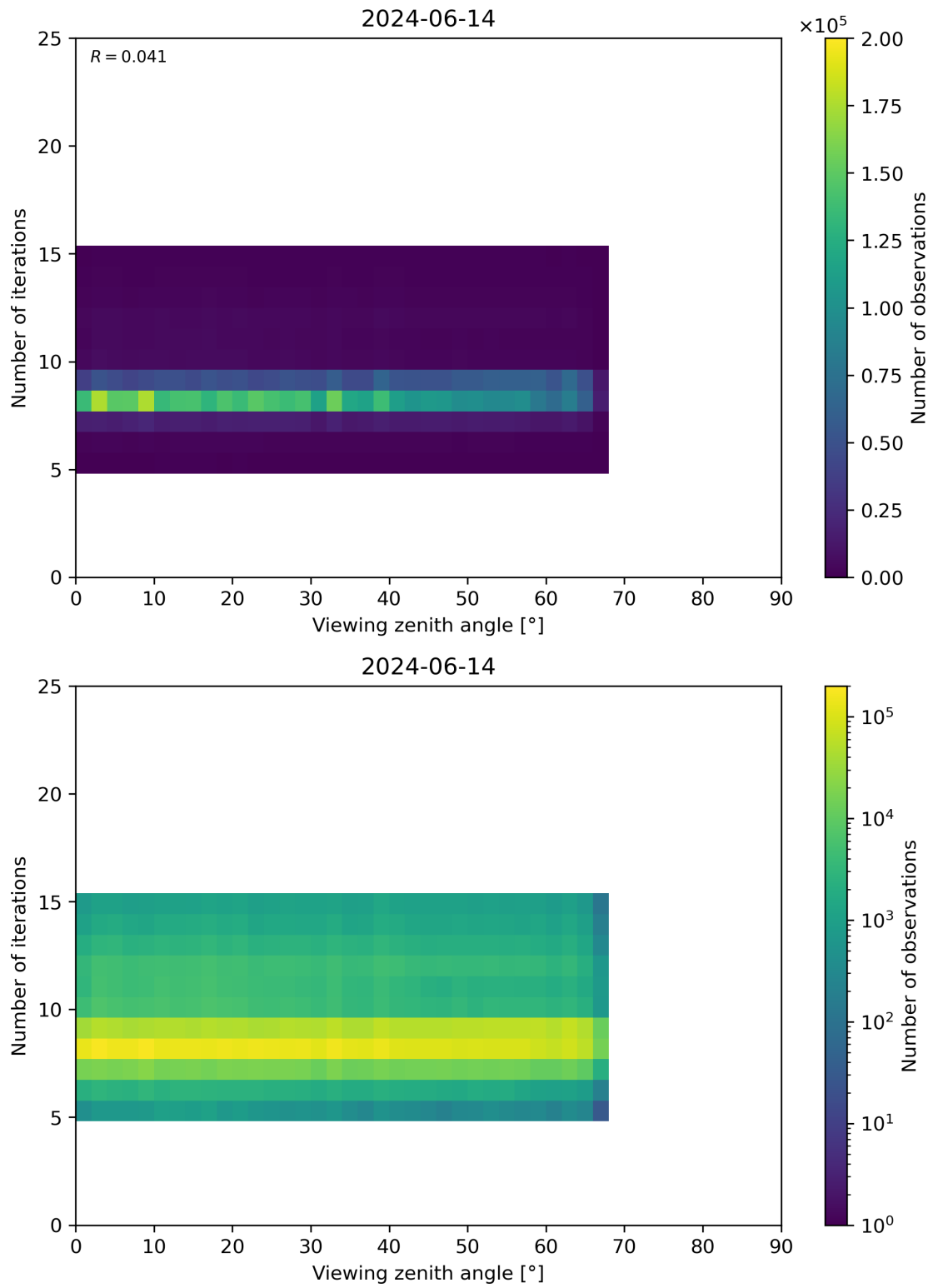
Figure 75: Scatter density plot of “Viewing zenith angle” against “Number of iterations” for 2024-06-13 to 2024-06-15.
