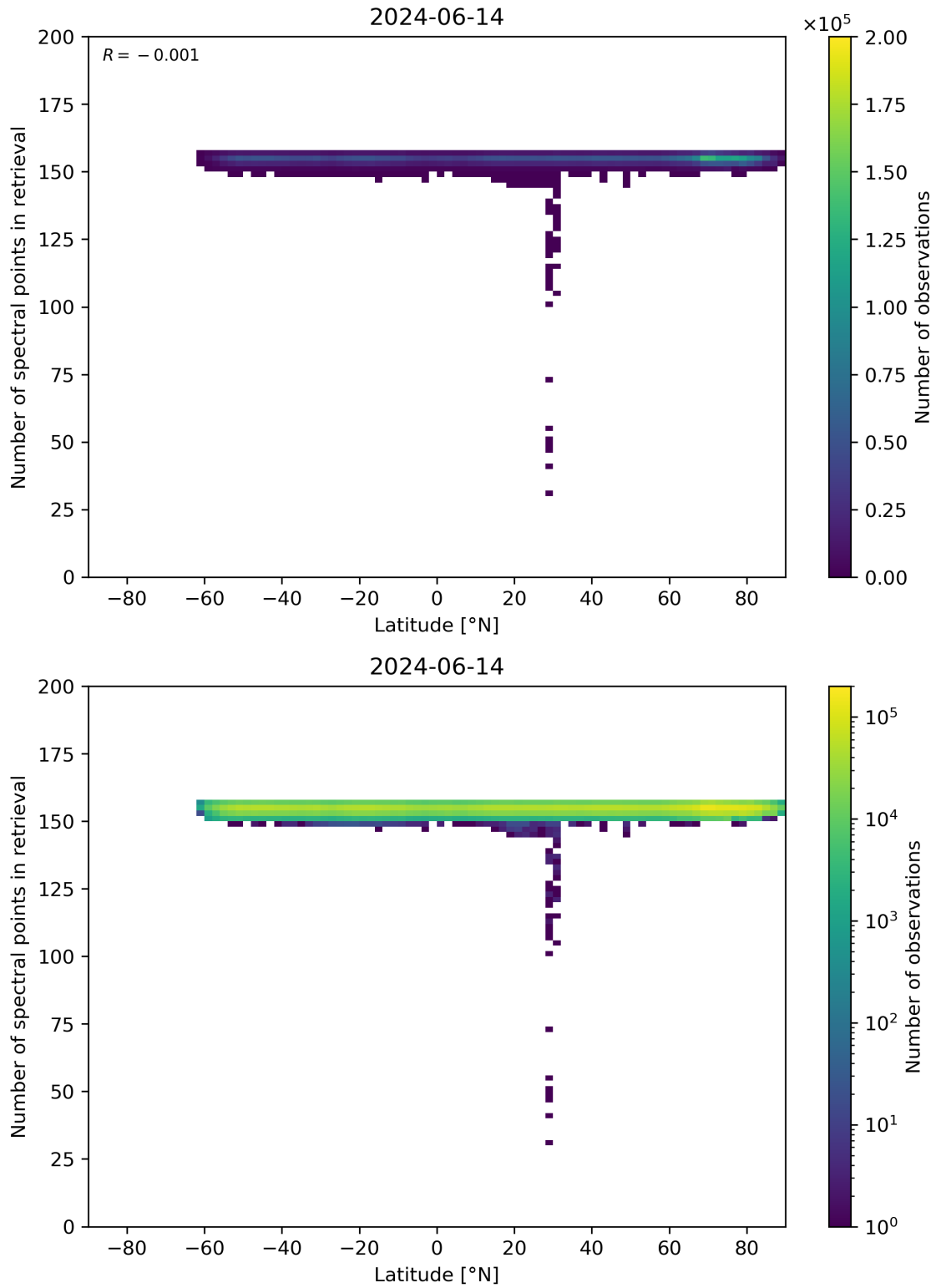
Figure 57: Scatter density plot of “Latitude” against “Number of spectral points in retrieval” for 2024-06-13 to 2024-06-15.
