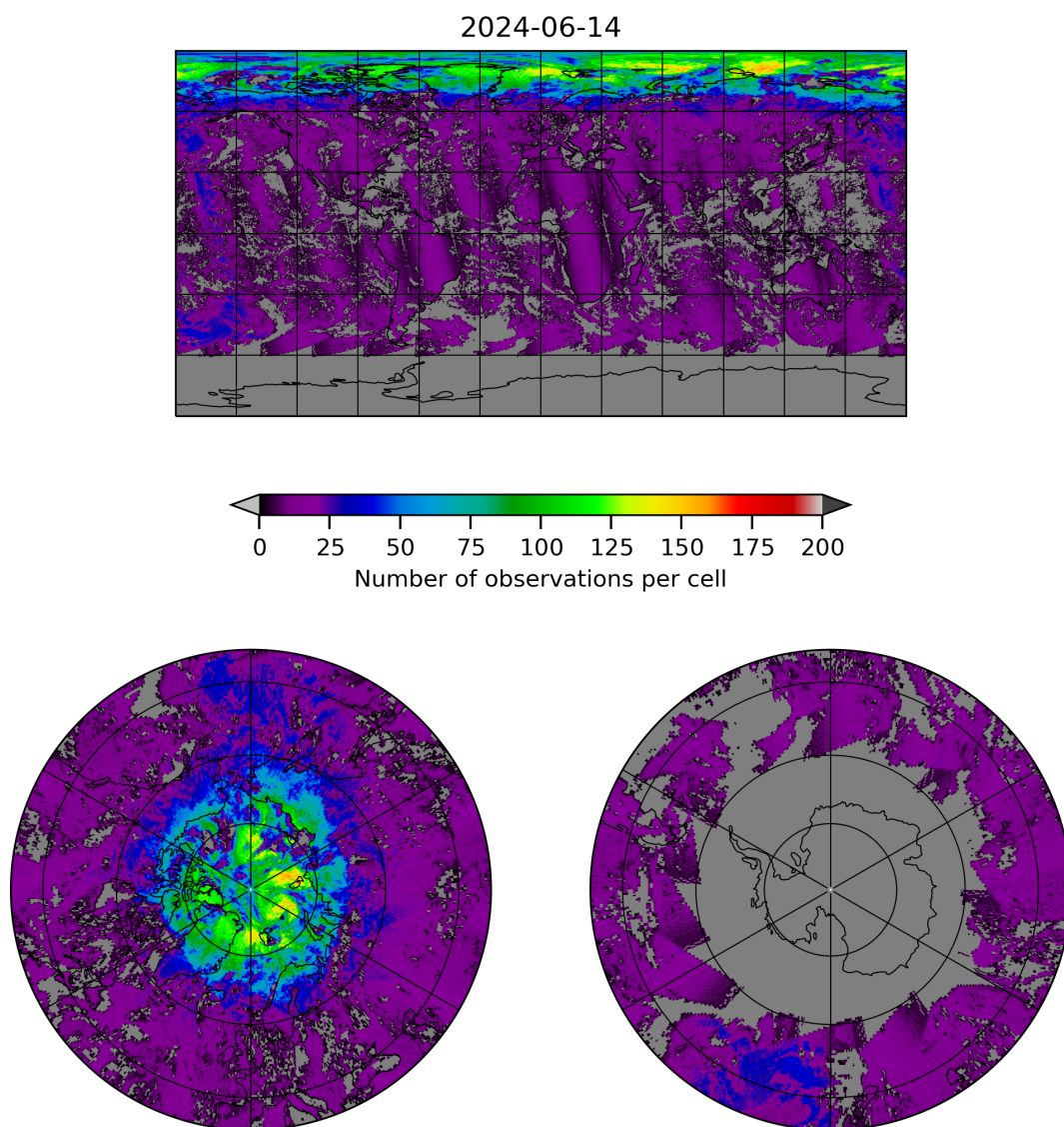
Figure 8: Map of the number of observations for 2024-06-13 to 2024-06-15
