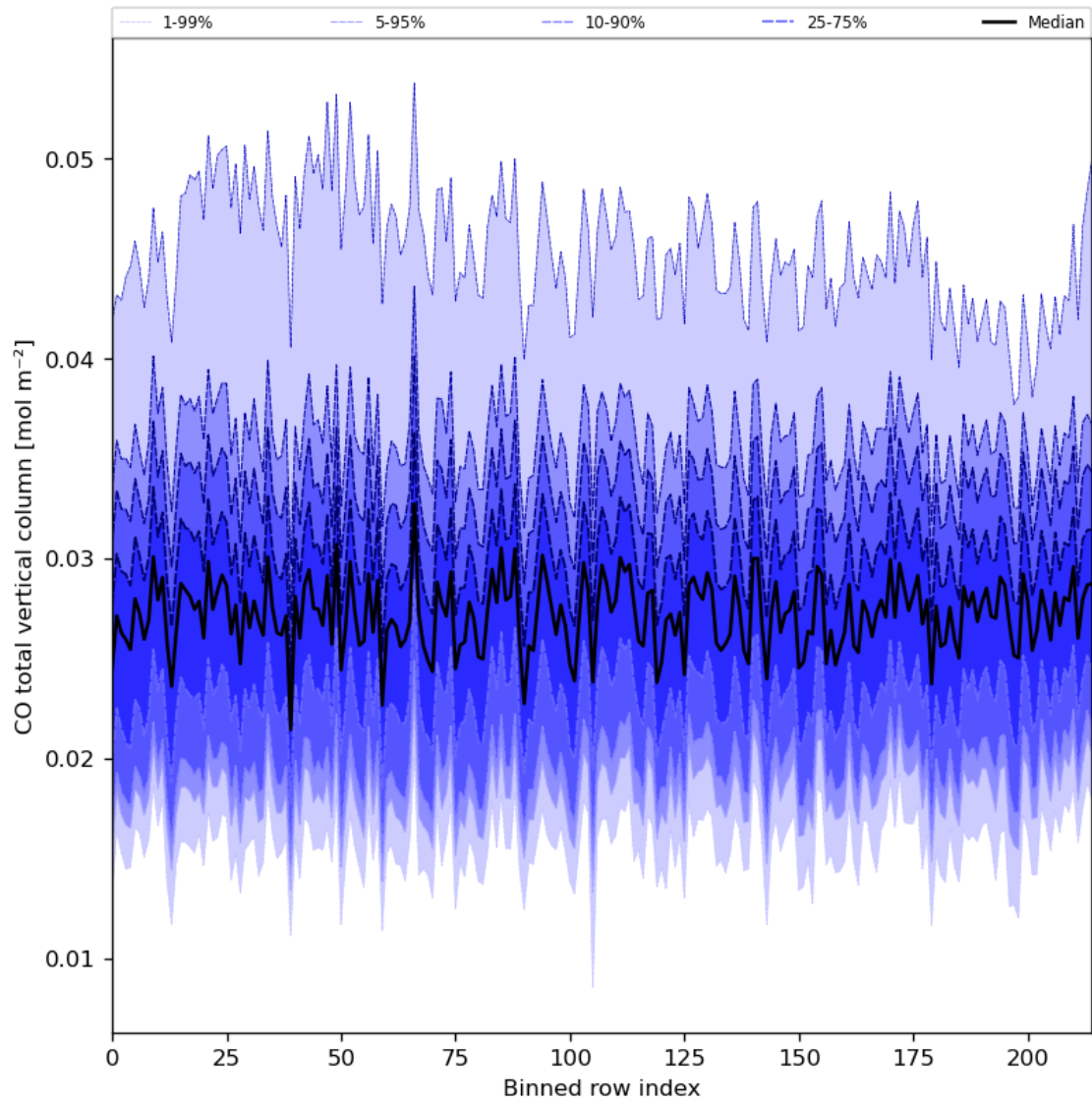
Figure 26: Along track statistics of “CO total vertical column” for 2024-06-13 to 2024-06-15
