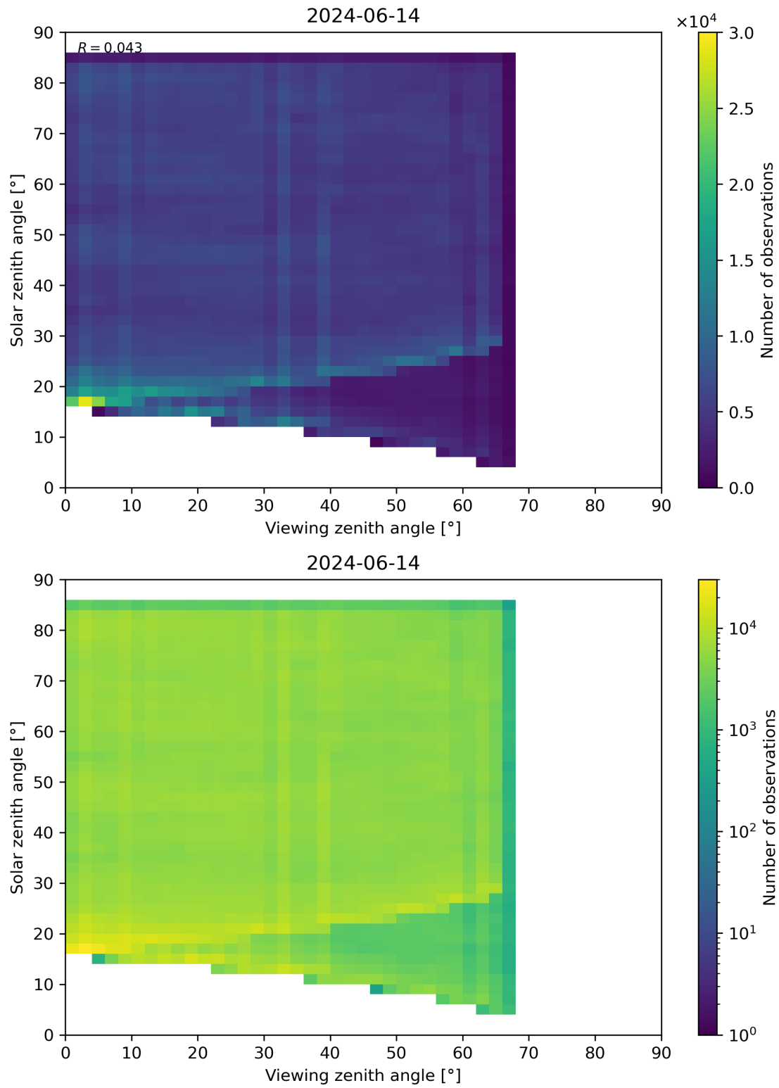
Figure 77: Scatter density plot of “Viewing zenith angle” against “Solar zenith angle” for 2024-06-13 to 2024-06-15.
