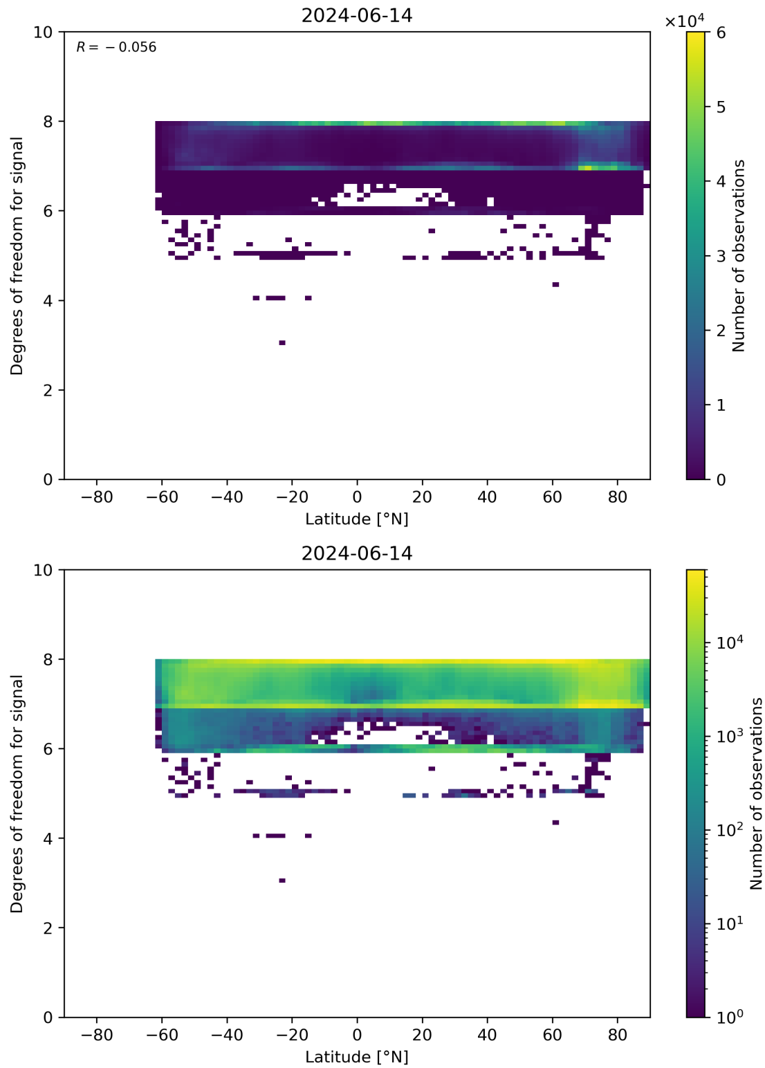
Figure 55: Scatter density plot of “Latitude” against “Degrees of freedom for signal” for 2024-06-13 to 2024-06-15.
