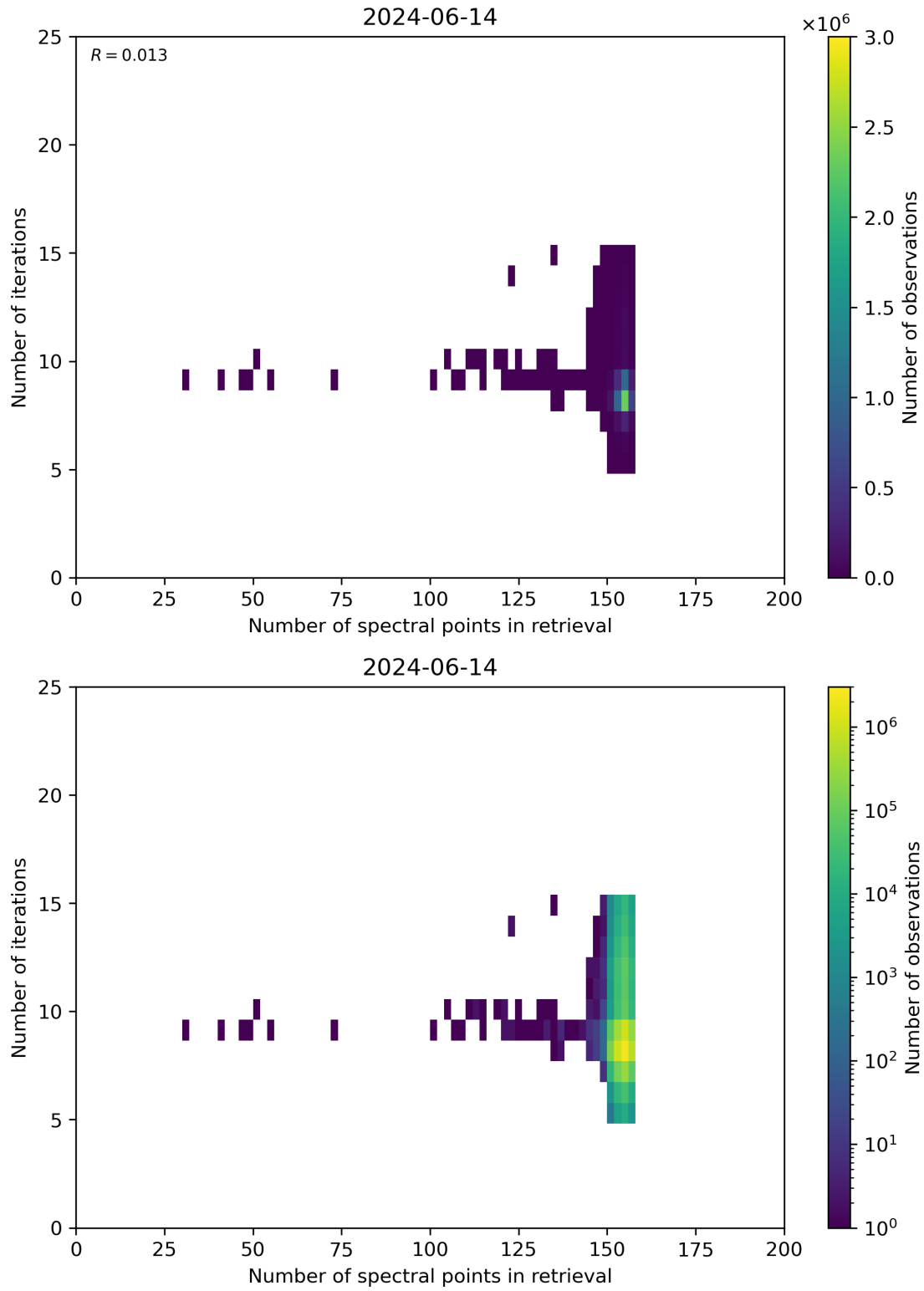
Figure 60: Scatter density plot of “Number of spectral points in retrieval” against “Number of iterations” for 2024-06-13 to 2024-06-15.
