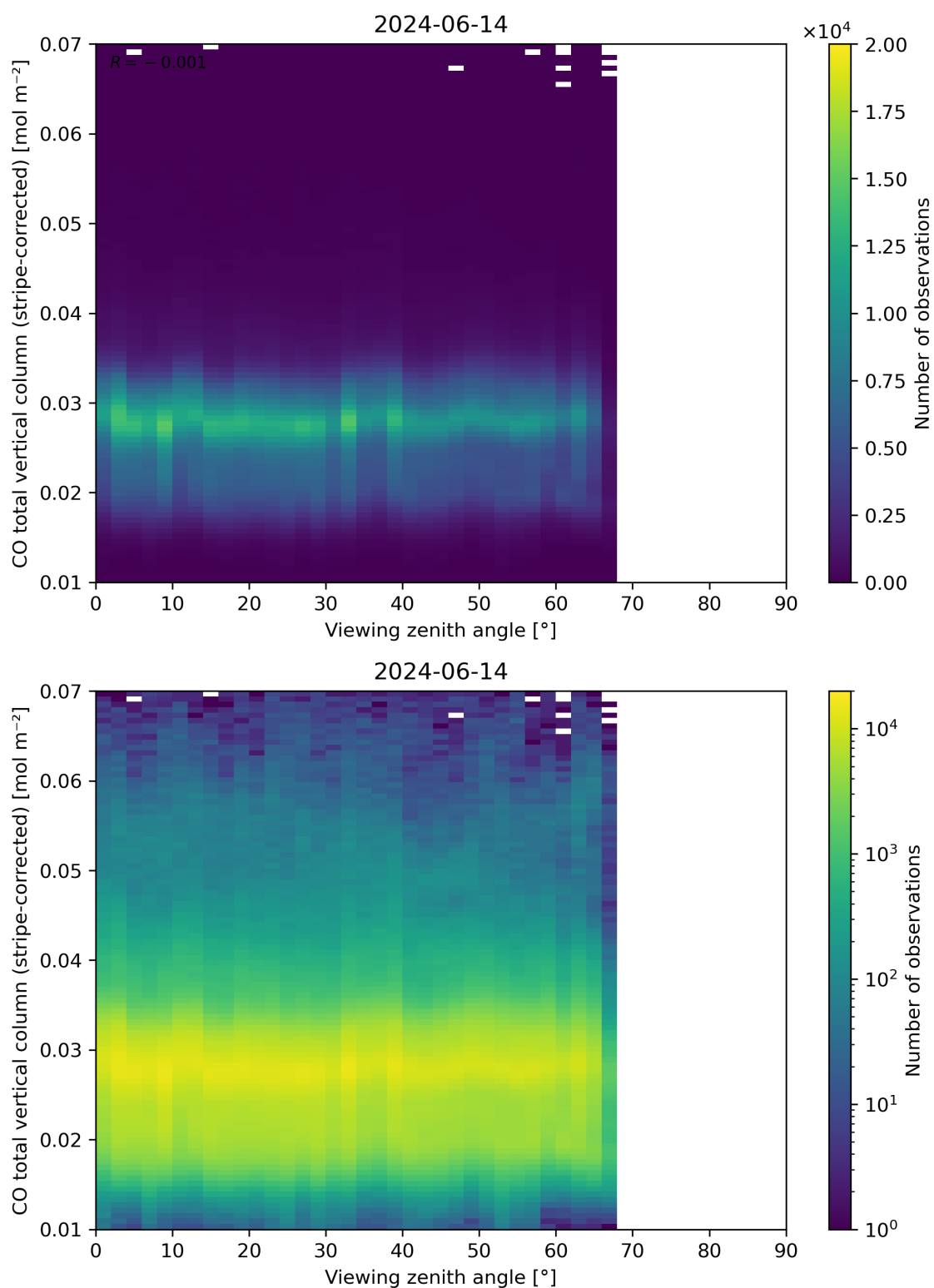
Figure 70: Scatter density plot of “Viewing zenith angle” against “CO total vertical column (stripe-corrected)” for 2024-06-13 to 2024-06-15.
