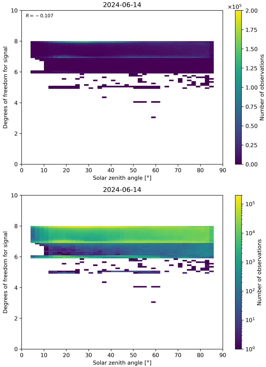
Figure 65: Scatter density plot of “Solar zenith angle” against “Degrees of freedom for signal” for 2024-06-13 to 2024-06-15.
