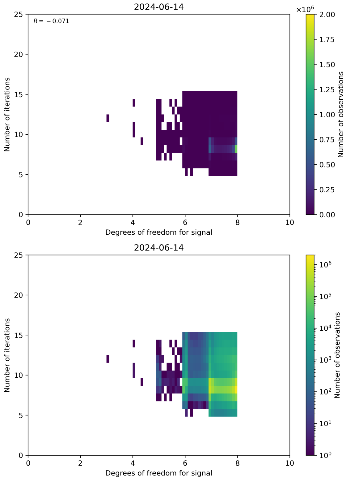
Figure 50: Scatter density plot of “Degrees of freedom for signal” against “Number of iterations” for 2024-06-13 to 2024-06-15.
