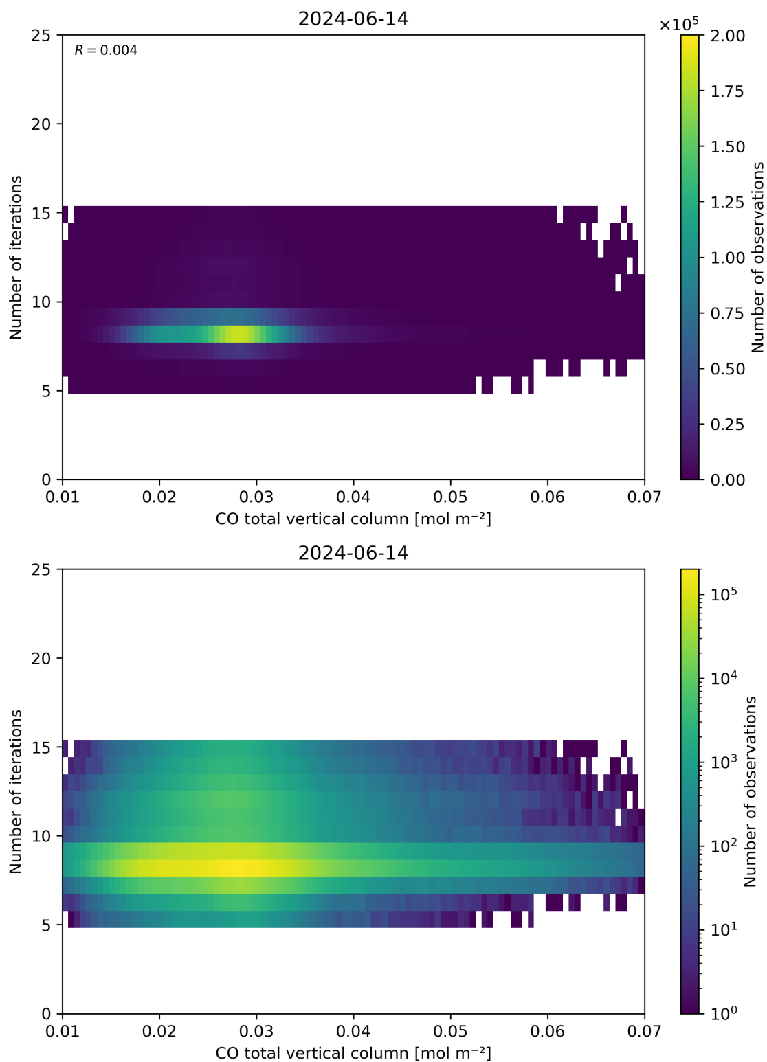
Figure 42: Scatter density plot of “CO total vertical column” against “Number of iterations” for 2024-06-13 to 2024-06-15.
