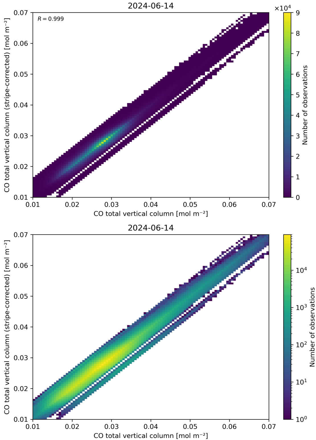
Figure 33: Scatter density plot of “CO total vertical column” against “CO total vertical column (stripe-corrected)” for 2024-06-13 to 2024-06-15.
