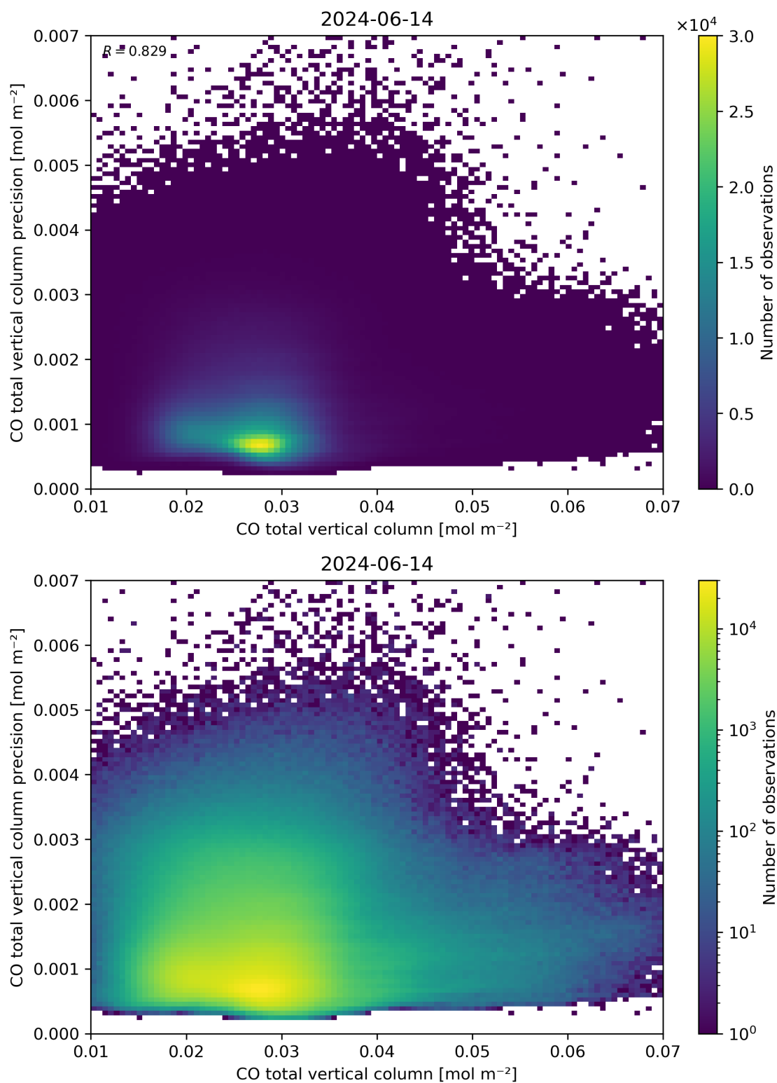
Figure 34: Scatter density plot of “CO total vertical column” against “CO total vertical column precision” for 2024-06-13 to 2024-06-15.
