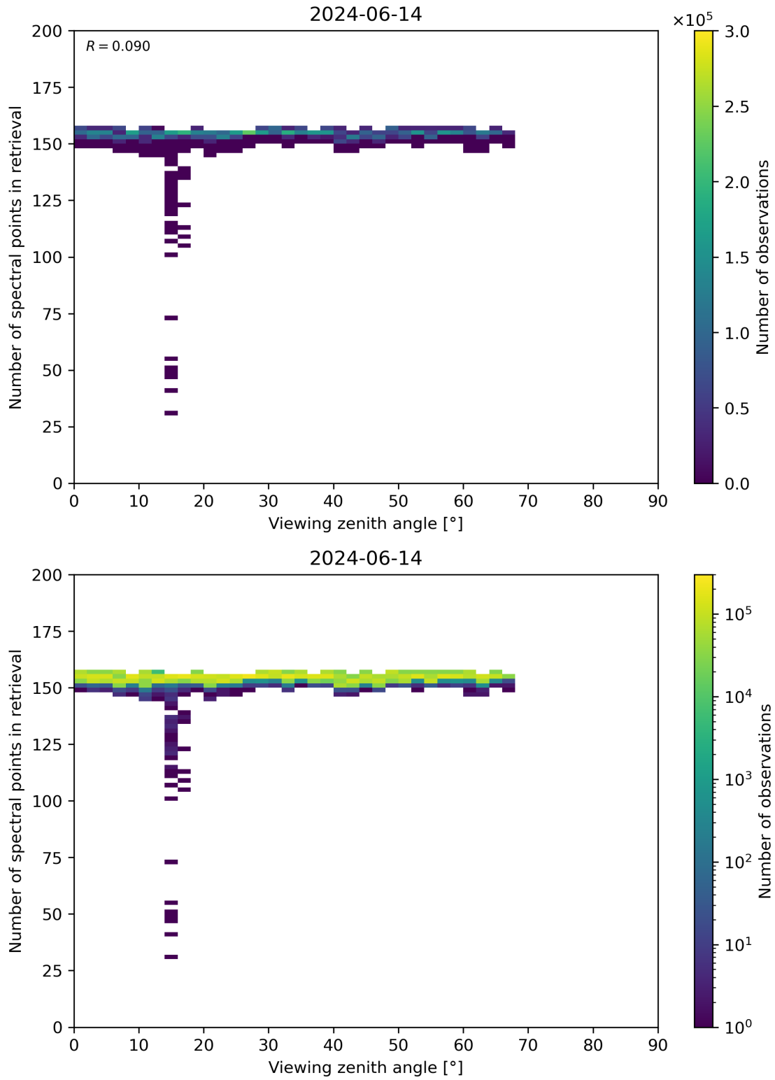
Figure 76: Scatter density plot of “Viewing zenith angle” against “Number of spectral points in retrieval” for 2024-06-13 to 2024-06-15.
