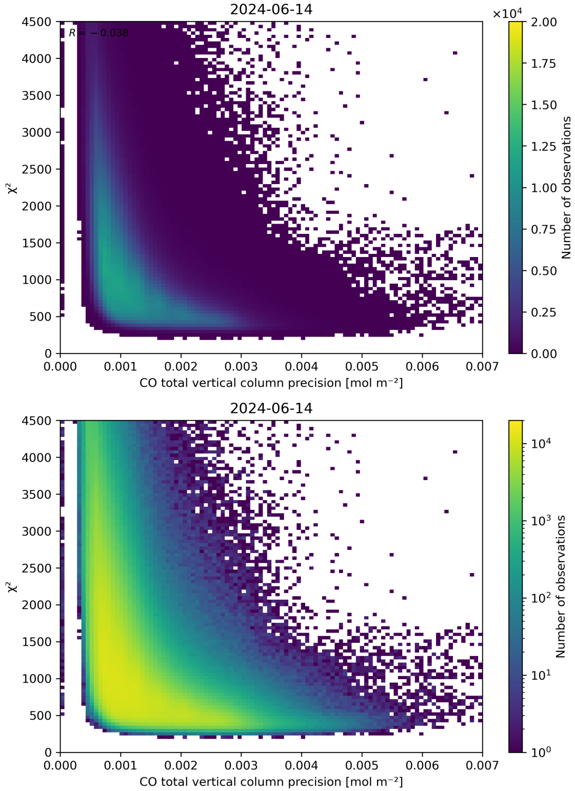
Figure 44: Scatter density plot of “CO total vertical column precision” against “ \chi^2 ” for 2024-06-13 to 2024-06-15.
