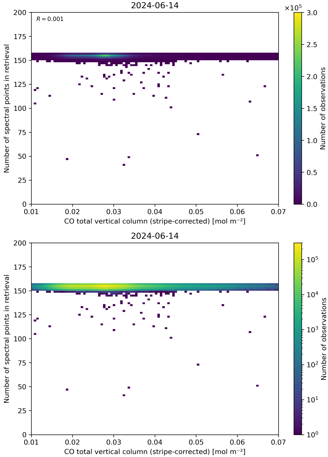
Figure 40: Scatter density plot of “CO total vertical column (stripe-corrected)” against “Number of spectral points in retrieval” for 2024-06-13 to 2024-06-15.
