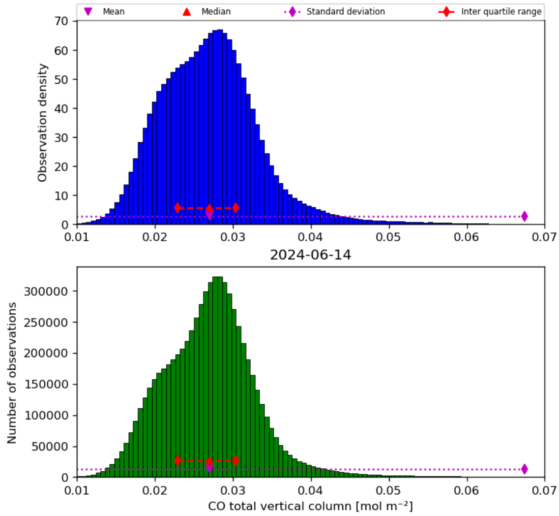
Figure 18: Histogram of “CO total vertical column” for 2024-06-13 to 2024-06-15
