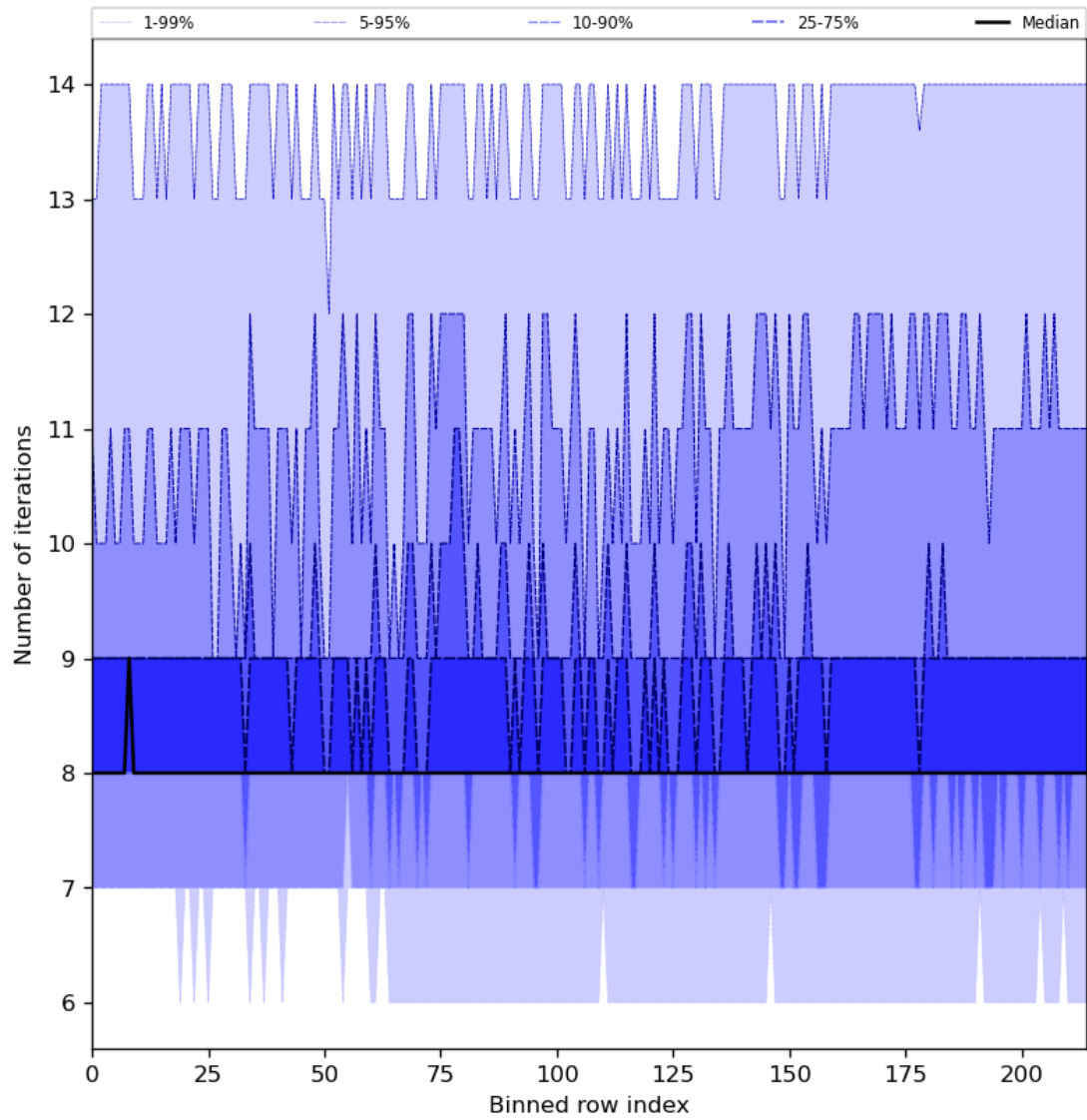
Figure 32: Along track statistics of “Number of iterations” for 2024-06-13 to 2024-06-15
