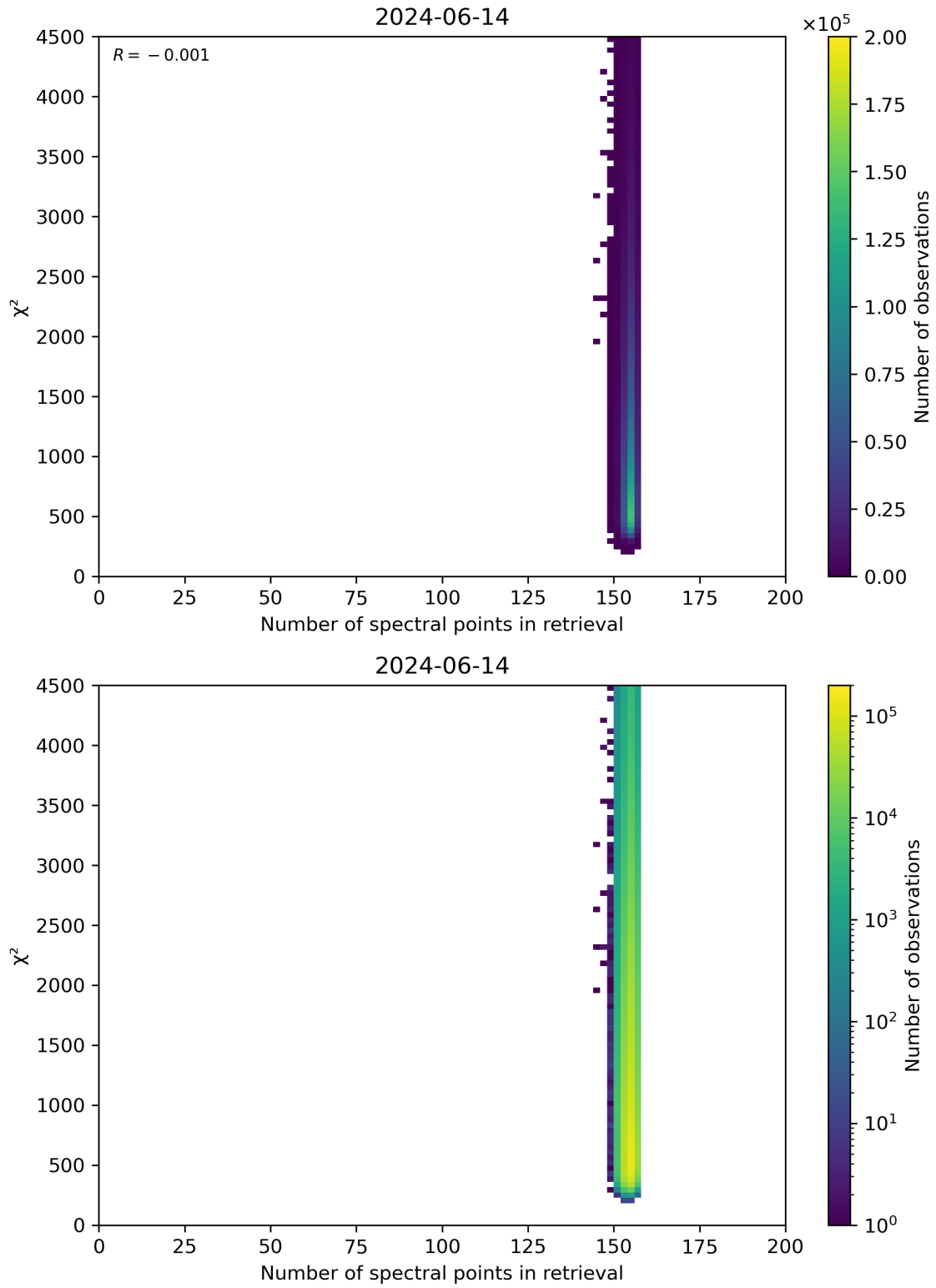
Figure 58: Scatter density plot of “Number of spectral points in retrieval” against “ \chi^2 ” for 2024-06-13 to 2024-06-15.
