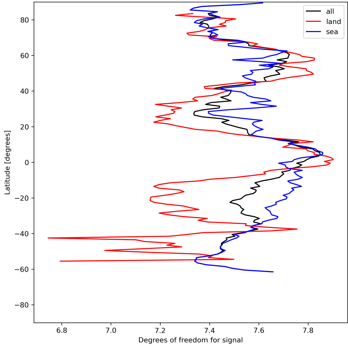
Figure 15: Zonal average of “Degrees of freedom for signal” for 2024-06-13 to 2024-06-15.
