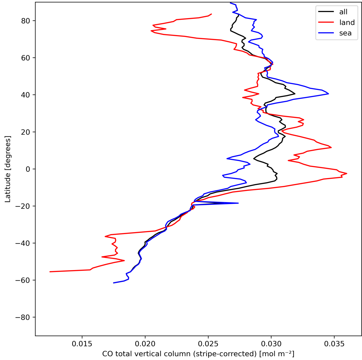
Figure 11: Zonal average of “CO total vertical column (stripe-corrected)” for 2024-06-13 to 2024-06-15.
