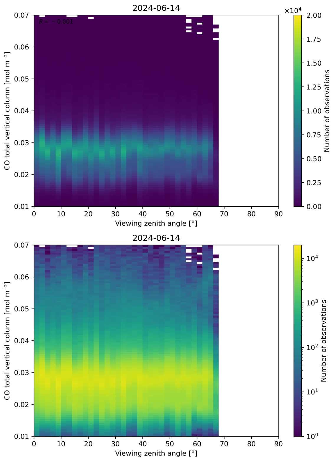
Figure 69: Scatter density plot of “Viewing zenith angle” against “CO total vertical column” for 2024-06-13 to 2024-06-15.
