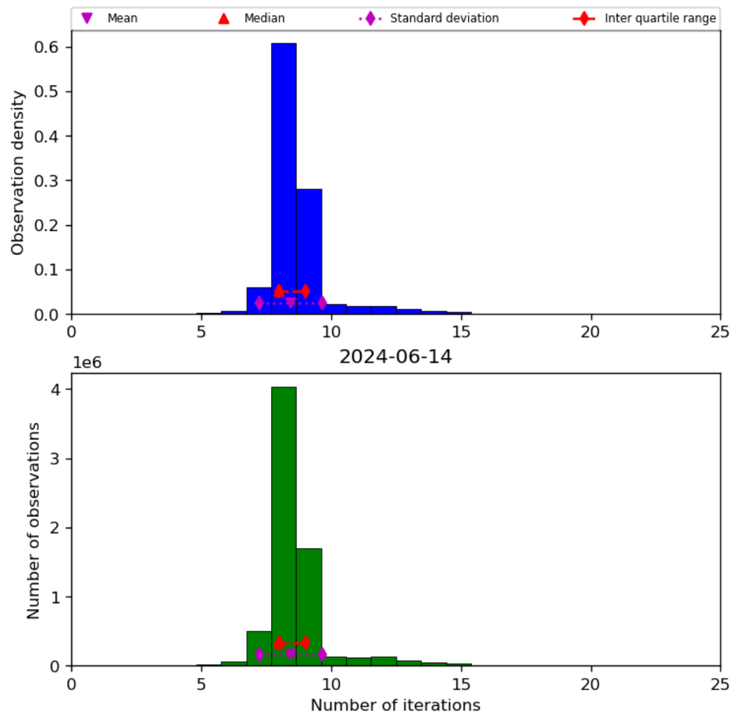
Figure 24: Histogram of “Number of iterations” for 2024-06-13 to 2024-06-15
