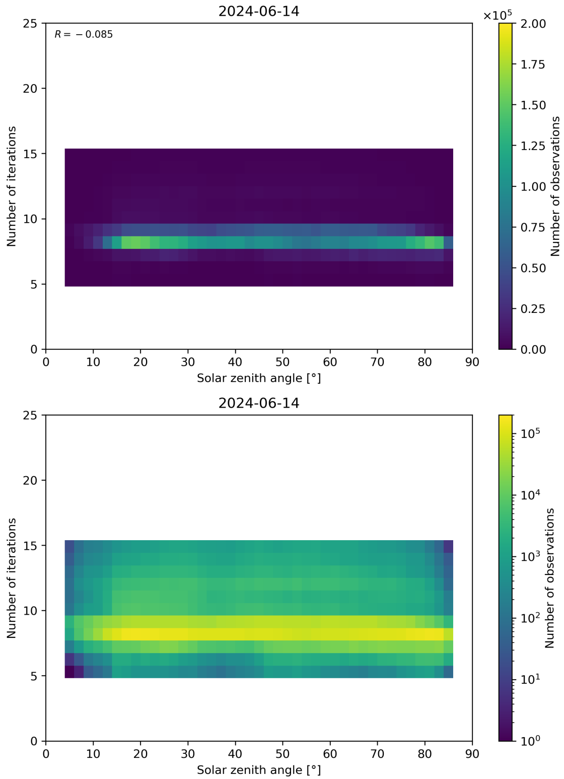
Figure 67: Scatter density plot of “Solar zenith angle” against “Number of iterations” for 2024-06-13 to 2024-06-15.
