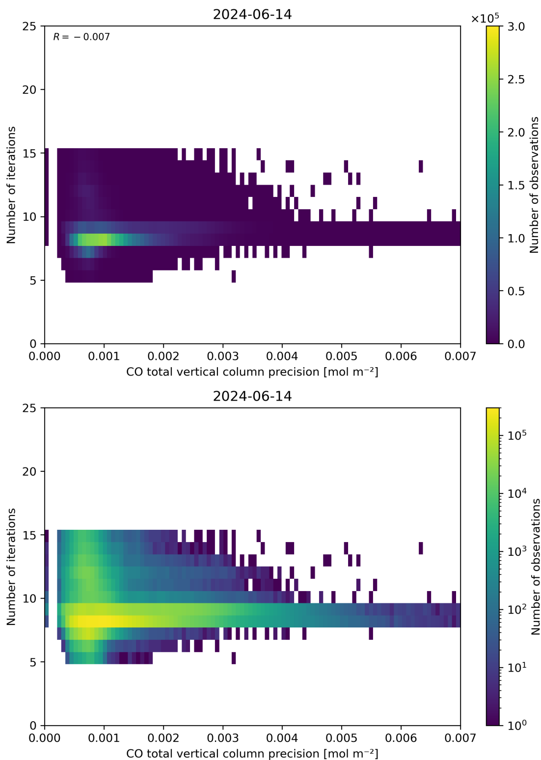
Figure 46: Scatter density plot of “CO total vertical column precision” against “Number of iterations” for 2024-06-13 to 2024-06-15.
