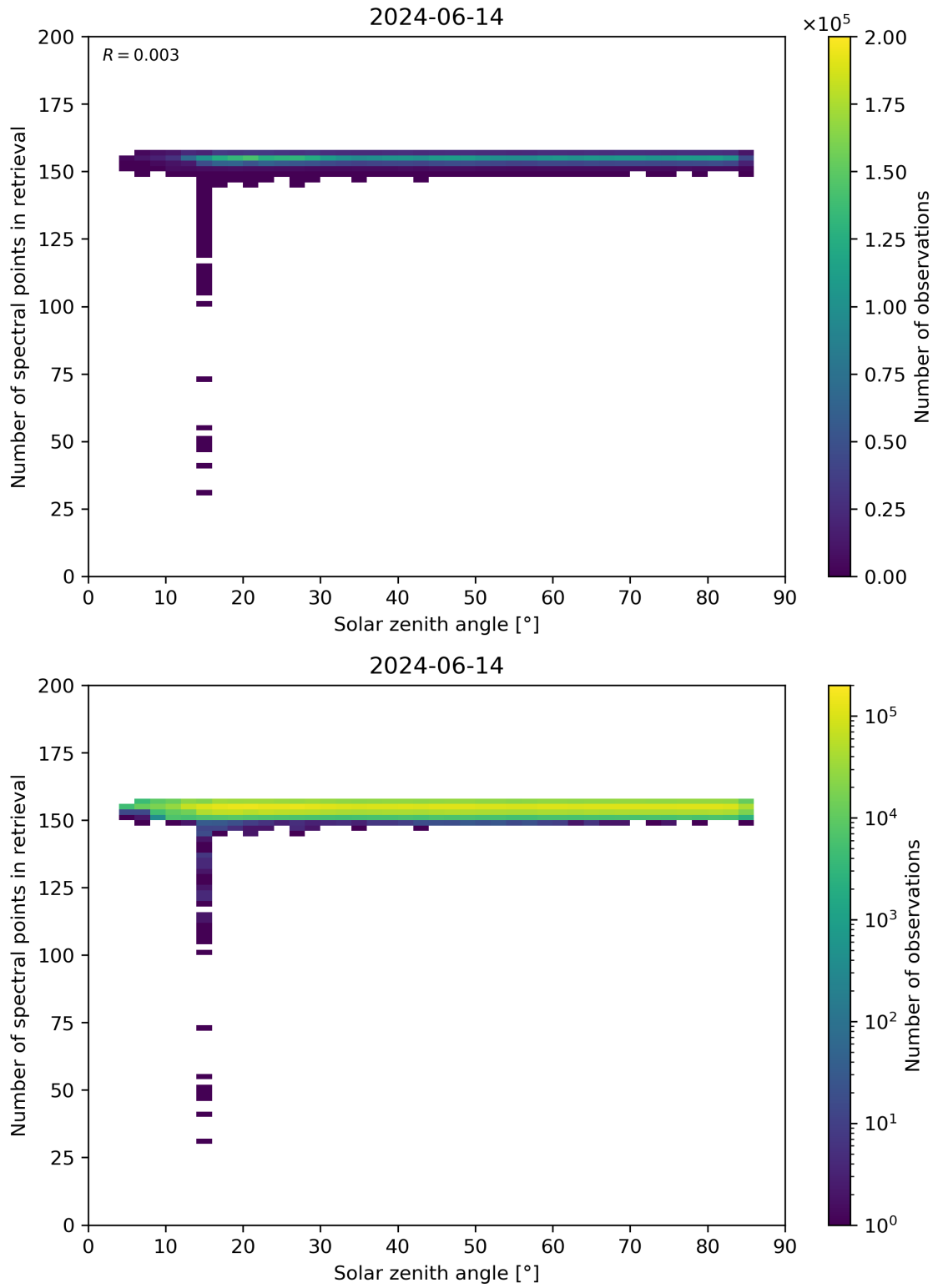
Figure 68: Scatter density plot of “Solar zenith angle” against “Number of spectral points in retrieval” for 2024-06-13 to 2024-06-15.
