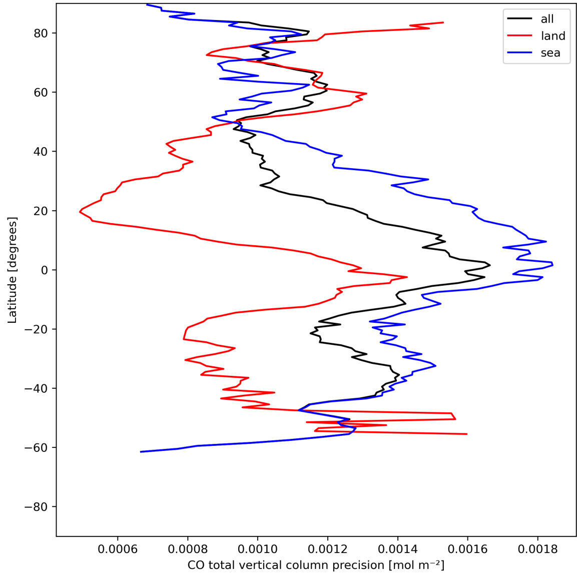
Figure 12: Zonal average of “CO total vertical column precision” for 2024-06-13 to 2024-06-15.
