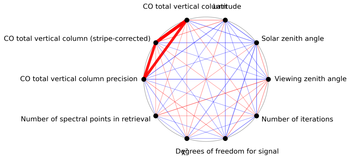
Figure 1: Map of correlation graph for 2024-06-13 to 2024-06-15.
