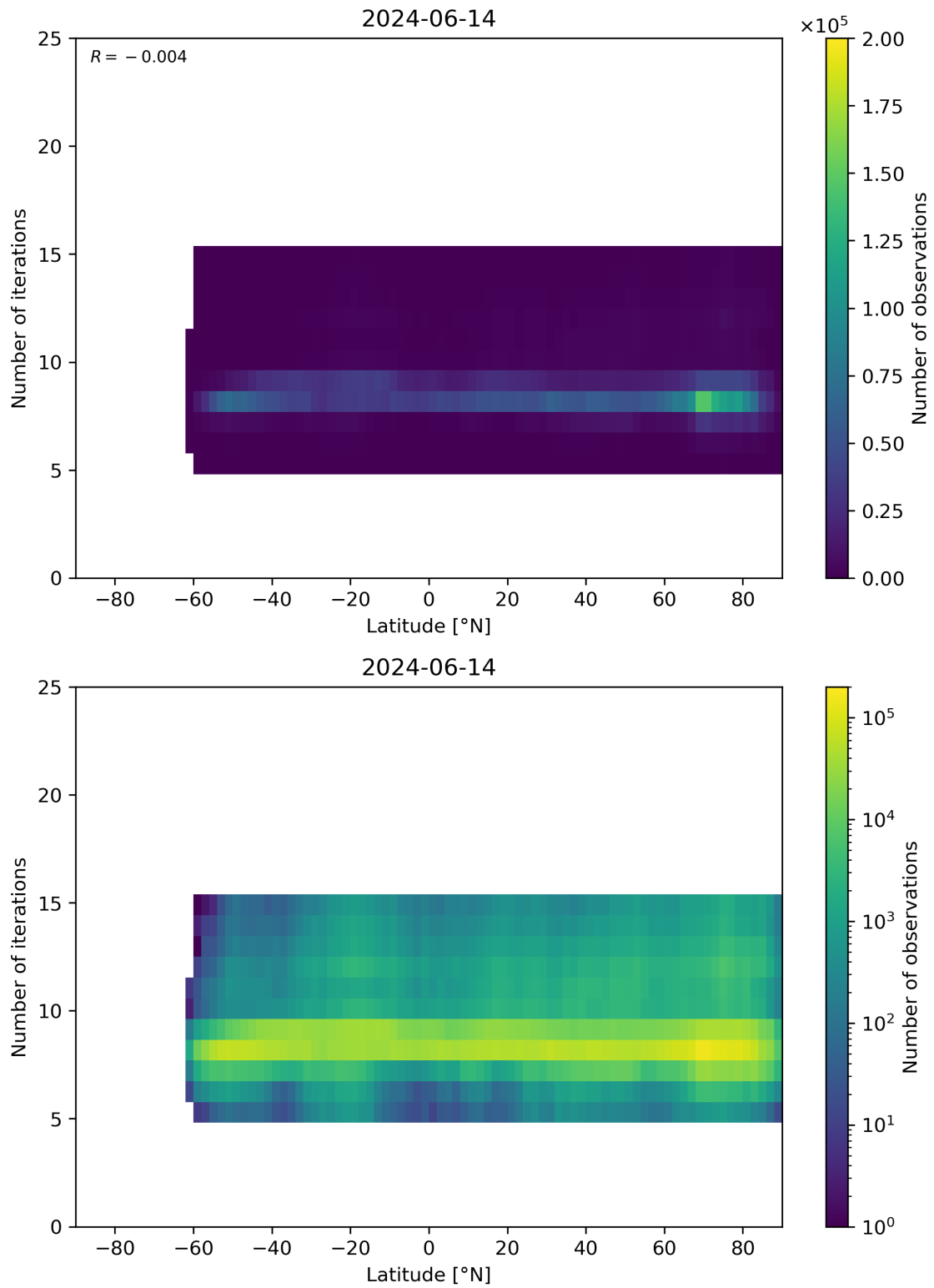
Figure 56: Scatter density plot of “Latitude” against “Number of iterations” for 2024-06-13 to 2024-06-15.
