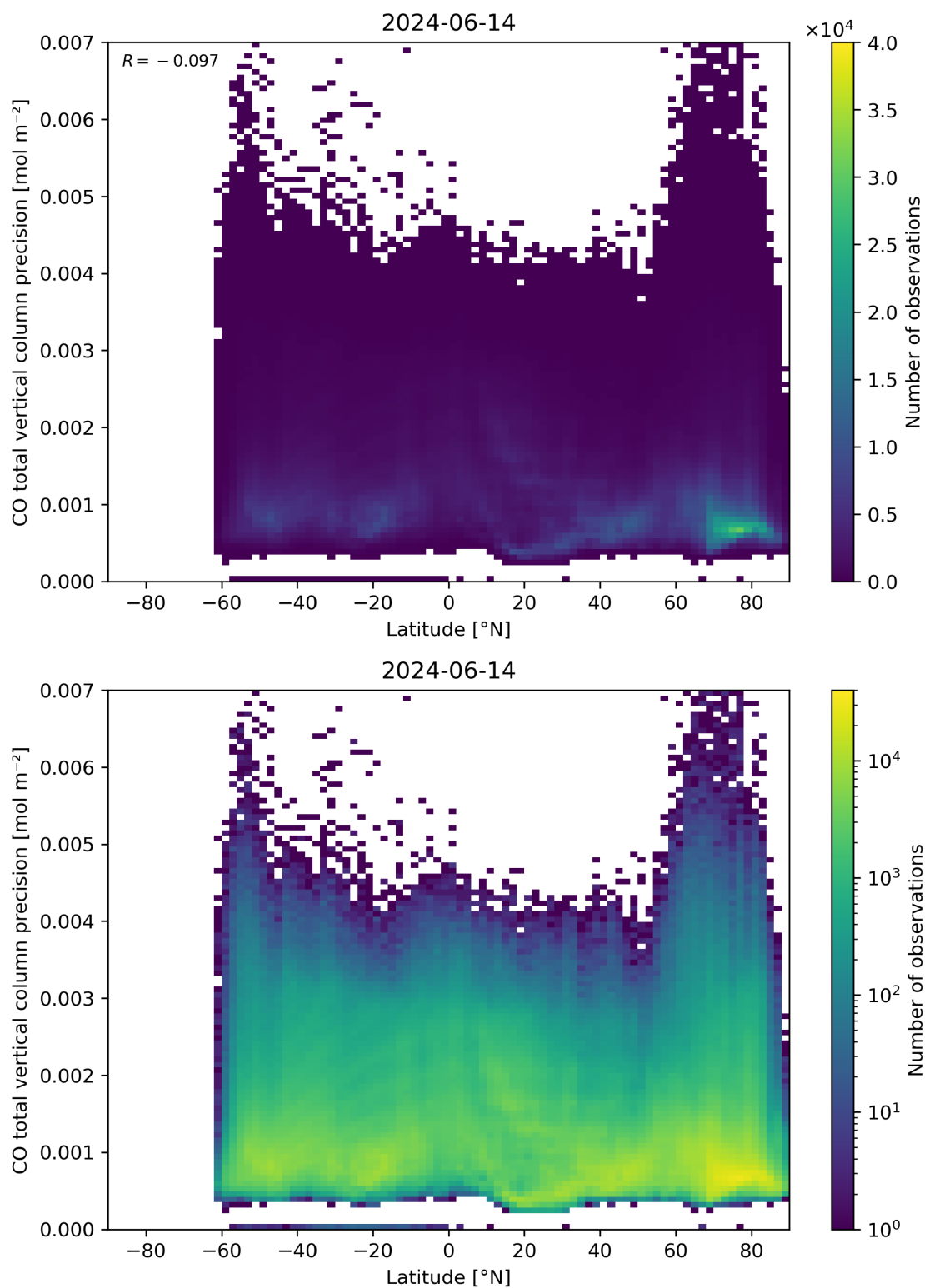
Figure 53: Scatter density plot of “Latitude” against “CO total vertical column precision” for 2024-06-13 to 2024-06-15.
