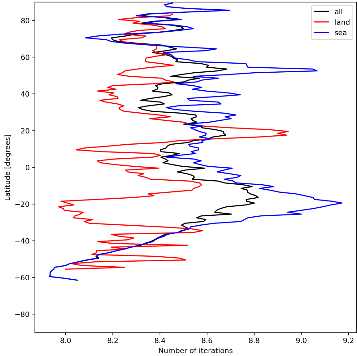
Figure 16: Zonal average of “Number of iterations” for 2024-06-13 to 2024-06-15.
