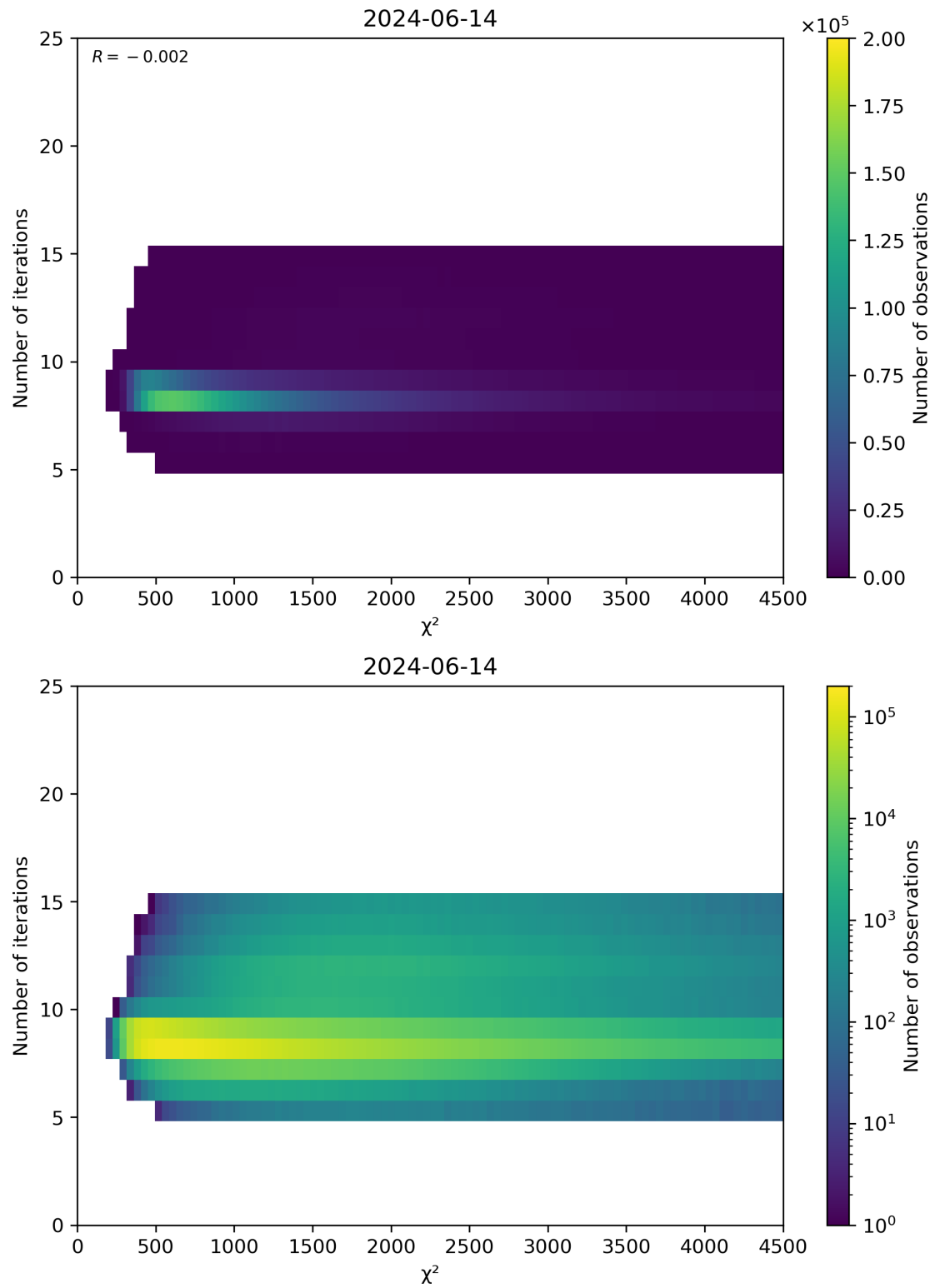
Figure 49: Scatter density plot of “ \chi^2 ” against “Number of iterations” for 2024-06-13 to 2024-06-15.
