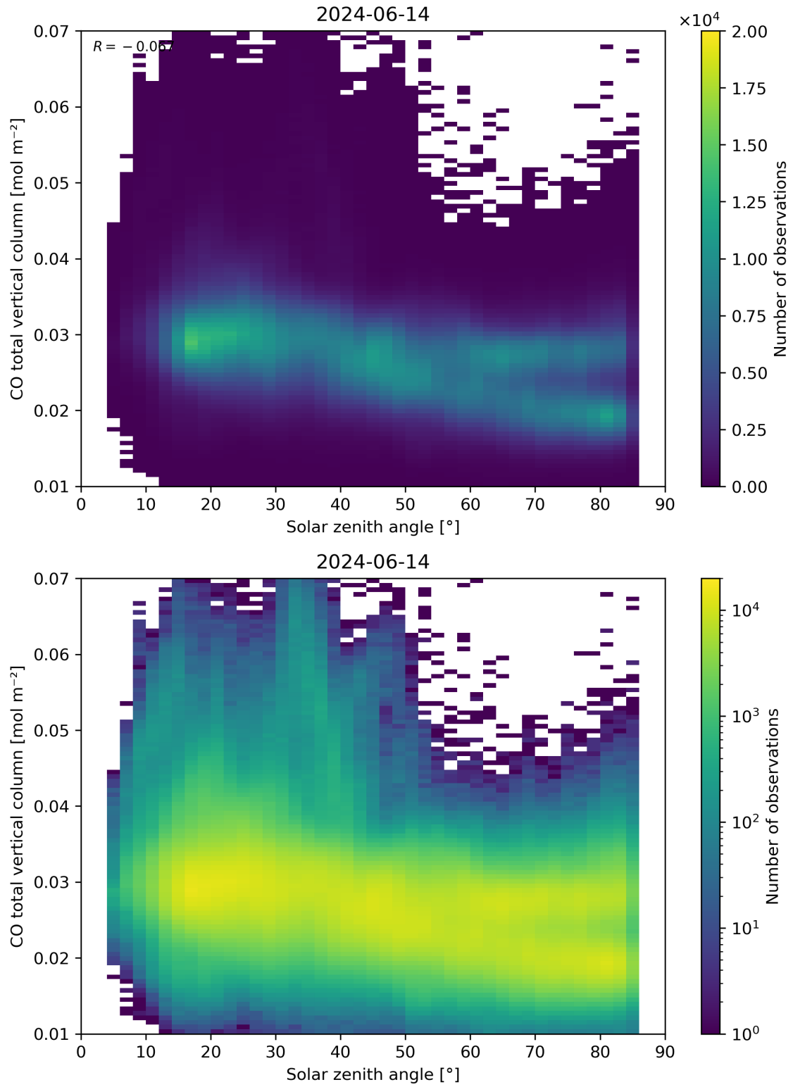
Figure 61: Scatter density plot of “Solar zenith angle” against “CO total vertical column” for 2024-06-13 to 2024-06-15.
