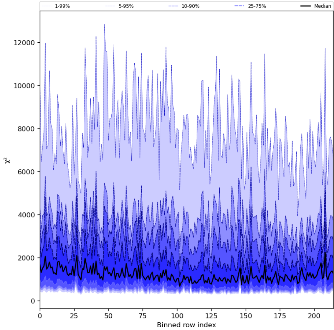
Figure 30: Along track statistics of “ \chi^2 ” for 2024-06-13 to 2024-06-15
