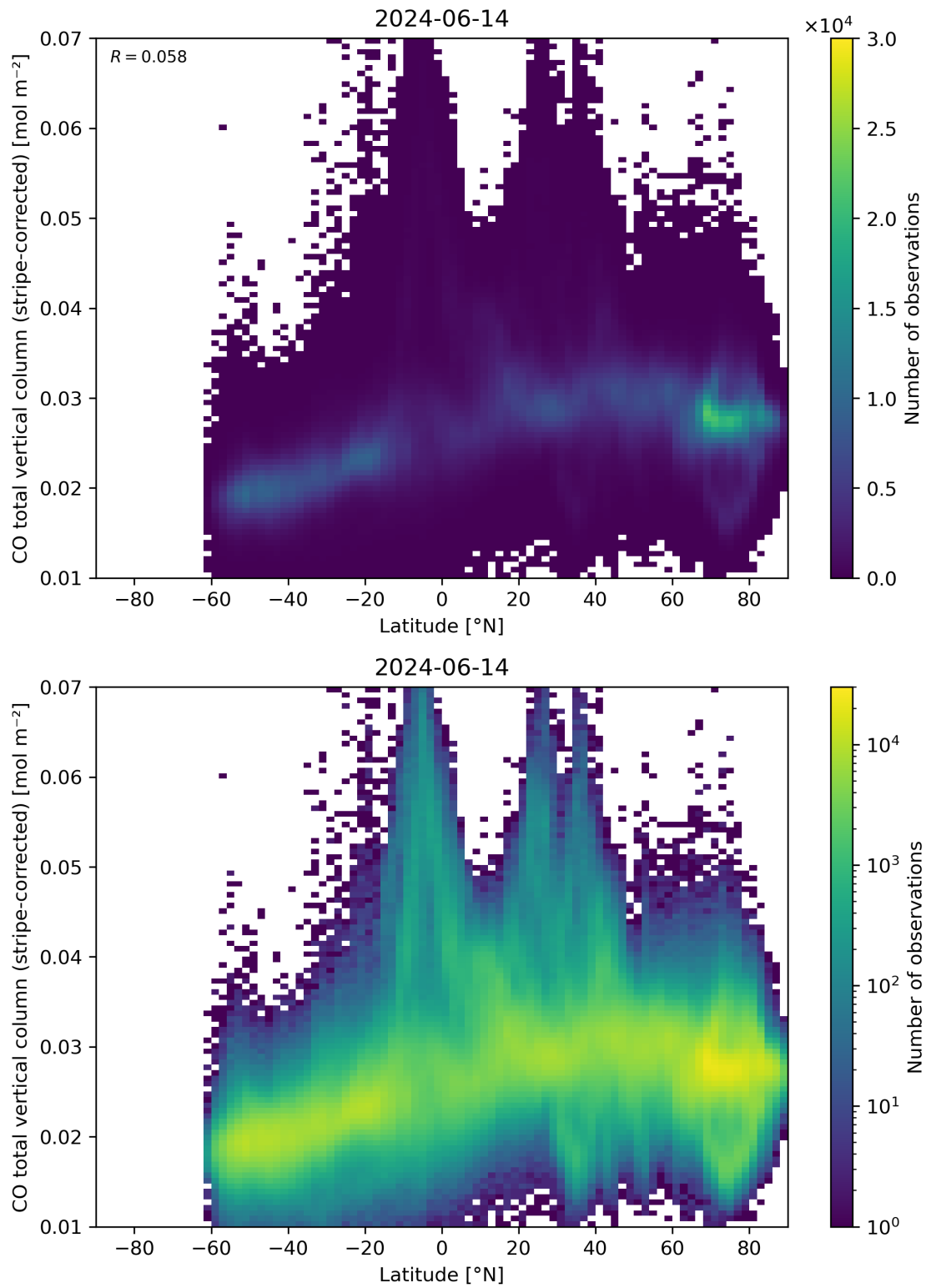
Figure 52: Scatter density plot of “Latitude” against “CO total vertical column (stripe-corrected)” for 2024-06-13 to 2024-06-15.
