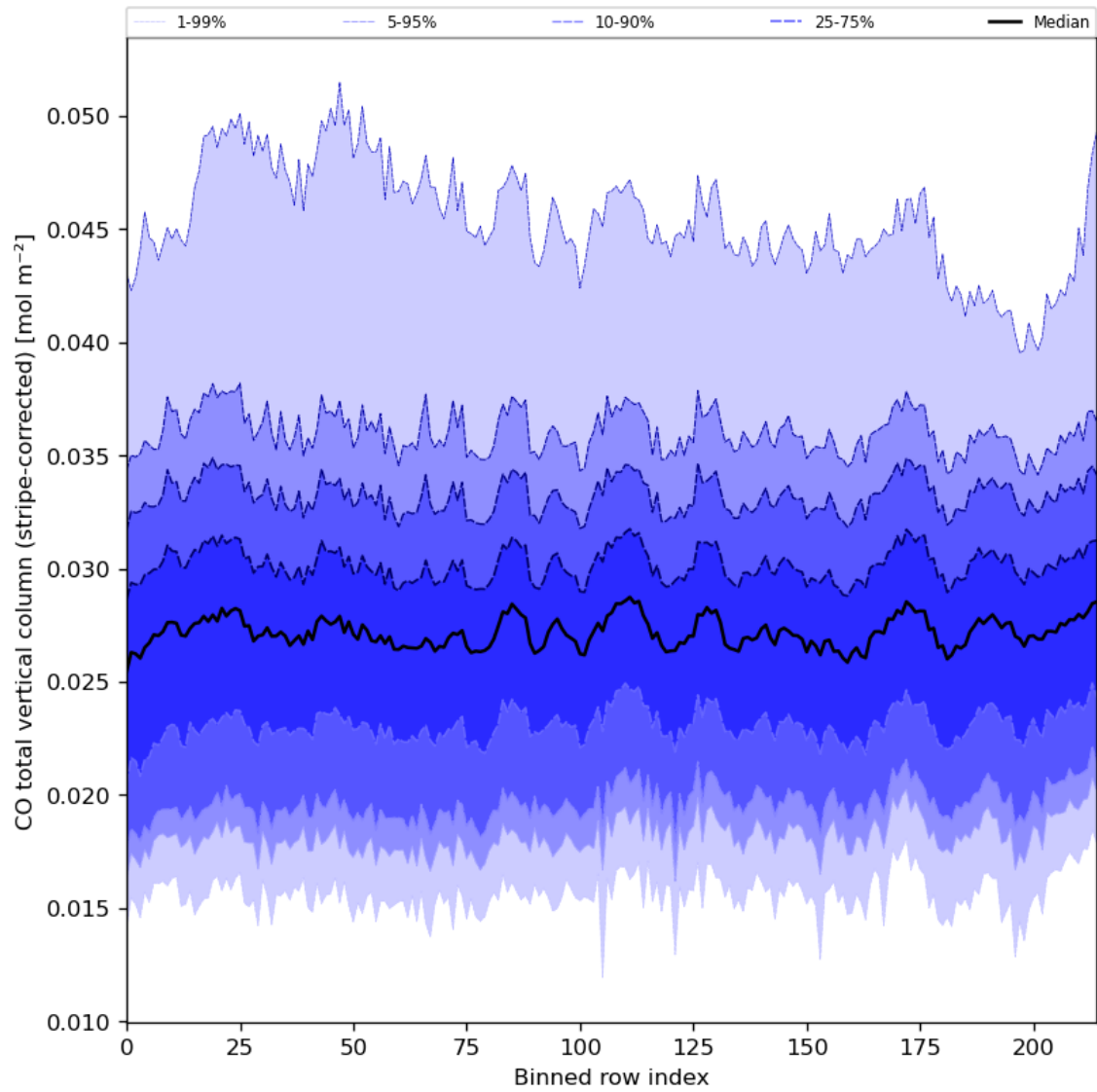
Figure 27: Along track statistics of “CO total vertical column (stripe-corrected)” for 2024-06-13 to 2024-06-15
