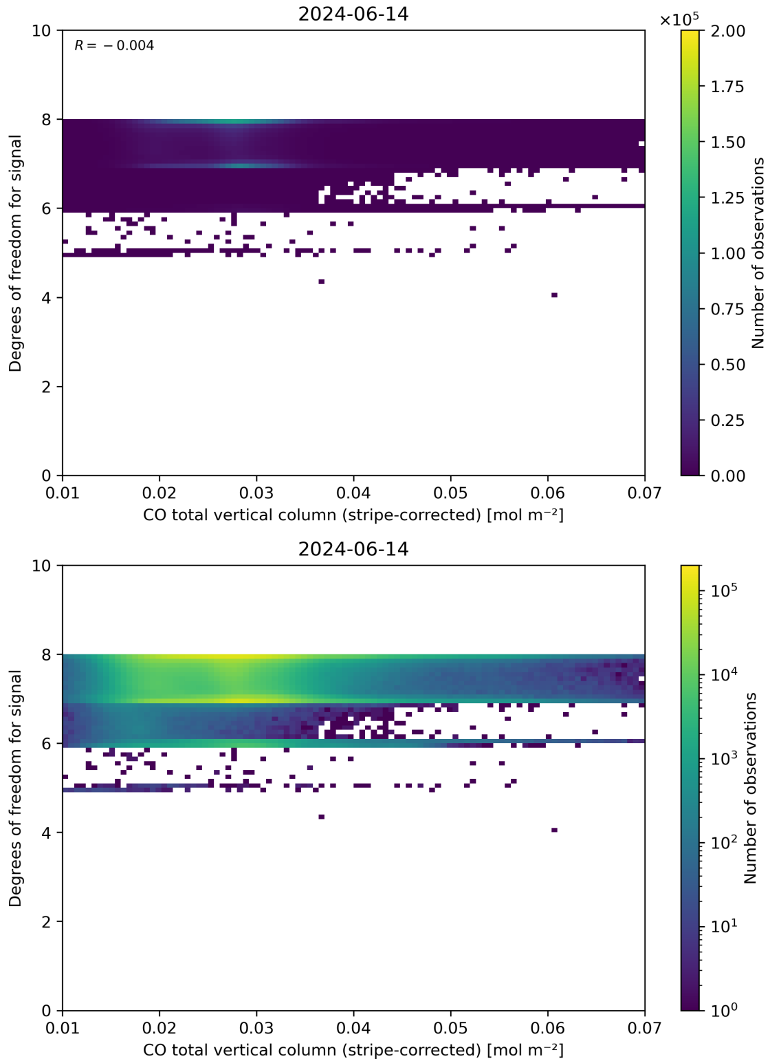
Figure 38: Scatter density plot of “CO total vertical column (stripe-corrected)” against “Degrees of freedom for signal” for 2024-06-13 to 2024-06-15.
