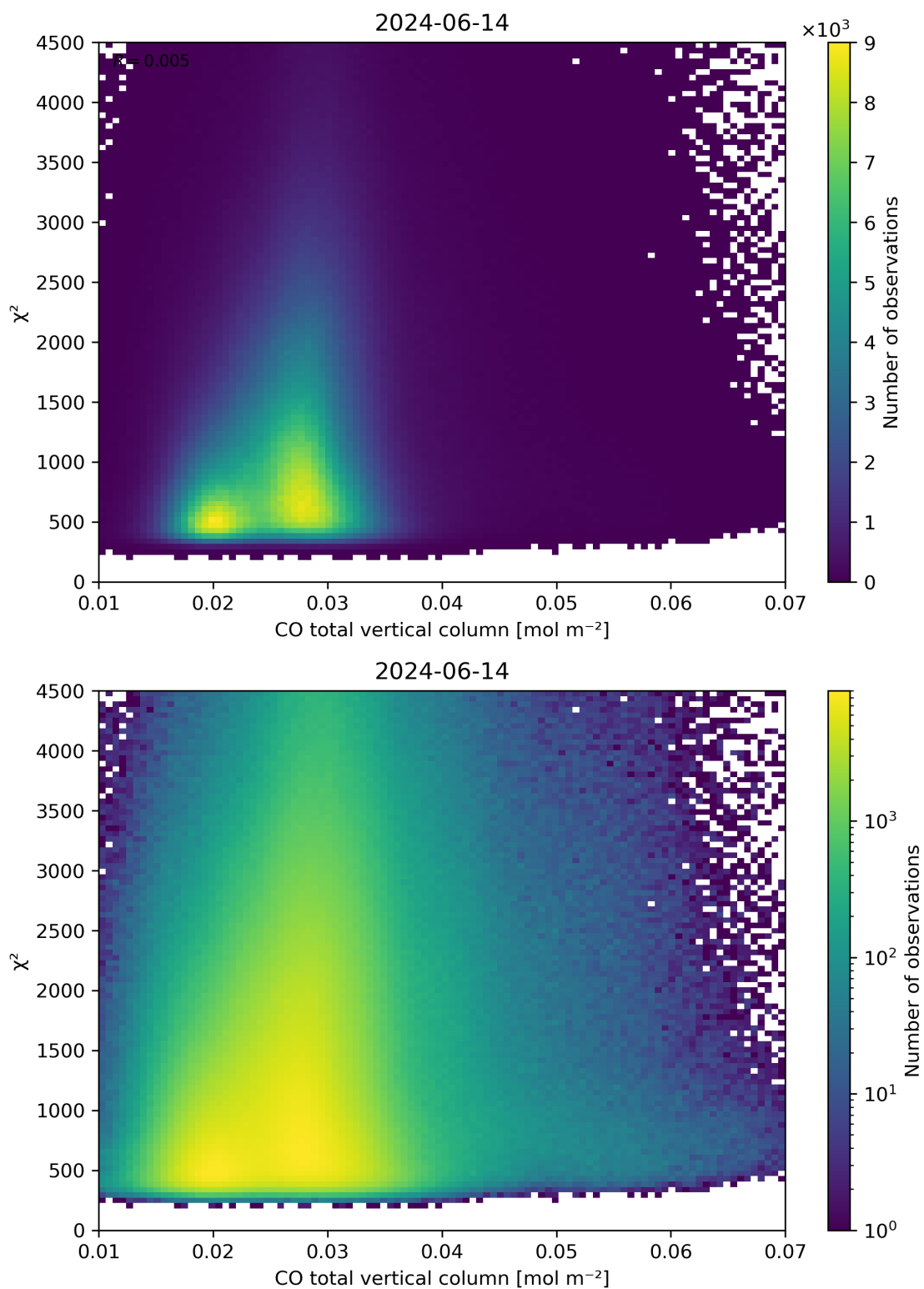
Figure 35: Scatter density plot of “CO total vertical column” against “ \chi^2 ” for 2024-06-13 to 2024-06-15.
