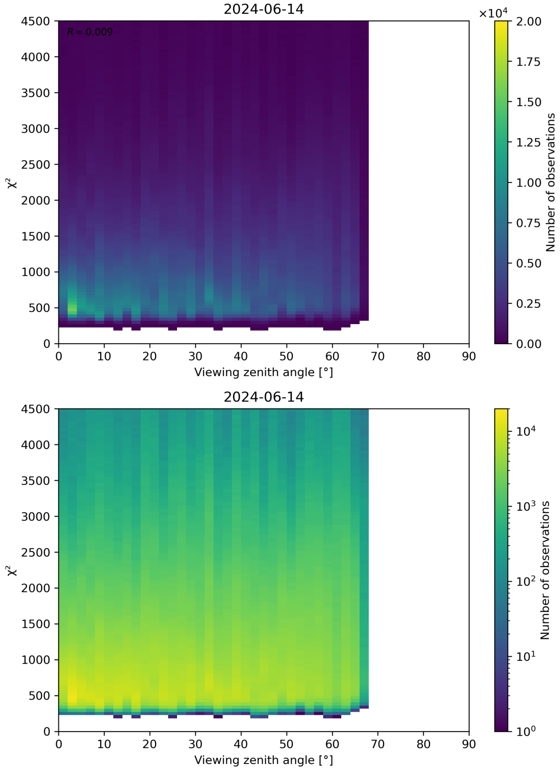
Figure 72: Scatter density plot of “Viewing zenith angle” against “ \chi^2 ” for 2024-06-13 to 2024-06-15.
