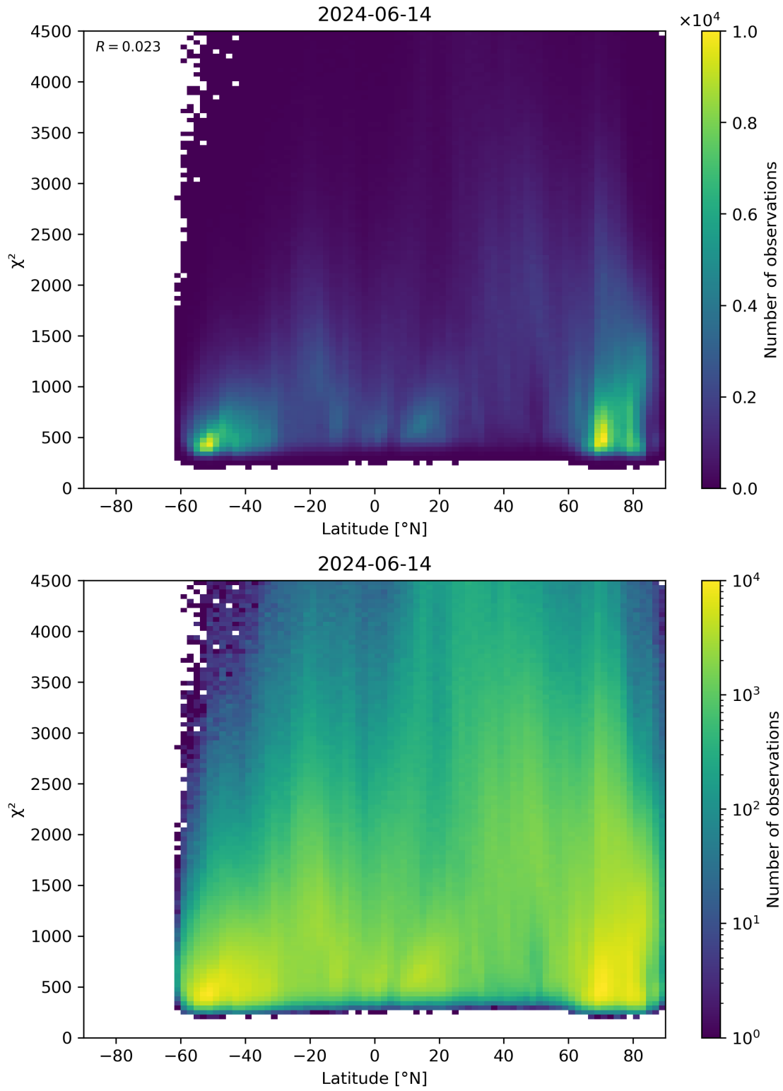
Figure 54: Scatter density plot of “Latitude” against “ \chi^2 ” for 2024-06-13 to 2024-06-15.
