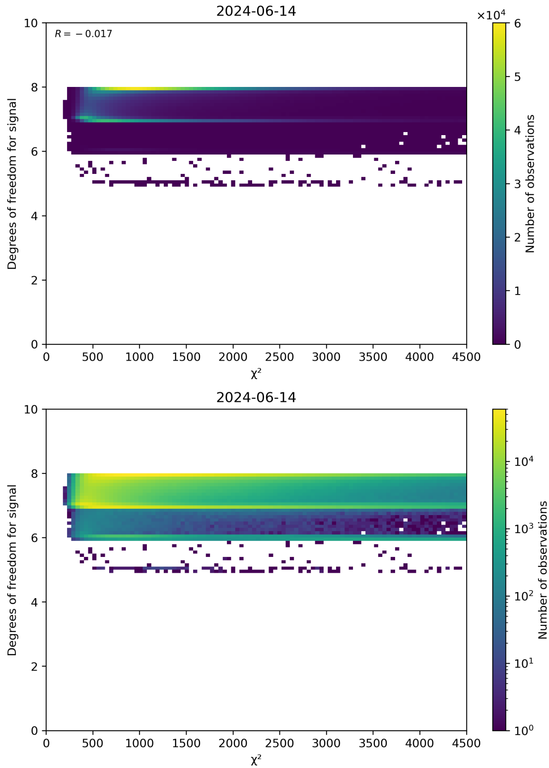
Figure 48: Scatter density plot of “ \chi^2 ” against “Degrees of freedom for signal” for 2024-06-13 to 2024-06-15.
