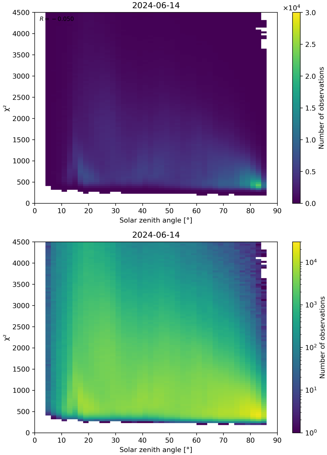
Figure 64: Scatter density plot of “Solar zenith angle” against “ \chi^2 ” for 2024-06-13 to 2024-06-15.
