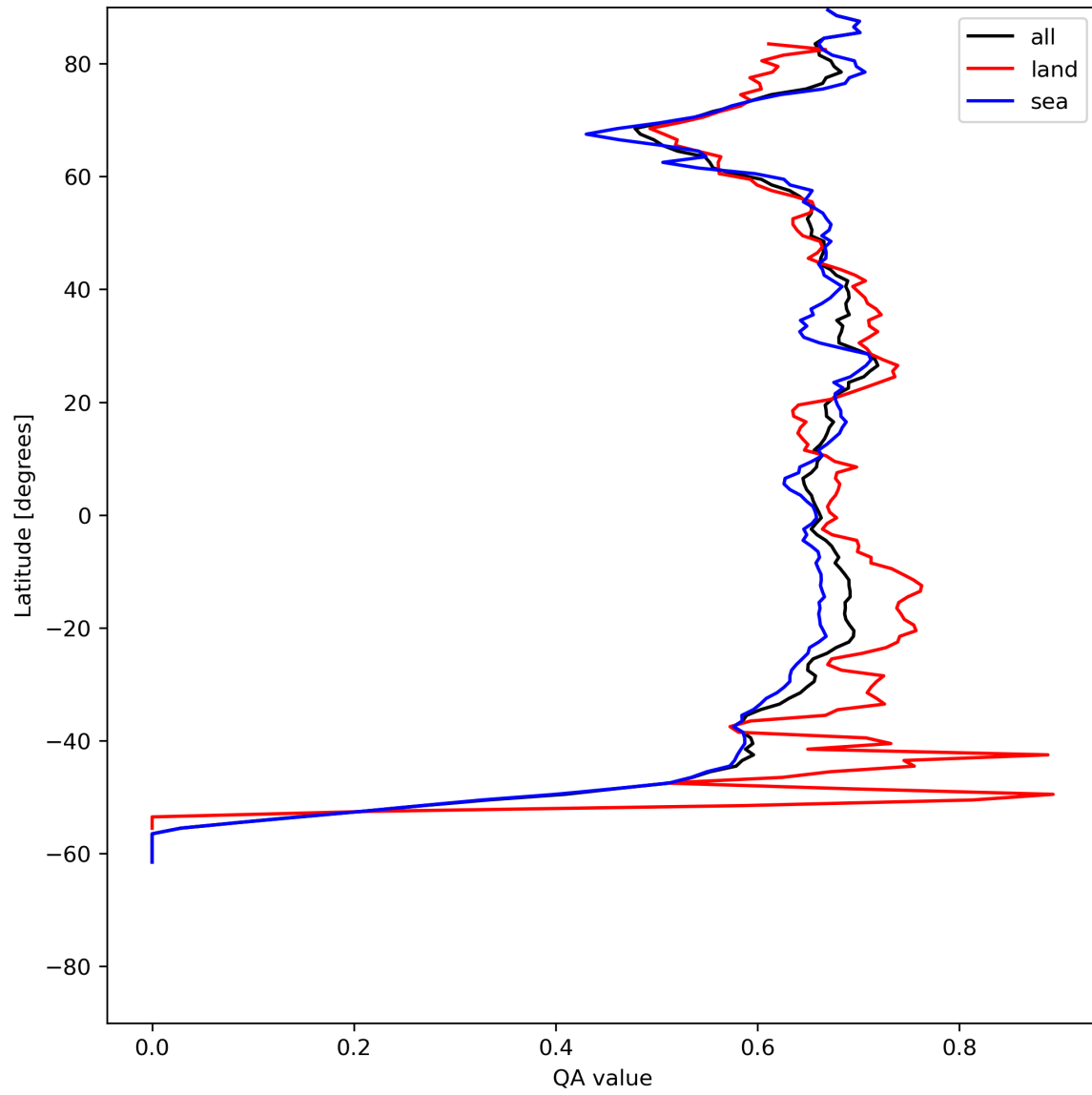
Figure 9: Zonal average of “QA value” for 2024-06-13 to 2024-06-15.
