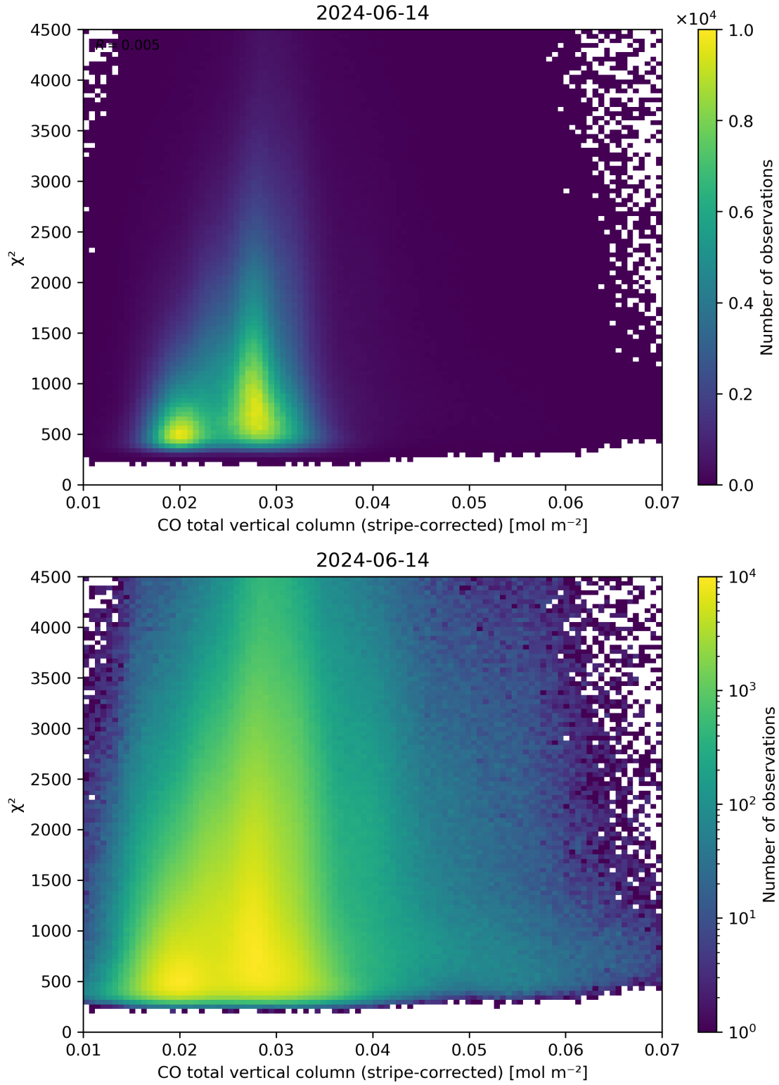
Figure 37: Scatter density plot of “CO total vertical column (stripe-corrected)” against “ \chi^2 ” for 2024-06-13 to 2024-06-15.
