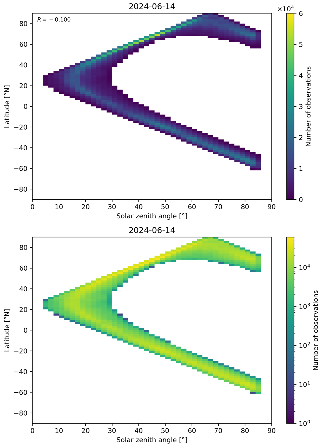
Figure 66: Scatter density plot of “Solar zenith angle” against “Latitude” for 2024-06-13 to 2024-06-15.
