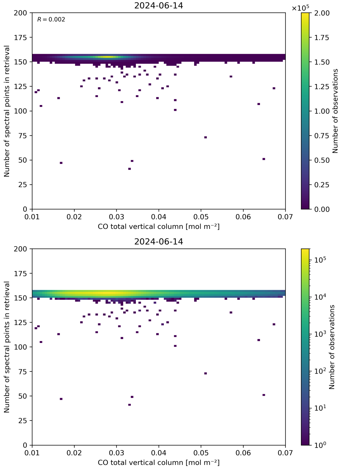
Figure 43: Scatter density plot of “CO total vertical column” against “Number of spectral points in retrieval” for 2024-06-13 to 2024-06-15.
