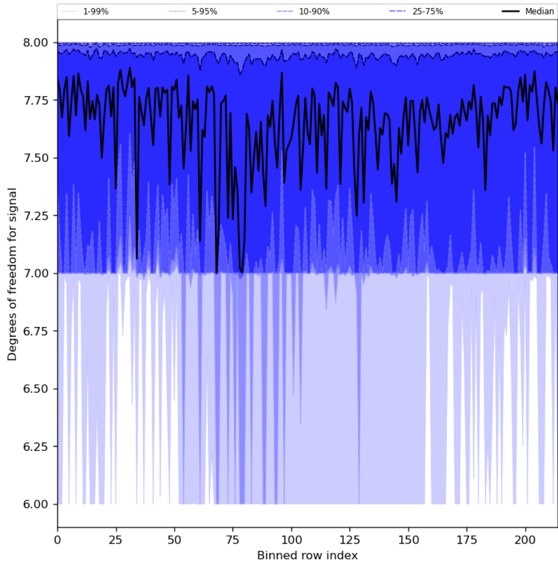
Figure 31: Along track statistics of “Degrees of freedom for signal” for 2024-06-13 to 2024-06-15
