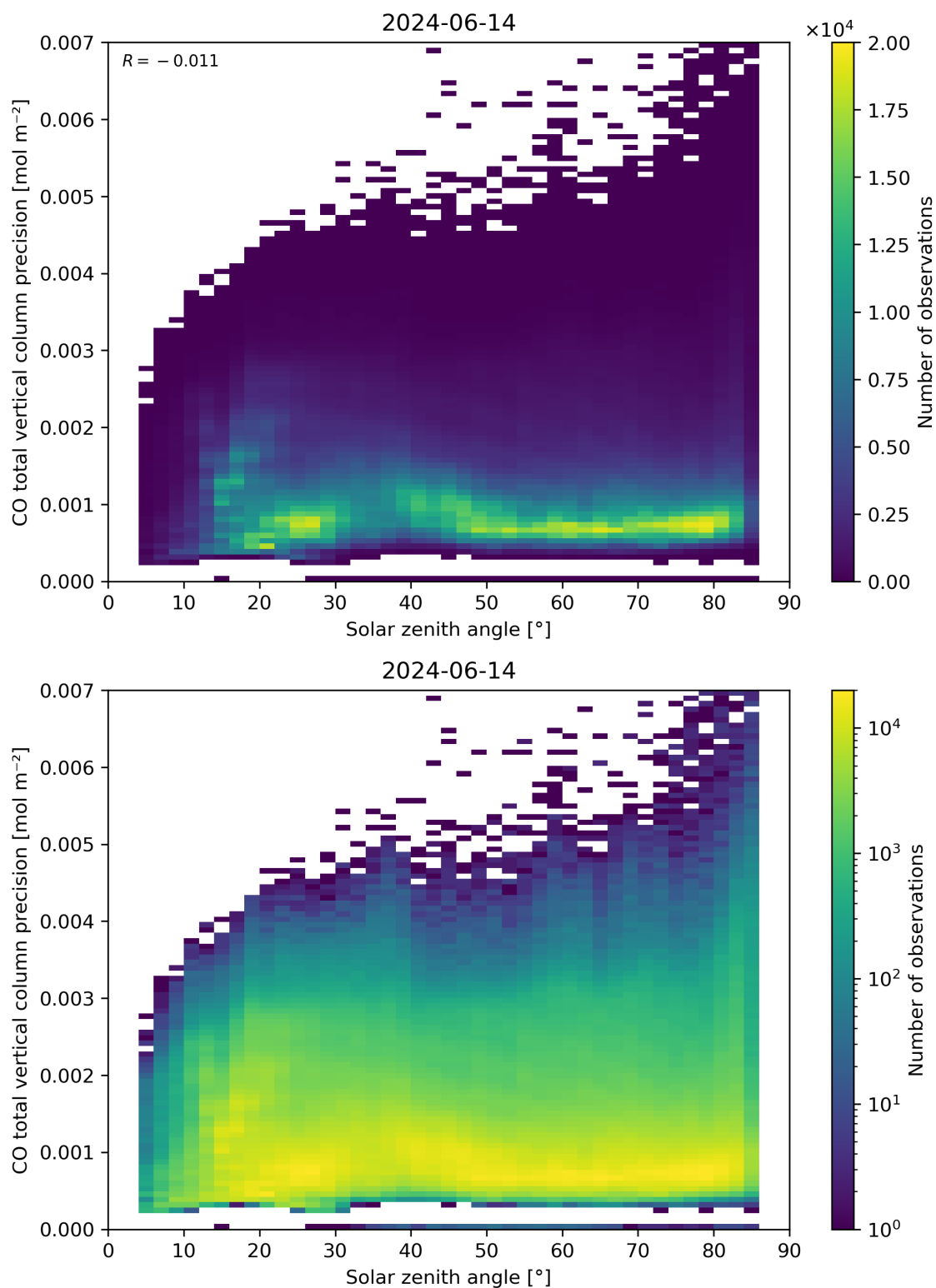
Figure 63: Scatter density plot of “Solar zenith angle” against “CO total vertical column precision” for 2024-06-13 to 2024-06-15.
