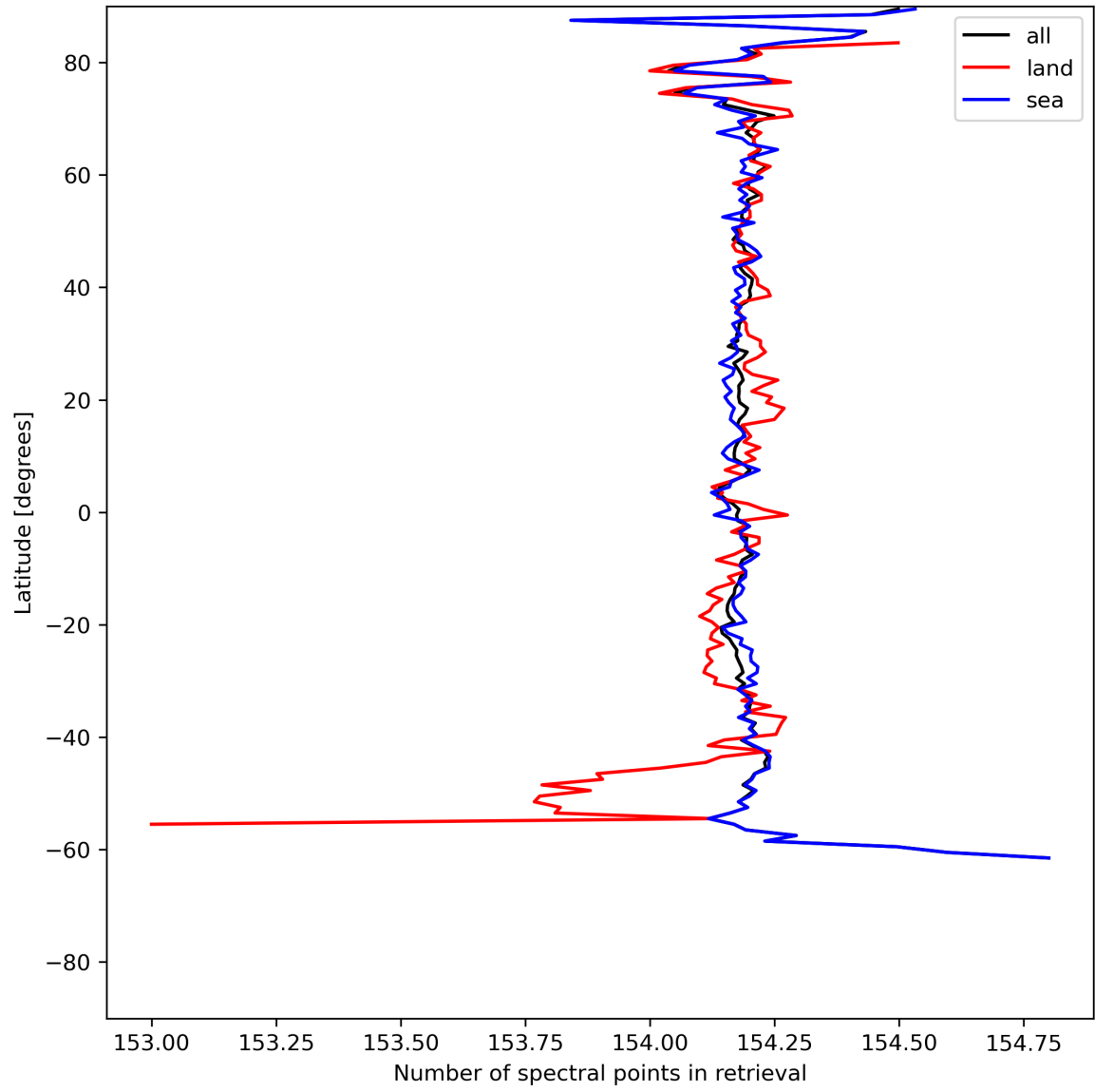
Figure 13: Zonal average of “Number of spectral points in retrieval” for 2024-06-13 to 2024-06-15.
