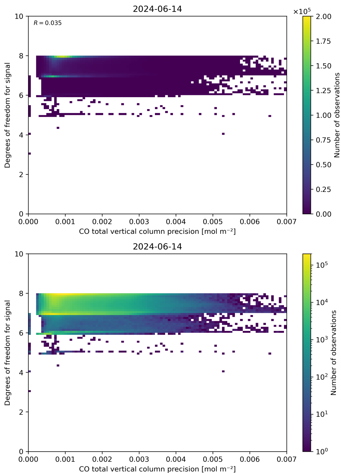
Figure 45: Scatter density plot of “CO total vertical column precision” against “Degrees of freedom for signal” for 2024-06-13 to 2024-06-15.
