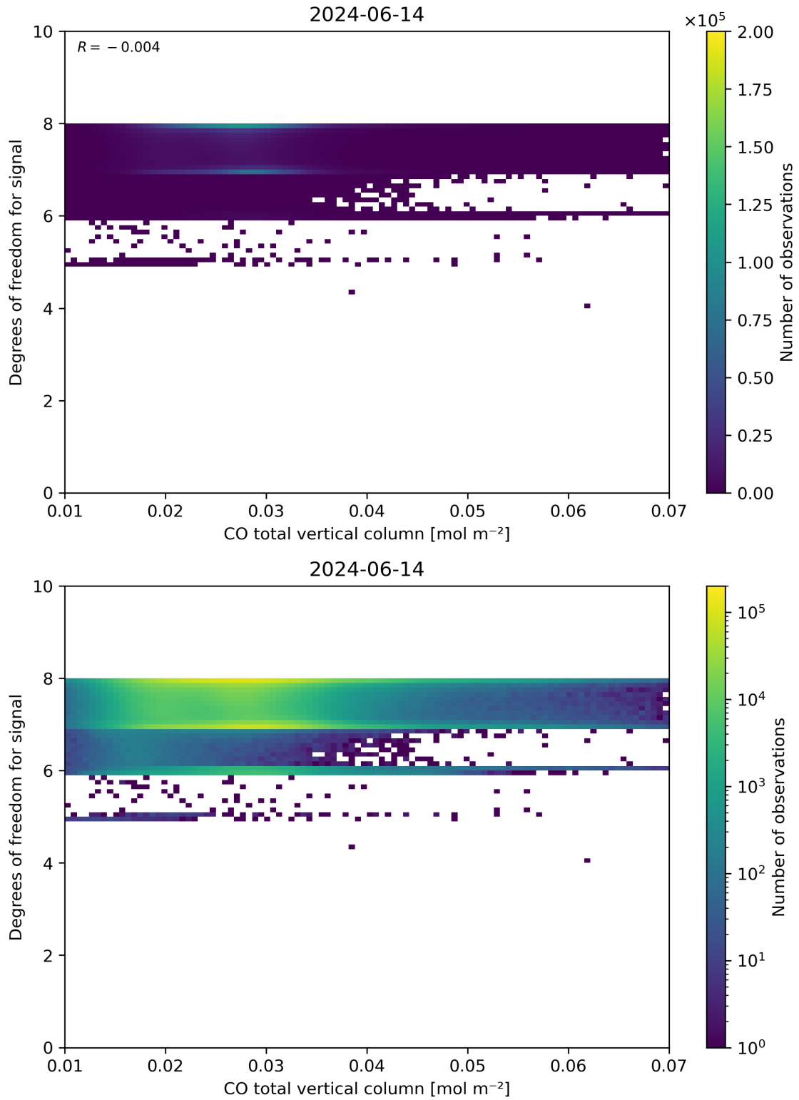
Figure 41: Scatter density plot of “CO total vertical column” against “Degrees of freedom for signal” for 2024-06-13 to 2024-06-15.
