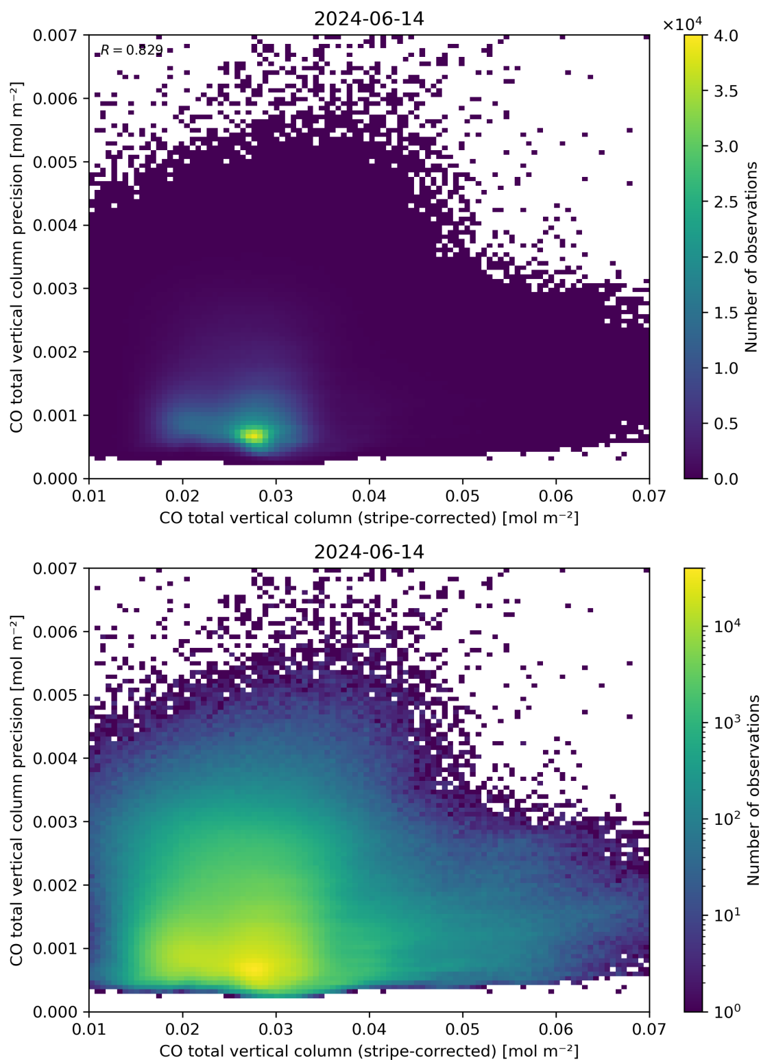
Figure 36: Scatter density plot of “CO total vertical column (stripe-corrected)” against “CO total vertical column precision” for 2024-06-13 to 2024-06-15.
