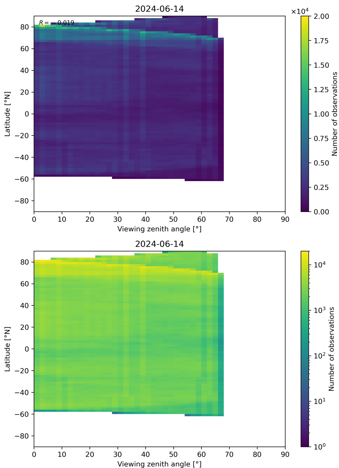
Figure 74: Scatter density plot of “Viewing zenith angle” against “Latitude” for 2024-06-13 to 2024-06-15.
