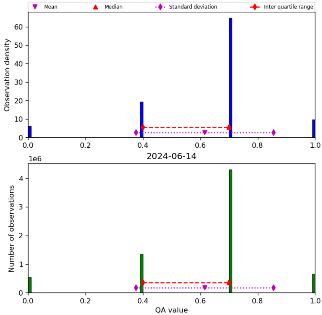
Figure 17: Histogram of “QA value” for 2024-06-13 to 2024-06-15
