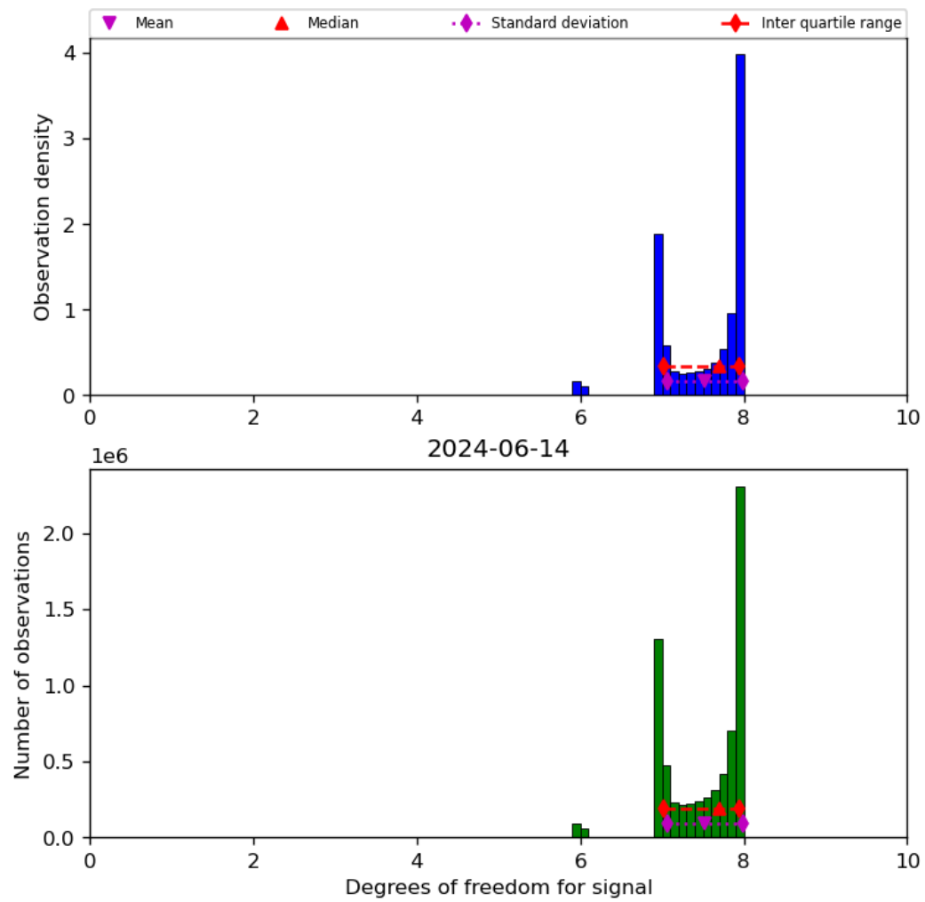
Figure 23: Histogram of “Degrees of freedom for signal” for 2024-06-13 to 2024-06-15
