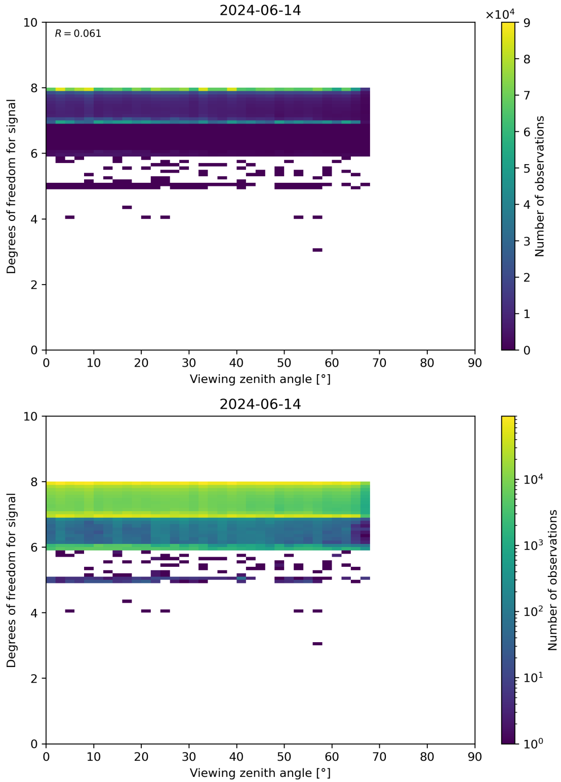
Figure 73: Scatter density plot of “Viewing zenith angle” against “Degrees of freedom for signal” for 2024-06-13 to 2024-06-15.
