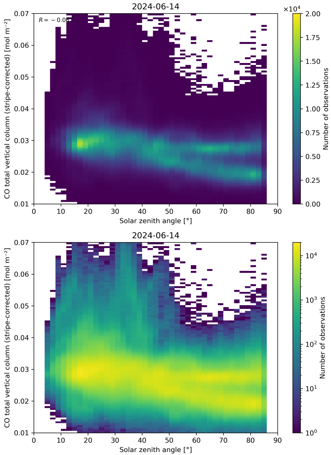
Figure 62: Scatter density plot of “Solar zenith angle” against “CO total vertical column (stripe-corrected)” for 2024-06-13 to 2024-06-15.
