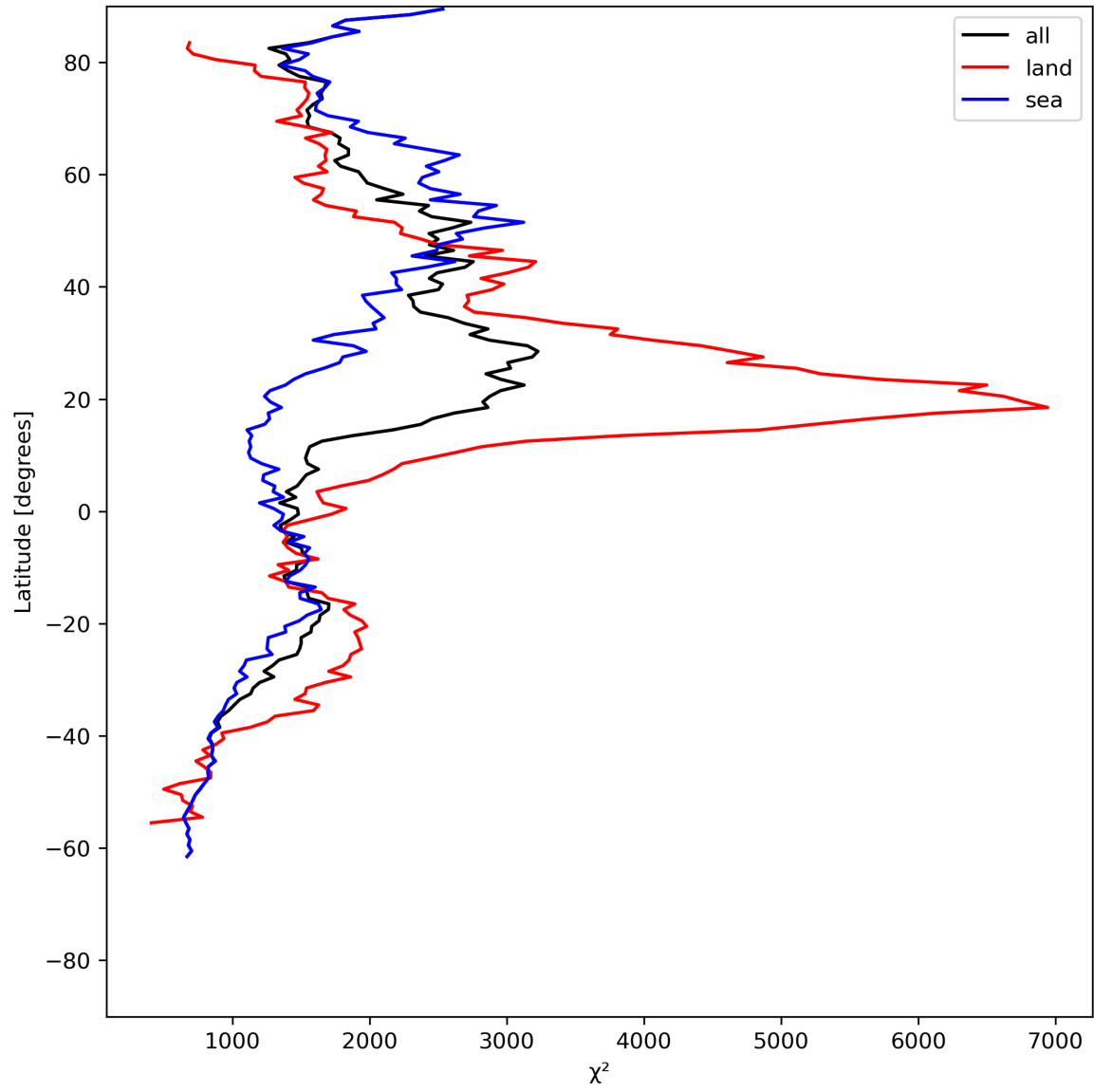
Figure 14: Zonal average of “ \chi^2 ” for 2024-06-13 to 2024-06-15.
