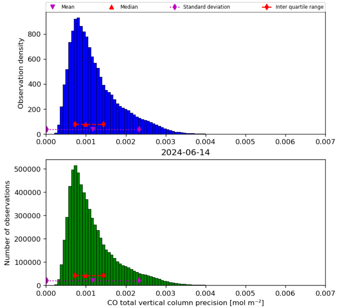
Figure 20: Histogram of “CO total vertical column precision” for 2024-06-13 to 2024-06-15
