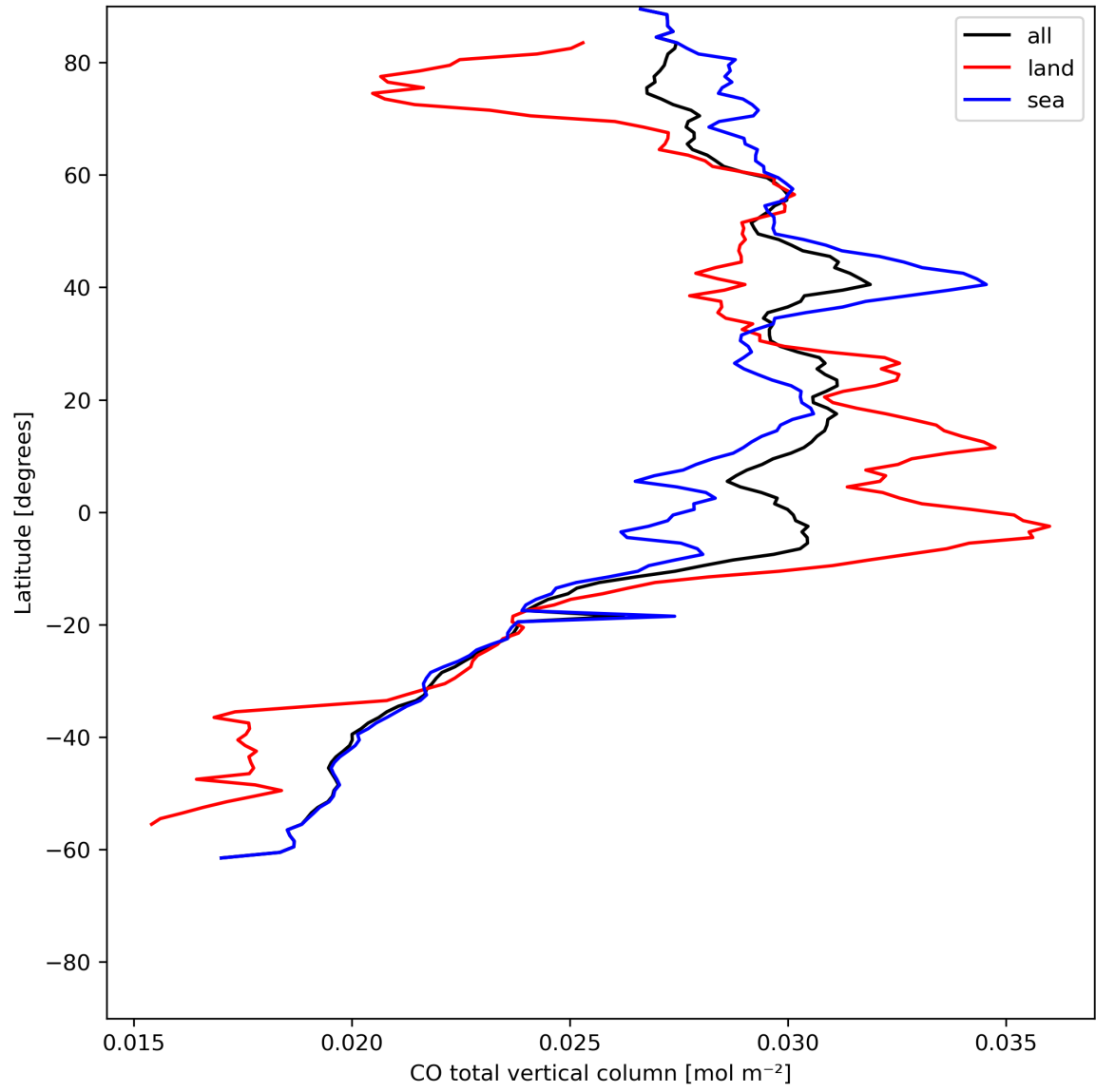
Figure 10: Zonal average of “CO total vertical column” for 2024-06-13 to 2024-06-15.
