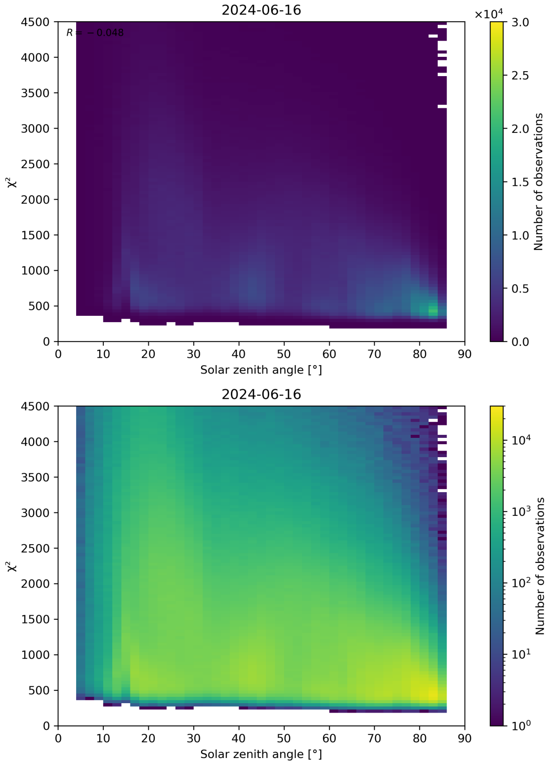
Figure 64: Scatter density plot of “Solar zenith angle” against “ \chi^2 ” for 2024-06-15 to 2024-06-17.
