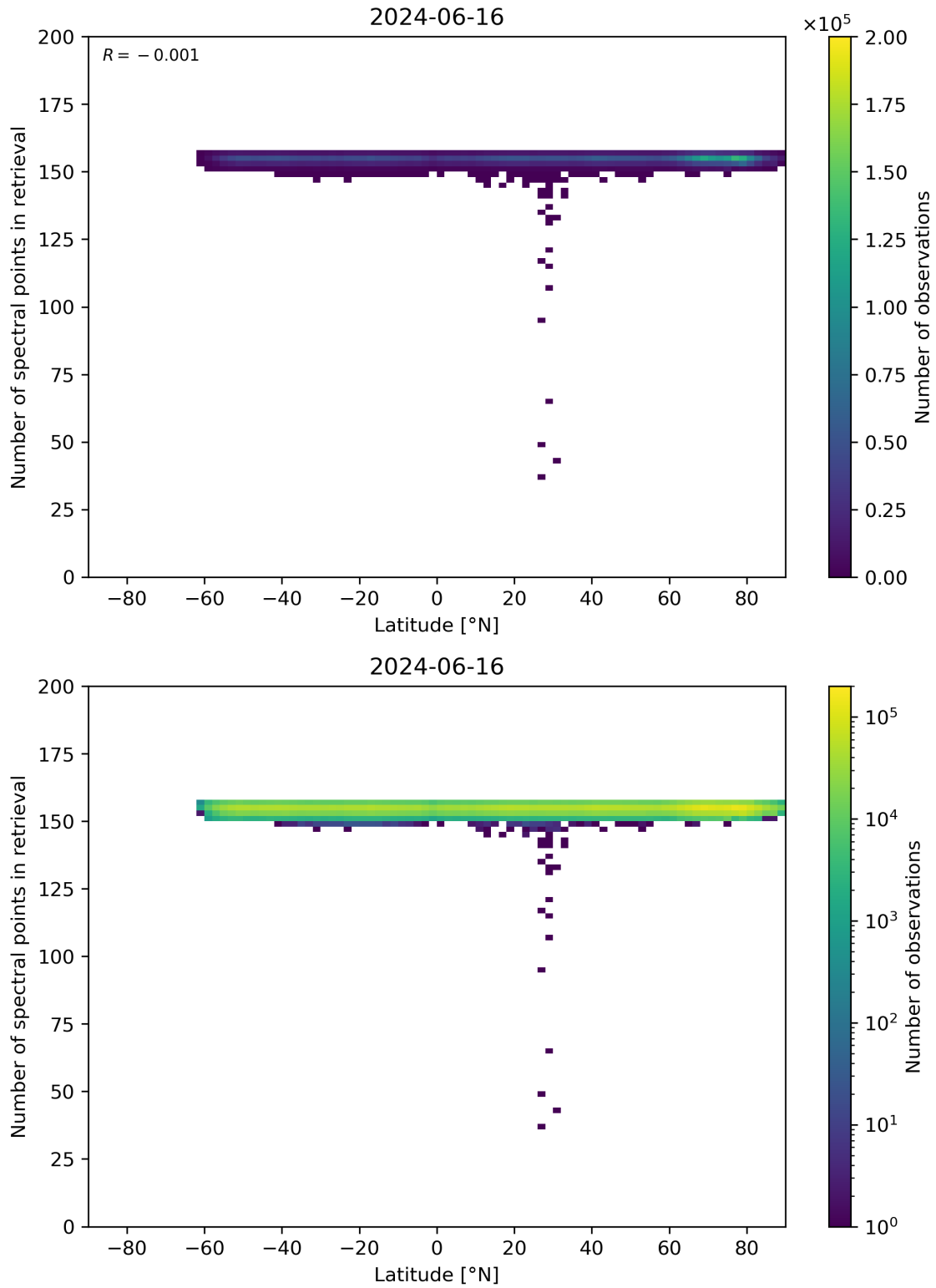
Figure 57: Scatter density plot of “Latitude” against “Number of spectral points in retrieval” for 2024-06-15 to 2024-06-17.
