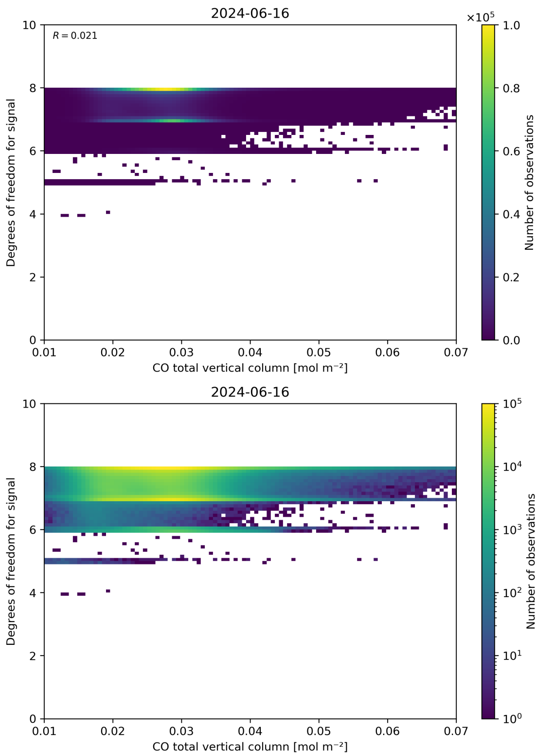
Figure 41: Scatter density plot of “CO total vertical column” against “Degrees of freedom for signal” for 2024-06-15 to 2024-06-17.
