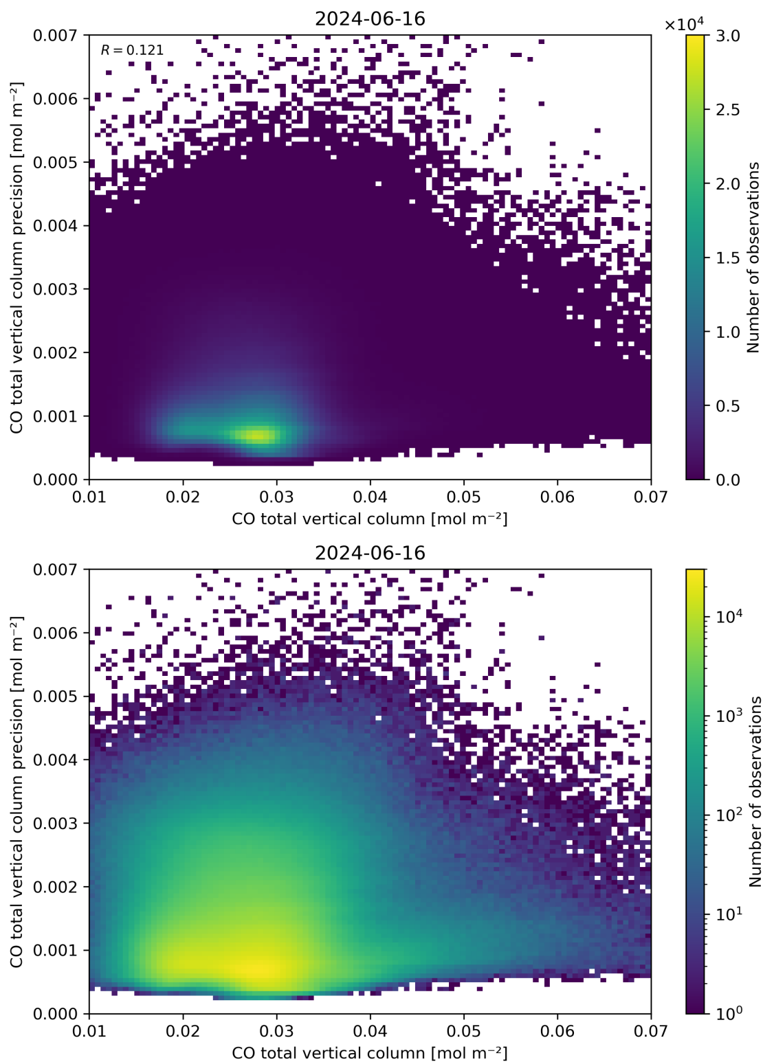
Figure 34: Scatter density plot of “CO total vertical column” against “CO total vertical column precision” for 2024-06-15 to 2024-06-17.
