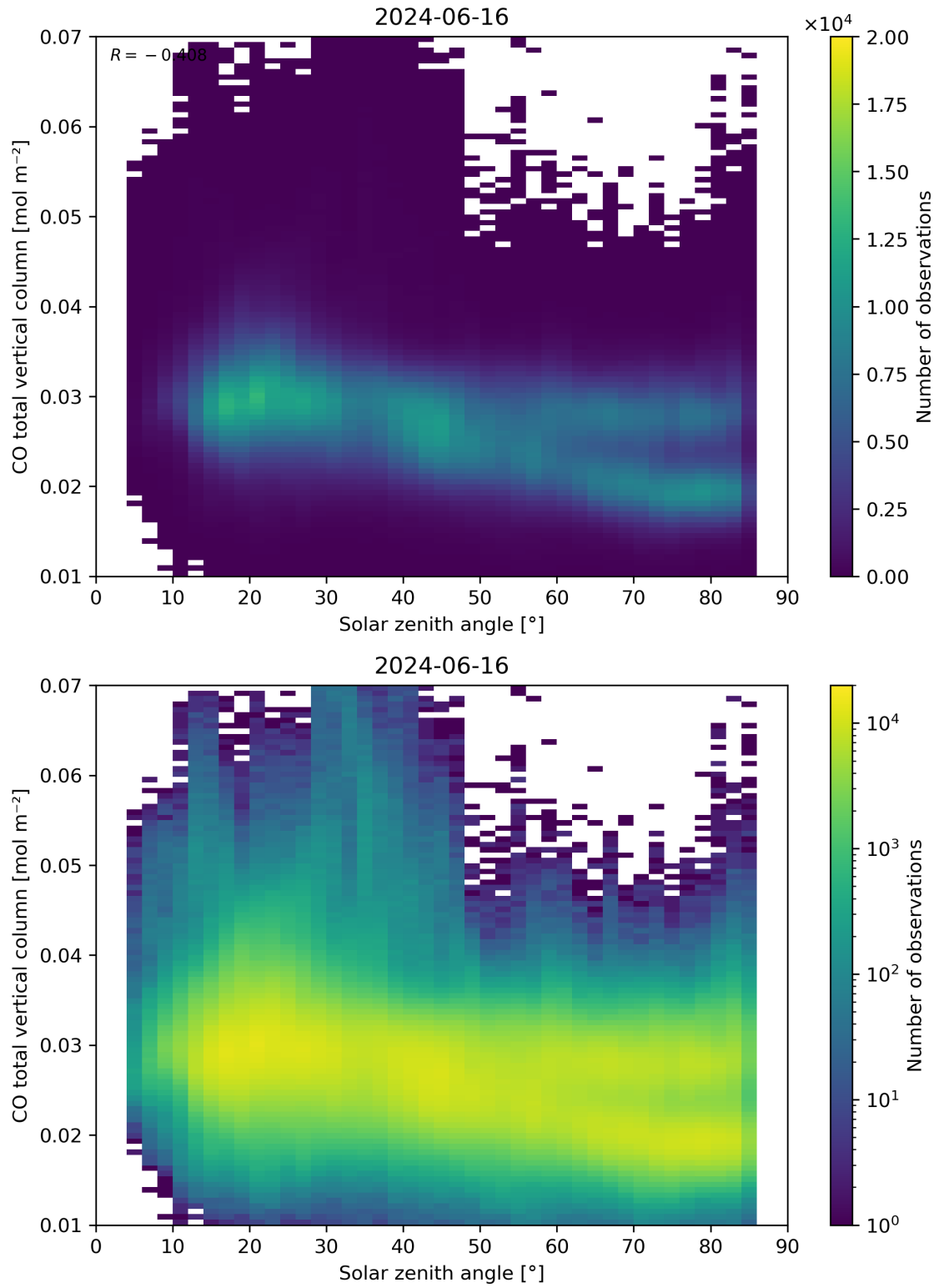
Figure 61: Scatter density plot of “Solar zenith angle” against “CO total vertical column” for 2024-06-15 to 2024-06-17.
