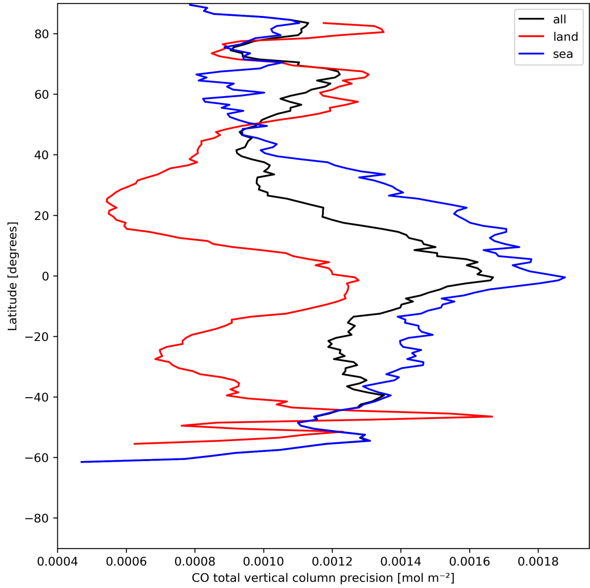
Figure 12: Zonal average of “CO total vertical column precision” for 2024-06-15 to 2024-06-17.
