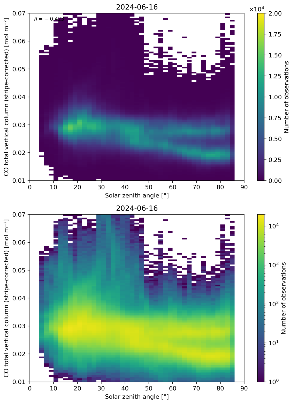
Figure 62: Scatter density plot of “Solar zenith angle” against “CO total vertical column (stripe-corrected)” for 2024-06-15 to 2024-06-17.
