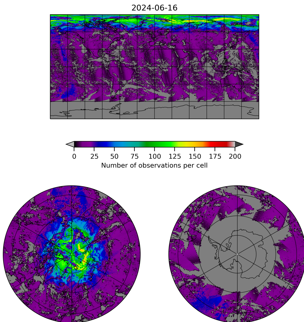
Figure 8: Map of the number of observations for 2024-06-15 to 2024-06-17
