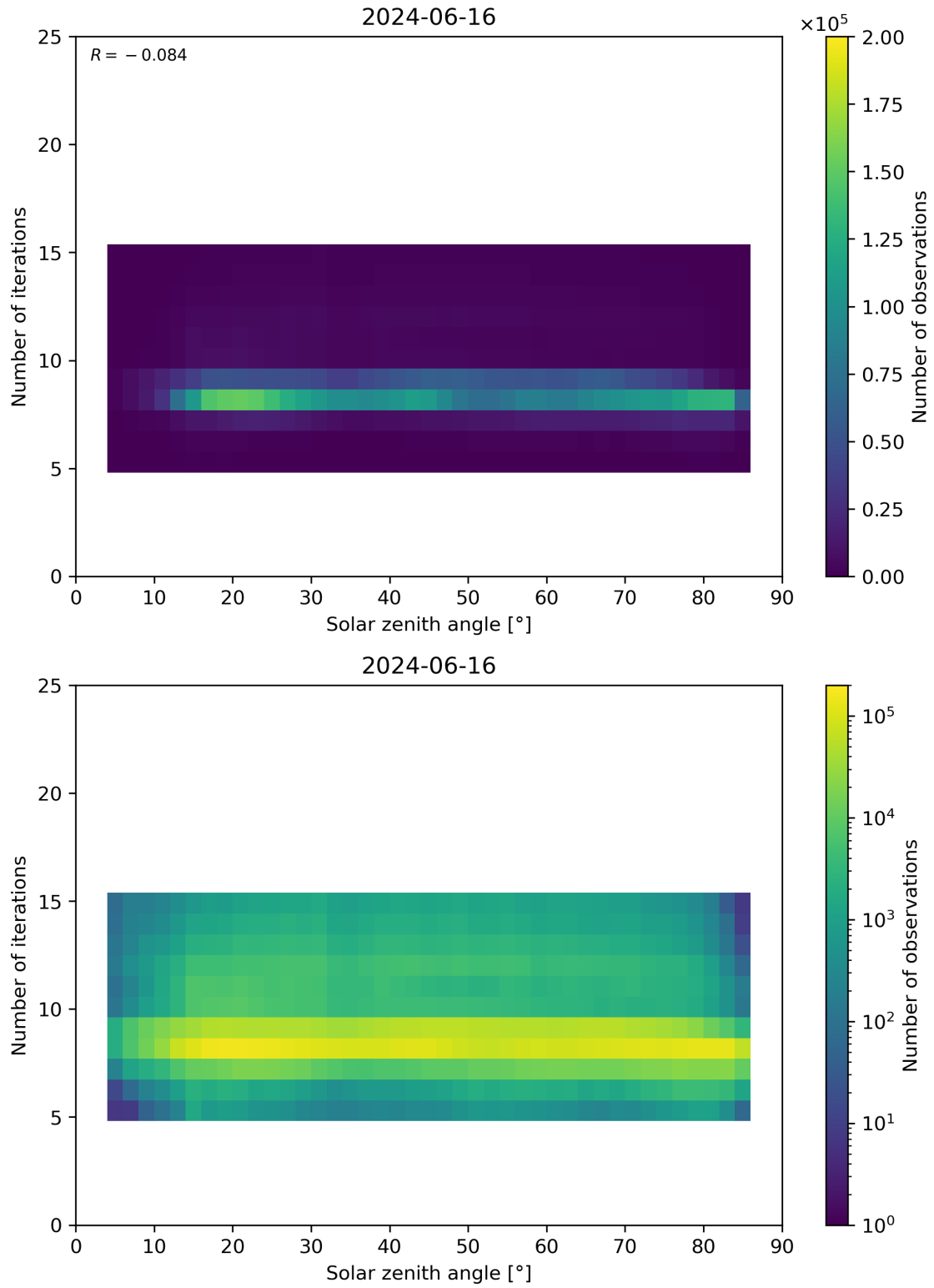
Figure 67: Scatter density plot of “Solar zenith angle” against “Number of iterations” for 2024-06-15 to 2024-06-17.
