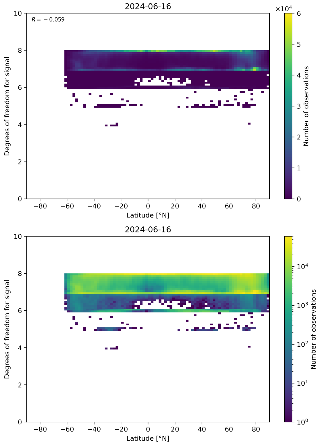
Figure 55: Scatter density plot of “Latitude” against “Degrees of freedom for signal” for 2024-06-15 to 2024-06-17.
