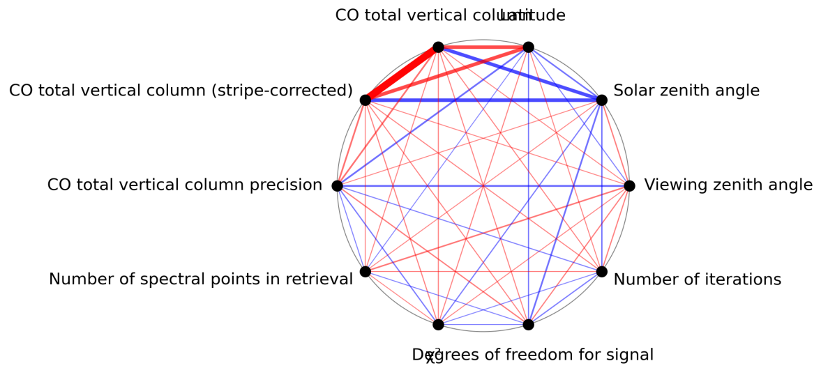
Figure 1: Map of correlation graph for 2024-06-15 to 2024-06-17.
