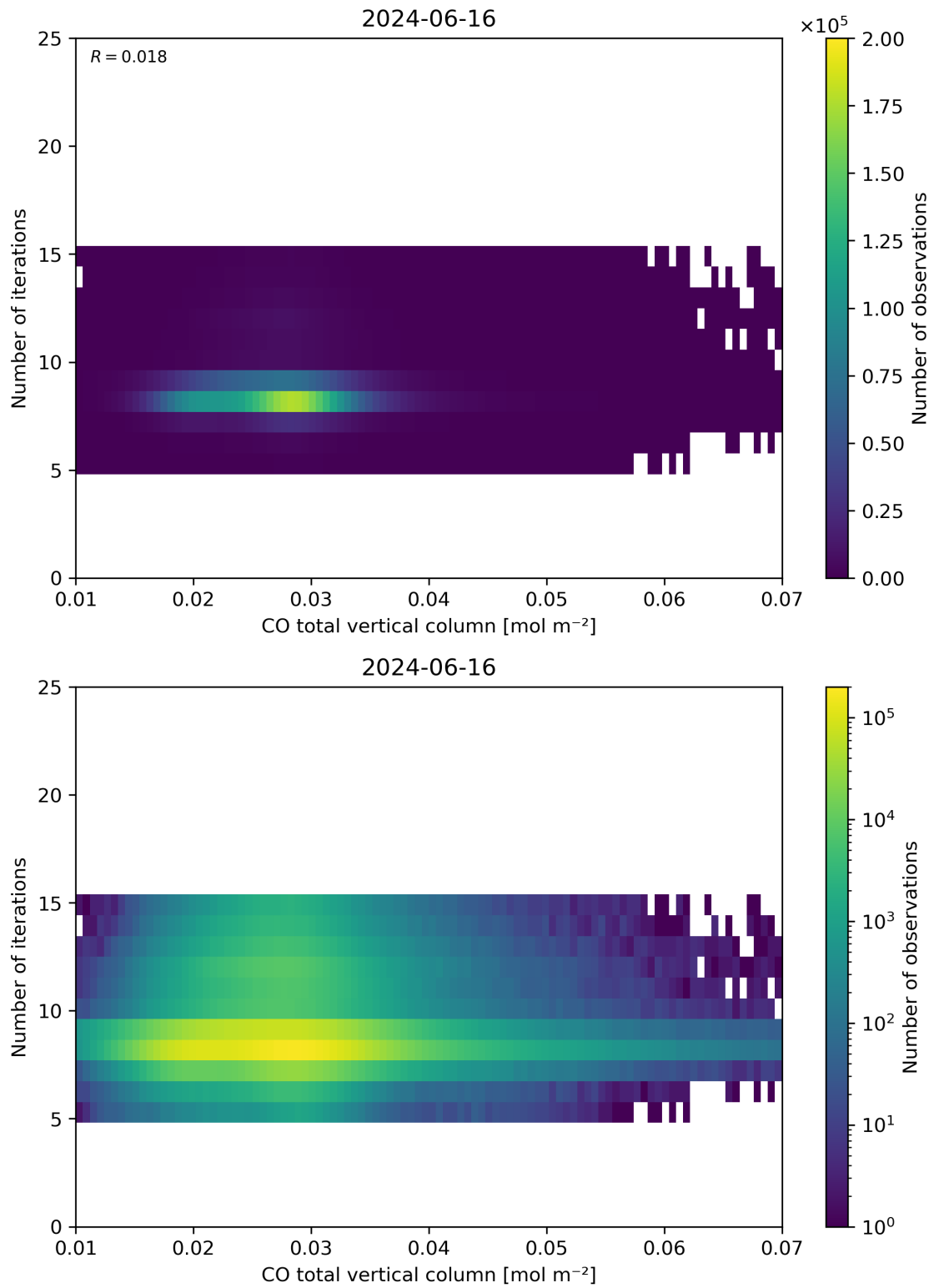
Figure 42: Scatter density plot of “CO total vertical column” against “Number of iterations” for 2024-06-15 to 2024-06-17.
