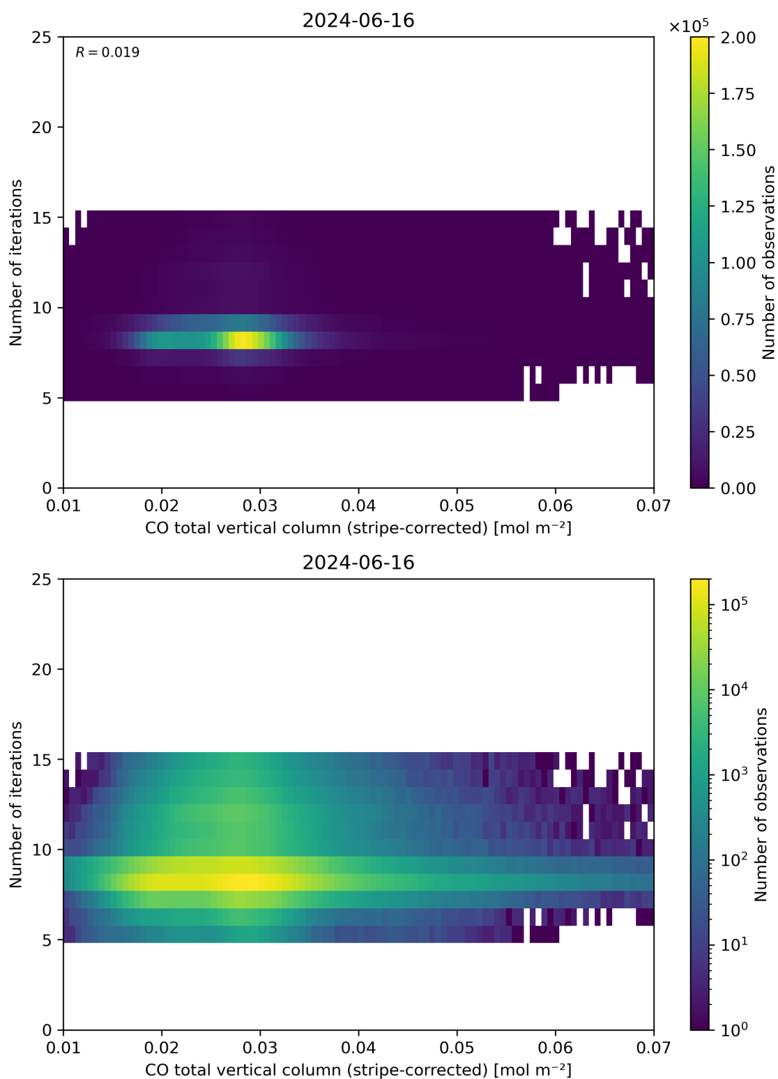
Figure 39: Scatter density plot of “CO total vertical column (stripe-corrected)” against “Number of iterations” for 2024-06-15 to 2024-06-17.
