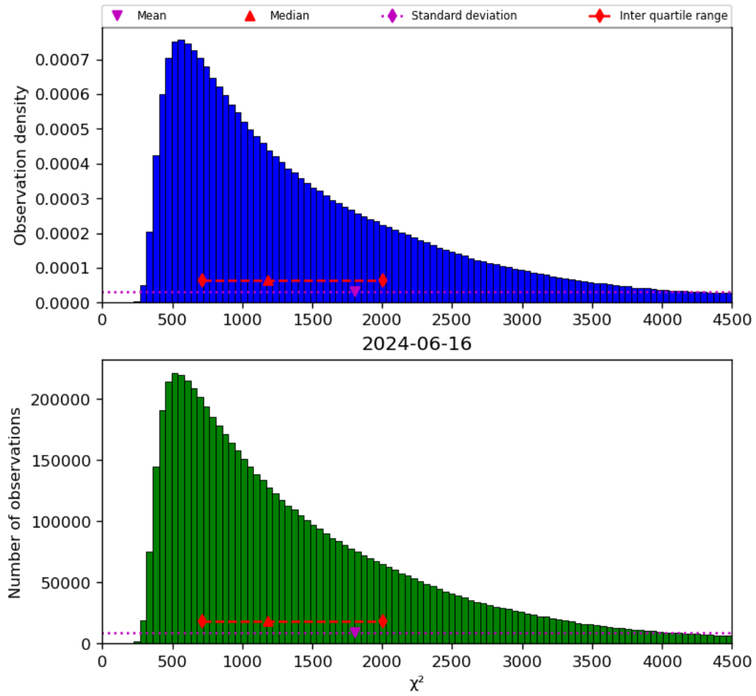
Figure 22: Histogram of “ \chi^2 ” for 2024-06-15 to 2024-06-17
