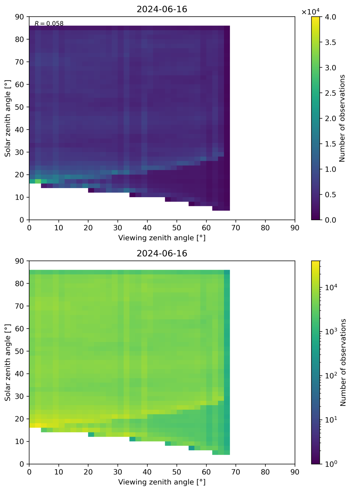
Figure 77: Scatter density plot of “Viewing zenith angle” against “Solar zenith angle” for 2024-06-15 to 2024-06-17.
