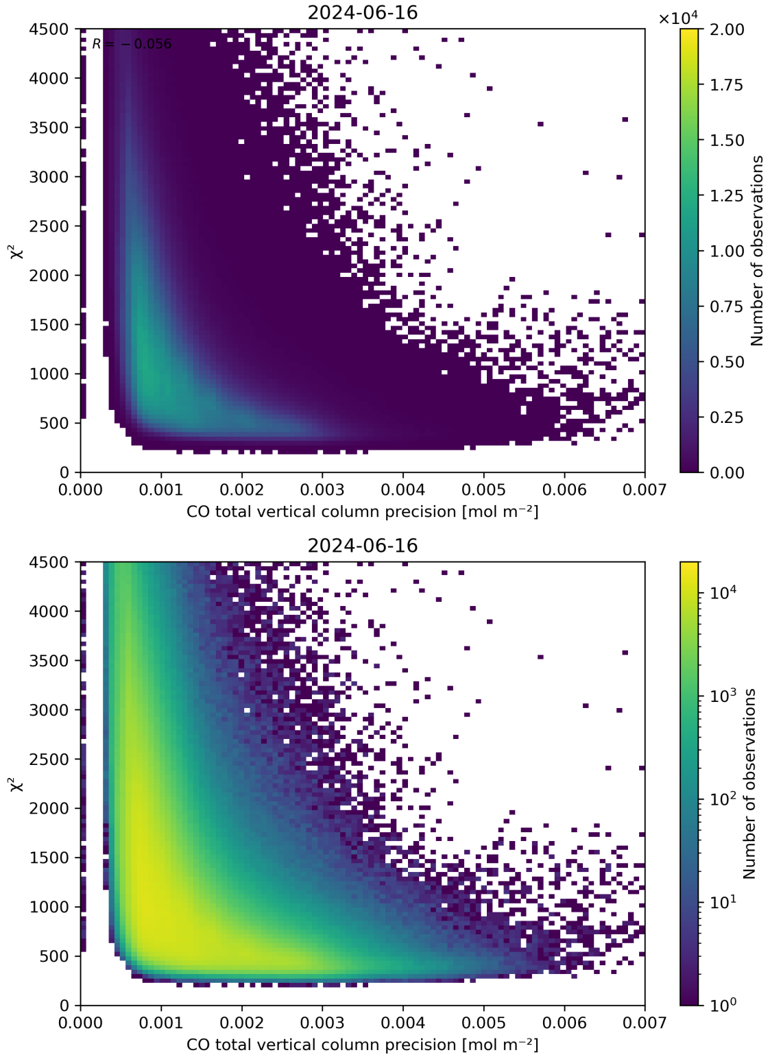
Figure 44: Scatter density plot of “CO total vertical column precision” against “ \chi^2 ” for 2024-06-15 to 2024-06-17.
