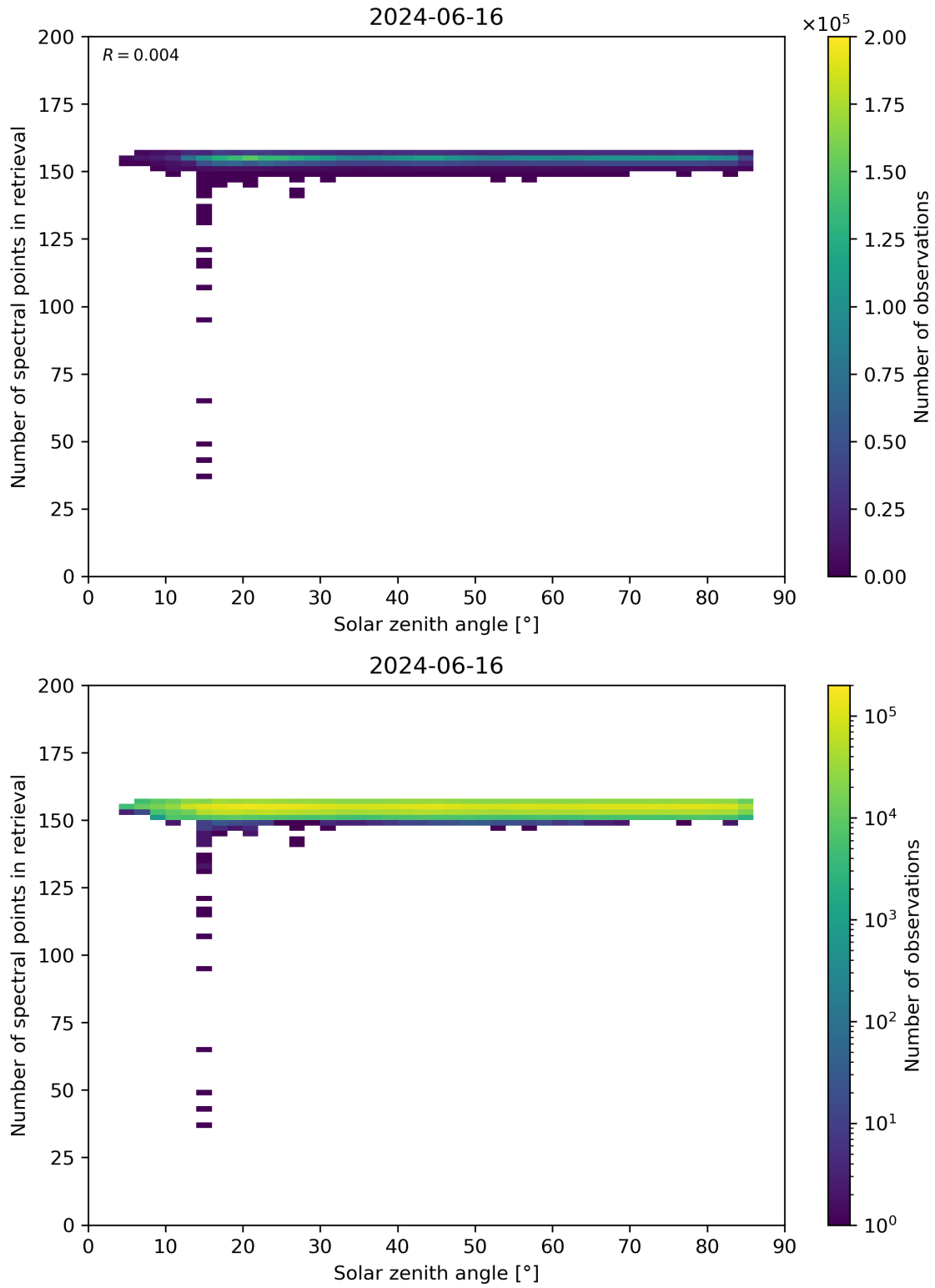
Figure 68: Scatter density plot of “Solar zenith angle” against “Number of spectral points in retrieval” for 2024-06-15 to 2024-06-17.
