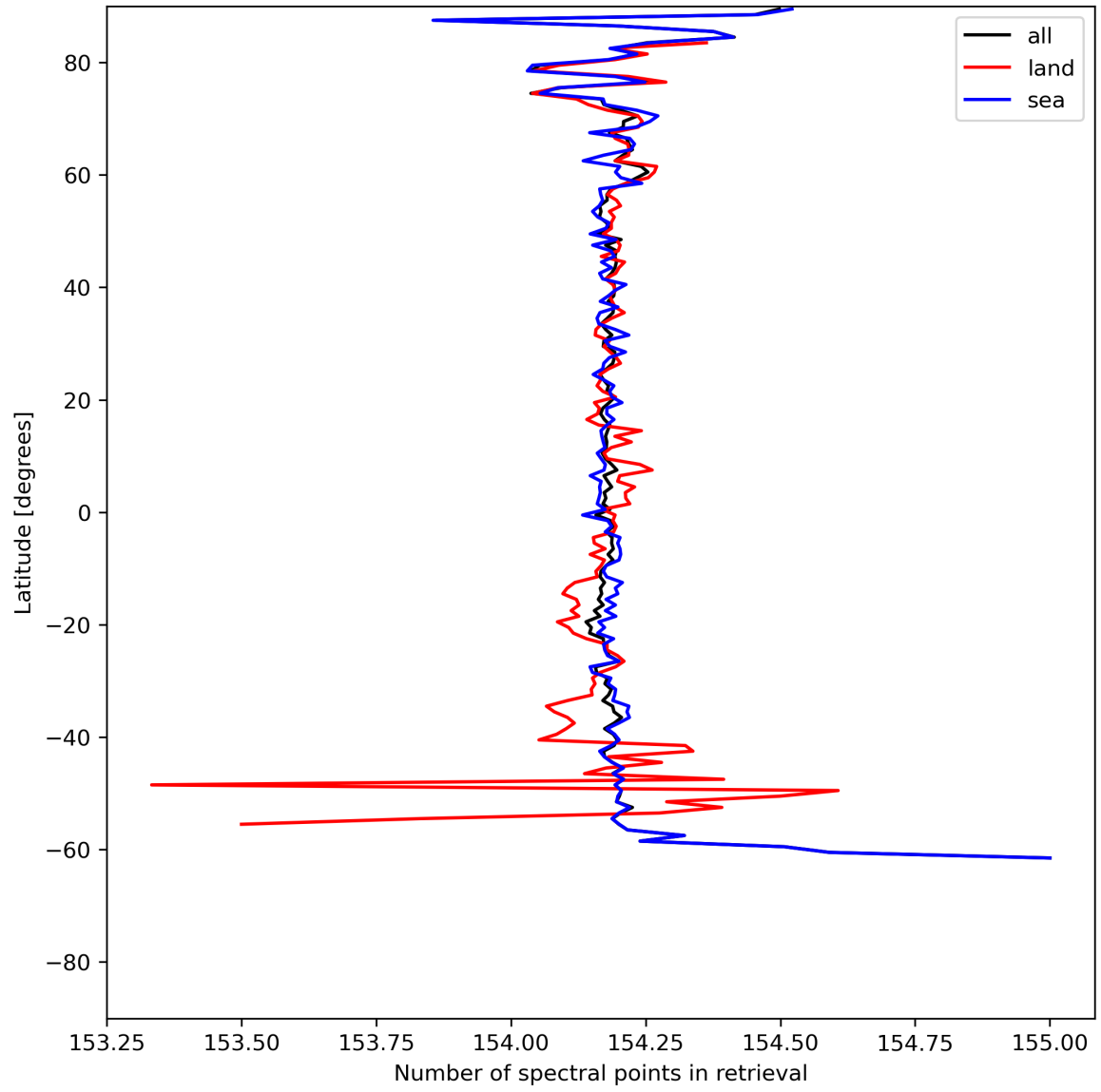
Figure 13: Zonal average of “Number of spectral points in retrieval” for 2024-06-15 to 2024-06-17.
