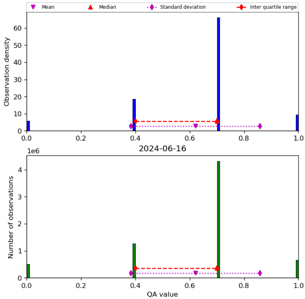
Figure 17: Histogram of “QA value” for 2024-06-15 to 2024-06-17
