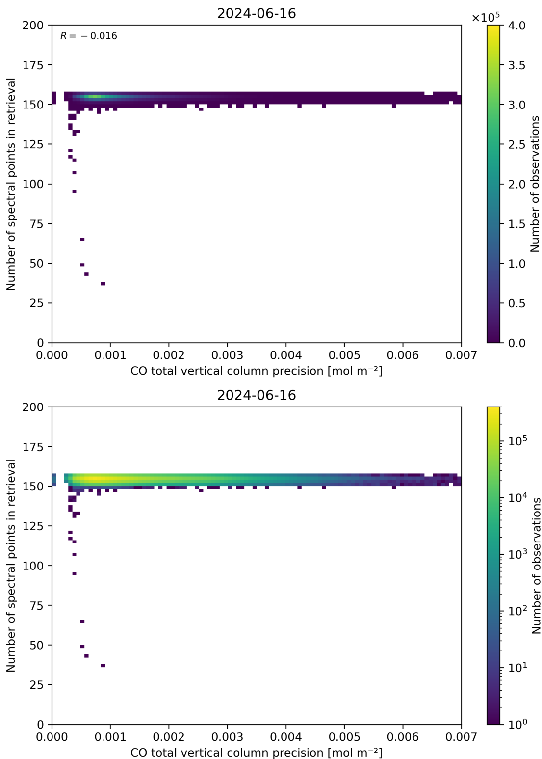
Figure 47: Scatter density plot of “CO total vertical column precision” against “Number of spectral points in retrieval” for 2024-06-15 to 2024-06-17.
