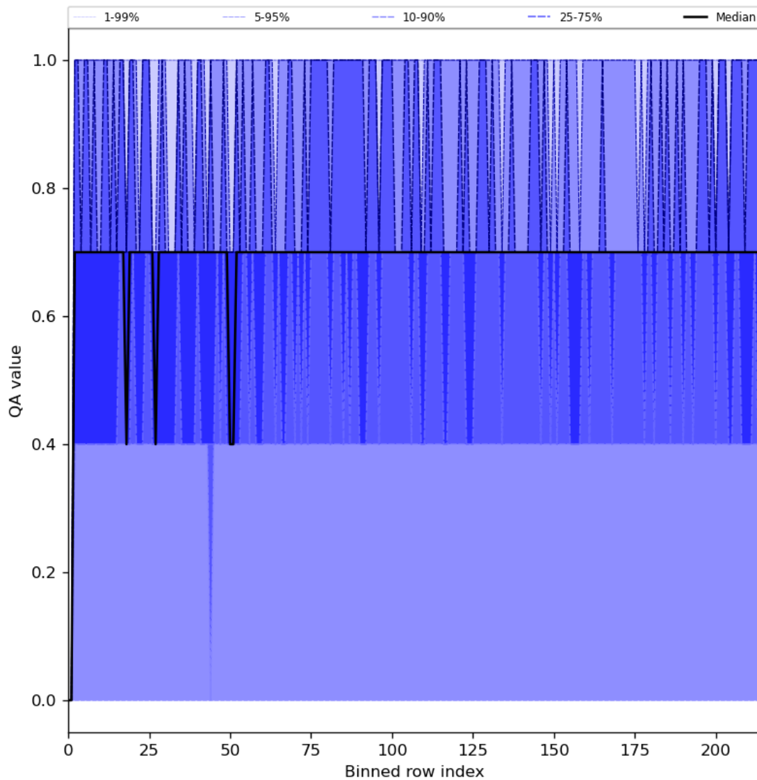
Figure 25: Along track statistics of “QA value” for 2024-06-15 to 2024-06-17
