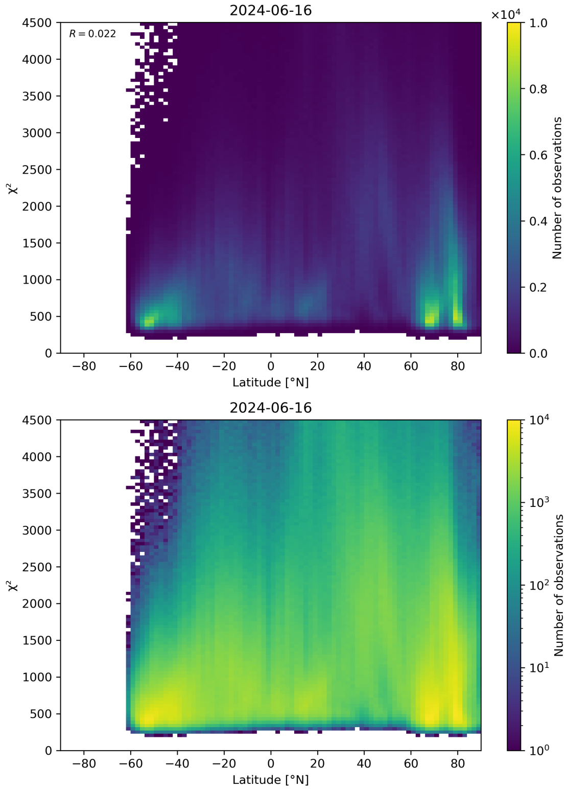
Figure 54: Scatter density plot of “Latitude” against “ \chi^2 ” for 2024-06-15 to 2024-06-17.
