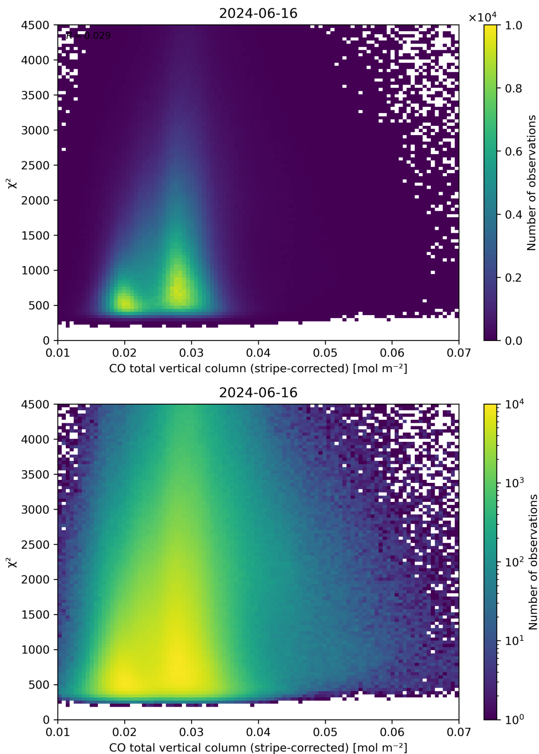
Figure 37: Scatter density plot of “CO total vertical column (stripe-corrected)” against “ \chi^2 ” for 2024-06-15 to 2024-06-17.
