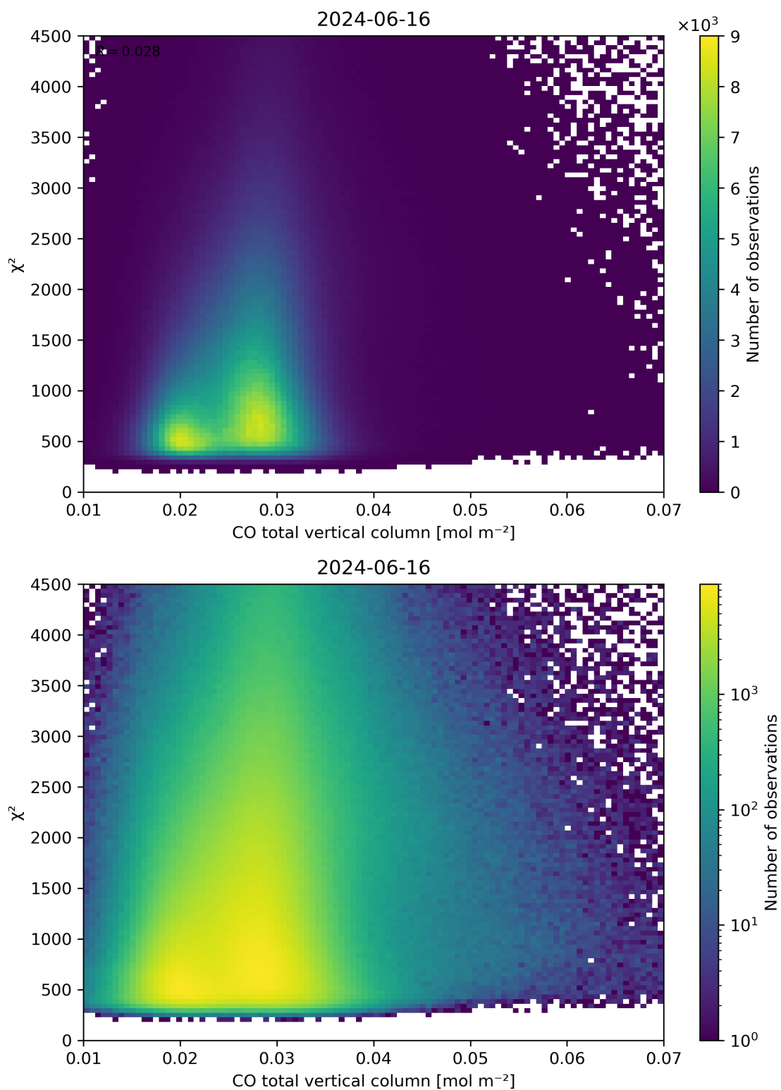
Figure 35: Scatter density plot of “CO total vertical column” against “ \chi^2 ” for 2024-06-15 to 2024-06-17.
