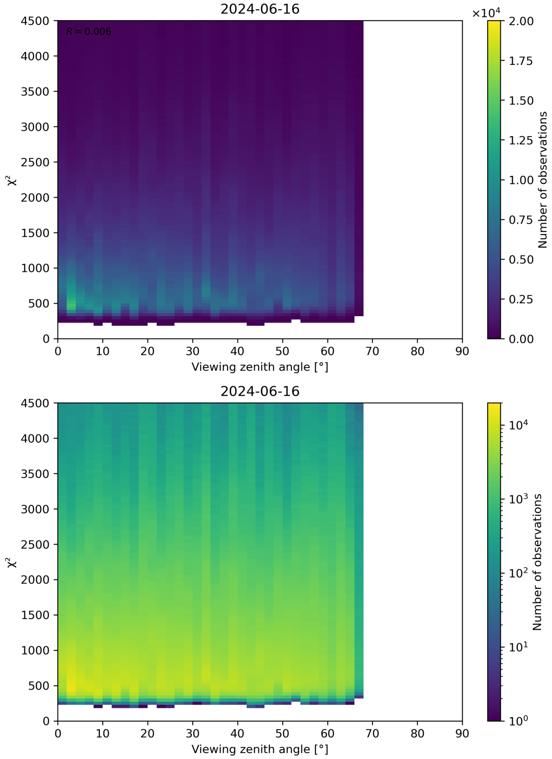
Figure 72: Scatter density plot of “Viewing zenith angle” against “ \chi^2 ” for 2024-06-15 to 2024-06-17.
