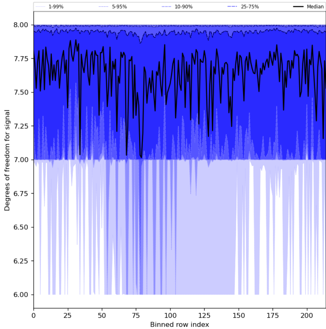
Figure 31: Along track statistics of “Degrees of freedom for signal” for 2024-06-15 to 2024-06-17
