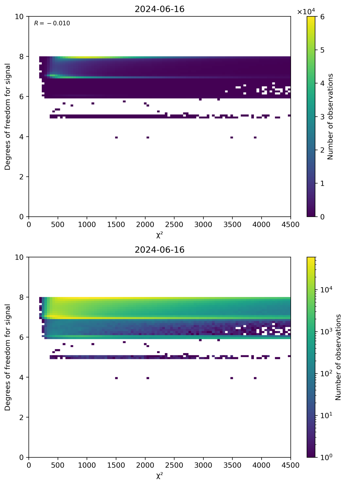
Figure 48: Scatter density plot of “ \chi^2 ” against “Degrees of freedom for signal” for 2024-06-15 to 2024-06-17.
