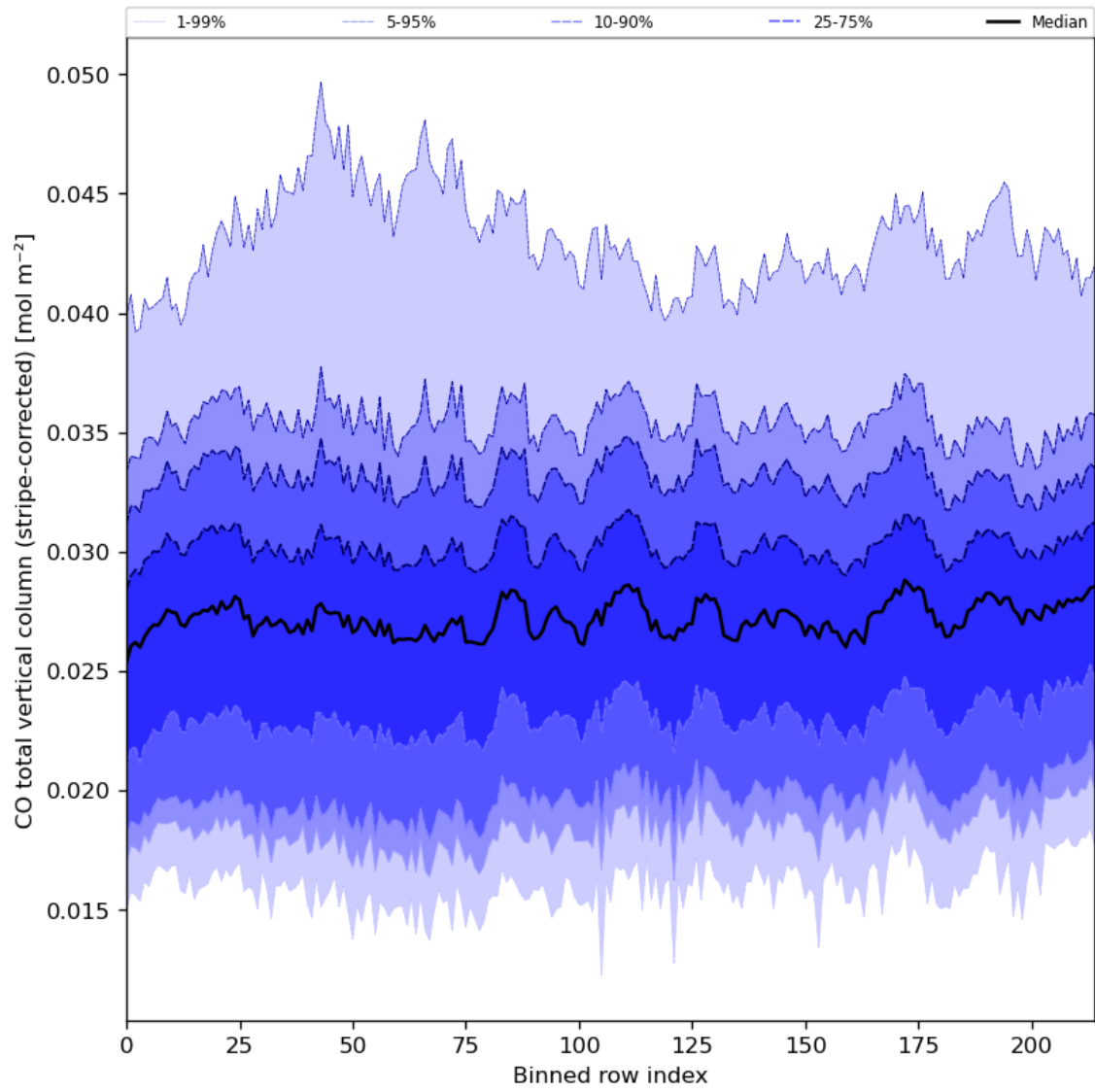
Figure 27: Along track statistics of “CO total vertical column (stripe-corrected)” for 2024-06-15 to 2024-06-17
