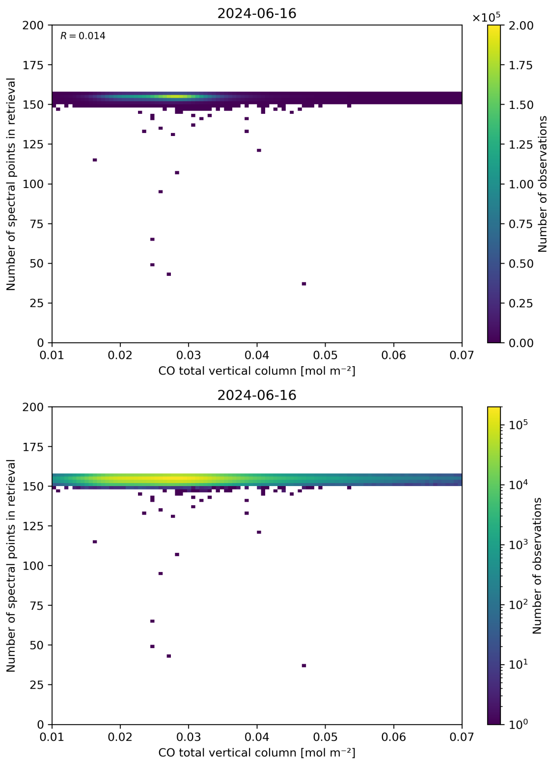
Figure 43: Scatter density plot of “CO total vertical column” against “Number of spectral points in retrieval” for 2024-06-15 to 2024-06-17.
