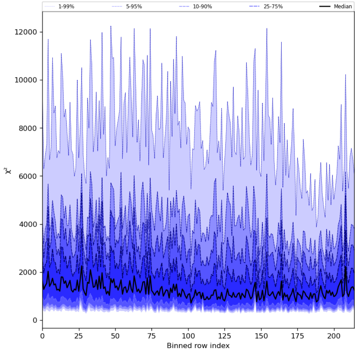
Figure 30: Along track statistics of “ \chi^2 ” for 2024-06-15 to 2024-06-17
