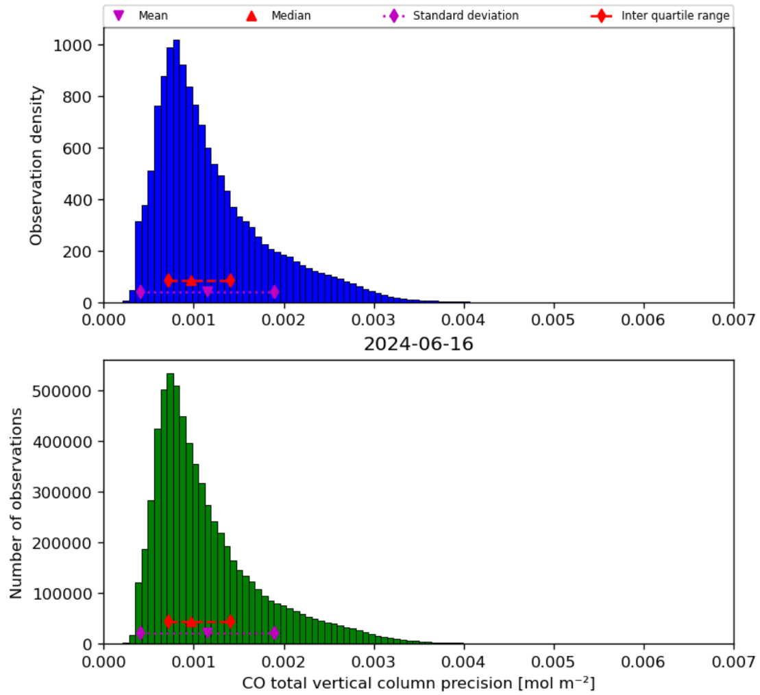
Figure 20: Histogram of “CO total vertical column precision” for 2024-06-15 to 2024-06-17
