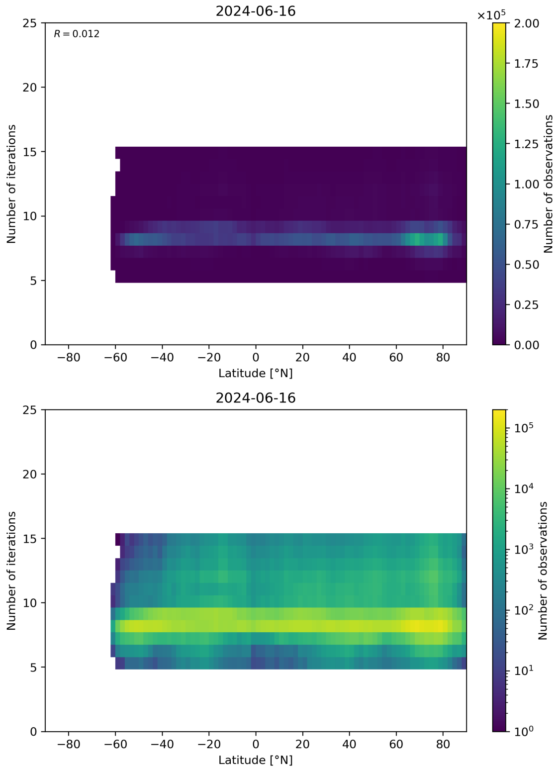
Figure 56: Scatter density plot of “Latitude” against “Number of iterations” for 2024-06-15 to 2024-06-17.
