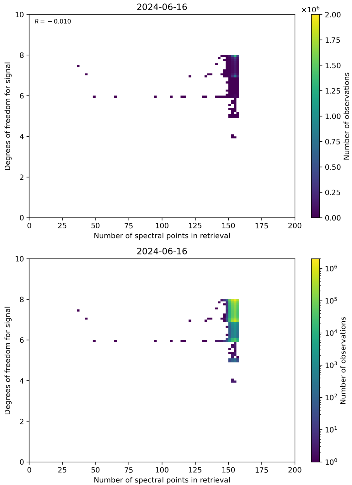
Figure 59: Scatter density plot of “Number of spectral points in retrieval” against “Degrees of freedom for signal” for 2024-06-15 to 2024-06-17.
