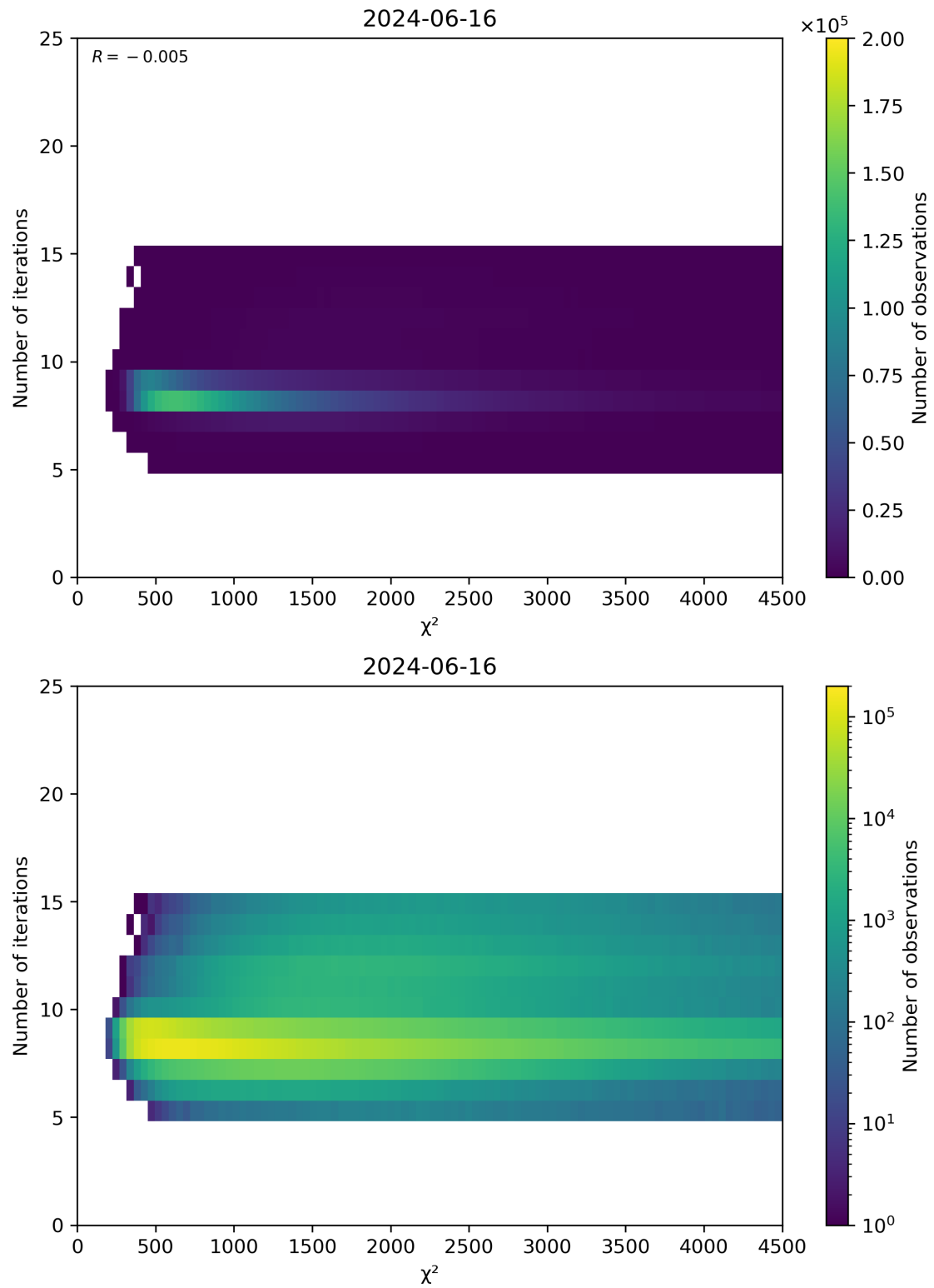
Figure 49: Scatter density plot of “ \chi^2 ” against “Number of iterations” for 2024-06-15 to 2024-06-17.
