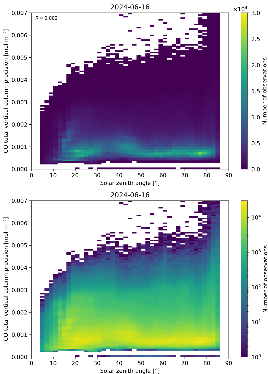
Figure 63: Scatter density plot of “Solar zenith angle” against “CO total vertical column precision” for 2024-06-15 to 2024-06-17.
