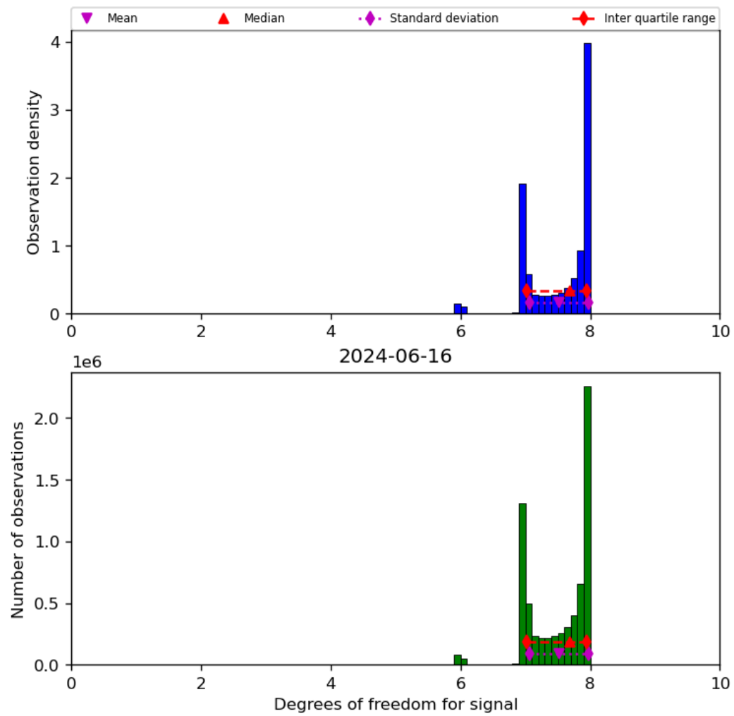
Figure 23: Histogram of “Degrees of freedom for signal” for 2024-06-15 to 2024-06-17
