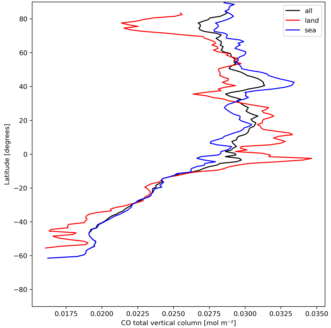
Figure 10: Zonal average of “CO total vertical column” for 2024-06-15 to 2024-06-17.
