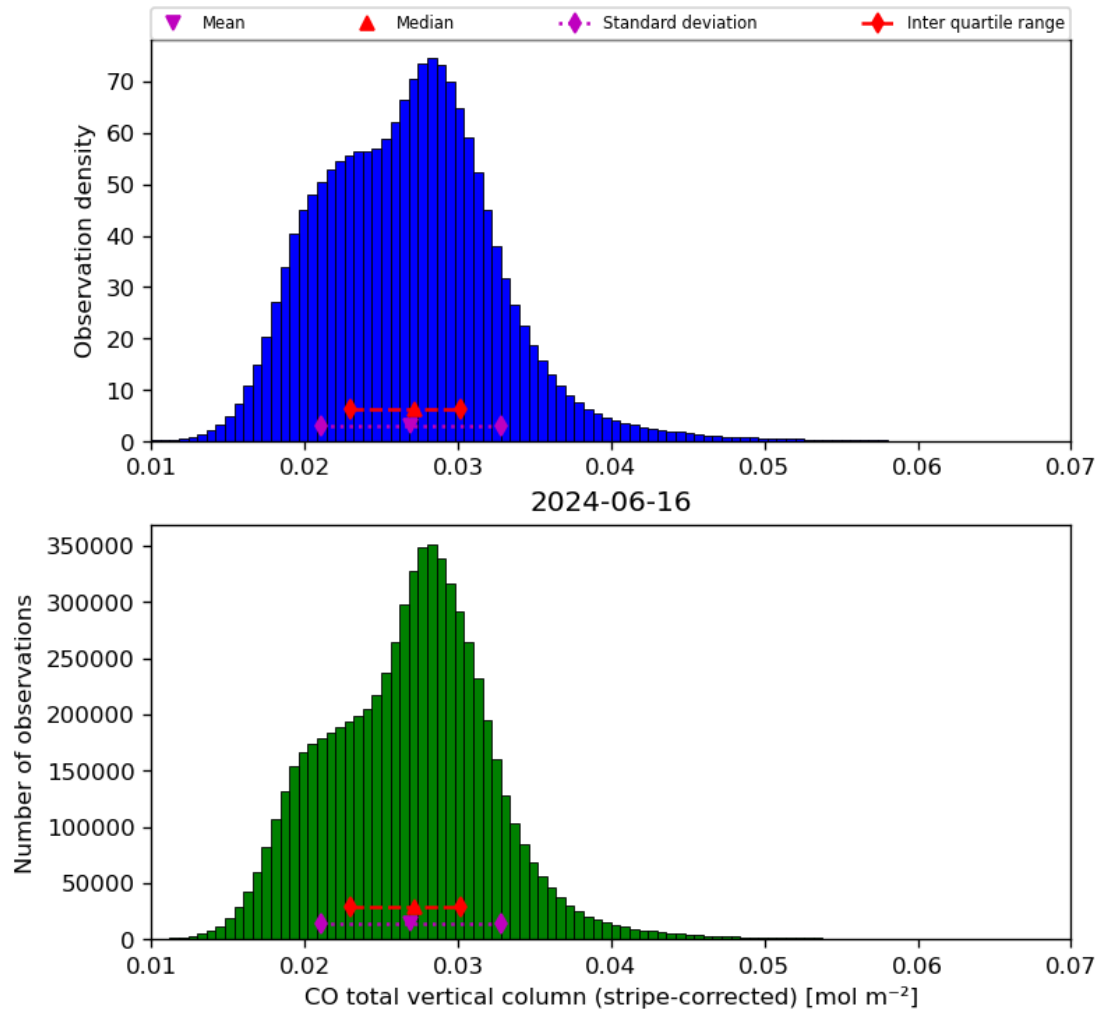
Figure 19: Histogram of “CO total vertical column (stripe-corrected)” for 2024-06-15 to 2024-06-17
