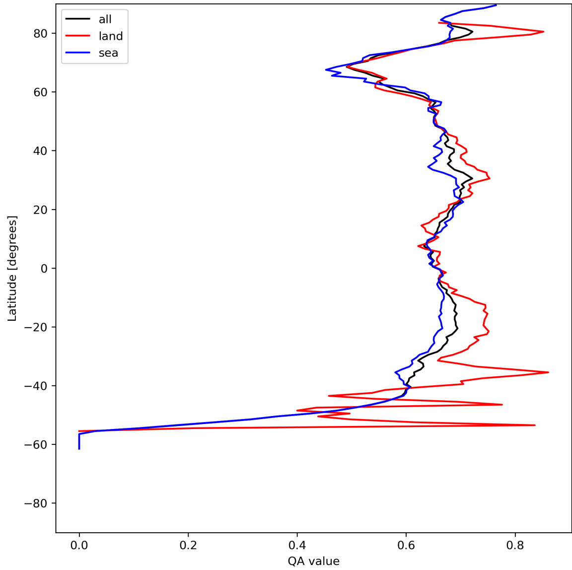
Figure 9: Zonal average of “QA value” for 2024-06-15 to 2024-06-17.
