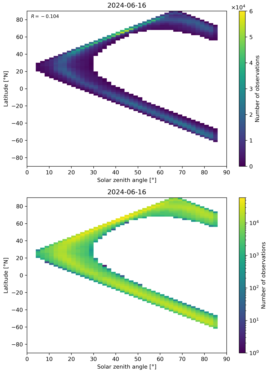
Figure 66: Scatter density plot of “Solar zenith angle” against “Latitude” for 2024-06-15 to 2024-06-17.
