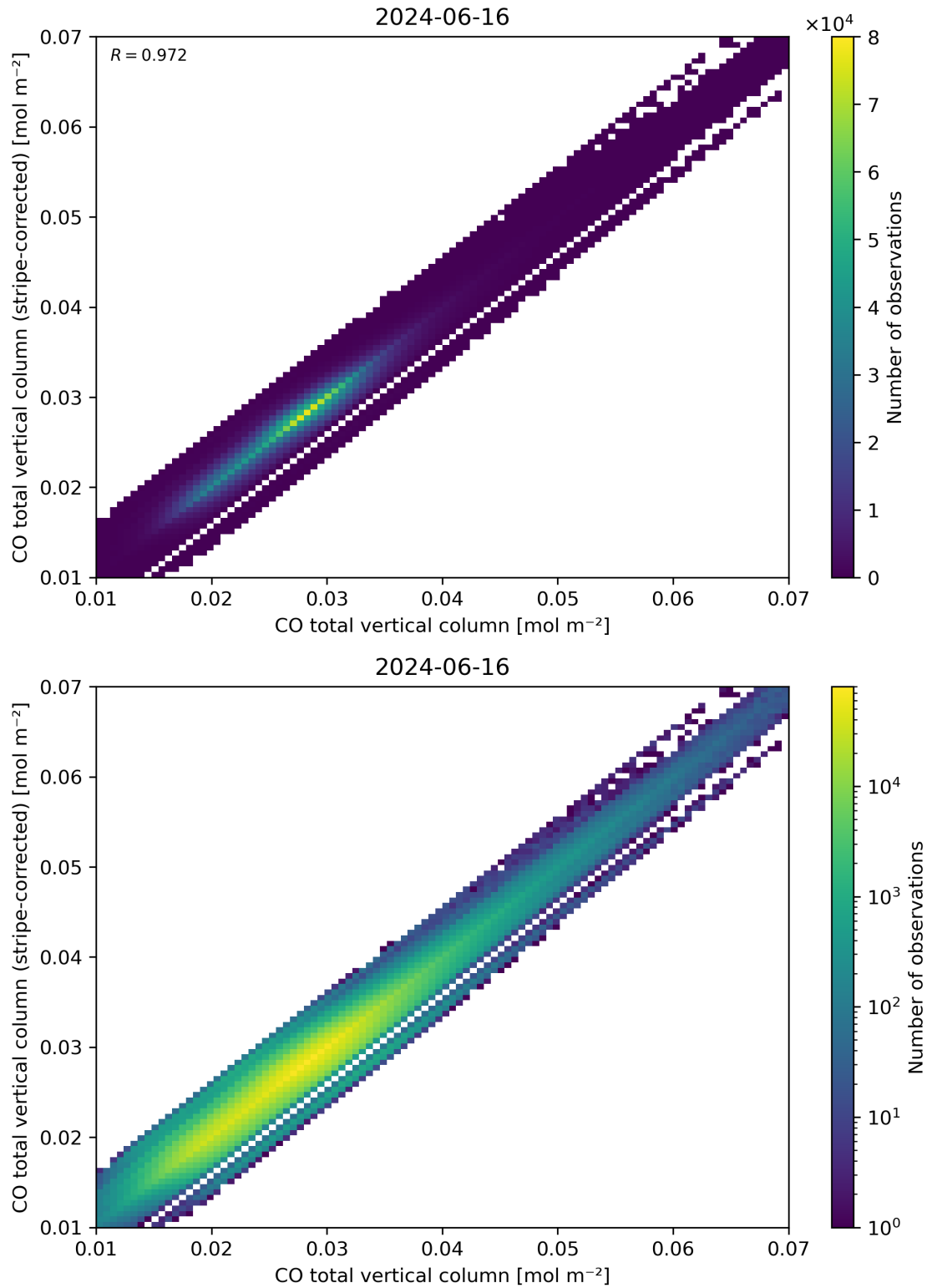
Figure 33: Scatter density plot of “CO total vertical column” against “CO total vertical column (stripe-corrected)” for 2024-06-15 to 2024-06-17.
