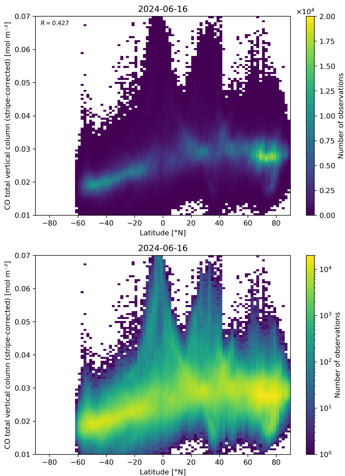
Figure 52: Scatter density plot of “Latitude” against “CO total vertical column (stripe-corrected)” for 2024-06-15 to 2024-06-17.
