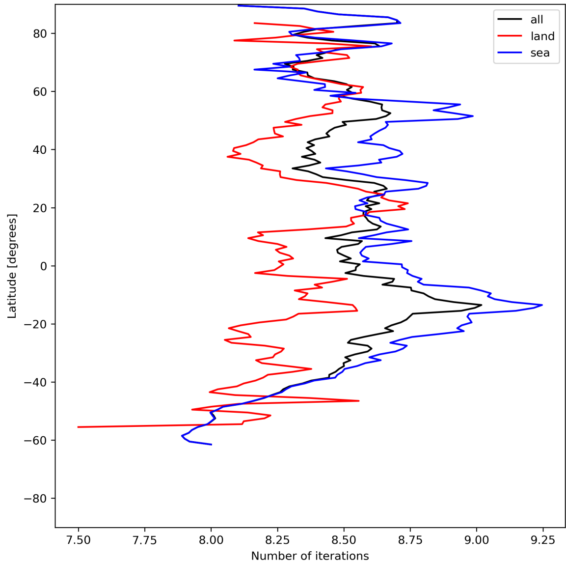
Figure 16: Zonal average of “Number of iterations” for 2024-06-15 to 2024-06-17.
