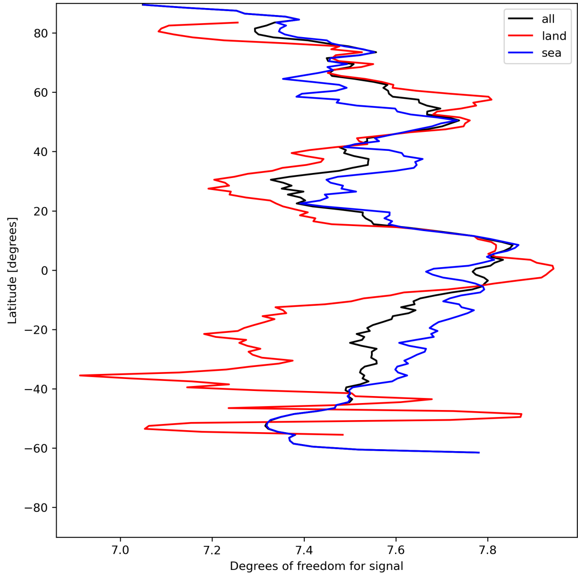
Figure 15: Zonal average of “Degrees of freedom for signal” for 2024-06-15 to 2024-06-17.
