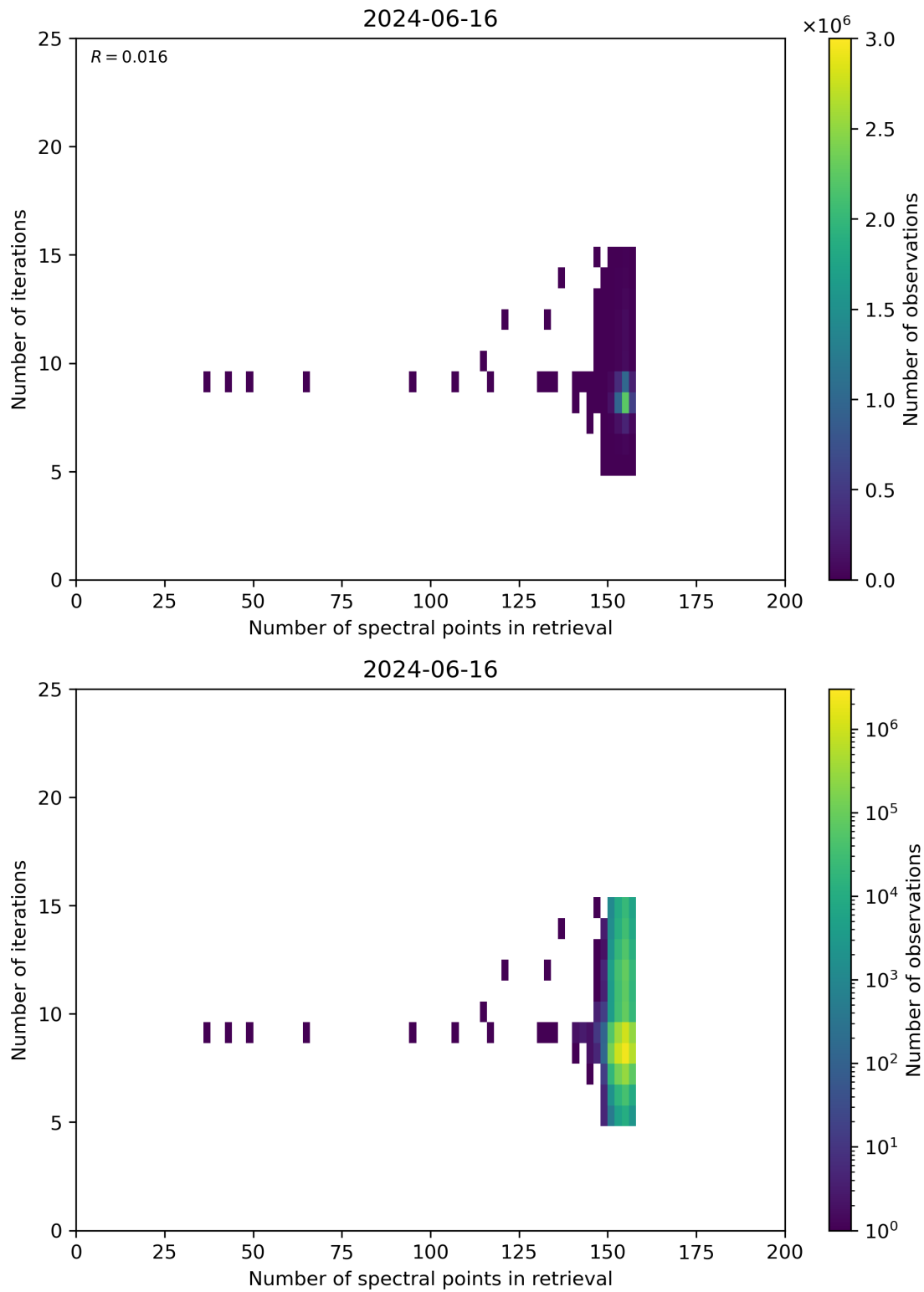
Figure 60: Scatter density plot of “Number of spectral points in retrieval” against “Number of iterations” for 2024-06-15 to 2024-06-17.
