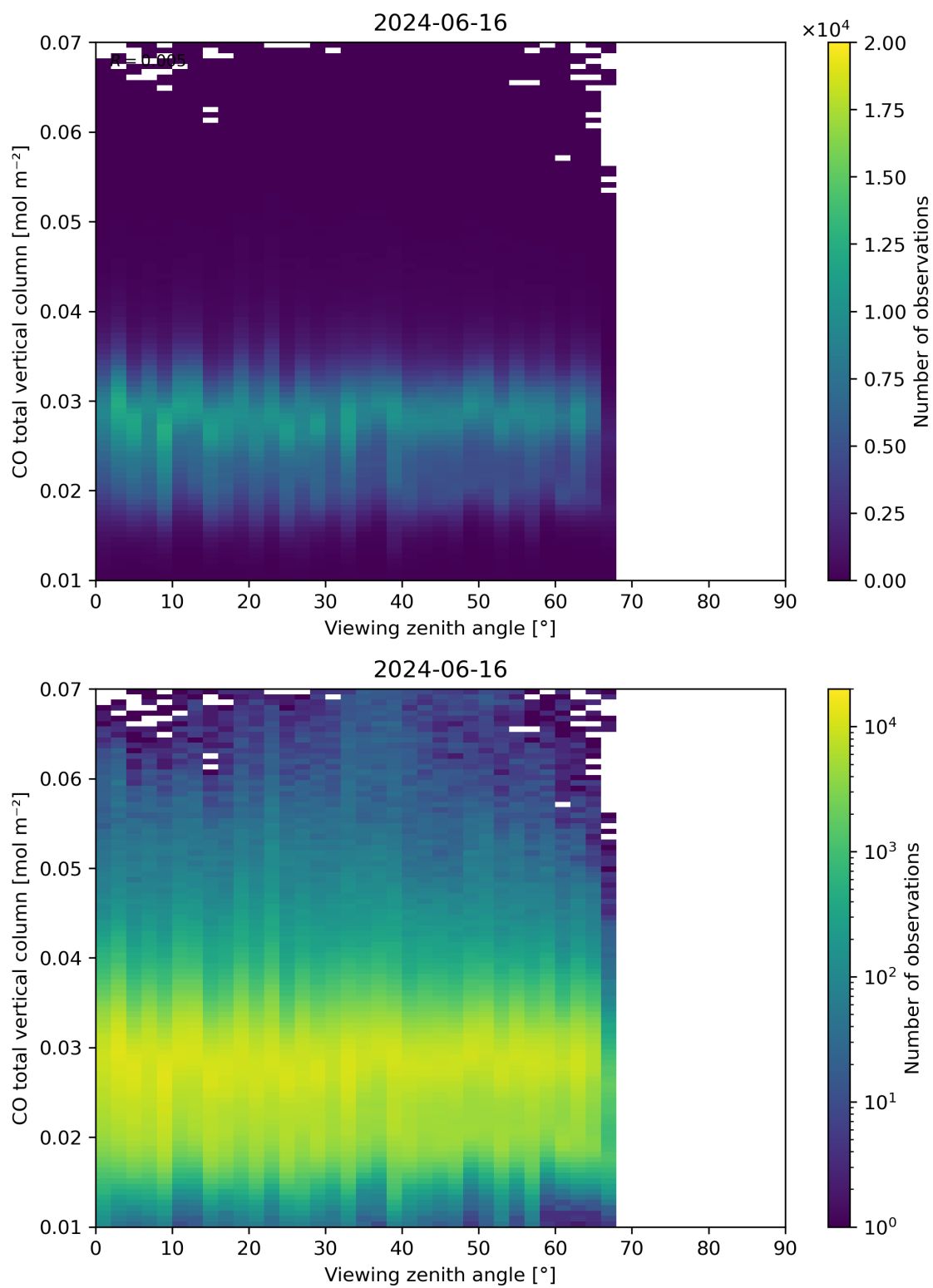
Figure 69: Scatter density plot of “Viewing zenith angle” against “CO total vertical column” for 2024-06-15 to 2024-06-17.
