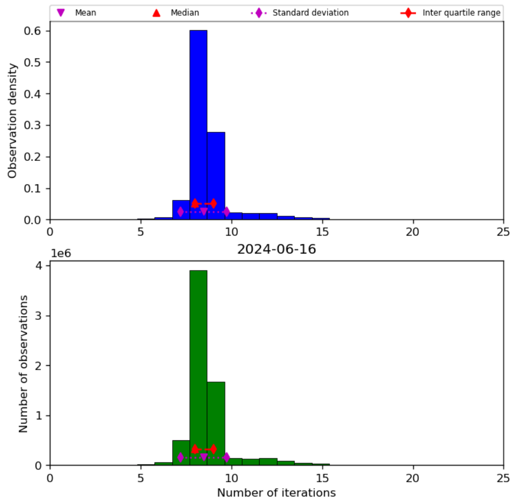
Figure 24: Histogram of “Number of iterations” for 2024-06-15 to 2024-06-17
