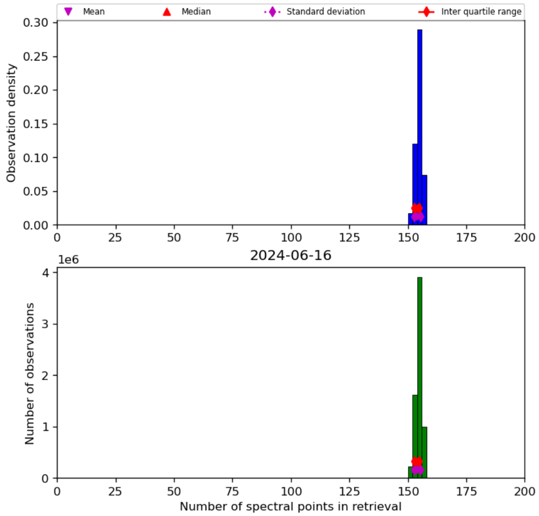
Figure 21: Histogram of “Number of spectral points in retrieval” for 2024-06-15 to 2024-06-17
