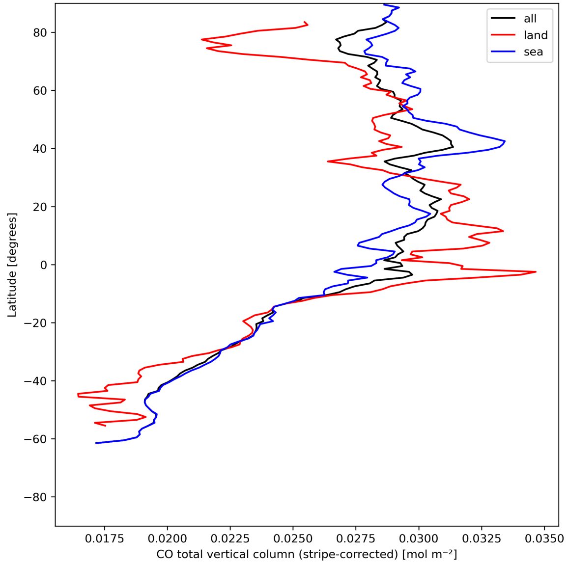
Figure 11: Zonal average of “CO total vertical column (stripe-corrected)” for 2024-06-15 to 2024-06-17.
