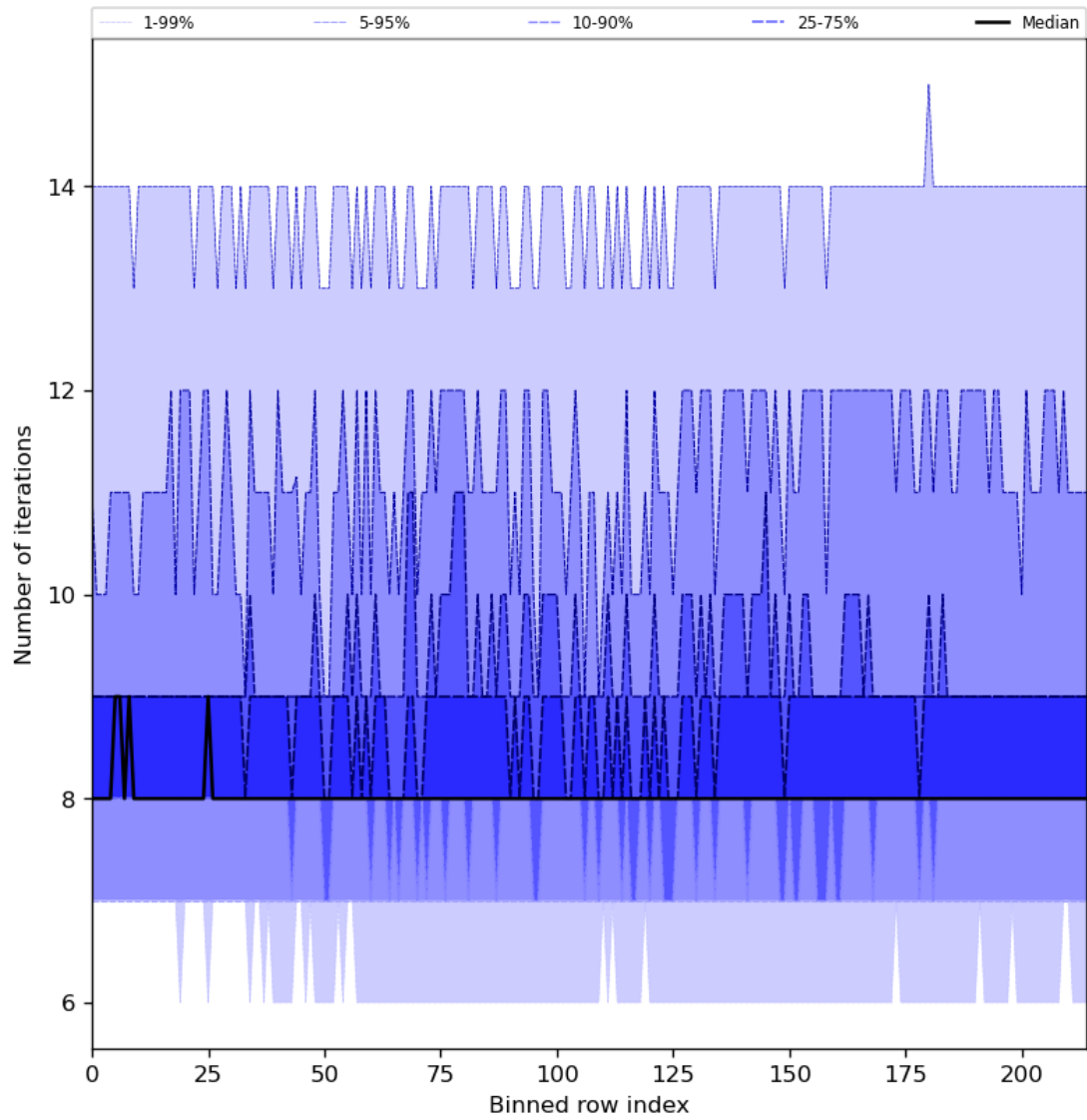
Figure 32: Along track statistics of “Number of iterations” for 2024-06-15 to 2024-06-17
