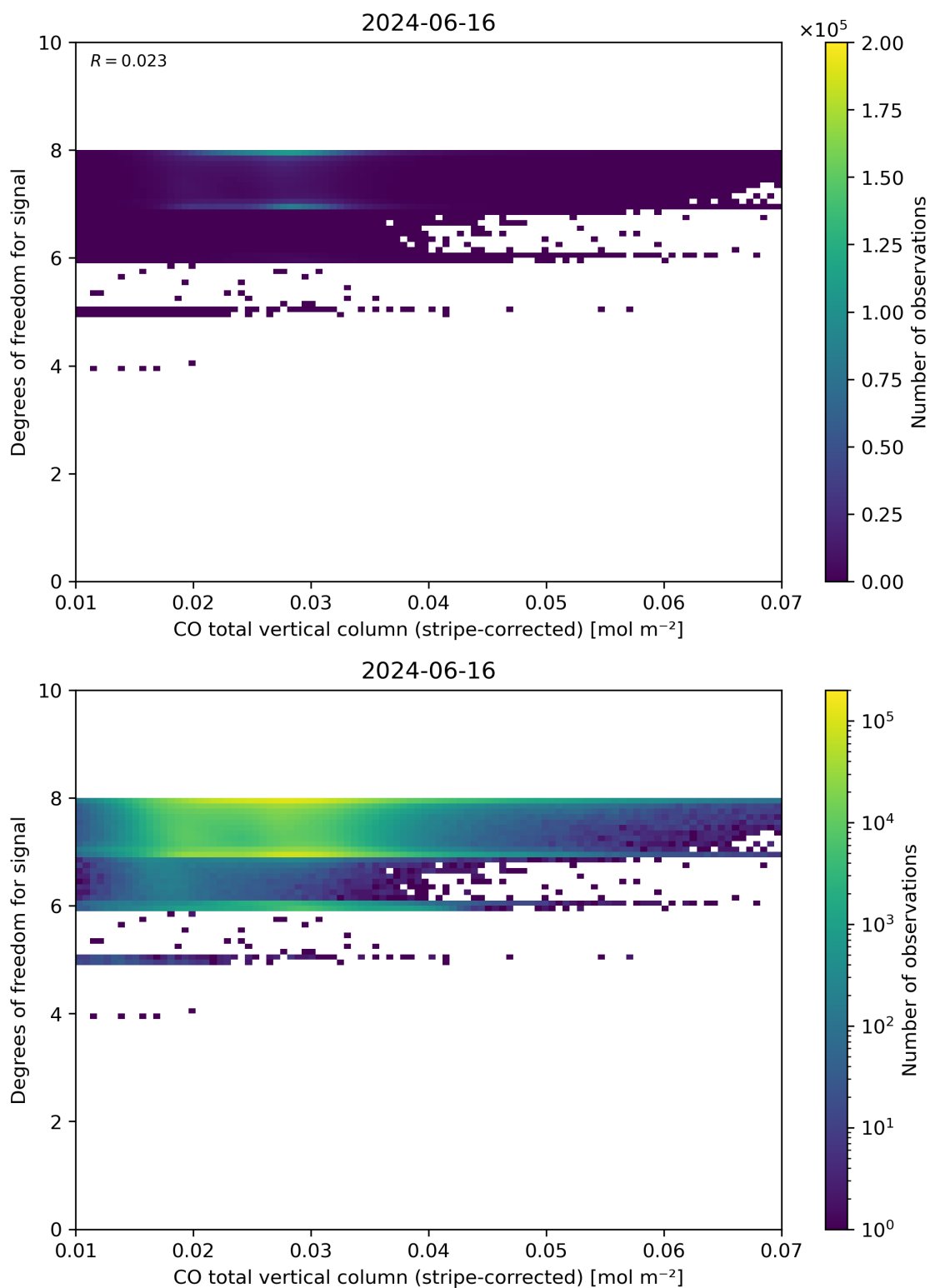
Figure 38: Scatter density plot of “CO total vertical column (stripe-corrected)” against “Degrees of freedom for signal” for 2024-06-15 to 2024-06-17.
