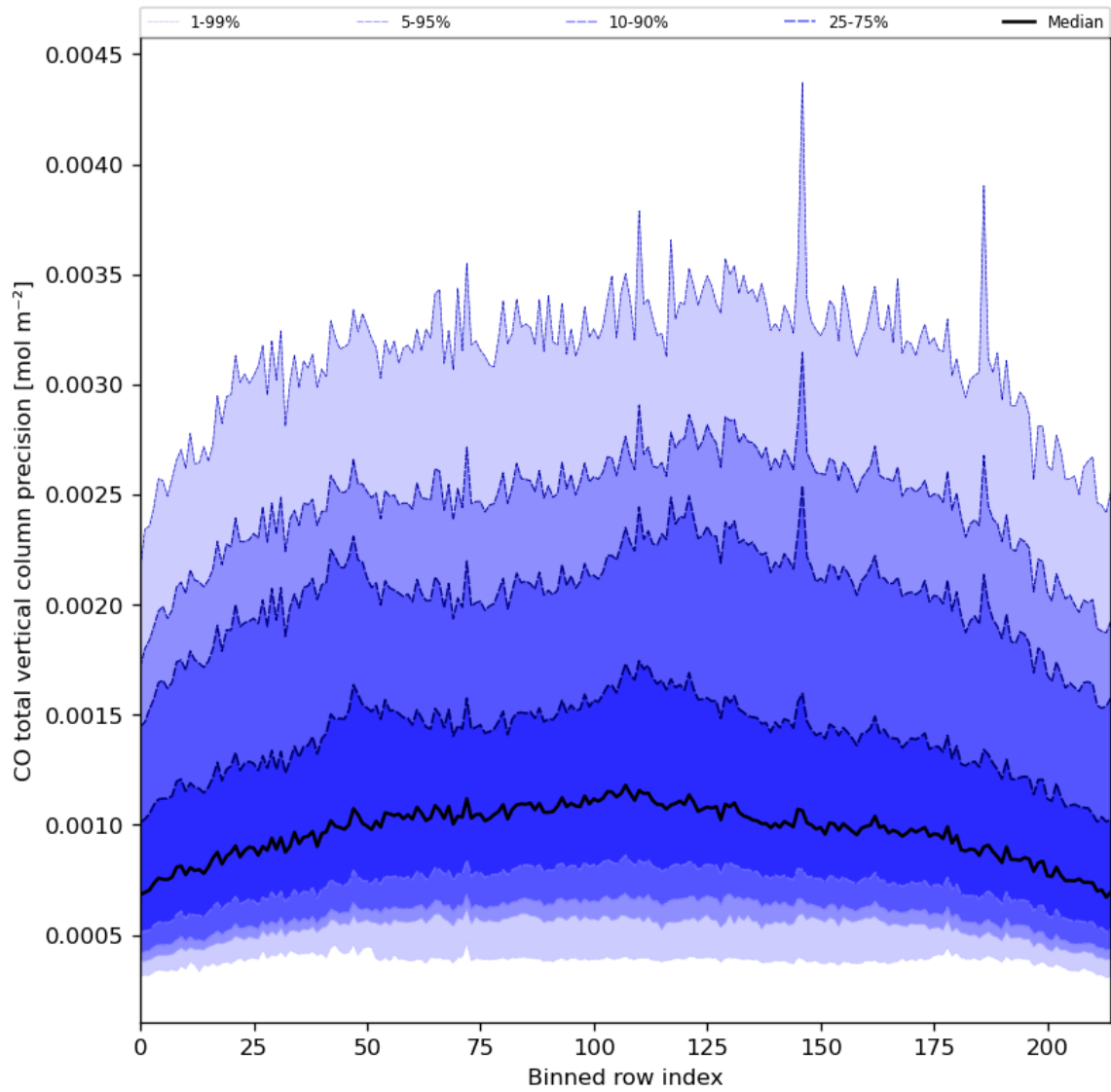
Figure 28: Along track statistics of “CO total vertical column precision” for 2024-06-15 to 2024-06-17
