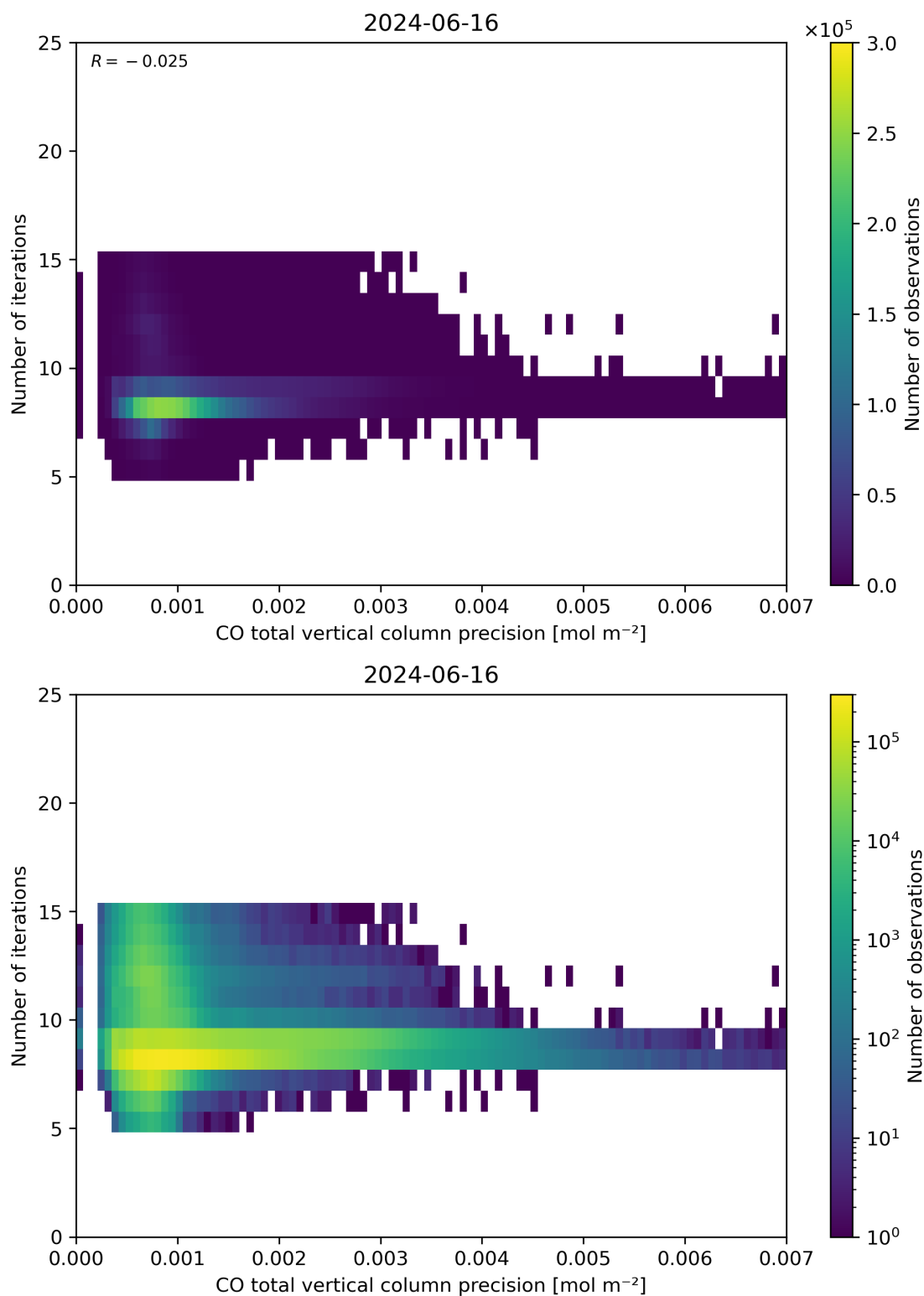
Figure 46: Scatter density plot of “CO total vertical column precision” against “Number of iterations” for 2024-06-15 to 2024-06-17.
