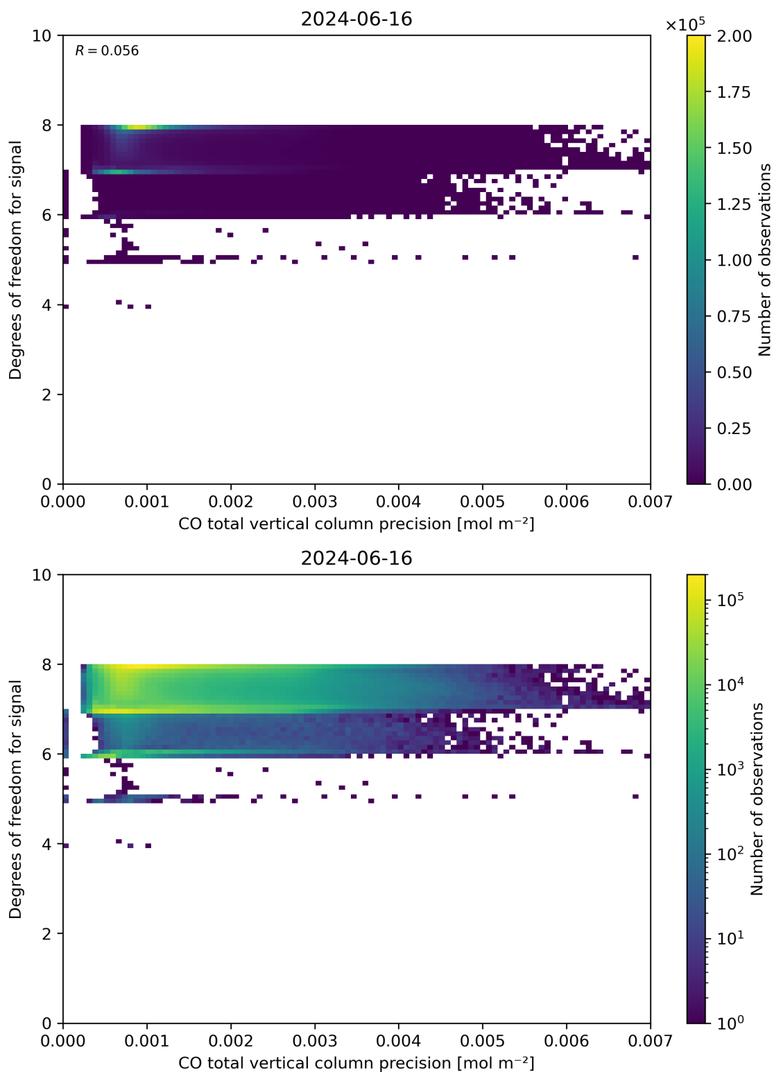
Figure 45: Scatter density plot of “CO total vertical column precision” against “Degrees of freedom for signal” for 2024-06-15 to 2024-06-17.
