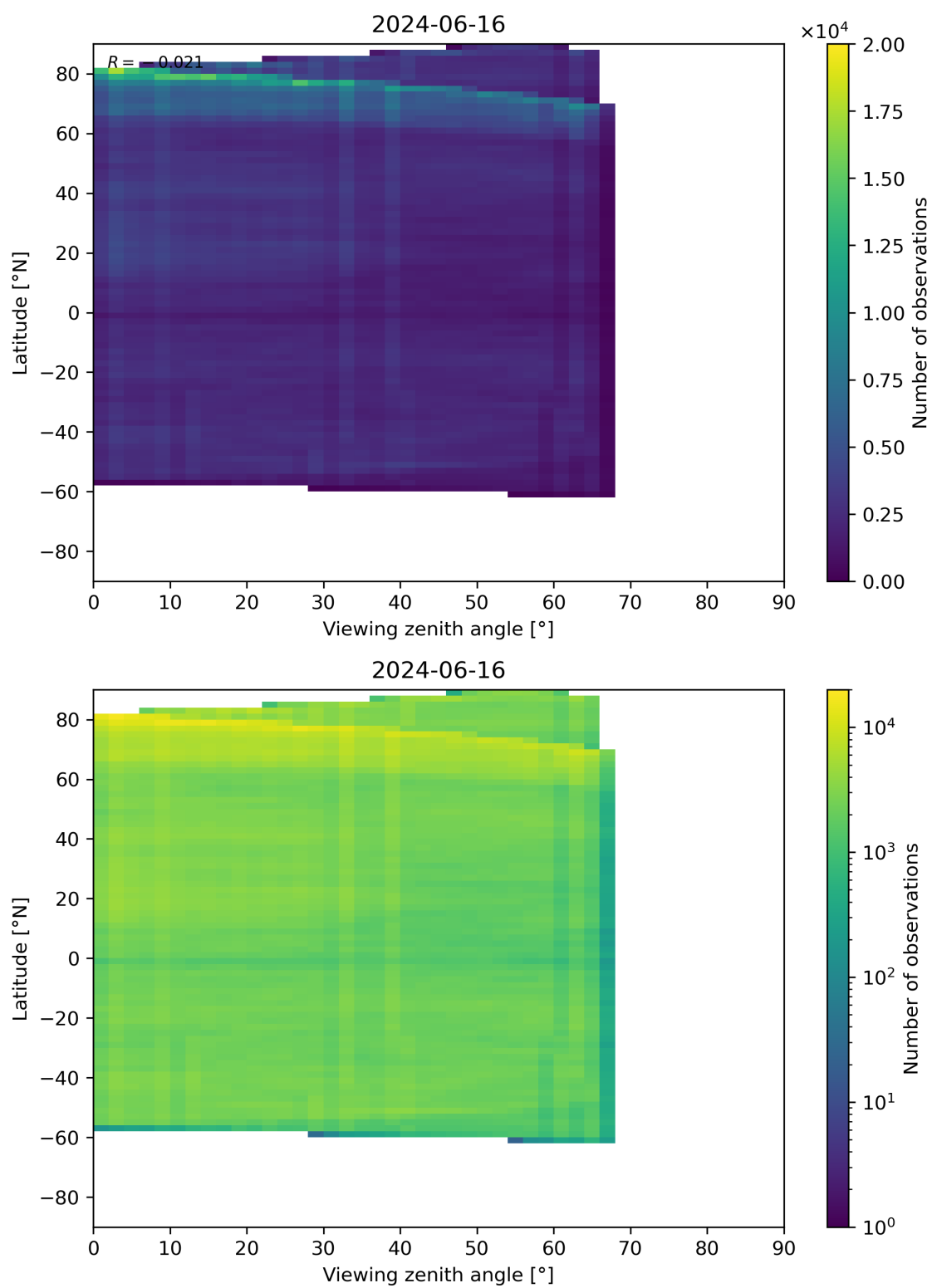
Figure 74: Scatter density plot of “Viewing zenith angle” against “Latitude” for 2024-06-15 to 2024-06-17.
