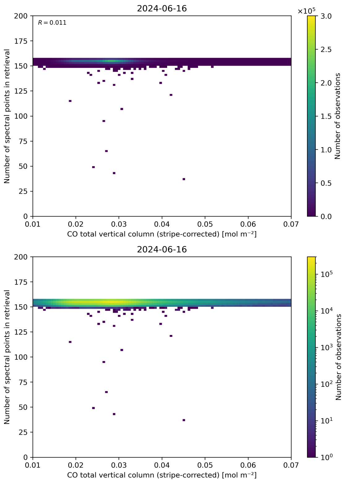
Figure 40: Scatter density plot of “CO total vertical column (stripe-corrected)” against “Number of spectral points in retrieval” for 2024-06-15 to 2024-06-17.
