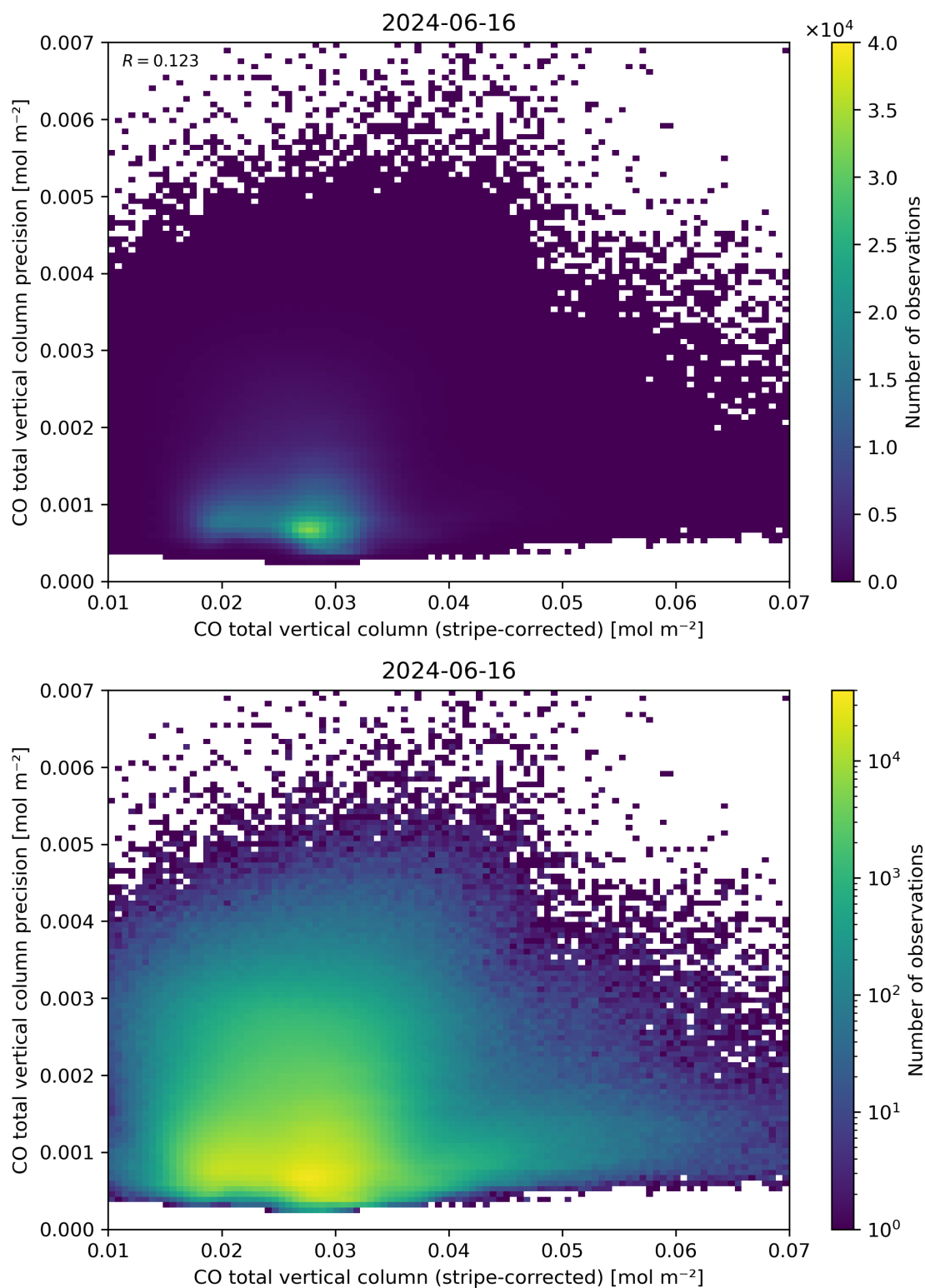
Figure 36: Scatter density plot of “CO total vertical column (stripe-corrected)” against “CO total vertical column precision” for 2024-06-15 to 2024-06-17.
