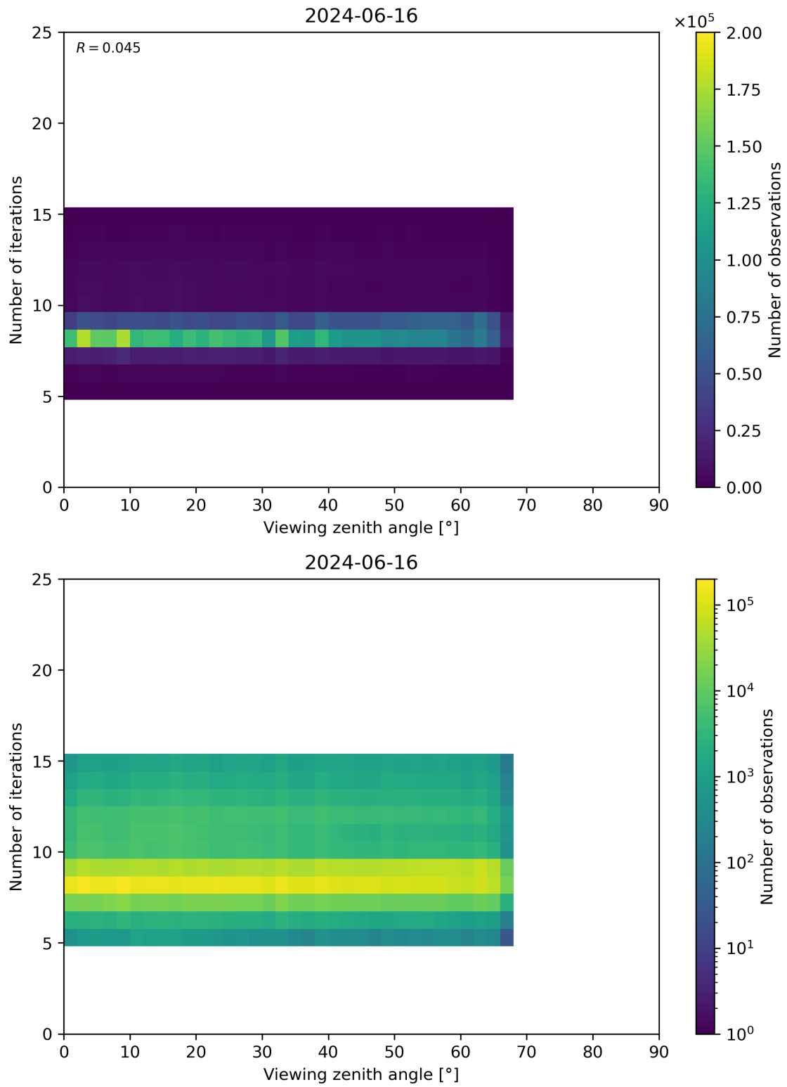
Figure 75: Scatter density plot of “Viewing zenith angle” against “Number of iterations” for 2024-06-15 to 2024-06-17.
