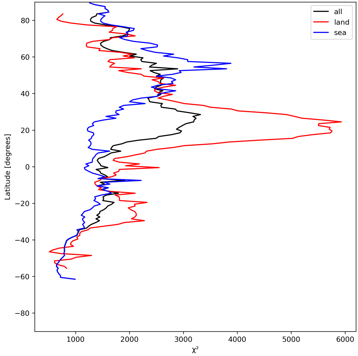
Figure 14: Zonal average of “ \chi^2 ” for 2024-06-15 to 2024-06-17.
