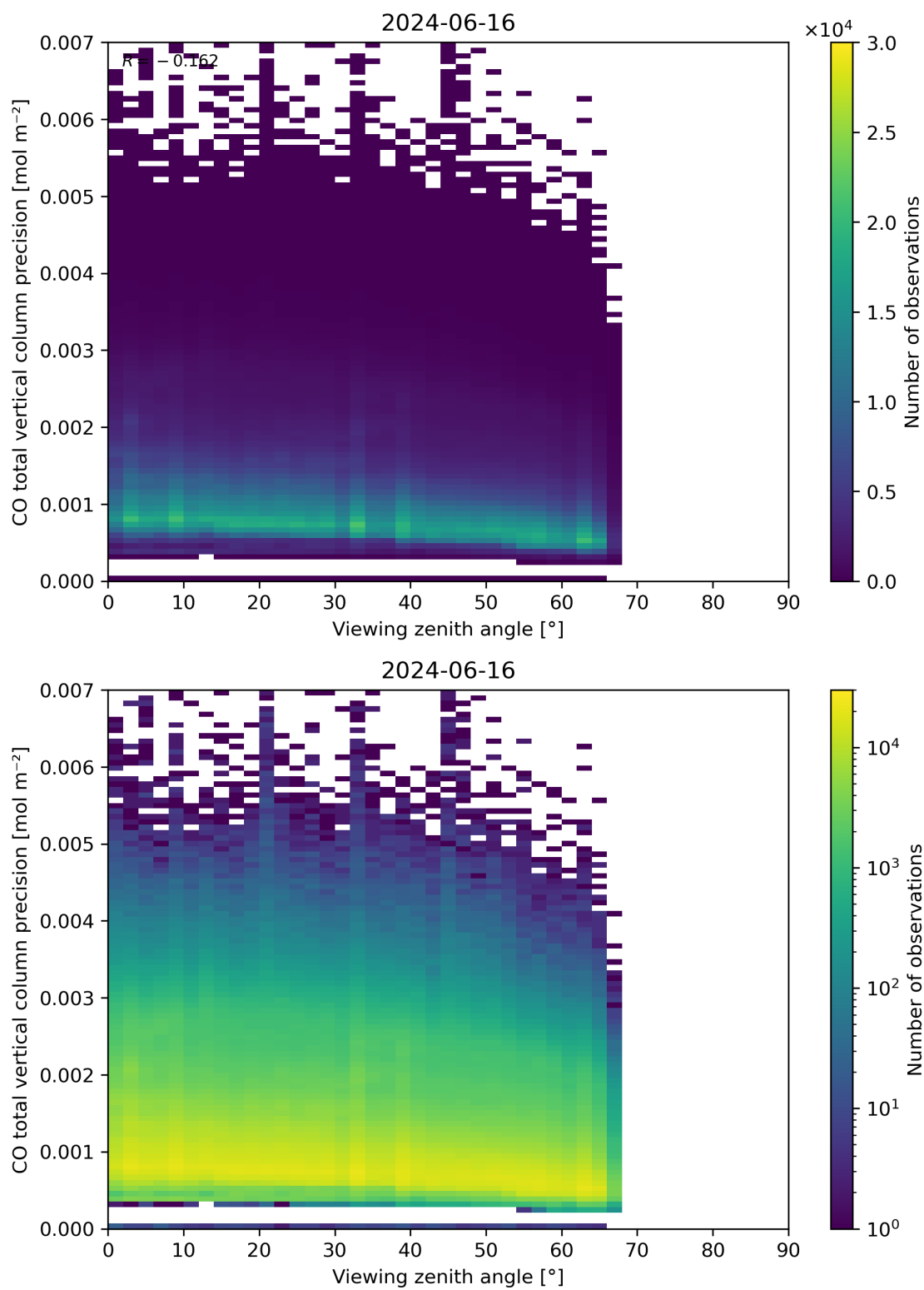
Figure 71: Scatter density plot of “Viewing zenith angle” against “CO total vertical column precision” for 2024-06-15 to 2024-06-17.
