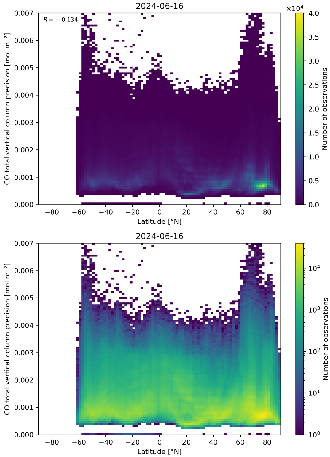
Figure 53: Scatter density plot of “Latitude” against “CO total vertical column precision” for 2024-06-15 to 2024-06-17.
