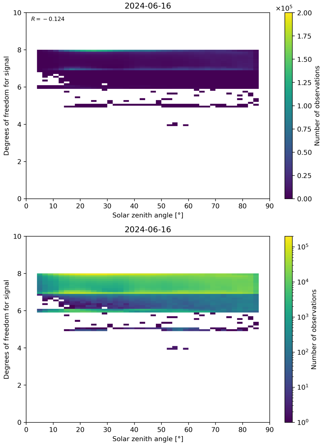
Figure 65: Scatter density plot of “Solar zenith angle” against “Degrees of freedom for signal” for 2024-06-15 to 2024-06-17.
