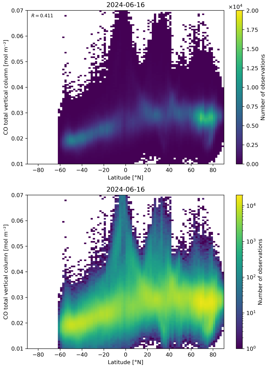
Figure 51: Scatter density plot of “Latitude” against “CO total vertical column” for 2024-06-15 to 2024-06-17.
