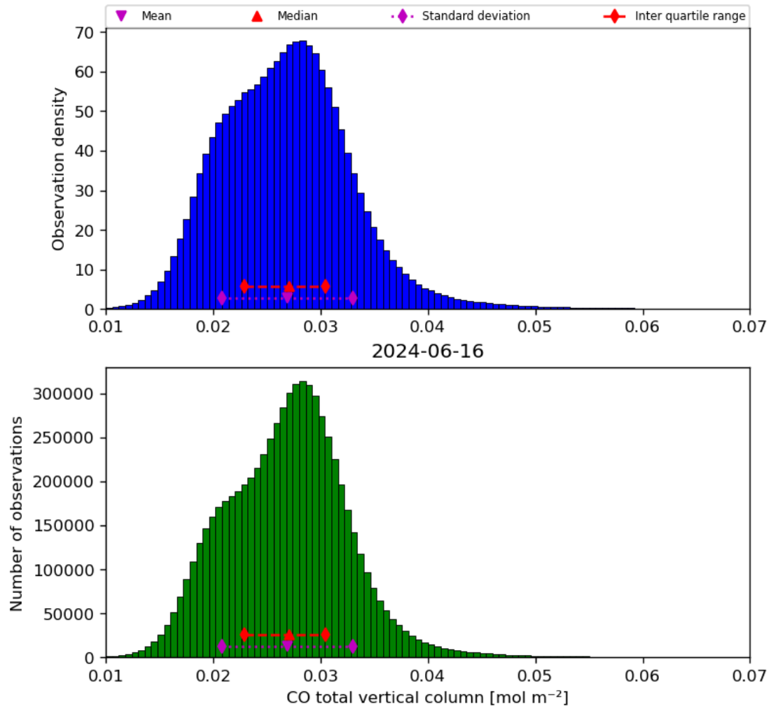
Figure 18: Histogram of “CO total vertical column” for 2024-06-15 to 2024-06-17
