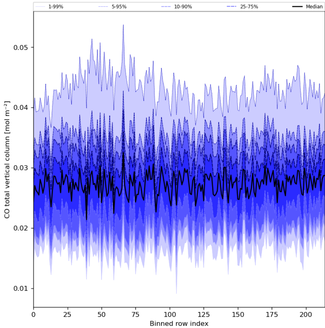
Figure 26: Along track statistics of “CO total vertical column” for 2024-06-15 to 2024-06-17
