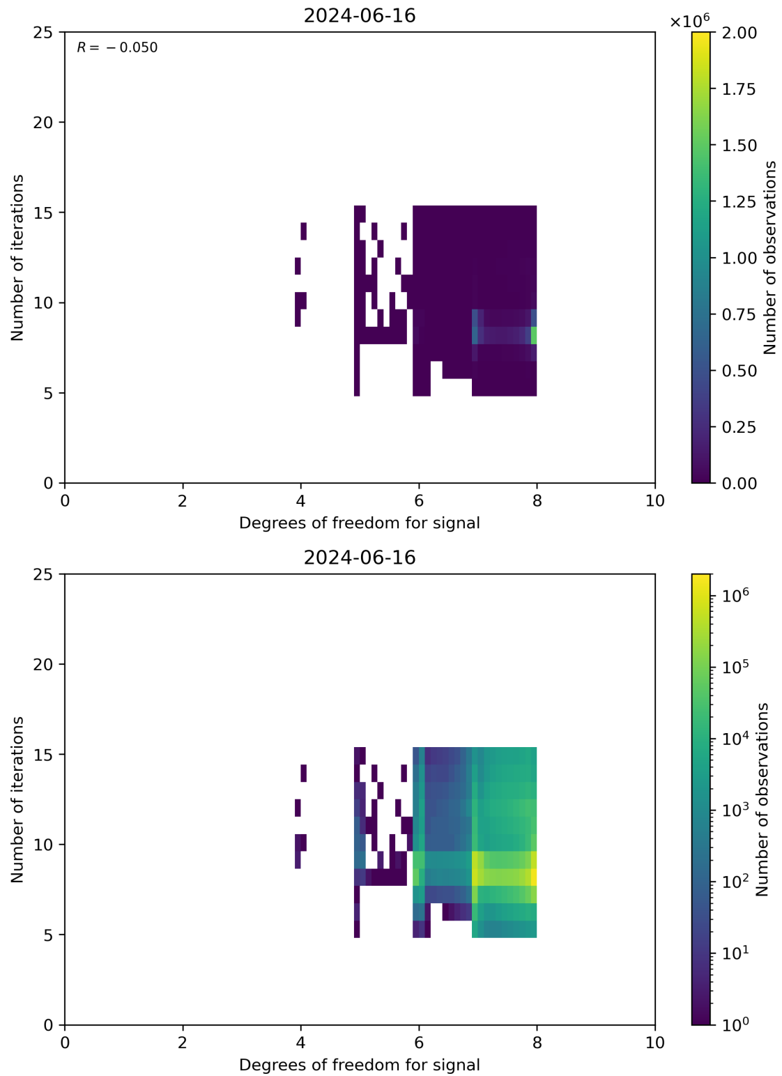
Figure 50: Scatter density plot of “Degrees of freedom for signal” against “Number of iterations” for 2024-06-15 to 2024-06-17.
