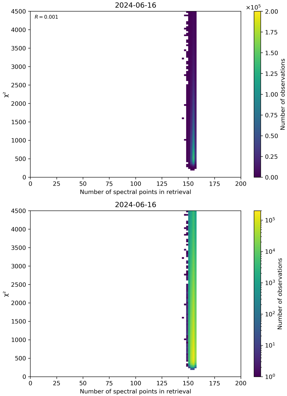
Figure 58: Scatter density plot of “Number of spectral points in retrieval” against “ \chi^2 ” for 2024-06-15 to 2024-06-17.
