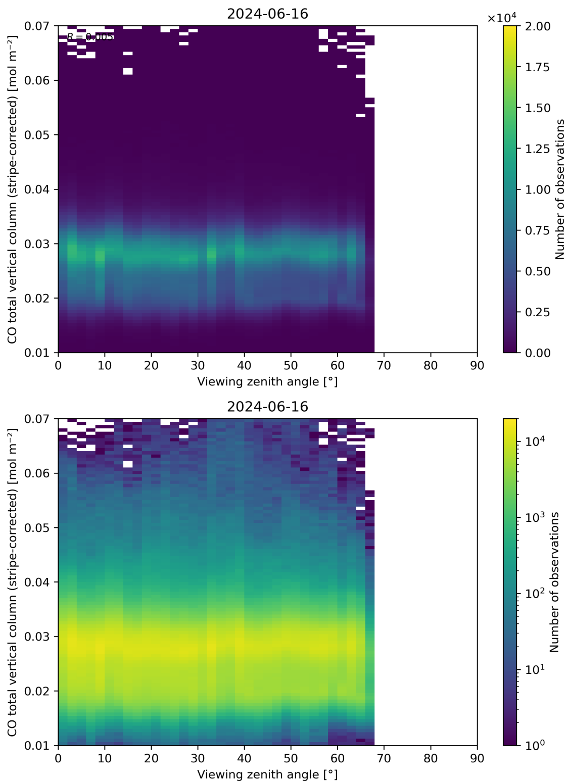
Figure 70: Scatter density plot of “Viewing zenith angle” against “CO total vertical column (stripe-corrected)” for 2024-06-15 to 2024-06-17.
