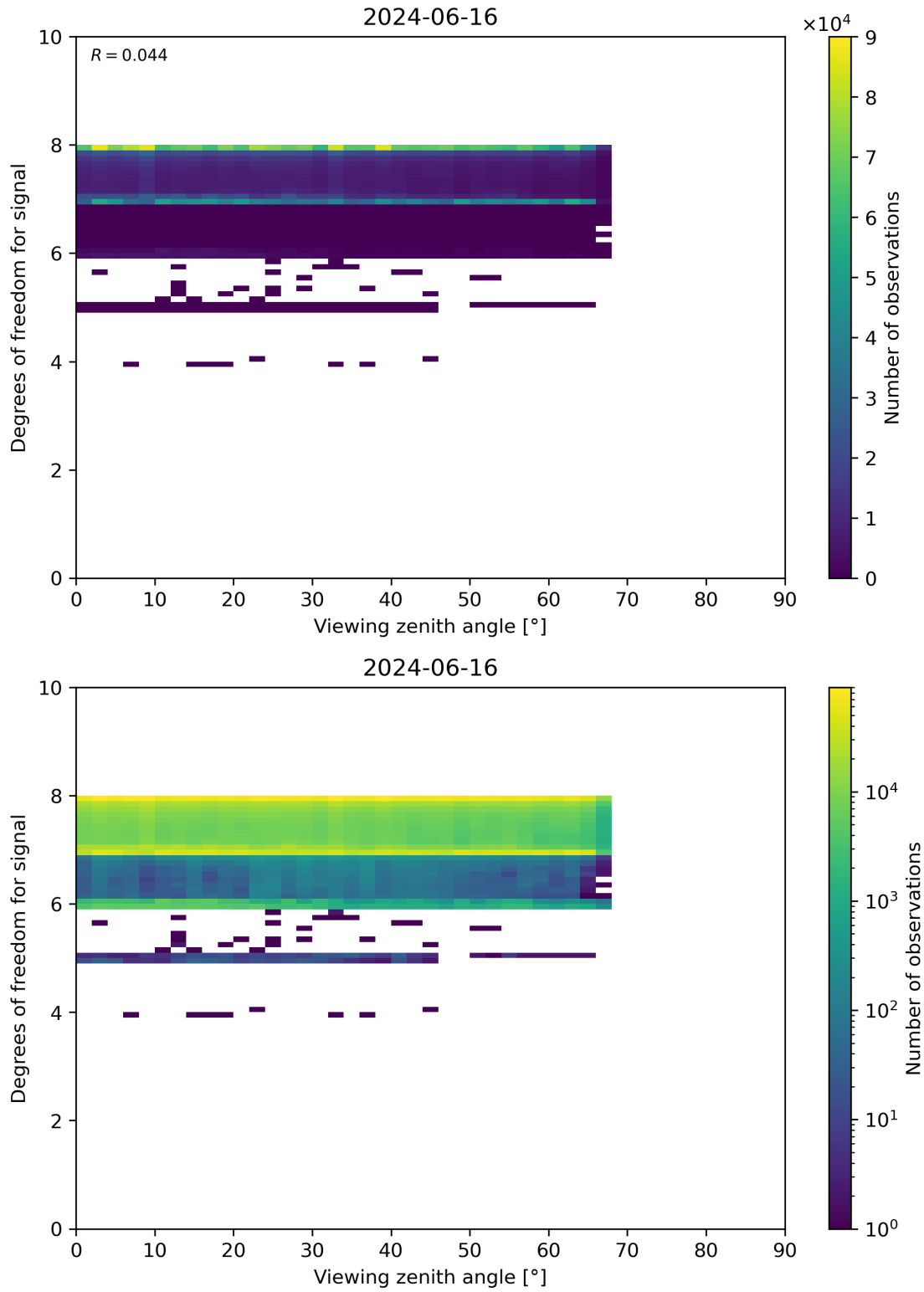
Figure 73: Scatter density plot of “Viewing zenith angle” against “Degrees of freedom for signal” for 2024-06-15 to 2024-06-17.
