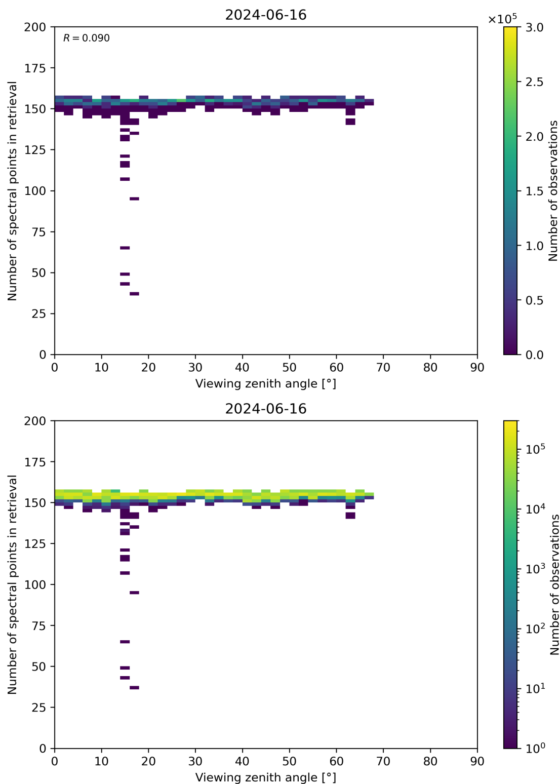
Figure 76: Scatter density plot of “Viewing zenith angle” against “Number of spectral points in retrieval” for 2024-06-15 to 2024-06-17.
