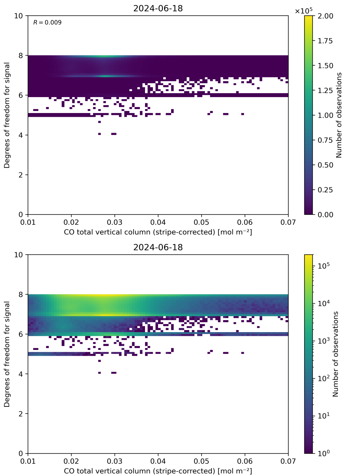
Figure 38: Scatter density plot of “CO total vertical column (stripe-corrected)” against “Degrees of freedom for signal” for 2024-06-17 to 2024-06-19.
