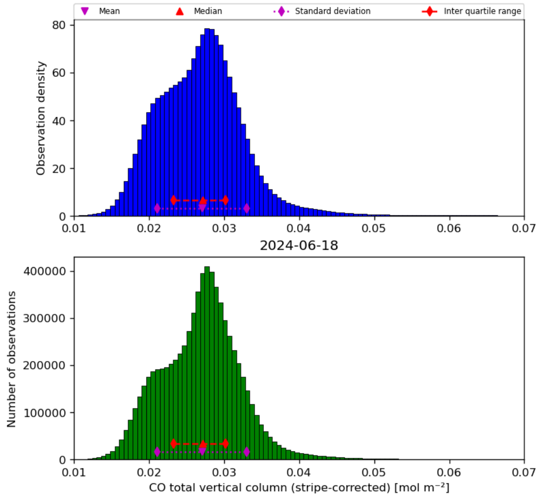
Figure 19: Histogram of “CO total vertical column (stripe-corrected)” for 2024-06-17 to 2024-06-19
