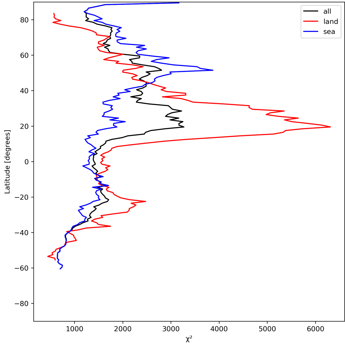
Figure 14: Zonal average of “ \chi^2 ” for 2024-06-17 to 2024-06-19.
