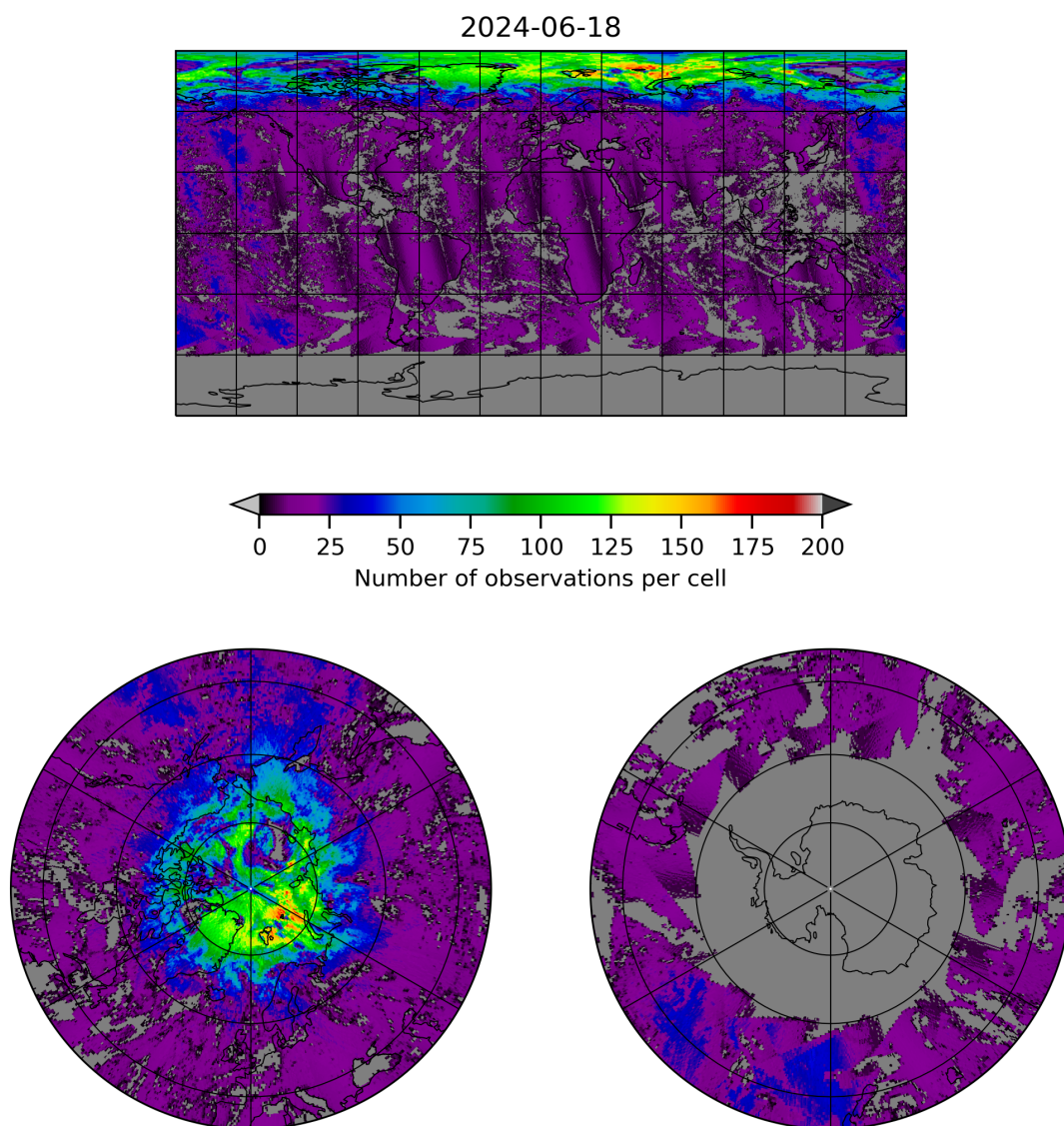
Figure 8: Map of the number of observations for 2024-06-17 to 2024-06-19
