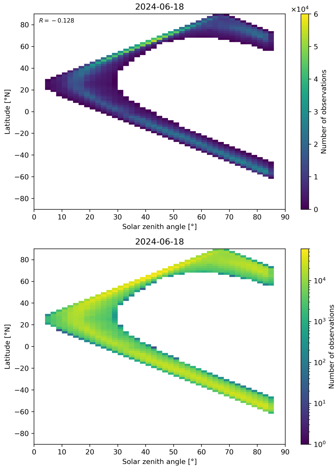
Figure 66: Scatter density plot of “Solar zenith angle” against “Latitude” for 2024-06-17 to 2024-06-19.
