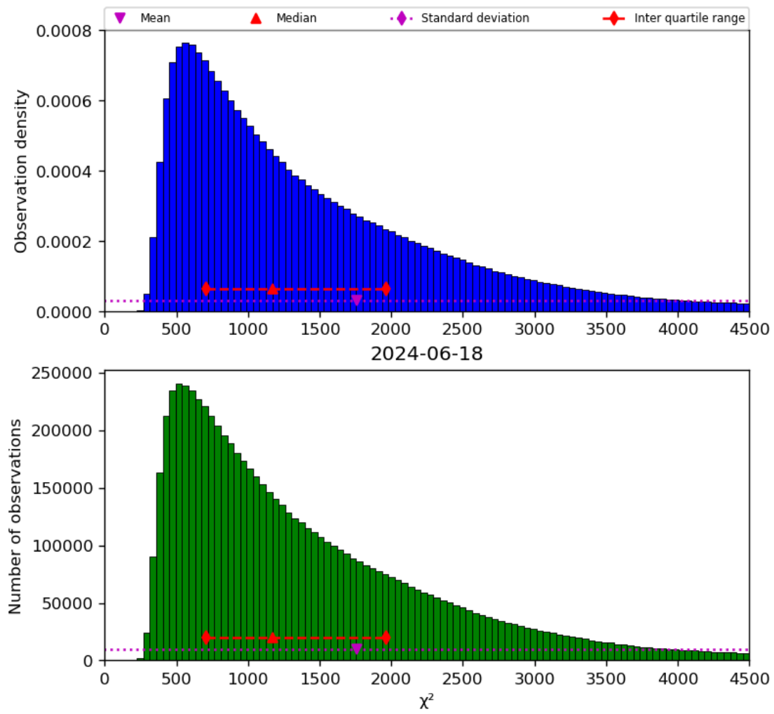
Figure 22: Histogram of “ \chi^2 ” for 2024-06-17 to 2024-06-19
