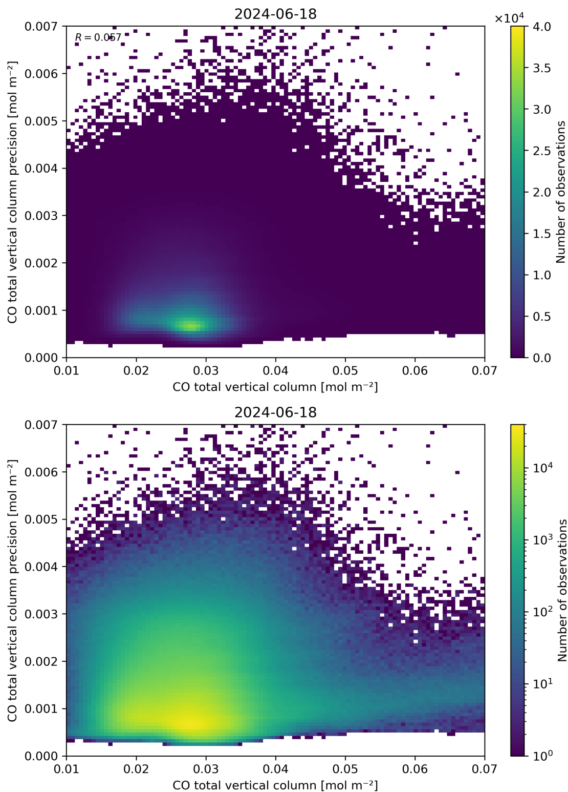
Figure 34: Scatter density plot of “CO total vertical column” against “CO total vertical column precision” for 2024-06-17 to 2024-06-19.
