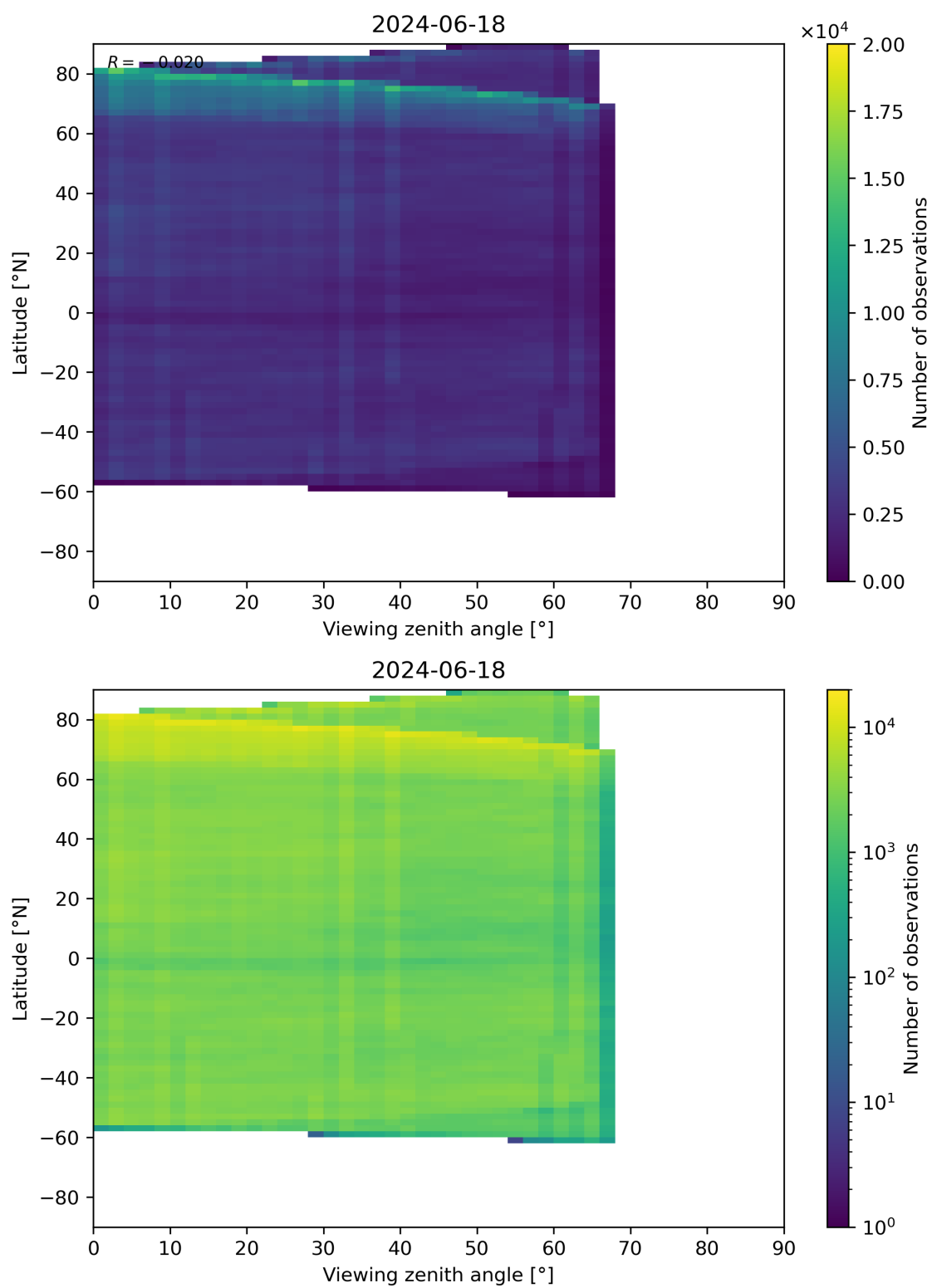
Figure 74: Scatter density plot of “Viewing zenith angle” against “Latitude” for 2024-06-17 to 2024-06-19.
