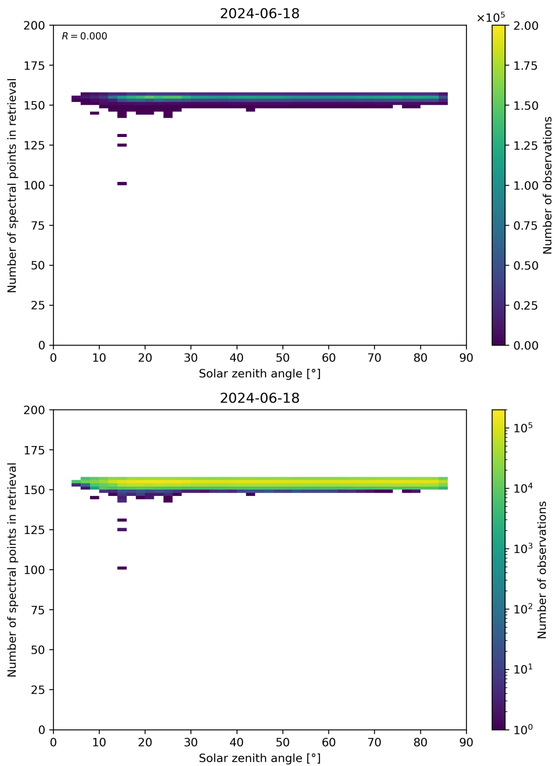
Figure 68: Scatter density plot of “Solar zenith angle” against “Number of spectral points in retrieval” for 2024-06-17 to 2024-06-19.
