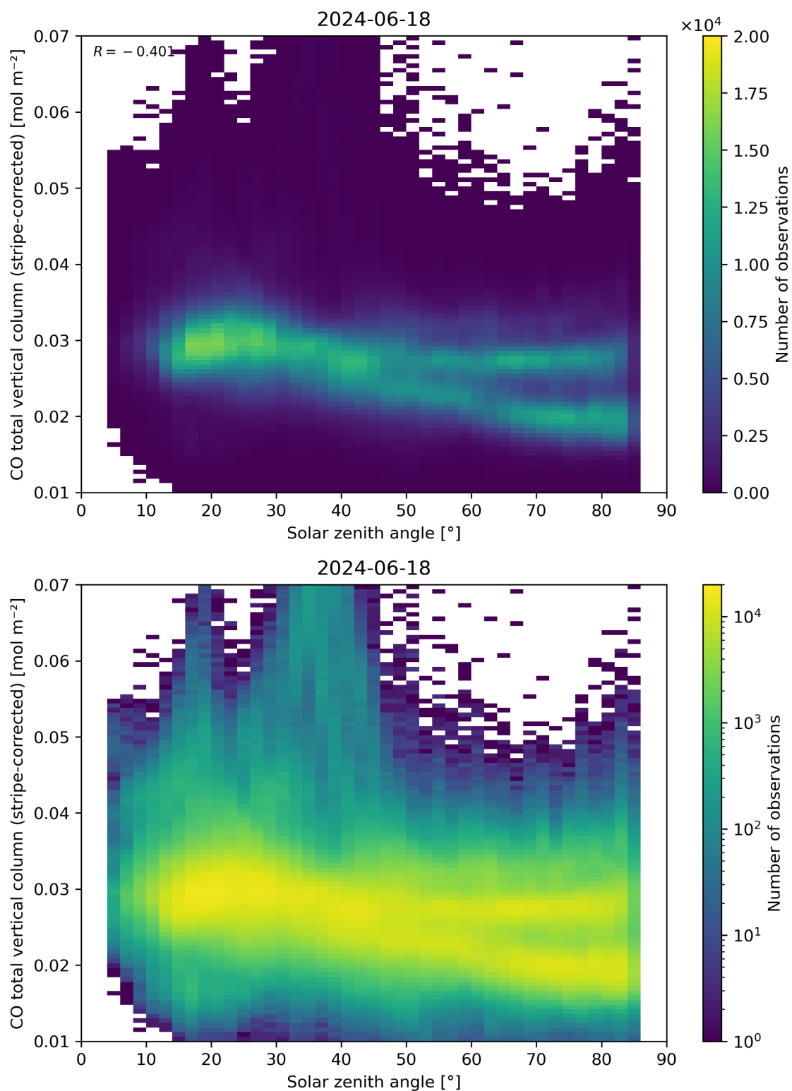
Figure 62: Scatter density plot of “Solar zenith angle” against “CO total vertical column (stripe-corrected)” for 2024-06-17 to 2024-06-19.
