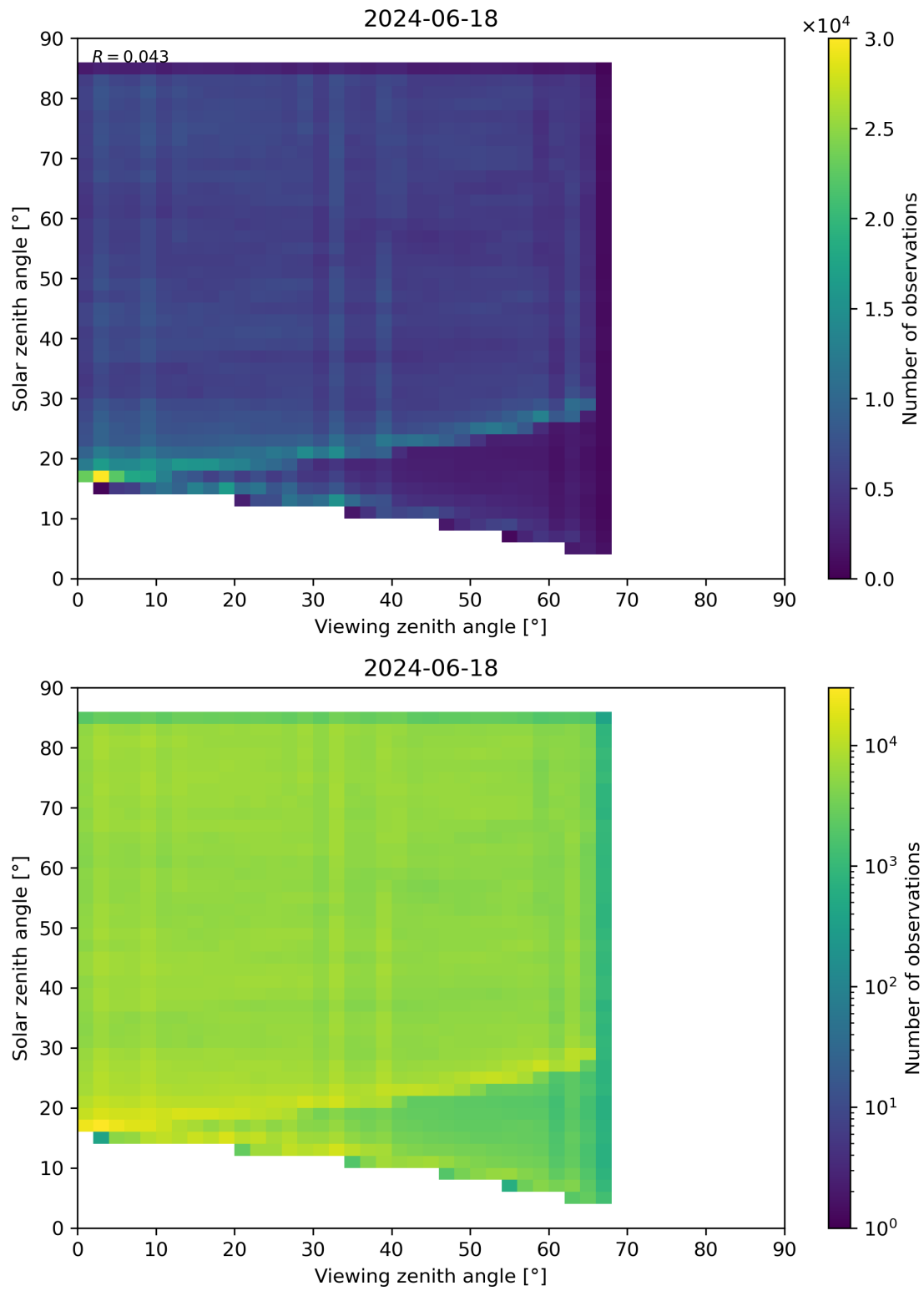
Figure 77: Scatter density plot of “Viewing zenith angle” against “Solar zenith angle” for 2024-06-17 to 2024-06-19.
