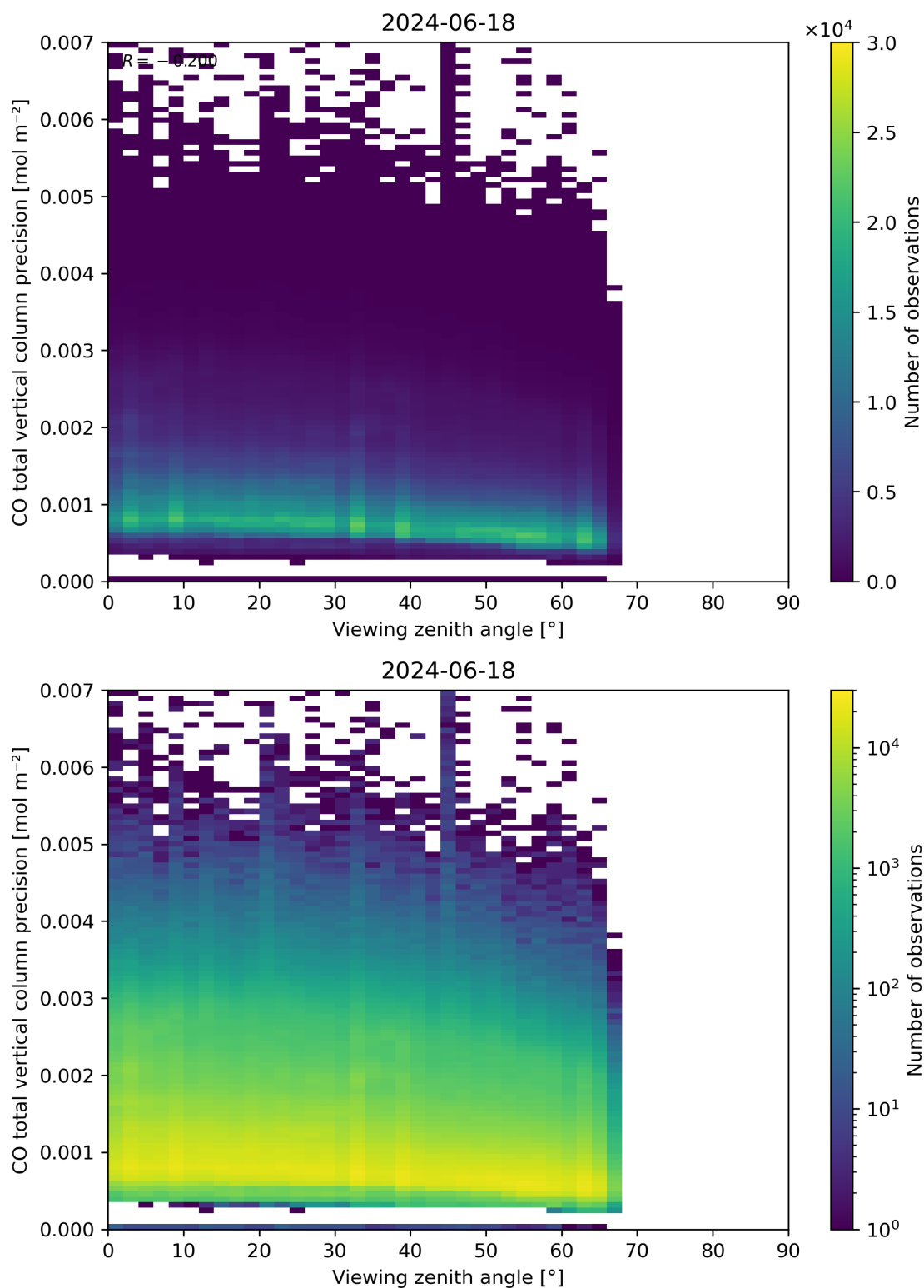
Figure 71: Scatter density plot of “Viewing zenith angle” against “CO total vertical column precision” for 2024-06-17 to 2024-06-19.
