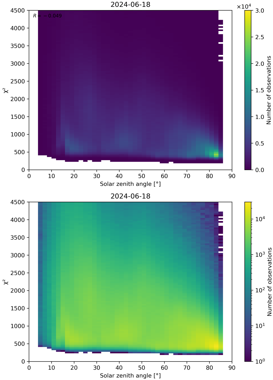
Figure 64: Scatter density plot of “Solar zenith angle” against “ \chi^2 ” for 2024-06-17 to 2024-06-19.
