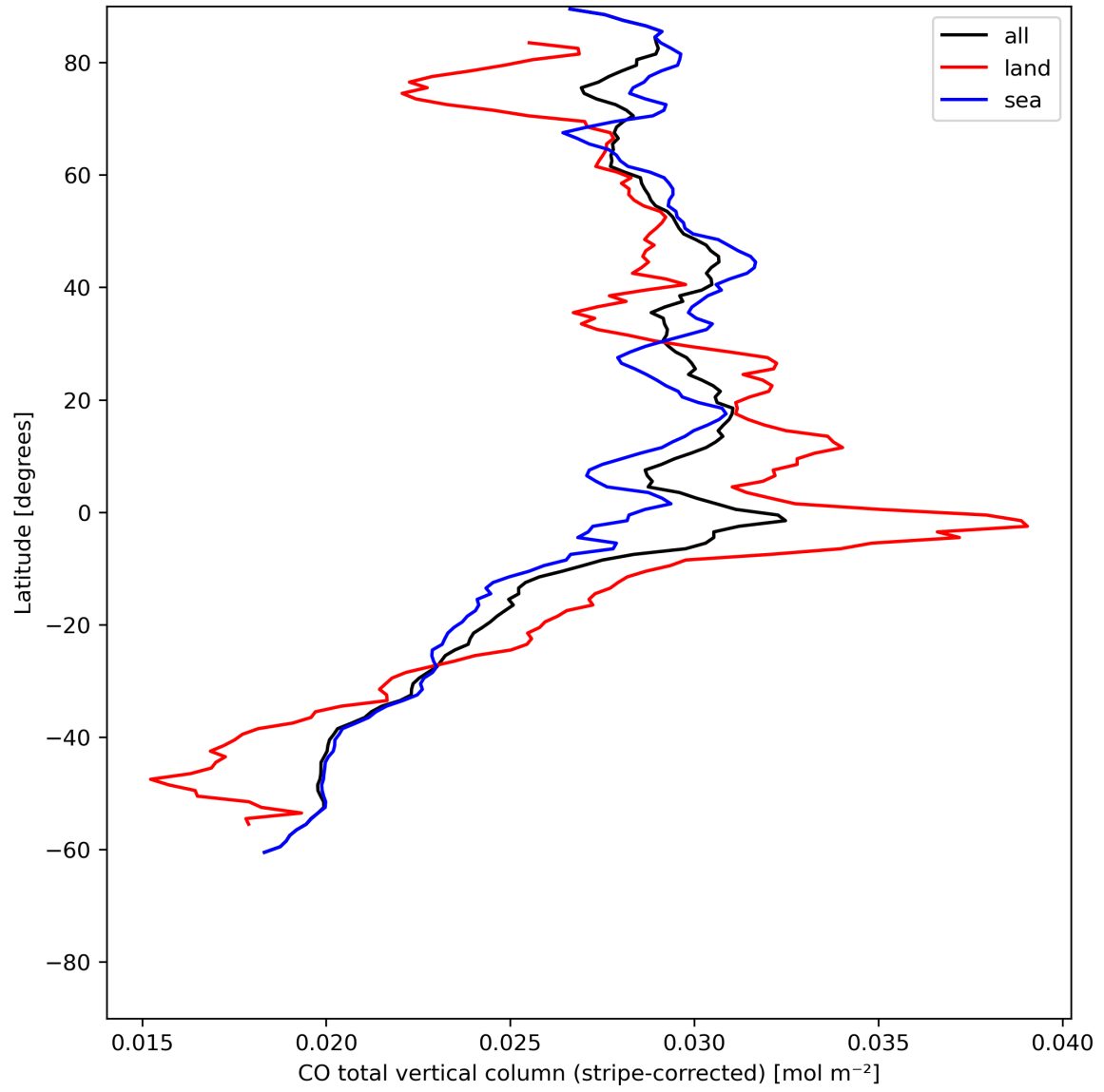
Figure 11: Zonal average of “CO total vertical column (stripe-corrected)” for 2024-06-17 to 2024-06-19.
