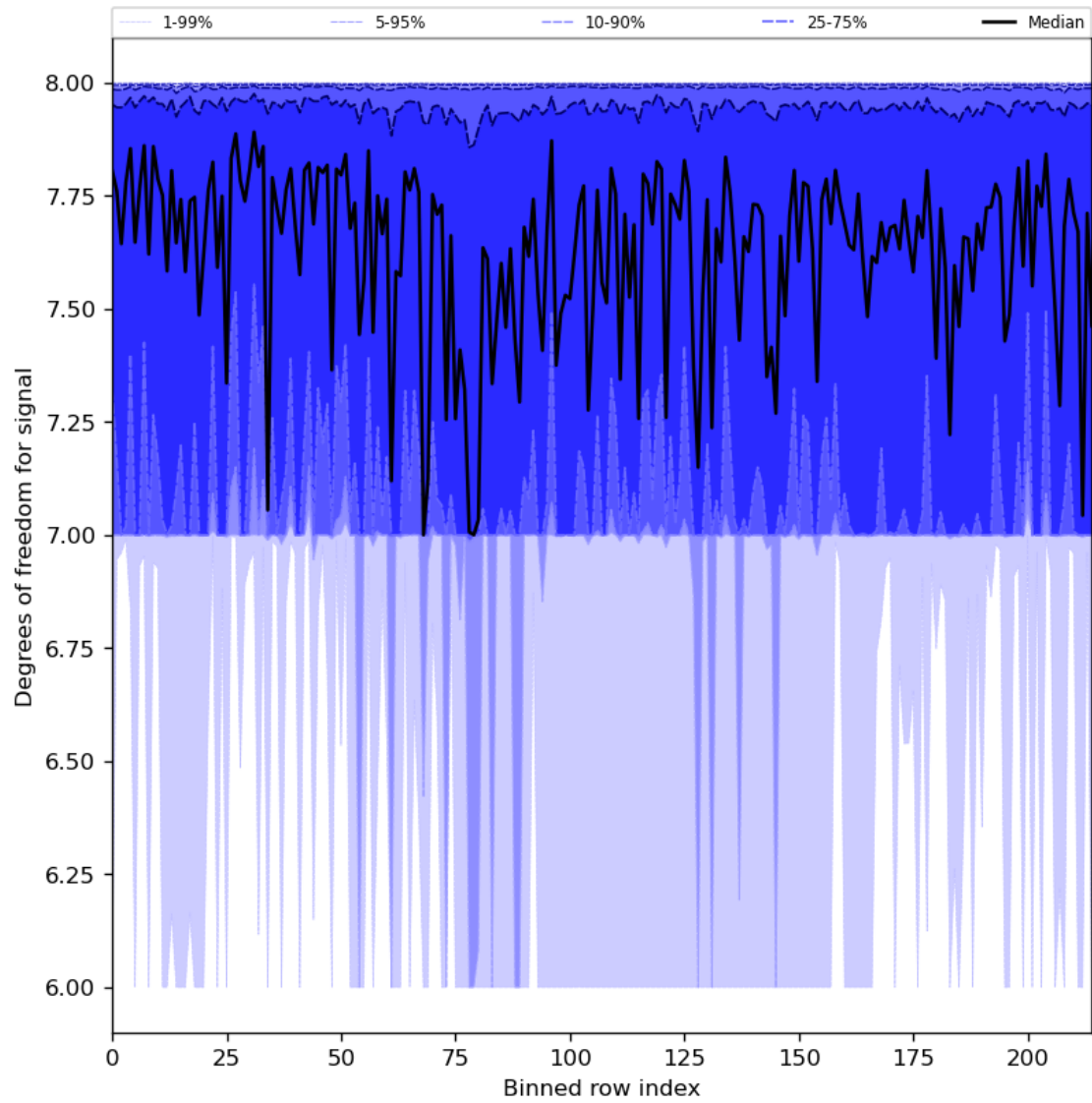
Figure 31: Along track statistics of “Degrees of freedom for signal” for 2024-06-17 to 2024-06-19
