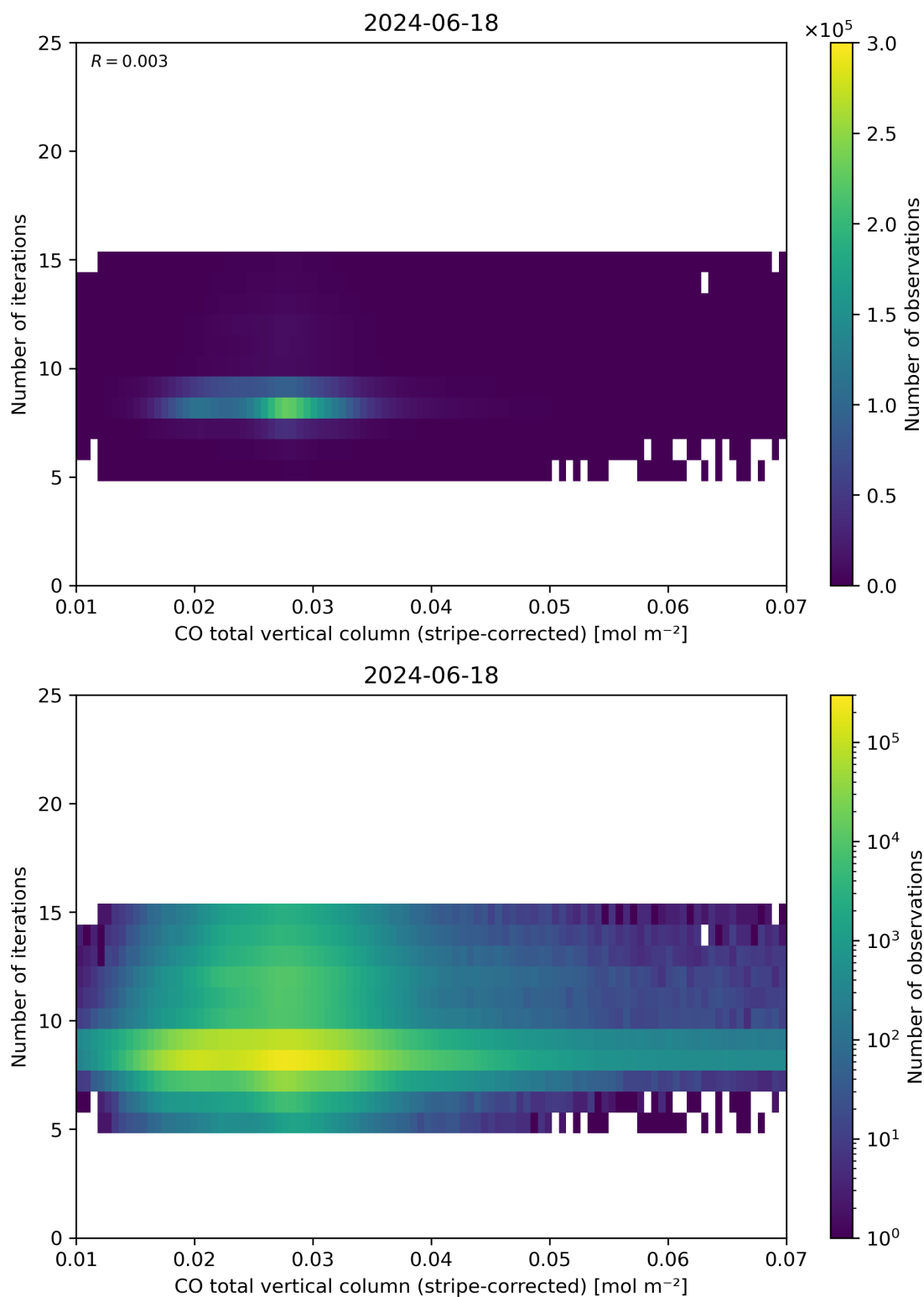
Figure 39: Scatter density plot of “CO total vertical column (stripe-corrected)” against “Number of iterations” for 2024-06-17 to 2024-06-19.
