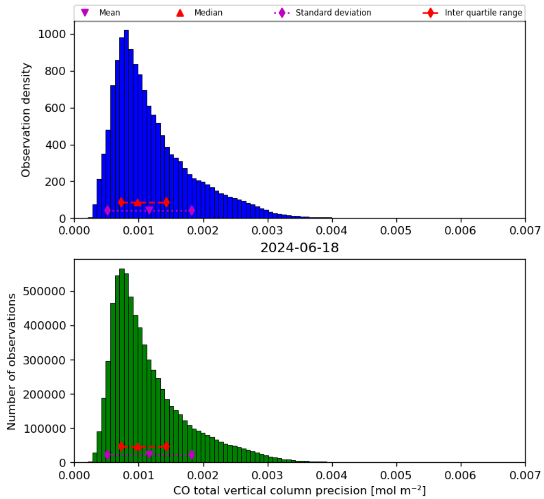
Figure 20: Histogram of “CO total vertical column precision” for 2024-06-17 to 2024-06-19
