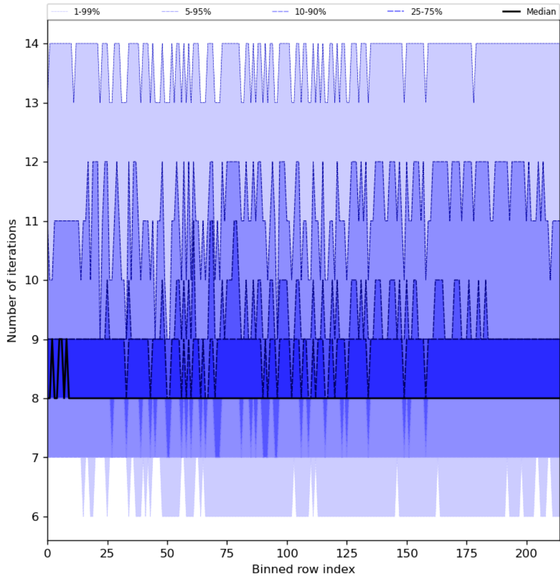
Figure 32: Along track statistics of “Number of iterations” for 2024-06-17 to 2024-06-19
