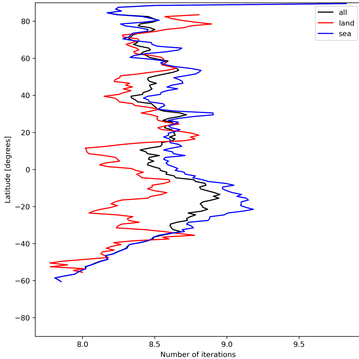
Figure 16: Zonal average of “Number of iterations” for 2024-06-17 to 2024-06-19.
