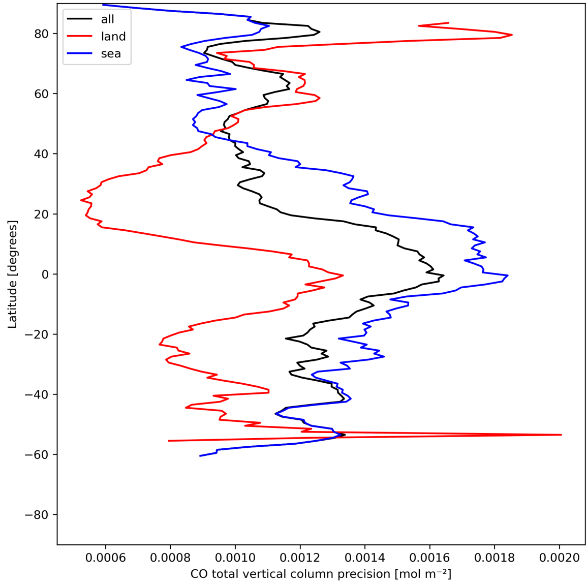
Figure 12: Zonal average of "CO total vertical column precision" for 2024-06-17 to 2024-06-19.
