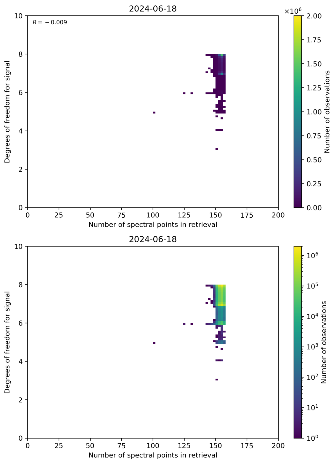
Figure 59: Scatter density plot of “Number of spectral points in retrieval” against “Degrees of freedom for signal” for 2024-06-17 to 2024-06-19.
