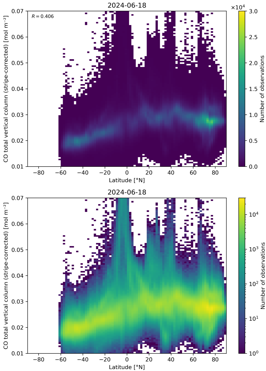
Figure 52: Scatter density plot of “Latitude” against “CO total vertical column (stripe-corrected)” for 2024-06-17 to 2024-06-19.
