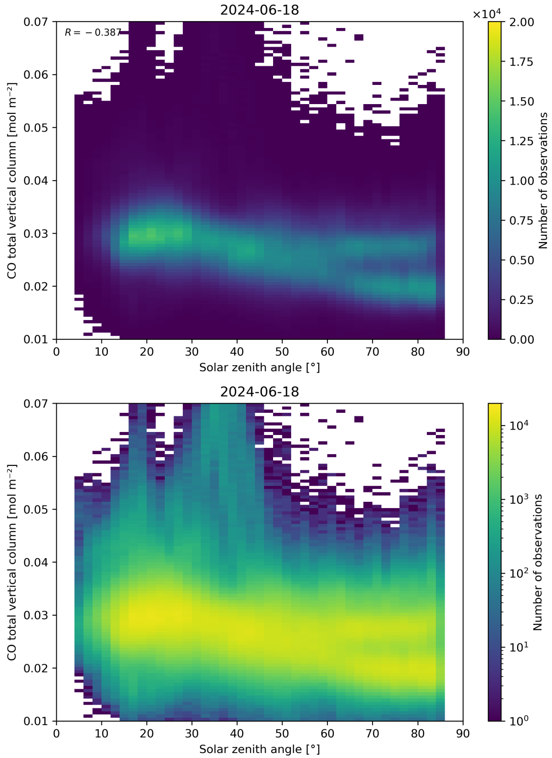
Figure 61: Scatter density plot of “Solar zenith angle” against “CO total vertical column” for 2024-06-17 to 2024-06-19.
