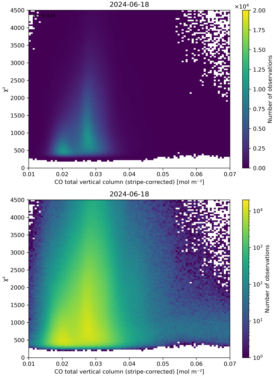
Figure 37: Scatter density plot of “CO total vertical column (stripe-corrected)” against “ \chi^2 ” for 2024-06-17 to 2024-06-19.
