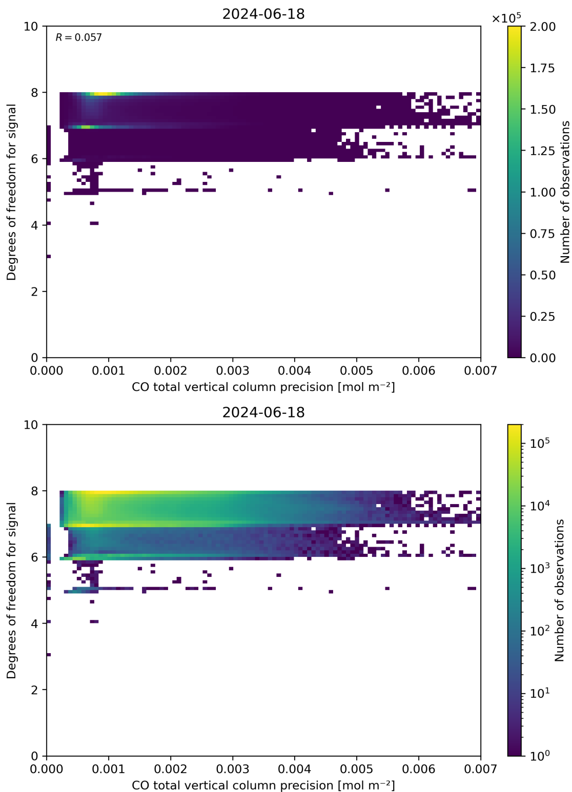
Figure 45: Scatter density plot of “CO total vertical column precision” against “Degrees of freedom for signal” for 2024-06-17 to 2024-06-19.
