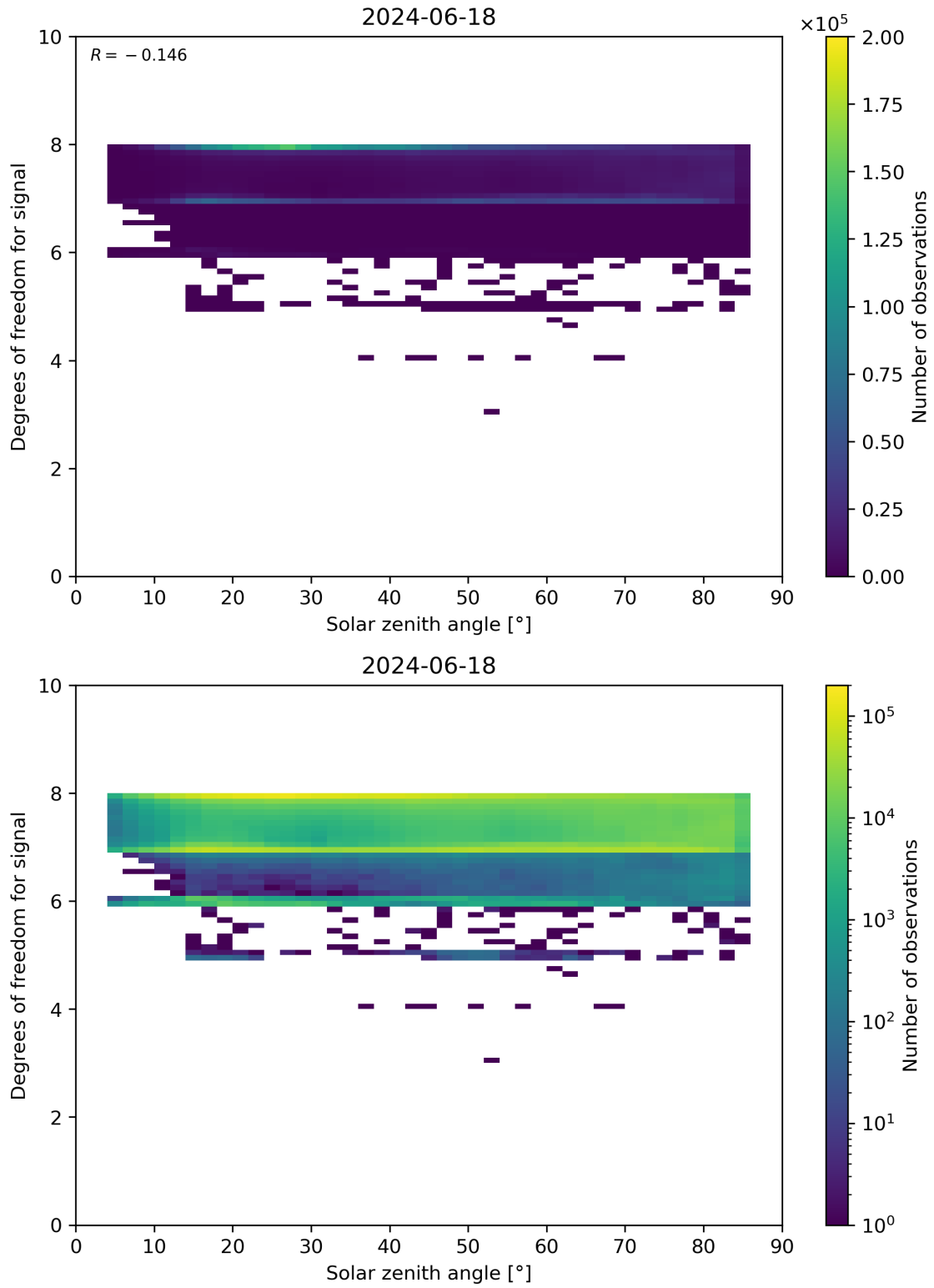
Figure 65: Scatter density plot of “Solar zenith angle” against “Degrees of freedom for signal” for 2024-06-17 to 2024-06-19.
