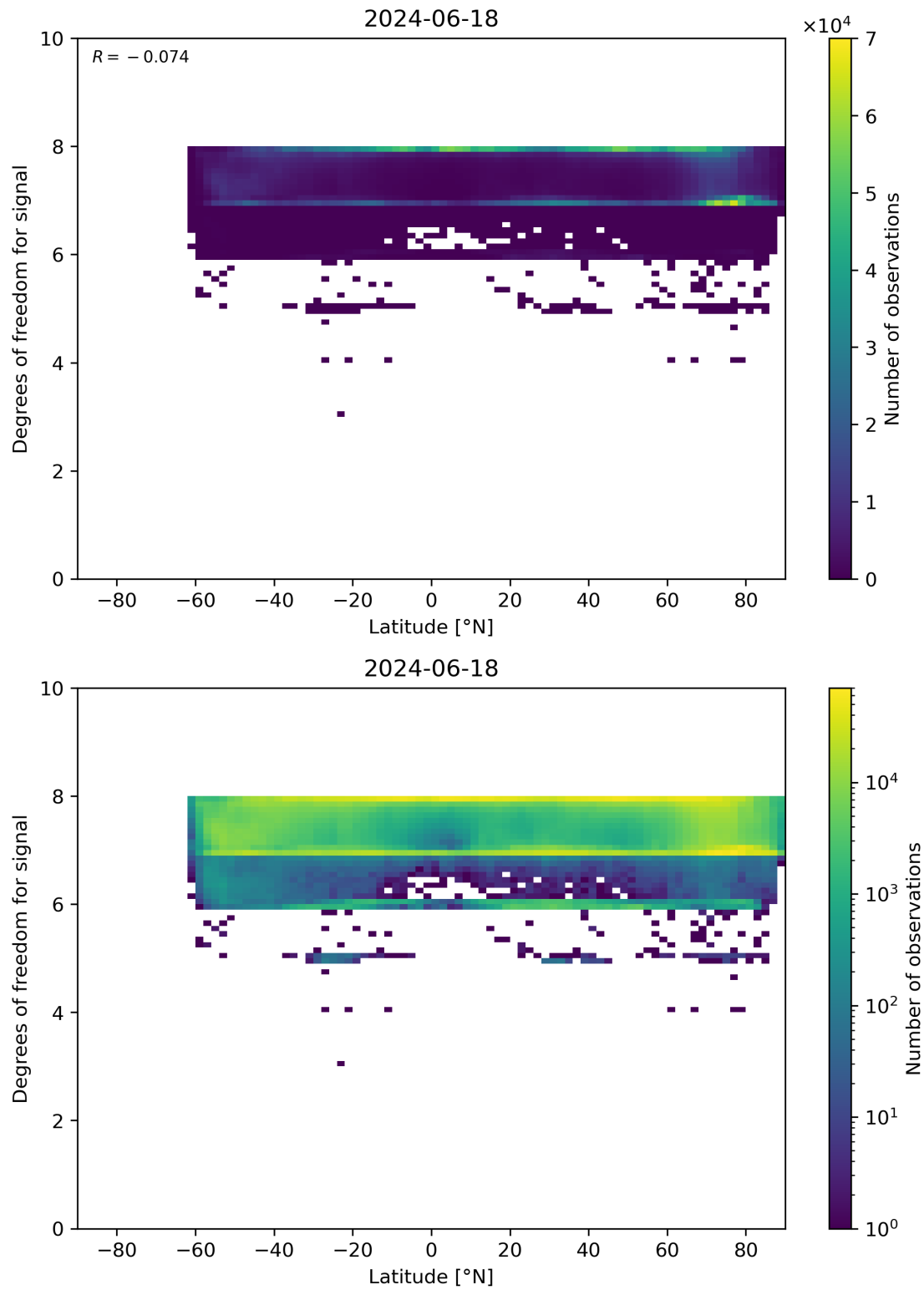
Figure 55: Scatter density plot of “Latitude” against “Degrees of freedom for signal” for 2024-06-17 to 2024-06-19.
