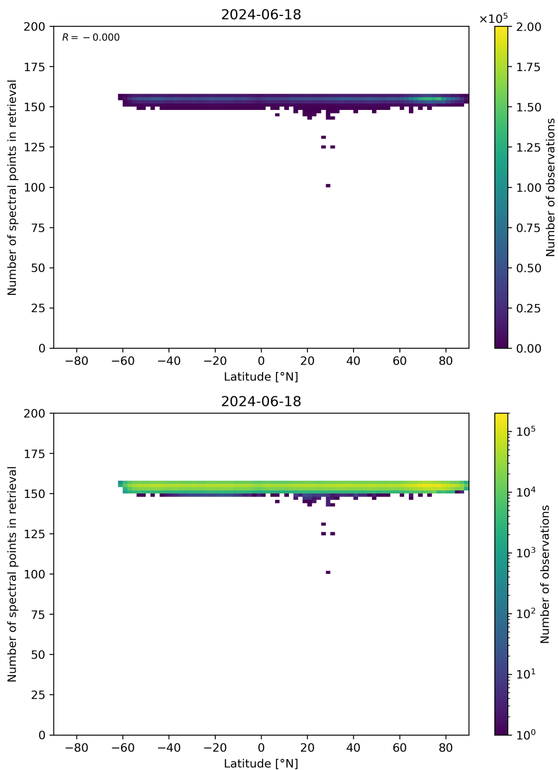
Figure 57: Scatter density plot of “Latitude” against “Number of spectral points in retrieval” for 2024-06-17 to 2024-06-19.
