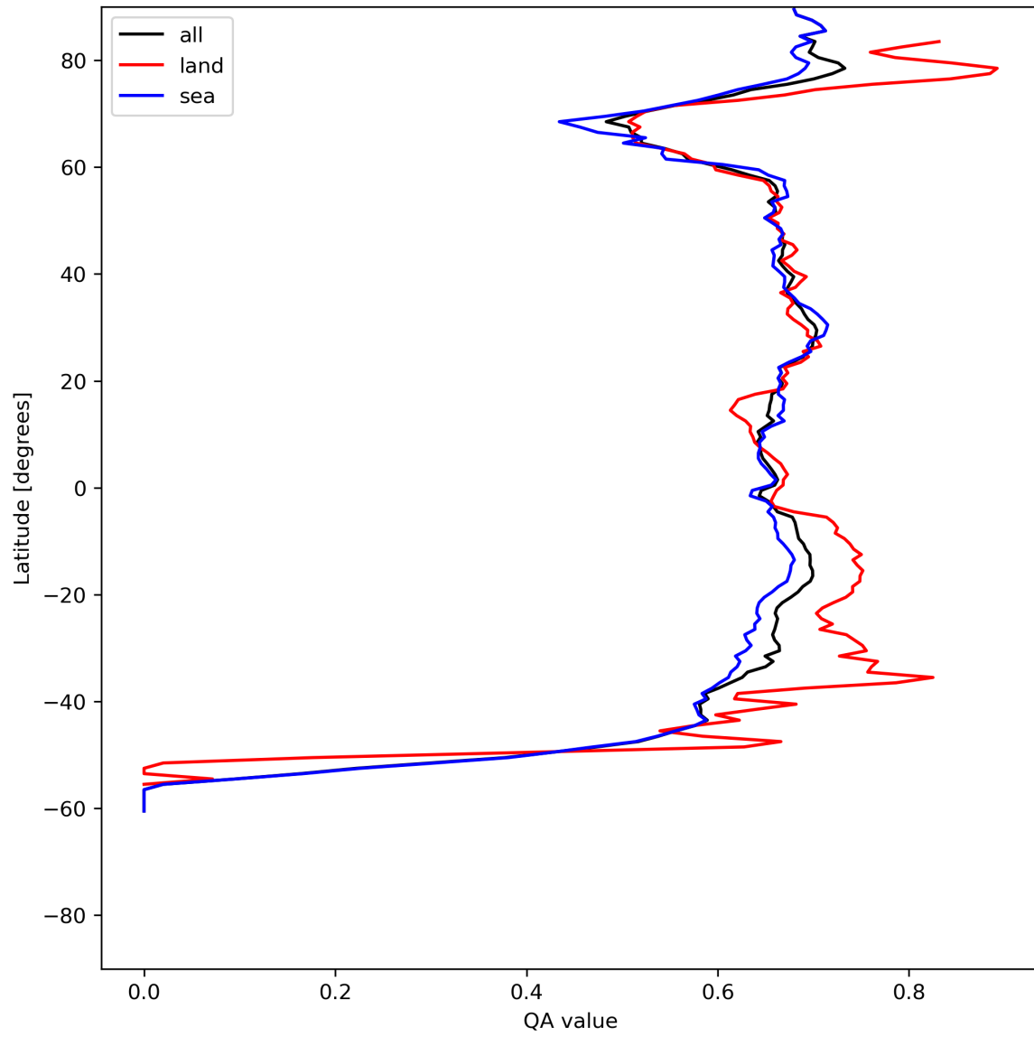
Figure 9: Zonal average of “QA value” for 2024-06-17 to 2024-06-19.
