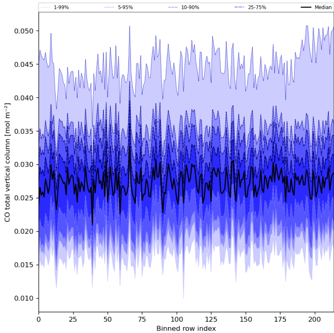
Figure 26: Along track statistics of “CO total vertical column” for 2024-06-17 to 2024-06-19
