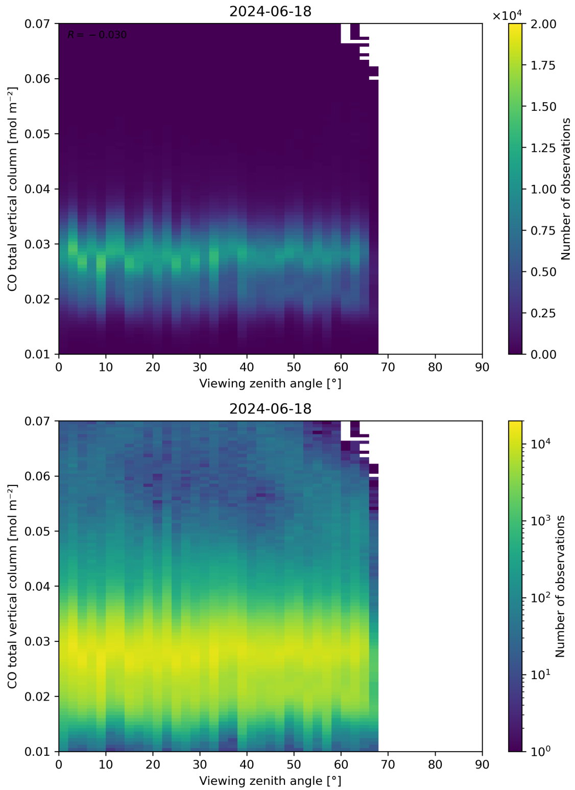
Figure 69: Scatter density plot of “Viewing zenith angle” against “CO total vertical column” for 2024-06-17 to 2024-06-19.
