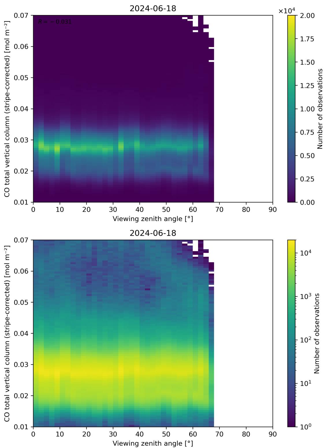
Figure 70: Scatter density plot of “Viewing zenith angle” against “CO total vertical column (stripe-corrected)” for 2024-06-17 to 2024-06-19.
