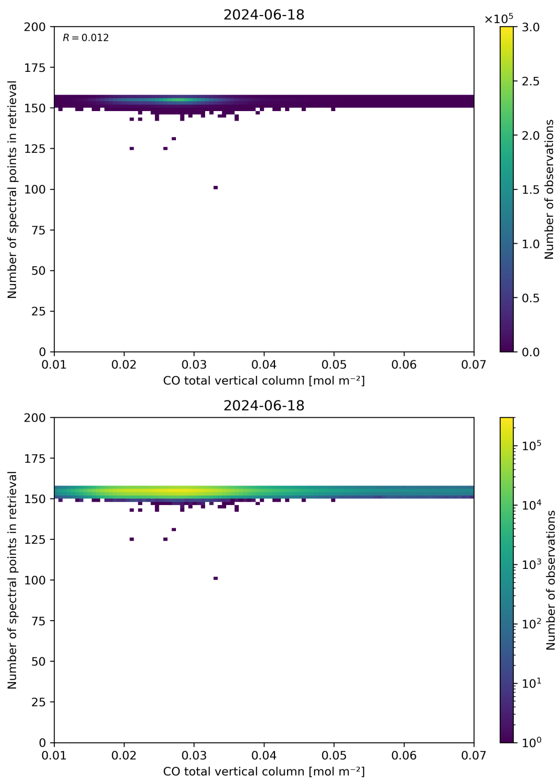
Figure 43: Scatter density plot of “CO total vertical column” against “Number of spectral points in retrieval” for 2024-06-17 to 2024-06-19.
