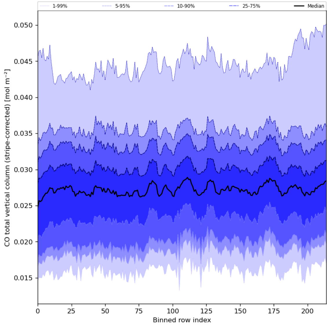
Figure 27: Along track statistics of “CO total vertical column (stripe-corrected)” for 2024-06-17 to 2024-06-19
