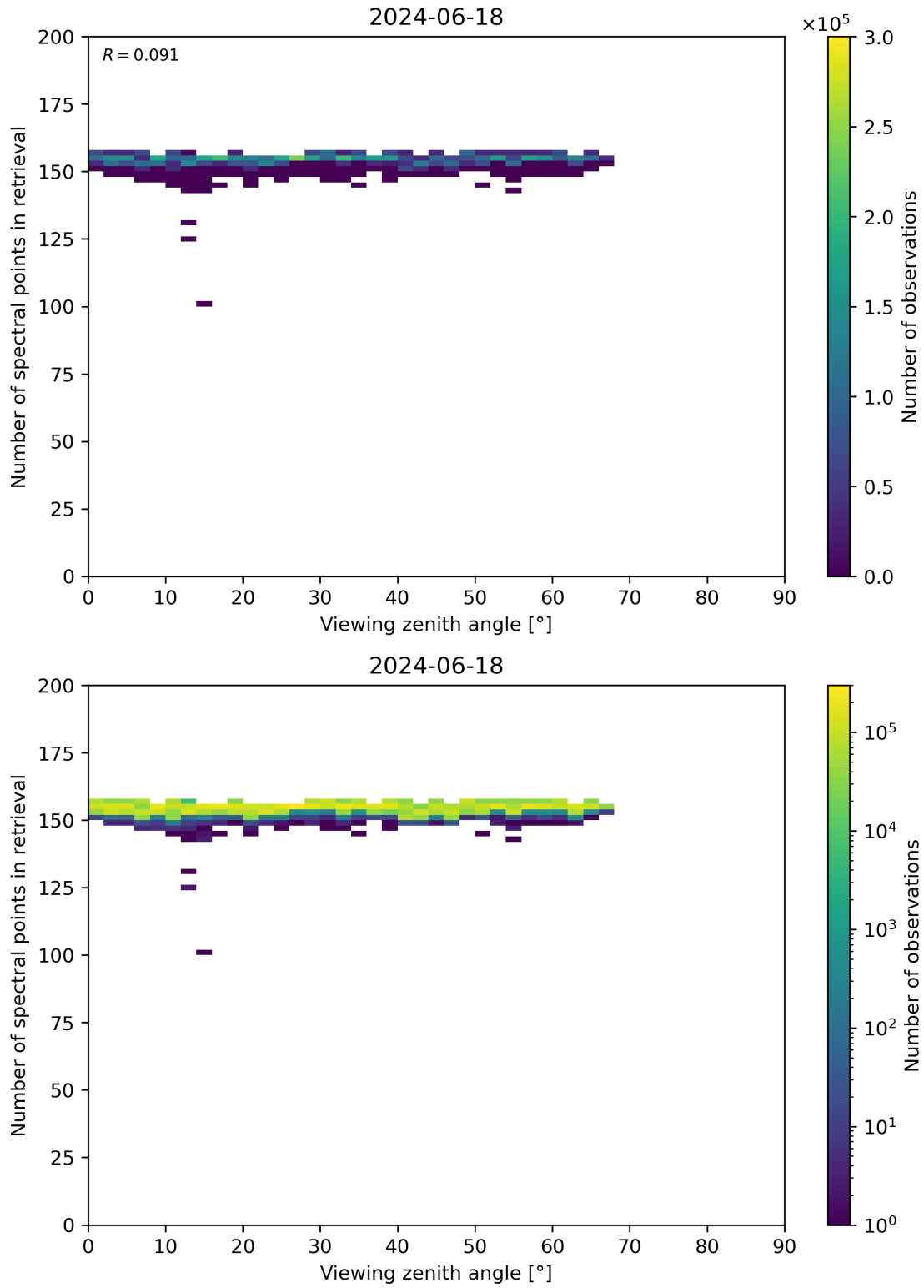
Figure 76: Scatter density plot of “Viewing zenith angle” against “Number of spectral points in retrieval” for 2024-06-17 to 2024-06-19.
