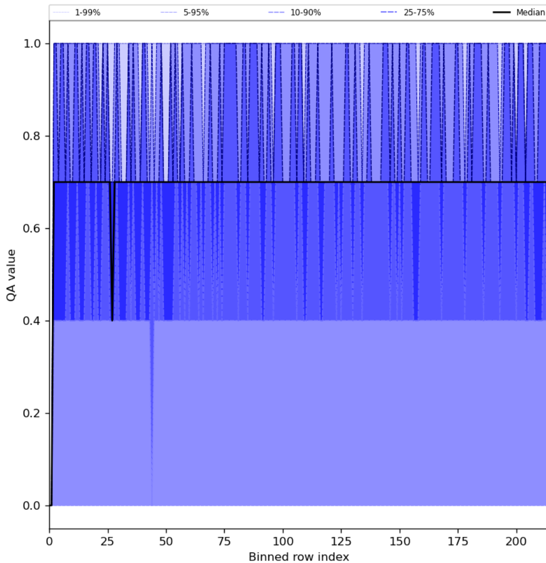
Figure 25: Along track statistics of “QA value” for 2024-06-17 to 2024-06-19
