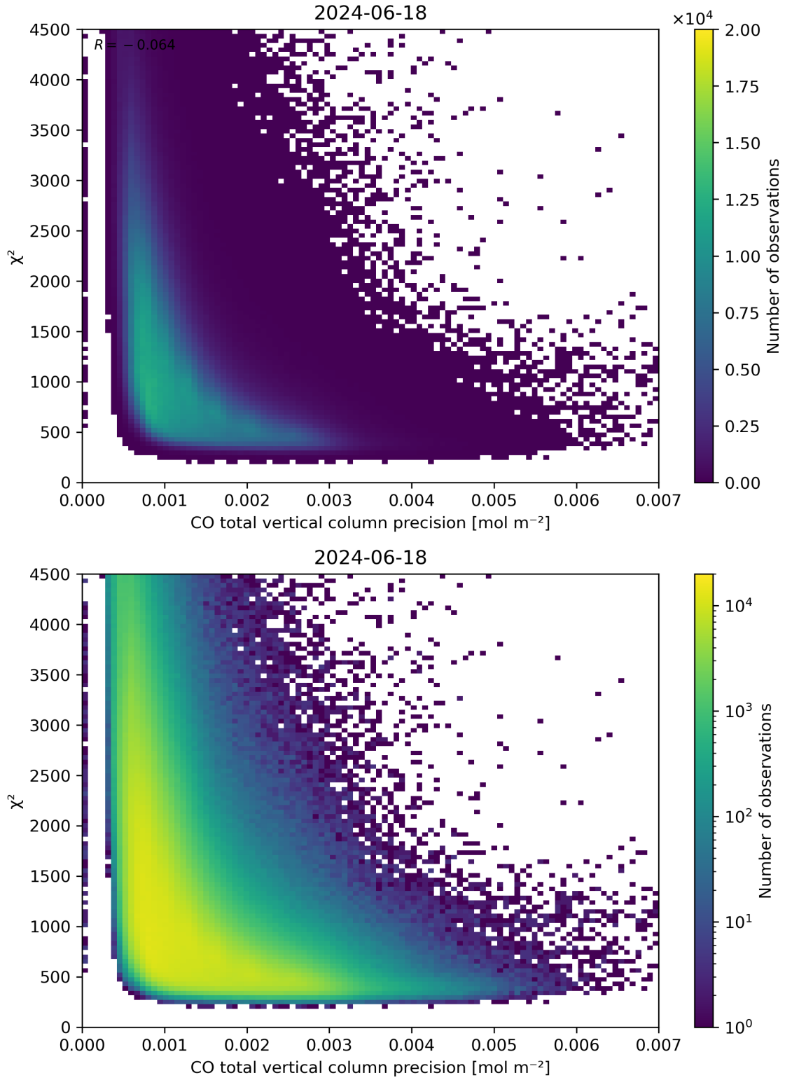
Figure 44: Scatter density plot of “CO total vertical column precision” against “ \chi^2 ” for 2024-06-17 to 2024-06-19.
