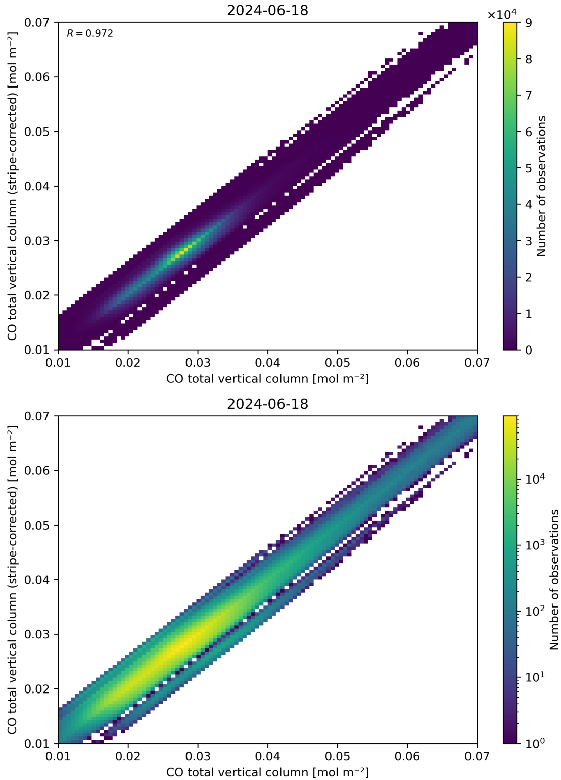
Figure 33: Scatter density plot of “CO total vertical column” against “CO total vertical column (stripe-corrected)” for 2024-06-17 to 2024-06-19.
