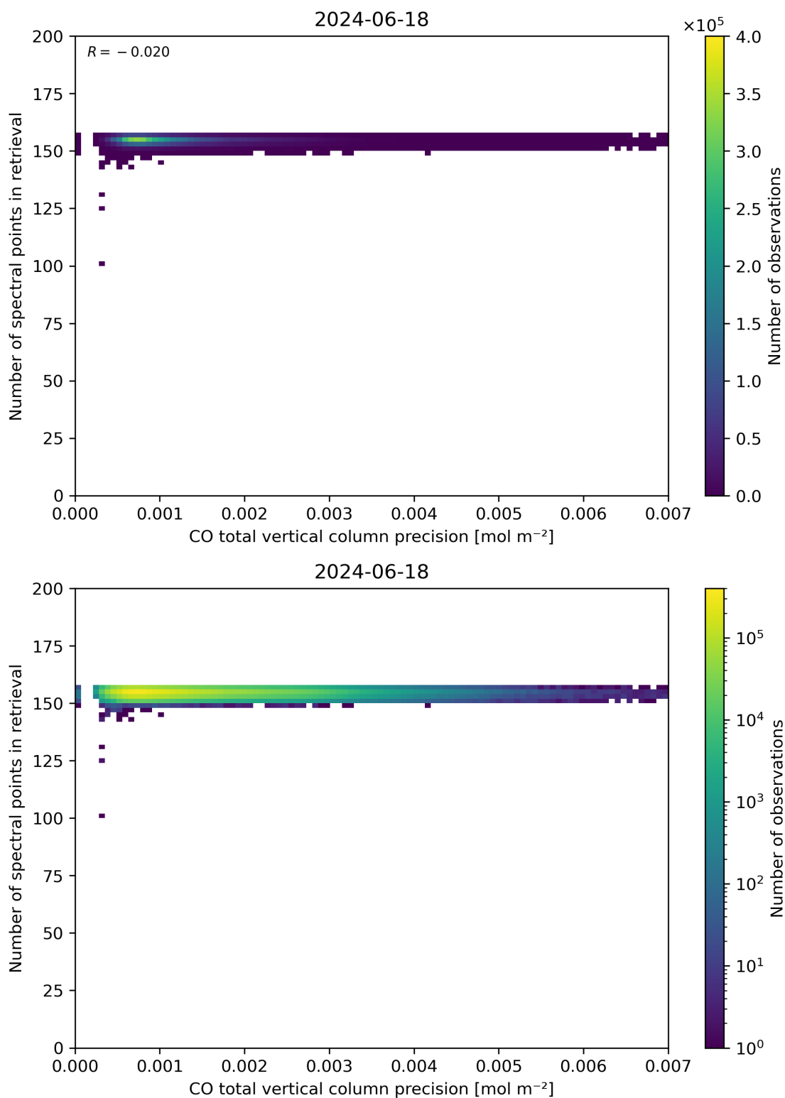
Figure 47: Scatter density plot of “CO total vertical column precision” against “Number of spectral points in retrieval” for 2024-06-17 to 2024-06-19.
