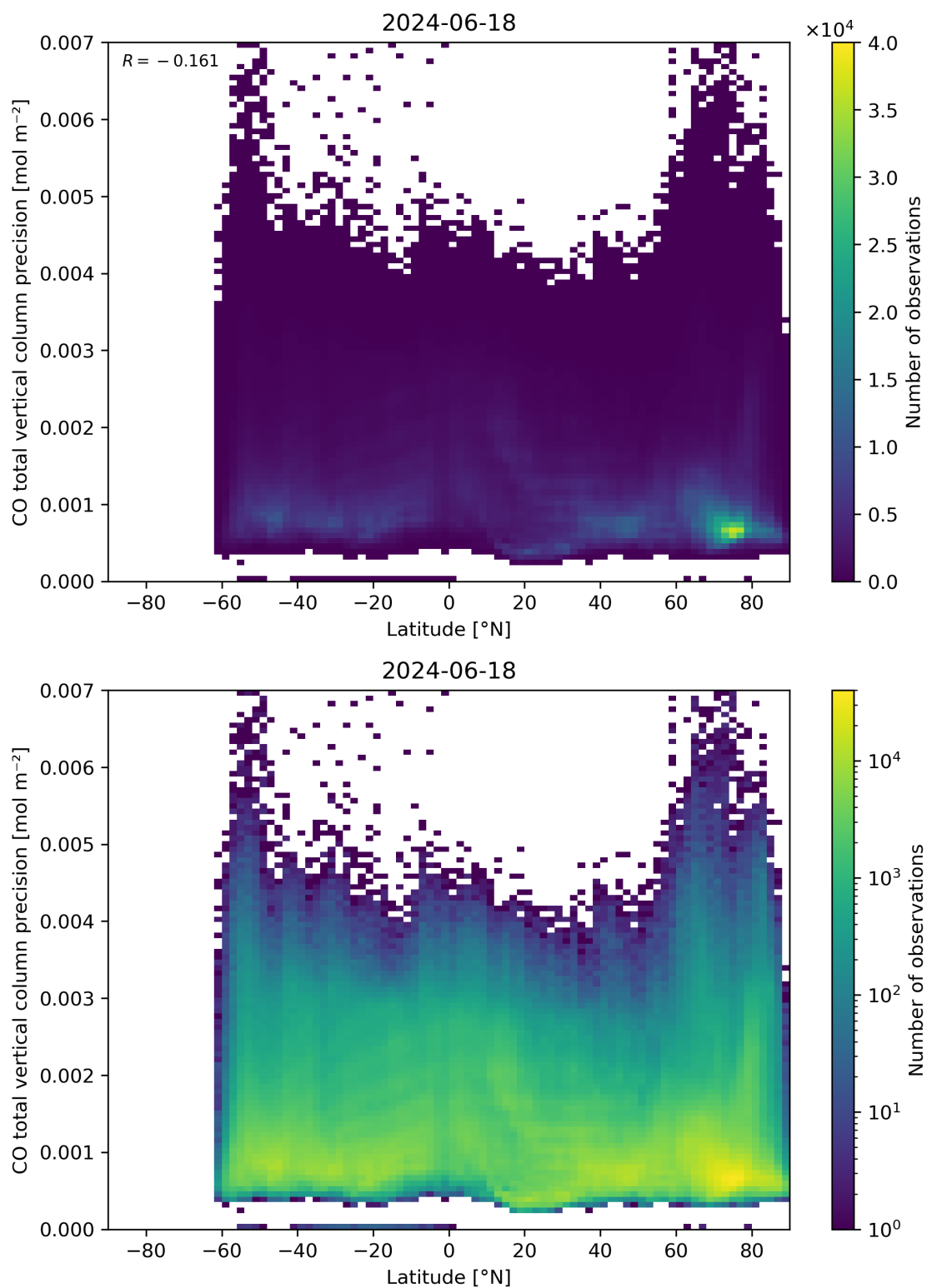
Figure 53: Scatter density plot of “Latitude” against “CO total vertical column precision” for 2024-06-17 to 2024-06-19.
