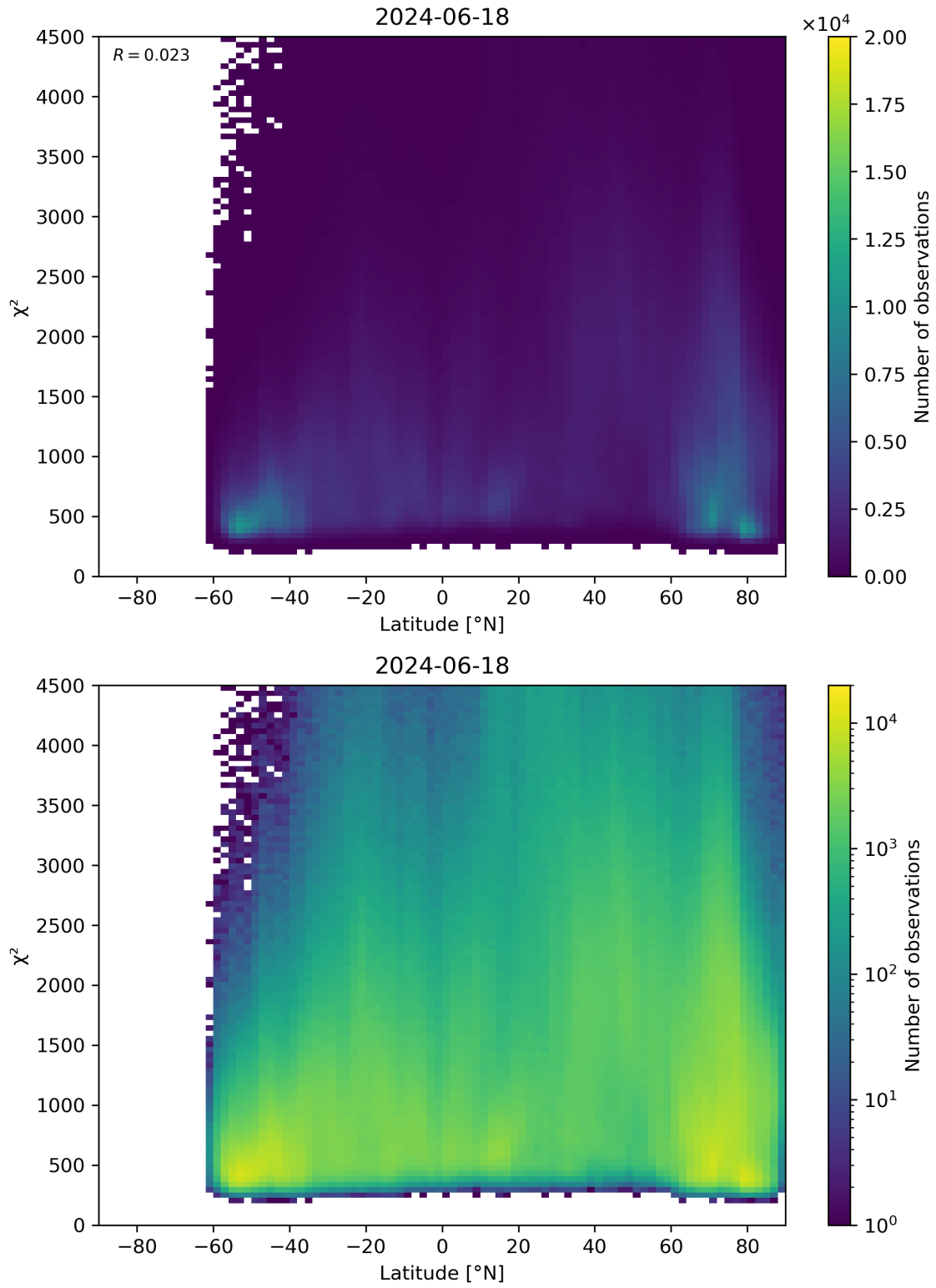
Figure 54: Scatter density plot of “Latitude” against “ \chi^2 ” for 2024-06-17 to 2024-06-19.
