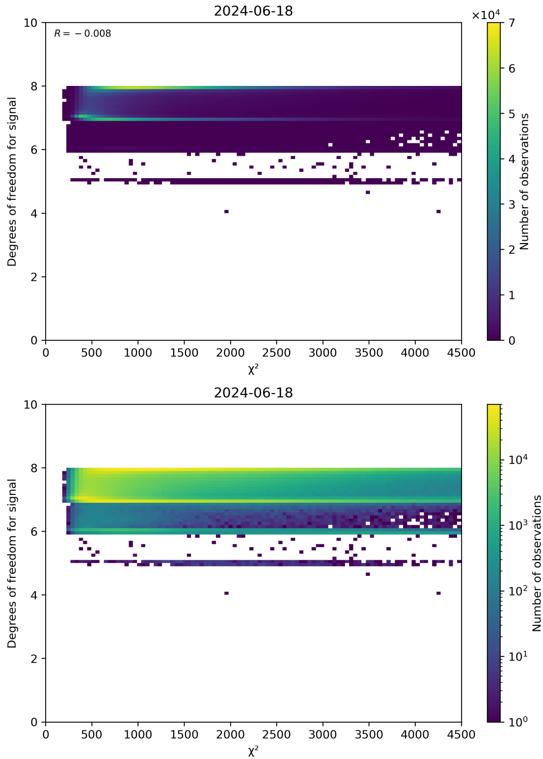
Figure 48: Scatter density plot of “ \chi^2 ” against “Degrees of freedom for signal” for 2024-06-17 to 2024-06-19.
