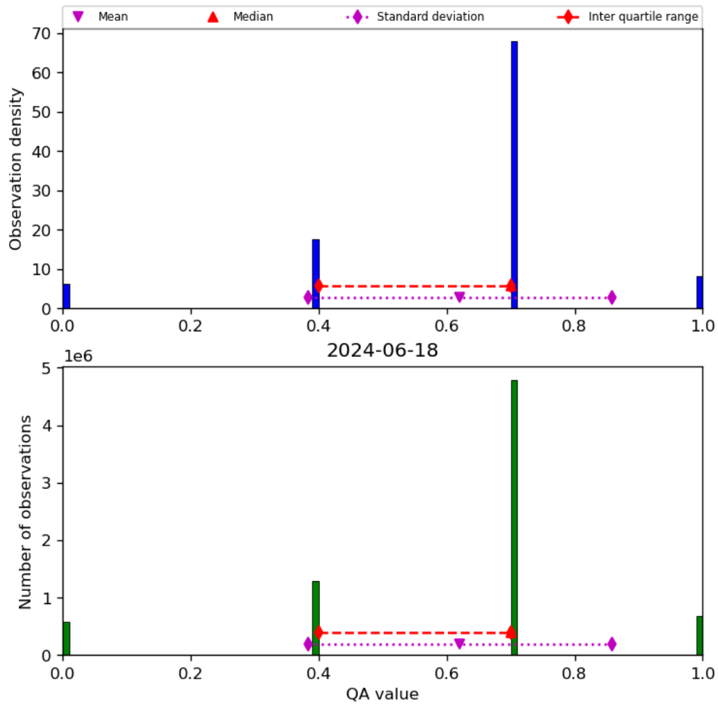
Figure 17: Histogram of "QA value" for 2024-06-17 to 2024-06-19
