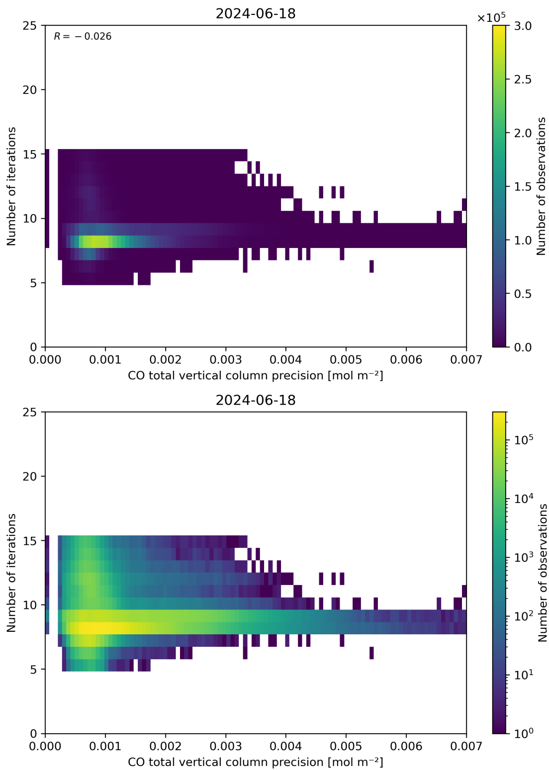
Figure 46: Scatter density plot of “CO total vertical column precision” against “Number of iterations” for 2024-06-17 to 2024-06-19.
