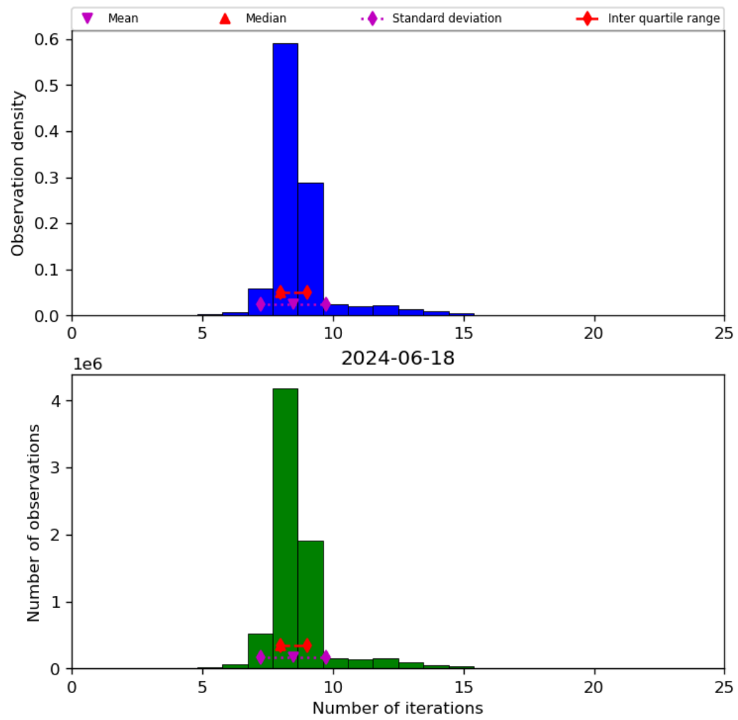
Figure 24: Histogram of “Number of iterations” for 2024-06-17 to 2024-06-19
