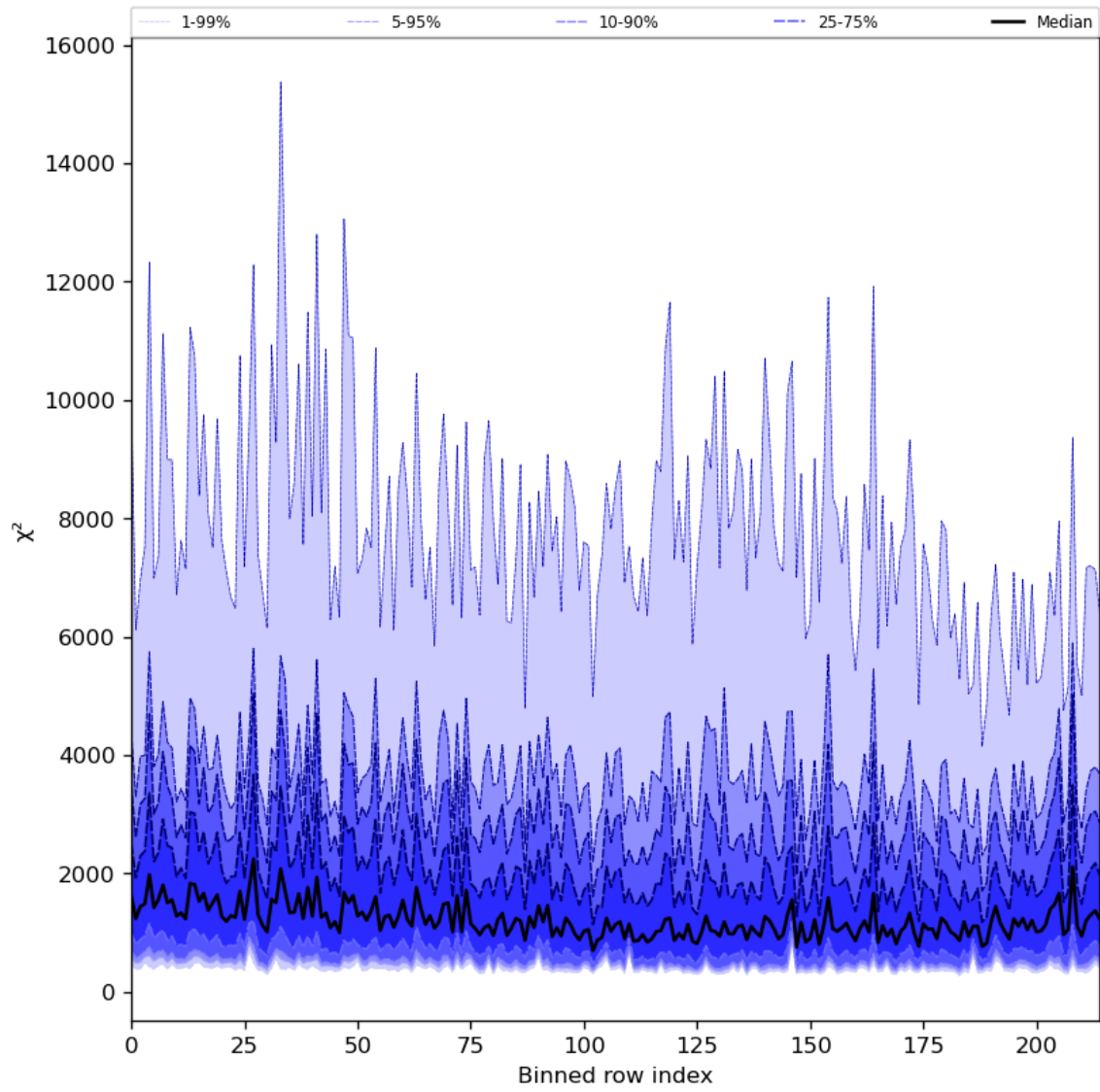
Figure 30: Along track statistics of “ \chi^2 ” for 2024-06-17 to 2024-06-19
