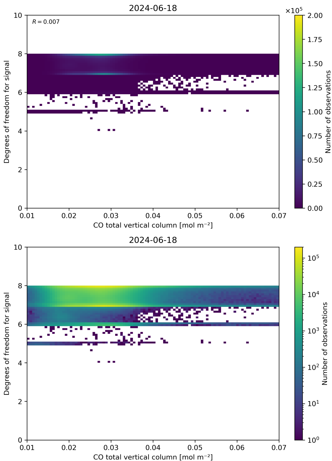
Figure 41: Scatter density plot of “CO total vertical column” against “Degrees of freedom for signal” for 2024-06-17 to 2024-06-19.
