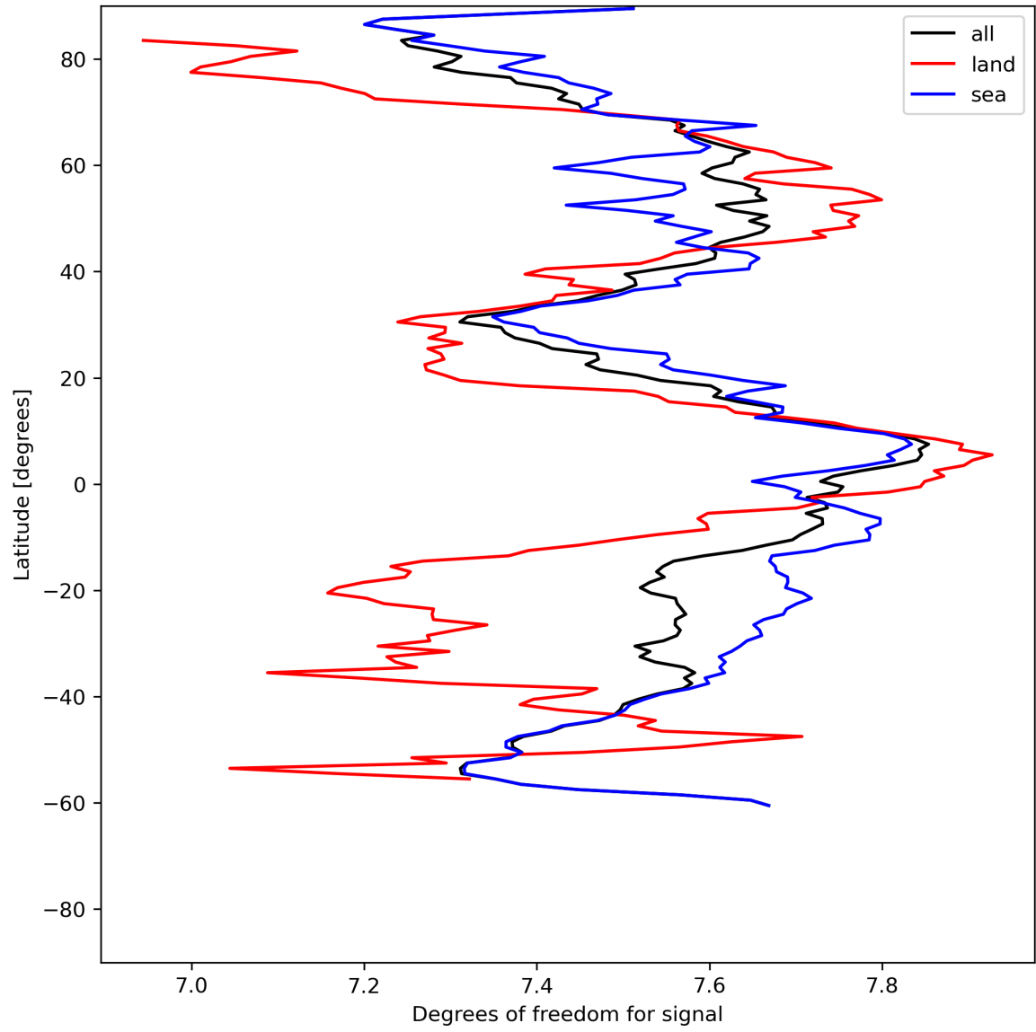
Figure 15: Zonal average of “Degrees of freedom for signal” for 2024-06-17 to 2024-06-19.
