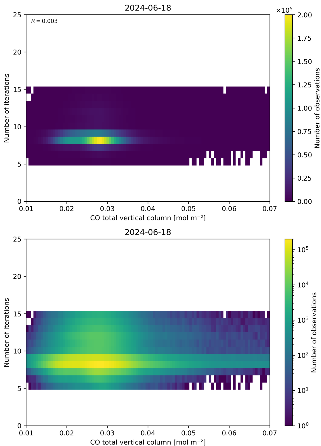
Figure 42: Scatter density plot of “CO total vertical column” against “Number of iterations” for 2024-06-17 to 2024-06-19.
