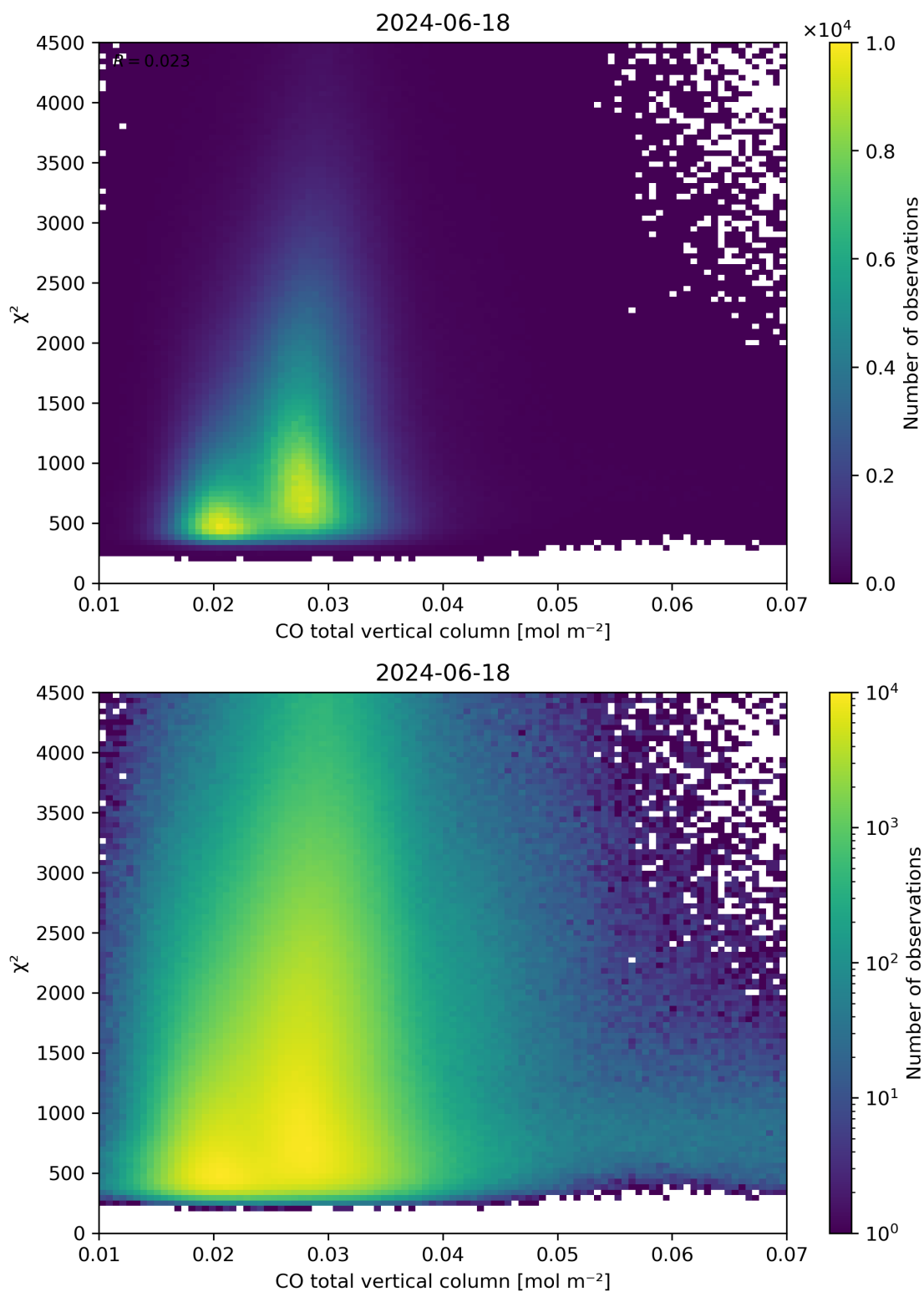
Figure 35: Scatter density plot of “CO total vertical column” against “ \chi^2 ” for 2024-06-17 to 2024-06-19.
