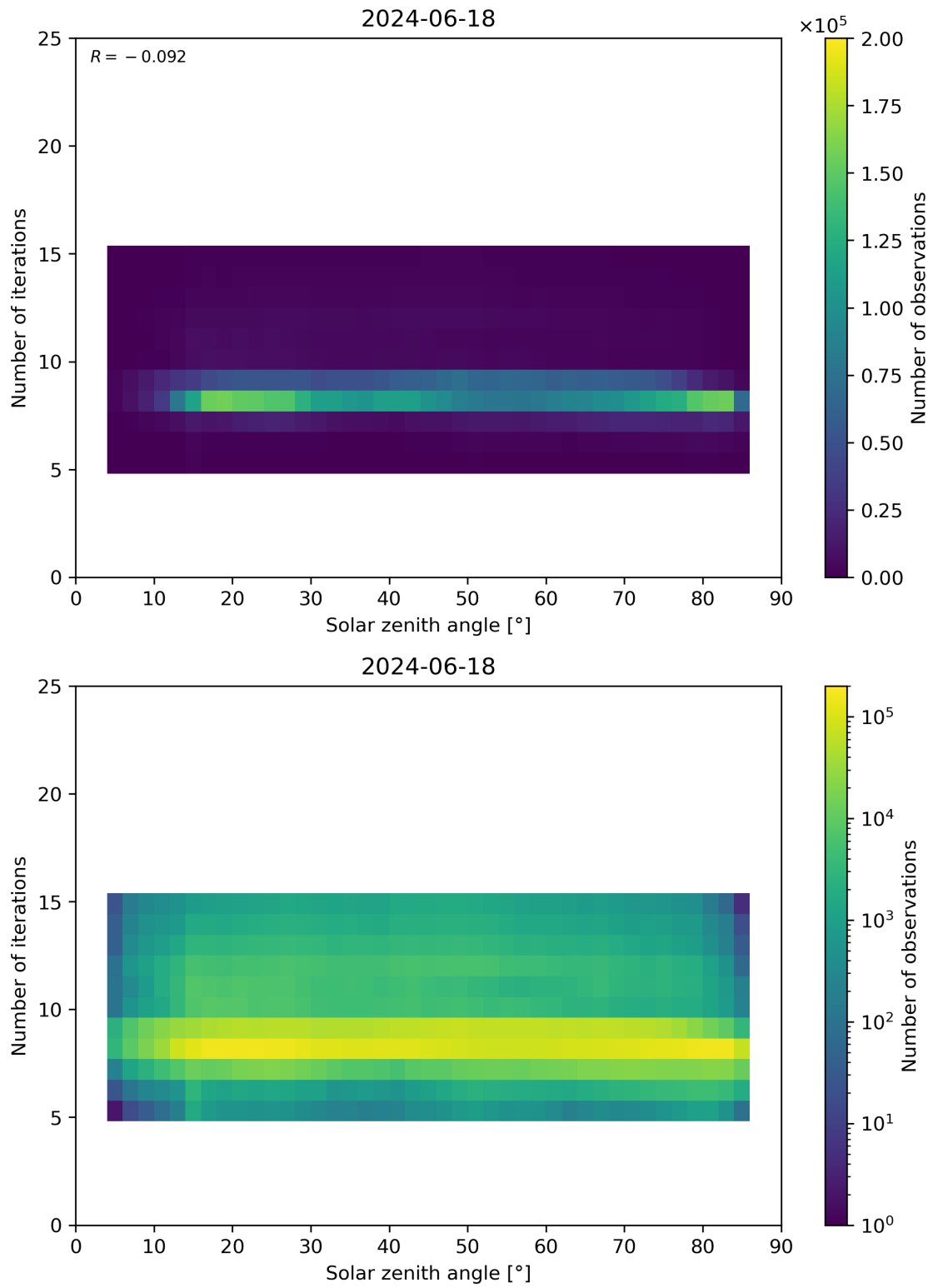
Figure 67: Scatter density plot of “Solar zenith angle” against “Number of iterations” for 2024-06-17 to 2024-06-19.
