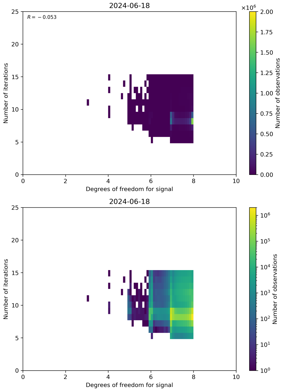
Figure 50: Scatter density plot of “Degrees of freedom for signal” against “Number of iterations” for 2024-06-17 to 2024-06-19.
