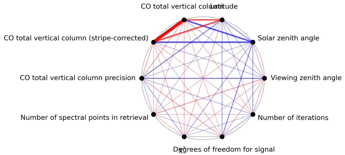
Figure 1: Map of correlation graph for 2024-06-17 to 2024-06-19.
