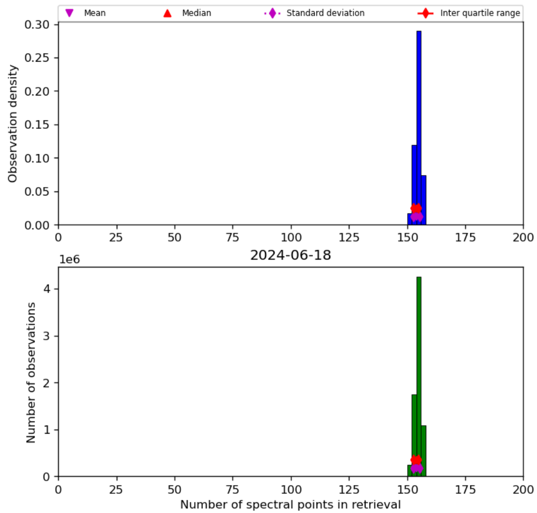
Figure 21: Histogram of “Number of spectral points in retrieval” for 2024-06-17 to 2024-06-19
