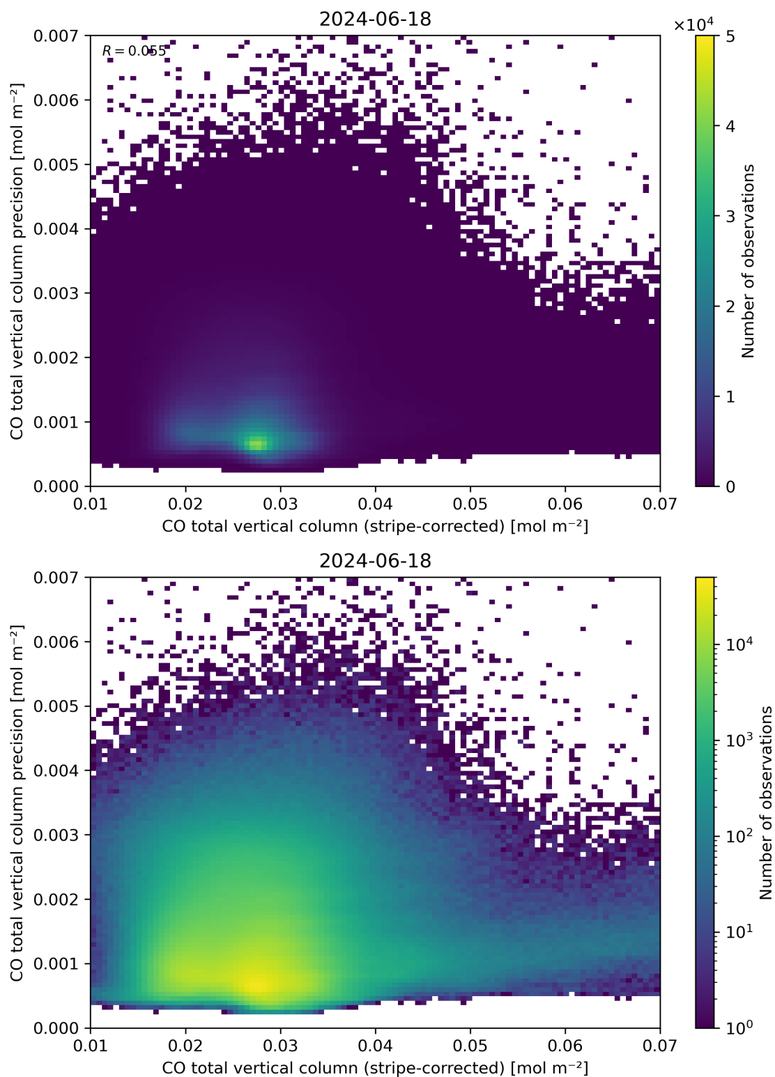
Figure 36: Scatter density plot of “CO total vertical column (stripe-corrected)” against “CO total vertical column precision” for 2024-06-17 to 2024-06-19.
