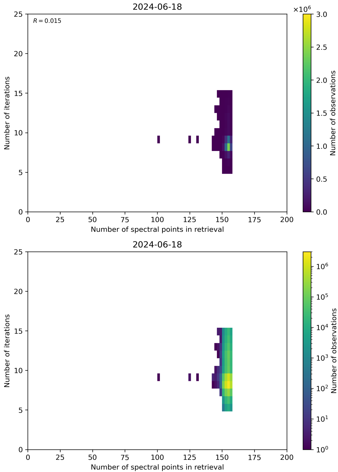
Figure 60: Scatter density plot of “Number of spectral points in retrieval” against “Number of iterations” for 2024-06-17 to 2024-06-19.
