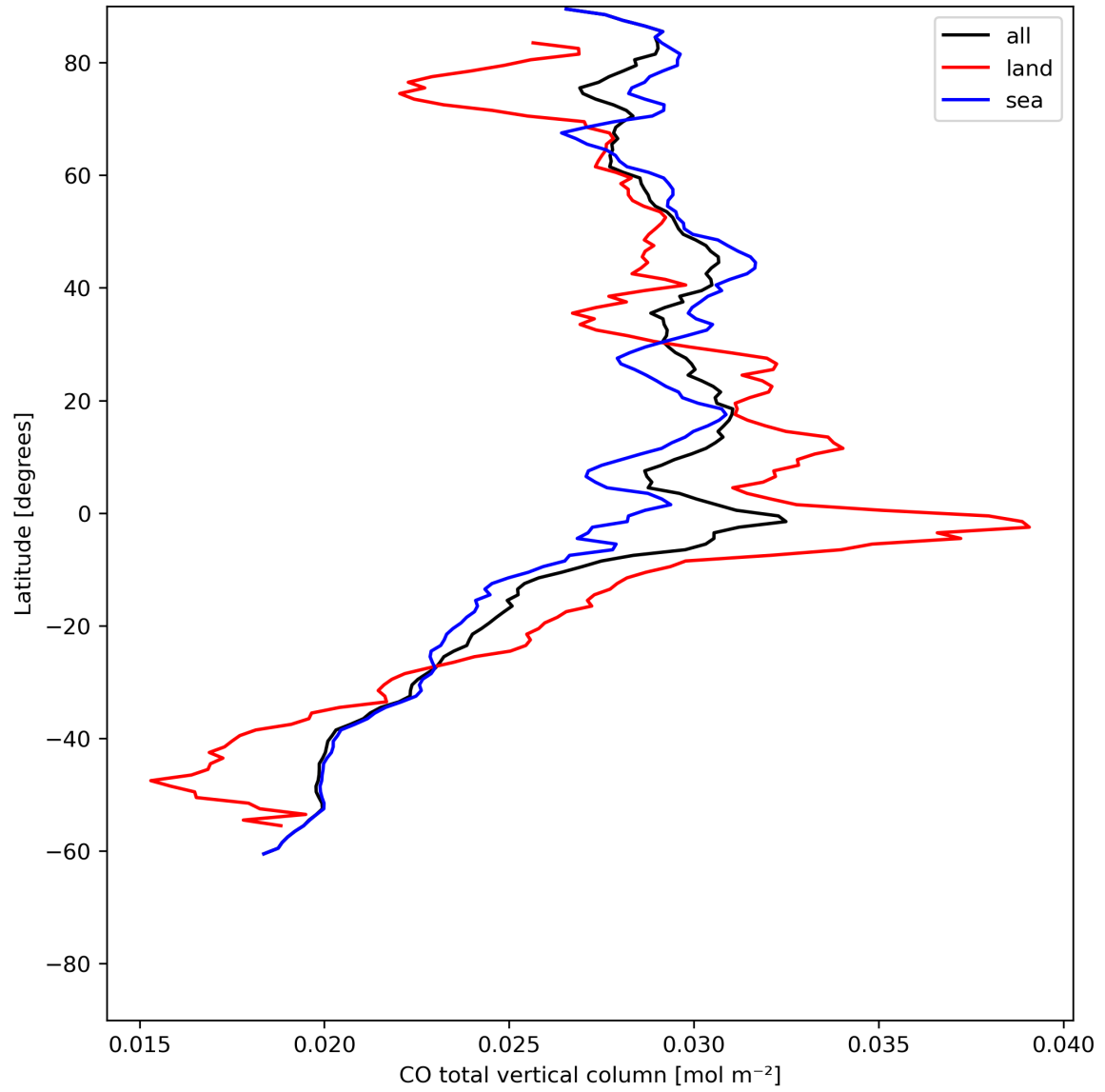
Figure 10: Zonal average of “CO total vertical column” for 2024-06-17 to 2024-06-19.
