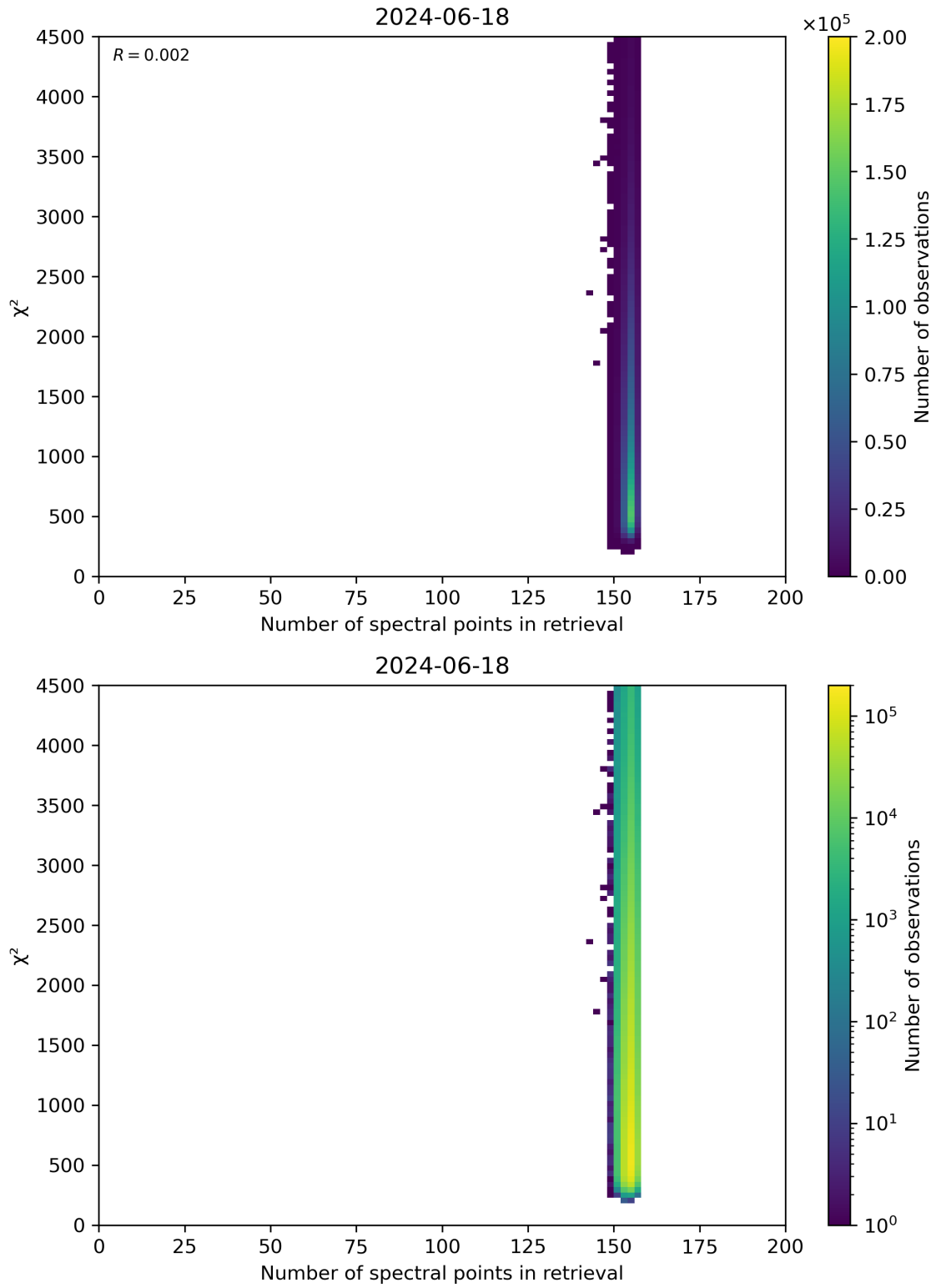
Figure 58: Scatter density plot of “Number of spectral points in retrieval” against “ \chi^2 ” for 2024-06-17 to 2024-06-19.
