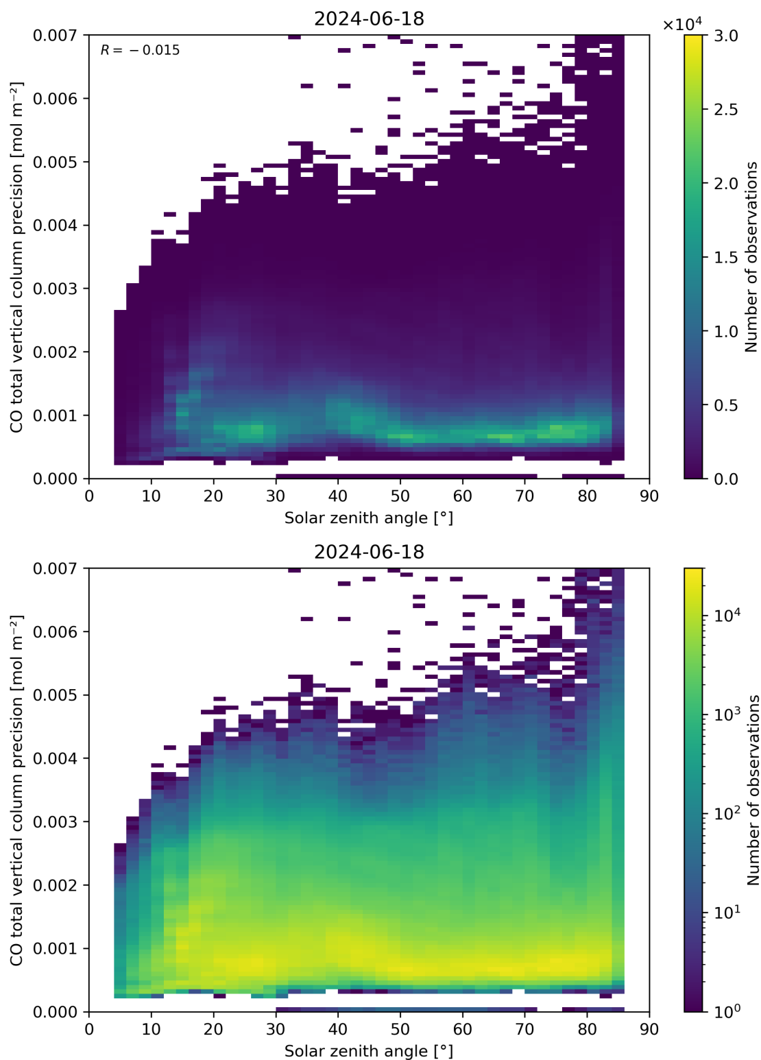
Figure 63: Scatter density plot of “Solar zenith angle” against “CO total vertical column precision” for 2024-06-17 to 2024-06-19.
