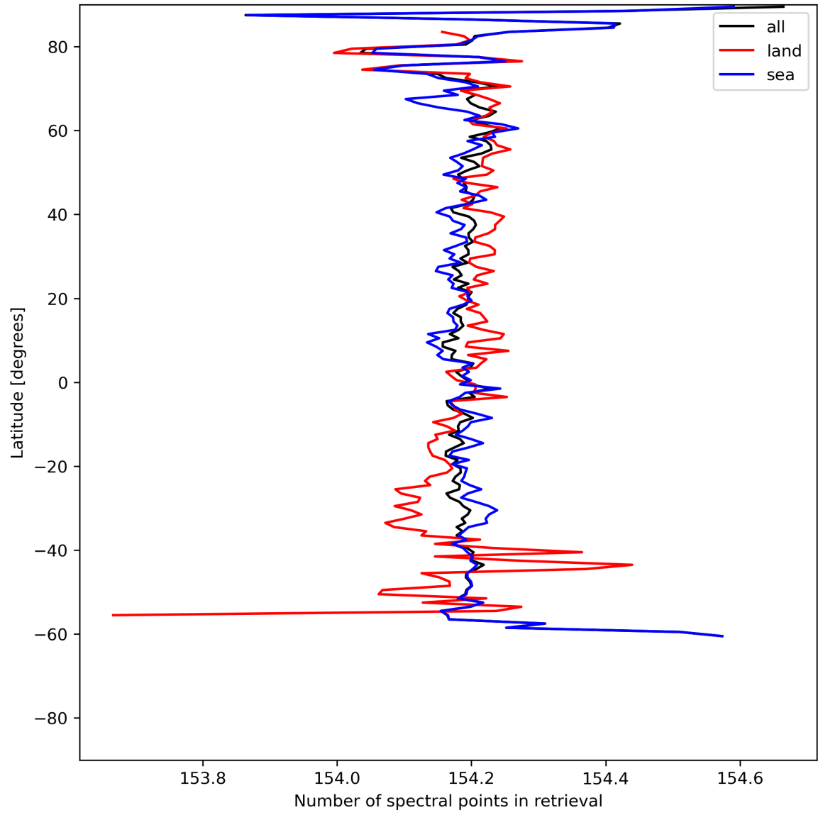
Figure 13: Zonal average of “Number of spectral points in retrieval” for 2024-06-17 to 2024-06-19.
