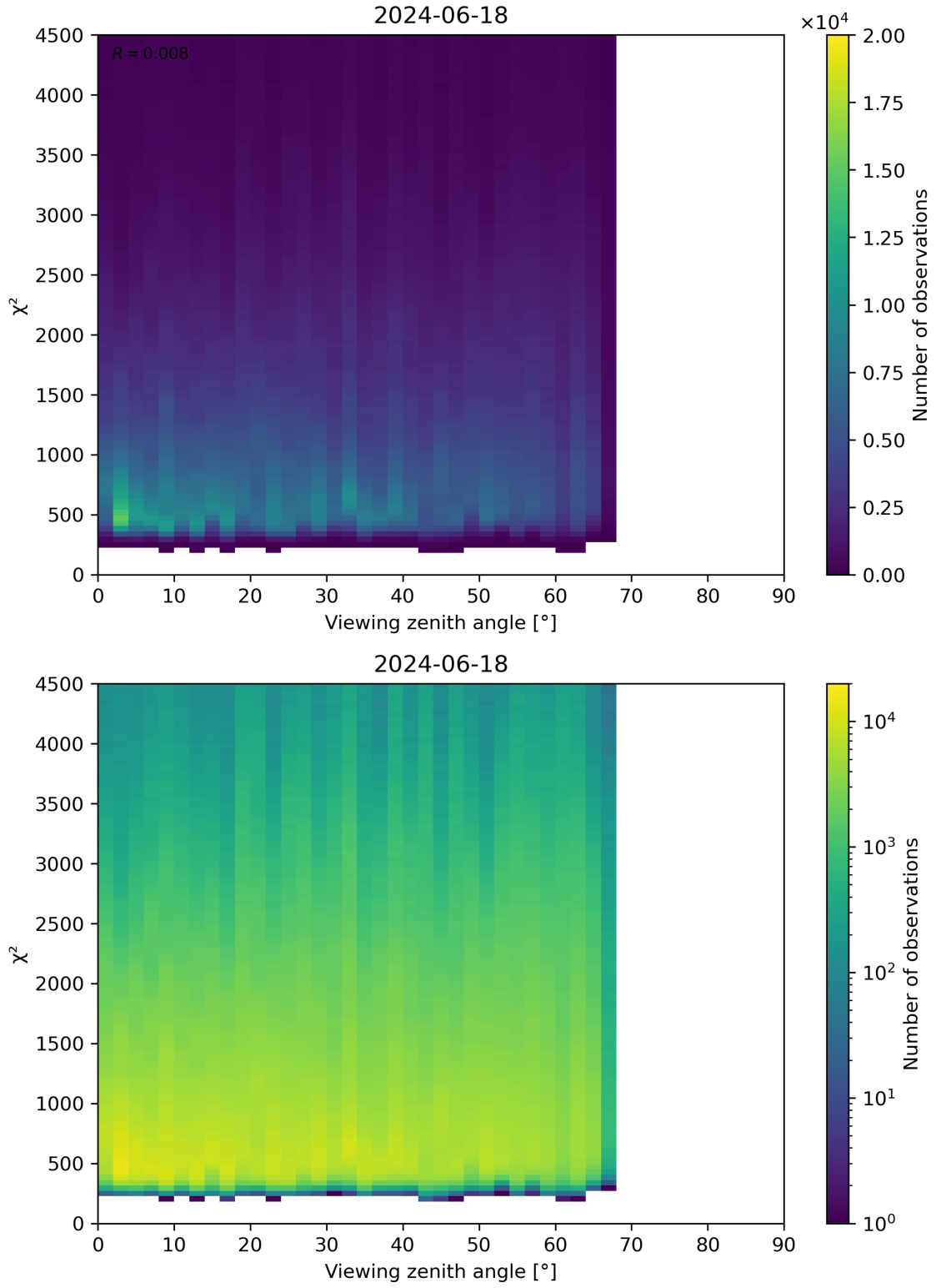
Figure 72: Scatter density plot of “Viewing zenith angle” against “ \chi^2 ” for 2024-06-17 to 2024-06-19.
