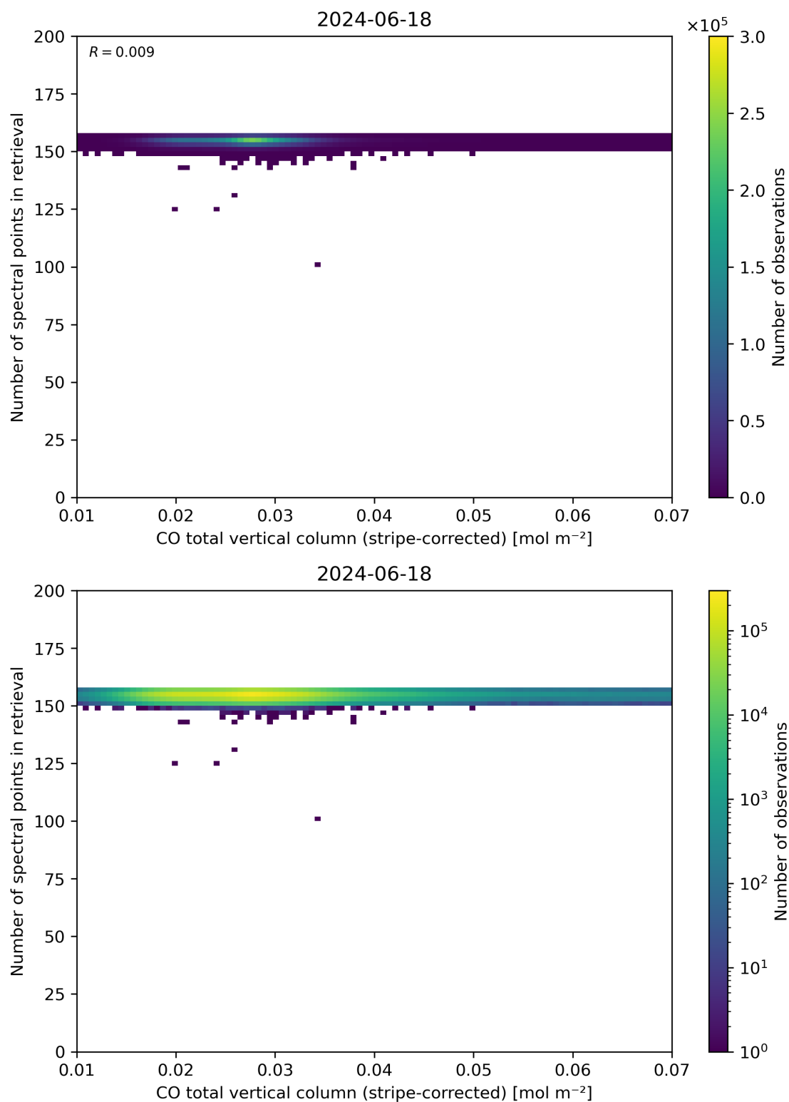
Figure 40: Scatter density plot of “CO total vertical column (stripe-corrected)” against “Number of spectral points in retrieval” for 2024-06-17 to 2024-06-19.
