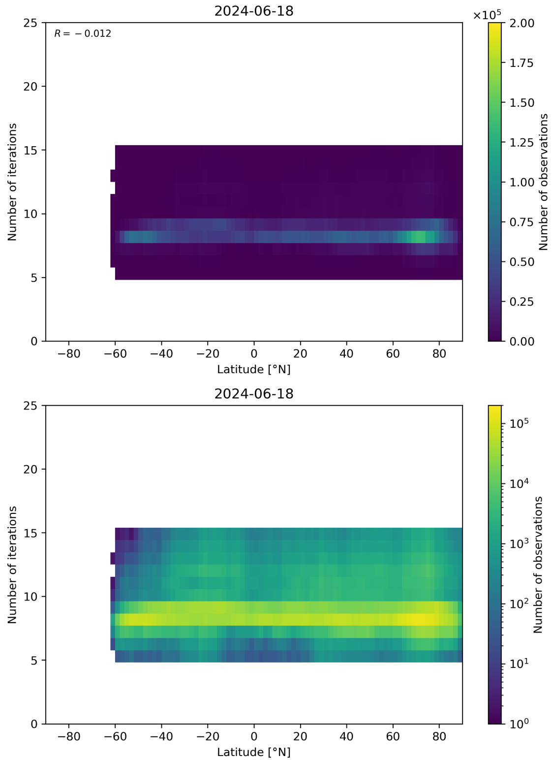
Figure 56: Scatter density plot of “Latitude” against “Number of iterations” for 2024-06-17 to 2024-06-19.
