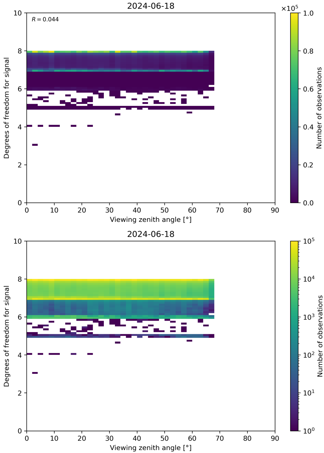
Figure 73: Scatter density plot of “Viewing zenith angle” against “Degrees of freedom for signal” for 2024-06-17 to 2024-06-19.
