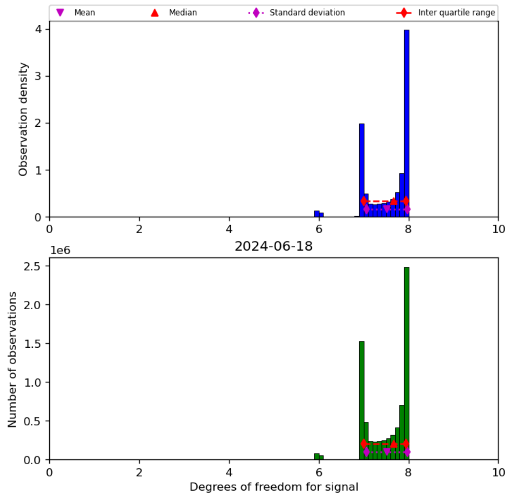
Figure 23: Histogram of “Degrees of freedom for signal” for 2024-06-17 to 2024-06-19
