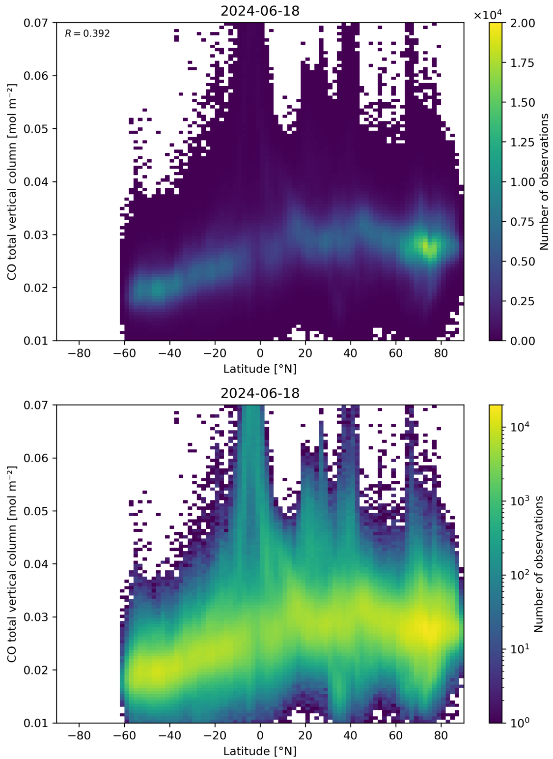
Figure 51: Scatter density plot of “Latitude” against “CO total vertical column” for 2024-06-17 to 2024-06-19.
