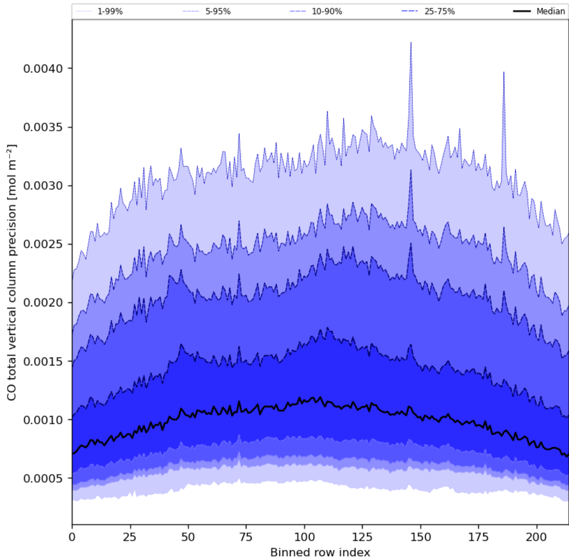
Figure 28: Along track statistics of “CO total vertical column precision” for 2024-06-17 to 2024-06-19
