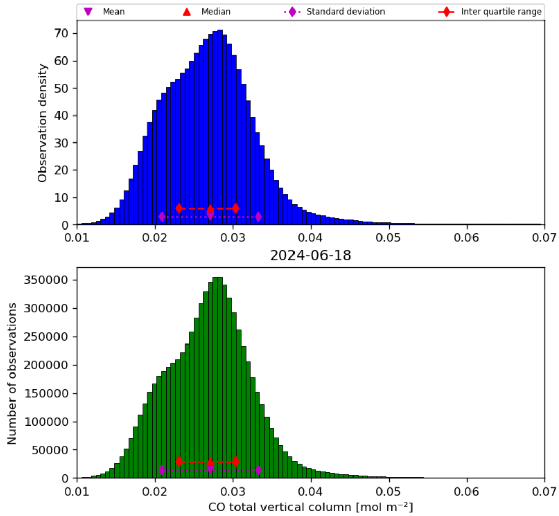
Figure 18: Histogram of “CO total vertical column” for 2024-06-17 to 2024-06-19
