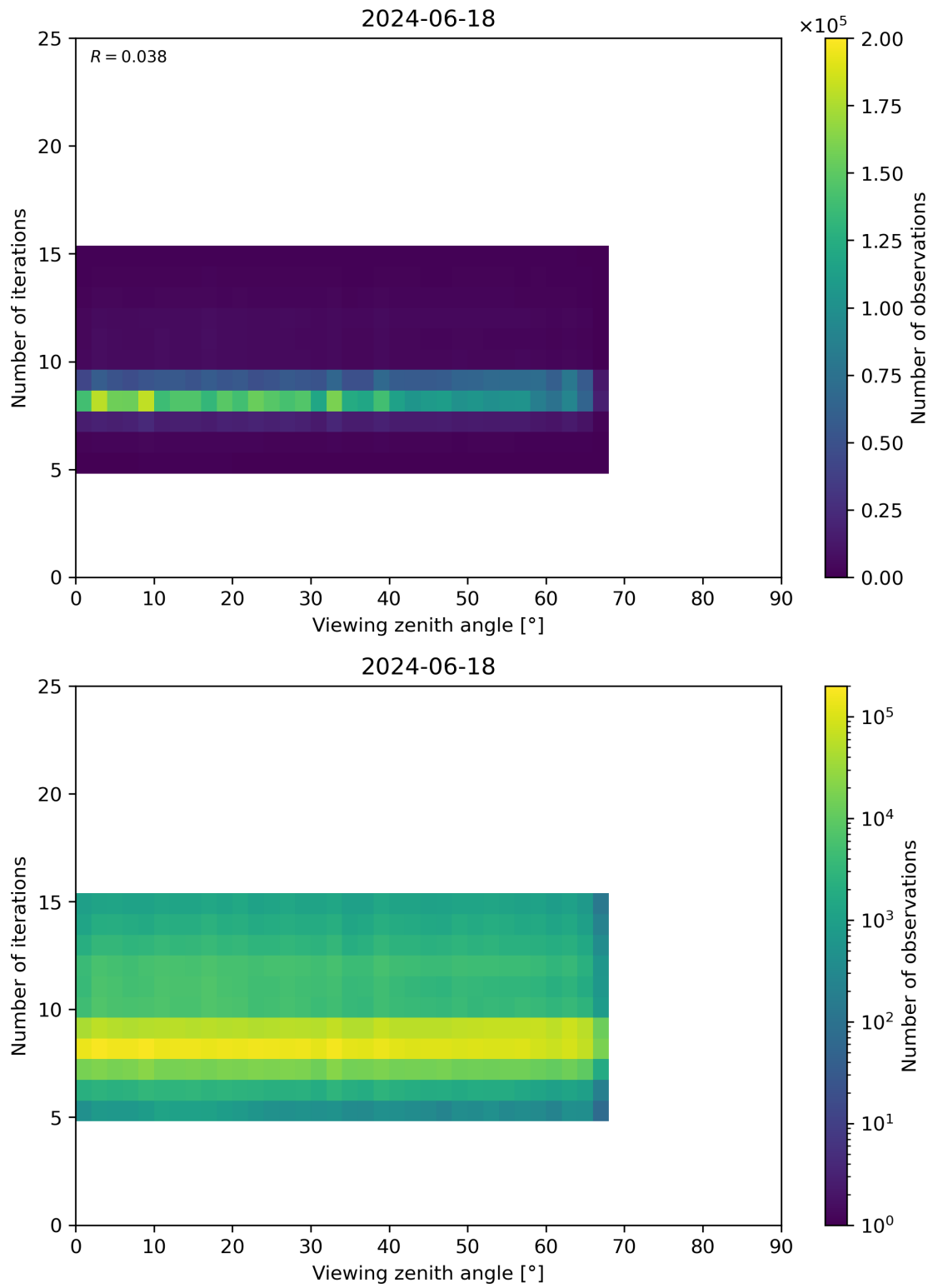
Figure 75: Scatter density plot of “Viewing zenith angle” against “Number of iterations” for 2024-06-17 to 2024-06-19.
