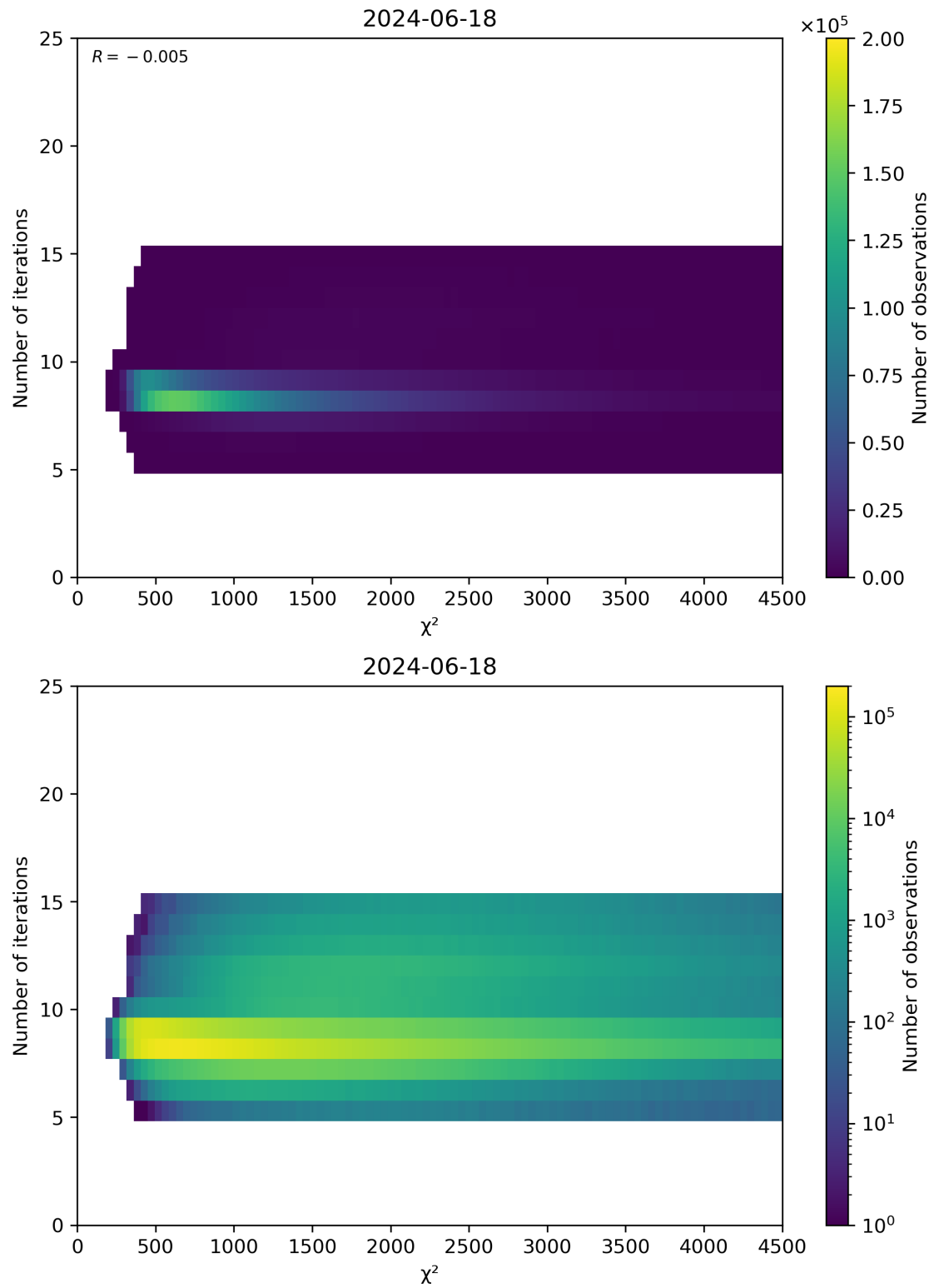
Figure 49: Scatter density plot of “ \chi^2 ” against “Number of iterations” for 2024-06-17 to 2024-06-19.
