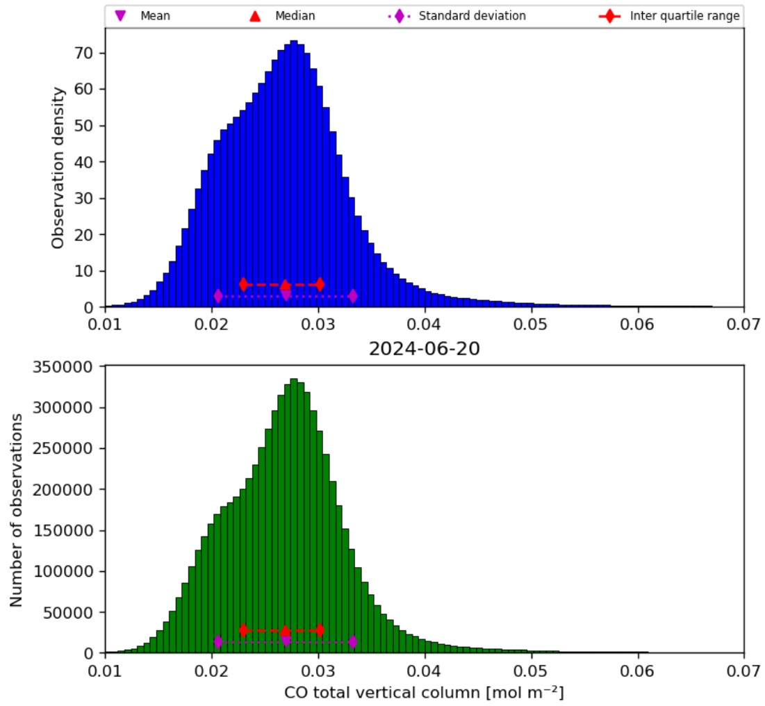
Figure 18: Histogram of “CO total vertical column” for 2024-06-19 to 2024-06-21
