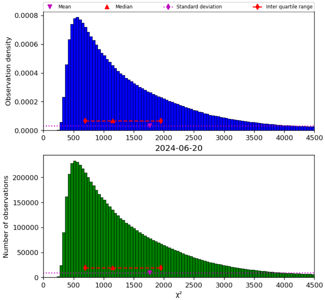
Figure 22: Histogram of “ \chi^2 ” for 2024-06-19 to 2024-06-21
