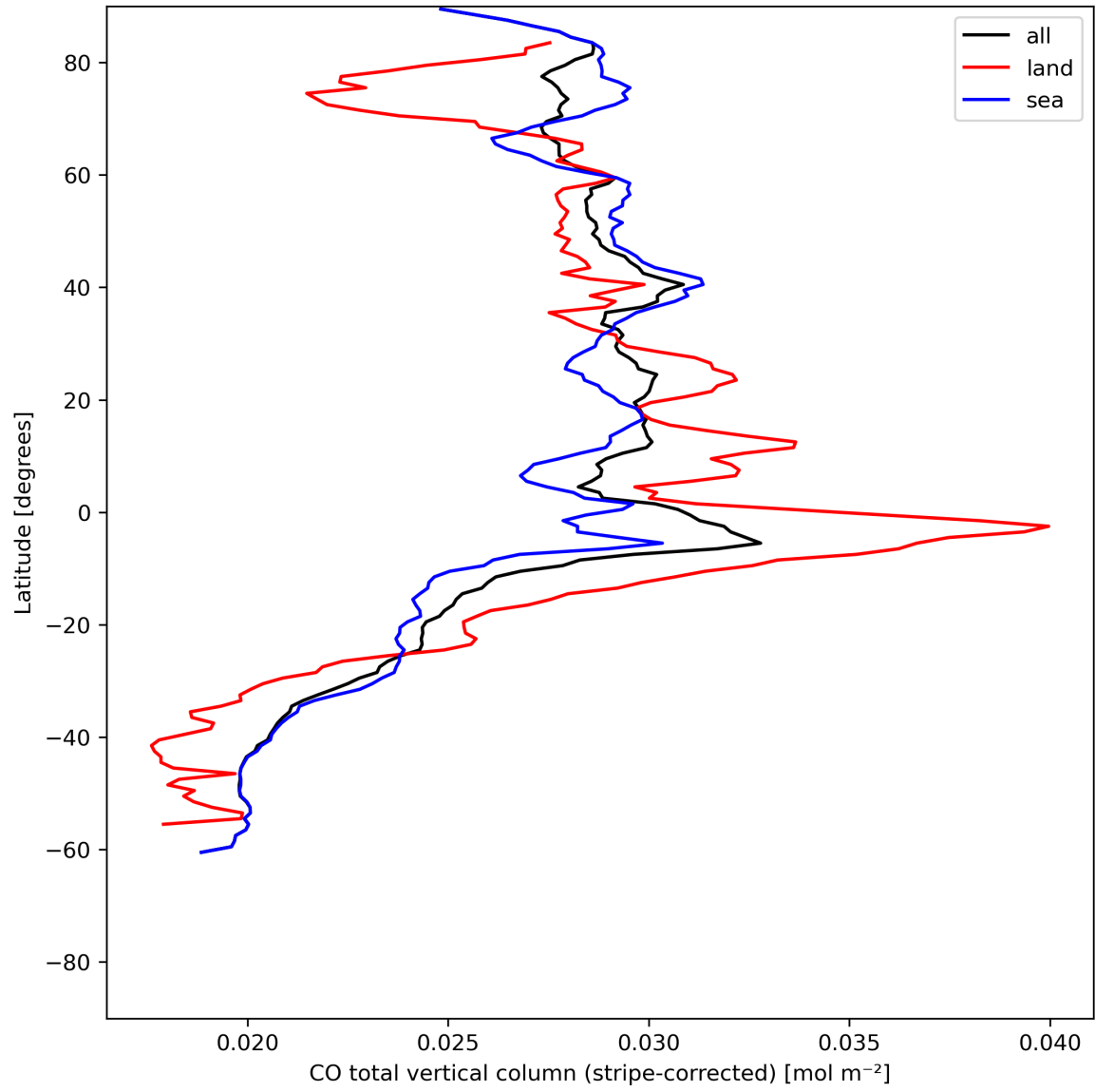
Figure 11: Zonal average of “CO total vertical column (stripe-corrected)” for 2024-06-19 to 2024-06-21.
