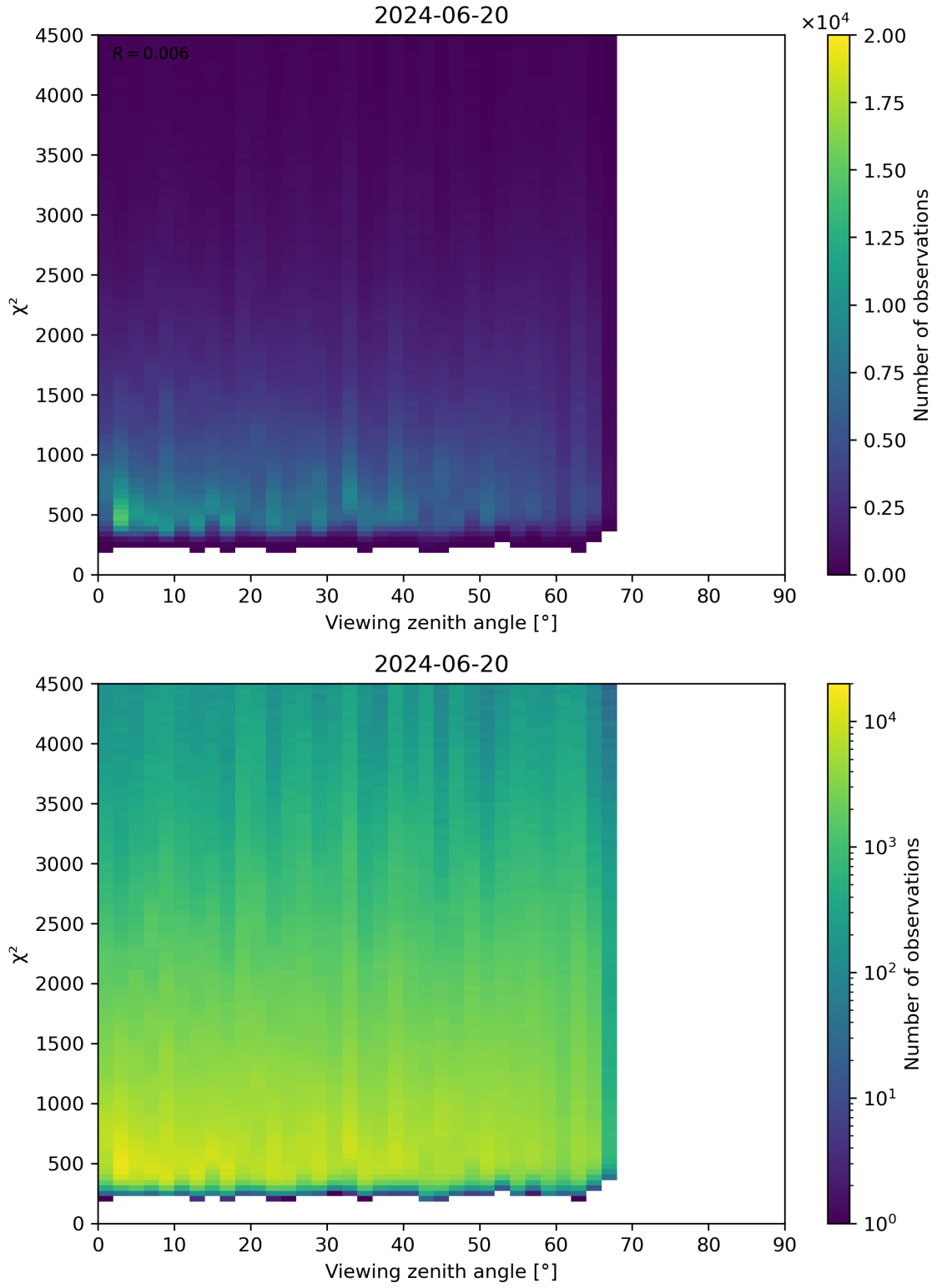
Figure 72: Scatter density plot of “Viewing zenith angle” against “ \chi^2 ” for 2024-06-19 to 2024-06-21.
