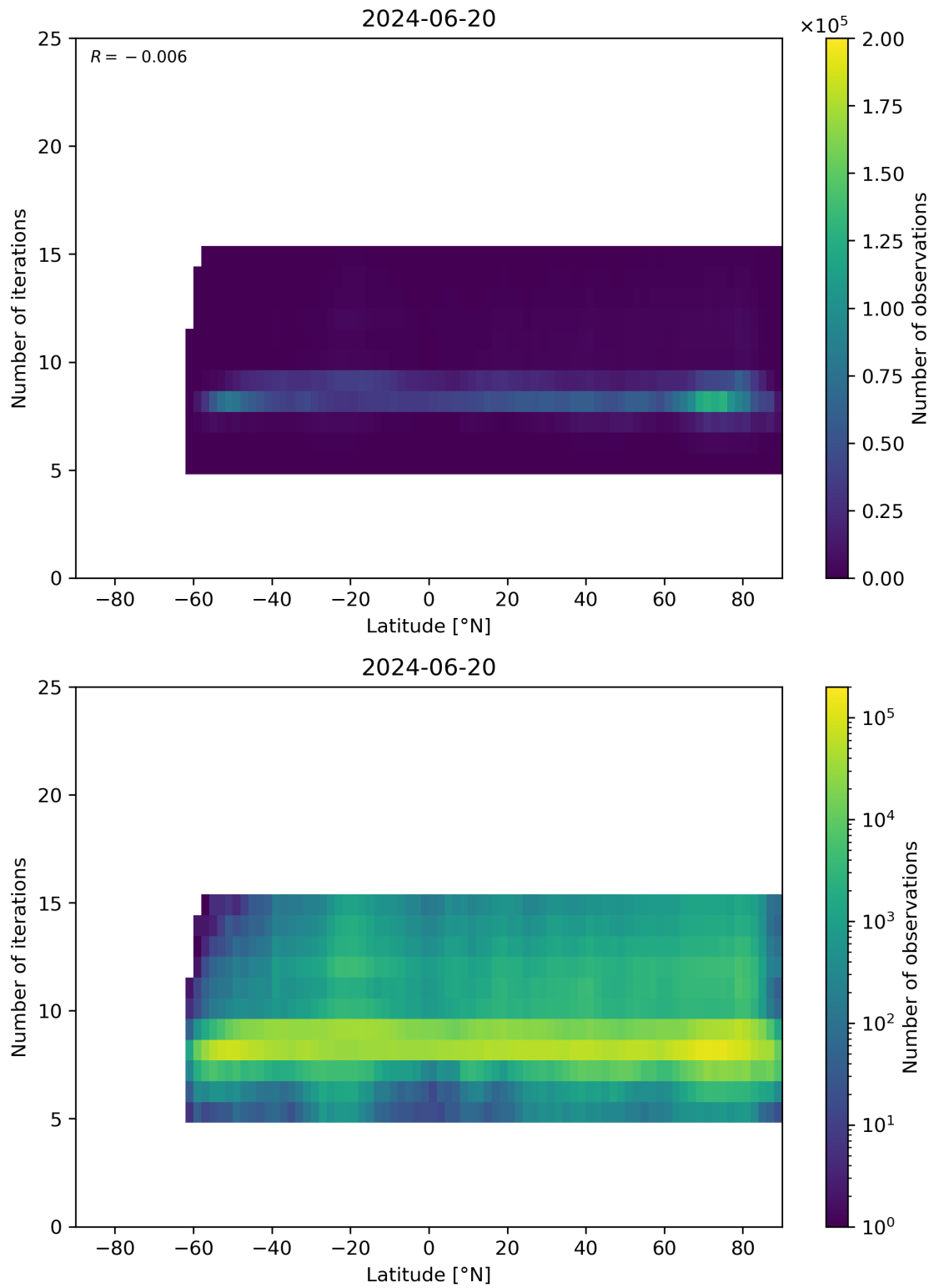
Figure 56: Scatter density plot of “Latitude” against “Number of iterations” for 2024-06-19 to 2024-06-21.
