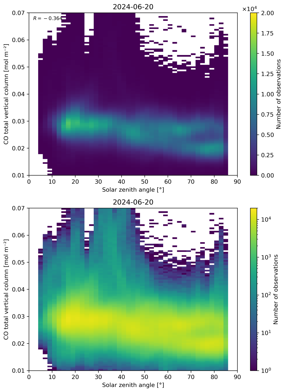
Figure 61: Scatter density plot of “Solar zenith angle” against “CO total vertical column” for 2024-06-19 to 2024-06-21.
