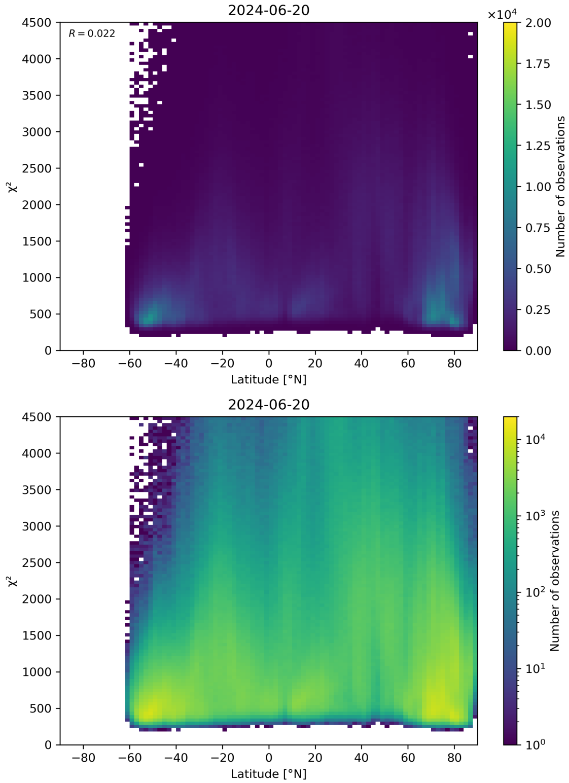
Figure 54: Scatter density plot of “Latitude” against “ \chi^2 ” for 2024-06-19 to 2024-06-21.
