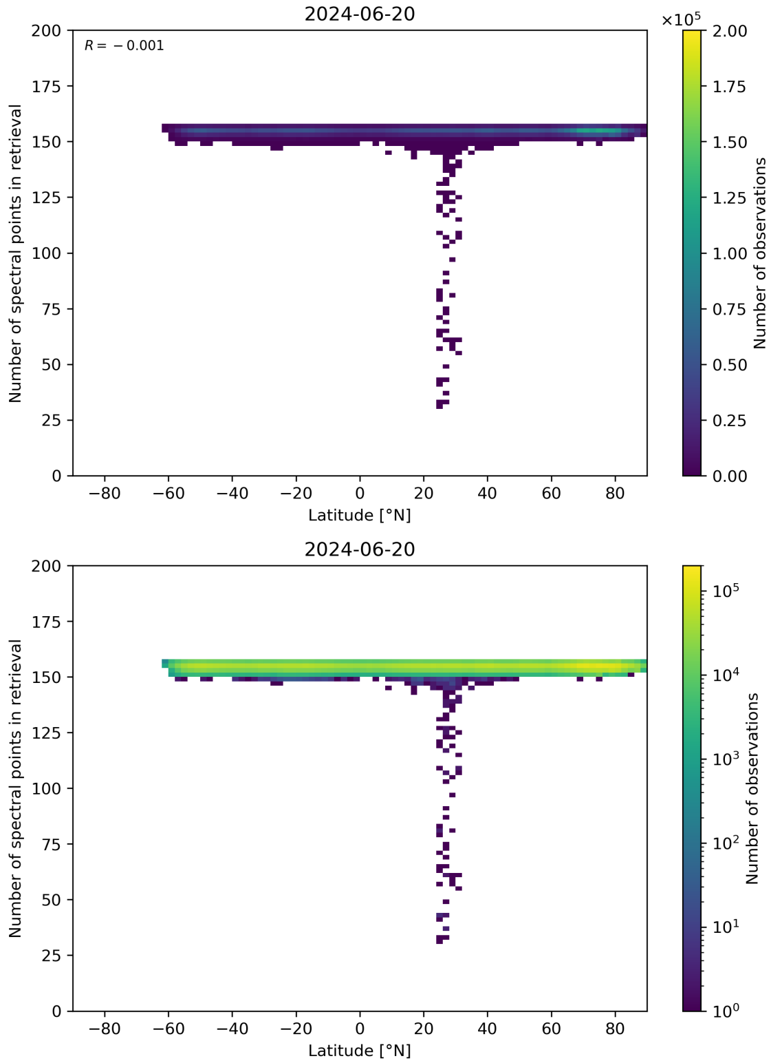
Figure 57: Scatter density plot of “Latitude” against “Number of spectral points in retrieval” for 2024-06-19 to 2024-06-21.
