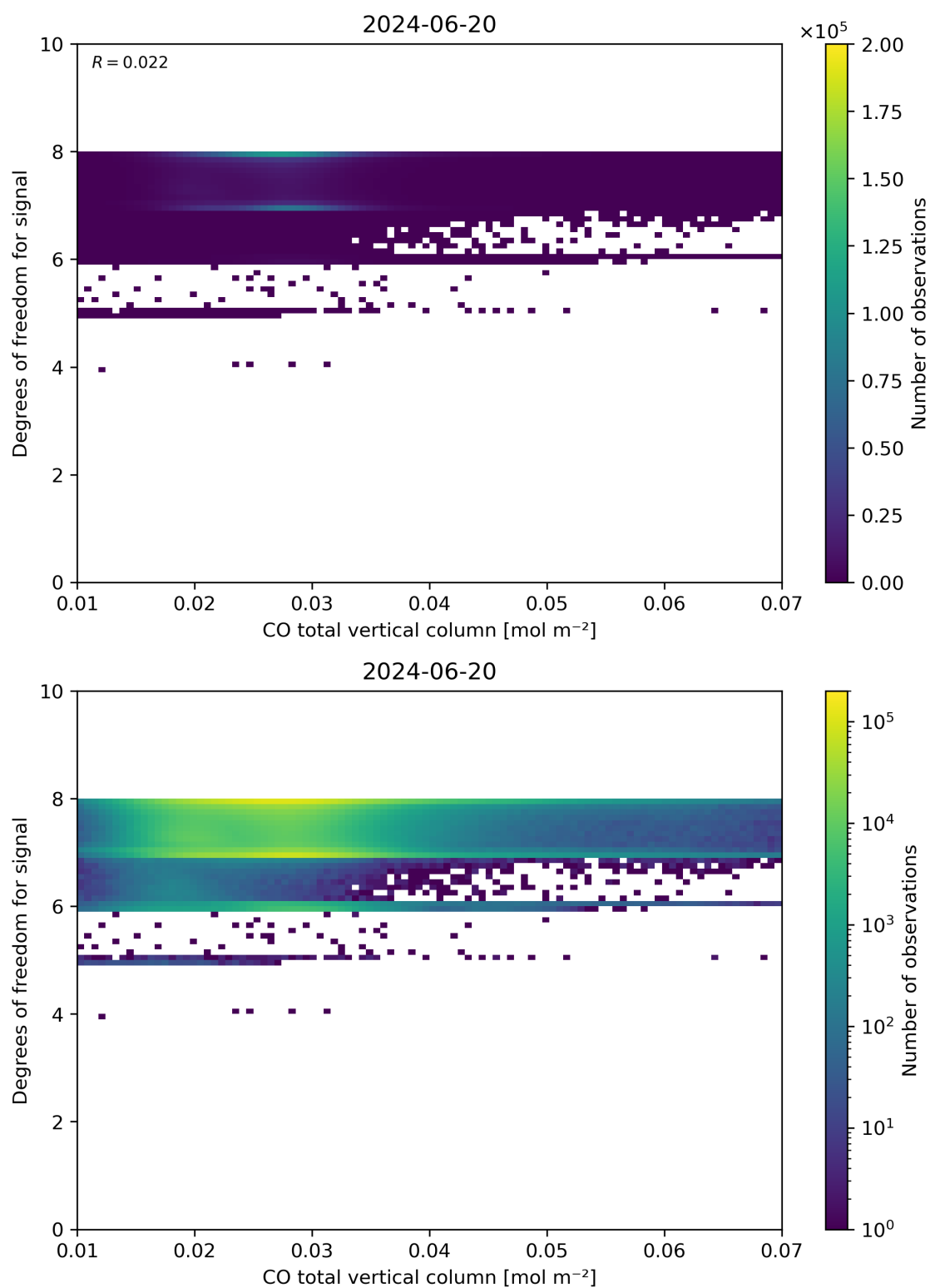
Figure 41: Scatter density plot of “CO total vertical column” against “Degrees of freedom for signal” for 2024-06-19 to 2024-06-21.
