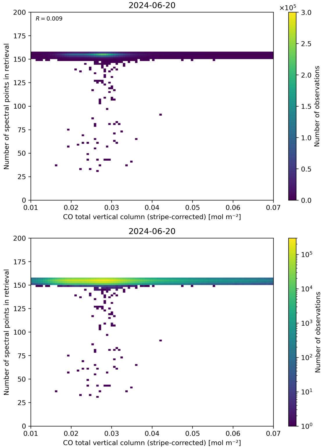
Figure 40: Scatter density plot of “CO total vertical column (stripe-corrected)” against “Number of spectral points in retrieval” for 2024-06-19 to 2024-06-21.
