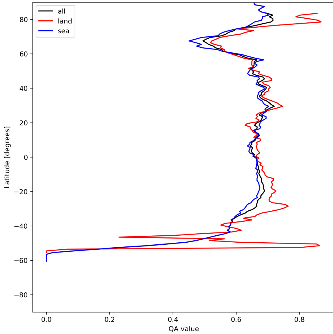
Figure 9: Zonal average of “QA value” for 2024-06-19 to 2024-06-21.
