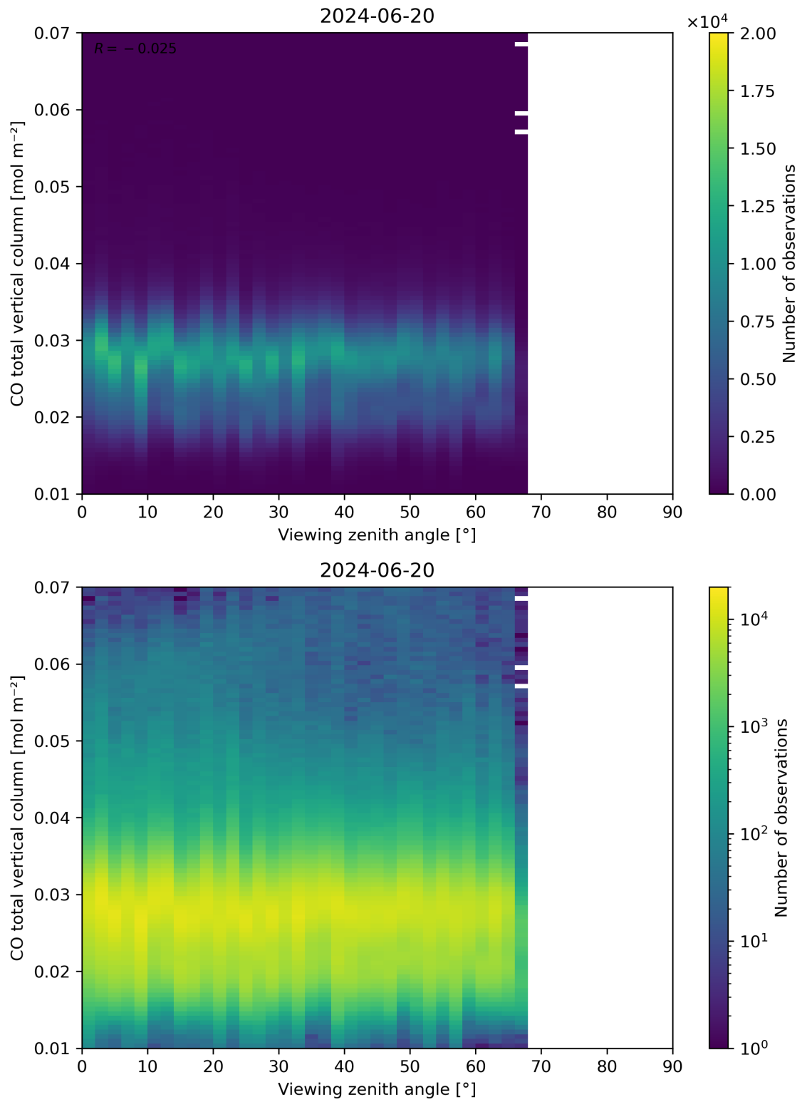
Figure 69: Scatter density plot of “Viewing zenith angle” against “CO total vertical column” for 2024-06-19 to 2024-06-21.
