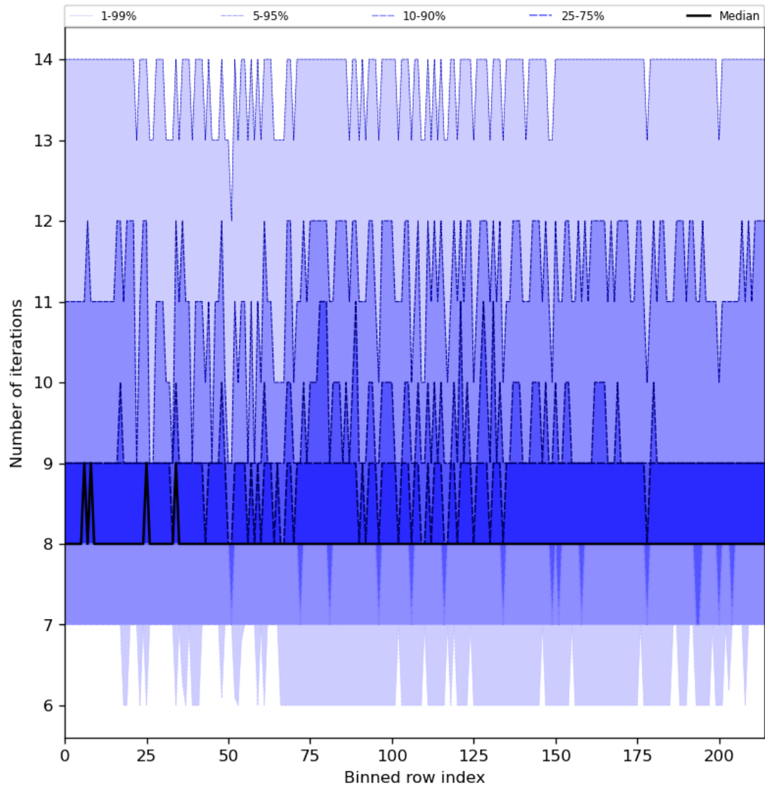
Figure 32: Along track statistics of “Number of iterations” for 2024-06-19 to 2024-06-21
