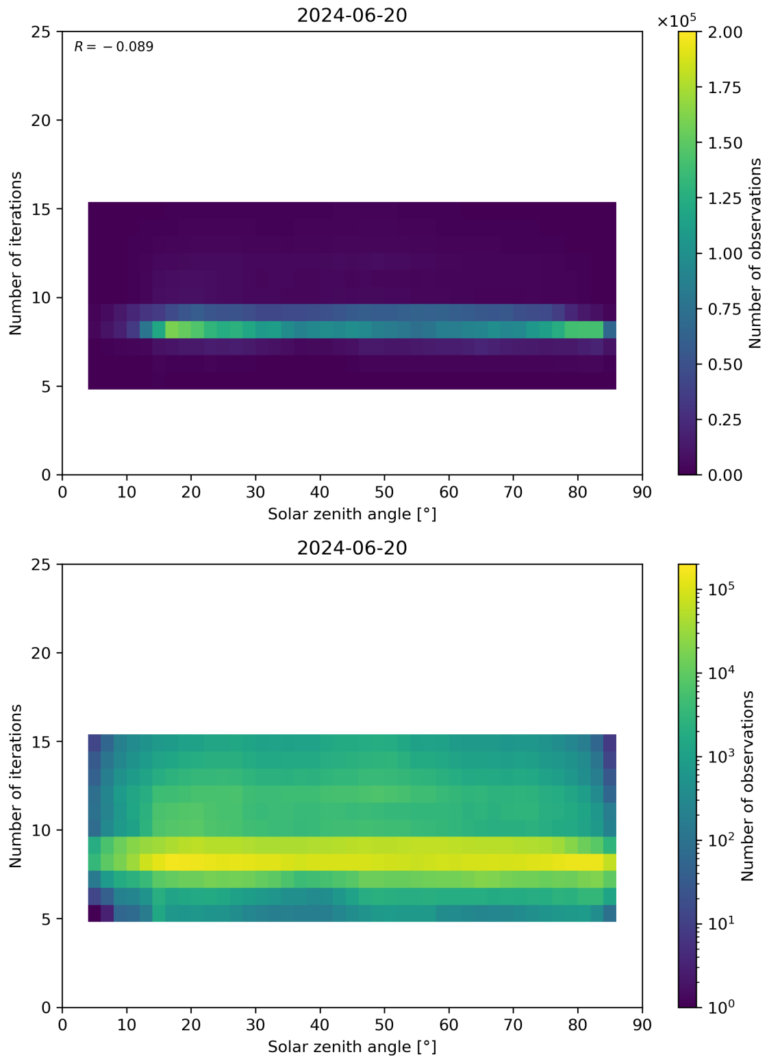
Figure 67: Scatter density plot of “Solar zenith angle” against “Number of iterations” for 2024-06-19 to 2024-06-21.
