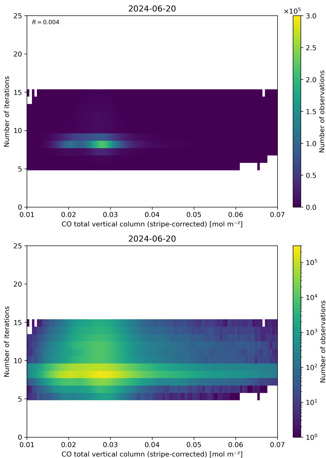
Figure 39: Scatter density plot of “CO total vertical column (stripe-corrected)” against “Number of iterations” for 2024-06-19 to 2024-06-21.
