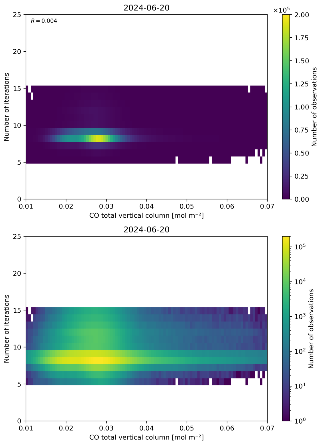
Figure 42: Scatter density plot of “CO total vertical column” against “Number of iterations” for 2024-06-19 to 2024-06-21.
