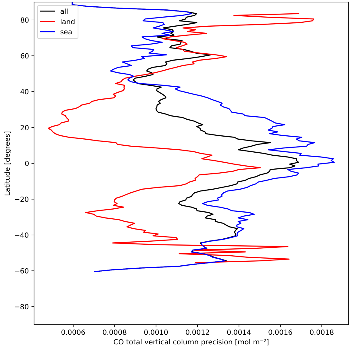
Figure 12: Zonal average of “CO total vertical column precision” for 2024-06-19 to 2024-06-21.
