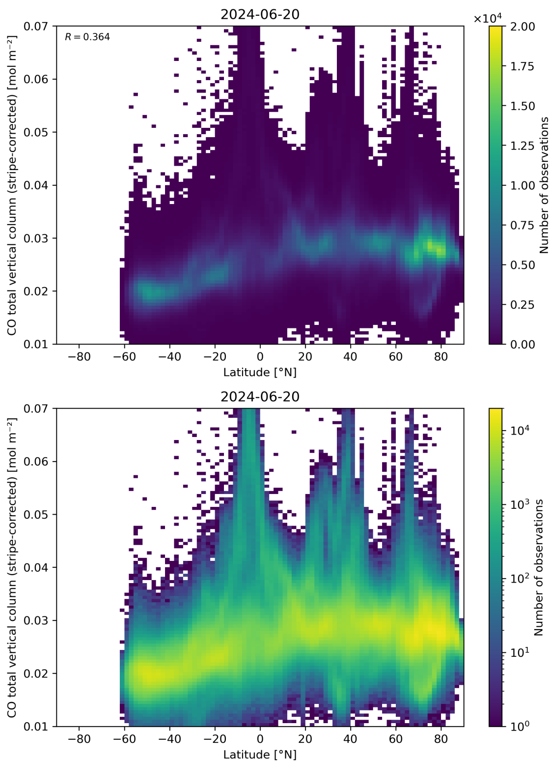
Figure 52: Scatter density plot of “Latitude” against “CO total vertical column (stripe-corrected)” for 2024-06-19 to 2024-06-21.
