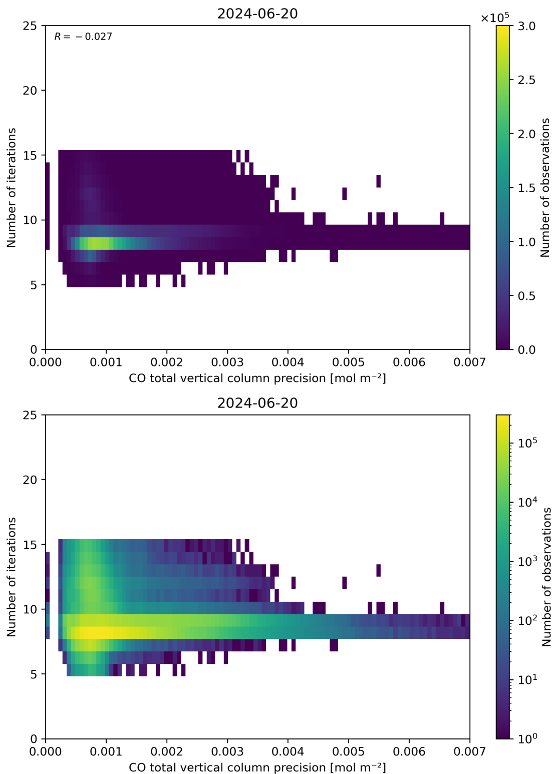
Figure 46: Scatter density plot of “CO total vertical column precision” against “Number of iterations” for 2024-06-19 to 2024-06-21.
