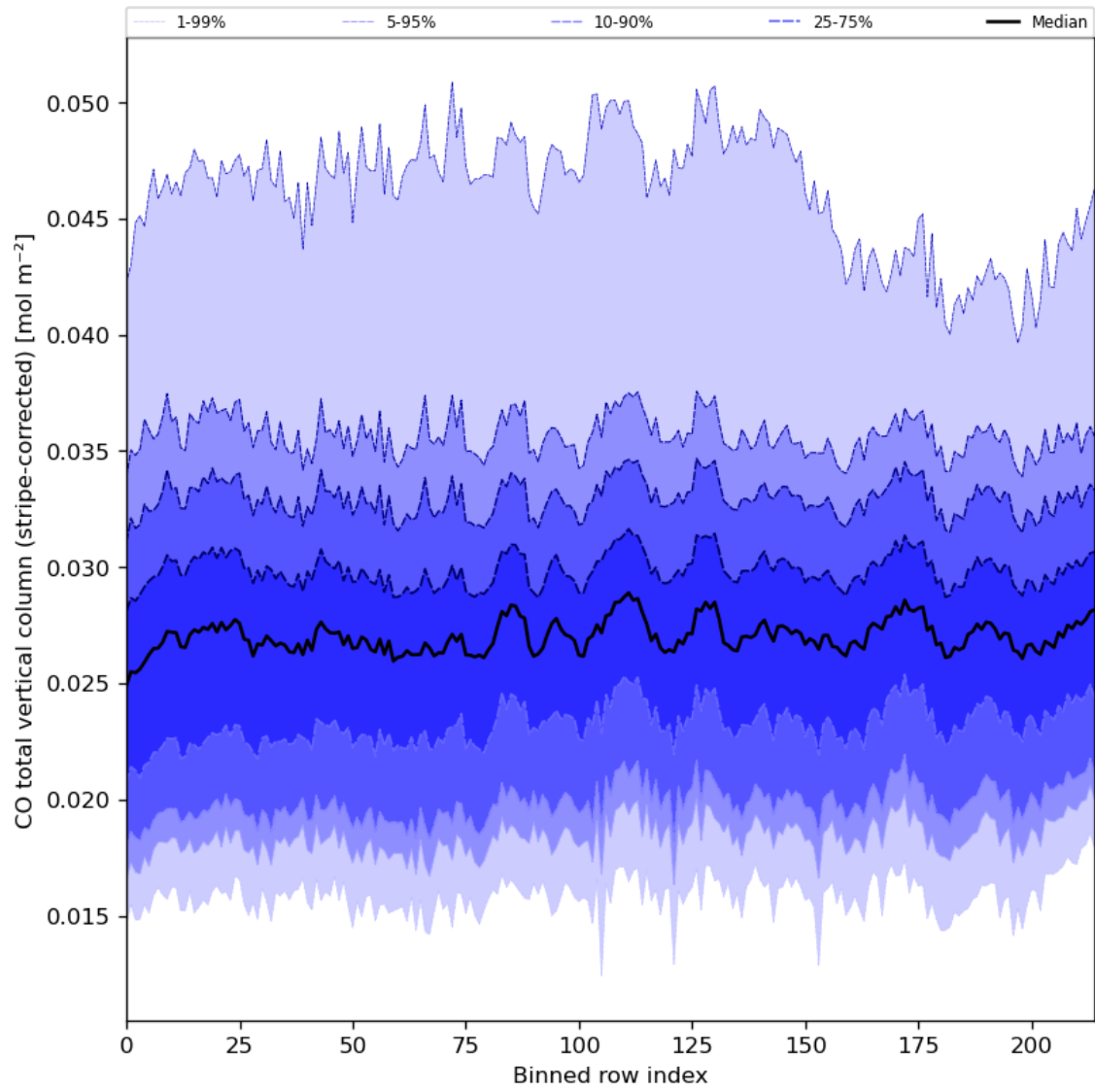
Figure 27: Along track statistics of “CO total vertical column (stripe-corrected)” for 2024-06-19 to 2024-06-21
