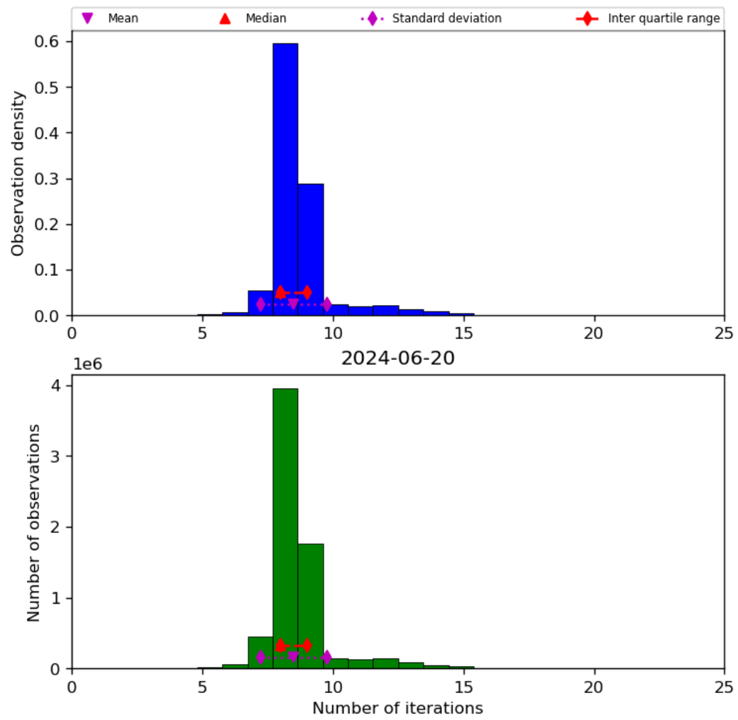
Figure 24: Histogram of “Number of iterations” for 2024-06-19 to 2024-06-21
