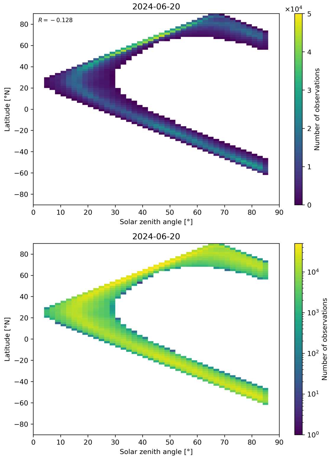
Figure 66: Scatter density plot of “Solar zenith angle” against “Latitude” for 2024-06-19 to 2024-06-21.
