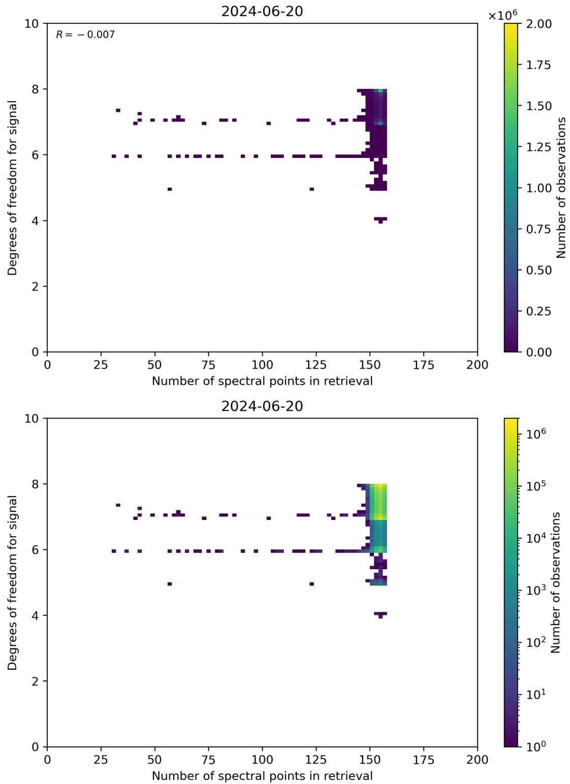
Figure 59: Scatter density plot of “Number of spectral points in retrieval” against “Degrees of freedom for signal” for 2024-06-19 to 2024-06-21.
