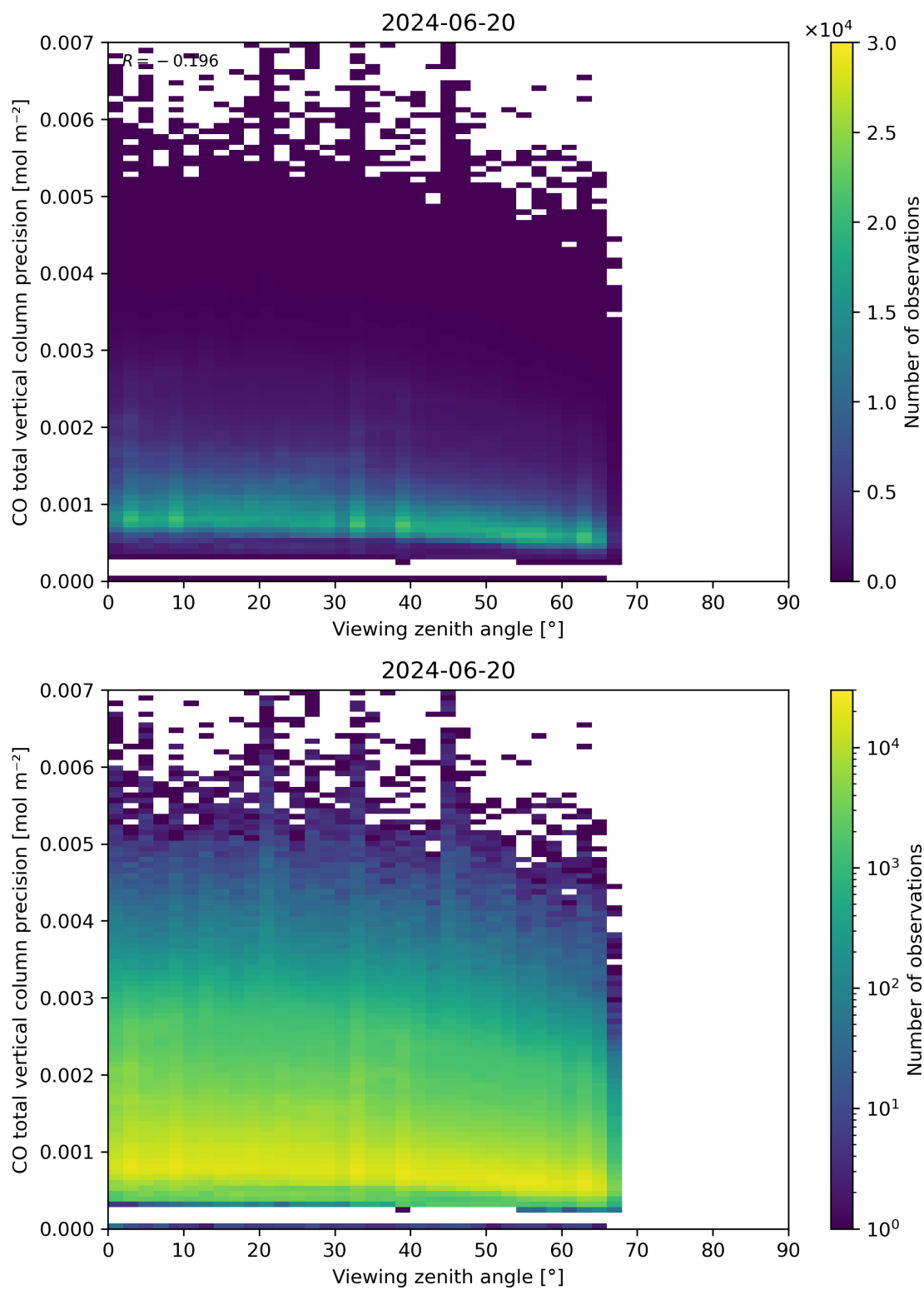
Figure 71: Scatter density plot of “Viewing zenith angle” against “CO total vertical column precision” for 2024-06-19 to 2024-06-21.
