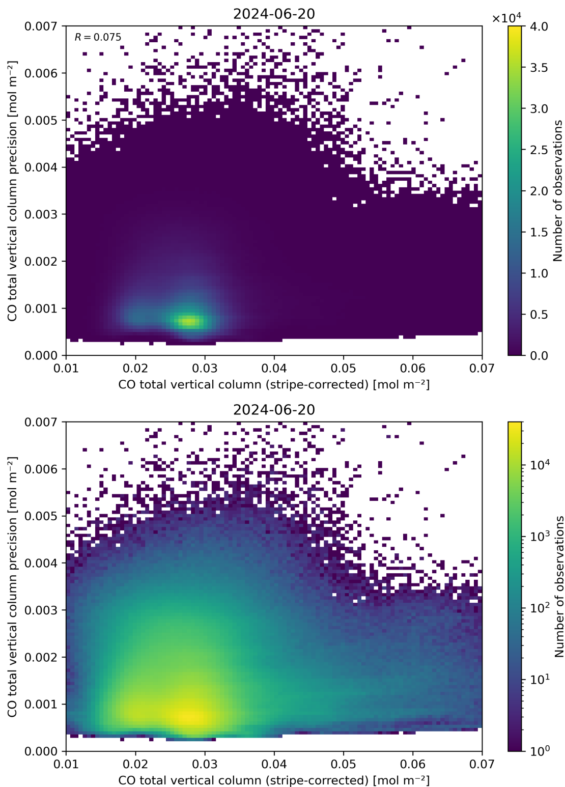
Figure 36: Scatter density plot of “CO total vertical column (stripe-corrected)” against “CO total vertical column precision” for 2024-06-19 to 2024-06-21.
