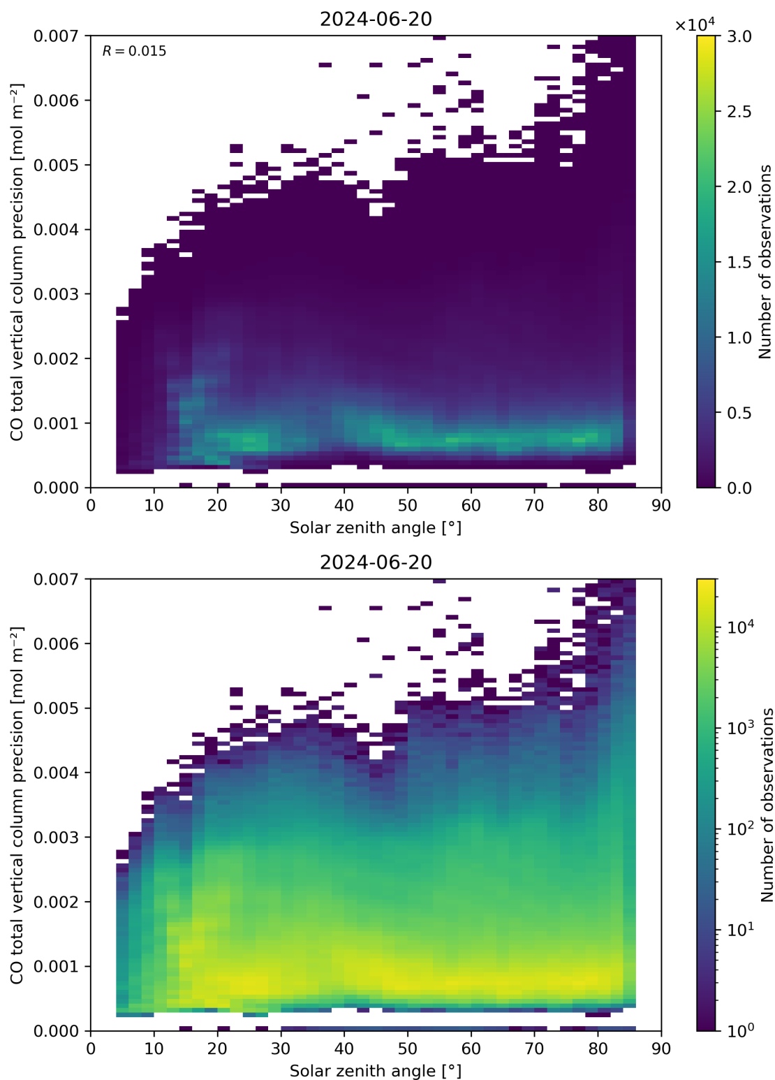
Figure 63: Scatter density plot of “Solar zenith angle” against “CO total vertical column precision” for 2024-06-19 to 2024-06-21.
