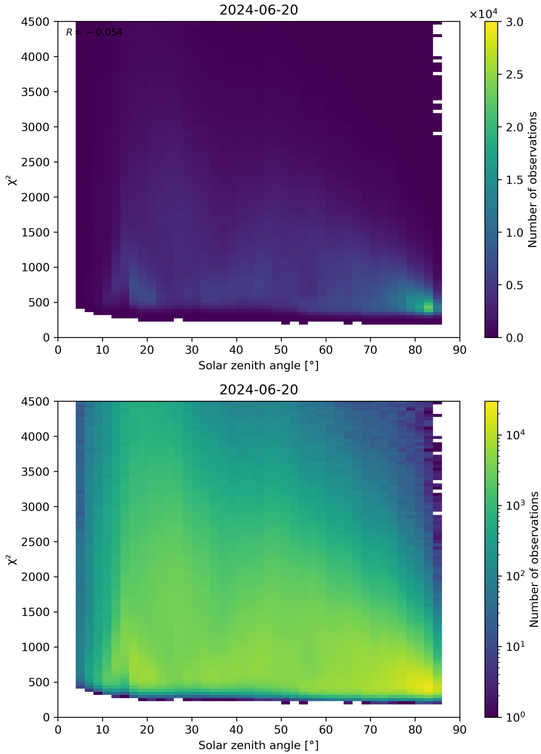
Figure 64: Scatter density plot of “Solar zenith angle” against “ \chi^2 ” for 2024-06-19 to 2024-06-21.
