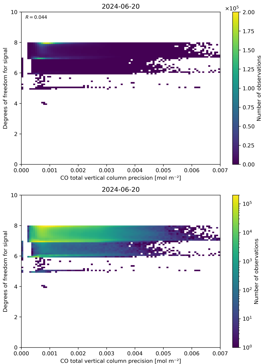
Figure 45: Scatter density plot of “CO total vertical column precision” against “Degrees of freedom for signal” for 2024-06-19 to 2024-06-21.
