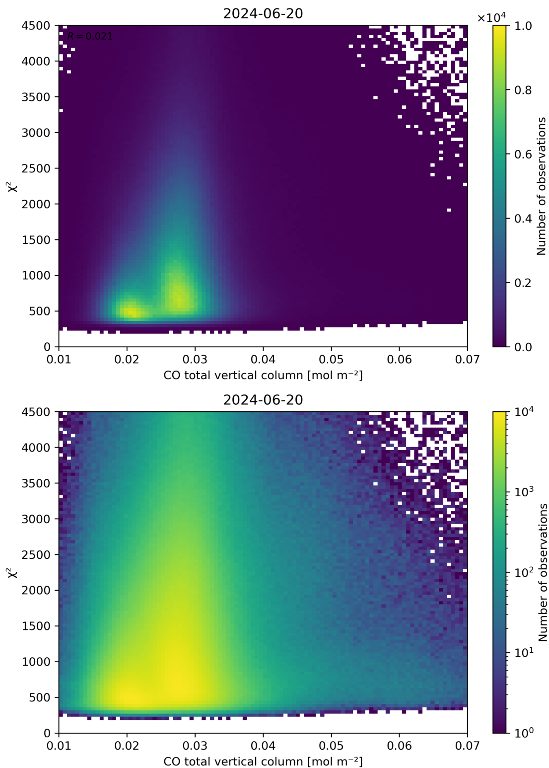
Figure 35: Scatter density plot of “CO total vertical column” against “ \chi^2 ” for 2024-06-19 to 2024-06-21.
