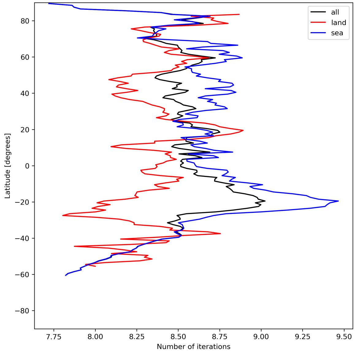
Figure 16: Zonal average of “Number of iterations” for 2024-06-19 to 2024-06-21.
