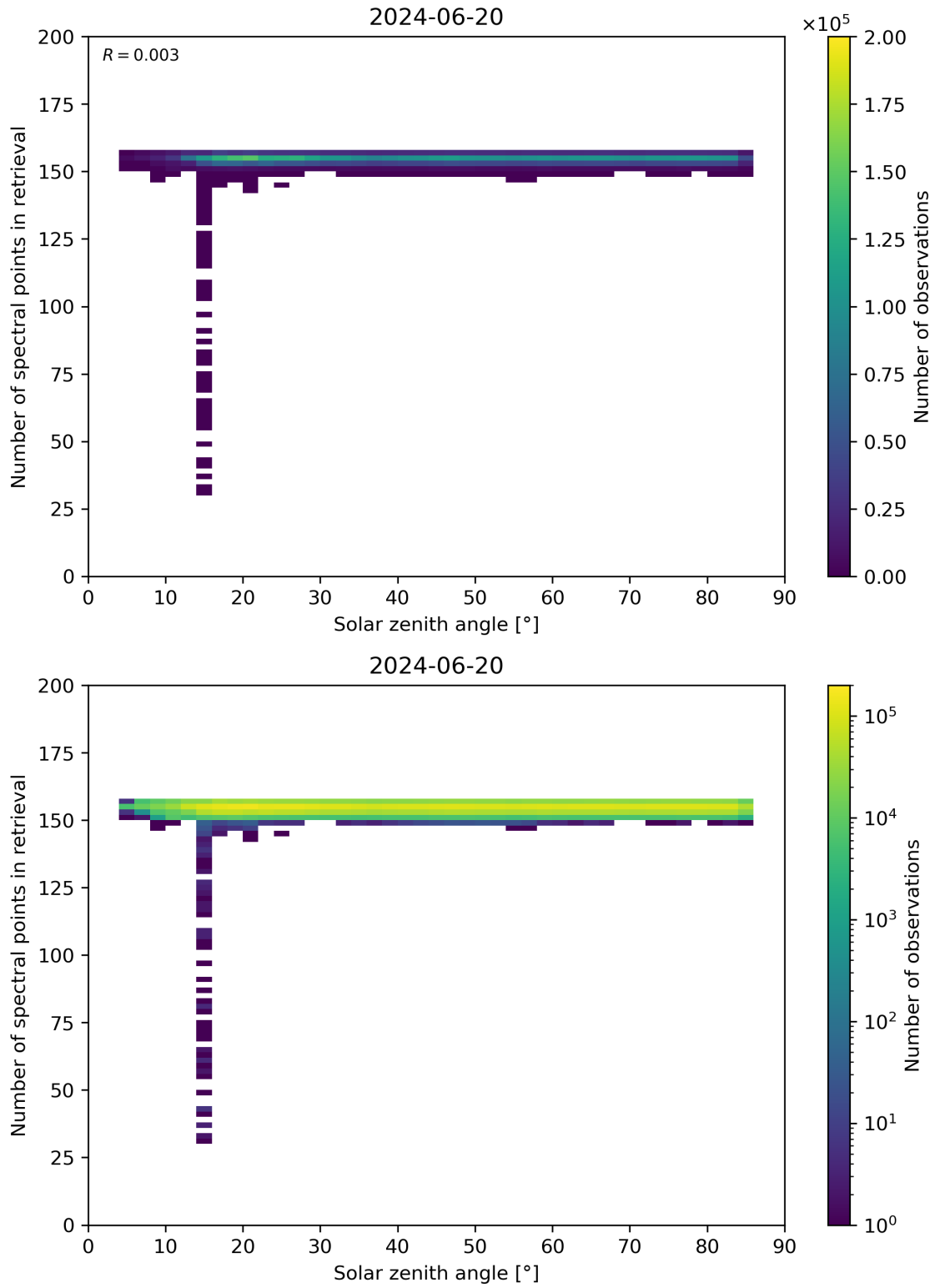
Figure 68: Scatter density plot of “Solar zenith angle” against “Number of spectral points in retrieval” for 2024-06-19 to 2024-06-21.
