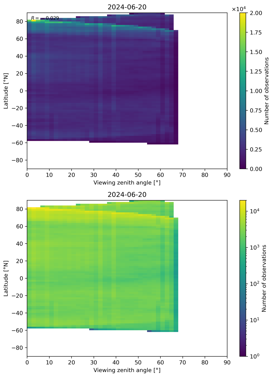
Figure 74: Scatter density plot of “Viewing zenith angle” against “Latitude” for 2024-06-19 to 2024-06-21.
