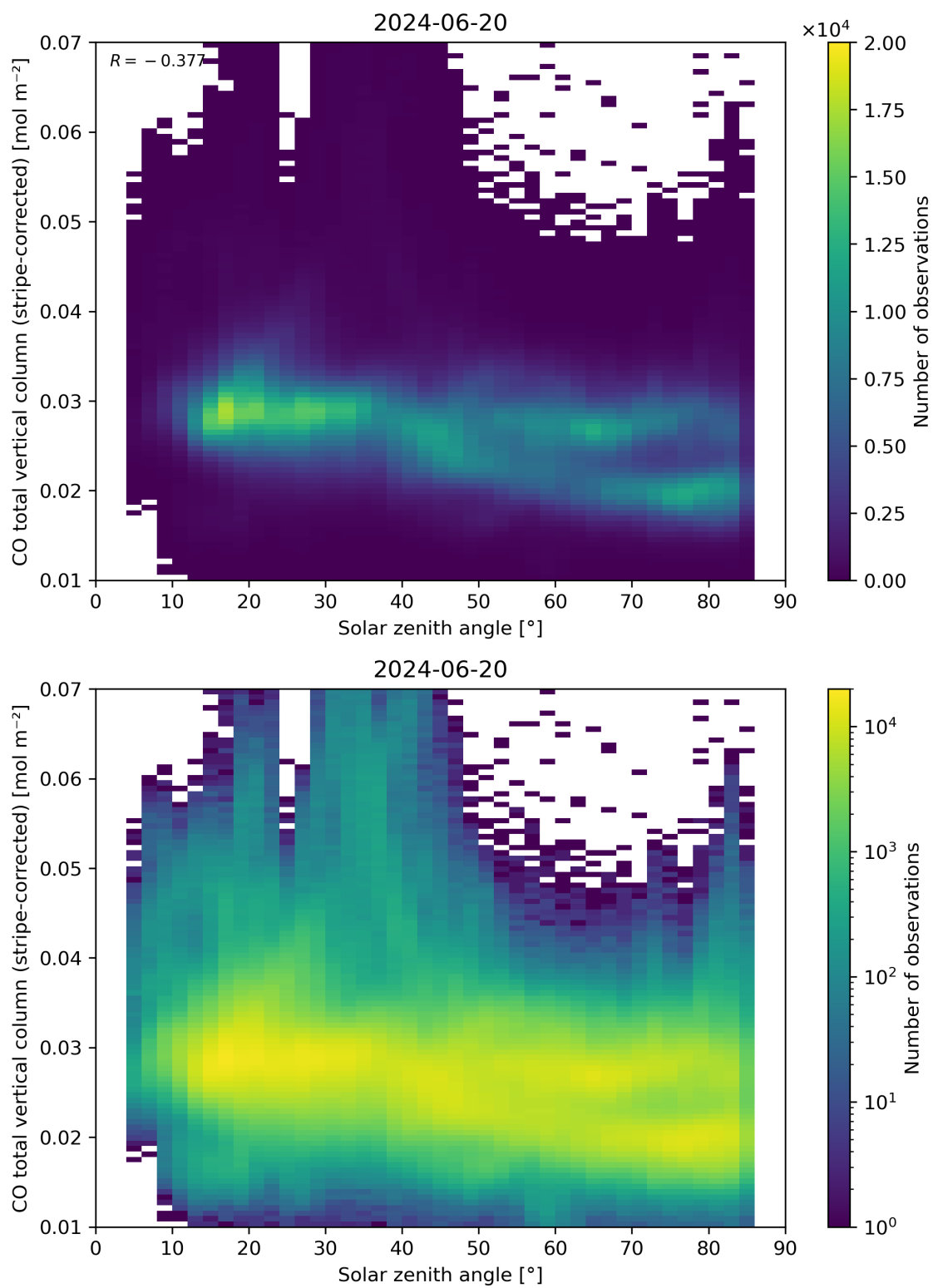
Figure 62: Scatter density plot of “Solar zenith angle” against “CO total vertical column (stripe-corrected)” for 2024-06-19 to 2024-06-21.
