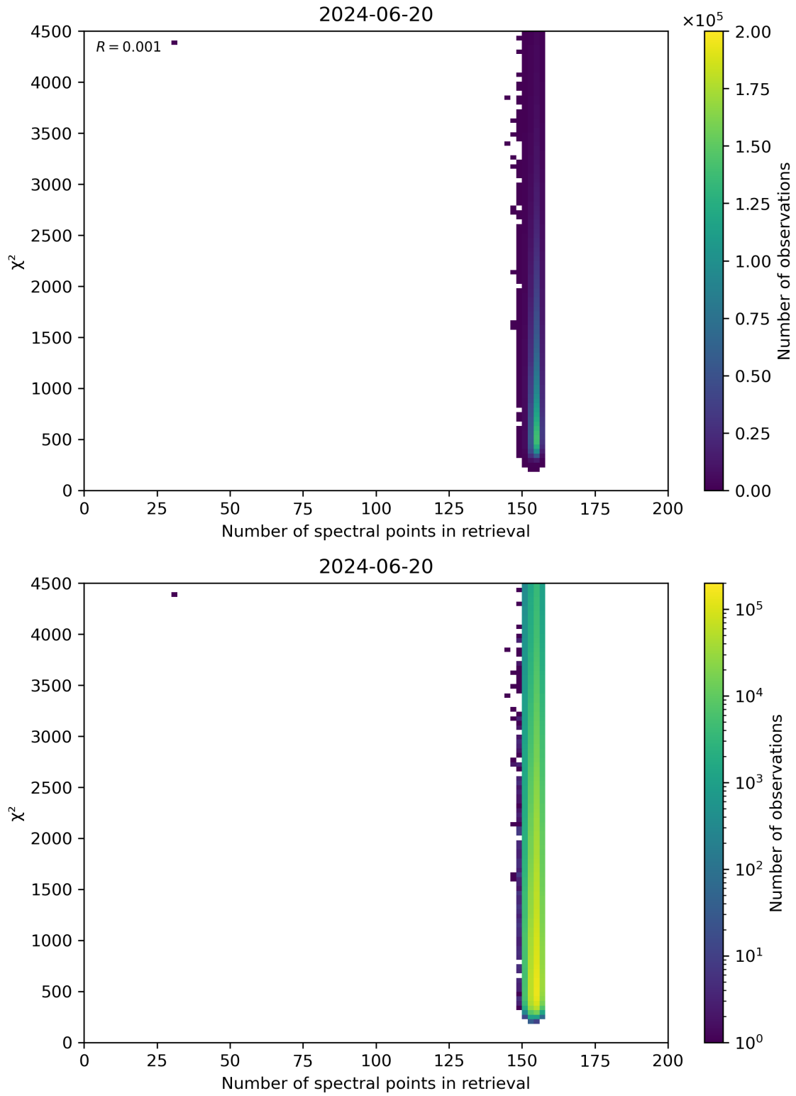
Figure 58: Scatter density plot of “Number of spectral points in retrieval” against “ \chi^2 ” for 2024-06-19 to 2024-06-21.
