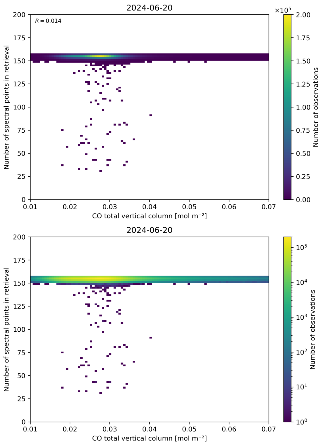
Figure 43: Scatter density plot of “CO total vertical column” against “Number of spectral points in retrieval” for 2024-06-19 to 2024-06-21.
