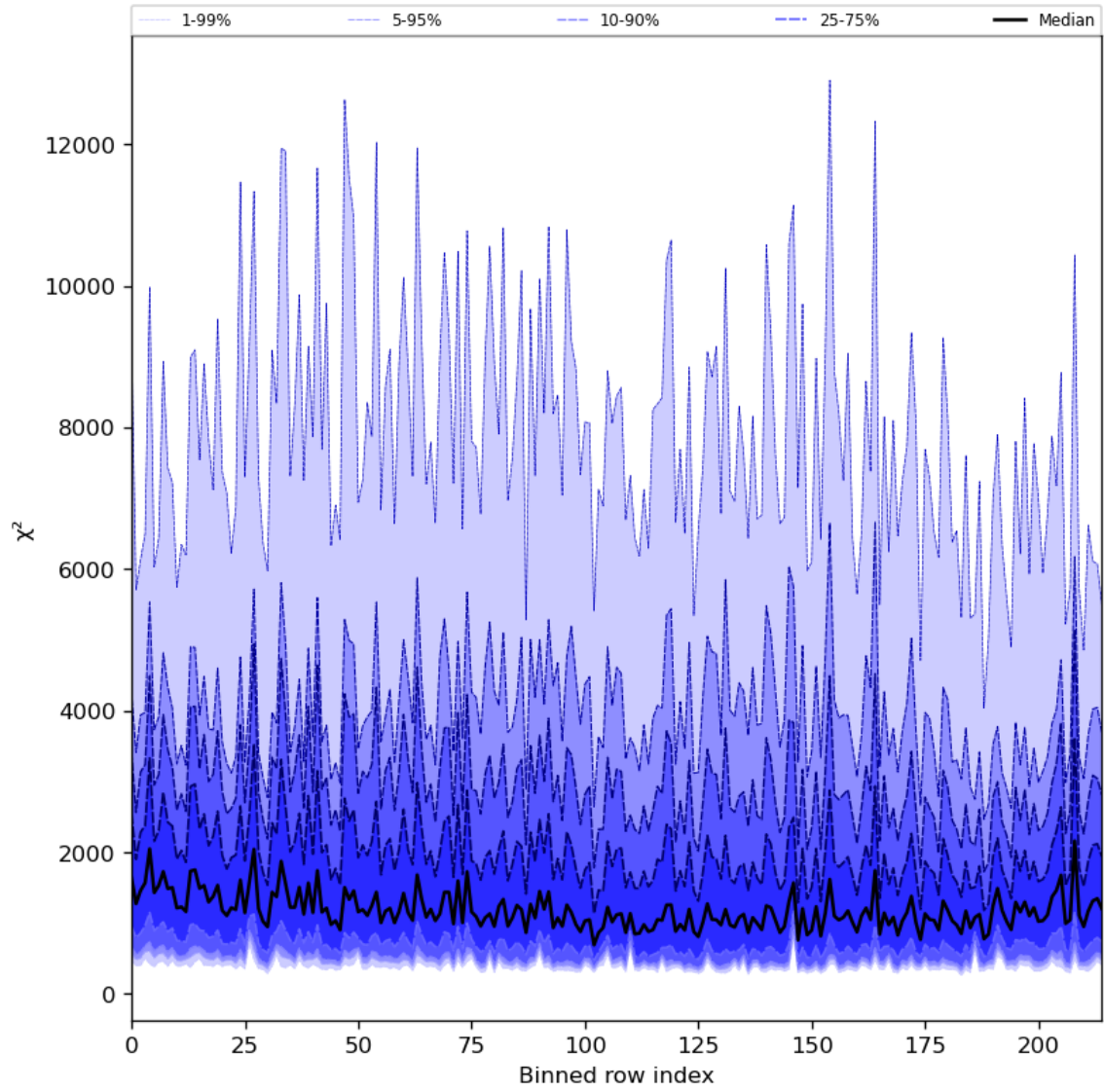
Figure 30: Along track statistics of “ \chi^2 ” for 2024-06-19 to 2024-06-21
