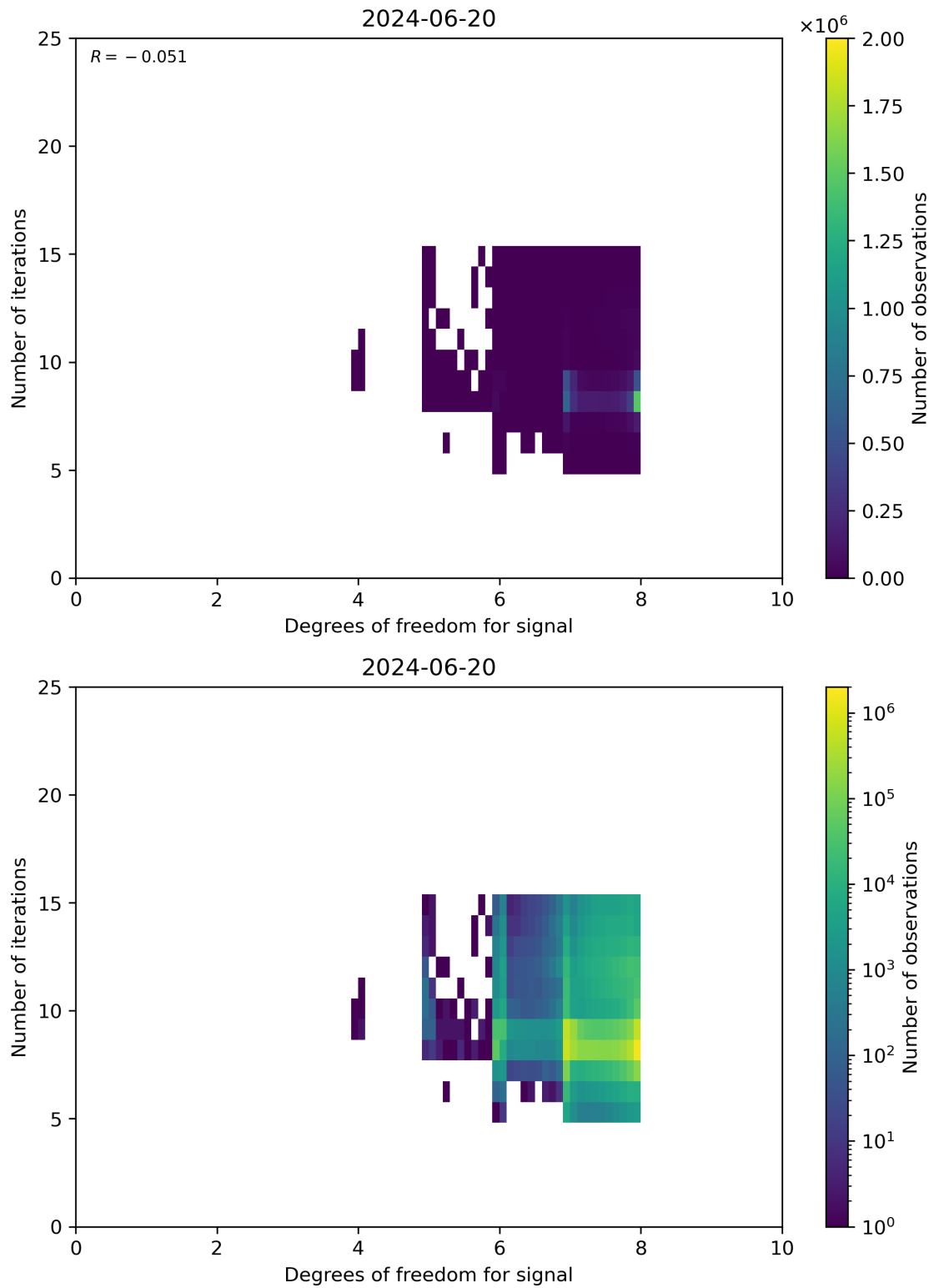
Figure 50: Scatter density plot of “Degrees of freedom for signal” against “Number of iterations” for 2024-06-19 to 2024-06-21.
