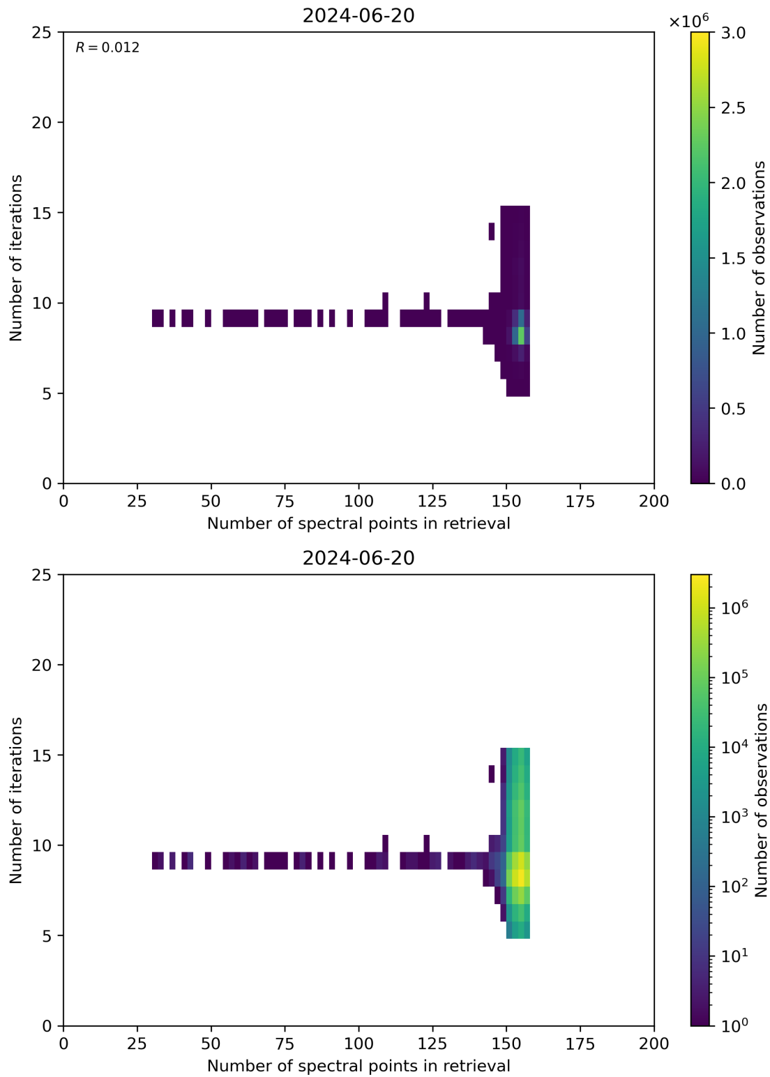
Figure 60: Scatter density plot of “Number of spectral points in retrieval” against “Number of iterations” for 2024-06-19 to 2024-06-21.
