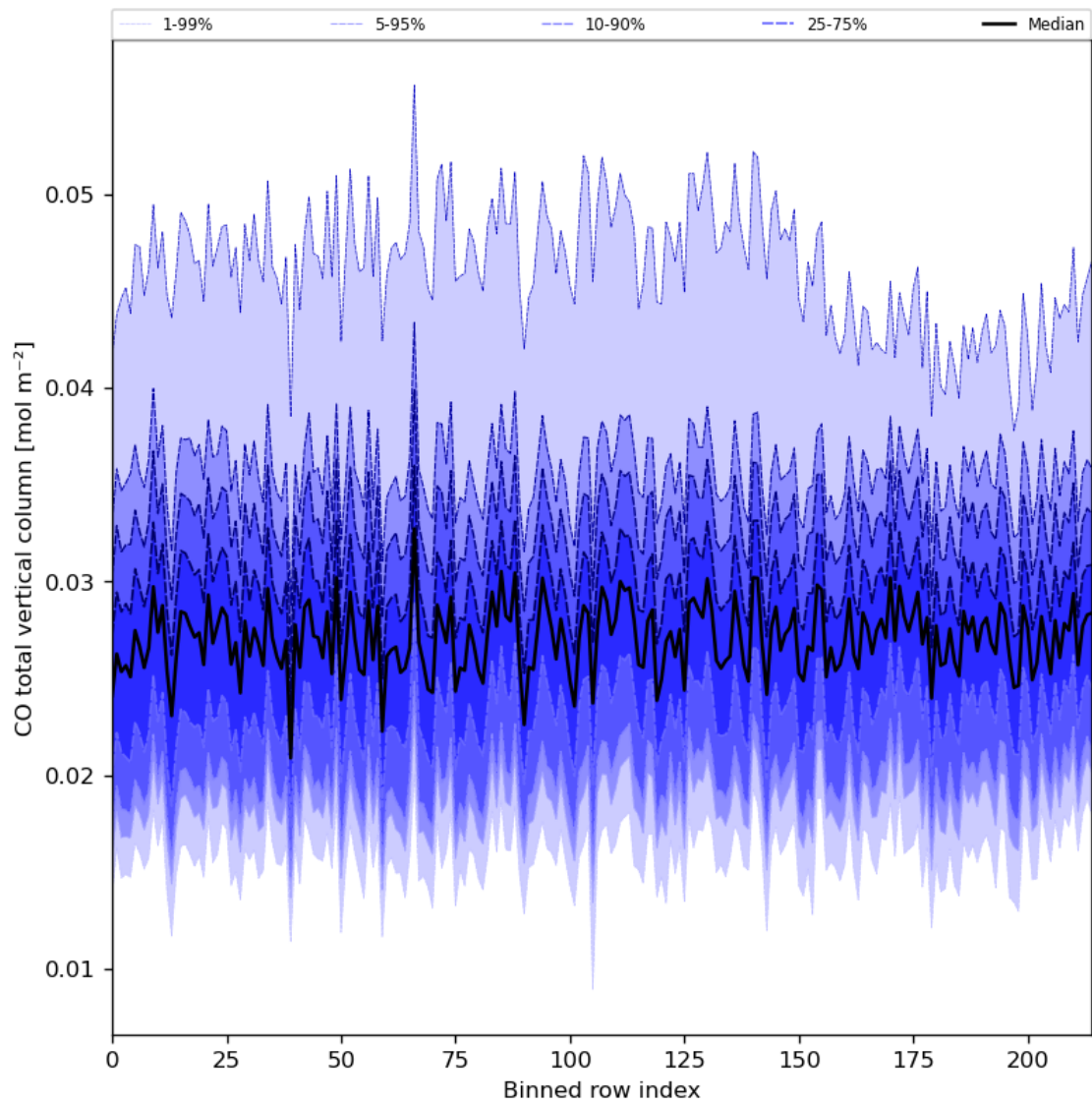
Figure 26: Along track statistics of “CO total vertical column” for 2024-06-19 to 2024-06-21
