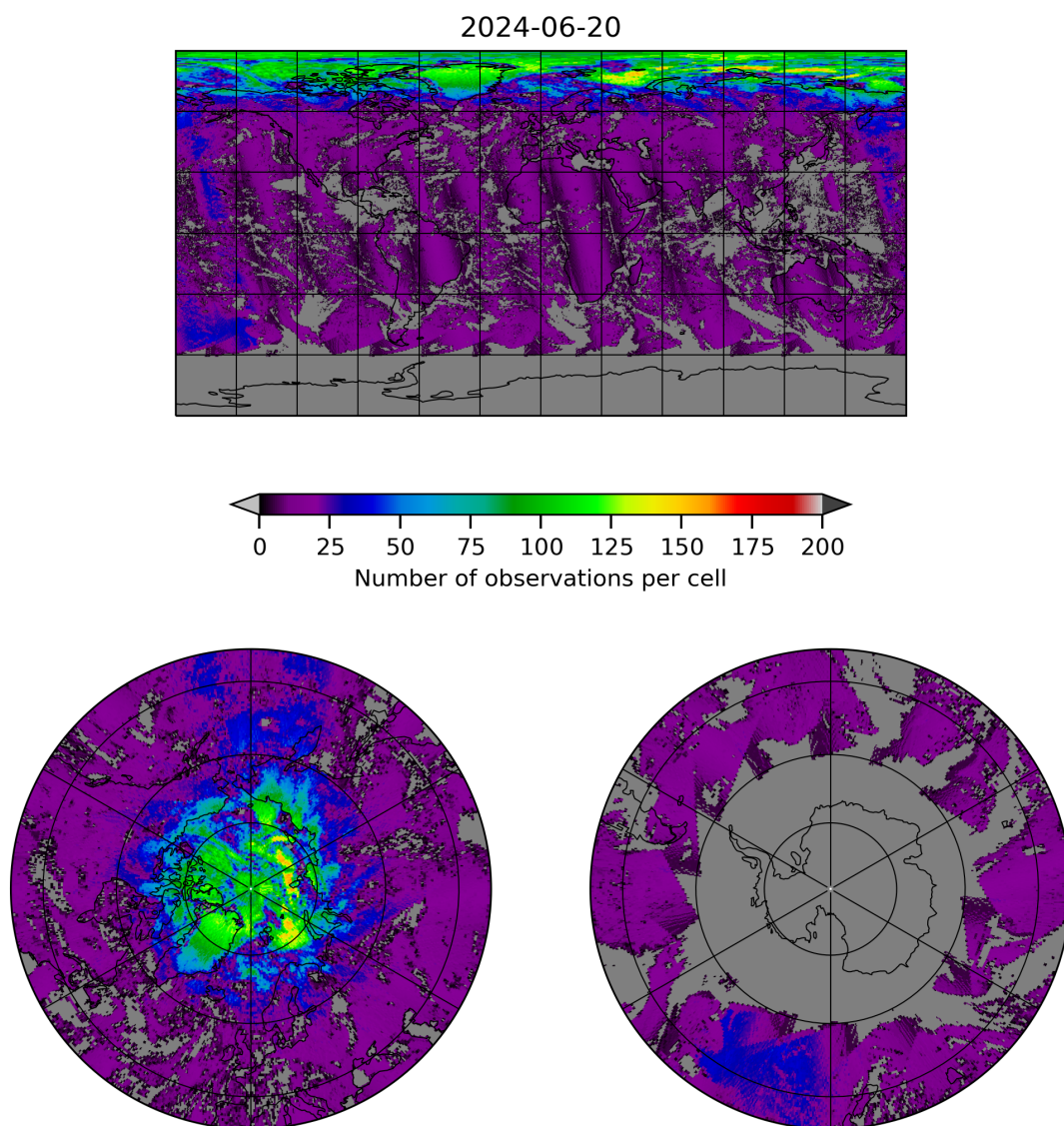
Figure 8: Map of the number of observations for 2024-06-19 to 2024-06-21
