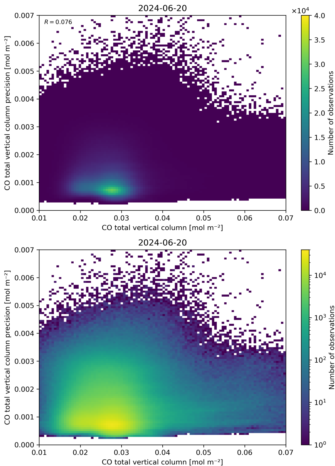
Figure 34: Scatter density plot of “CO total vertical column” against “CO total vertical column precision” for 2024-06-19 to 2024-06-21.
