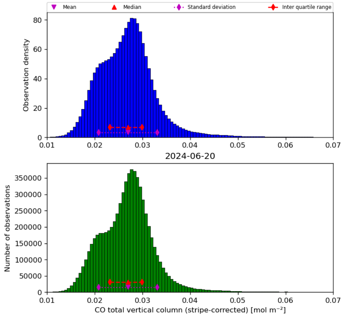
Figure 19: Histogram of “CO total vertical column (stripe-corrected)” for 2024-06-19 to 2024-06-21
