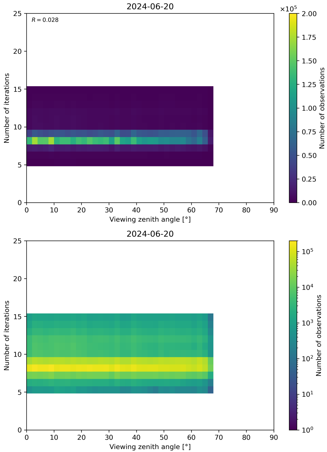
Figure 75: Scatter density plot of “Viewing zenith angle” against “Number of iterations” for 2024-06-19 to 2024-06-21.
