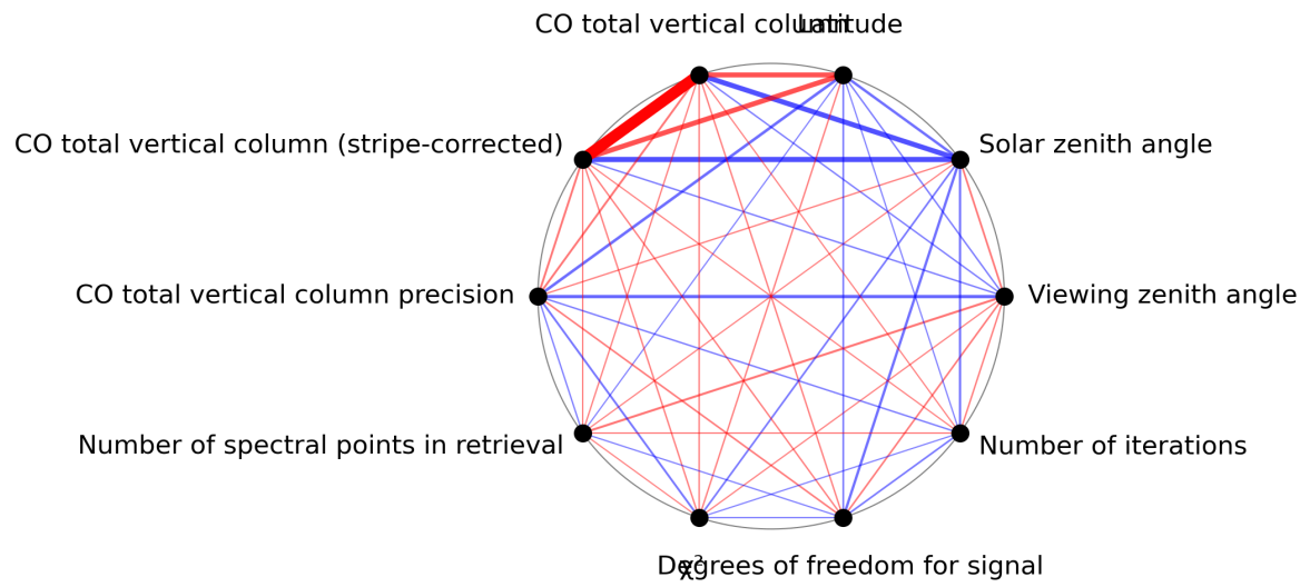
Figure 1: Map of correlation graph for 2024-06-19 to 2024-06-21.
