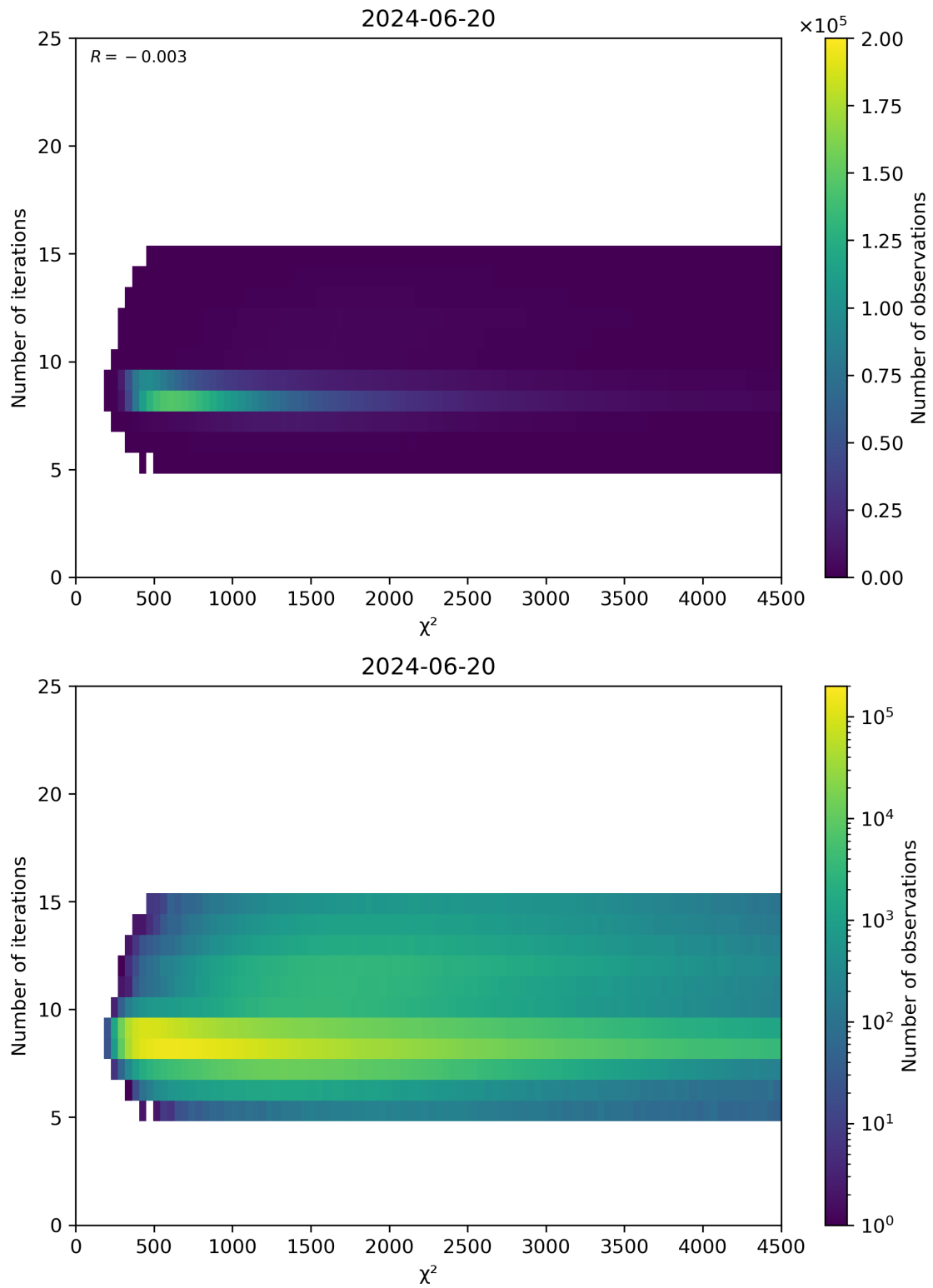
Figure 49: Scatter density plot of “ \chi^2 ” against “Number of iterations” for 2024-06-19 to 2024-06-21.
