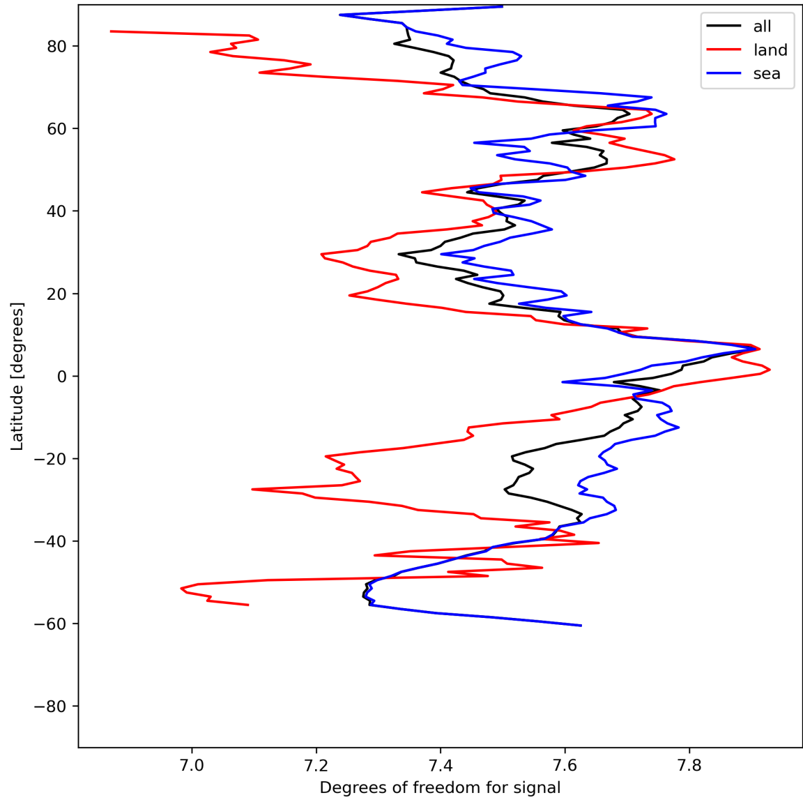
Figure 15: Zonal average of “Degrees of freedom for signal” for 2024-06-19 to 2024-06-21.
