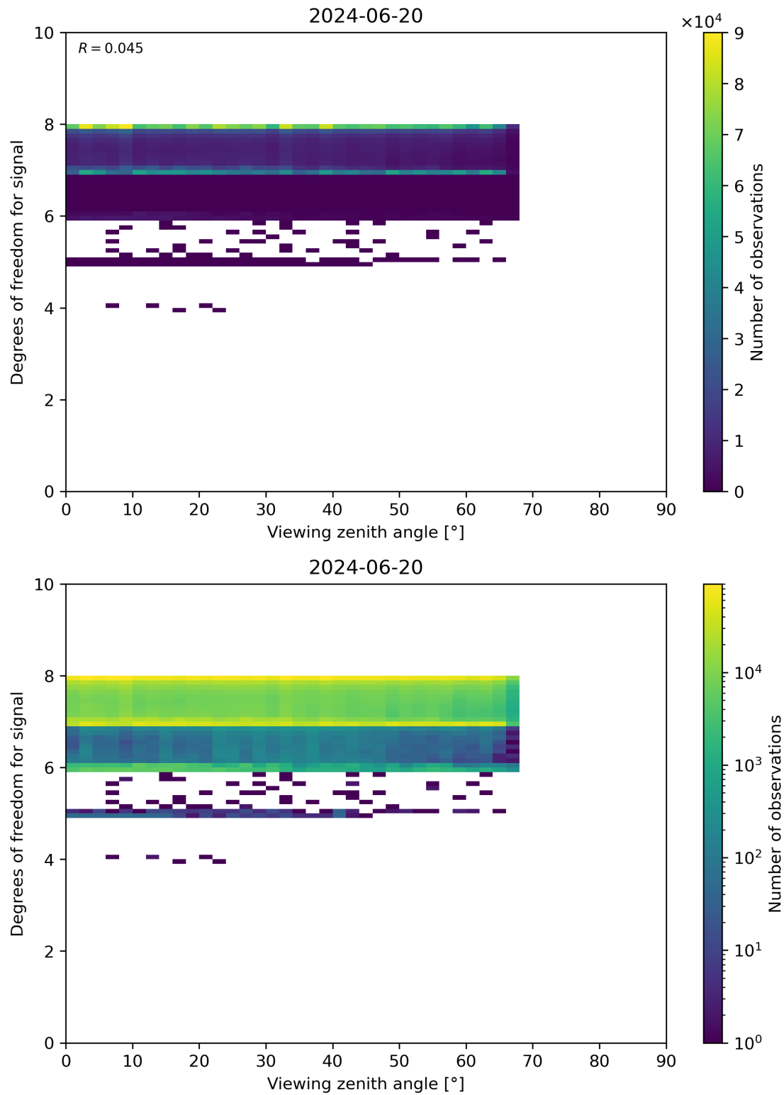
Figure 73: Scatter density plot of “Viewing zenith angle” against “Degrees of freedom for signal” for 2024-06-19 to 2024-06-21.
