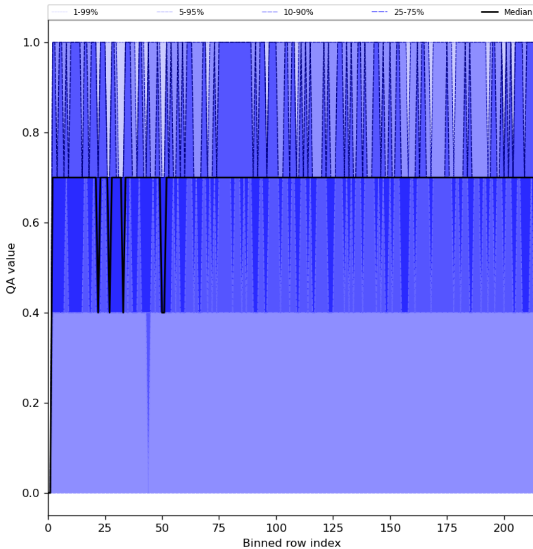
Figure 25: Along track statistics of “QA value” for 2024-06-19 to 2024-06-21
