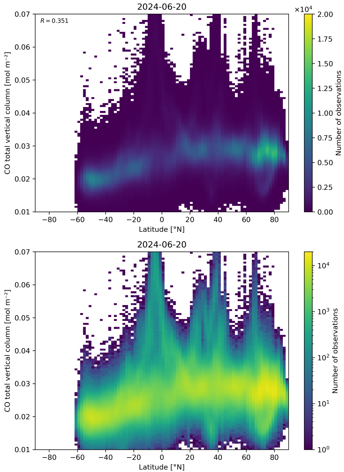
Figure 51: Scatter density plot of “Latitude” against “CO total vertical column” for 2024-06-19 to 2024-06-21.
