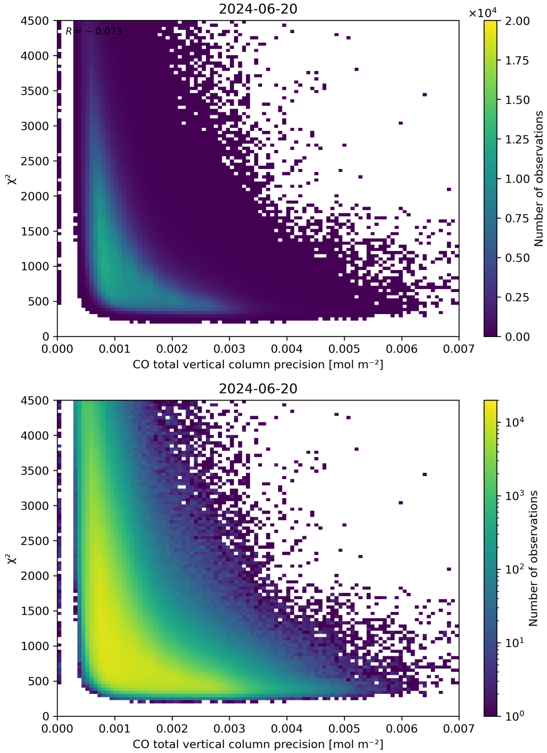
Figure 44: Scatter density plot of “CO total vertical column precision” against “ \chi^2 ” for 2024-06-19 to 2024-06-21.
