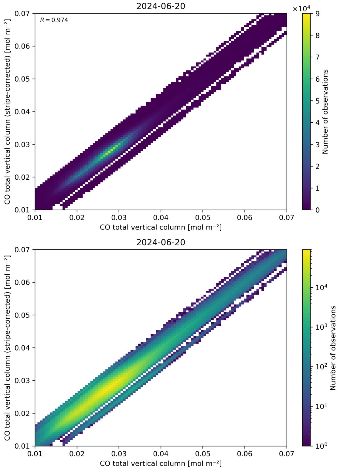
Figure 33: Scatter density plot of “CO total vertical column” against “CO total vertical column (stripe-corrected)” for 2024-06-19 to 2024-06-21.
