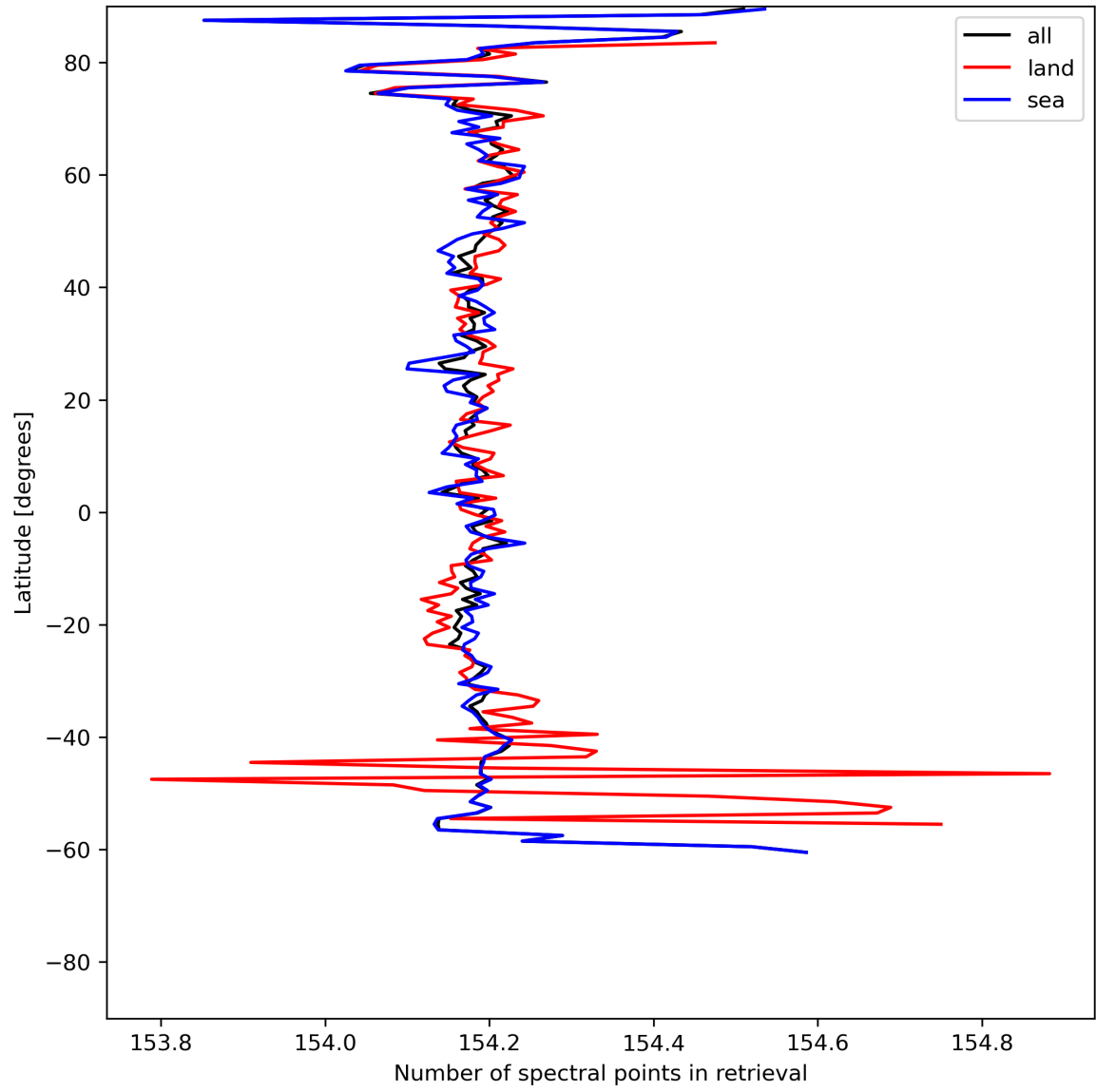
Figure 13: Zonal average of “Number of spectral points in retrieval” for 2024-06-19 to 2024-06-21.
