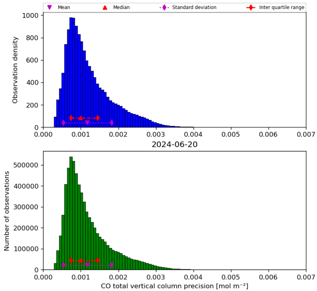
Figure 20: Histogram of “CO total vertical column precision” for 2024-06-19 to 2024-06-21
