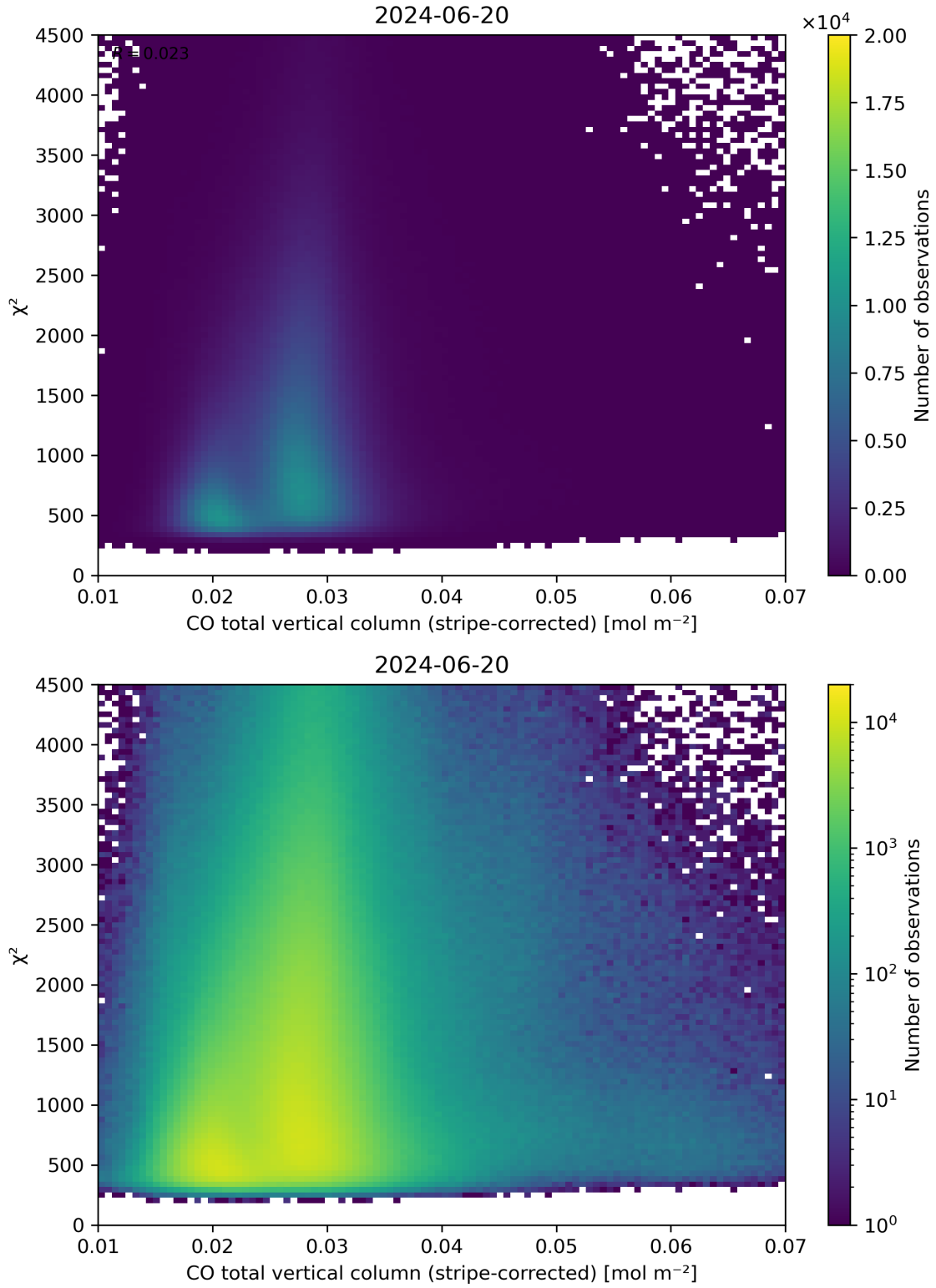
Figure 37: Scatter density plot of “CO total vertical column (stripe-corrected)” against “ \chi^2 ” for 2024-06-19 to 2024-06-21.
