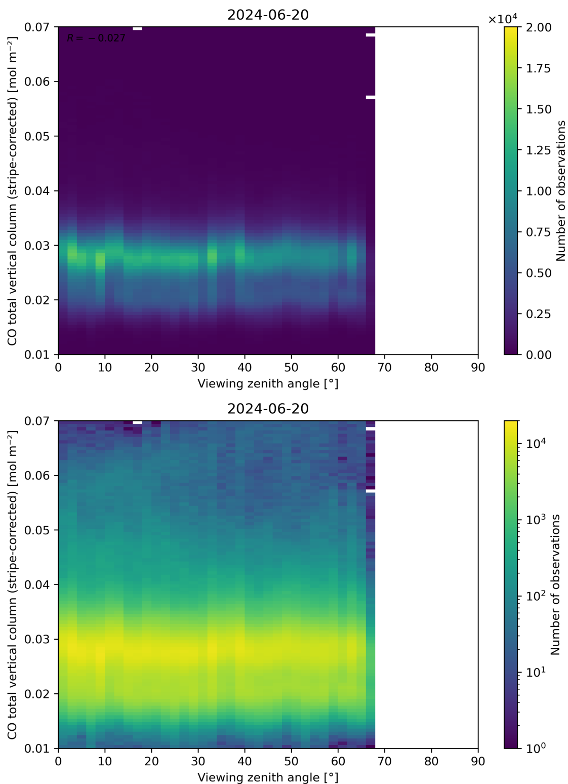
Figure 70: Scatter density plot of “Viewing zenith angle” against “CO total vertical column (stripe-corrected)” for 2024-06-19 to 2024-06-21.
