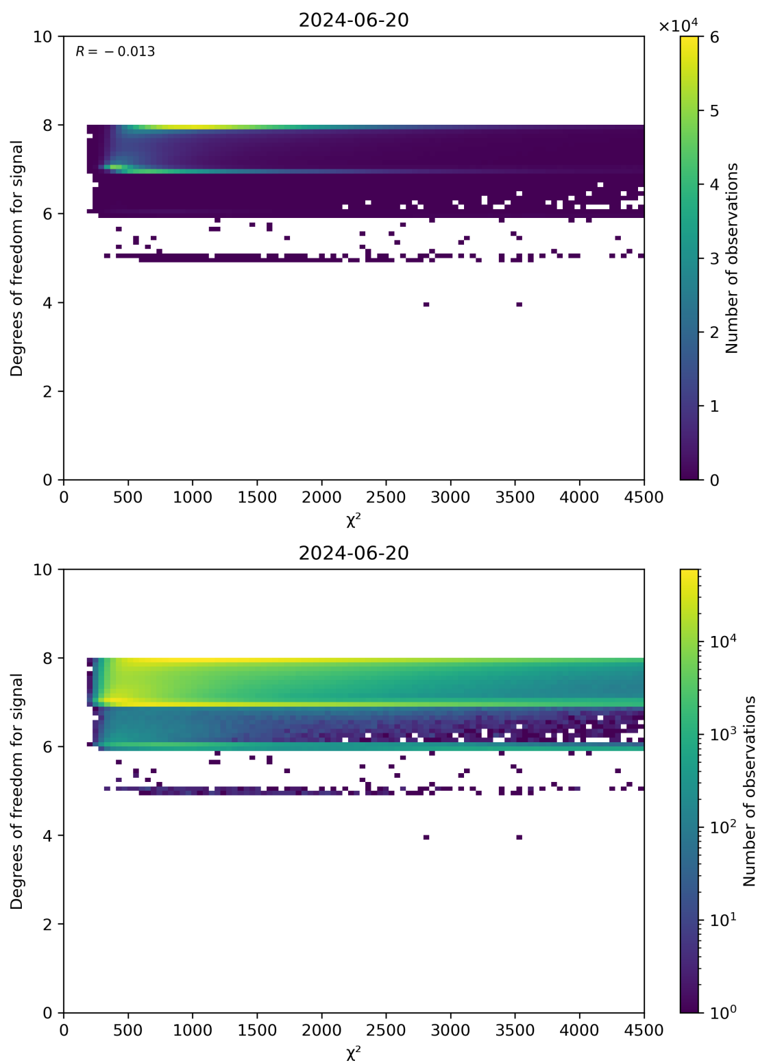
Figure 48: Scatter density plot of “ \chi^2 ” against “Degrees of freedom for signal” for 2024-06-19 to 2024-06-21.
