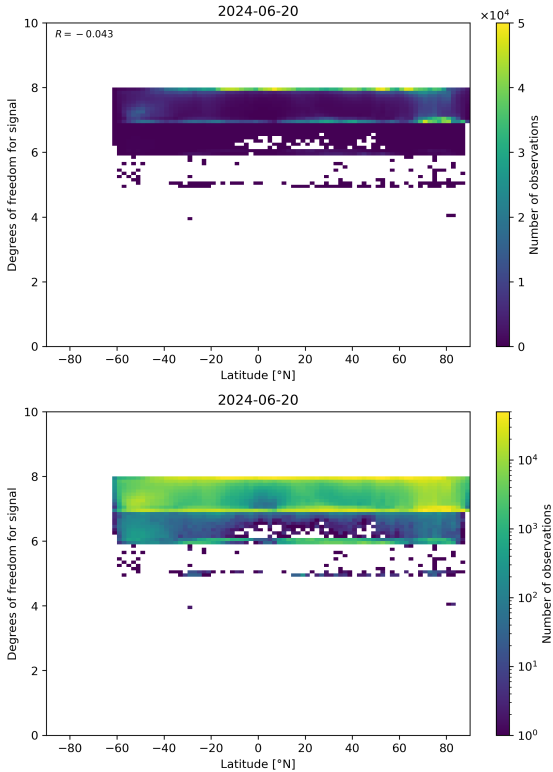
Figure 55: Scatter density plot of “Latitude” against “Degrees of freedom for signal” for 2024-06-19 to 2024-06-21.
