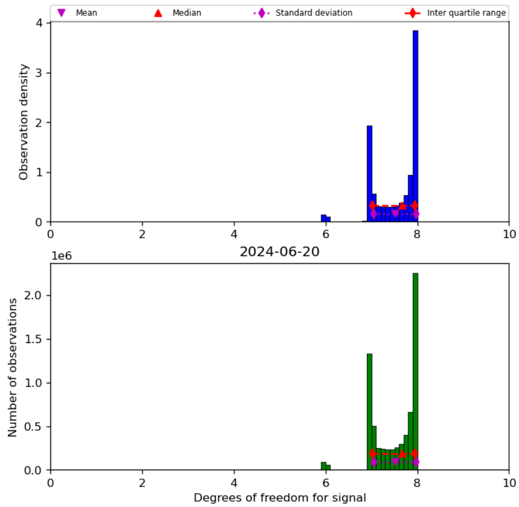
Figure 23: Histogram of “Degrees of freedom for signal” for 2024-06-19 to 2024-06-21
