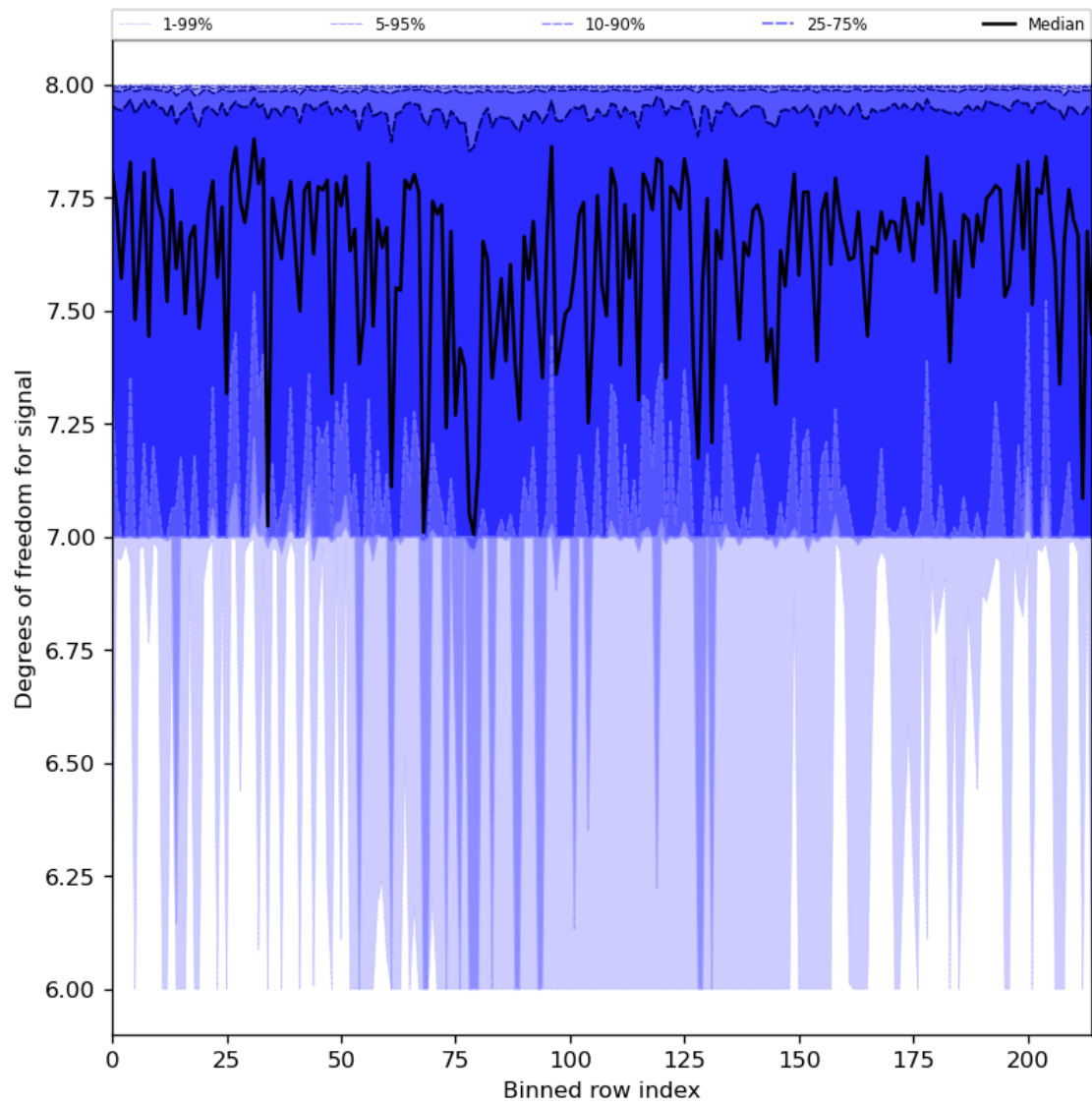
Figure 31: Along track statistics of “Degrees of freedom for signal” for 2024-06-19 to 2024-06-21
