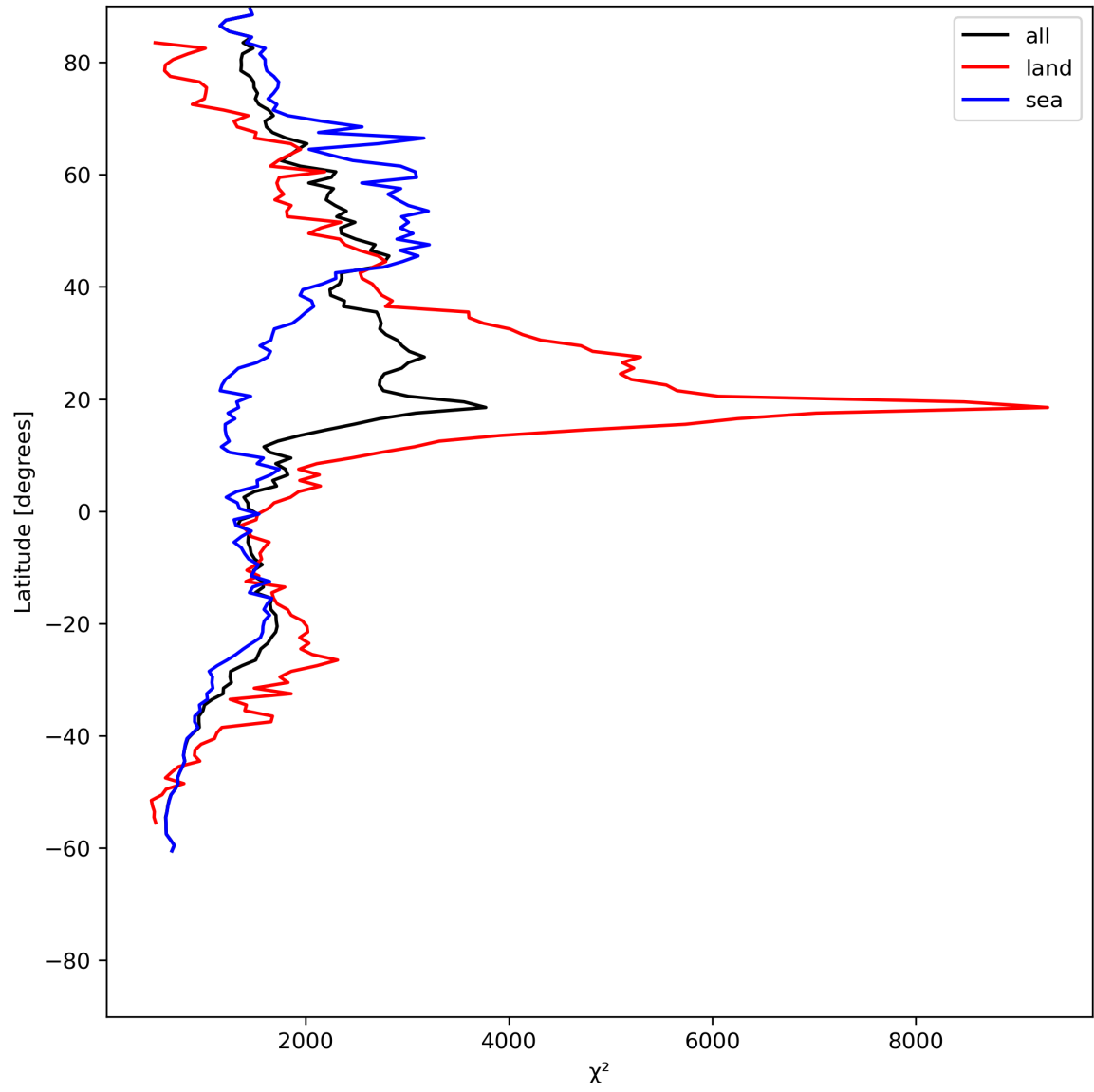
Figure 14: Zonal average of “ \chi^2 ” for 2024-06-19 to 2024-06-21.
