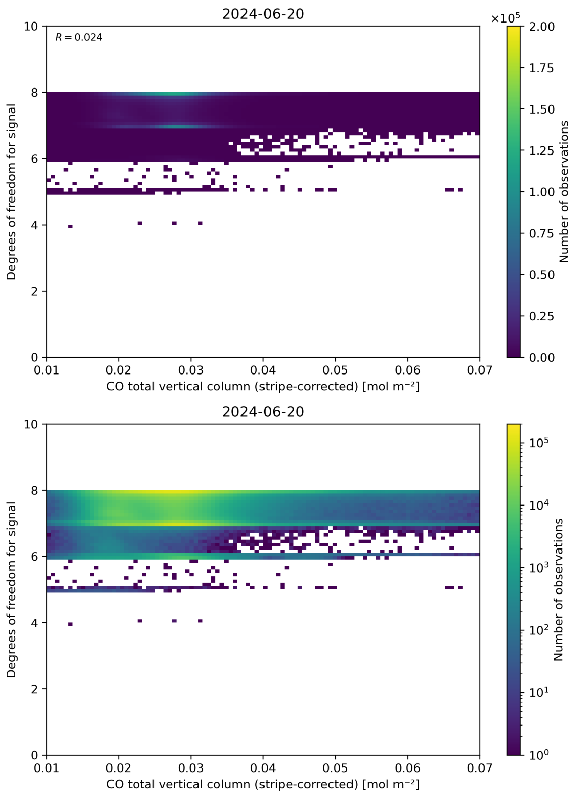
Figure 38: Scatter density plot of “CO total vertical column (stripe-corrected)” against “Degrees of freedom for signal” for 2024-06-19 to 2024-06-21.
