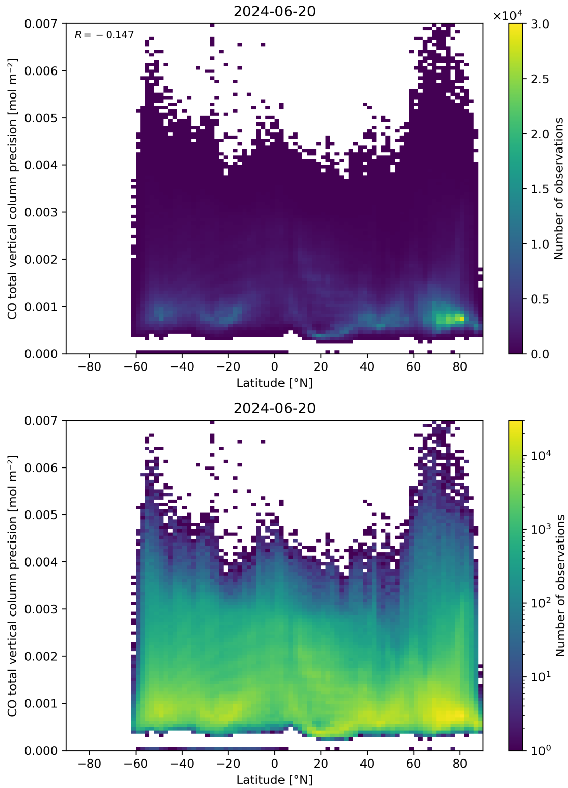
Figure 53: Scatter density plot of “Latitude” against “CO total vertical column precision” for 2024-06-19 to 2024-06-21.
