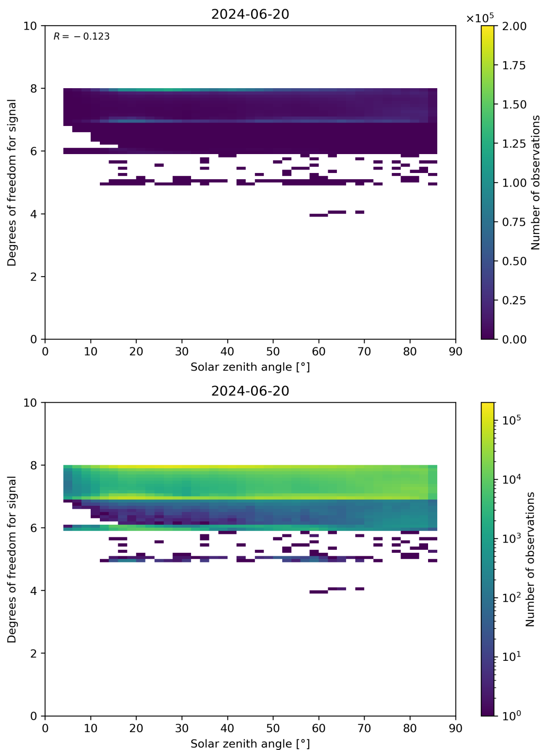
Figure 65: Scatter density plot of “Solar zenith angle” against “Degrees of freedom for signal” for 2024-06-19 to 2024-06-21.
