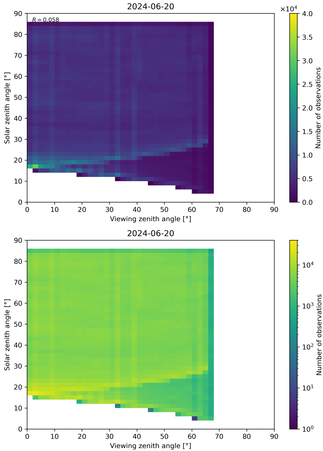
Figure 77: Scatter density plot of “Viewing zenith angle” against “Solar zenith angle” for 2024-06-19 to 2024-06-21.
