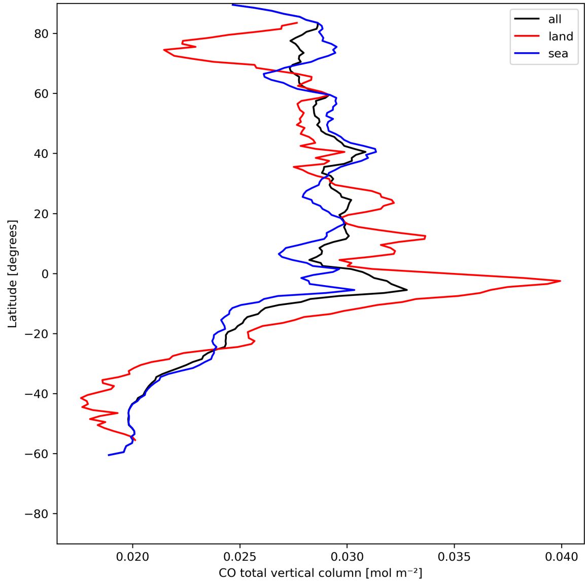
Figure 10: Zonal average of “CO total vertical column” for 2024-06-19 to 2024-06-21.
