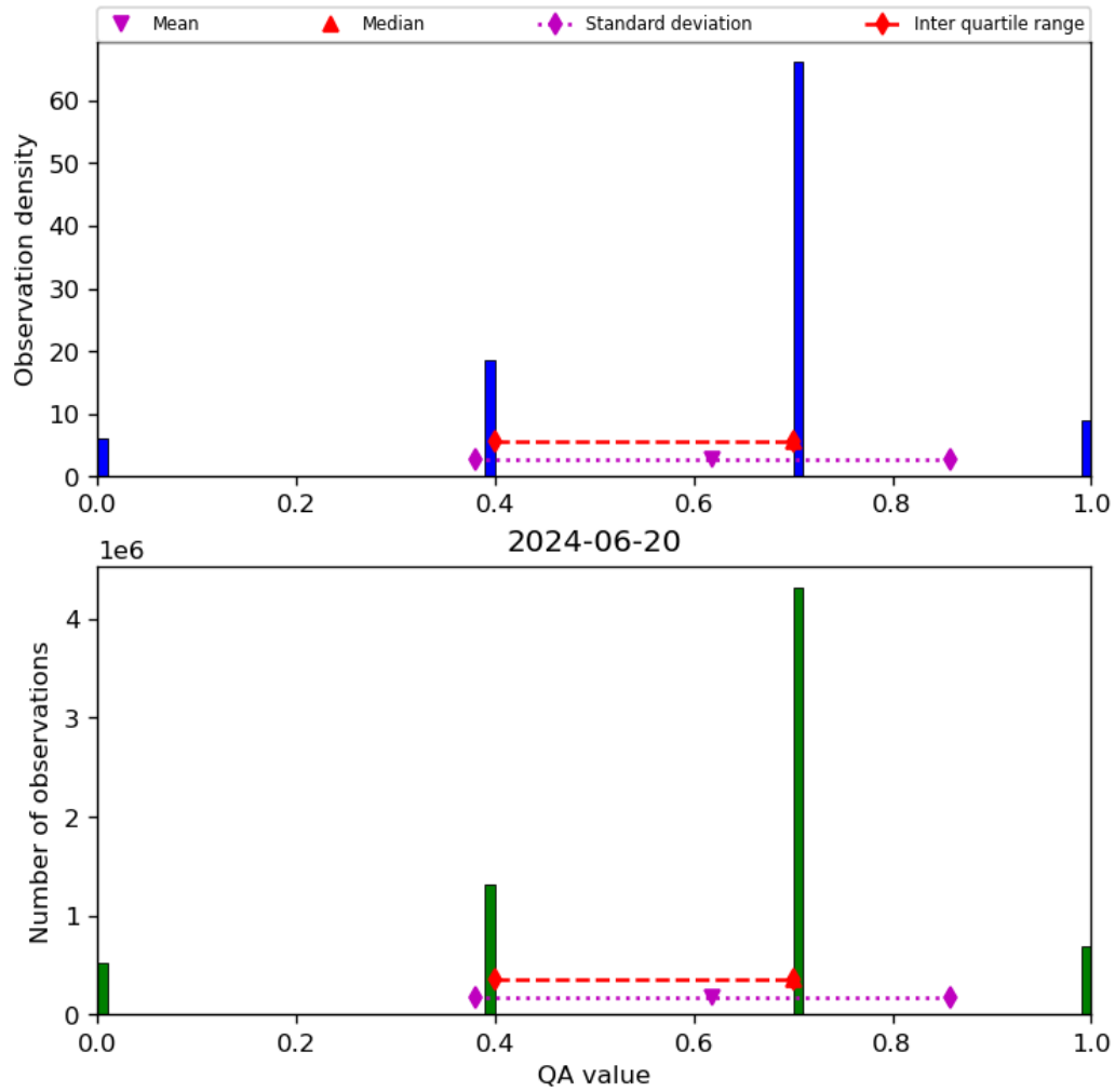
Figure 17: Histogram of “QA value” for 2024-06-19 to 2024-06-21
