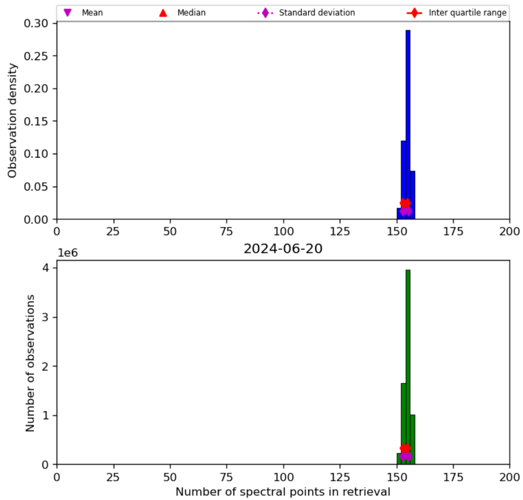
Figure 21: Histogram of “Number of spectral points in retrieval” for 2024-06-19 to 2024-06-21
