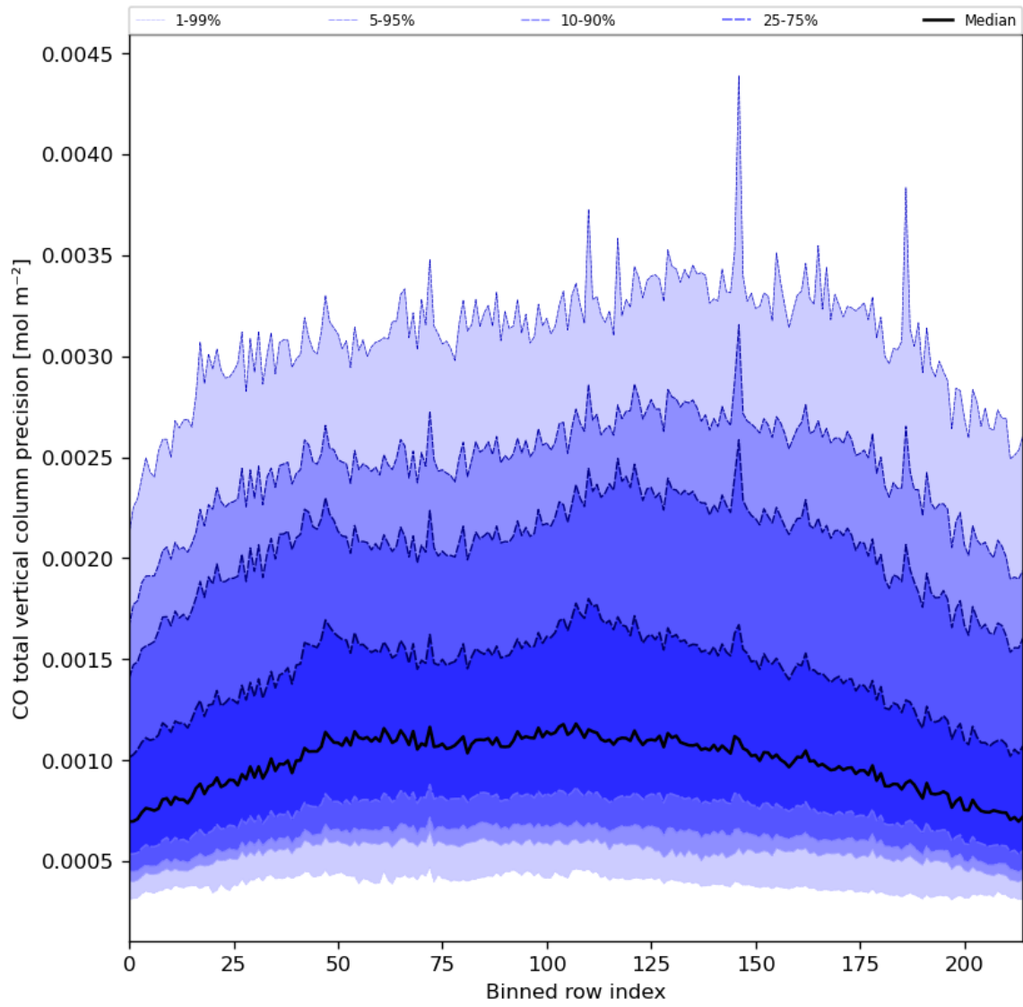
Figure 28: Along track statistics of “CO total vertical column precision” for 2024-06-19 to 2024-06-21
