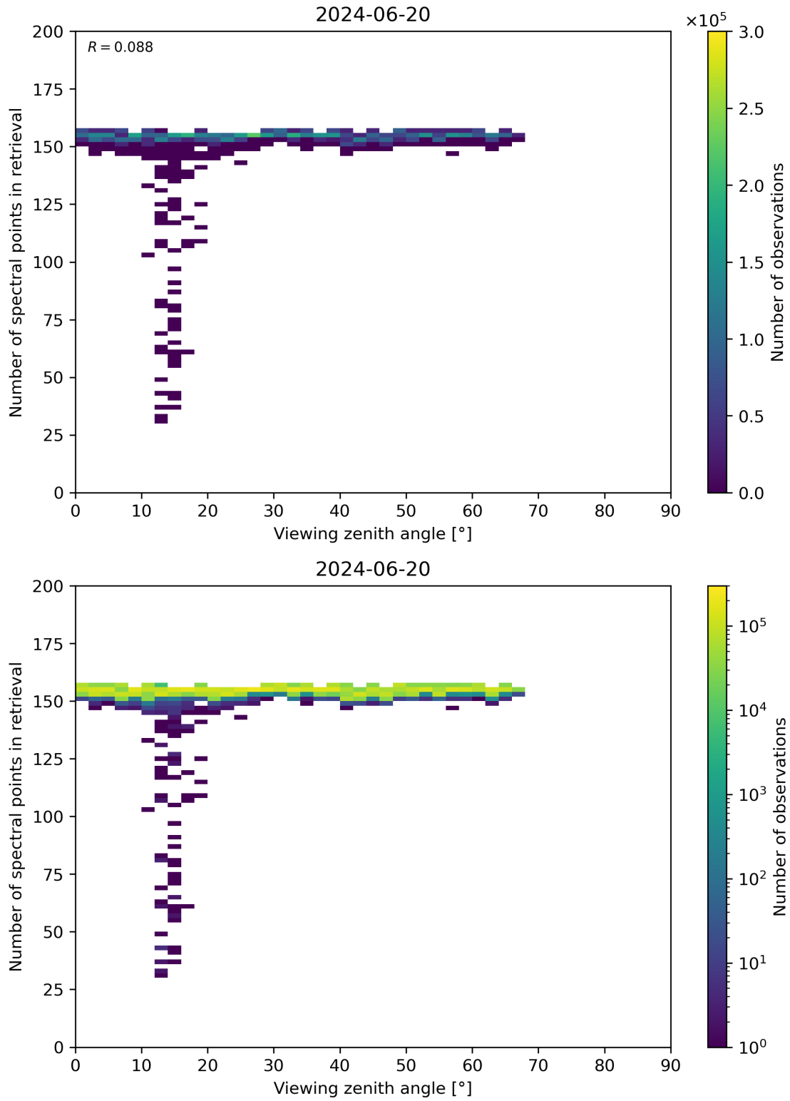
Figure 76: Scatter density plot of “Viewing zenith angle” against “Number of spectral points in retrieval” for 2024-06-19 to 2024-06-21.
