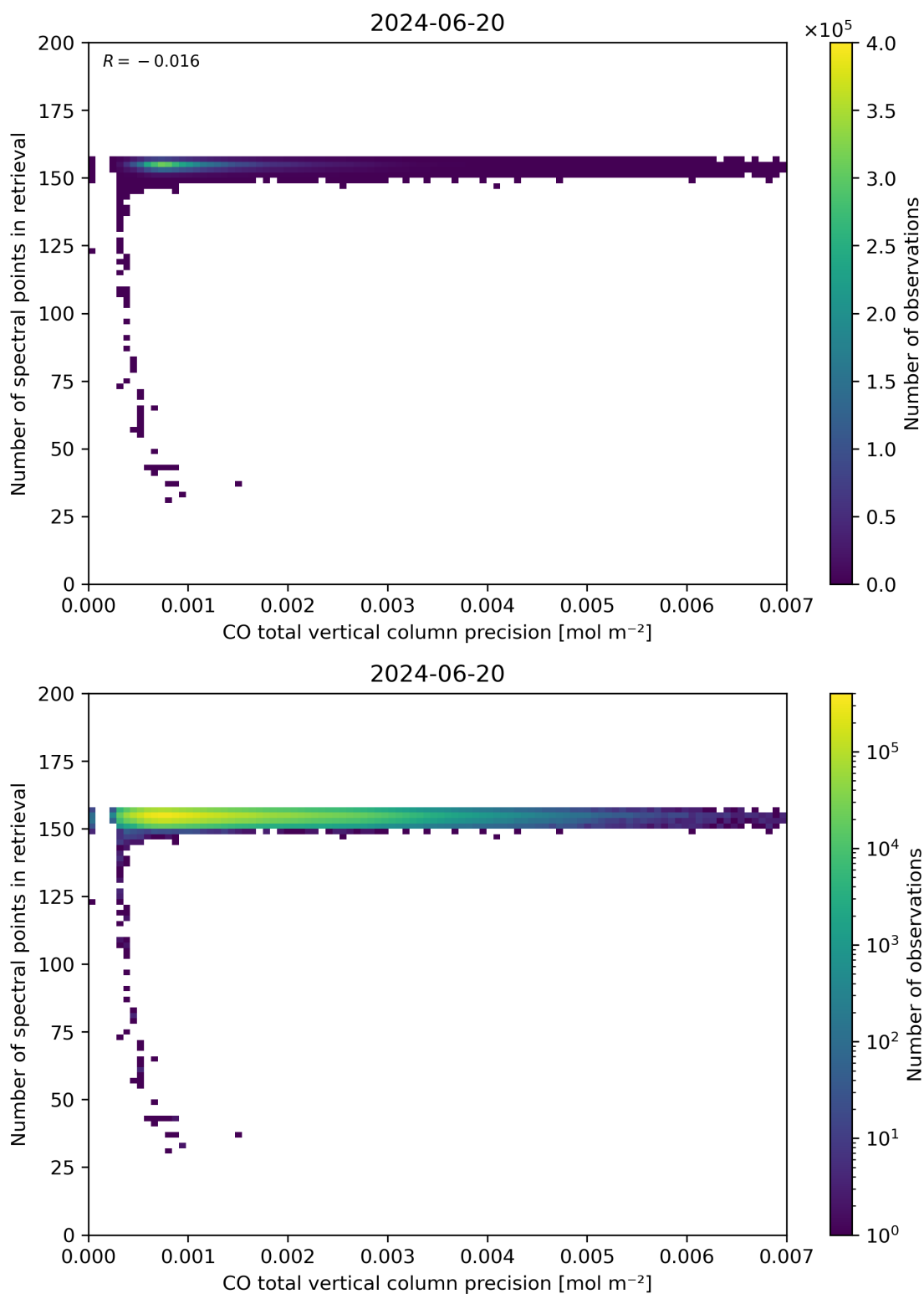
Figure 47: Scatter density plot of “CO total vertical column precision” against “Number of spectral points in retrieval” for 2024-06-19 to 2024-06-21.
