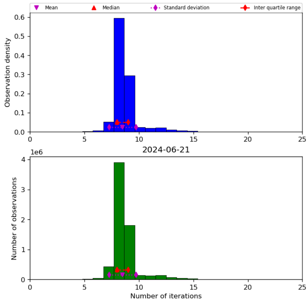
Figure 24: Histogram of “Number of iterations” for 2024-06-20 to 2024-06-22
