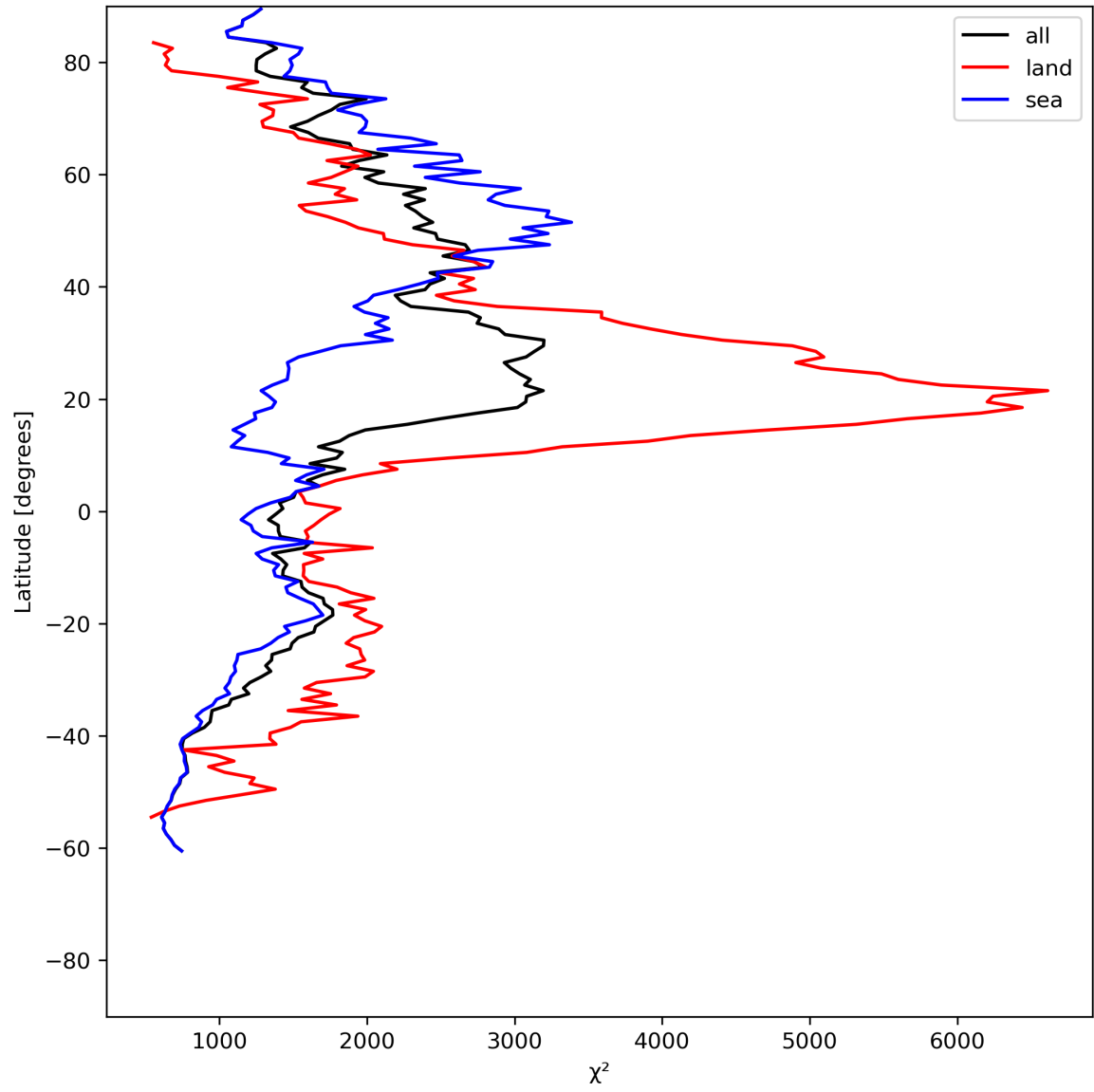
Figure 14: Zonal average of “ \chi^2 ” for 2024-06-20 to 2024-06-22.
