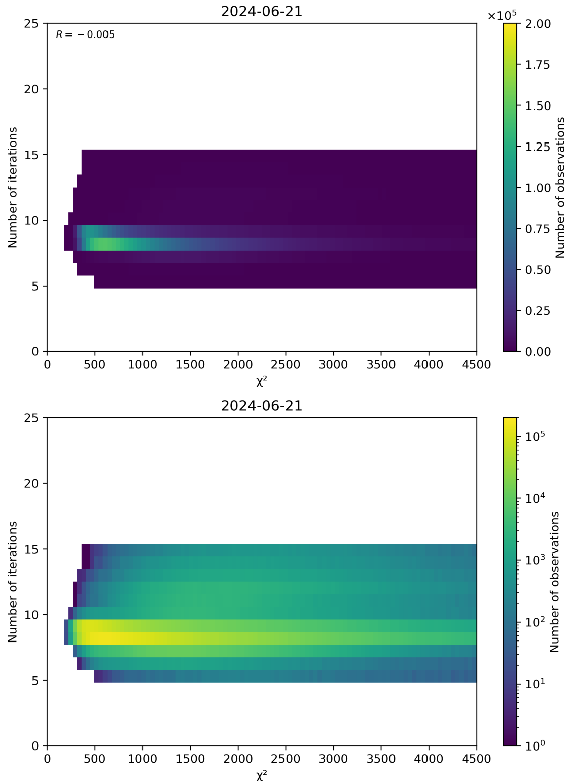
Figure 49: Scatter density plot of “ \chi^2 ” against “Number of iterations” for 2024-06-20 to 2024-06-22.
