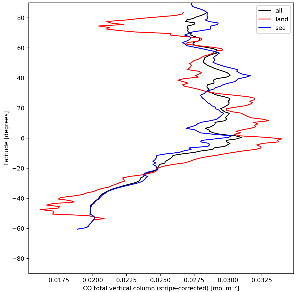
Figure 11: Zonal average of “CO total vertical column (stripe-corrected)” for 2024-06-20 to 2024-06-22.
