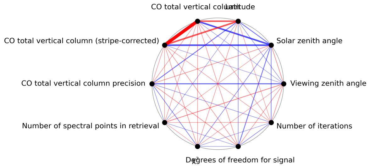
Figure 1: Map of correlation graph for 2024-06-20 to 2024-06-22.
