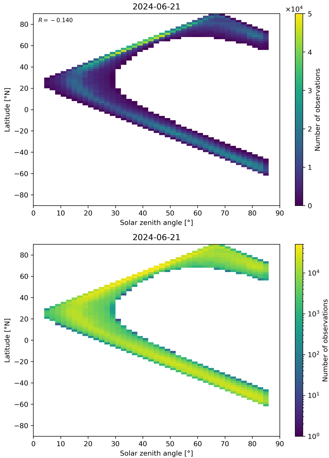
Figure 66: Scatter density plot of “Solar zenith angle” against “Latitude” for 2024-06-20 to 2024-06-22.
