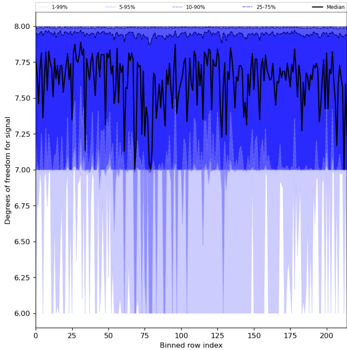
Figure 31: Along track statistics of “Degrees of freedom for signal” for 2024-06-20 to 2024-06-22
