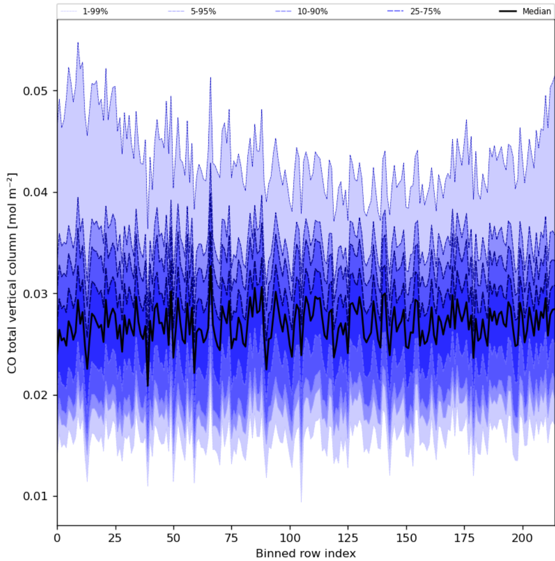
Figure 26: Along track statistics of “CO total vertical column” for 2024-06-20 to 2024-06-22
