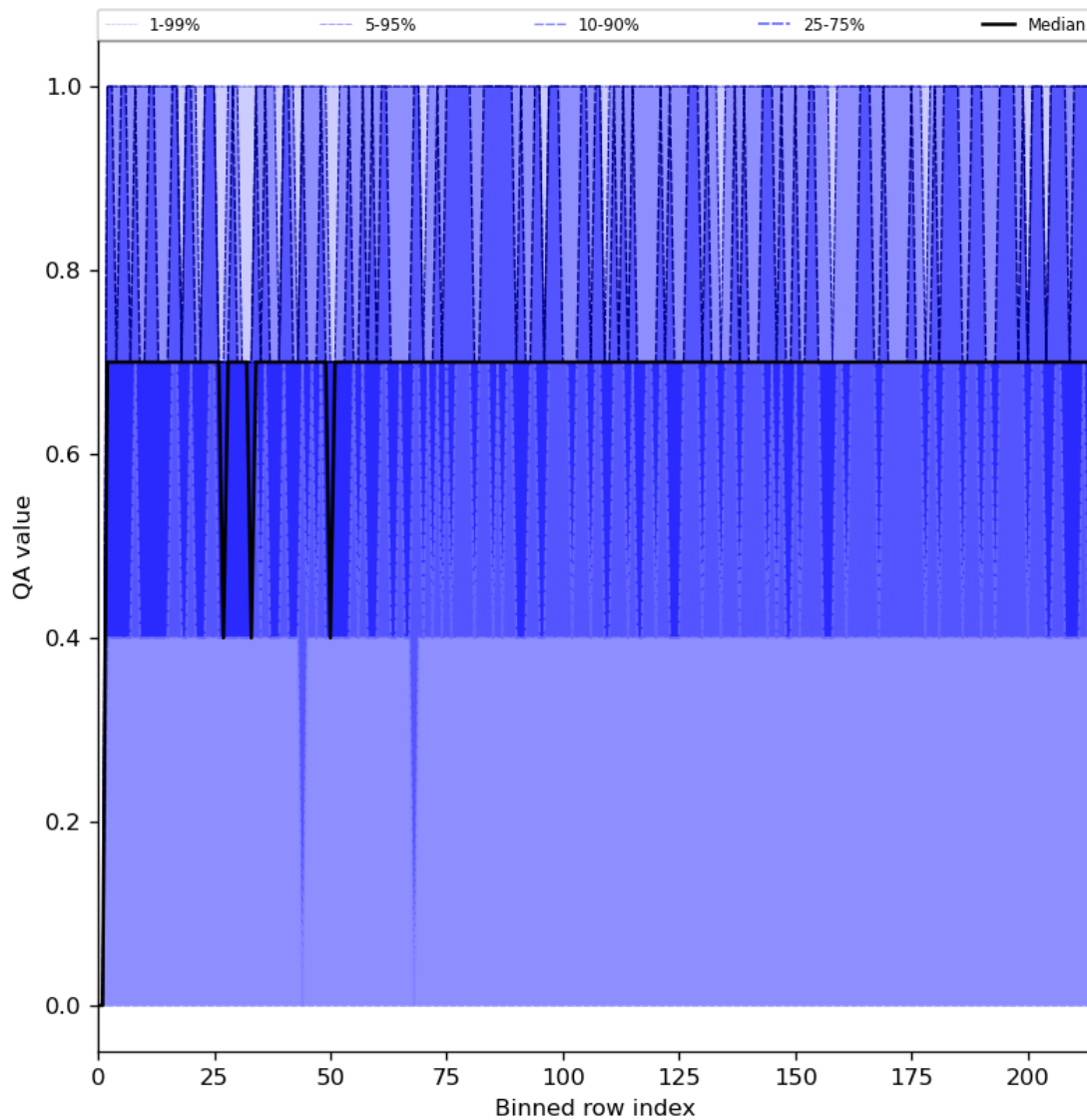
Figure 25: Along track statistics of “QA value” for 2024-06-20 to 2024-06-22
