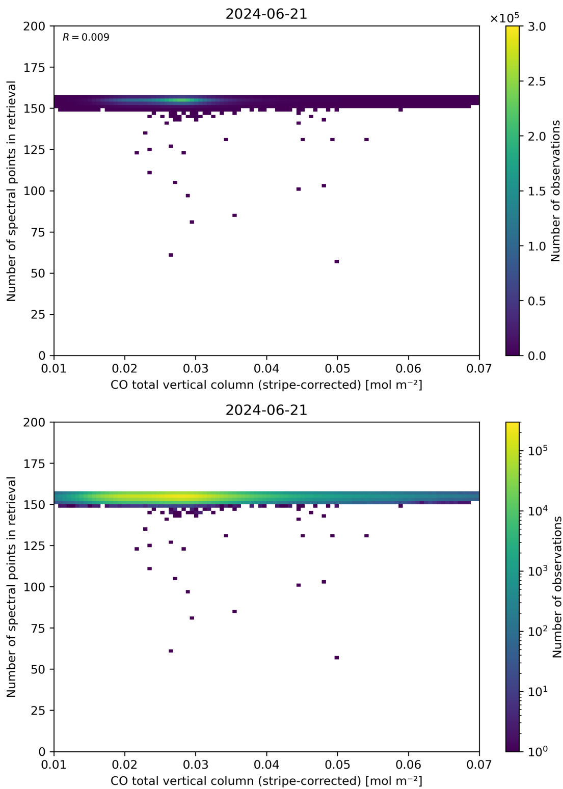
Figure 40: Scatter density plot of “CO total vertical column (stripe-corrected)” against “Number of spectral points in retrieval” for 2024-06-20 to 2024-06-22.
