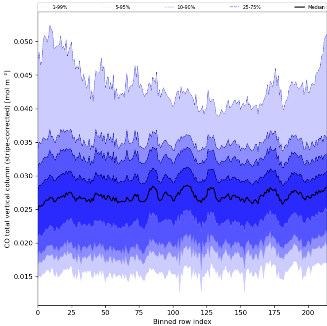
Figure 27: Along track statistics of “CO total vertical column (stripe-corrected)” for 2024-06-20 to 2024-06-22
