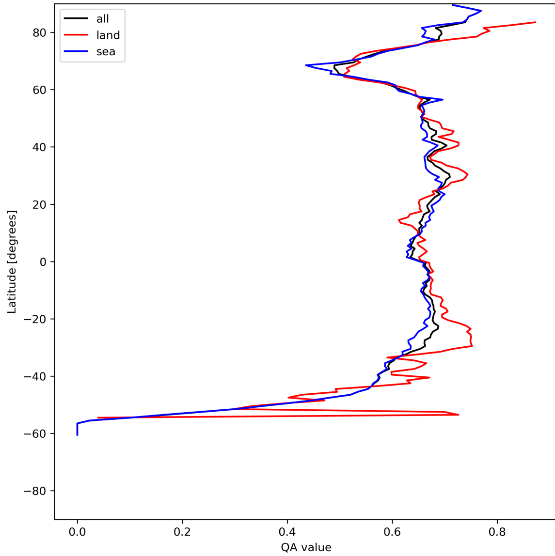
Figure 9: Zonal average of “QA value” for 2024-06-20 to 2024-06-22.
