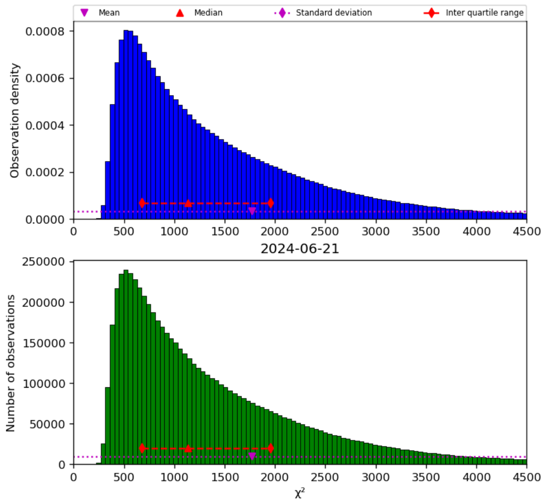
Figure 22: Histogram of “ \chi^2 ” for 2024-06-20 to 2024-06-22
