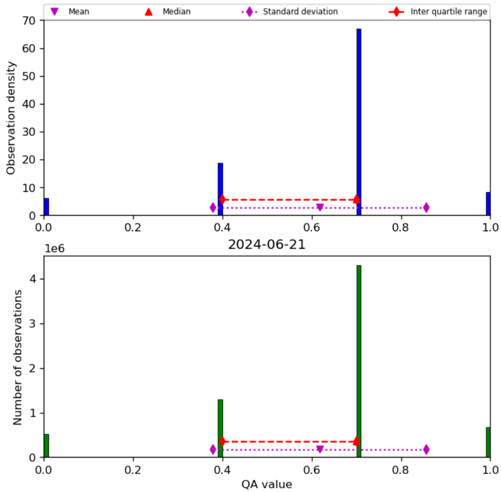
Figure 17: Histogram of “QA value” for 2024-06-20 to 2024-06-22
