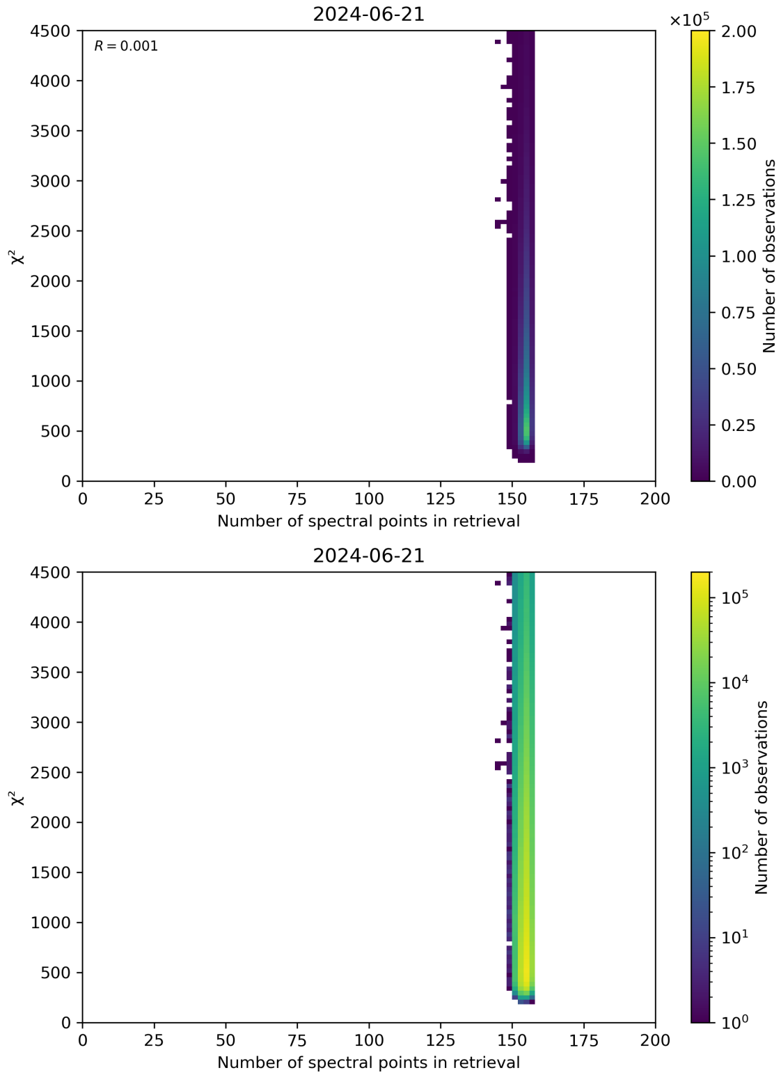
Figure 58: Scatter density plot of “Number of spectral points in retrieval” against “ \chi^2 ” for 2024-06-20 to 2024-06-22.
