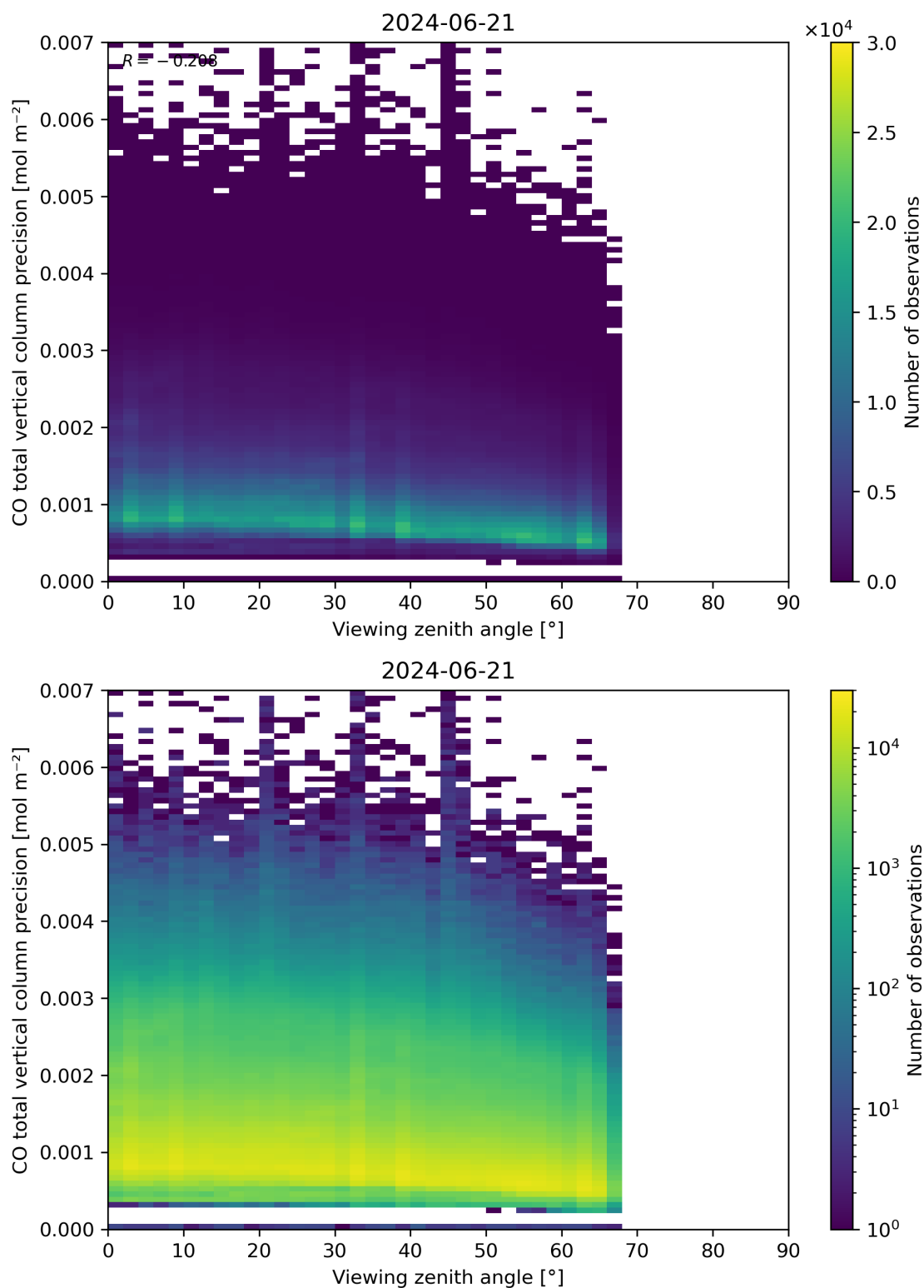
Figure 71: Scatter density plot of “Viewing zenith angle” against “CO total vertical column precision” for 2024-06-20 to 2024-06-22.
