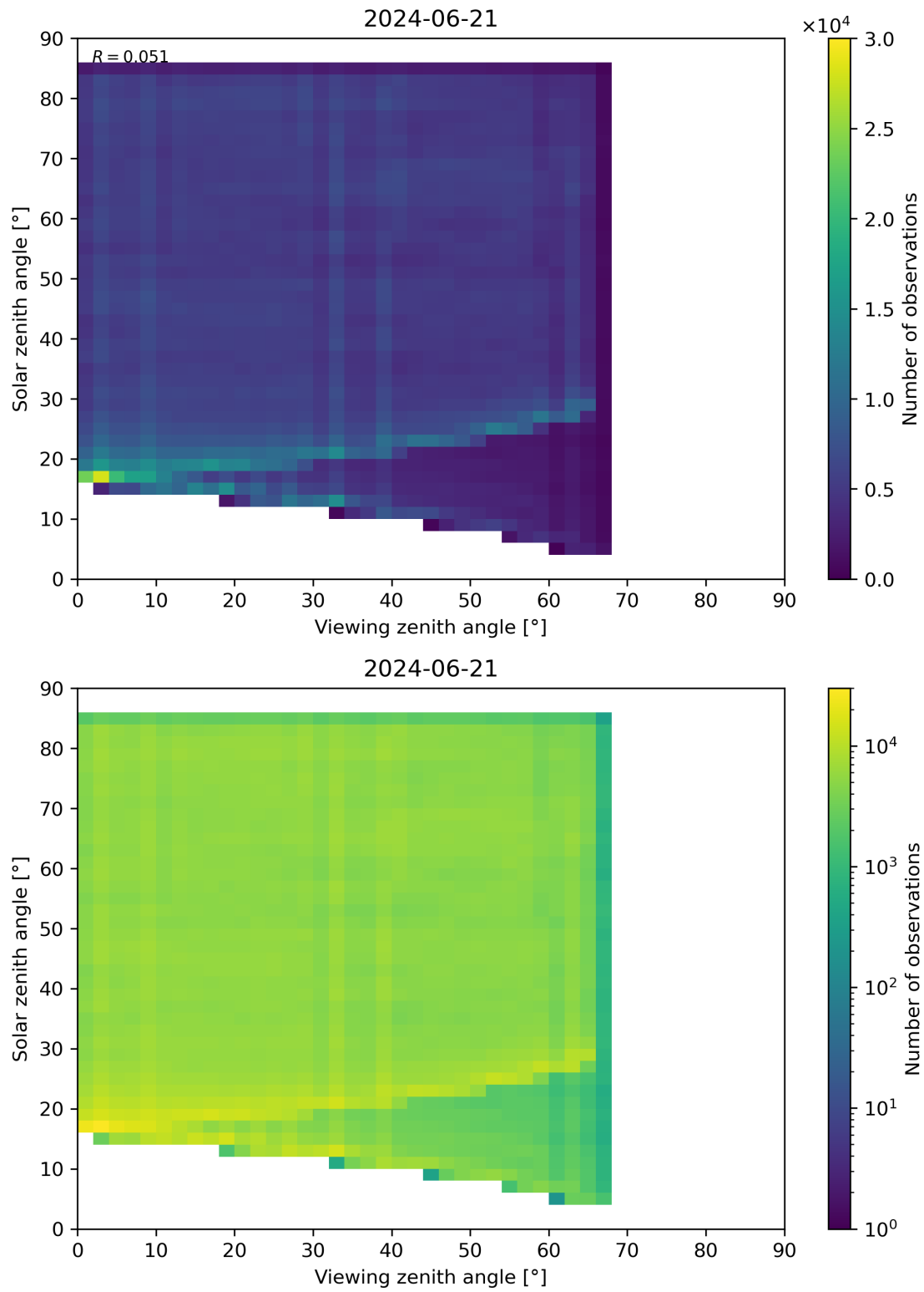
Figure 77: Scatter density plot of “Viewing zenith angle” against “Solar zenith angle” for 2024-06-20 to 2024-06-22.
