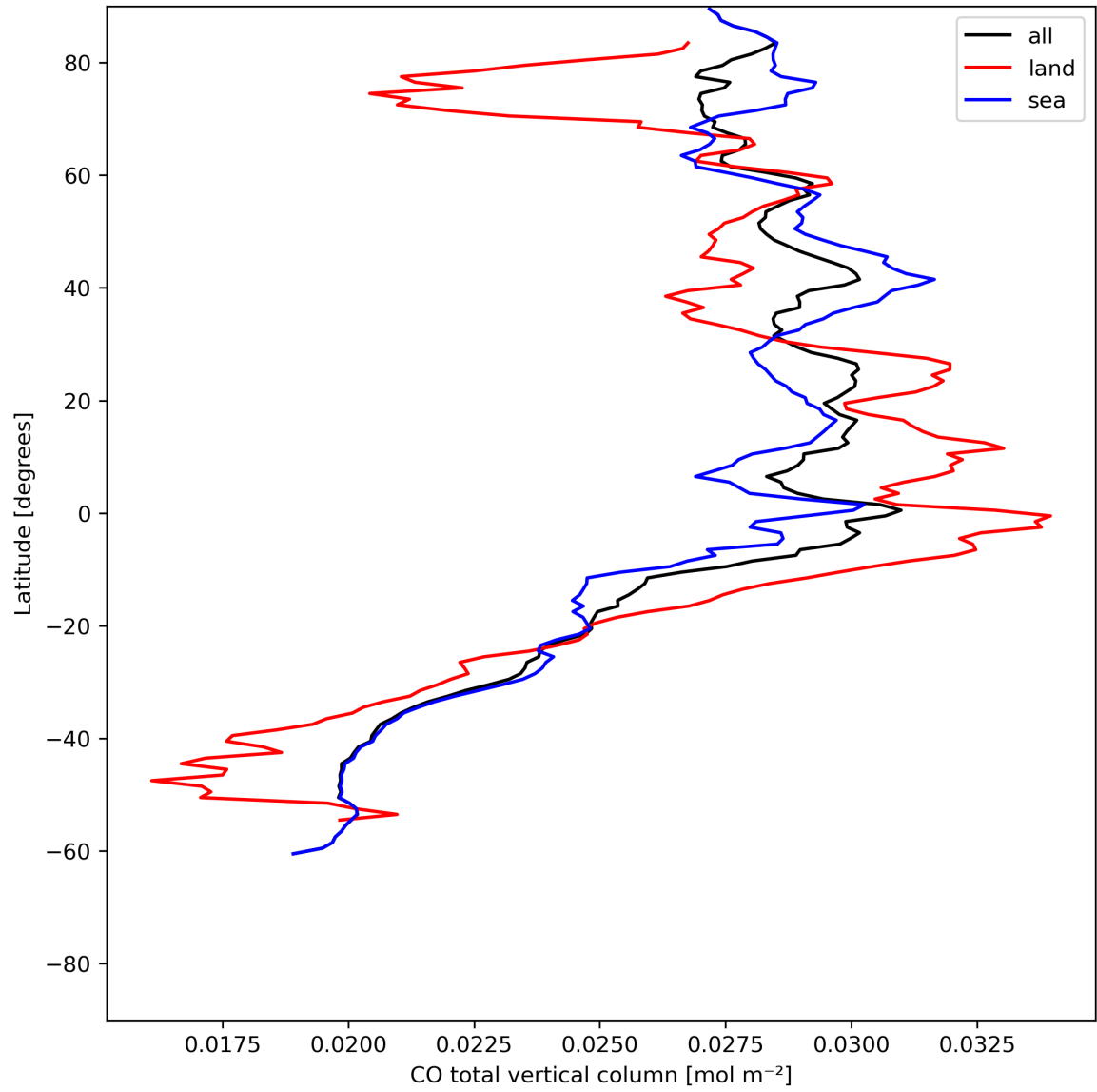
Figure 10: Zonal average of “CO total vertical column” for 2024-06-20 to 2024-06-22.
