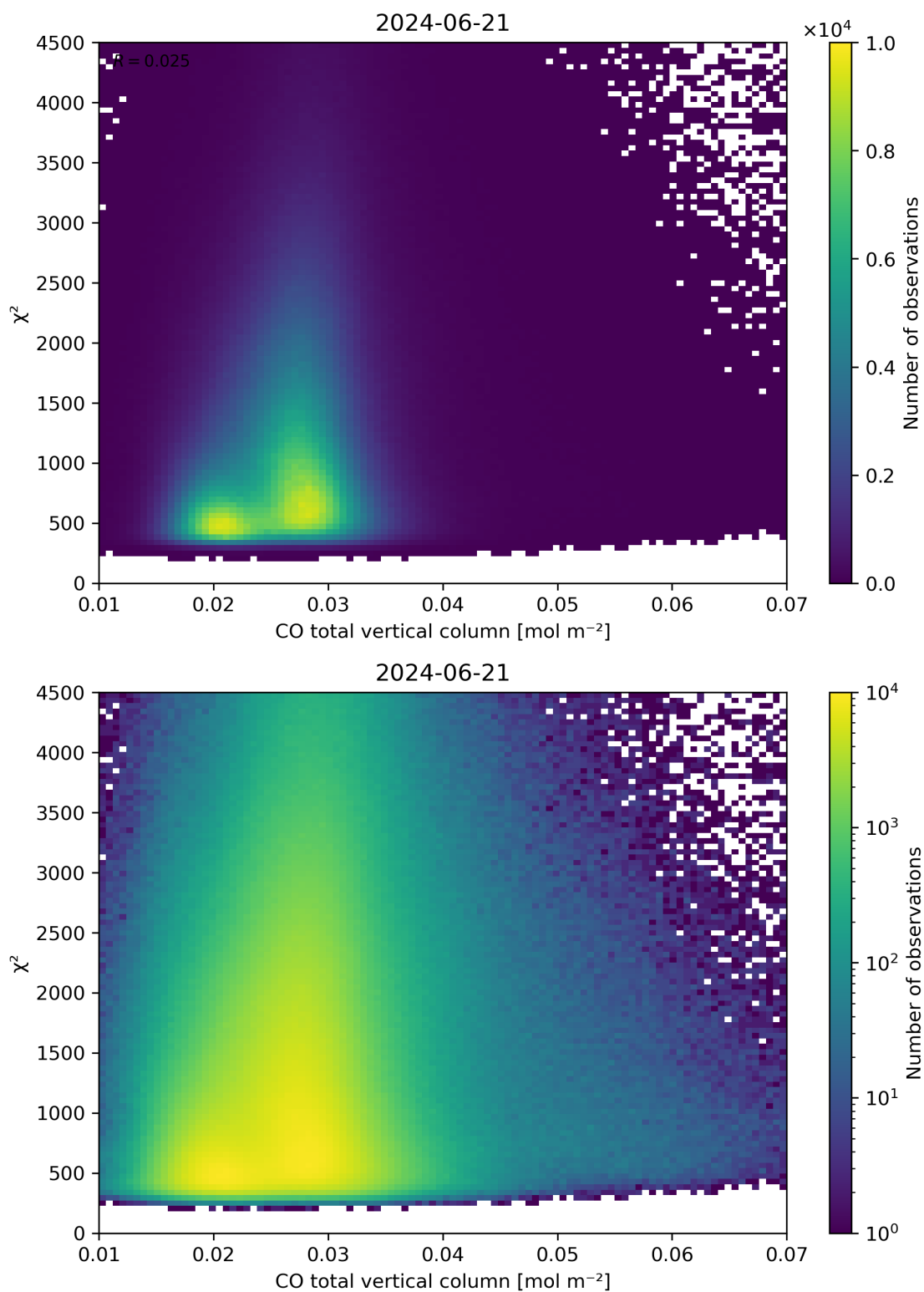
Figure 35: Scatter density plot of “CO total vertical column” against “ \chi^2 ” for 2024-06-20 to 2024-06-22.
