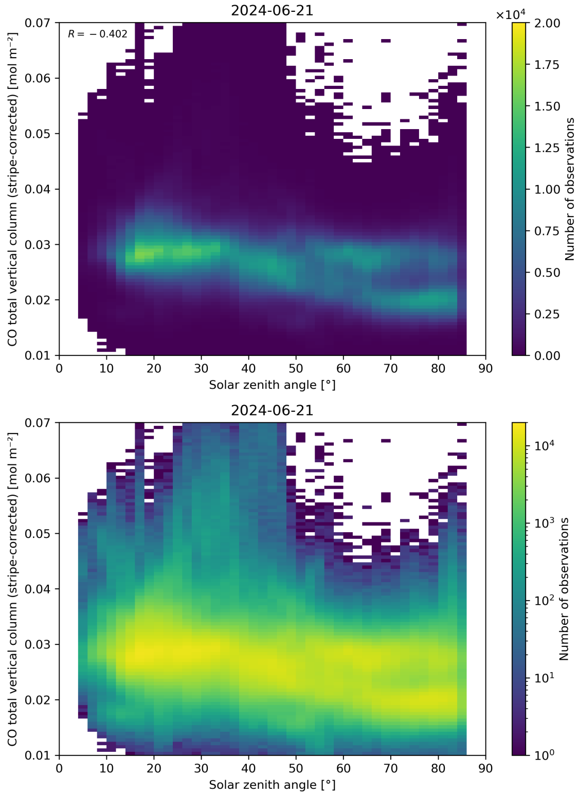
Figure 62: Scatter density plot of “Solar zenith angle” against “CO total vertical column (stripe-corrected)” for 2024-06-20 to 2024-06-22.
