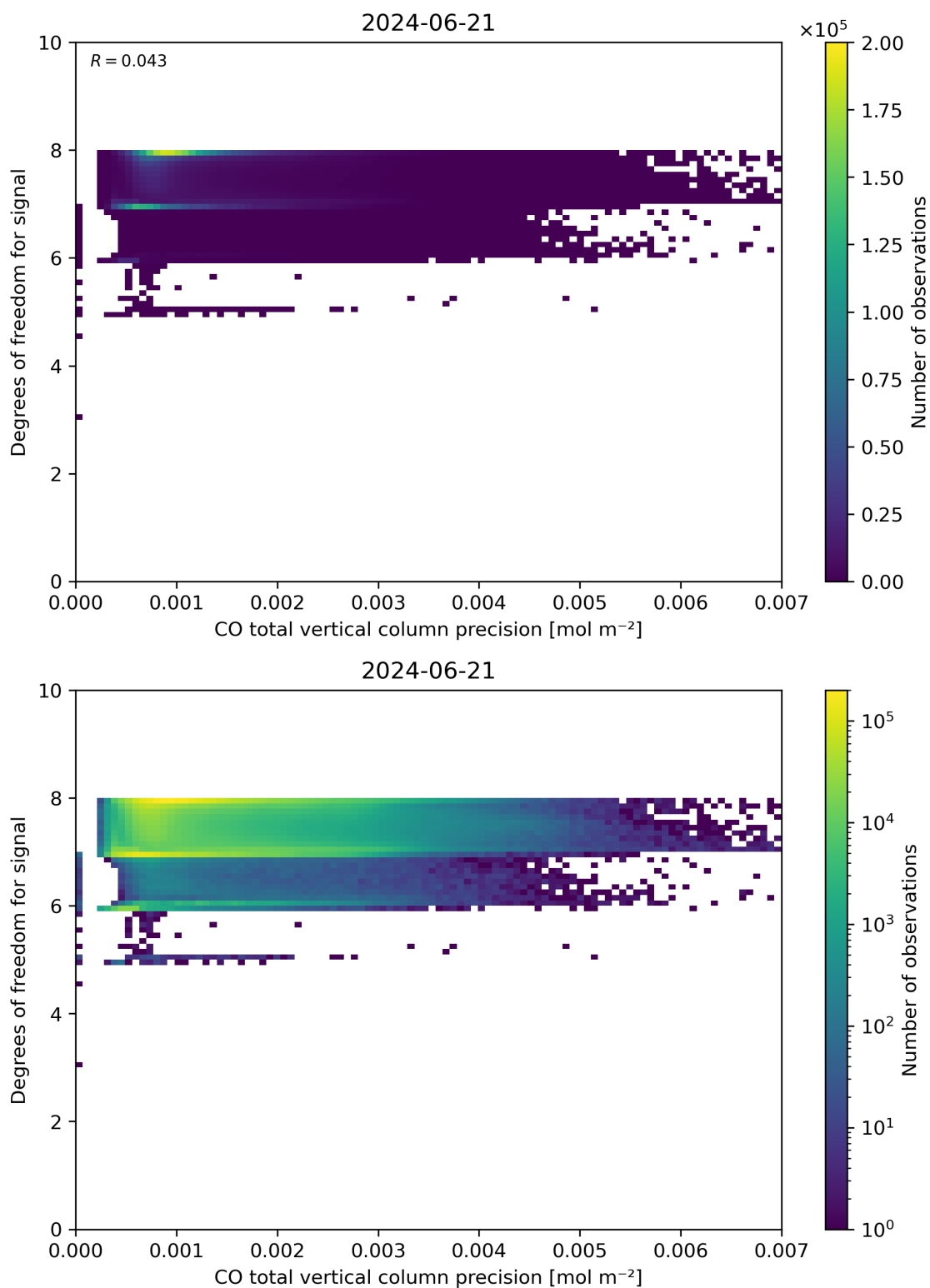
Figure 45: Scatter density plot of “CO total vertical column precision” against “Degrees of freedom for signal” for 2024-06-20 to 2024-06-22.
