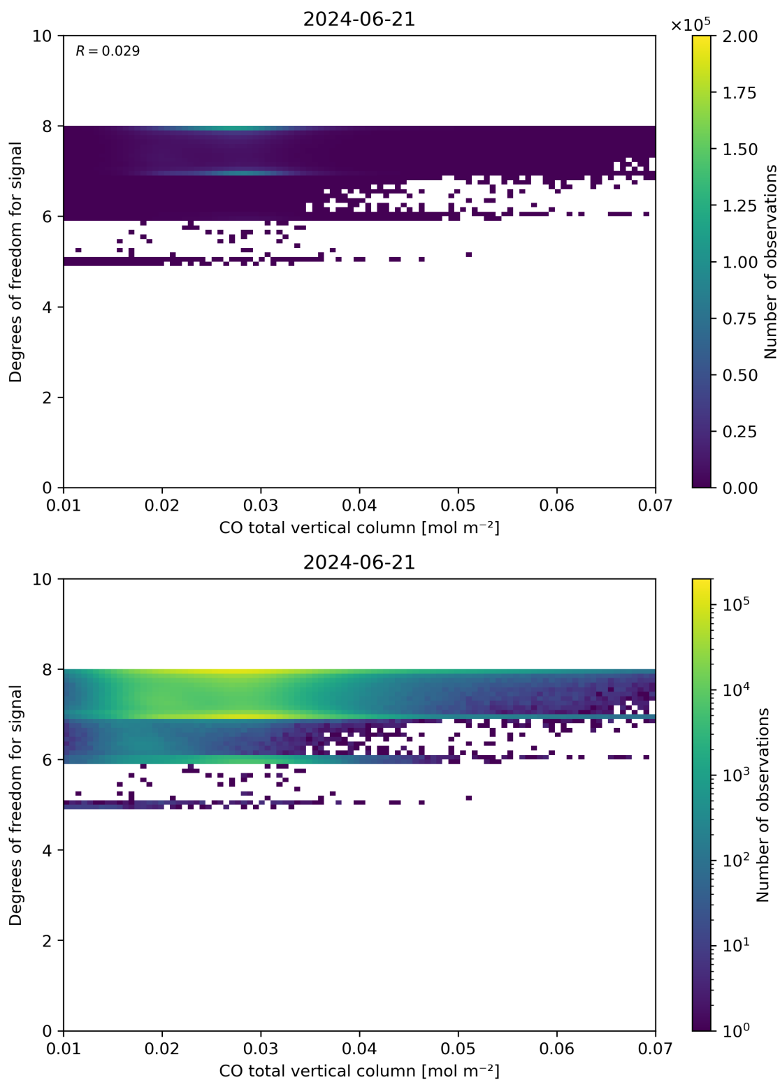
Figure 41: Scatter density plot of “CO total vertical column” against “Degrees of freedom for signal” for 2024-06-20 to 2024-06-22.
