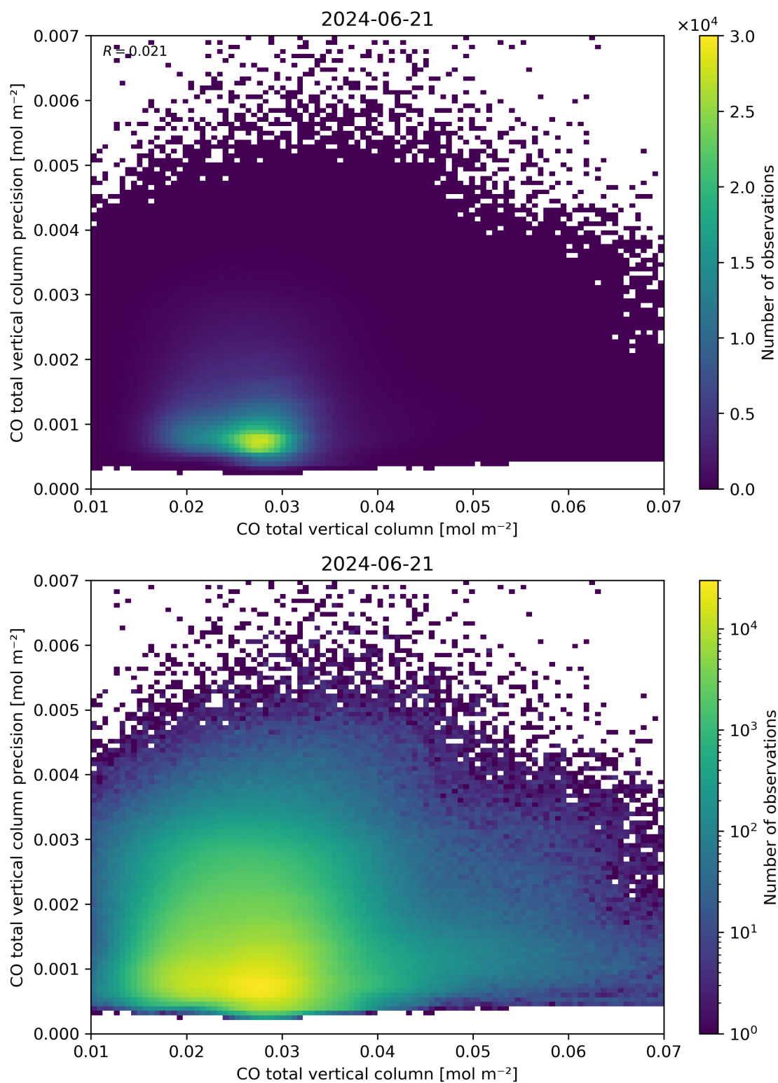
Figure 34: Scatter density plot of “CO total vertical column” against “CO total vertical column precision” for 2024-06-20 to 2024-06-22.
