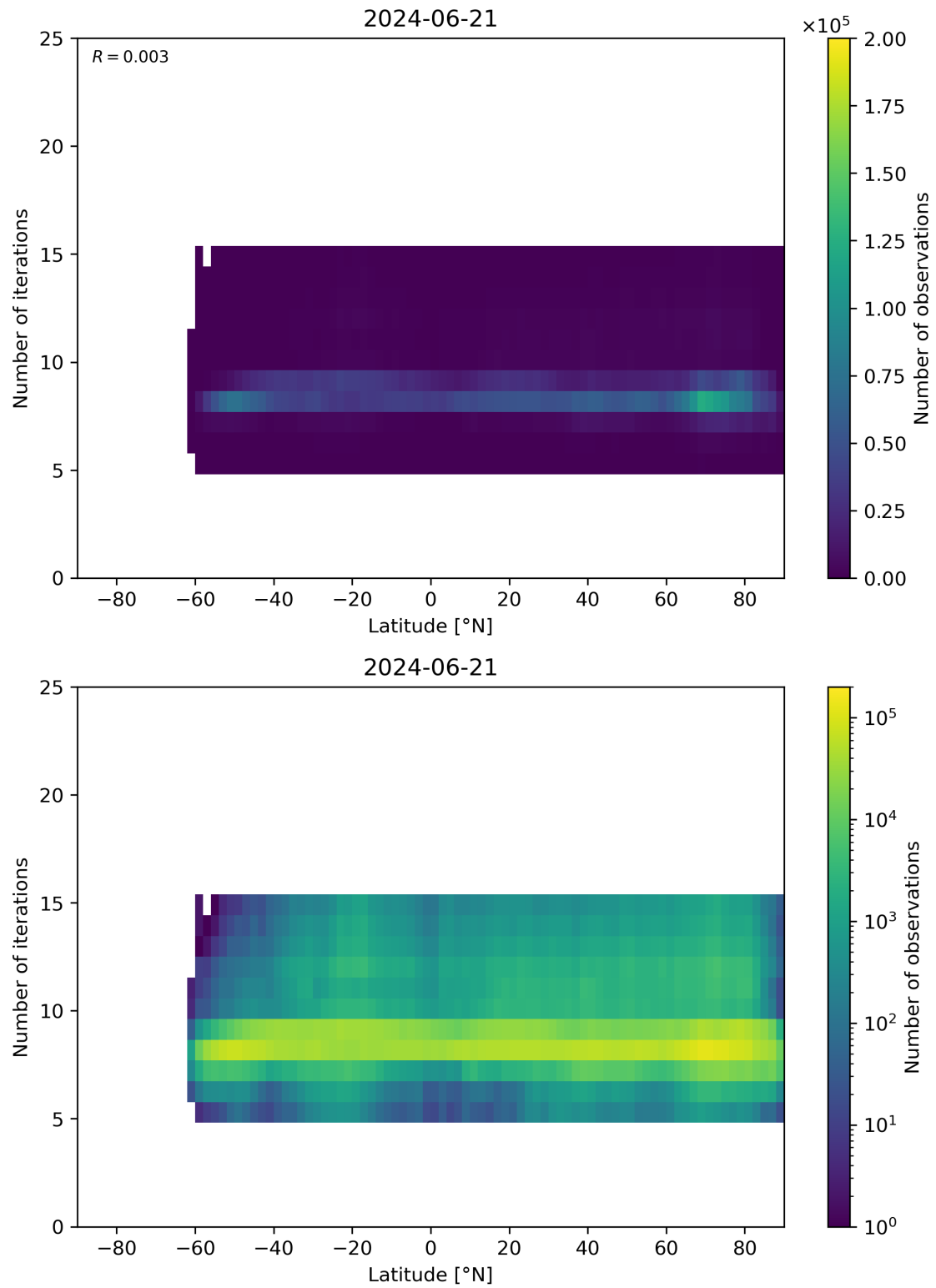
Figure 56: Scatter density plot of “Latitude” against “Number of iterations” for 2024-06-20 to 2024-06-22.
