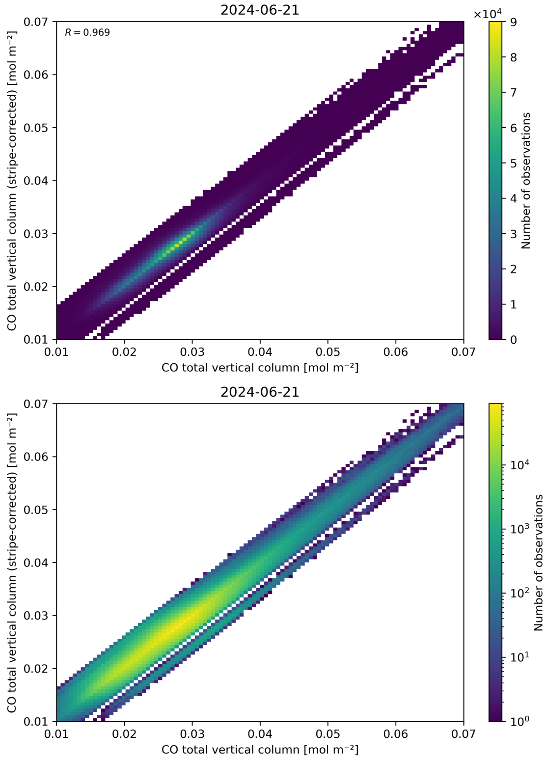
Figure 33: Scatter density plot of “CO total vertical column” against “CO total vertical column (stripe-corrected)” for 2024-06-20 to 2024-06-22.
