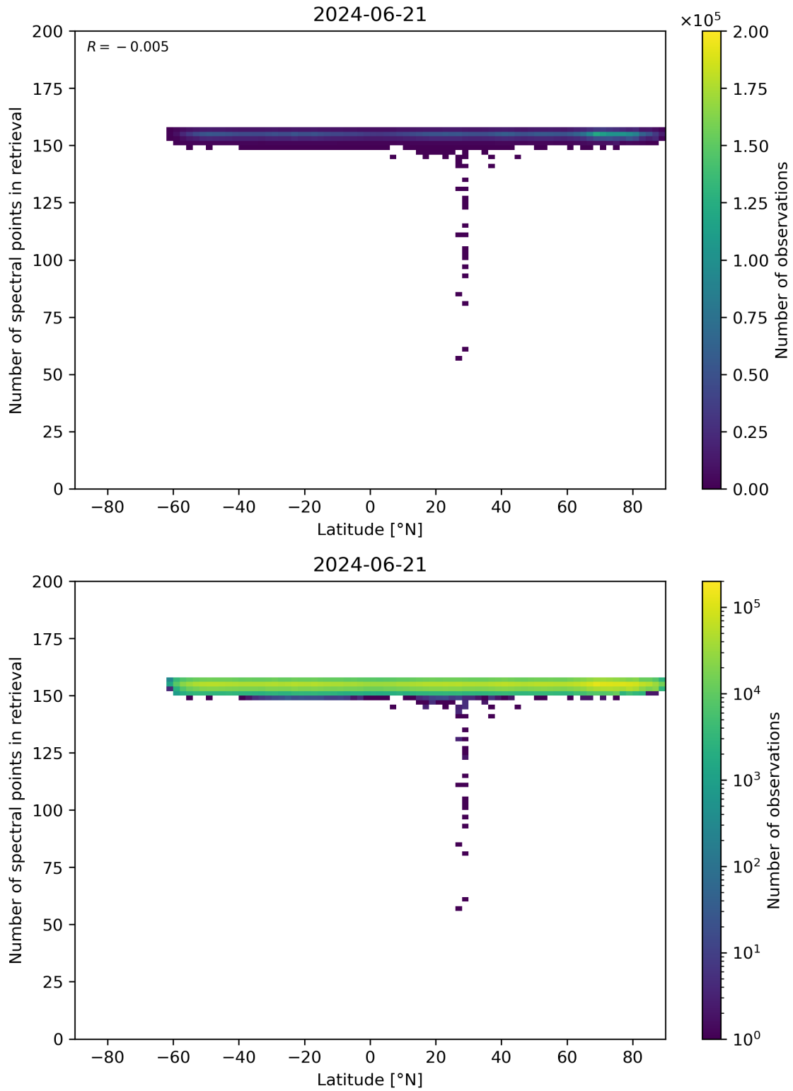
Figure 57: Scatter density plot of “Latitude” against “Number of spectral points in retrieval” for 2024-06-20 to 2024-06-22.
