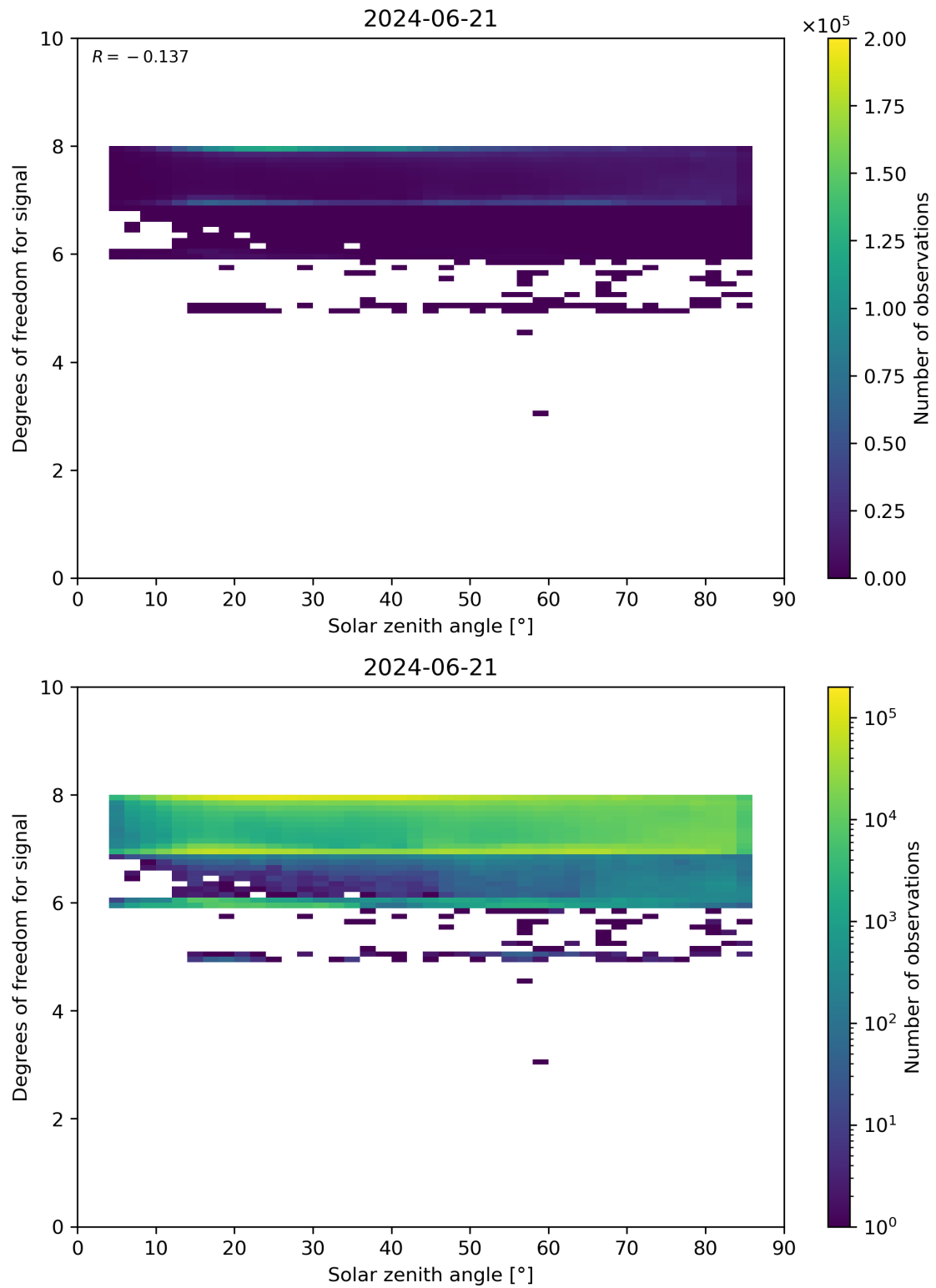
Figure 65: Scatter density plot of “Solar zenith angle” against “Degrees of freedom for signal” for 2024-06-20 to 2024-06-22.
