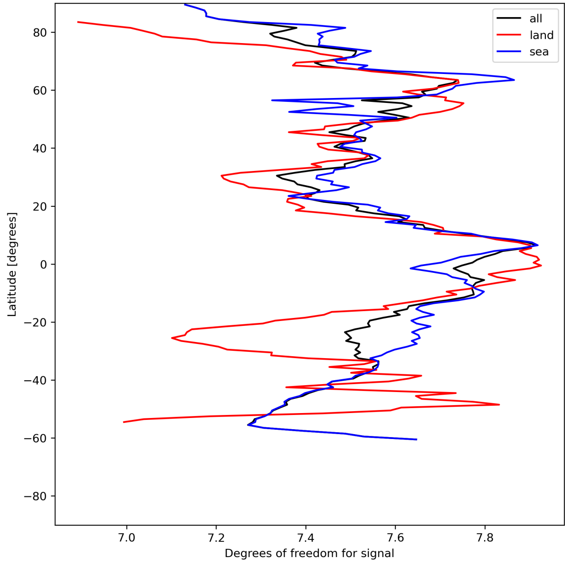
Figure 15: Zonal average of “Degrees of freedom for signal” for 2024-06-20 to 2024-06-22.
