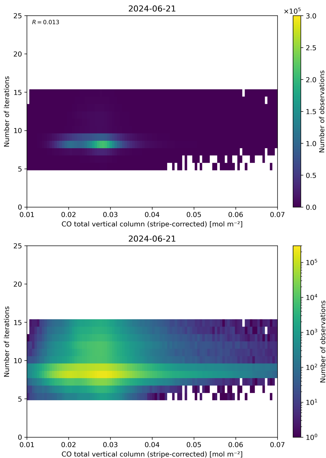
Figure 39: Scatter density plot of “CO total vertical column (stripe-corrected)” against “Number of iterations” for 2024-06-20 to 2024-06-22.
