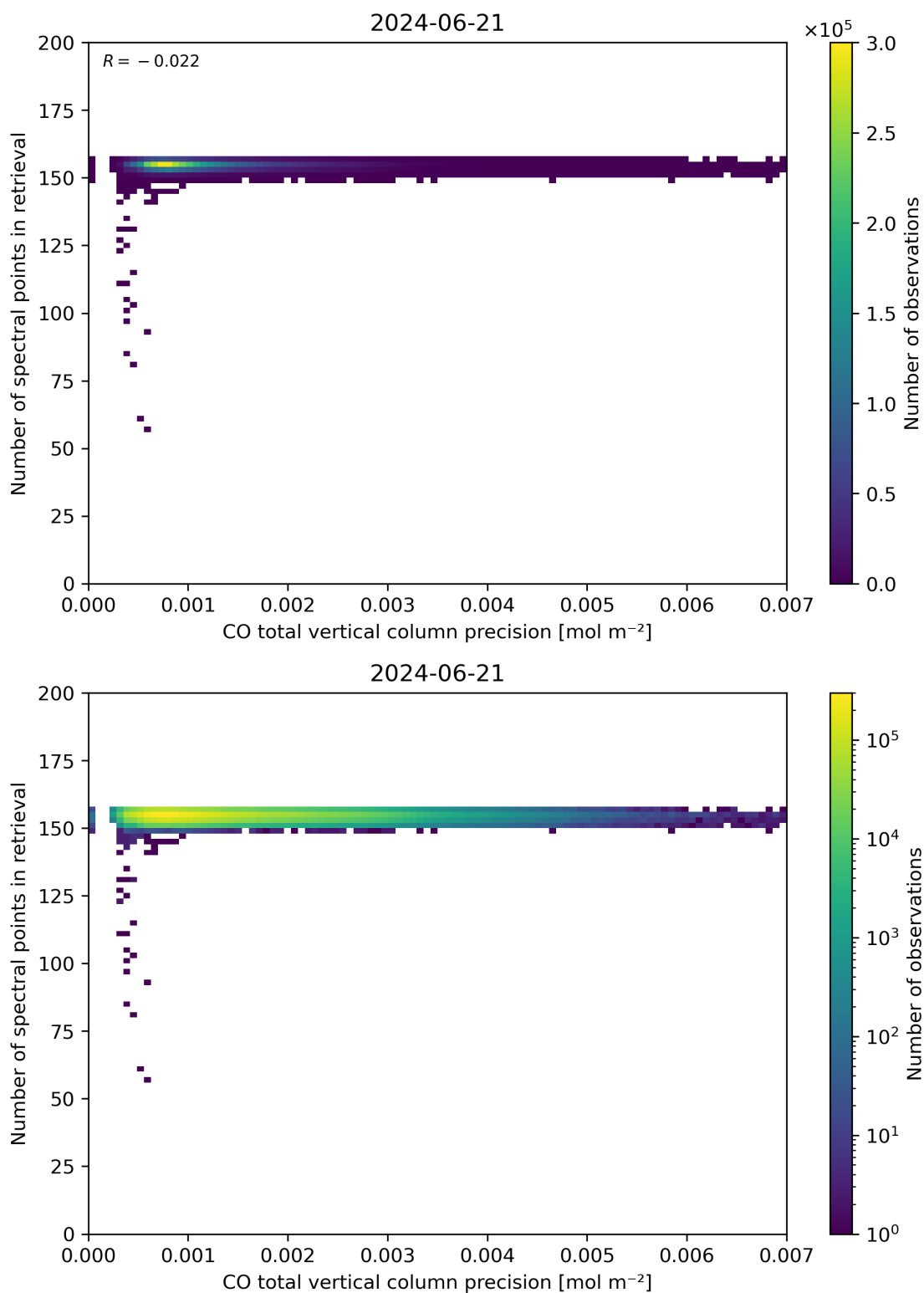
Figure 47: Scatter density plot of “CO total vertical column precision” against “Number of spectral points in retrieval” for 2024-06-20 to 2024-06-22.
