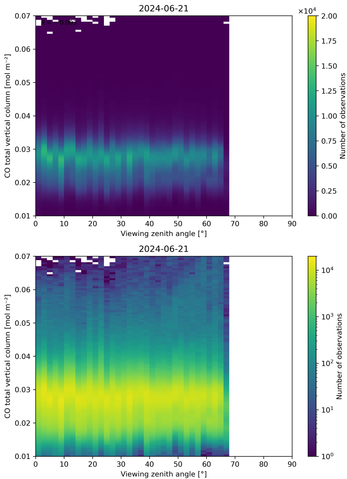
Figure 69: Scatter density plot of “Viewing zenith angle” against “CO total vertical column” for 2024-06-20 to 2024-06-22.
