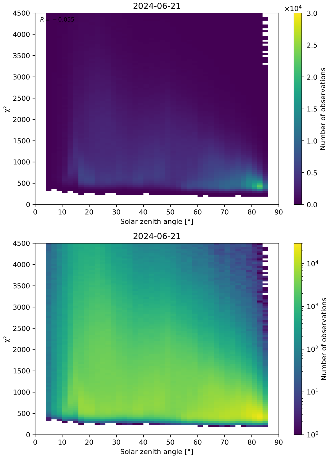
Figure 64: Scatter density plot of “Solar zenith angle” against “ \chi^2 ” for 2024-06-20 to 2024-06-22.
