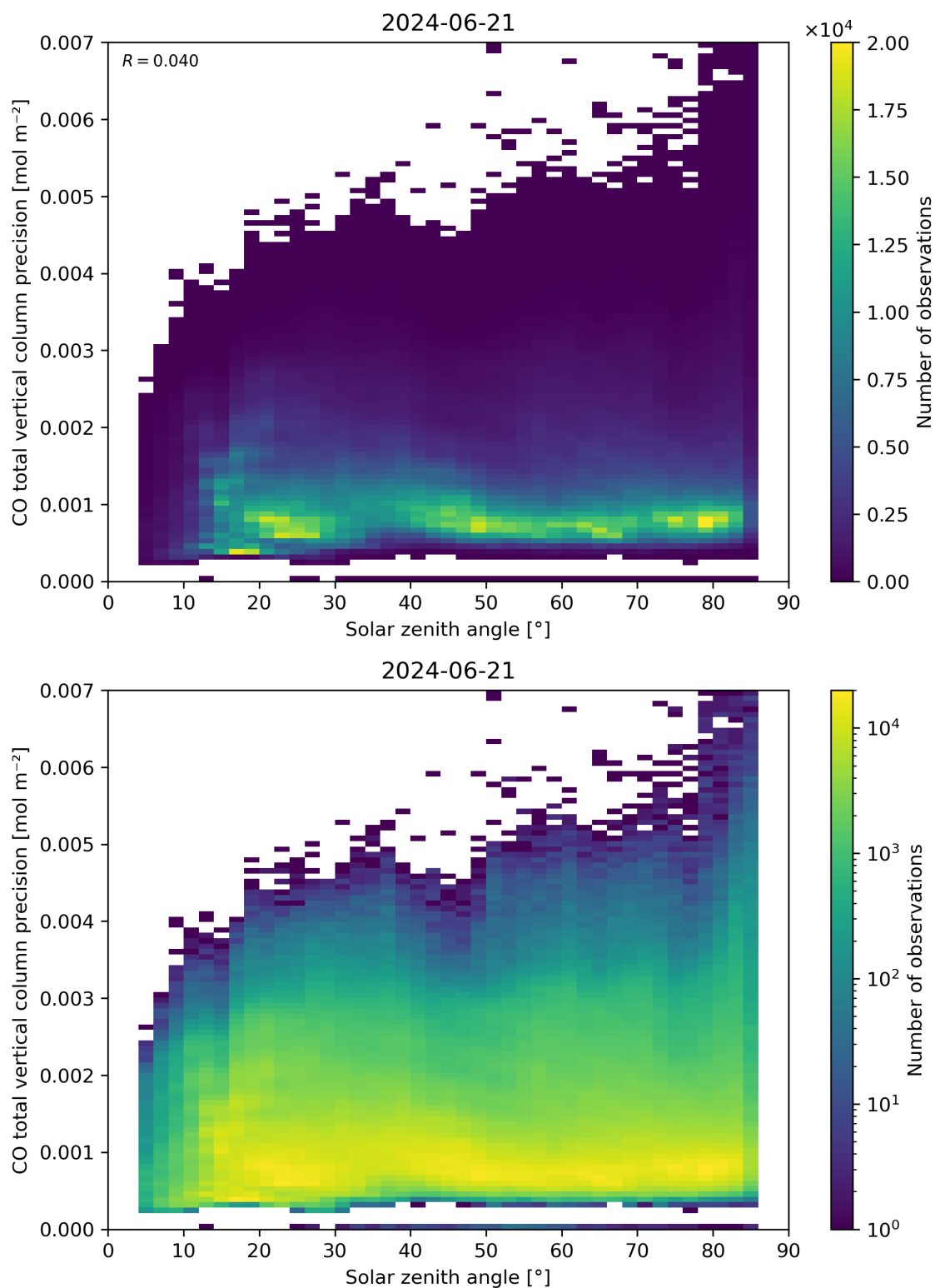
Figure 63: Scatter density plot of “Solar zenith angle” against “CO total vertical column precision” for 2024-06-20 to 2024-06-22.
