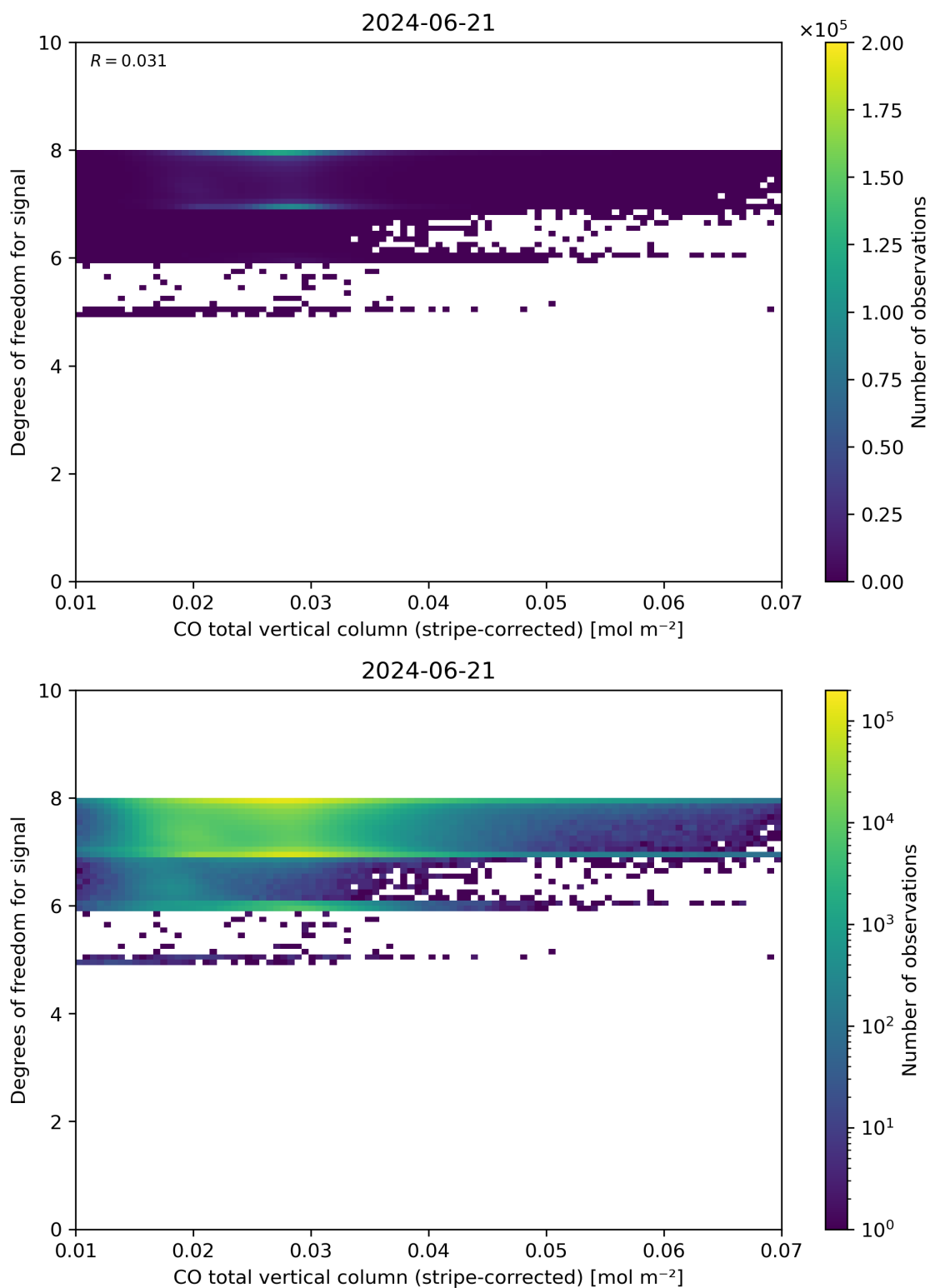
Figure 38: Scatter density plot of “CO total vertical column (stripe-corrected)” against “Degrees of freedom for signal” for 2024-06-20 to 2024-06-22.
