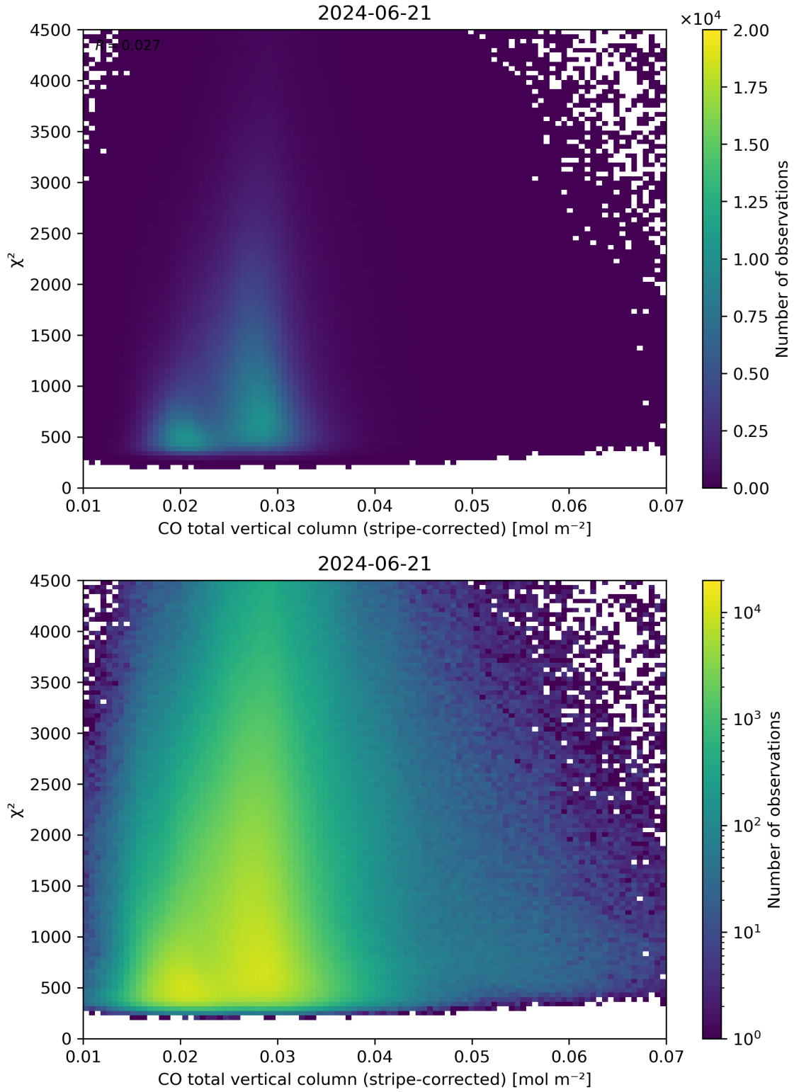
Figure 37: Scatter density plot of “CO total vertical column (stripe-corrected)” against “ \chi^2 ” for 2024-06-20 to 2024-06-22.
