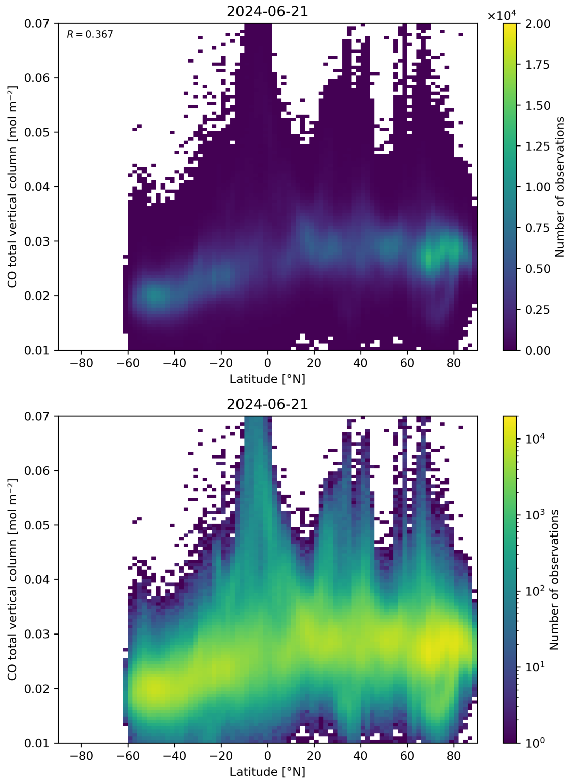
Figure 51: Scatter density plot of “Latitude” against “CO total vertical column” for 2024-06-20 to 2024-06-22.
