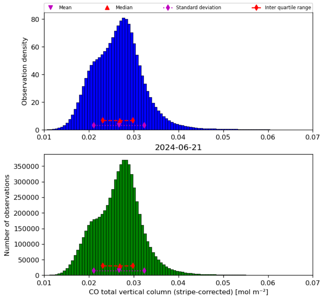
Figure 19: Histogram of “CO total vertical column (stripe-corrected)” for 2024-06-20 to 2024-06-22
