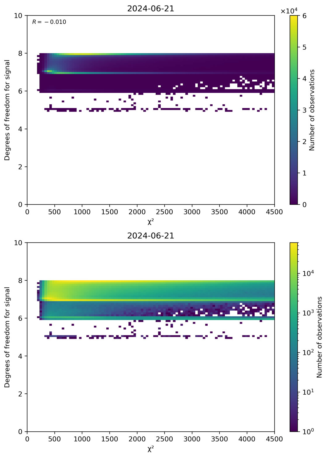
Figure 48: Scatter density plot of “ \chi^2 ” against “Degrees of freedom for signal” for 2024-06-20 to 2024-06-22.
