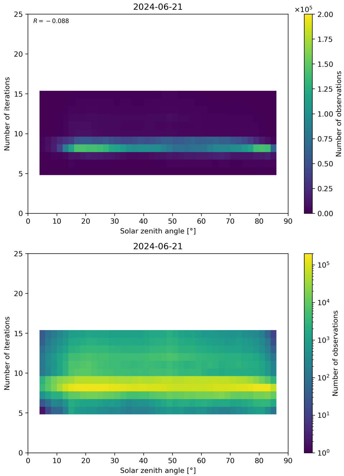
Figure 67: Scatter density plot of “Solar zenith angle” against “Number of iterations” for 2024-06-20 to 2024-06-22.
