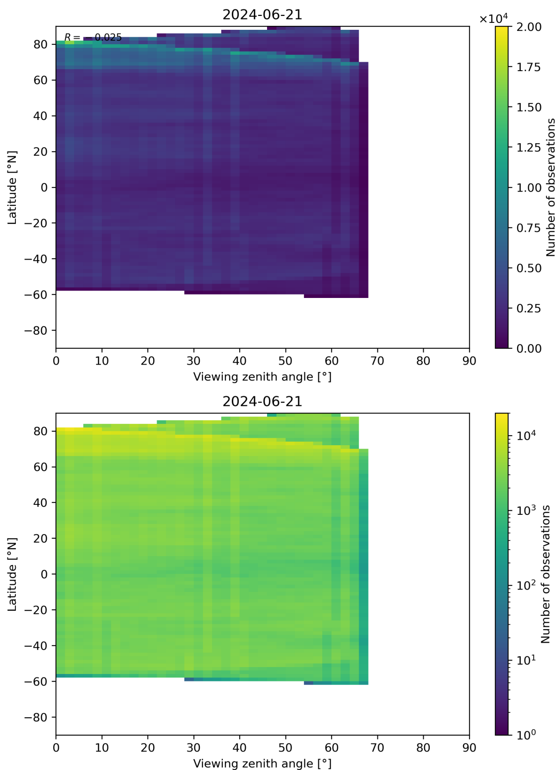
Figure 74: Scatter density plot of “Viewing zenith angle” against “Latitude” for 2024-06-20 to 2024-06-22.
