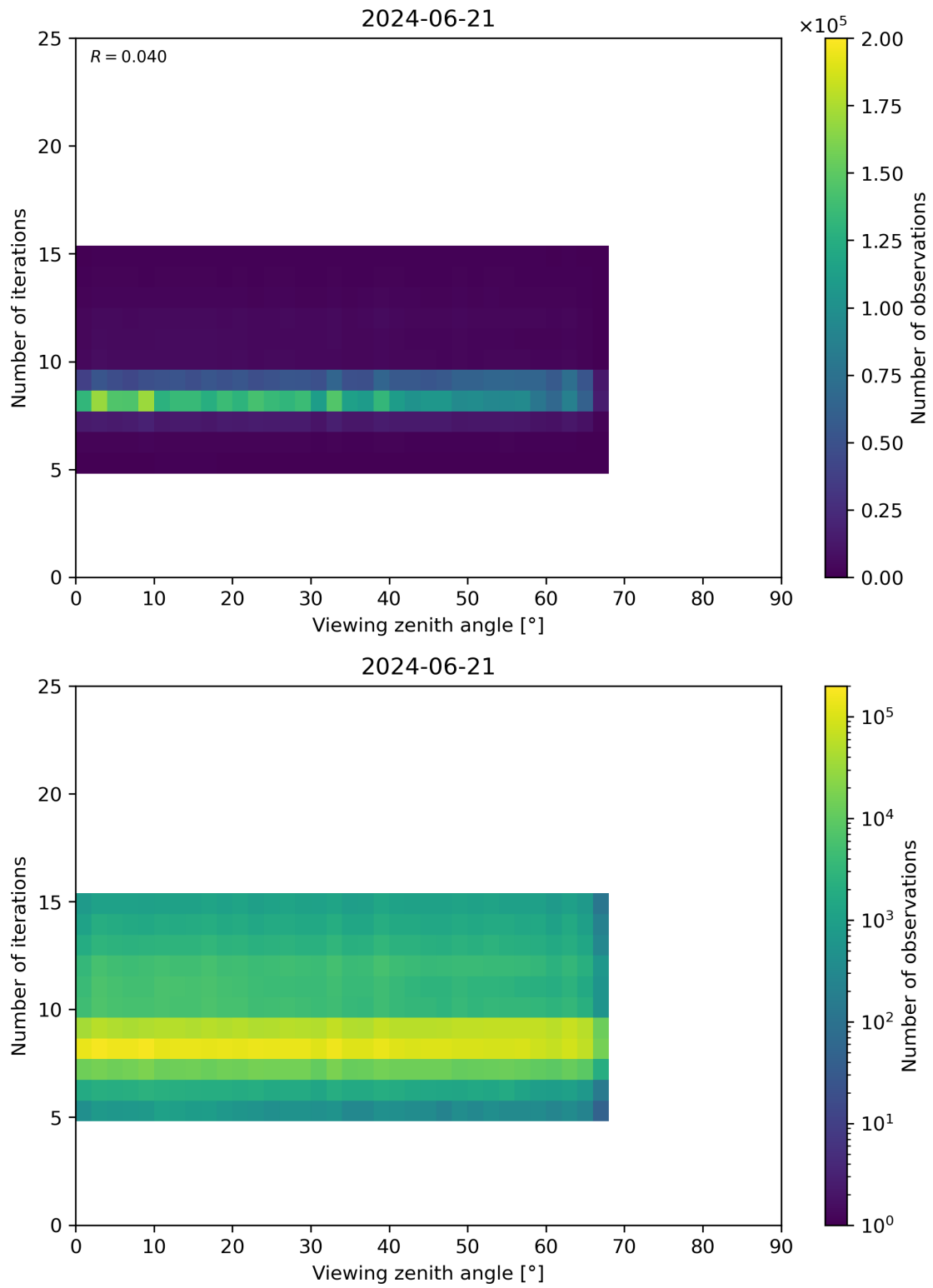
Figure 75: Scatter density plot of “Viewing zenith angle” against “Number of iterations” for 2024-06-20 to 2024-06-22.
