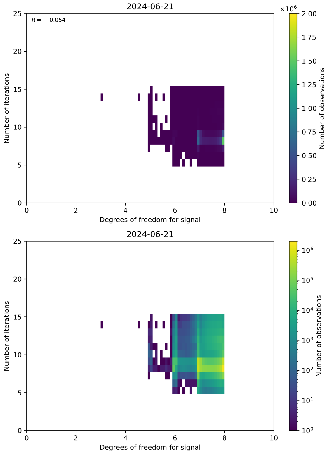
Figure 50: Scatter density plot of “Degrees of freedom for signal” against “Number of iterations” for 2024-06-20 to 2024-06-22.
