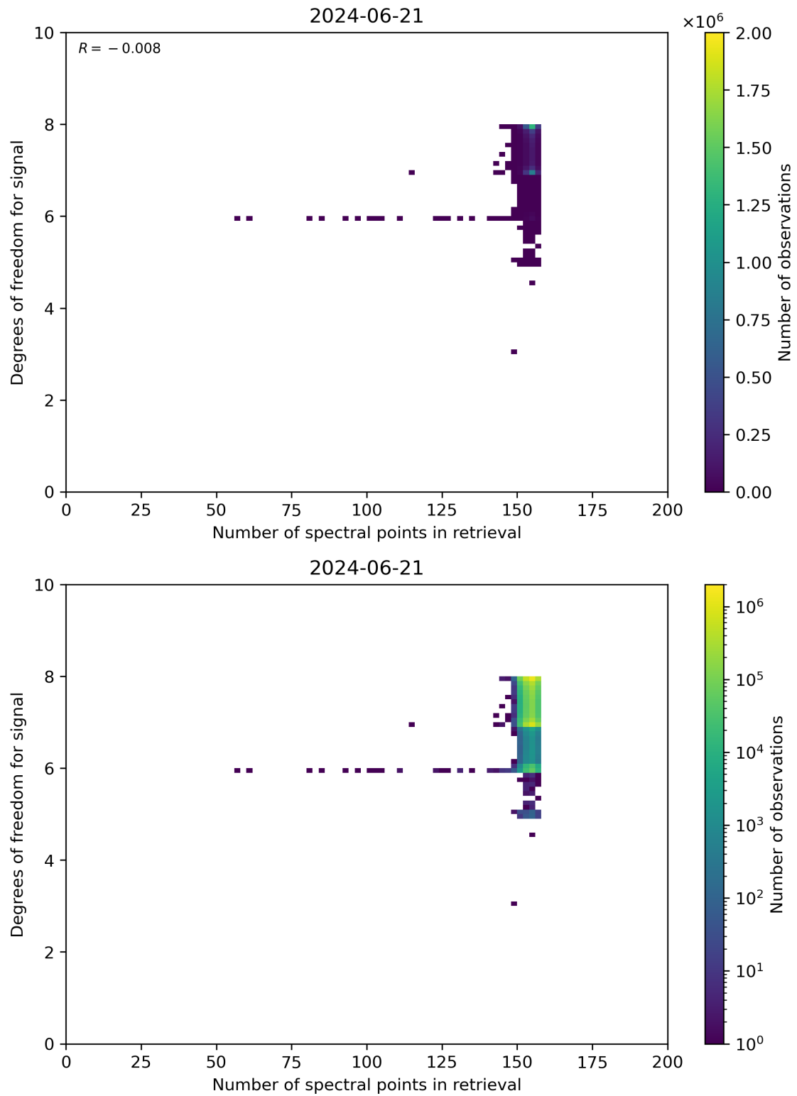
Figure 59: Scatter density plot of “Number of spectral points in retrieval” against “Degrees of freedom for signal” for 2024-06-20 to 2024-06-22.
