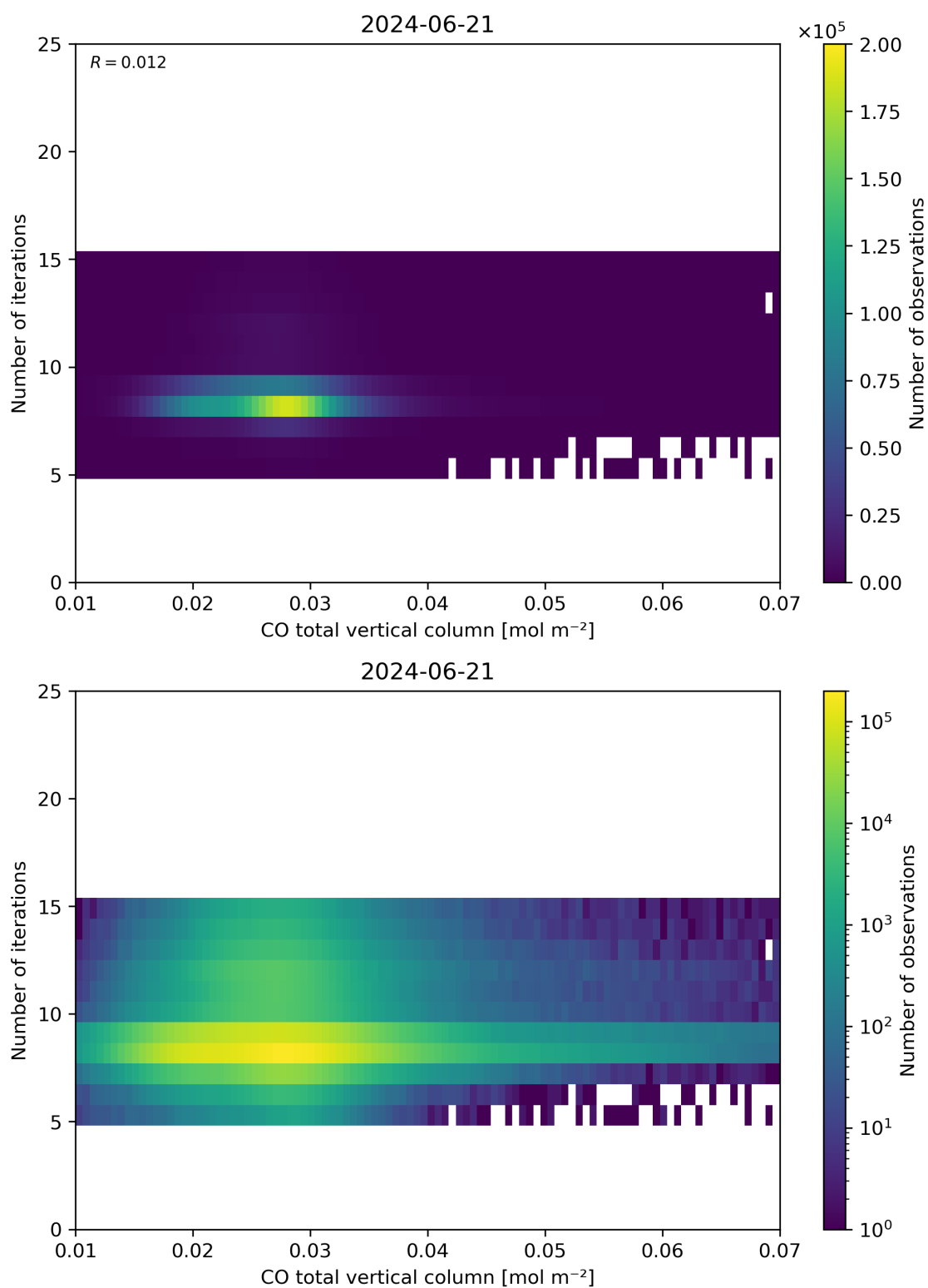
Figure 42: Scatter density plot of “CO total vertical column” against “Number of iterations” for 2024-06-20 to 2024-06-22.
