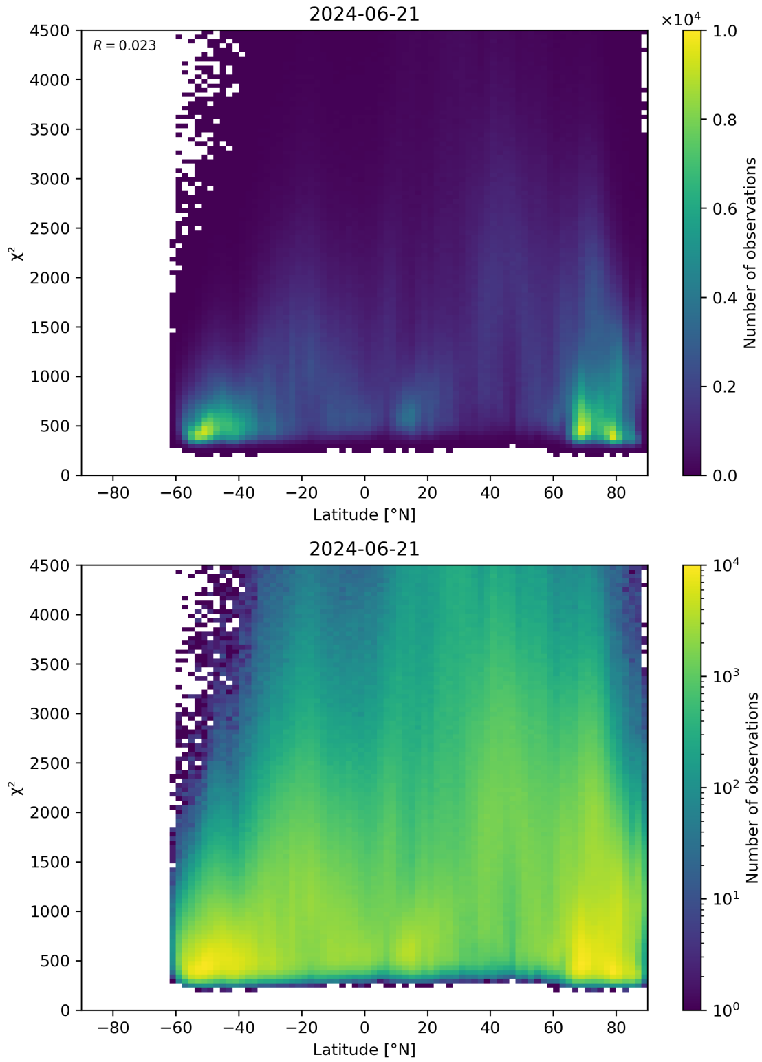
Figure 54: Scatter density plot of “Latitude” against “ \chi^2 ” for 2024-06-20 to 2024-06-22.
