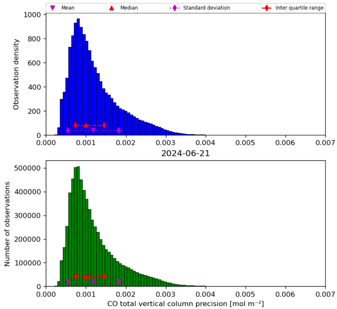
Figure 20: Histogram of “CO total vertical column precision” for 2024-06-20 to 2024-06-22
