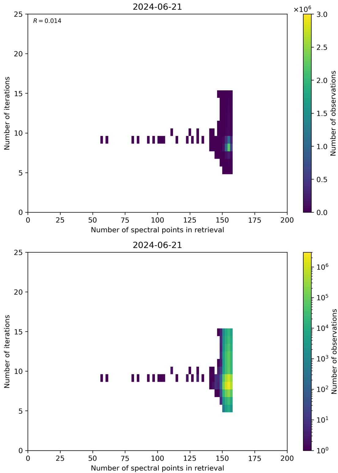
Figure 60: Scatter density plot of “Number of spectral points in retrieval” against “Number of iterations” for 2024-06-20 to 2024-06-22.
