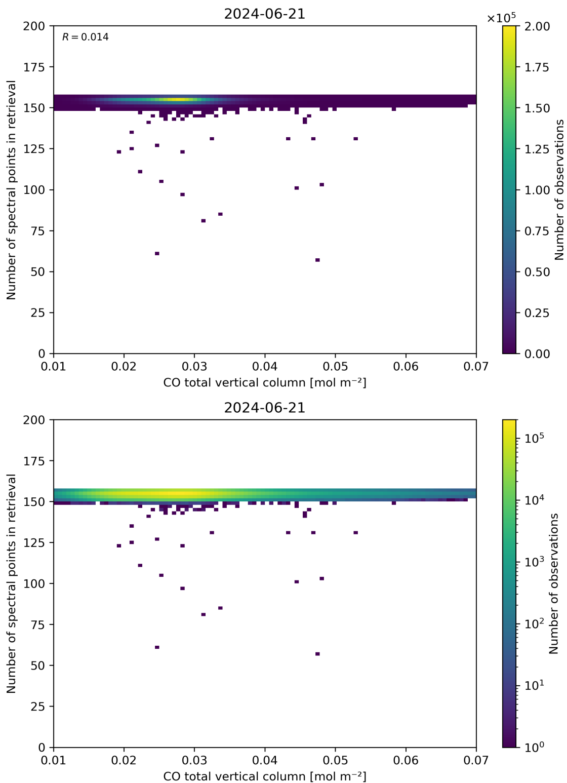
Figure 43: Scatter density plot of “CO total vertical column” against “Number of spectral points in retrieval” for 2024-06-20 to 2024-06-22.
