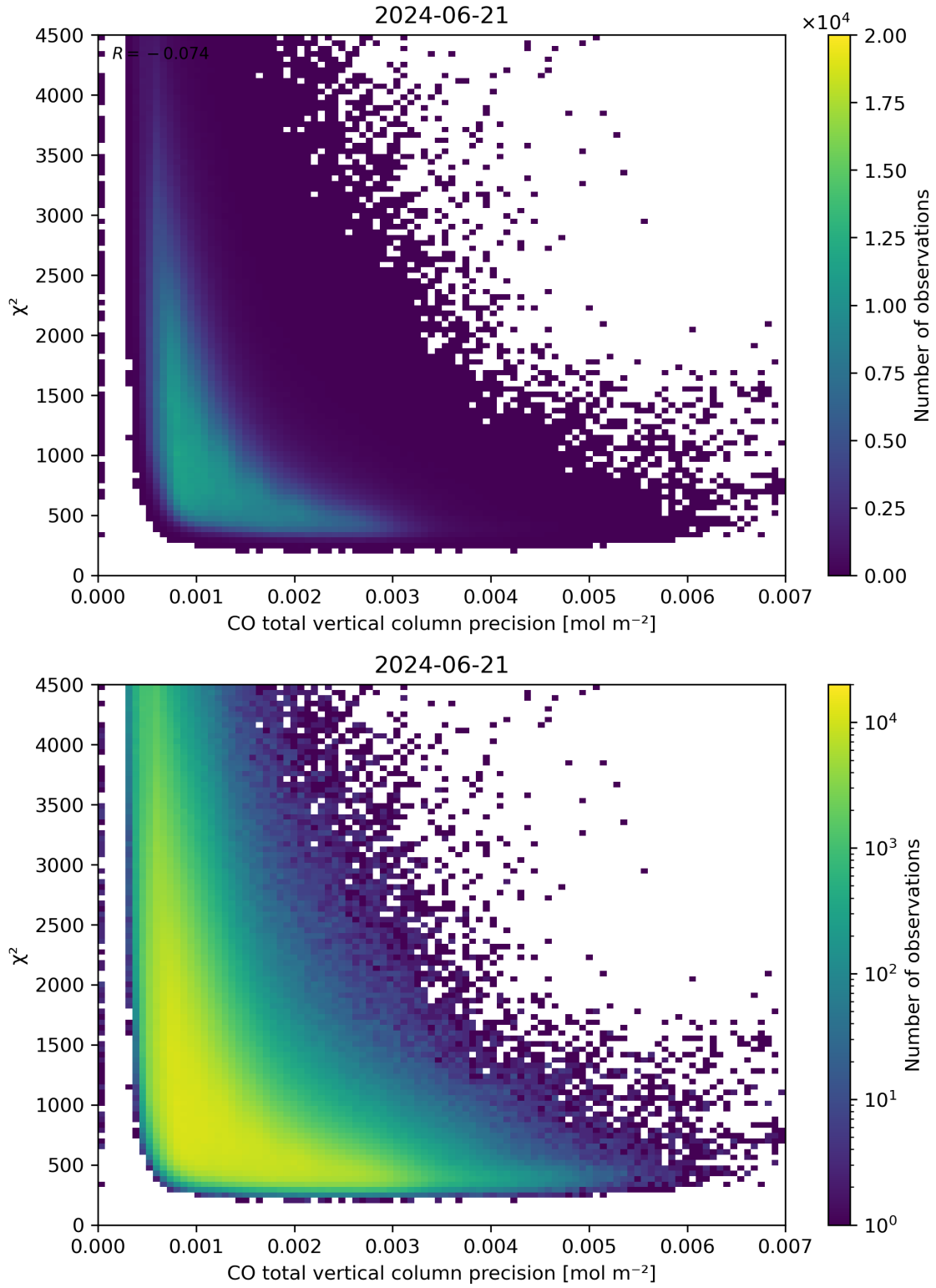
Figure 44: Scatter density plot of “CO total vertical column precision” against “ \chi^2 ” for 2024-06-20 to 2024-06-22.
