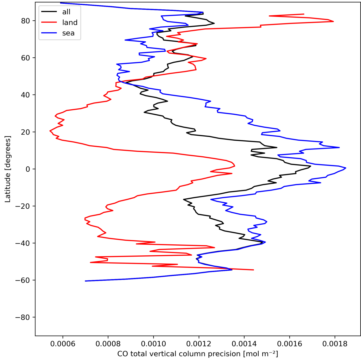
Figure 12: Zonal average of “CO total vertical column precision” for 2024-06-20 to 2024-06-22.
