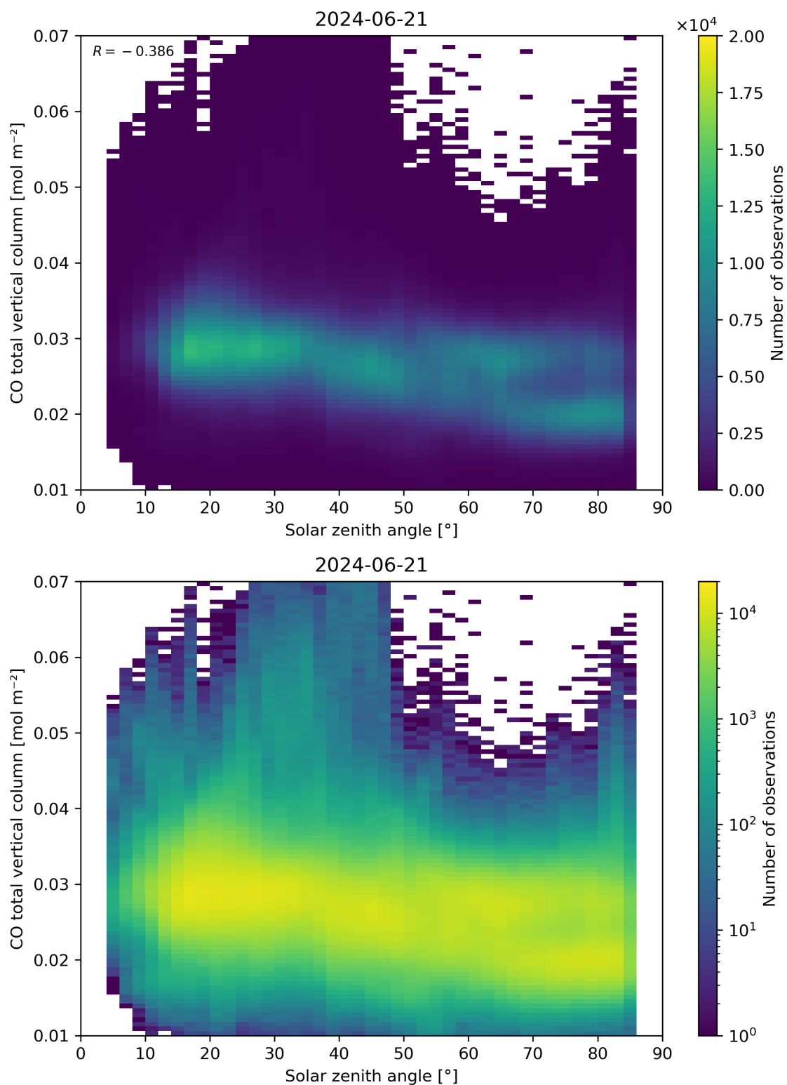
Figure 61: Scatter density plot of “Solar zenith angle” against “CO total vertical column” for 2024-06-20 to 2024-06-22.
