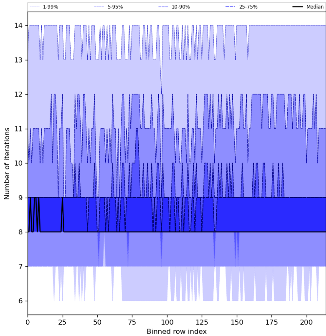
Figure 32: Along track statistics of “Number of iterations” for 2024-06-20 to 2024-06-22
