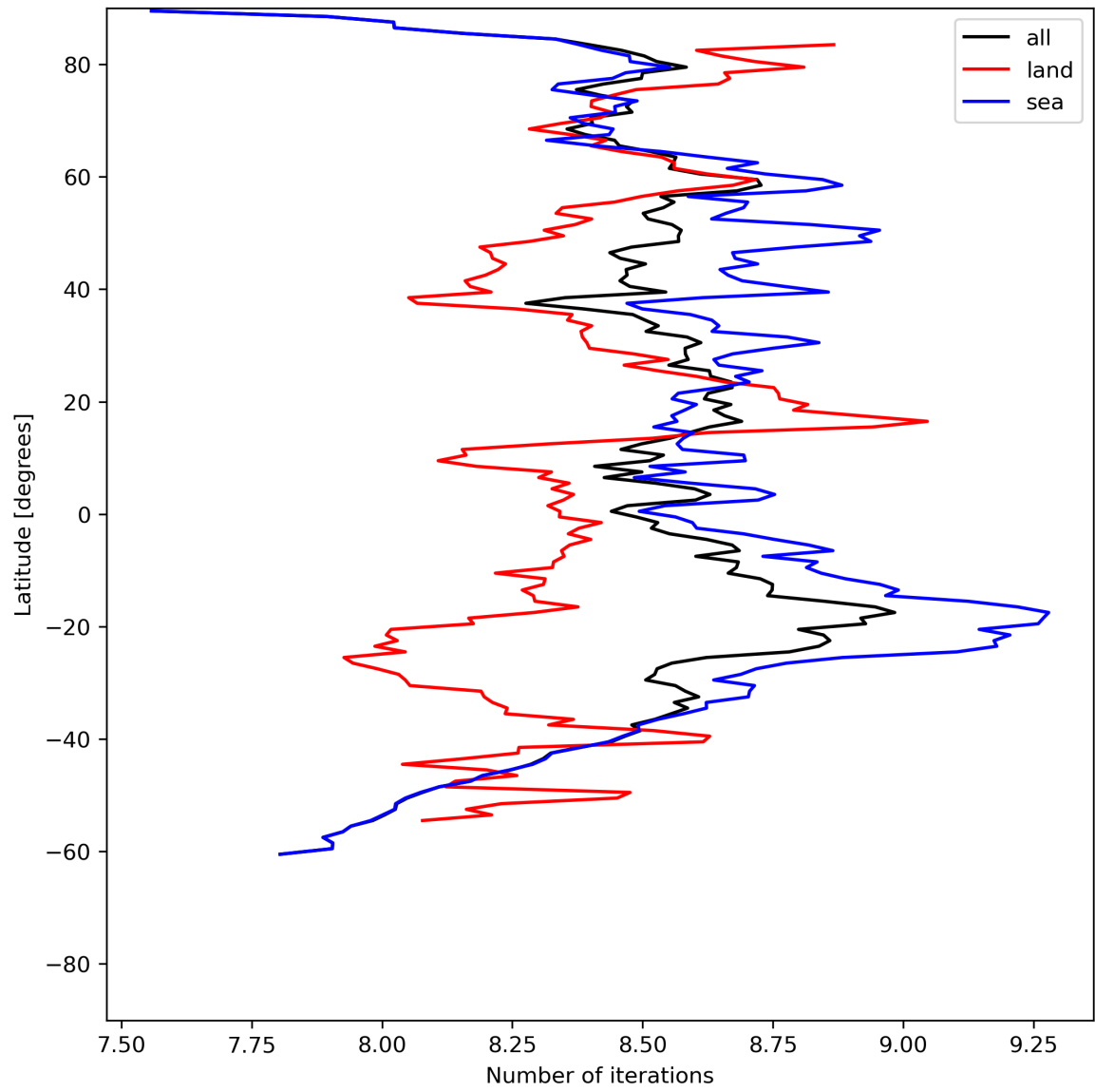
Figure 16: Zonal average of “Number of iterations” for 2024-06-20 to 2024-06-22.
