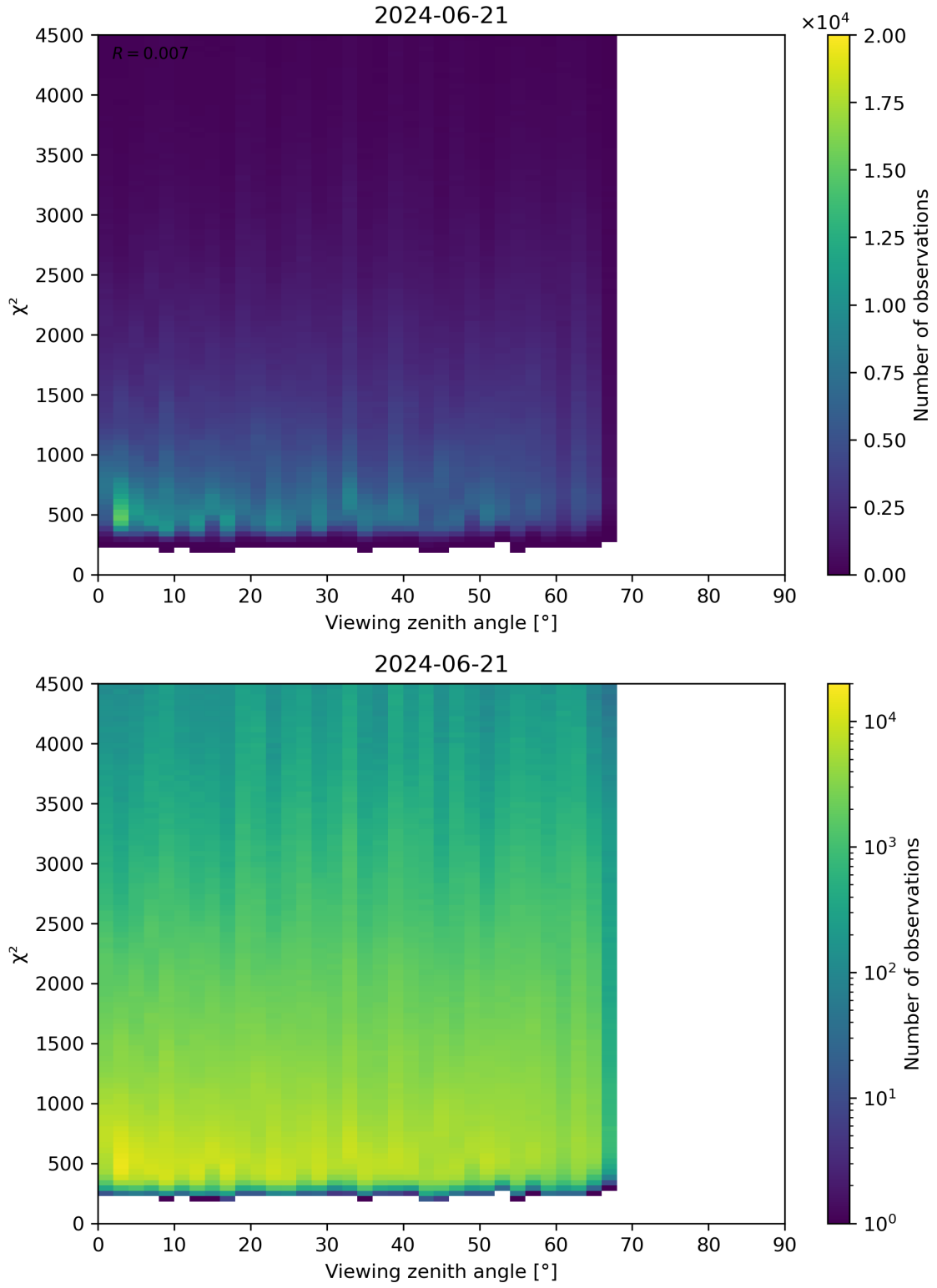
Figure 72: Scatter density plot of “Viewing zenith angle” against “ \chi^2 ” for 2024-06-20 to 2024-06-22.
