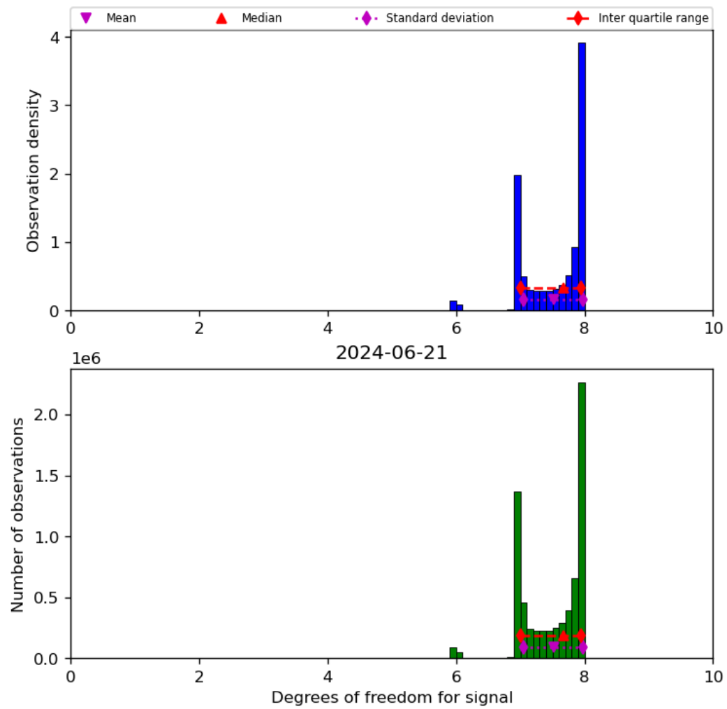
Figure 23: Histogram of “Degrees of freedom for signal” for 2024-06-20 to 2024-06-22
