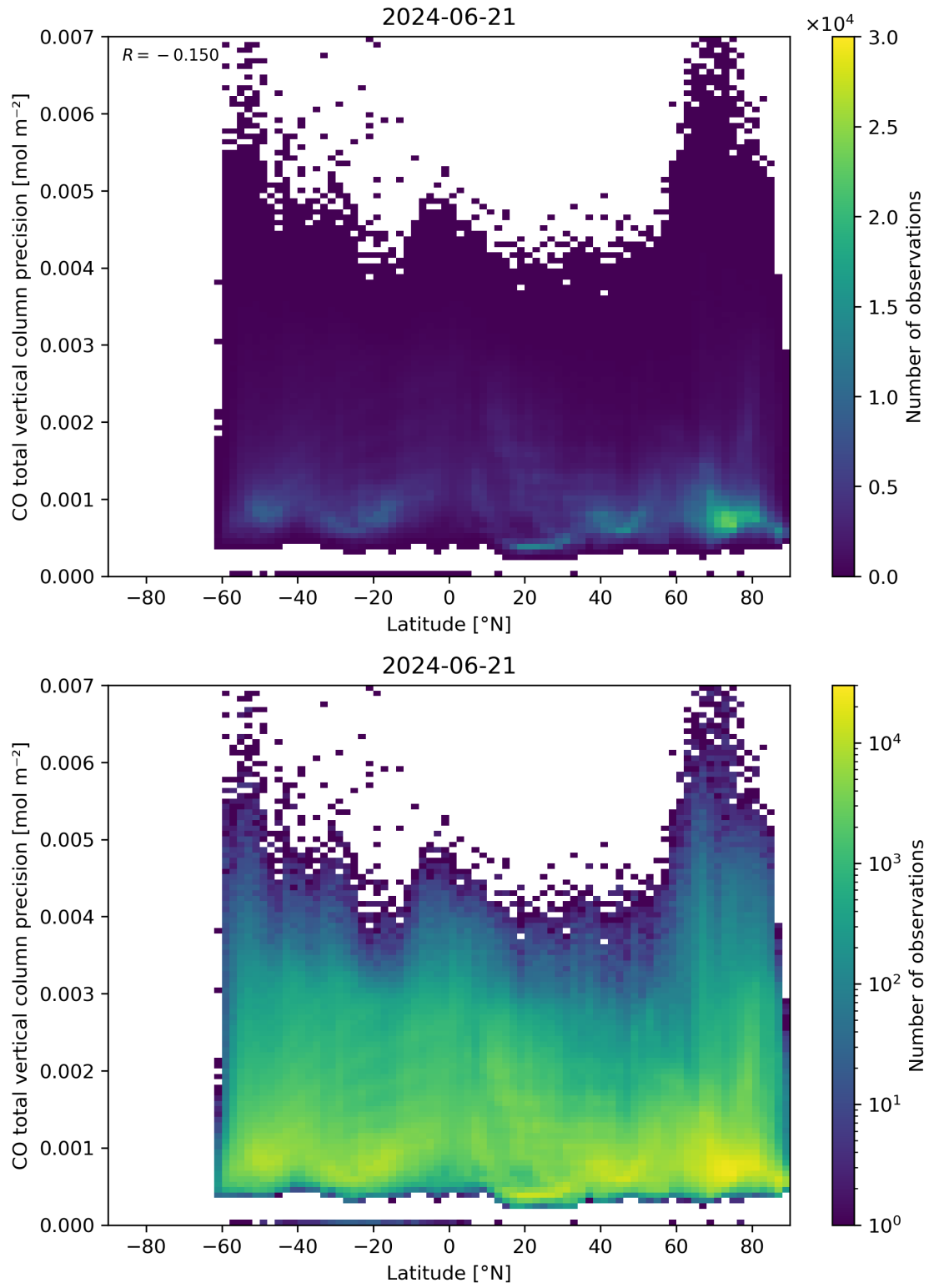
Figure 53: Scatter density plot of “Latitude” against “CO total vertical column precision” for 2024-06-20 to 2024-06-22.
