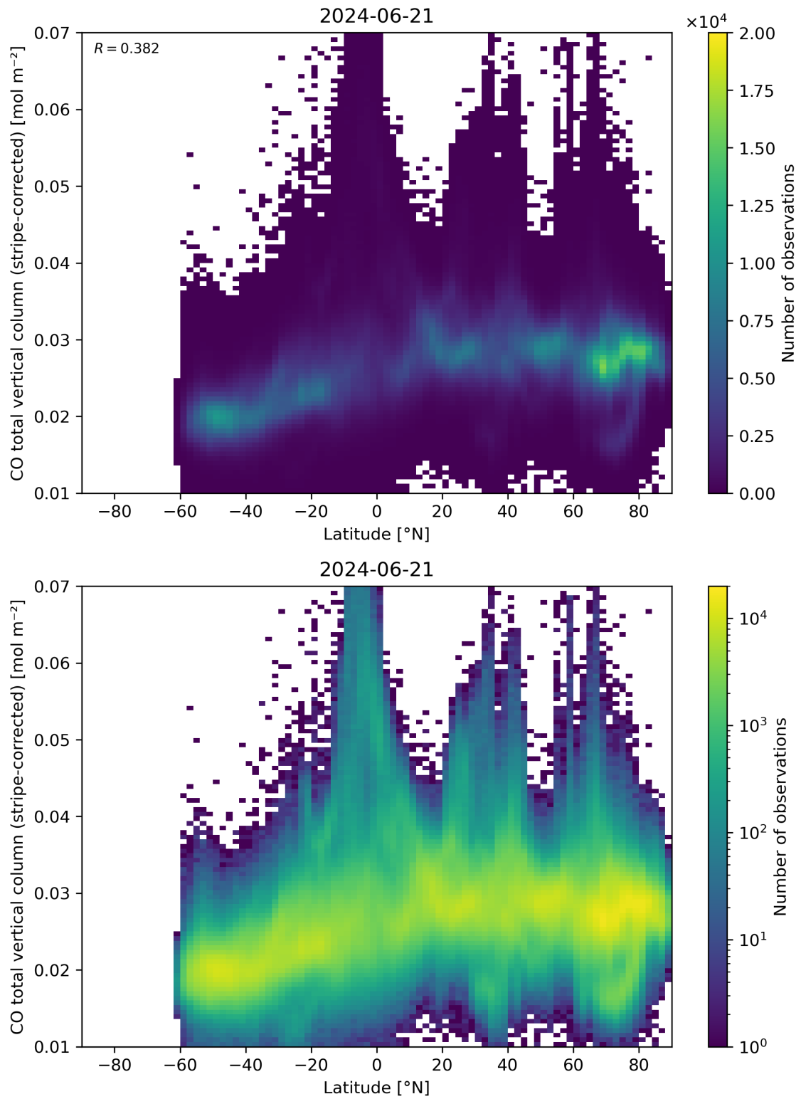
Figure 52: Scatter density plot of “Latitude” against “CO total vertical column (stripe-corrected)” for 2024-06-20 to 2024-06-22.
