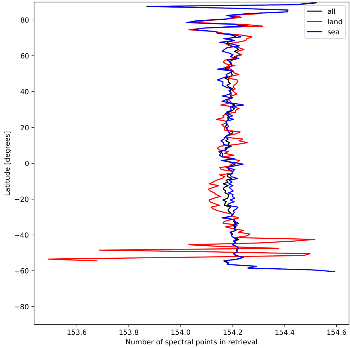
Figure 13: Zonal average of “Number of spectral points in retrieval” for 2024-06-20 to 2024-06-22.
