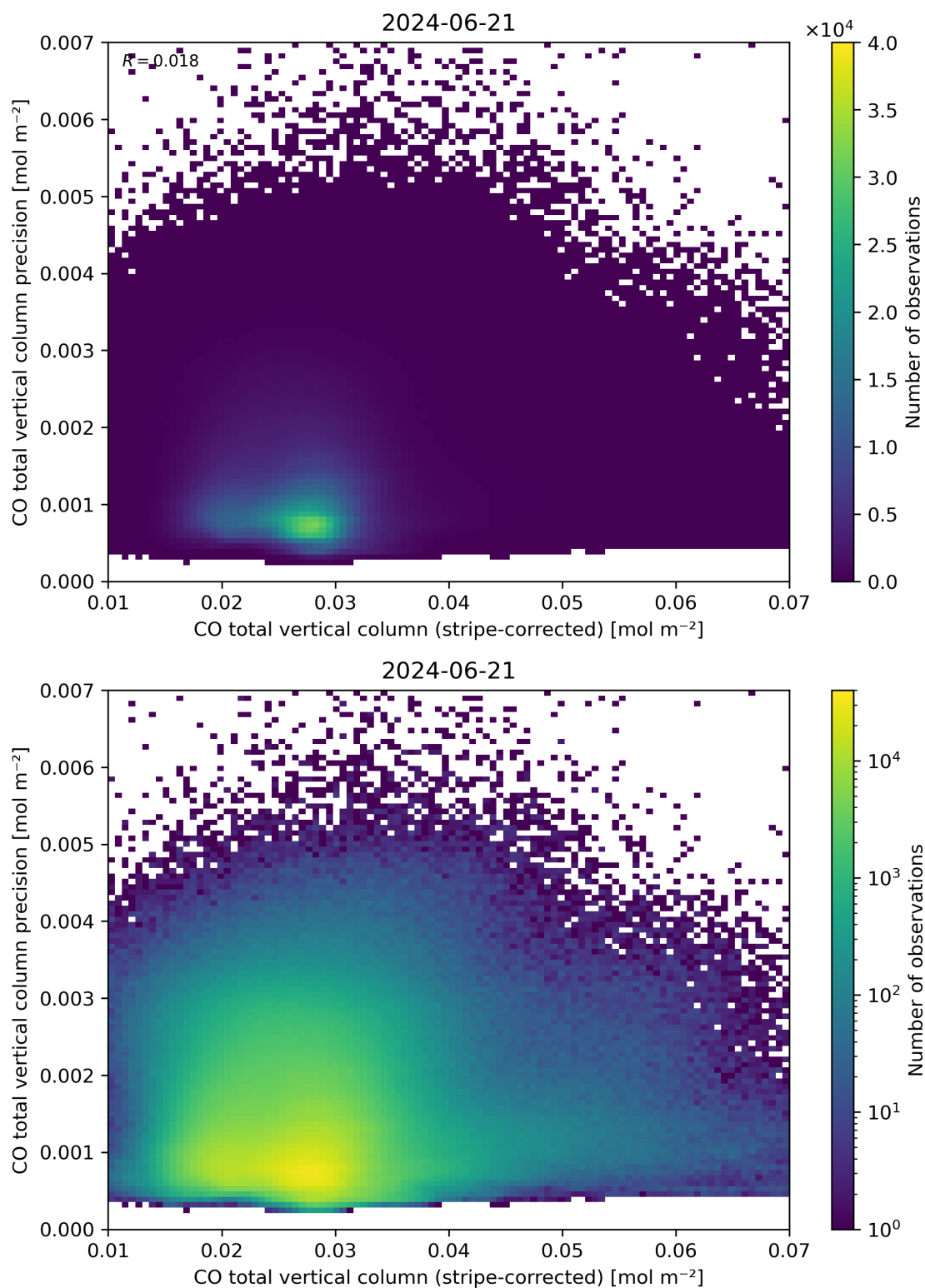
Figure 36: Scatter density plot of “CO total vertical column (stripe-corrected)” against “CO total vertical column precision” for 2024-06-20 to 2024-06-22.
