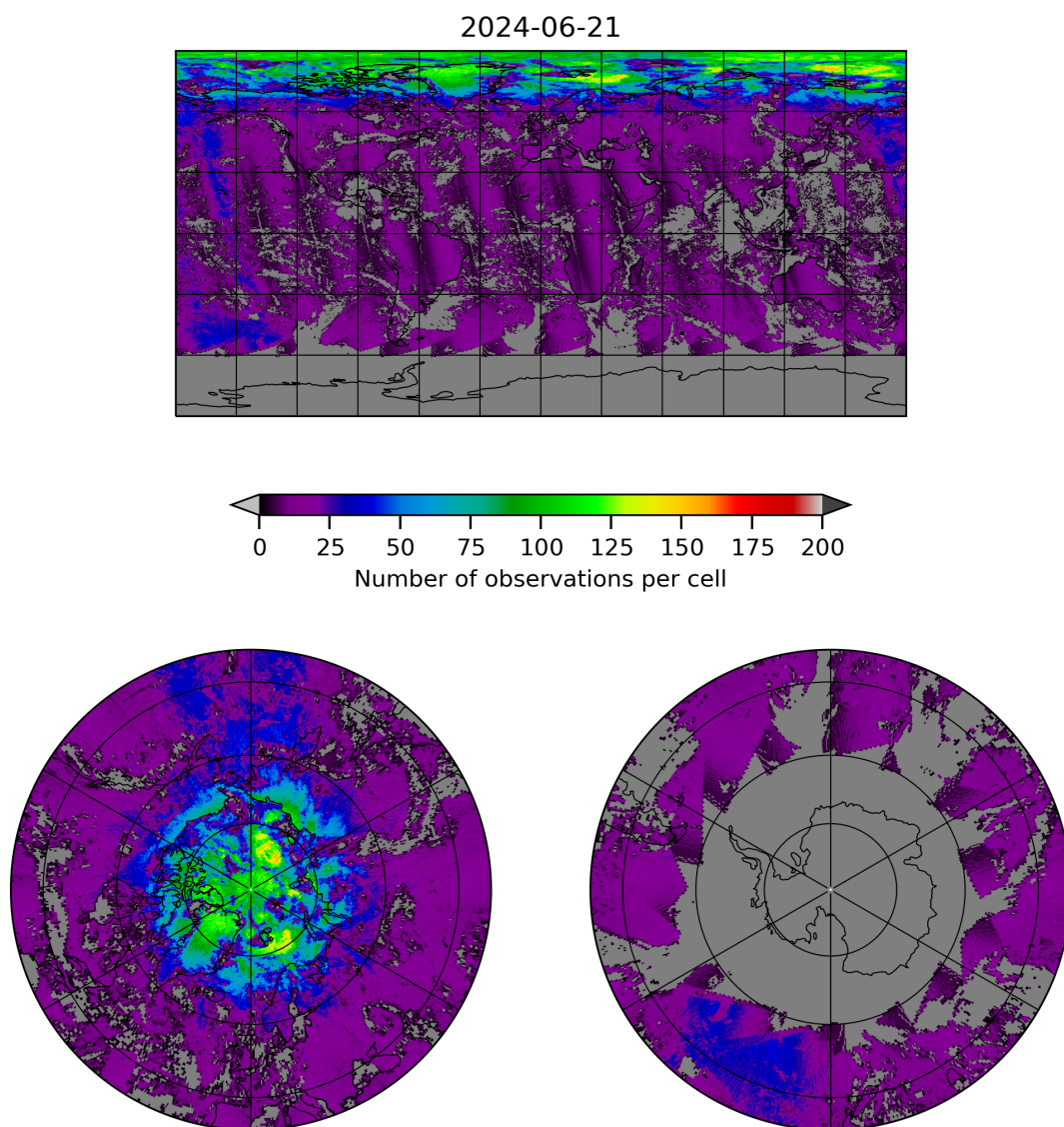
Figure 8: Map of the number of observations for 2024-06-20 to 2024-06-22
