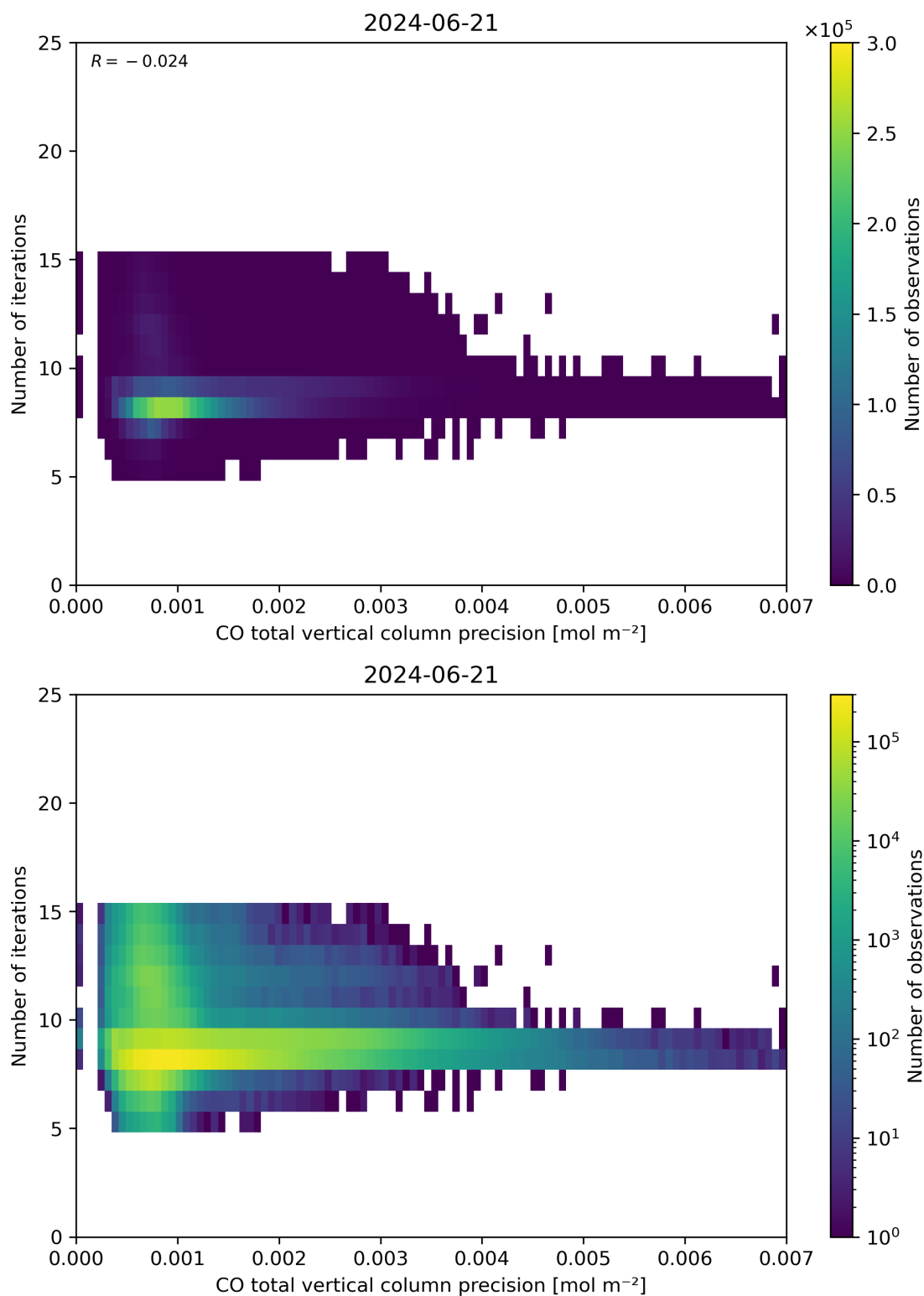
Figure 46: Scatter density plot of “CO total vertical column precision” against “Number of iterations” for 2024-06-20 to 2024-06-22.
