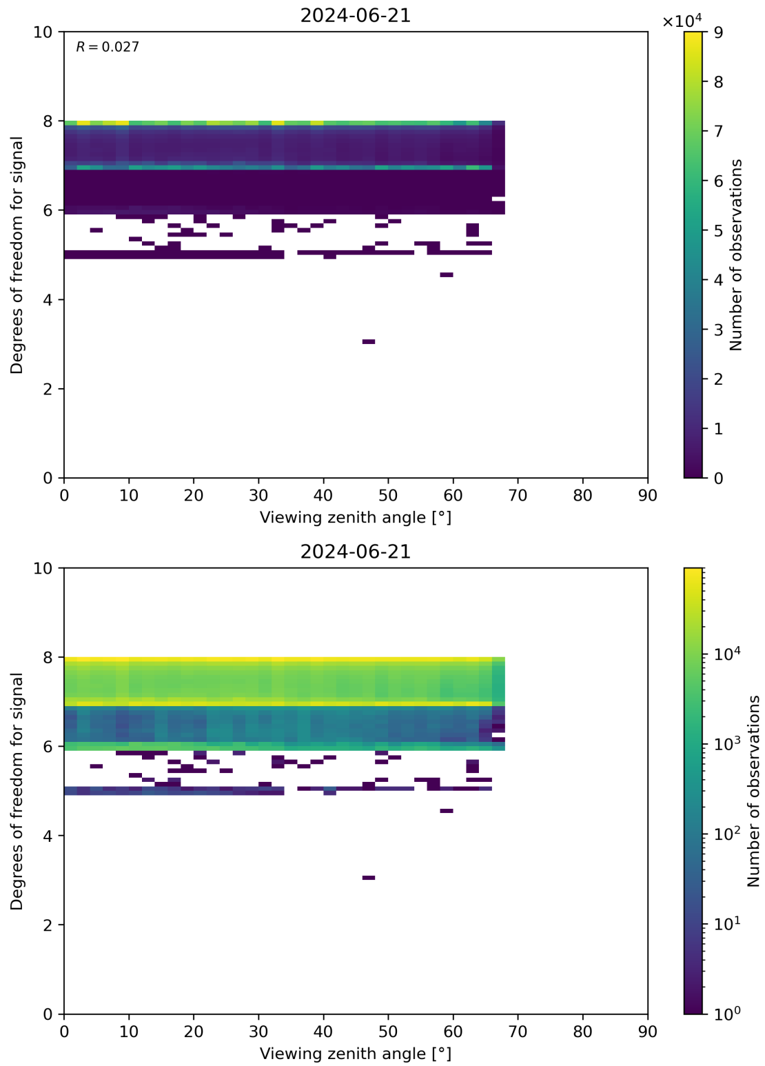
Figure 73: Scatter density plot of “Viewing zenith angle” against “Degrees of freedom for signal” for 2024-06-20 to 2024-06-22.
