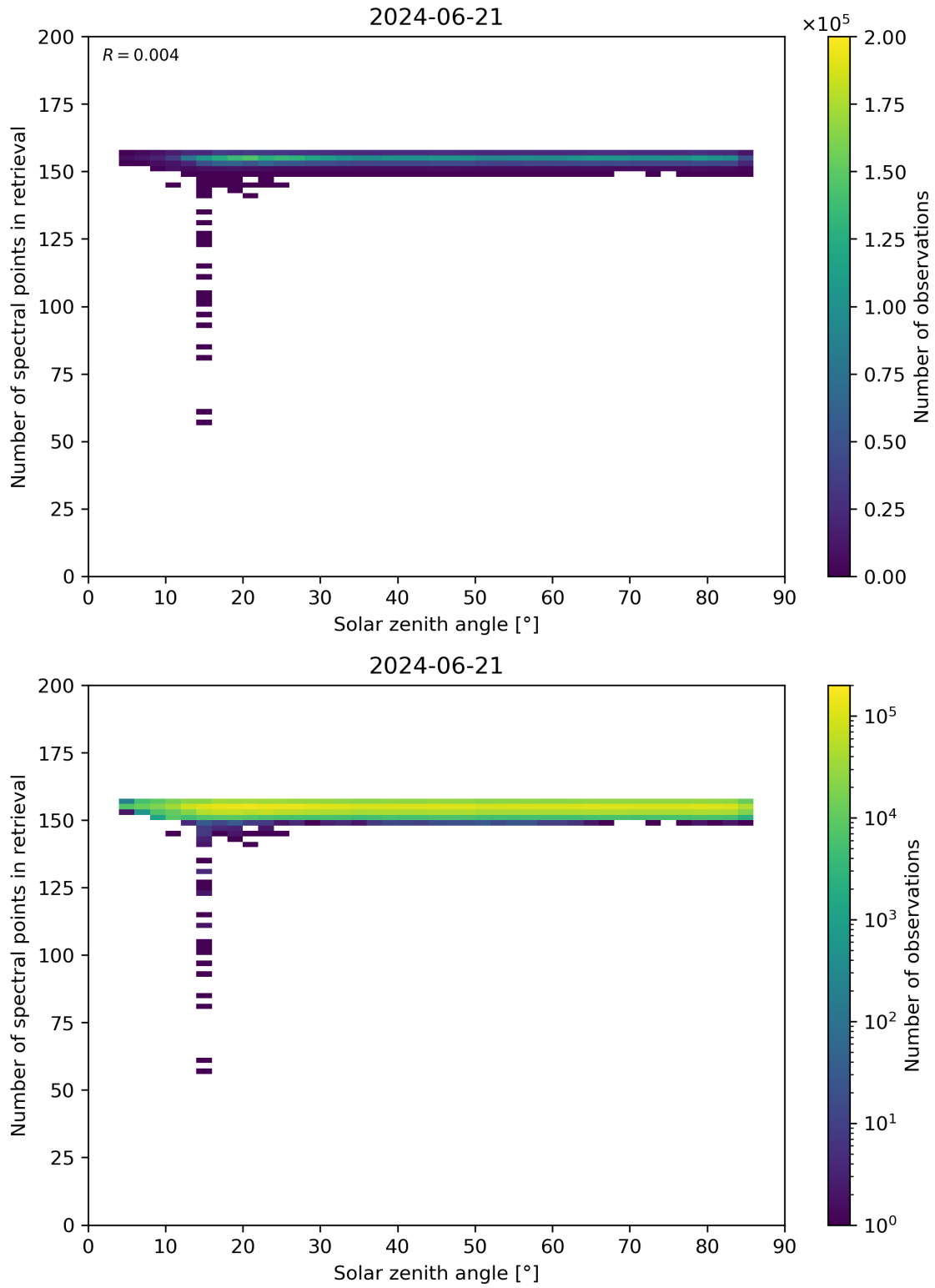
Figure 68: Scatter density plot of “Solar zenith angle” against “Number of spectral points in retrieval” for 2024-06-20 to 2024-06-22.
