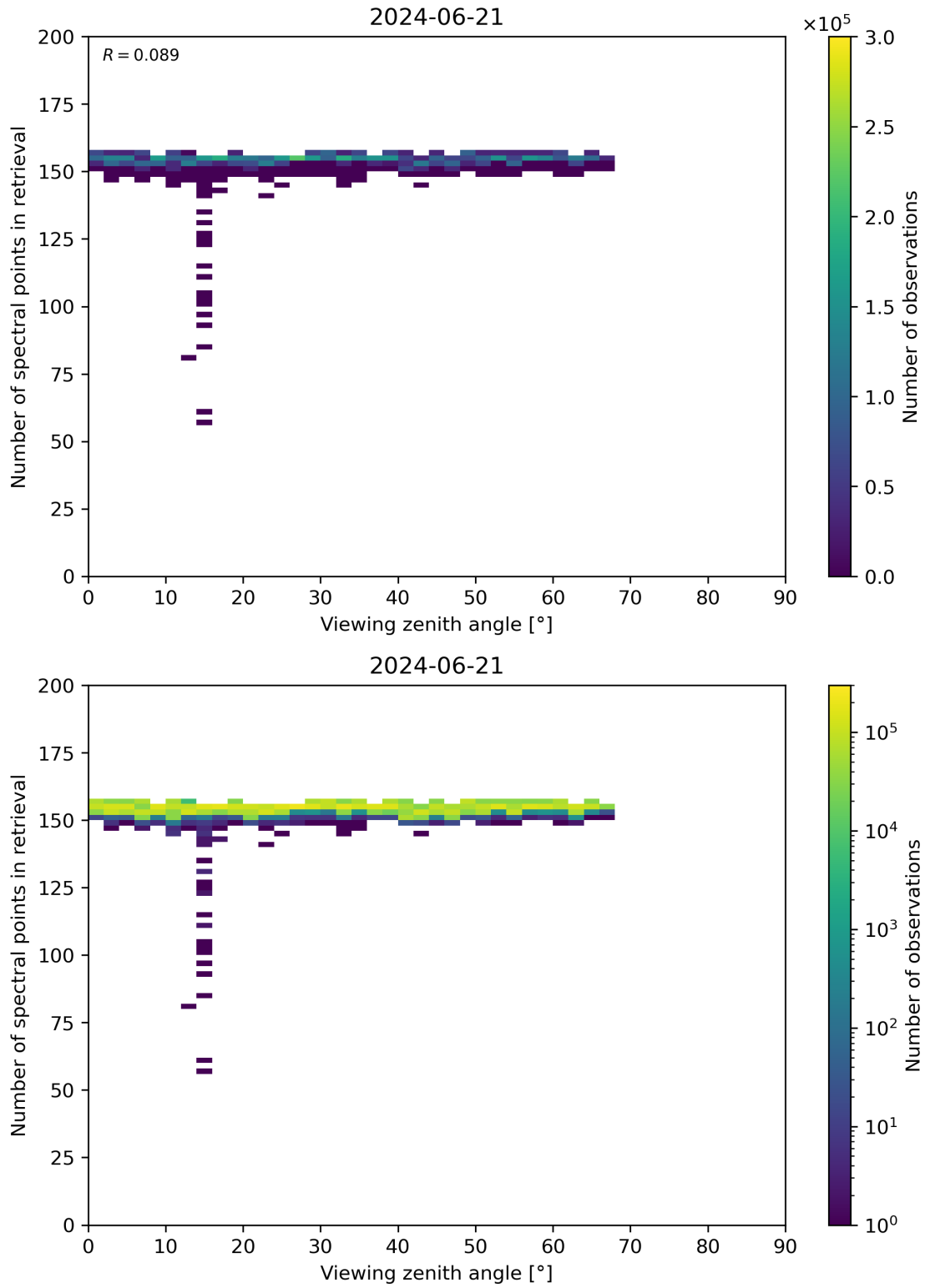
Figure 76: Scatter density plot of “Viewing zenith angle” against “Number of spectral points in retrieval” for 2024-06-20 to 2024-06-22.
