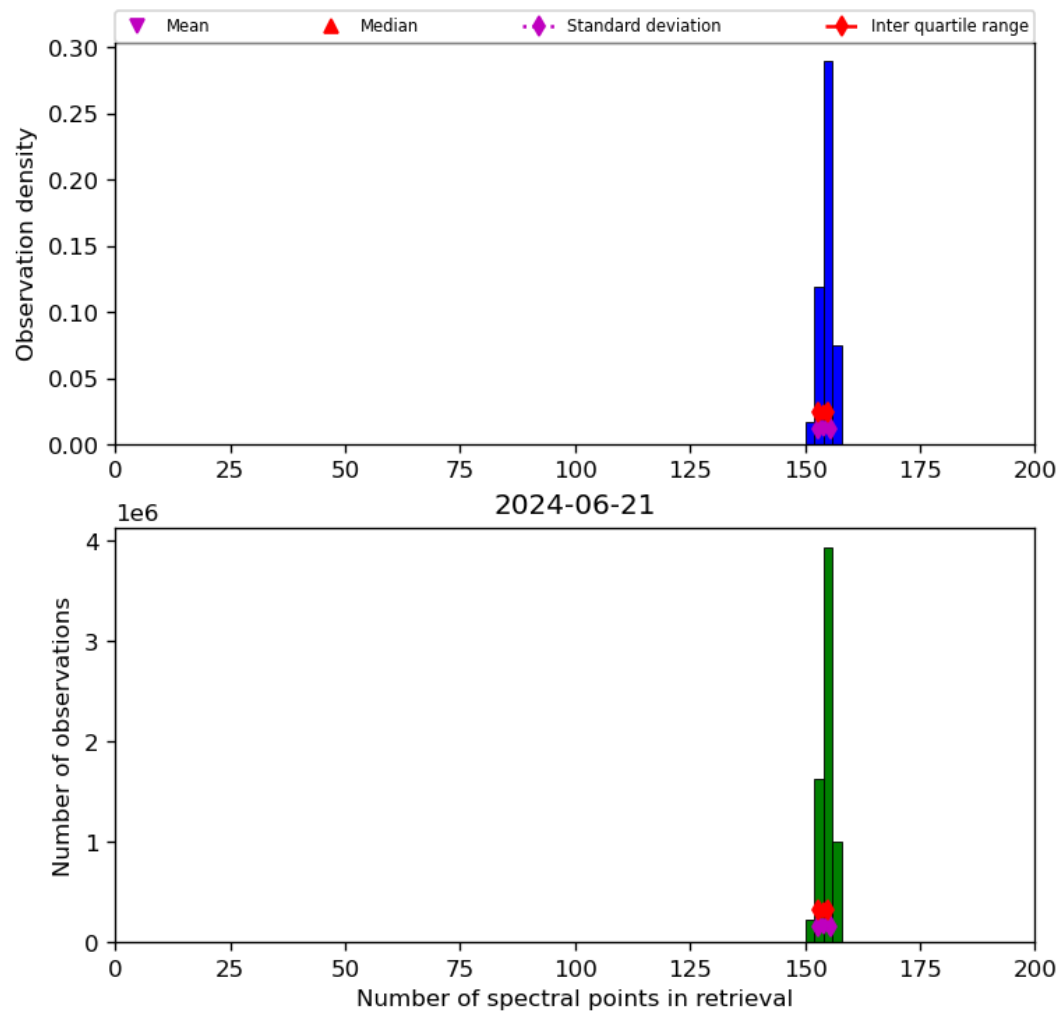
Figure 21: Histogram of “Number of spectral points in retrieval” for 2024-06-20 to 2024-06-22
