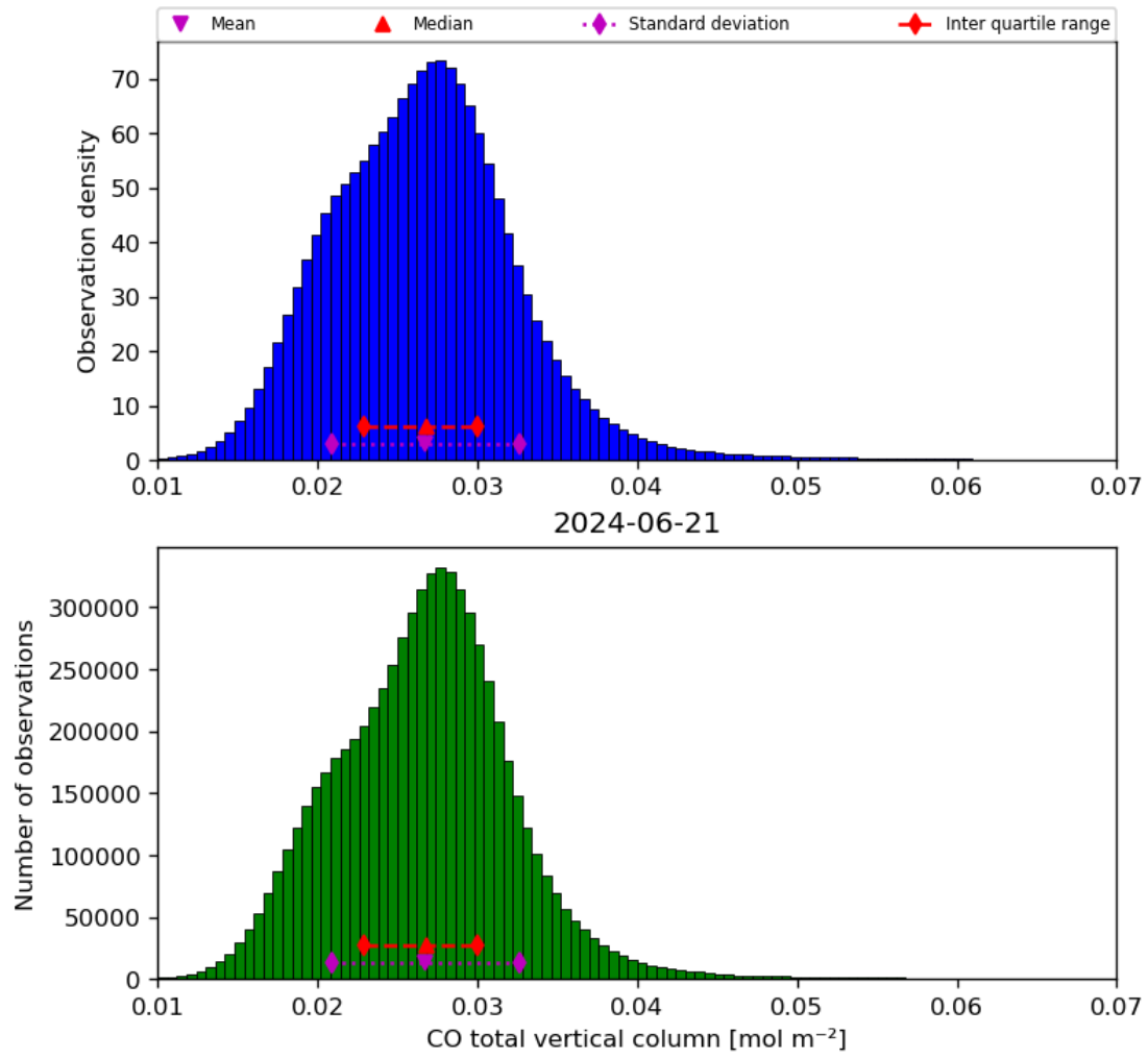
Figure 18: Histogram of “CO total vertical column” for 2024-06-20 to 2024-06-22
