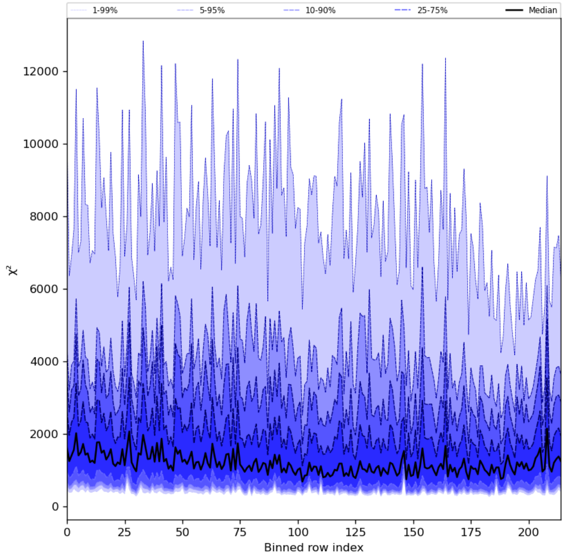
Figure 30: Along track statistics of “ \chi^2 ” for 2024-06-20 to 2024-06-22
