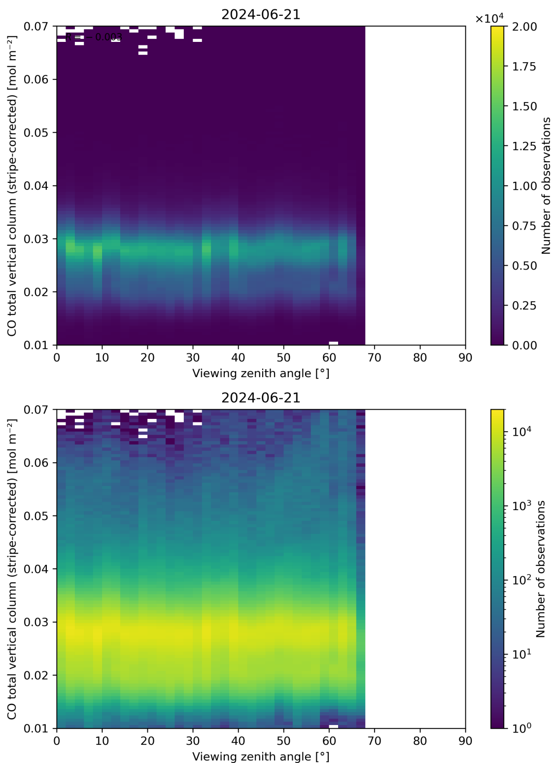
Figure 70: Scatter density plot of “Viewing zenith angle” against “CO total vertical column (stripe-corrected)” for 2024-06-20 to 2024-06-22.
