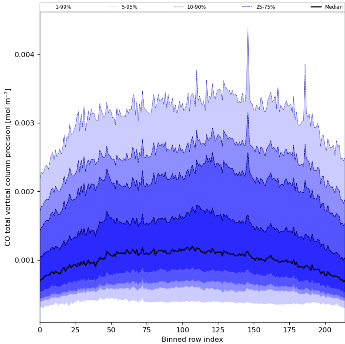
Figure 28: Along track statistics of “CO total vertical column precision” for 2024-06-20 to 2024-06-22
