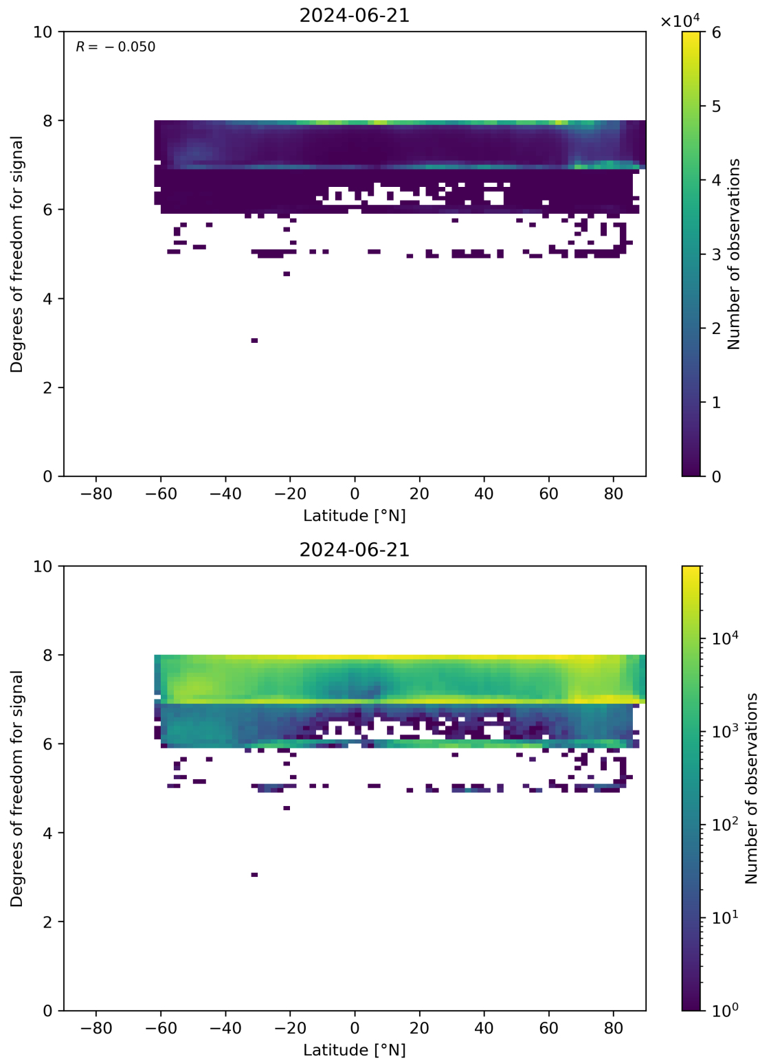
Figure 55: Scatter density plot of “Latitude” against “Degrees of freedom for signal” for 2024-06-20 to 2024-06-22.
