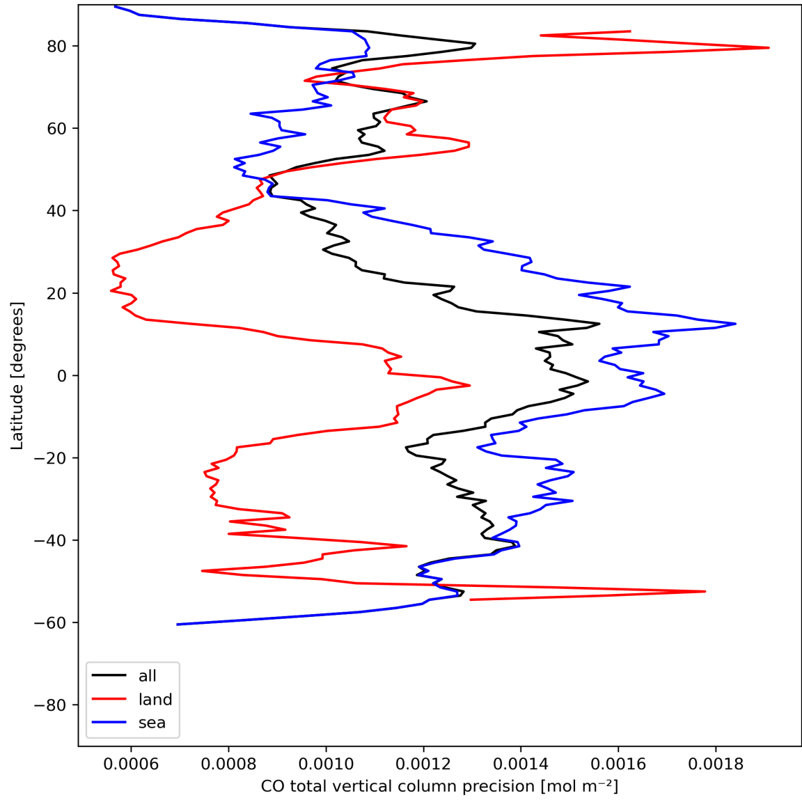
Figure 12: Zonal average of “CO total vertical column precision” for 2024-06-21 to 2024-06-23.
