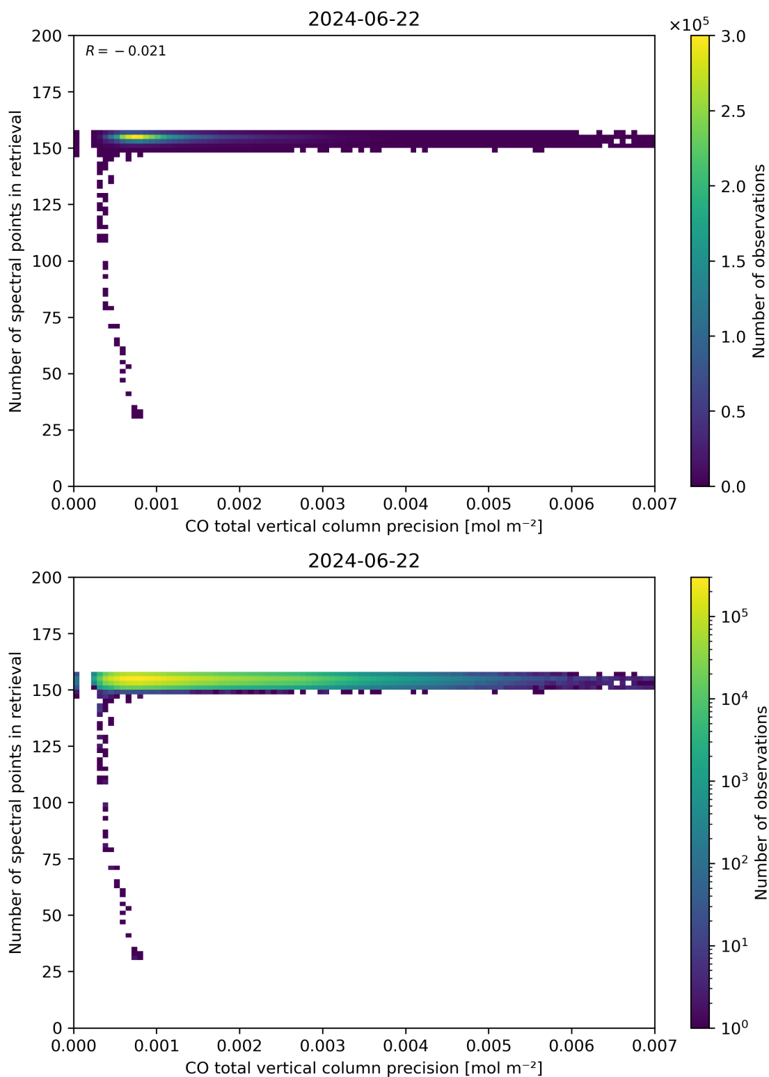
Figure 47: Scatter density plot of “CO total vertical column precision” against “Number of spectral points in retrieval” for 2024-06-21 to 2024-06-23.
