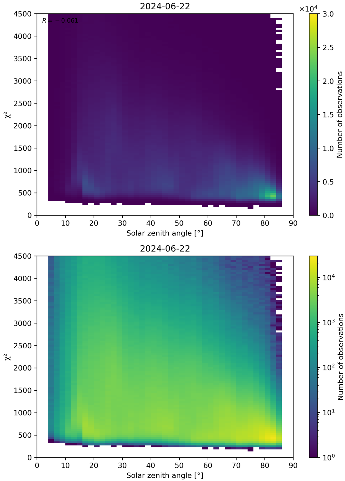
Figure 64: Scatter density plot of “Solar zenith angle” against “ \chi^2 ” for 2024-06-21 to 2024-06-23.
