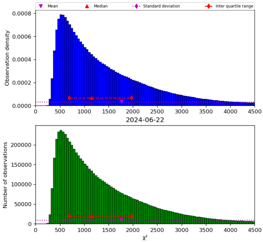
Figure 22: Histogram of “ \chi^2 ” for 2024-06-21 to 2024-06-23
