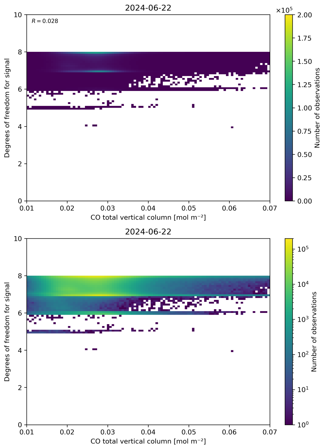
Figure 41: Scatter density plot of “CO total vertical column” against “Degrees of freedom for signal” for 2024-06-21 to 2024-06-23.
