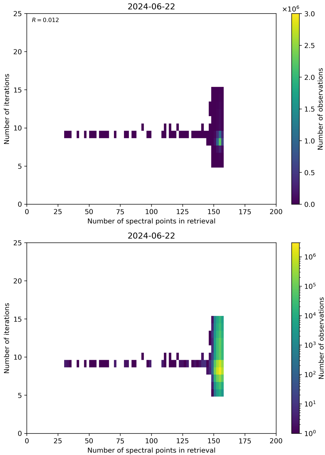
Figure 60: Scatter density plot of “Number of spectral points in retrieval” against “Number of iterations” for 2024-06-21 to 2024-06-23.
