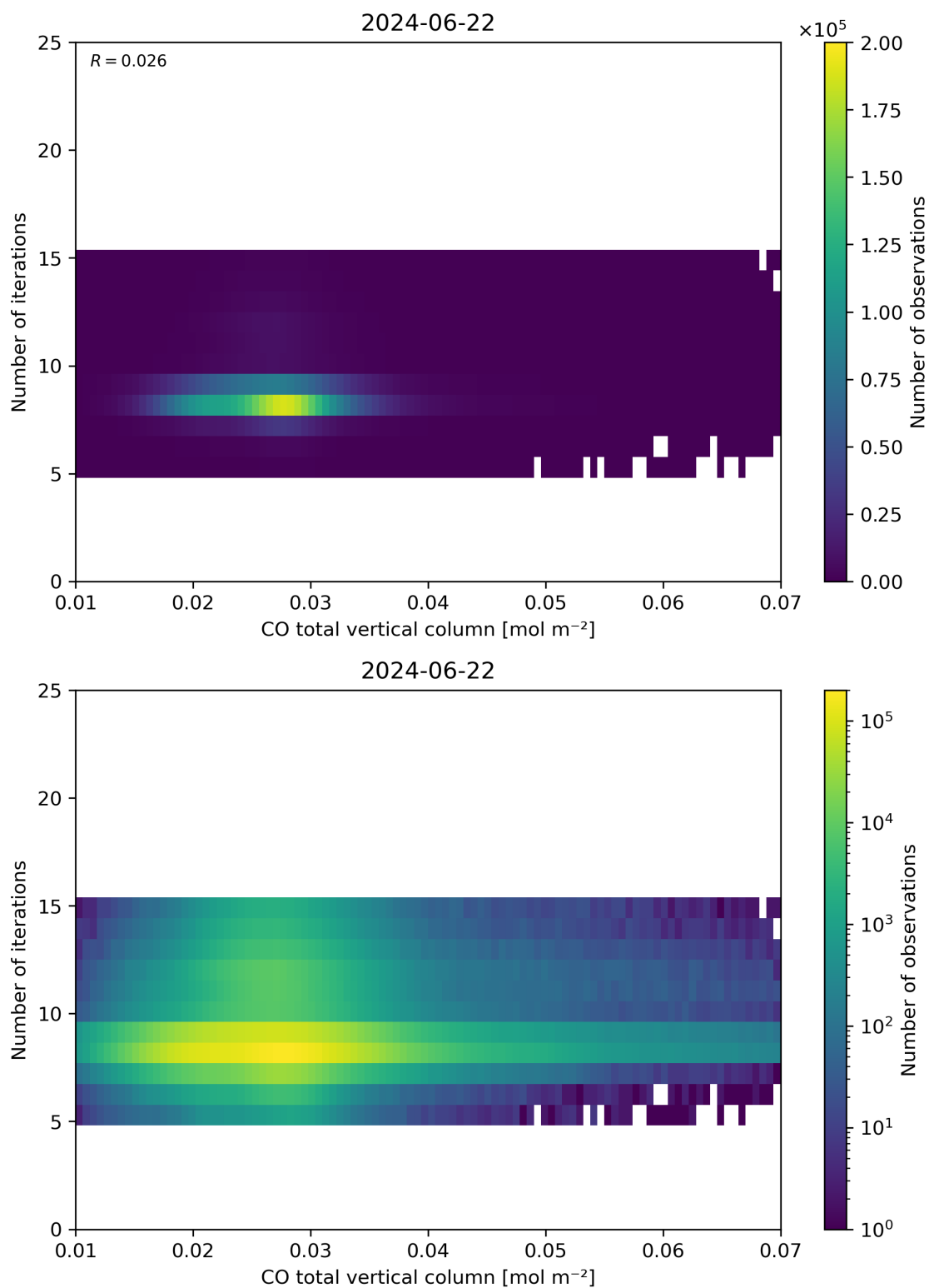
Figure 42: Scatter density plot of “CO total vertical column” against “Number of iterations” for 2024-06-21 to 2024-06-23.
