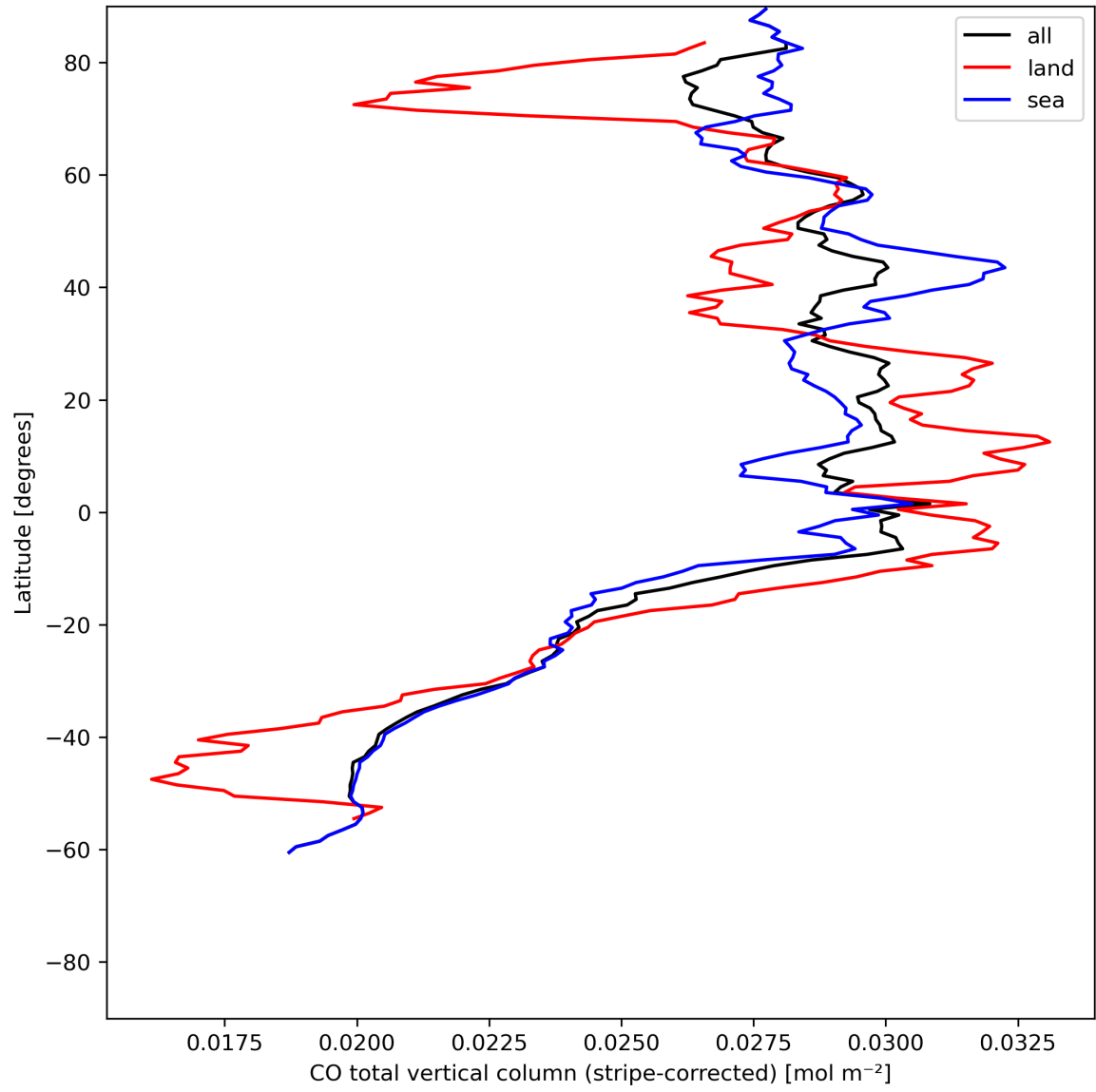
Figure 11: Zonal average of “CO total vertical column (stripe-corrected)” for 2024-06-21 to 2024-06-23.
