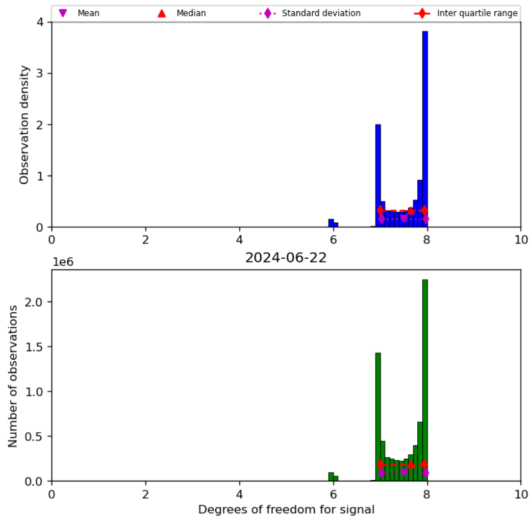
Figure 23: Histogram of “Degrees of freedom for signal” for 2024-06-21 to 2024-06-23
