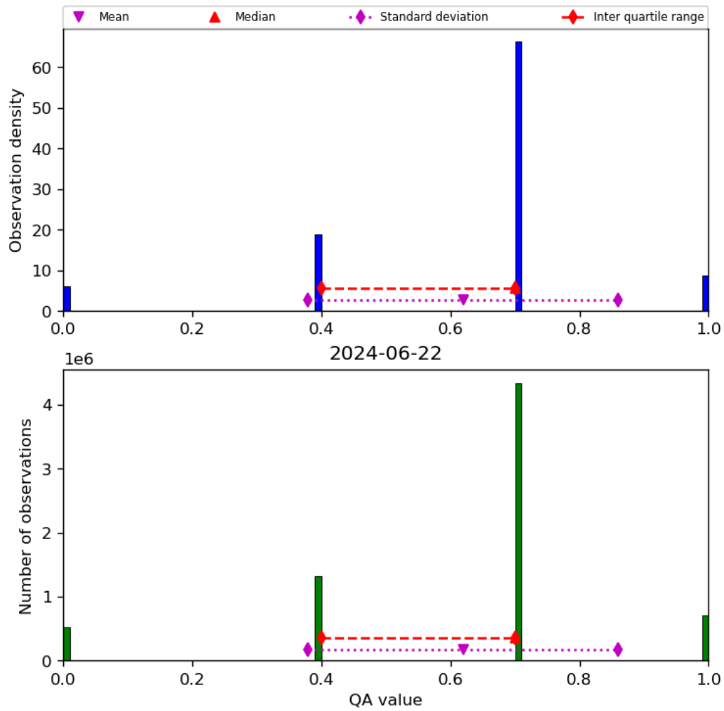
Figure 17: Histogram of “QA value” for 2024-06-21 to 2024-06-23
