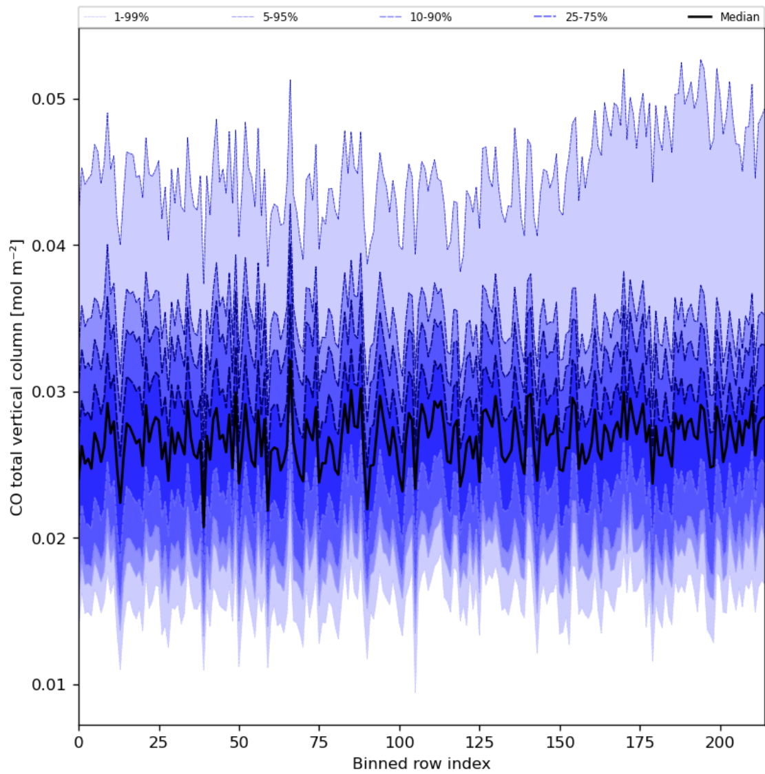
Figure 26: Along track statistics of “CO total vertical column” for 2024-06-21 to 2024-06-23
