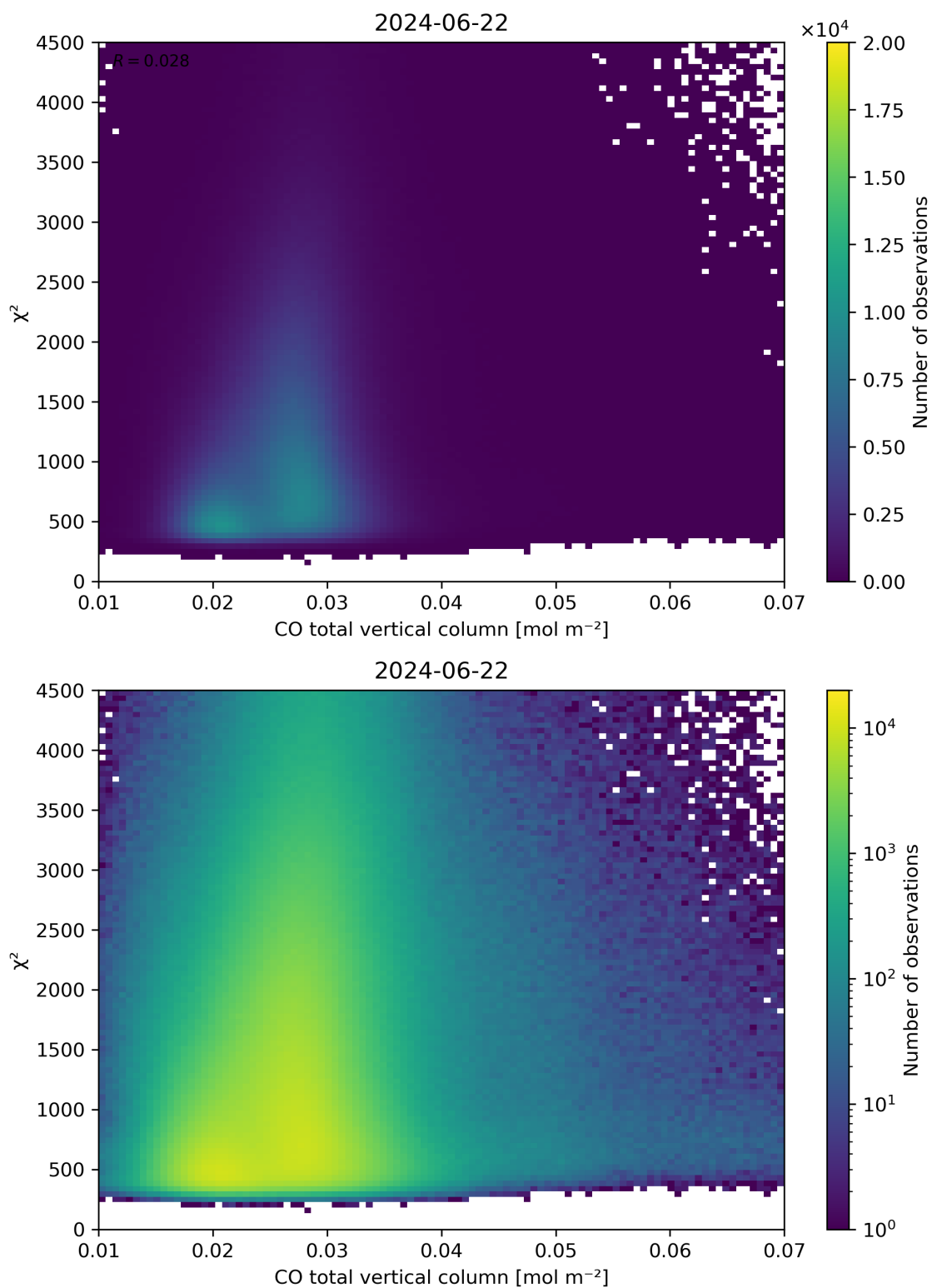
Figure 35: Scatter density plot of “CO total vertical column” against “ \chi^2 ” for 2024-06-21 to 2024-06-23.
