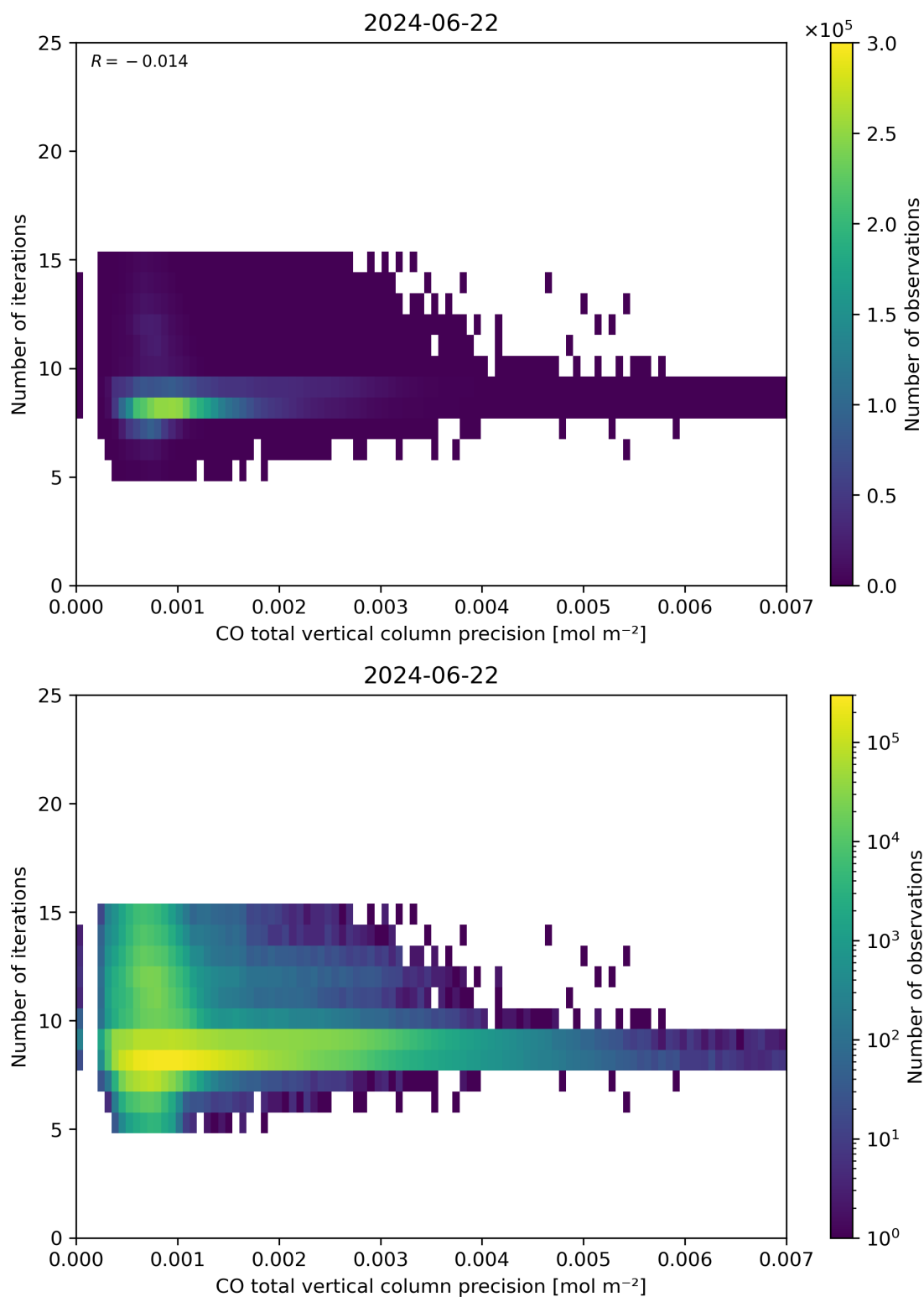
Figure 46: Scatter density plot of “CO total vertical column precision” against “Number of iterations” for 2024-06-21 to 2024-06-23.
