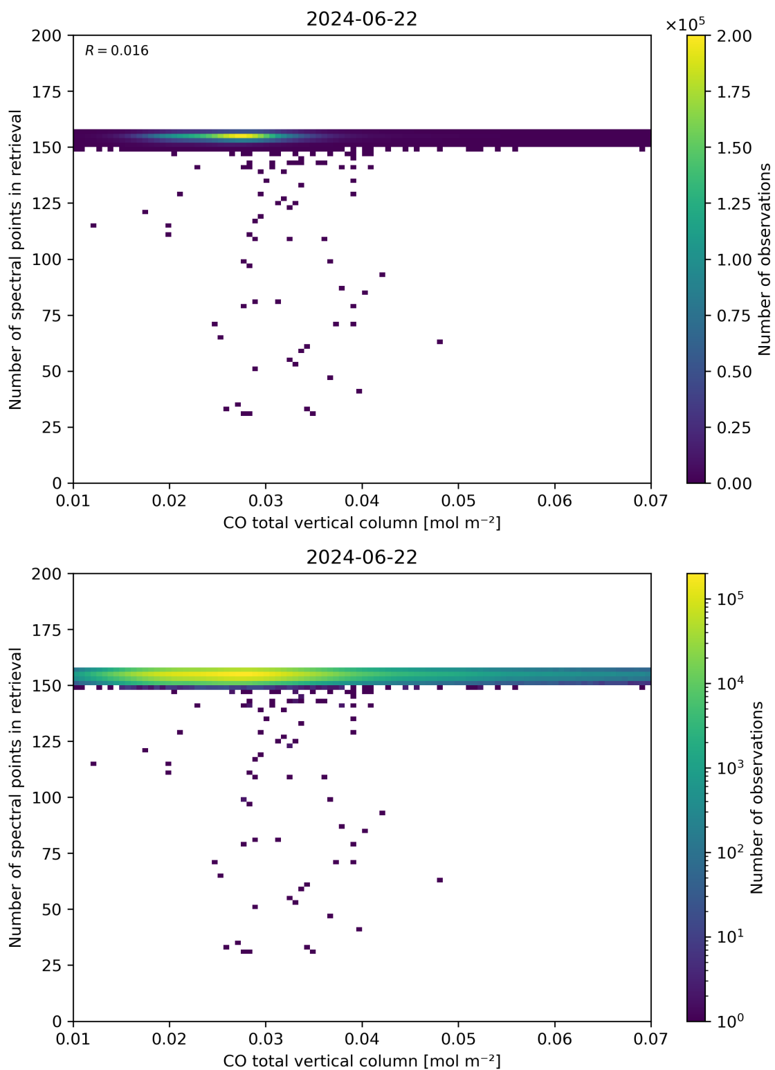
Figure 43: Scatter density plot of “CO total vertical column” against “Number of spectral points in retrieval” for 2024-06-21 to 2024-06-23.
