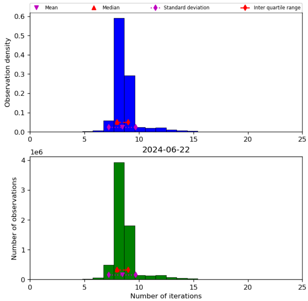
Figure 24: Histogram of “Number of iterations” for 2024-06-21 to 2024-06-23
