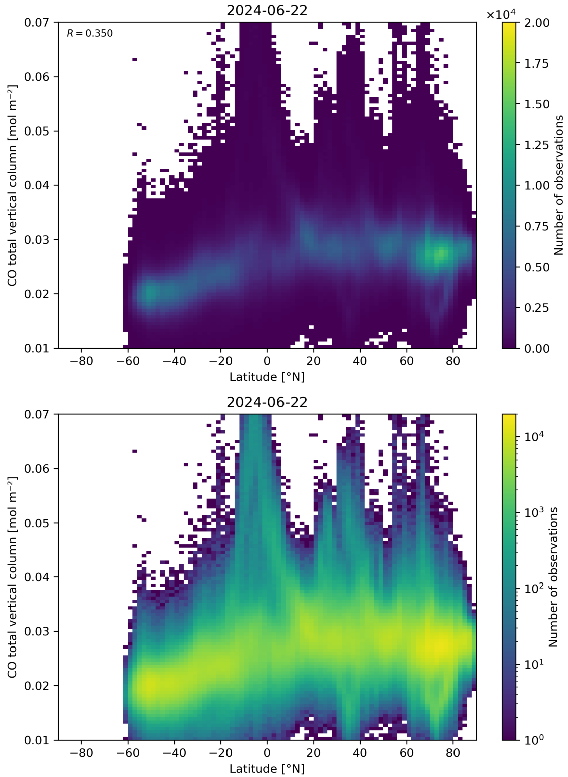
Figure 51: Scatter density plot of “Latitude” against “CO total vertical column” for 2024-06-21 to 2024-06-23.
