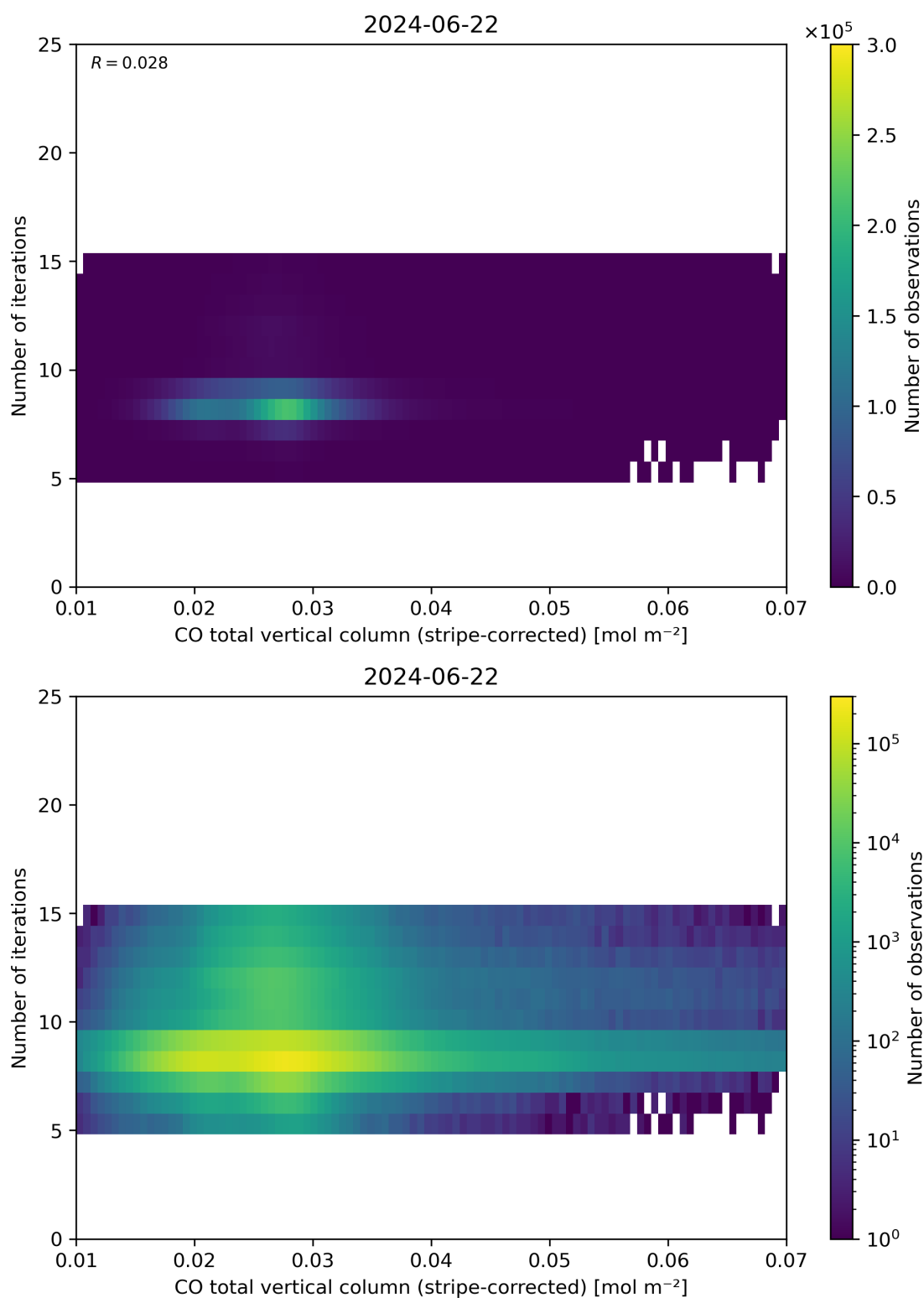
Figure 39: Scatter density plot of “CO total vertical column (stripe-corrected)” against “Number of iterations” for 2024-06-21 to 2024-06-23.
