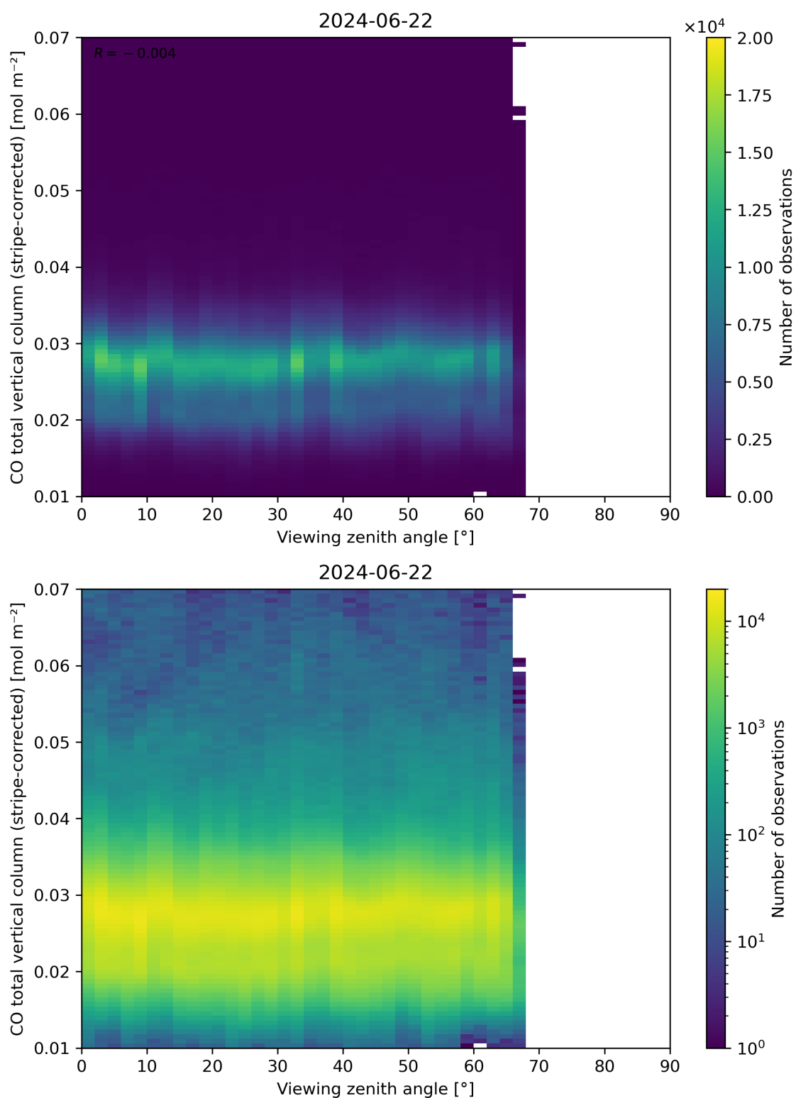
Figure 70: Scatter density plot of “Viewing zenith angle” against “CO total vertical column (stripe-corrected)” for 2024-06-21 to 2024-06-23.
