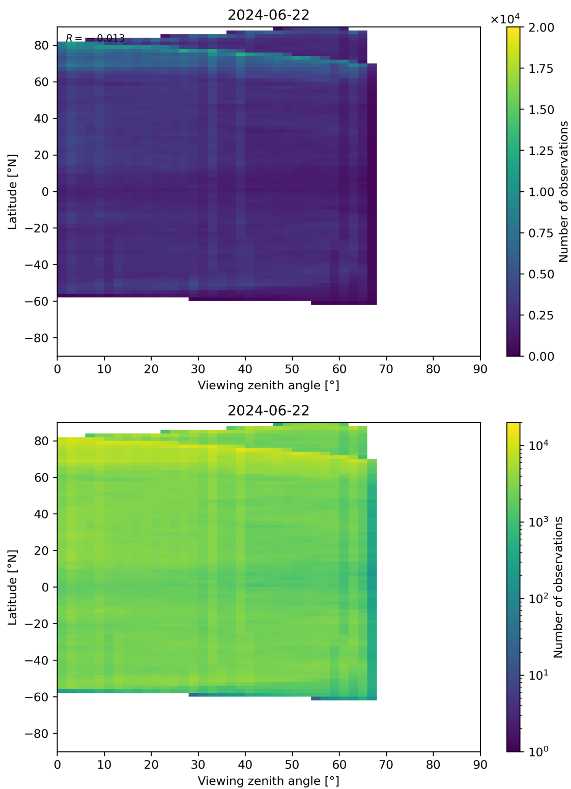
Figure 74: Scatter density plot of “Viewing zenith angle” against “Latitude” for 2024-06-21 to 2024-06-23.
