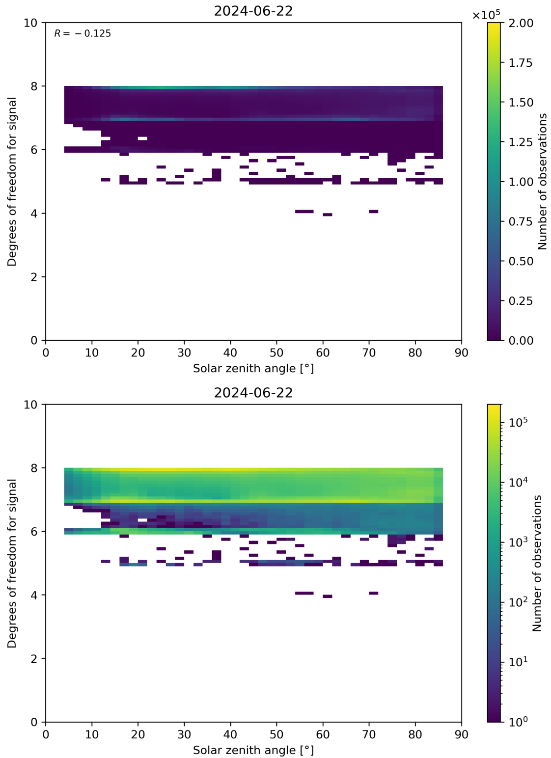
Figure 65: Scatter density plot of “Solar zenith angle” against “Degrees of freedom for signal” for 2024-06-21 to 2024-06-23.
