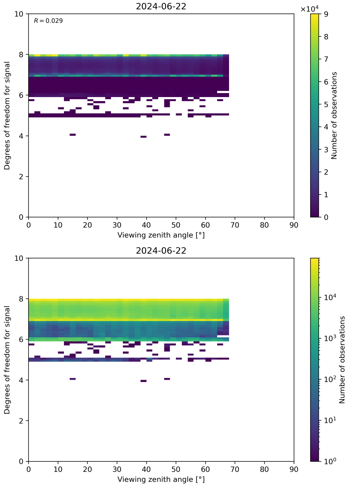
Figure 73: Scatter density plot of “Viewing zenith angle” against “Degrees of freedom for signal” for 2024-06-21 to 2024-06-23.
