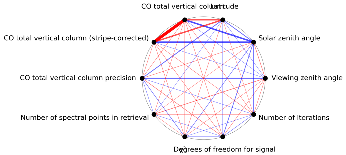
Figure 1: Map of correlation graph for 2024-06-21 to 2024-06-23.
