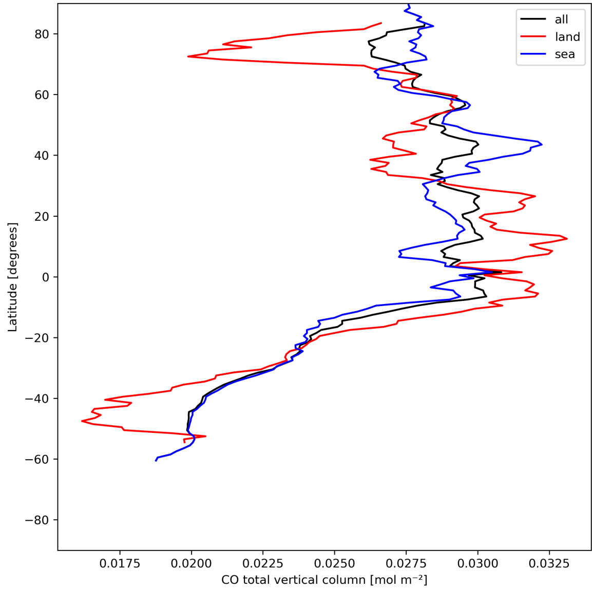
Figure 10: Zonal average of “CO total vertical column” for 2024-06-21 to 2024-06-23.
