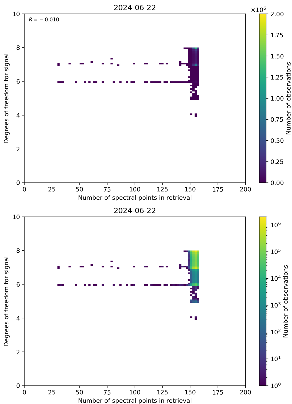
Figure 59: Scatter density plot of “Number of spectral points in retrieval” against “Degrees of freedom for signal” for 2024-06-21 to 2024-06-23.
