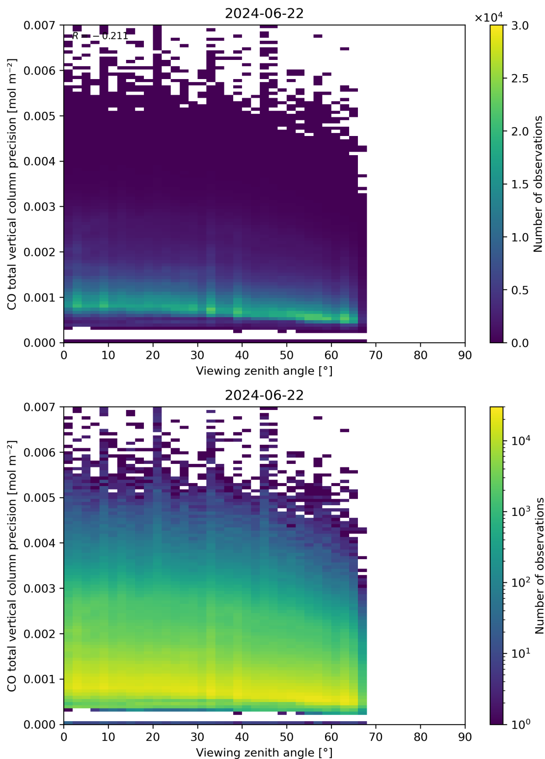
Figure 71: Scatter density plot of “Viewing zenith angle” against “CO total vertical column precision” for 2024-06-21 to 2024-06-23.
