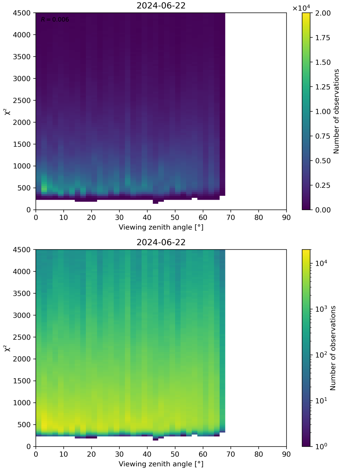
Figure 72: Scatter density plot of “Viewing zenith angle” against “ \chi^2 ” for 2024-06-21 to 2024-06-23.
