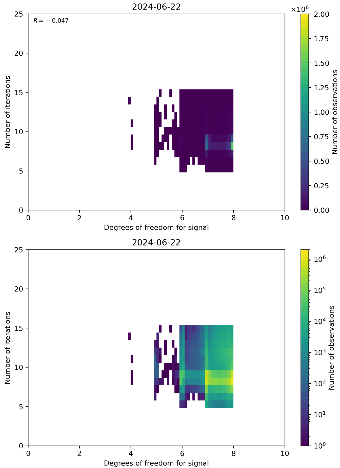
Figure 50: Scatter density plot of “Degrees of freedom for signal” against “Number of iterations” for 2024-06-21 to 2024-06-23.
