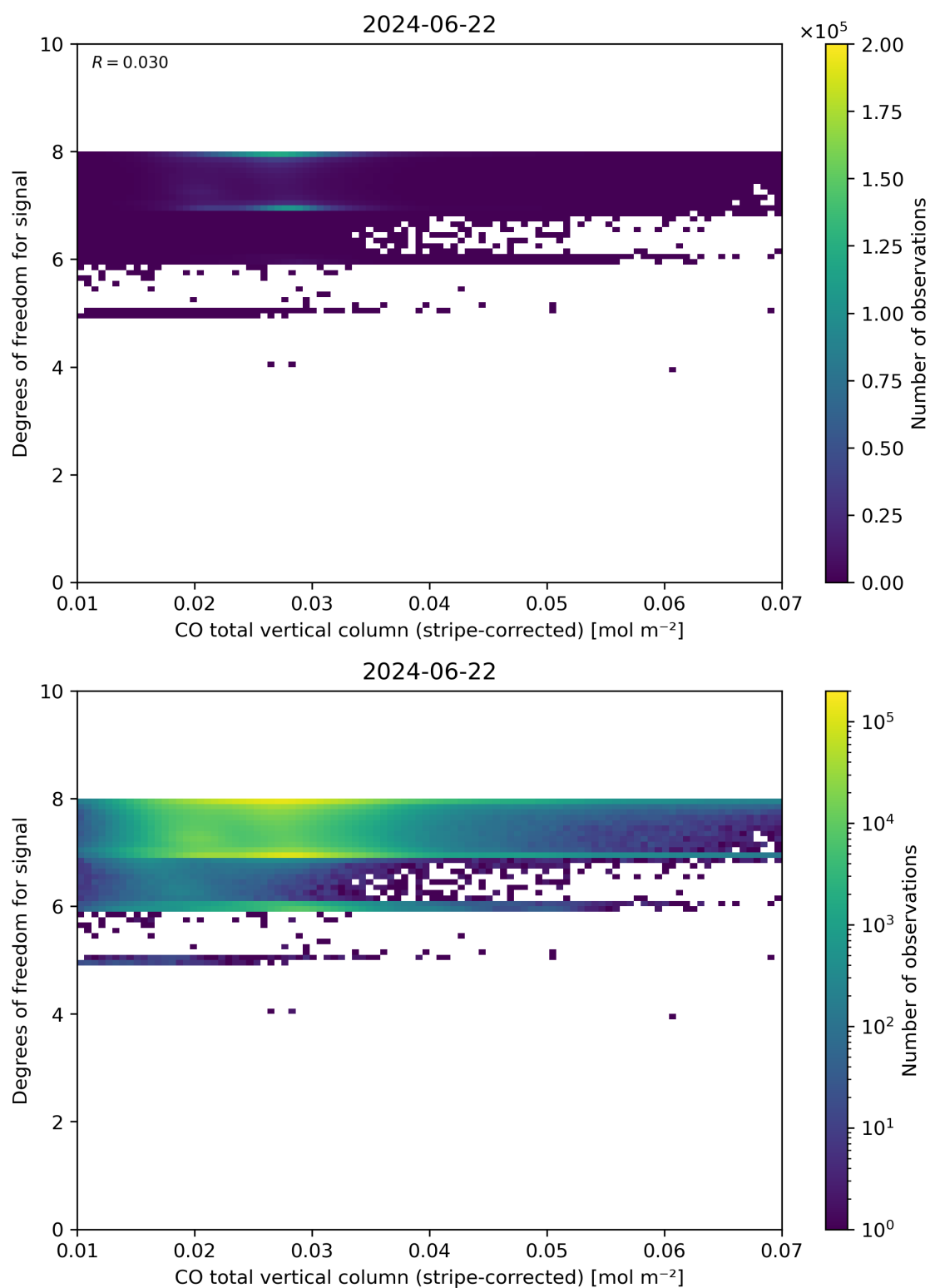
Figure 38: Scatter density plot of “CO total vertical column (stripe-corrected)” against “Degrees of freedom for signal” for 2024-06-21 to 2024-06-23.
