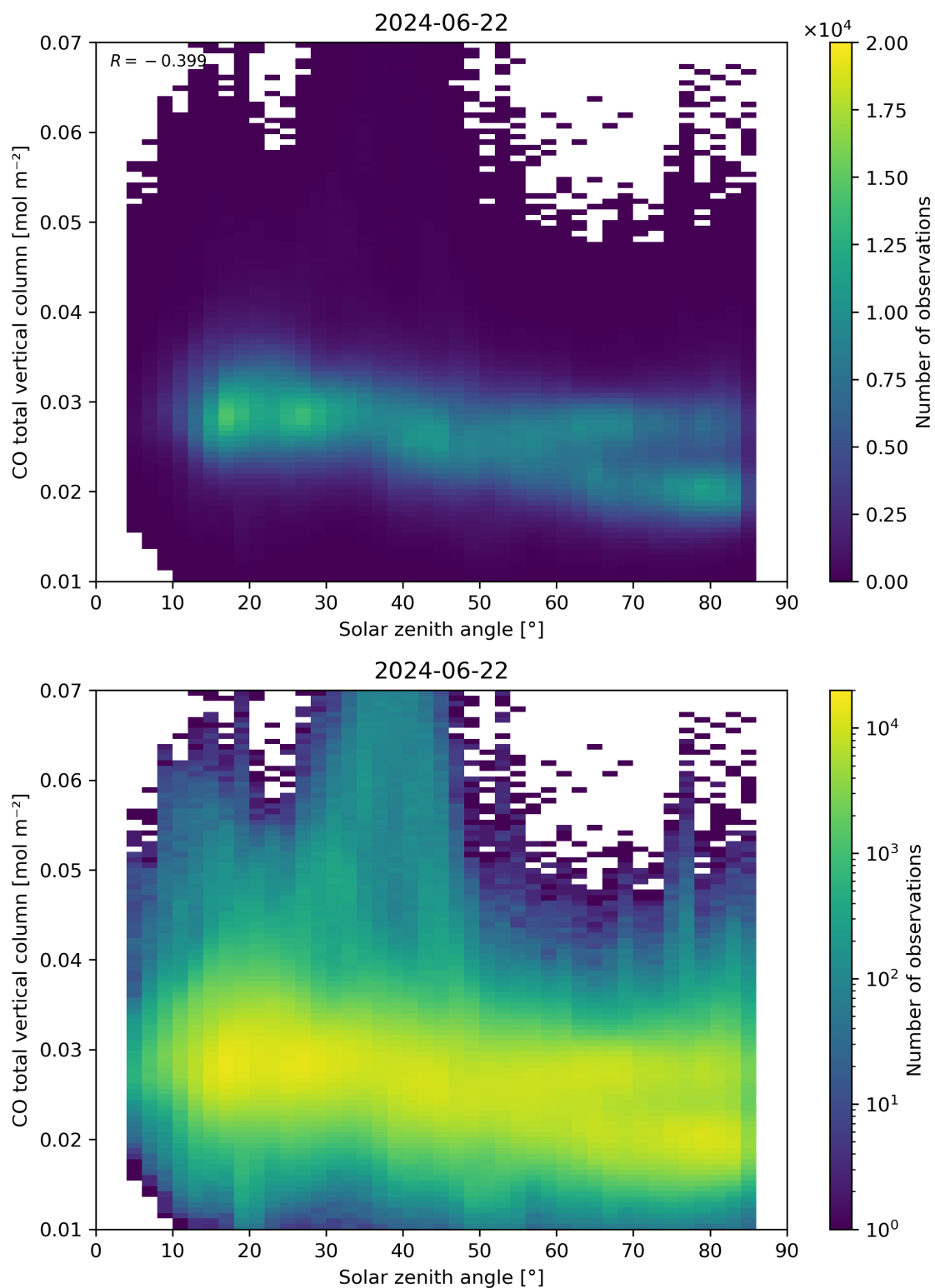
Figure 61: Scatter density plot of “Solar zenith angle” against “CO total vertical column” for 2024-06-21 to 2024-06-23.
