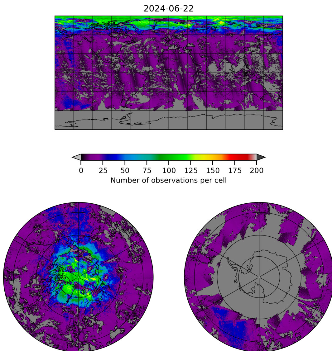
Figure 8: Map of the number of observations for 2024-06-21 to 2024-06-23
