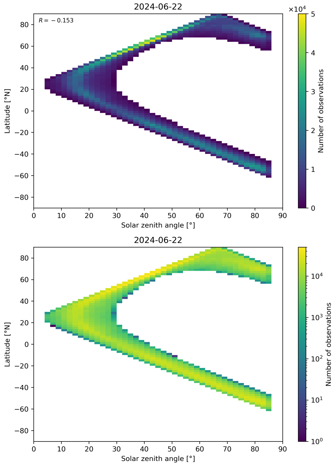
Figure 66: Scatter density plot of “Solar zenith angle” against “Latitude” for 2024-06-21 to 2024-06-23.
