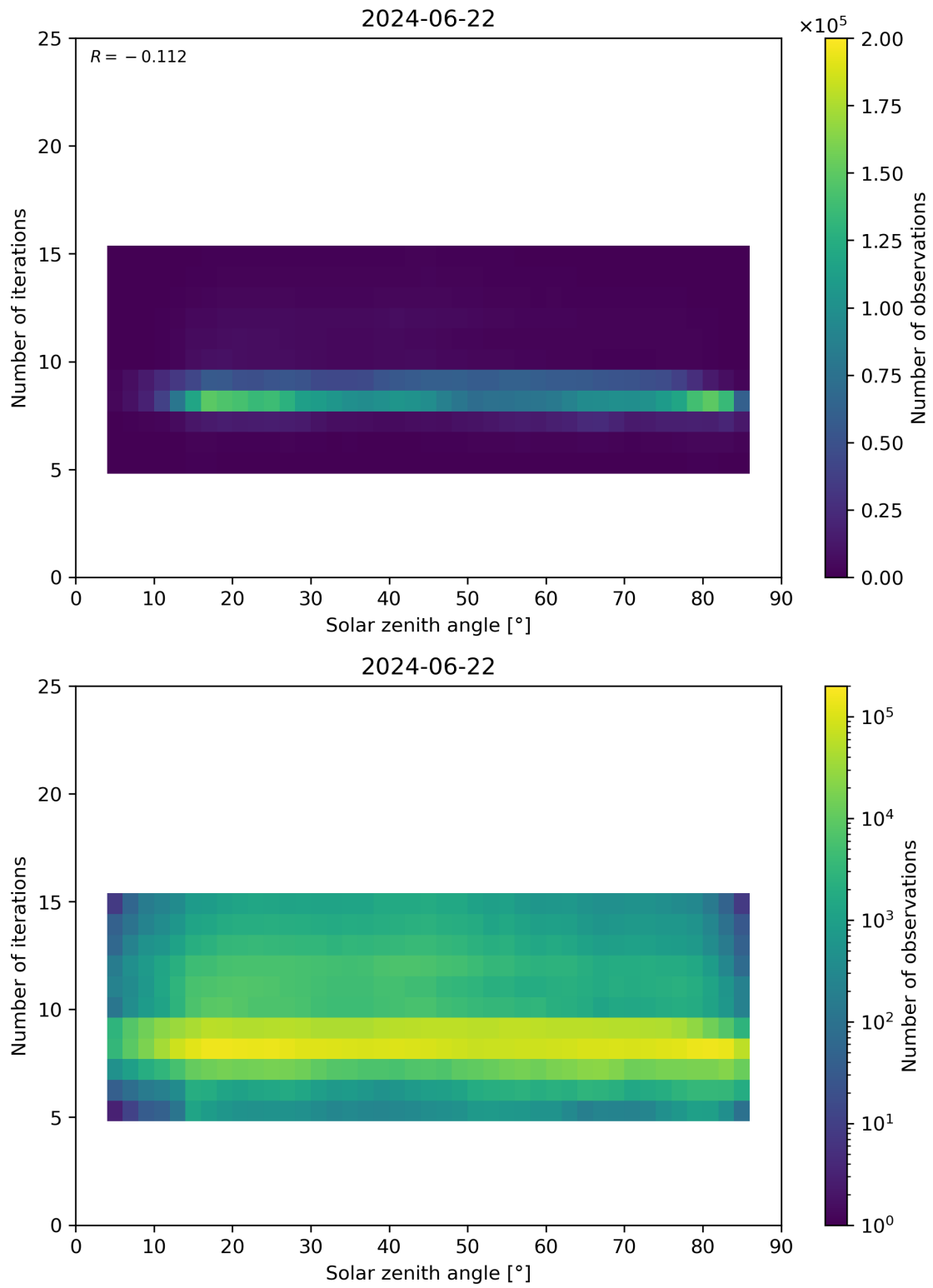
Figure 67: Scatter density plot of “Solar zenith angle” against “Number of iterations” for 2024-06-21 to 2024-06-23.
