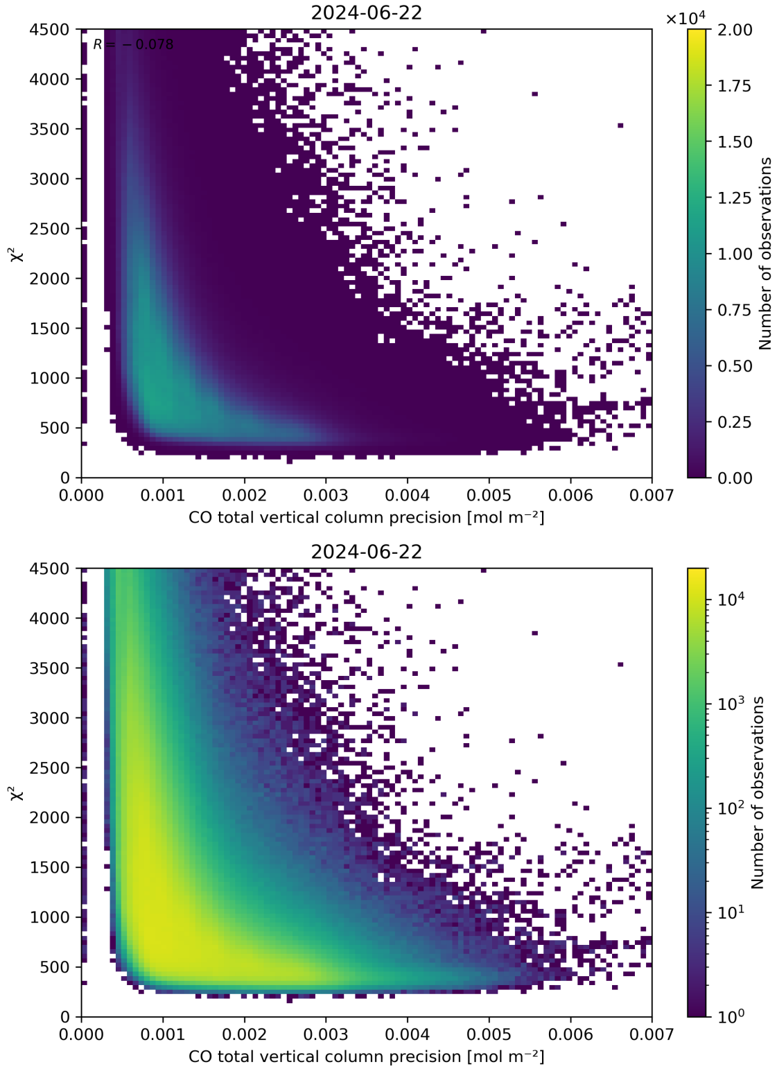
Figure 44: Scatter density plot of “CO total vertical column precision” against “ \chi^2 ” for 2024-06-21 to 2024-06-23.
