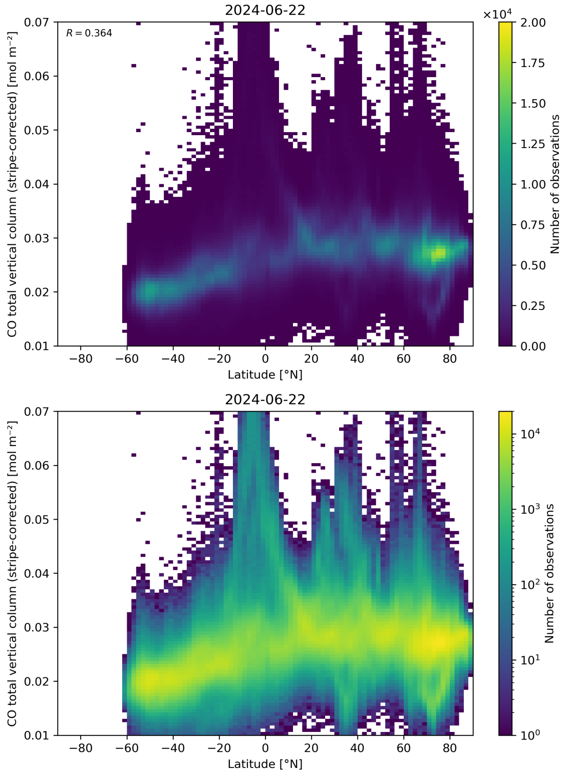
Figure 52: Scatter density plot of “Latitude” against “CO total vertical column (stripe-corrected)” for 2024-06-21 to 2024-06-23.
