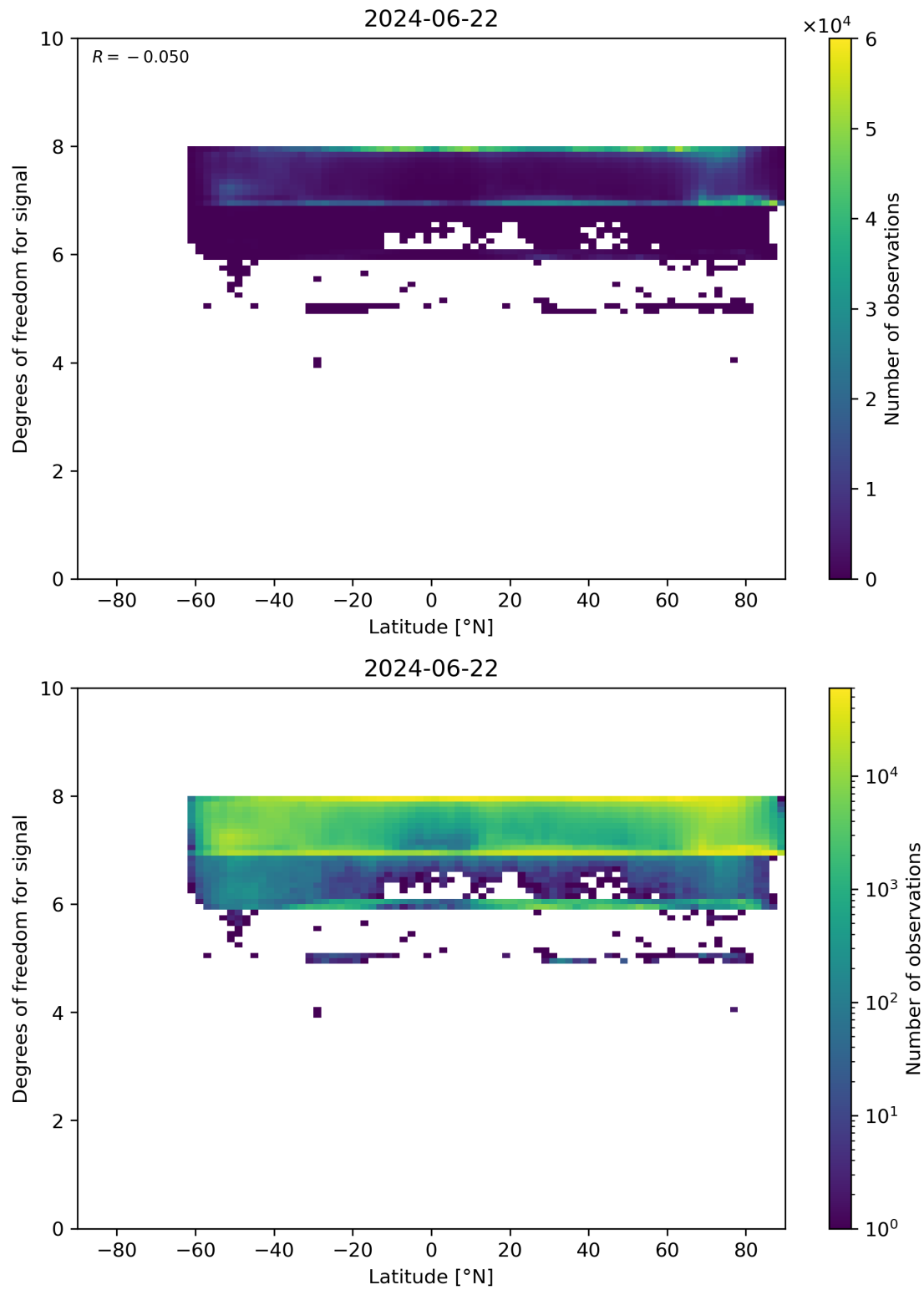
Figure 55: Scatter density plot of “Latitude” against “Degrees of freedom for signal” for 2024-06-21 to 2024-06-23.
