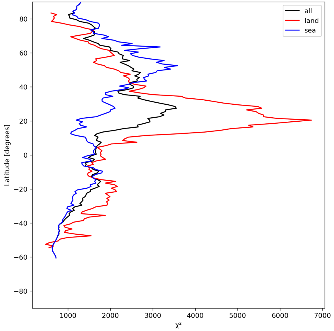
Figure 14: Zonal average of “ \chi^2 ” for 2024-06-21 to 2024-06-23.
