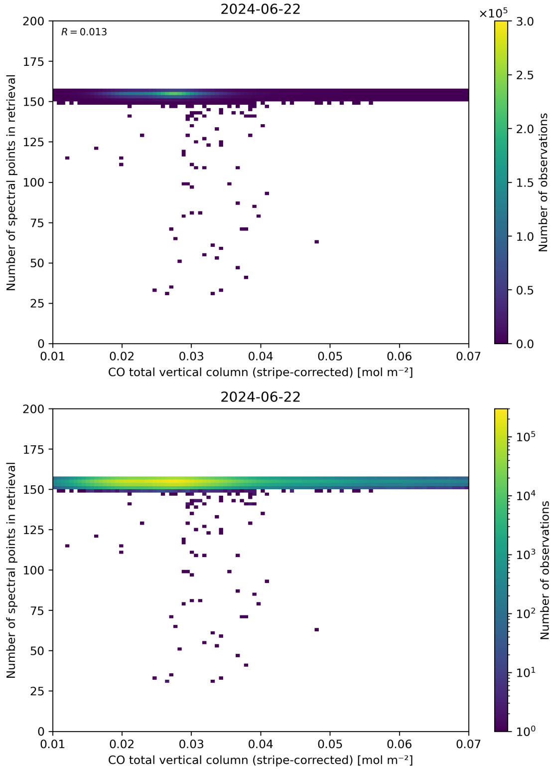
Figure 40: Scatter density plot of “CO total vertical column (stripe-corrected)” against “Number of spectral points in retrieval” for 2024-06-21 to 2024-06-23.
