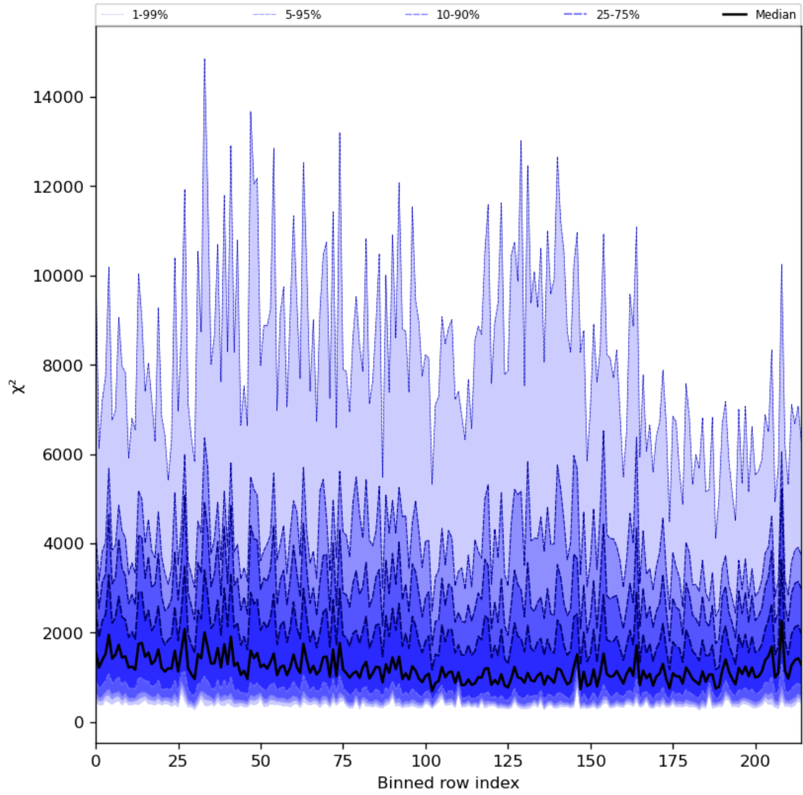
Figure 30: Along track statistics of “ \chi^2 ” for 2024-06-21 to 2024-06-23
