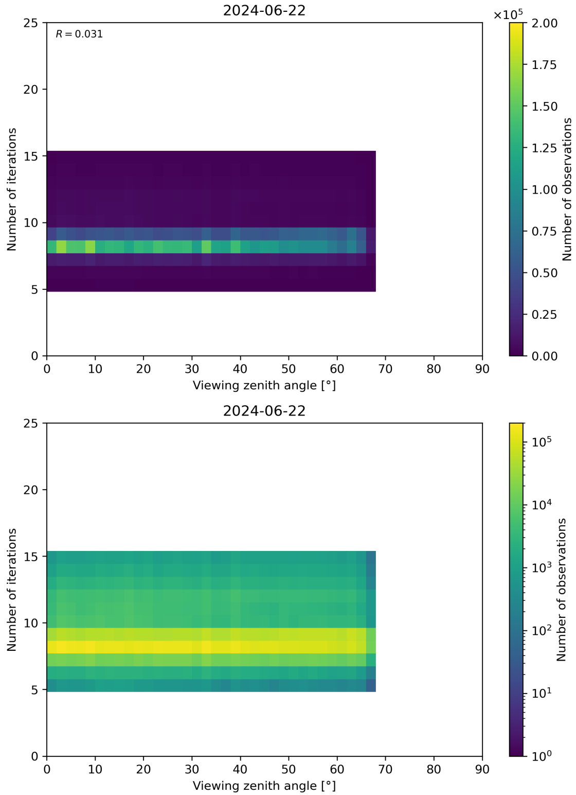
Figure 75: Scatter density plot of “Viewing zenith angle” against “Number of iterations” for 2024-06-21 to 2024-06-23.
