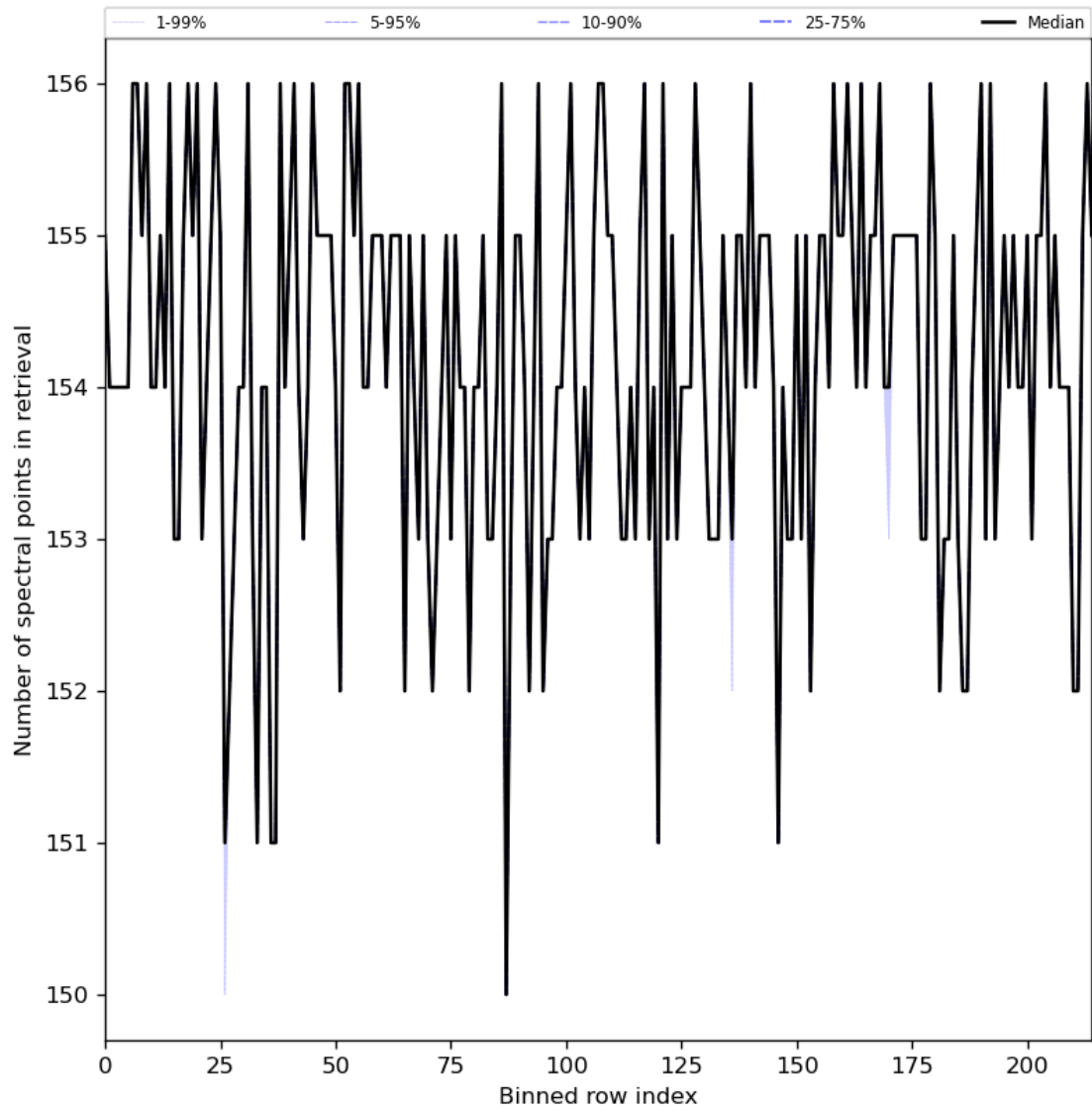
Figure 29: Along track statistics of “Number of spectral points in retrieval” for 2024-06-21 to 2024-06-23
