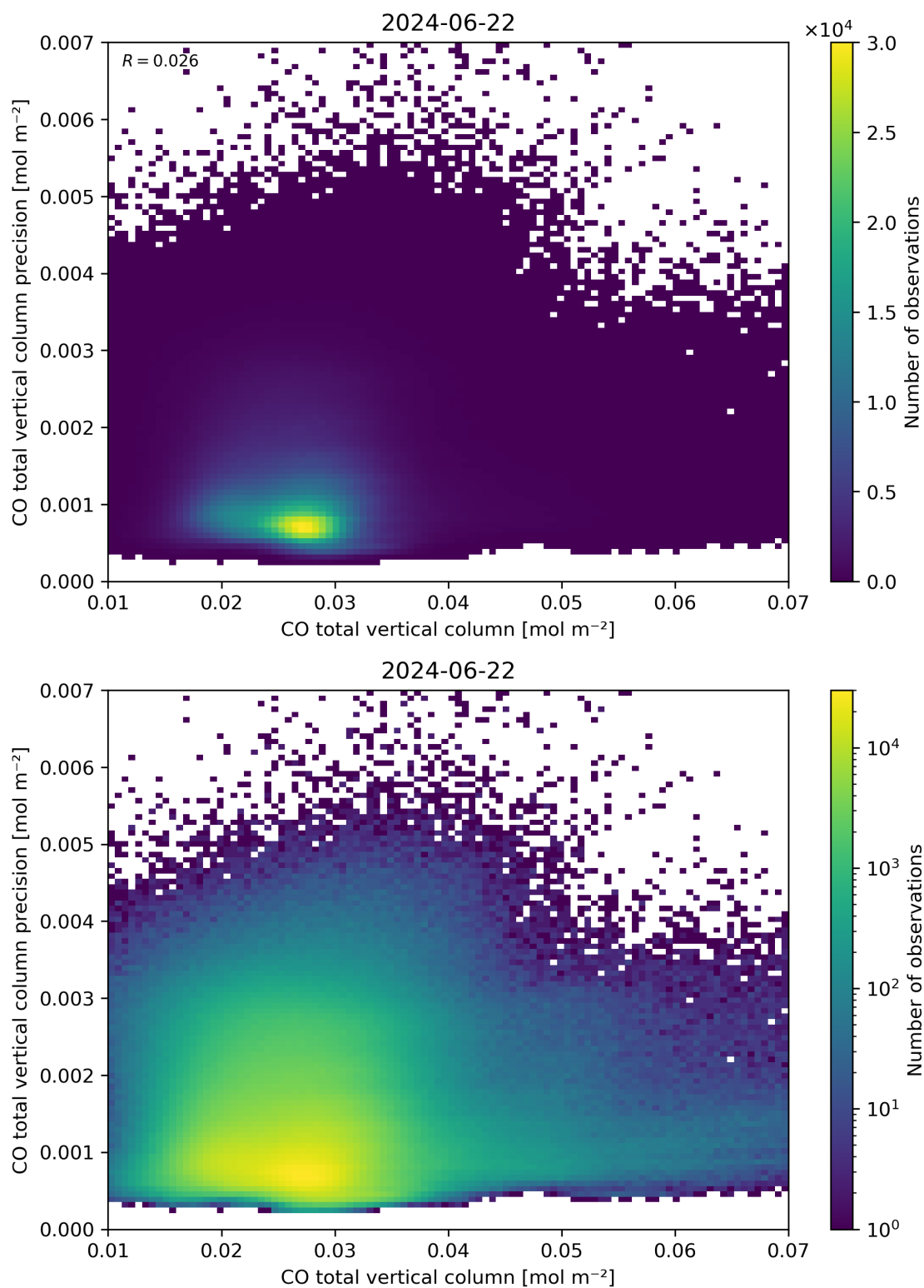
Figure 34: Scatter density plot of “CO total vertical column” against “CO total vertical column precision” for 2024-06-21 to 2024-06-23.
