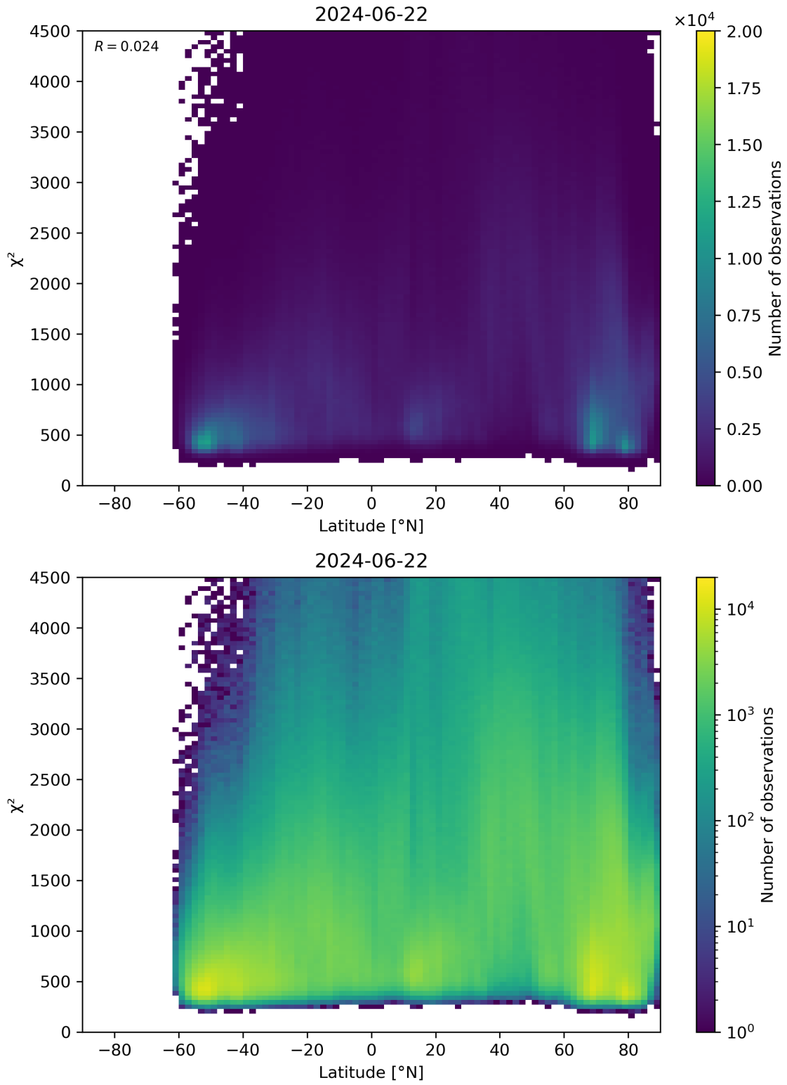
Figure 54: Scatter density plot of “Latitude” against “ \chi^2 ” for 2024-06-21 to 2024-06-23.
