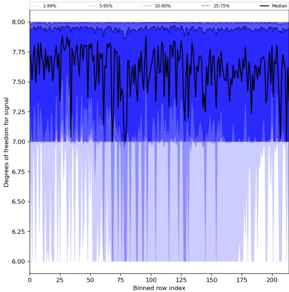
Figure 31: Along track statistics of “Degrees of freedom for signal” for 2024-06-21 to 2024-06-23
