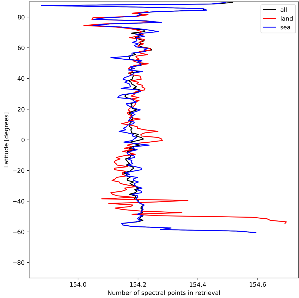
Figure 13: Zonal average of “Number of spectral points in retrieval” for 2024-06-21 to 2024-06-23.
