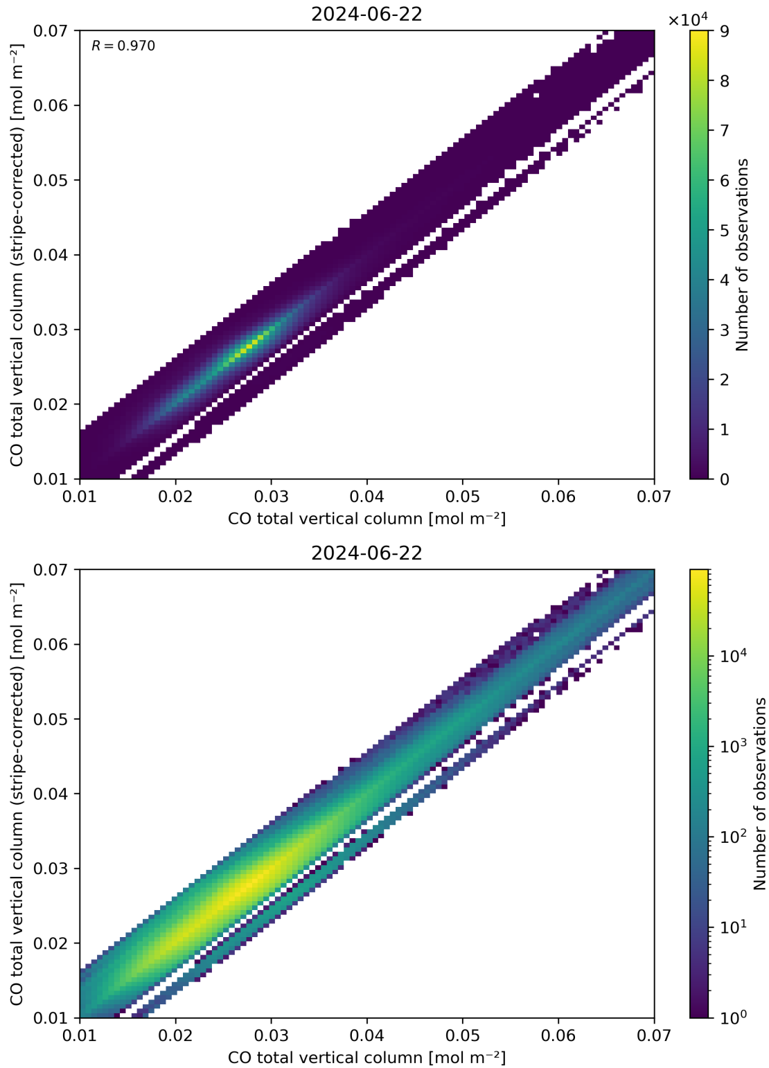
Figure 33: Scatter density plot of “CO total vertical column” against “CO total vertical column (stripe-corrected)” for 2024-06-21 to 2024-06-23.
