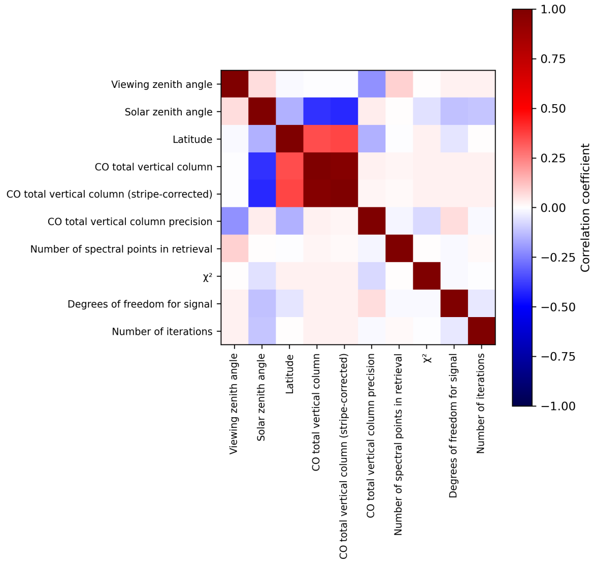
Figure 2: Map of correlation matrix for 2024-06-21 to 2024-06-23.
