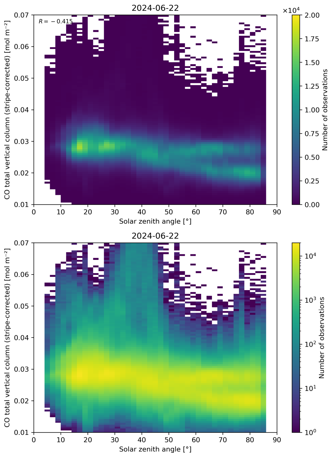
Figure 62: Scatter density plot of “Solar zenith angle” against “CO total vertical column (stripe-corrected)” for 2024-06-21 to 2024-06-23.
