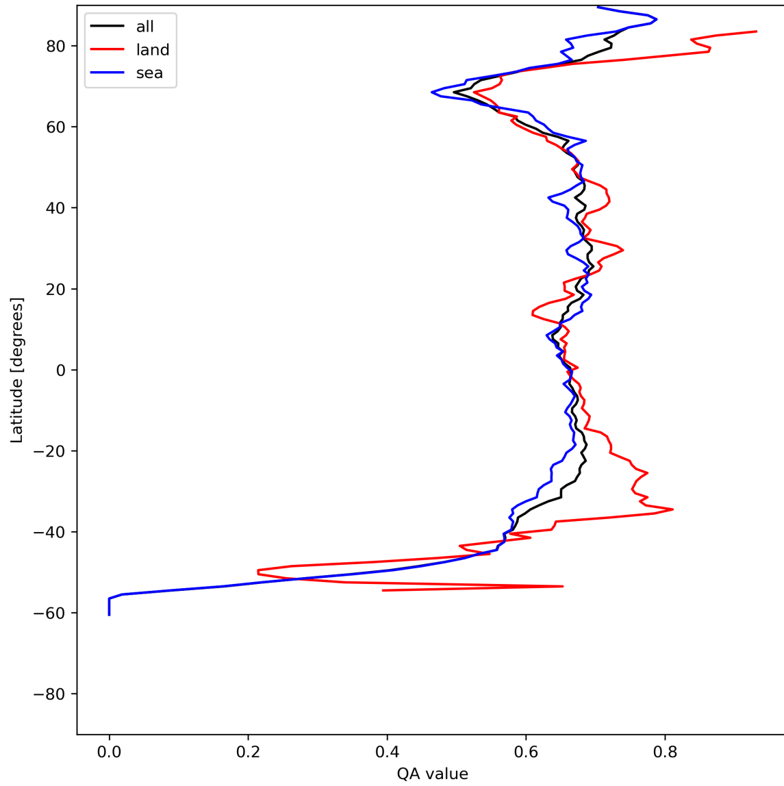
Figure 9: Zonal average of “QA value” for 2024-06-21 to 2024-06-23.
