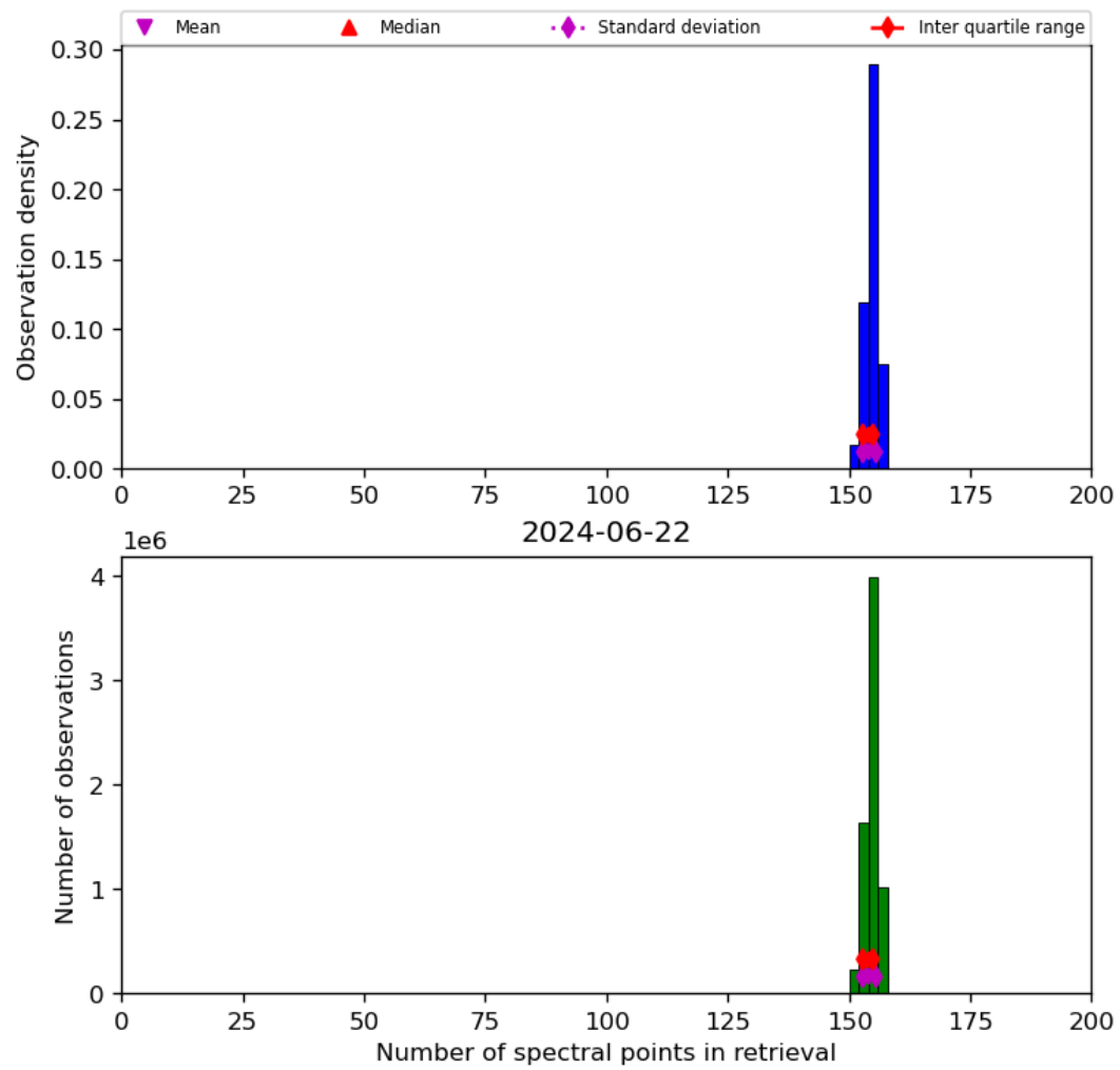
Figure 21: Histogram of “Number of spectral points in retrieval” for 2024-06-21 to 2024-06-23
