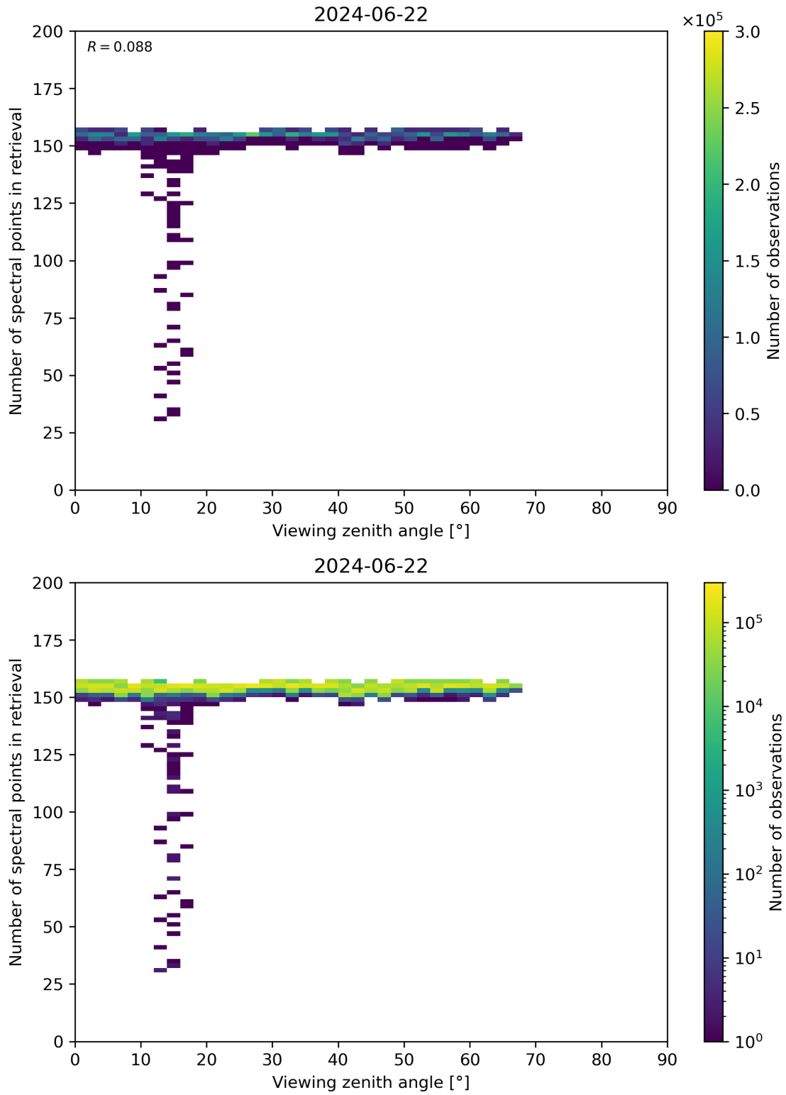
Figure 76: Scatter density plot of “Viewing zenith angle” against “Number of spectral points in retrieval” for 2024-06-21 to 2024-06-23.
