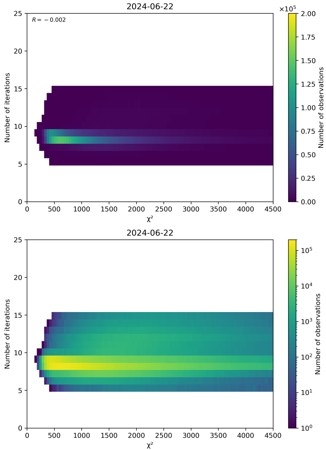
Figure 49: Scatter density plot of “ \chi^2 ” against “Number of iterations” for 2024-06-21 to 2024-06-23.
