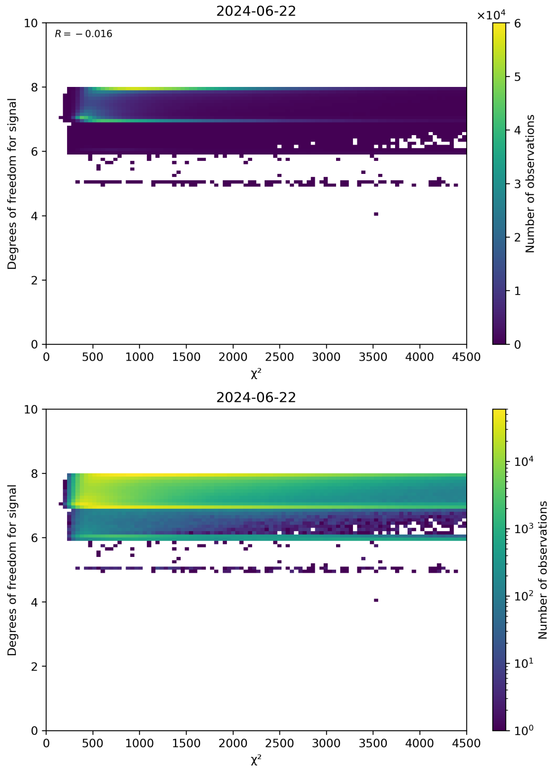
Figure 48: Scatter density plot of “ \chi^2 ” against “Degrees of freedom for signal” for 2024-06-21 to 2024-06-23.
