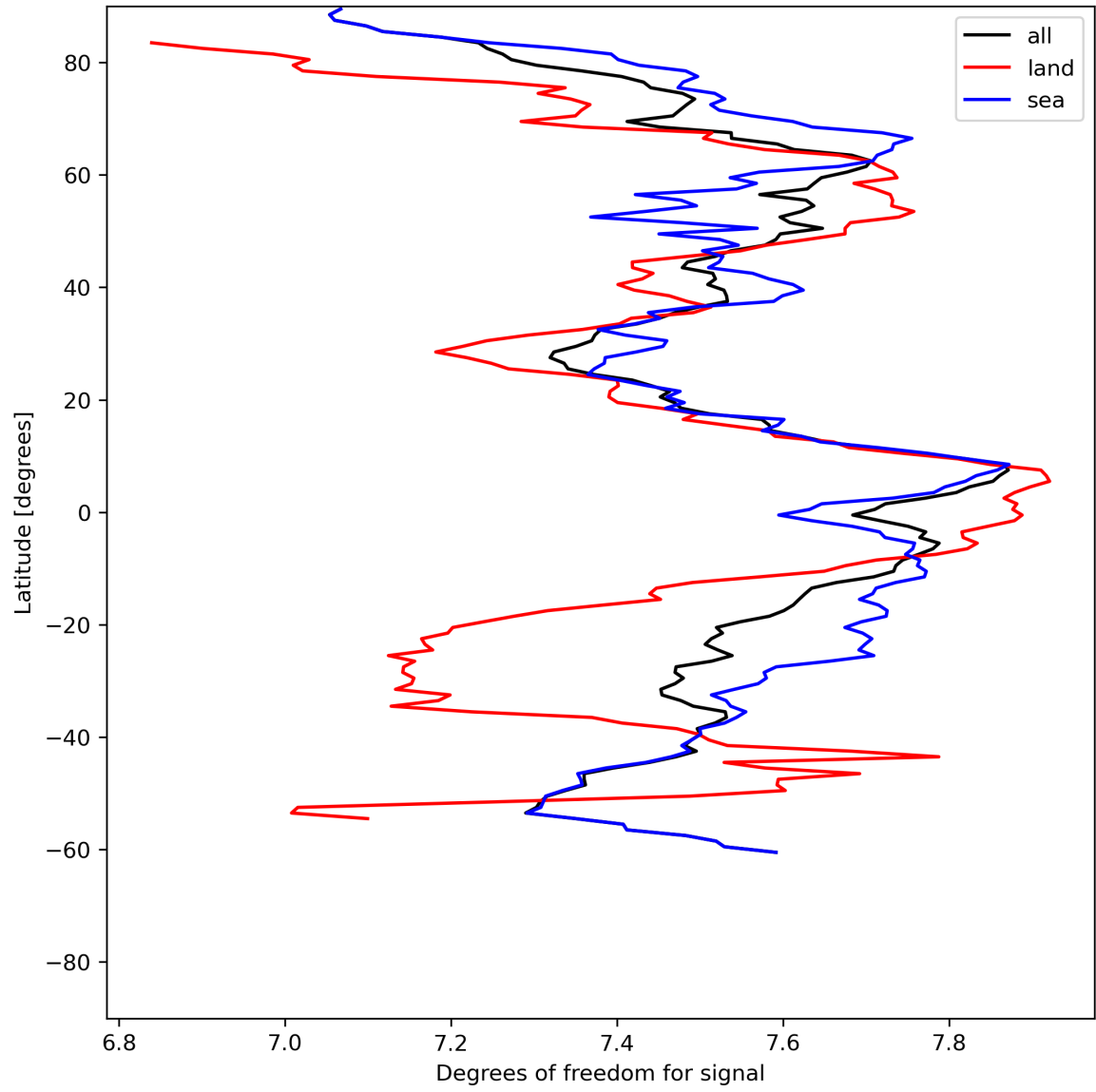
Figure 15: Zonal average of “Degrees of freedom for signal” for 2024-06-21 to 2024-06-23.
