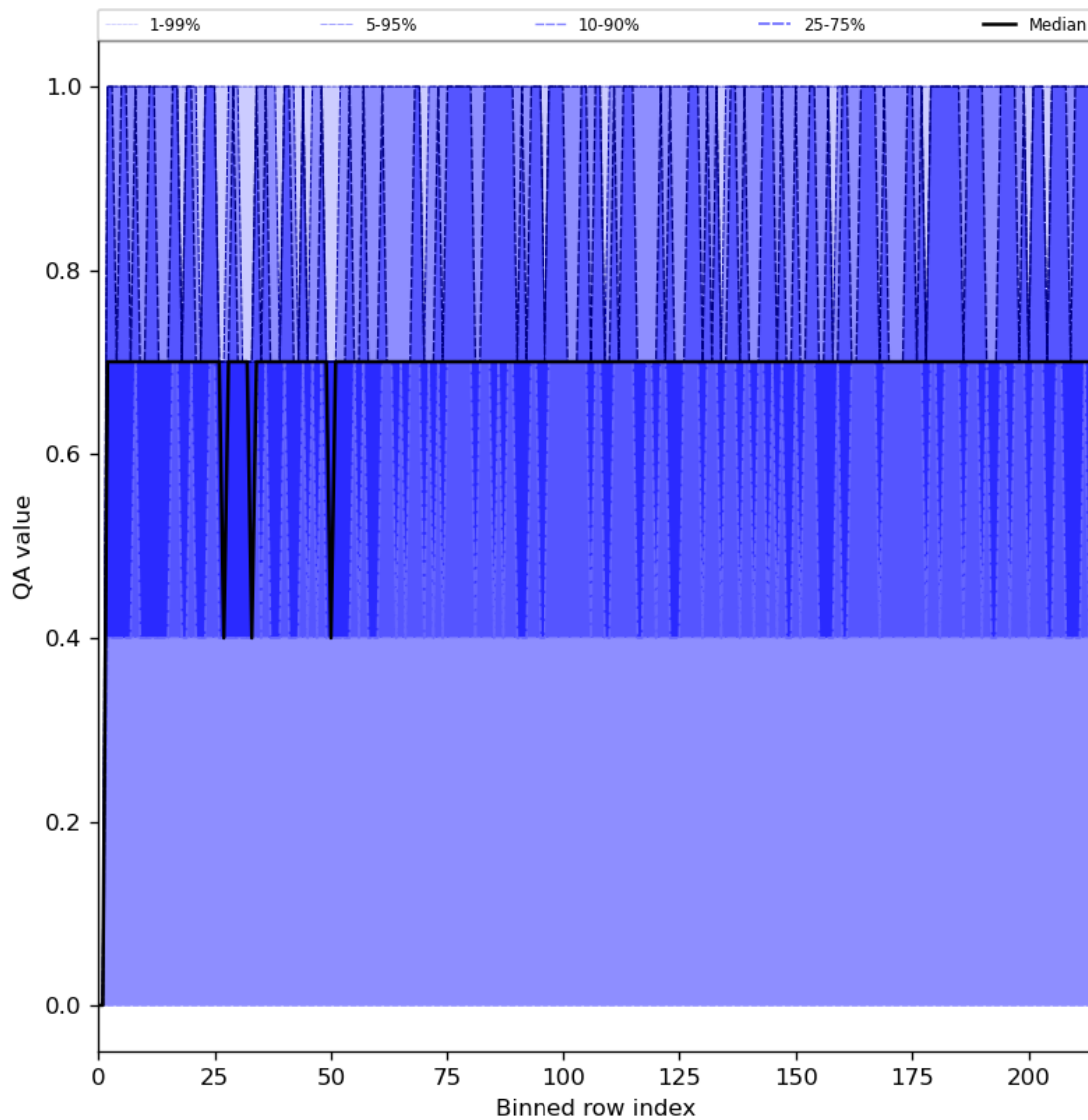
Figure 25: Along track statistics of “QA value” for 2024-06-21 to 2024-06-23
