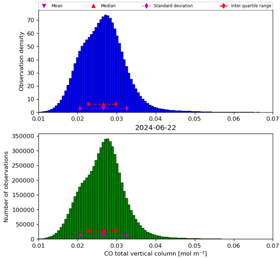
Figure 18: Histogram of “CO total vertical column” for 2024-06-21 to 2024-06-23
