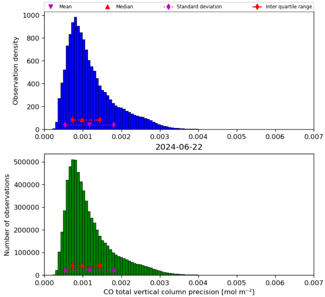
Figure 20: Histogram of “CO total vertical column precision” for 2024-06-21 to 2024-06-23
