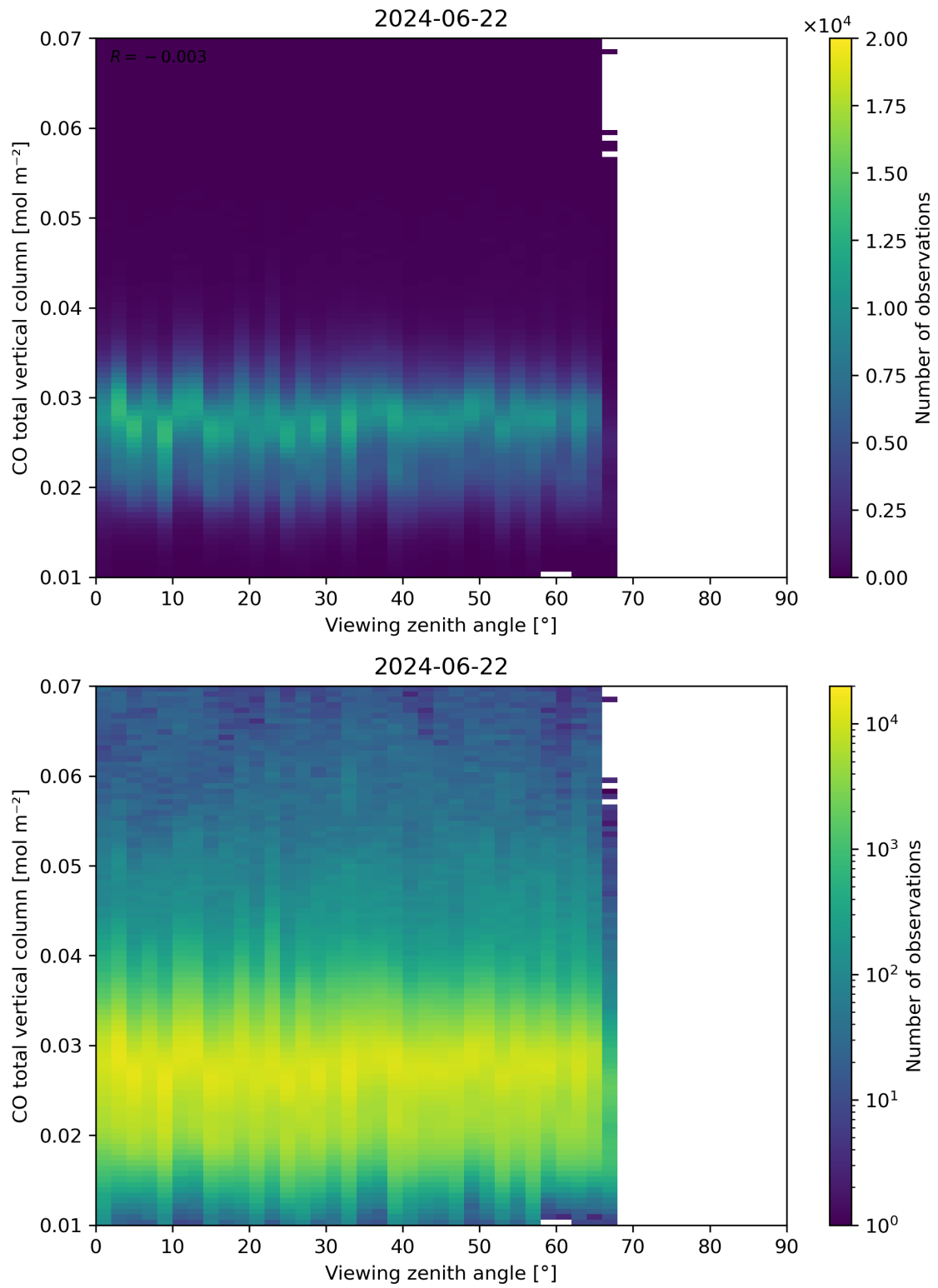
Figure 69: Scatter density plot of “Viewing zenith angle” against “CO total vertical column” for 2024-06-21 to 2024-06-23.
