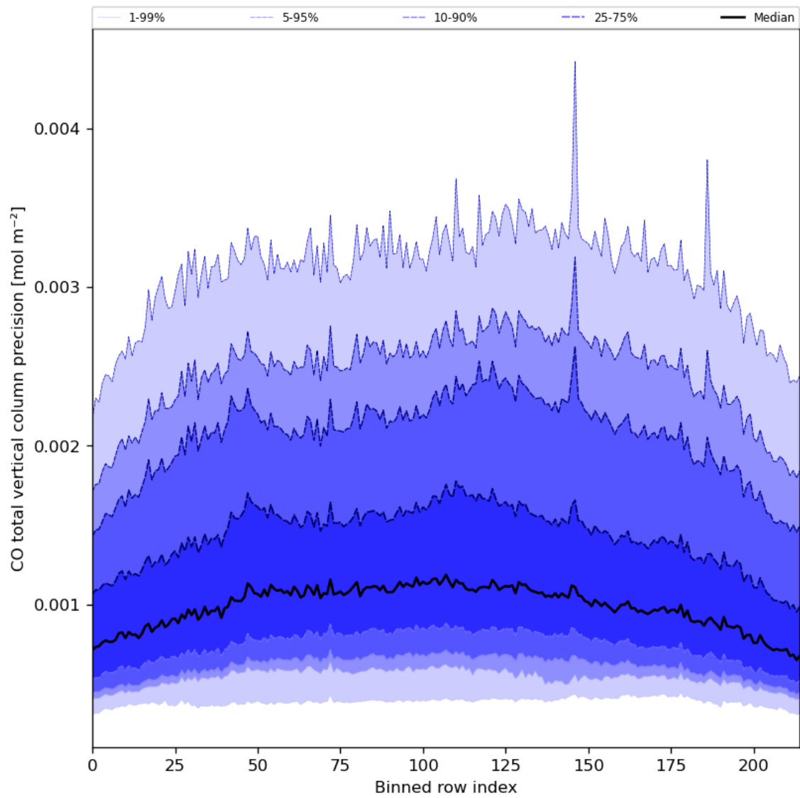
Figure 28: Along track statistics of “CO total vertical column precision” for 2024-06-21 to 2024-06-23
