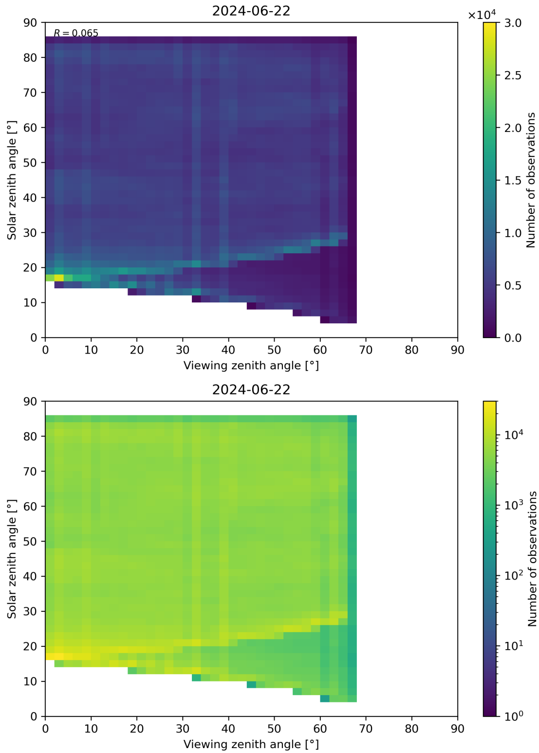
Figure 77: Scatter density plot of “Viewing zenith angle” against “Solar zenith angle” for 2024-06-21 to 2024-06-23.
