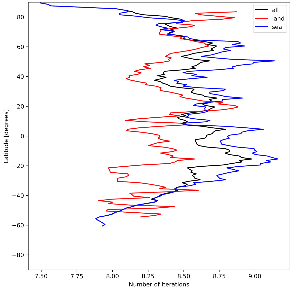
Figure 16: Zonal average of “Number of iterations” for 2024-06-21 to 2024-06-23.
