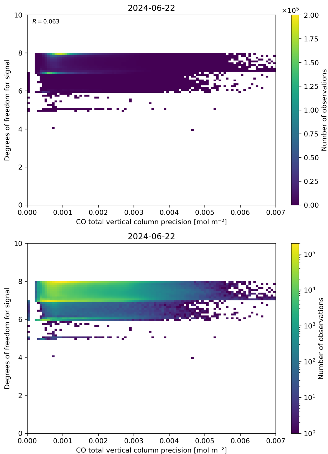
Figure 45: Scatter density plot of “CO total vertical column precision” against “Degrees of freedom for signal” for 2024-06-21 to 2024-06-23.
