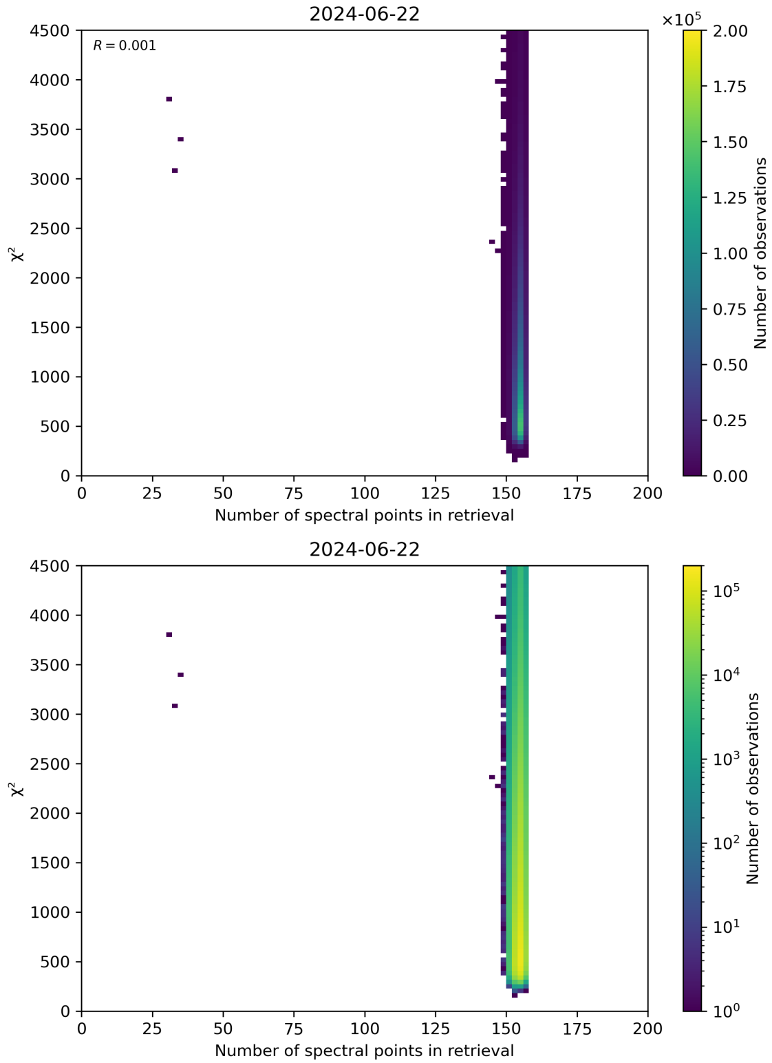
Figure 58: Scatter density plot of “Number of spectral points in retrieval” against “ \chi^2 ” for 2024-06-21 to 2024-06-23.
