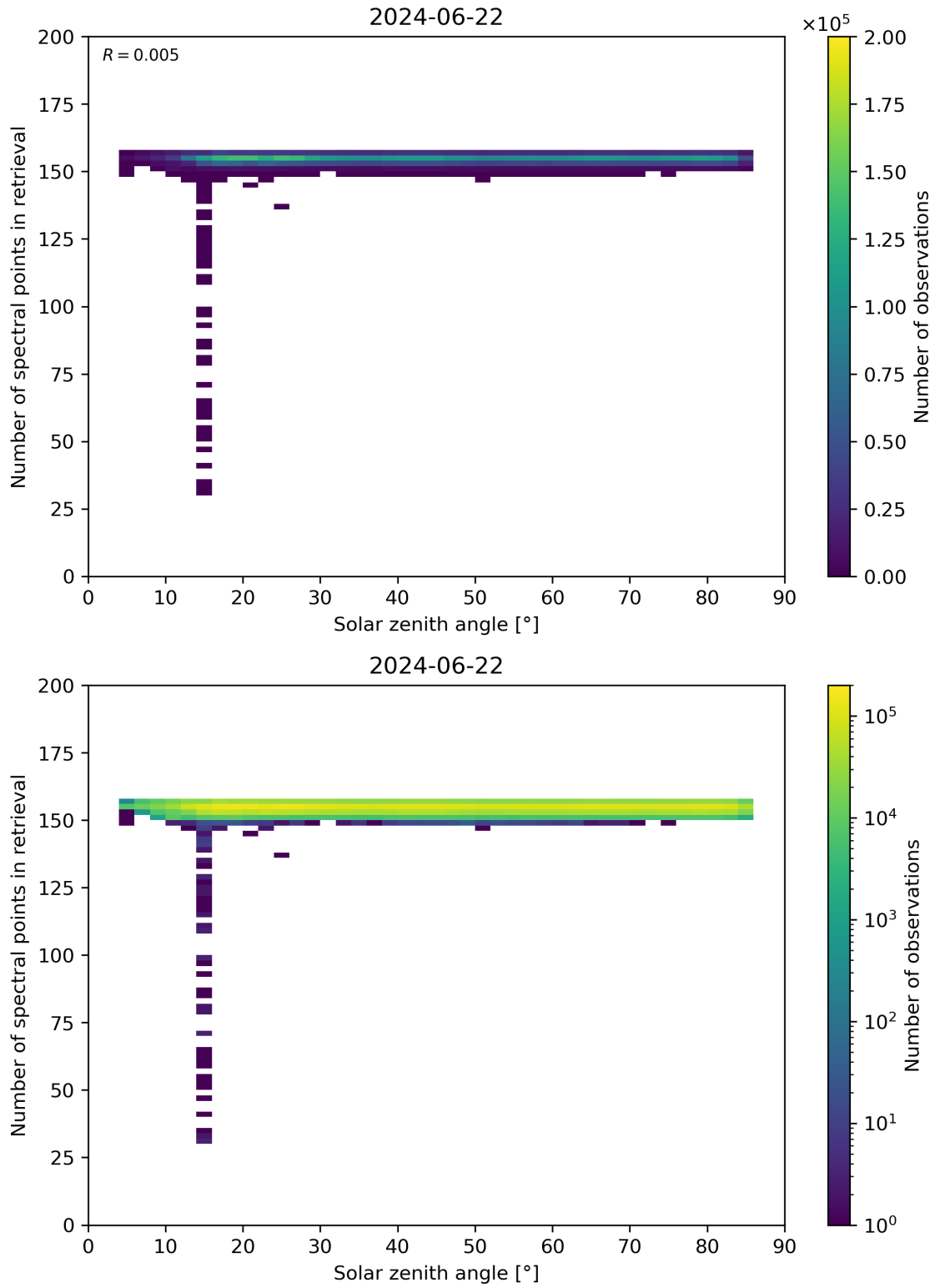
Figure 68: Scatter density plot of “Solar zenith angle” against “Number of spectral points in retrieval” for 2024-06-21 to 2024-06-23.
