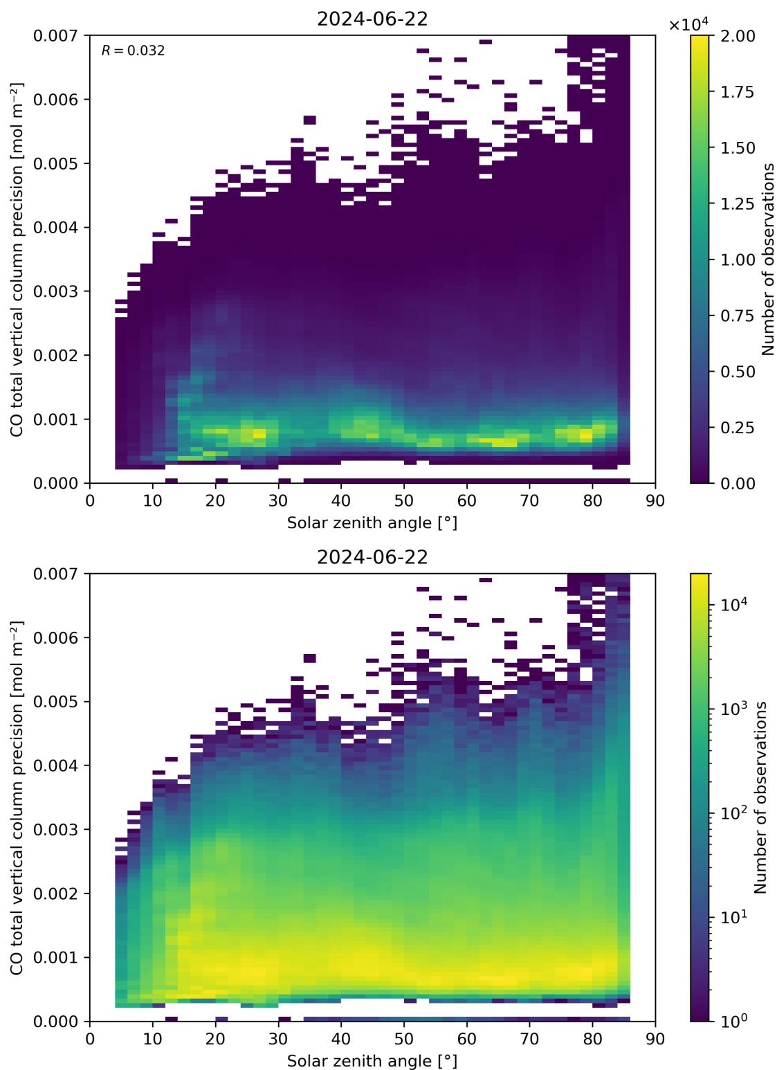
Figure 63: Scatter density plot of “Solar zenith angle” against “CO total vertical column precision” for 2024-06-21 to 2024-06-23.
