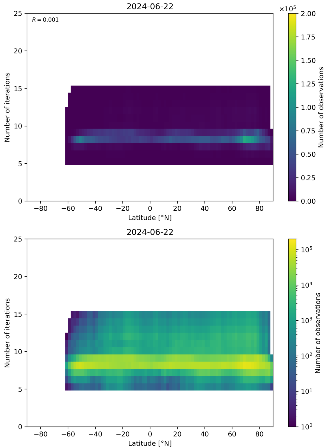
Figure 56: Scatter density plot of “Latitude” against “Number of iterations” for 2024-06-21 to 2024-06-23.
