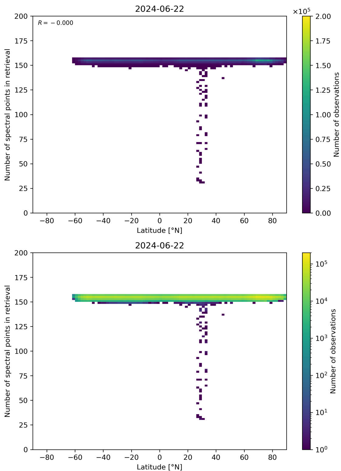
Figure 57: Scatter density plot of “Latitude” against “Number of spectral points in retrieval” for 2024-06-21 to 2024-06-23.
