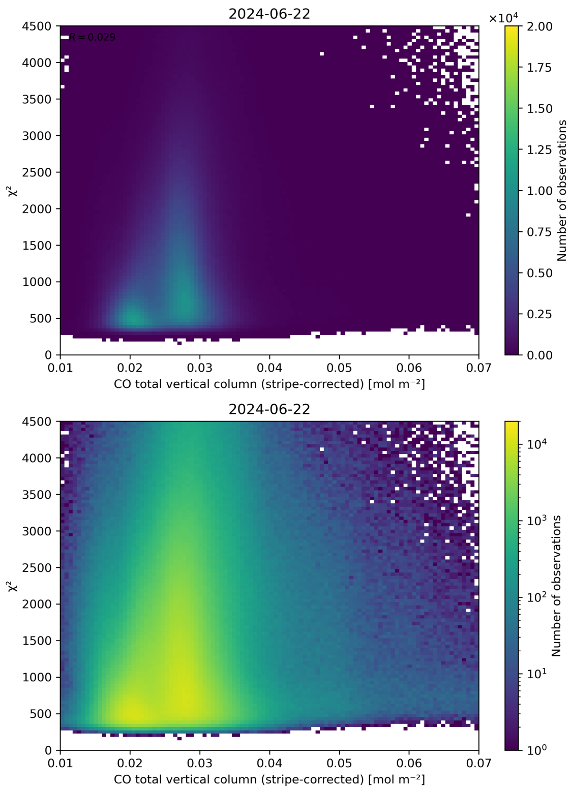
Figure 37: Scatter density plot of “CO total vertical column (stripe-corrected)” against “ \chi^2 ” for 2024-06-21 to 2024-06-23.
