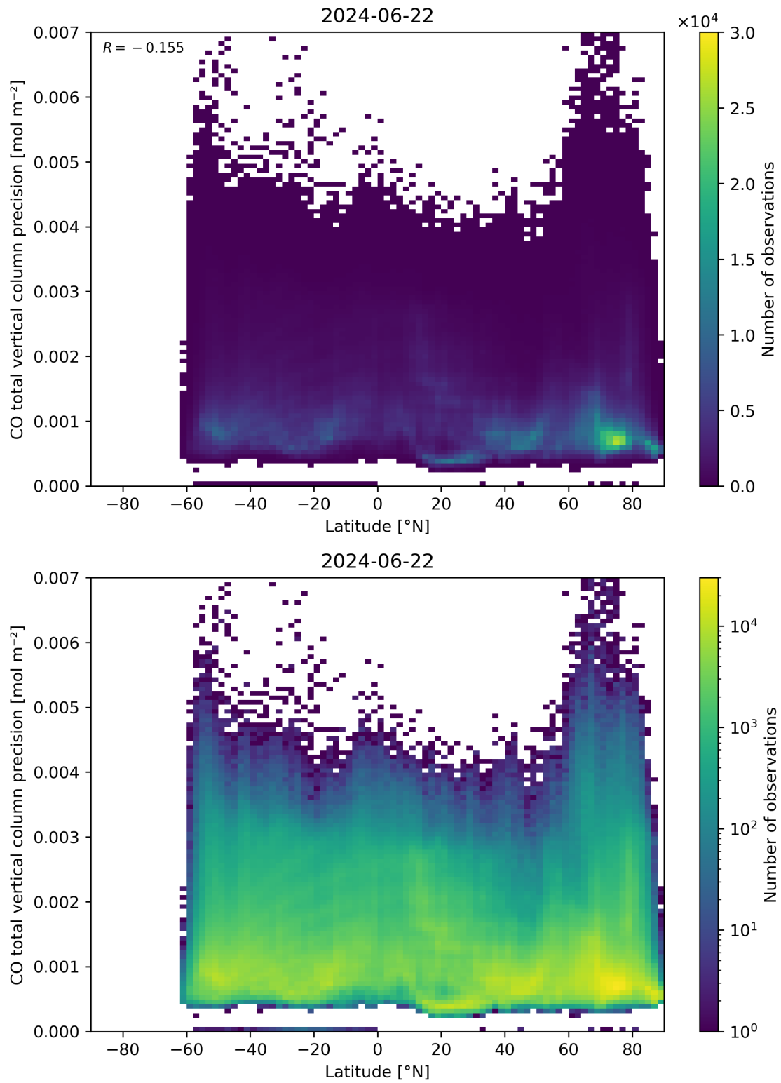
Figure 53: Scatter density plot of “Latitude” against “CO total vertical column precision” for 2024-06-21 to 2024-06-23.
