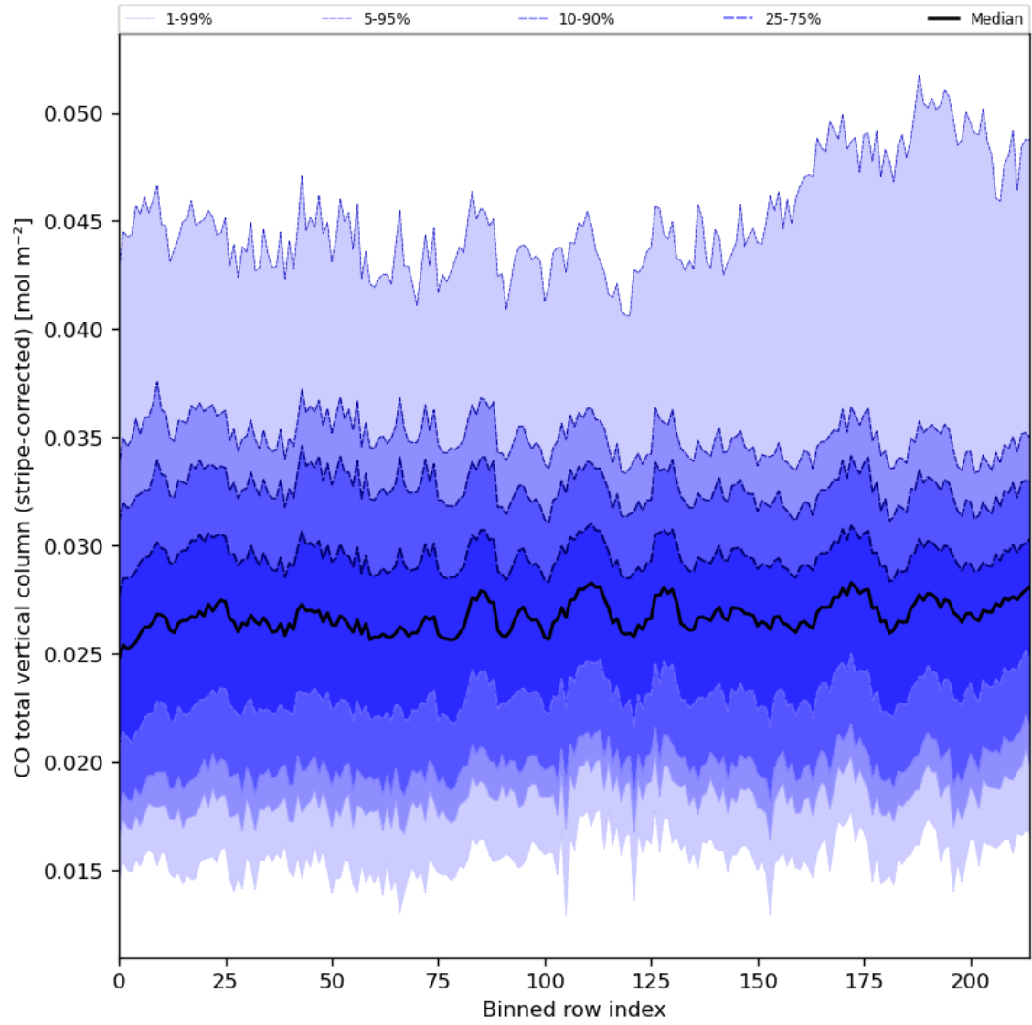
Figure 27: Along track statistics of “CO total vertical column (stripe-corrected)” for 2024-06-21 to 2024-06-23
