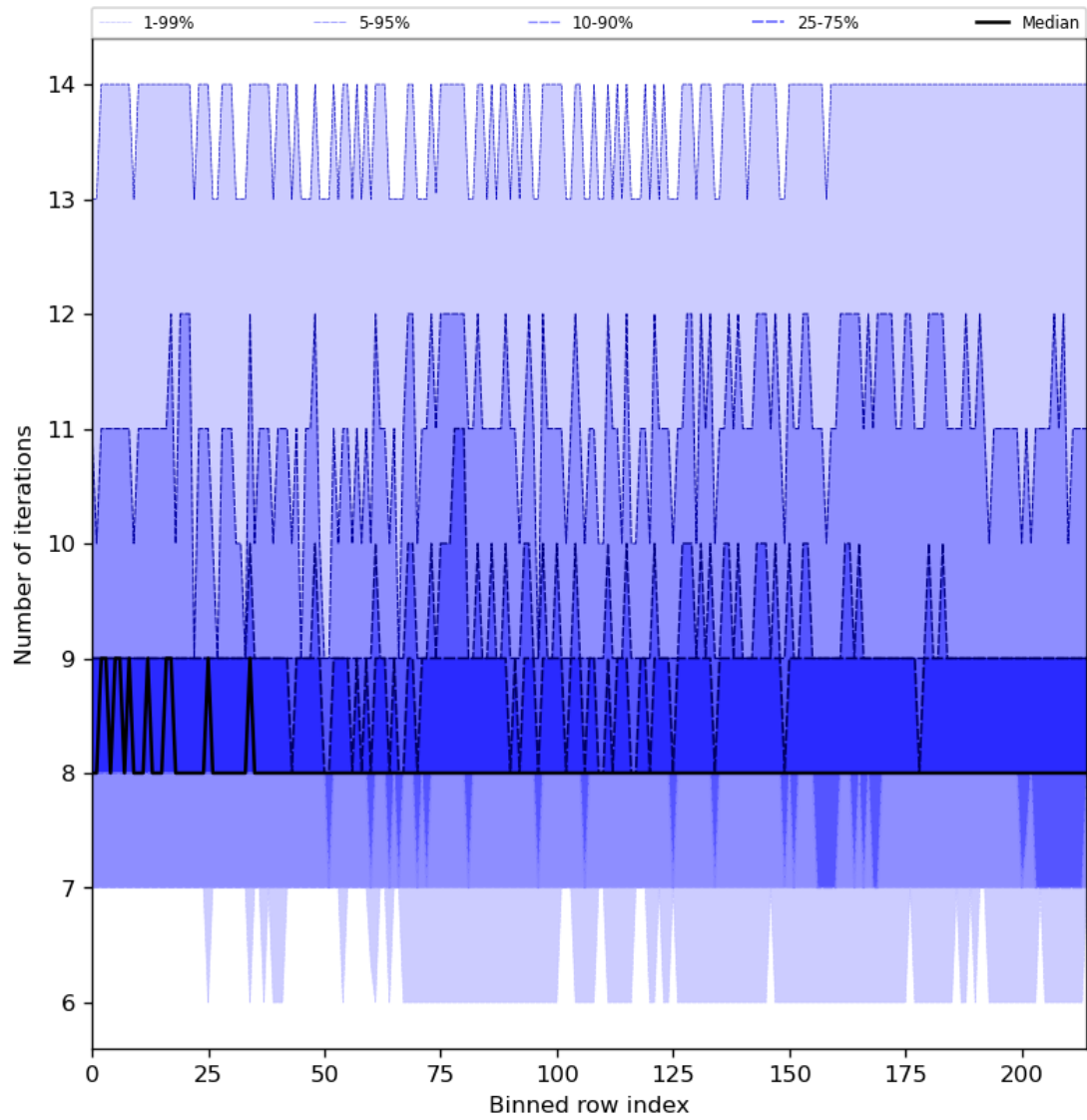
Figure 32: Along track statistics of “Number of iterations” for 2024-06-21 to 2024-06-23
