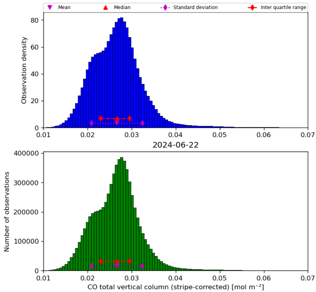
Figure 19: Histogram of “CO total vertical column (stripe-corrected)” for 2024-06-21 to 2024-06-23
