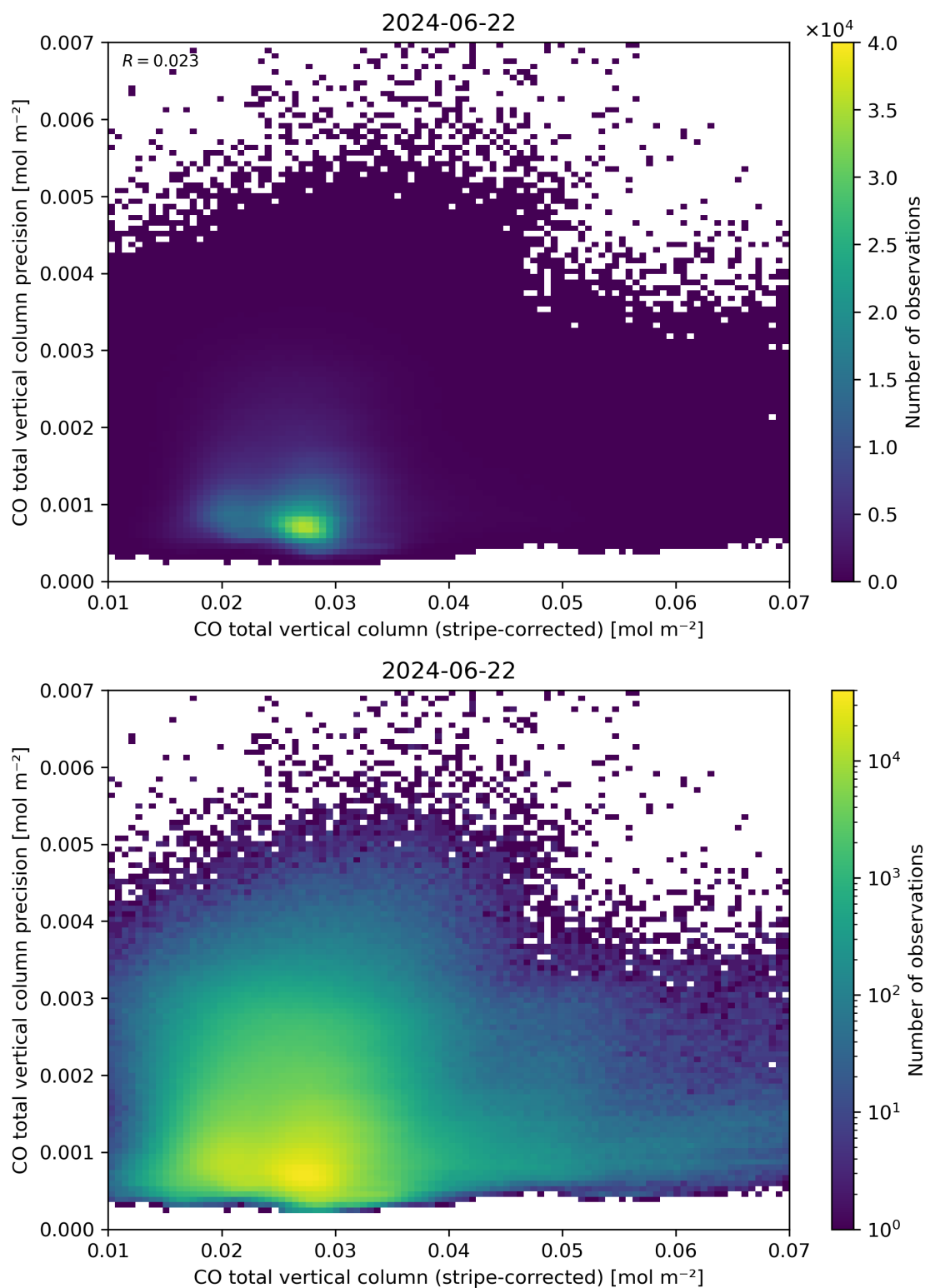
Figure 36: Scatter density plot of “CO total vertical column (stripe-corrected)” against “CO total vertical column precision” for 2024-06-21 to 2024-06-23.
