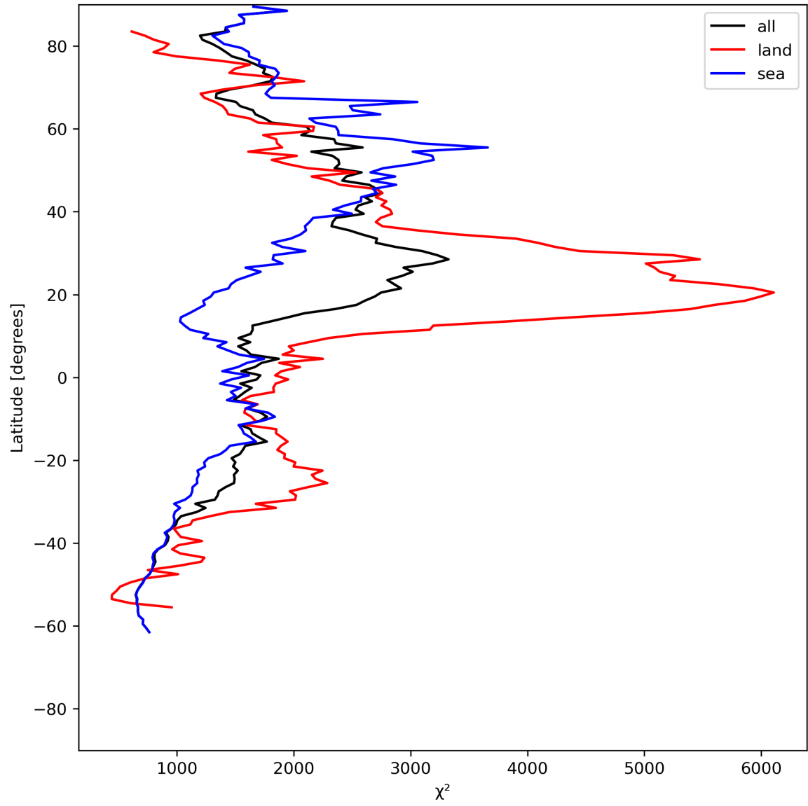
Figure 14: Zonal average of “ \chi^2 ” for 2024-06-22 to 2024-06-24.
