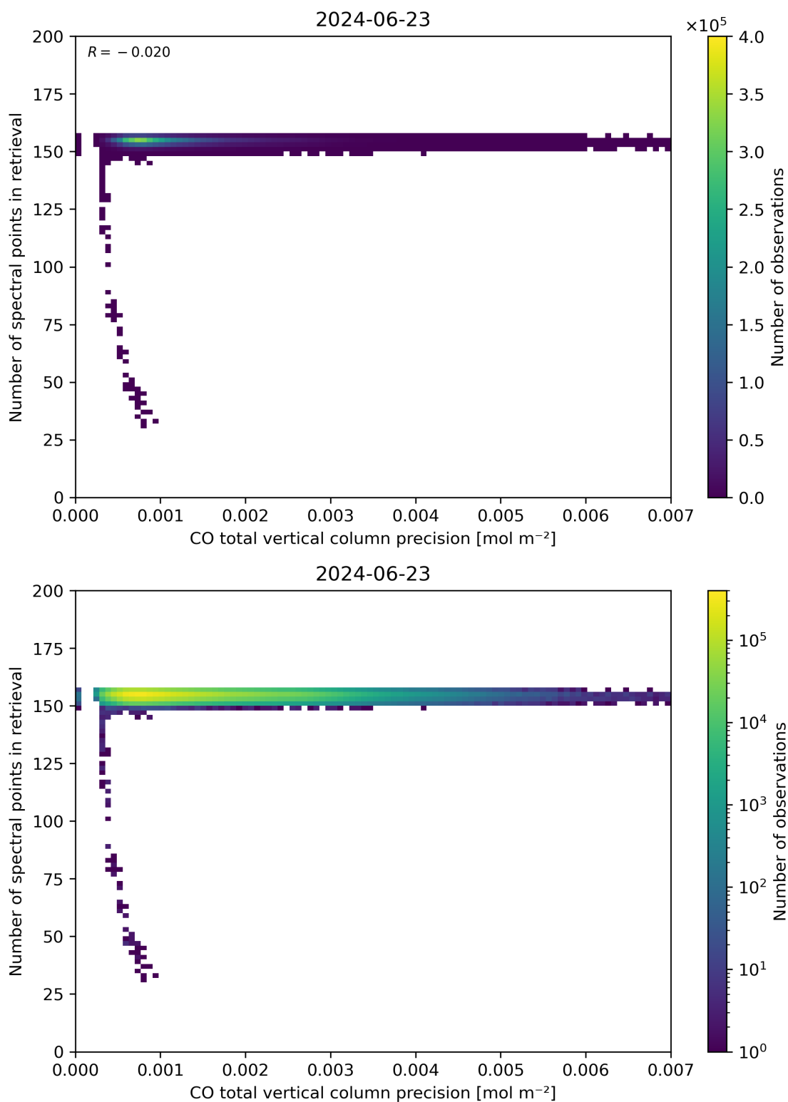
Figure 47: Scatter density plot of “CO total vertical column precision” against “Number of spectral points in retrieval” for 2024-06-22 to 2024-06-24.
