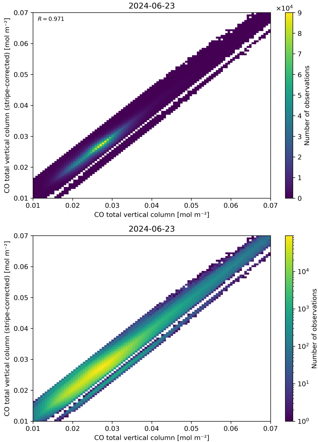
Figure 33: Scatter density plot of “CO total vertical column” against “CO total vertical column (stripe-corrected)” for 2024-06-22 to 2024-06-24.
