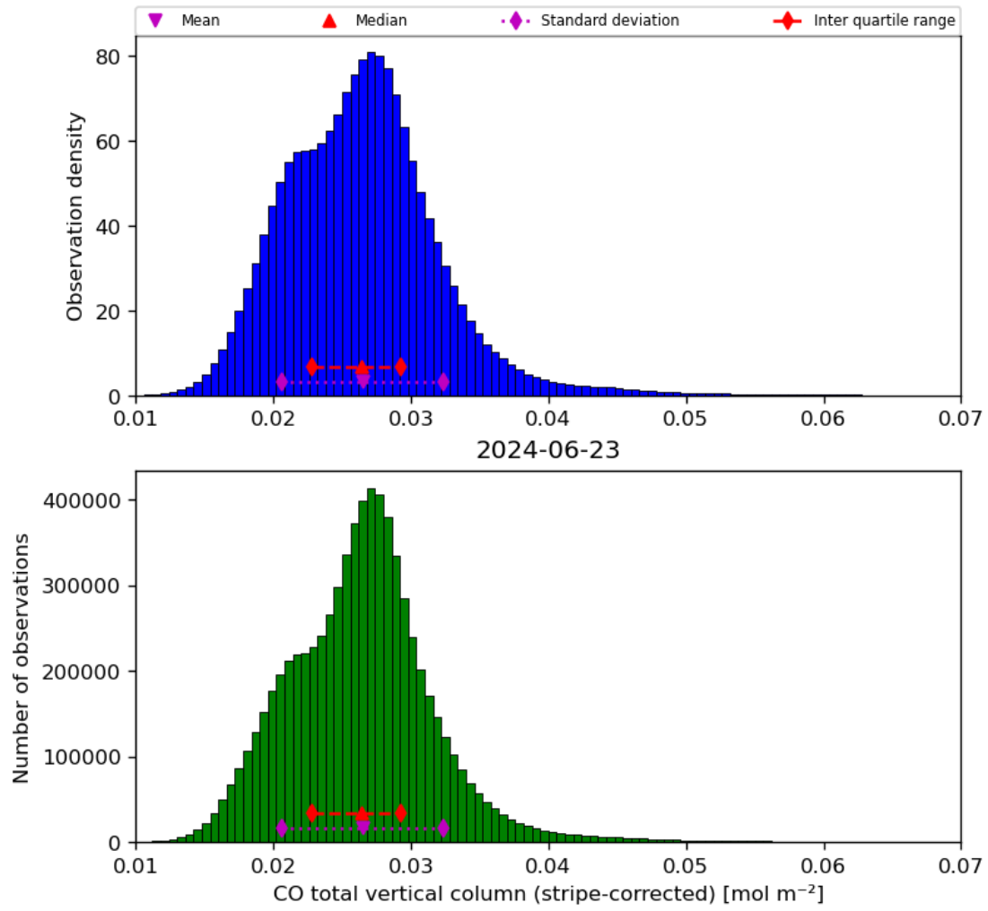
Figure 19: Histogram of “CO total vertical column (stripe-corrected)” for 2024-06-22 to 2024-06-24
