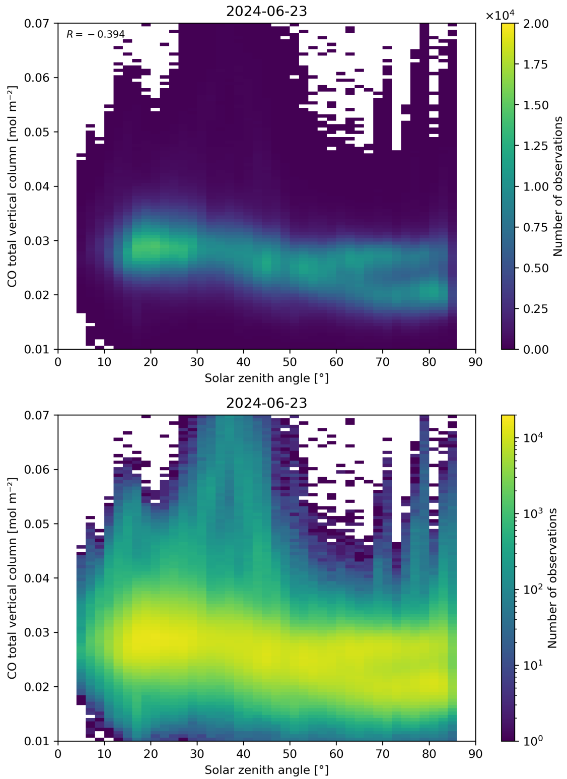
Figure 61: Scatter density plot of “Solar zenith angle” against “CO total vertical column” for 2024-06-22 to 2024-06-24.
