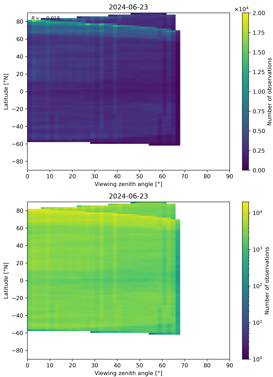
Figure 74: Scatter density plot of “Viewing zenith angle” against “Latitude” for 2024-06-22 to 2024-06-24.
