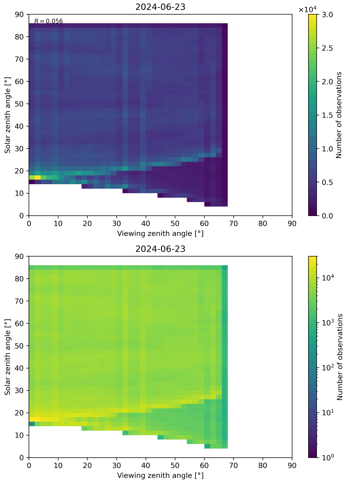
Figure 77: Scatter density plot of “Viewing zenith angle” against “Solar zenith angle” for 2024-06-22 to 2024-06-24.
