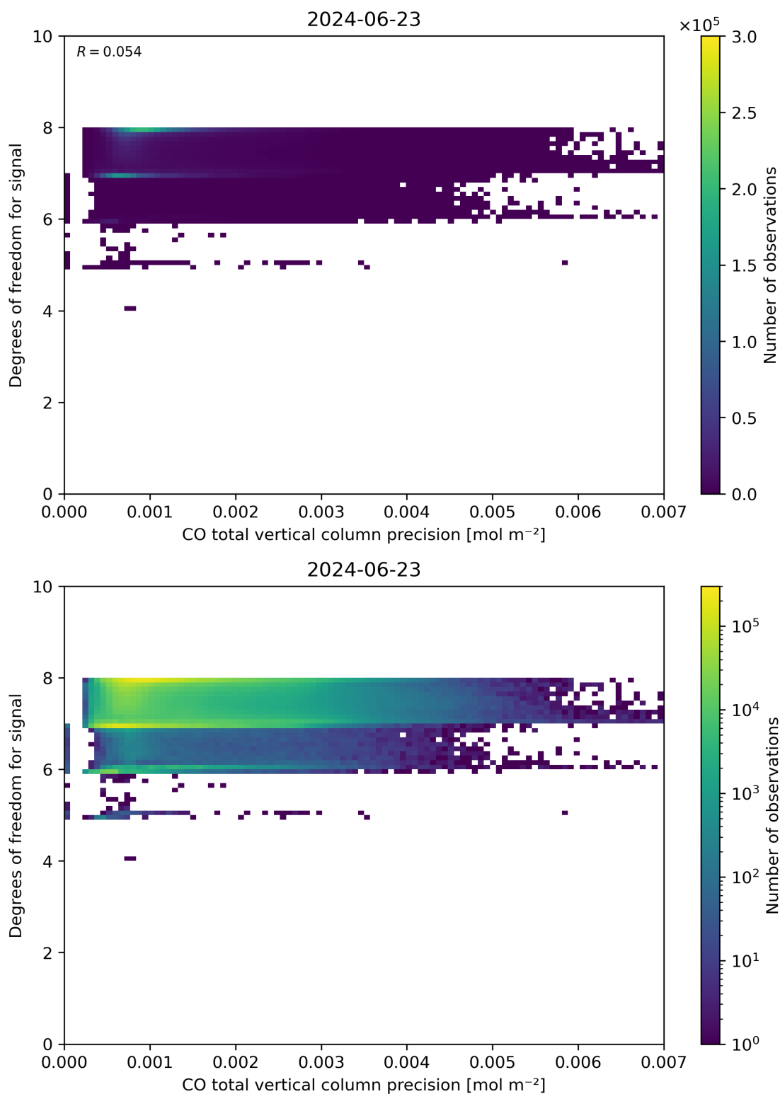
Figure 45: Scatter density plot of “CO total vertical column precision” against “Degrees of freedom for signal” for 2024-06-22 to 2024-06-24.
