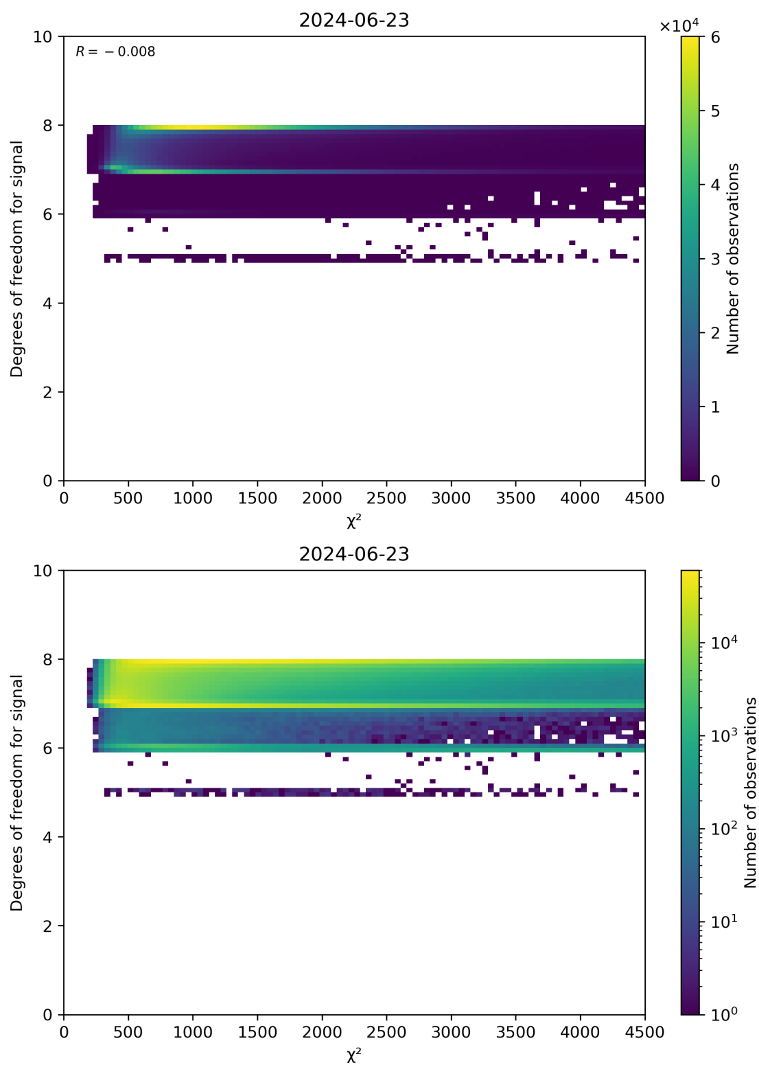
Figure 48: Scatter density plot of “ \chi^2 ” against “Degrees of freedom for signal” for 2024-06-22 to 2024-06-24.
