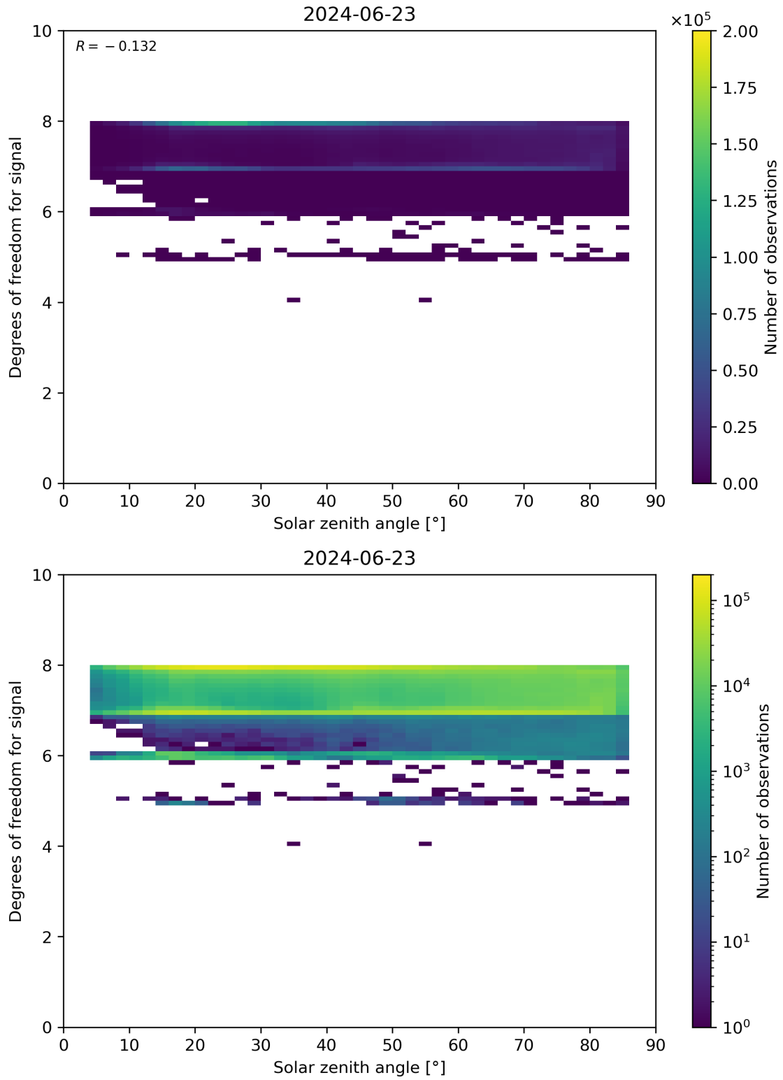
Figure 65: Scatter density plot of “Solar zenith angle” against “Degrees of freedom for signal” for 2024-06-22 to 2024-06-24.
