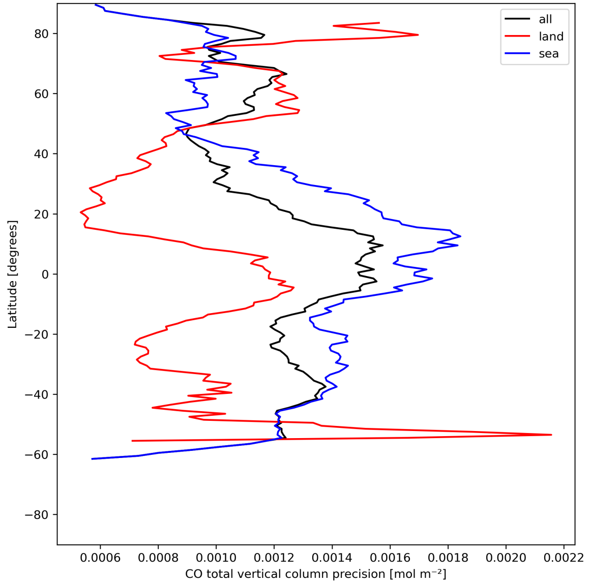
Figure 12: Zonal average of “CO total vertical column precision” for 2024-06-22 to 2024-06-24.
