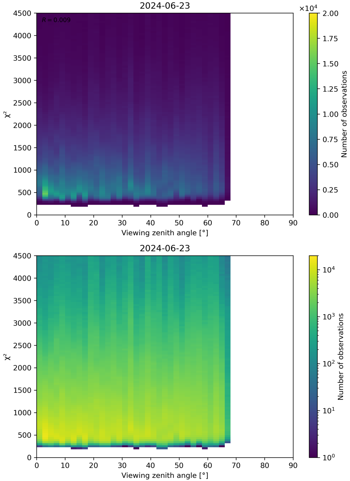
Figure 72: Scatter density plot of “Viewing zenith angle” against “ \chi^2 ” for 2024-06-22 to 2024-06-24.
