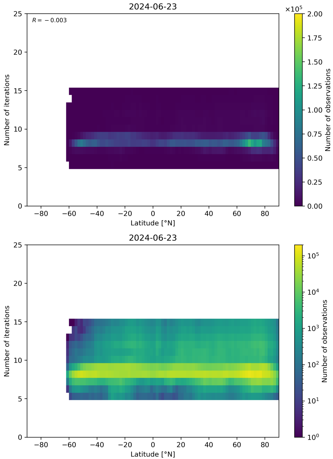
Figure 56: Scatter density plot of “Latitude” against “Number of iterations” for 2024-06-22 to 2024-06-24.
