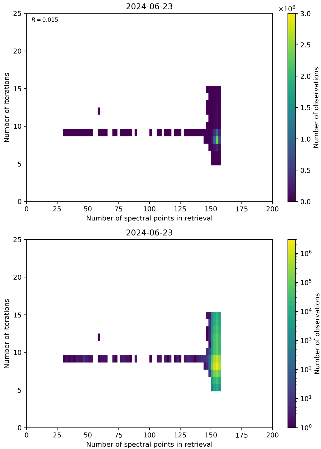
Figure 60: Scatter density plot of “Number of spectral points in retrieval” against “Number of iterations” for 2024-06-22 to 2024-06-24.
