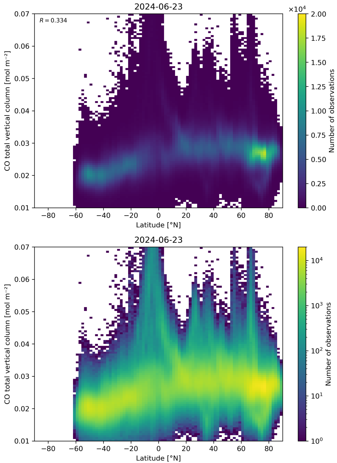
Figure 51: Scatter density plot of “Latitude” against “CO total vertical column” for 2024-06-22 to 2024-06-24.
