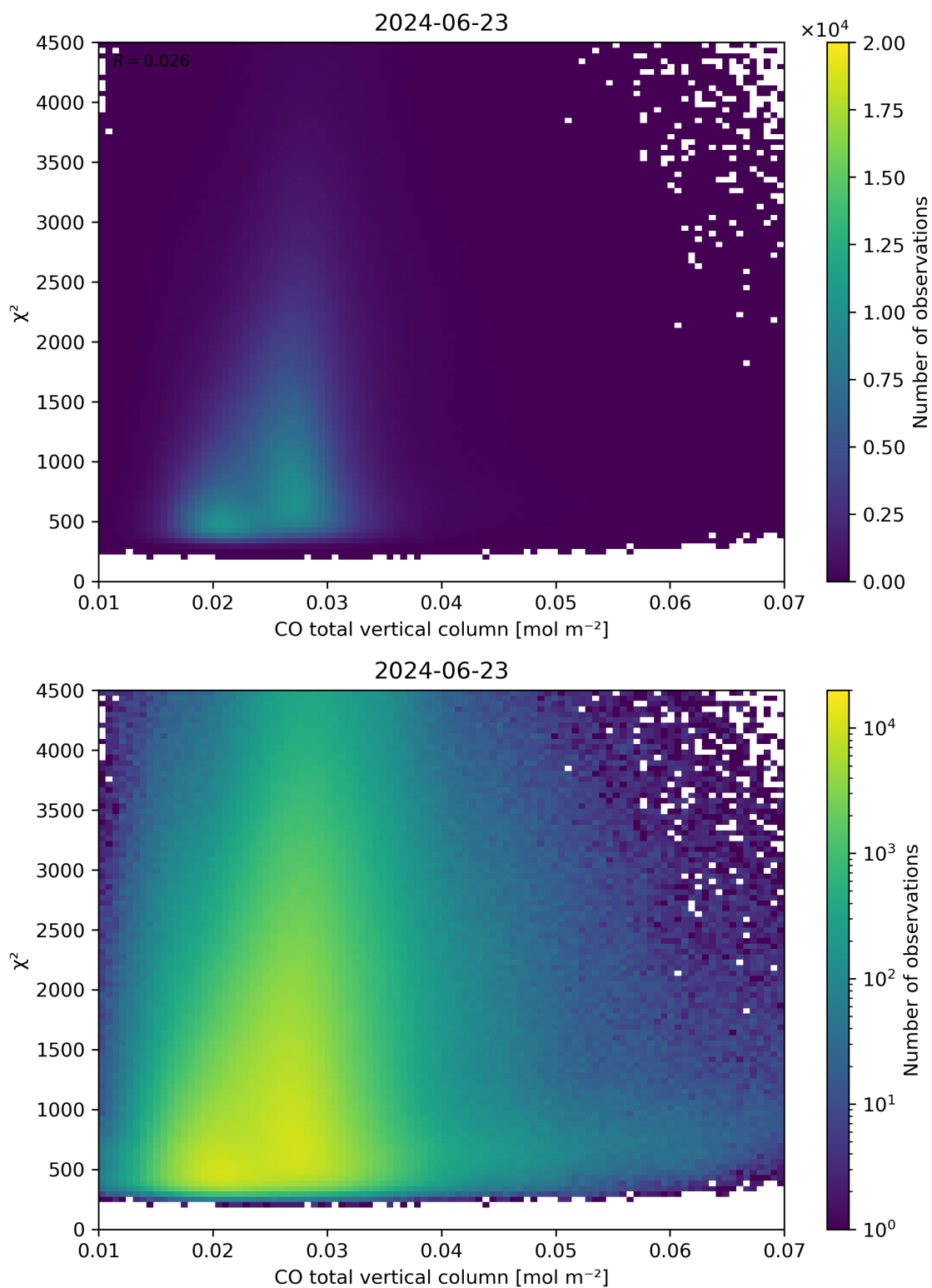
Figure 35: Scatter density plot of “CO total vertical column” against “ \chi^2 ” for 2024-06-22 to 2024-06-24.
