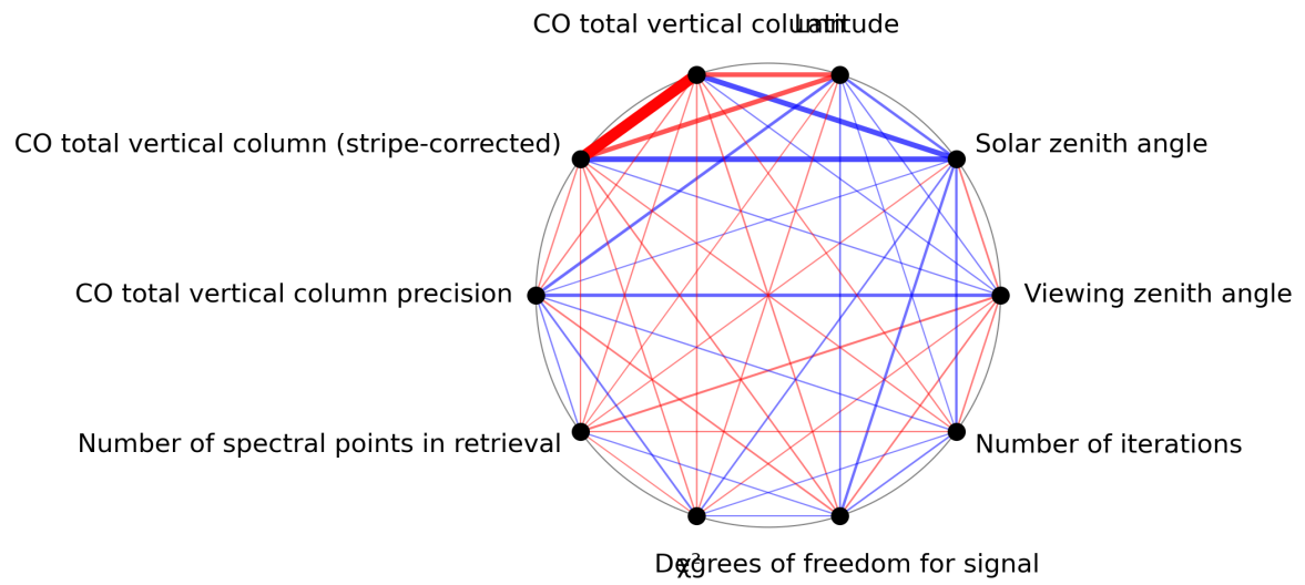
Figure 1: Map of correlation graph for 2024-06-22 to 2024-06-24.
