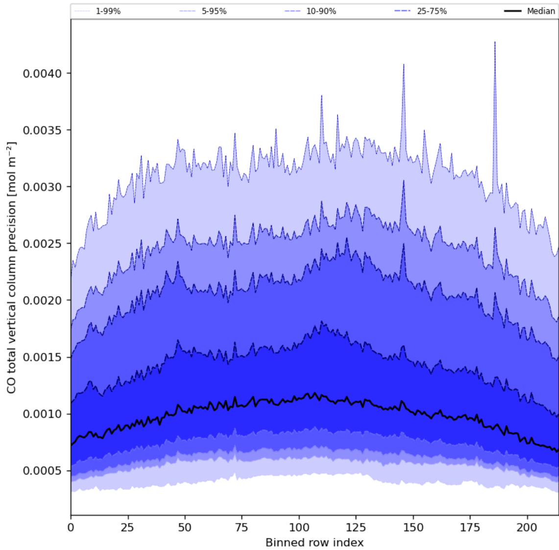
Figure 28: Along track statistics of “CO total vertical column precision” for 2024-06-22 to 2024-06-24
