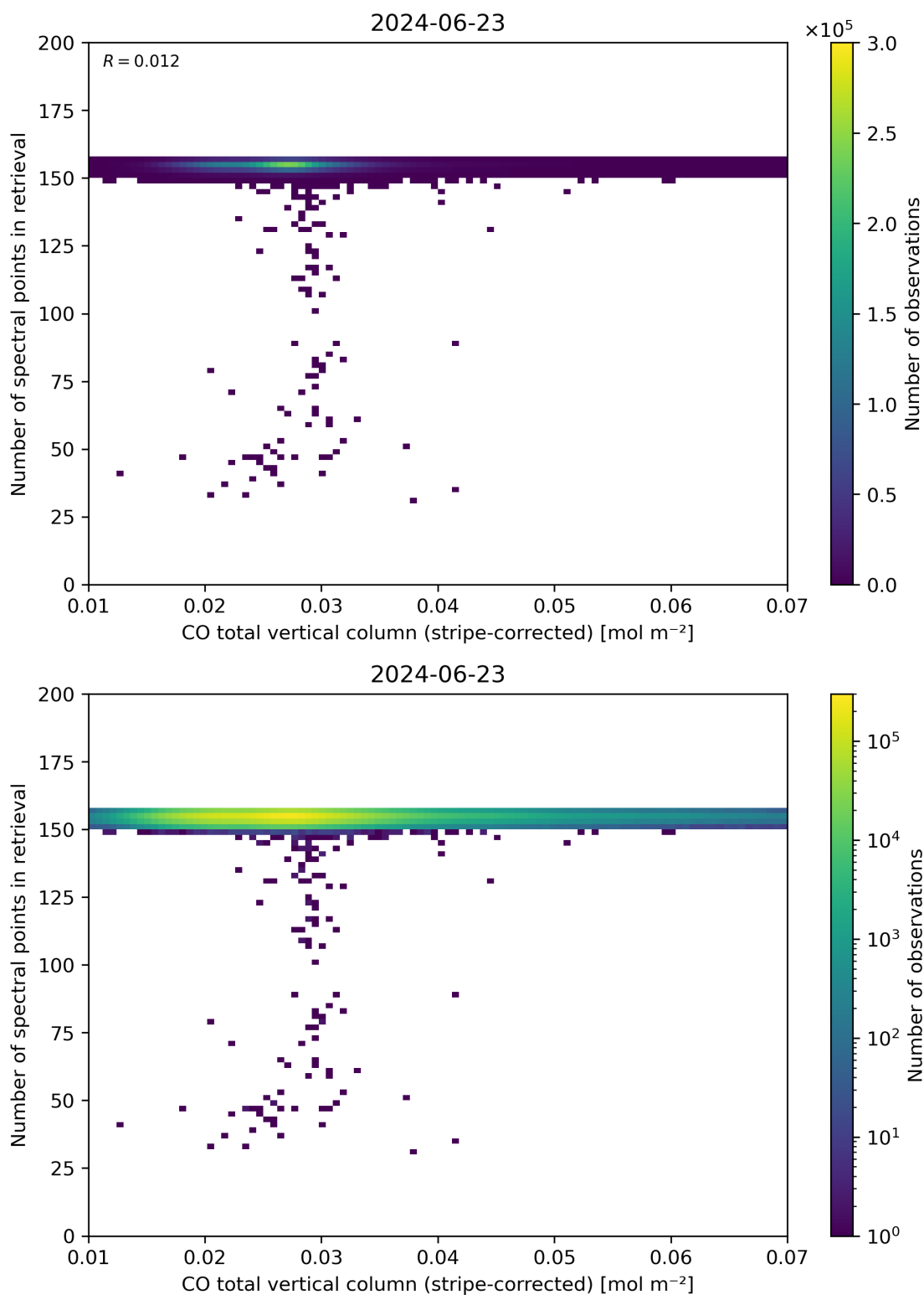
Figure 40: Scatter density plot of “CO total vertical column (stripe-corrected)” against “Number of spectral points in retrieval” for 2024-06-22 to 2024-06-24.
