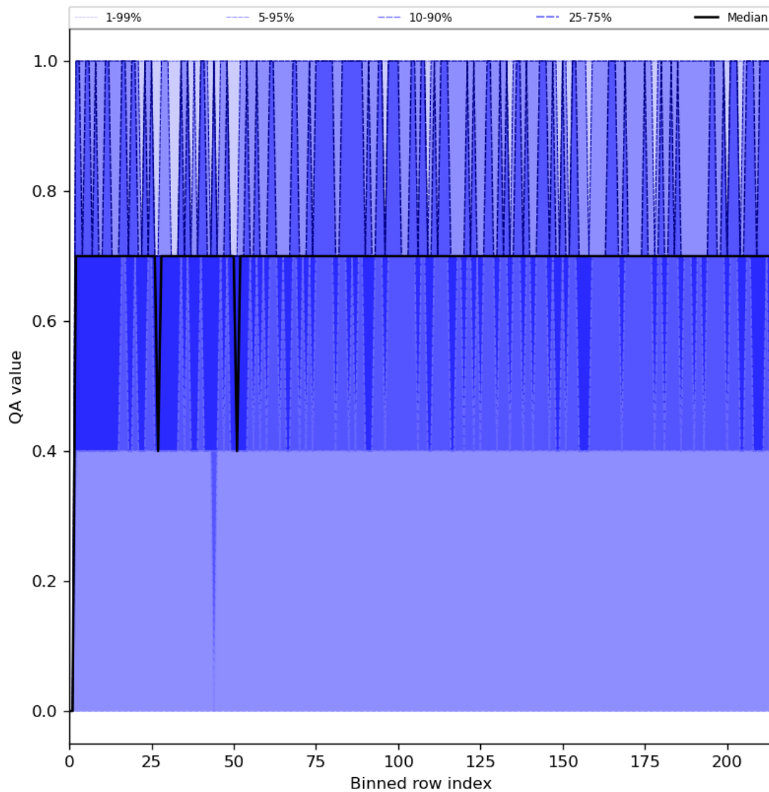
Figure 25: Along track statistics of “QA value” for 2024-06-22 to 2024-06-24
