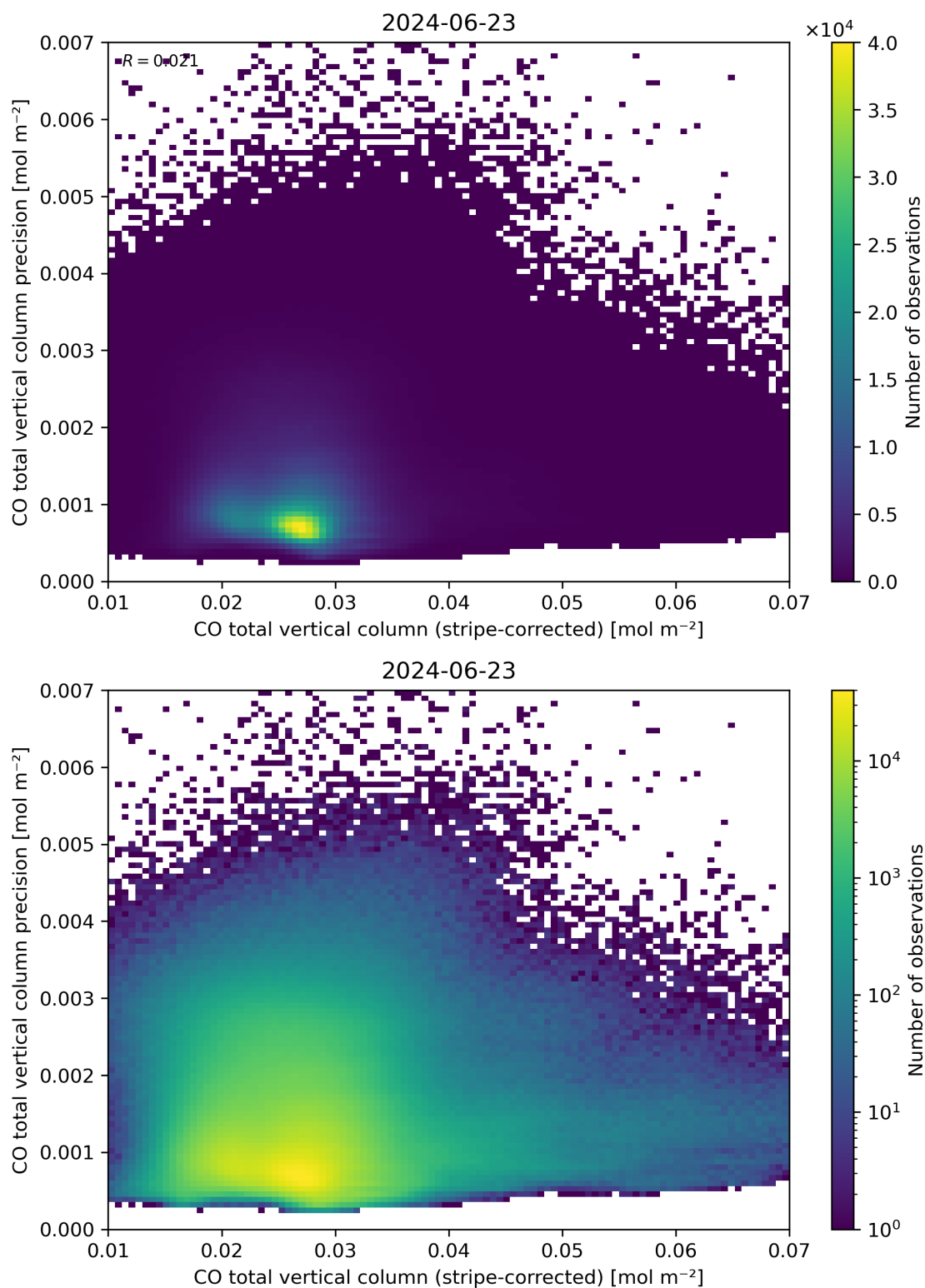
Figure 36: Scatter density plot of “CO total vertical column (stripe-corrected)” against “CO total vertical column precision” for 2024-06-22 to 2024-06-24.
