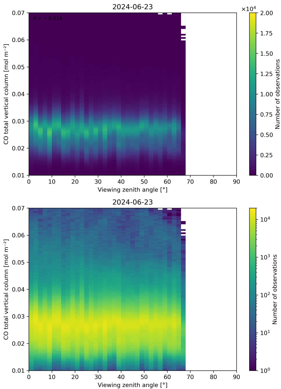
Figure 69: Scatter density plot of “Viewing zenith angle” against “CO total vertical column” for 2024-06-22 to 2024-06-24.
