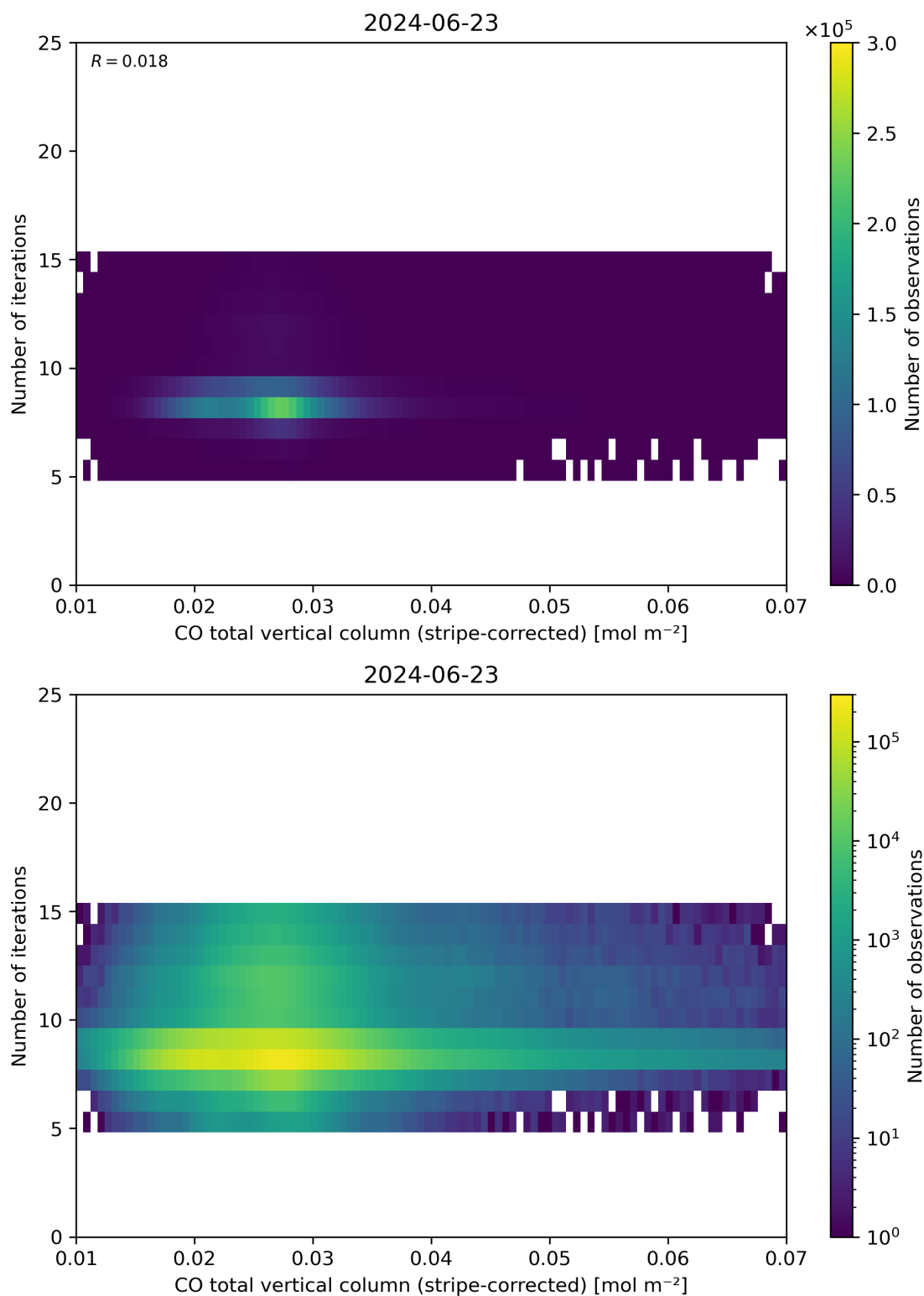
Figure 39: Scatter density plot of “CO total vertical column (stripe-corrected)” against “Number of iterations” for 2024-06-22 to 2024-06-24.
