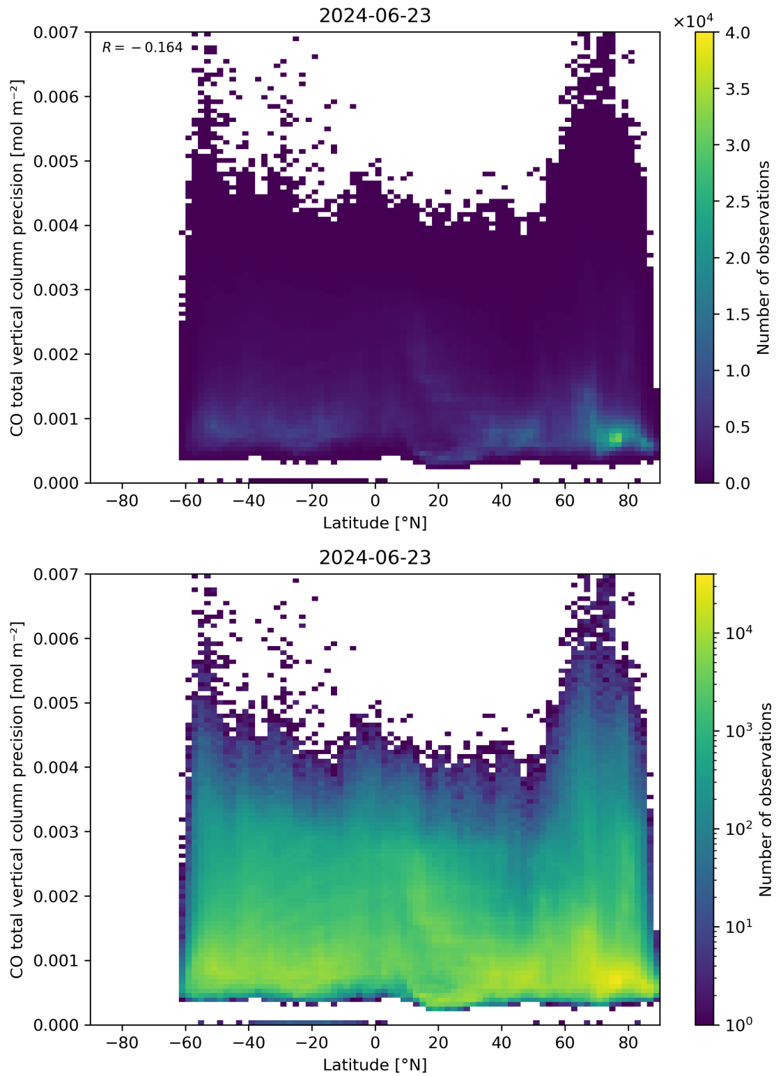
Figure 53: Scatter density plot of “Latitude” against “CO total vertical column precision” for 2024-06-22 to 2024-06-24.
