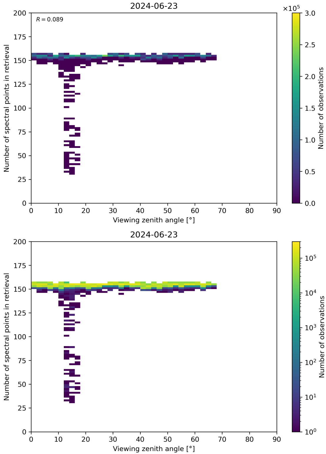
Figure 76: Scatter density plot of “Viewing zenith angle” against “Number of spectral points in retrieval” for 2024-06-22 to 2024-06-24.
