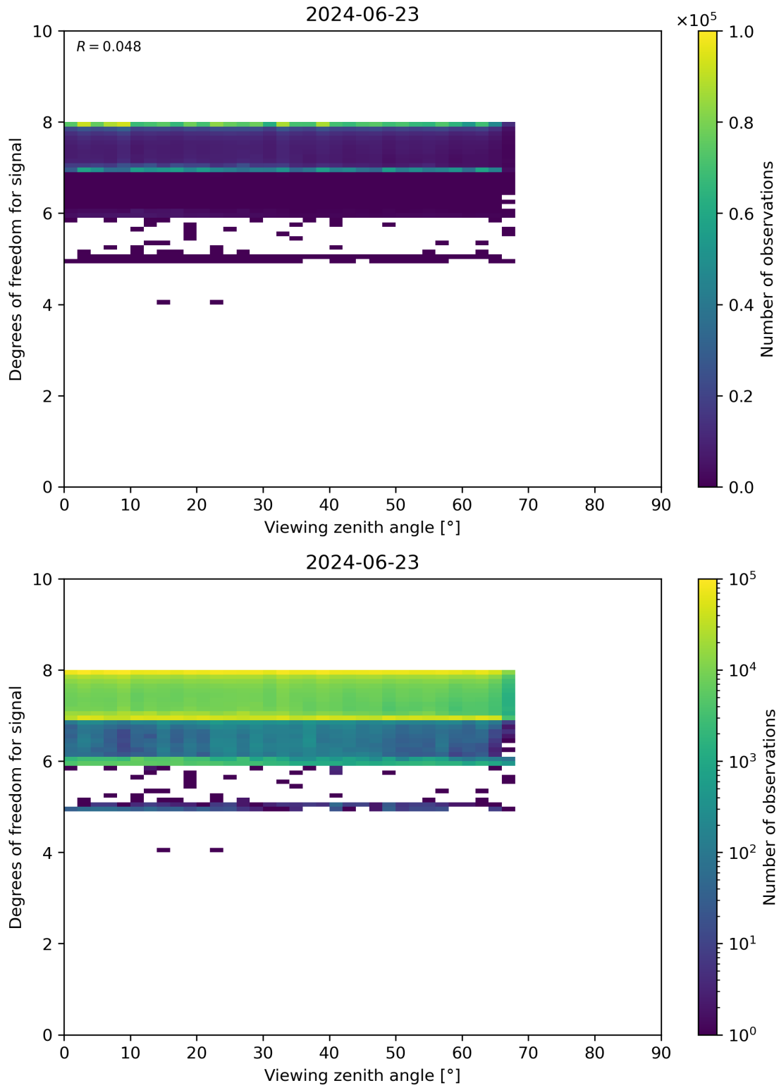
Figure 73: Scatter density plot of “Viewing zenith angle” against “Degrees of freedom for signal” for 2024-06-22 to 2024-06-24.
