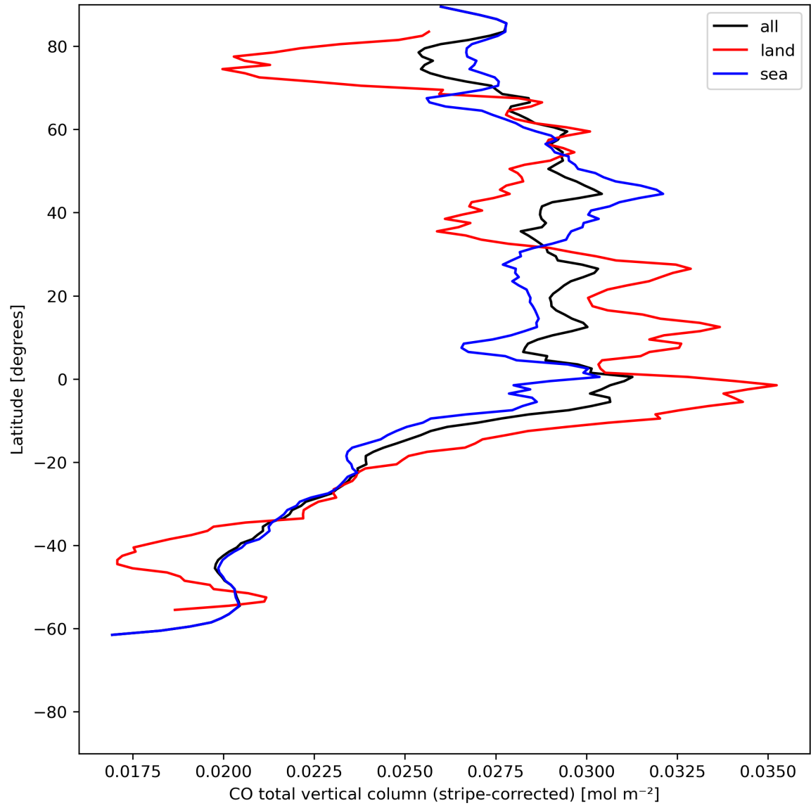
Figure 11: Zonal average of “CO total vertical column (stripe-corrected)” for 2024-06-22 to 2024-06-24.
