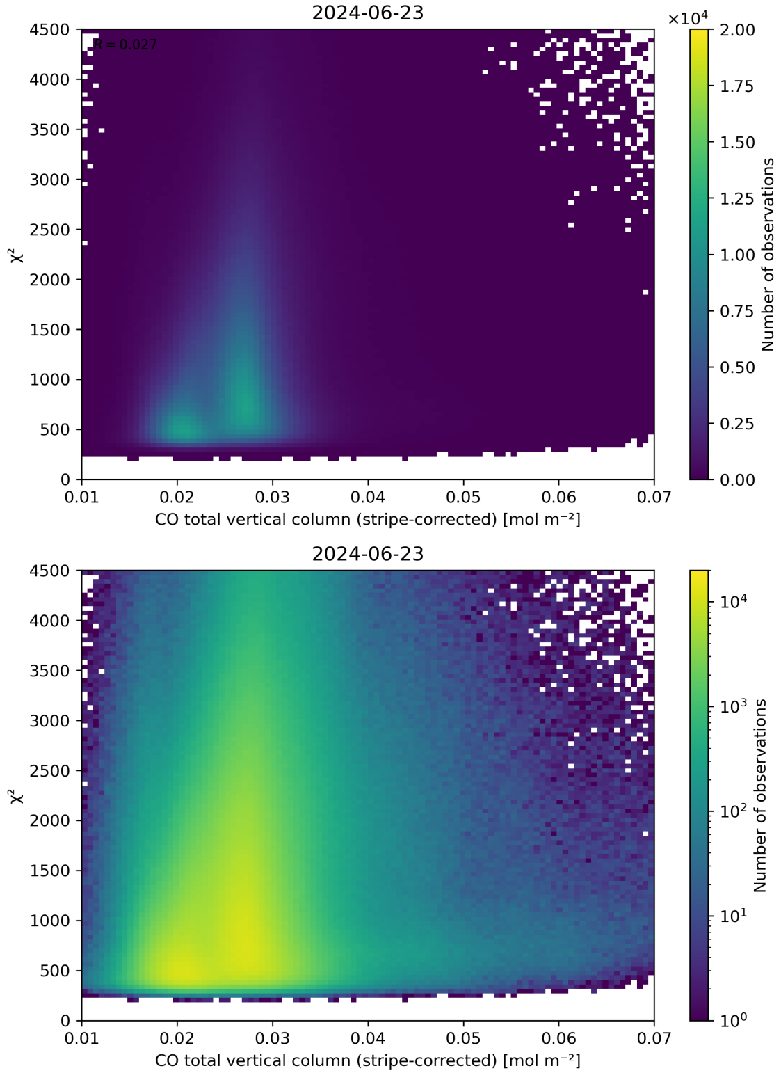
Figure 37: Scatter density plot of “CO total vertical column (stripe-corrected)” against “ \chi^2 ” for 2024-06-22 to 2024-06-24.
