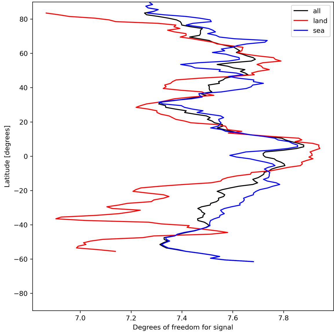
Figure 15: Zonal average of “Degrees of freedom for signal” for 2024-06-22 to 2024-06-24.
