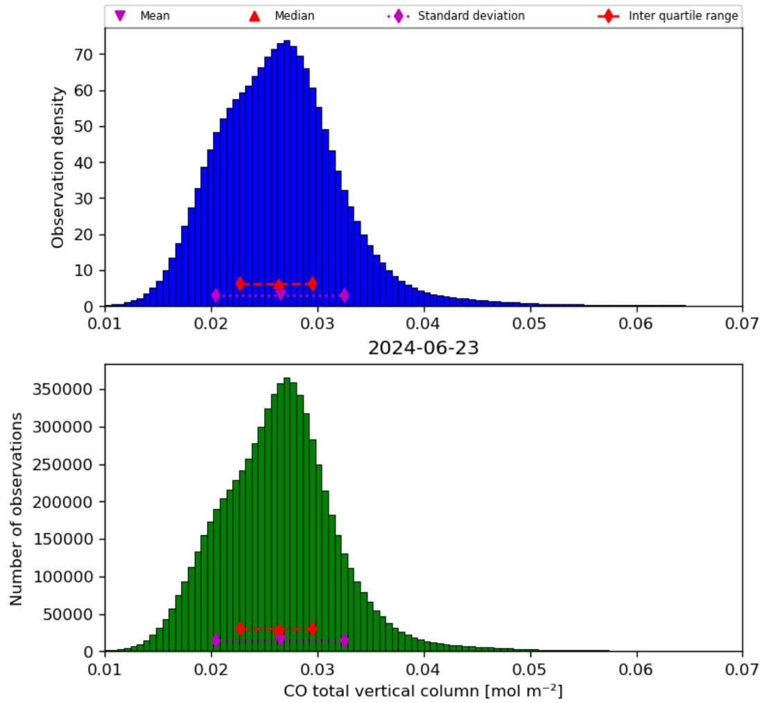
Figure 18: Histogram of “CO total vertical column” for 2024-06-22 to 2024-06-24
