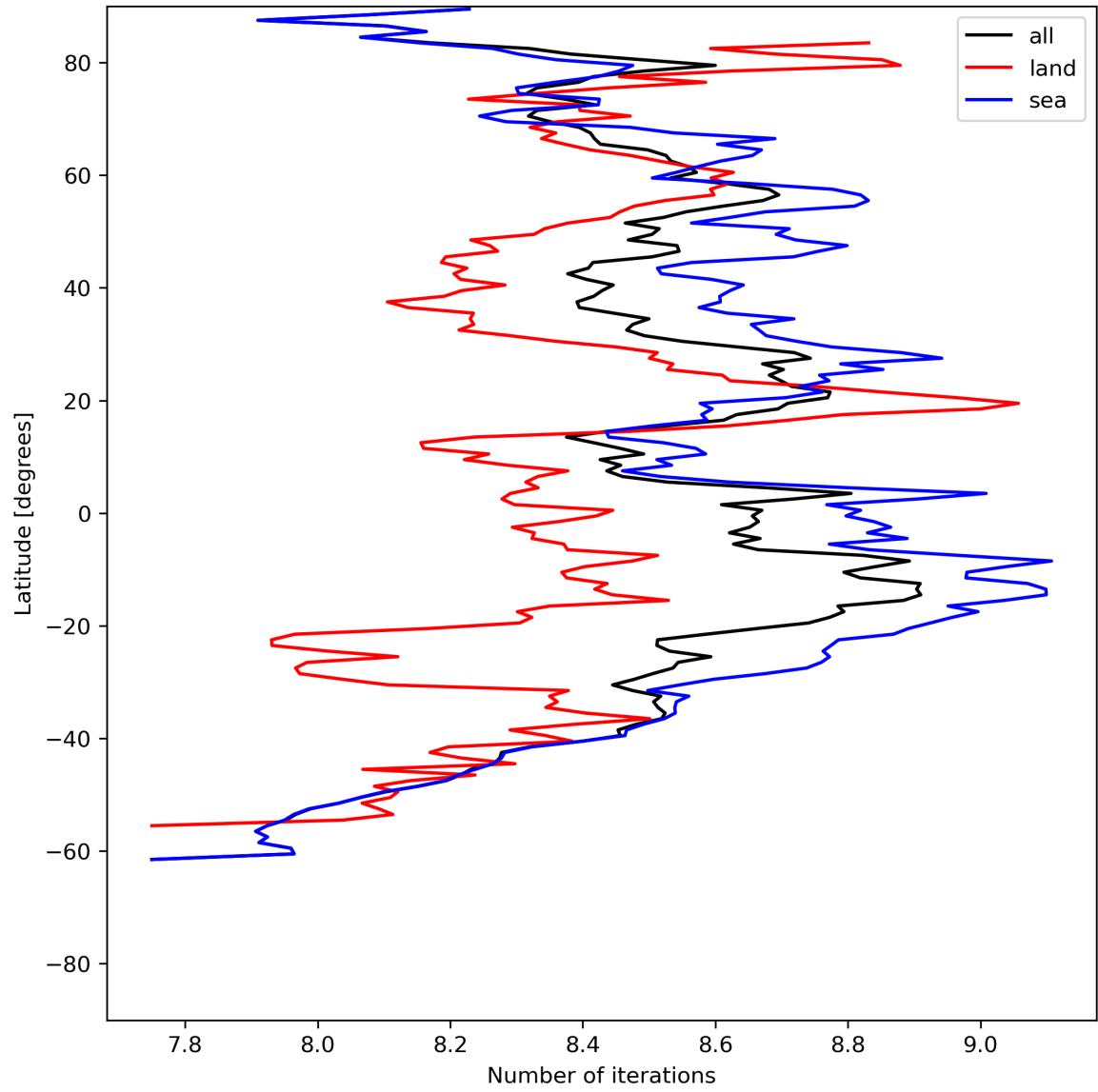
Figure 16: Zonal average of “Number of iterations” for 2024-06-22 to 2024-06-24.
