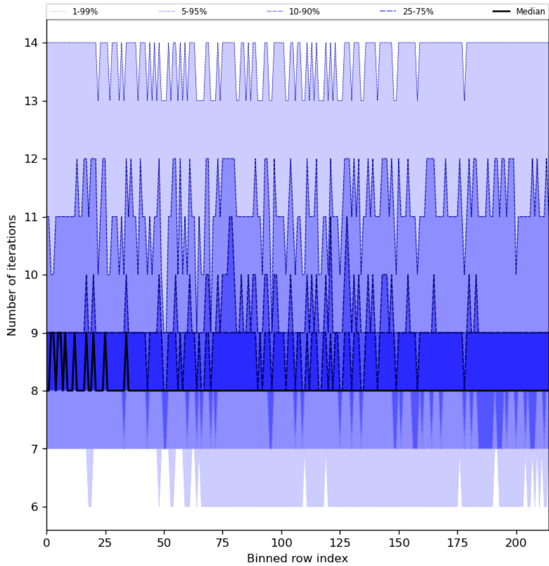
Figure 32: Along track statistics of “Number of iterations” for 2024-06-22 to 2024-06-24
