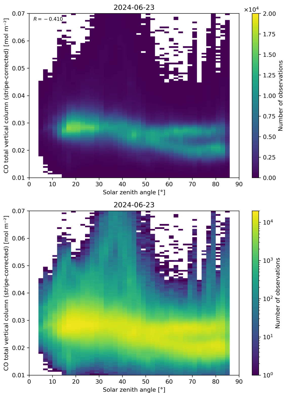
Figure 62: Scatter density plot of “Solar zenith angle” against “CO total vertical column (stripe-corrected)” for 2024-06-22 to 2024-06-24.
