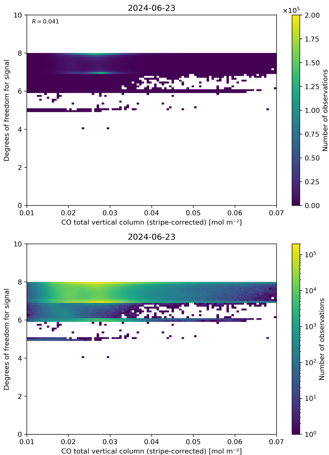
Figure 38: Scatter density plot of “CO total vertical column (stripe-corrected)” against “Degrees of freedom for signal” for 2024-06-22 to 2024-06-24.
