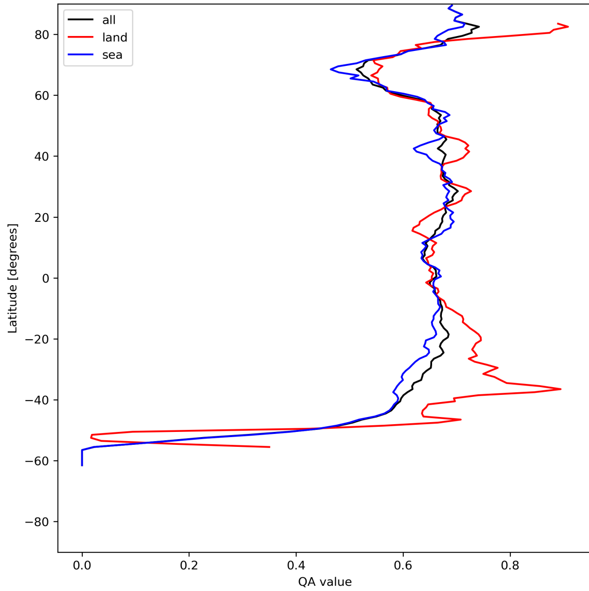
Figure 9: Zonal average of “QA value” for 2024-06-22 to 2024-06-24.
