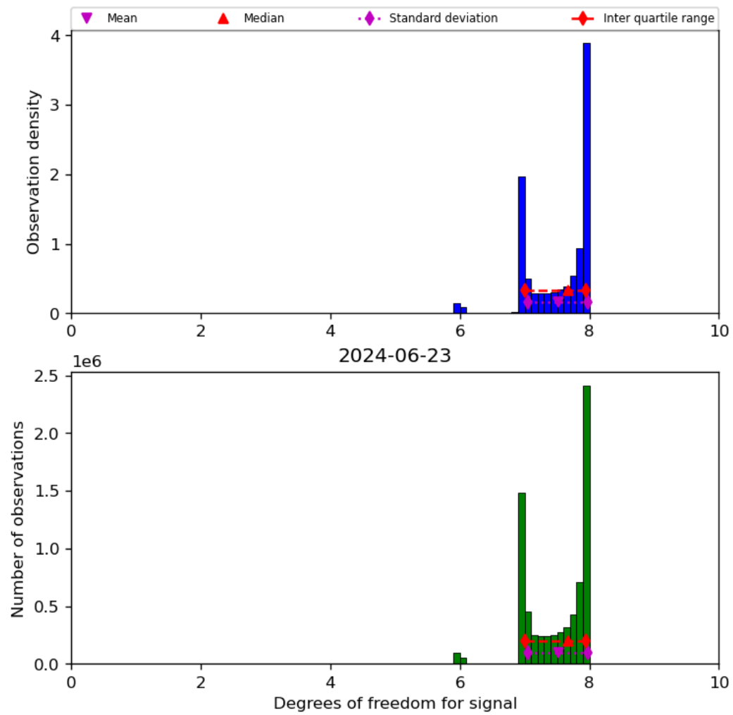
Figure 23: Histogram of “Degrees of freedom for signal” for 2024-06-22 to 2024-06-24
