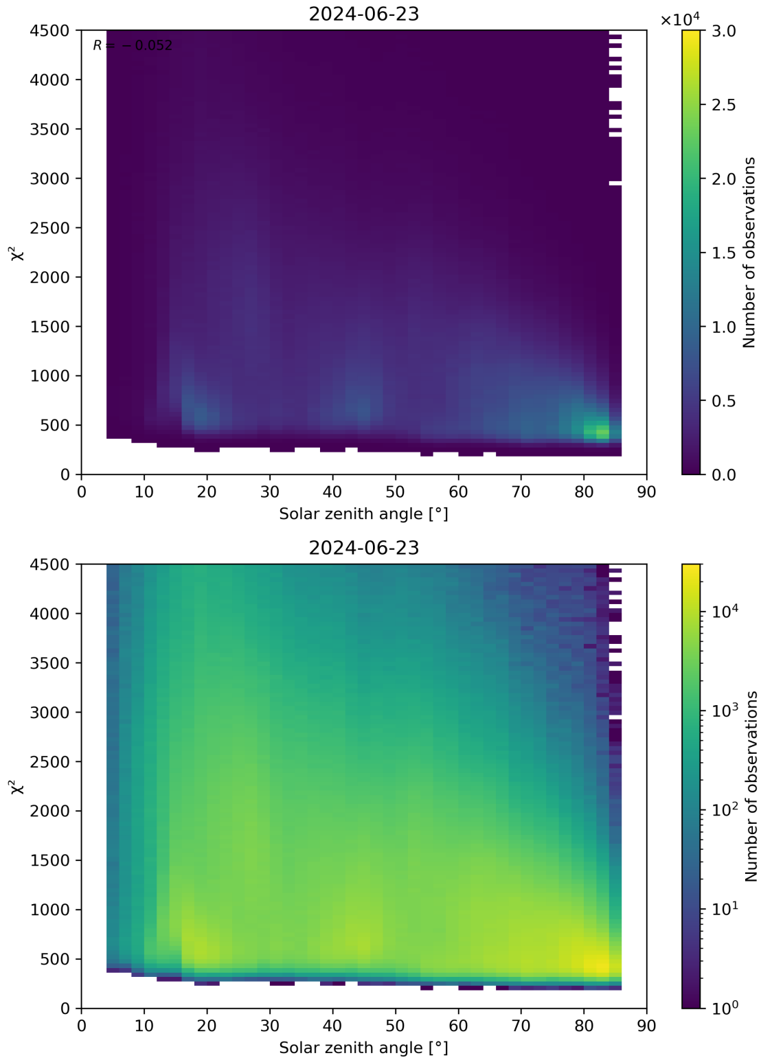
Figure 64: Scatter density plot of “Solar zenith angle” against “ \chi^2 ” for 2024-06-22 to 2024-06-24.
