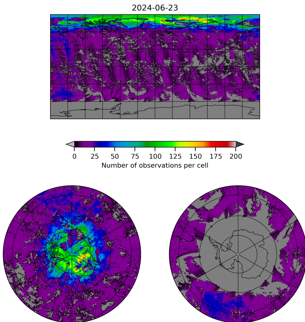
Figure 8: Map of the number of observations for 2024-06-22 to 2024-06-24
