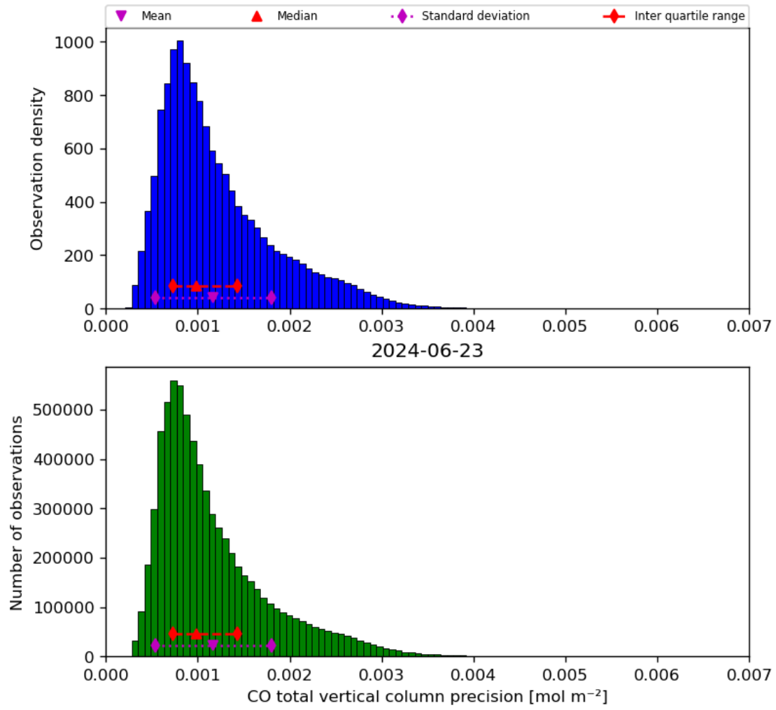
Figure 20: Histogram of “CO total vertical column precision” for 2024-06-22 to 2024-06-24
