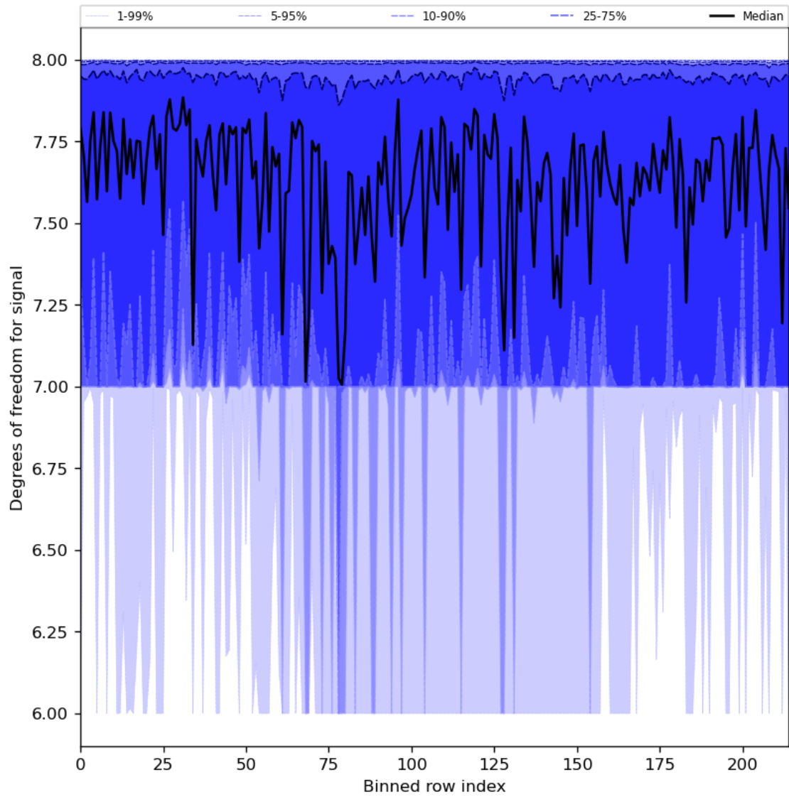
Figure 31: Along track statistics of “Degrees of freedom for signal” for 2024-06-22 to 2024-06-24
