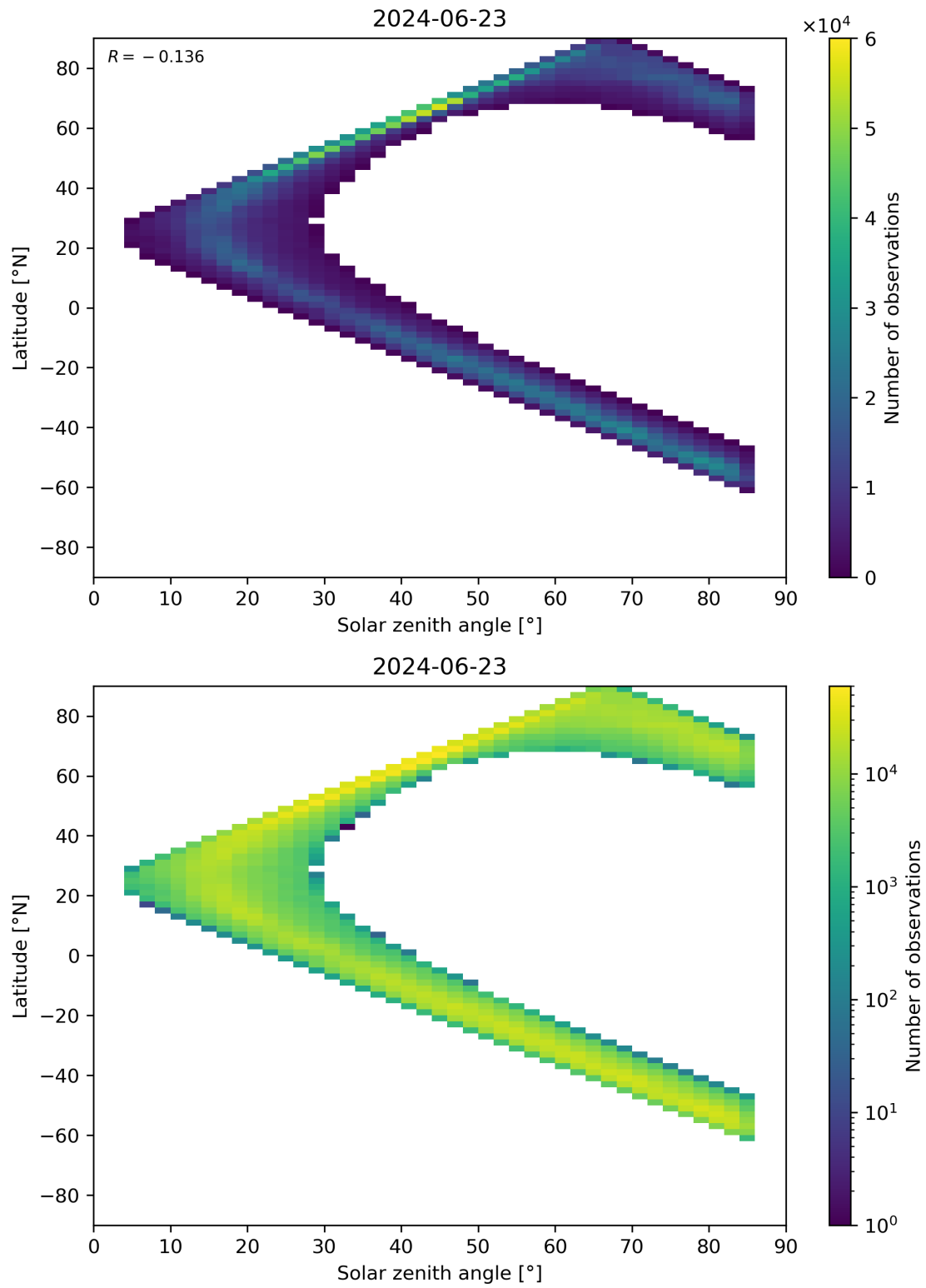
Figure 66: Scatter density plot of “Solar zenith angle” against “Latitude” for 2024-06-22 to 2024-06-24.
