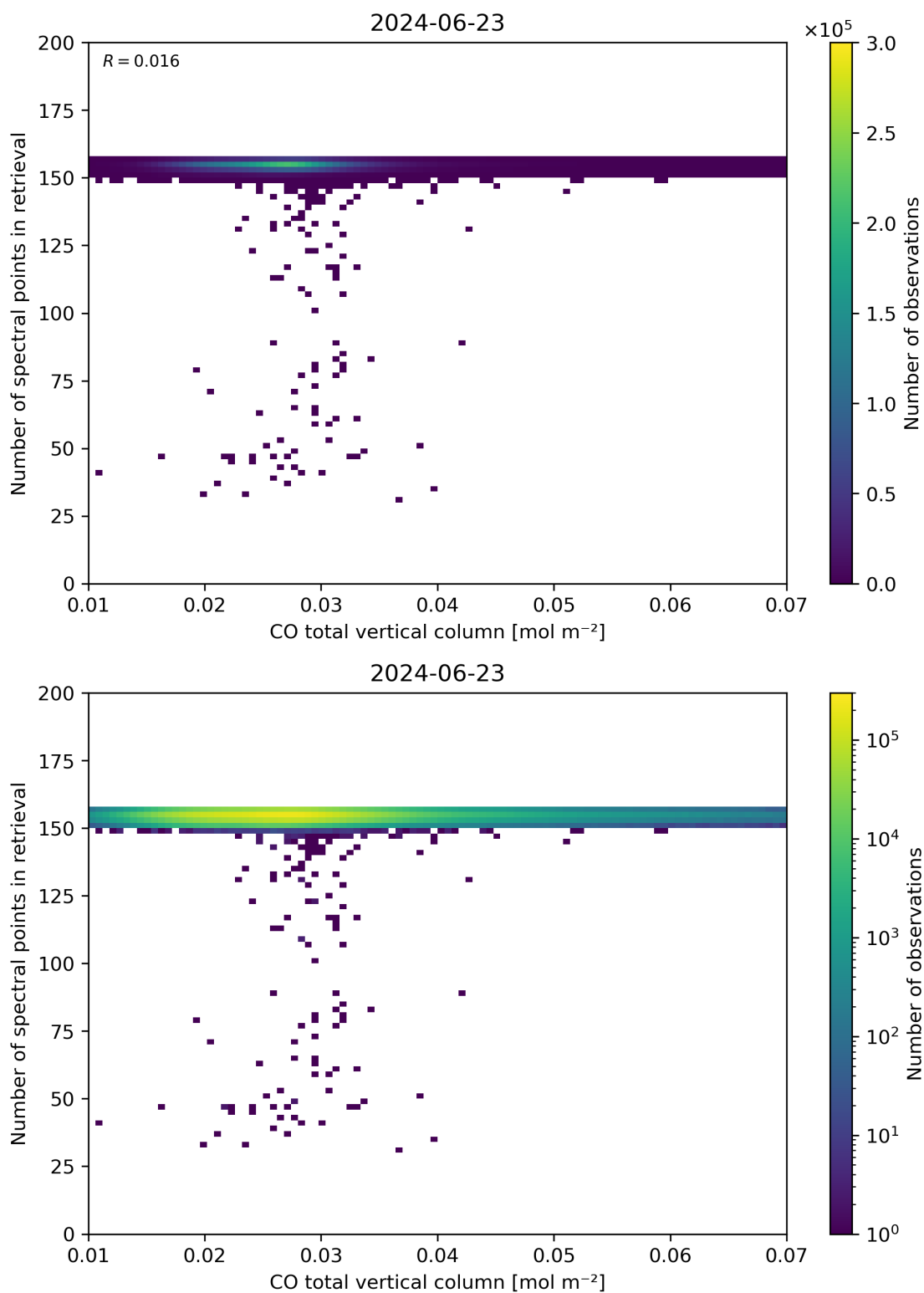
Figure 43: Scatter density plot of “CO total vertical column” against “Number of spectral points in retrieval” for 2024-06-22 to 2024-06-24.
