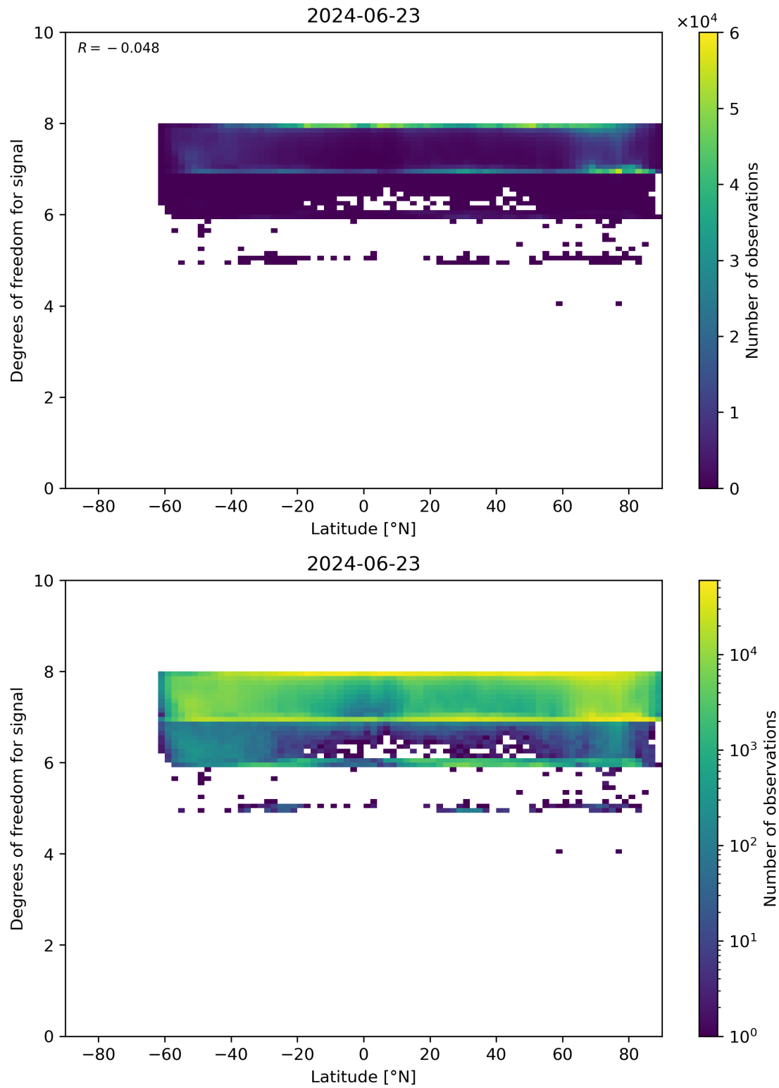
Figure 55: Scatter density plot of “Latitude” against “Degrees of freedom for signal” for 2024-06-22 to 2024-06-24.
