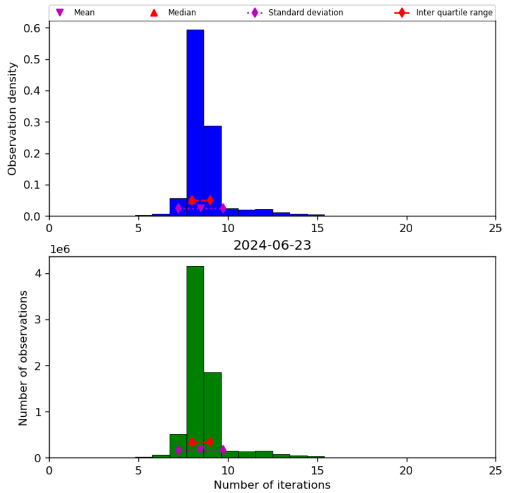
Figure 24: Histogram of “Number of iterations” for 2024-06-22 to 2024-06-24
