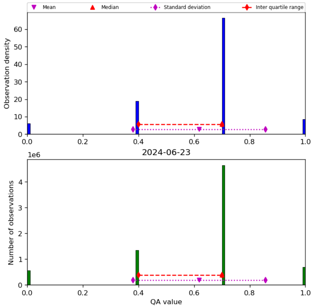
Figure 17: Histogram of “QA value” for 2024-06-22 to 2024-06-24
