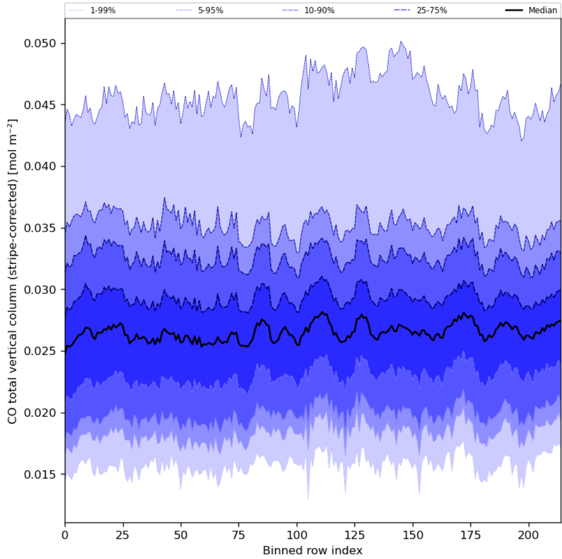
Figure 27: Along track statistics of “CO total vertical column (stripe-corrected)” for 2024-06-22 to 2024-06-24
