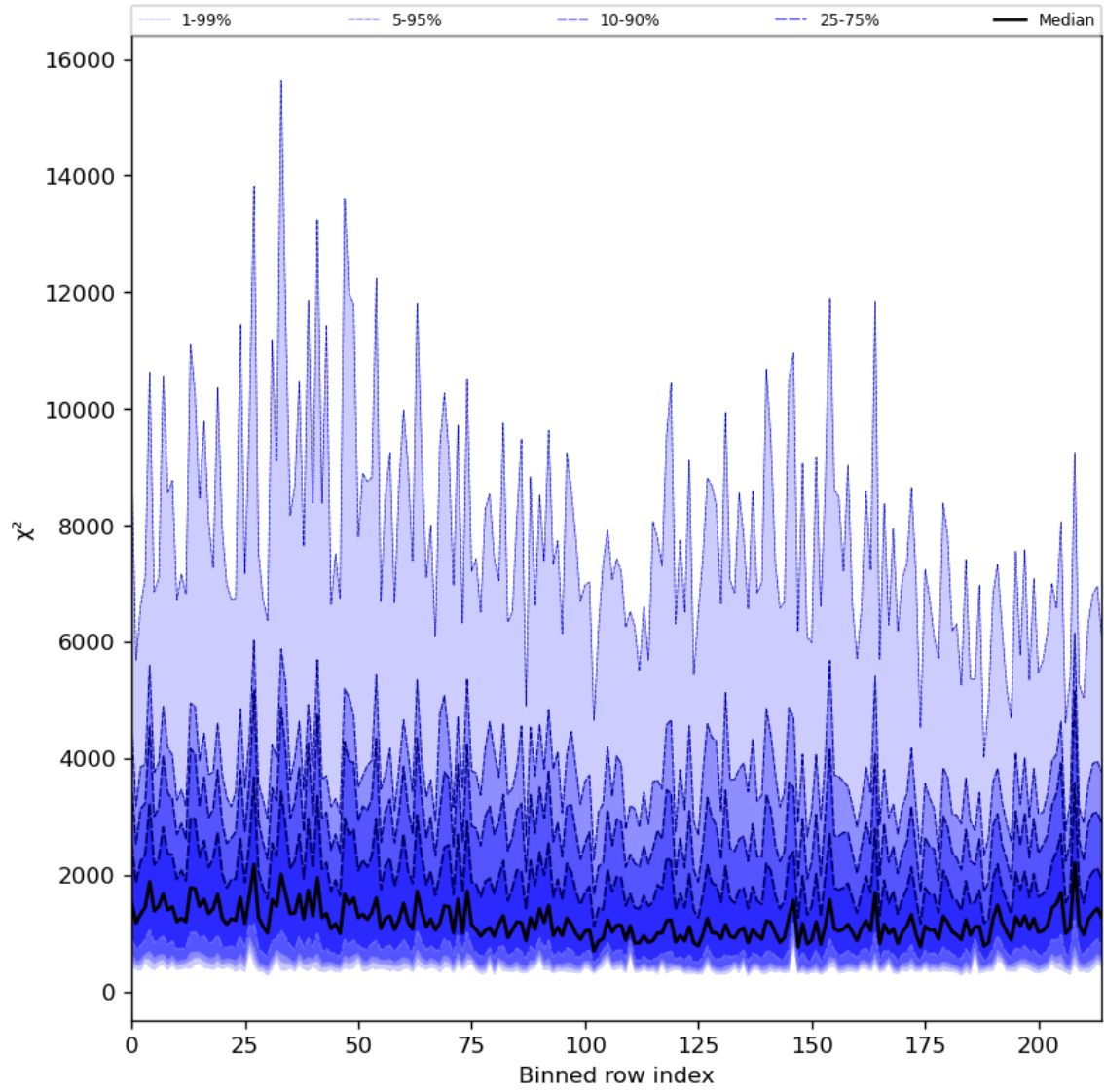
Figure 30: Along track statistics of “ \chi^2 ” for 2024-06-22 to 2024-06-24
