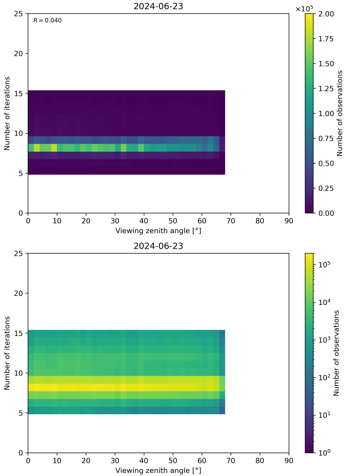
Figure 75: Scatter density plot of “Viewing zenith angle” against “Number of iterations” for 2024-06-22 to 2024-06-24.
