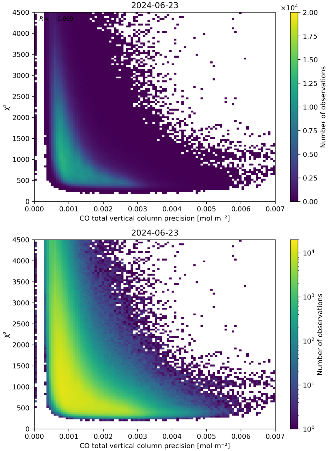
Figure 44: Scatter density plot of “CO total vertical column precision” against “ \chi^2 ” for 2024-06-22 to 2024-06-24.
