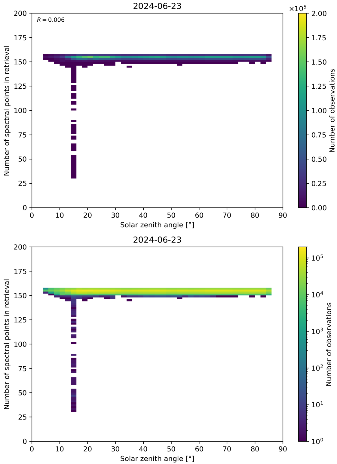
Figure 68: Scatter density plot of “Solar zenith angle” against “Number of spectral points in retrieval” for 2024-06-22 to 2024-06-24.
