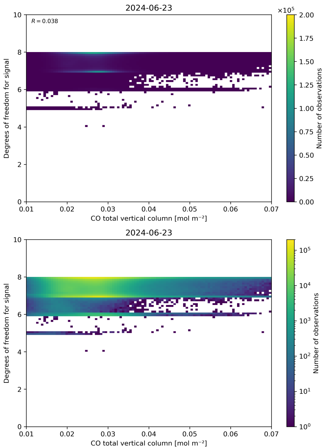
Figure 41: Scatter density plot of “CO total vertical column” against “Degrees of freedom for signal” for 2024-06-22 to 2024-06-24.
