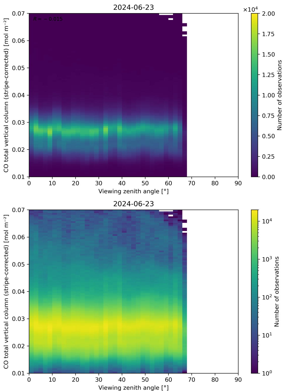
Figure 70: Scatter density plot of “Viewing zenith angle” against “CO total vertical column (stripe-corrected)” for 2024-06-22 to 2024-06-24.
