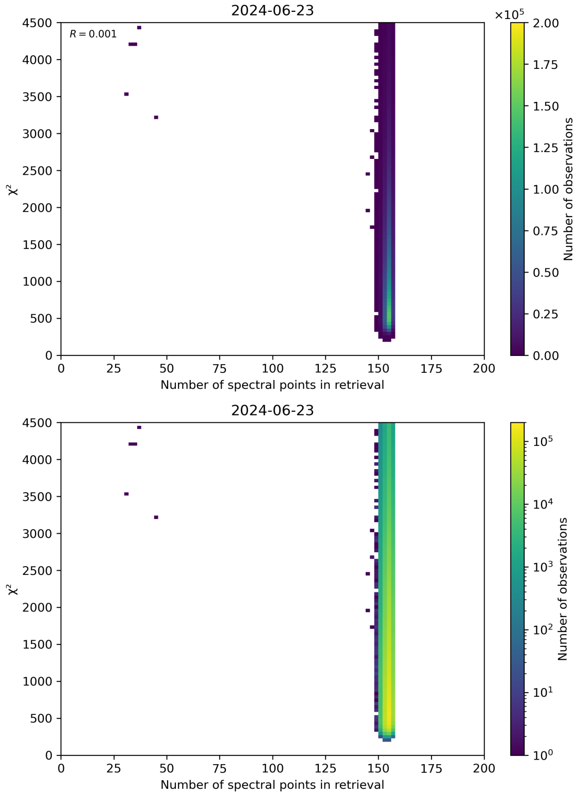
Figure 58: Scatter density plot of “Number of spectral points in retrieval” against “ \chi^2 ” for 2024-06-22 to 2024-06-24.
