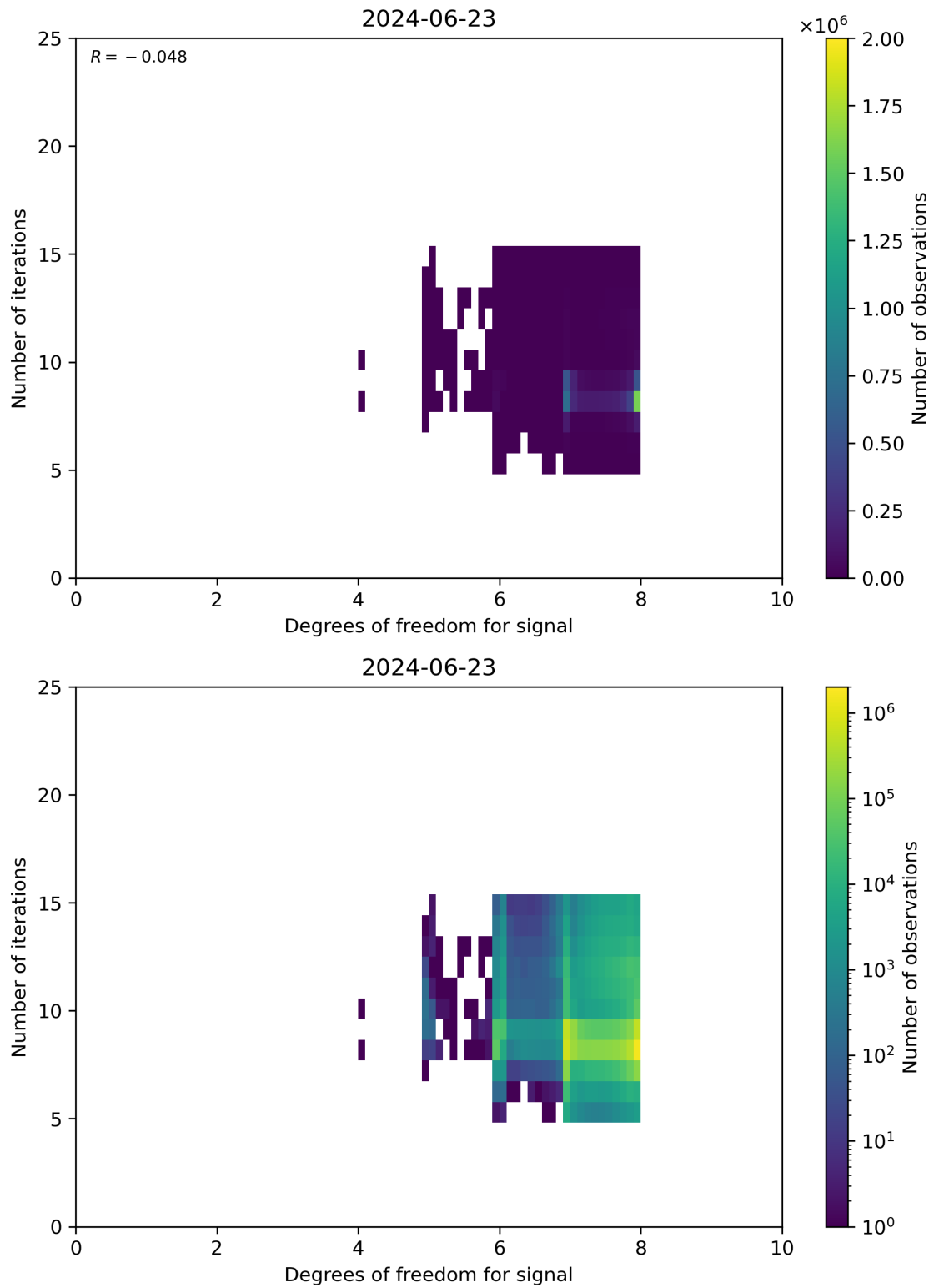
Figure 50: Scatter density plot of “Degrees of freedom for signal” against “Number of iterations” for 2024-06-22 to 2024-06-24.
