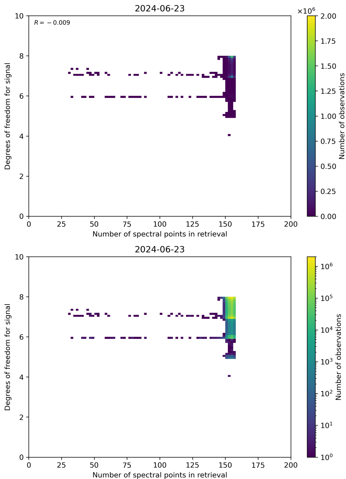
Figure 59: Scatter density plot of “Number of spectral points in retrieval” against “Degrees of freedom for signal” for 2024-06-22 to 2024-06-24.
