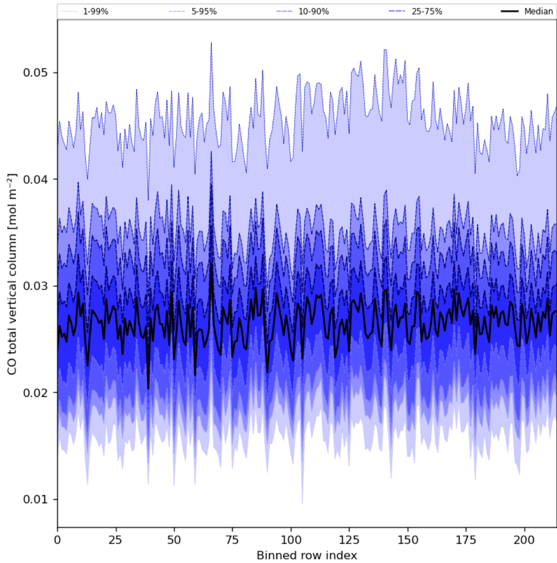
Figure 26: Along track statistics of “CO total vertical column” for 2024-06-22 to 2024-06-24
