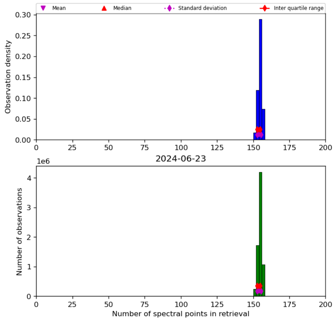
Figure 21: Histogram of “Number of spectral points in retrieval” for 2024-06-22 to 2024-06-24
