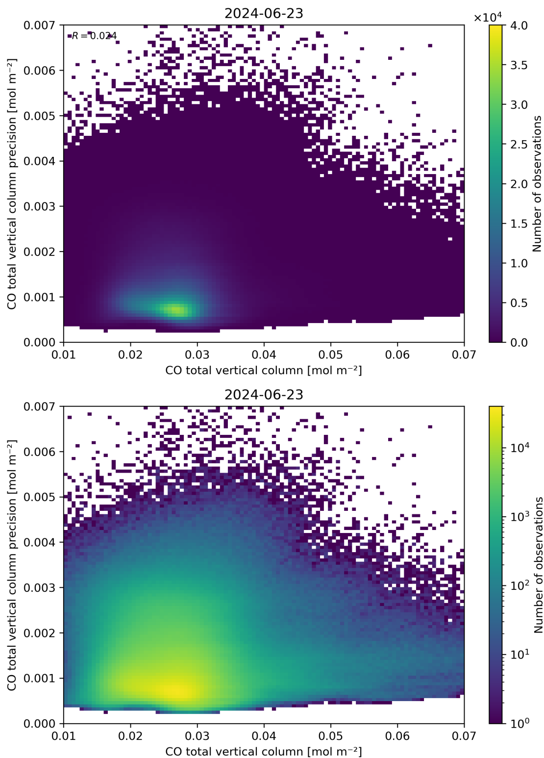
Figure 34: Scatter density plot of “CO total vertical column” against “CO total vertical column precision” for 2024-06-22 to 2024-06-24.
