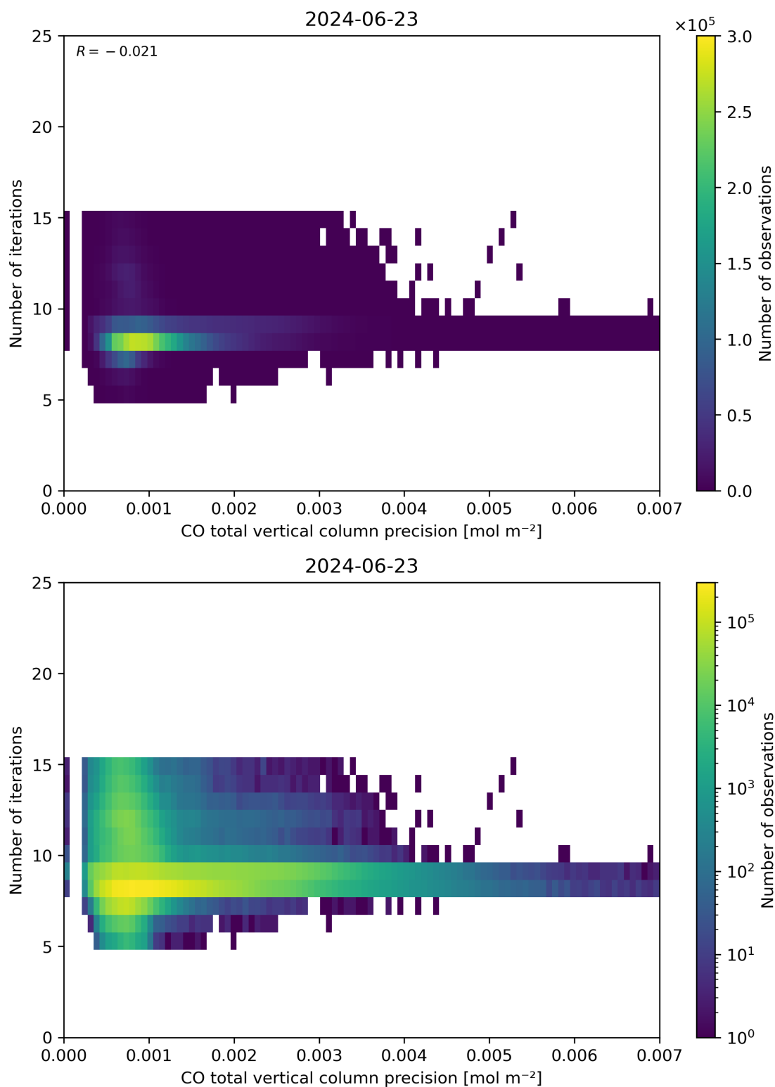
Figure 46: Scatter density plot of “CO total vertical column precision” against “Number of iterations” for 2024-06-22 to 2024-06-24.
