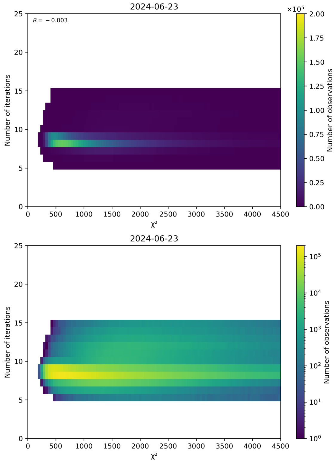
Figure 49: Scatter density plot of “ \chi^2 ” against “Number of iterations” for 2024-06-22 to 2024-06-24.
