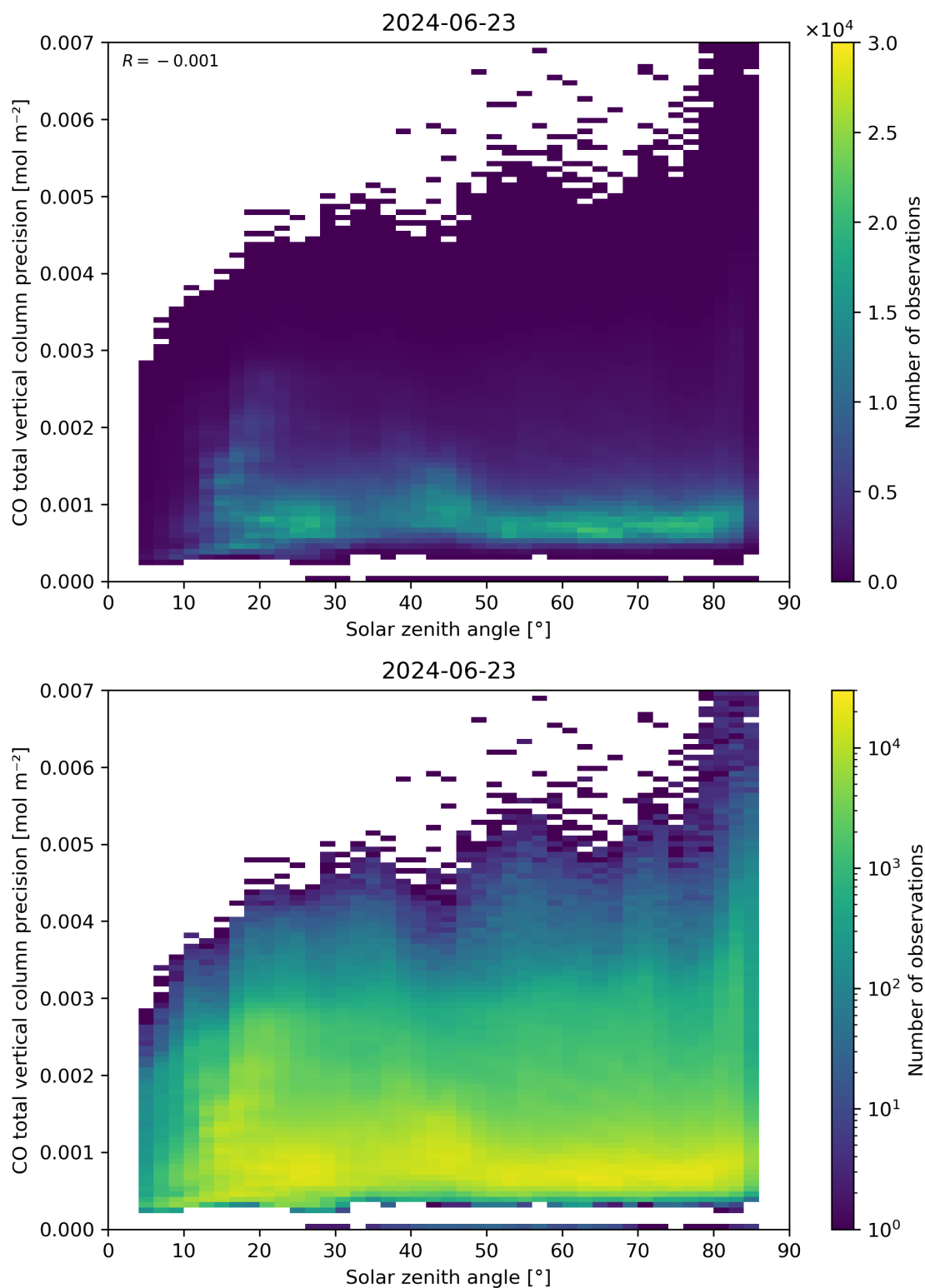
Figure 63: Scatter density plot of “Solar zenith angle” against “CO total vertical column precision” for 2024-06-22 to 2024-06-24.
