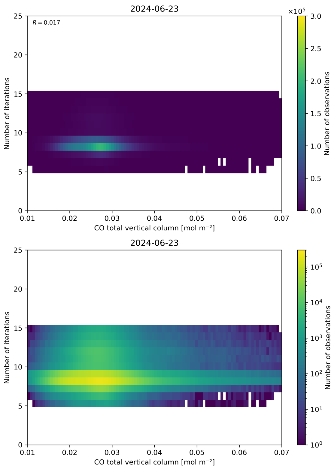
Figure 42: Scatter density plot of “CO total vertical column” against “Number of iterations” for 2024-06-22 to 2024-06-24.
