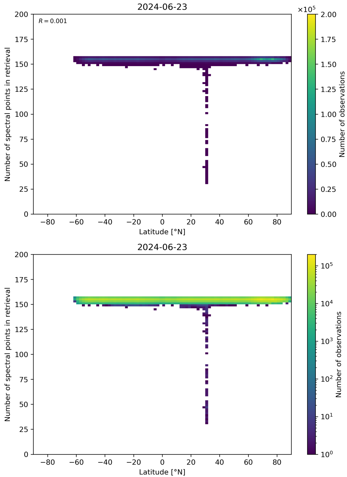
Figure 57: Scatter density plot of “Latitude” against “Number of spectral points in retrieval” for 2024-06-22 to 2024-06-24.
