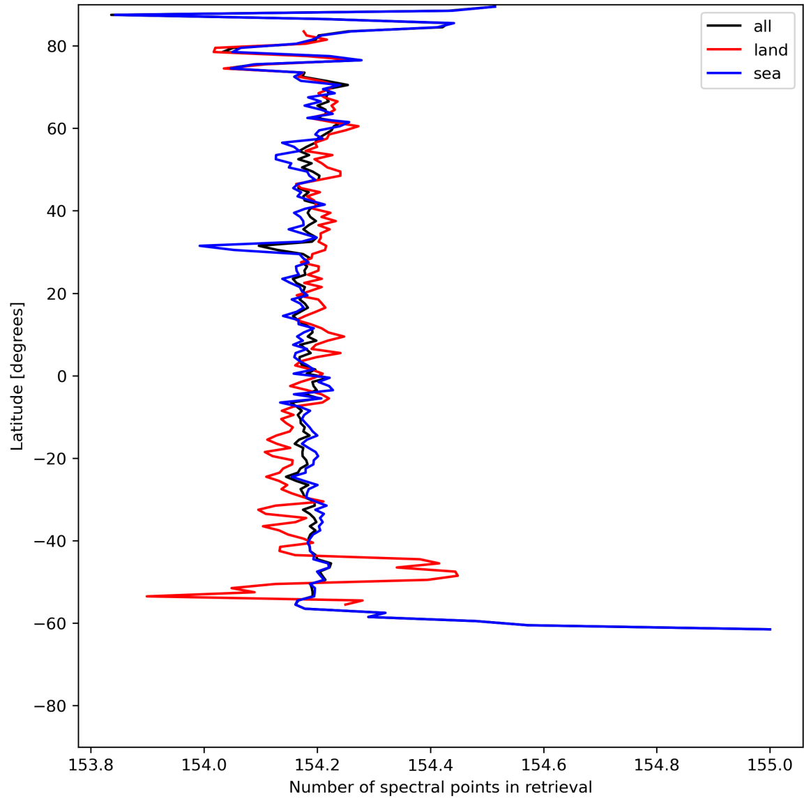
Figure 13: Zonal average of “Number of spectral points in retrieval” for 2024-06-22 to 2024-06-24.
