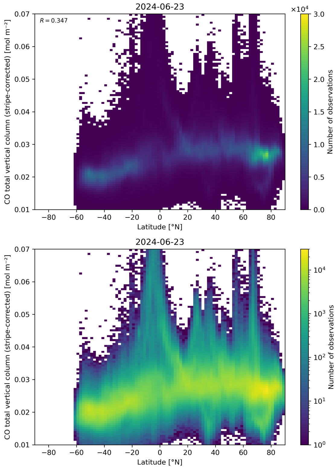
Figure 52: Scatter density plot of “Latitude” against “CO total vertical column (stripe-corrected)” for 2024-06-22 to 2024-06-24.
