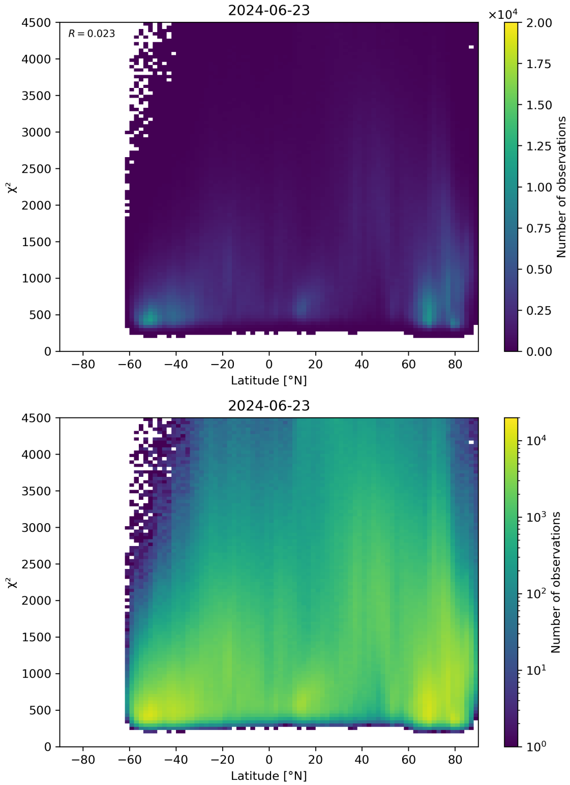
Figure 54: Scatter density plot of “Latitude” against “ \chi^2 ” for 2024-06-22 to 2024-06-24.
