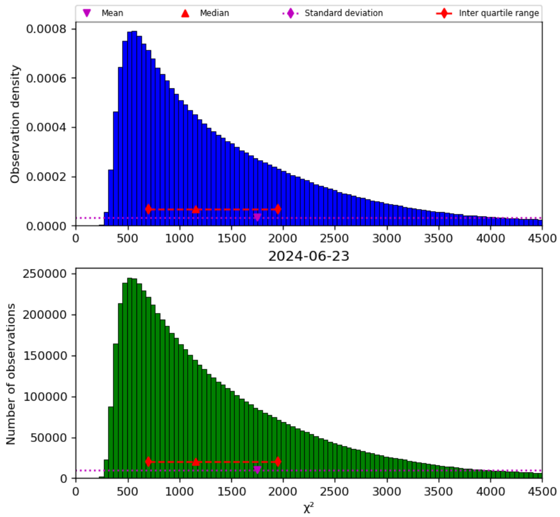
Figure 22: Histogram of “ \chi^2 ” for 2024-06-22 to 2024-06-24
