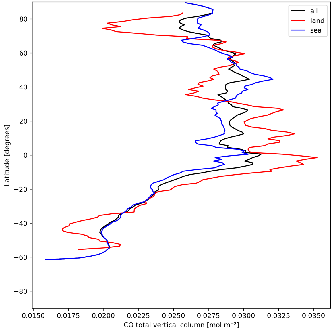
Figure 10: Zonal average of “CO total vertical column” for 2024-06-22 to 2024-06-24.
