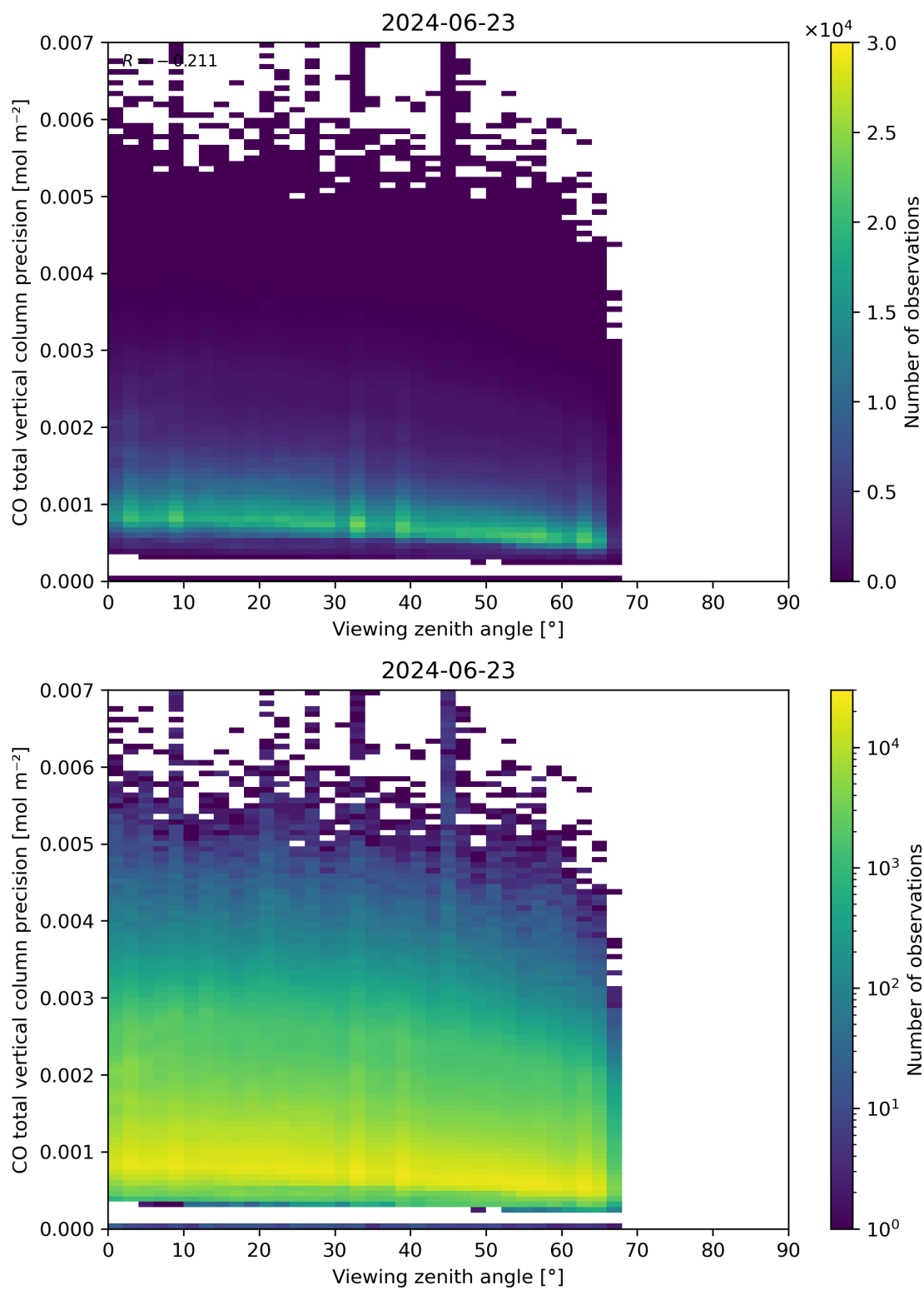
Figure 71: Scatter density plot of “Viewing zenith angle” against “CO total vertical column precision” for 2024-06-22 to 2024-06-24.
