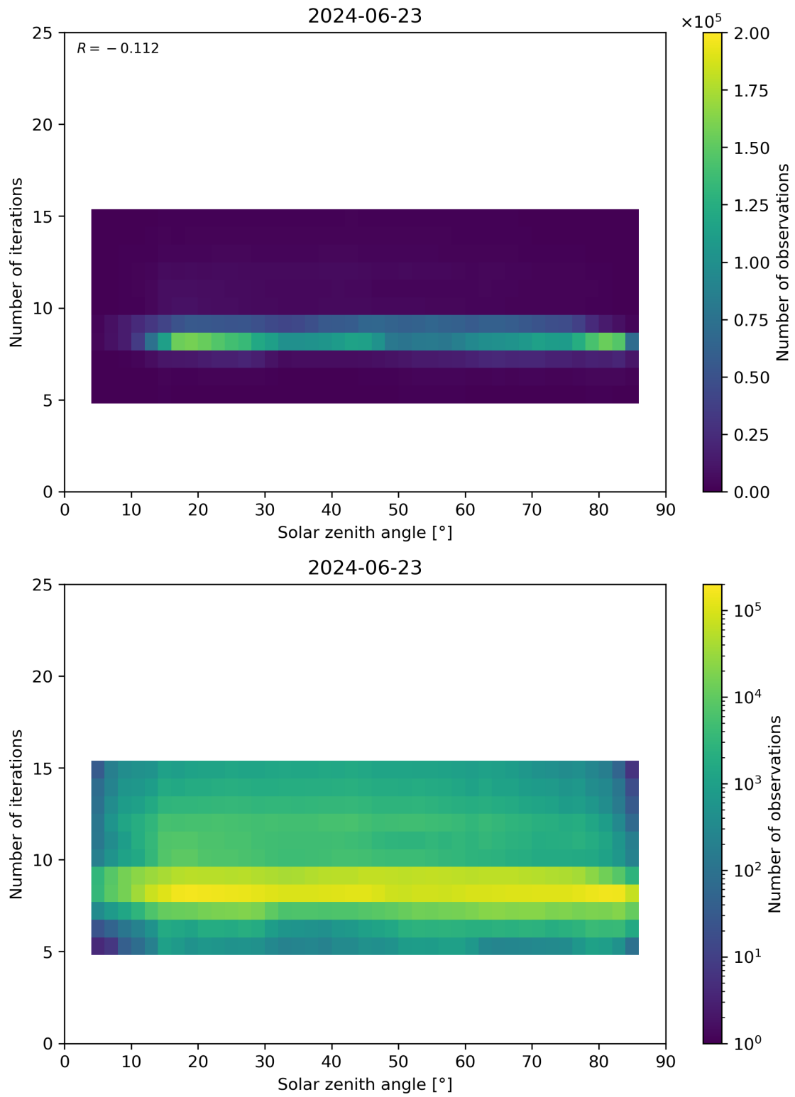
Figure 67: Scatter density plot of “Solar zenith angle” against “Number of iterations” for 2024-06-22 to 2024-06-24.
