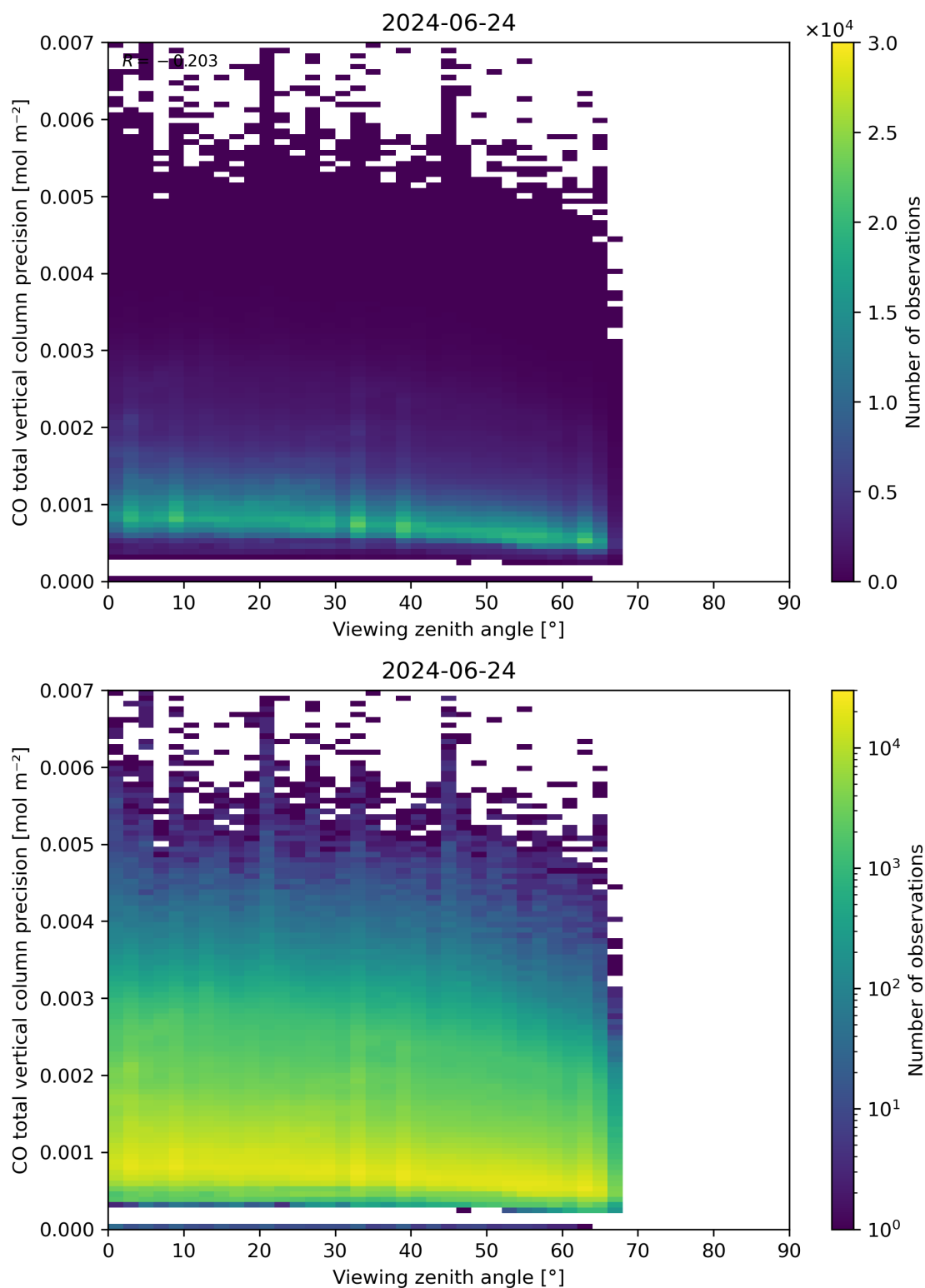
Figure 71: Scatter density plot of “Viewing zenith angle” against “CO total vertical column precision” for 2024-06-24 to 2024-06-25.
