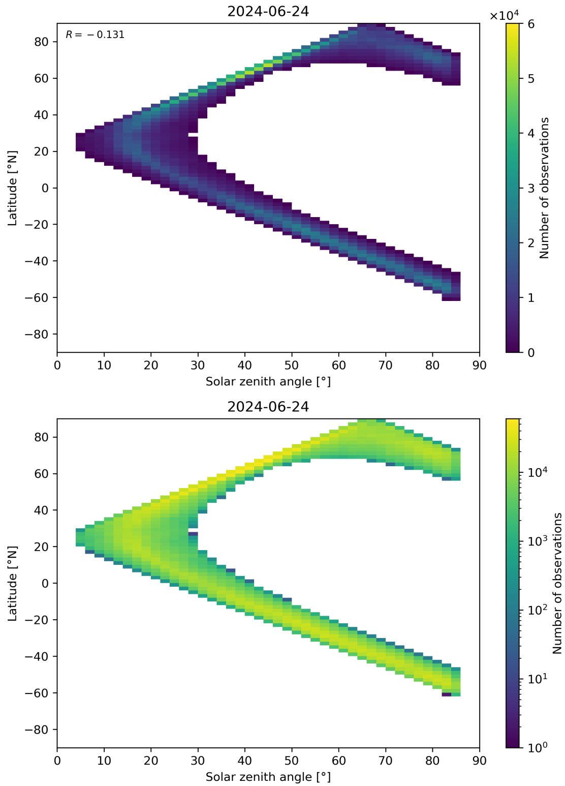
Figure 66: Scatter density plot of “Solar zenith angle” against “Latitude” for 2024-06-24 to 2024-06-25.
