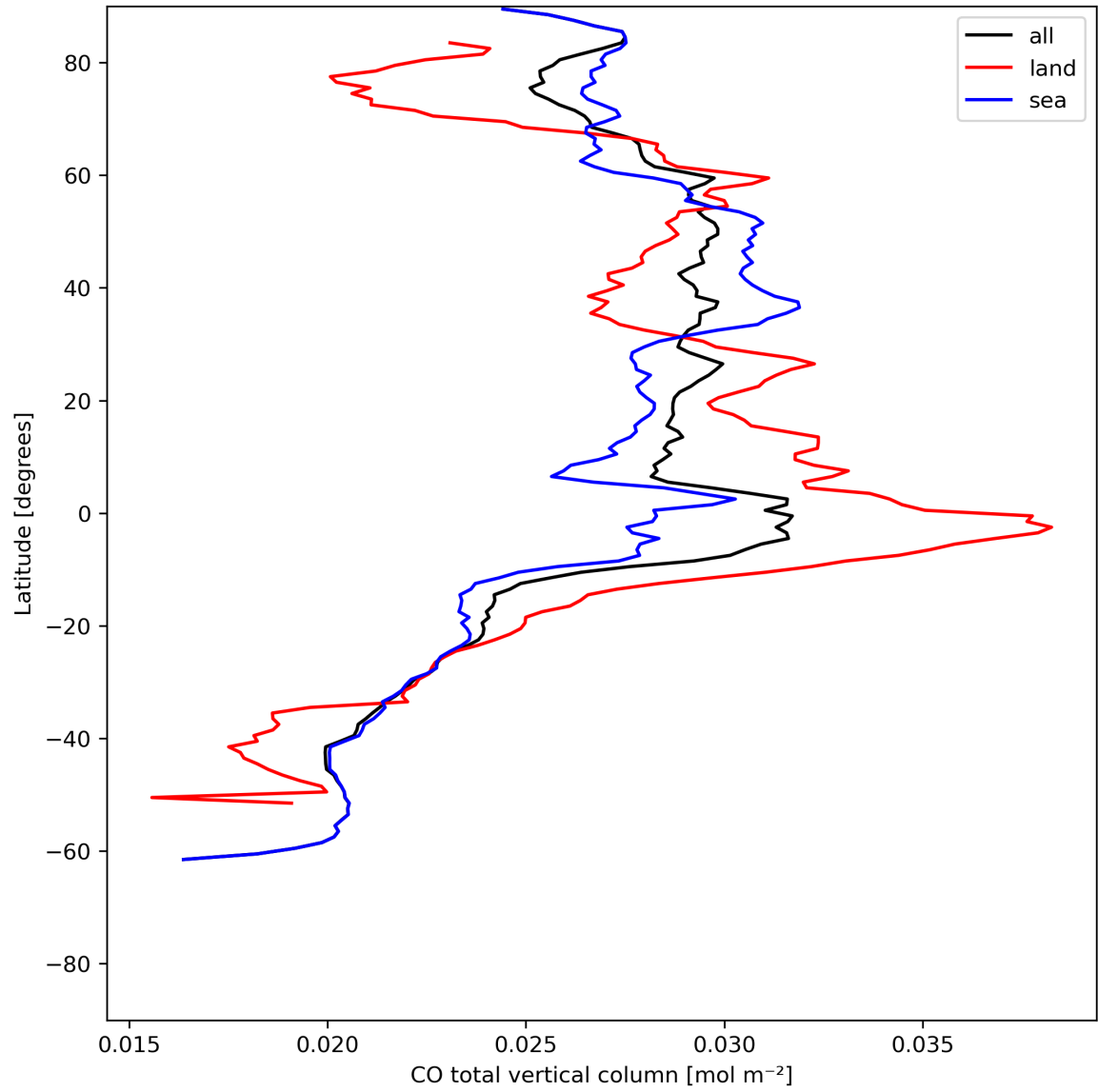
Figure 10: Zonal average of “CO total vertical column” for 2024-06-24 to 2024-06-25.
