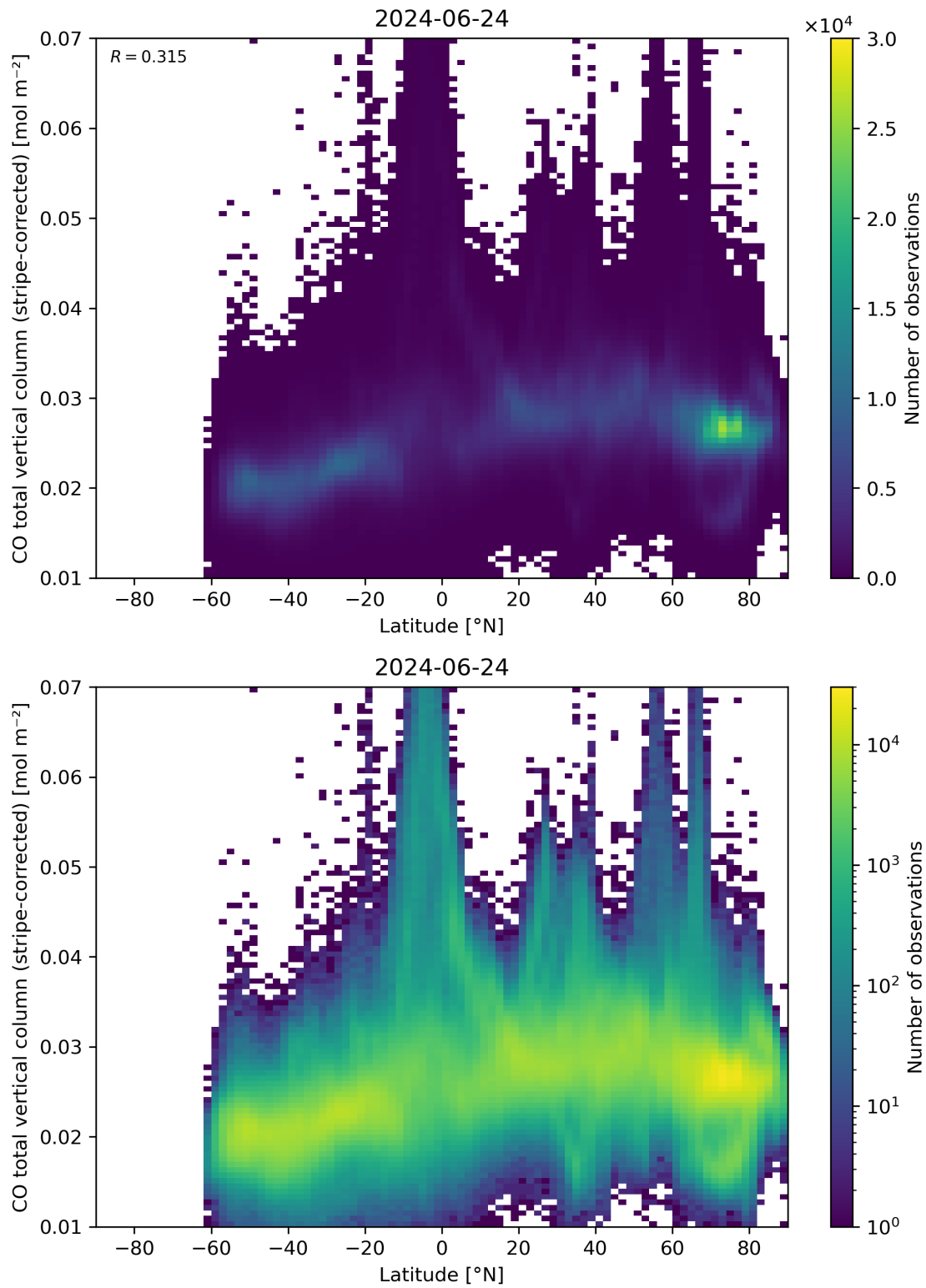
Figure 52: Scatter density plot of “Latitude” against “CO total vertical column (stripe-corrected)” for 2024-06-24 to 2024-06-25.
