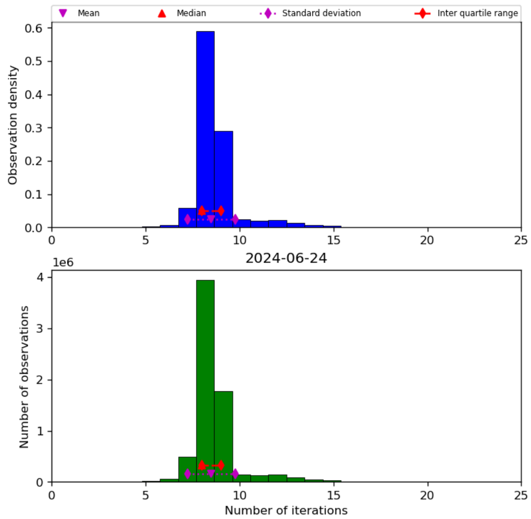
Figure 24: Histogram of “Number of iterations” for 2024-06-24 to 2024-06-25
