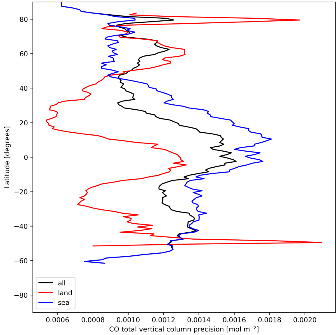
Figure 12: Zonal average of “CO total vertical column precision” for 2024-06-24 to 2024-06-25.
