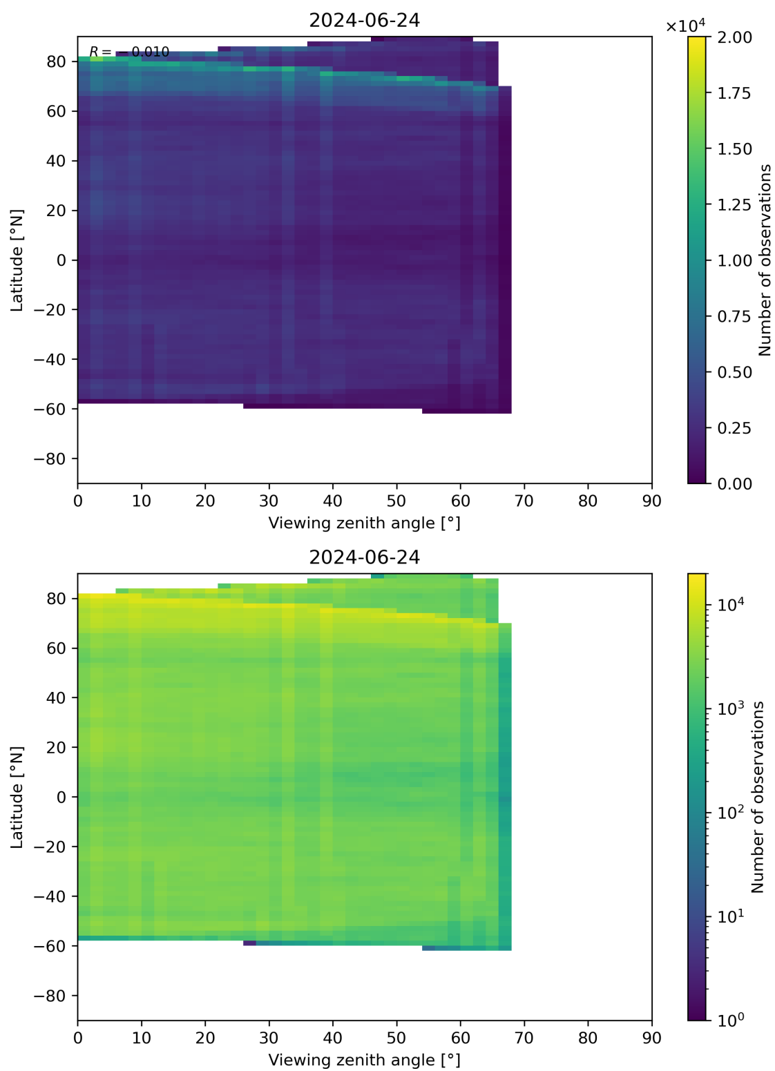
Figure 74: Scatter density plot of “Viewing zenith angle” against “Latitude” for 2024-06-24 to 2024-06-25.
