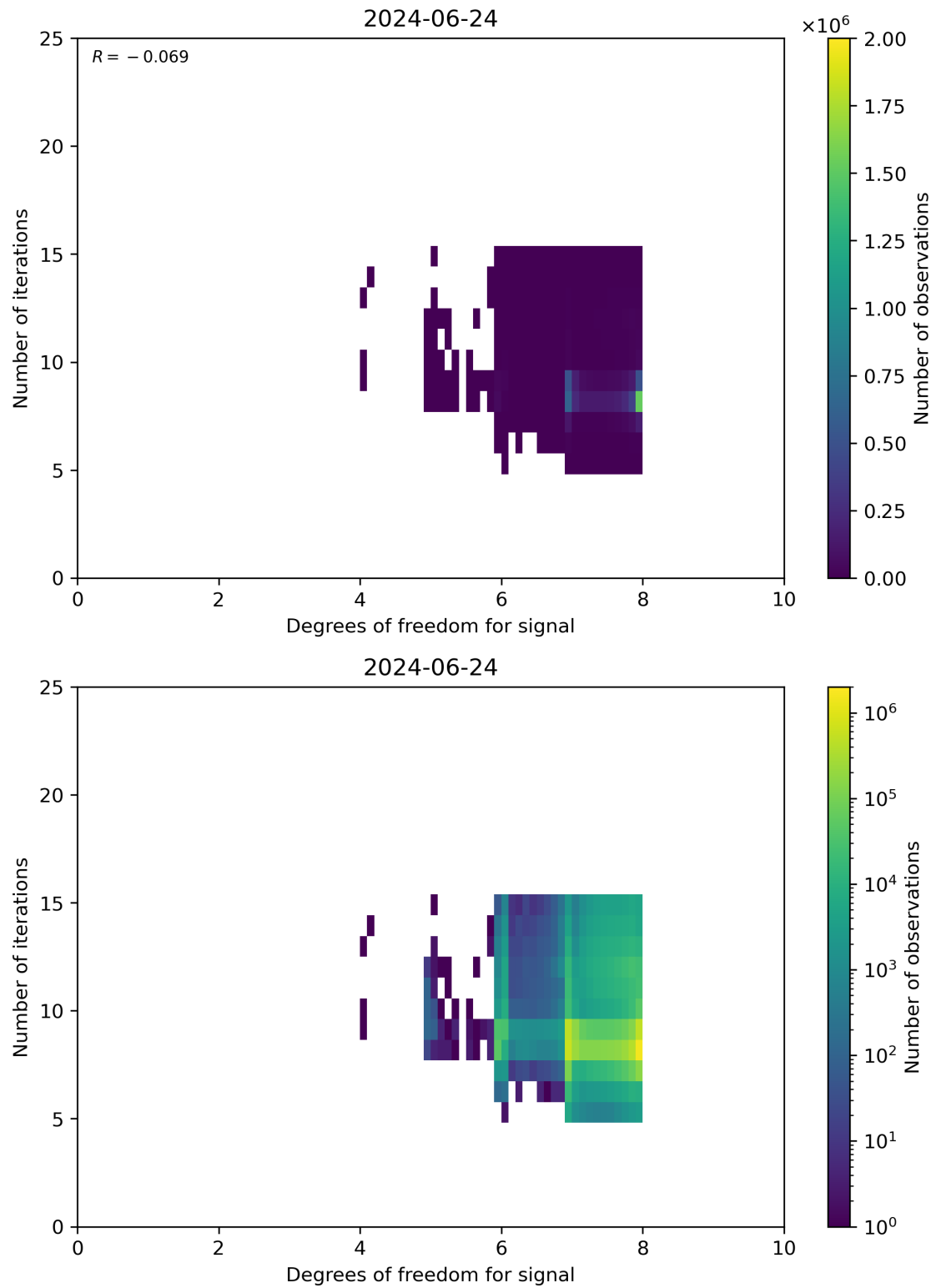
Figure 50: Scatter density plot of “Degrees of freedom for signal” against “Number of iterations” for 2024-06-24 to 2024-06-25.
