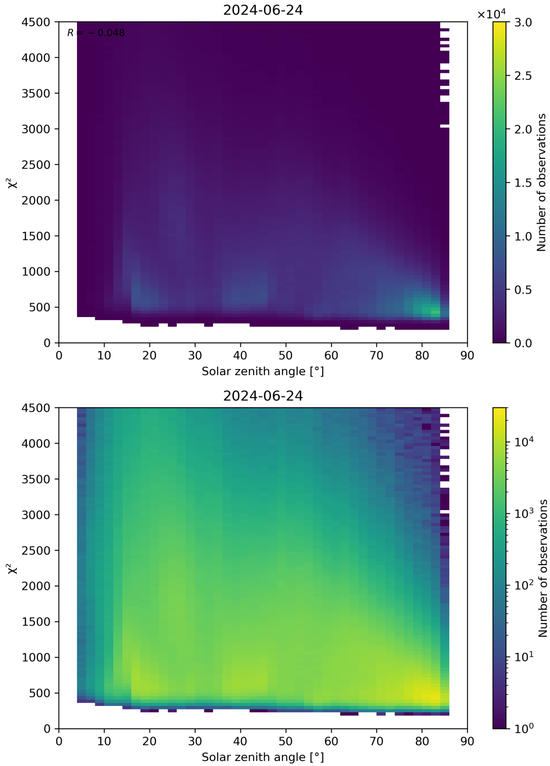
Figure 64: Scatter density plot of “Solar zenith angle” against “ \chi^2 ” for 2024-06-24 to 2024-06-25.
