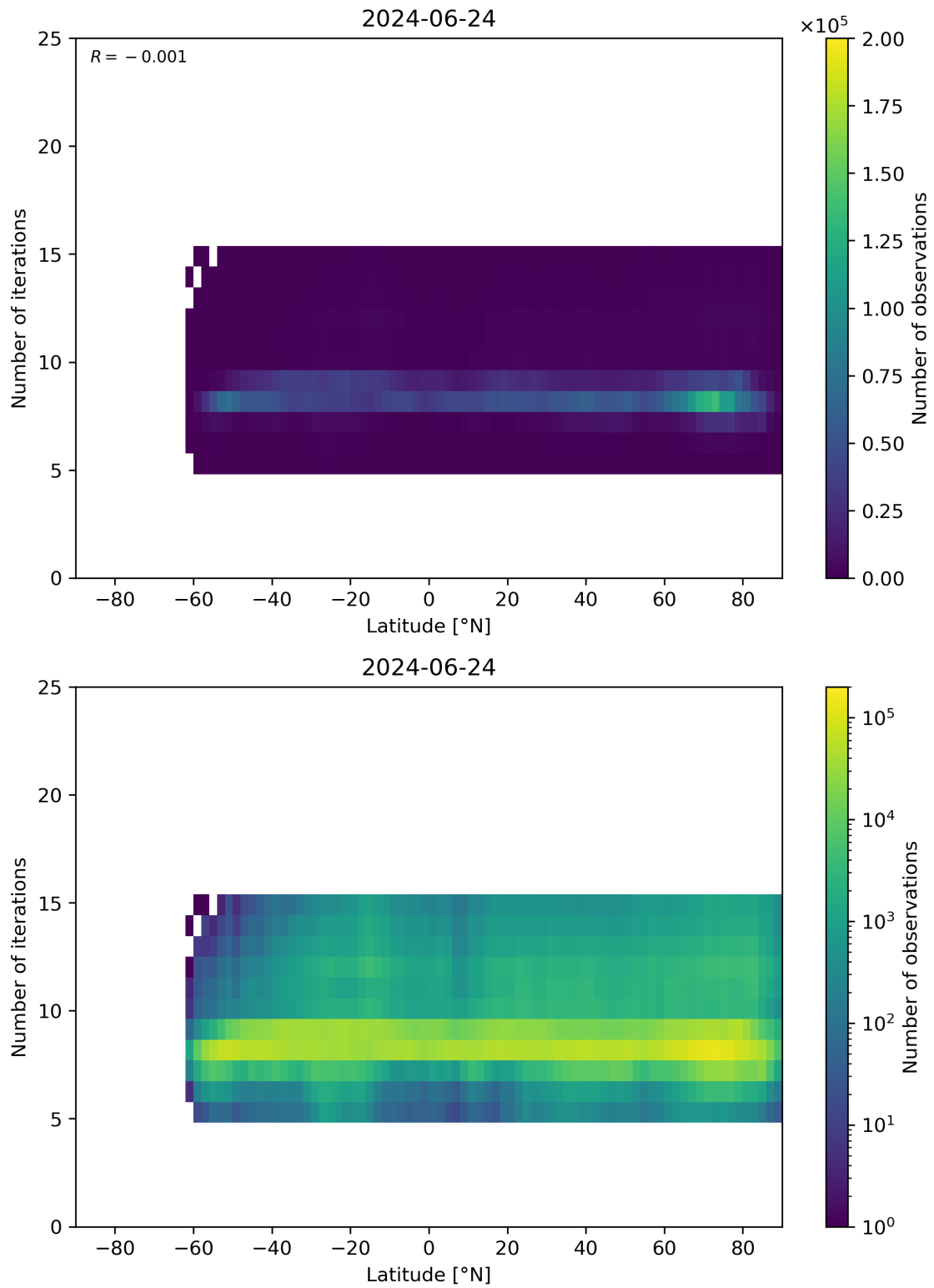
Figure 56: Scatter density plot of “Latitude” against “Number of iterations” for 2024-06-24 to 2024-06-25.
