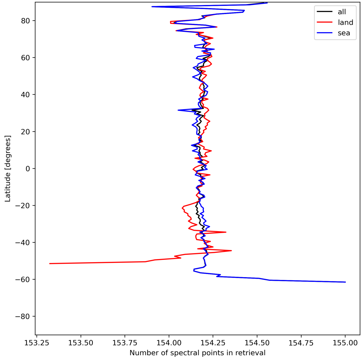
Figure 13: Zonal average of “Number of spectral points in retrieval” for 2024-06-24 to 2024-06-25.
