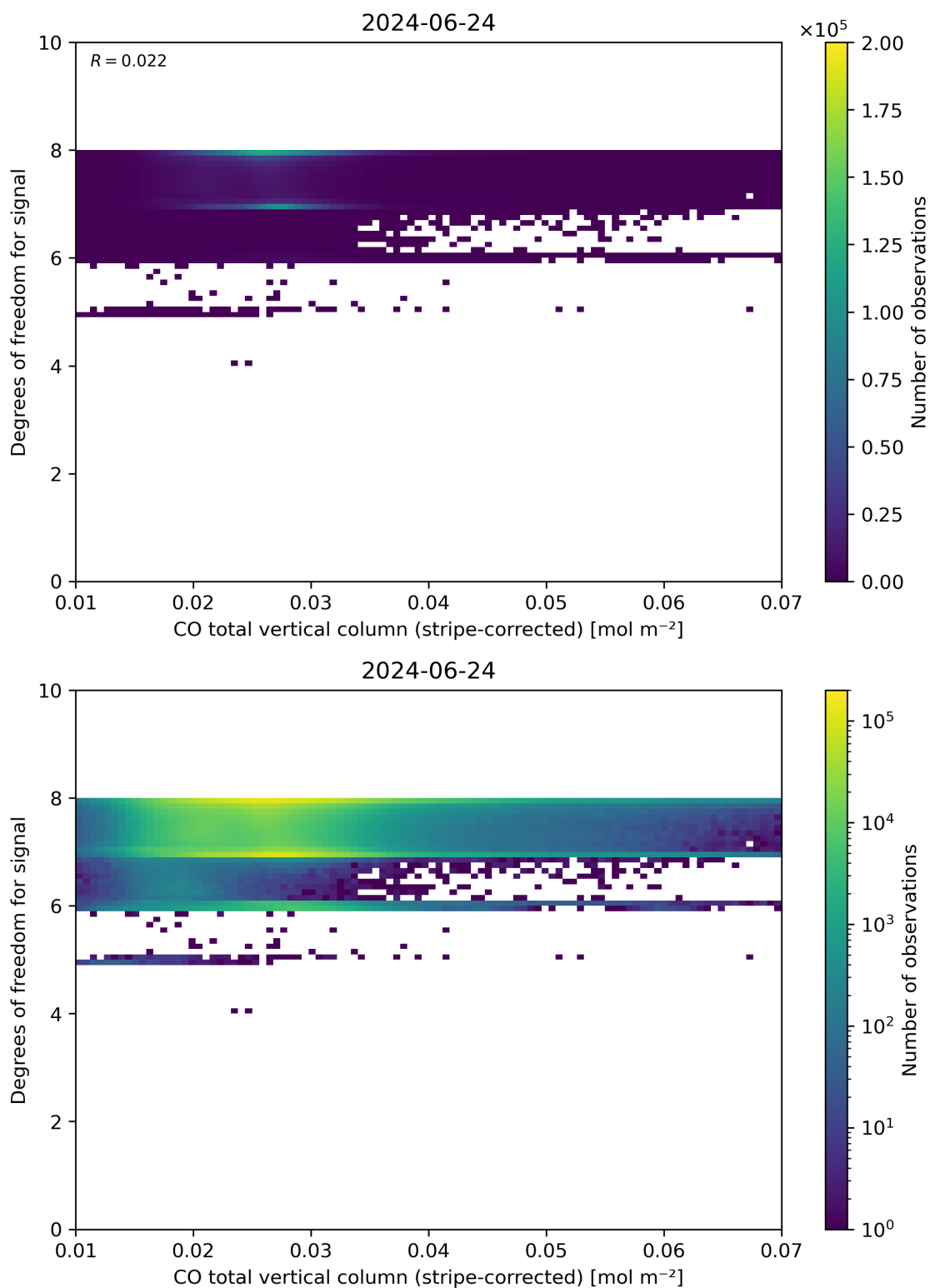
Figure 38: Scatter density plot of “CO total vertical column (stripe-corrected)” against “Degrees of freedom for signal” for 2024-06-24 to 2024-06-25.
