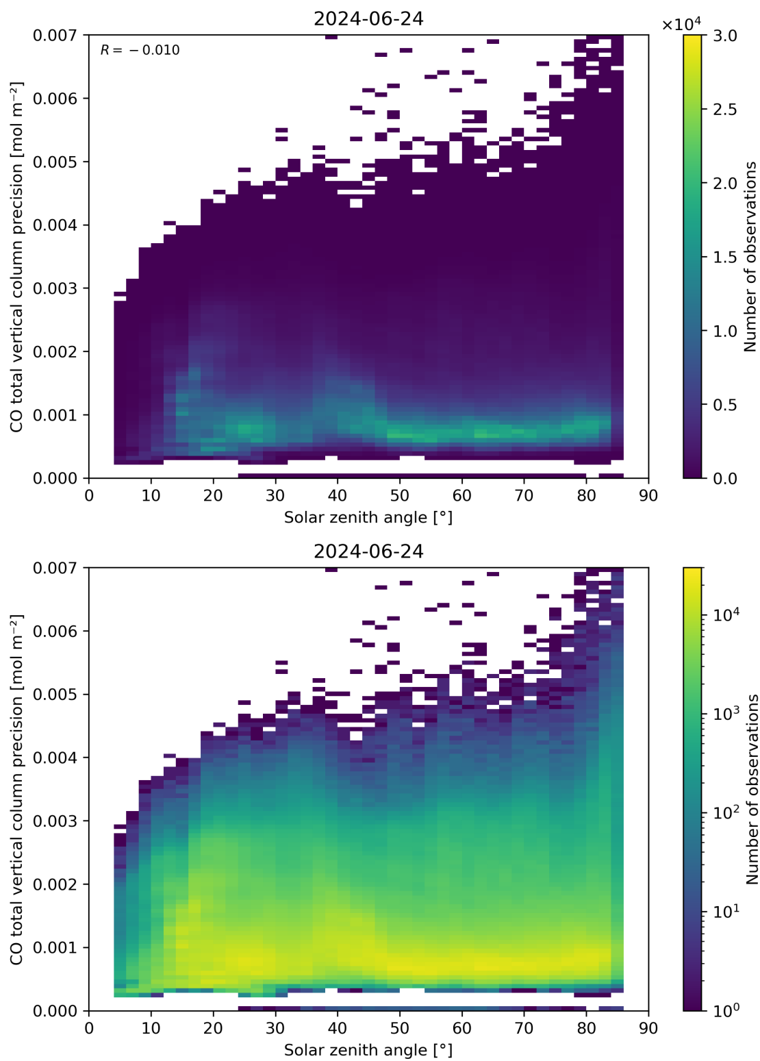
Figure 63: Scatter density plot of “Solar zenith angle” against “CO total vertical column precision” for 2024-06-24 to 2024-06-25.
