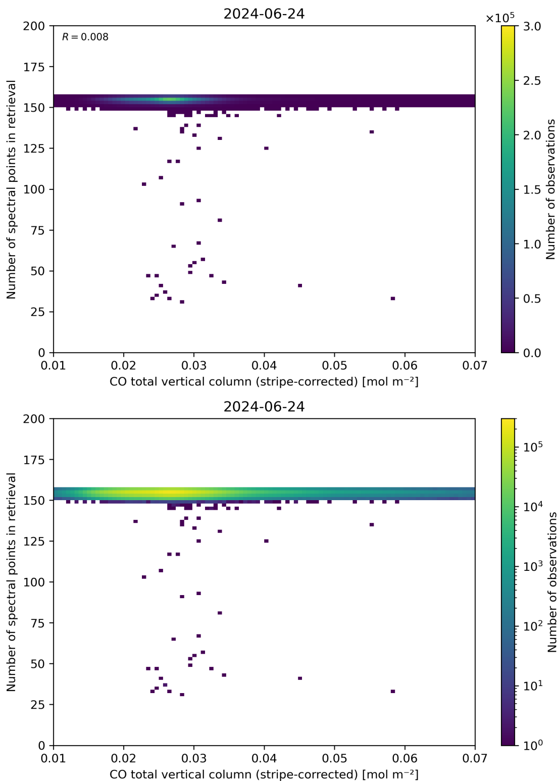
Figure 40: Scatter density plot of “CO total vertical column (stripe-corrected)” against “Number of spectral points in retrieval” for 2024-06-24 to 2024-06-25.
