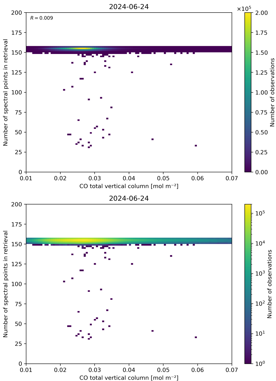
Figure 43: Scatter density plot of “CO total vertical column” against “Number of spectral points in retrieval” for 2024-06-24 to 2024-06-25.
