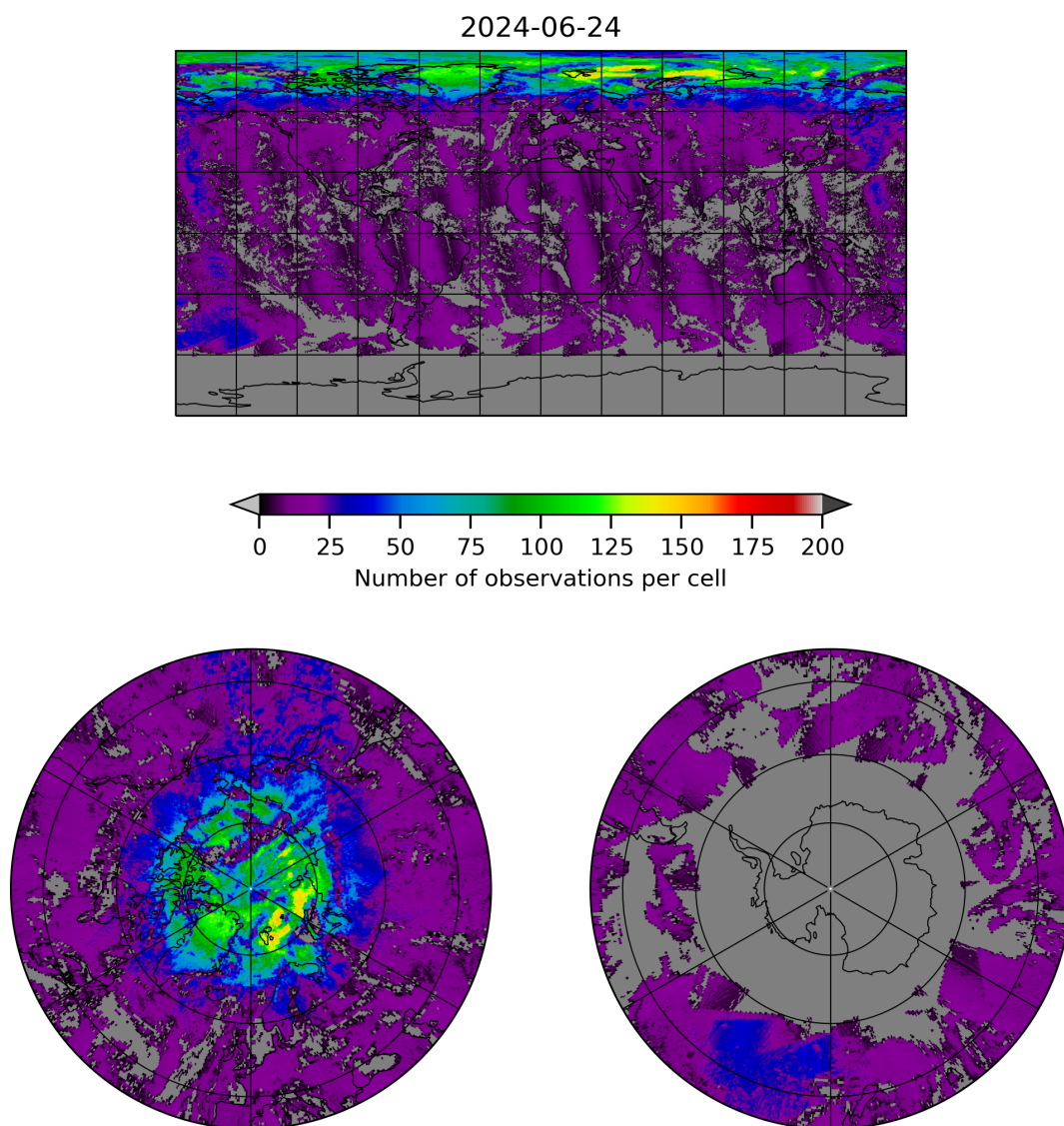
Figure 8: Map of the number of observations for 2024-06-24 to 2024-06-25
