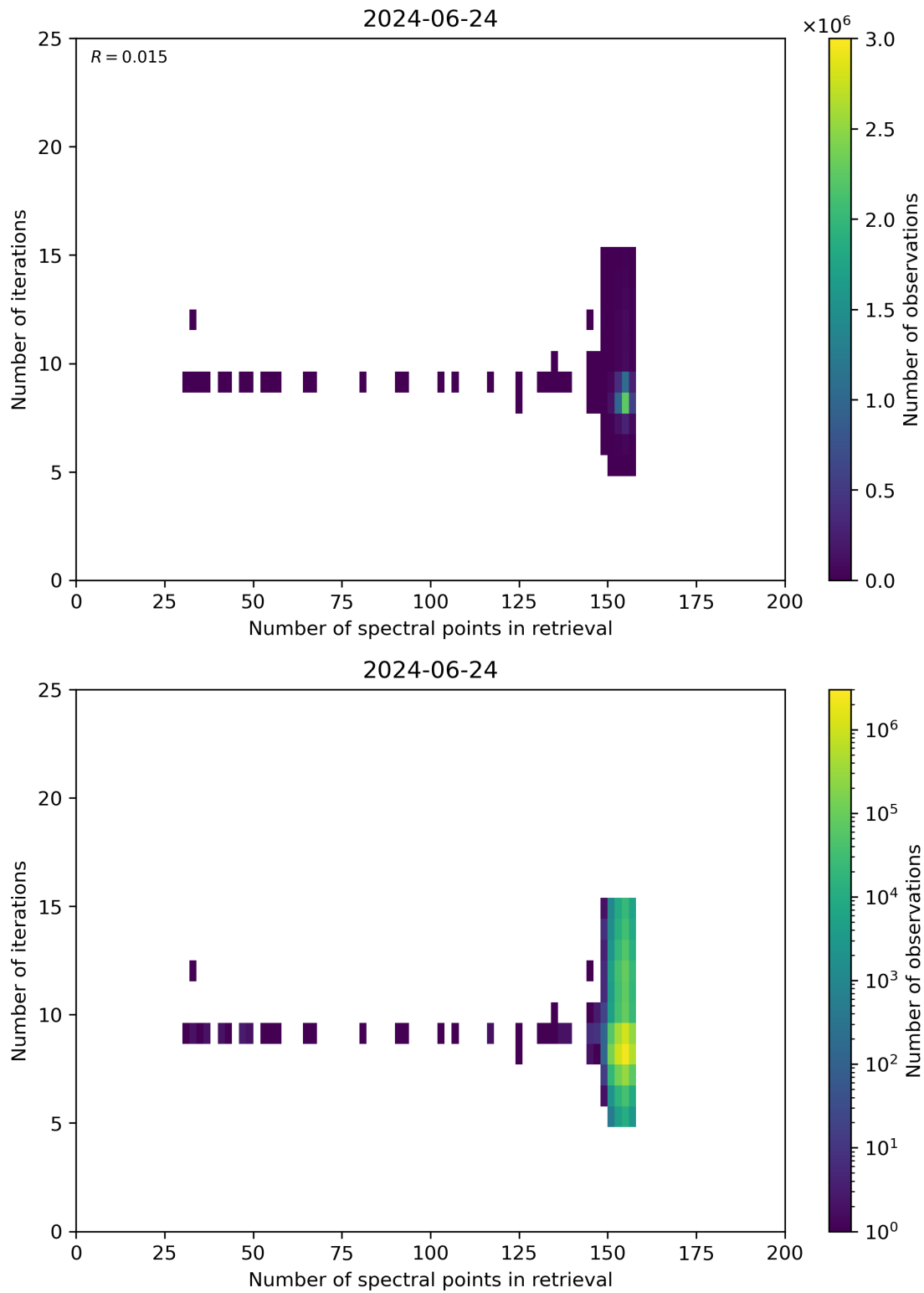
Figure 60: Scatter density plot of “Number of spectral points in retrieval” against “Number of iterations” for 2024-06-24 to 2024-06-25.
