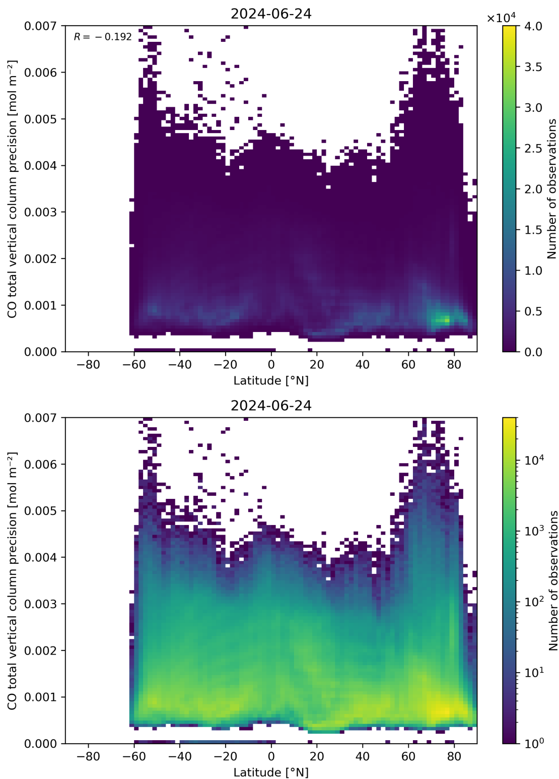
Figure 53: Scatter density plot of “Latitude” against “CO total vertical column precision” for 2024-06-24 to 2024-06-25.
