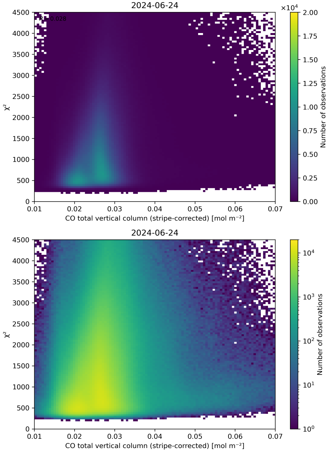
Figure 37: Scatter density plot of “CO total vertical column (stripe-corrected)” against “ \chi^2 ” for 2024-06-24 to 2024-06-25.
