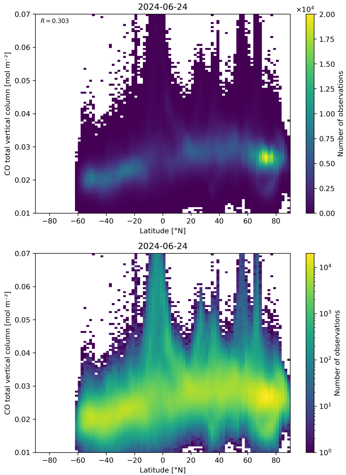
Figure 51: Scatter density plot of “Latitude” against “CO total vertical column” for 2024-06-24 to 2024-06-25.
