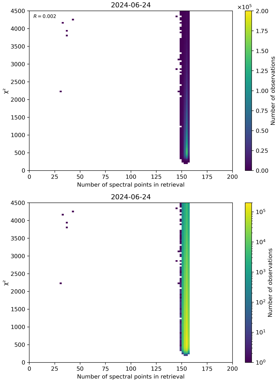
Figure 58: Scatter density plot of “Number of spectral points in retrieval” against “ \chi^2 ” for 2024-06-24 to 2024-06-25.
