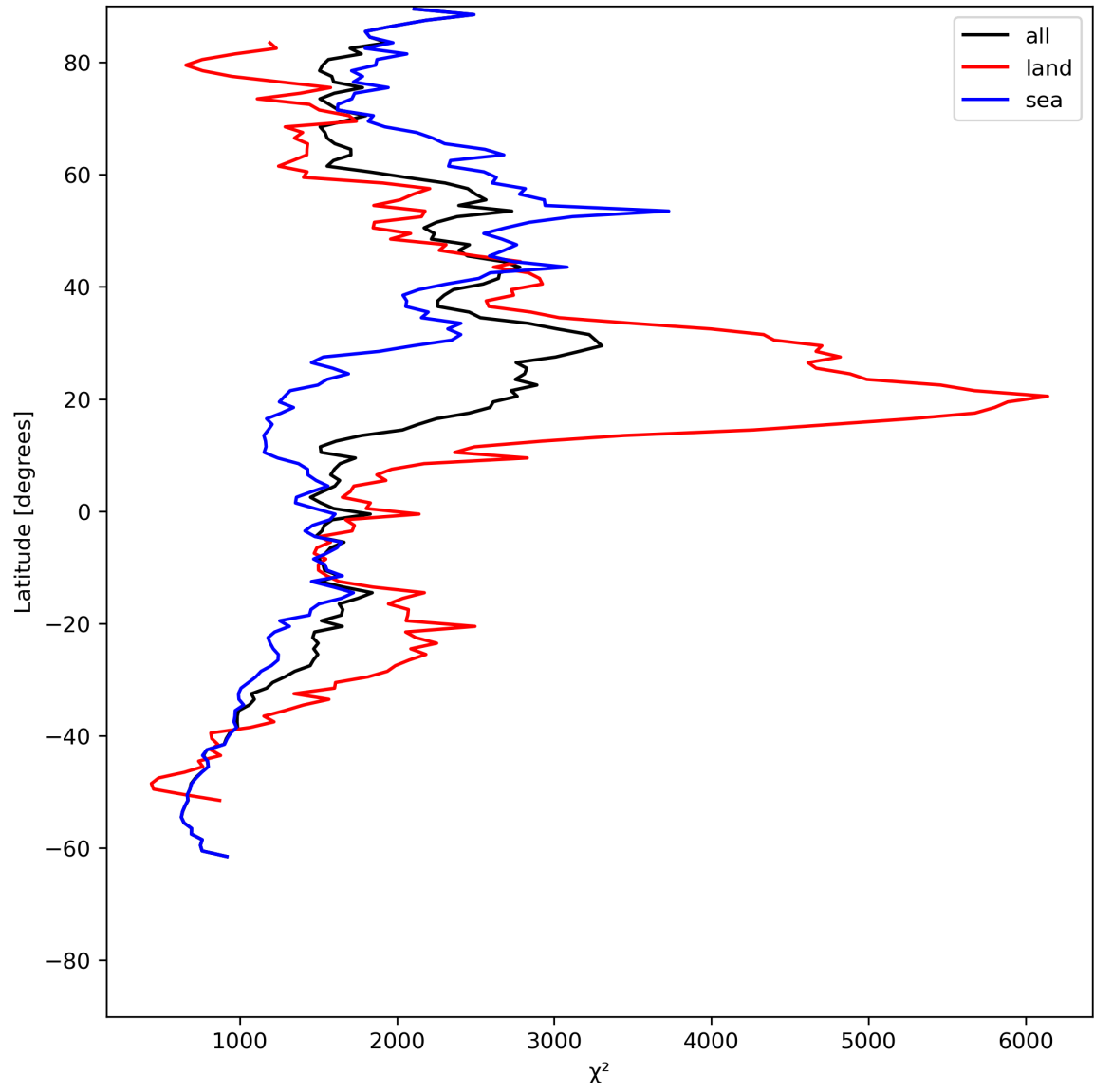
Figure 14: Zonal average of “ \chi^2 ” for 2024-06-24 to 2024-06-25.
