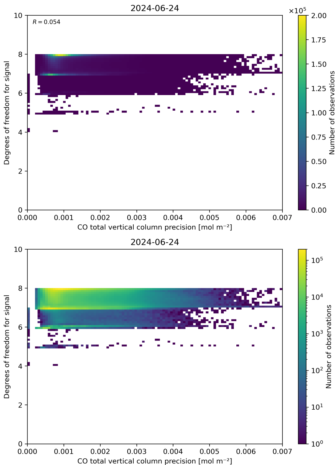
Figure 45: Scatter density plot of “CO total vertical column precision” against “Degrees of freedom for signal” for 2024-06-24 to 2024-06-25.
