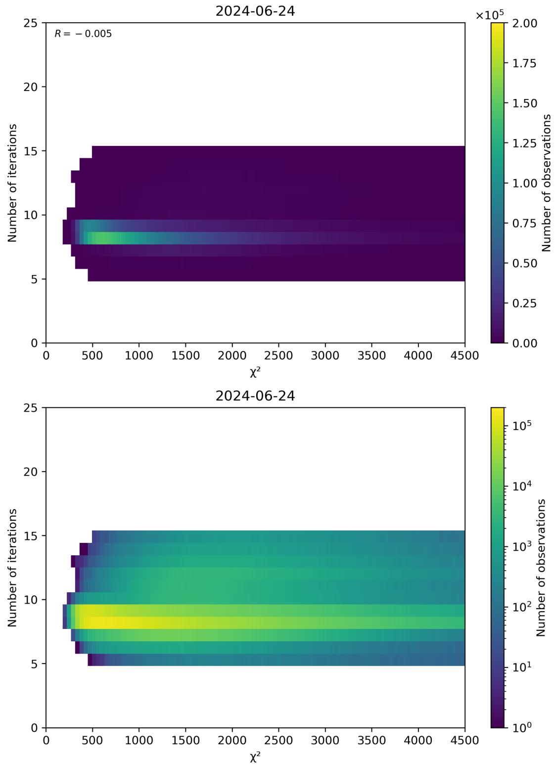
Figure 49: Scatter density plot of “ \chi^2 ” against “Number of iterations” for 2024-06-24 to 2024-06-25.
