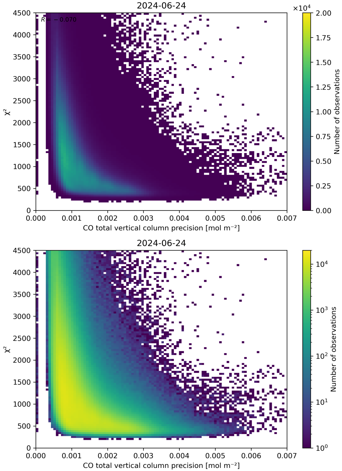
Figure 44: Scatter density plot of “CO total vertical column precision” against “ \chi^2 ” for 2024-06-24 to 2024-06-25.
