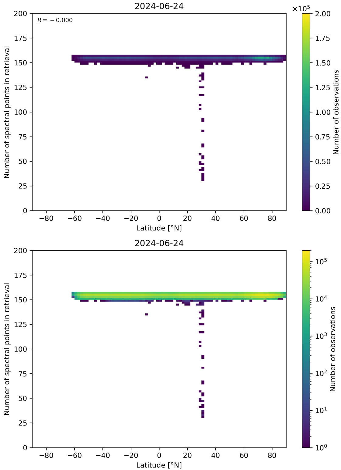
Figure 57: Scatter density plot of “Latitude” against “Number of spectral points in retrieval” for 2024-06-24 to 2024-06-25.
