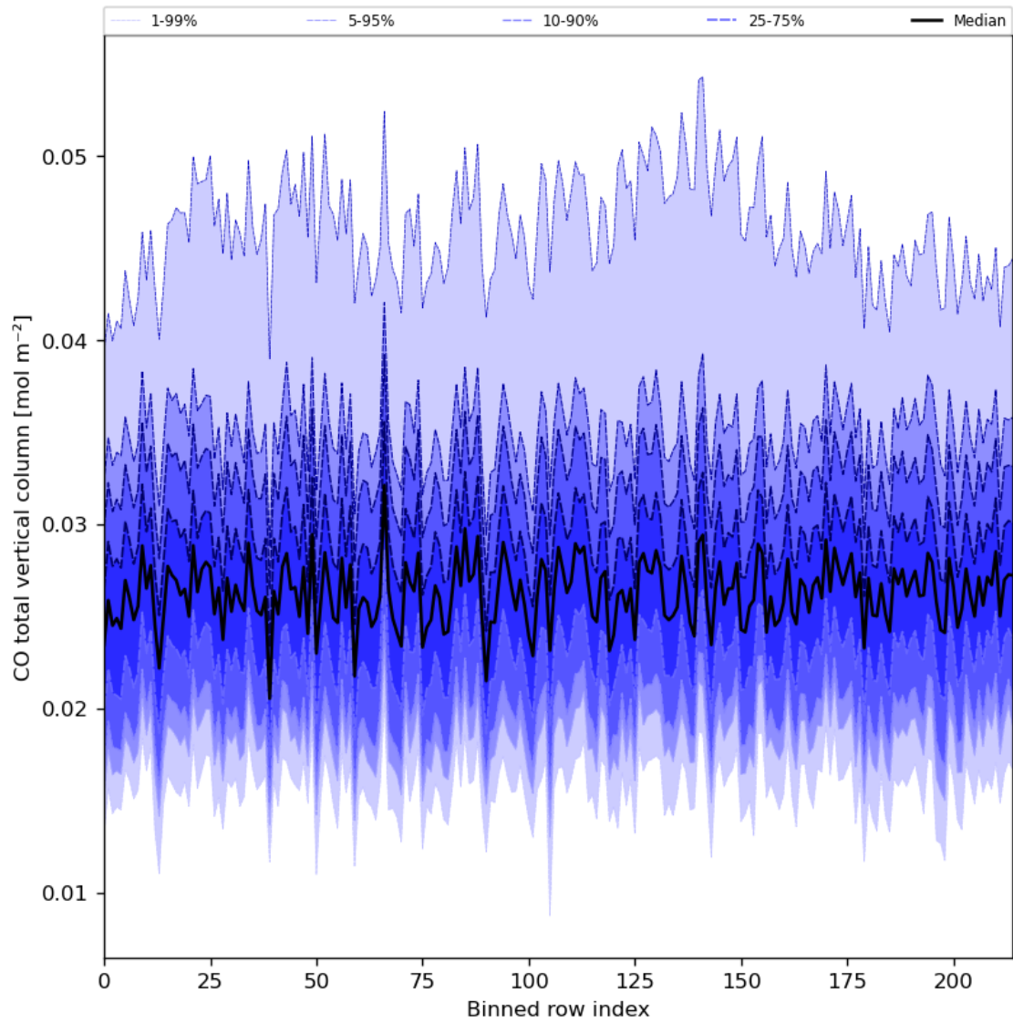
Figure 26: Along track statistics of “CO total vertical column” for 2024-06-24 to 2024-06-25
