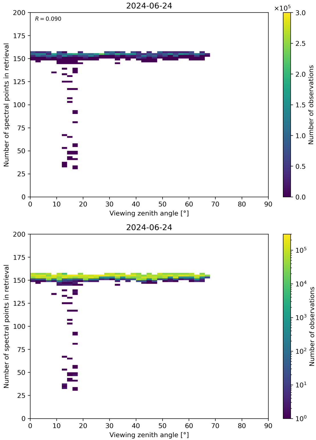
Figure 76: Scatter density plot of “Viewing zenith angle” against “Number of spectral points in retrieval” for 2024-06-24 to 2024-06-25.
