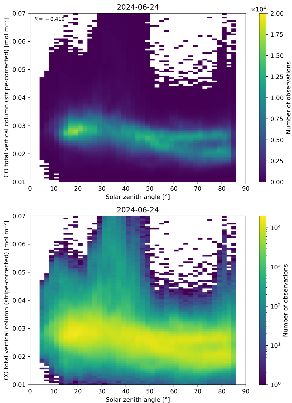
Figure 62: Scatter density plot of “Solar zenith angle” against “CO total vertical column (stripe-corrected)” for 2024-06-24 to 2024-06-25.
