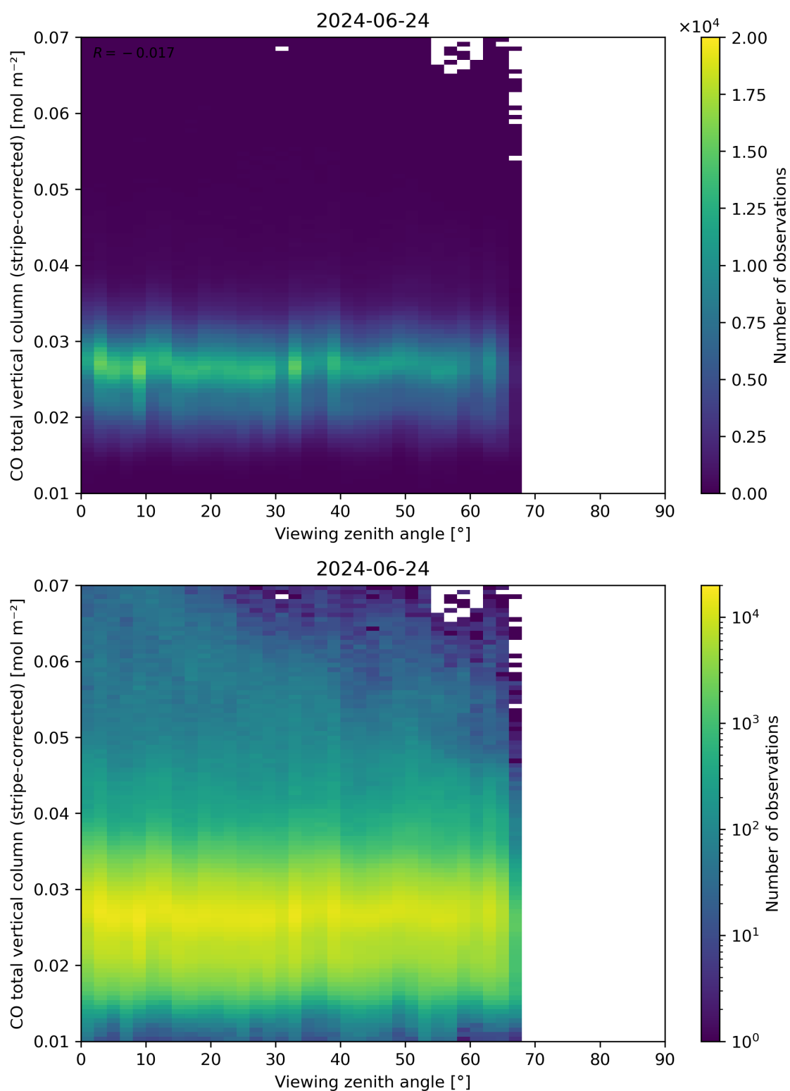
Figure 70: Scatter density plot of “Viewing zenith angle” against “CO total vertical column (stripe-corrected)” for 2024-06-24 to 2024-06-25.
