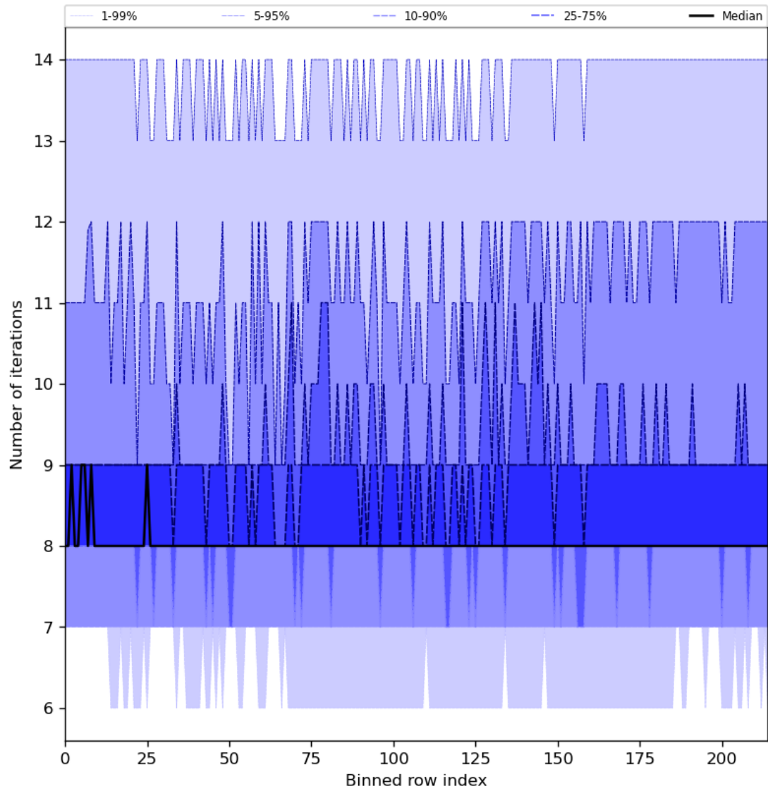
Figure 32: Along track statistics of “Number of iterations” for 2024-06-24 to 2024-06-25
