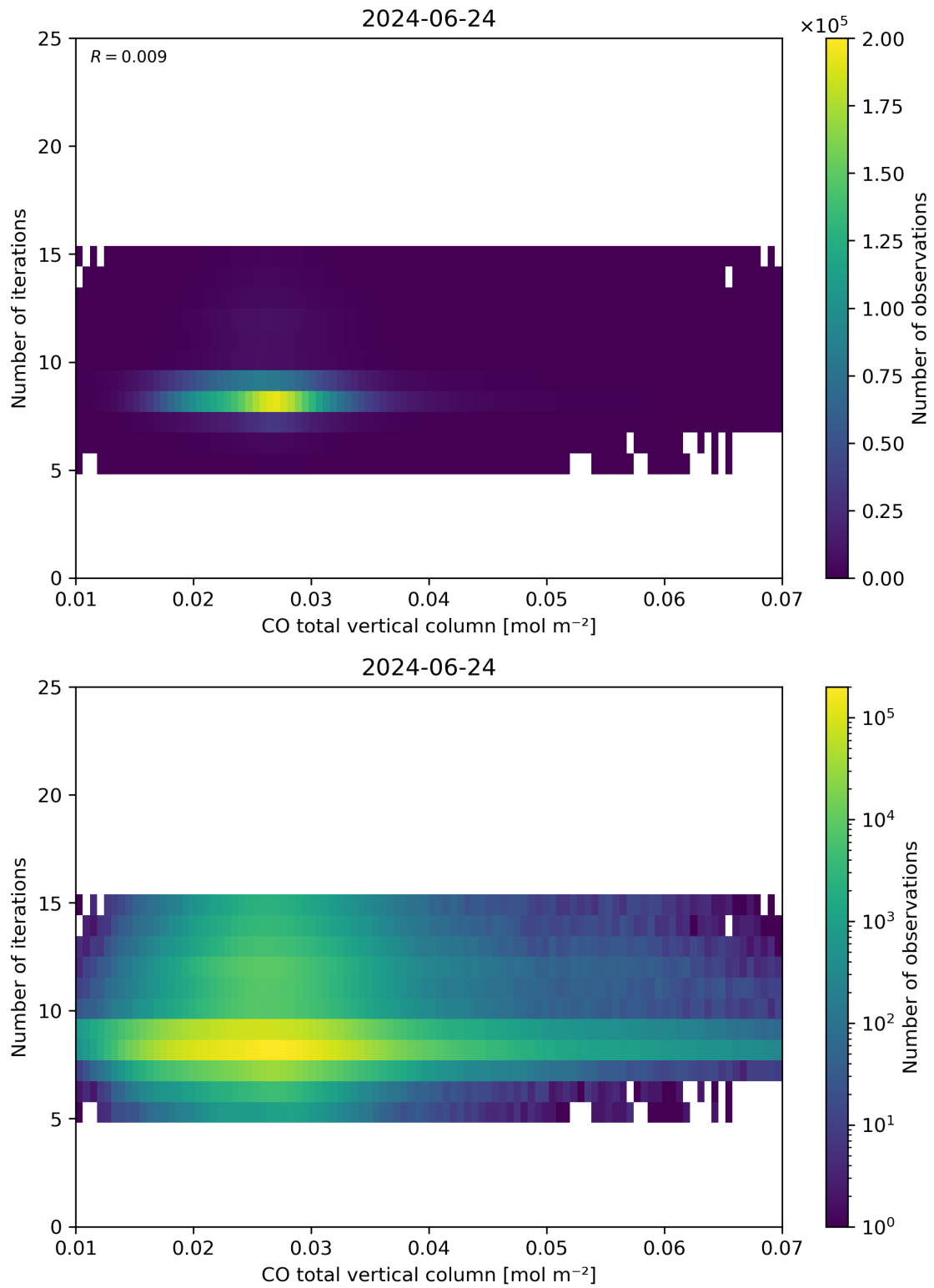
Figure 42: Scatter density plot of “CO total vertical column” against “Number of iterations” for 2024-06-24 to 2024-06-25.
