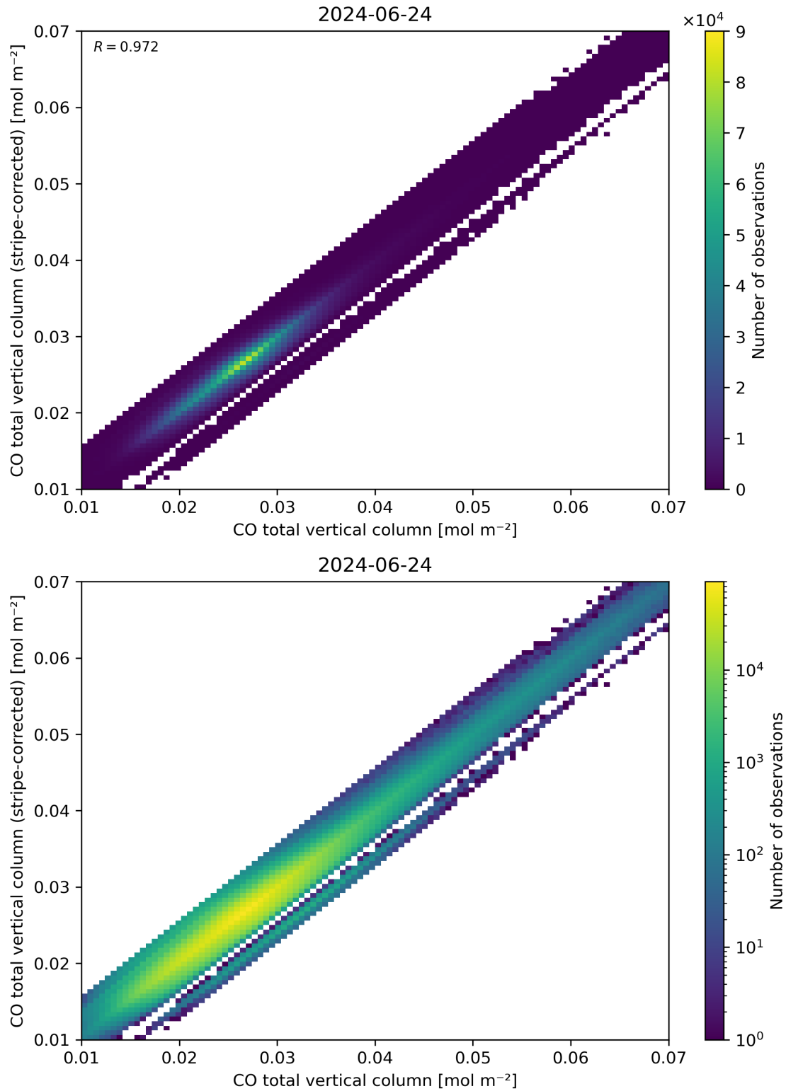
Figure 33: Scatter density plot of “CO total vertical column” against “CO total vertical column (stripe-corrected)” for 2024-06-24 to 2024-06-25.
