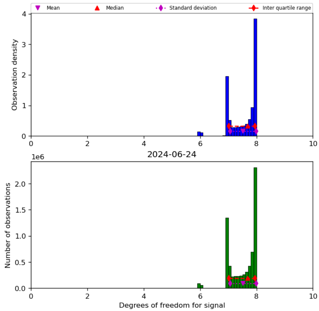
Figure 23: Histogram of “Degrees of freedom for signal” for 2024-06-24 to 2024-06-25
