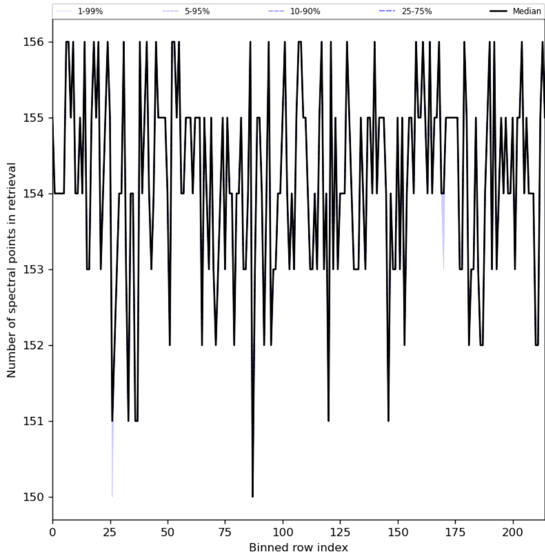
Figure 29: Along track statistics of “Number of spectral points in retrieval” for 2024-06-24 to 2024-06-25
