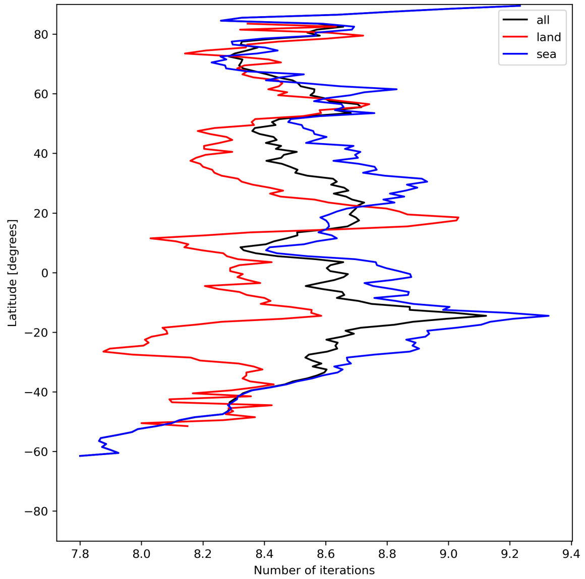
Figure 16: Zonal average of “Number of iterations” for 2024-06-24 to 2024-06-25.
