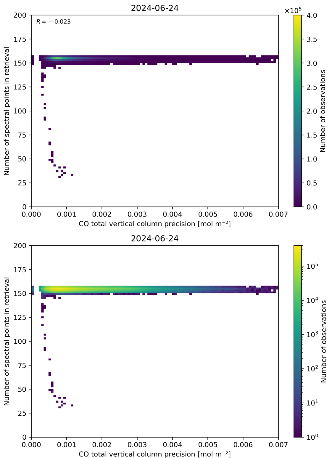
Figure 47: Scatter density plot of “CO total vertical column precision” against “Number of spectral points in retrieval” for 2024-06-24 to 2024-06-25.
