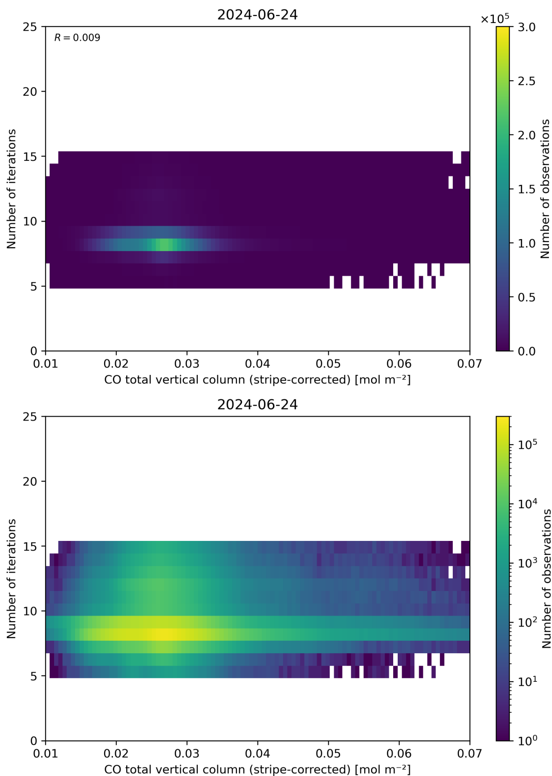
Figure 39: Scatter density plot of “CO total vertical column (stripe-corrected)” against “Number of iterations” for 2024-06-24 to 2024-06-25.
