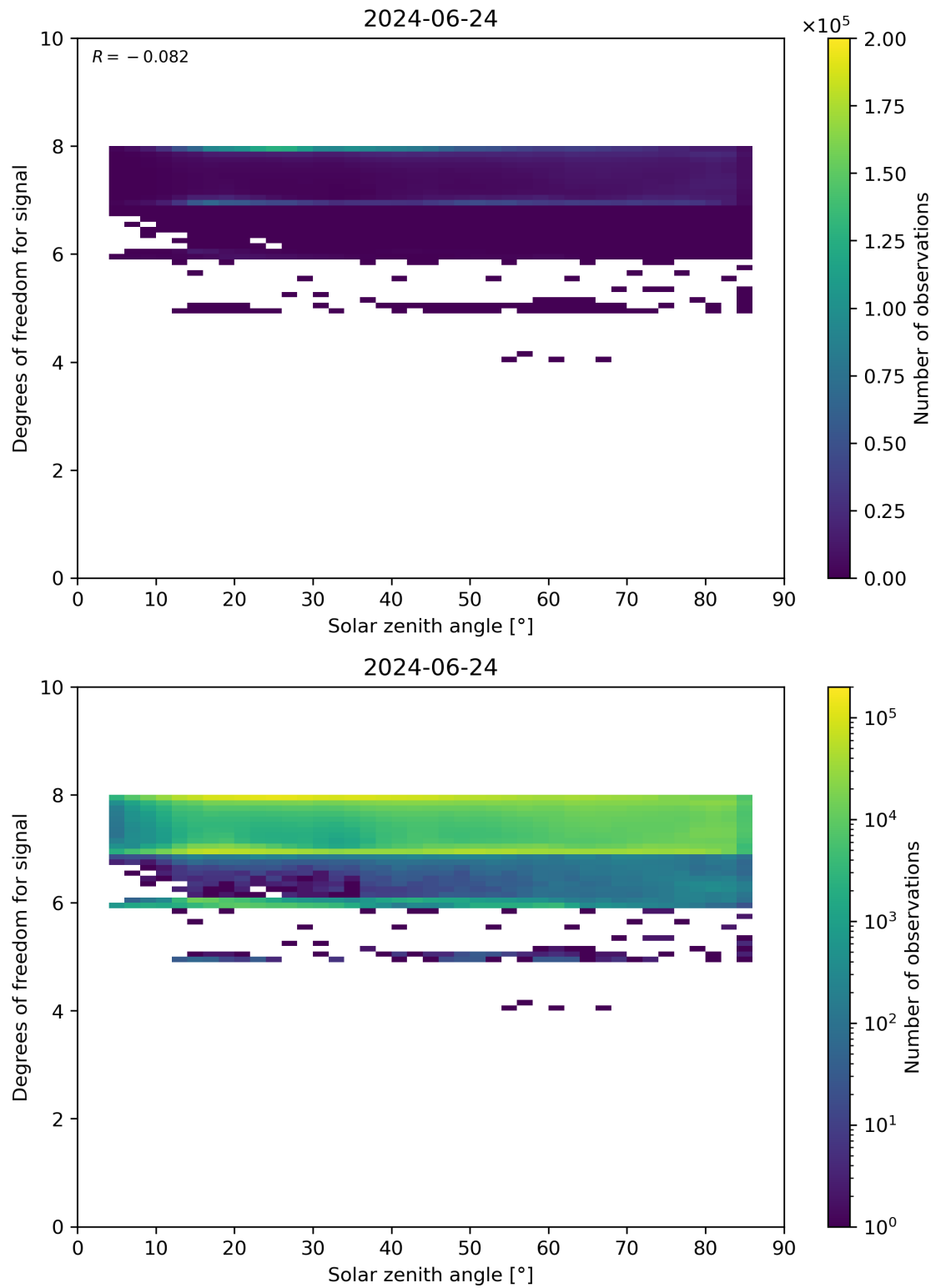
Figure 65: Scatter density plot of “Solar zenith angle” against “Degrees of freedom for signal” for 2024-06-24 to 2024-06-25.
