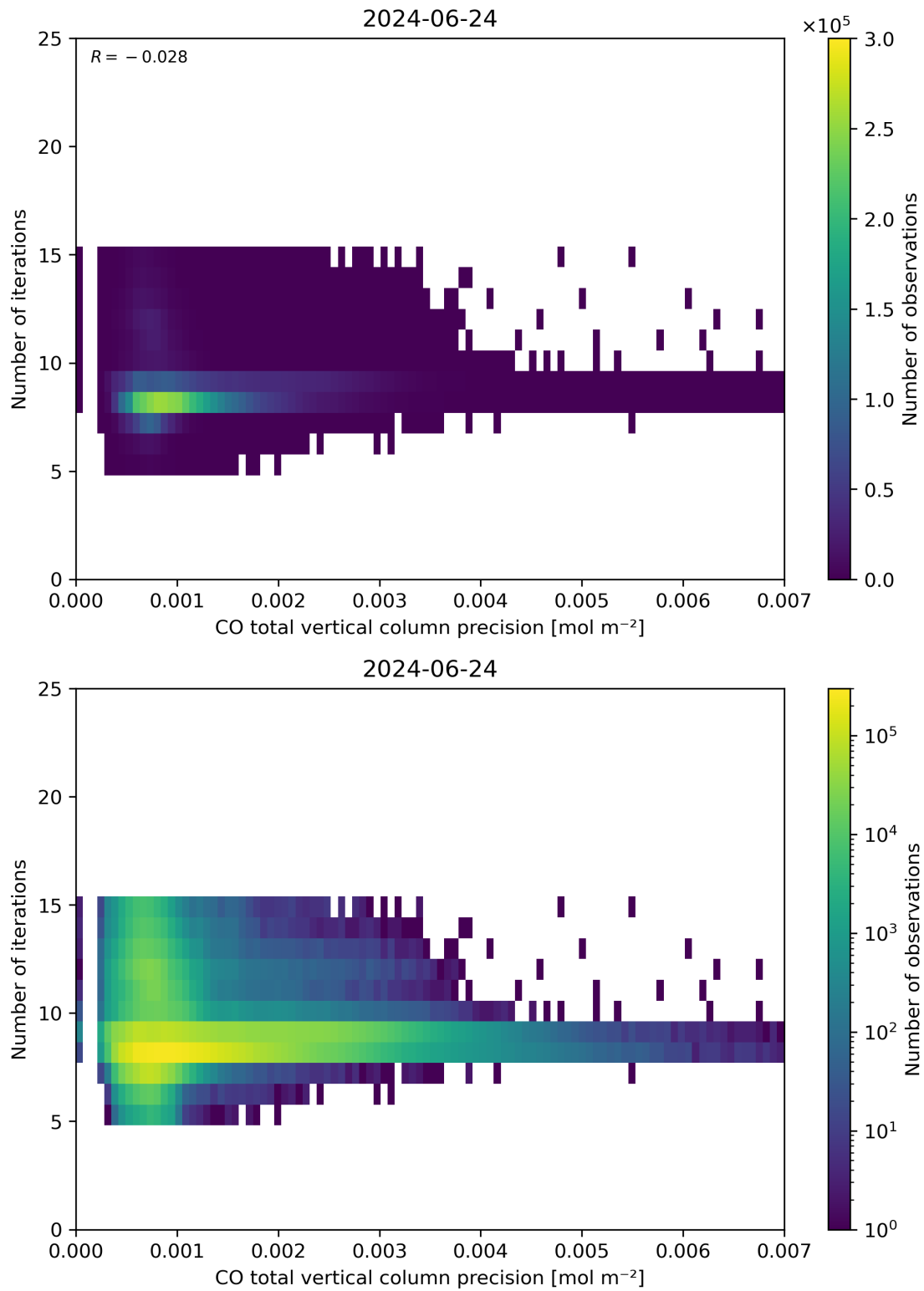
Figure 46: Scatter density plot of “CO total vertical column precision” against “Number of iterations” for 2024-06-24 to 2024-06-25.
