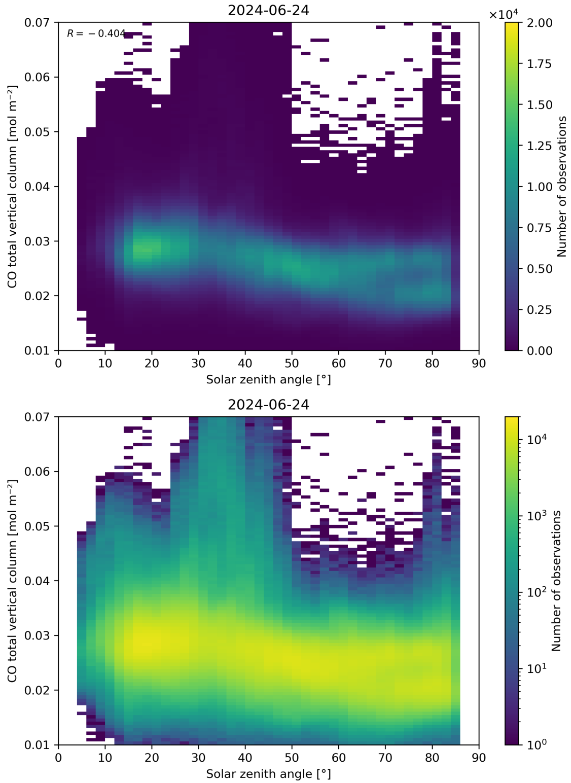
Figure 61: Scatter density plot of “Solar zenith angle” against “CO total vertical column” for 2024-06-24 to 2024-06-25.
