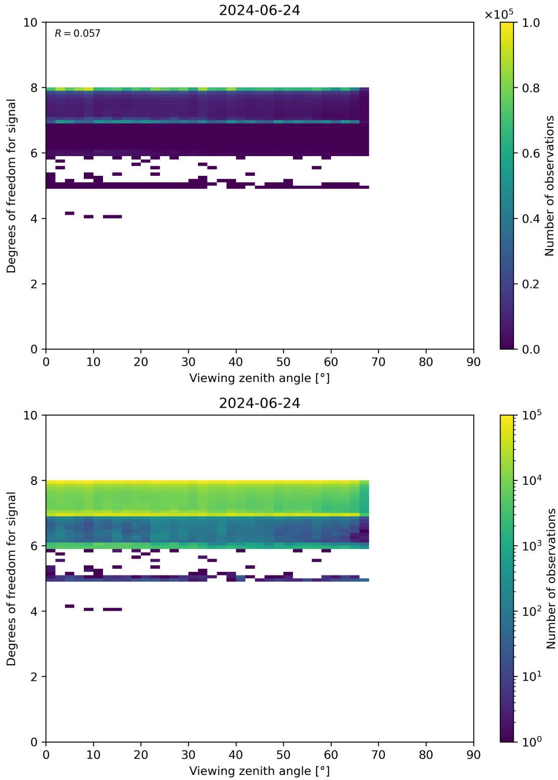
Figure 73: Scatter density plot of “Viewing zenith angle” against “Degrees of freedom for signal” for 2024-06-24 to 2024-06-25.
