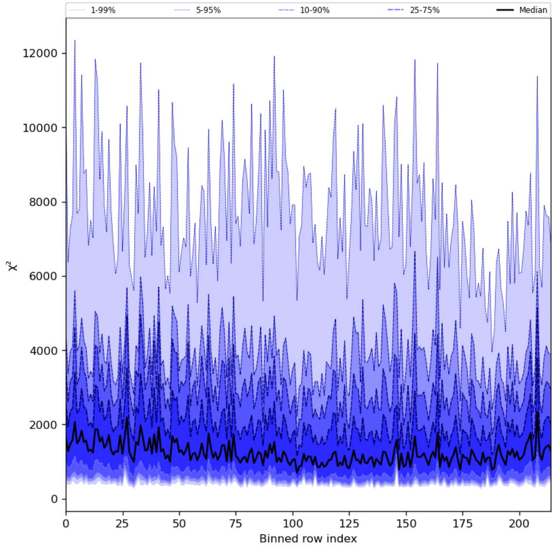
Figure 30: Along track statistics of “ \chi^2 ” for 2024-06-24 to 2024-06-25
