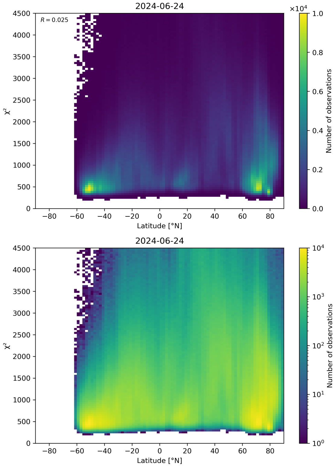
Figure 54: Scatter density plot of “Latitude” against “ \chi^2 ” for 2024-06-24 to 2024-06-25.
