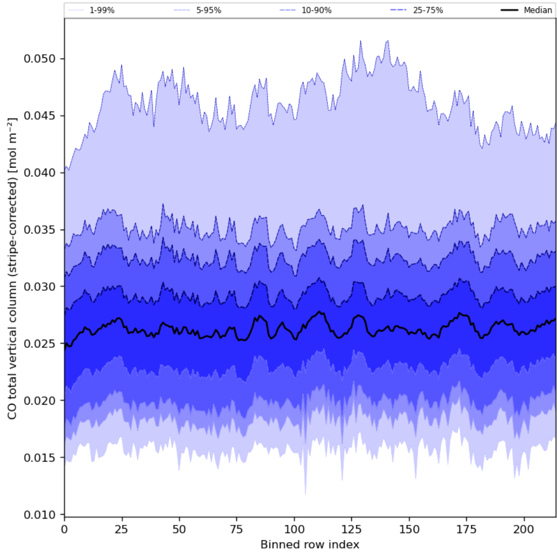
Figure 27: Along track statistics of “CO total vertical column (stripe-corrected)” for 2024-06-24 to 2024-06-25
