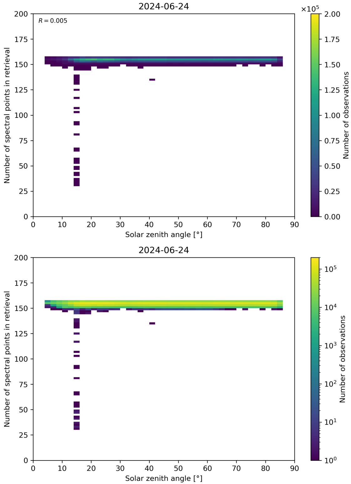
Figure 68: Scatter density plot of “Solar zenith angle” against “Number of spectral points in retrieval” for 2024-06-24 to 2024-06-25.
