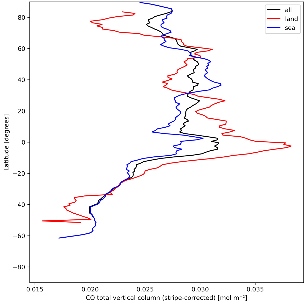
Figure 11: Zonal average of “CO total vertical column (stripe-corrected)” for 2024-06-24 to 2024-06-25.
