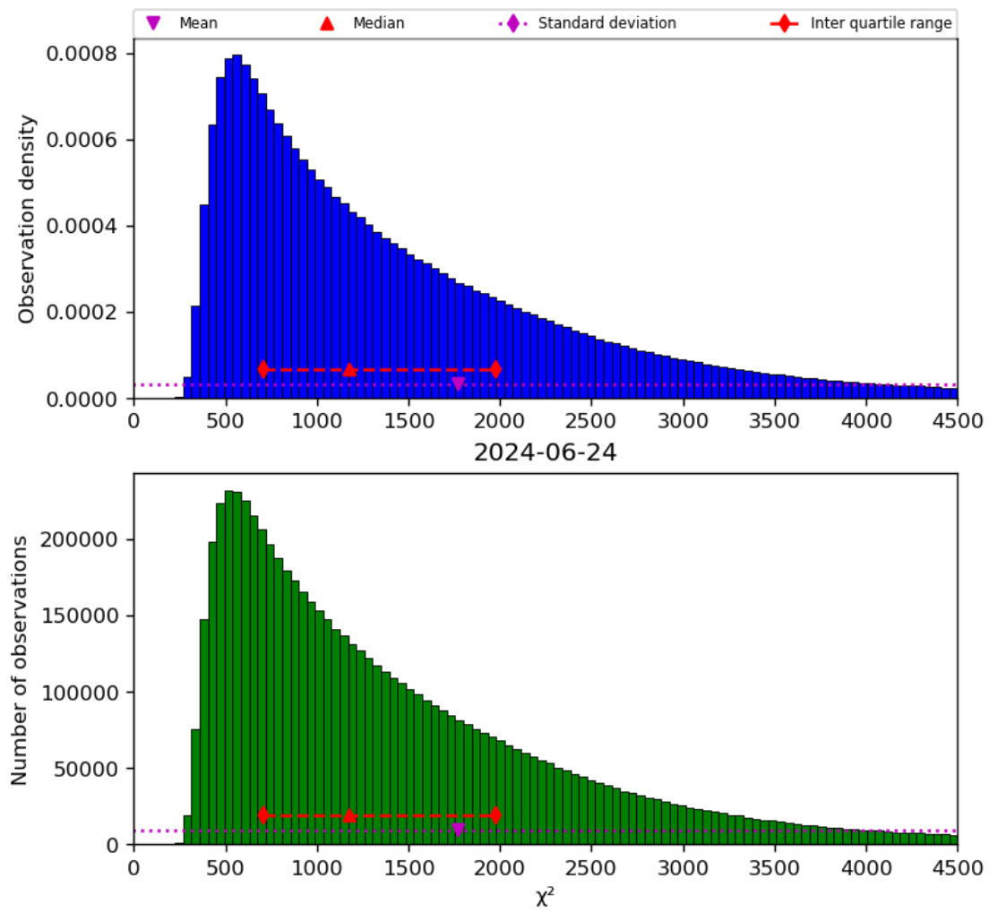
Figure 22: Histogram of “ \chi^2 ” for 2024-06-24 to 2024-06-25
