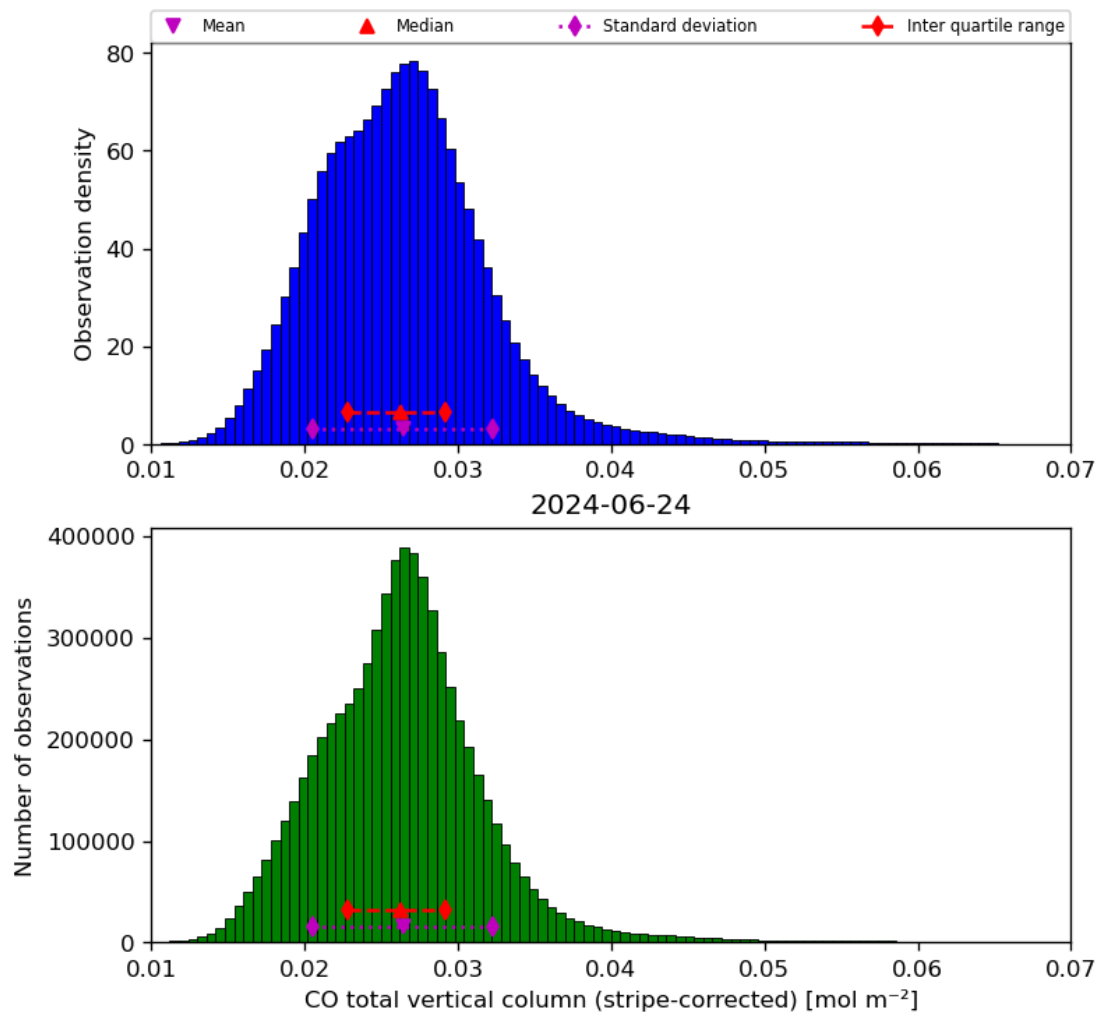
Figure 19: Histogram of “CO total vertical column (stripe-corrected)” for 2024-06-24 to 2024-06-25
