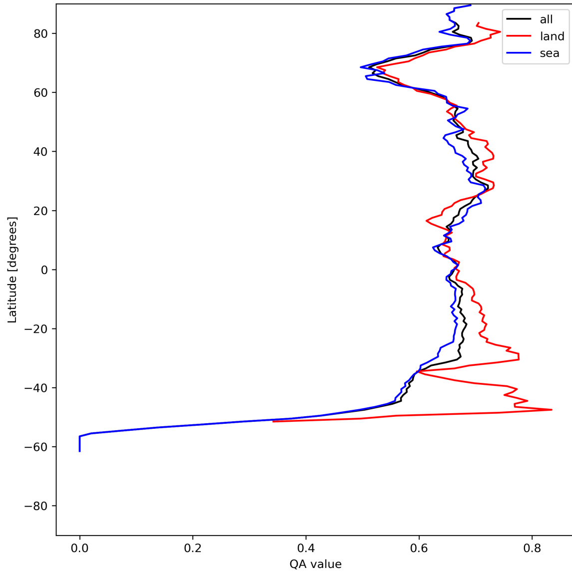
Figure 9: Zonal average of “QA value” for 2024-06-24 to 2024-06-25.
