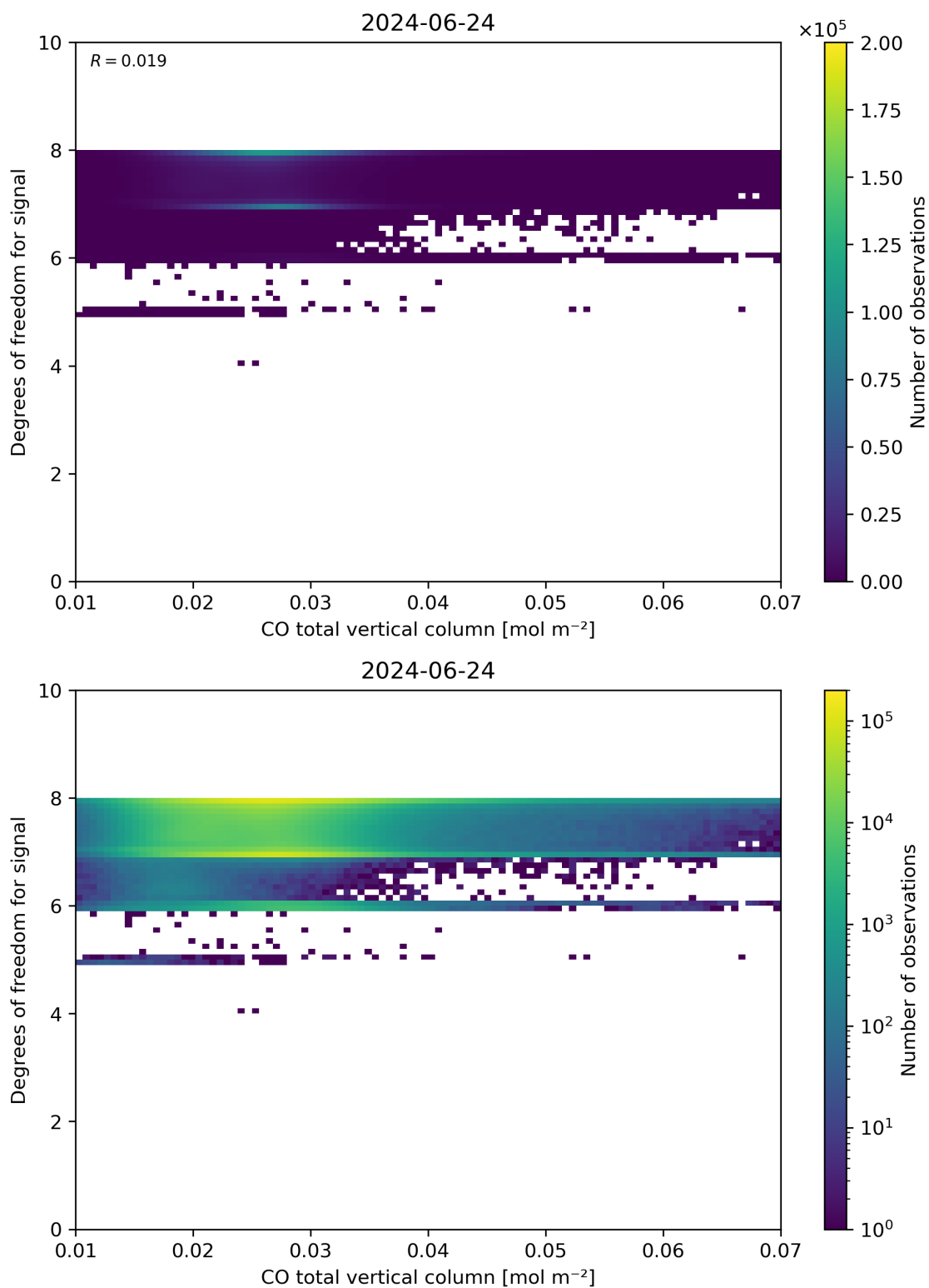
Figure 41: Scatter density plot of “CO total vertical column” against “Degrees of freedom for signal” for 2024-06-24 to 2024-06-25.
