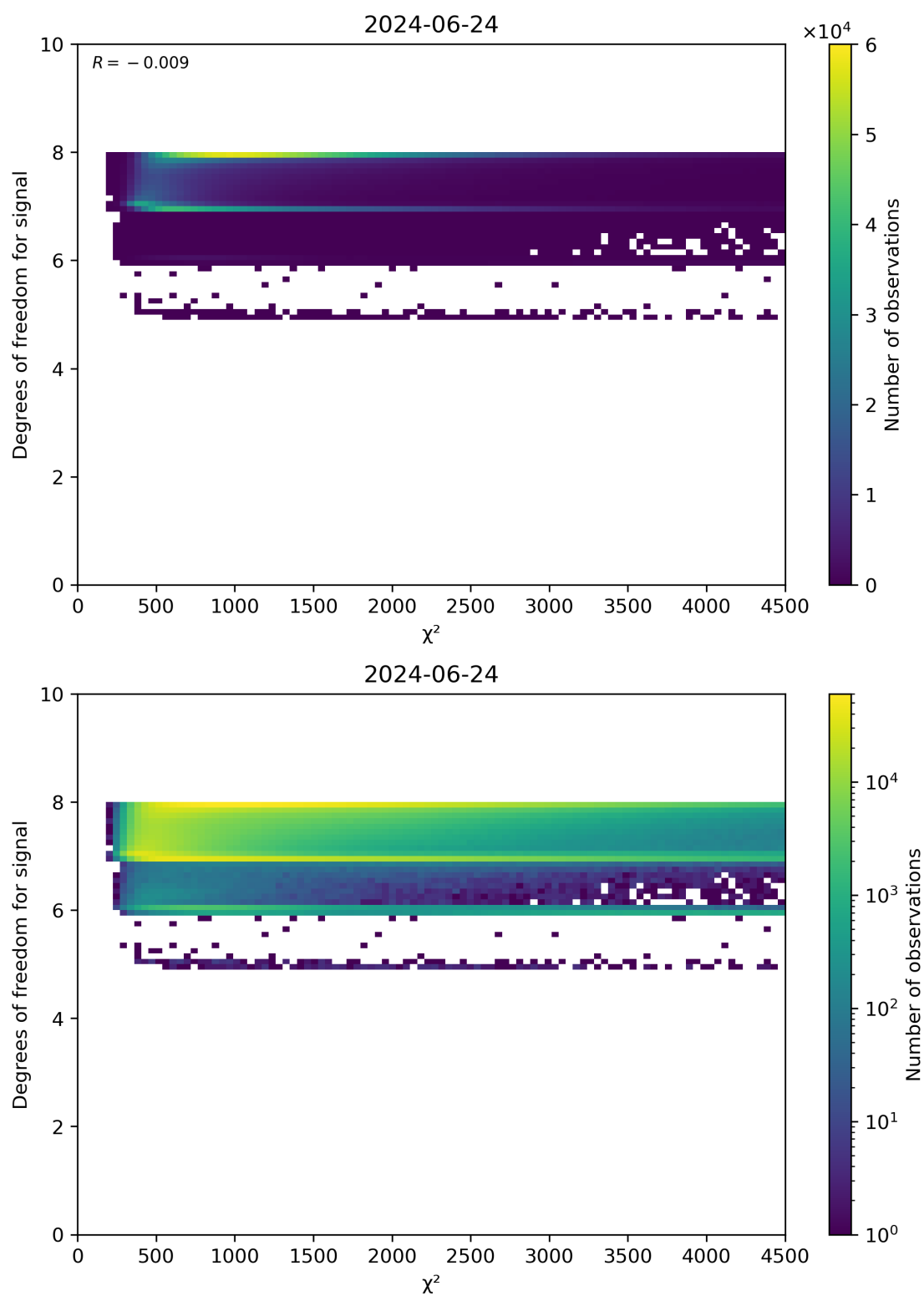
Figure 48: Scatter density plot of “ \chi^2 ” against “Degrees of freedom for signal” for 2024-06-24 to 2024-06-25.
