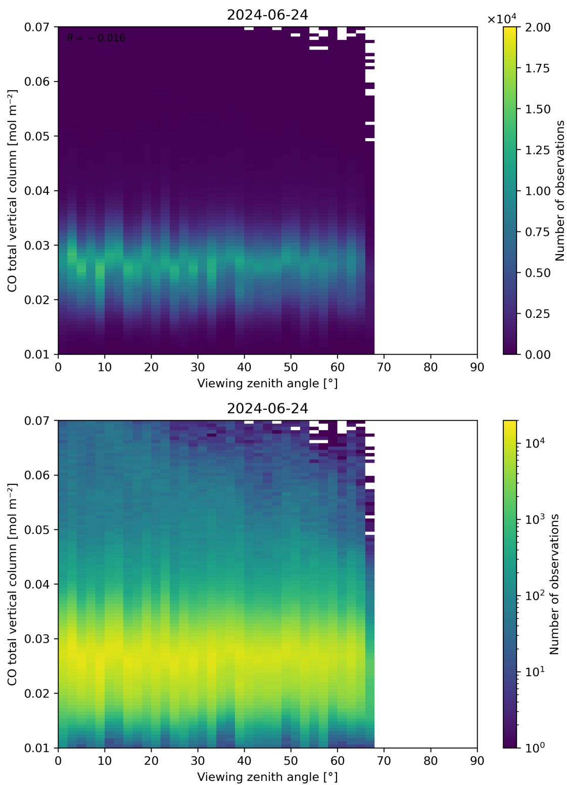
Figure 69: Scatter density plot of “Viewing zenith angle” against “CO total vertical column” for 2024-06-24 to 2024-06-25.
