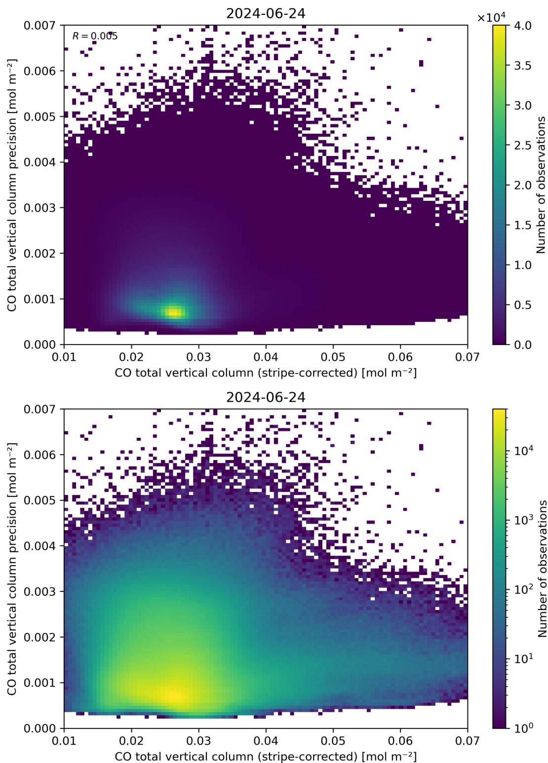
Figure 36: Scatter density plot of “CO total vertical column (stripe-corrected)” against “CO total vertical column precision” for 2024-06-24 to 2024-06-25.
