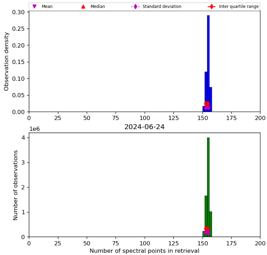
Figure 21: Histogram of “Number of spectral points in retrieval” for 2024-06-24 to 2024-06-25
