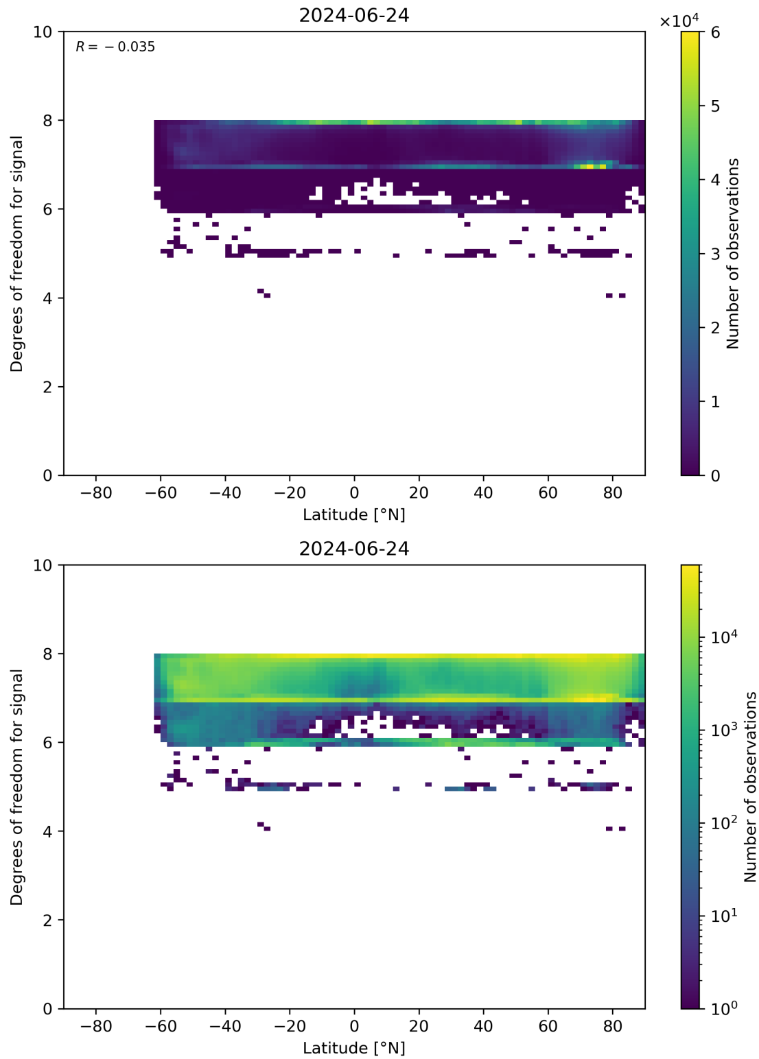
Figure 55: Scatter density plot of “Latitude” against “Degrees of freedom for signal” for 2024-06-24 to 2024-06-25.
