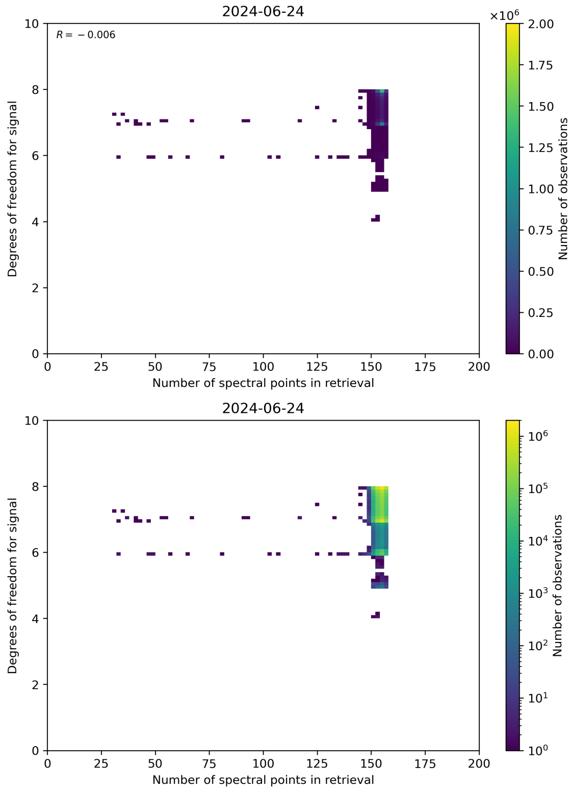
Figure 59: Scatter density plot of “Number of spectral points in retrieval” against “Degrees of freedom for signal” for 2024-06-24 to 2024-06-25.
