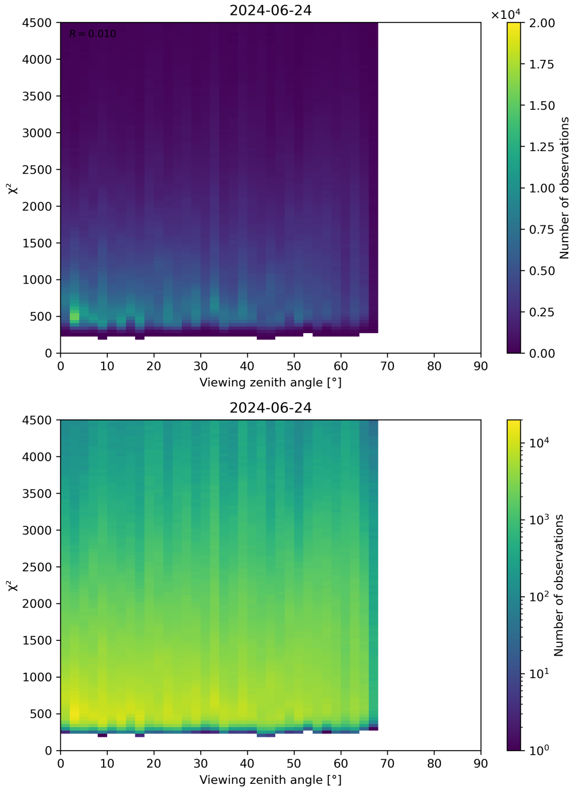
Figure 72: Scatter density plot of “Viewing zenith angle” against “ \chi^2 ” for 2024-06-24 to 2024-06-25.
