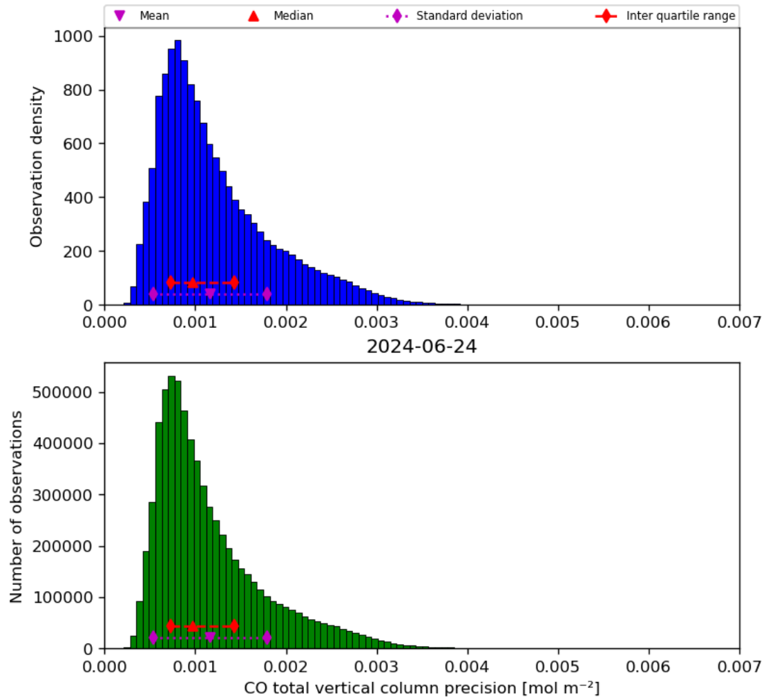
Figure 20: Histogram of “CO total vertical column precision” for 2024-06-24 to 2024-06-25
