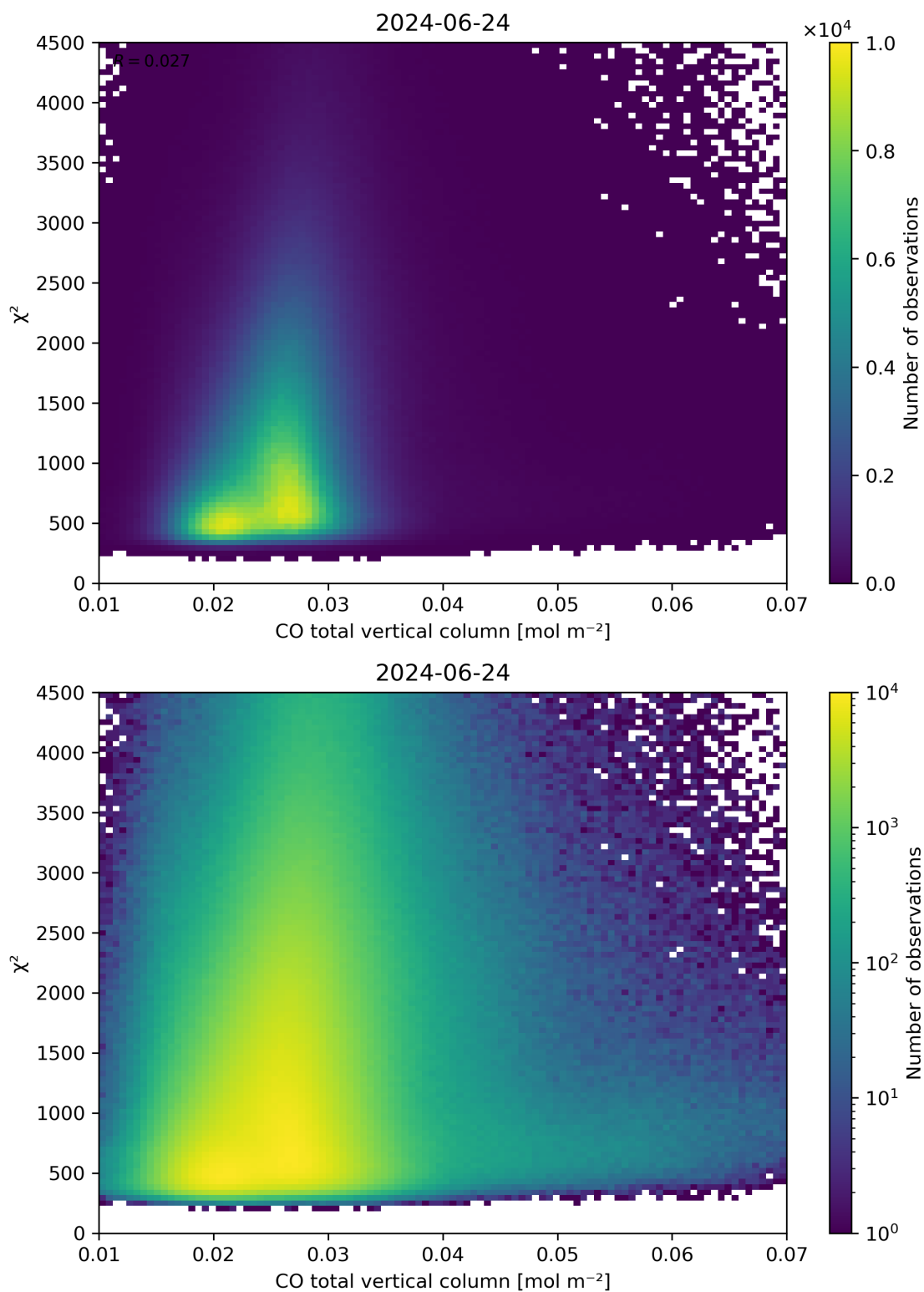
Figure 35: Scatter density plot of “CO total vertical column” against “ \chi^2 ” for 2024-06-24 to 2024-06-25.
