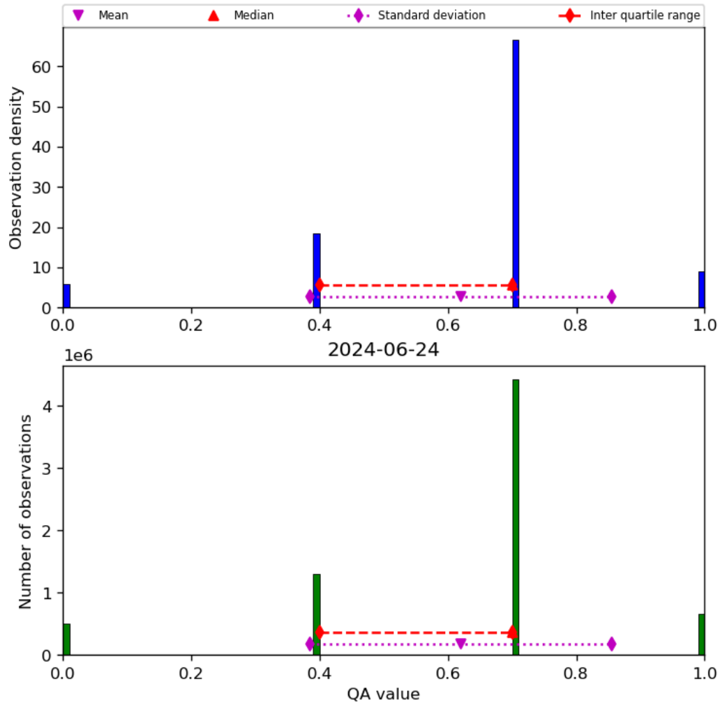
Figure 17: Histogram of “QA value” for 2024-06-24 to 2024-06-25
