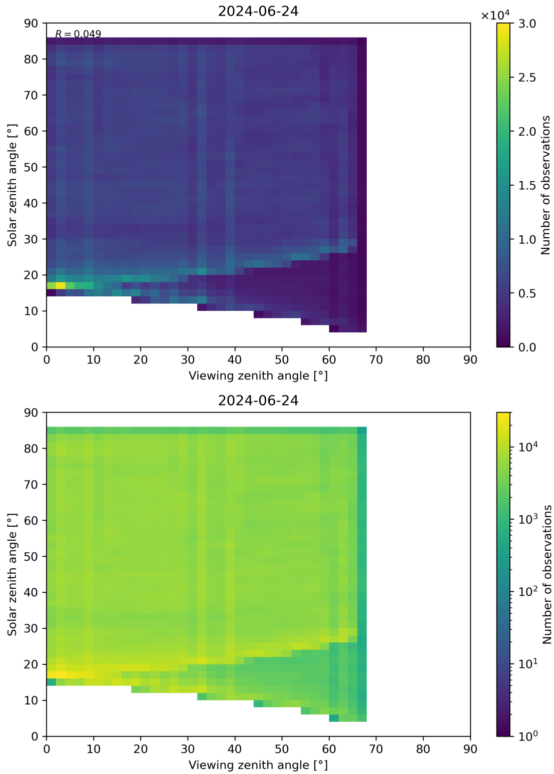
Figure 77: Scatter density plot of “Viewing zenith angle” against “Solar zenith angle” for 2024-06-24 to 2024-06-25.
