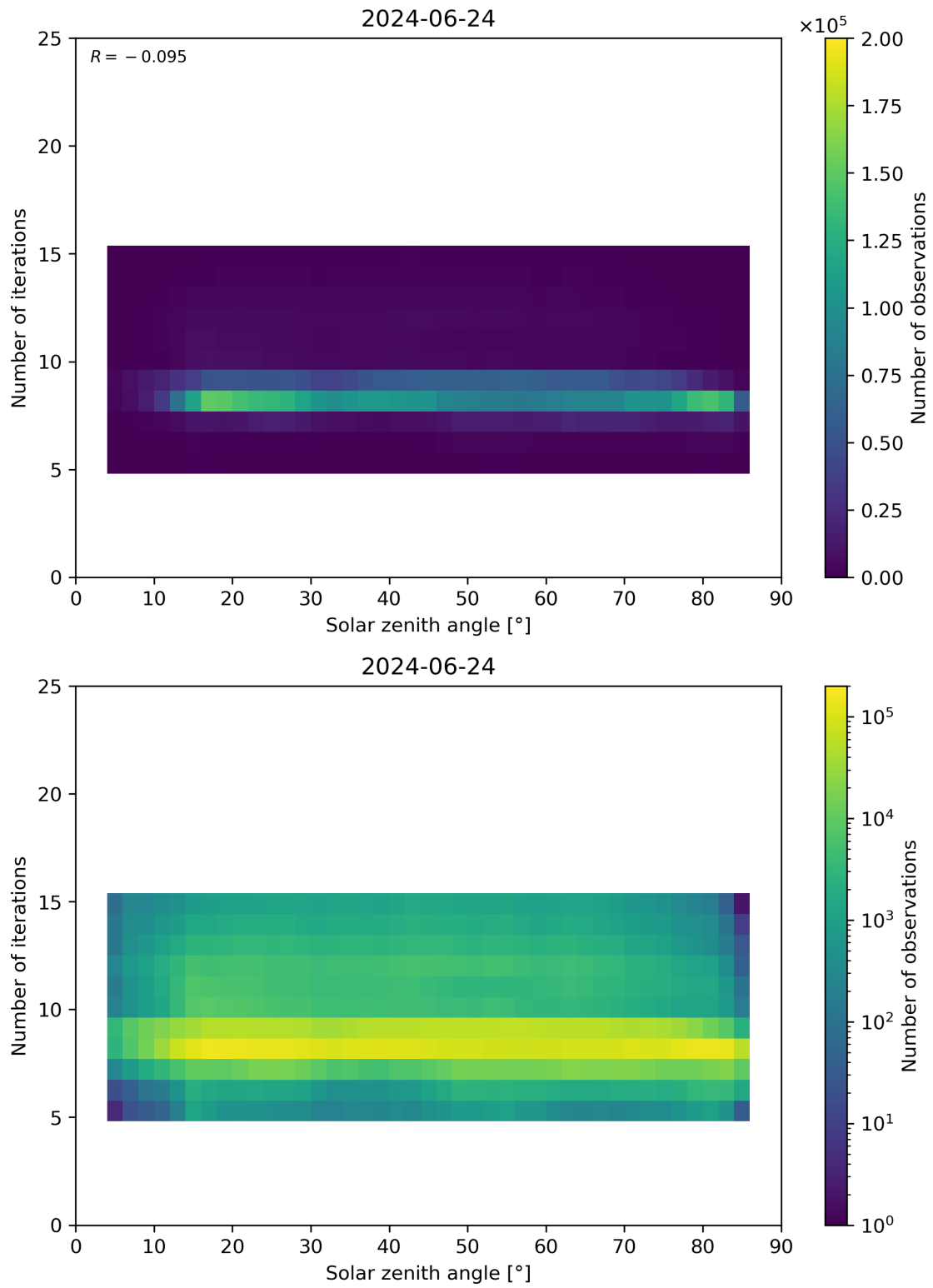
Figure 67: Scatter density plot of “Solar zenith angle” against “Number of iterations” for 2024-06-24 to 2024-06-25.
