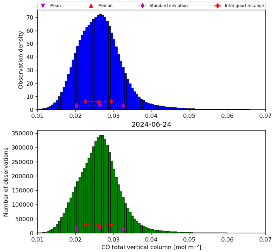
Figure 18: Histogram of “CO total vertical column” for 2024-06-24 to 2024-06-25
