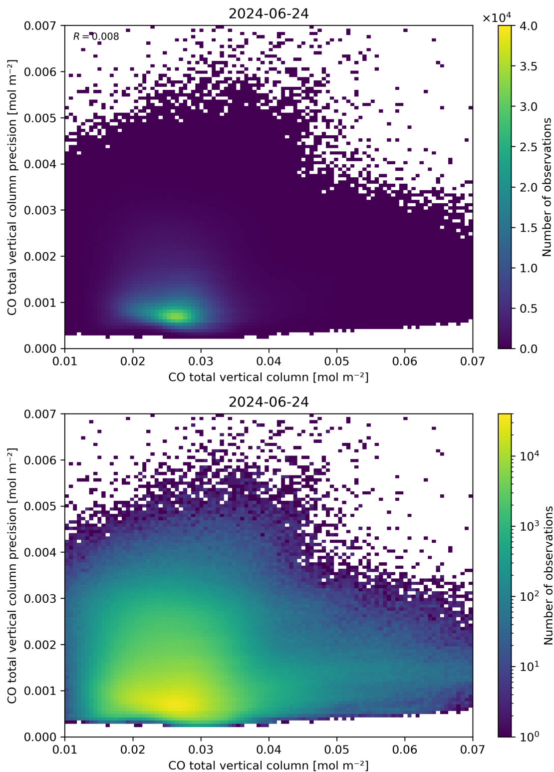
Figure 34: Scatter density plot of “CO total vertical column” against “CO total vertical column precision” for 2024-06-24 to 2024-06-25.
