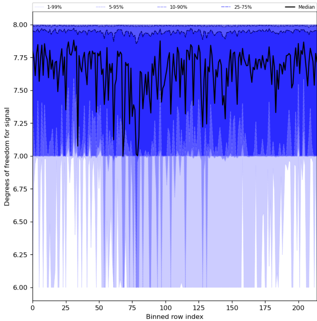
Figure 31: Along track statistics of “Degrees of freedom for signal” for 2024-06-24 to 2024-06-25
