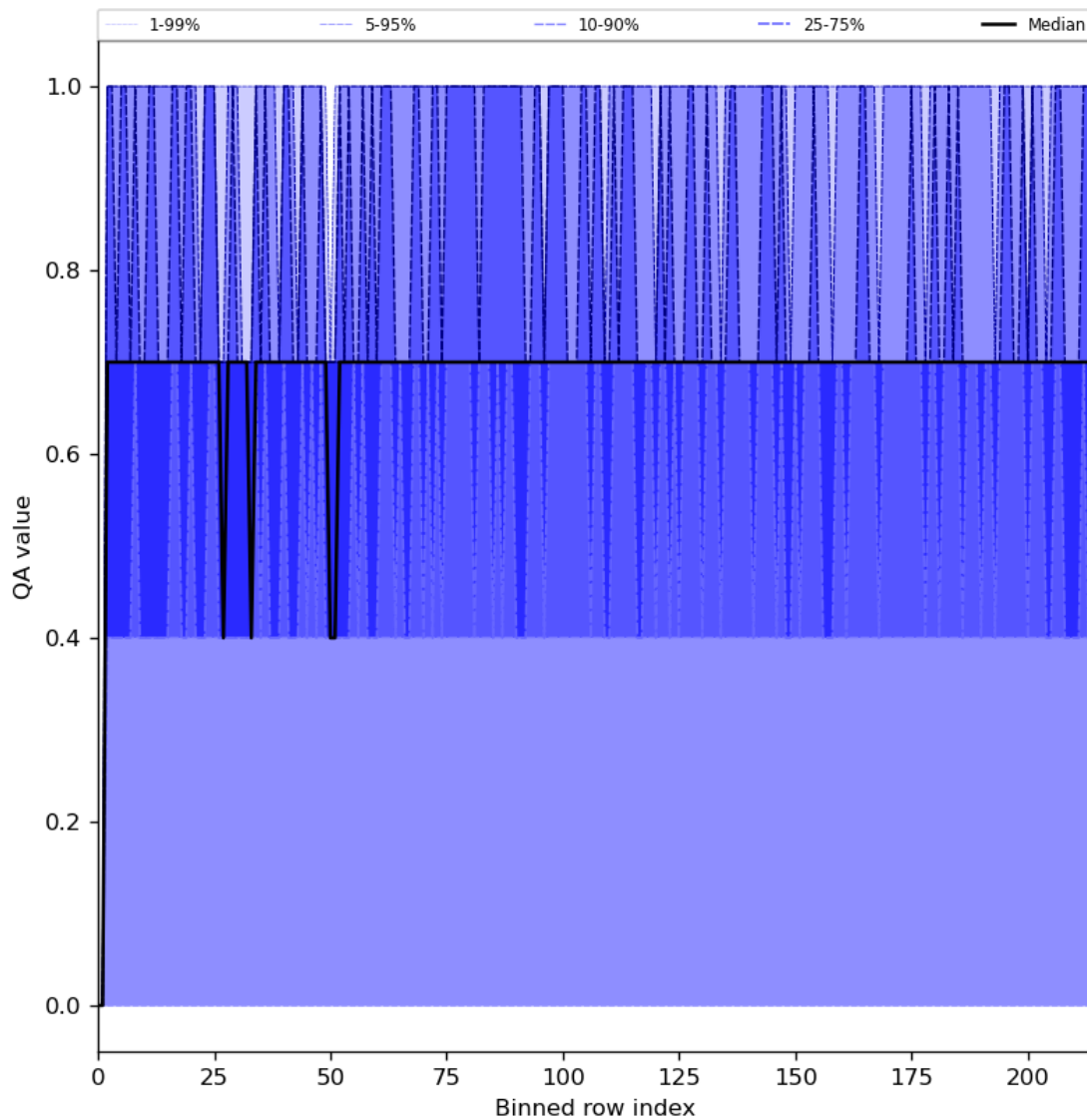
Figure 25: Along track statistics of “QA value” for 2024-06-24 to 2024-06-25
