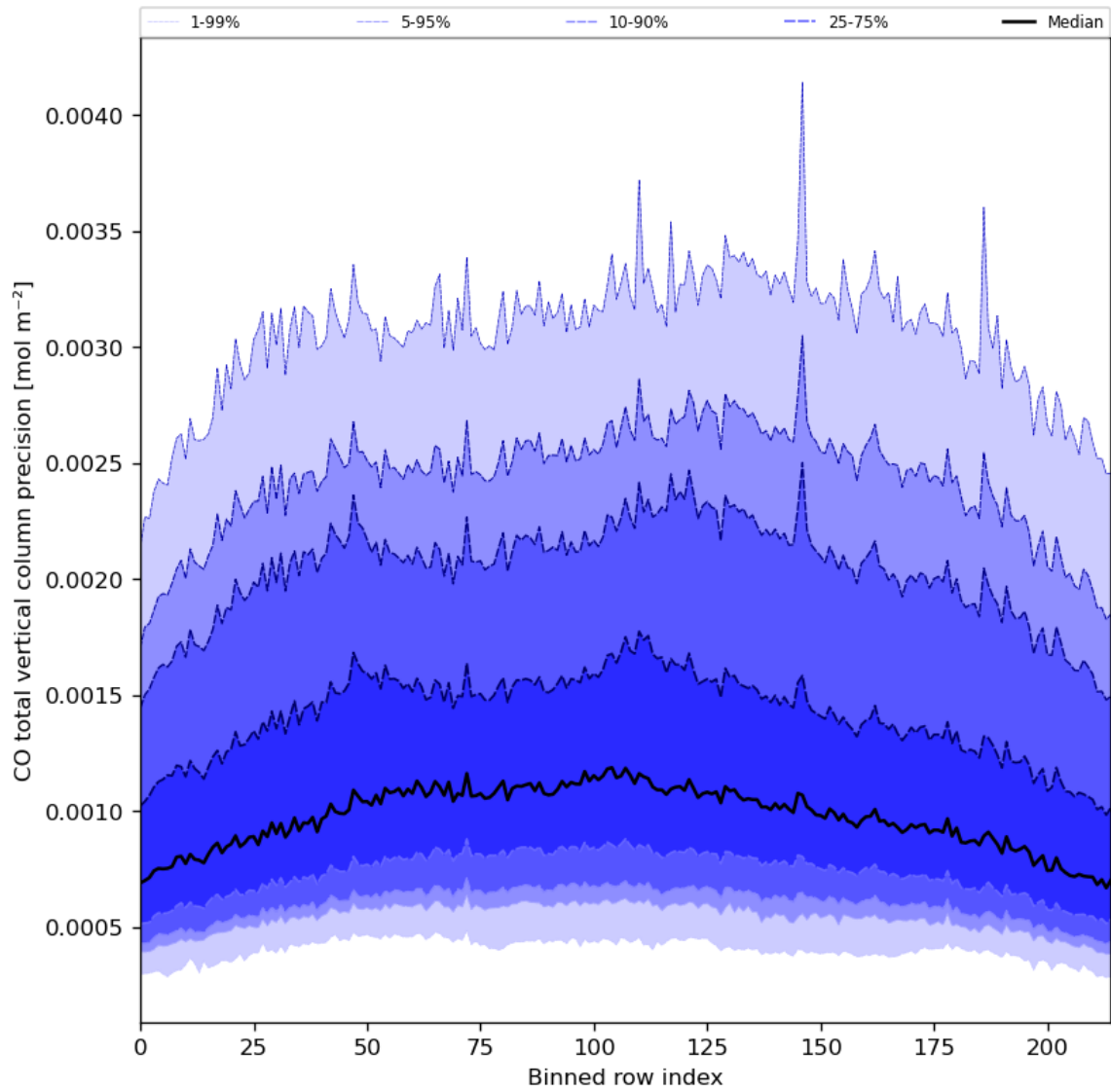
Figure 28: Along track statistics of “CO total vertical column precision” for 2024-06-24 to 2024-06-25
