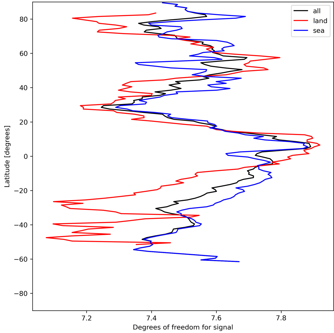
Figure 15: Zonal average of “Degrees of freedom for signal” for 2024-06-24 to 2024-06-25.
