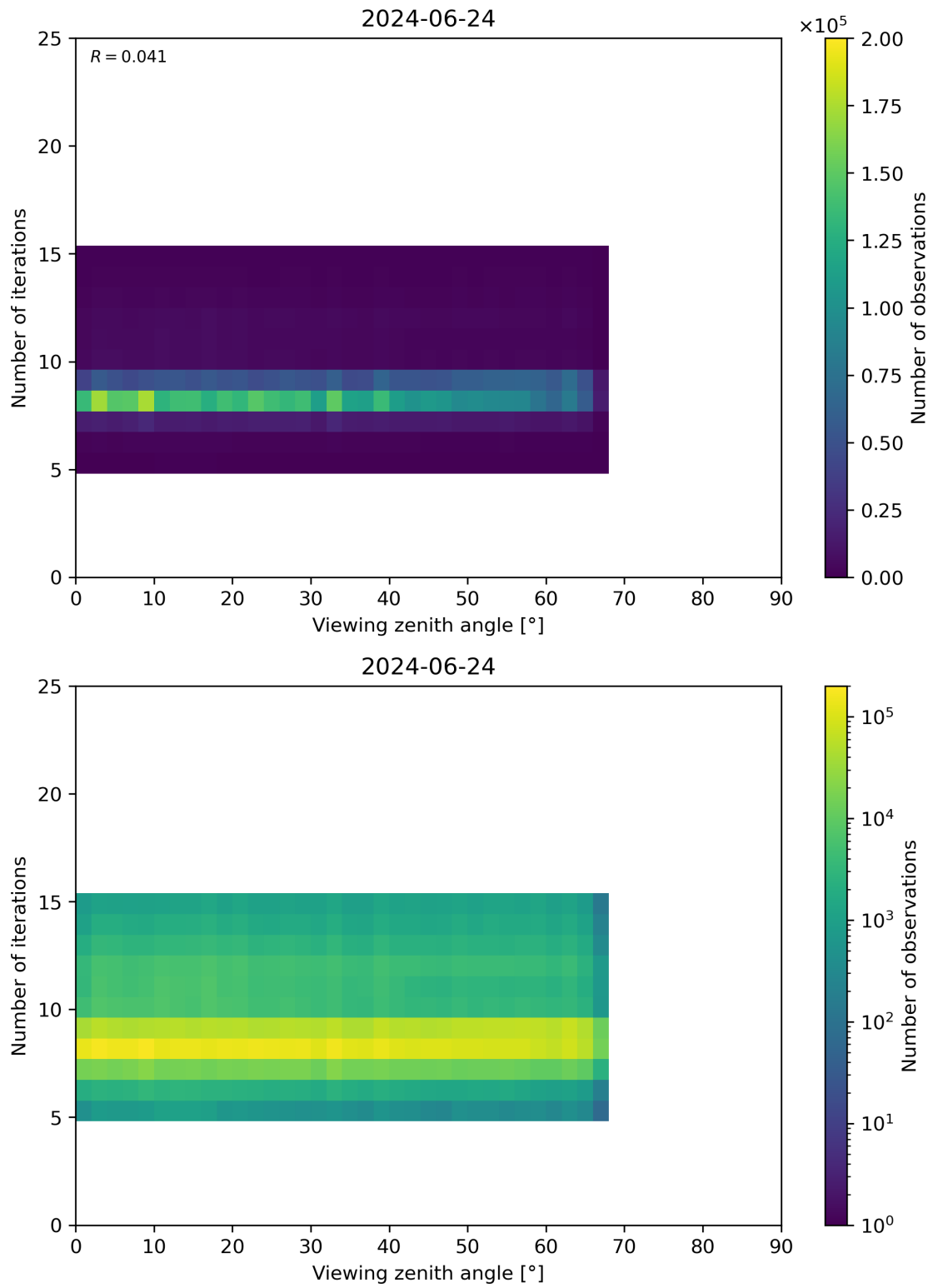
Figure 75: Scatter density plot of “Viewing zenith angle” against “Number of iterations” for 2024-06-24 to 2024-06-25.
