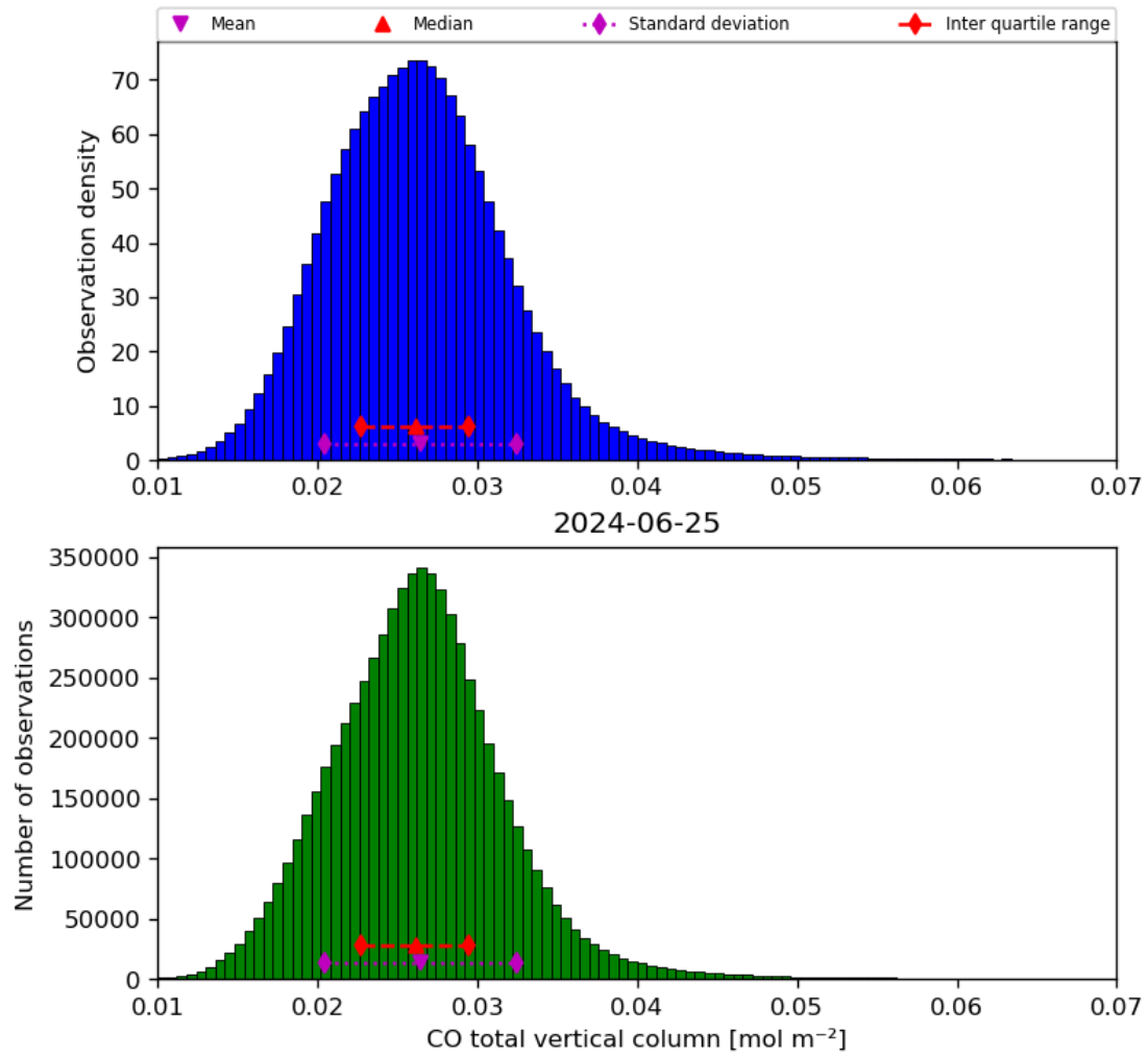
Figure 18: Histogram of “CO total vertical column” for 2024-06-24 to 2024-06-26
