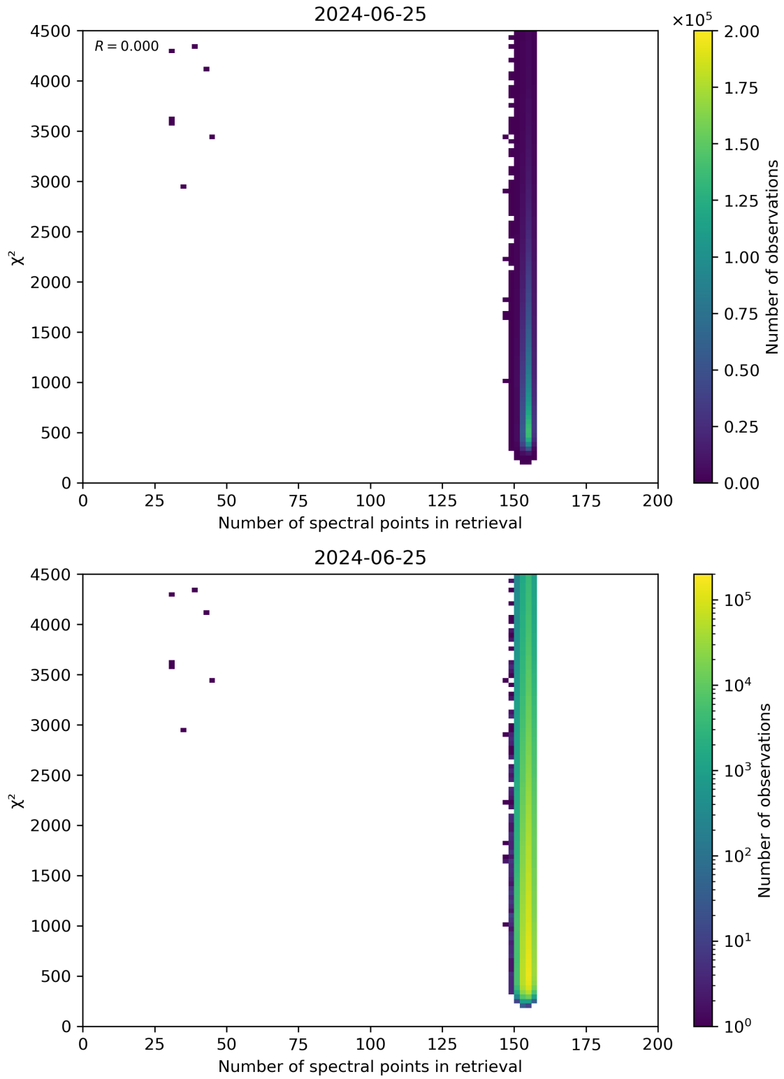
Figure 58: Scatter density plot of “Number of spectral points in retrieval” against “ \chi^2 ” for 2024-06-24 to 2024-06-26.
