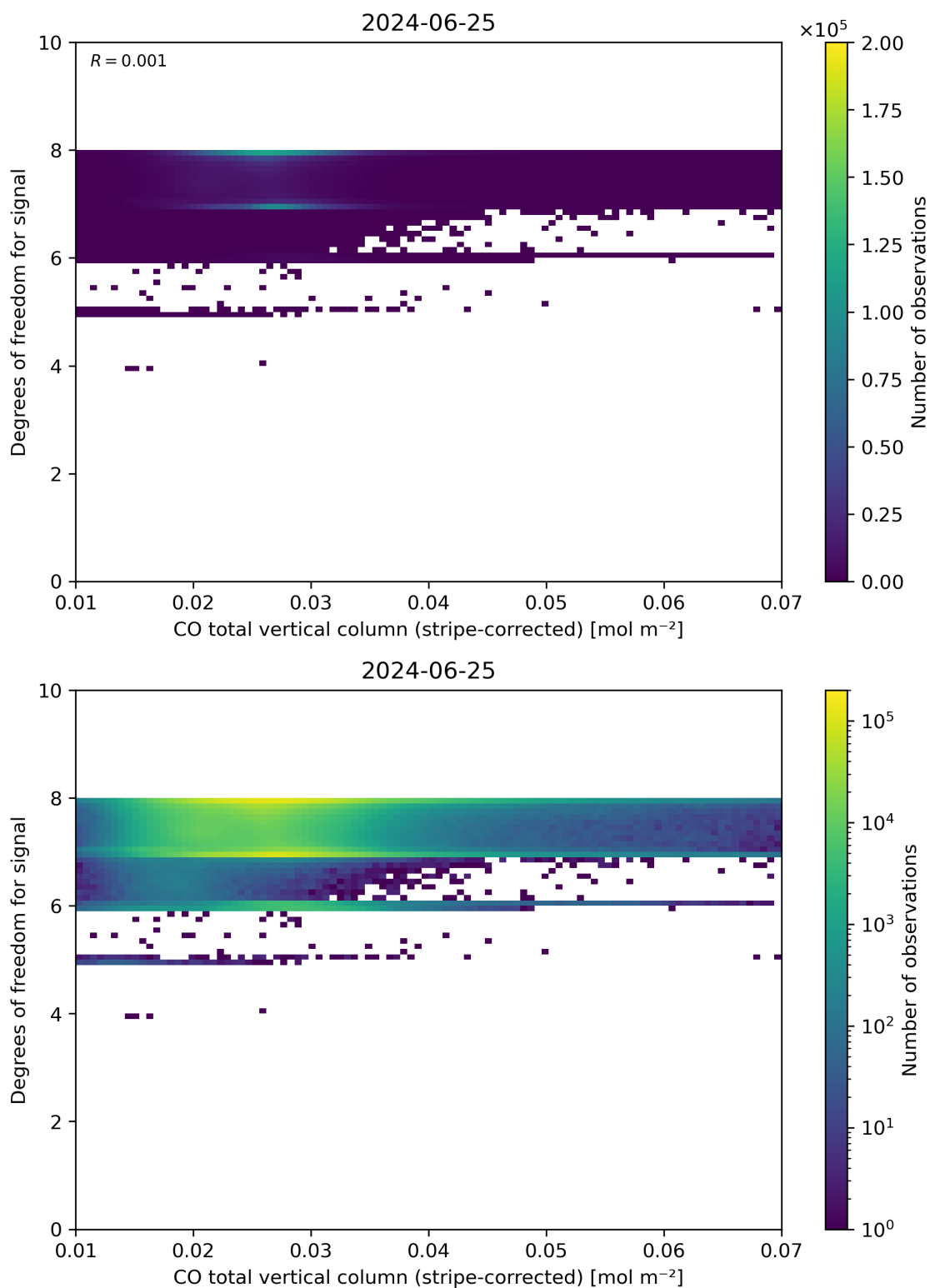
Figure 38: Scatter density plot of “CO total vertical column (stripe-corrected)” against “Degrees of freedom for signal” for 2024-06-24 to 2024-06-26.
