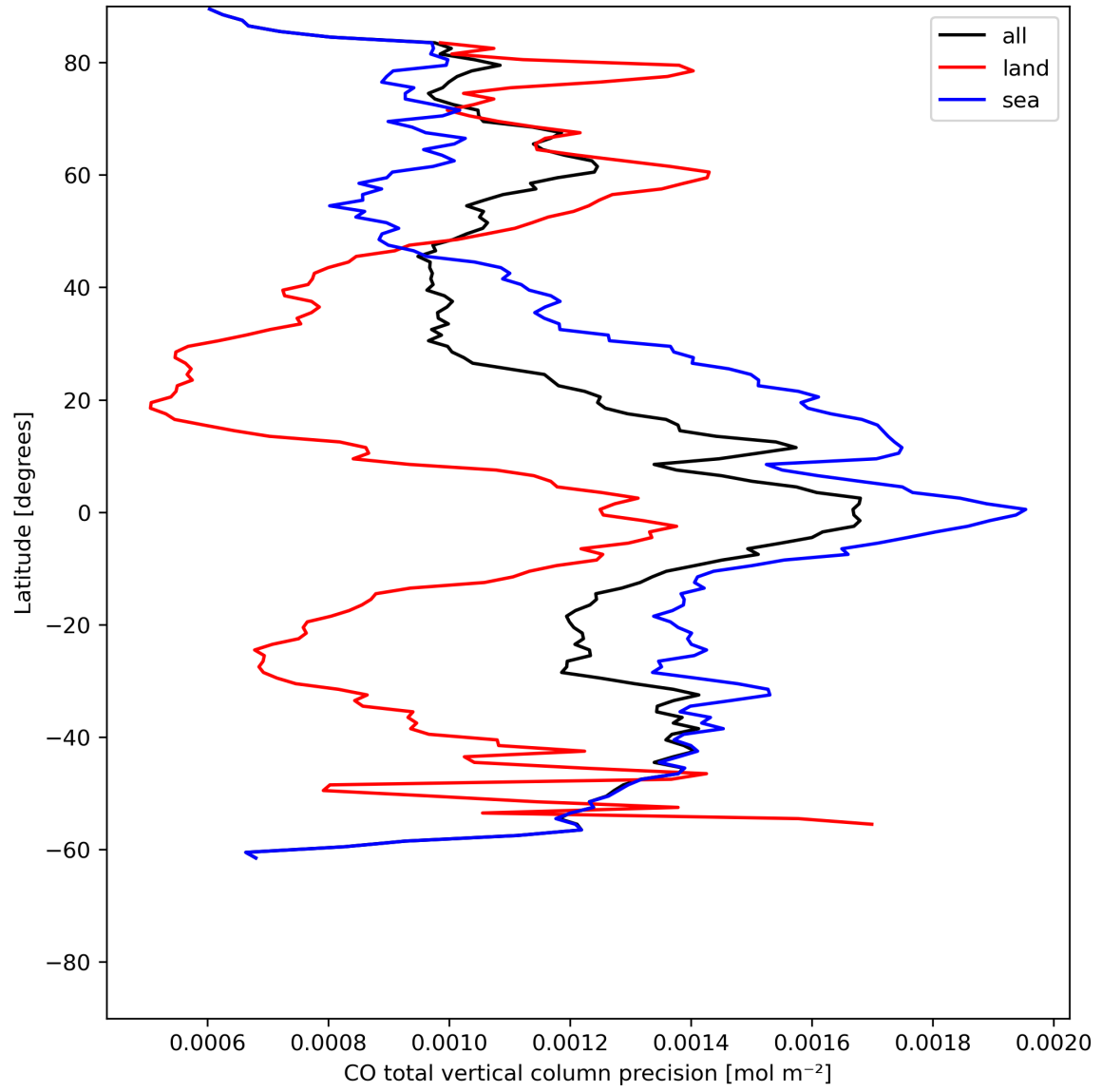
Figure 12: Zonal average of “CO total vertical column precision” for 2024-06-24 to 2024-06-26.
