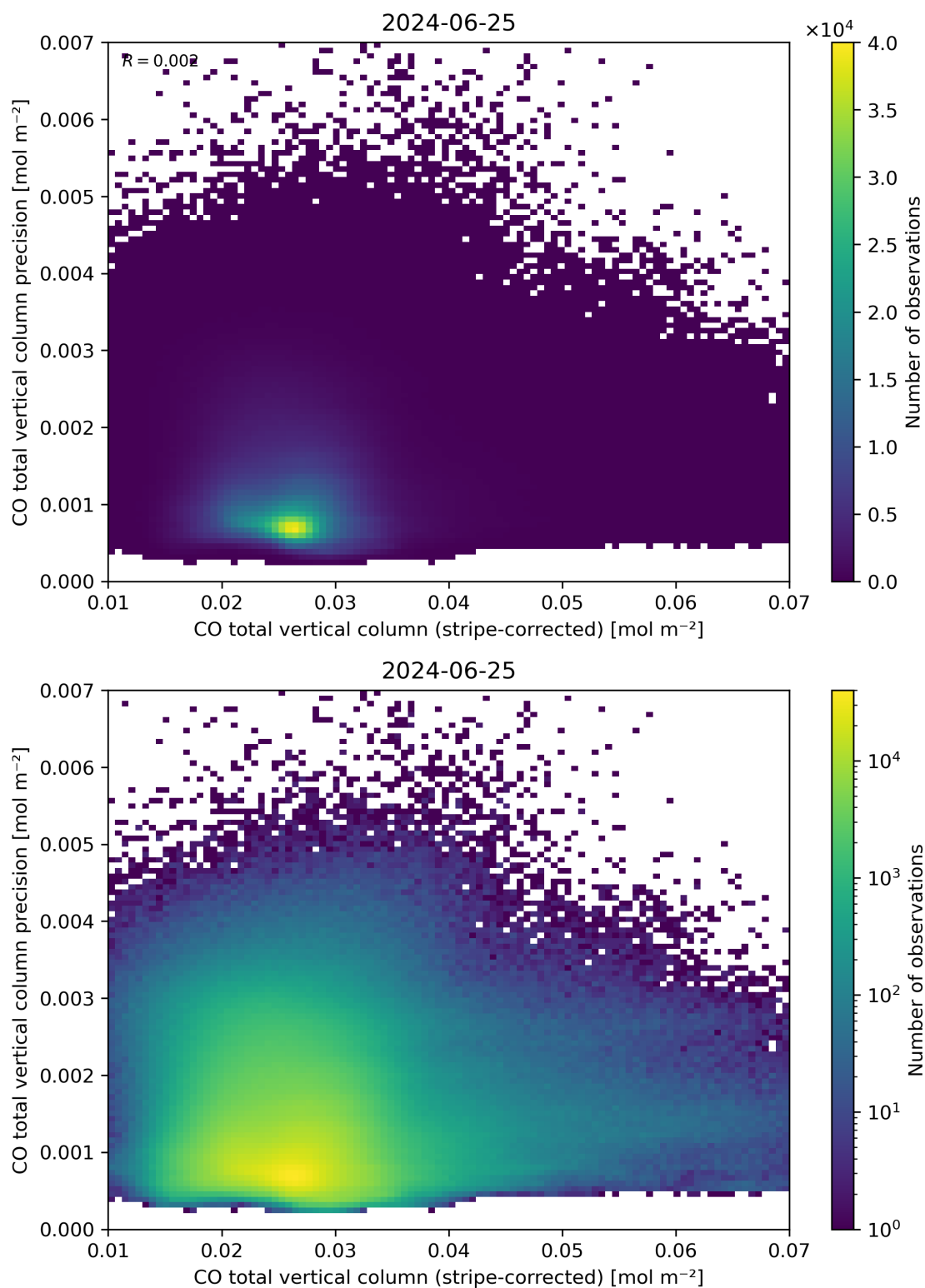
Figure 36: Scatter density plot of “CO total vertical column (stripe-corrected)” against “CO total vertical column precision” for 2024-06-24 to 2024-06-26.
