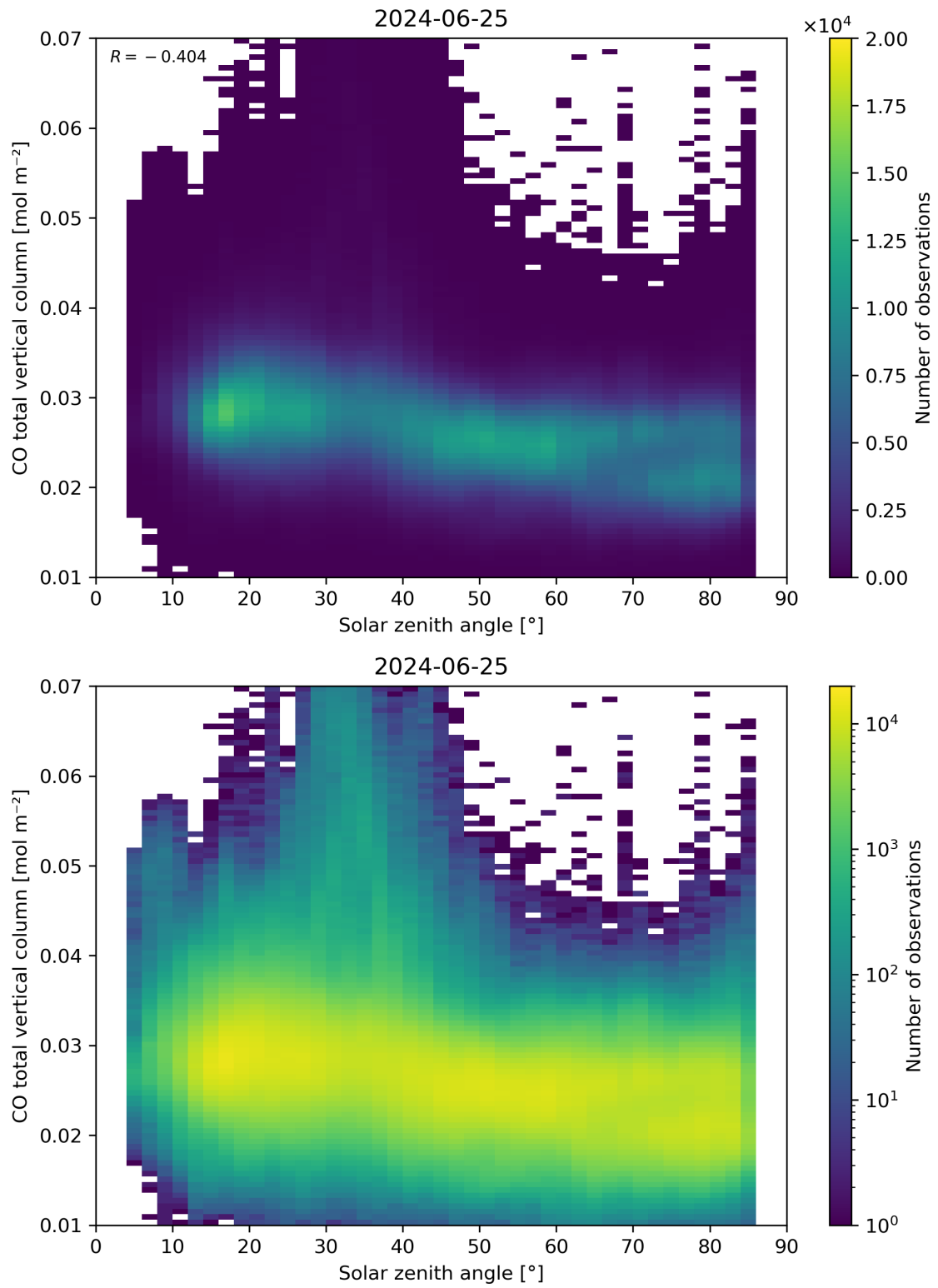
Figure 61: Scatter density plot of “Solar zenith angle” against “CO total vertical column” for 2024-06-24 to 2024-06-26.
