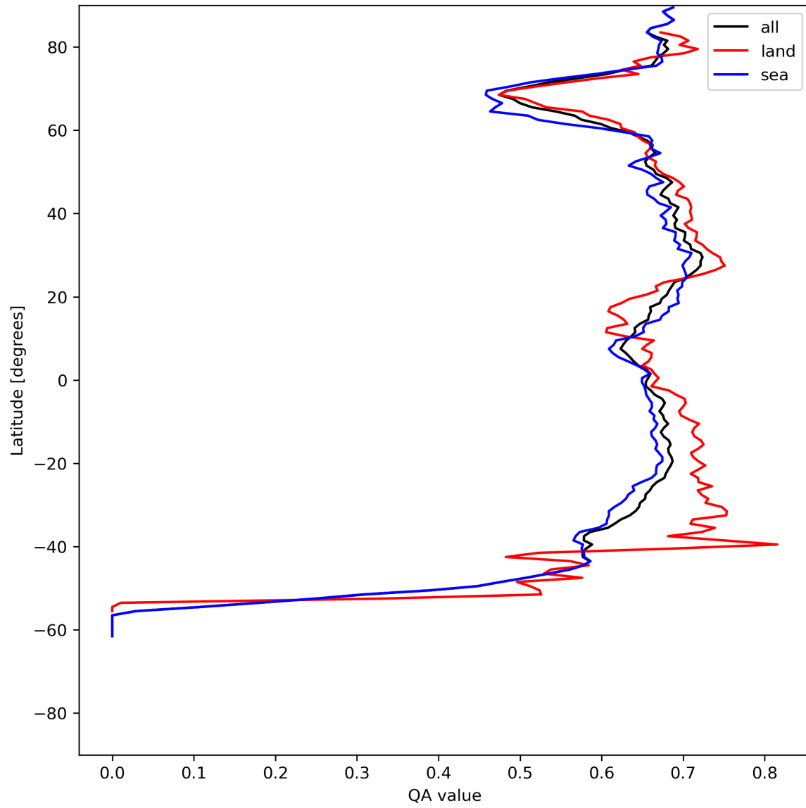
Figure 9: Zonal average of “QA value” for 2024-06-24 to 2024-06-26.
