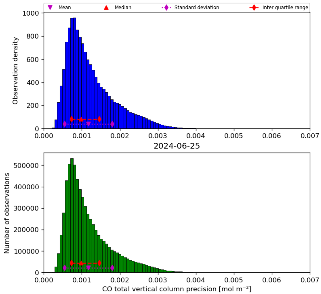
Figure 20: Histogram of “CO total vertical column precision” for 2024-06-24 to 2024-06-26
