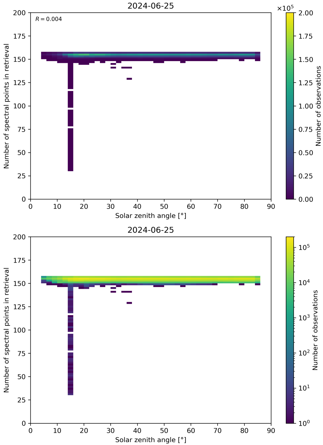
Figure 68: Scatter density plot of “Solar zenith angle” against “Number of spectral points in retrieval” for 2024-06-24 to 2024-06-26.
