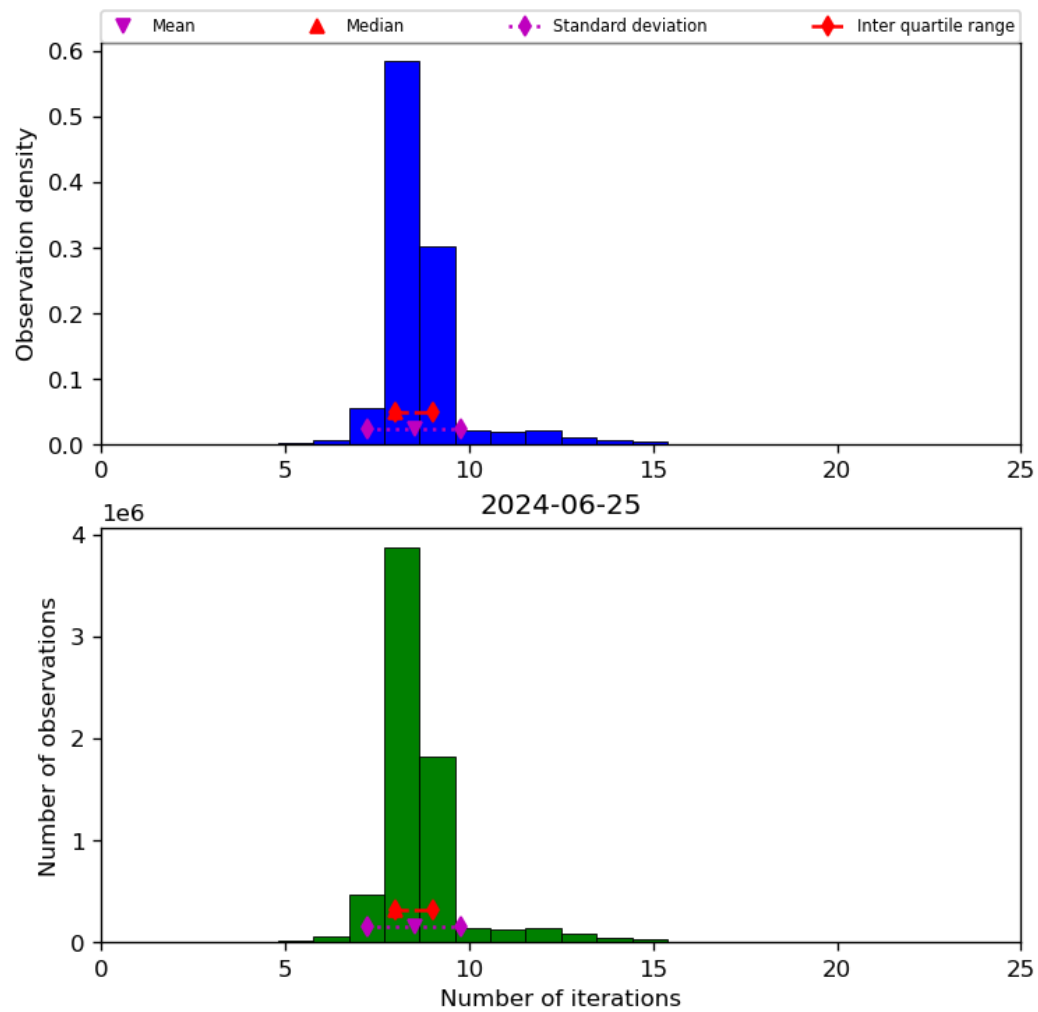
Figure 24: Histogram of “Number of iterations” for 2024-06-24 to 2024-06-26
