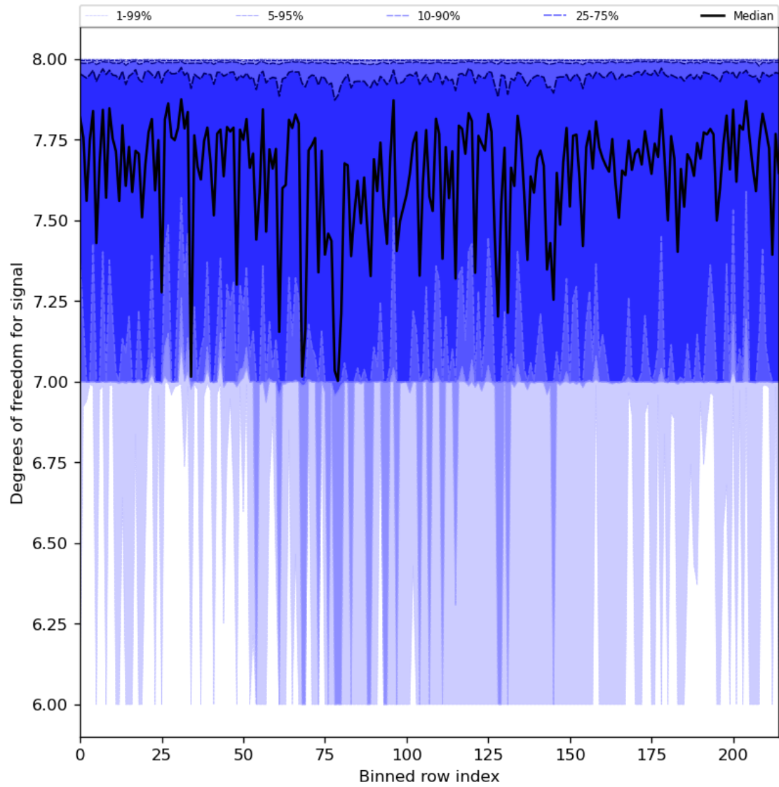
Figure 31: Along track statistics of “Degrees of freedom for signal” for 2024-06-24 to 2024-06-26
