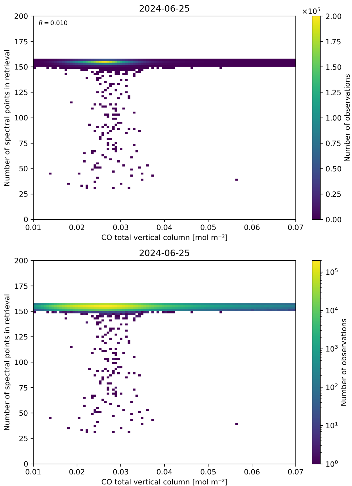
Figure 43: Scatter density plot of “CO total vertical column” against “Number of spectral points in retrieval” for 2024-06-24 to 2024-06-26.
