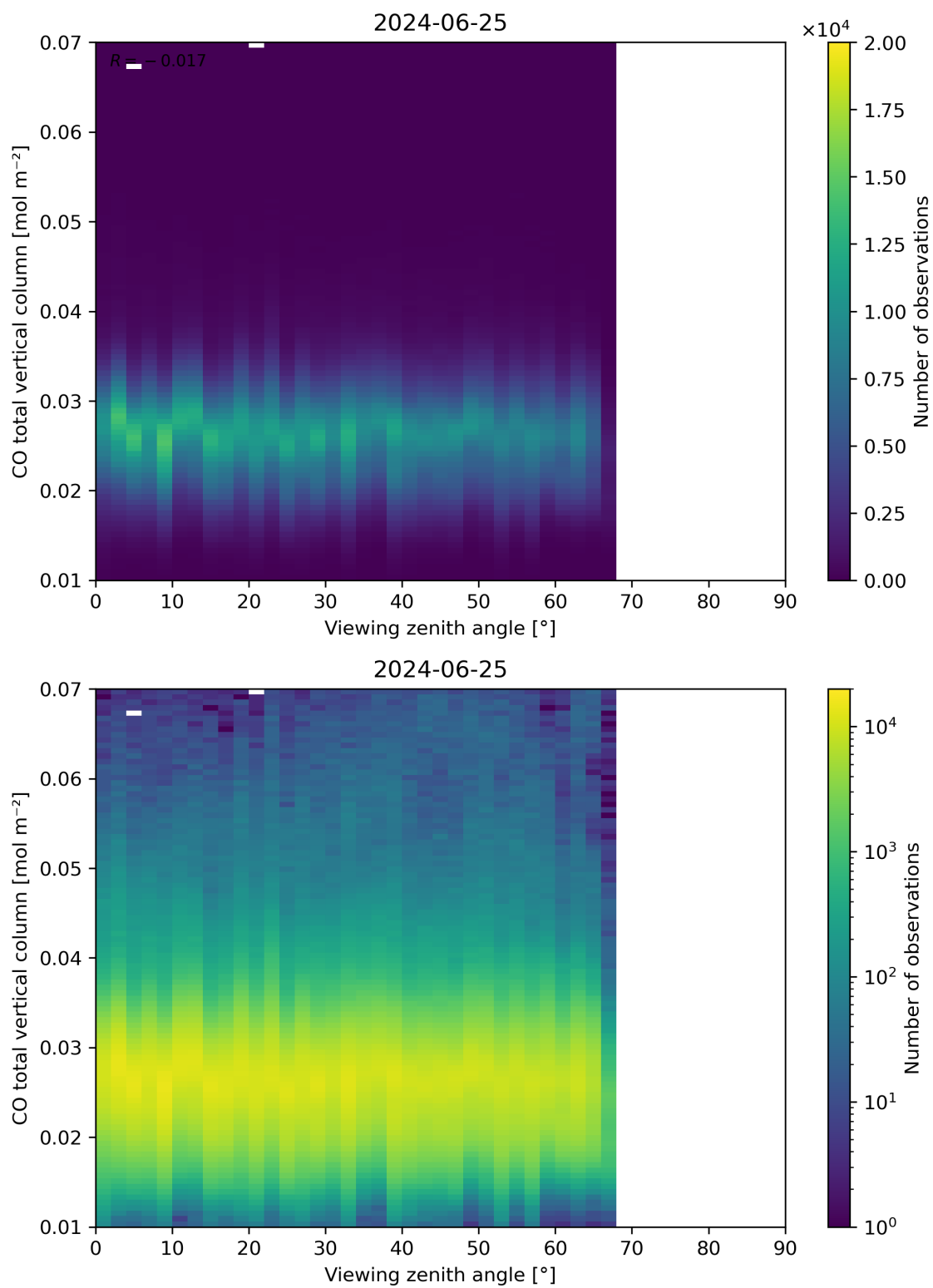
Figure 69: Scatter density plot of “Viewing zenith angle” against “CO total vertical column” for 2024-06-24 to 2024-06-26.
