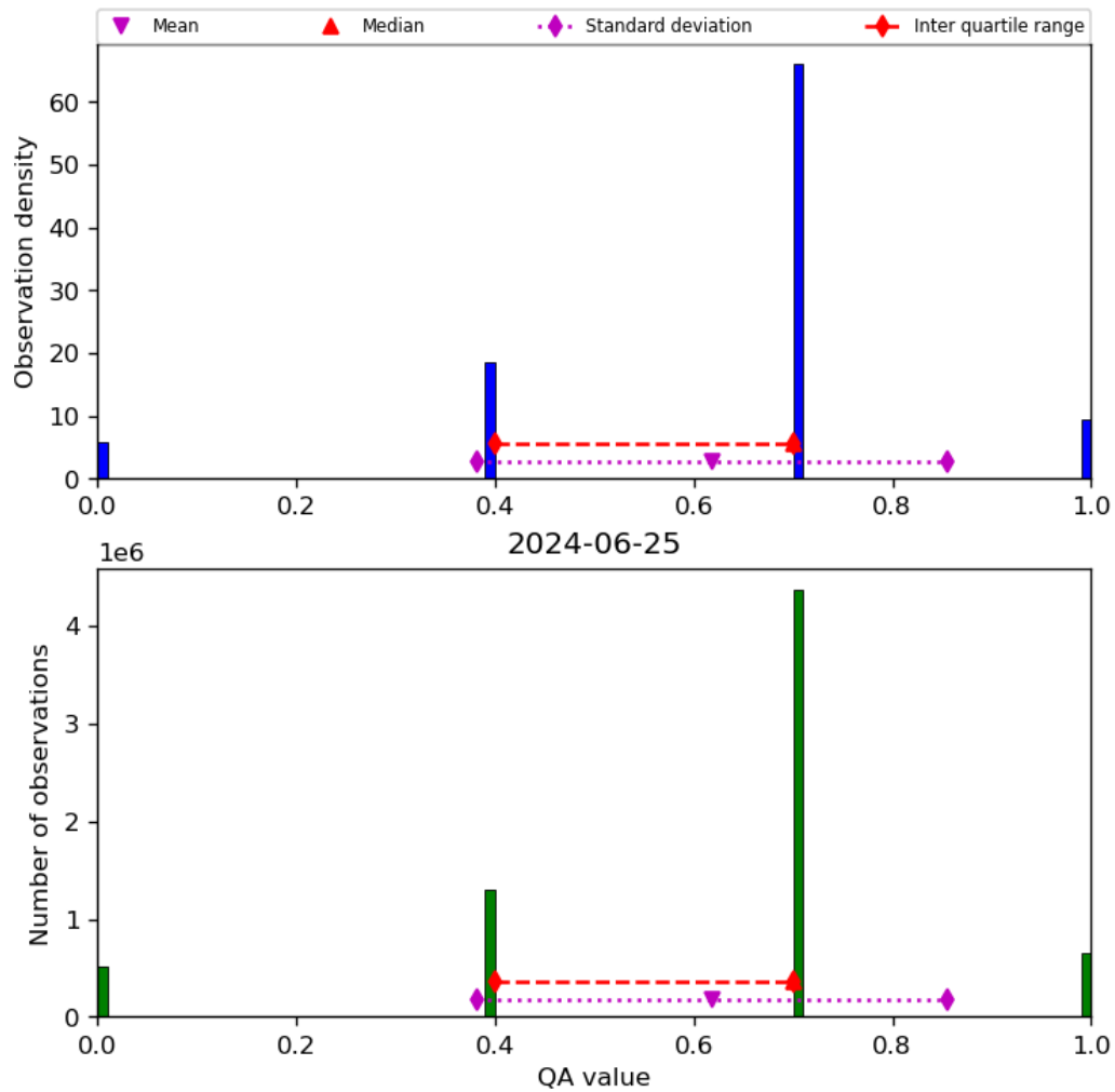
Figure 17: Histogram of “QA value” for 2024-06-24 to 2024-06-26
