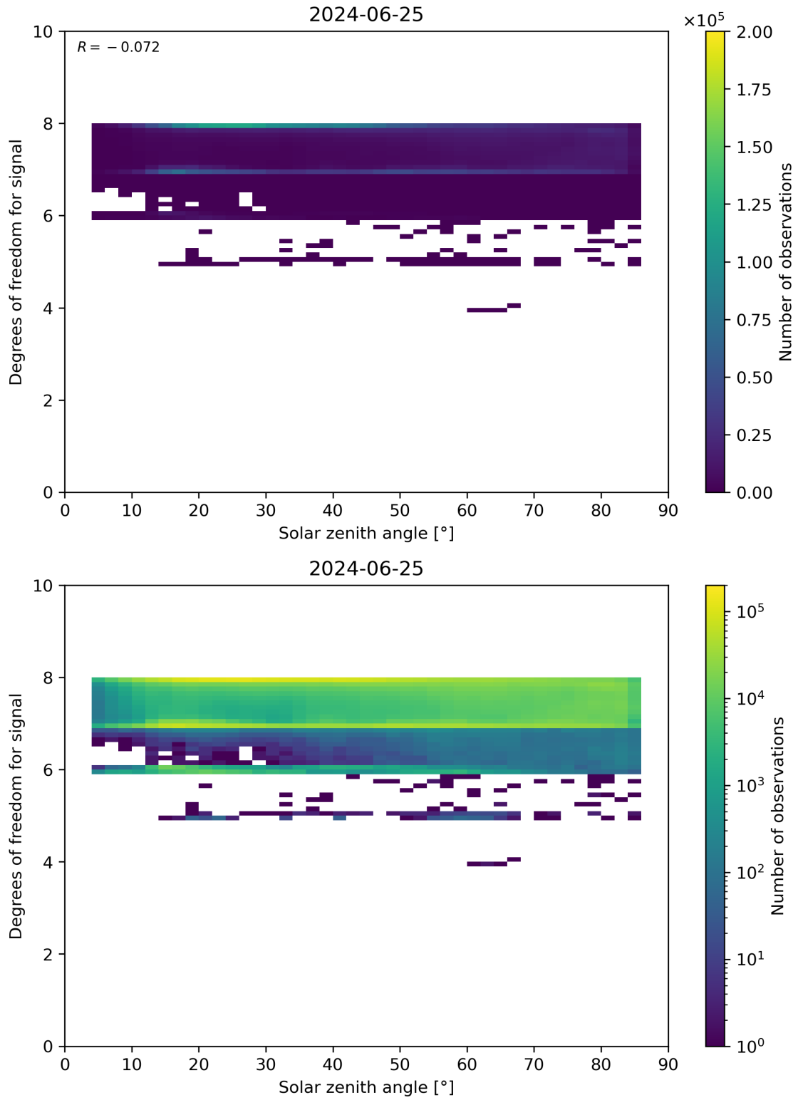
Figure 65: Scatter density plot of “Solar zenith angle” against “Degrees of freedom for signal” for 2024-06-24 to 2024-06-26.
