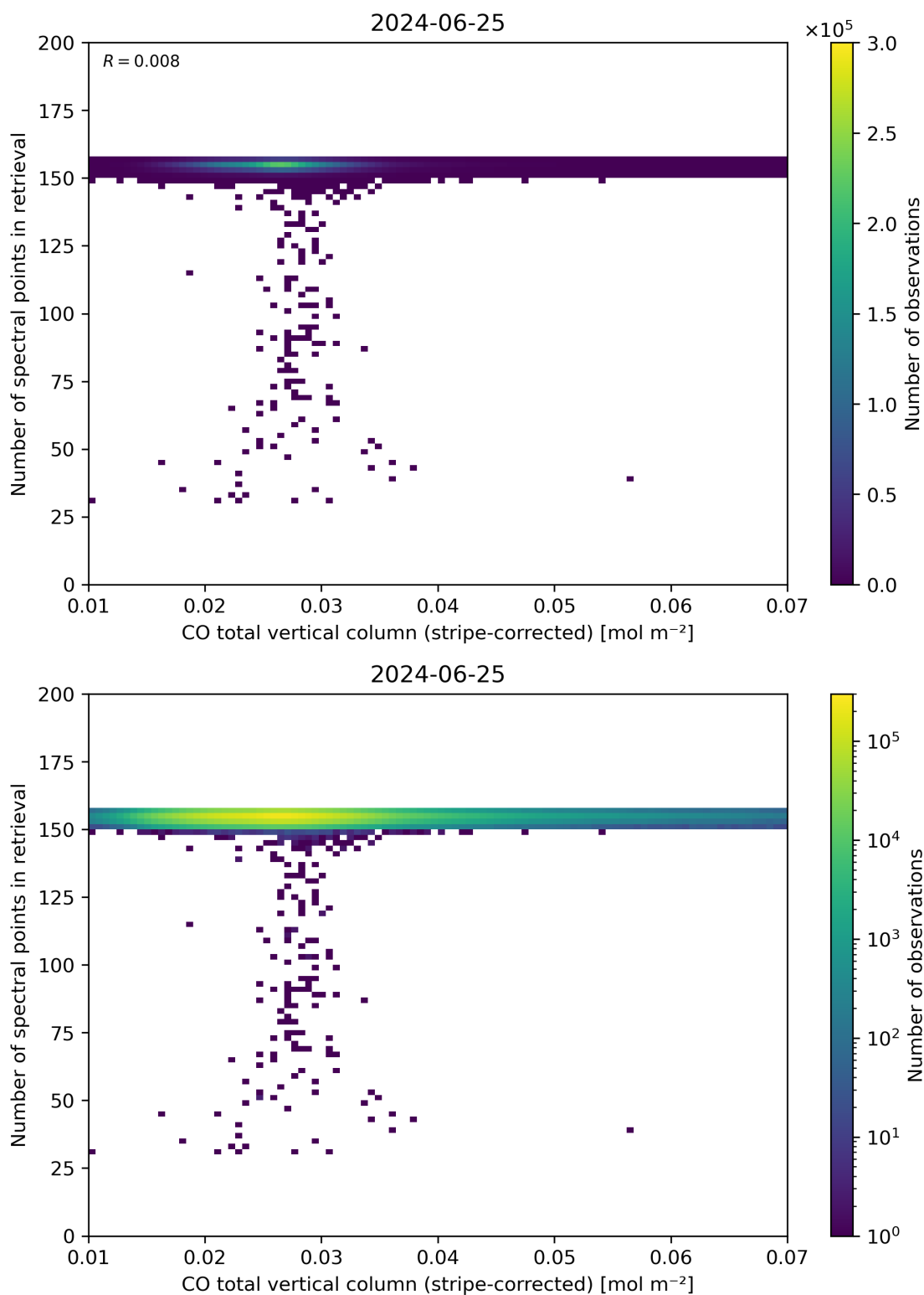
Figure 40: Scatter density plot of “CO total vertical column (stripe-corrected)” against “Number of spectral points in retrieval” for 2024-06-24 to 2024-06-26.
