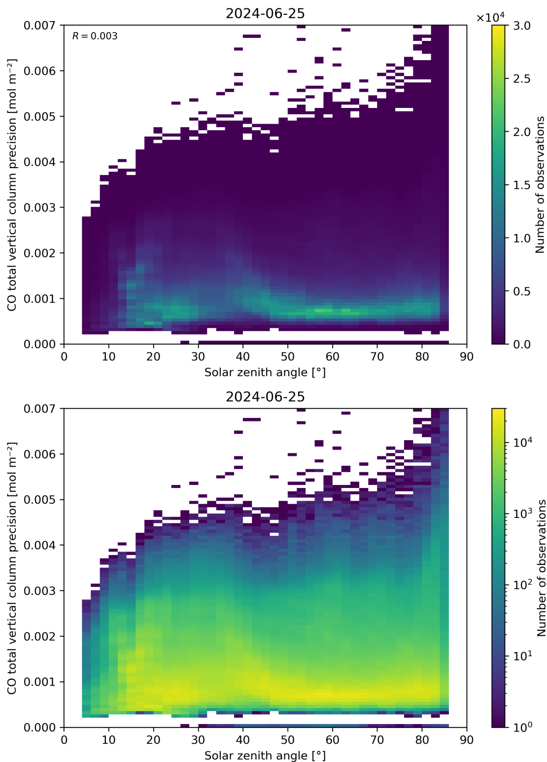
Figure 63: Scatter density plot of “Solar zenith angle” against “CO total vertical column precision” for 2024-06-24 to 2024-06-26.
