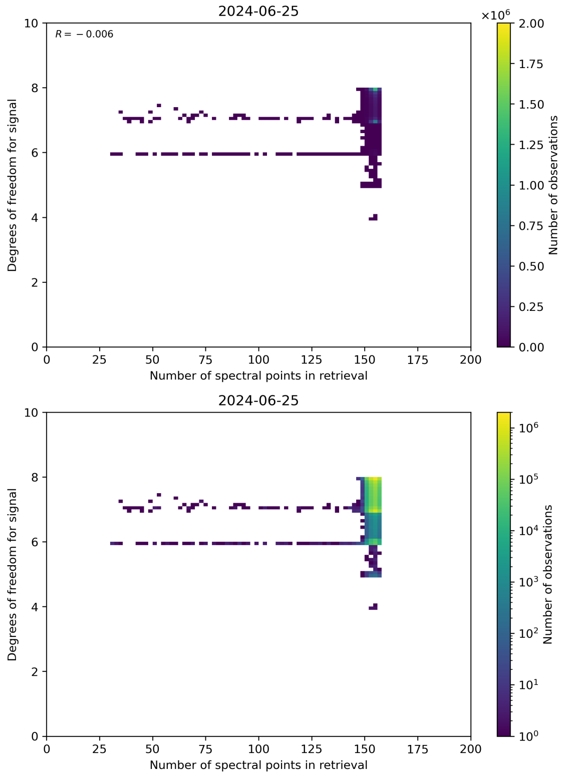
Figure 59: Scatter density plot of “Number of spectral points in retrieval” against “Degrees of freedom for signal” for 2024-06-24 to 2024-06-26.
