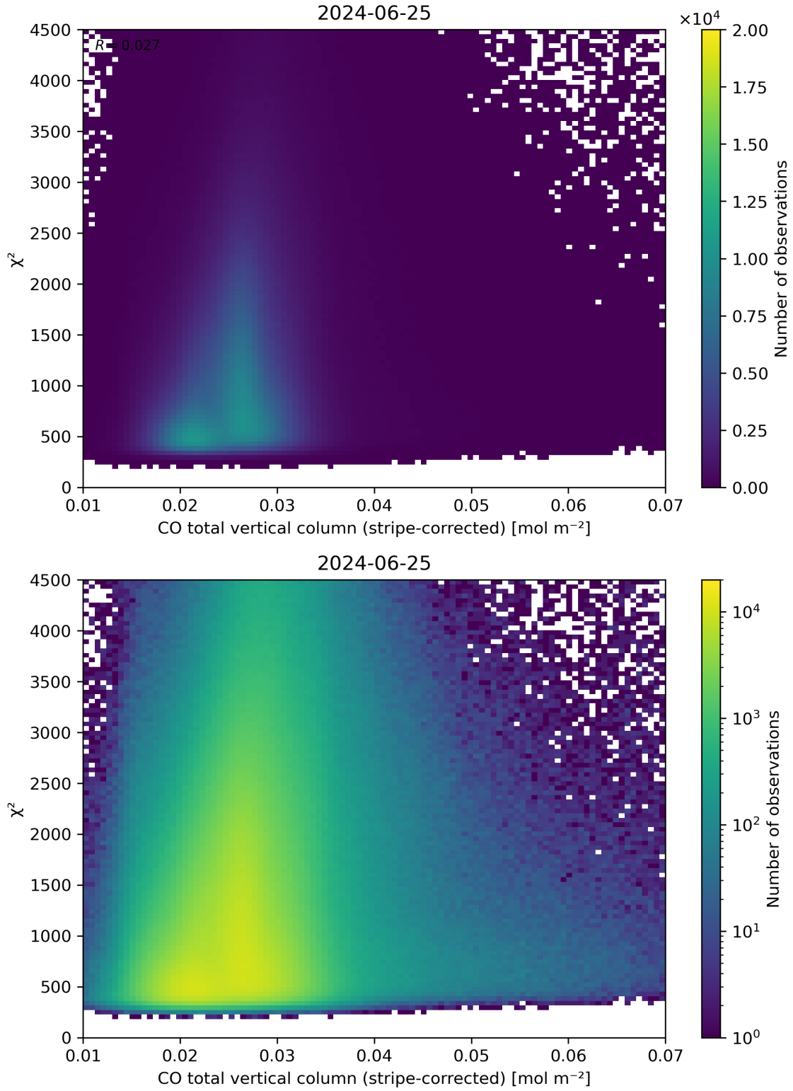
Figure 37: Scatter density plot of “CO total vertical column (stripe-corrected)” against “ \chi^2 ” for 2024-06-24 to 2024-06-26.
