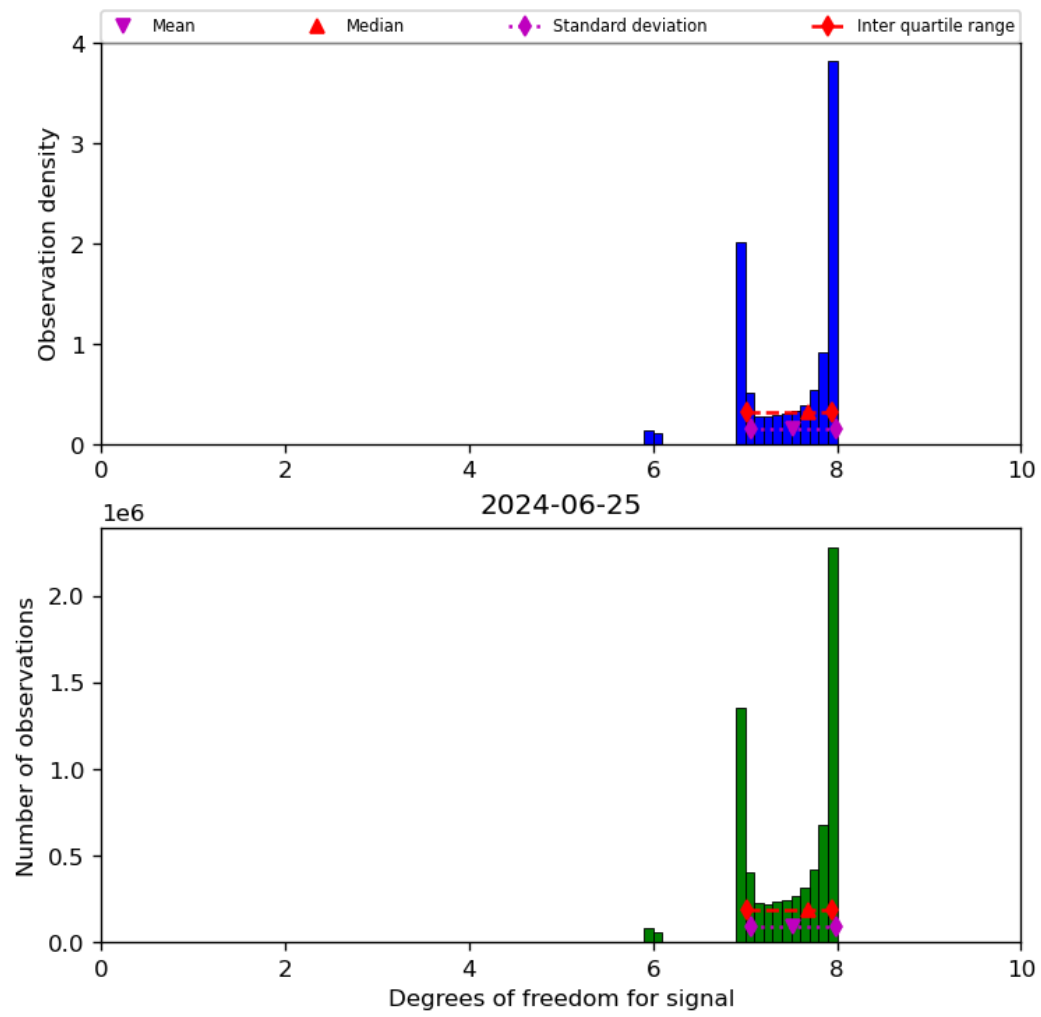
Figure 23: Histogram of “Degrees of freedom for signal” for 2024-06-24 to 2024-06-26
