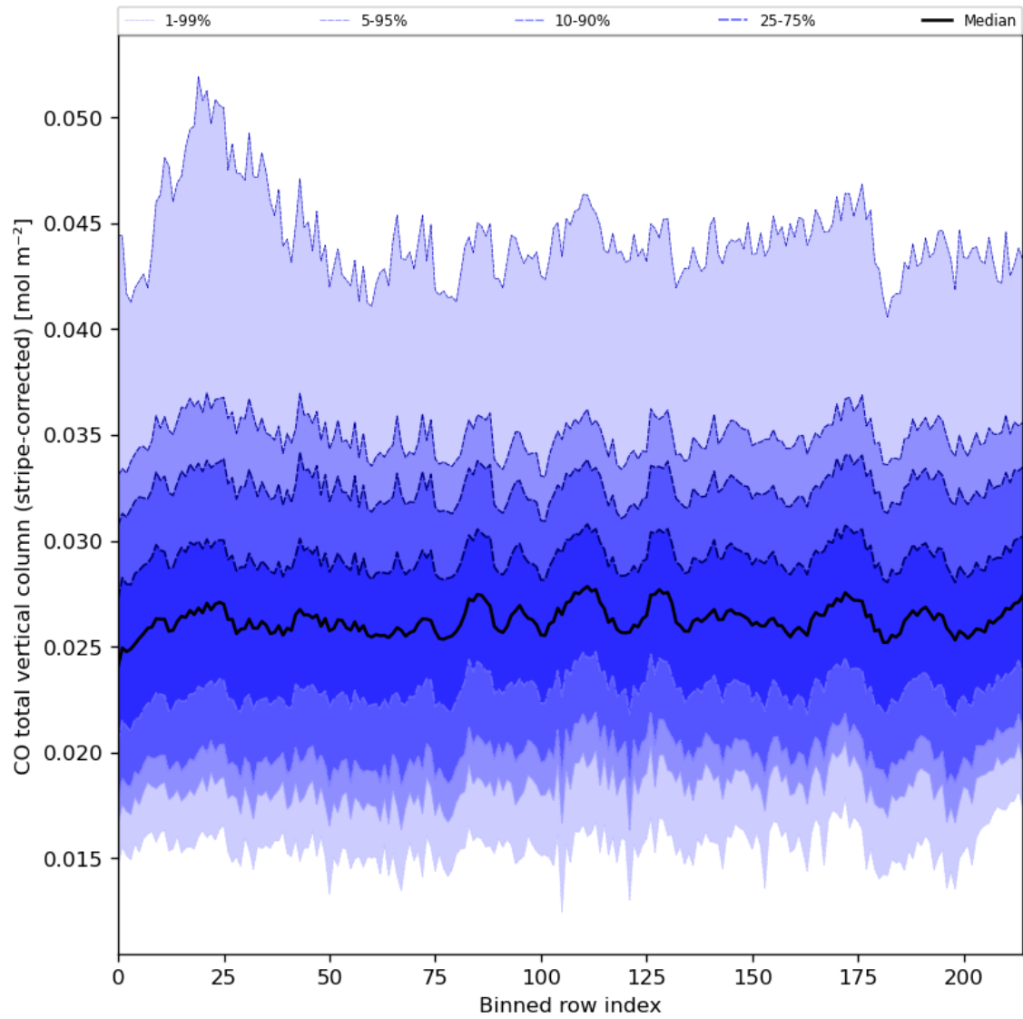
Figure 27: Along track statistics of “CO total vertical column (stripe-corrected)” for 2024-06-24 to 2024-06-26
