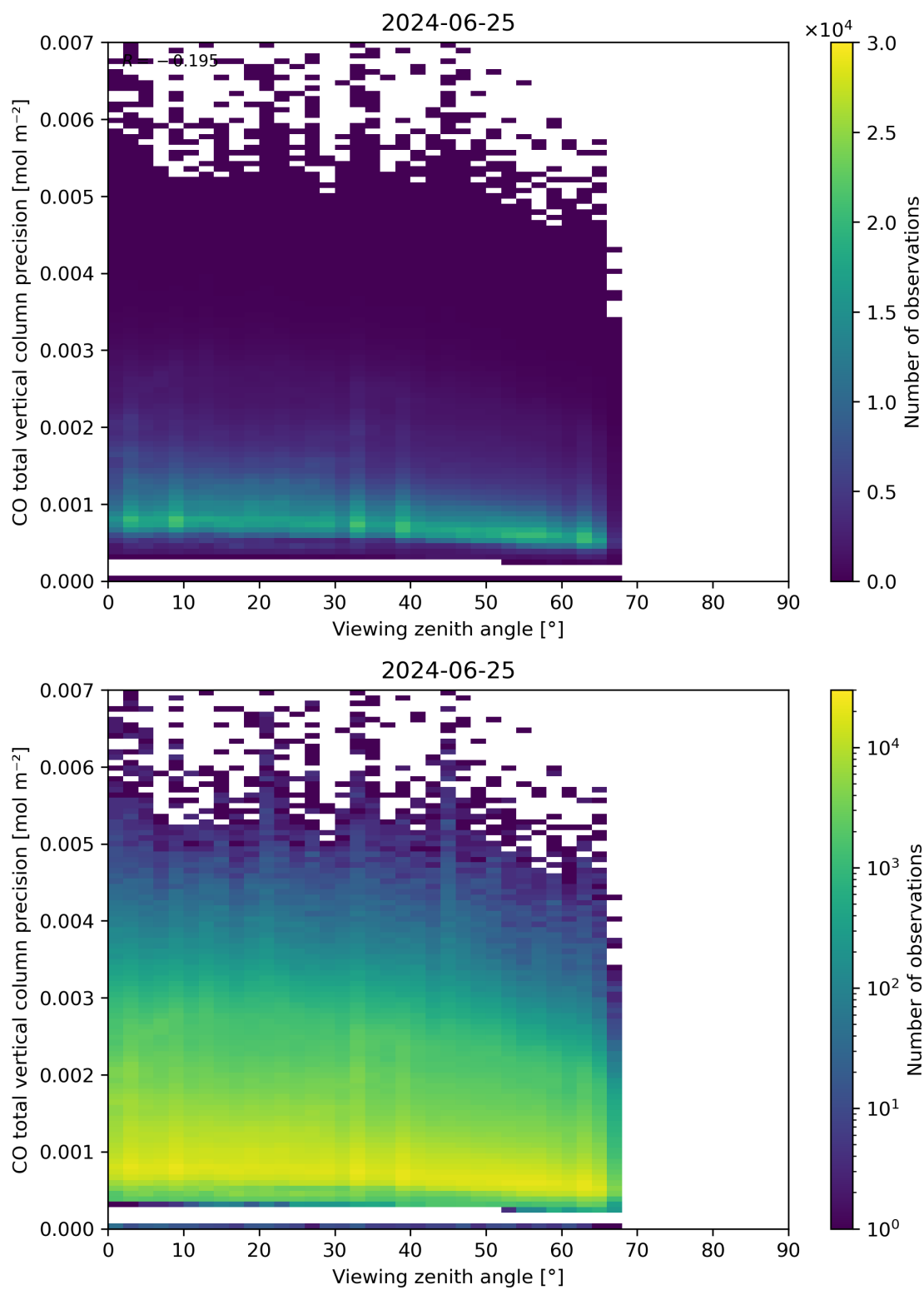
Figure 71: Scatter density plot of “Viewing zenith angle” against “CO total vertical column precision” for 2024-06-24 to 2024-06-26.
