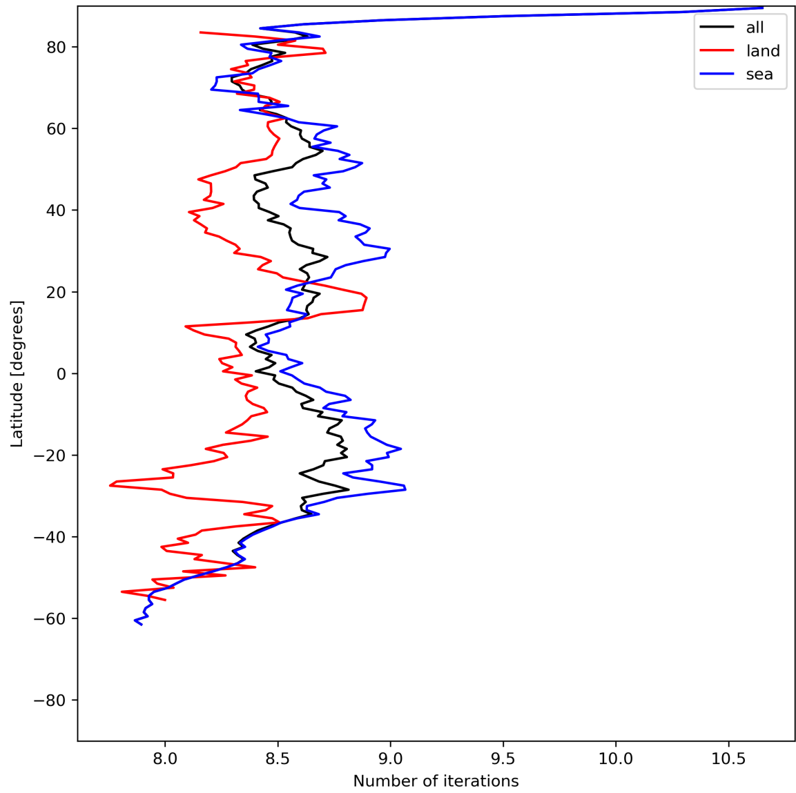
Figure 16: Zonal average of “Number of iterations” for 2024-06-24 to 2024-06-26.
