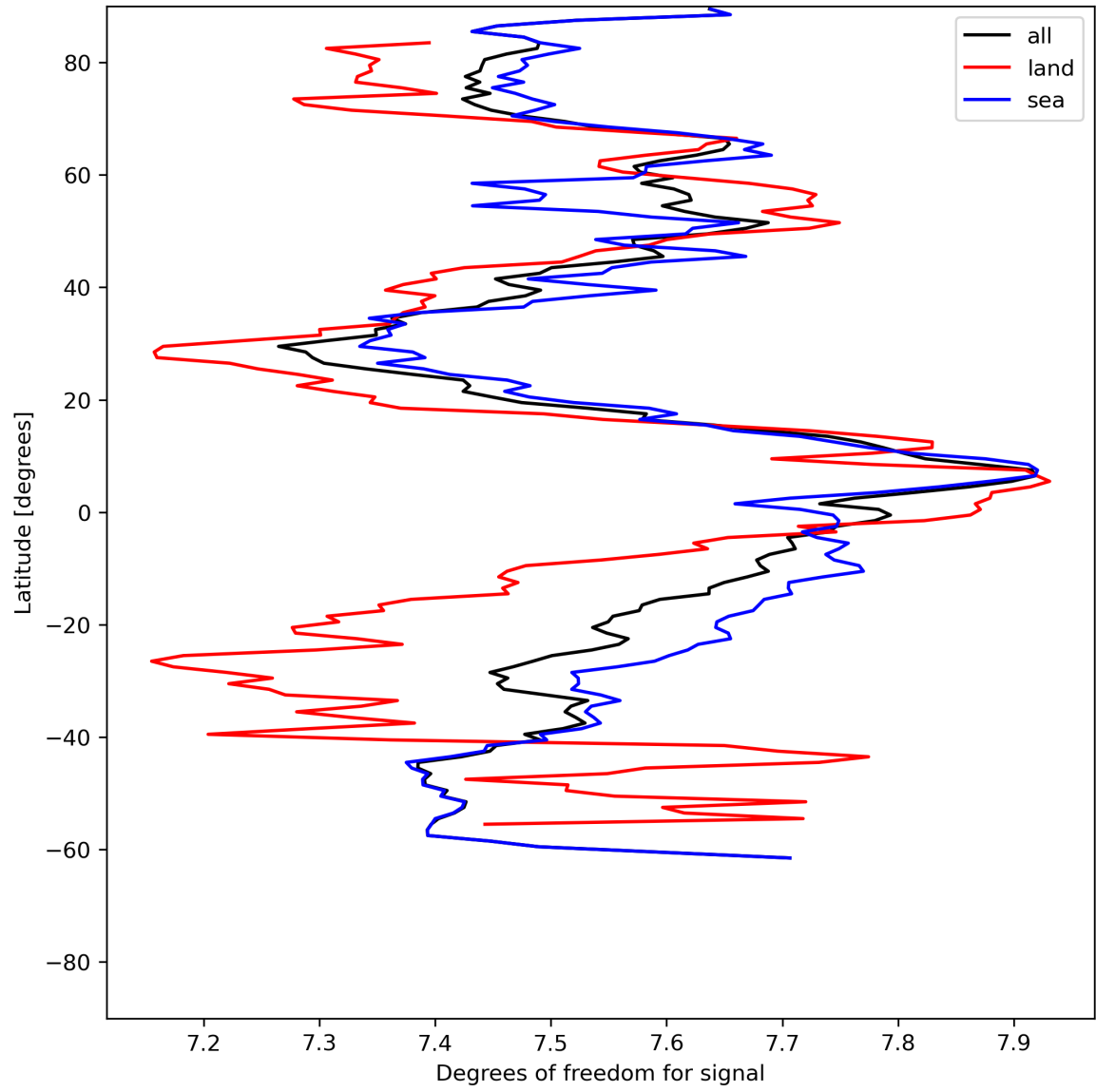
Figure 15: Zonal average of “Degrees of freedom for signal” for 2024-06-24 to 2024-06-26.
