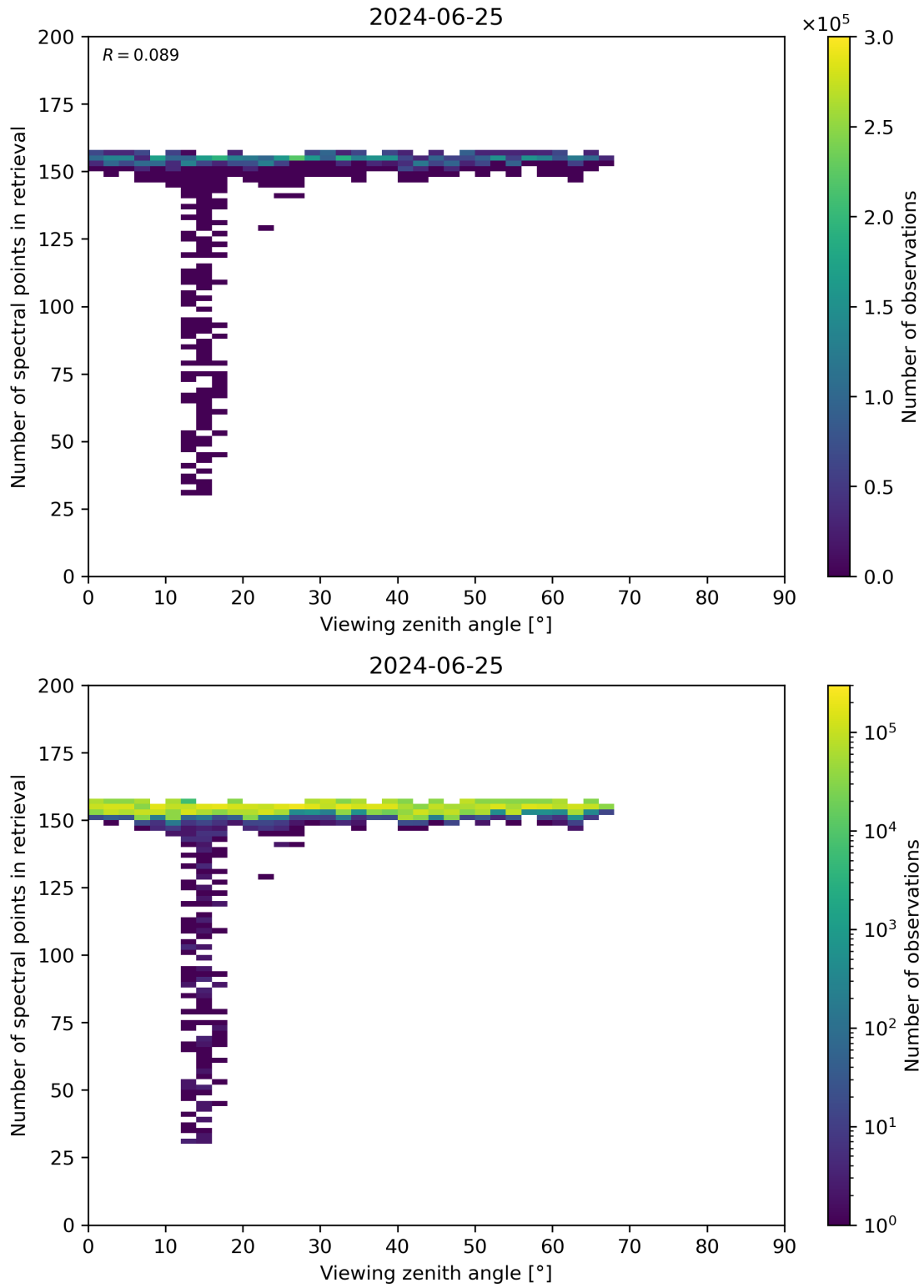
Figure 76: Scatter density plot of “Viewing zenith angle” against “Number of spectral points in retrieval” for 2024-06-24 to 2024-06-26.
