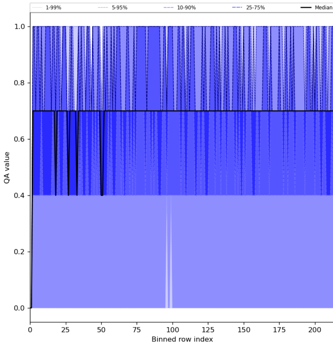
Figure 25: Along track statistics of “QA value” for 2024-06-24 to 2024-06-26
