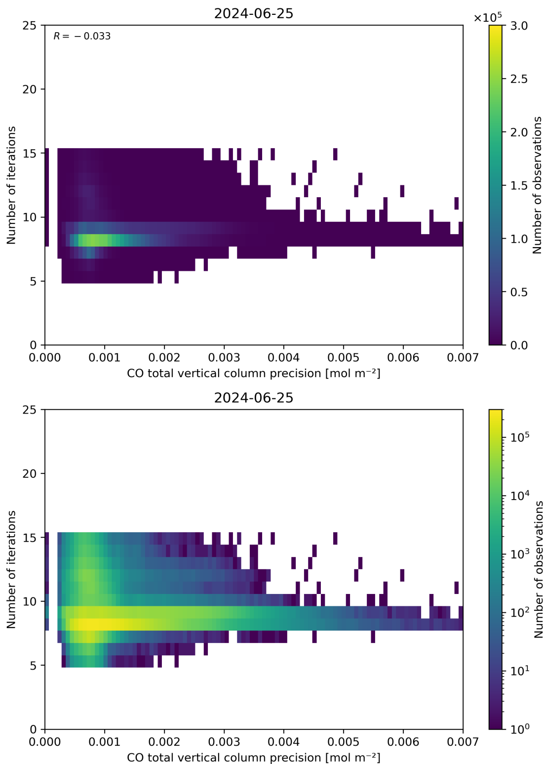
Figure 46: Scatter density plot of “CO total vertical column precision” against “Number of iterations” for 2024-06-24 to 2024-06-26.
