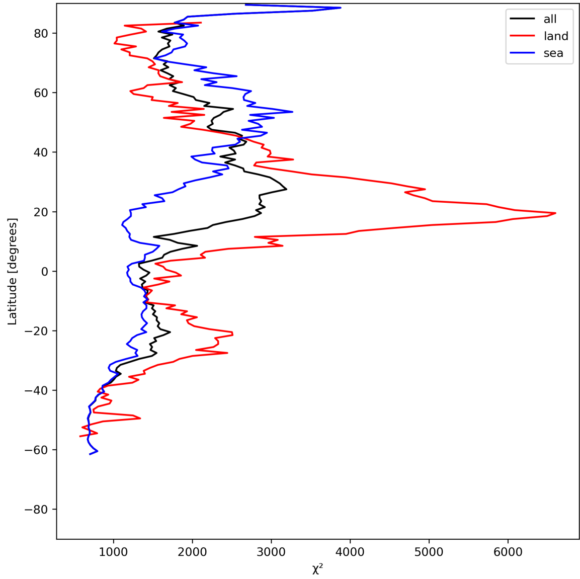
Figure 14: Zonal average of “ \chi^2 ” for 2024-06-24 to 2024-06-26.
