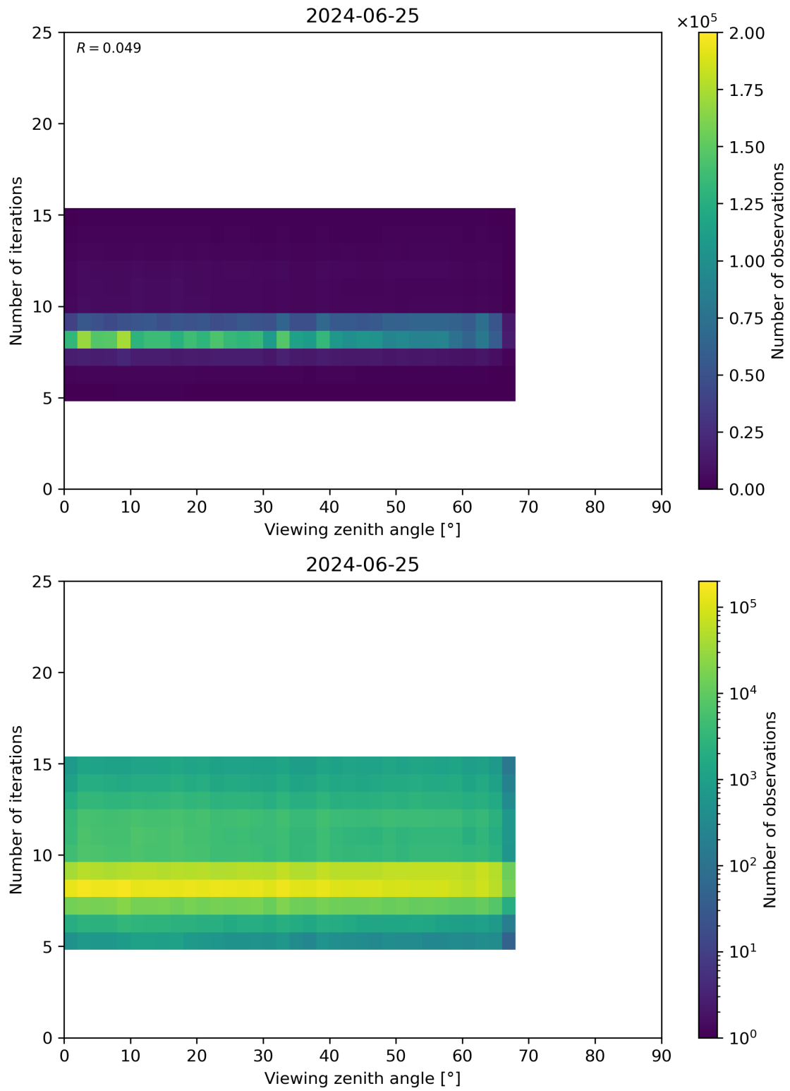
Figure 75: Scatter density plot of “Viewing zenith angle” against “Number of iterations” for 2024-06-24 to 2024-06-26.
