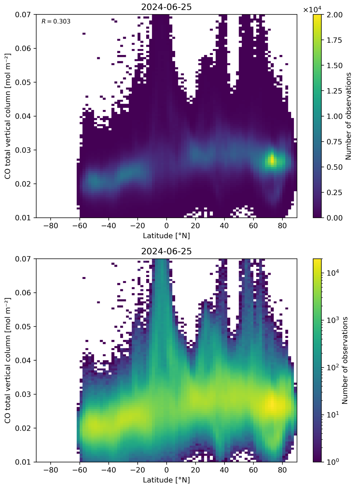
Figure 51: Scatter density plot of “Latitude” against “CO total vertical column” for 2024-06-24 to 2024-06-26.
