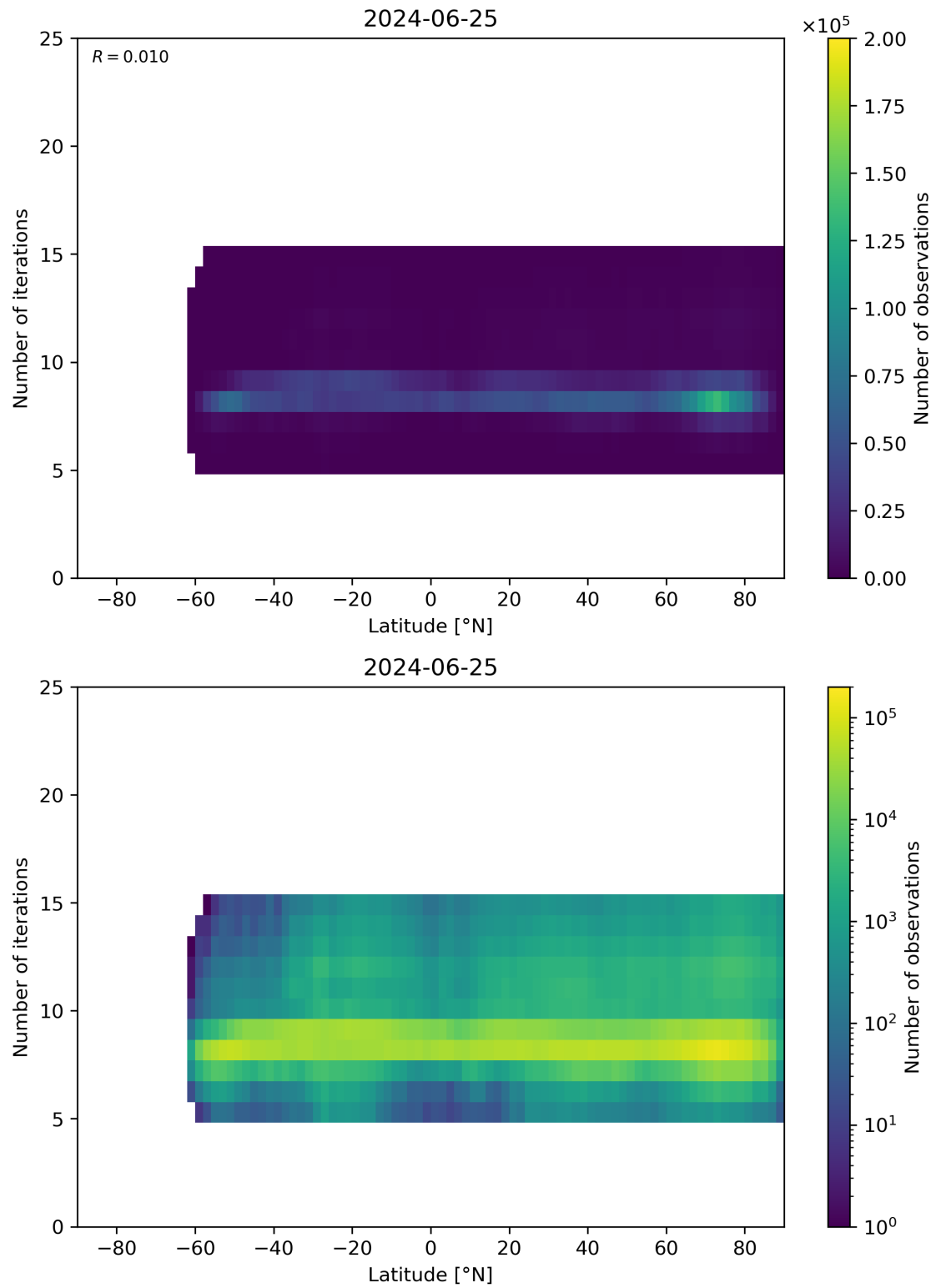
Figure 56: Scatter density plot of “Latitude” against “Number of iterations” for 2024-06-24 to 2024-06-26.
