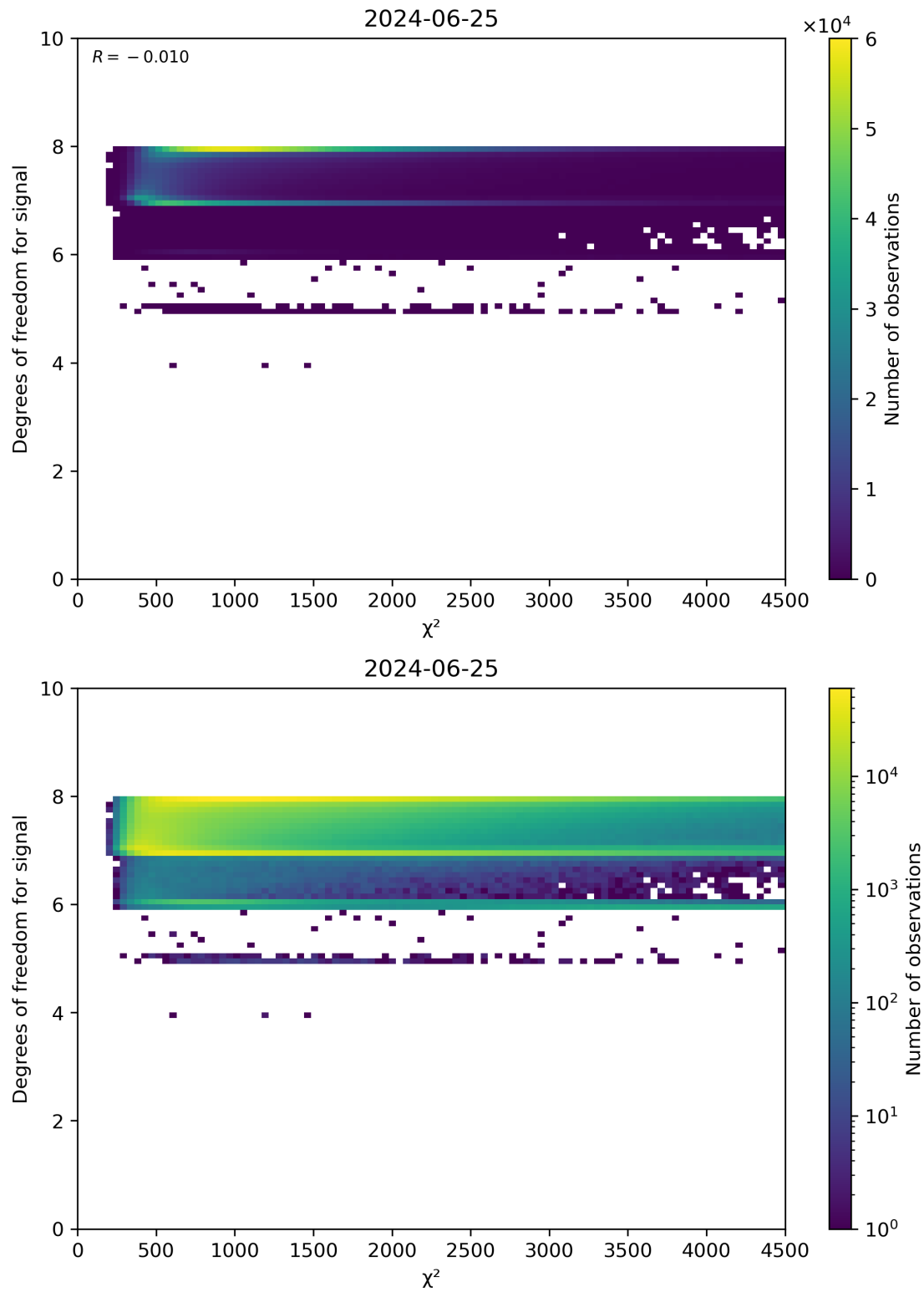
Figure 48: Scatter density plot of “ \chi^2 ” against “Degrees of freedom for signal” for 2024-06-24 to 2024-06-26.
