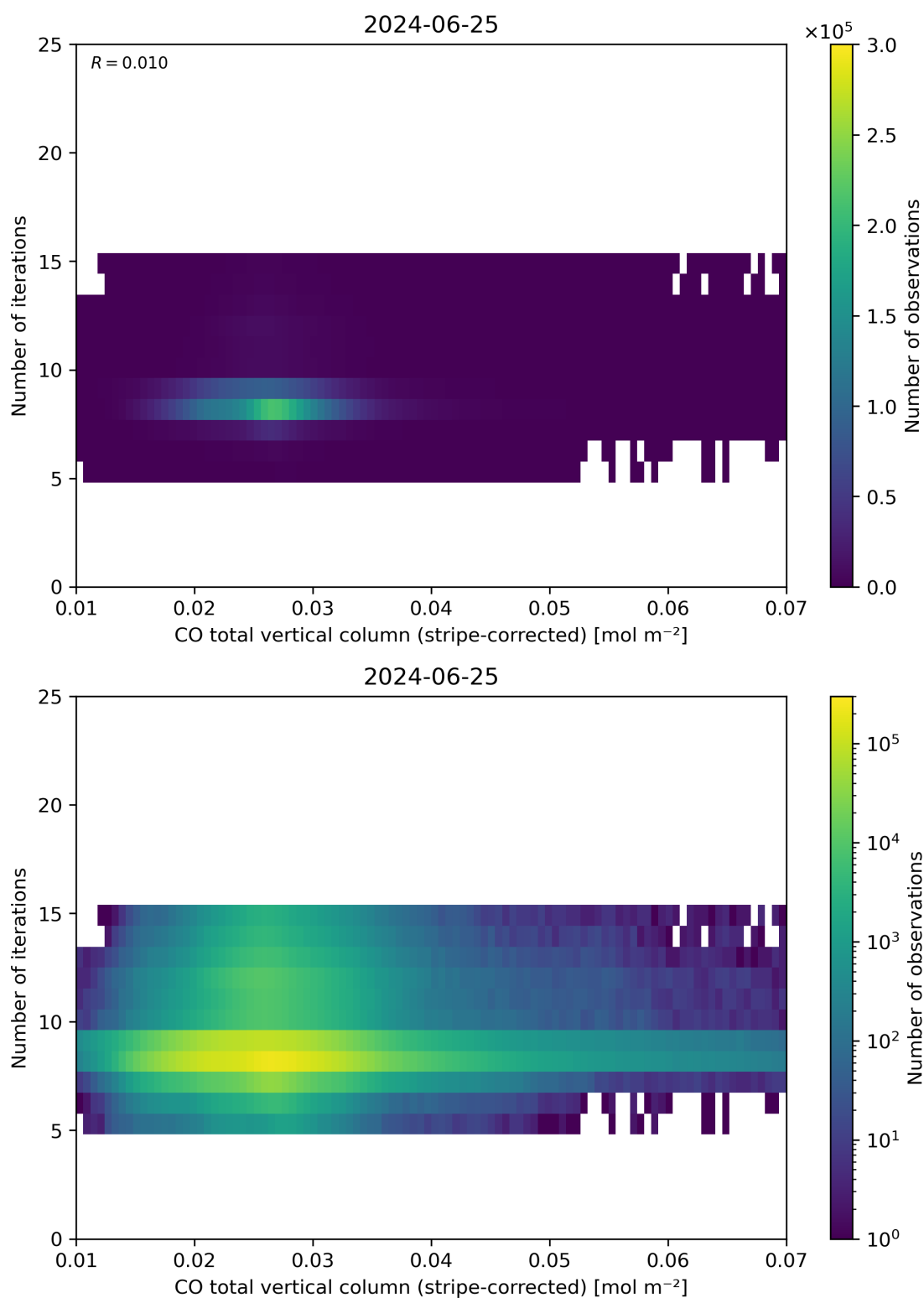
Figure 39: Scatter density plot of “CO total vertical column (stripe-corrected)” against “Number of iterations” for 2024-06-24 to 2024-06-26.
