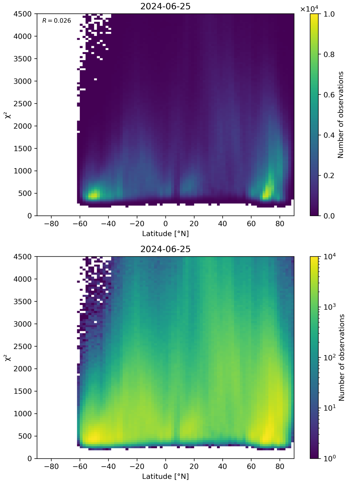
Figure 54: Scatter density plot of “Latitude” against “ \chi^2 ” for 2024-06-24 to 2024-06-26.
