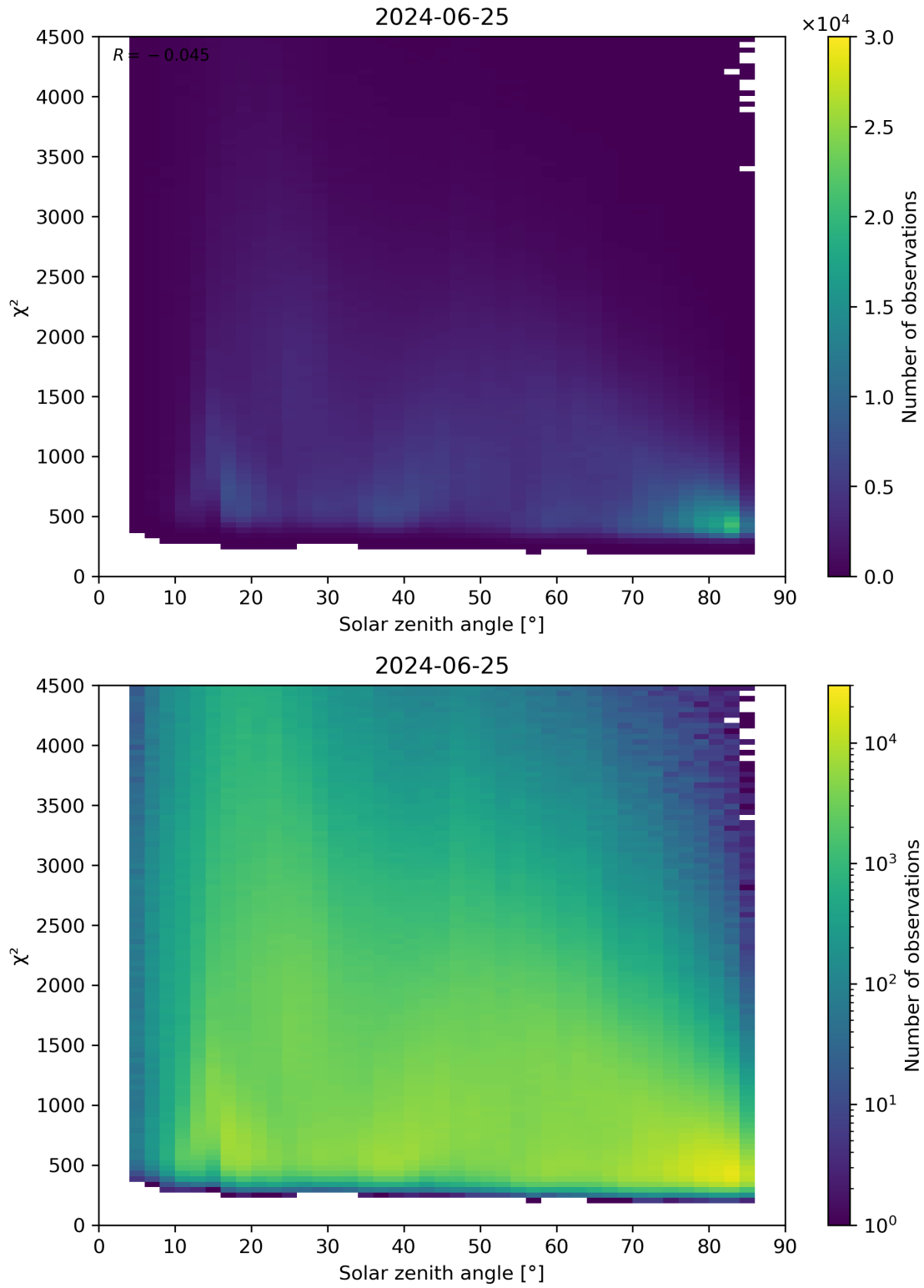
Figure 64: Scatter density plot of “Solar zenith angle” against “ \chi^2 ” for 2024-06-24 to 2024-06-26.
