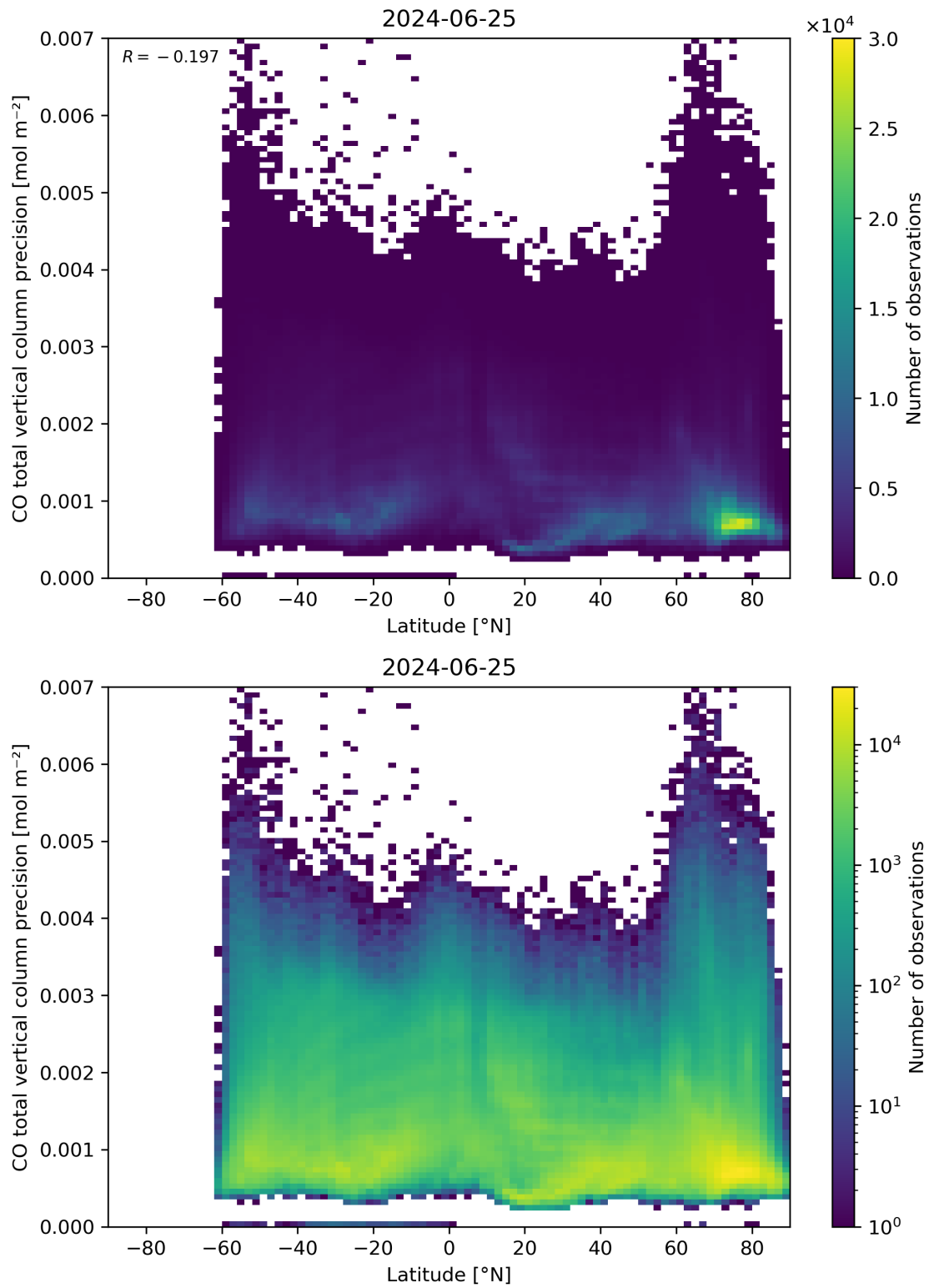
Figure 53: Scatter density plot of “Latitude” against “CO total vertical column precision” for 2024-06-24 to 2024-06-26.
