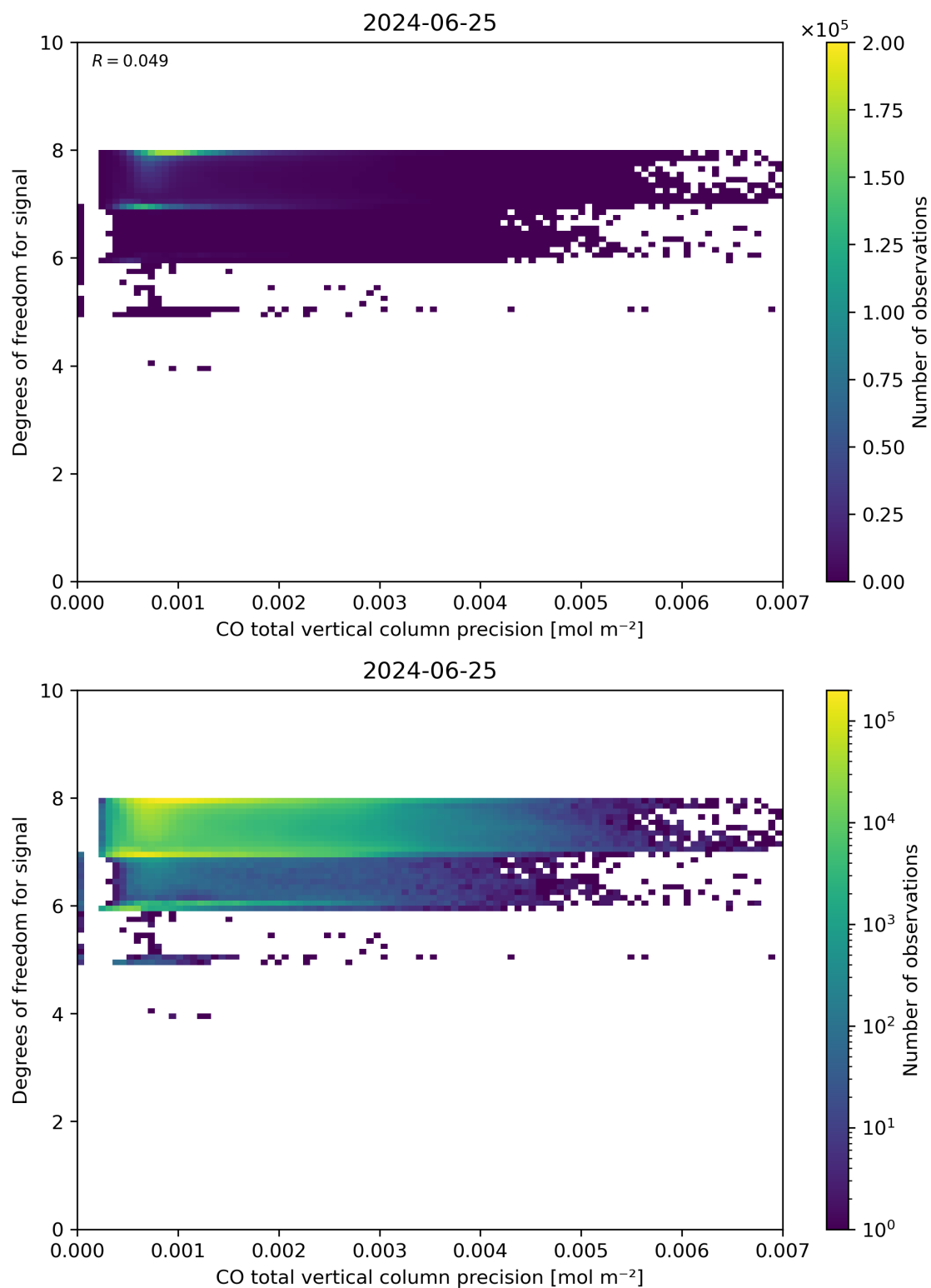
Figure 45: Scatter density plot of “CO total vertical column precision” against “Degrees of freedom for signal” for 2024-06-24 to 2024-06-26.
