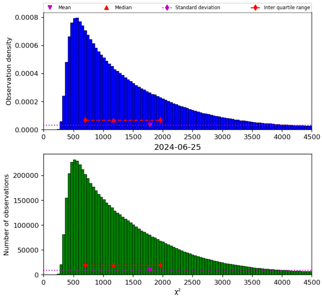
Figure 22: Histogram of “ \chi^2 ” for 2024-06-24 to 2024-06-26
