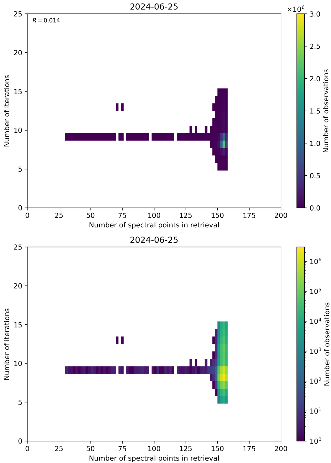
Figure 60: Scatter density plot of “Number of spectral points in retrieval” against “Number of iterations” for 2024-06-24 to 2024-06-26.
