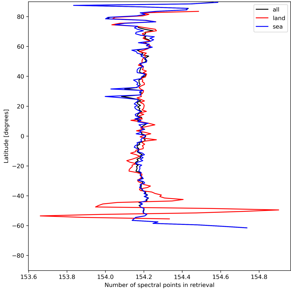
Figure 13: Zonal average of “Number of spectral points in retrieval” for 2024-06-24 to 2024-06-26.
