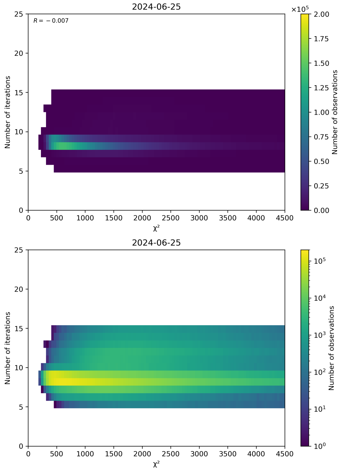
Figure 49: Scatter density plot of “ \chi^2 ” against “Number of iterations” for 2024-06-24 to 2024-06-26.
