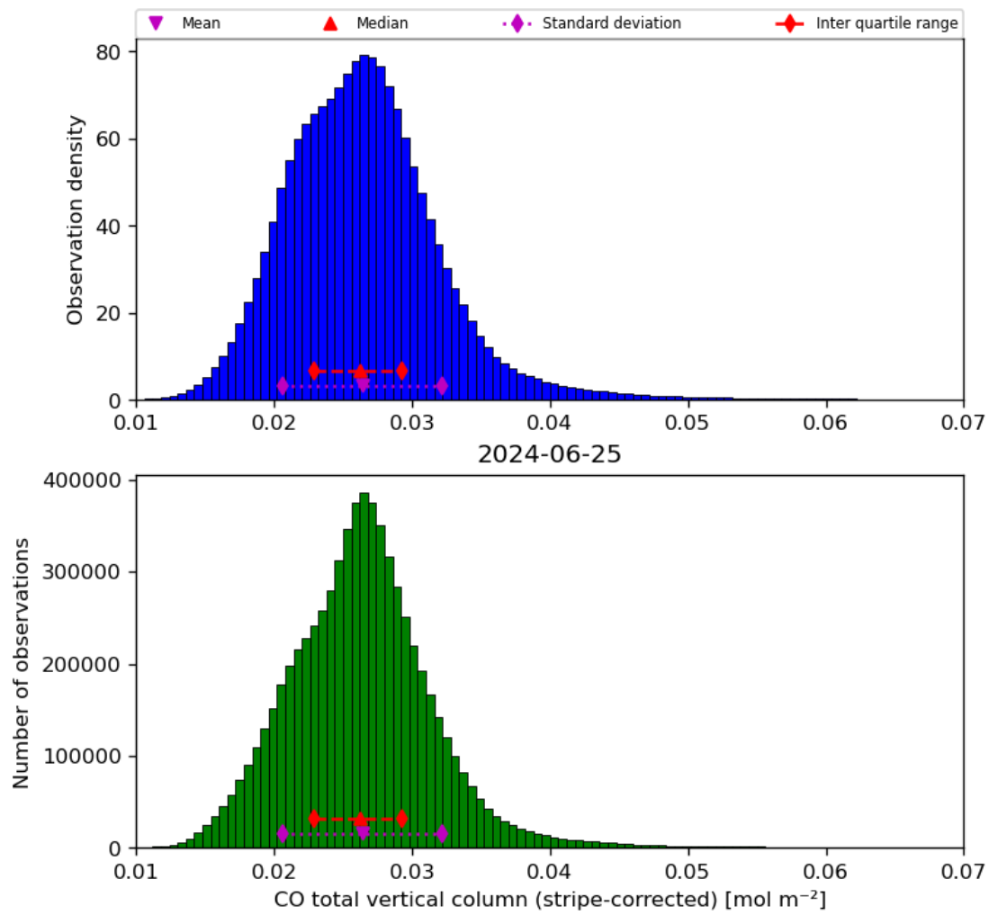
Figure 19: Histogram of “CO total vertical column (stripe-corrected)” for 2024-06-24 to 2024-06-26
