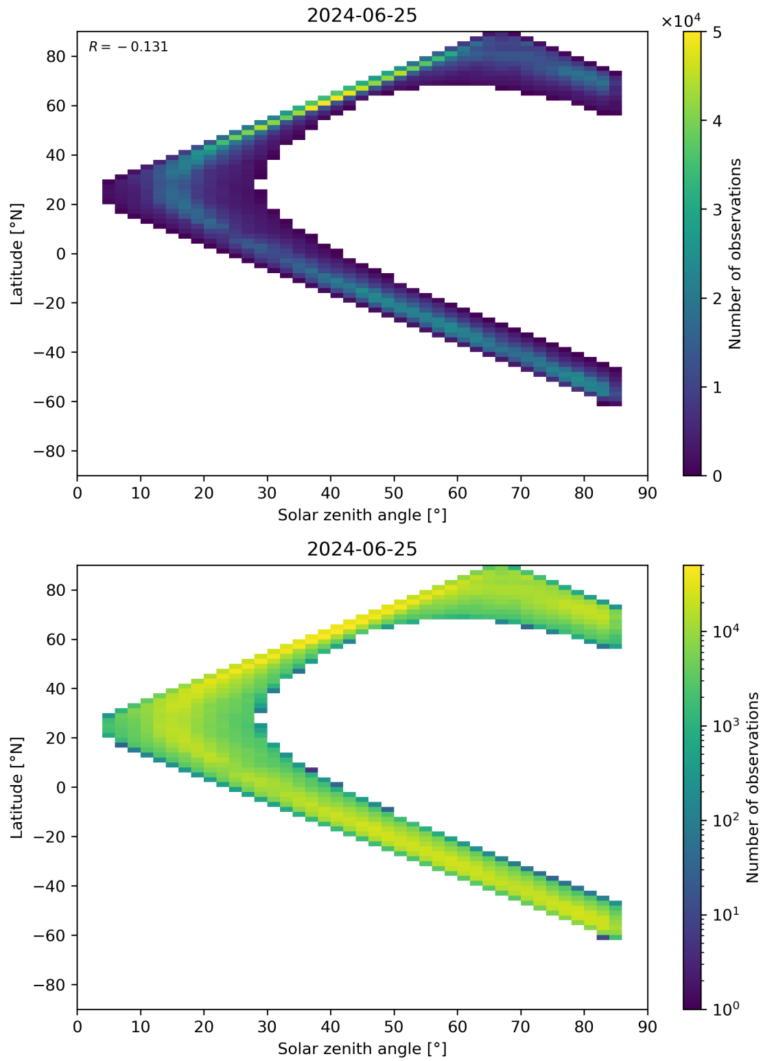
Figure 66: Scatter density plot of “Solar zenith angle” against “Latitude” for 2024-06-24 to 2024-06-26.
