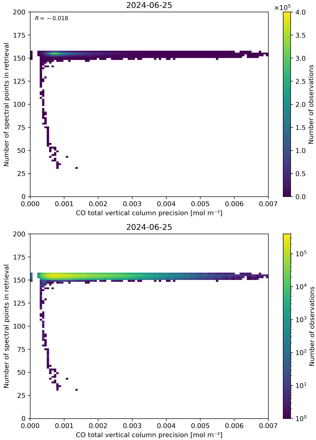
Figure 47: Scatter density plot of “CO total vertical column precision” against “Number of spectral points in retrieval” for 2024-06-24 to 2024-06-26.
