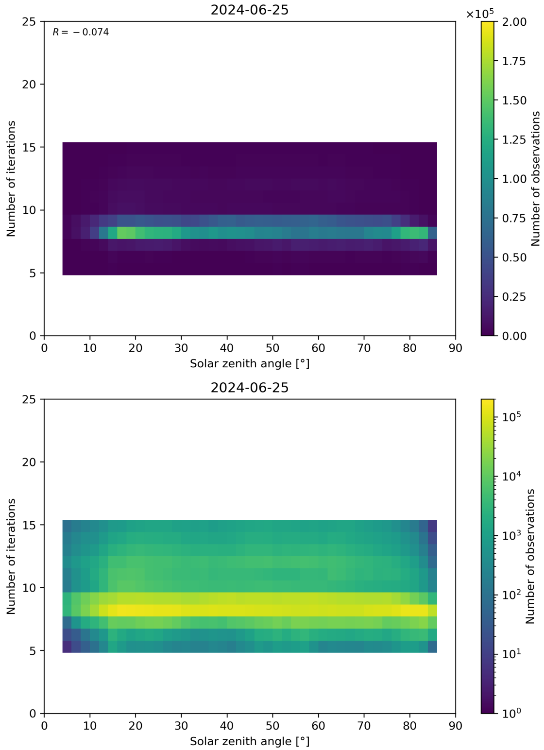
Figure 67: Scatter density plot of “Solar zenith angle” against “Number of iterations” for 2024-06-24 to 2024-06-26.
