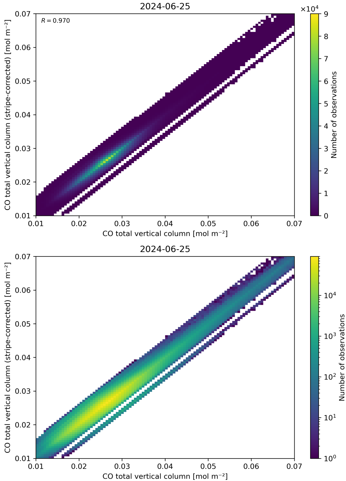
Figure 33: Scatter density plot of “CO total vertical column” against “CO total vertical column (stripe-corrected)” for 2024-06-24 to 2024-06-26.
