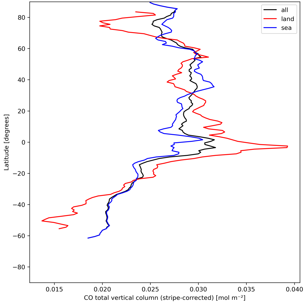
Figure 11: Zonal average of “CO total vertical column (stripe-corrected)” for 2024-06-24 to 2024-06-26.
