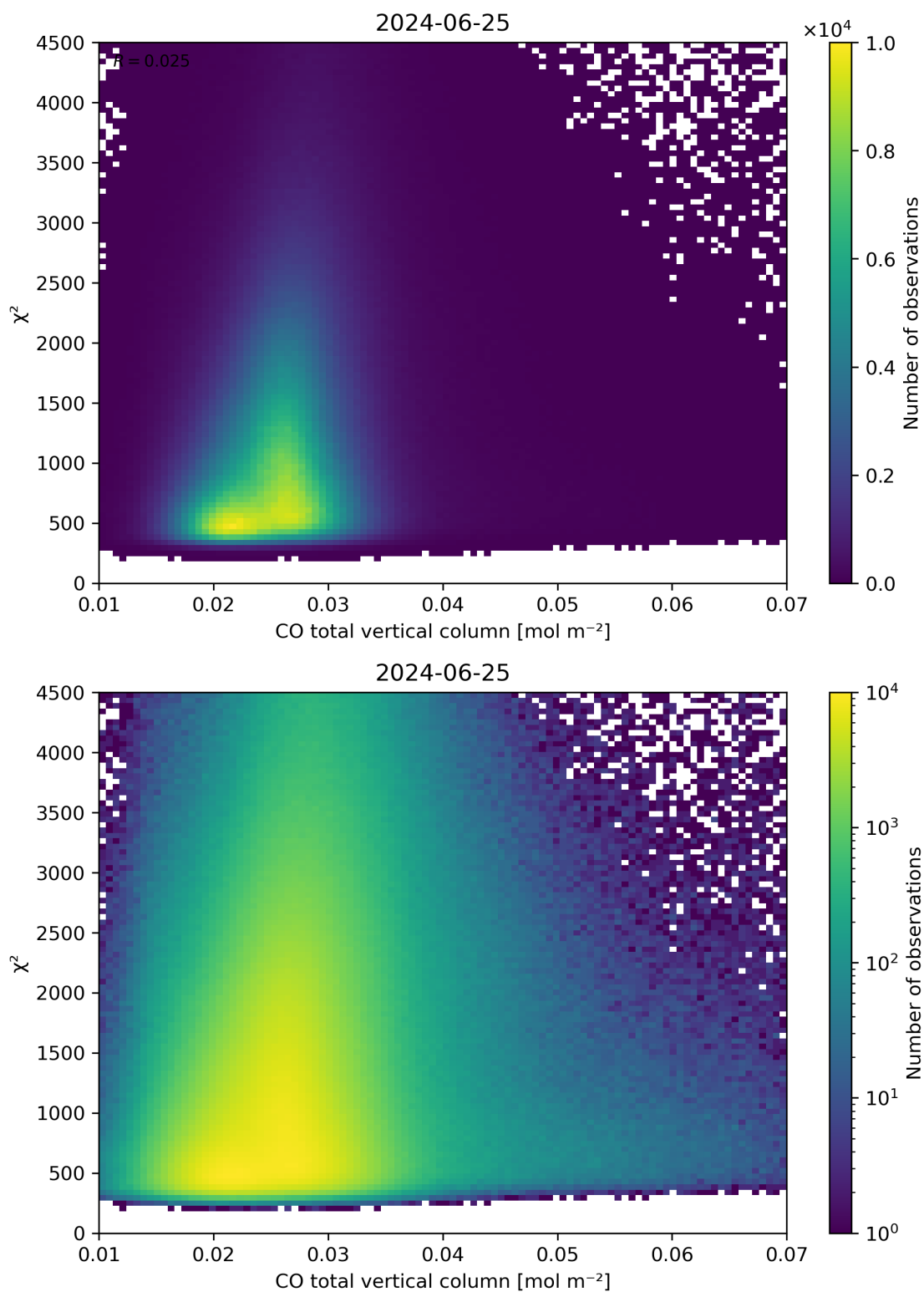
Figure 35: Scatter density plot of “CO total vertical column” against “ \chi^2 ” for 2024-06-24 to 2024-06-26.
