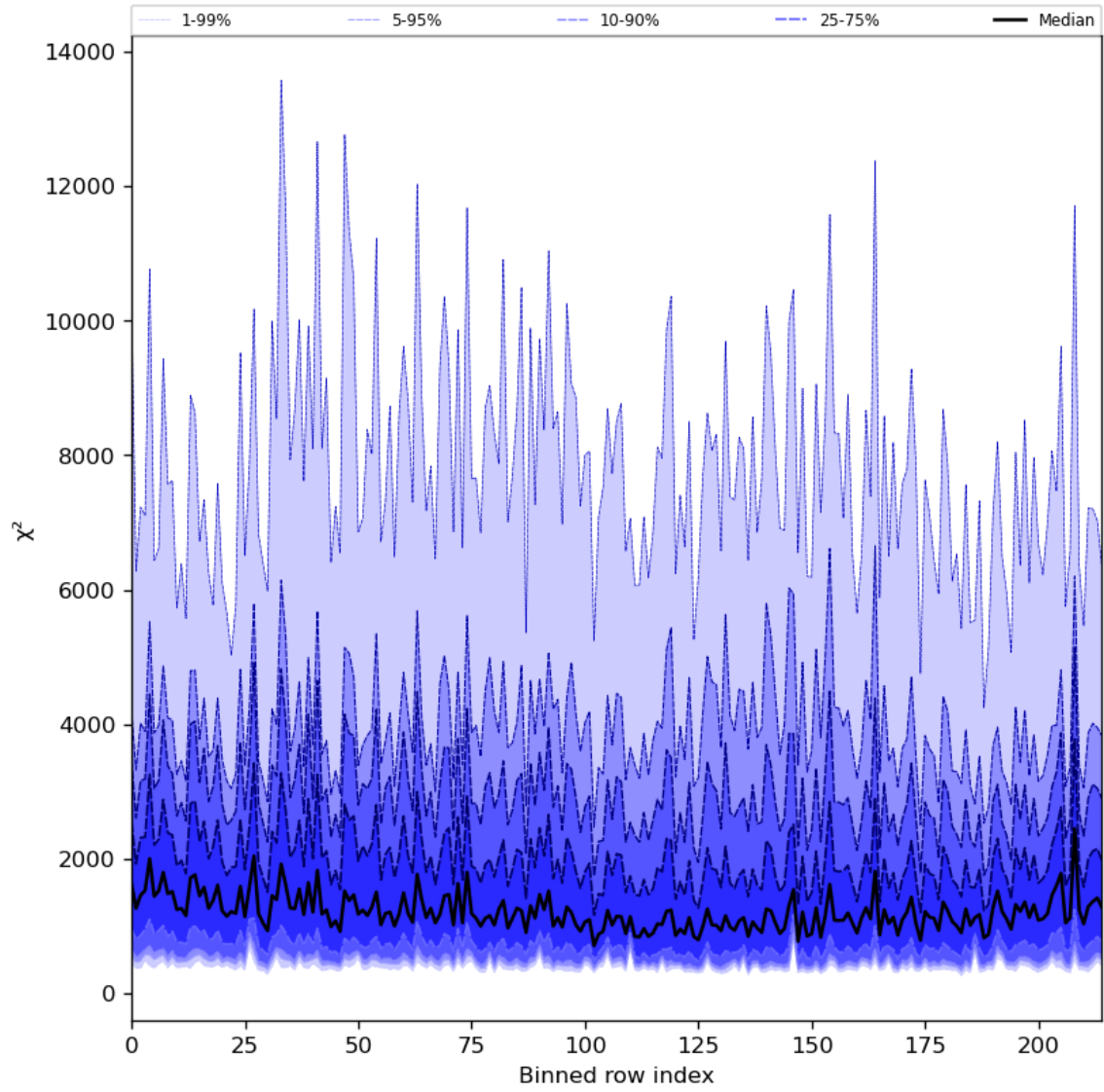
Figure 30: Along track statistics of “ \chi^2 ” for 2024-06-24 to 2024-06-26
