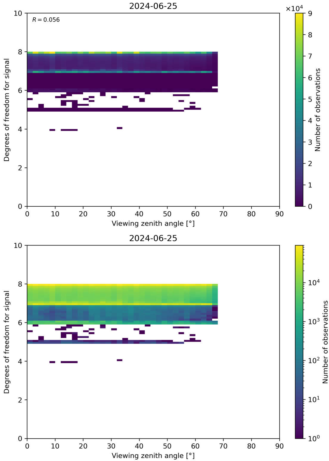
Figure 73: Scatter density plot of “Viewing zenith angle” against “Degrees of freedom for signal” for 2024-06-24 to 2024-06-26.
