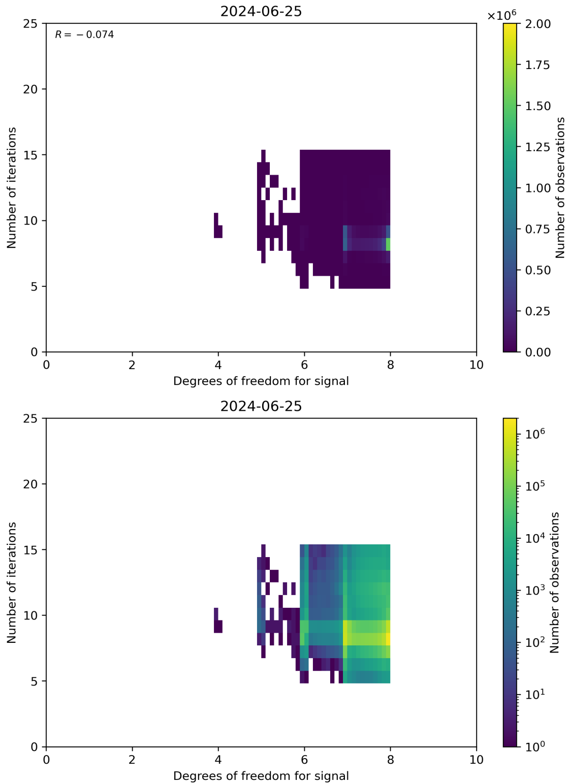
Figure 50: Scatter density plot of “Degrees of freedom for signal” against “Number of iterations” for 2024-06-24 to 2024-06-26.
