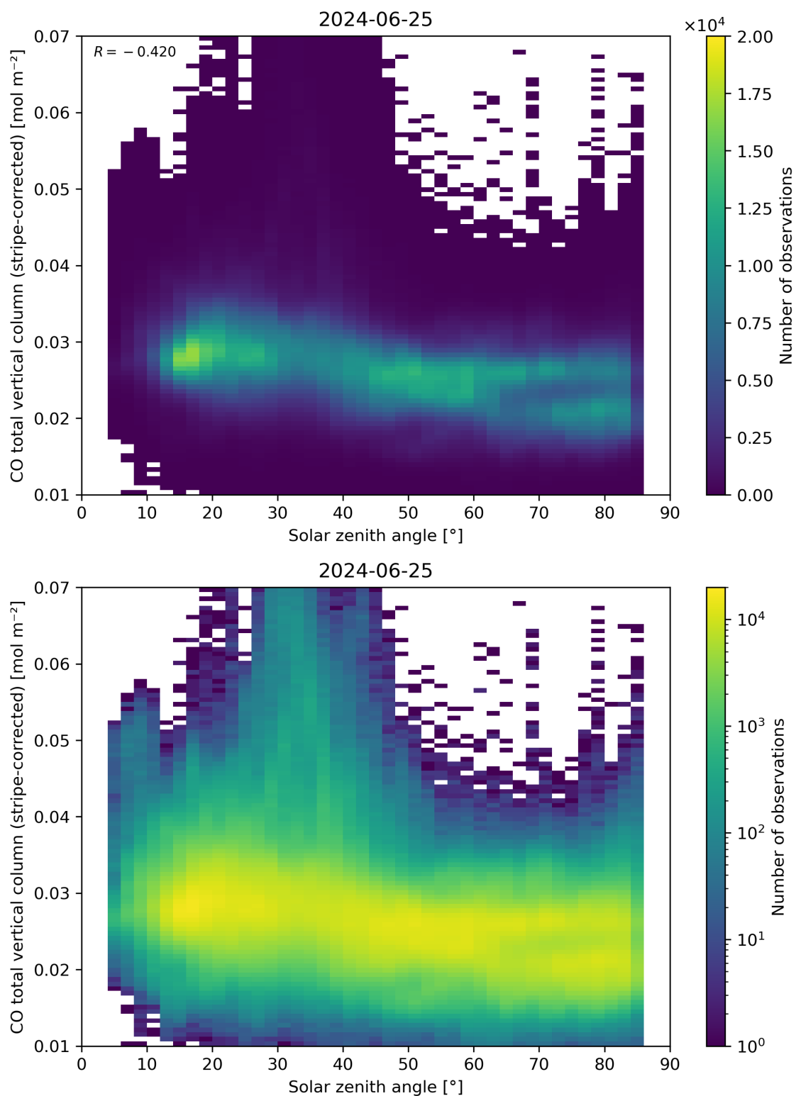
Figure 62: Scatter density plot of “Solar zenith angle” against “CO total vertical column (stripe-corrected)” for 2024-06-24 to 2024-06-26.
