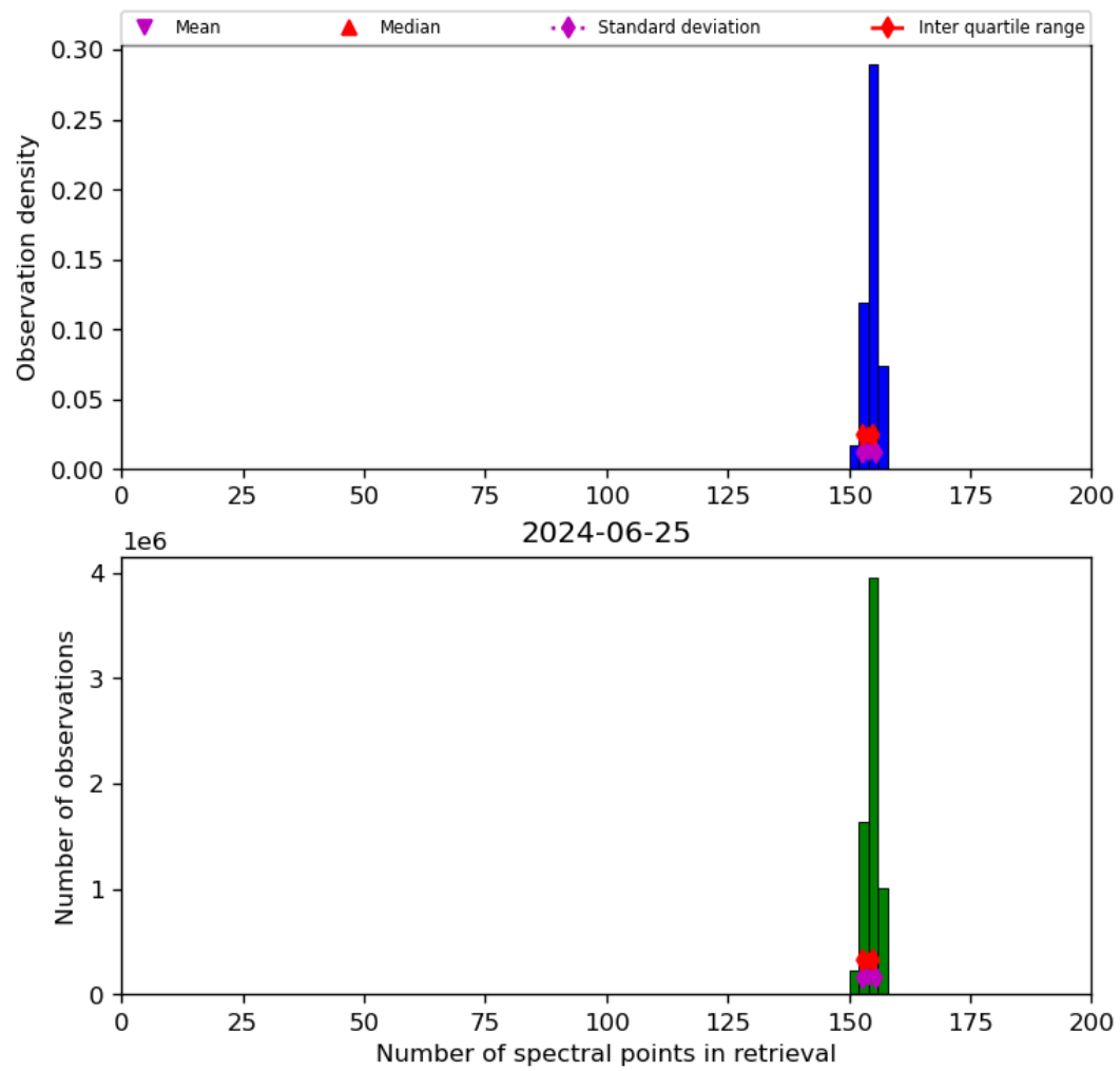
Figure 21: Histogram of “Number of spectral points in retrieval” for 2024-06-24 to 2024-06-26
