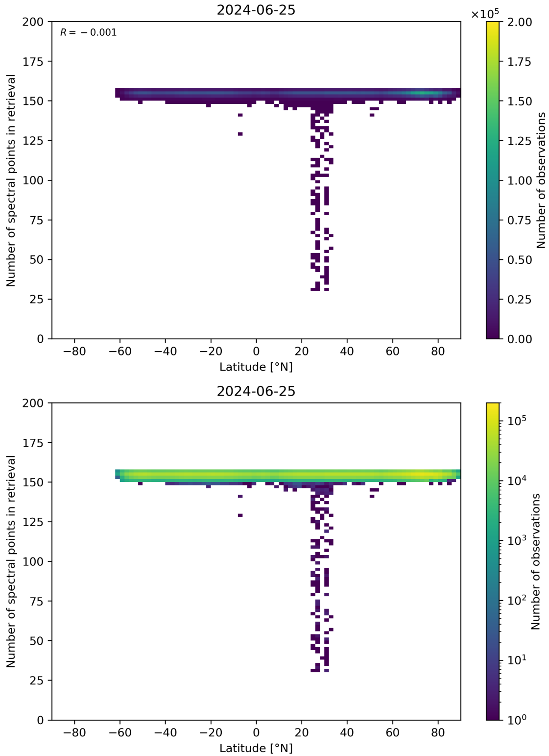
Figure 57: Scatter density plot of “Latitude” against “Number of spectral points in retrieval” for 2024-06-24 to 2024-06-26.
