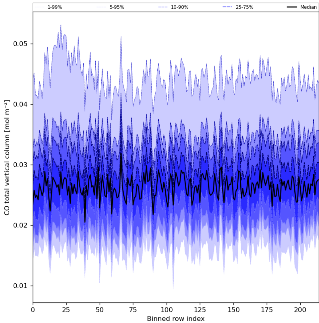
Figure 26: Along track statistics of “CO total vertical column” for 2024-06-24 to 2024-06-26
