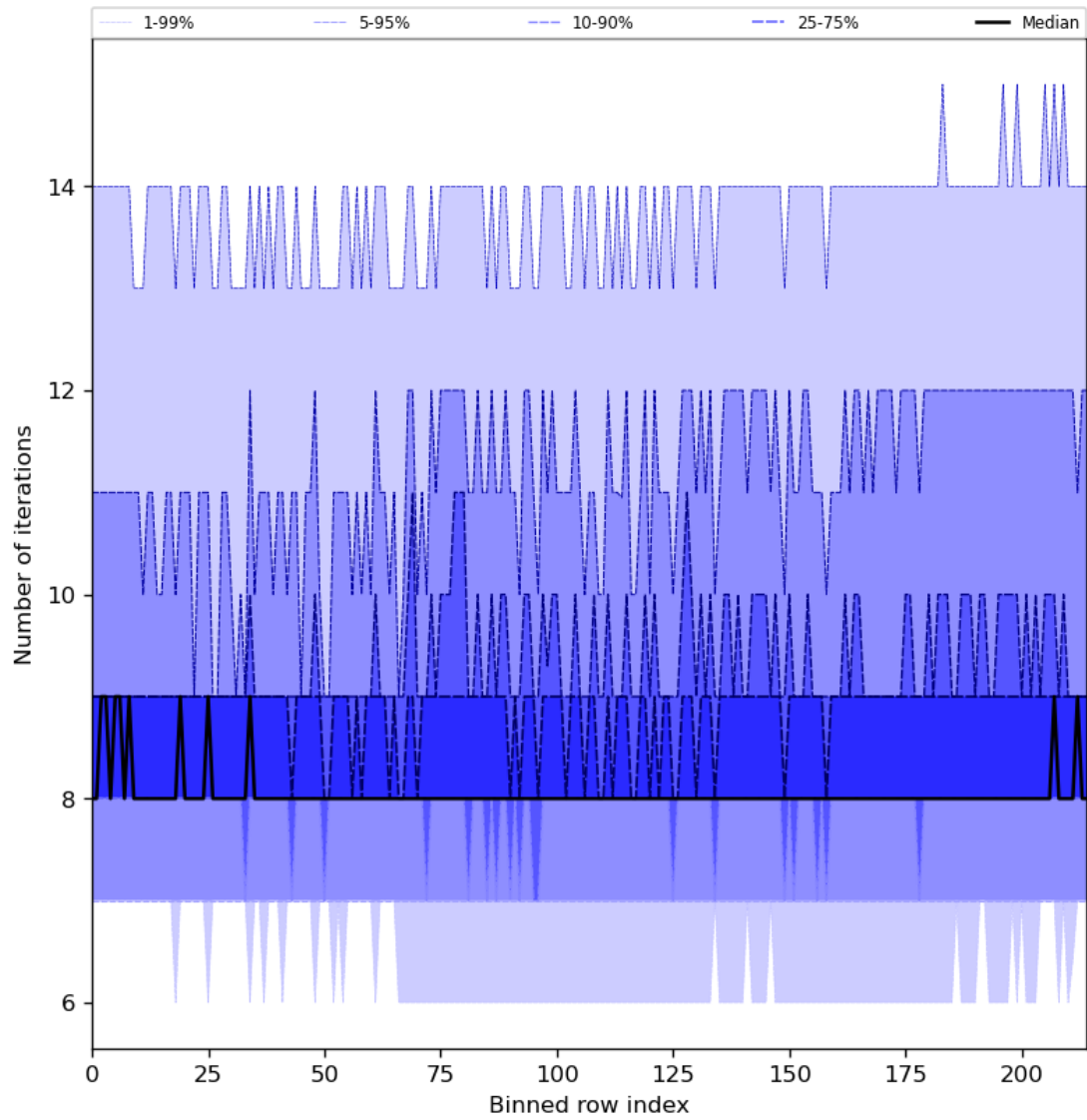
Figure 32: Along track statistics of “Number of iterations” for 2024-06-24 to 2024-06-26
