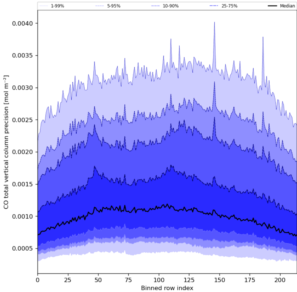
Figure 28: Along track statistics of “CO total vertical column precision” for 2024-06-24 to 2024-06-26
