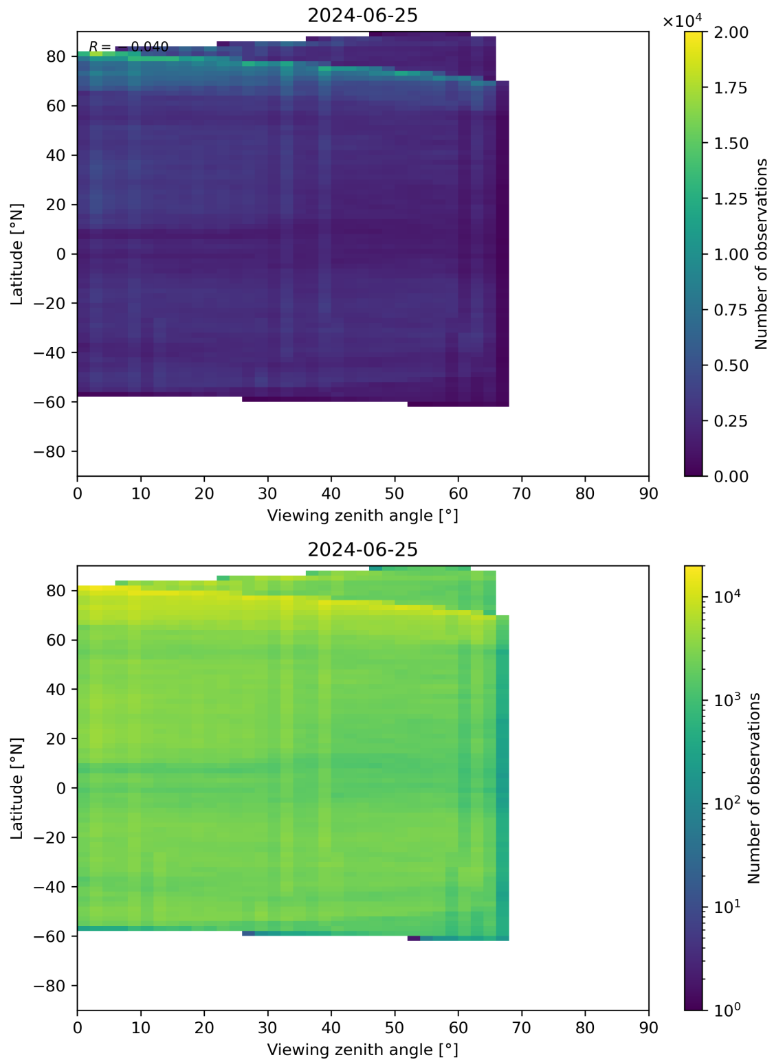
Figure 74: Scatter density plot of “Viewing zenith angle” against “Latitude” for 2024-06-24 to 2024-06-26.
