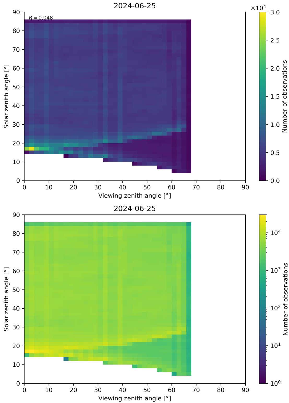
Figure 77: Scatter density plot of “Viewing zenith angle” against “Solar zenith angle” for 2024-06-24 to 2024-06-26.
