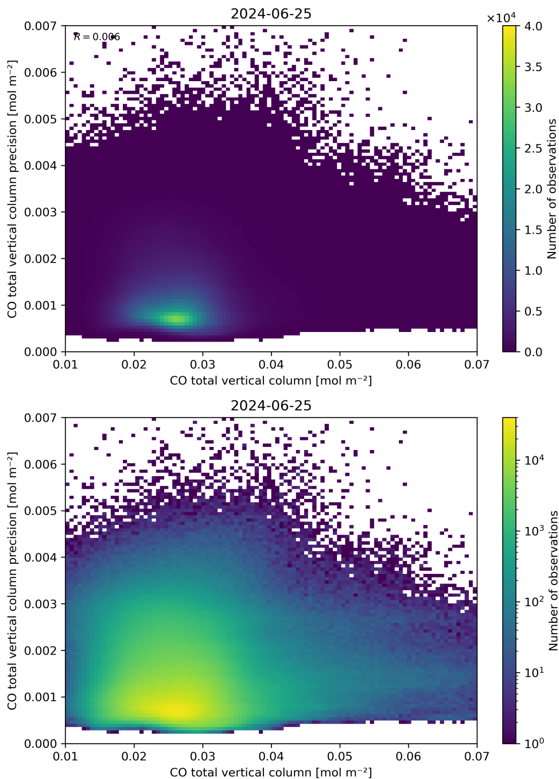
Figure 34: Scatter density plot of “CO total vertical column” against “CO total vertical column precision” for 2024-06-24 to 2024-06-26.
