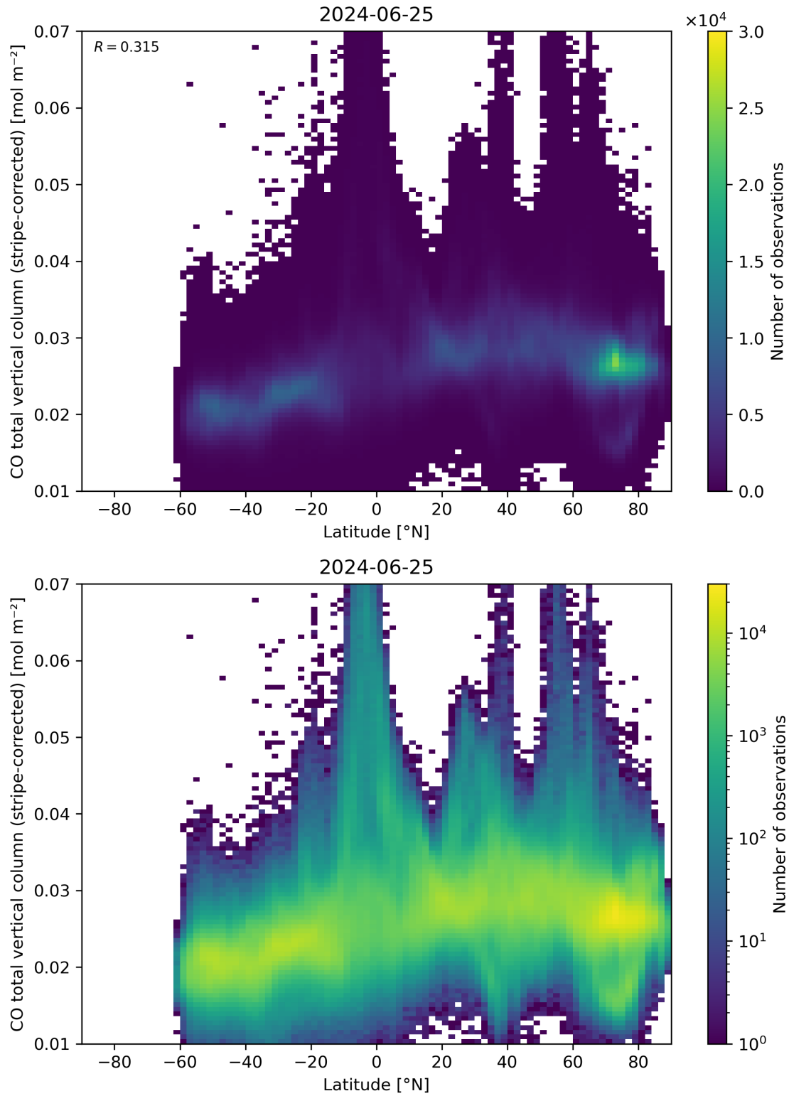
Figure 52: Scatter density plot of “Latitude” against “CO total vertical column (stripe-corrected)” for 2024-06-24 to 2024-06-26.
