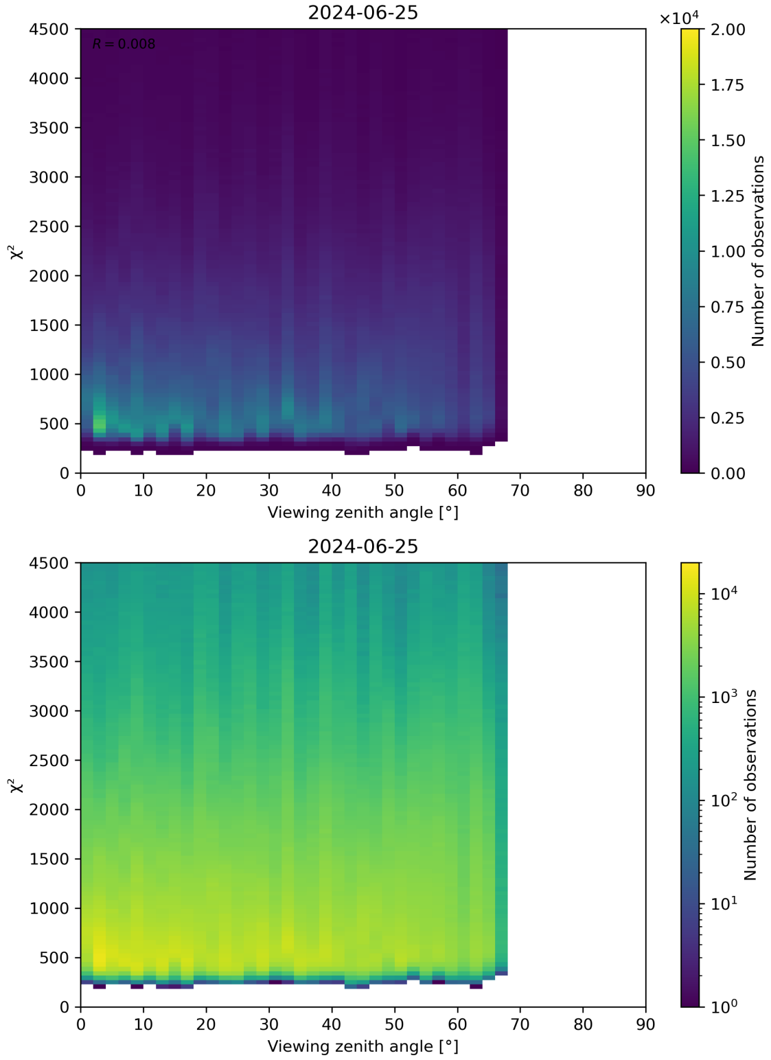
Figure 72: Scatter density plot of “Viewing zenith angle” against “ \chi^2 ” for 2024-06-24 to 2024-06-26.
