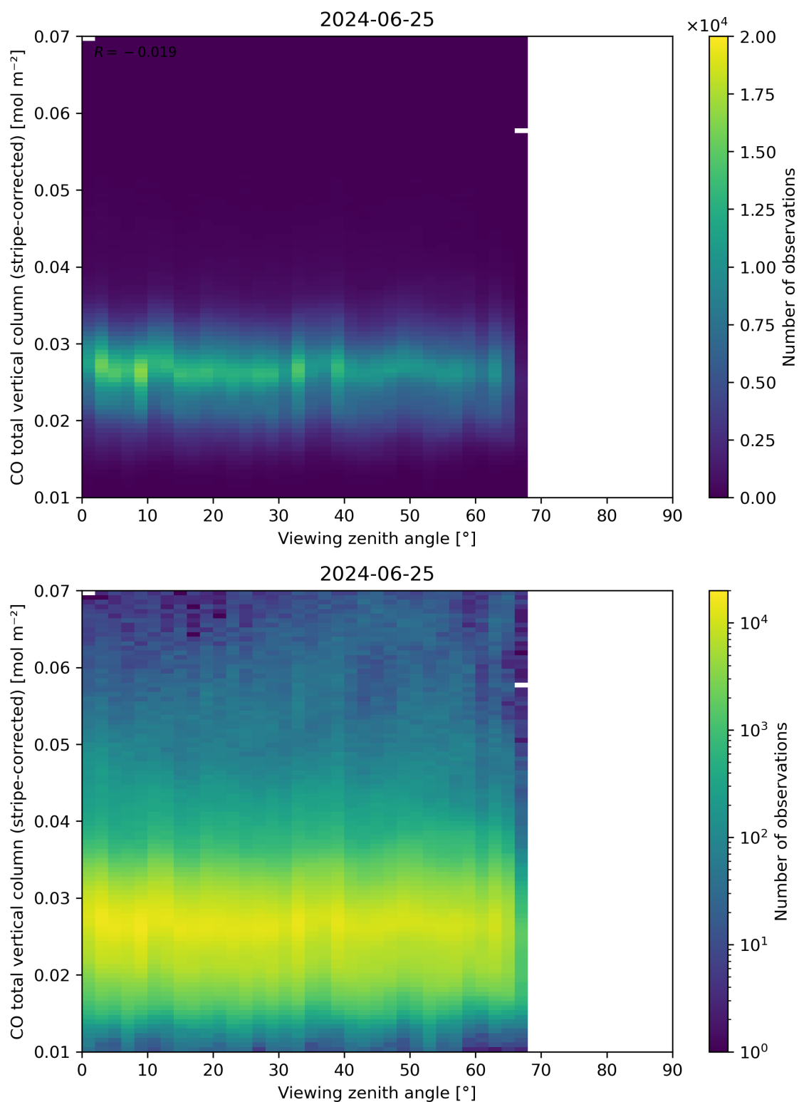
Figure 70: Scatter density plot of “Viewing zenith angle” against “CO total vertical column (stripe-corrected)” for 2024-06-24 to 2024-06-26.
