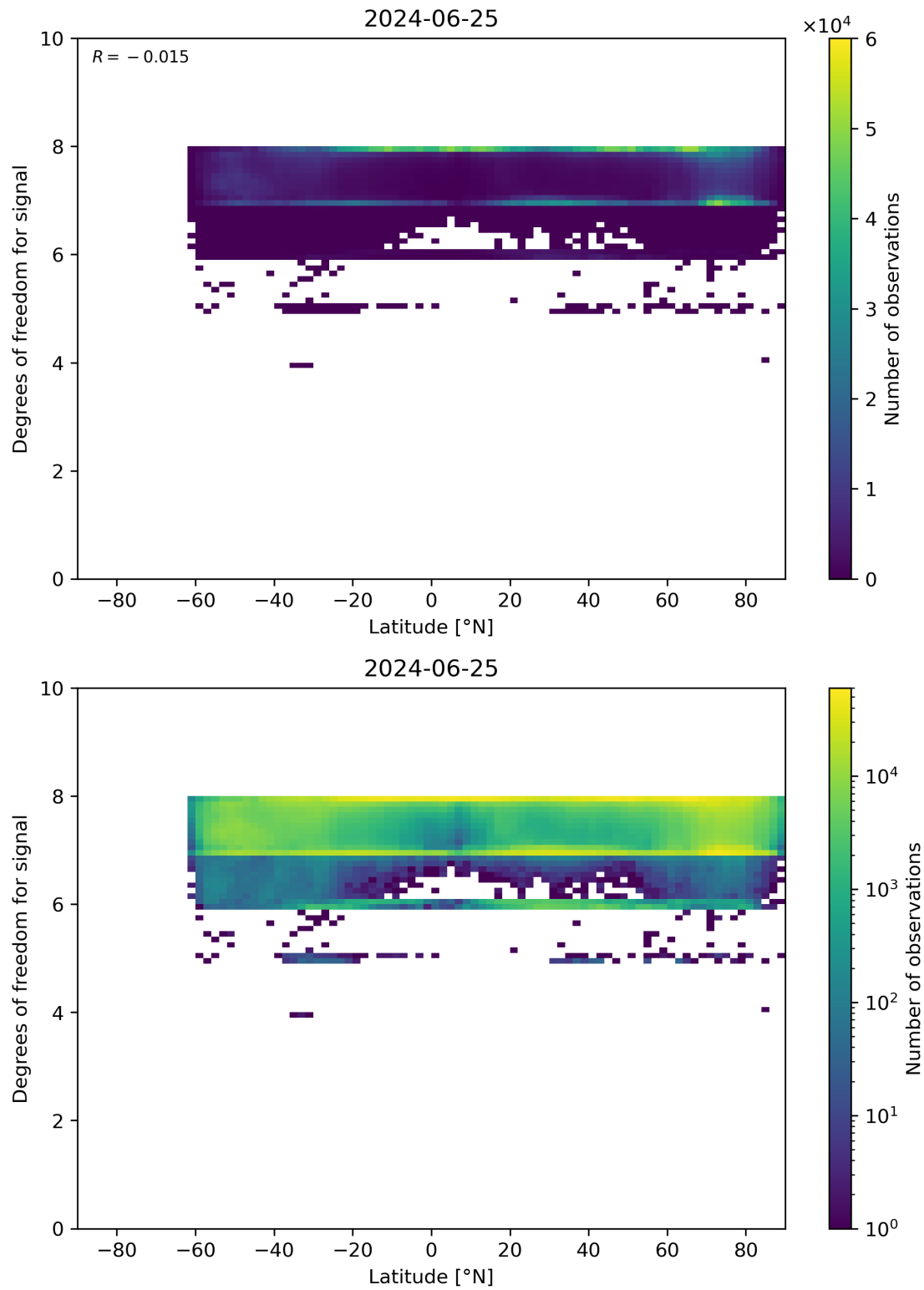
Figure 55: Scatter density plot of “Latitude” against “Degrees of freedom for signal” for 2024-06-24 to 2024-06-26.
