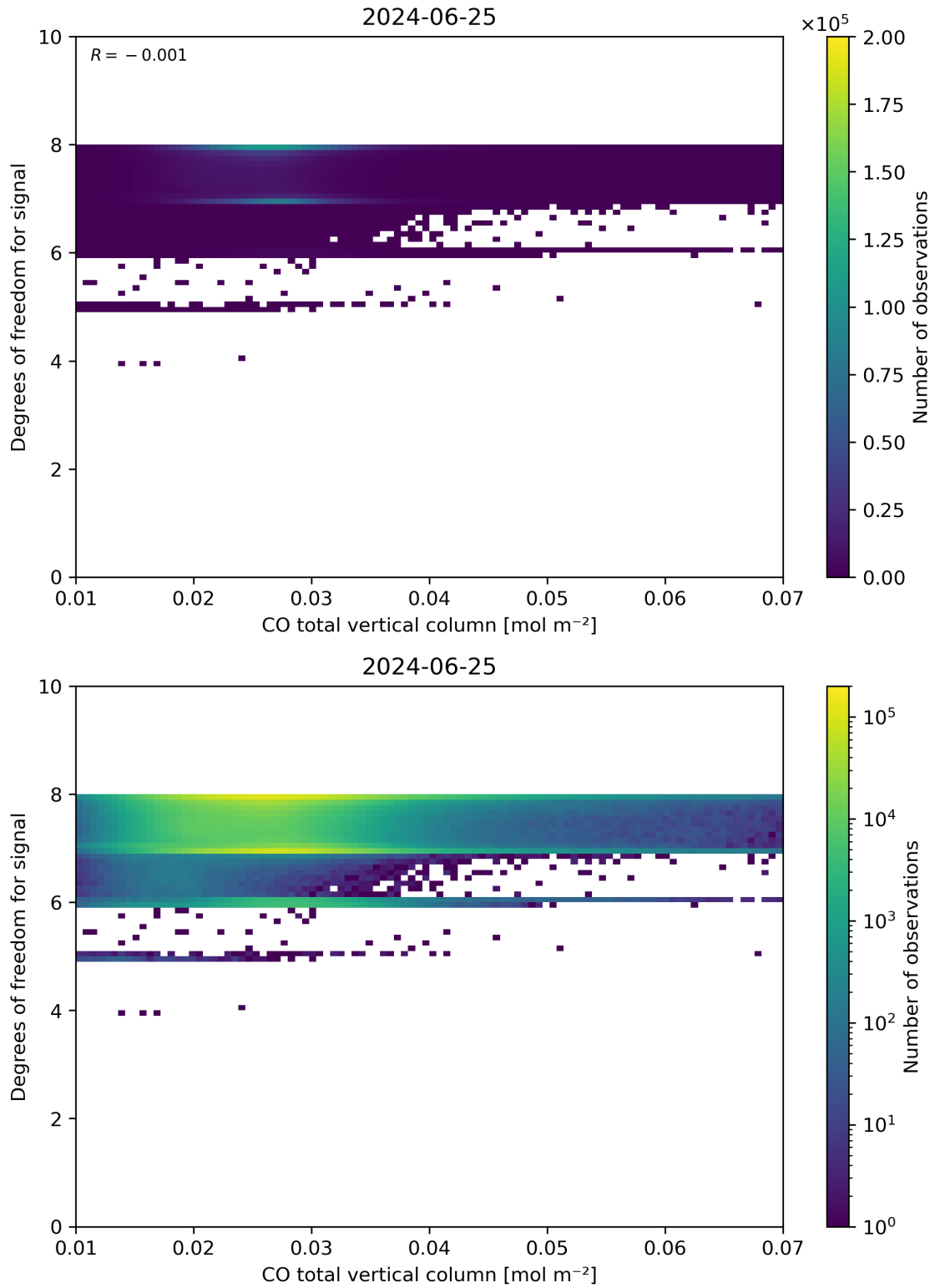
Figure 41: Scatter density plot of “CO total vertical column” against “Degrees of freedom for signal” for 2024-06-24 to 2024-06-26.
