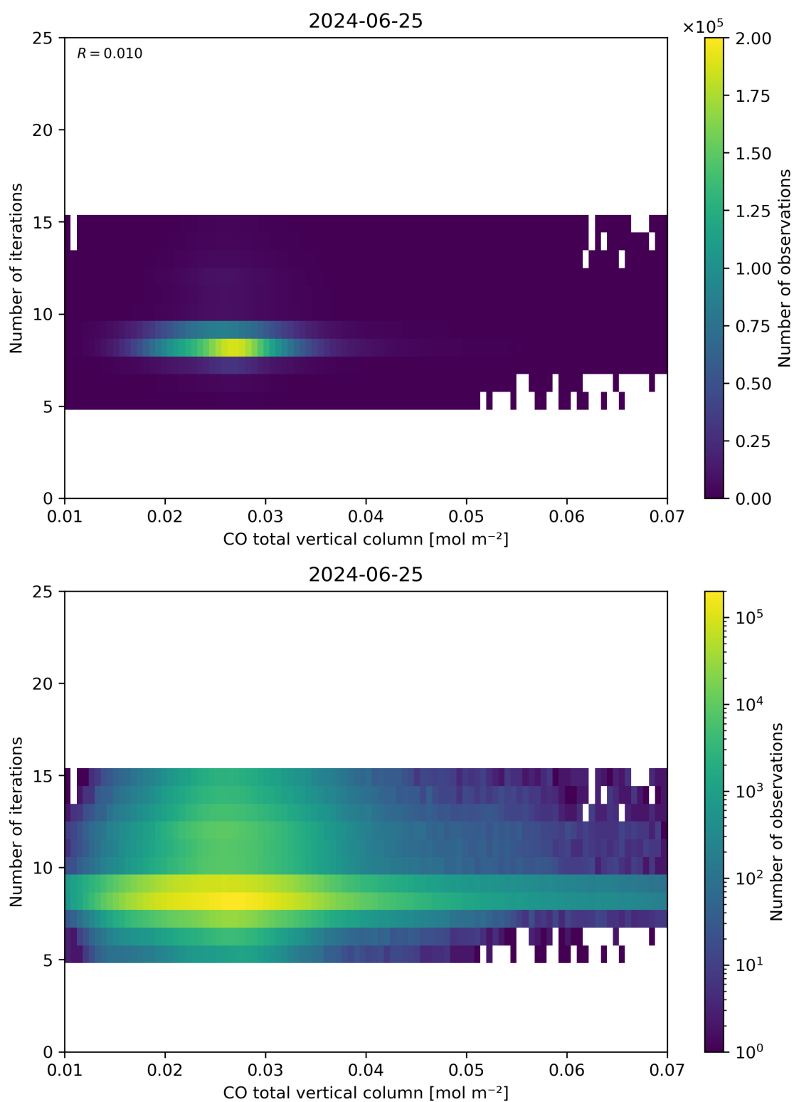
Figure 42: Scatter density plot of “CO total vertical column” against “Number of iterations” for 2024-06-24 to 2024-06-26.
