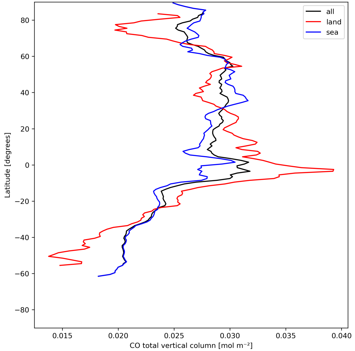
Figure 10: Zonal average of “CO total vertical column” for 2024-06-24 to 2024-06-26.
