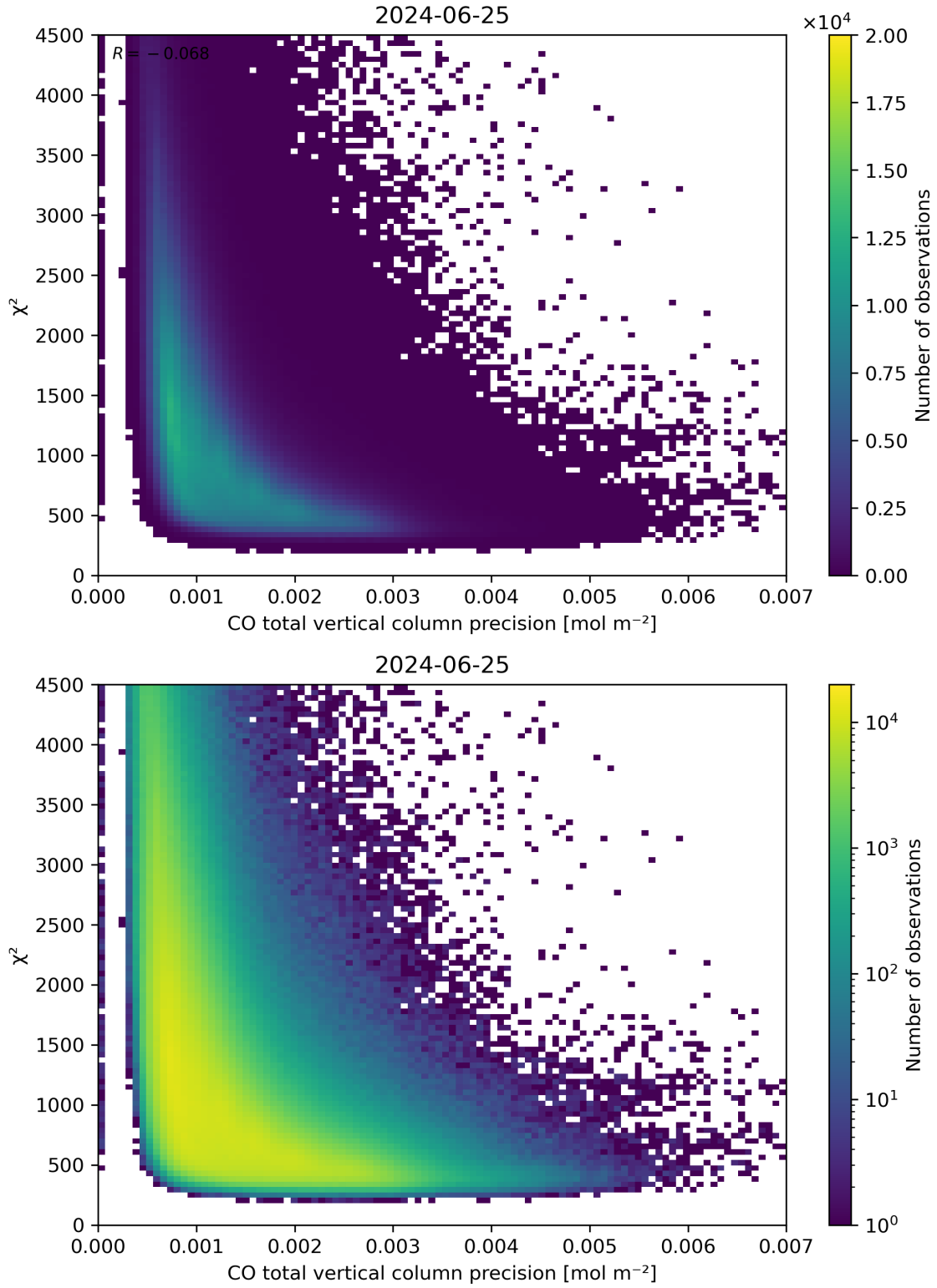
Figure 44: Scatter density plot of “CO total vertical column precision” against “ \chi^2 ” for 2024-06-24 to 2024-06-26.
