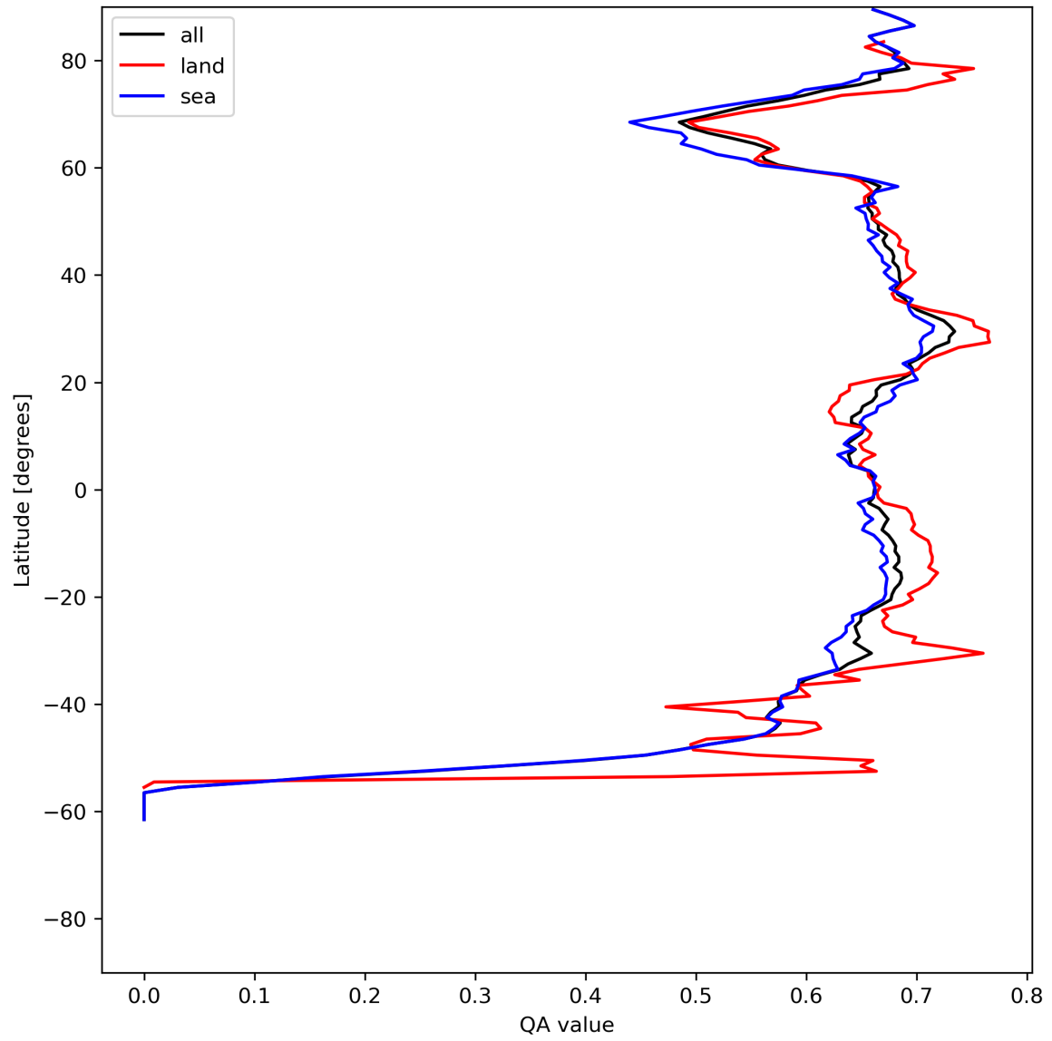
Figure 9: Zonal average of “QA value” for 2024-06-25 to 2024-06-27.
