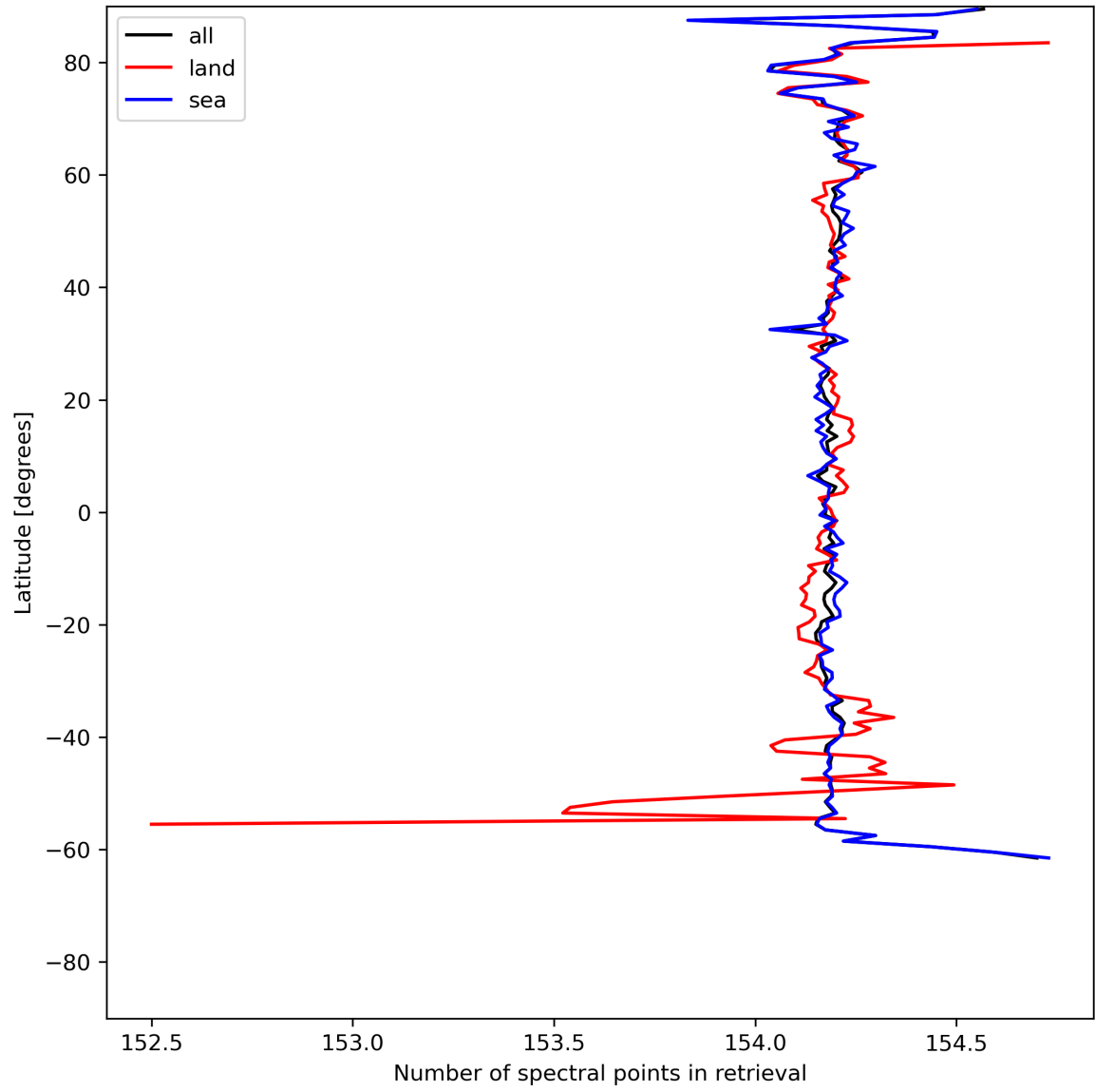
Figure 13: Zonal average of “Number of spectral points in retrieval” for 2024-06-25 to 2024-06-27.
