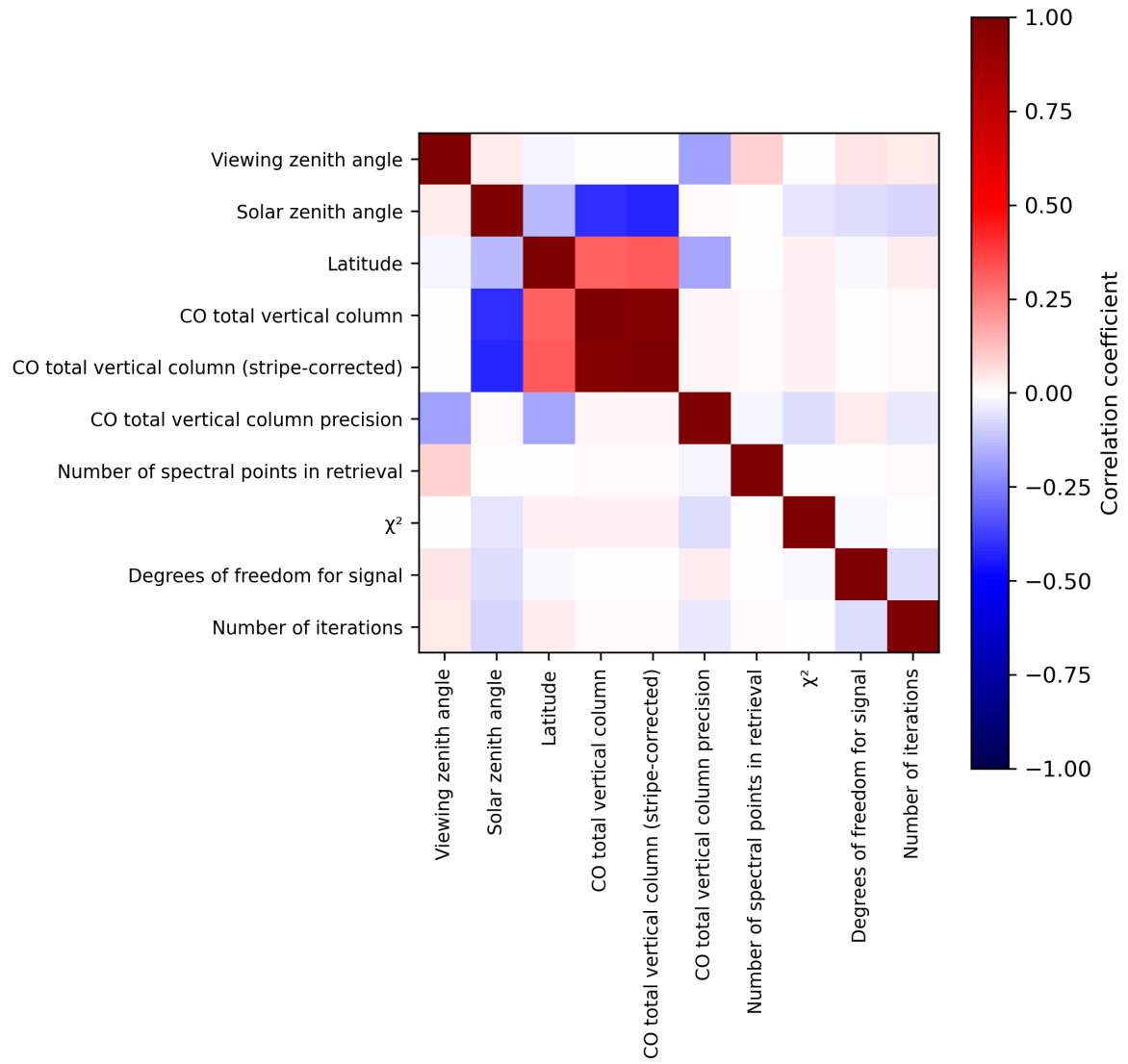
Figure 2: Map of correlation matrix for 2024-06-25 to 2024-06-27.
