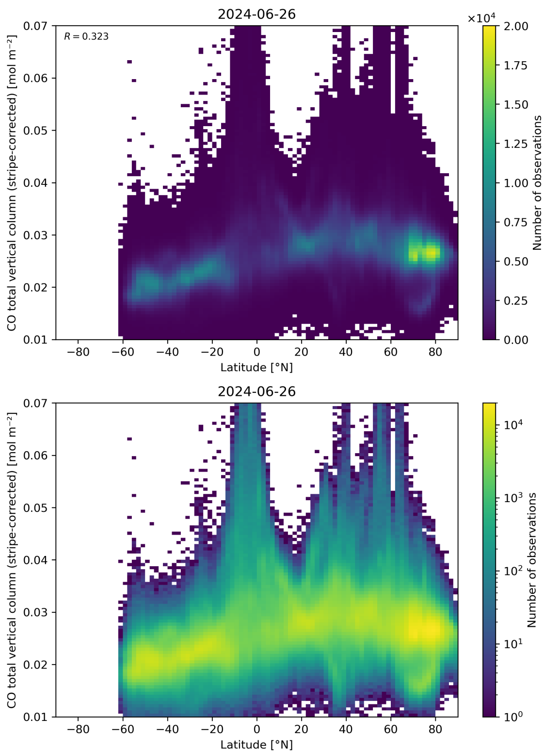
Figure 52: Scatter density plot of “Latitude” against “CO total vertical column (stripe-corrected)” for 2024-06-25 to 2024-06-27.
