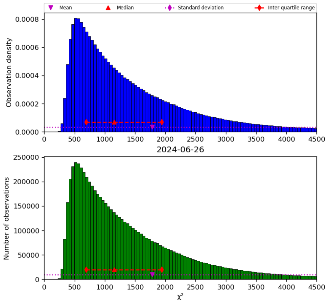
Figure 22: Histogram of “ \chi^2 ” for 2024-06-25 to 2024-06-27
