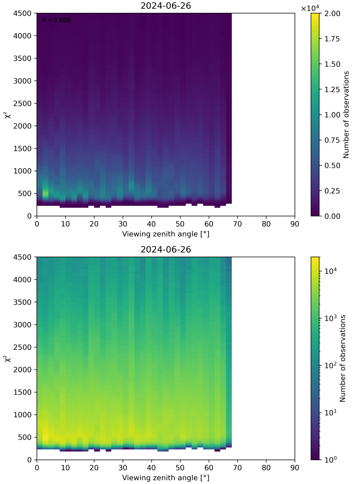
Figure 72: Scatter density plot of “Viewing zenith angle” against “ \chi^2 ” for 2024-06-25 to 2024-06-27.
