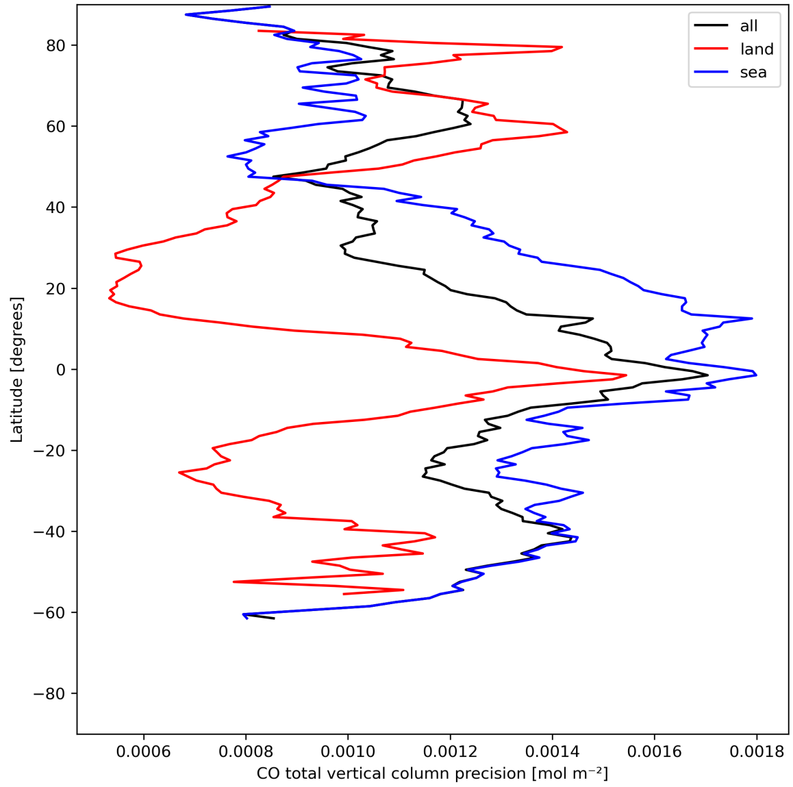
Figure 12: Zonal average of “CO total vertical column precision” for 2024-06-25 to 2024-06-27.
