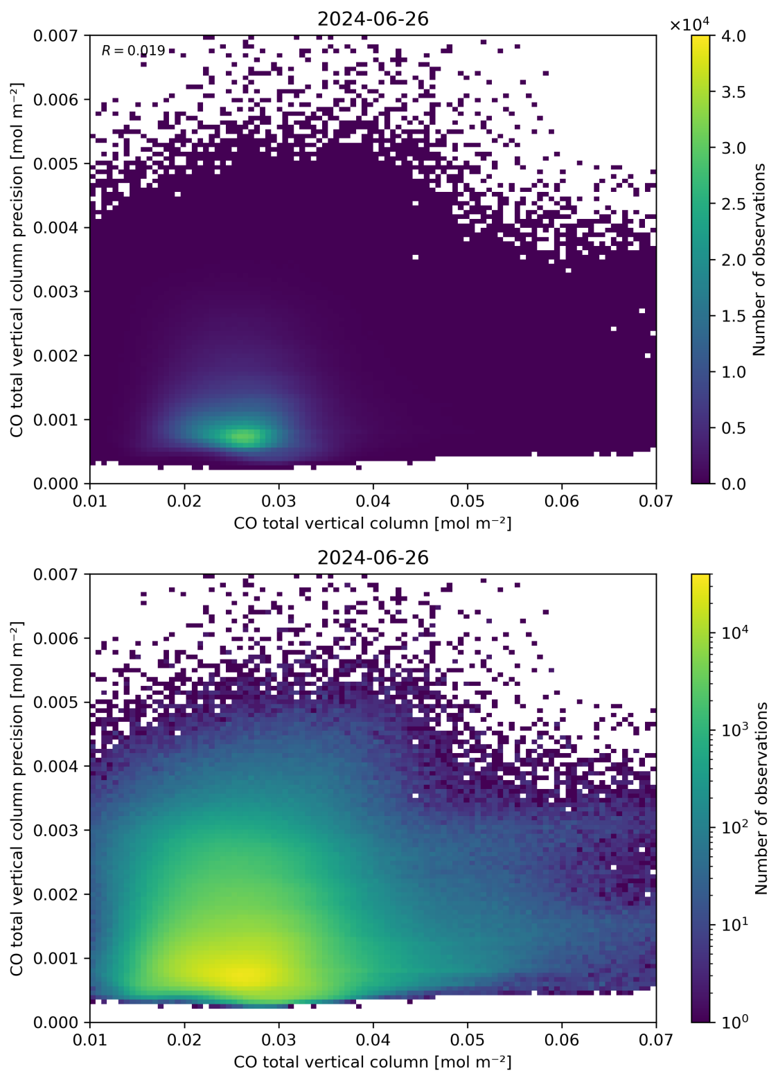
Figure 34: Scatter density plot of “CO total vertical column” against “CO total vertical column precision” for 2024-06-25 to 2024-06-27.
