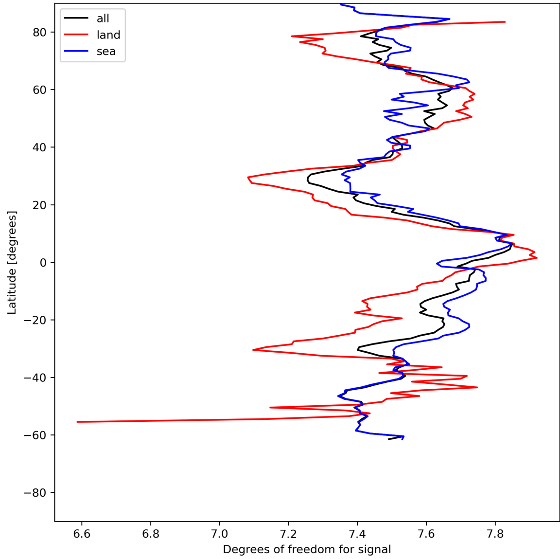
Figure 15: Zonal average of “Degrees of freedom for signal” for 2024-06-25 to 2024-06-27.
