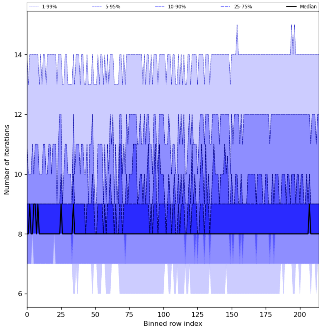
Figure 32: Along track statistics of “Number of iterations” for 2024-06-25 to 2024-06-27
