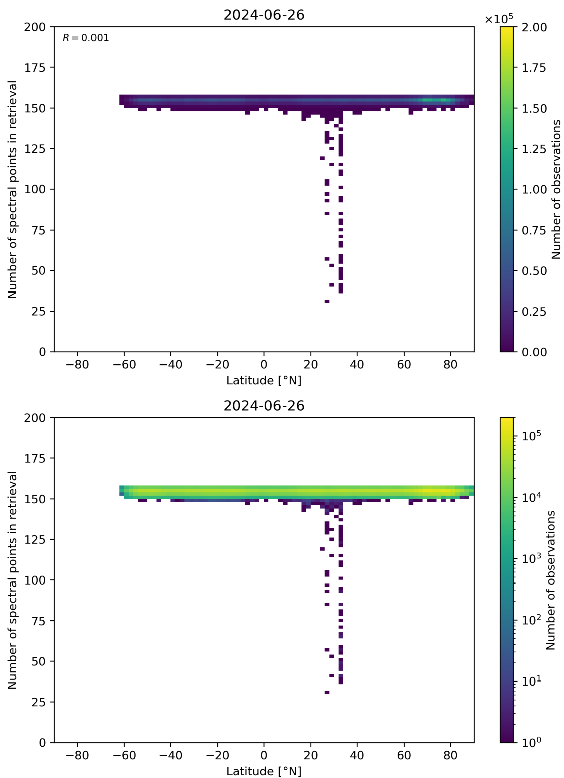
Figure 57: Scatter density plot of “Latitude” against “Number of spectral points in retrieval” for 2024-06-25 to 2024-06-27.
