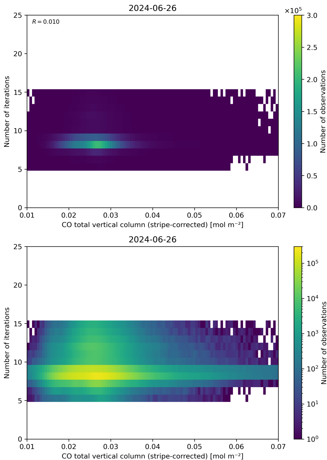
Figure 39: Scatter density plot of “CO total vertical column (stripe-corrected)” against “Number of iterations” for 2024-06-25 to 2024-06-27.
