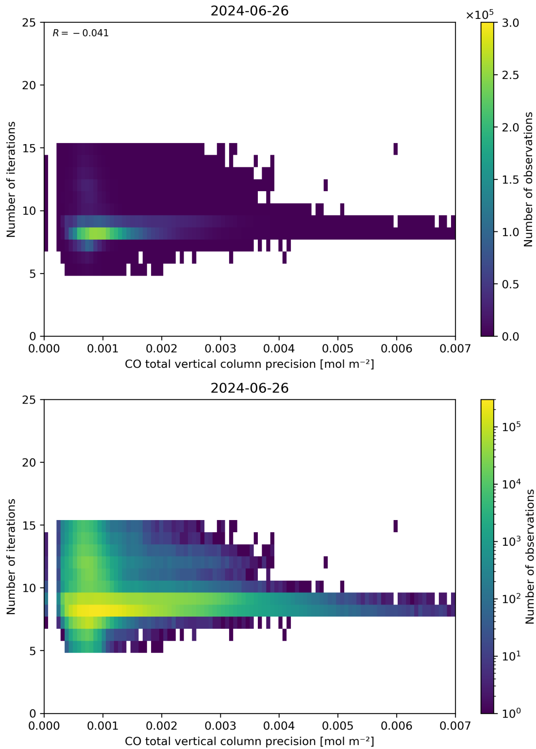
Figure 46: Scatter density plot of “CO total vertical column precision” against “Number of iterations” for 2024-06-25 to 2024-06-27.
