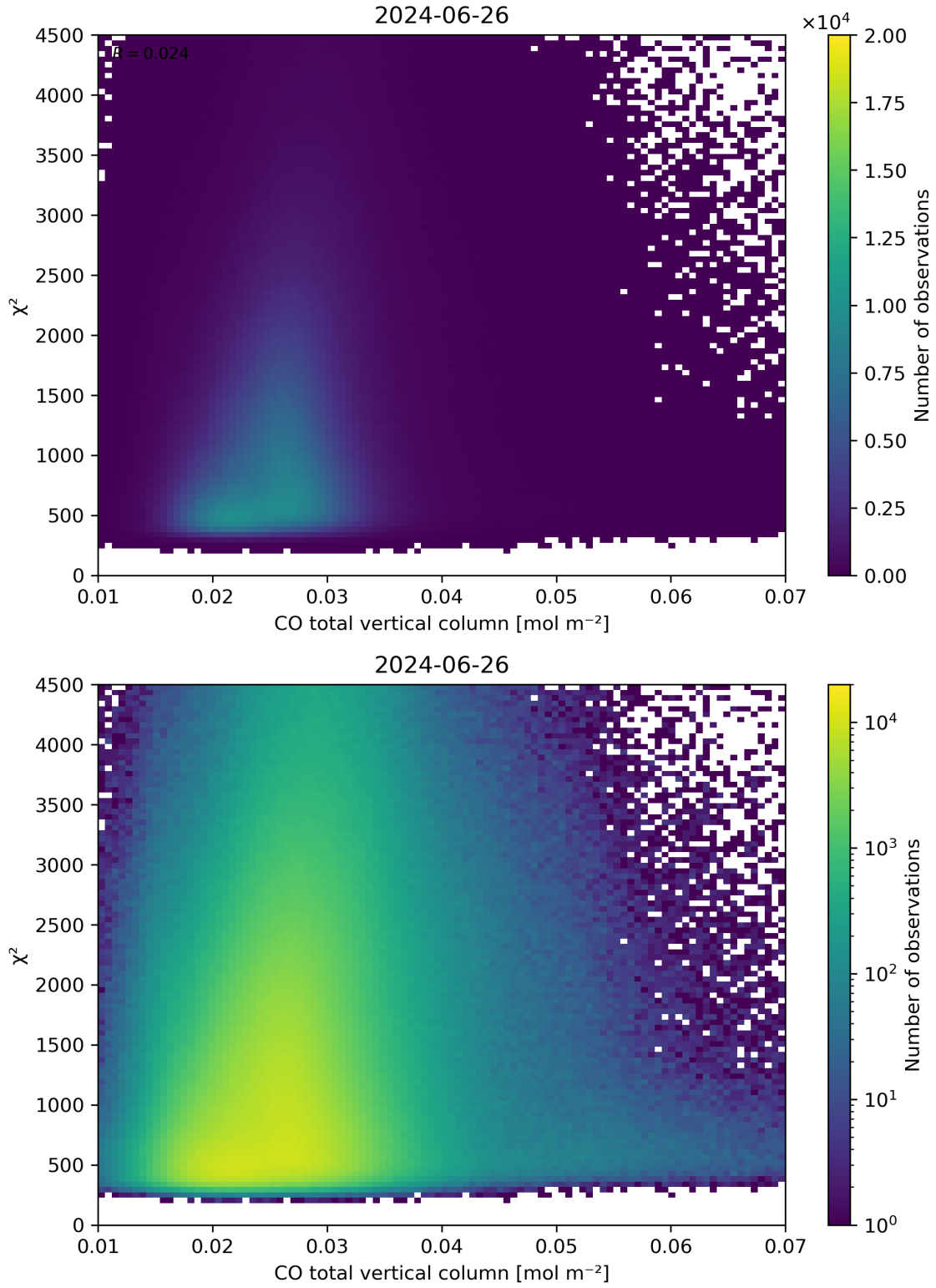
Figure 35: Scatter density plot of “CO total vertical column” against “ \chi^2 ” for 2024-06-25 to 2024-06-27.
