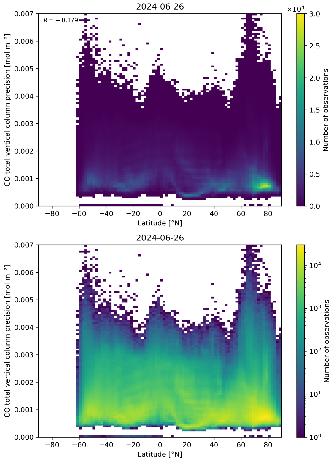
Figure 53: Scatter density plot of “Latitude” against “CO total vertical column precision” for 2024-06-25 to 2024-06-27.
