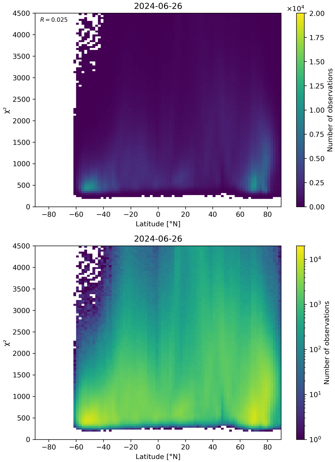
Figure 54: Scatter density plot of “Latitude” against “ \chi^2 ” for 2024-06-25 to 2024-06-27.
