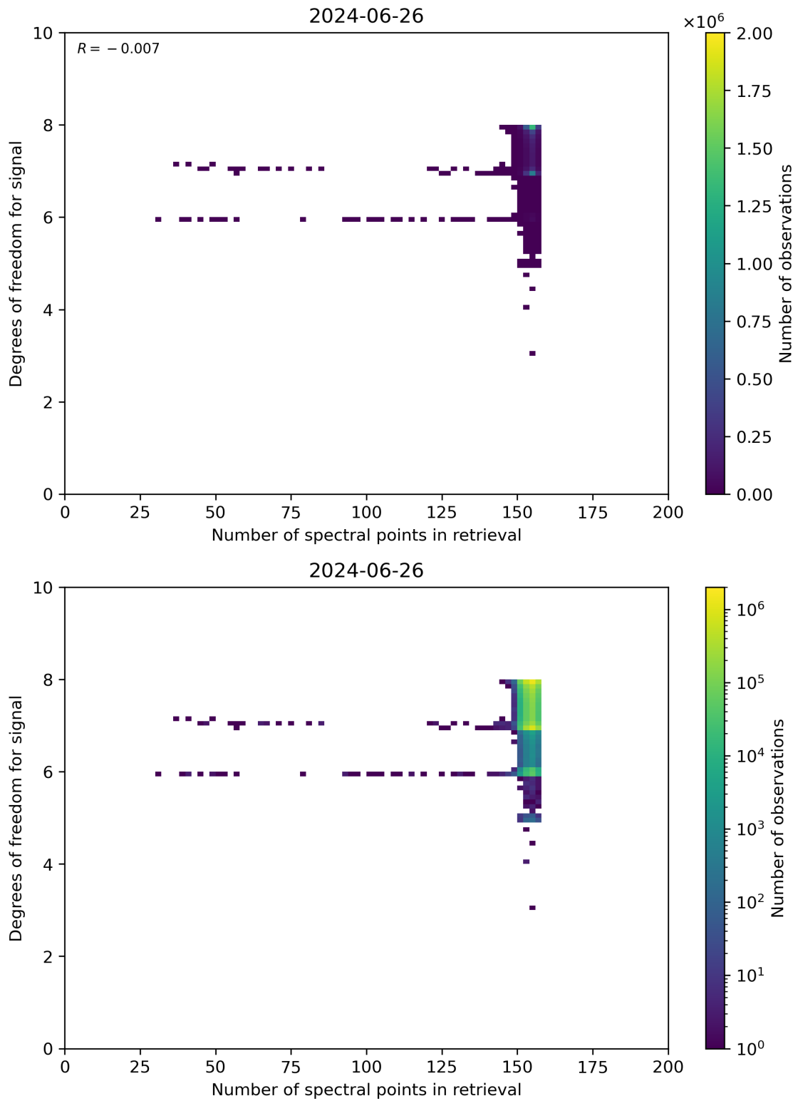
Figure 59: Scatter density plot of “Number of spectral points in retrieval” against “Degrees of freedom for signal” for 2024-06-25 to 2024-06-27.
