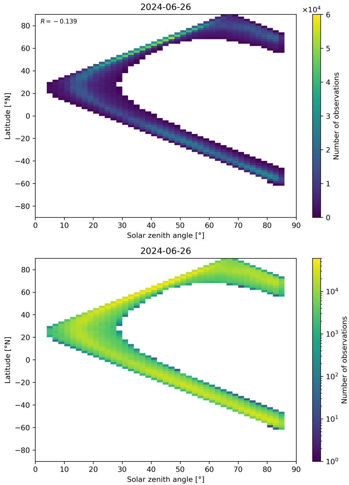
Figure 66: Scatter density plot of “Solar zenith angle” against “Latitude” for 2024-06-25 to 2024-06-27.
