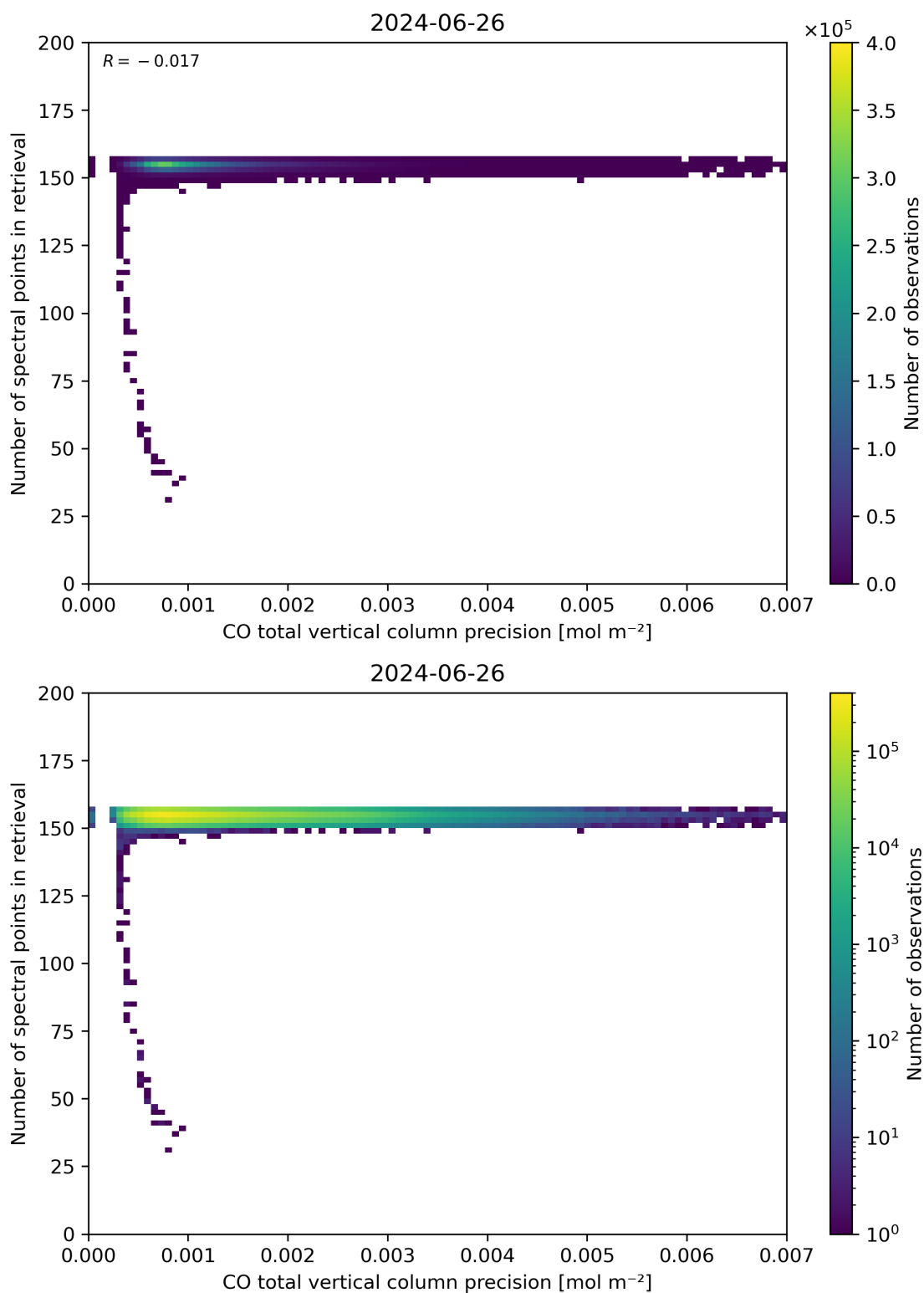
Figure 47: Scatter density plot of “CO total vertical column precision” against “Number of spectral points in retrieval” for 2024-06-25 to 2024-06-27.
