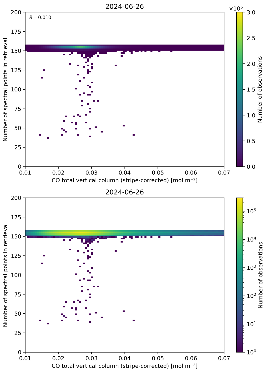
Figure 40: Scatter density plot of “CO total vertical column (stripe-corrected)” against “Number of spectral points in retrieval” for 2024-06-25 to 2024-06-27.
