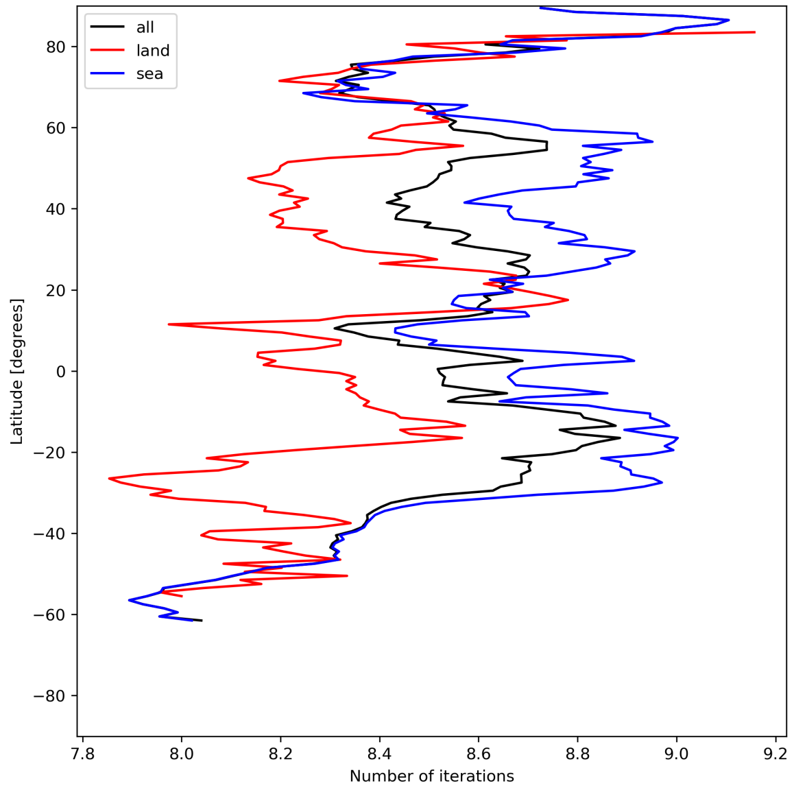
Figure 16: Zonal average of “Number of iterations” for 2024-06-25 to 2024-06-27.
