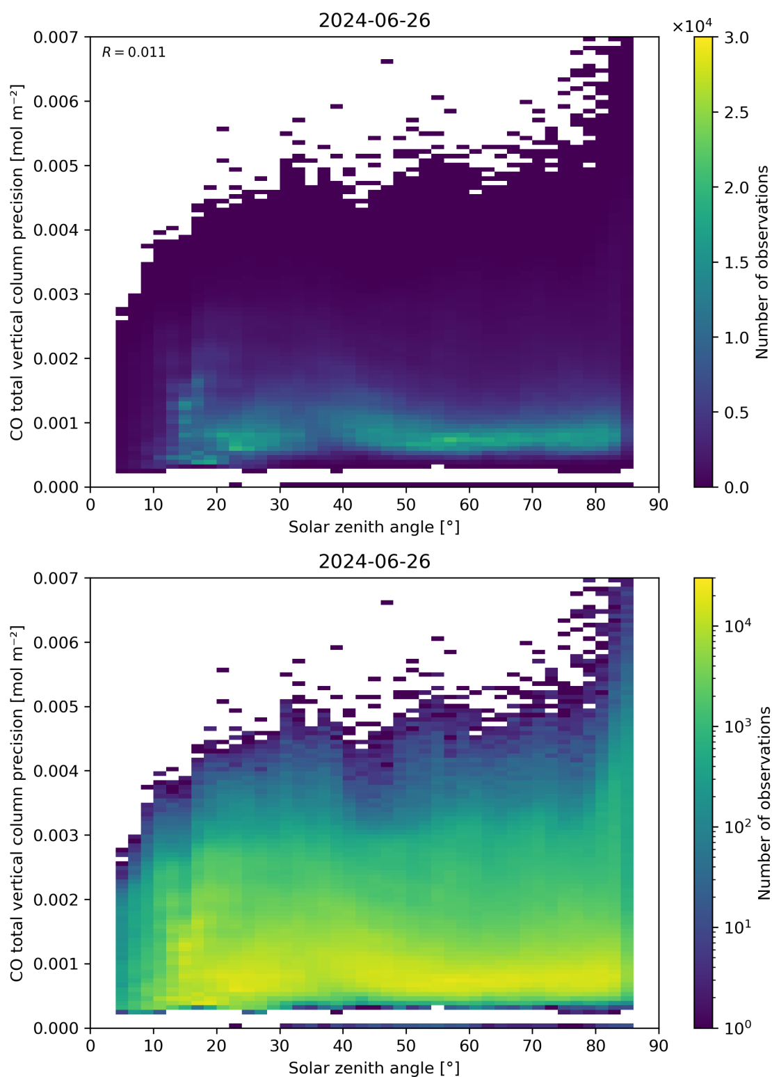
Figure 63: Scatter density plot of “Solar zenith angle” against “CO total vertical column precision” for 2024-06-25 to 2024-06-27.
