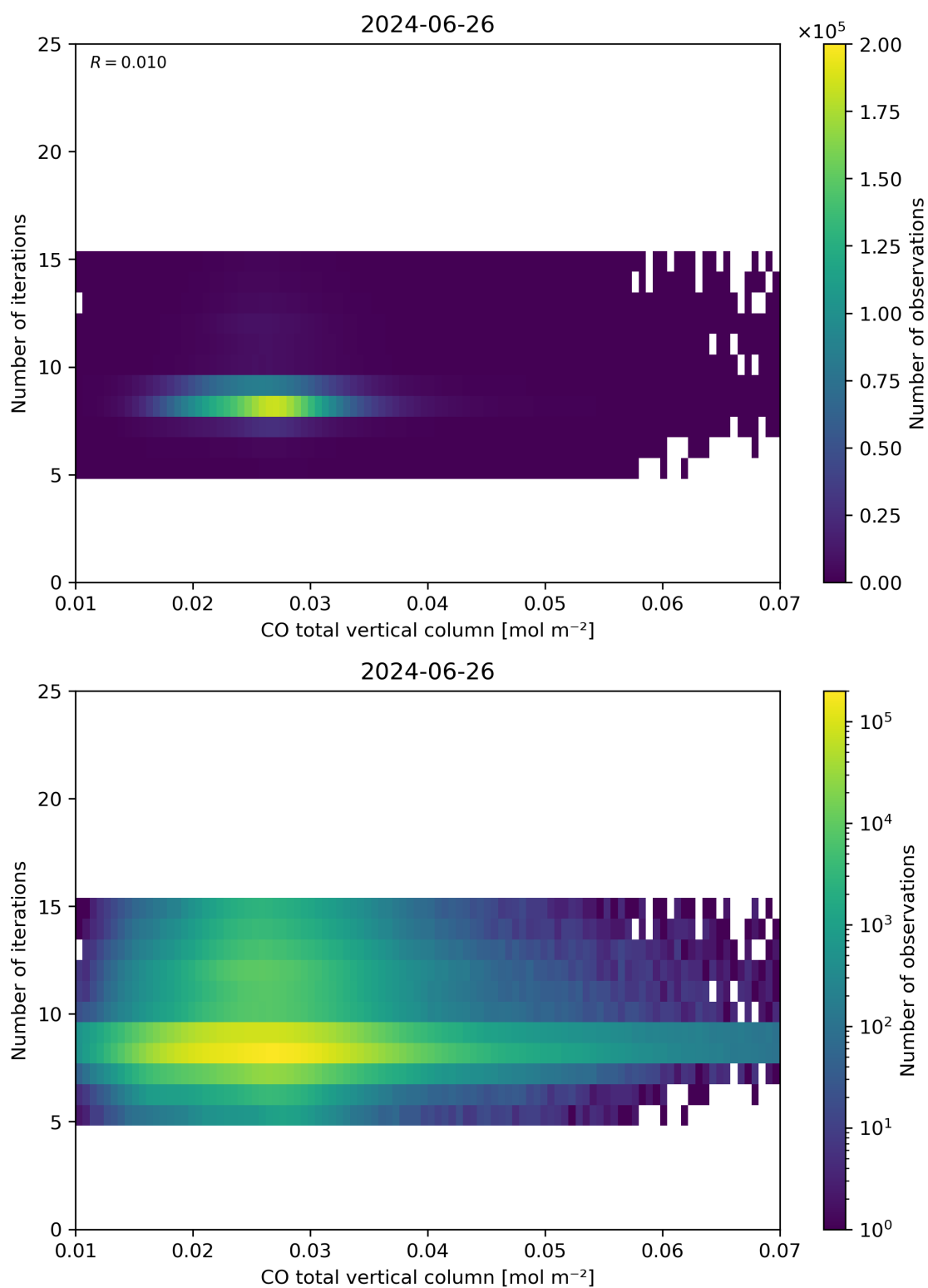
Figure 42: Scatter density plot of “CO total vertical column” against “Number of iterations” for 2024-06-25 to 2024-06-27.
