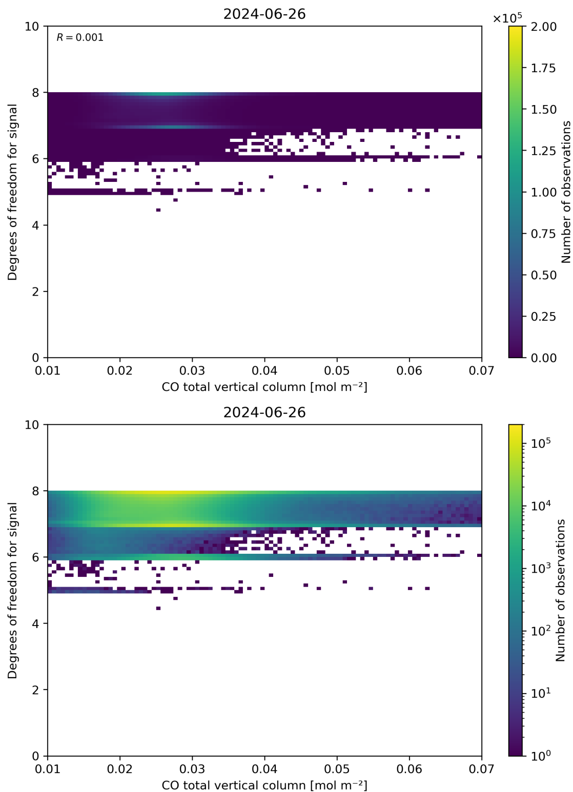
Figure 41: Scatter density plot of “CO total vertical column” against “Degrees of freedom for signal” for 2024-06-25 to 2024-06-27.
