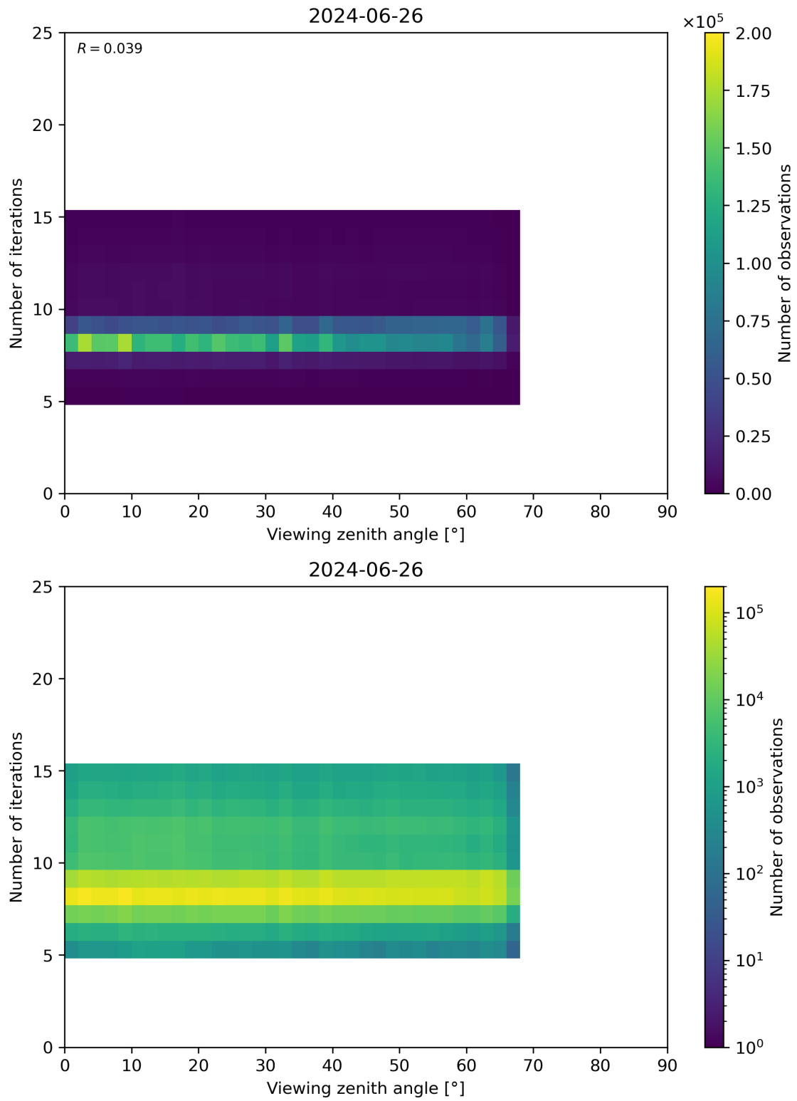
Figure 75: Scatter density plot of “Viewing zenith angle” against “Number of iterations” for 2024-06-25 to 2024-06-27.
