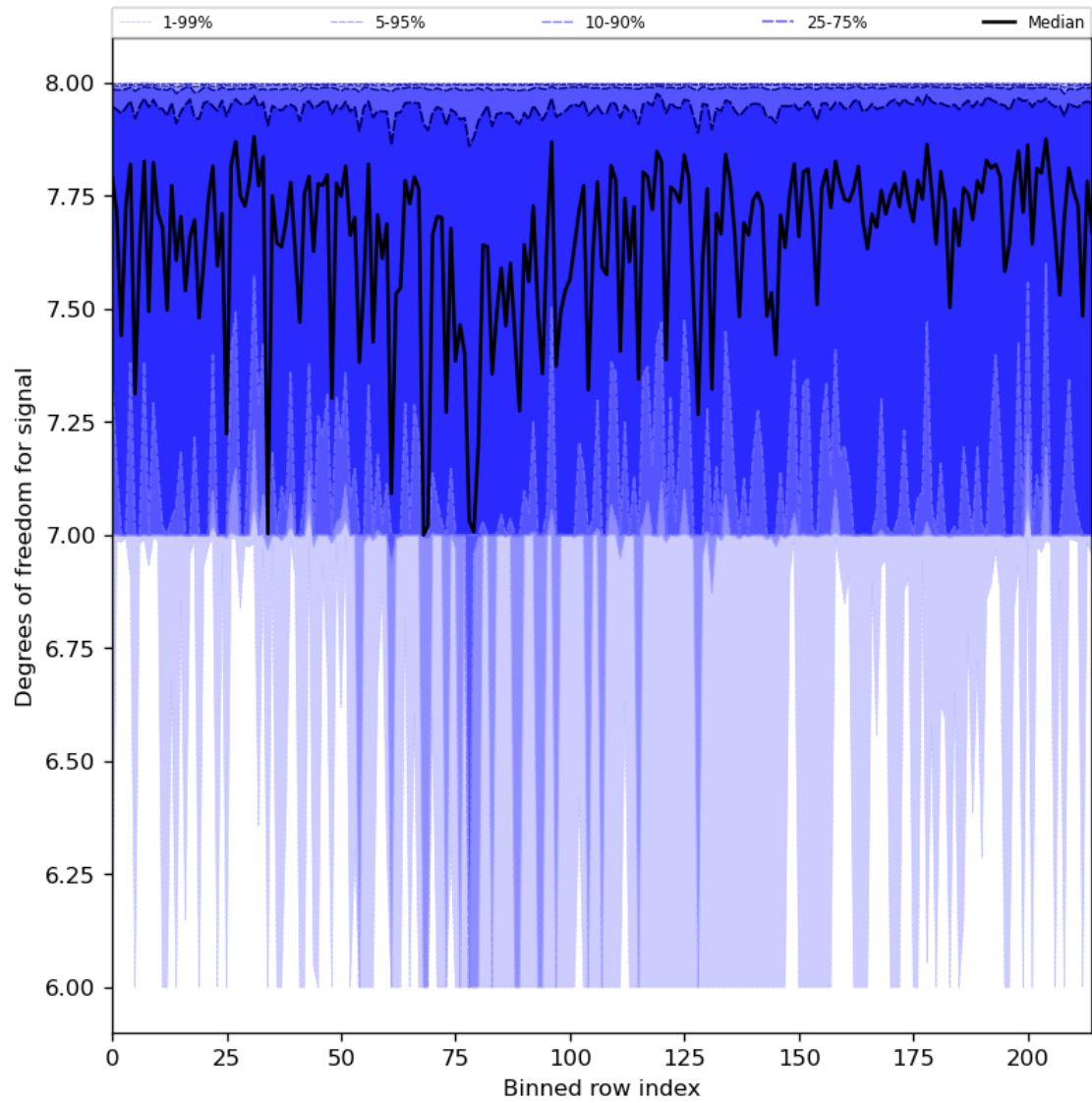
Figure 31: Along track statistics of “Degrees of freedom for signal” for 2024-06-25 to 2024-06-27
