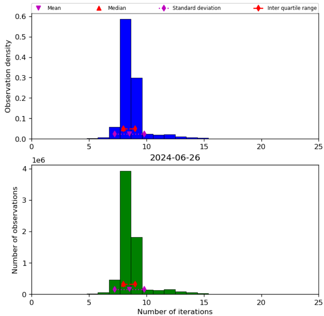
Figure 24: Histogram of “Number of iterations” for 2024-06-25 to 2024-06-27
