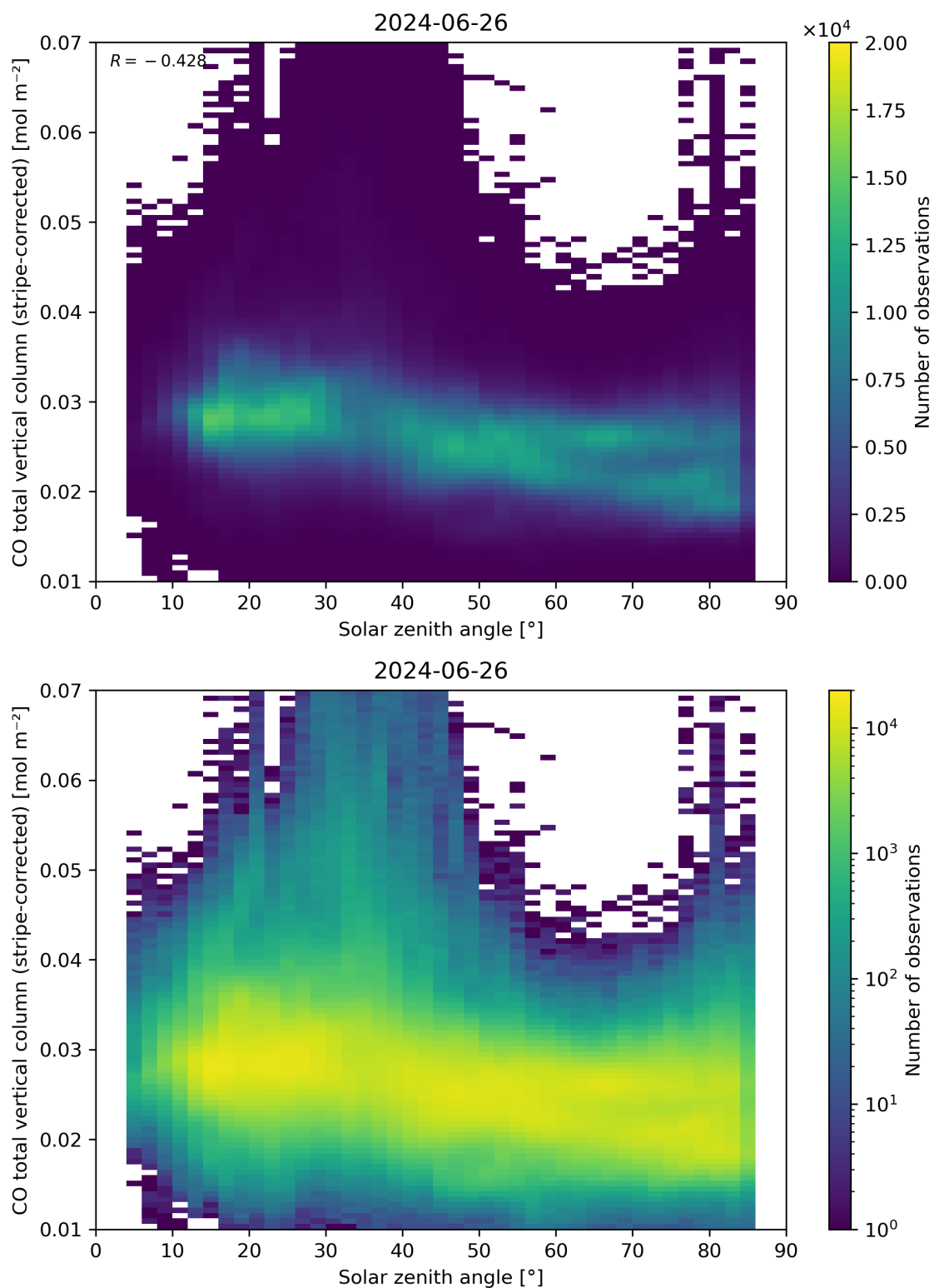
Figure 62: Scatter density plot of “Solar zenith angle” against “CO total vertical column (stripe-corrected)” for 2024-06-25 to 2024-06-27.
