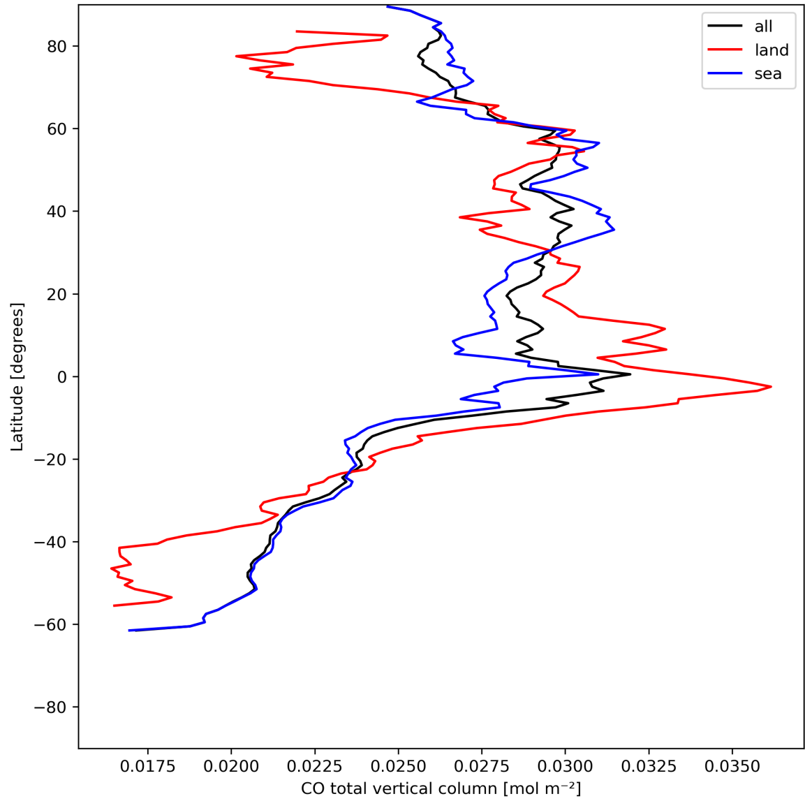
Figure 10: Zonal average of “CO total vertical column” for 2024-06-25 to 2024-06-27.
