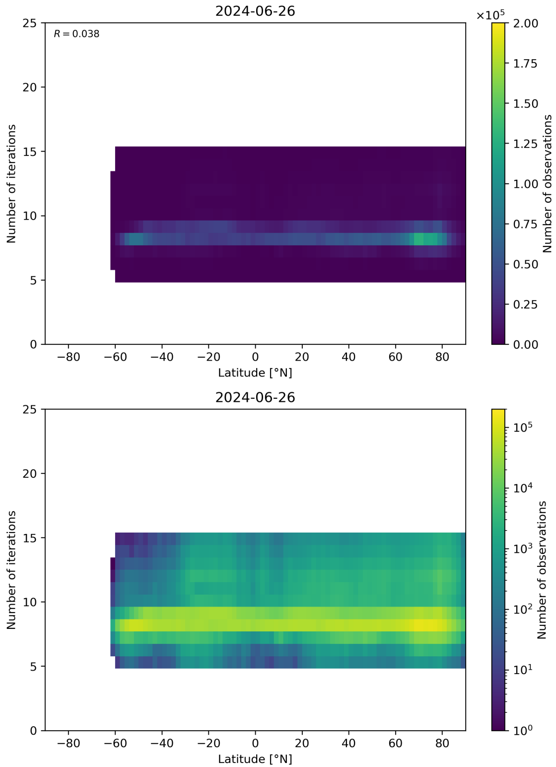
Figure 56: Scatter density plot of “Latitude” against “Number of iterations” for 2024-06-25 to 2024-06-27.
