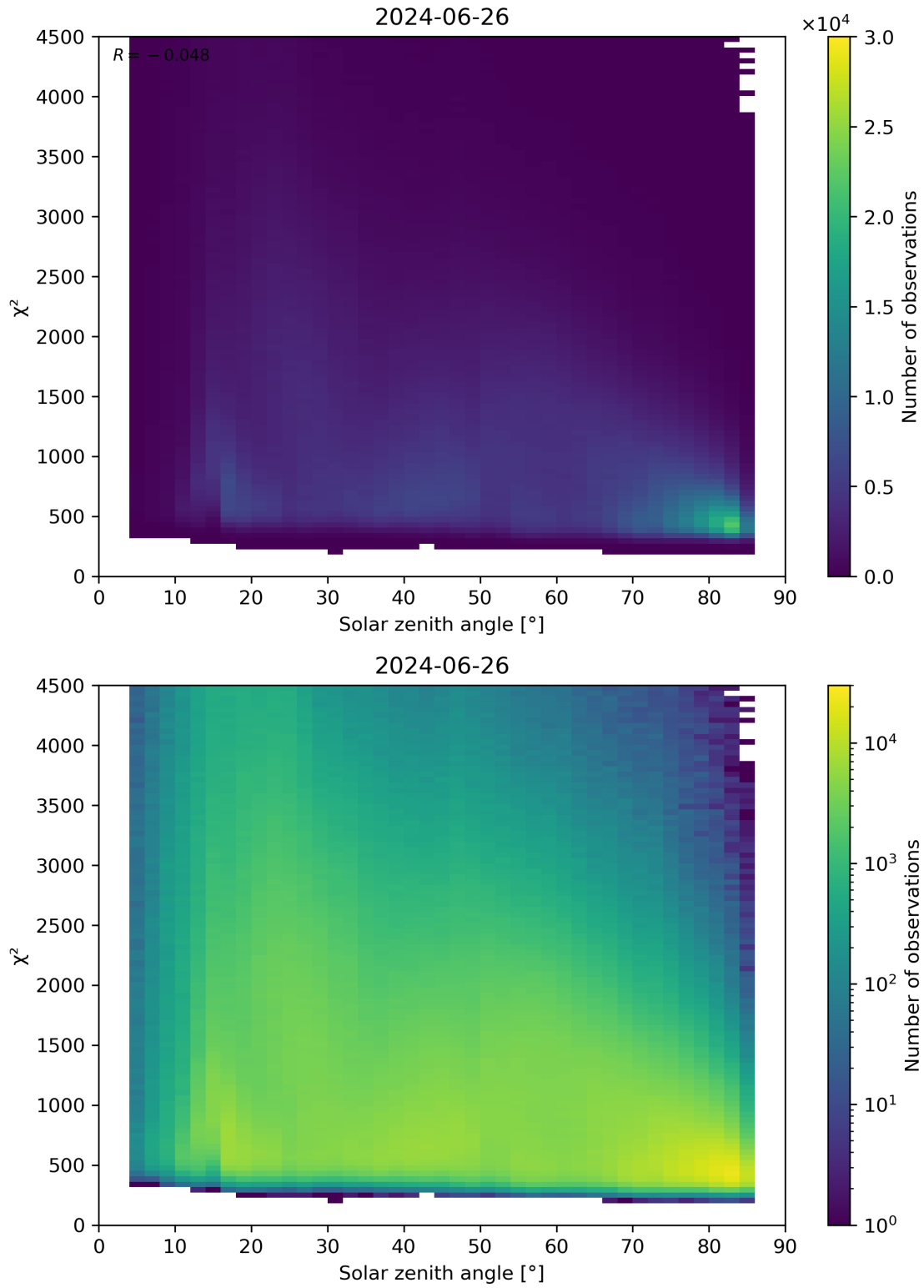
Figure 64: Scatter density plot of “Solar zenith angle” against “ \chi^2 ” for 2024-06-25 to 2024-06-27.
