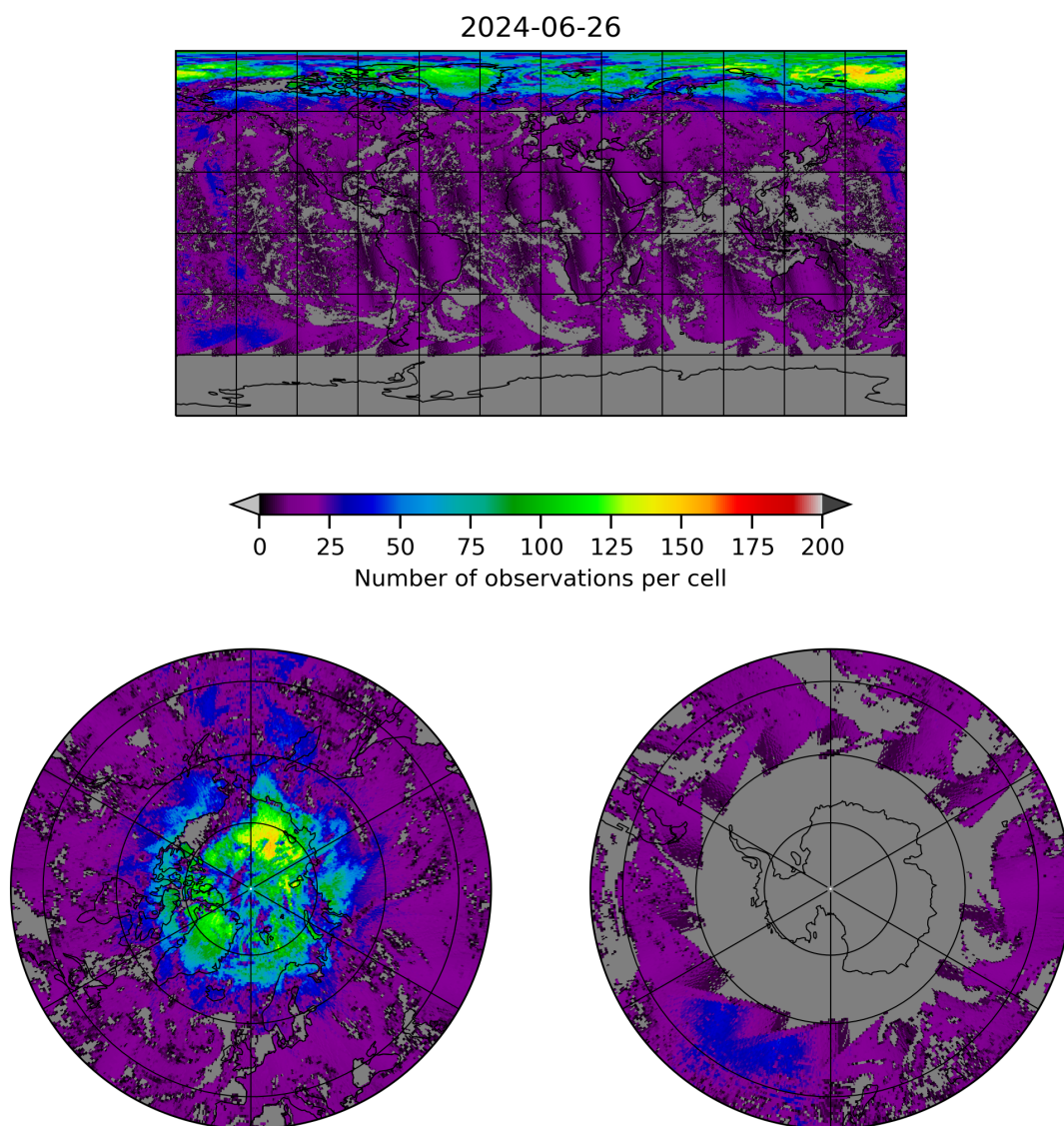
Figure 8: Map of the number of observations for 2024-06-25 to 2024-06-27
