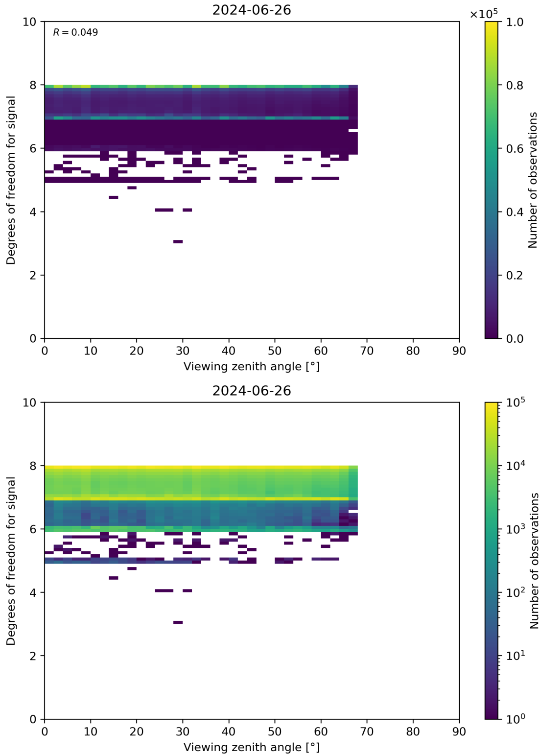
Figure 73: Scatter density plot of “Viewing zenith angle” against “Degrees of freedom for signal” for 2024-06-25 to 2024-06-27.
