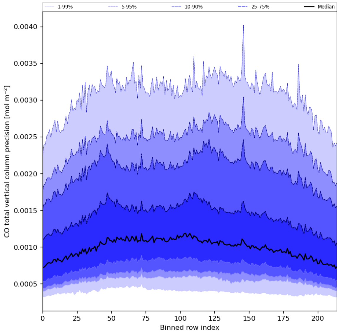
Figure 28: Along track statistics of “CO total vertical column precision” for 2024-06-25 to 2024-06-27
