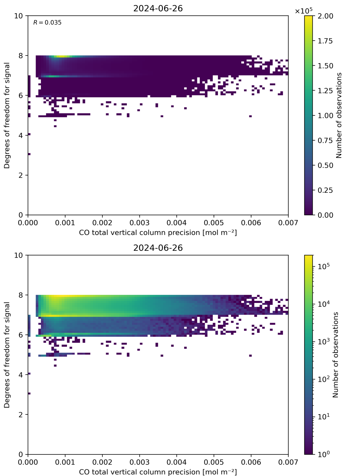
Figure 45: Scatter density plot of “CO total vertical column precision” against “Degrees of freedom for signal” for 2024-06-25 to 2024-06-27.
