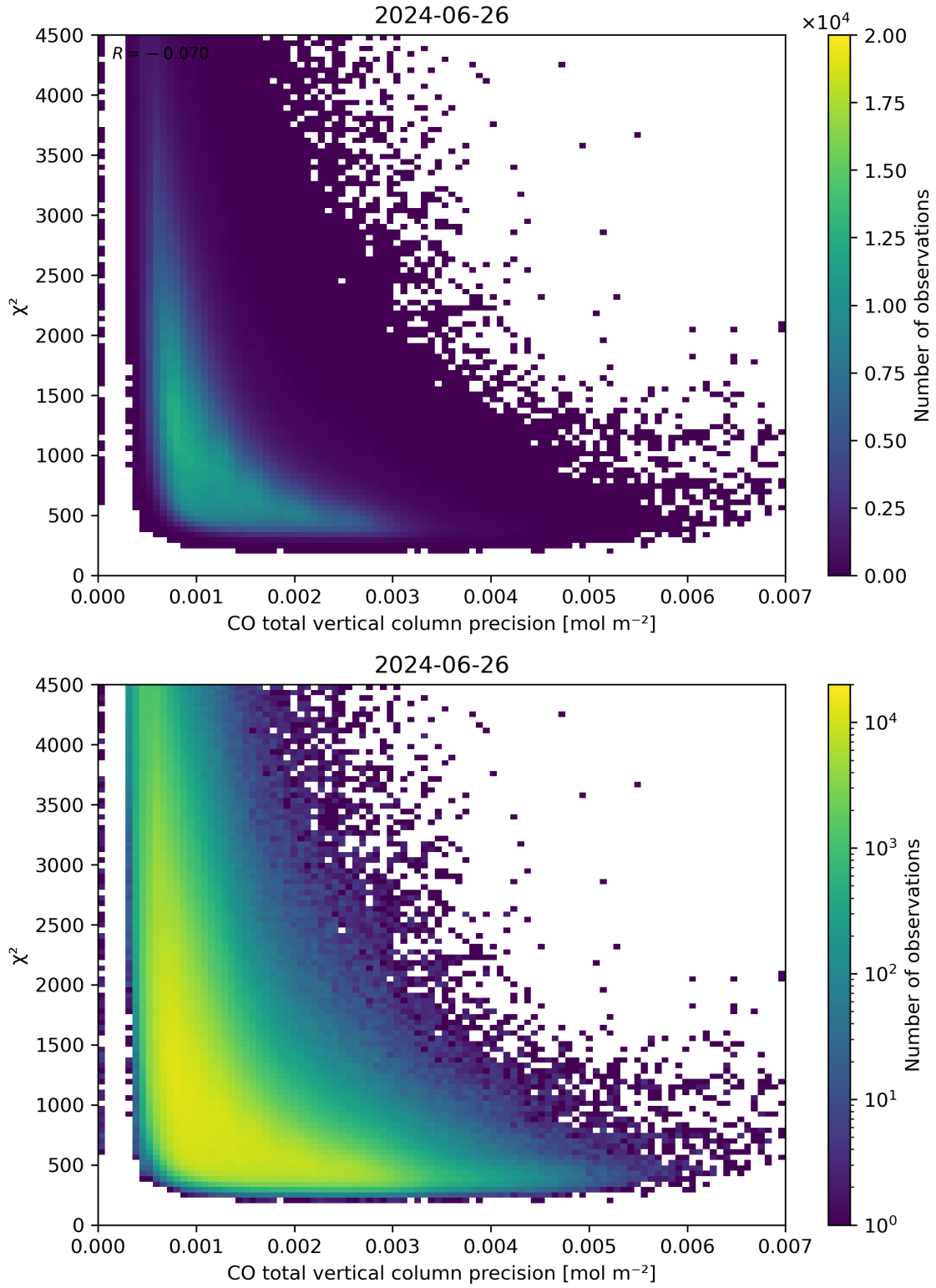
Figure 44: Scatter density plot of “CO total vertical column precision” against “ \chi^2 ” for 2024-06-25 to 2024-06-27.
