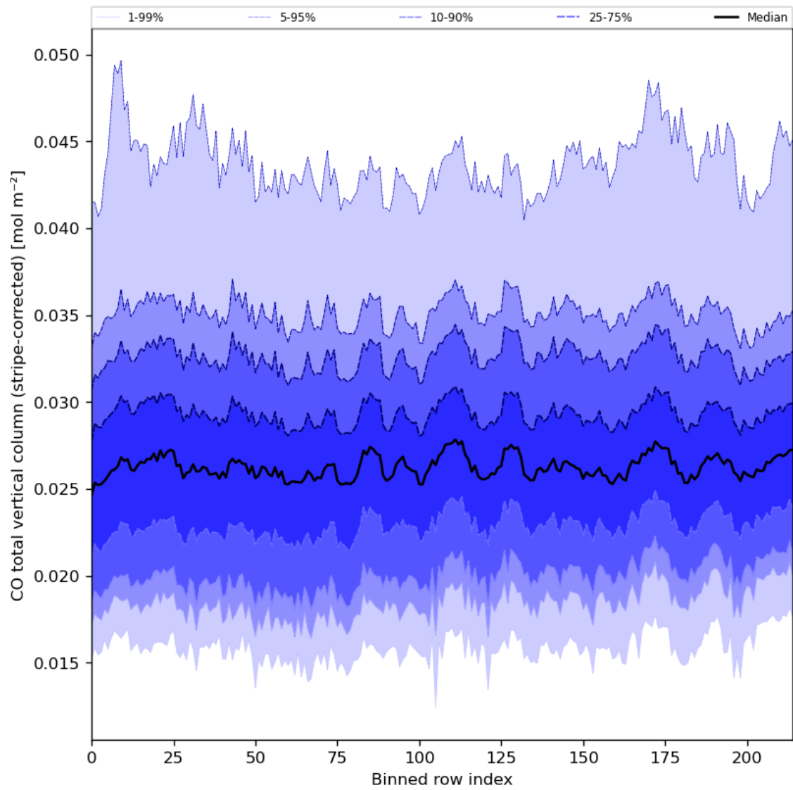
Figure 27: Along track statistics of “CO total vertical column (stripe-corrected)” for 2024-06-25 to 2024-06-27
