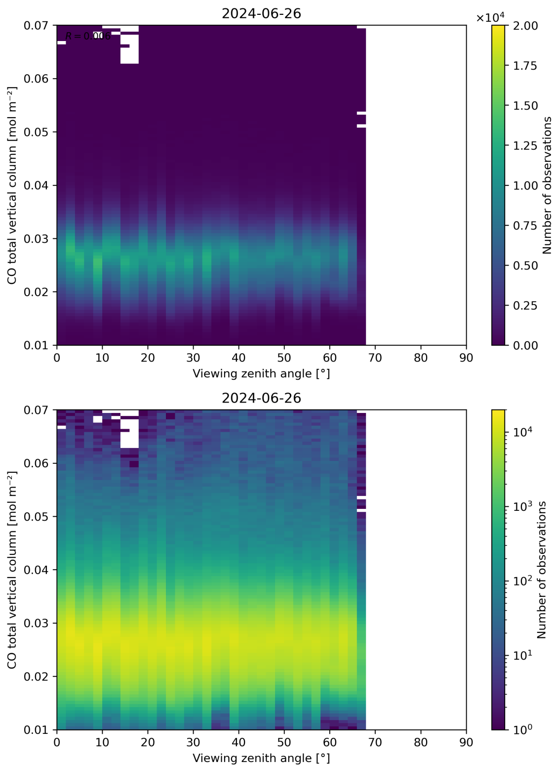
Figure 69: Scatter density plot of “Viewing zenith angle” against “CO total vertical column” for 2024-06-25 to 2024-06-27.
