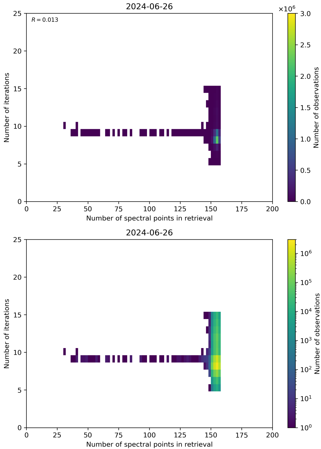
Figure 60: Scatter density plot of “Number of spectral points in retrieval” against “Number of iterations” for 2024-06-25 to 2024-06-27.
