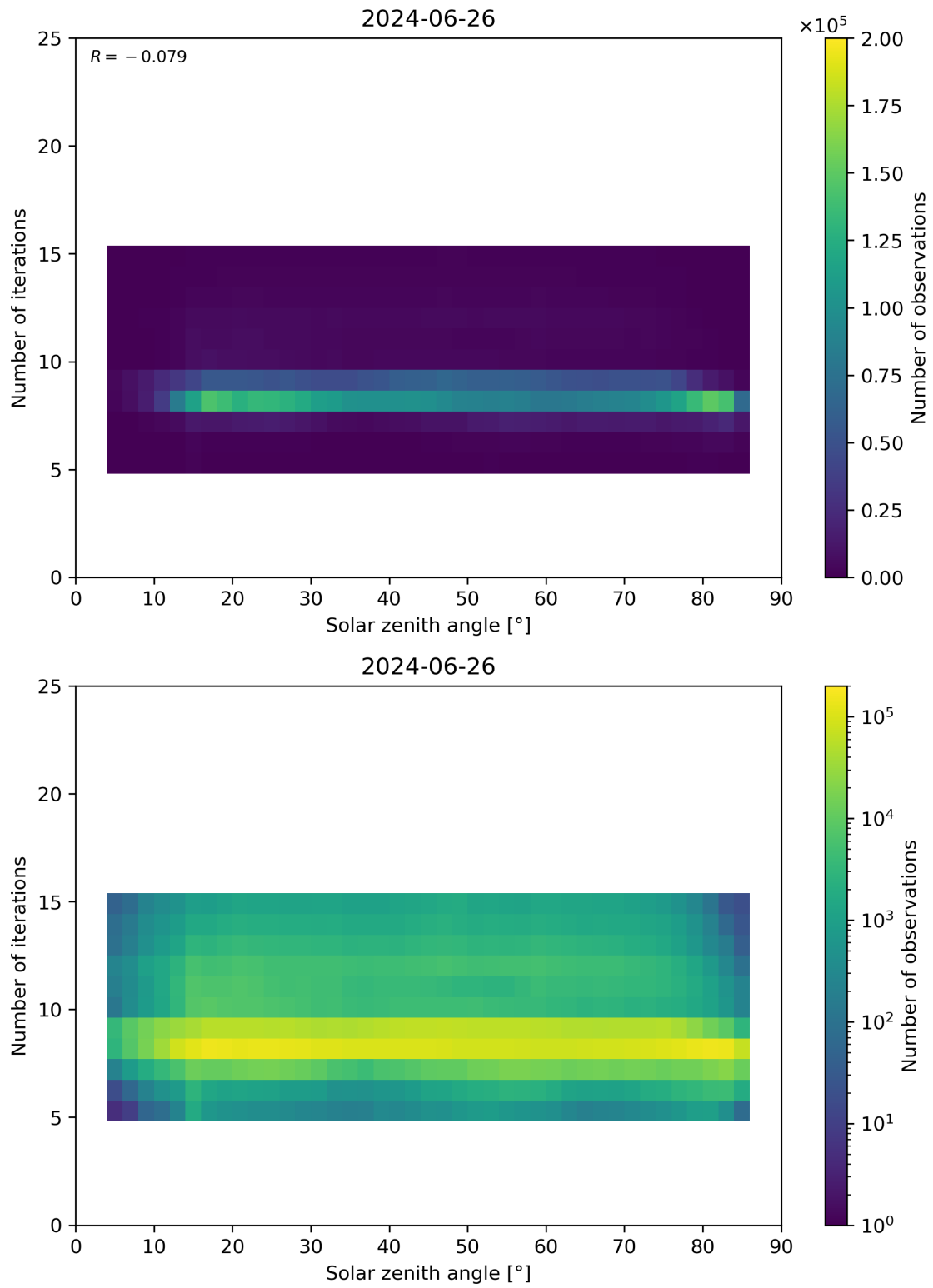
Figure 67: Scatter density plot of “Solar zenith angle” against “Number of iterations” for 2024-06-25 to 2024-06-27.
