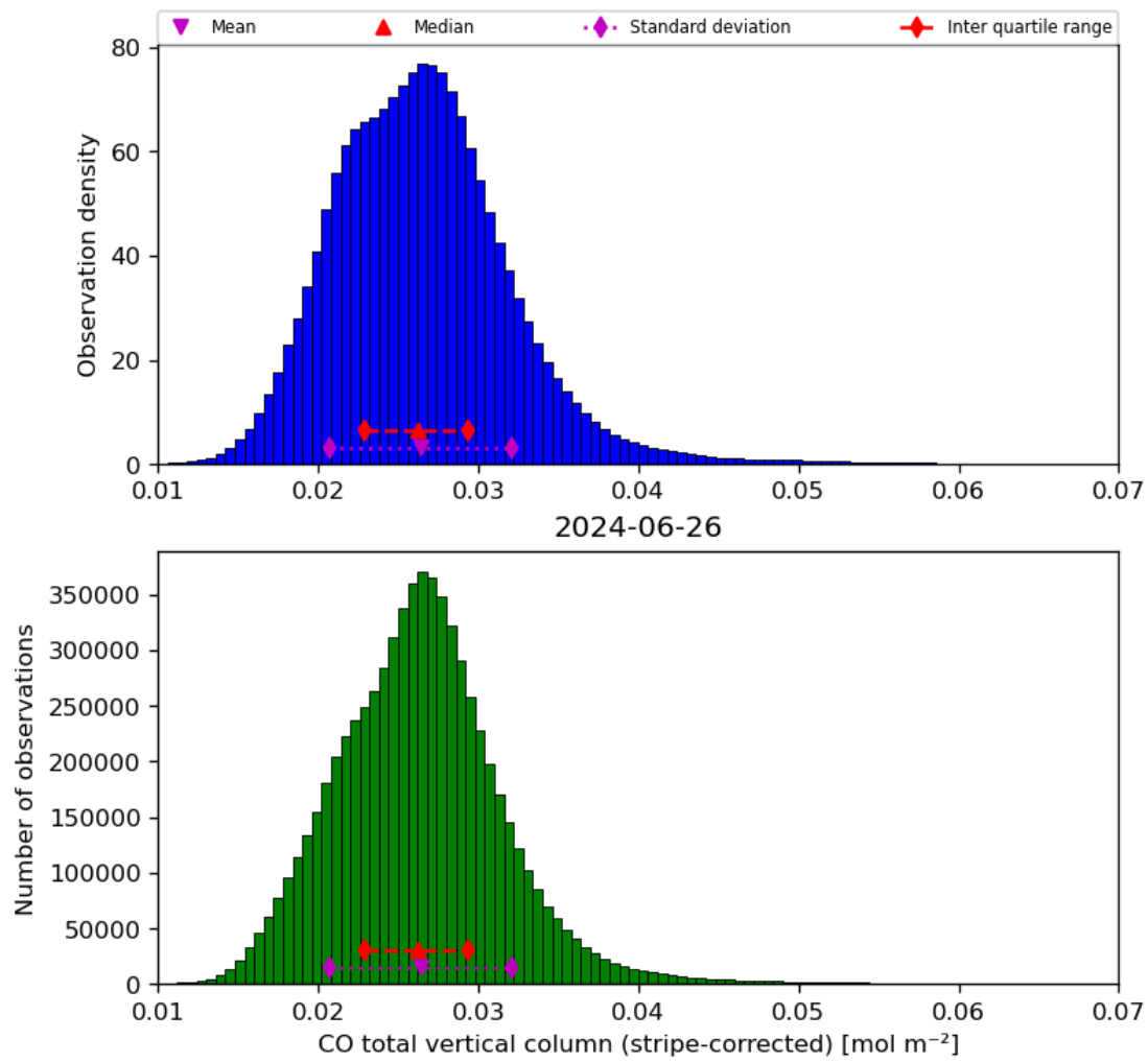
Figure 19: Histogram of “CO total vertical column (stripe-corrected)” for 2024-06-25 to 2024-06-27
