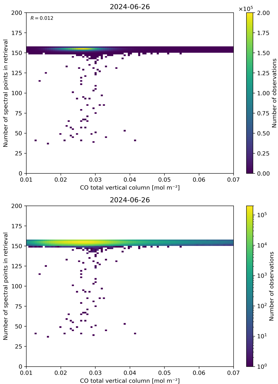
Figure 43: Scatter density plot of “CO total vertical column” against “Number of spectral points in retrieval” for 2024-06-25 to 2024-06-27.
