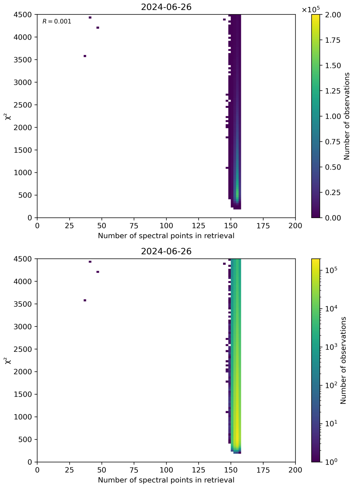
Figure 58: Scatter density plot of “Number of spectral points in retrieval” against “ \chi^2 ” for 2024-06-25 to 2024-06-27.
