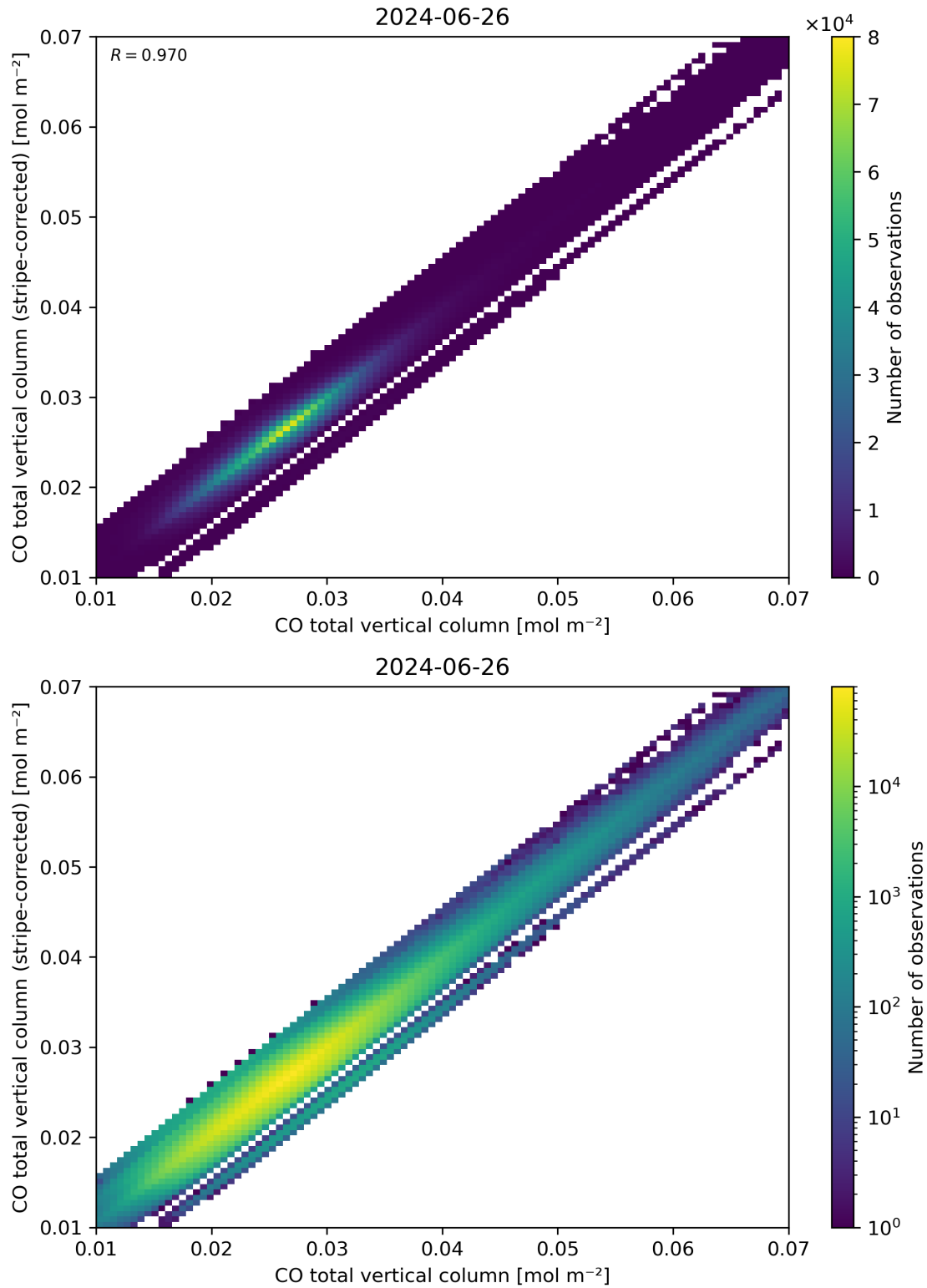
Figure 33: Scatter density plot of “CO total vertical column” against “CO total vertical column (stripe-corrected)” for 2024-06-25 to 2024-06-27.
