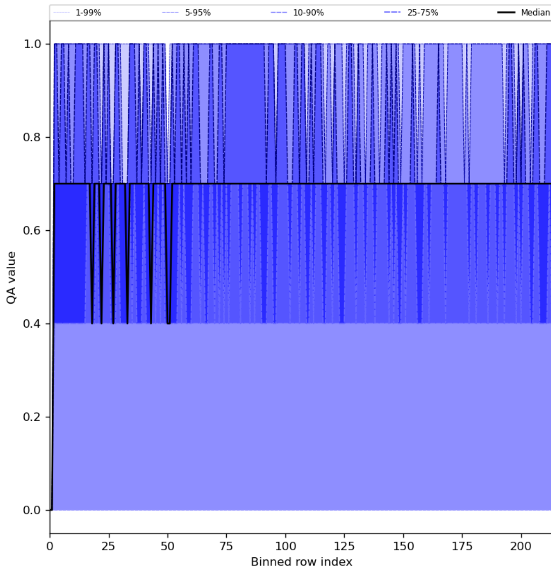
Figure 25: Along track statistics of “QA value” for 2024-06-25 to 2024-06-27
