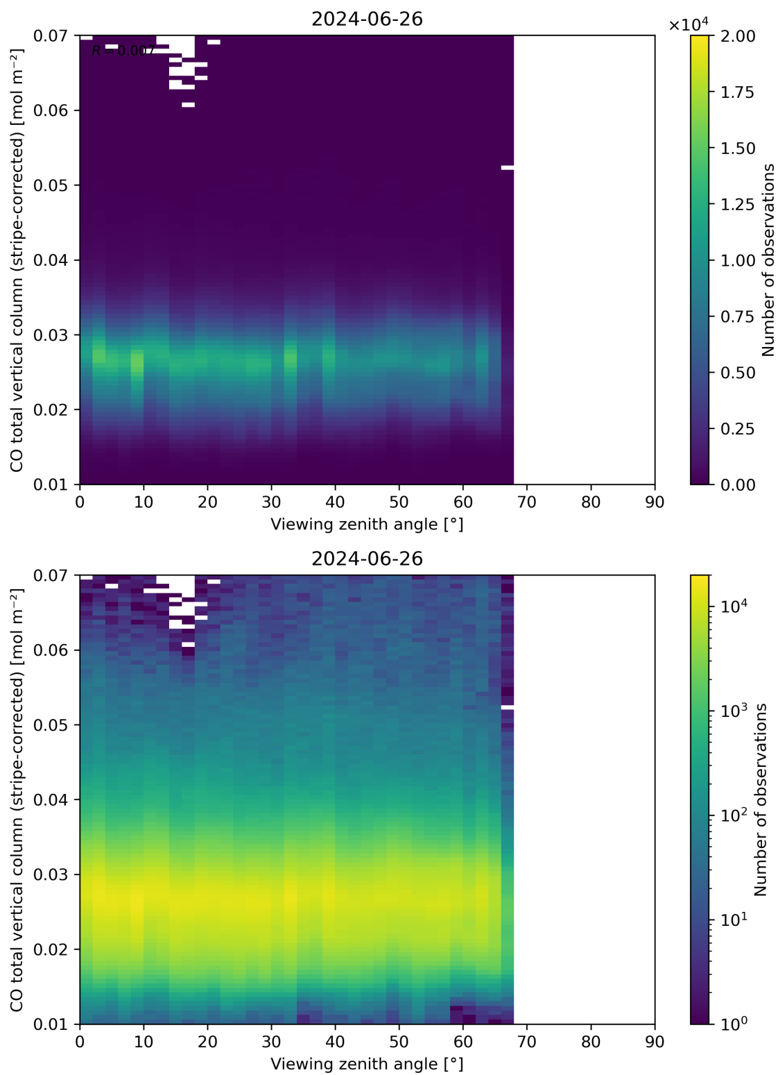
Figure 70: Scatter density plot of “Viewing zenith angle” against “CO total vertical column (stripe-corrected)” for 2024-06-25 to 2024-06-27.
