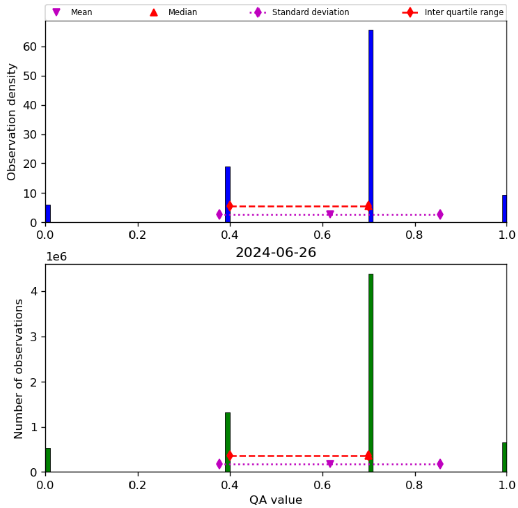
Figure 17: Histogram of “QA value” for 2024-06-25 to 2024-06-27
