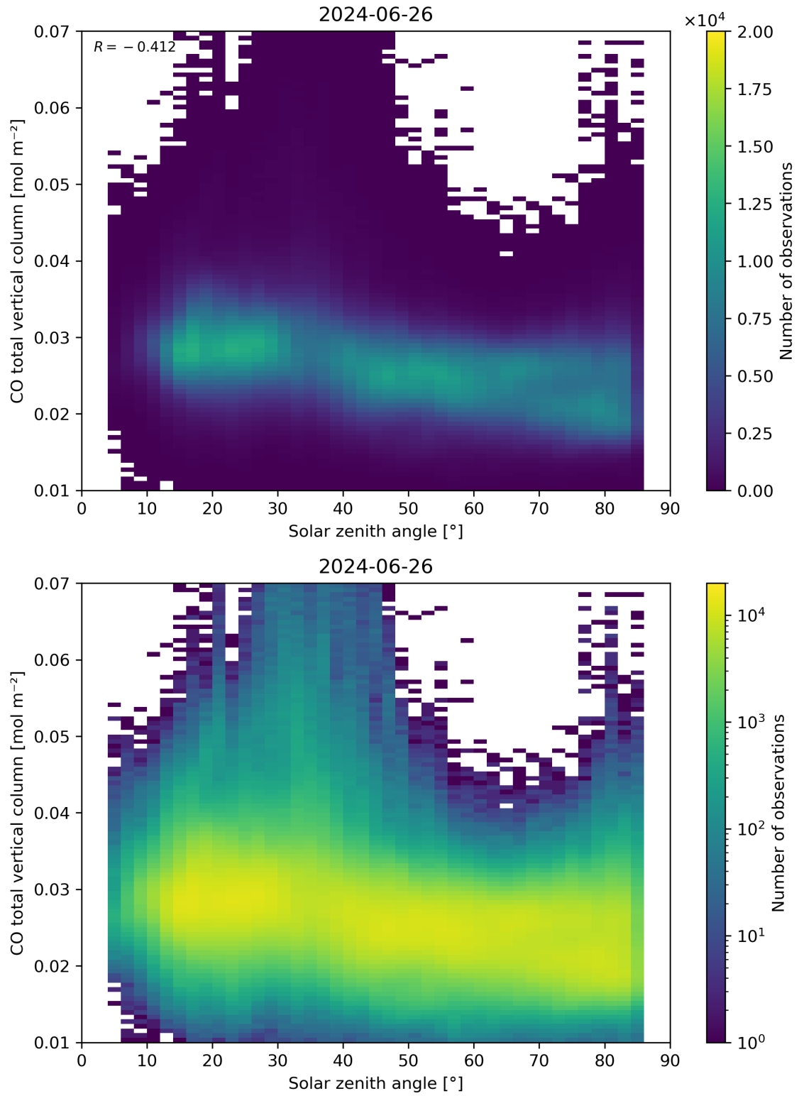
Figure 61: Scatter density plot of “Solar zenith angle” against “CO total vertical column” for 2024-06-25 to 2024-06-27.
