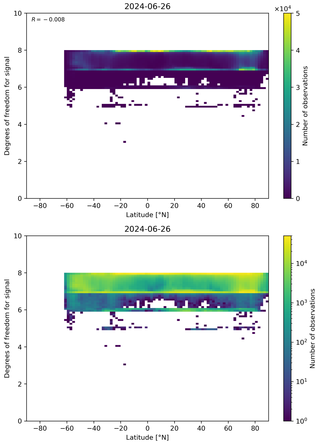
Figure 55: Scatter density plot of “Latitude” against “Degrees of freedom for signal” for 2024-06-25 to 2024-06-27.
