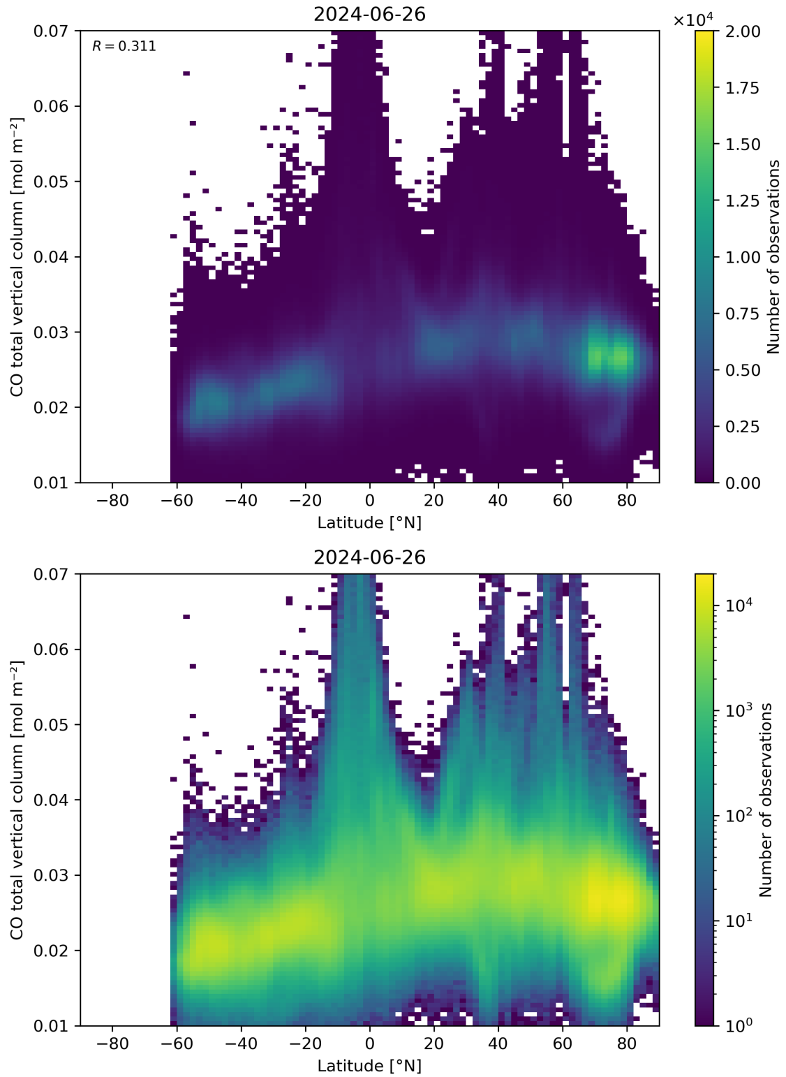
Figure 51: Scatter density plot of “Latitude” against “CO total vertical column” for 2024-06-25 to 2024-06-27.
