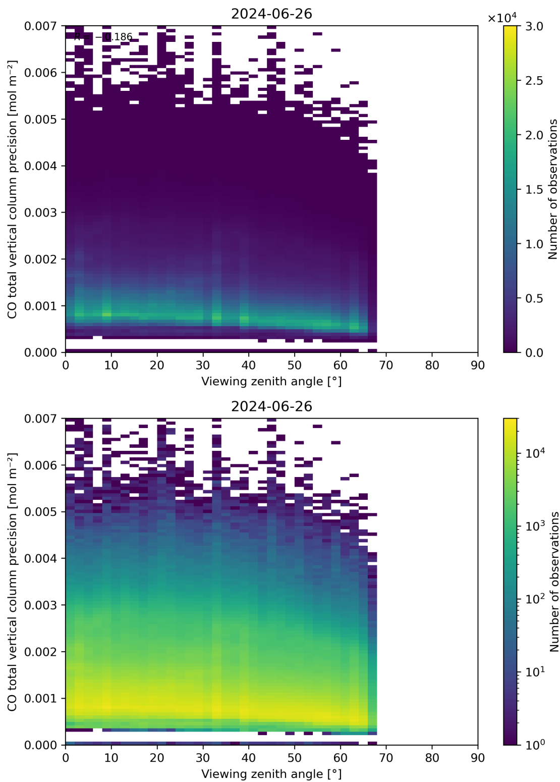
Figure 71: Scatter density plot of “Viewing zenith angle” against “CO total vertical column precision” for 2024-06-25 to 2024-06-27.
