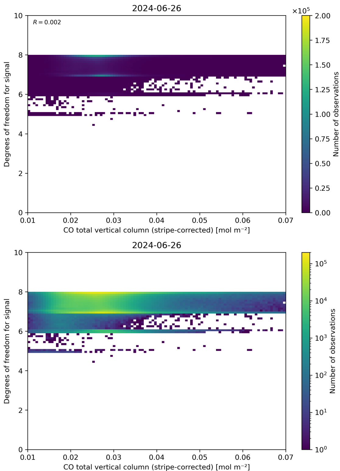
Figure 38: Scatter density plot of “CO total vertical column (stripe-corrected)” against “Degrees of freedom for signal” for 2024-06-25 to 2024-06-27.
