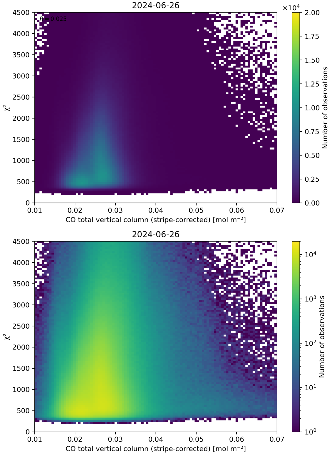
Figure 37: Scatter density plot of “CO total vertical column (stripe-corrected)” against “ \chi^2 ” for 2024-06-25 to 2024-06-27.
