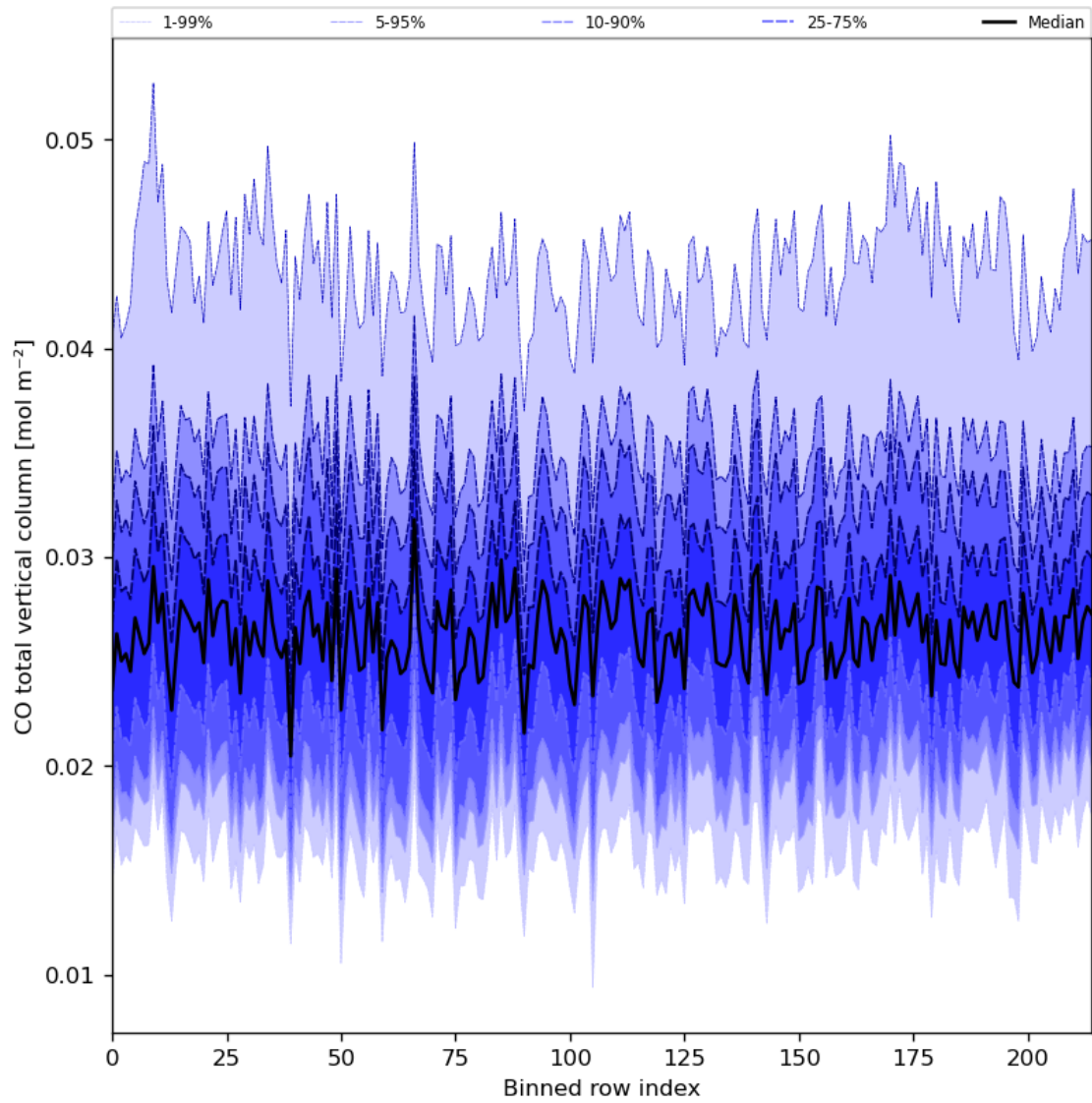
Figure 26: Along track statistics of “CO total vertical column” for 2024-06-25 to 2024-06-27
