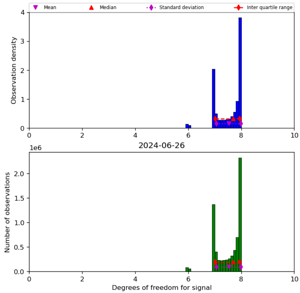
Figure 23: Histogram of “Degrees of freedom for signal” for 2024-06-25 to 2024-06-27
