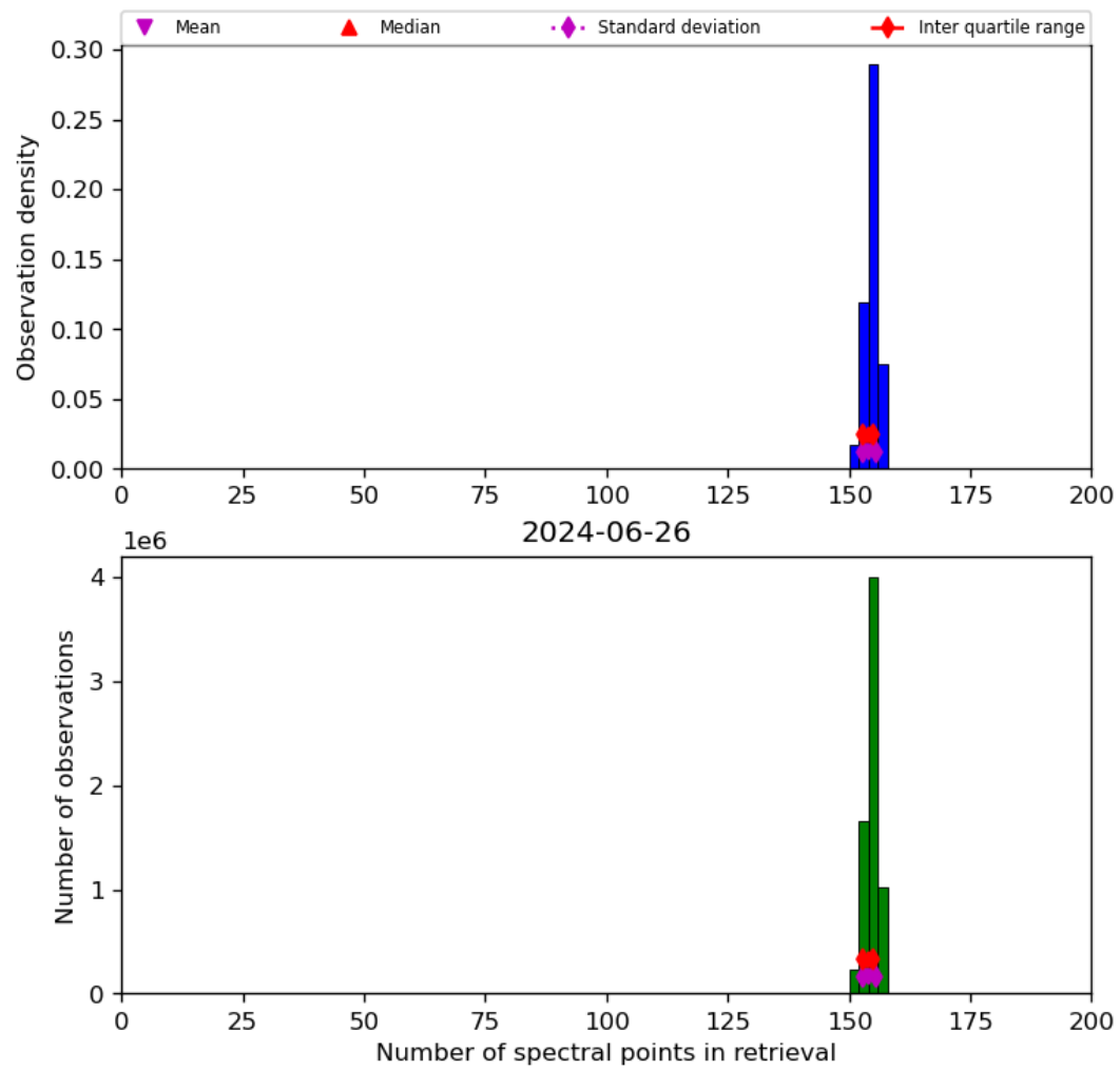
Figure 21: Histogram of “Number of spectral points in retrieval” for 2024-06-25 to 2024-06-27
