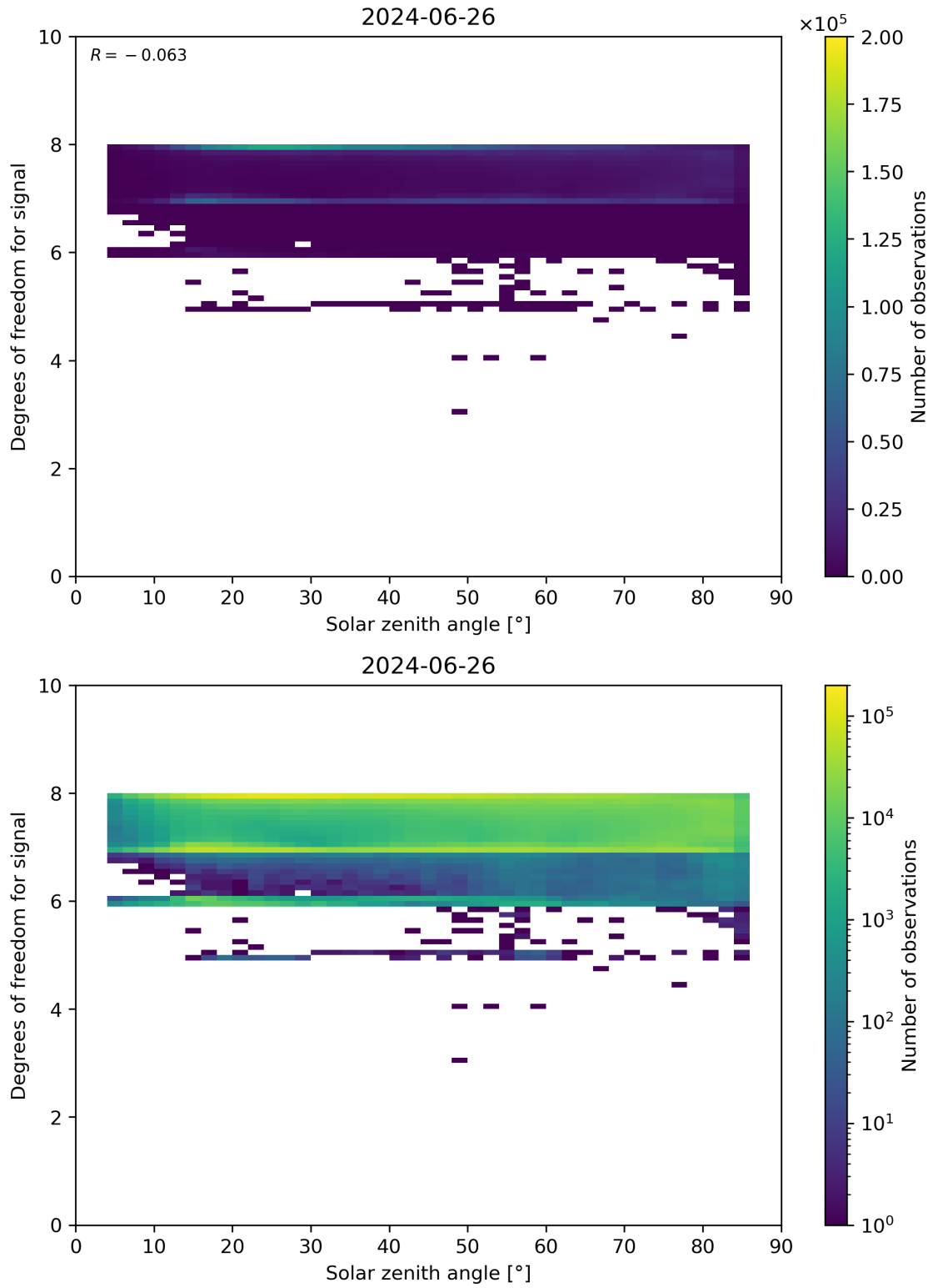
Figure 65: Scatter density plot of “Solar zenith angle” against “Degrees of freedom for signal” for 2024-06-25 to 2024-06-27.
