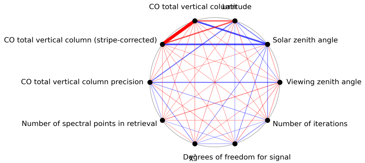
Figure 1: Map of correlation graph for 2024-06-25 to 2024-06-27.
