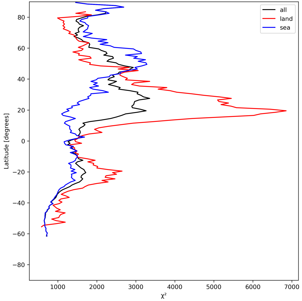
Figure 14: Zonal average of “ \chi^2 ” for 2024-06-25 to 2024-06-27.
