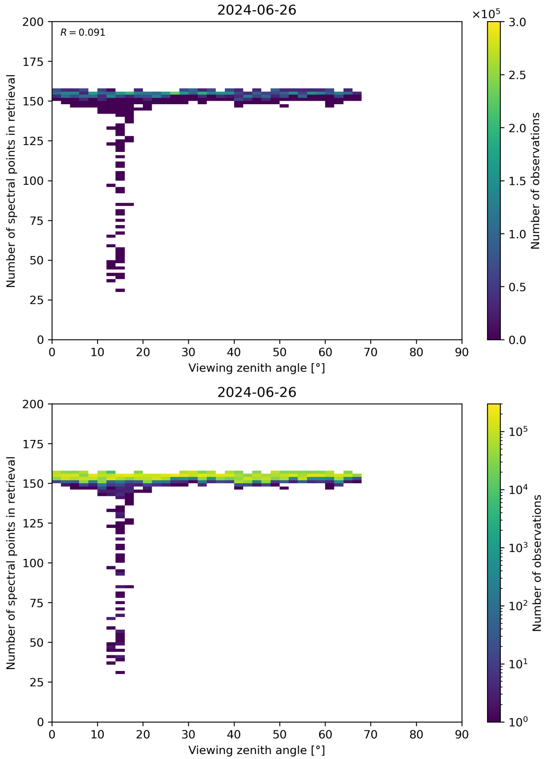
Figure 76: Scatter density plot of “Viewing zenith angle” against “Number of spectral points in retrieval” for 2024-06-25 to 2024-06-27.
