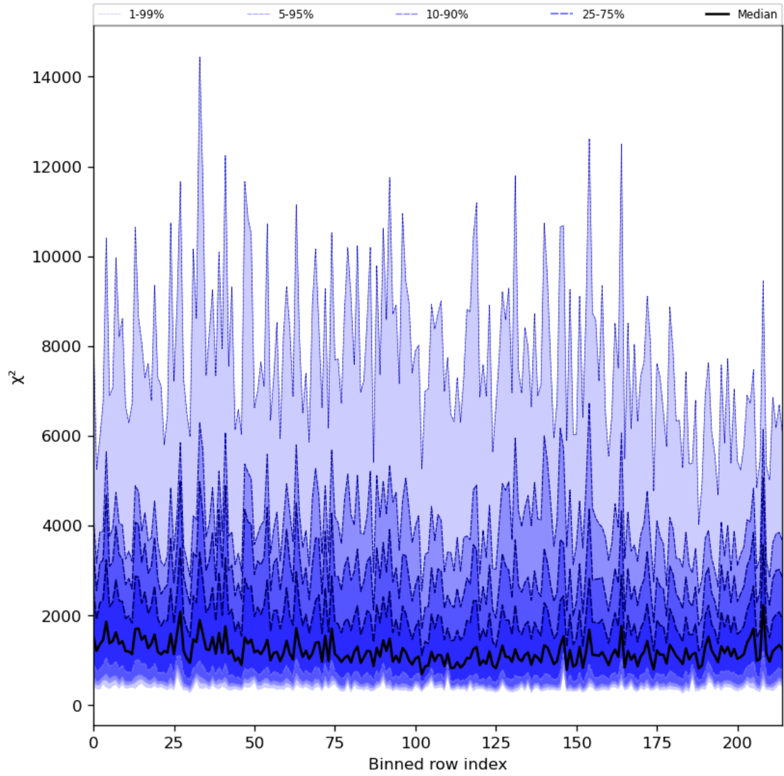
Figure 30: Along track statistics of “ \chi^2 ” for 2024-06-25 to 2024-06-27
