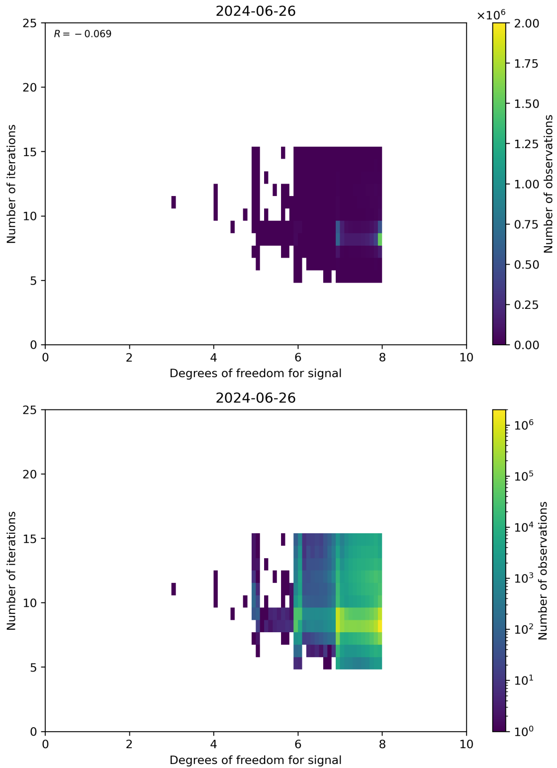
Figure 50: Scatter density plot of “Degrees of freedom for signal” against “Number of iterations” for 2024-06-25 to 2024-06-27.
