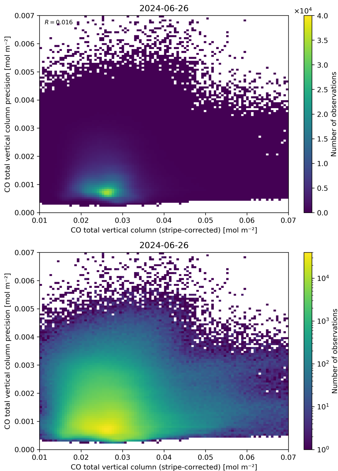
Figure 36: Scatter density plot of “CO total vertical column (stripe-corrected)” against “CO total vertical column precision” for 2024-06-25 to 2024-06-27.
