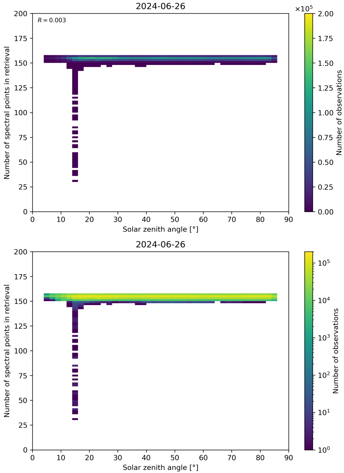
Figure 68: Scatter density plot of “Solar zenith angle” against “Number of spectral points in retrieval” for 2024-06-25 to 2024-06-27.
