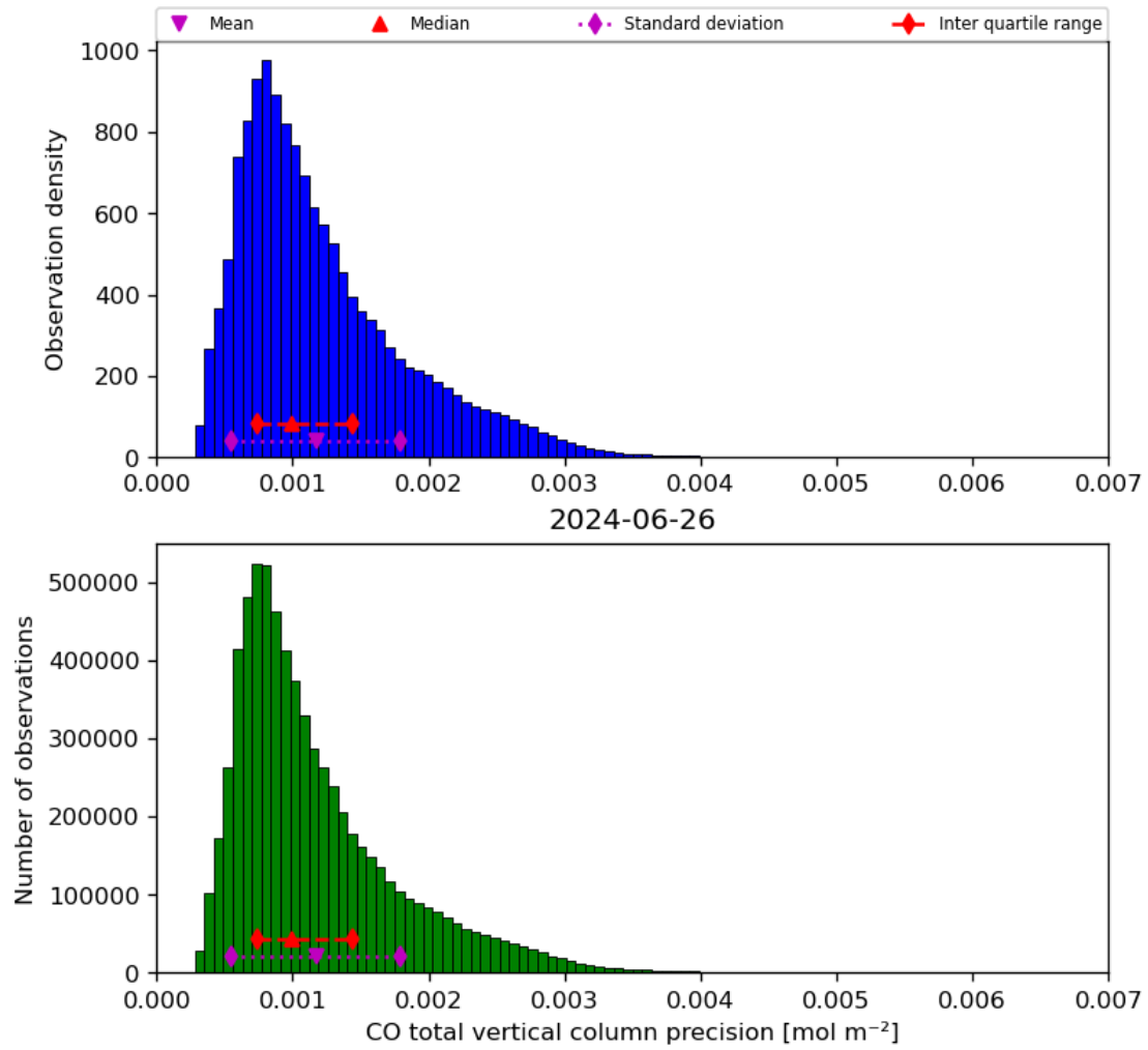
Figure 20: Histogram of “CO total vertical column precision” for 2024-06-25 to 2024-06-27
