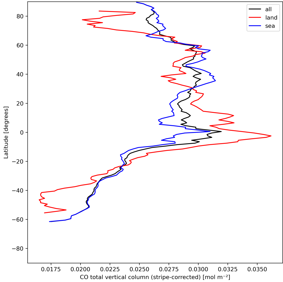
Figure 11: Zonal average of “CO total vertical column (stripe-corrected)” for 2024-06-25 to 2024-06-27.
