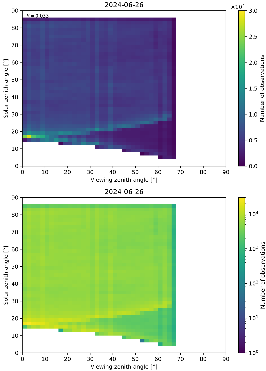
Figure 77: Scatter density plot of “Viewing zenith angle” against “Solar zenith angle” for 2024-06-25 to 2024-06-27.
