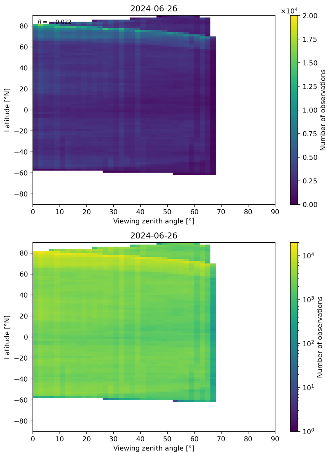
Figure 74: Scatter density plot of “Viewing zenith angle” against “Latitude” for 2024-06-25 to 2024-06-27.
