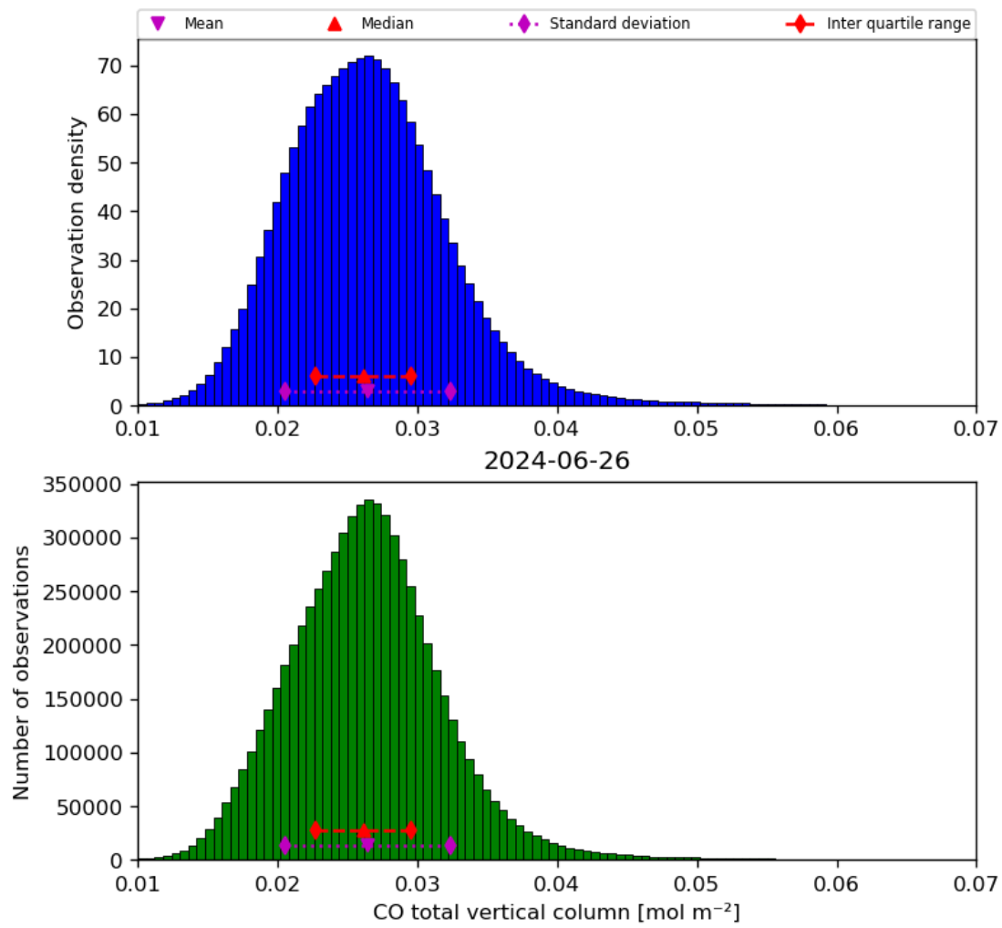
Figure 18: Histogram of “CO total vertical column” for 2024-06-25 to 2024-06-27
