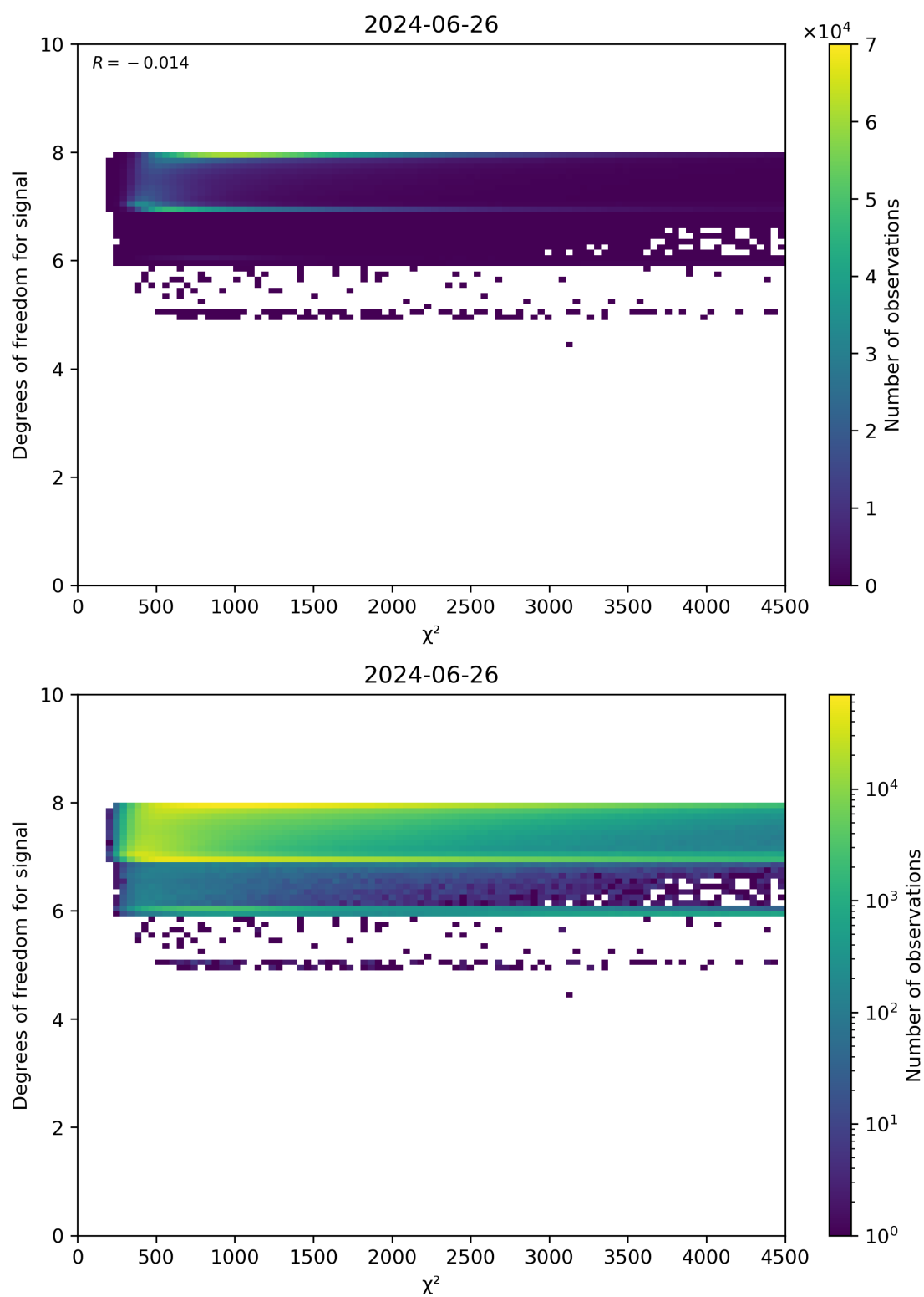
Figure 48: Scatter density plot of “ \chi^2 ” against “Degrees of freedom for signal” for 2024-06-25 to 2024-06-27.
