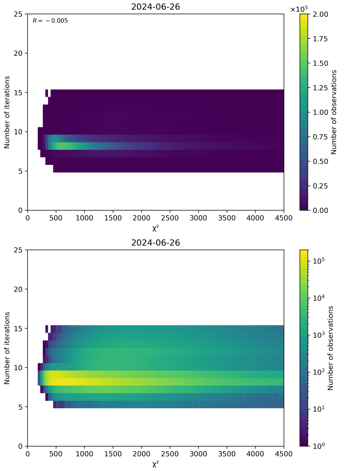
Figure 49: Scatter density plot of “ \chi^2 ” against “Number of iterations” for 2024-06-25 to 2024-06-27.
