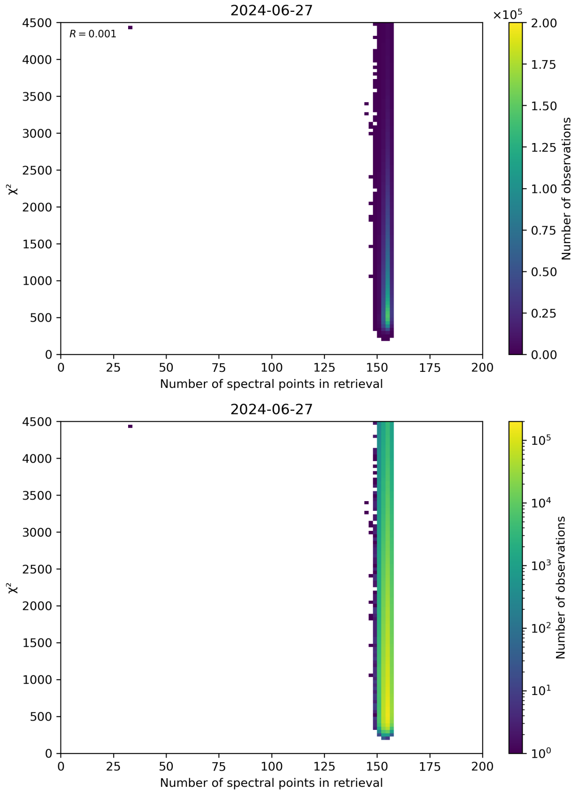
Figure 58: Scatter density plot of “Number of spectral points in retrieval” against “ \chi^2 ” for 2024-06-26 to 2024-06-28.
