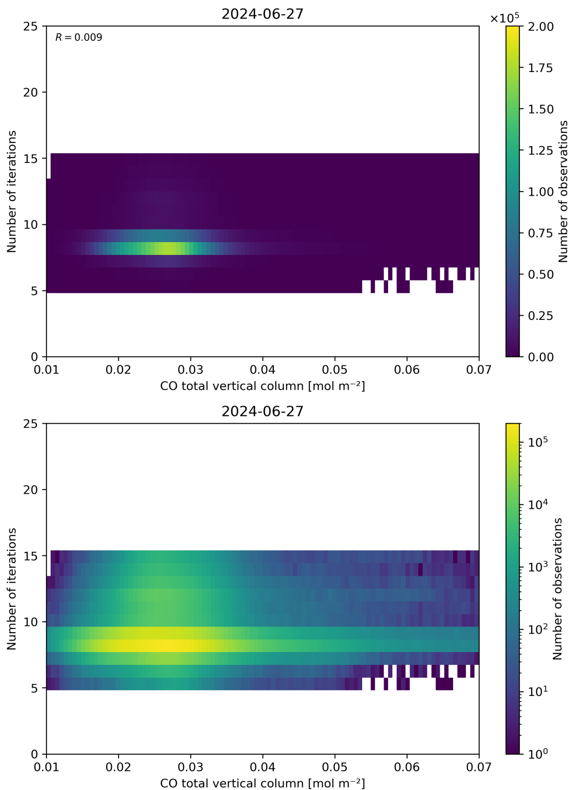
Figure 42: Scatter density plot of “CO total vertical column” against “Number of iterations” for 2024-06-26 to 2024-06-28.
