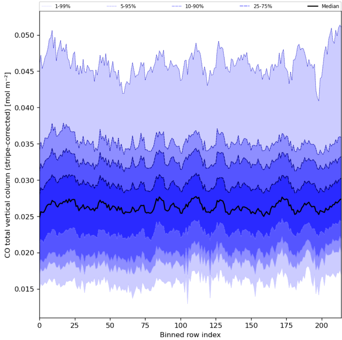
Figure 27: Along track statistics of “CO total vertical column (stripe-corrected)” for 2024-06-26 to 2024-06-28
