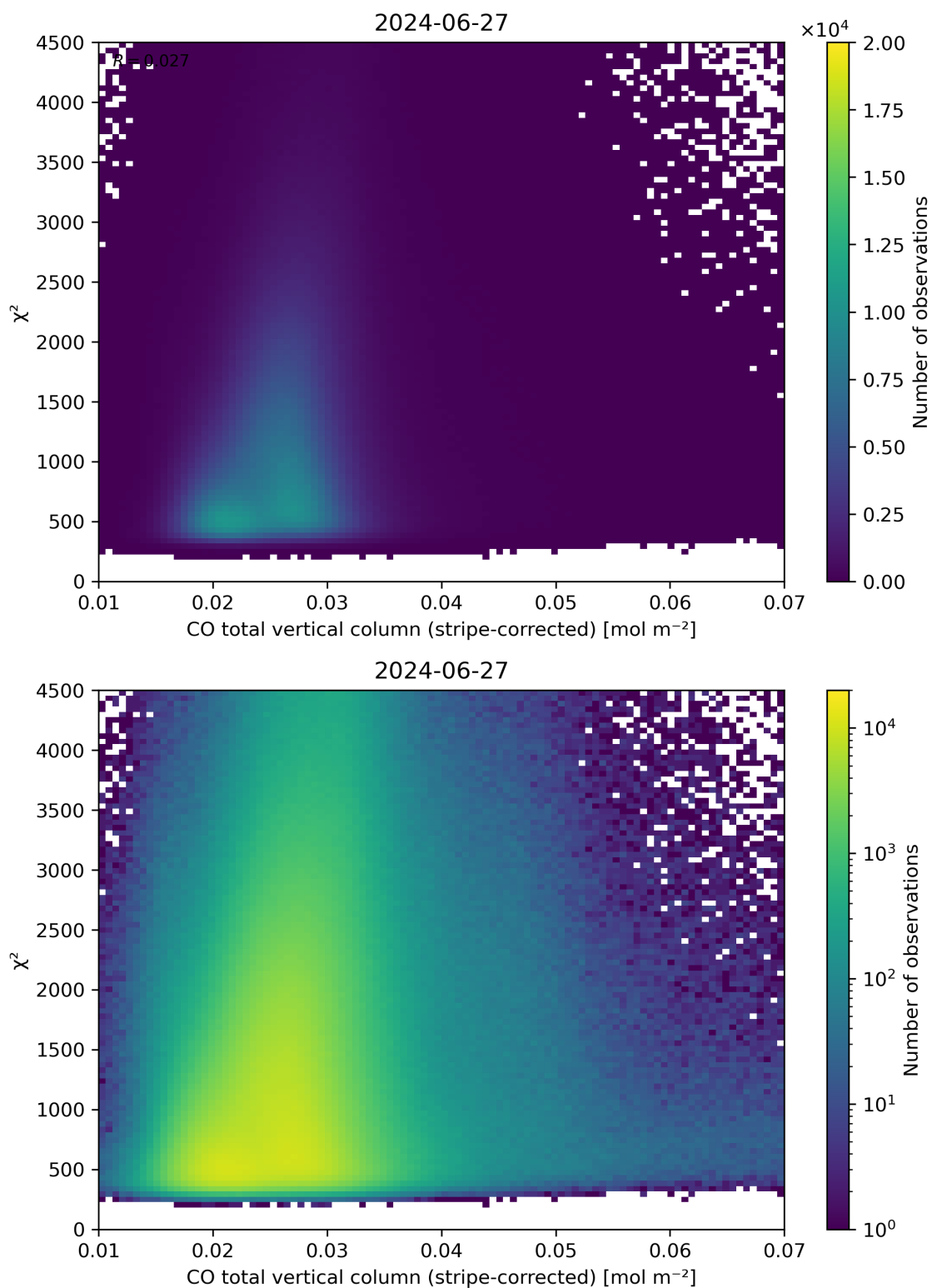
Figure 37: Scatter density plot of “CO total vertical column (stripe-corrected)” against “ \chi^2 ” for 2024-06-26 to 2024-06-28.
