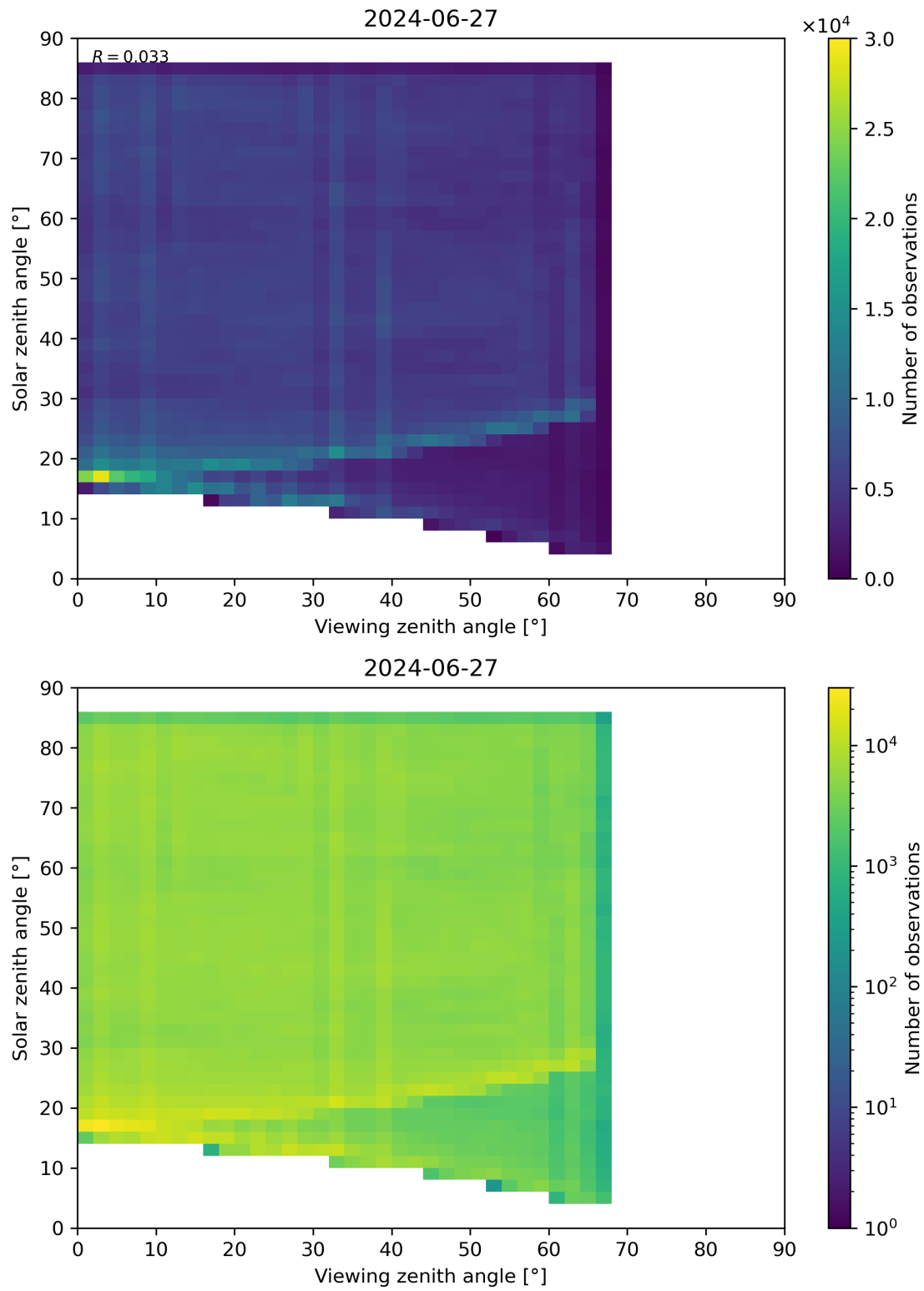
Figure 77: Scatter density plot of “Viewing zenith angle” against “Solar zenith angle” for 2024-06-26 to 2024-06-28.
