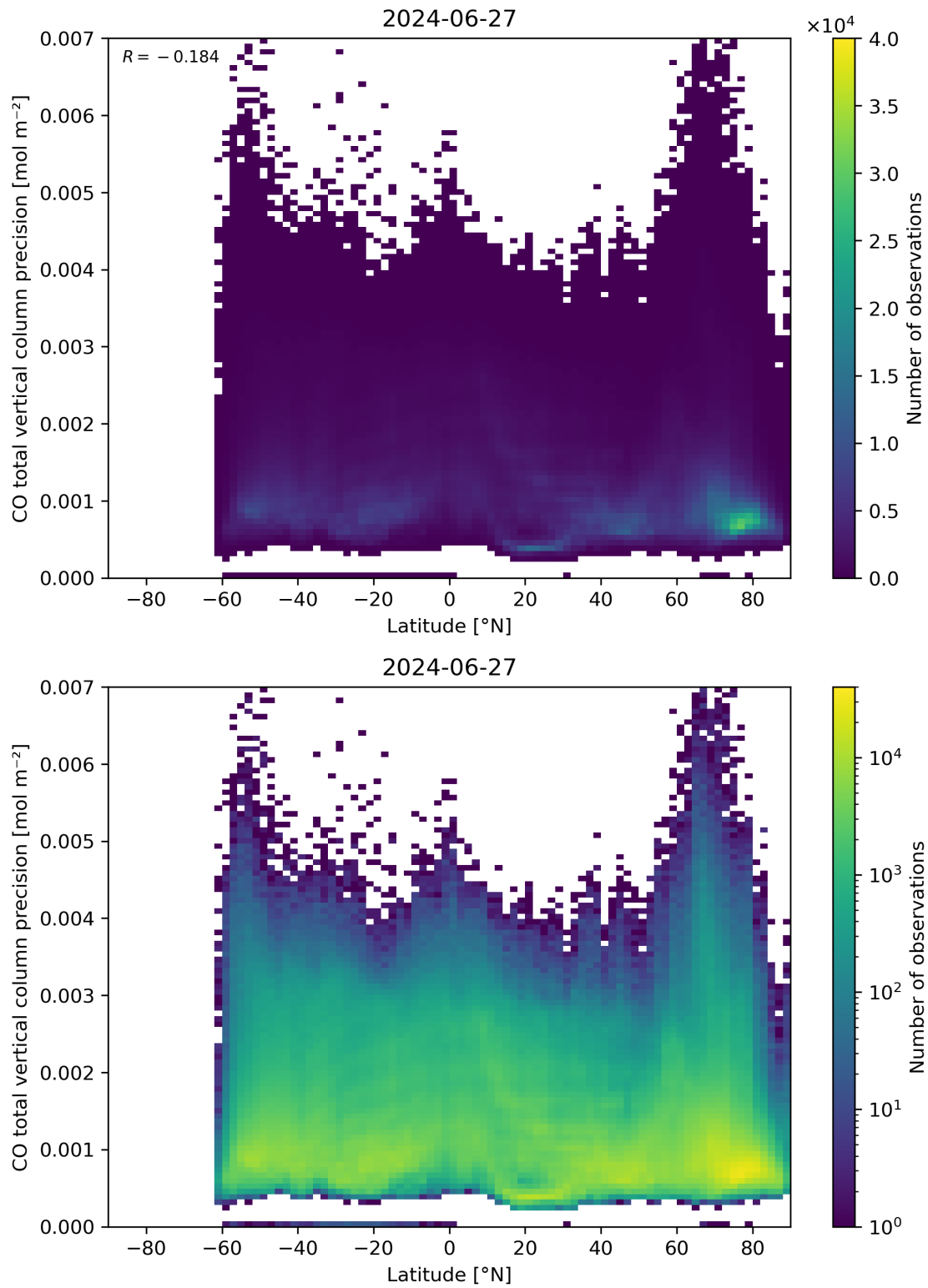
Figure 53: Scatter density plot of “Latitude” against “CO total vertical column precision” for 2024-06-26 to 2024-06-28.
