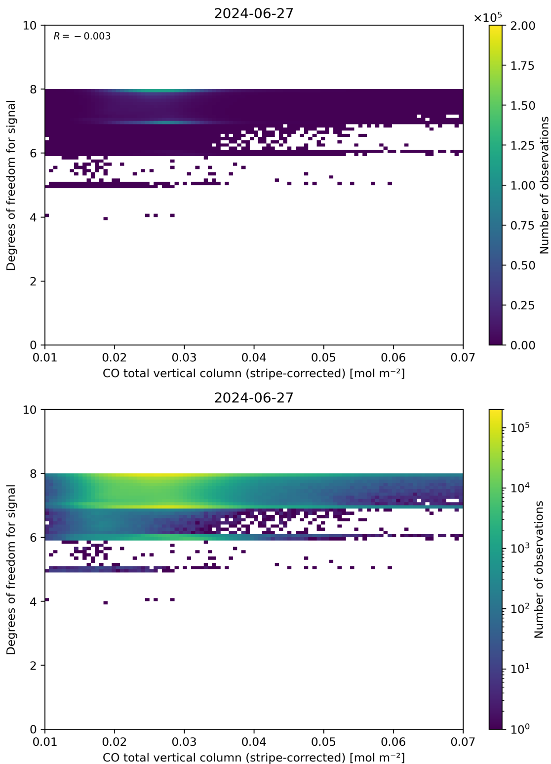
Figure 38: Scatter density plot of “CO total vertical column (stripe-corrected)” against “Degrees of freedom for signal” for 2024-06-26 to 2024-06-28.
