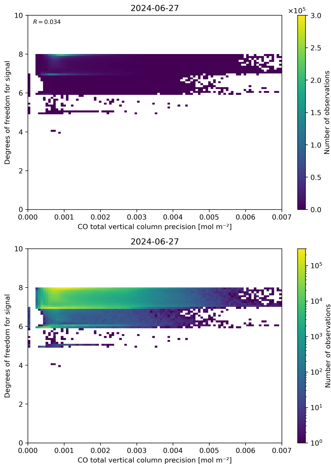
Figure 45: Scatter density plot of “CO total vertical column precision” against “Degrees of freedom for signal” for 2024-06-26 to 2024-06-28.
