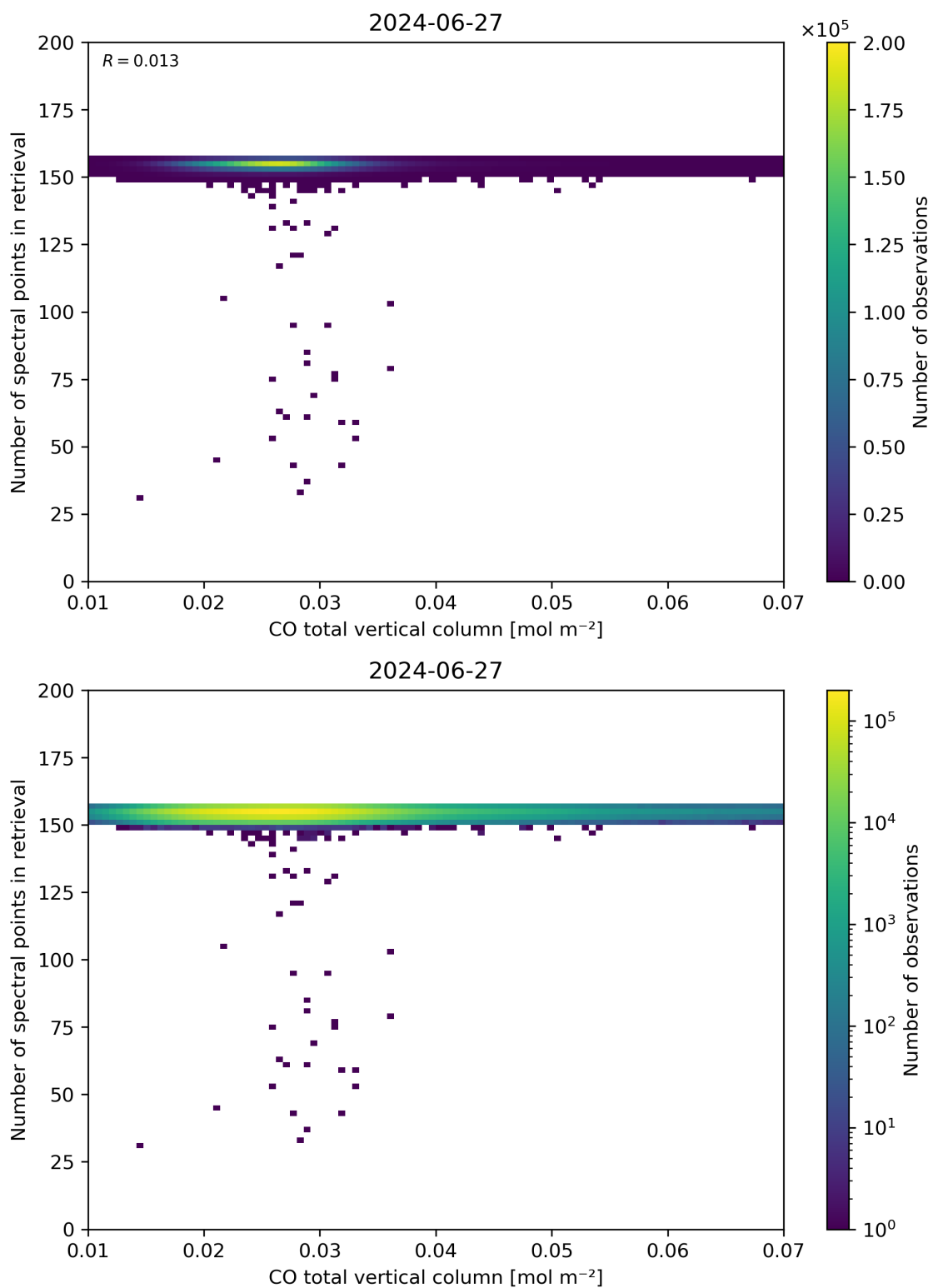
Figure 43: Scatter density plot of “CO total vertical column” against “Number of spectral points in retrieval” for 2024-06-26 to 2024-06-28.
