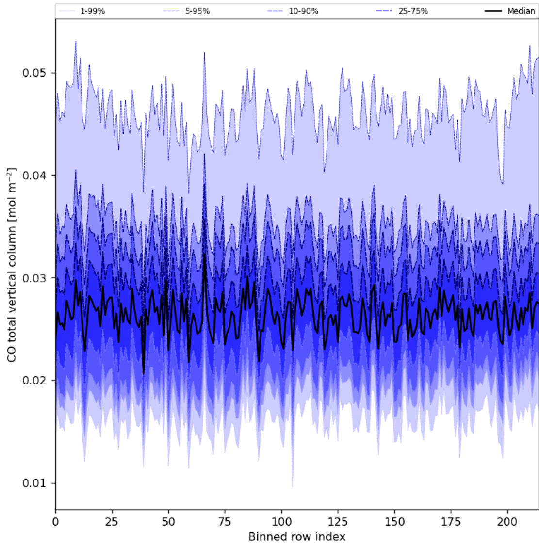
Figure 26: Along track statistics of “CO total vertical column” for 2024-06-26 to 2024-06-28
