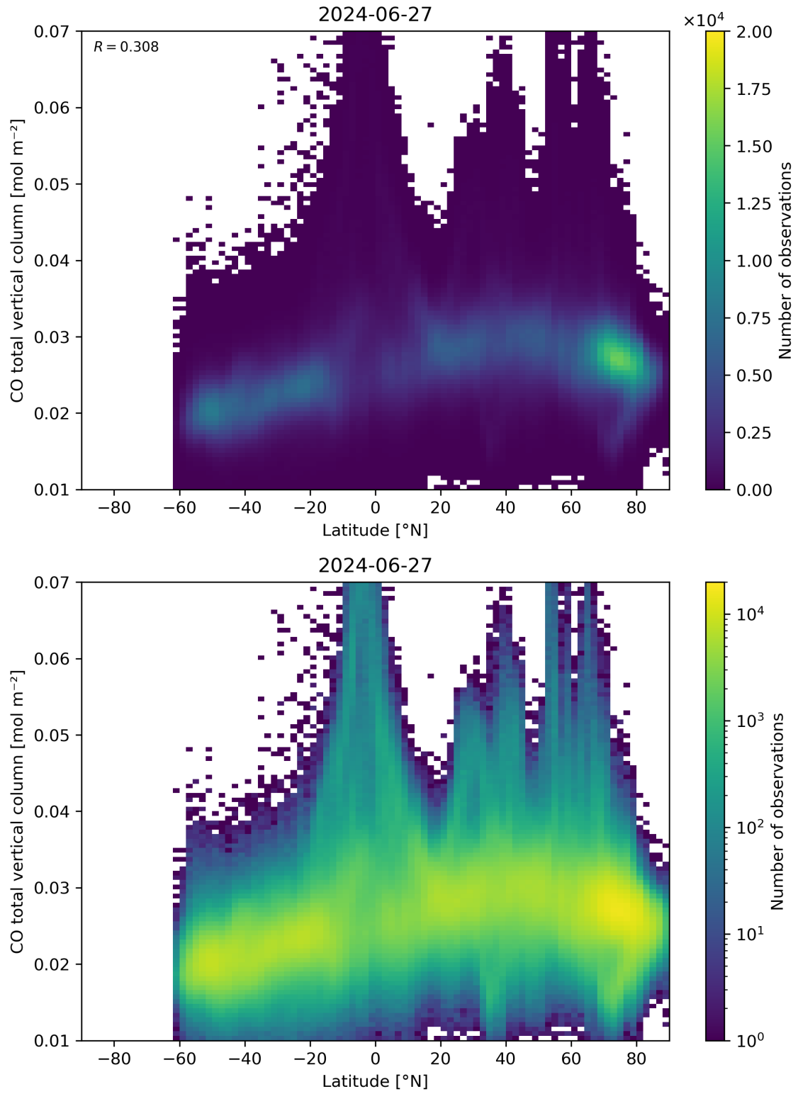
Figure 51: Scatter density plot of “Latitude” against “CO total vertical column” for 2024-06-26 to 2024-06-28.
