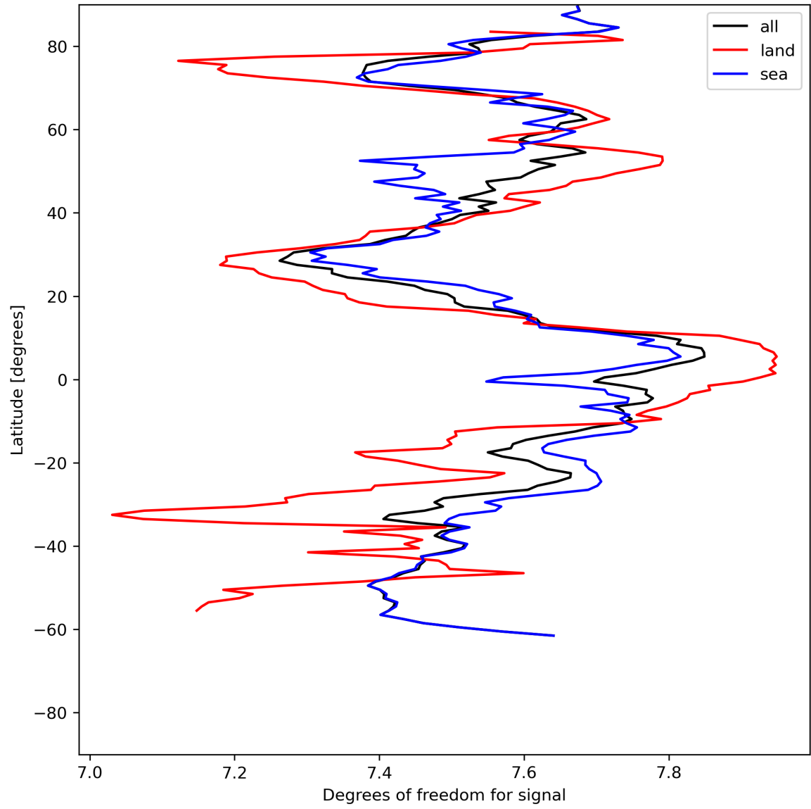
Figure 15: Zonal average of “Degrees of freedom for signal” for 2024-06-26 to 2024-06-28.
