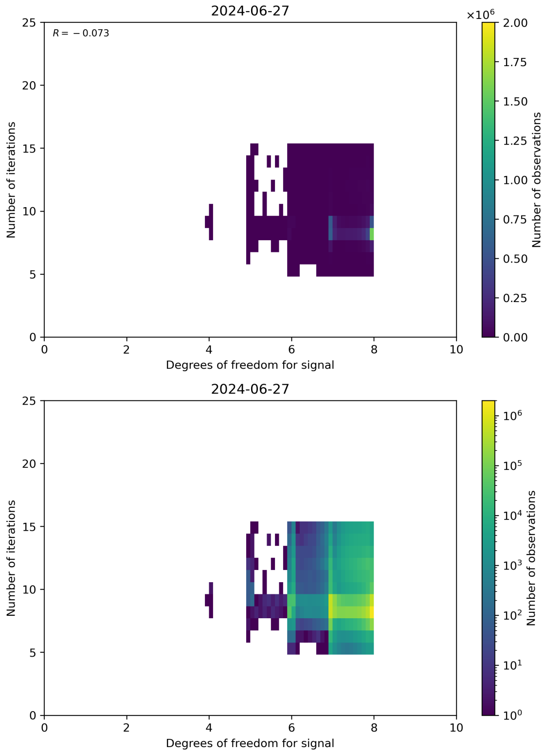
Figure 50: Scatter density plot of “Degrees of freedom for signal” against “Number of iterations” for 2024-06-26 to 2024-06-28.
