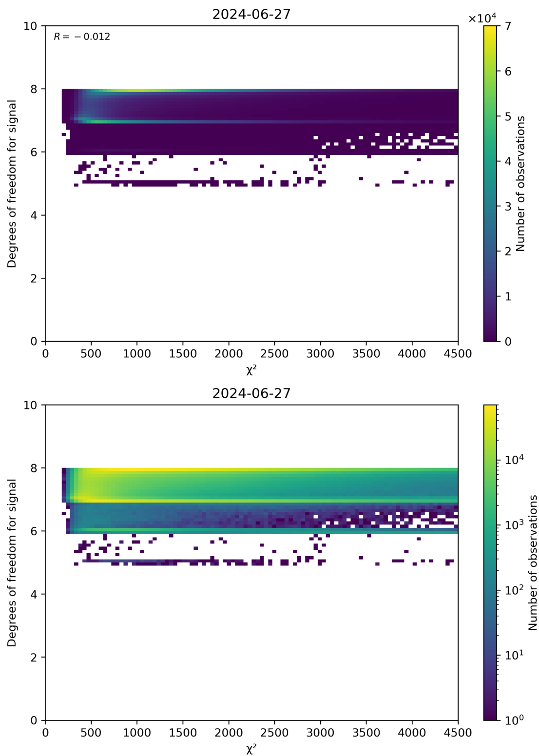
Figure 48: Scatter density plot of “ \chi^2 ” against “Degrees of freedom for signal” for 2024-06-26 to 2024-06-28.
