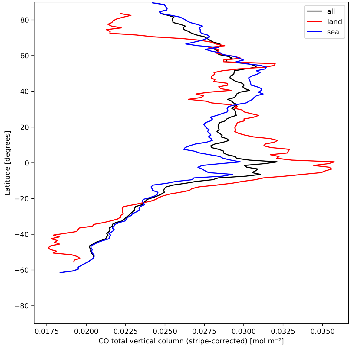
Figure 11: Zonal average of “CO total vertical column (stripe-corrected)” for 2024-06-26 to 2024-06-28.
