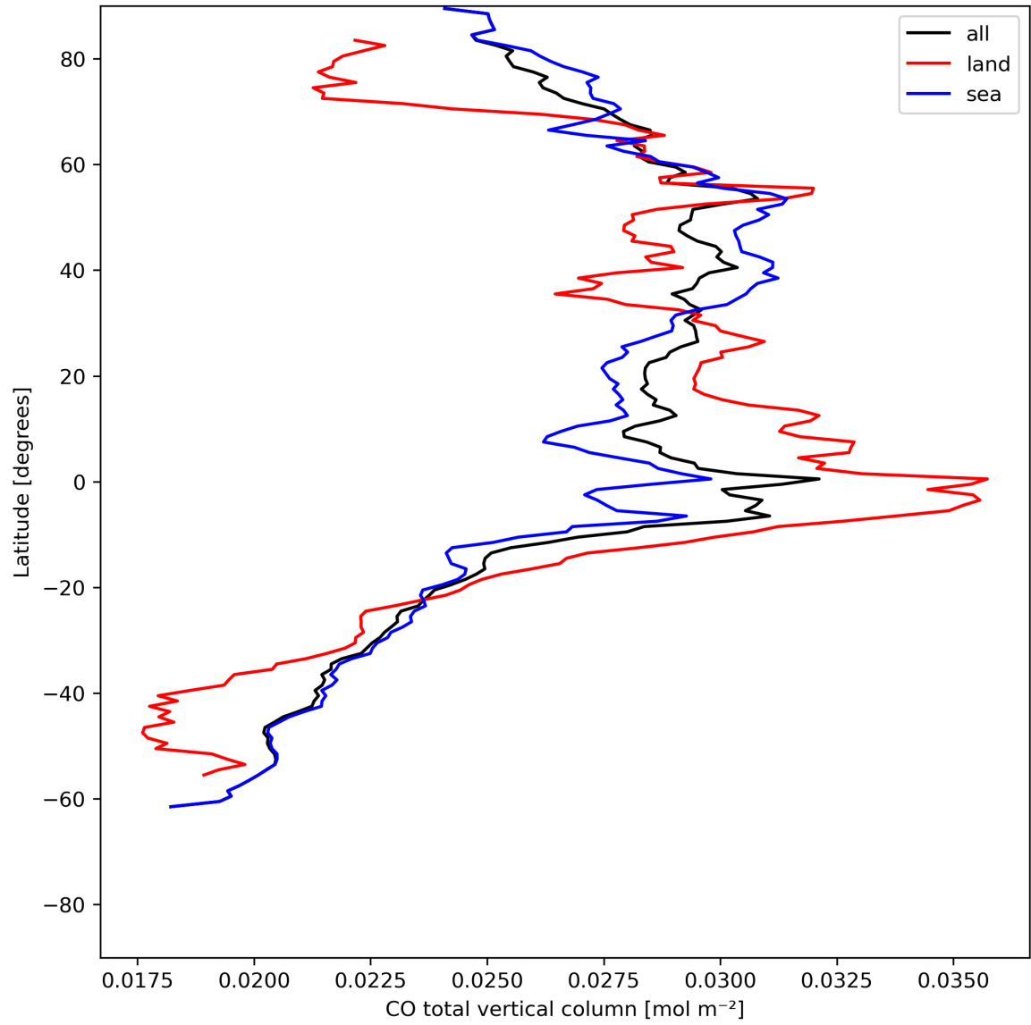
Figure 10: Zonal average of “CO total vertical column” for 2024-06-26 to 2024-06-28.
