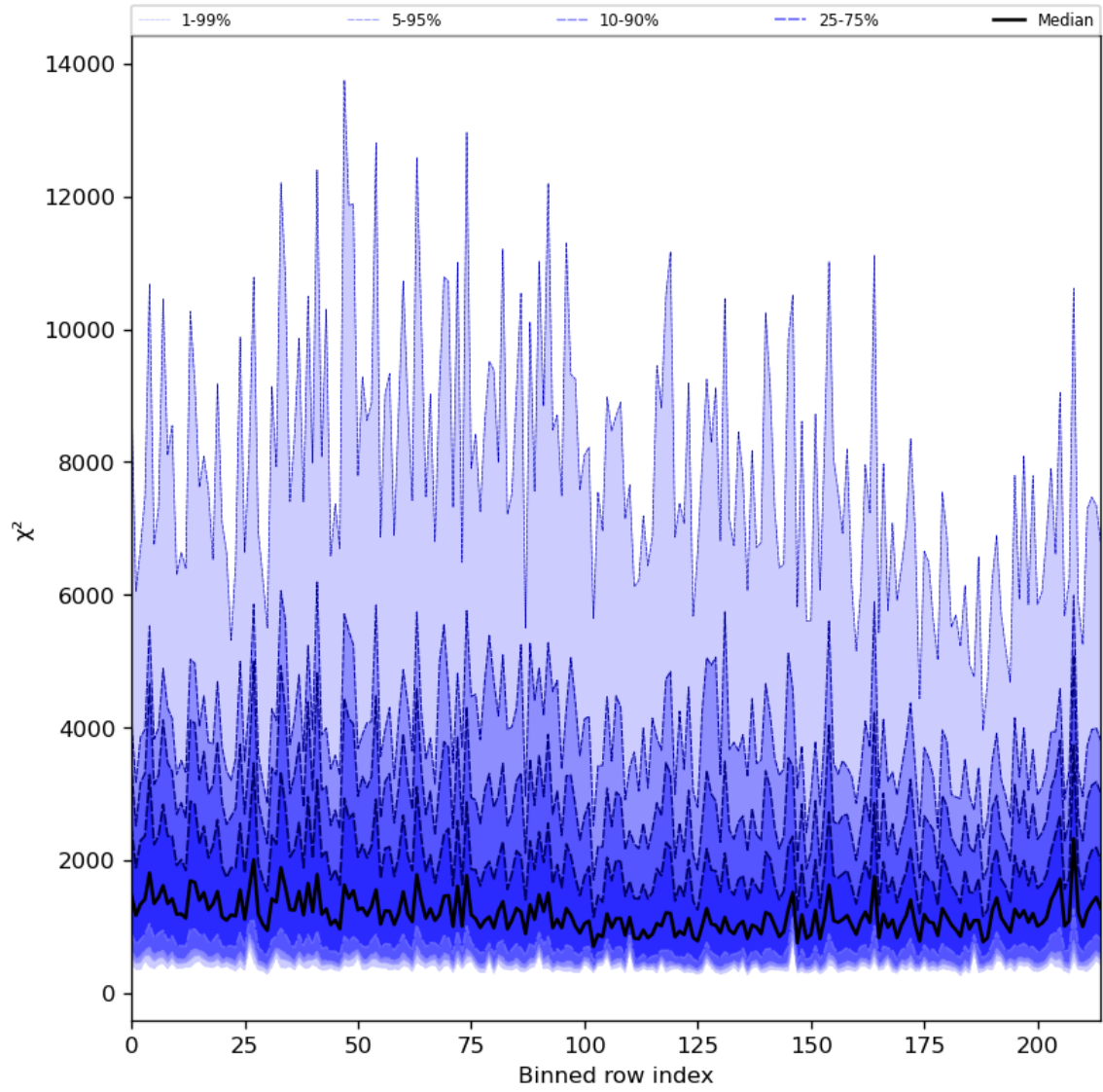
Figure 30: Along track statistics of “ \chi^2 ” for 2024-06-26 to 2024-06-28
