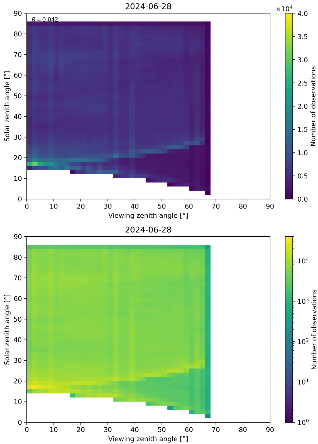
Figure 77: Scatter density plot of “Viewing zenith angle” against “Solar zenith angle” for 2024-06-27 to 2024-06-29.
