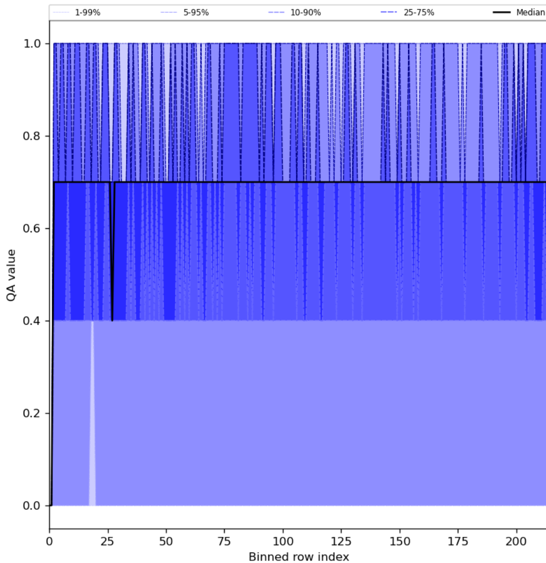
Figure 25: Along track statistics of “QA value” for 2024-06-27 to 2024-06-29
