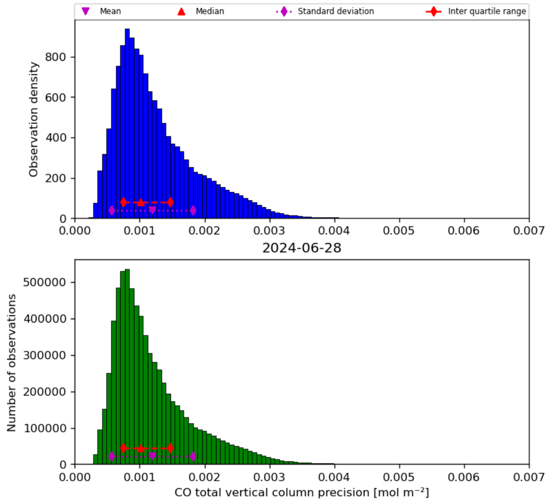
Figure 20: Histogram of “CO total vertical column precision” for 2024-06-27 to 2024-06-29
