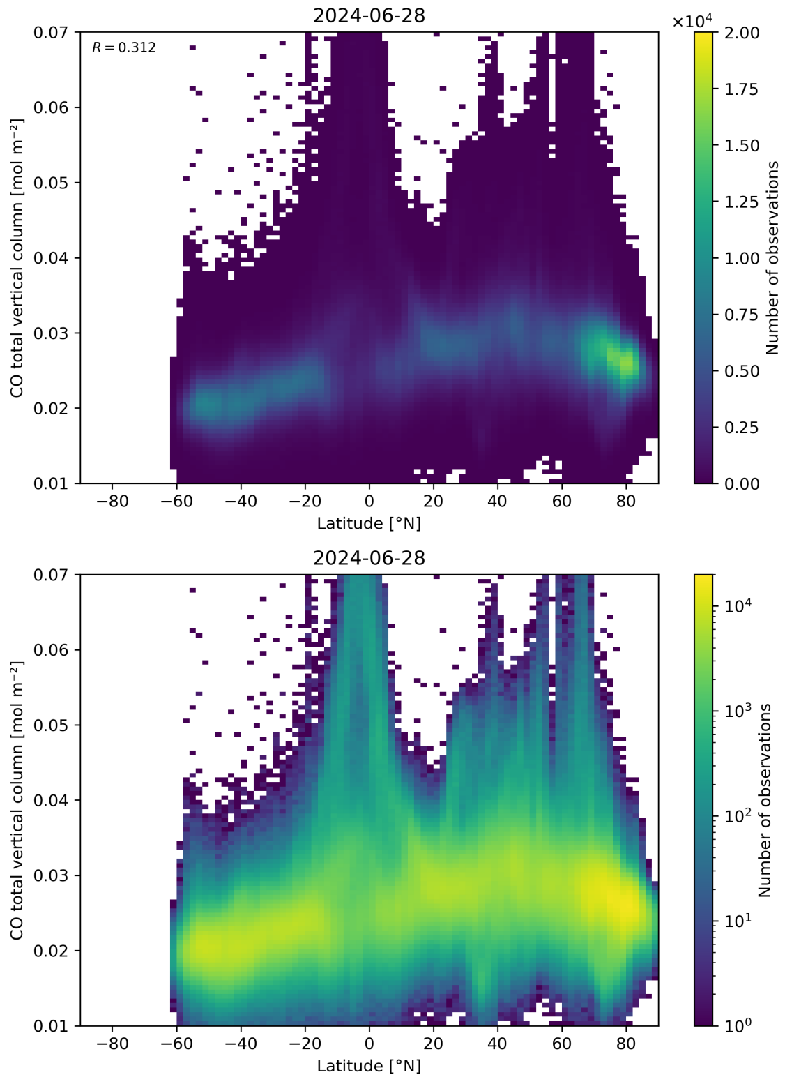
Figure 51: Scatter density plot of “Latitude” against “CO total vertical column” for 2024-06-27 to 2024-06-29.
