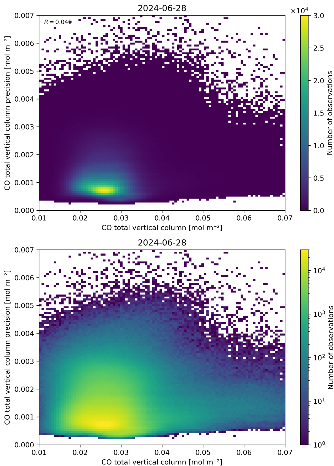
Figure 34: Scatter density plot of “CO total vertical column” against “CO total vertical column precision” for 2024-06-27 to 2024-06-29.
