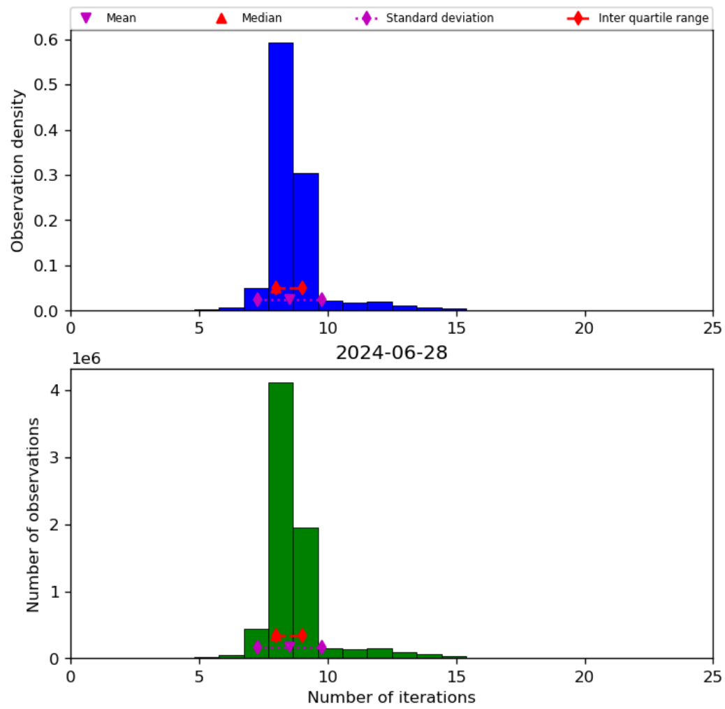
Figure 24: Histogram of “Number of iterations” for 2024-06-27 to 2024-06-29
