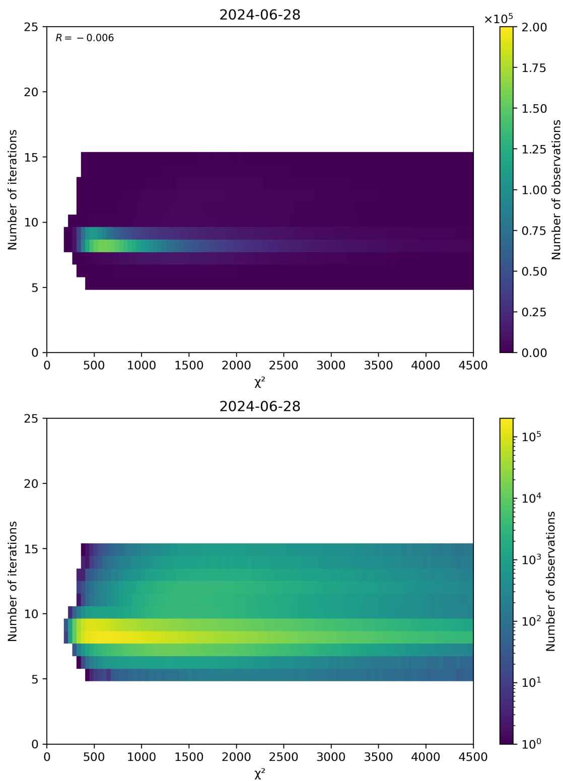
Figure 49: Scatter density plot of “ \chi^2 ” against “Number of iterations” for 2024-06-27 to 2024-06-29.
