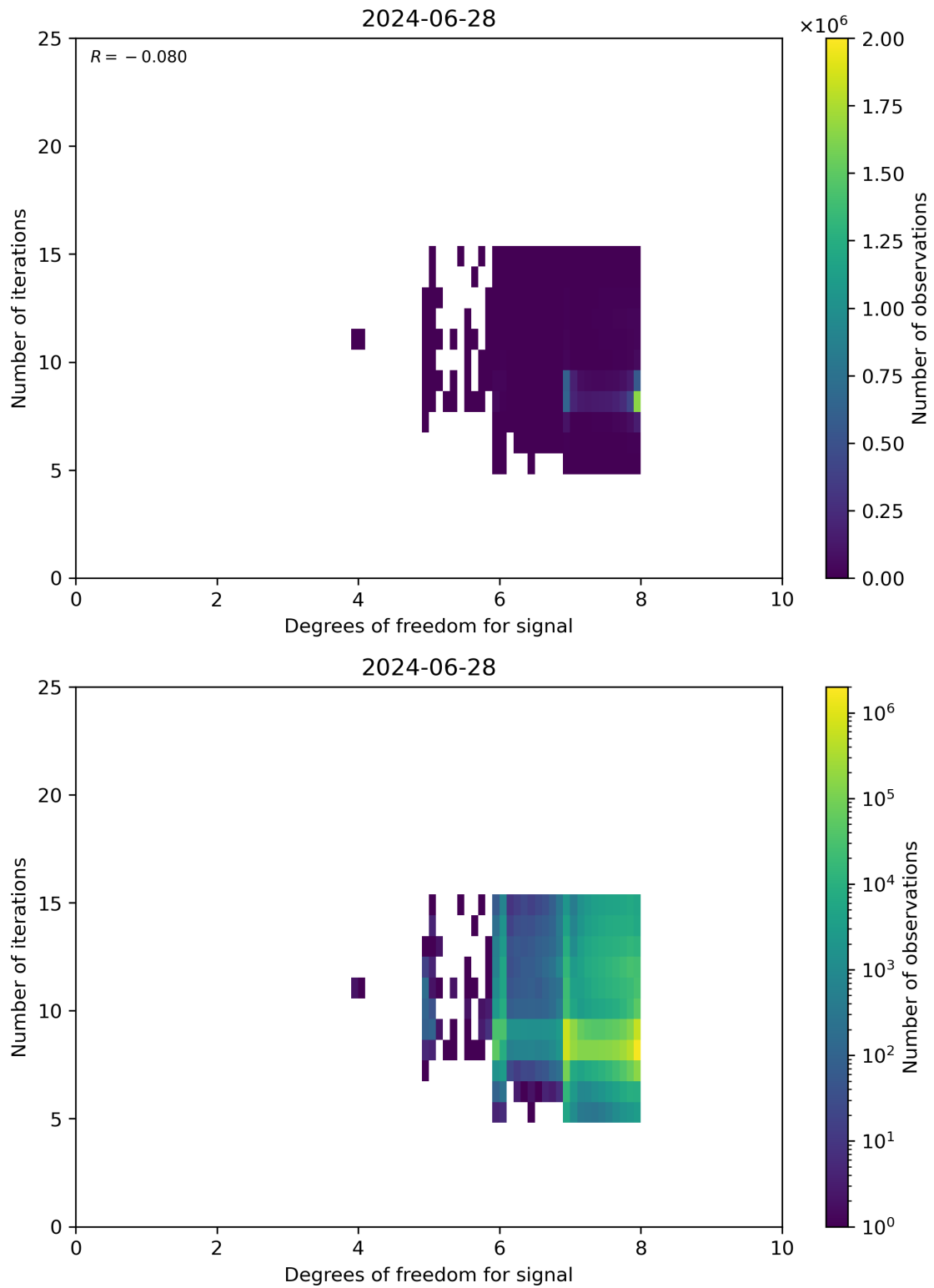
Figure 50: Scatter density plot of “Degrees of freedom for signal” against “Number of iterations” for 2024-06-27 to 2024-06-29.
