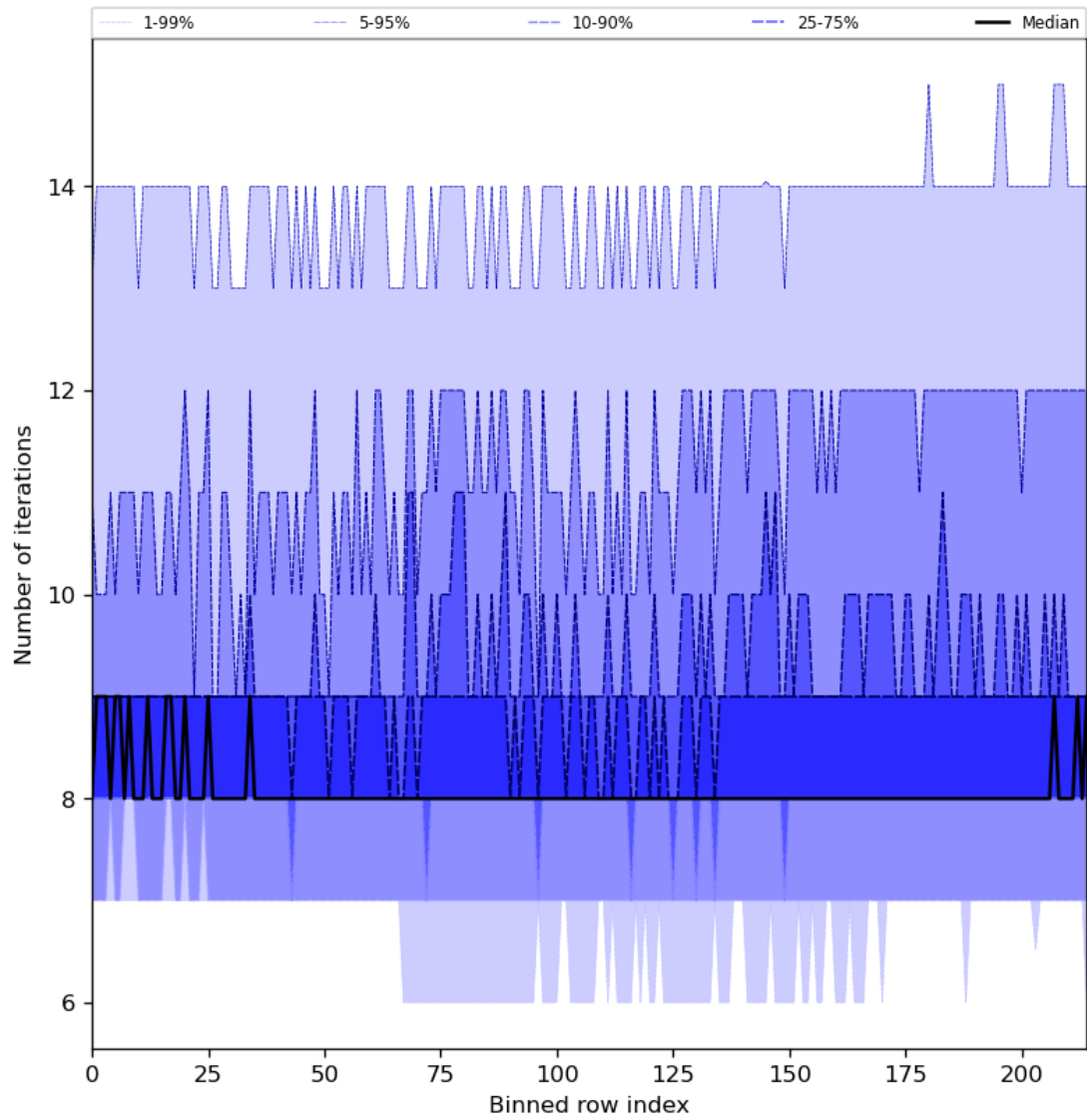
Figure 32: Along track statistics of “Number of iterations” for 2024-06-27 to 2024-06-29
