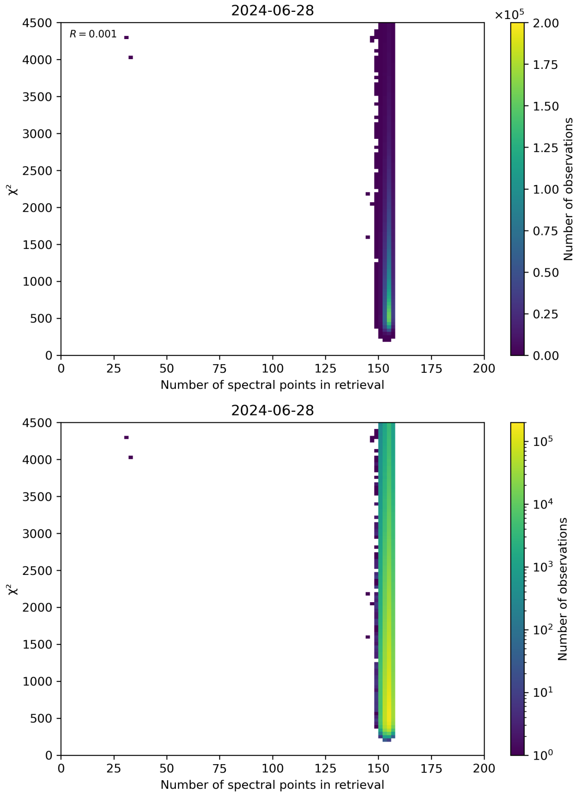
Figure 58: Scatter density plot of “Number of spectral points in retrieval” against “ \chi^2 ” for 2024-06-27 to 2024-06-29.
