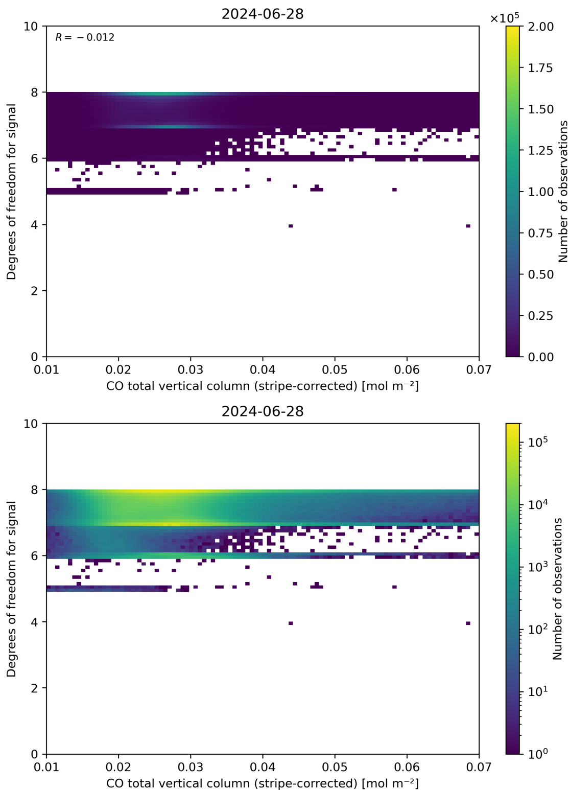
Figure 38: Scatter density plot of “CO total vertical column (stripe-corrected)” against “Degrees of freedom for signal” for 2024-06-27 to 2024-06-29.
