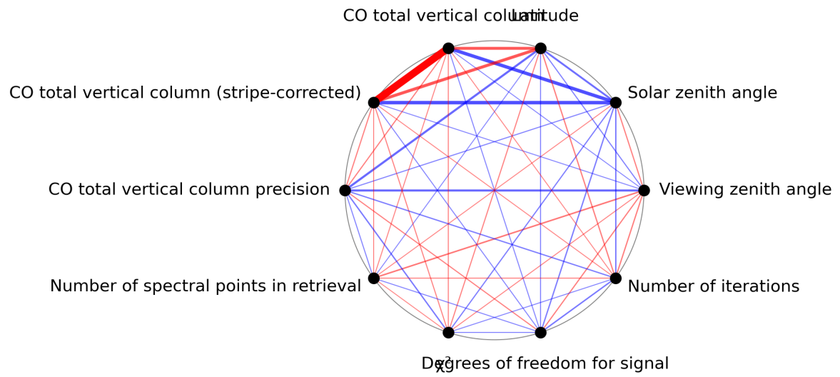
Figure 1: Map of correlation graph for 2024-06-27 to 2024-06-29.
