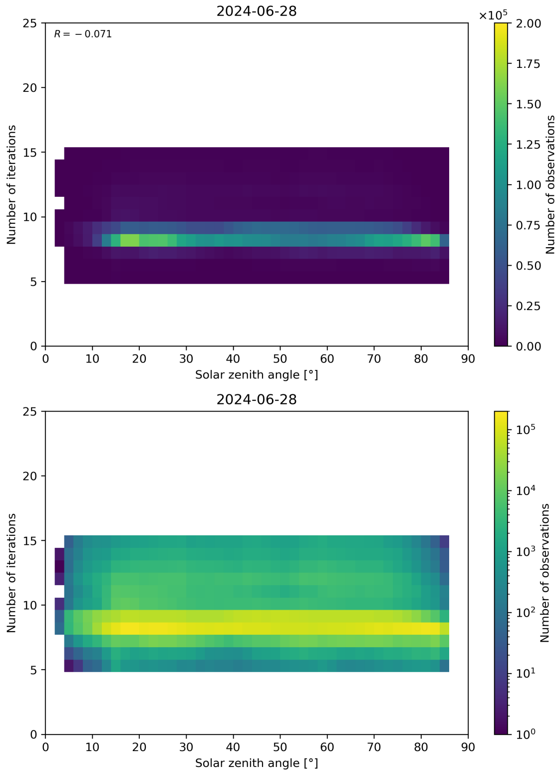
Figure 67: Scatter density plot of “Solar zenith angle” against “Number of iterations” for 2024-06-27 to 2024-06-29.
