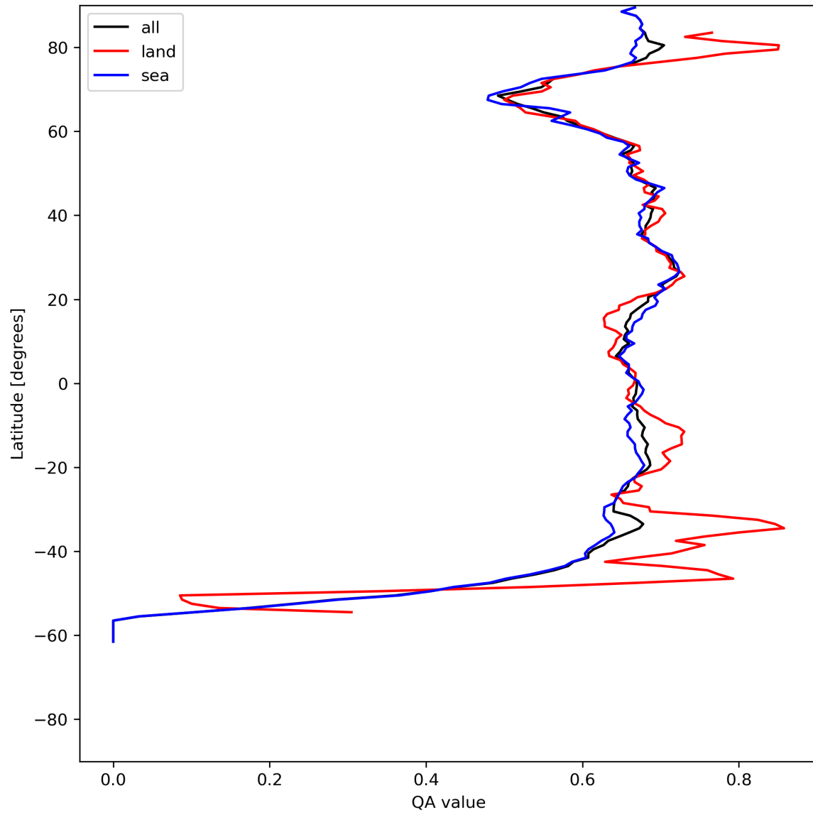
Figure 9: Zonal average of “QA value” for 2024-06-27 to 2024-06-29.
