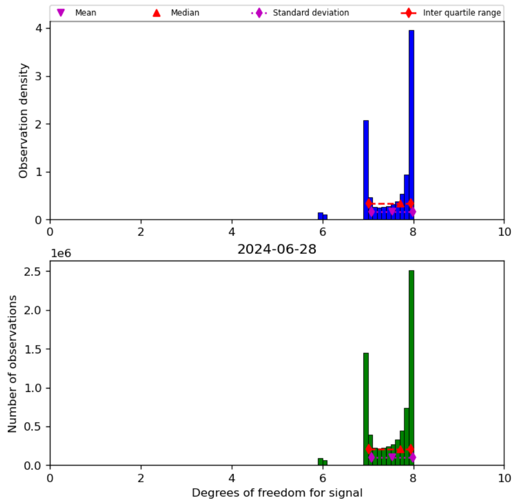
Figure 23: Histogram of “Degrees of freedom for signal” for 2024-06-27 to 2024-06-29
