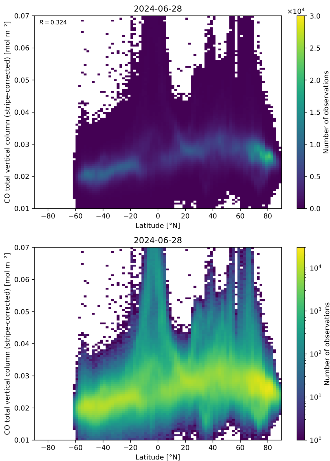
Figure 52: Scatter density plot of “Latitude” against “CO total vertical column (stripe-corrected)” for 2024-06-27 to 2024-06-29.
