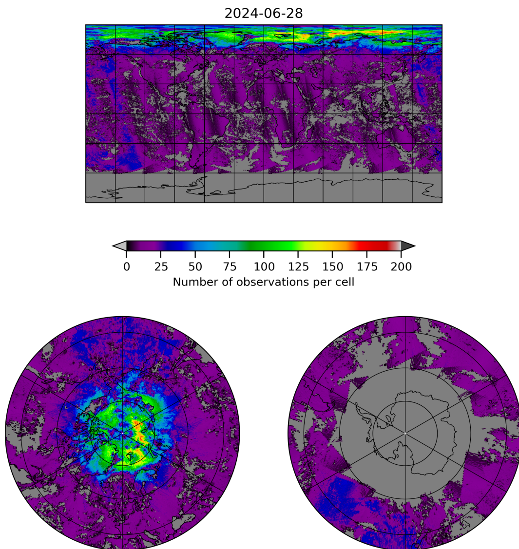
Figure 8: Map of the number of observations for 2024-06-27 to 2024-06-29
