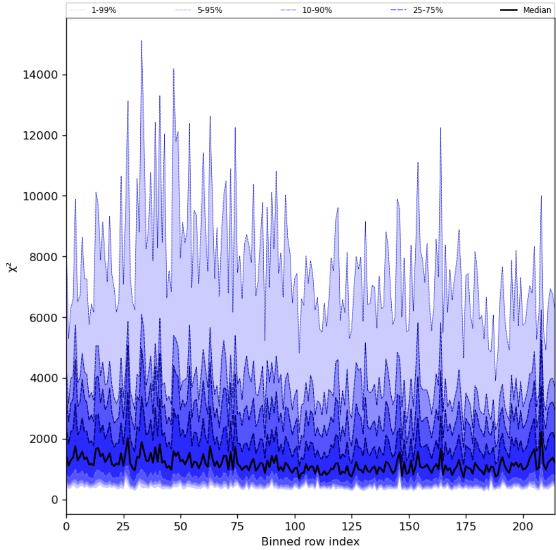
Figure 30: Along track statistics of “ \chi^2 ” for 2024-06-27 to 2024-06-29
