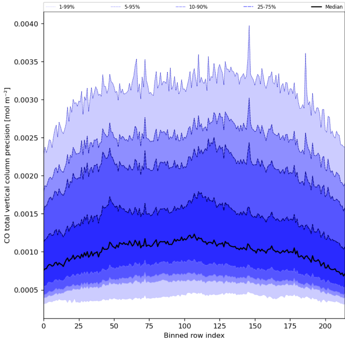
Figure 28: Along track statistics of “CO total vertical column precision” for 2024-06-27 to 2024-06-29
