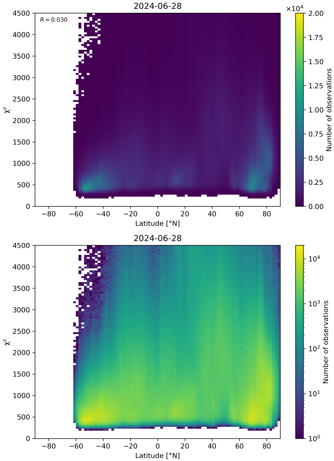
Figure 54: Scatter density plot of “Latitude” against “ \chi^2 ” for 2024-06-27 to 2024-06-29.
