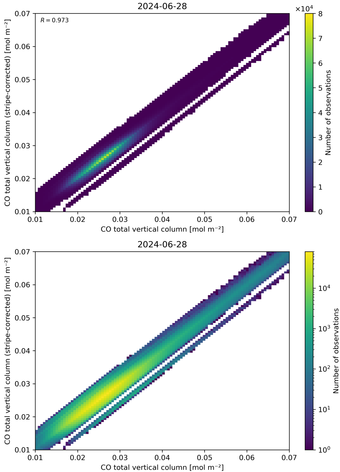
Figure 33: Scatter density plot of “CO total vertical column” against “CO total vertical column (stripe-corrected)” for 2024-06-27 to 2024-06-29.
