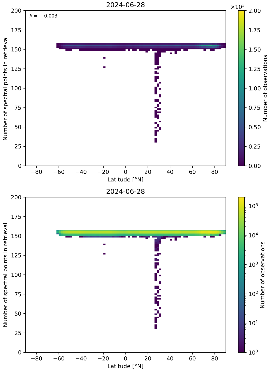
Figure 57: Scatter density plot of “Latitude” against “Number of spectral points in retrieval” for 2024-06-27 to 2024-06-29.
