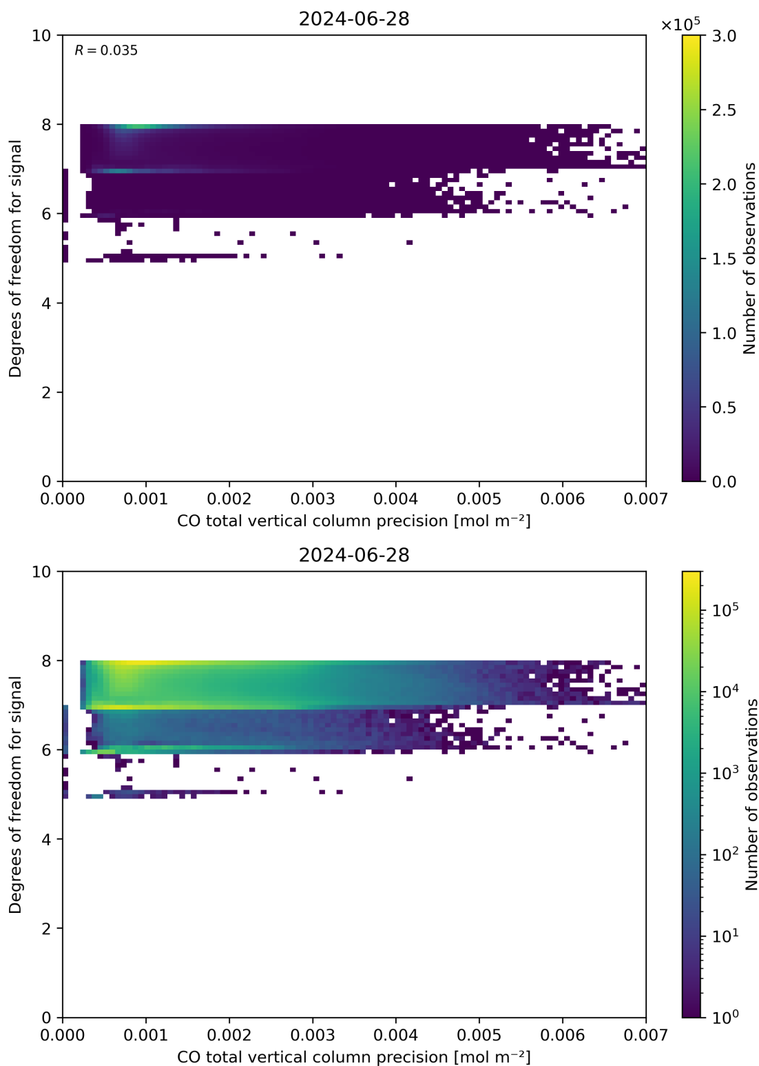
Figure 45: Scatter density plot of “CO total vertical column precision” against “Degrees of freedom for signal” for 2024-06-27 to 2024-06-29.
