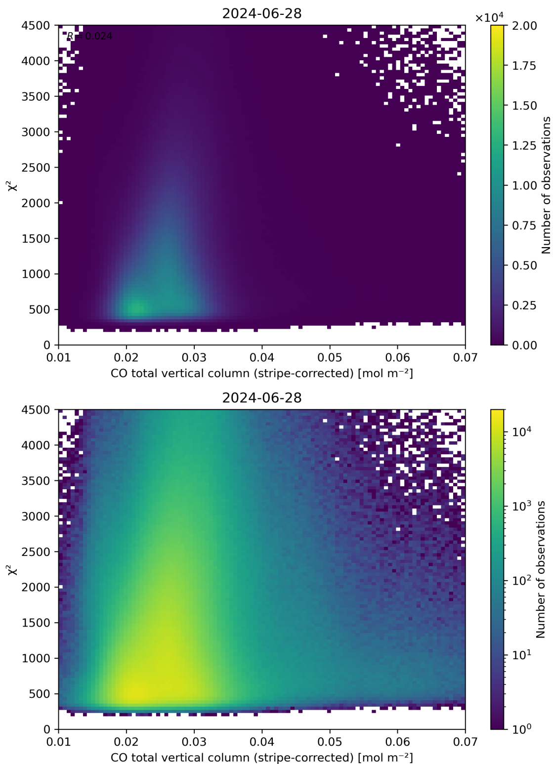
Figure 37: Scatter density plot of “CO total vertical column (stripe-corrected)” against “ \chi^2 ” for 2024-06-27 to 2024-06-29.
