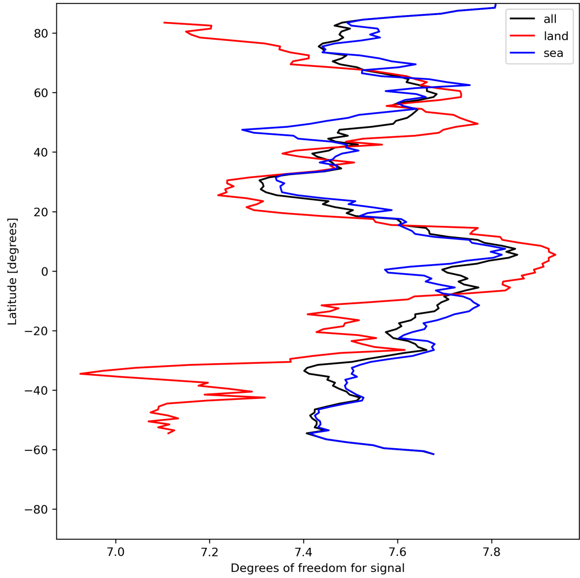
Figure 15: Zonal average of “Degrees of freedom for signal” for 2024-06-27 to 2024-06-29.
