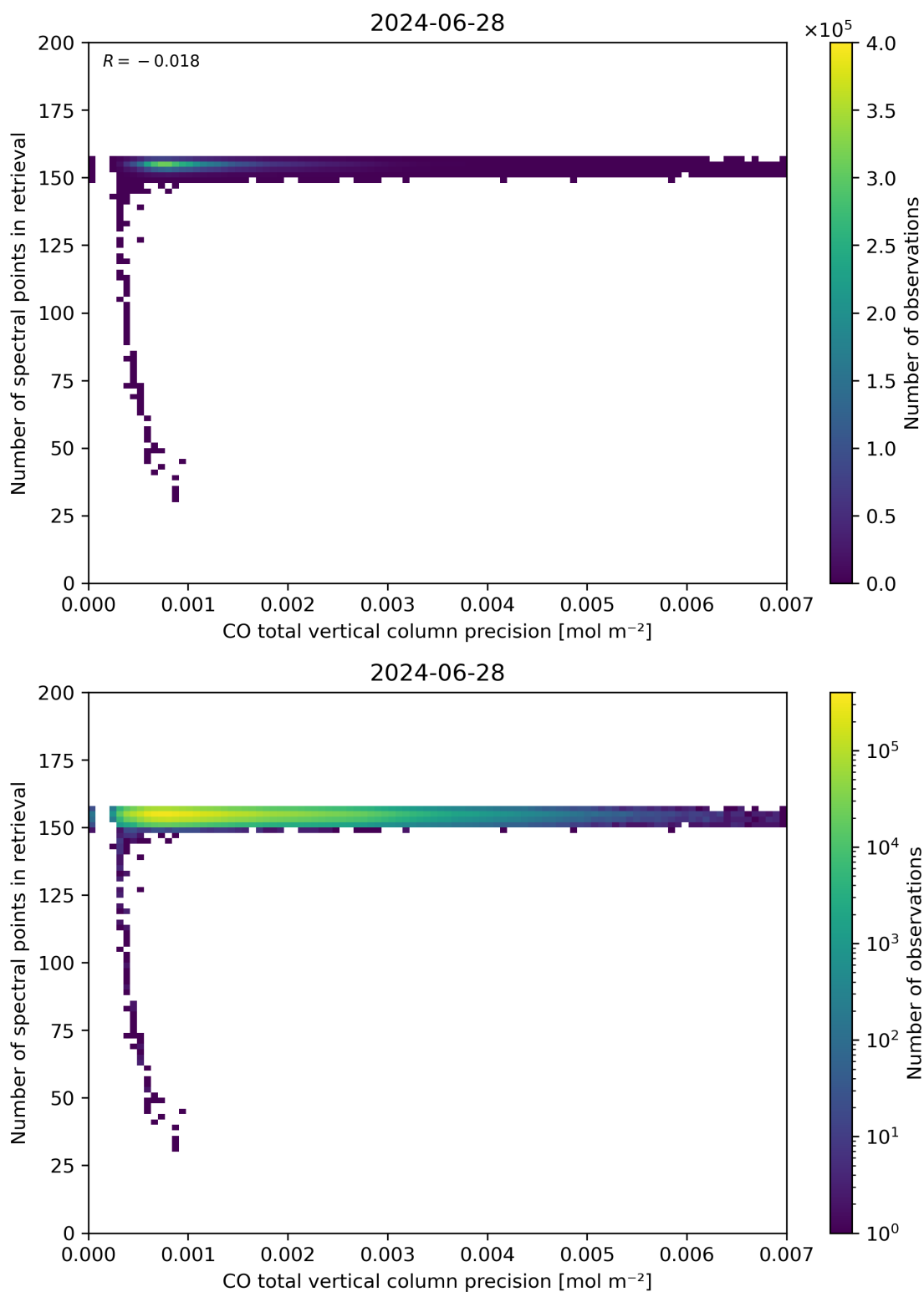
Figure 47: Scatter density plot of “CO total vertical column precision” against “Number of spectral points in retrieval” for 2024-06-27 to 2024-06-29.
