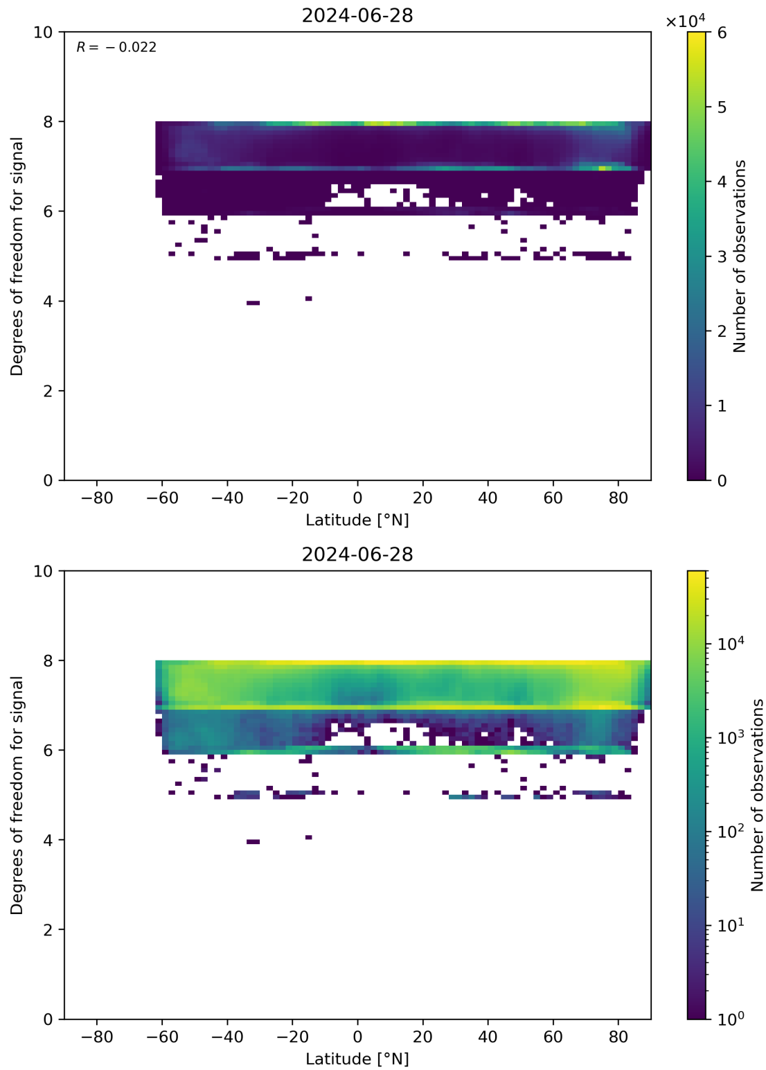
Figure 55: Scatter density plot of “Latitude” against “Degrees of freedom for signal” for 2024-06-27 to 2024-06-29.
