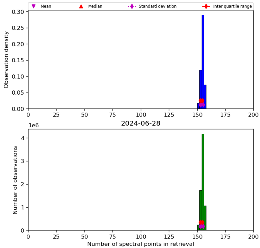
Figure 21: Histogram of “Number of spectral points in retrieval” for 2024-06-27 to 2024-06-29
