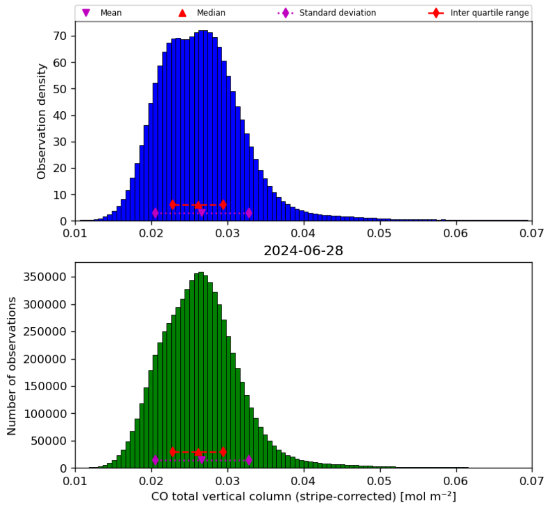
Figure 19: Histogram of “CO total vertical column (stripe-corrected)” for 2024-06-27 to 2024-06-29
