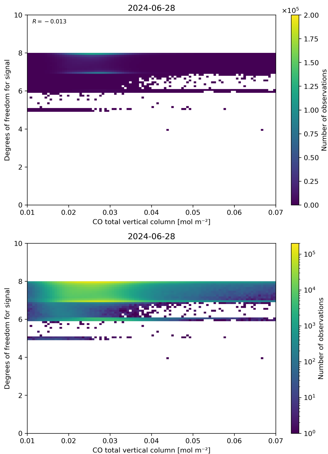
Figure 41: Scatter density plot of “CO total vertical column” against “Degrees of freedom for signal” for 2024-06-27 to 2024-06-29.
