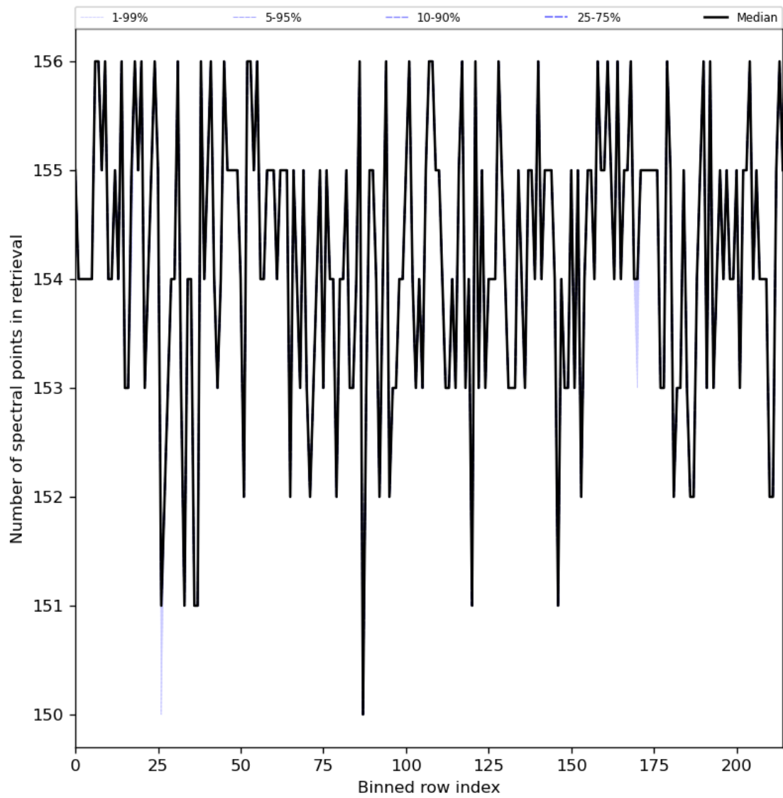
Figure 29: Along track statistics of “Number of spectral points in retrieval” for 2024-06-27 to 2024-06-29
