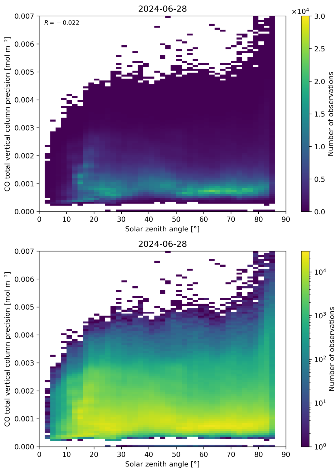
Figure 63: Scatter density plot of “Solar zenith angle” against “CO total vertical column precision” for 2024-06-27 to 2024-06-29.
