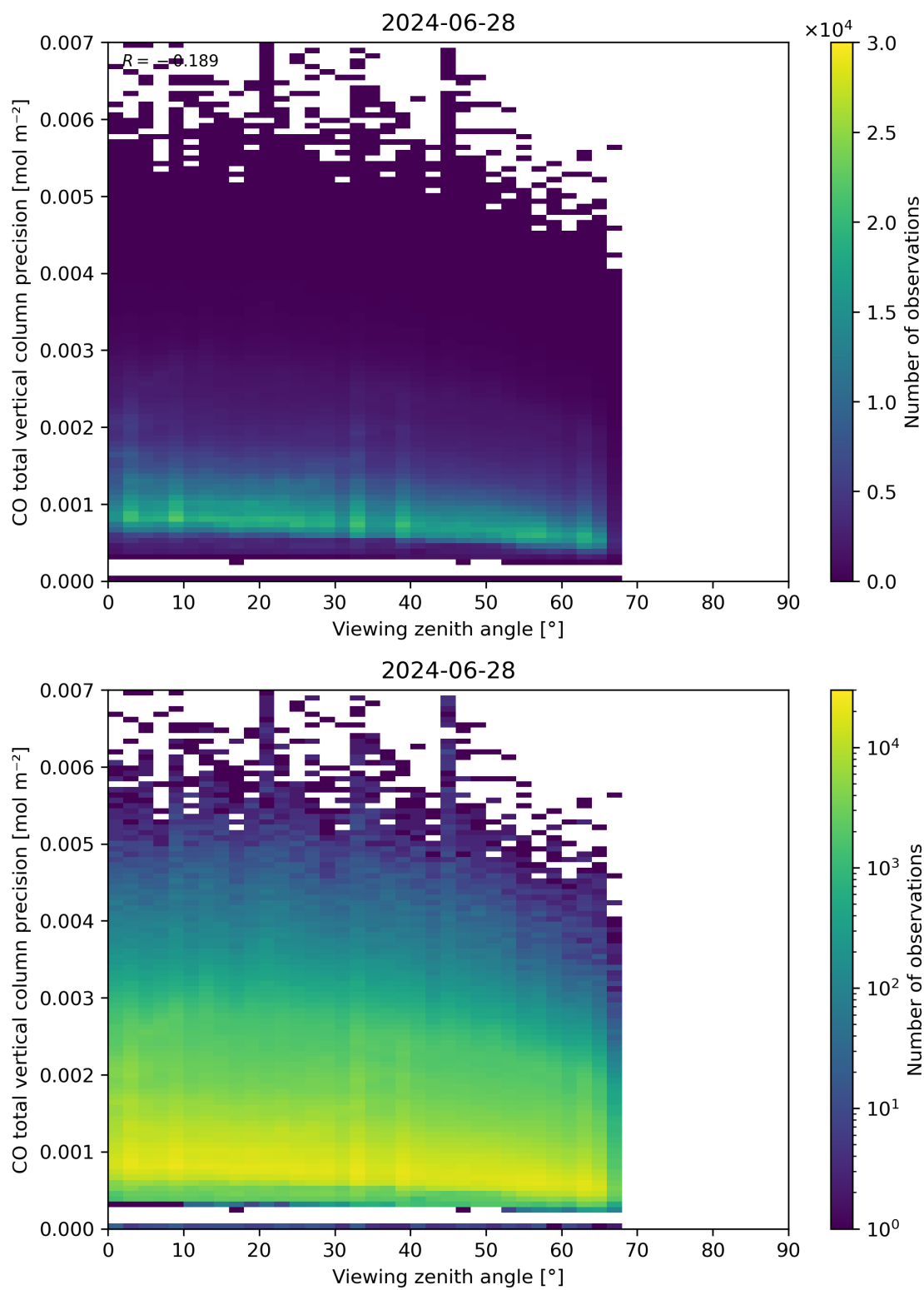
Figure 71: Scatter density plot of “Viewing zenith angle” against “CO total vertical column precision” for 2024-06-27 to 2024-06-29.
