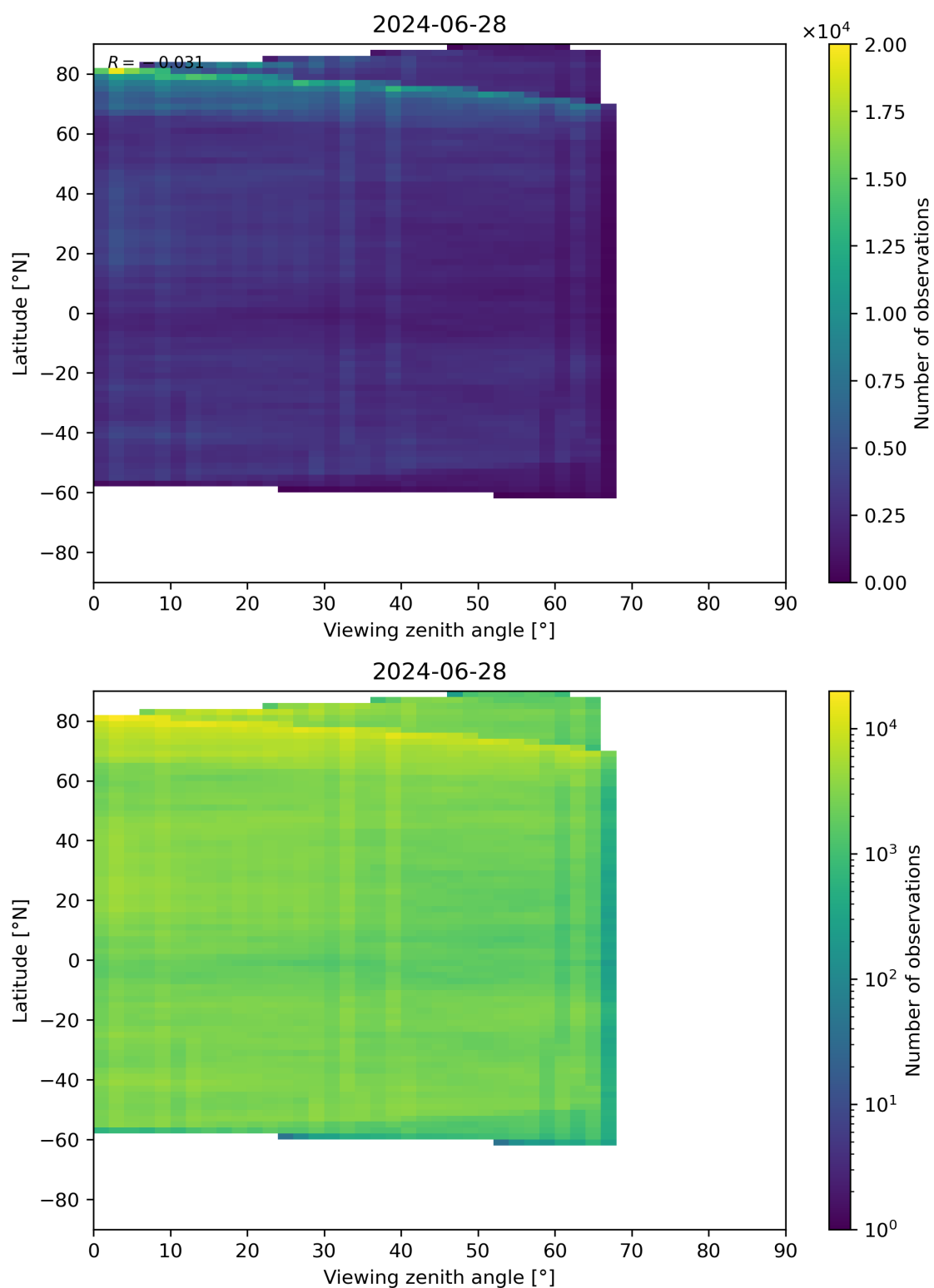
Figure 74: Scatter density plot of “Viewing zenith angle” against “Latitude” for 2024-06-27 to 2024-06-29.
