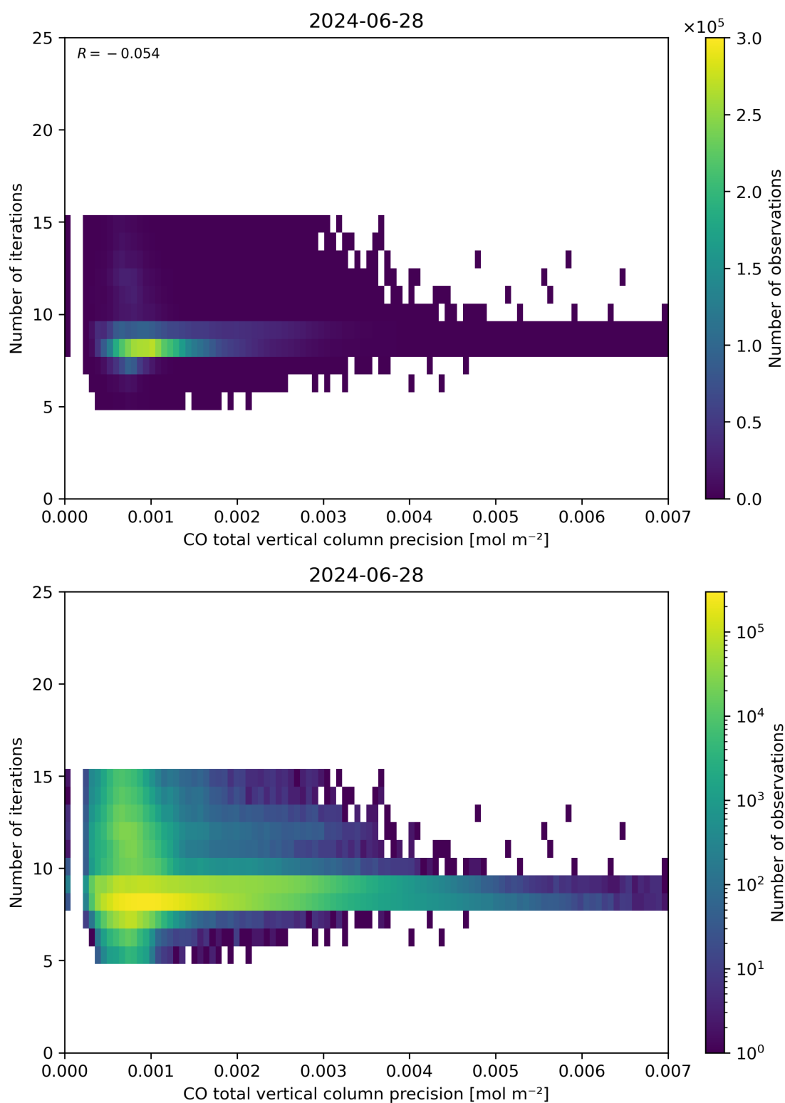
Figure 46: Scatter density plot of “CO total vertical column precision” against “Number of iterations” for 2024-06-27 to 2024-06-29.
