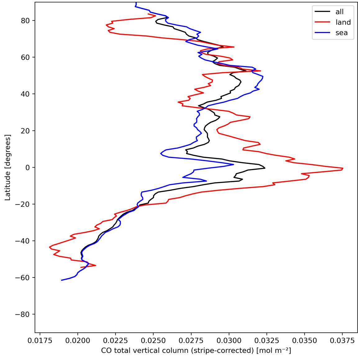
Figure 11: Zonal average of “CO total vertical column (stripe-corrected)” for 2024-06-27 to 2024-06-29.
