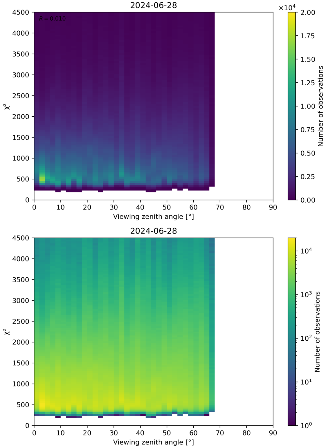
Figure 72: Scatter density plot of “Viewing zenith angle” against “ \chi^2 ” for 2024-06-27 to 2024-06-29.
