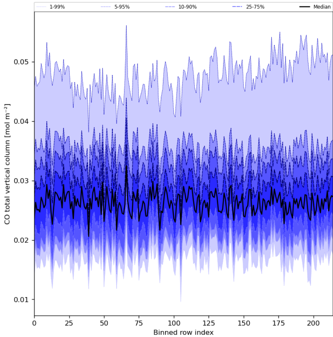
Figure 26: Along track statistics of “CO total vertical column” for 2024-06-27 to 2024-06-29
