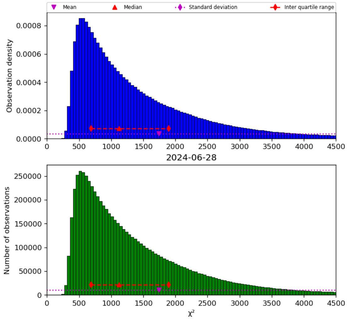
Figure 22: Histogram of “ \chi^2 ” for 2024-06-27 to 2024-06-29
