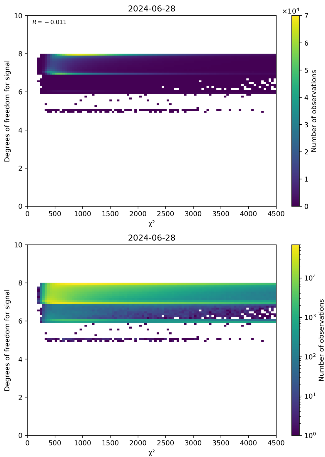
Figure 48: Scatter density plot of “ \chi^2 ” against “Degrees of freedom for signal” for 2024-06-27 to 2024-06-29.
