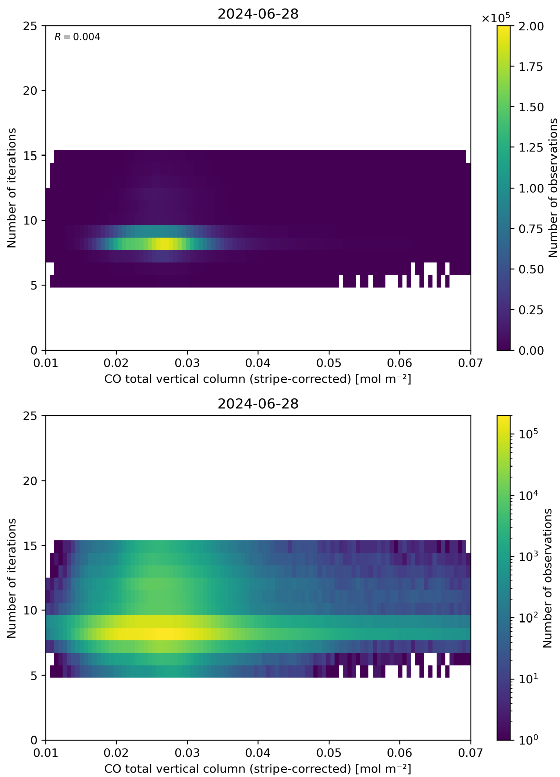
Figure 39: Scatter density plot of “CO total vertical column (stripe-corrected)” against “Number of iterations” for 2024-06-27 to 2024-06-29.
