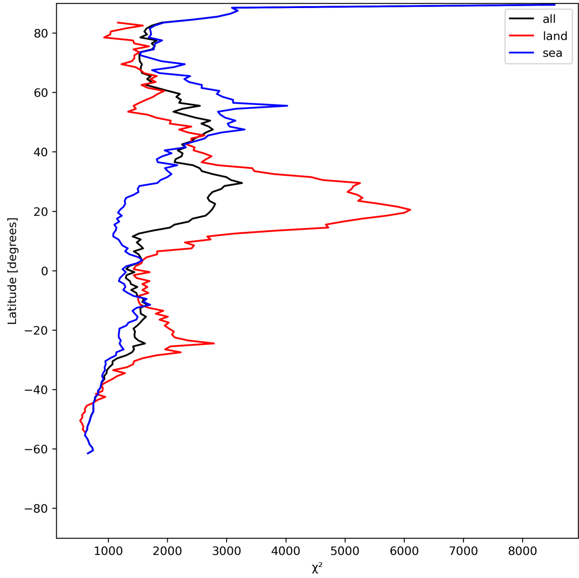
Figure 14: Zonal average of “ \chi^2 ” for 2024-06-27 to 2024-06-29.
