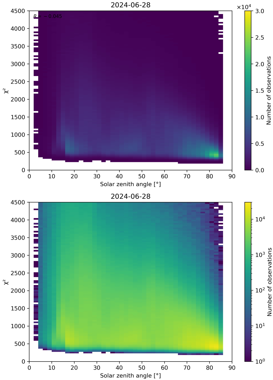
Figure 64: Scatter density plot of “Solar zenith angle” against “ \chi^2 ” for 2024-06-27 to 2024-06-29.
