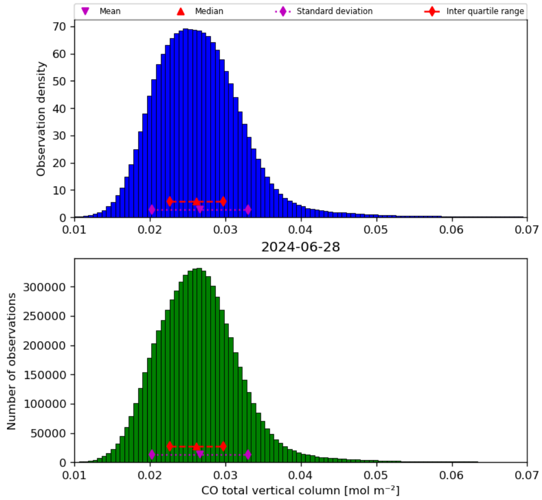
Figure 18: Histogram of “CO total vertical column” for 2024-06-27 to 2024-06-29
