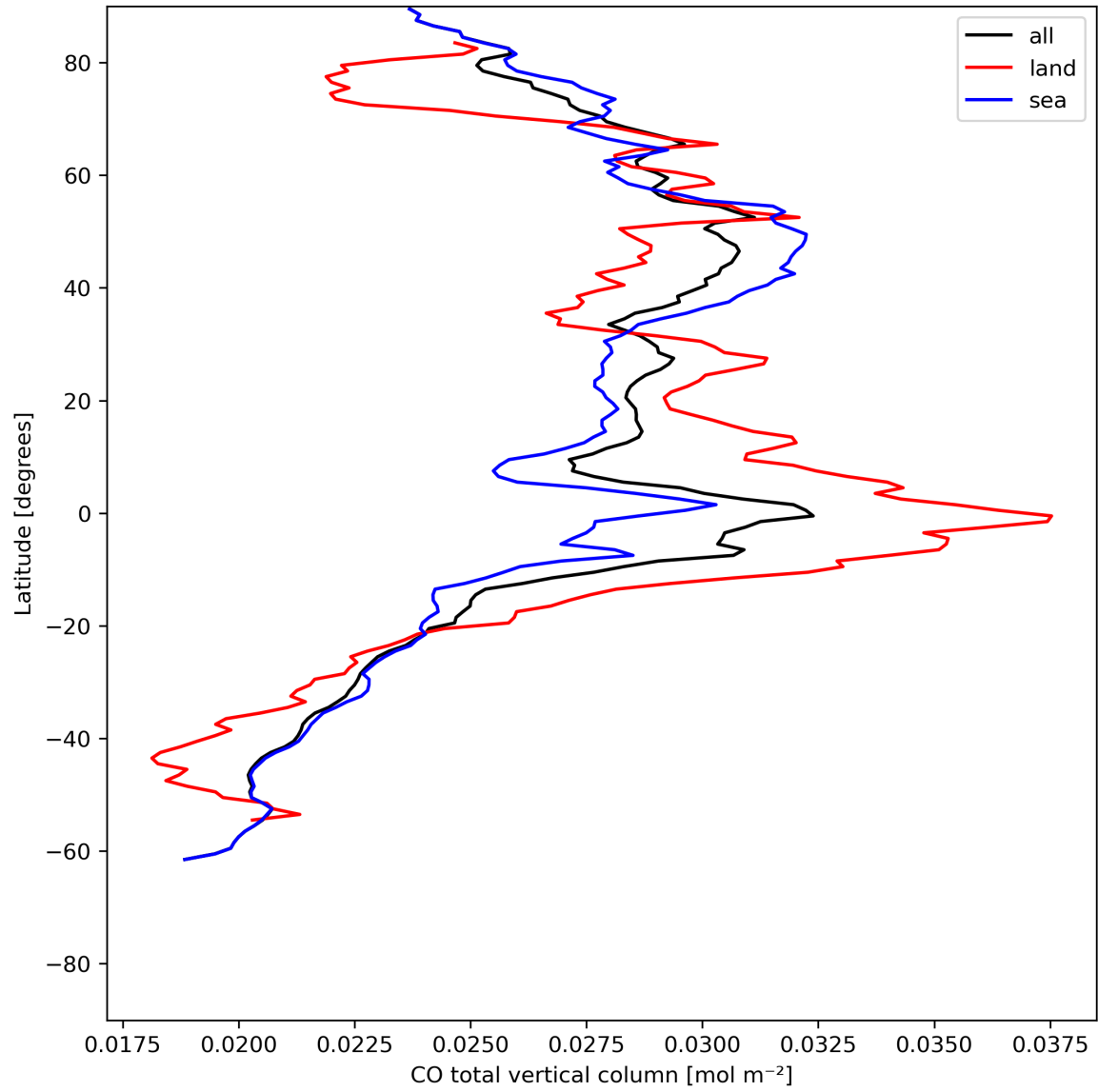
Figure 10: Zonal average of “CO total vertical column” for 2024-06-27 to 2024-06-29.
