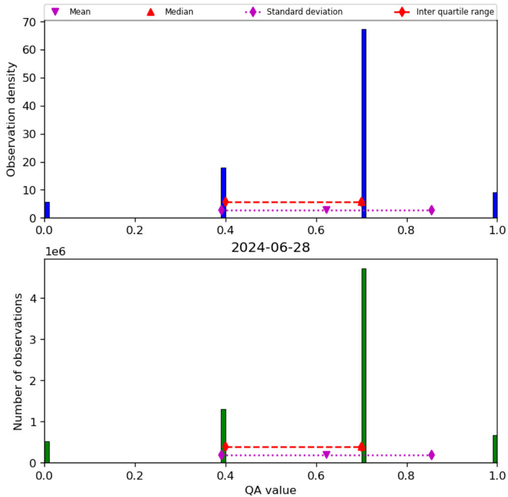
Figure 17: Histogram of “QA value” for 2024-06-27 to 2024-06-29
