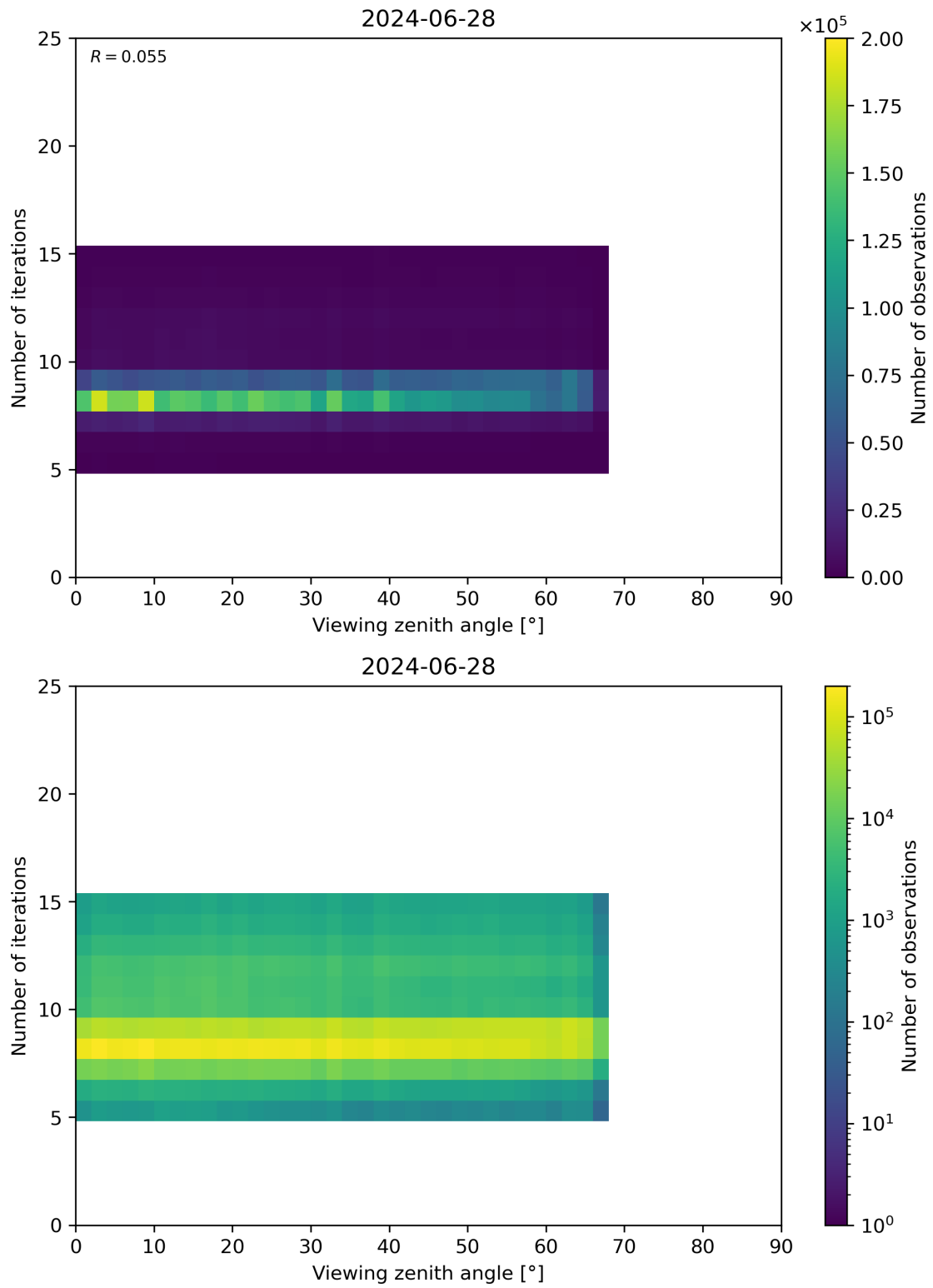
Figure 75: Scatter density plot of “Viewing zenith angle” against “Number of iterations” for 2024-06-27 to 2024-06-29.
