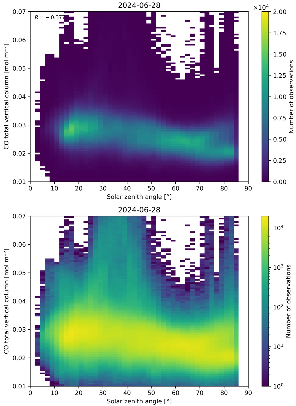
Figure 61: Scatter density plot of “Solar zenith angle” against “CO total vertical column” for 2024-06-27 to 2024-06-29.
