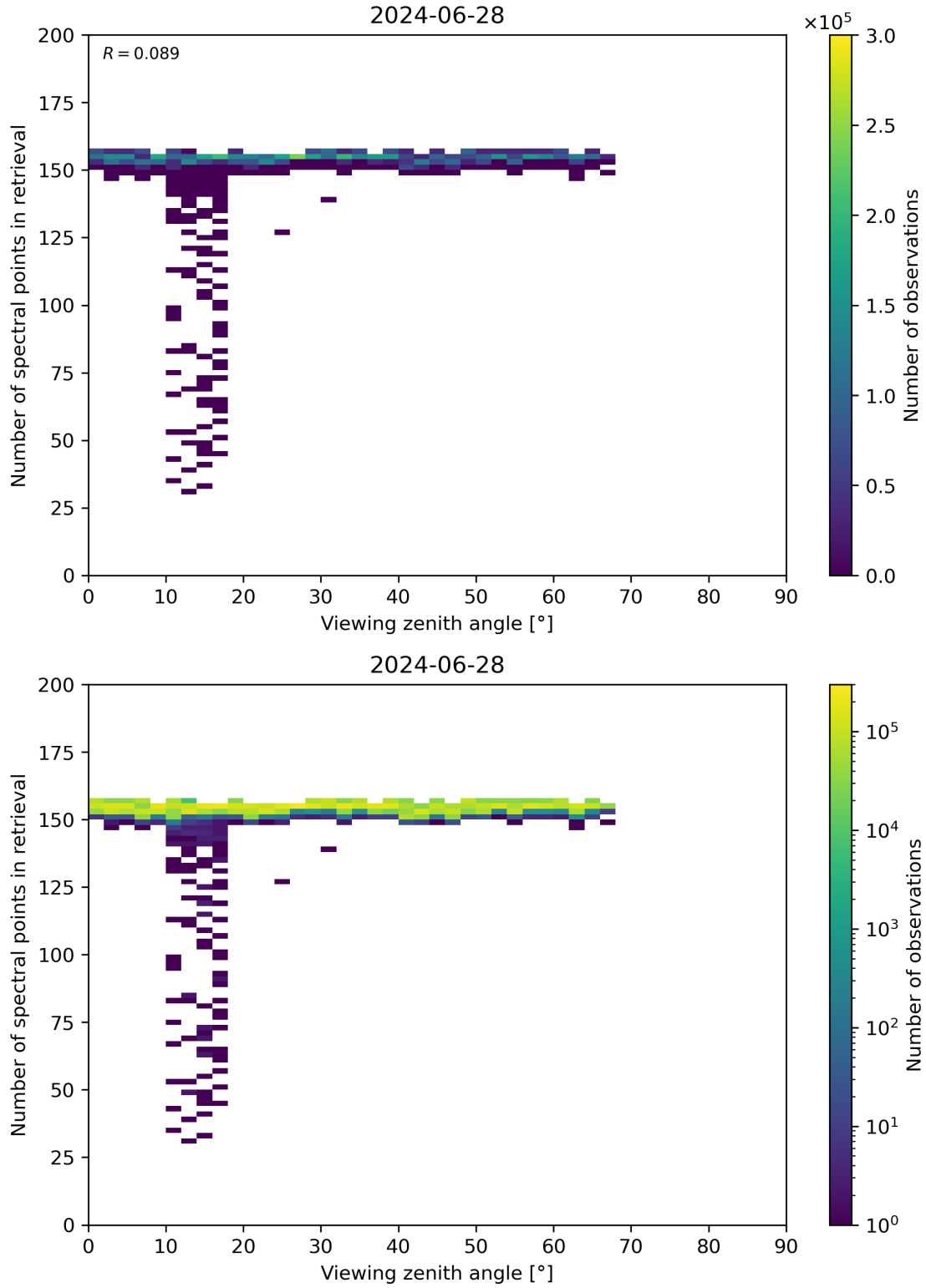
Figure 76: Scatter density plot of “Viewing zenith angle” against “Number of spectral points in retrieval” for 2024-06-27 to 2024-06-29.
