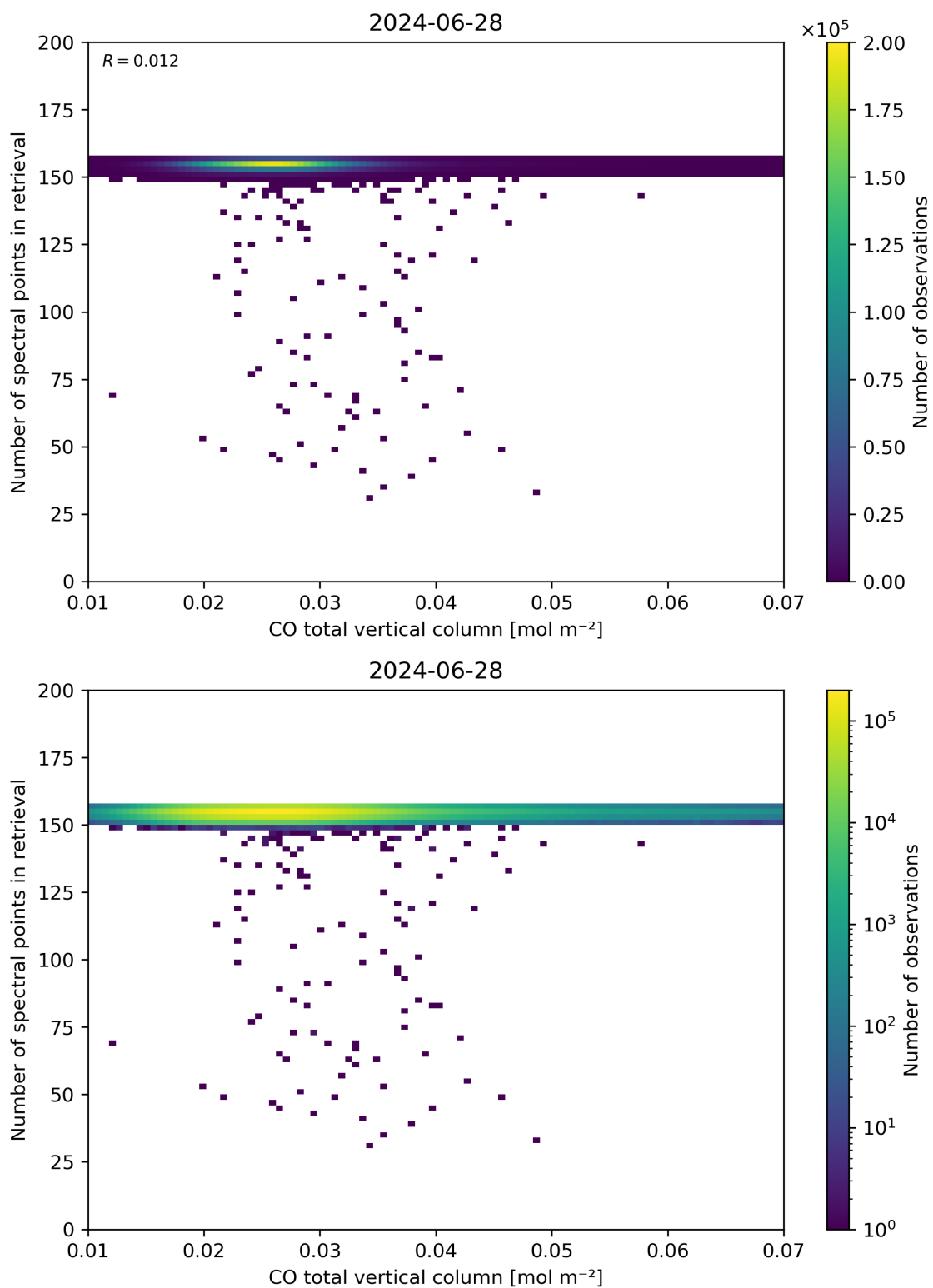
Figure 43: Scatter density plot of “CO total vertical column” against “Number of spectral points in retrieval” for 2024-06-27 to 2024-06-29.
