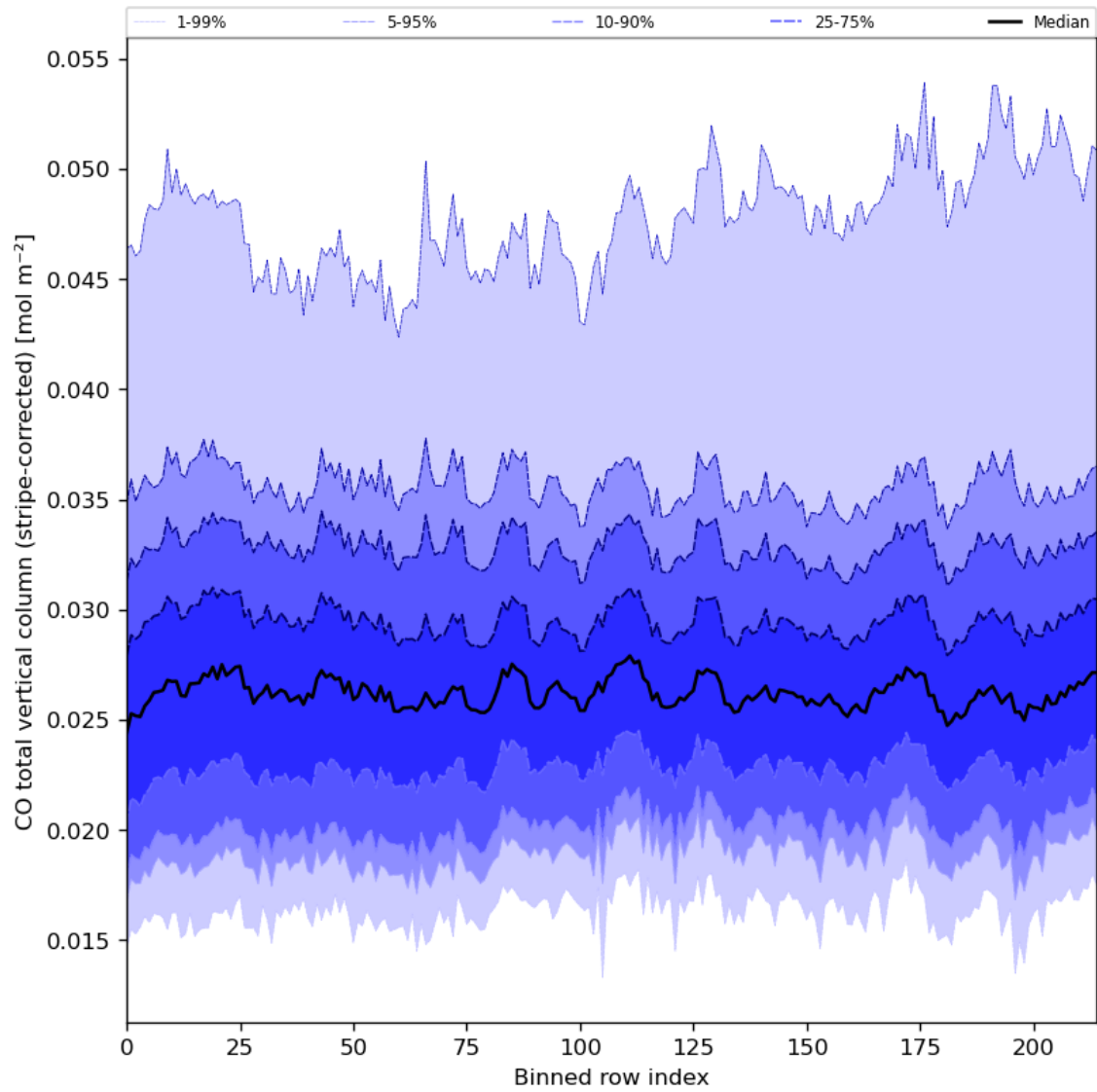
Figure 27: Along track statistics of “CO total vertical column (stripe-corrected)” for 2024-06-27 to 2024-06-29
