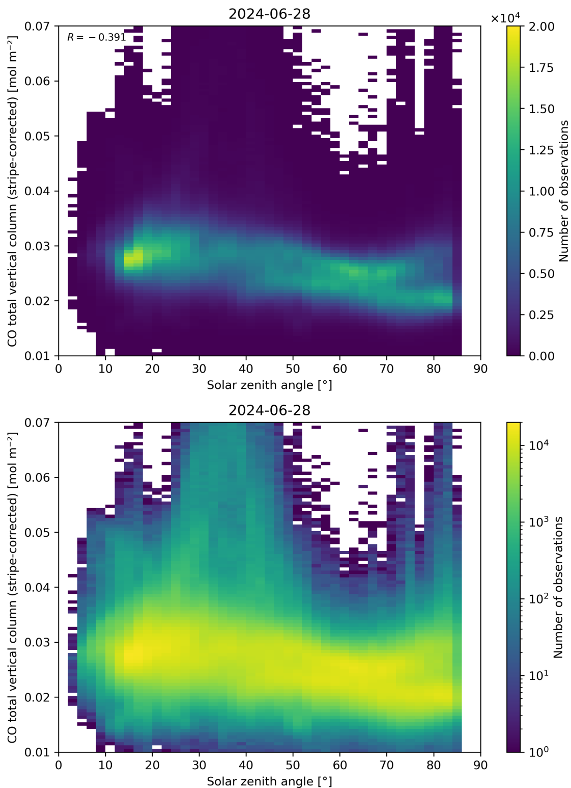
Figure 62: Scatter density plot of “Solar zenith angle” against “CO total vertical column (stripe-corrected)” for 2024-06-27 to 2024-06-29.
