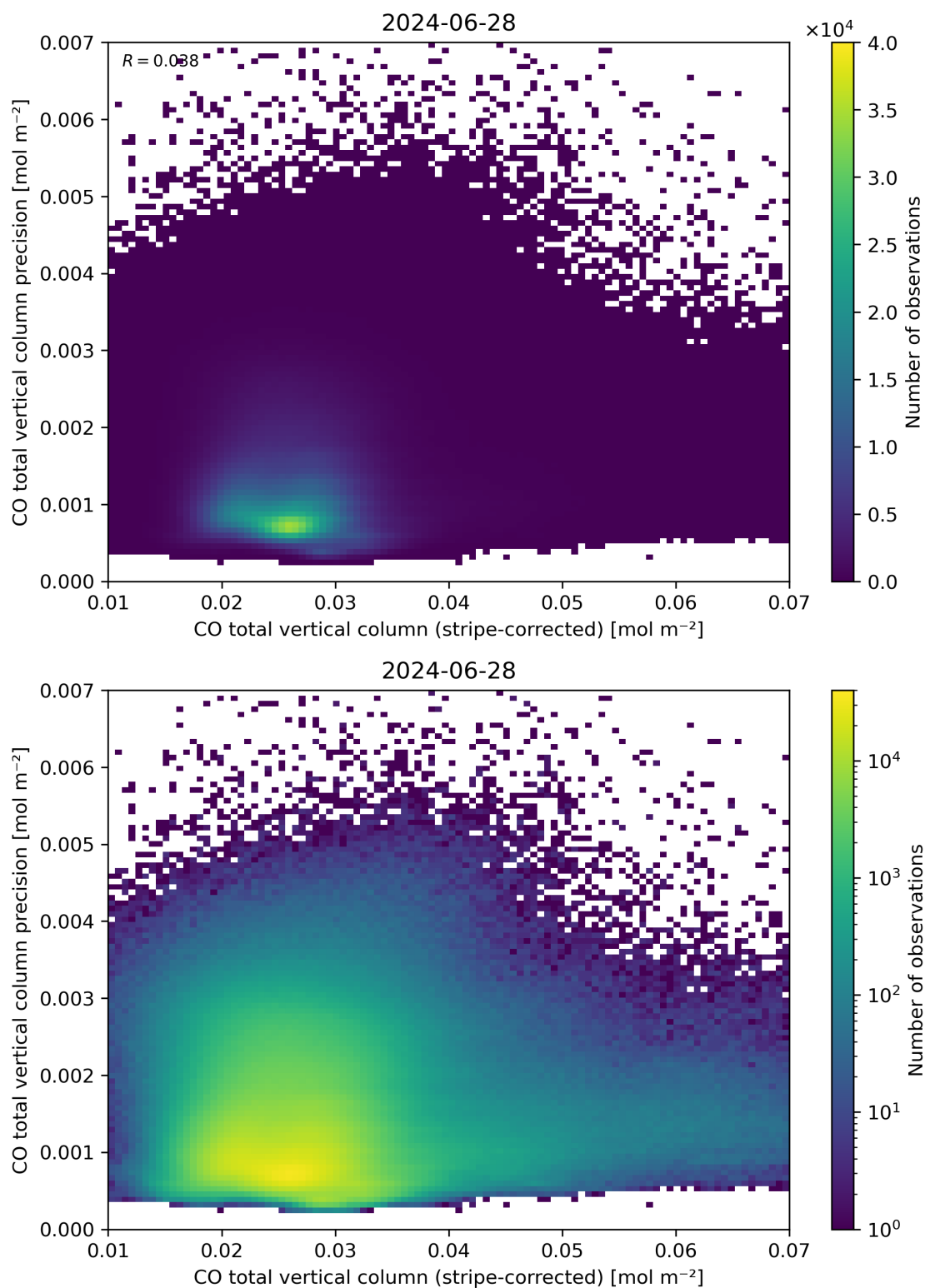
Figure 36: Scatter density plot of “CO total vertical column (stripe-corrected)” against “CO total vertical column precision” for 2024-06-27 to 2024-06-29.
