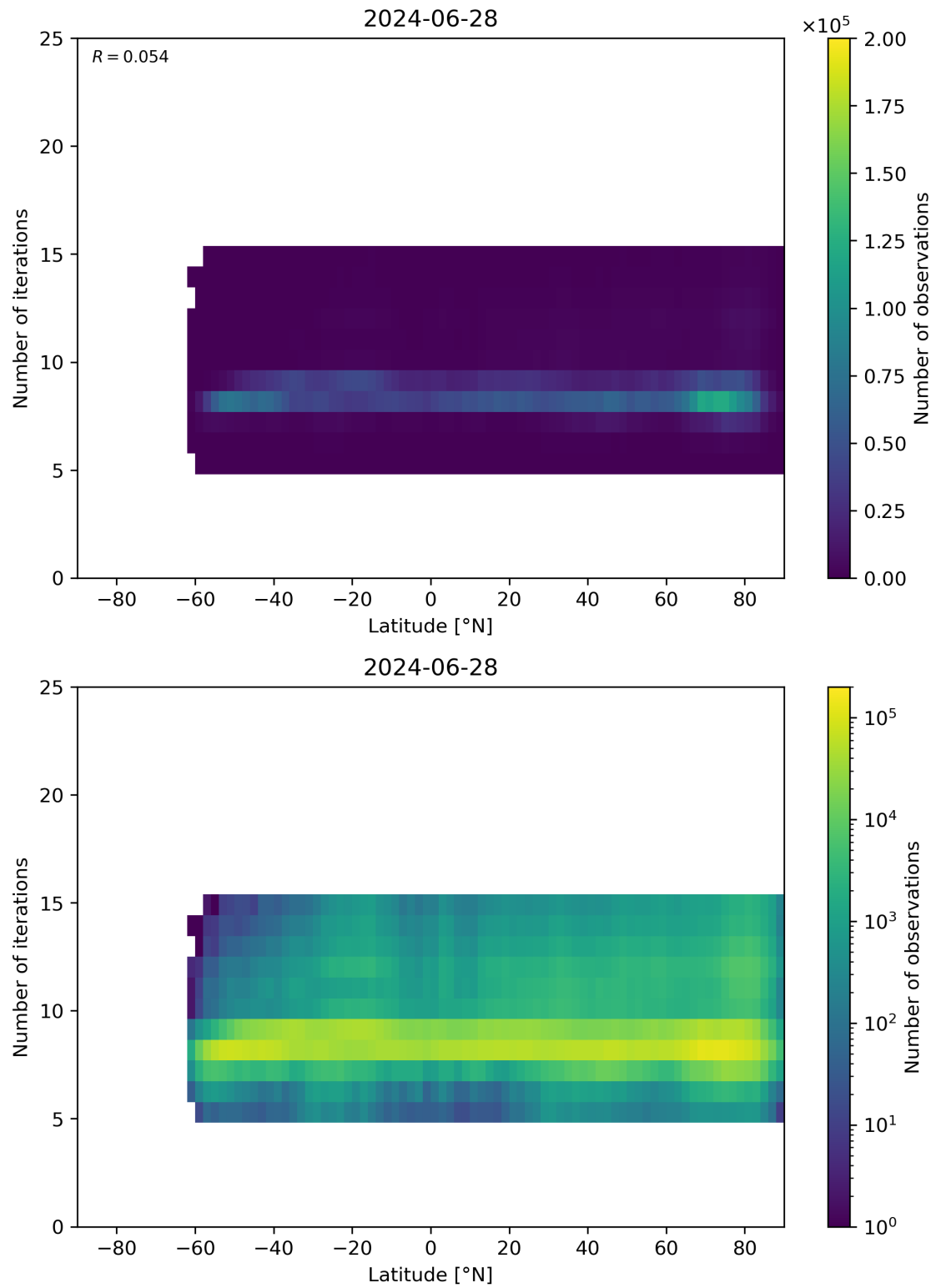
Figure 56: Scatter density plot of “Latitude” against “Number of iterations” for 2024-06-27 to 2024-06-29.
