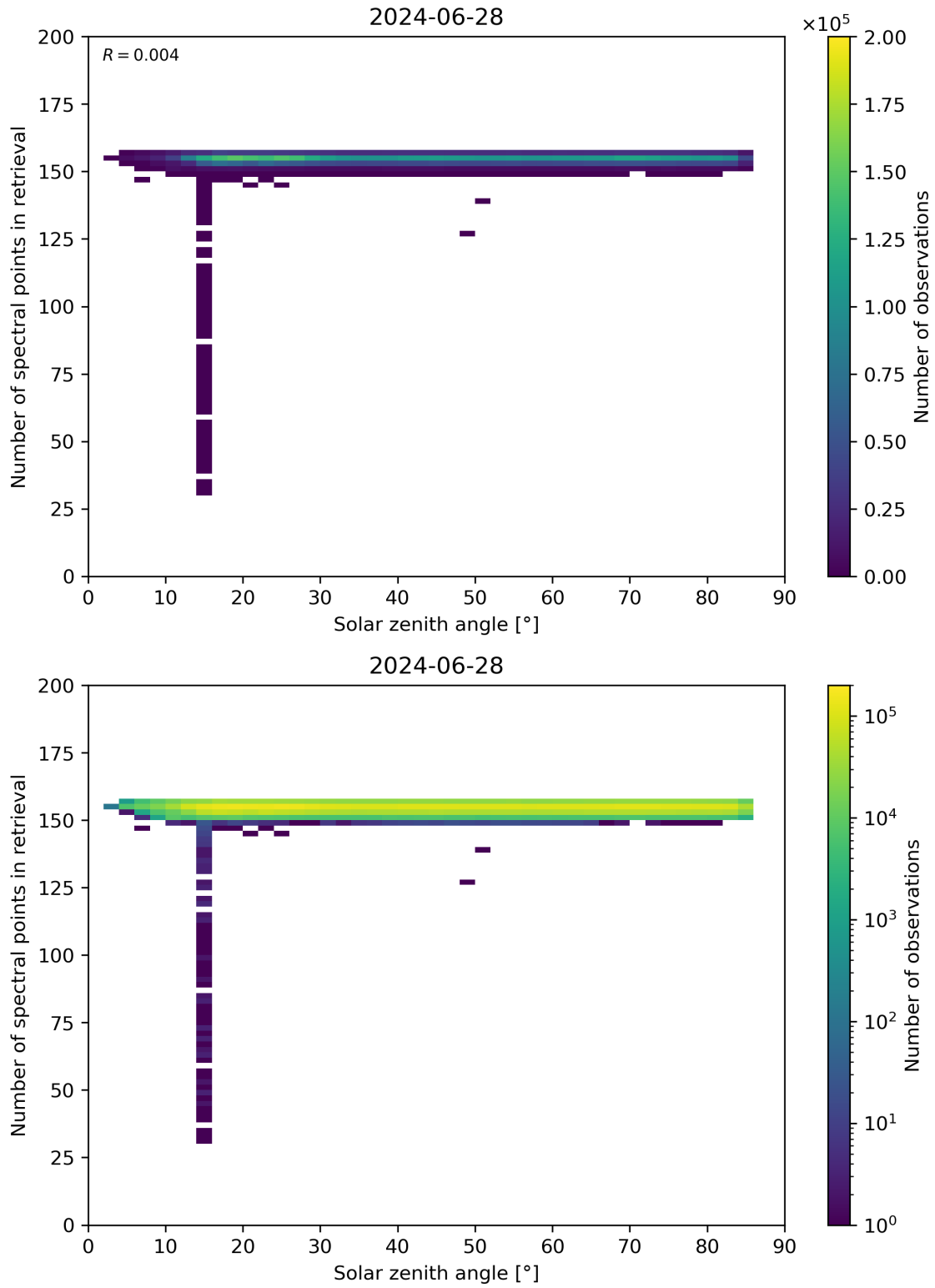
Figure 68: Scatter density plot of “Solar zenith angle” against “Number of spectral points in retrieval” for 2024-06-27 to 2024-06-29.
