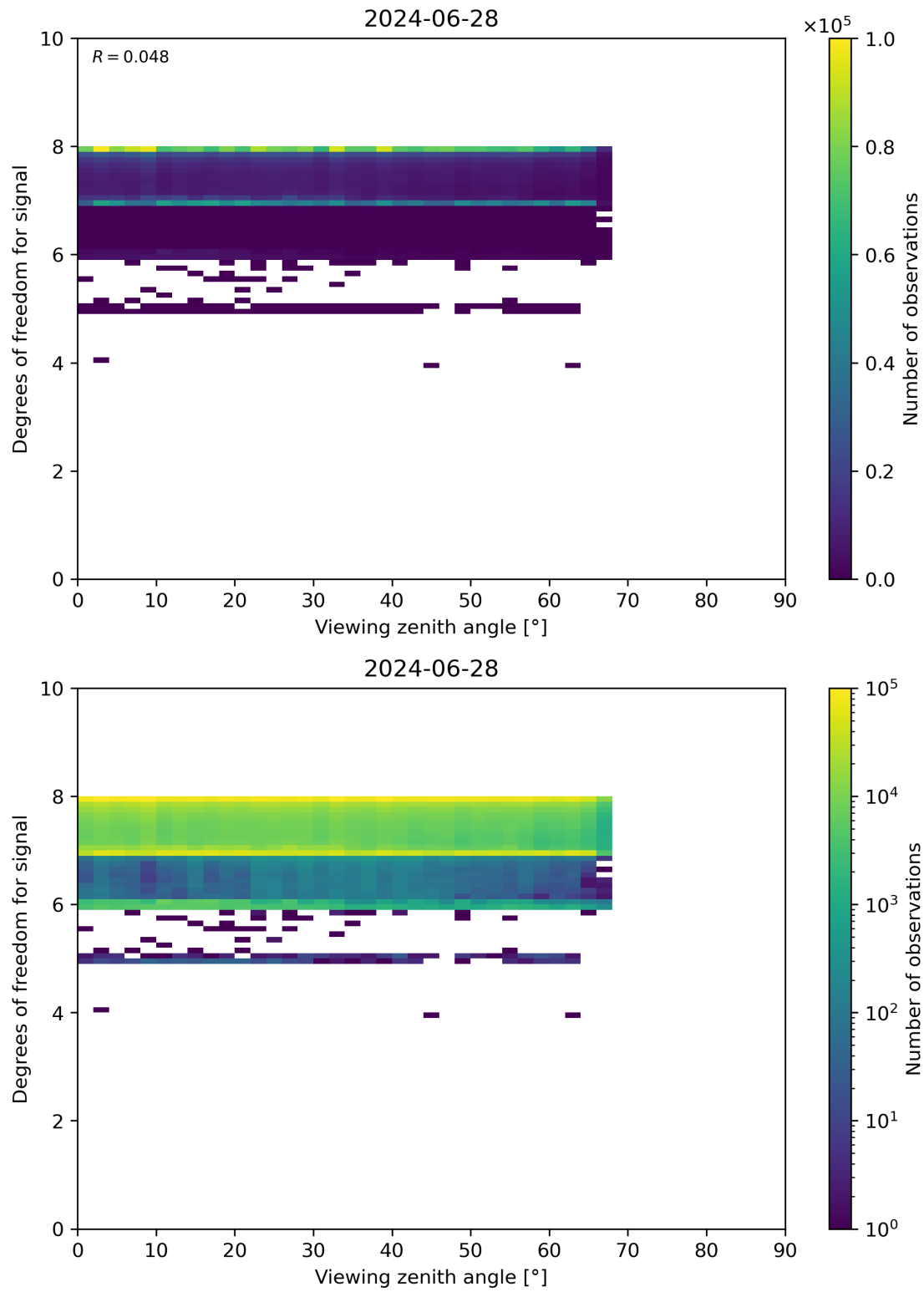
Figure 73: Scatter density plot of “Viewing zenith angle” against “Degrees of freedom for signal” for 2024-06-27 to 2024-06-29.
