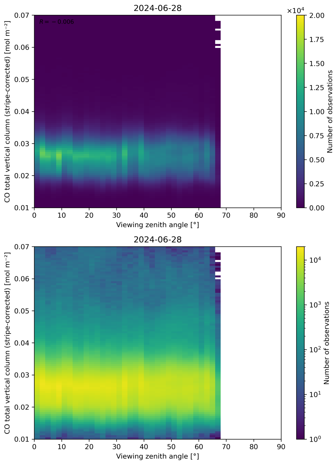
Figure 70: Scatter density plot of “Viewing zenith angle” against “CO total vertical column (stripe-corrected)” for 2024-06-27 to 2024-06-29.
