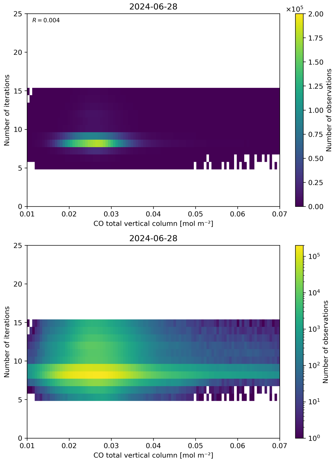
Figure 42: Scatter density plot of “CO total vertical column” against “Number of iterations” for 2024-06-27 to 2024-06-29.
