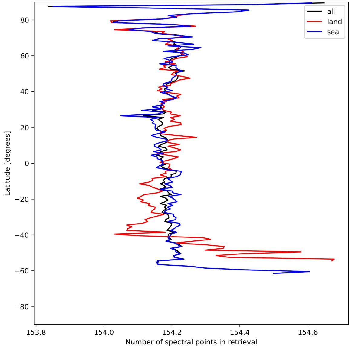
Figure 13: Zonal average of “Number of spectral points in retrieval” for 2024-06-27 to 2024-06-29.
