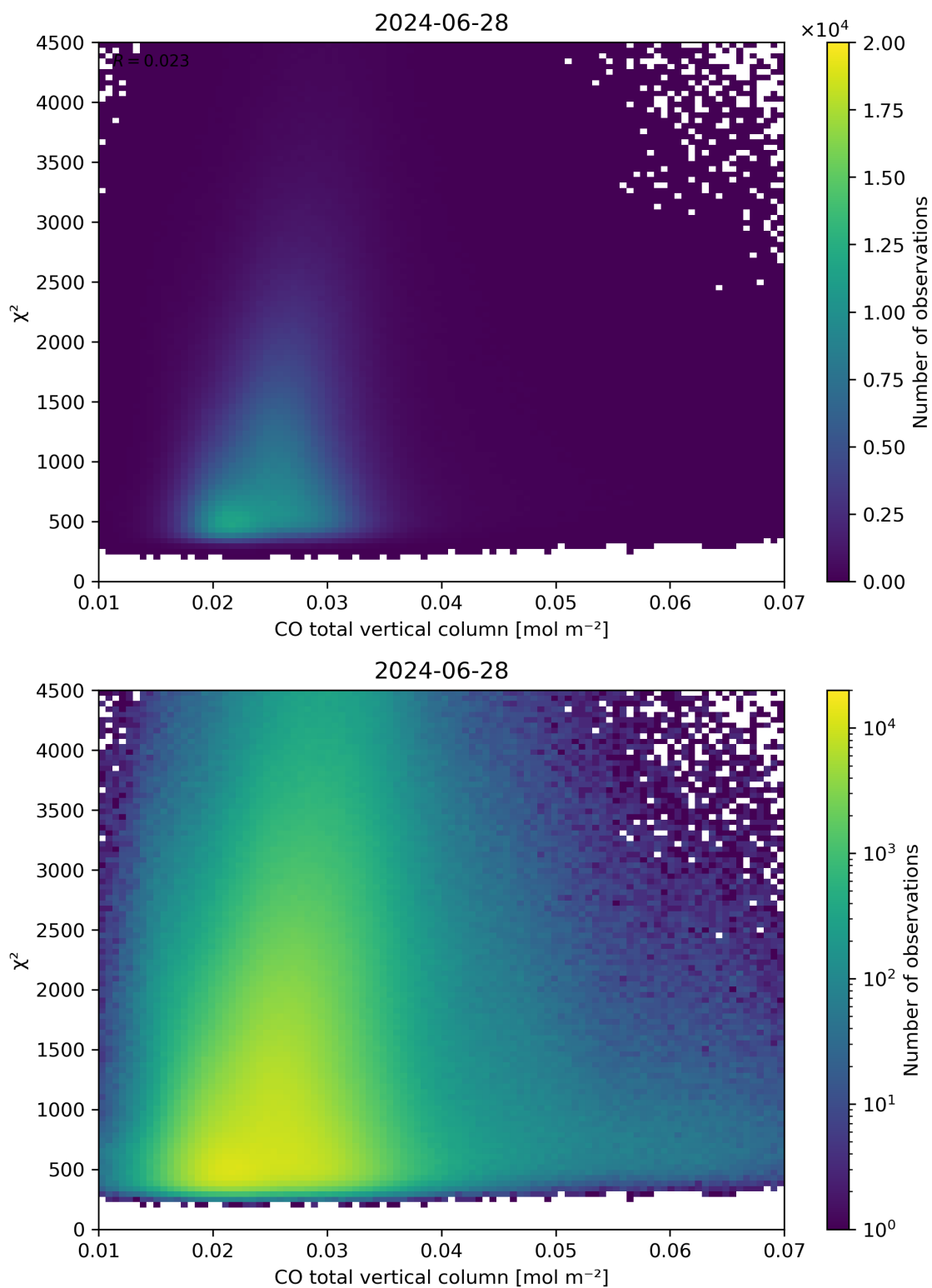
Figure 35: Scatter density plot of “CO total vertical column” against “ \chi^2 ” for 2024-06-27 to 2024-06-29.
