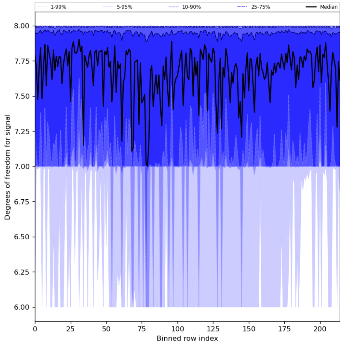
Figure 31: Along track statistics of “Degrees of freedom for signal” for 2024-06-27 to 2024-06-29
