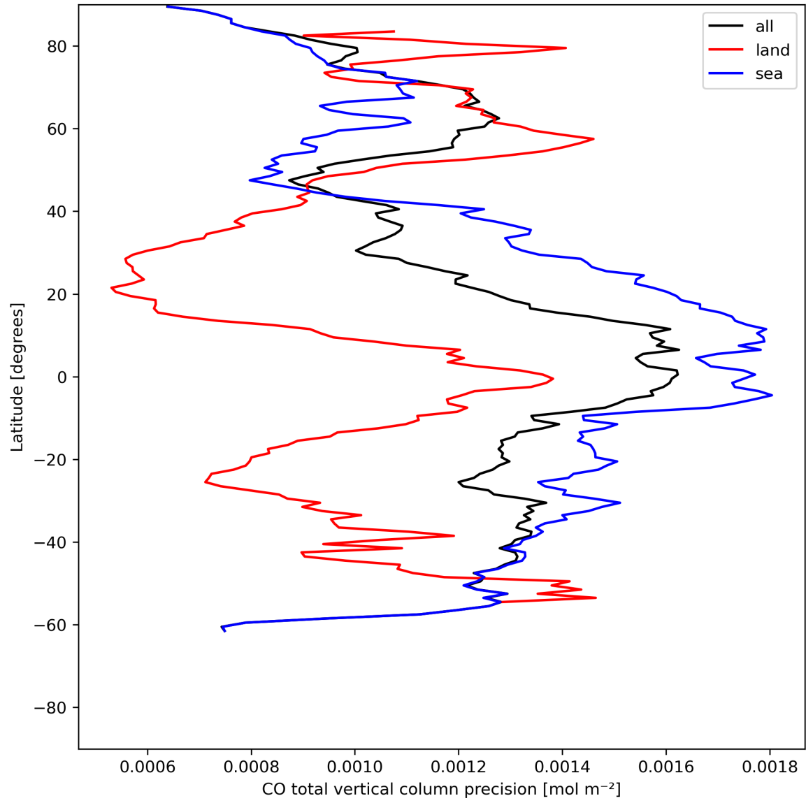
Figure 12: Zonal average of “CO total vertical column precision” for 2024-06-27 to 2024-06-29.
