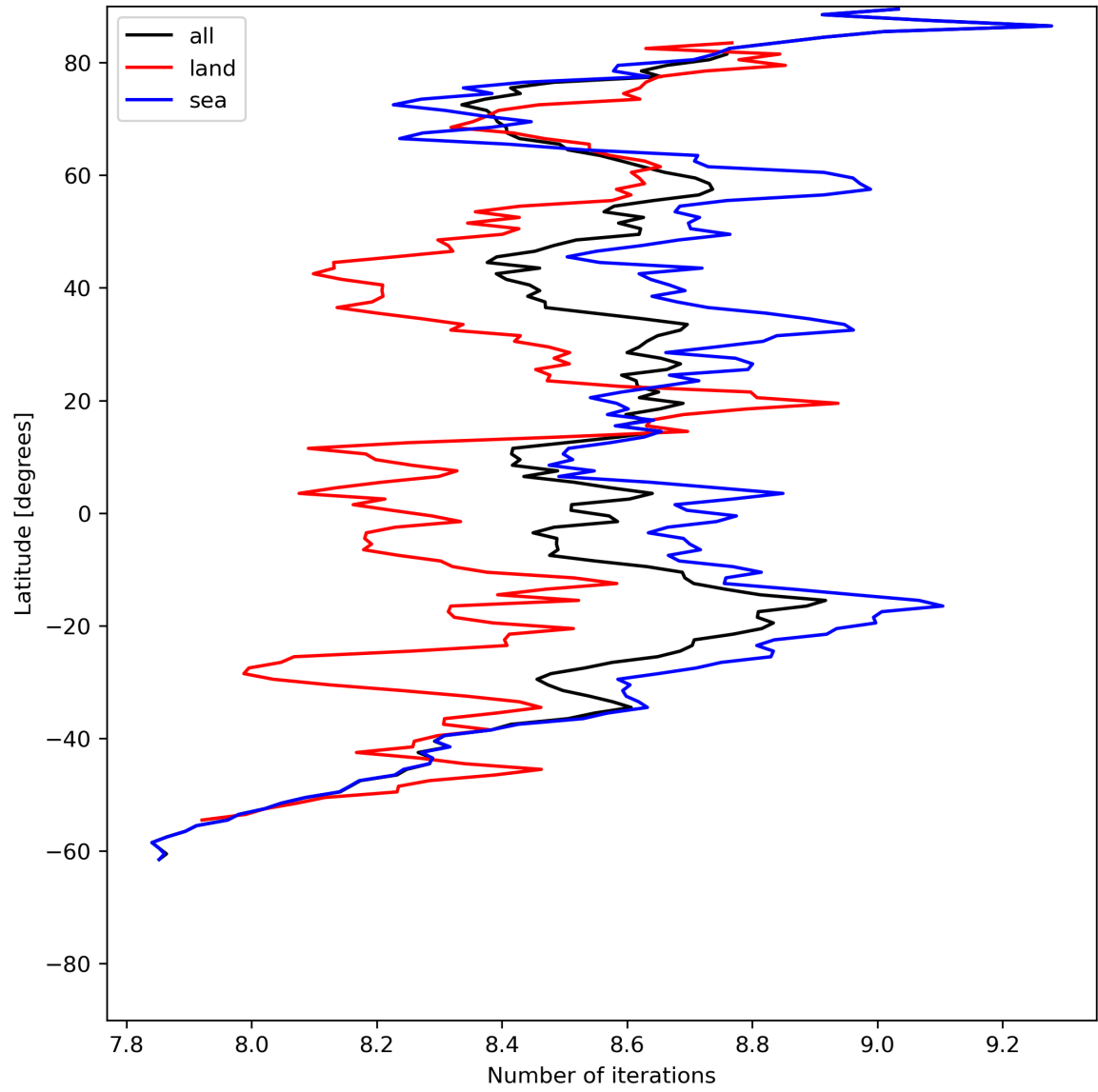
Figure 16: Zonal average of “Number of iterations” for 2024-06-27 to 2024-06-29.
