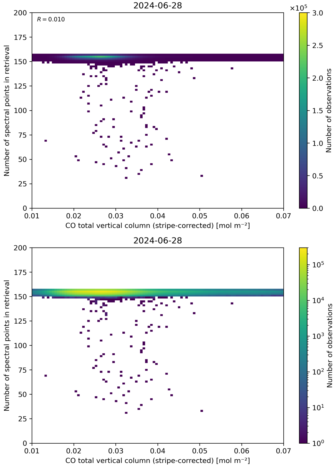
Figure 40: Scatter density plot of “CO total vertical column (stripe-corrected)” against “Number of spectral points in retrieval” for 2024-06-27 to 2024-06-29.
