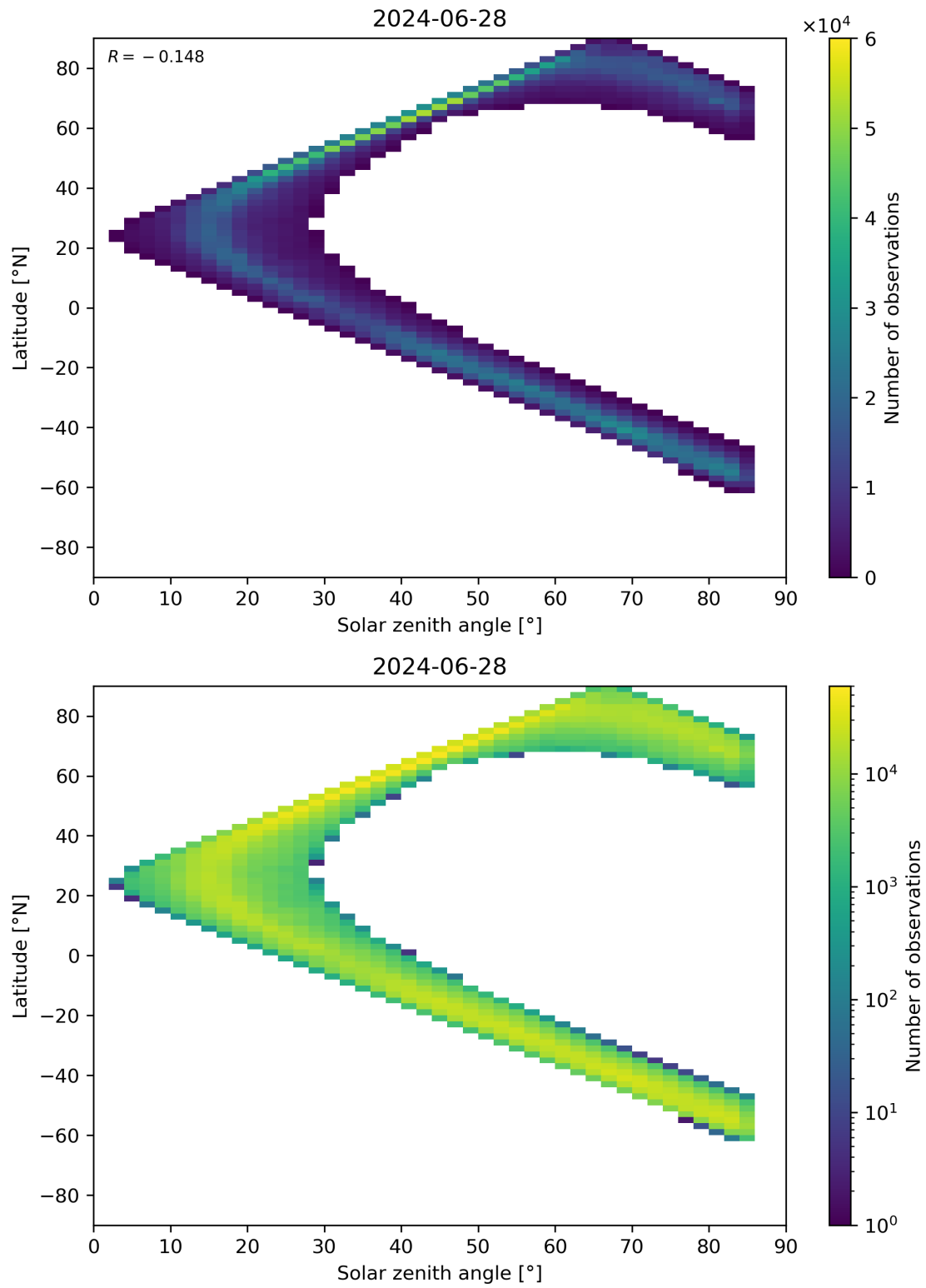
Figure 66: Scatter density plot of “Solar zenith angle” against “Latitude” for 2024-06-27 to 2024-06-29.
