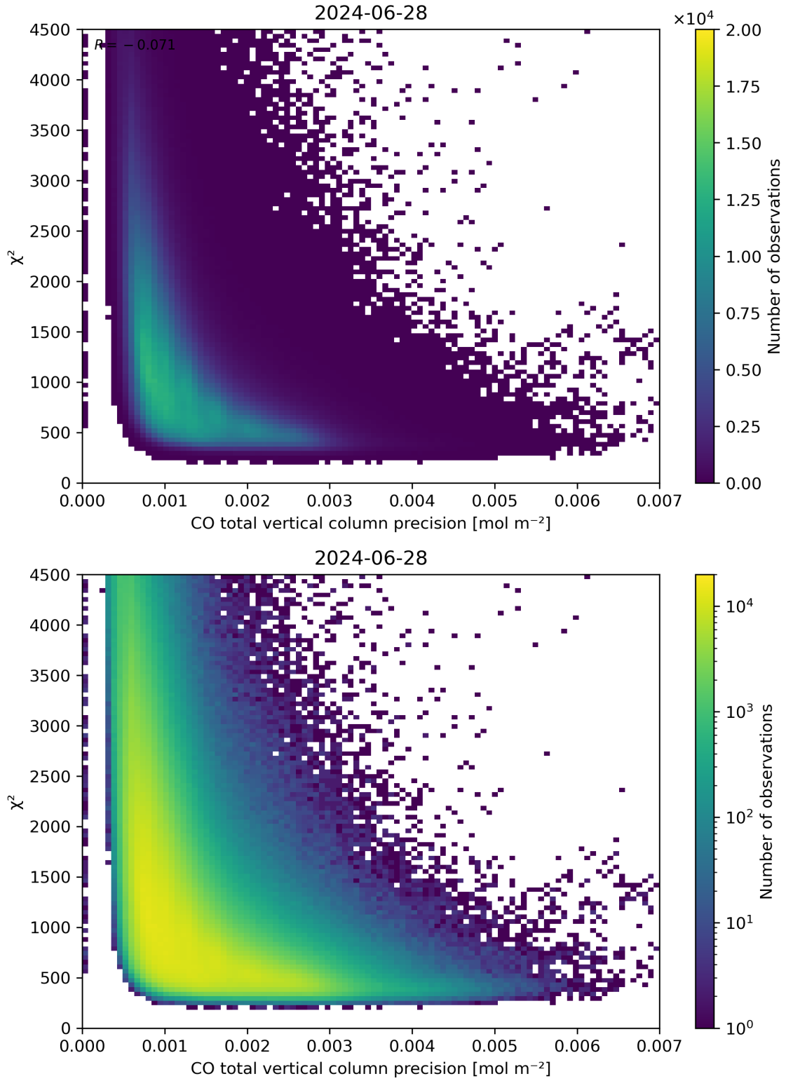
Figure 44: Scatter density plot of “CO total vertical column precision” against “ \chi^2 ” for 2024-06-27 to 2024-06-29.
