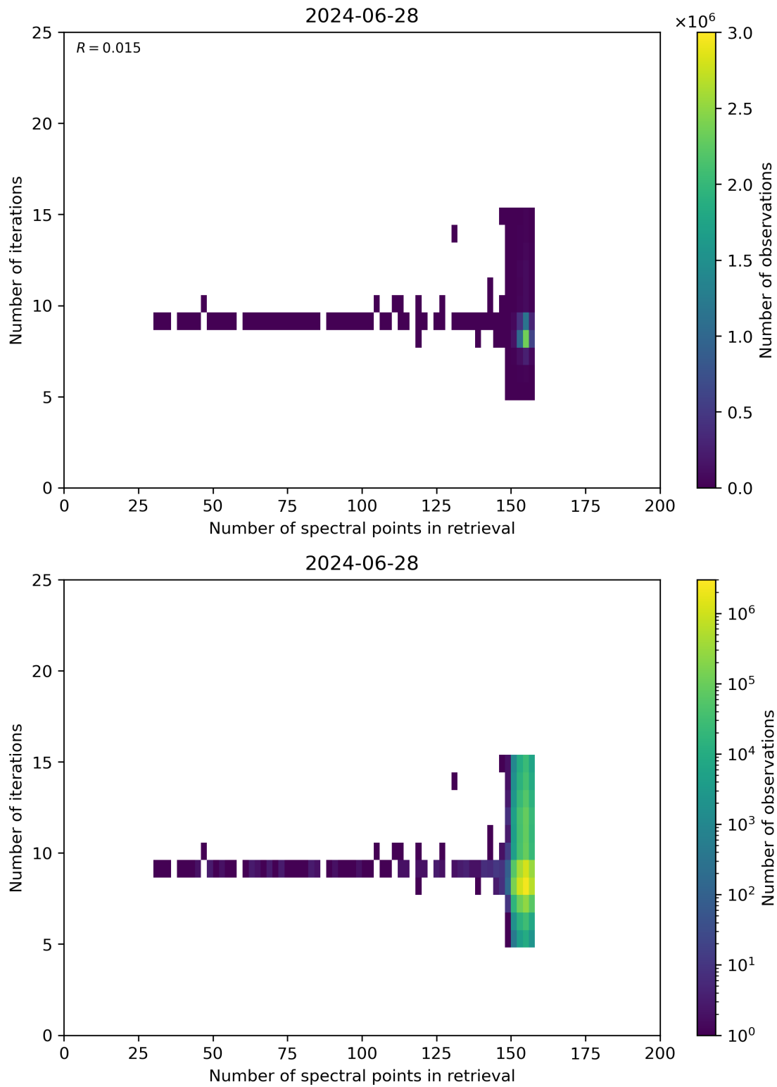
Figure 60: Scatter density plot of “Number of spectral points in retrieval” against “Number of iterations” for 2024-06-27 to 2024-06-29.
