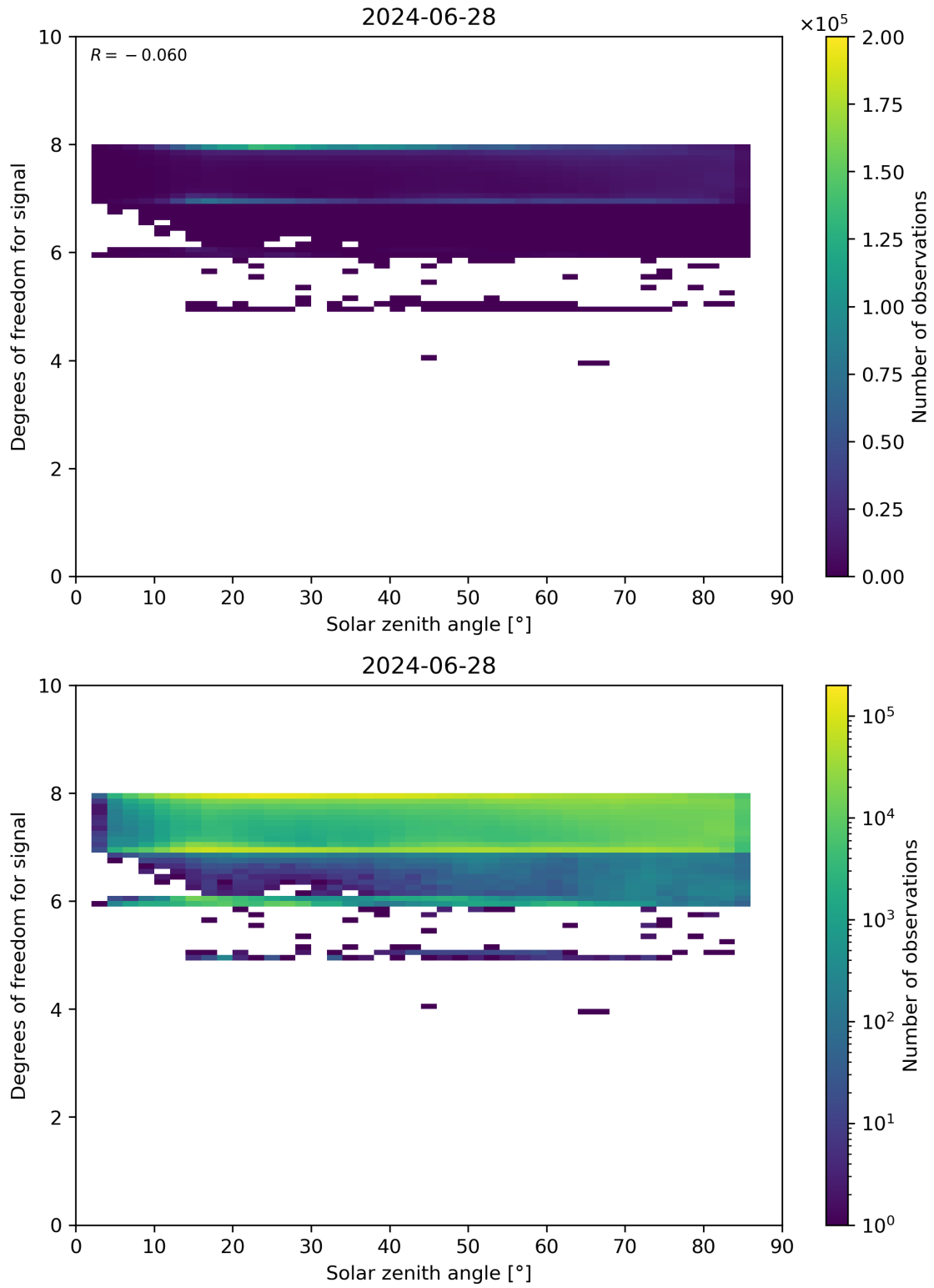
Figure 65: Scatter density plot of “Solar zenith angle” against “Degrees of freedom for signal” for 2024-06-27 to 2024-06-29.
