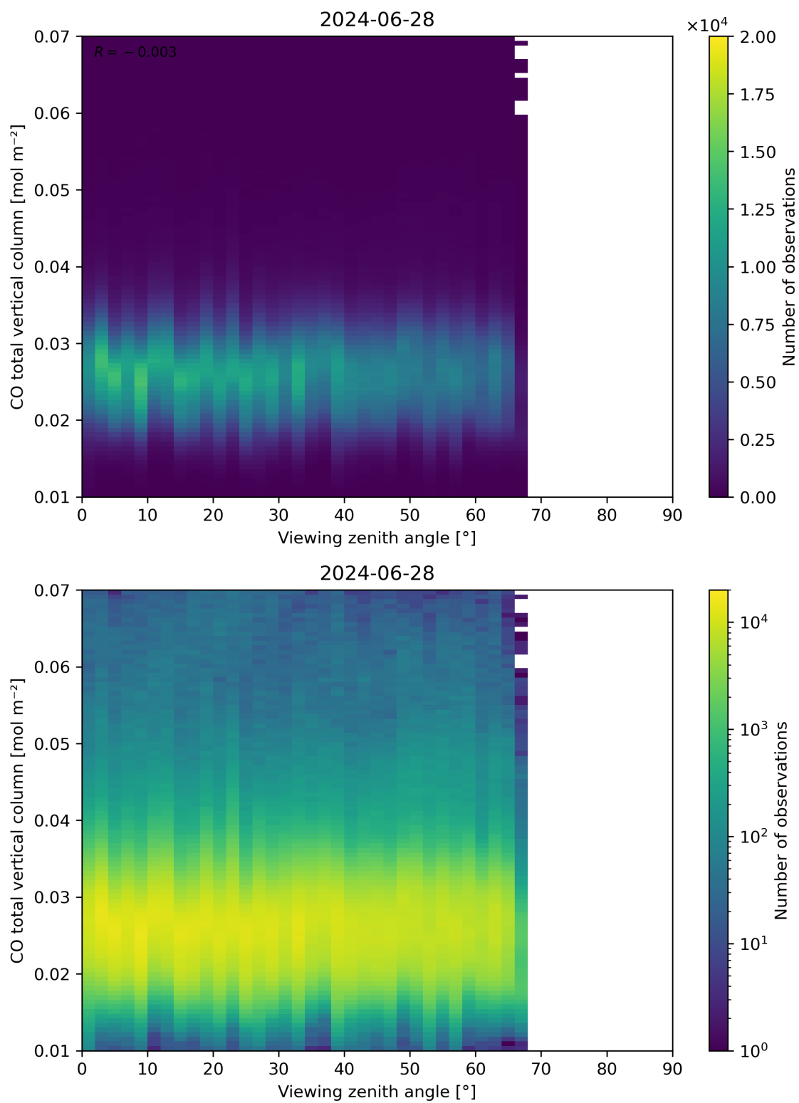
Figure 69: Scatter density plot of “Viewing zenith angle” against “CO total vertical column” for 2024-06-27 to 2024-06-29.
