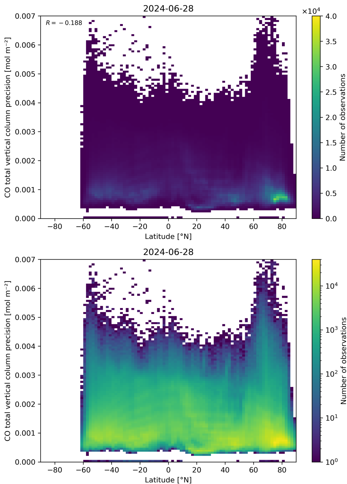
Figure 53: Scatter density plot of “Latitude” against “CO total vertical column precision” for 2024-06-27 to 2024-06-29.
