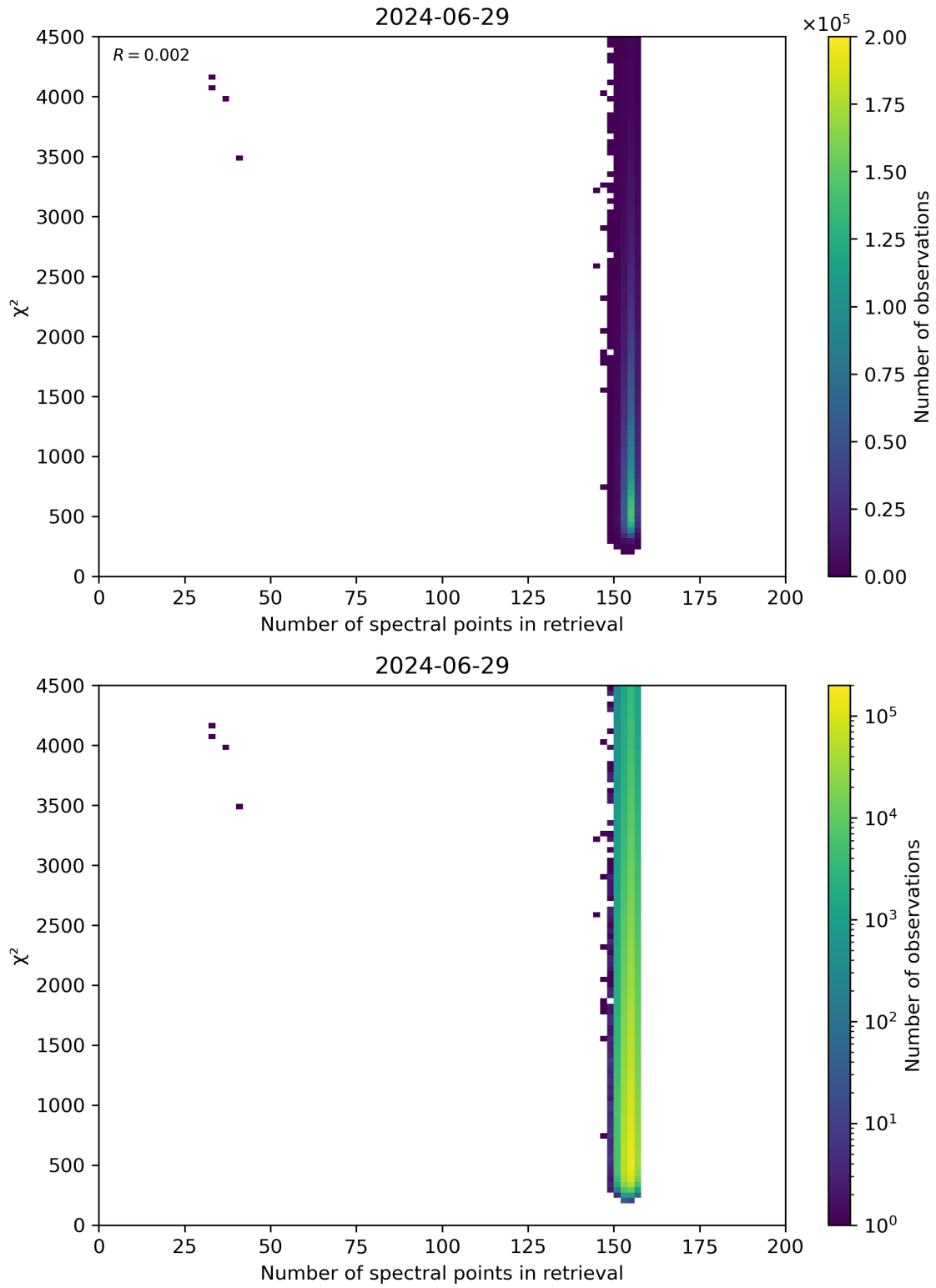
Figure 58: Scatter density plot of “Number of spectral points in retrieval” against “ \chi^2 ” for 2024-06-29 to 2024-06-30.
