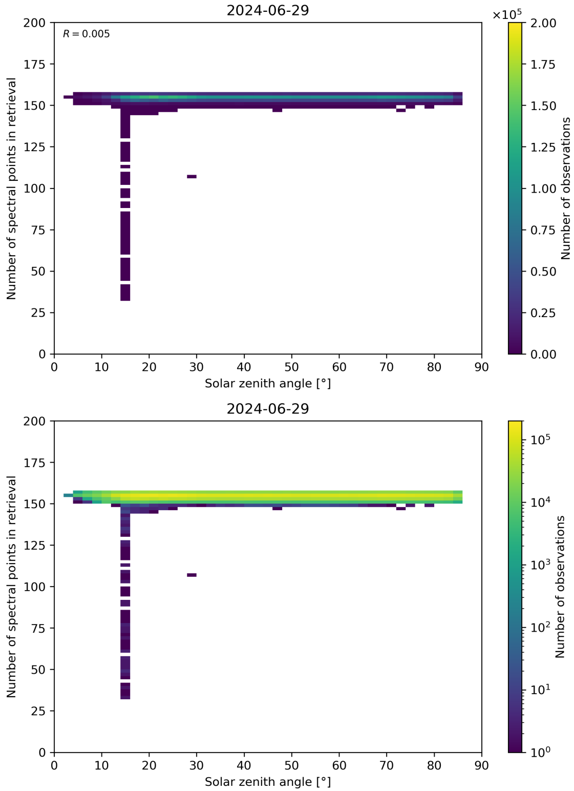
Figure 68: Scatter density plot of “Solar zenith angle” against “Number of spectral points in retrieval” for 2024-06-29 to 2024-06-30.
