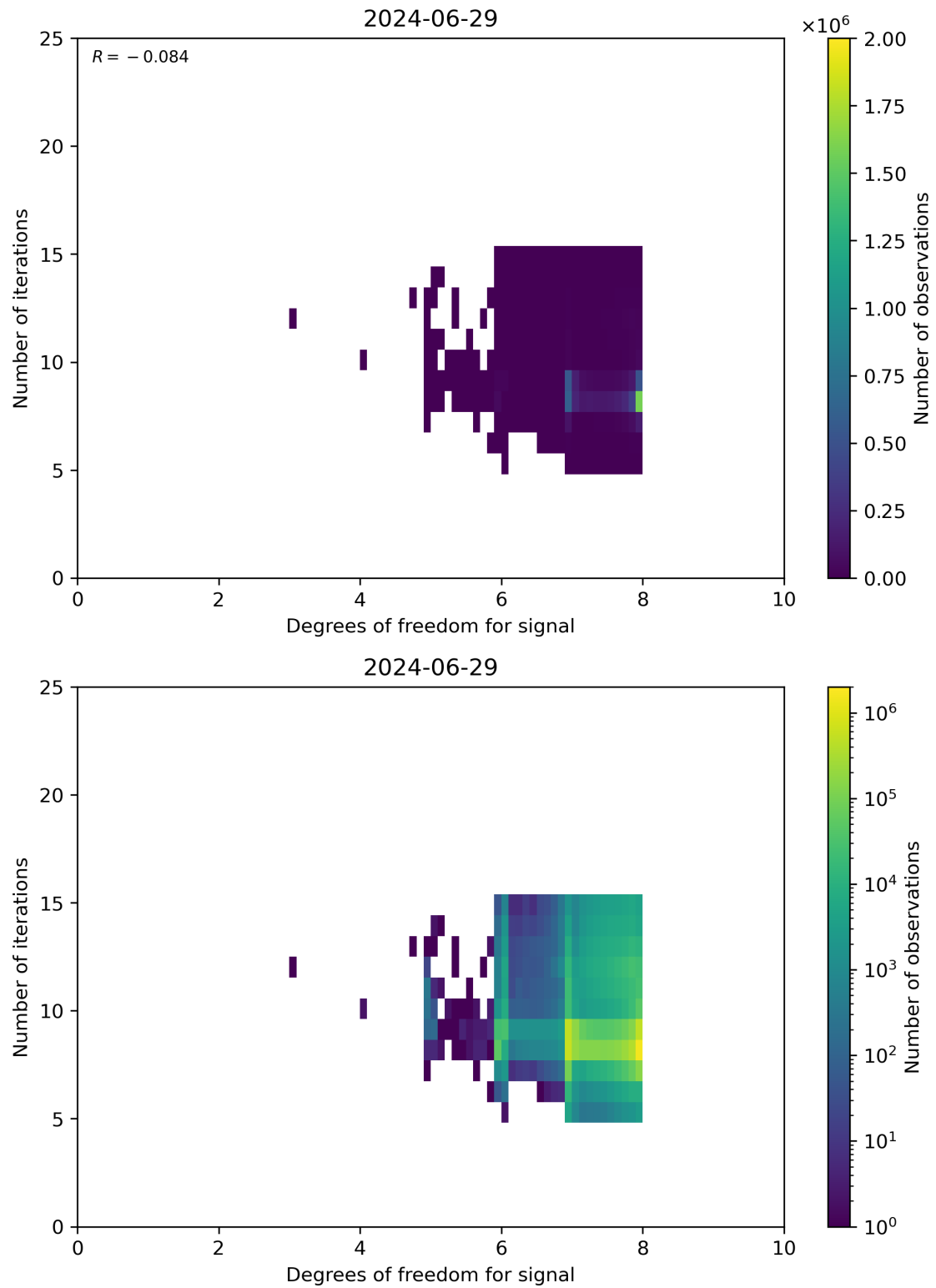
Figure 50: Scatter density plot of “Degrees of freedom for signal” against “Number of iterations” for 2024-06-29 to 2024-06-30.
