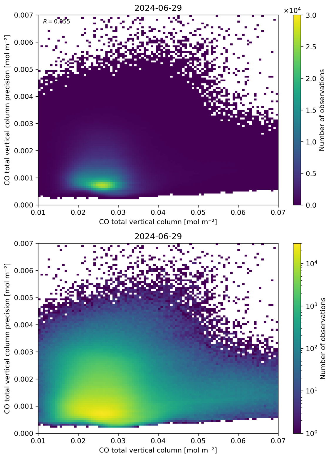
Figure 34: Scatter density plot of “CO total vertical column” against “CO total vertical column precision” for 2024-06-29 to 2024-06-30.
