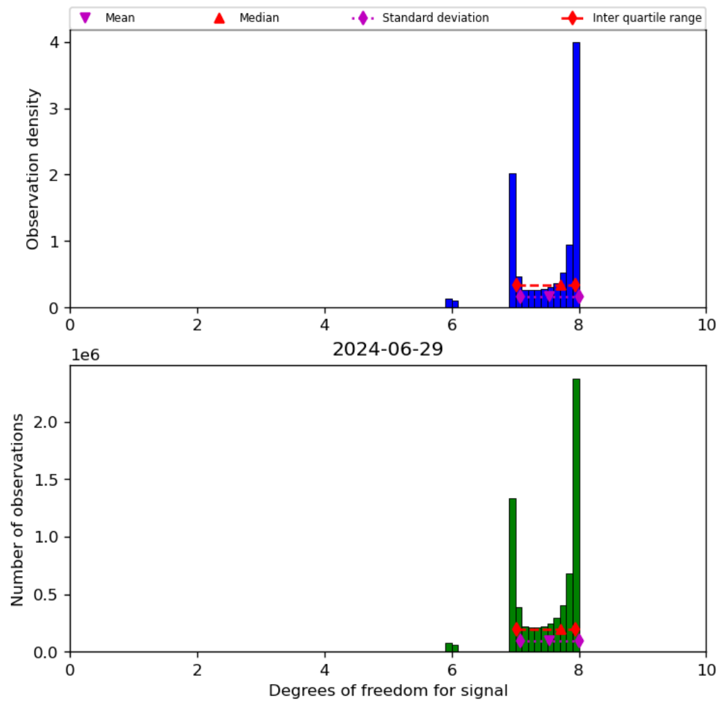
Figure 23: Histogram of “Degrees of freedom for signal” for 2024-06-29 to 2024-06-30
