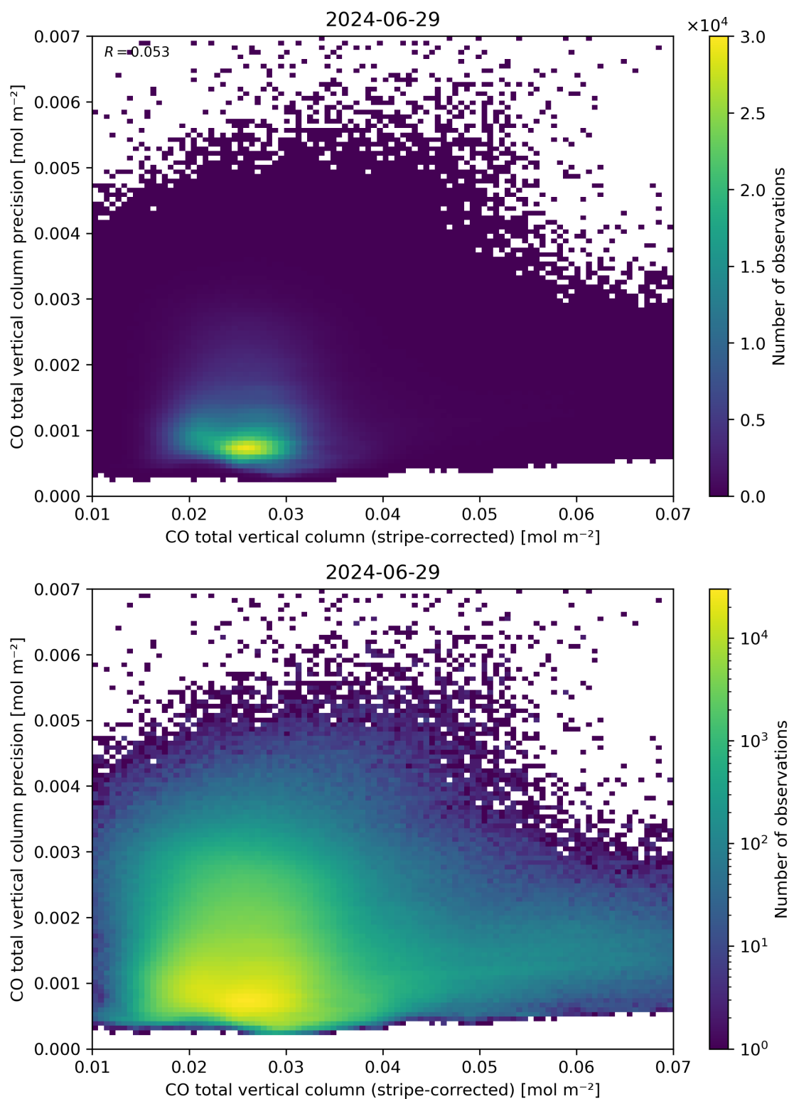
Figure 36: Scatter density plot of “CO total vertical column (stripe-corrected)” against “CO total vertical column precision” for 2024-06-29 to 2024-06-30.
