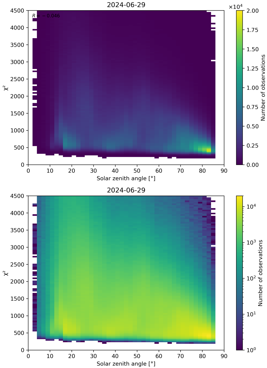
Figure 64: Scatter density plot of “Solar zenith angle” against “ \chi^2 ” for 2024-06-29 to 2024-06-30.
