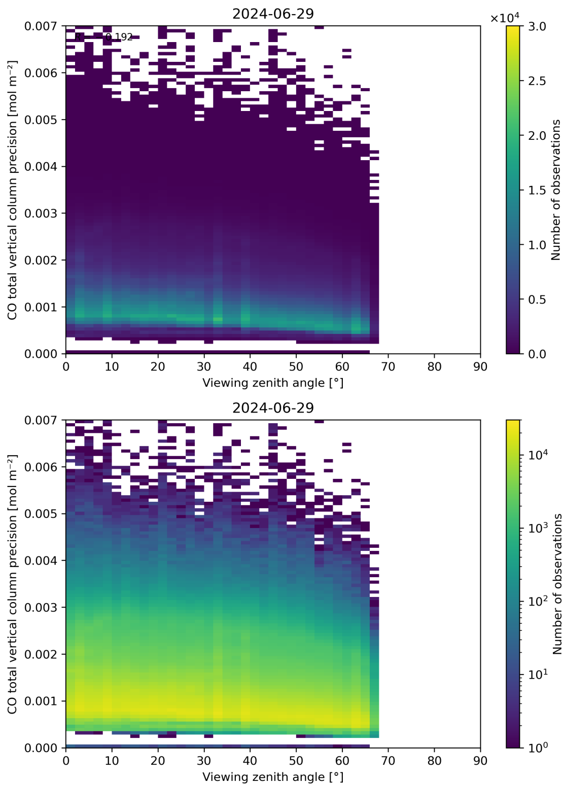
Figure 71: Scatter density plot of “Viewing zenith angle” against “CO total vertical column precision” for 2024-06-29 to 2024-06-30.
