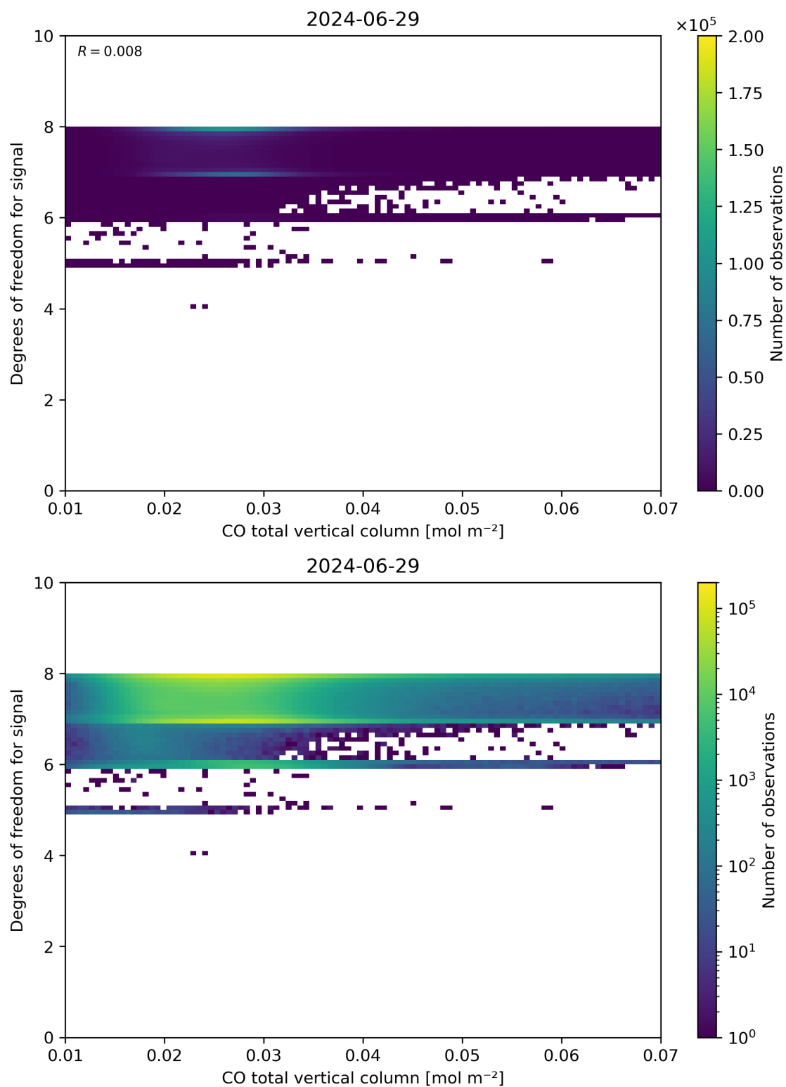
Figure 41: Scatter density plot of “CO total vertical column” against “Degrees of freedom for signal” for 2024-06-29 to 2024-06-30.
