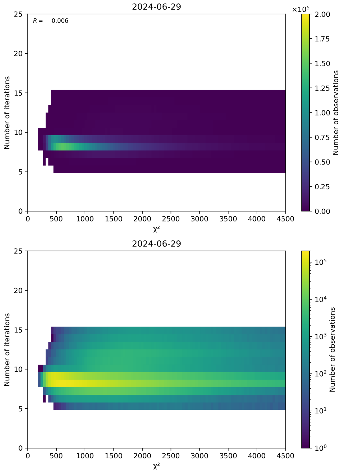
Figure 49: Scatter density plot of “ \chi^2 ” against “Number of iterations” for 2024-06-29 to 2024-06-30.
