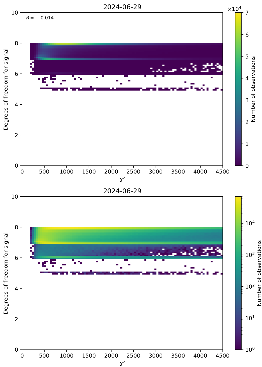
Figure 48: Scatter density plot of “ \chi^2 ” against “Degrees of freedom for signal” for 2024-06-29 to 2024-06-30.
