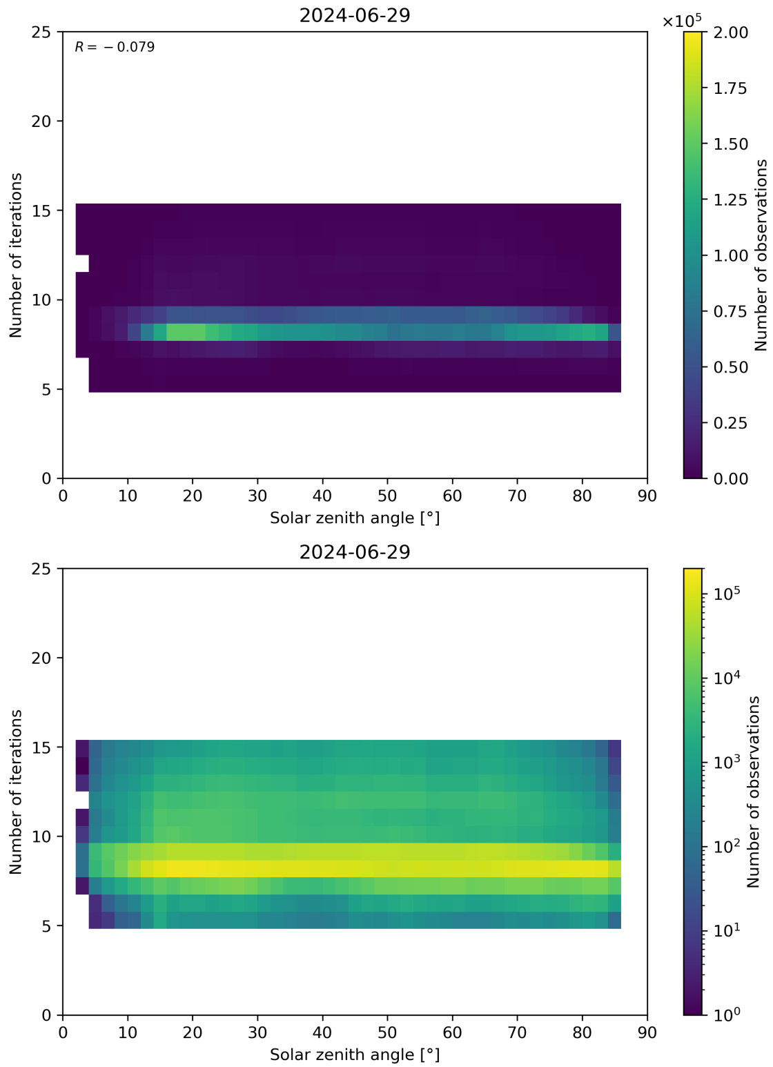
Figure 67: Scatter density plot of “Solar zenith angle” against “Number of iterations” for 2024-06-29 to 2024-06-30.
