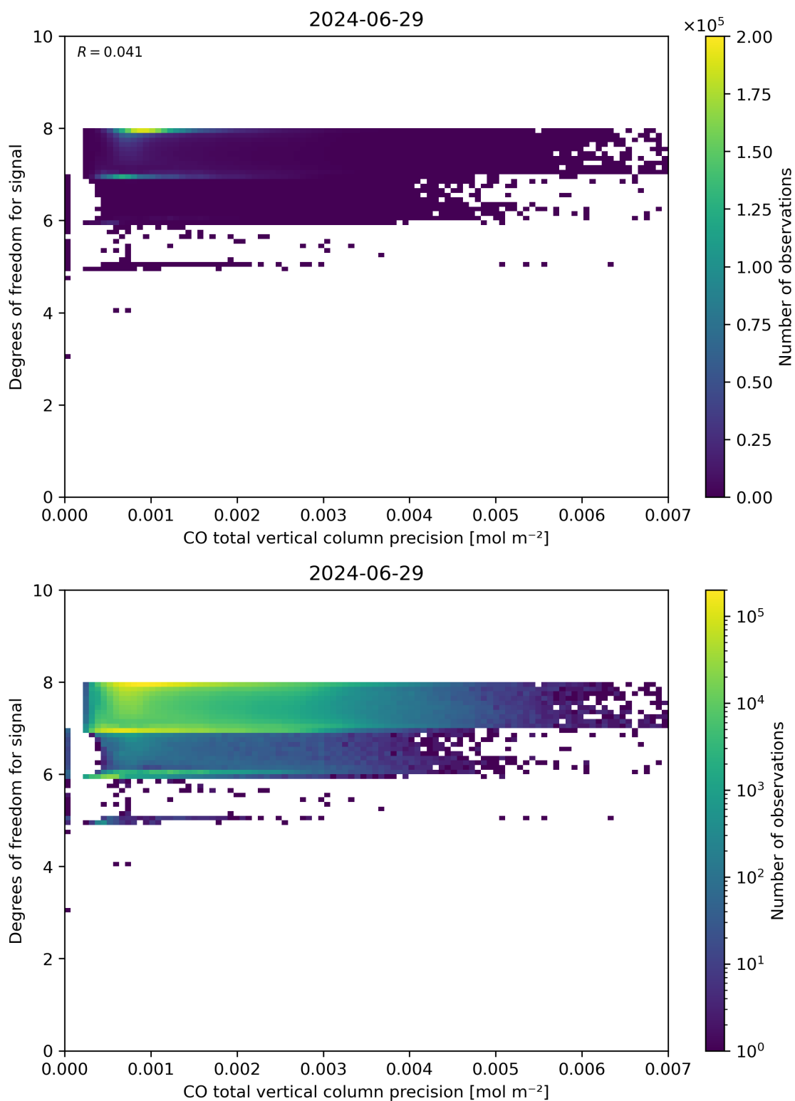
Figure 45: Scatter density plot of “CO total vertical column precision” against “Degrees of freedom for signal” for 2024-06-29 to 2024-06-30.
