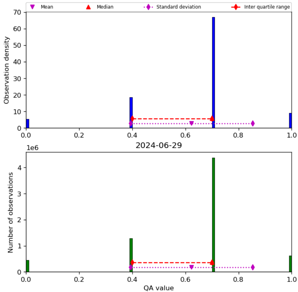
Figure 17: Histogram of “QA value” for 2024-06-29 to 2024-06-30
