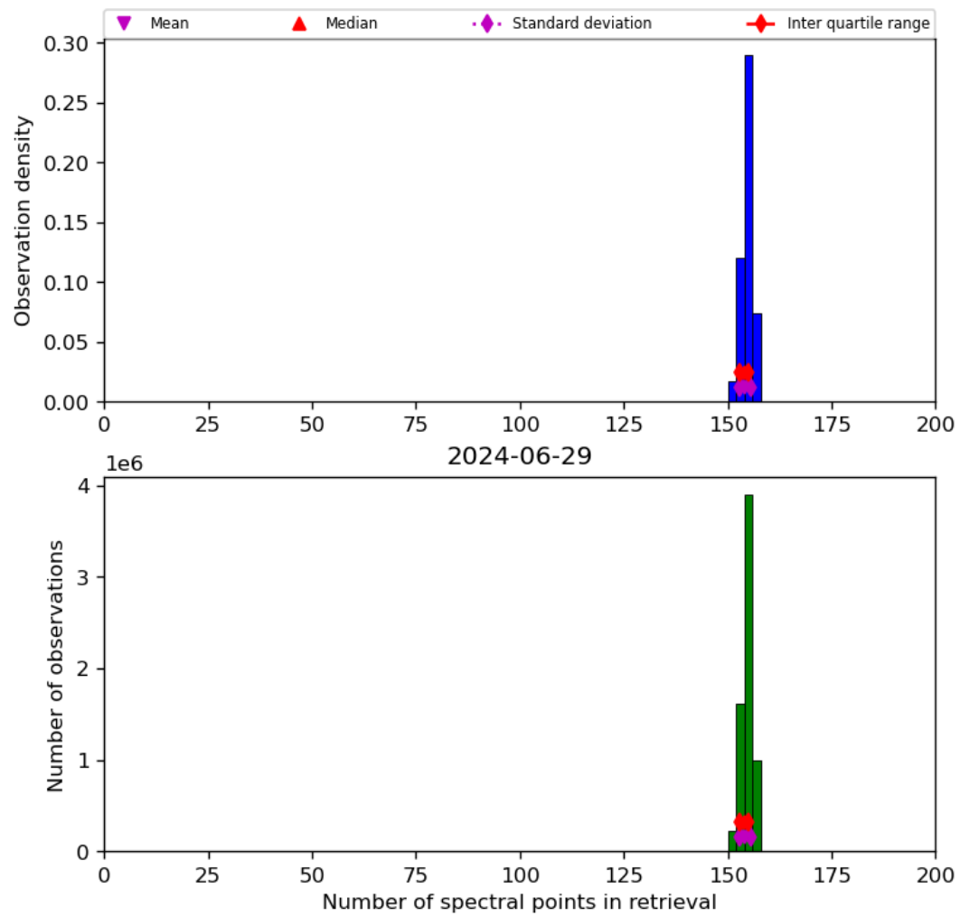
Figure 21: Histogram of “Number of spectral points in retrieval” for 2024-06-29 to 2024-06-30
