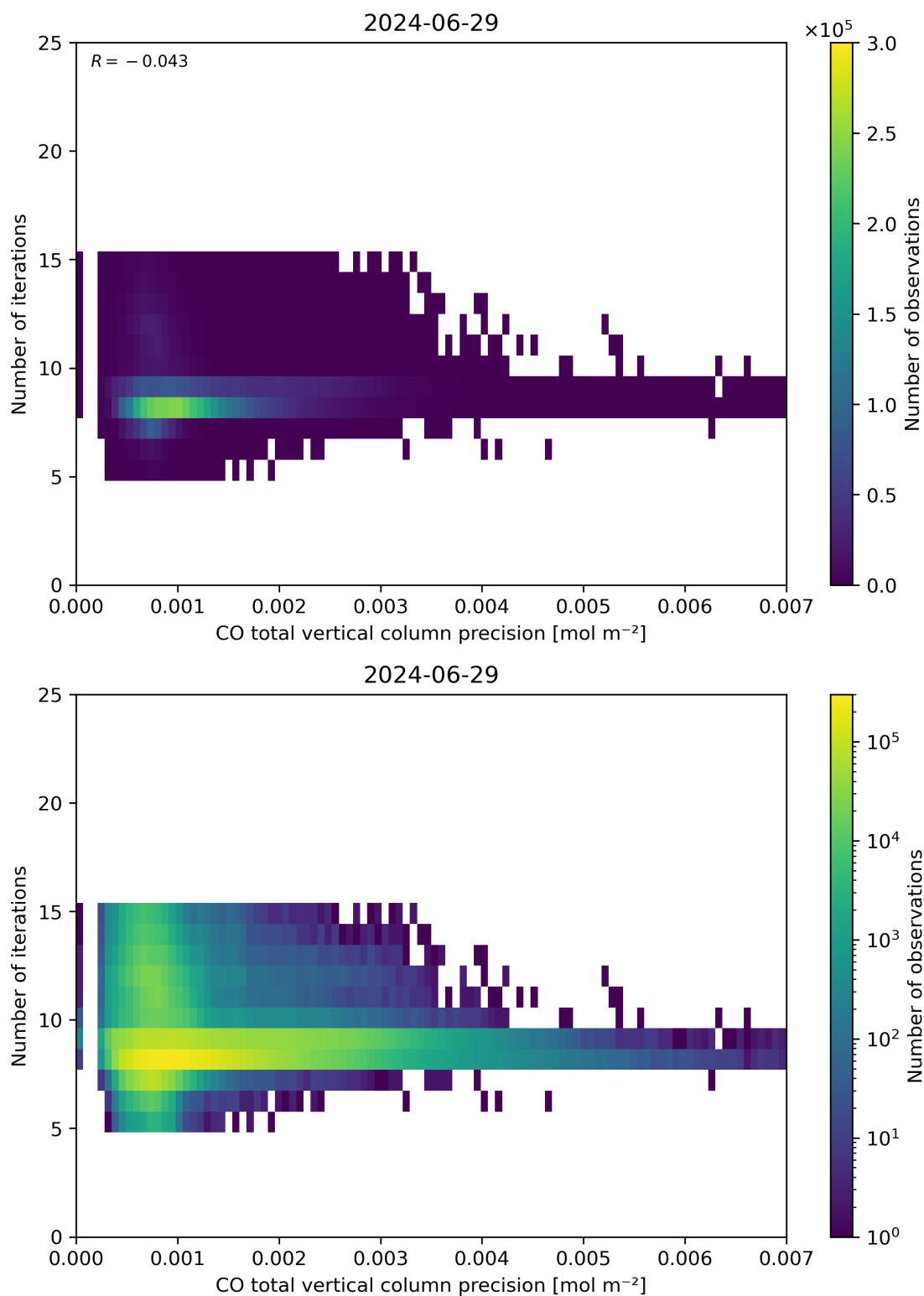
Figure 46: Scatter density plot of “CO total vertical column precision” against “Number of iterations” for 2024-06-29 to 2024-06-30.
