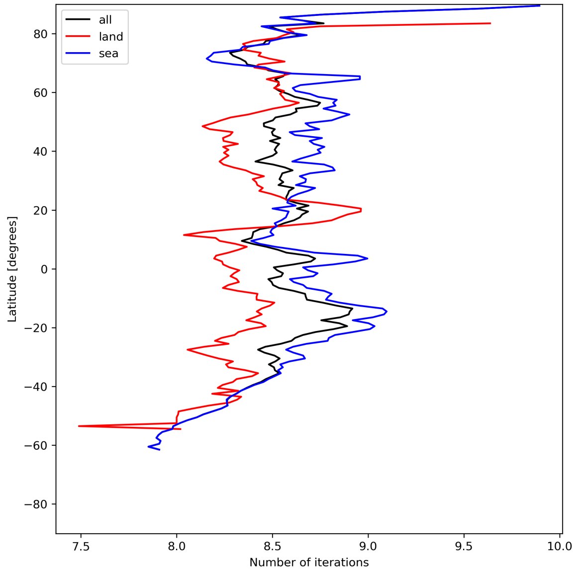
Figure 16: Zonal average of “Number of iterations” for 2024-06-29 to 2024-06-30.
