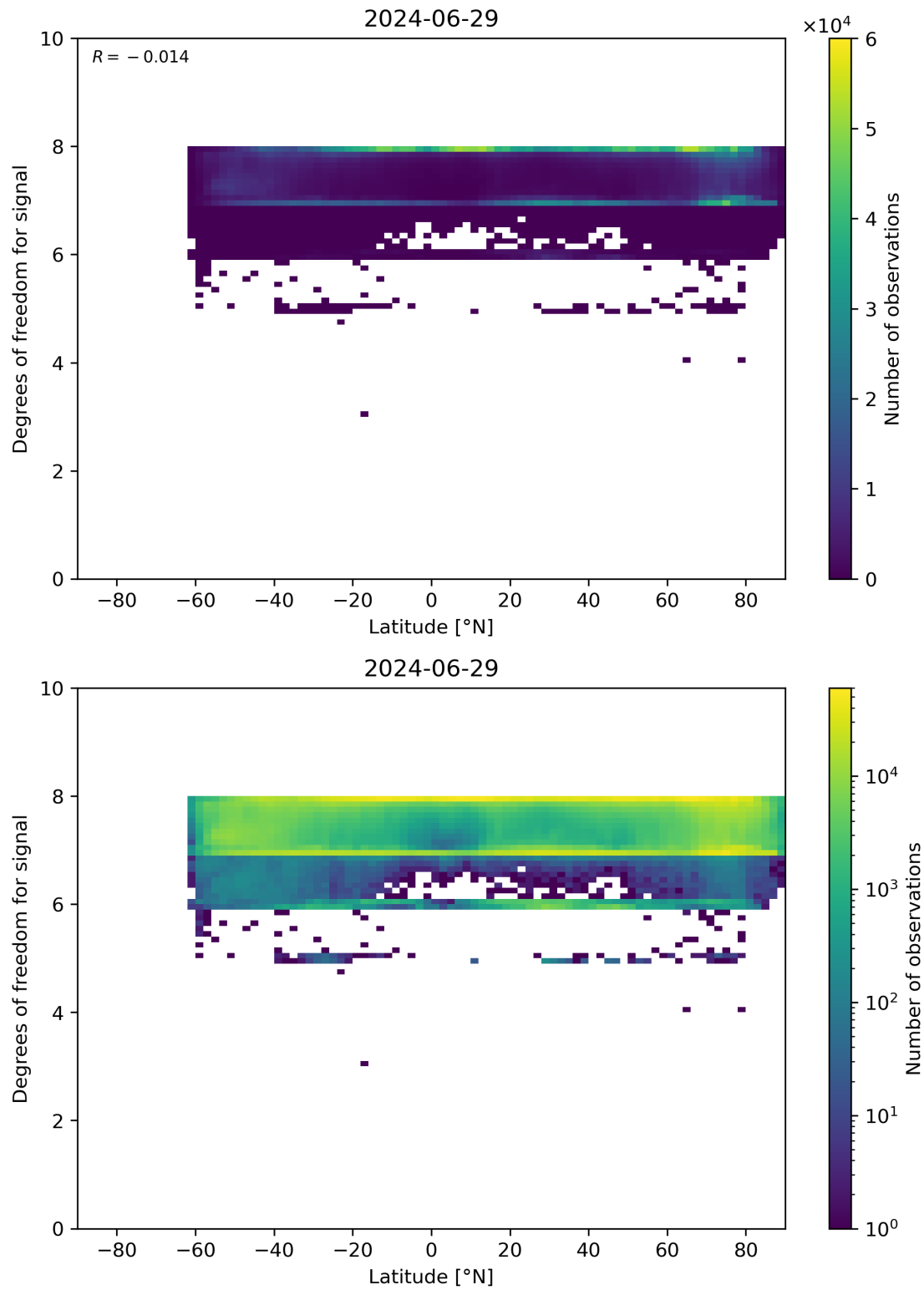
Figure 55: Scatter density plot of “Latitude” against “Degrees of freedom for signal” for 2024-06-29 to 2024-06-30.
