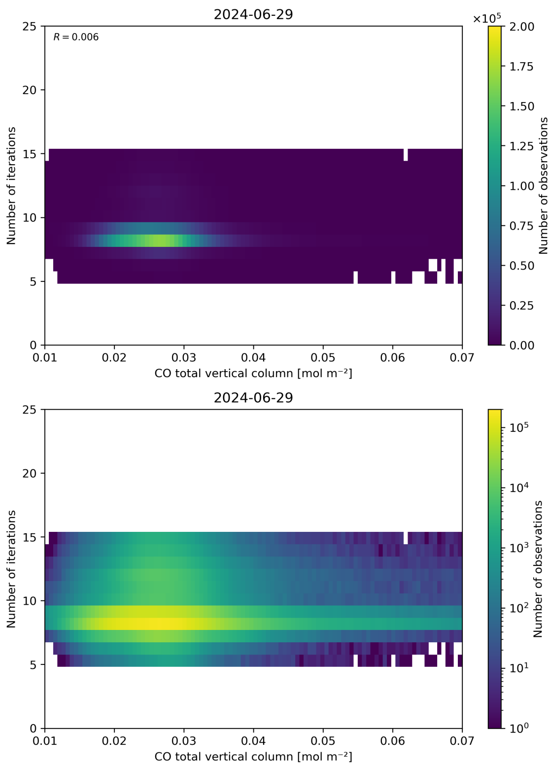
Figure 42: Scatter density plot of “CO total vertical column” against “Number of iterations” for 2024-06-29 to 2024-06-30.
