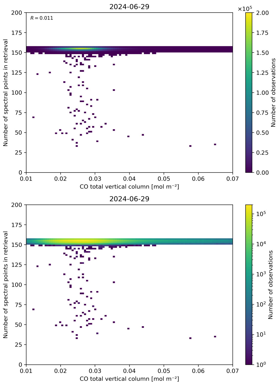
Figure 43: Scatter density plot of “CO total vertical column” against “Number of spectral points in retrieval” for 2024-06-29 to 2024-06-30.
