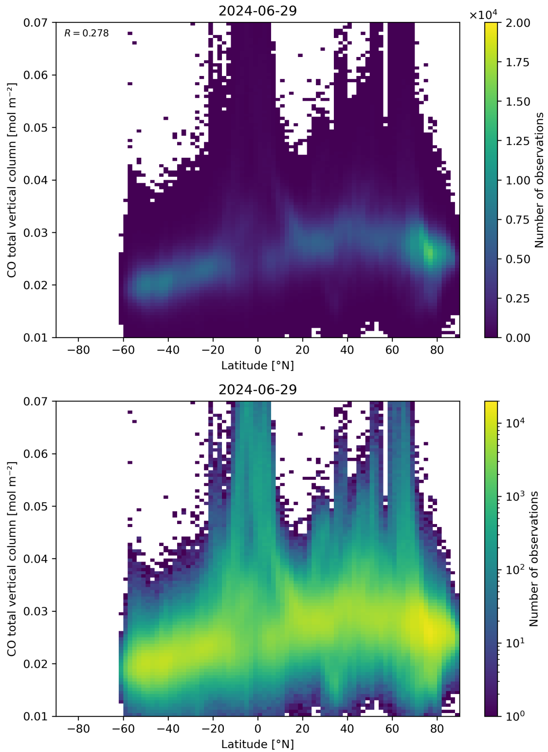
Figure 51: Scatter density plot of “Latitude” against “CO total vertical column” for 2024-06-29 to 2024-06-30.
