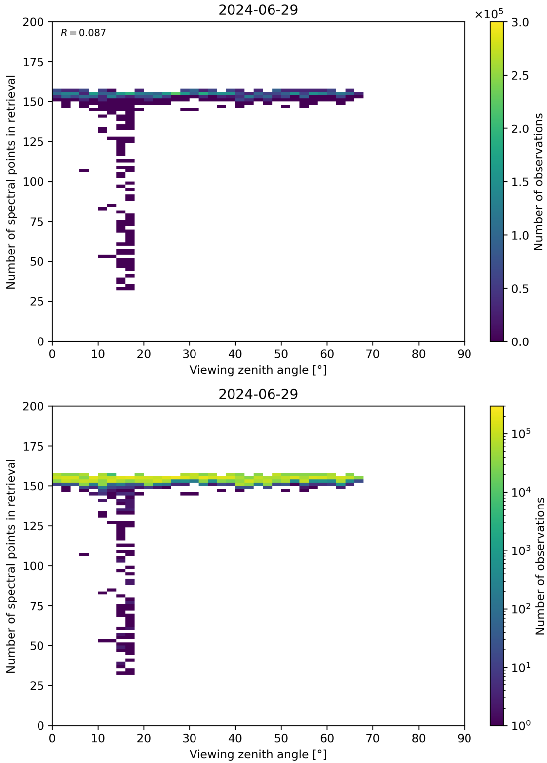
Figure 76: Scatter density plot of “Viewing zenith angle” against “Number of spectral points in retrieval” for 2024-06-29 to 2024-06-30.
