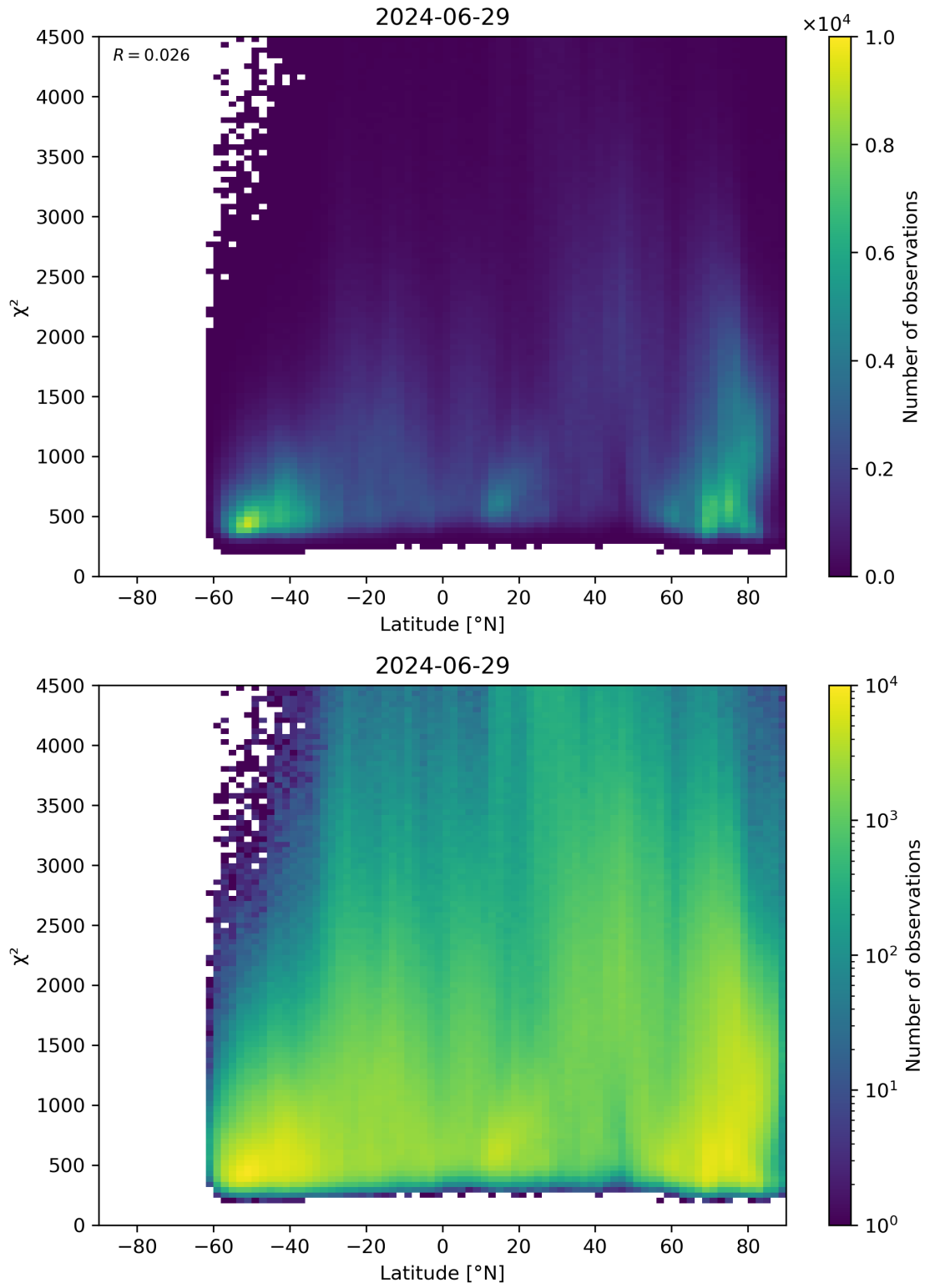
Figure 54: Scatter density plot of “Latitude” against “ \chi^2 ” for 2024-06-29 to 2024-06-30.
