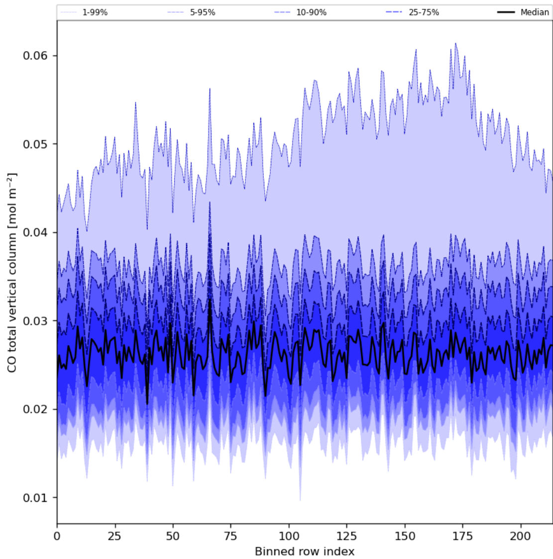
Figure 26: Along track statistics of “CO total vertical column” for 2024-06-29 to 2024-06-30
