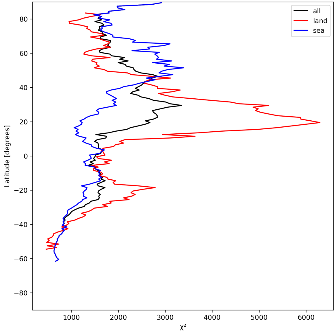
Figure 14: Zonal average of “ \chi^2 ” for 2024-06-29 to 2024-06-30.
