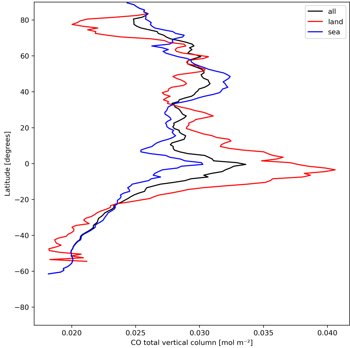
Figure 10: Zonal average of “CO total vertical column” for 2024-06-29 to 2024-06-30.
