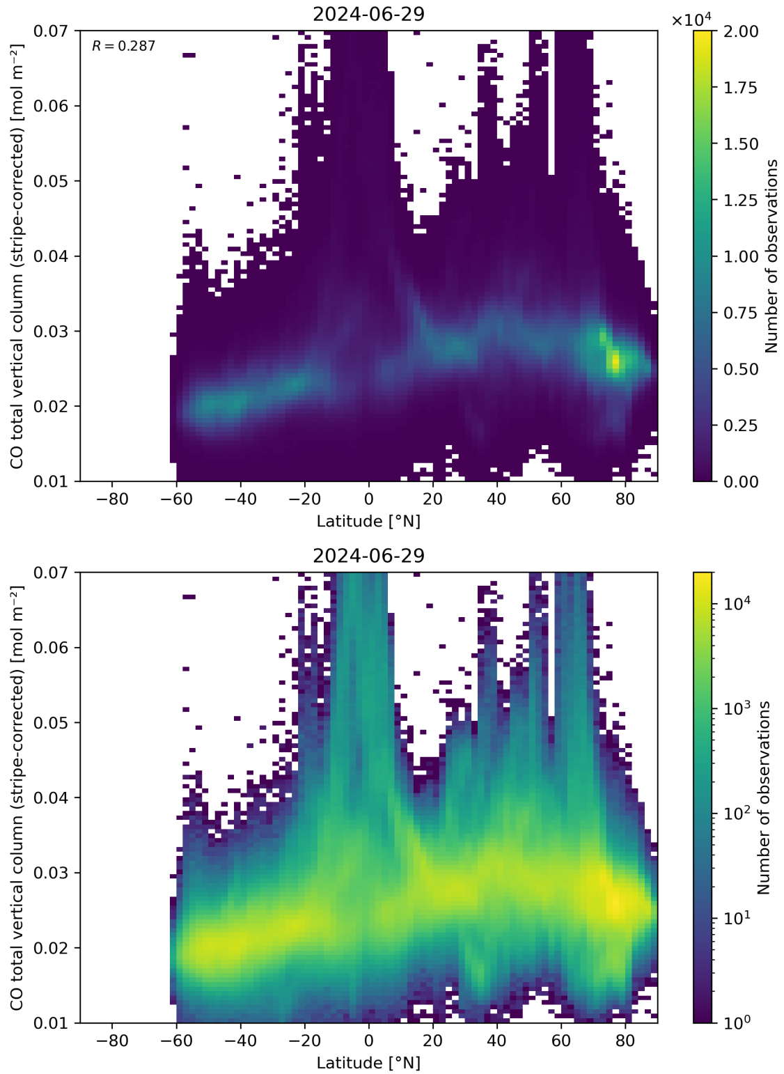
Figure 52: Scatter density plot of “Latitude” against “CO total vertical column (stripe-corrected)” for 2024-06-29 to 2024-06-30.
