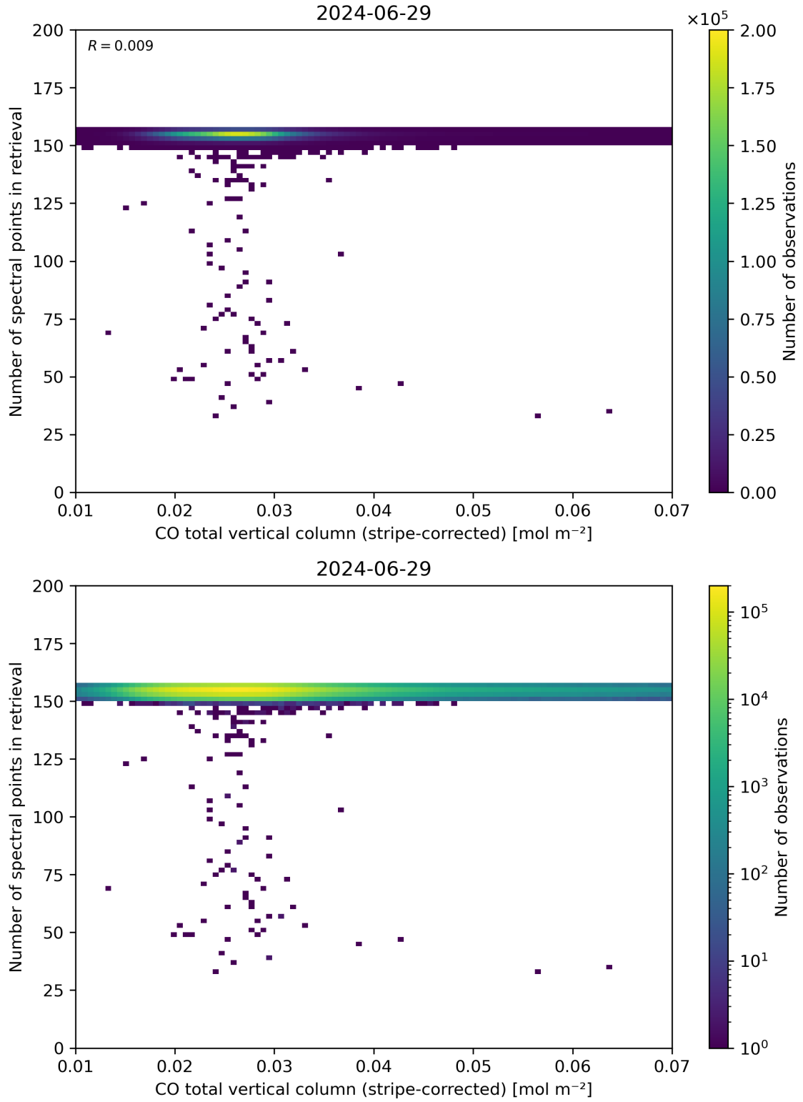
Figure 40: Scatter density plot of “CO total vertical column (stripe-corrected)” against “Number of spectral points in retrieval” for 2024-06-29 to 2024-06-30.
