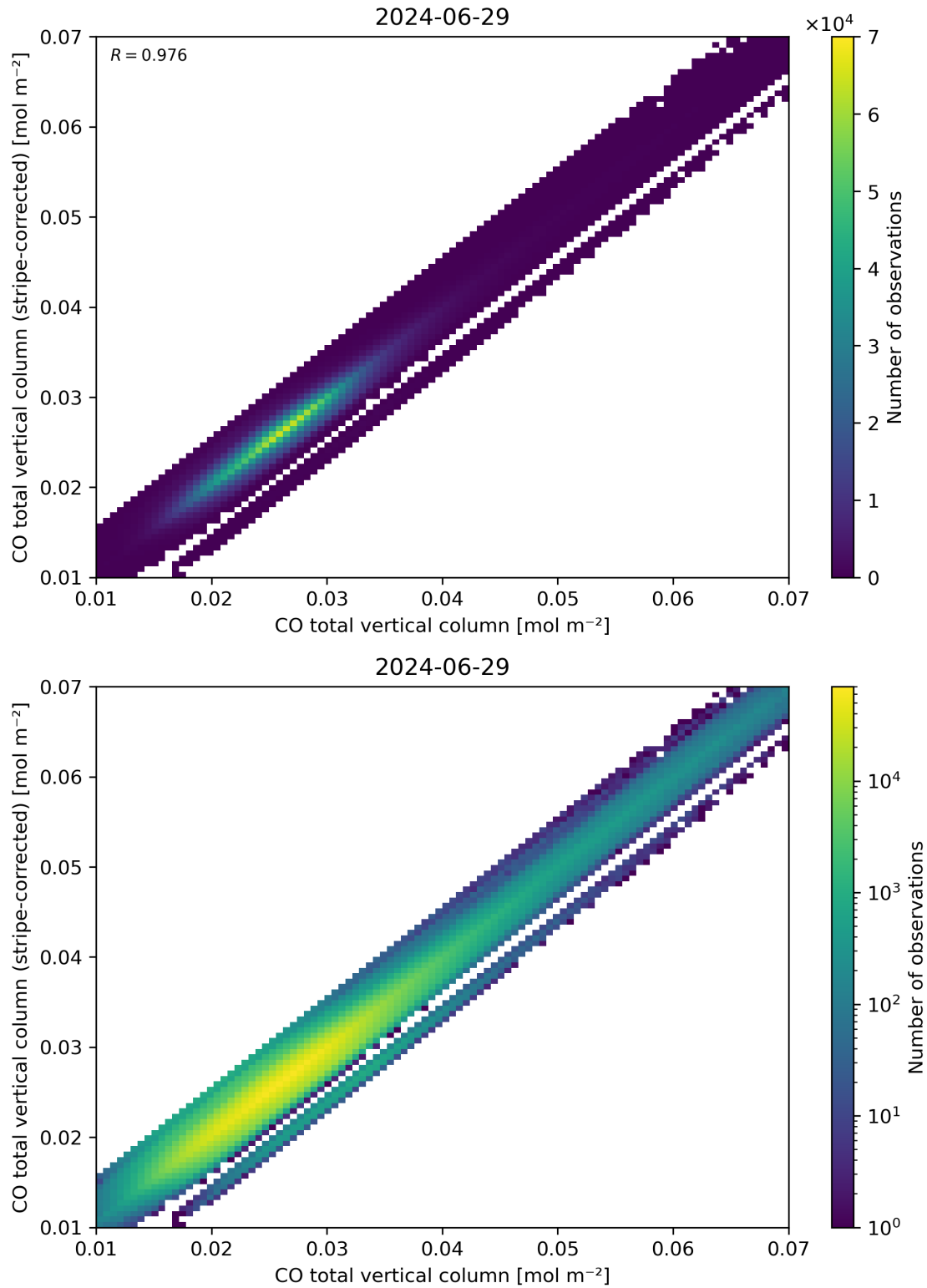
Figure 33: Scatter density plot of “CO total vertical column” against “CO total vertical column (stripe-corrected)” for 2024-06-29 to 2024-06-30.
