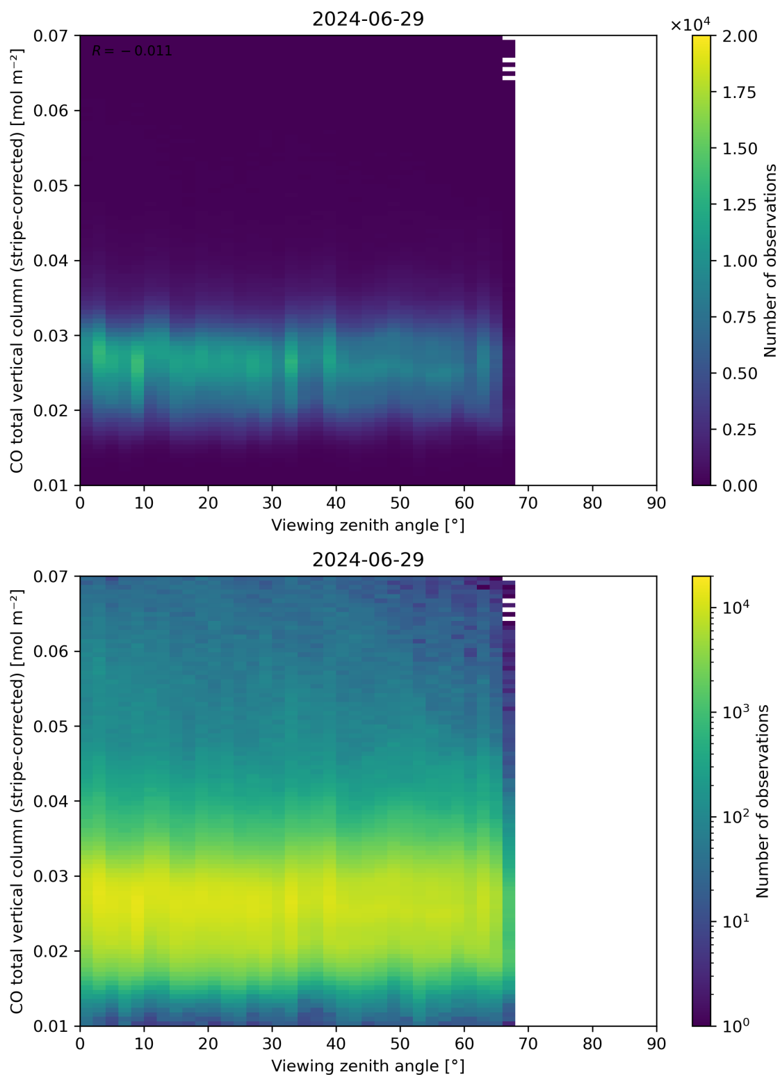
Figure 70: Scatter density plot of “Viewing zenith angle” against “CO total vertical column (stripe-corrected)” for 2024-06-29 to 2024-06-30.
