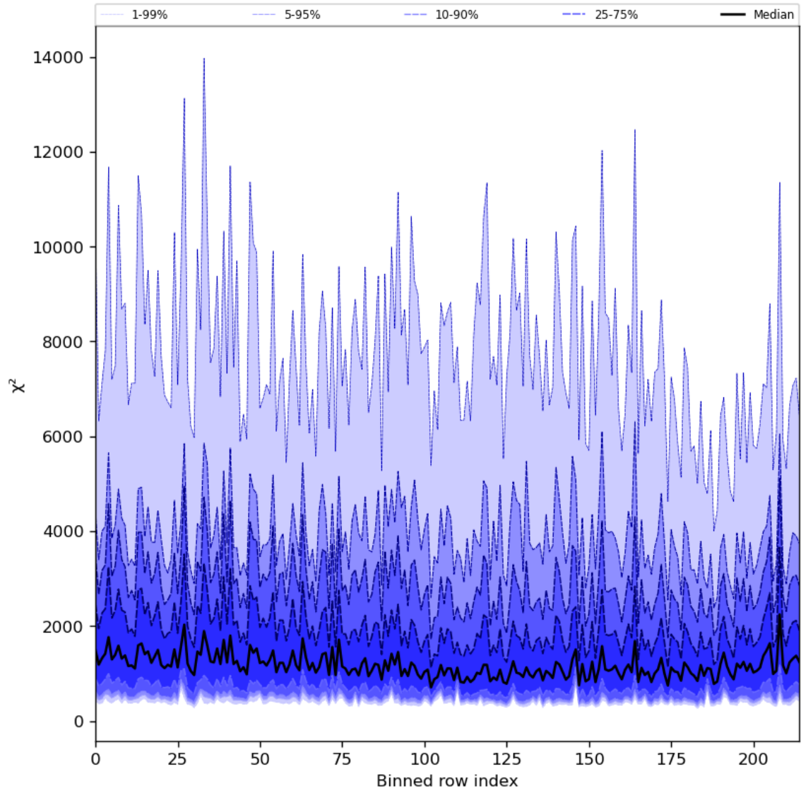
Figure 30: Along track statistics of “ \chi^2 ” for 2024-06-29 to 2024-06-30
