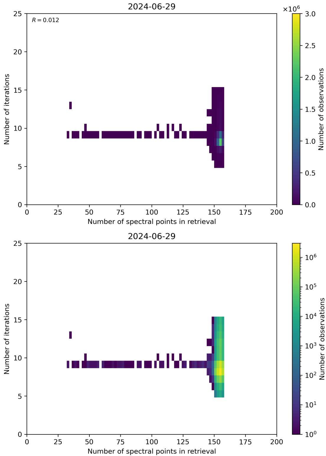
Figure 60: Scatter density plot of “Number of spectral points in retrieval” against “Number of iterations” for 2024-06-29 to 2024-06-30.
