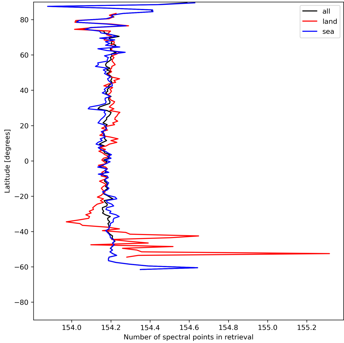
Figure 13: Zonal average of “Number of spectral points in retrieval” for 2024-06-29 to 2024-06-30.
