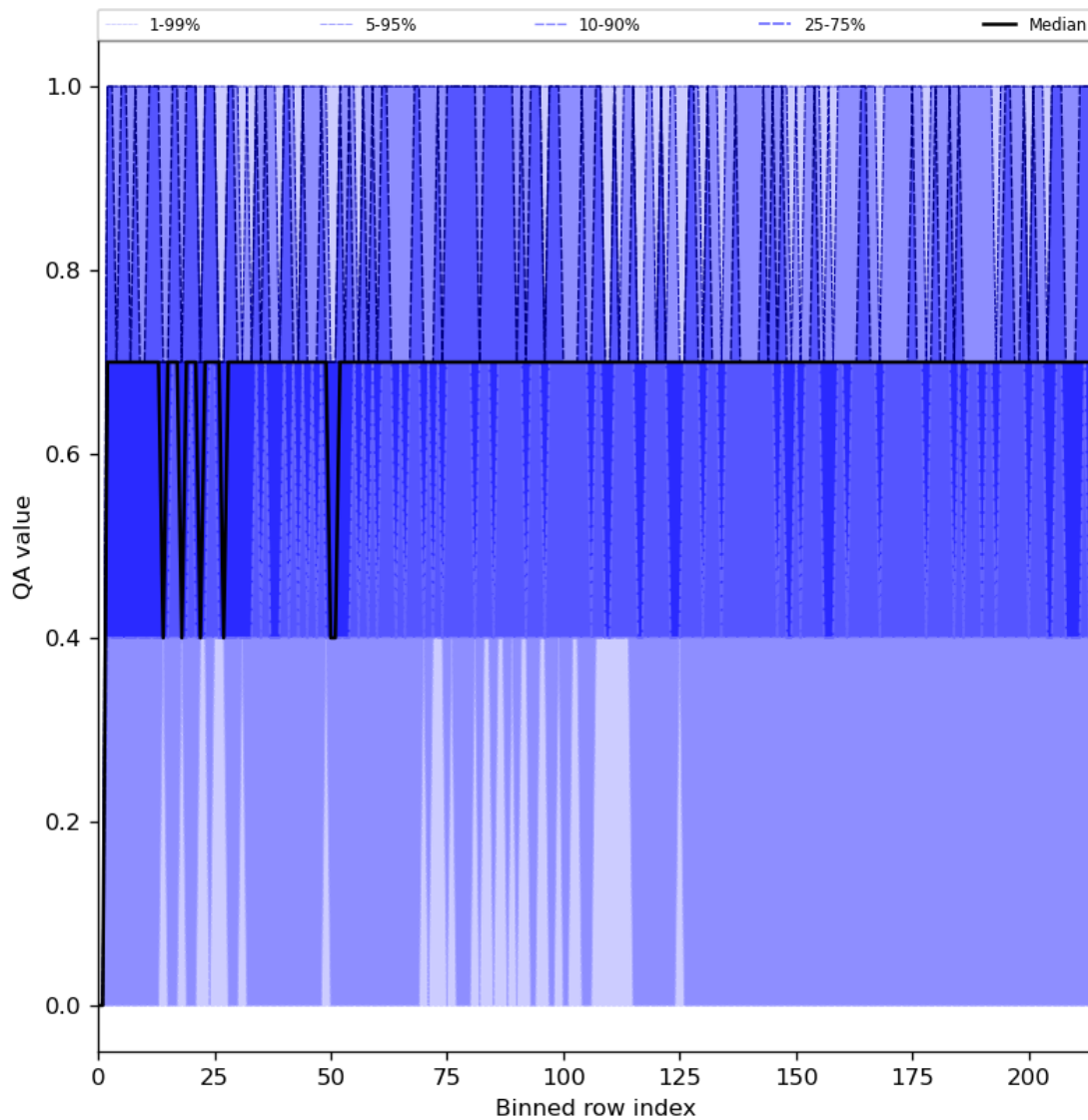
Figure 25: Along track statistics of “QA value” for 2024-06-29 to 2024-06-30
