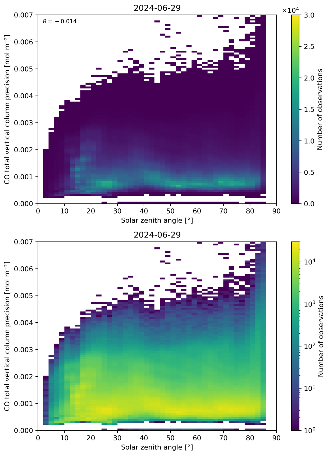
Figure 63: Scatter density plot of “Solar zenith angle” against “CO total vertical column precision” for 2024-06-29 to 2024-06-30.
