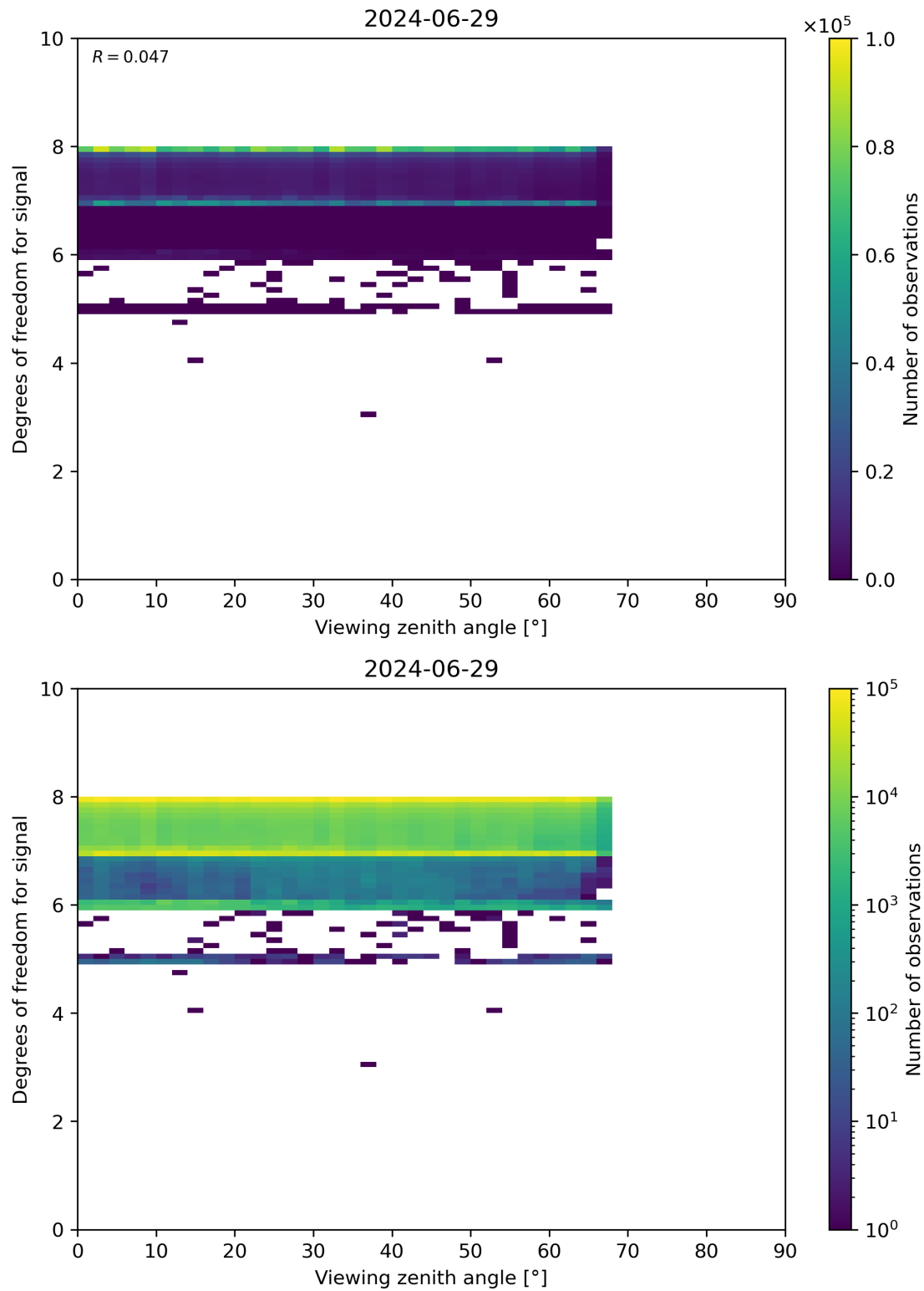
Figure 73: Scatter density plot of “Viewing zenith angle” against “Degrees of freedom for signal” for 2024-06-29 to 2024-06-30.
