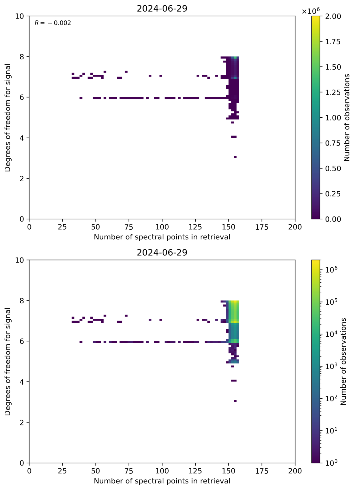
Figure 59: Scatter density plot of “Number of spectral points in retrieval” against “Degrees of freedom for signal” for 2024-06-29 to 2024-06-30.
