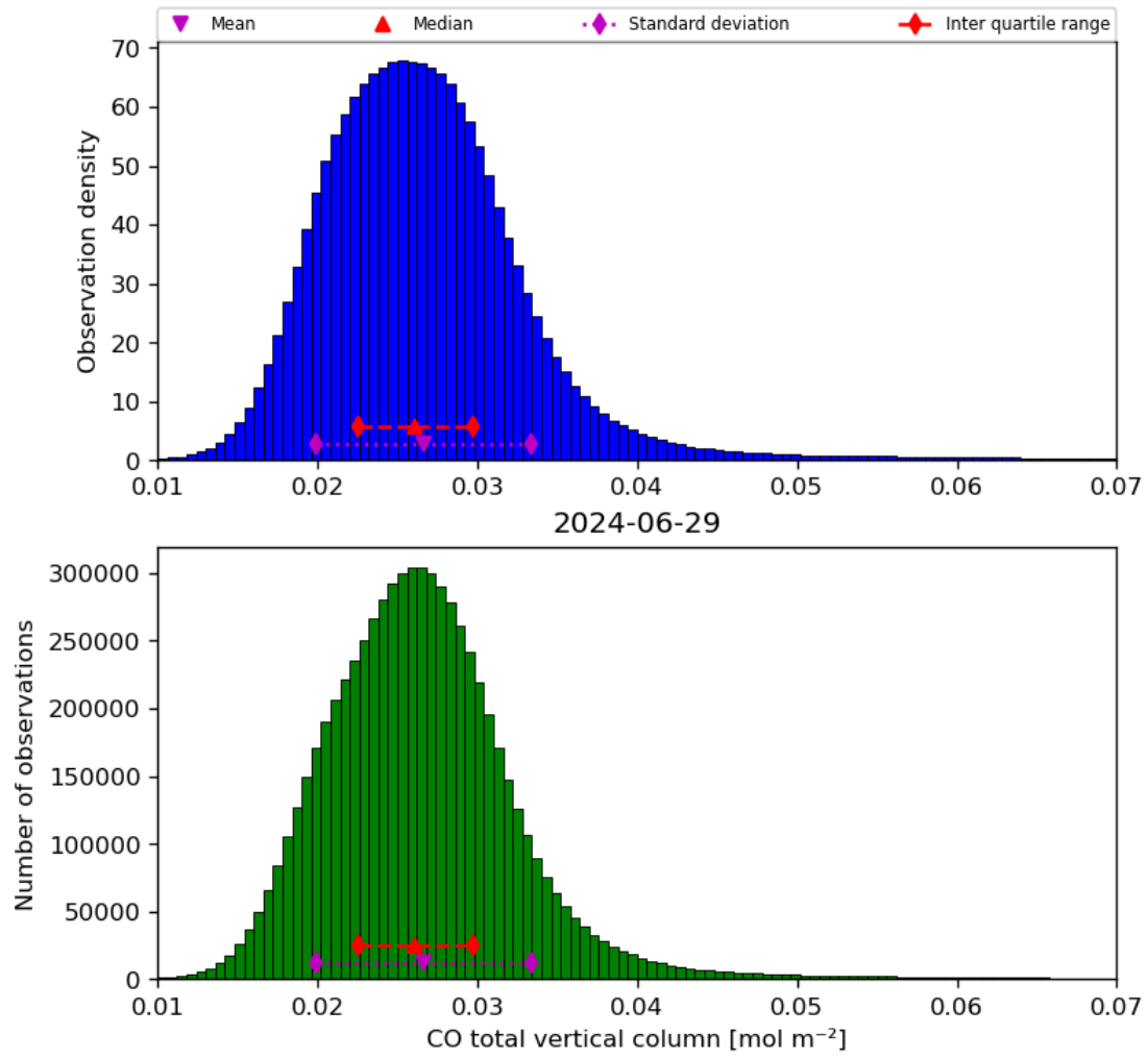
Figure 18: Histogram of “CO total vertical column” for 2024-06-29 to 2024-06-30
