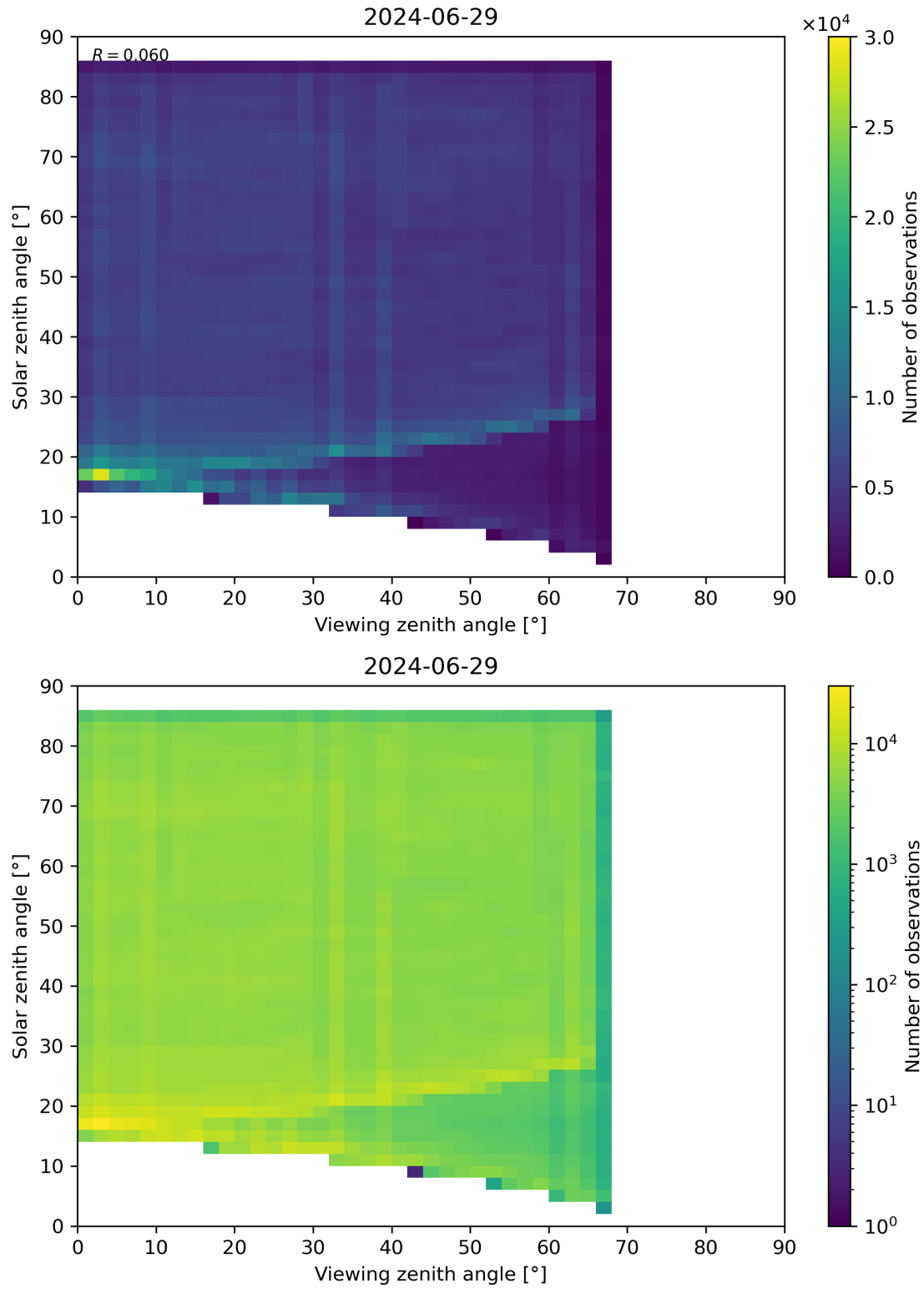
Figure 77: Scatter density plot of “Viewing zenith angle” against “Solar zenith angle” for 2024-06-29 to 2024-06-30.
