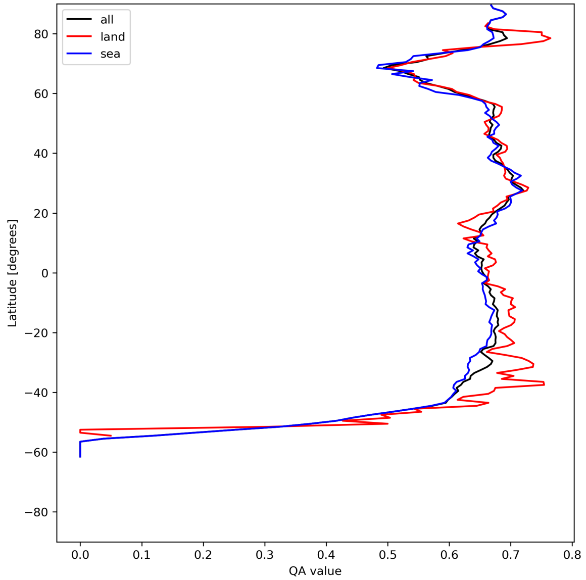
Figure 9: Zonal average of “QA value” for 2024-06-29 to 2024-06-30.
