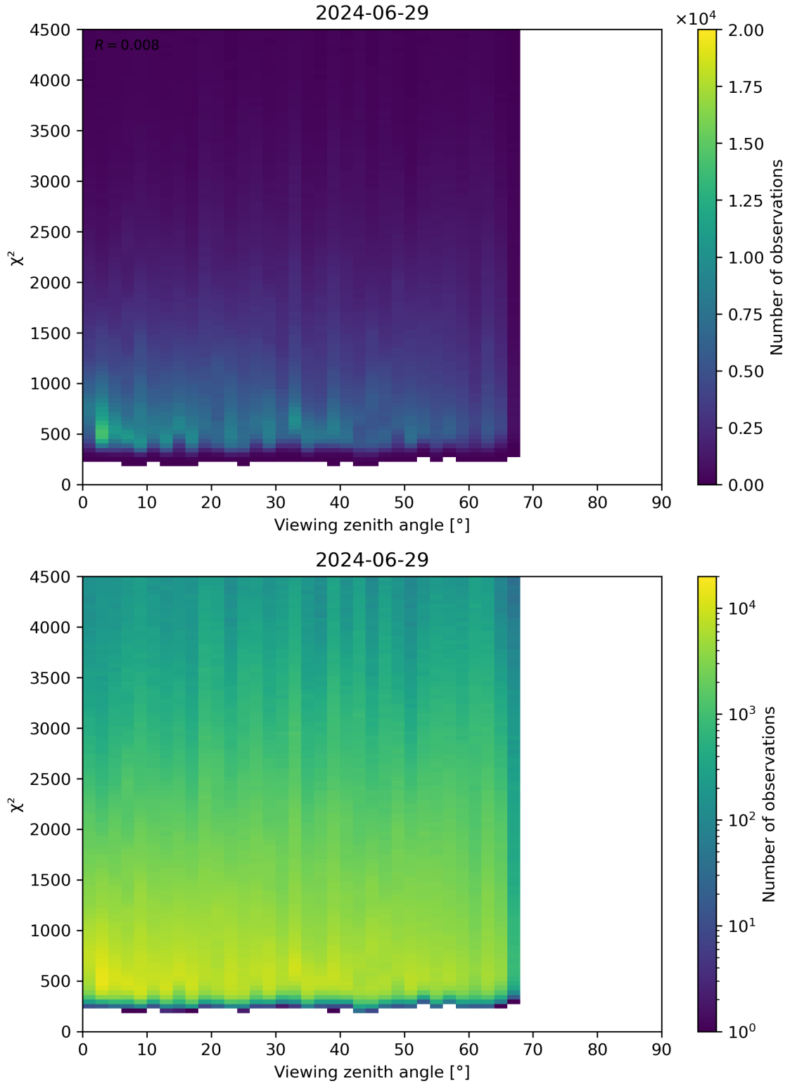
Figure 72: Scatter density plot of “Viewing zenith angle” against “ \chi^2 ” for 2024-06-29 to 2024-06-30.
