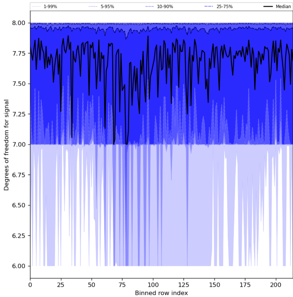
Figure 31: Along track statistics of “Degrees of freedom for signal” for 2024-06-29 to 2024-06-30
