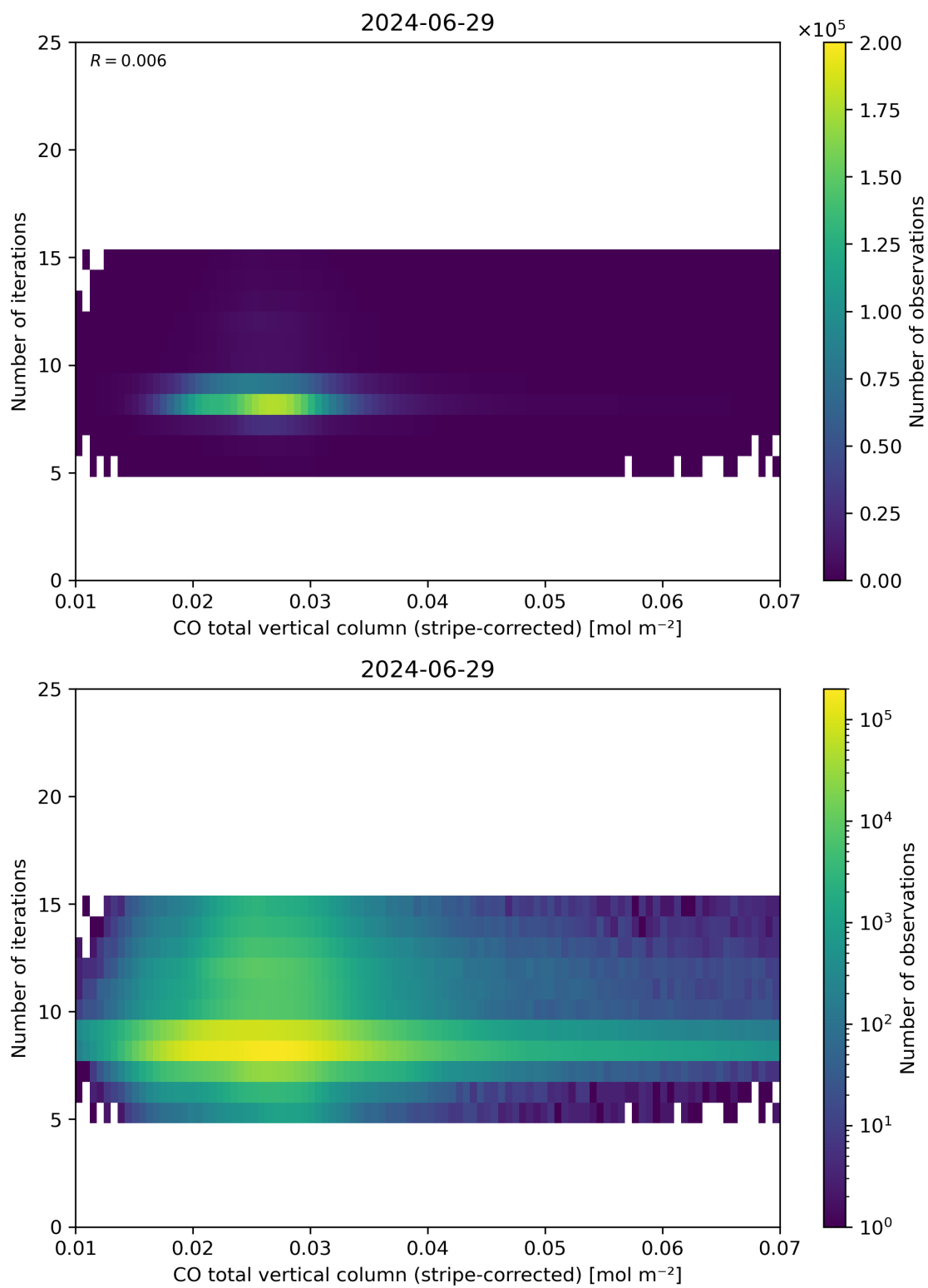
Figure 39: Scatter density plot of “CO total vertical column (stripe-corrected)” against “Number of iterations” for 2024-06-29 to 2024-06-30.
