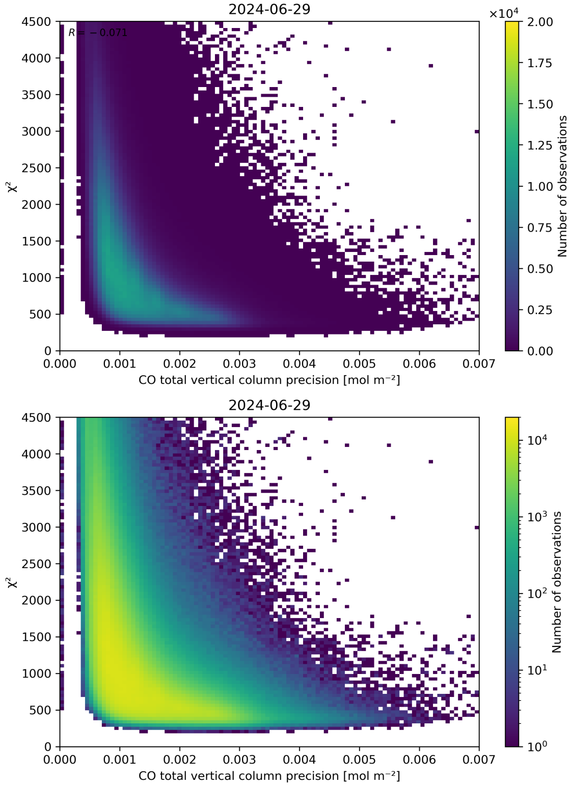
Figure 44: Scatter density plot of “CO total vertical column precision” against “ \chi^2 ” for 2024-06-29 to 2024-06-30.
