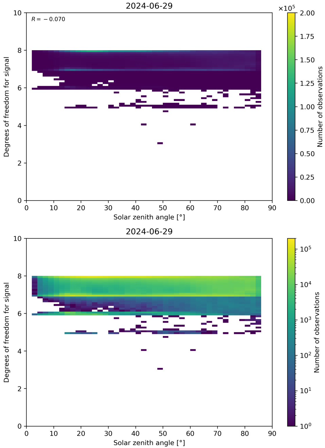
Figure 65: Scatter density plot of “Solar zenith angle” against “Degrees of freedom for signal” for 2024-06-29 to 2024-06-30.
