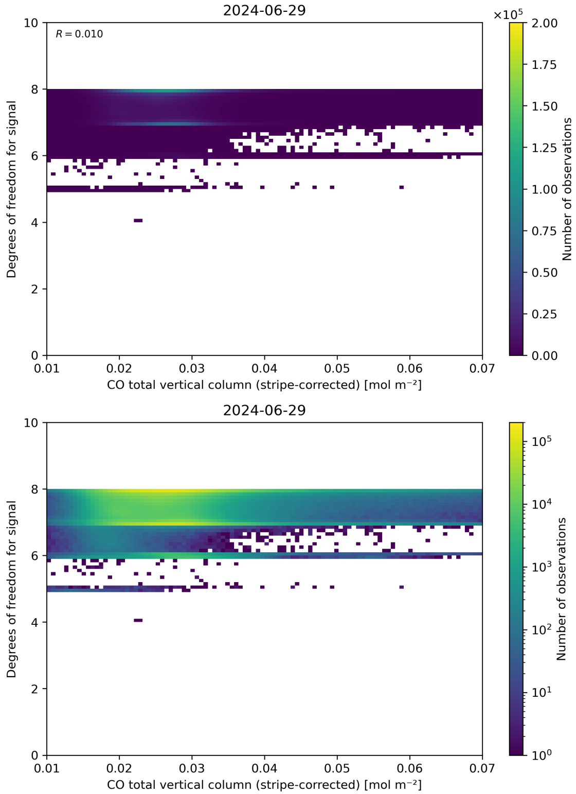
Figure 38: Scatter density plot of “CO total vertical column (stripe-corrected)” against “Degrees of freedom for signal” for 2024-06-29 to 2024-06-30.
