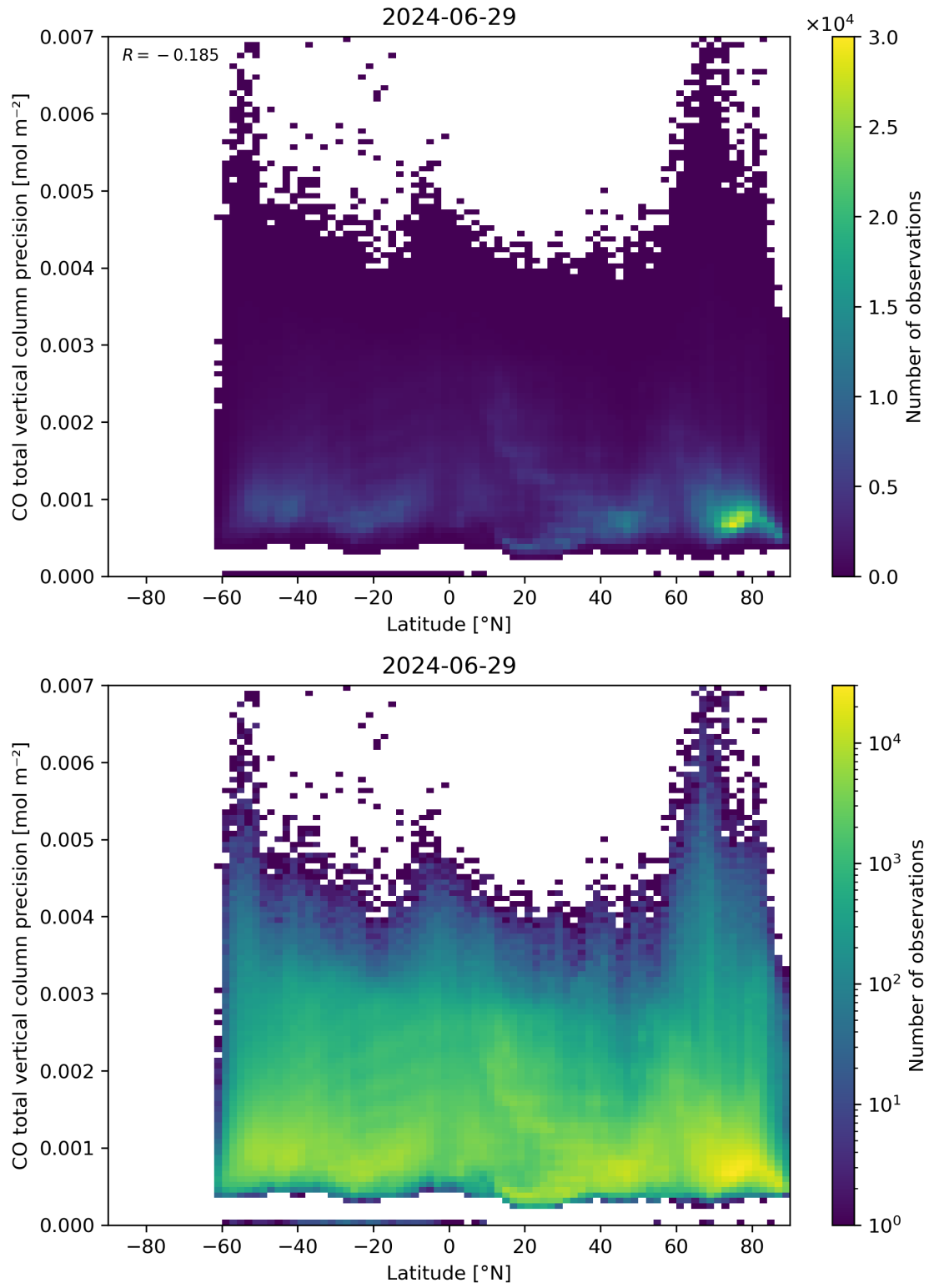
Figure 53: Scatter density plot of “Latitude” against “CO total vertical column precision” for 2024-06-29 to 2024-06-30.
