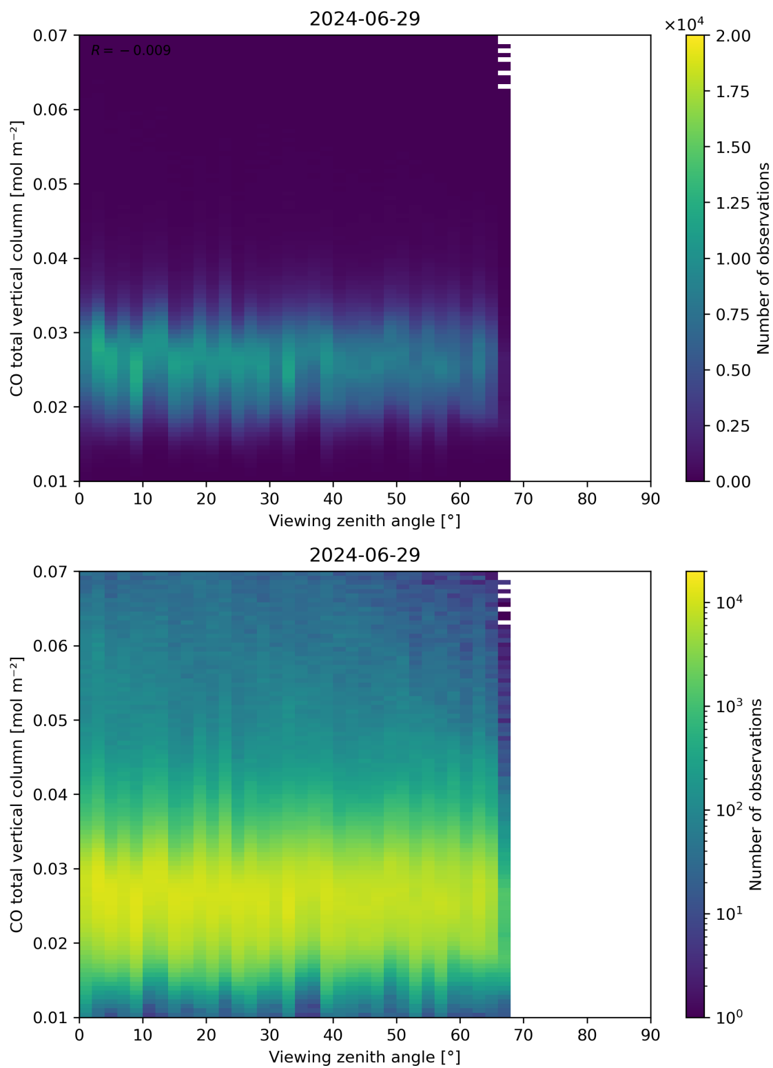
Figure 69: Scatter density plot of “Viewing zenith angle” against “CO total vertical column” for 2024-06-29 to 2024-06-30.
