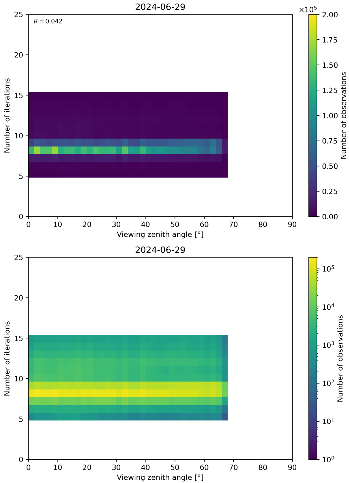
Figure 75: Scatter density plot of “Viewing zenith angle” against “Number of iterations” for 2024-06-29 to 2024-06-30.
