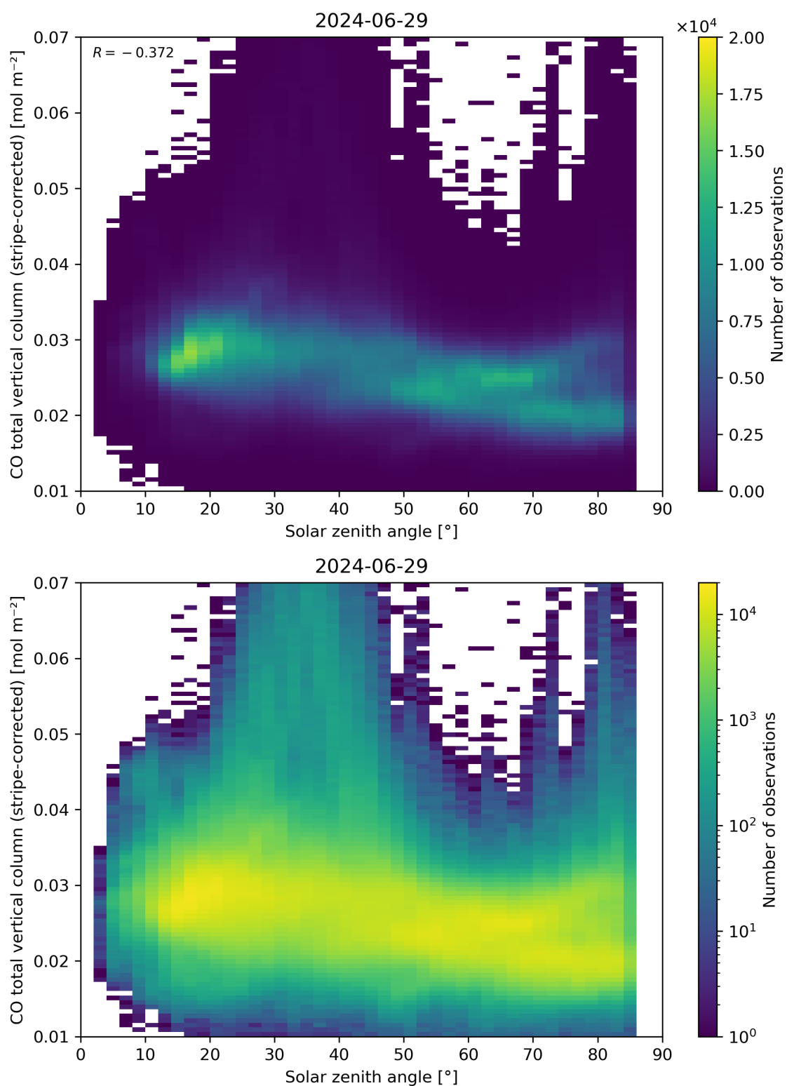
Figure 62: Scatter density plot of “Solar zenith angle” against “CO total vertical column (stripe-corrected)” for 2024-06-29 to 2024-06-30.
