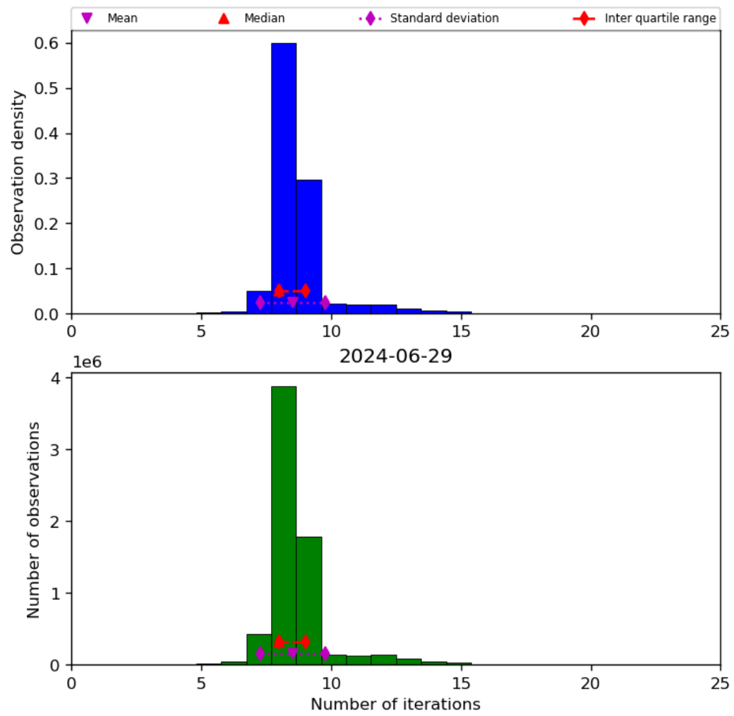
Figure 24: Histogram of “Number of iterations” for 2024-06-29 to 2024-06-30
