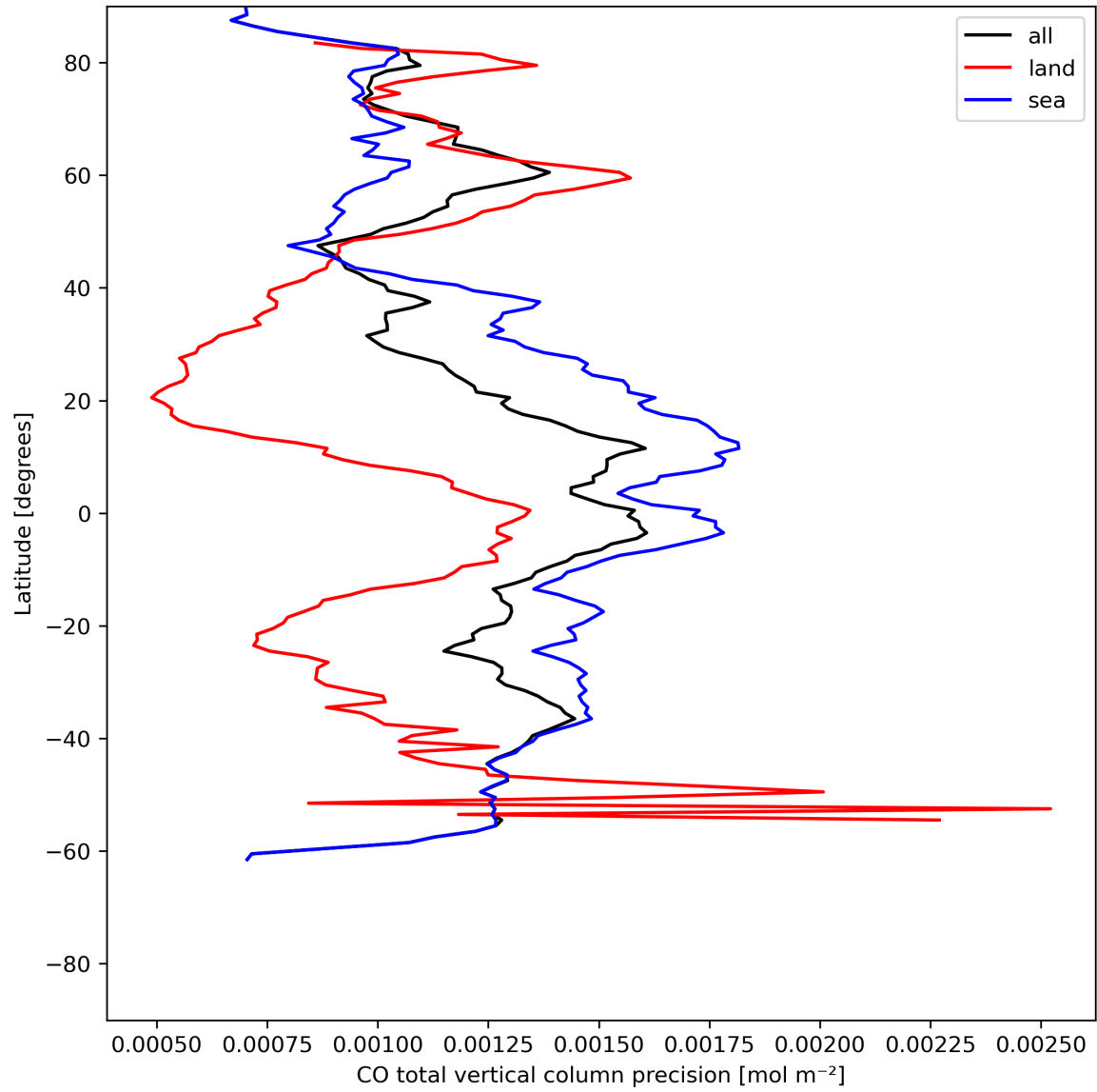
Figure 12: Zonal average of “CO total vertical column precision” for 2024-06-29 to 2024-06-30.
