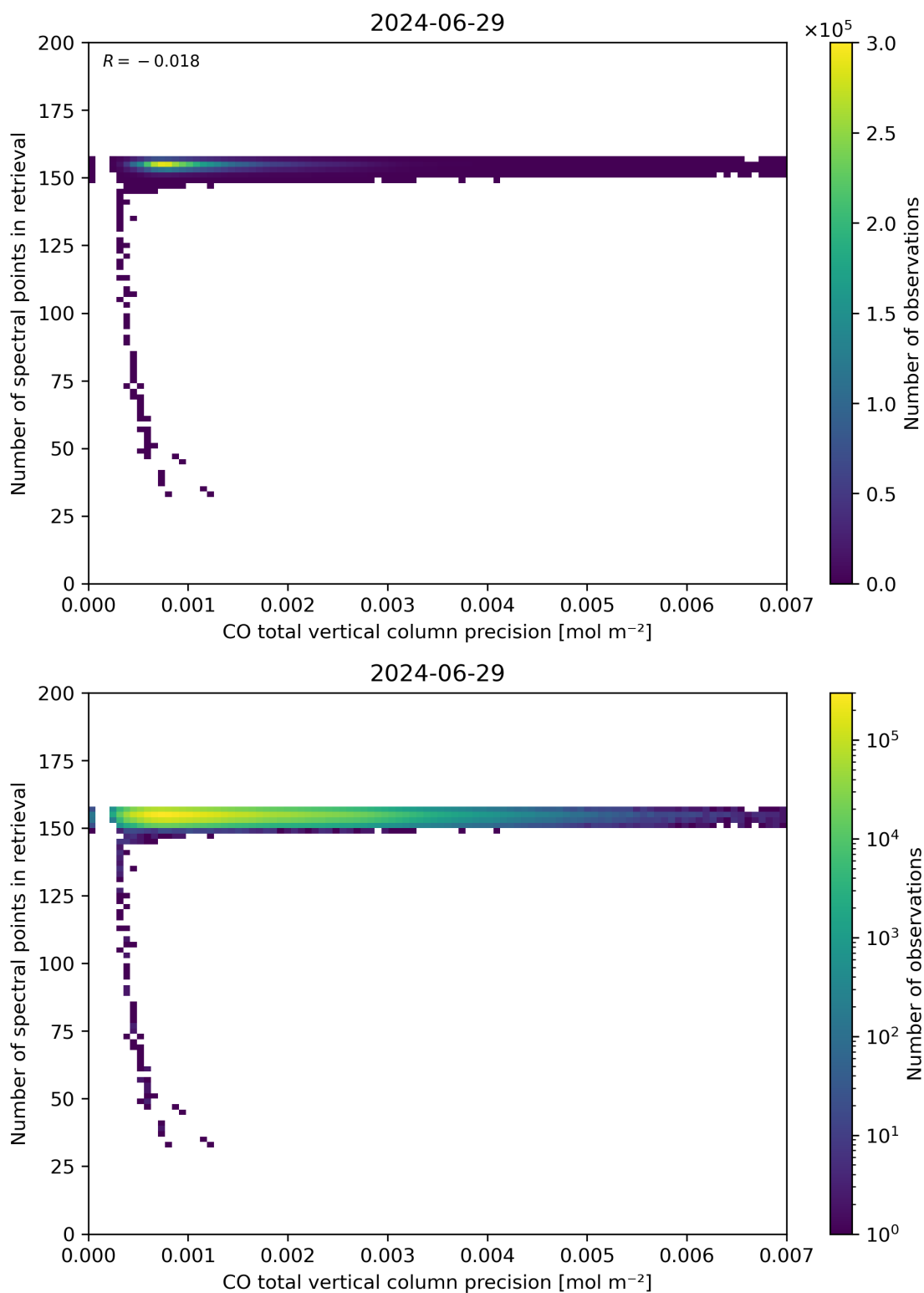
Figure 47: Scatter density plot of “CO total vertical column precision” against “Number of spectral points in retrieval” for 2024-06-29 to 2024-06-30.
