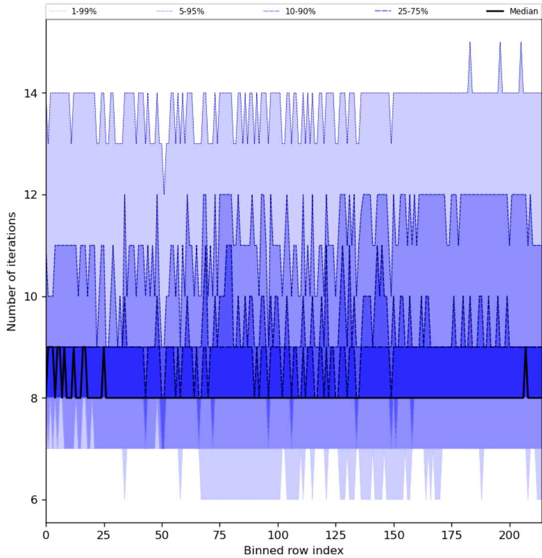
Figure 32: Along track statistics of “Number of iterations” for 2024-06-29 to 2024-06-30
