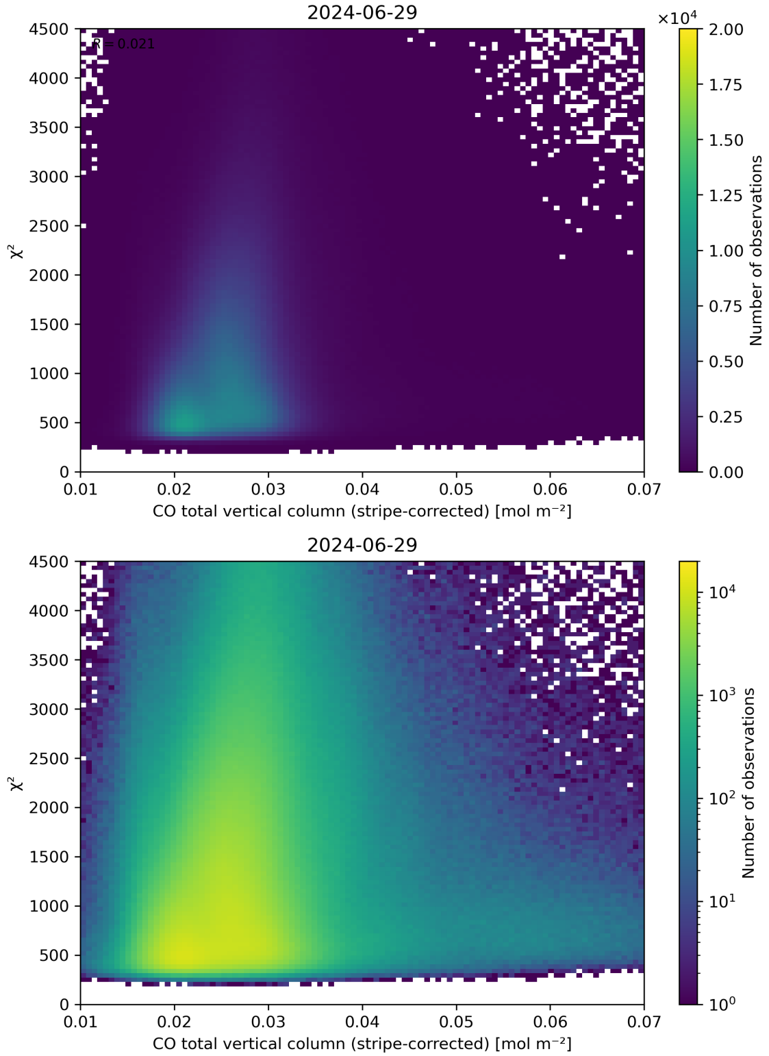
Figure 37: Scatter density plot of “CO total vertical column (stripe-corrected)” against “ \chi^2 ” for 2024-06-29 to 2024-06-30.
