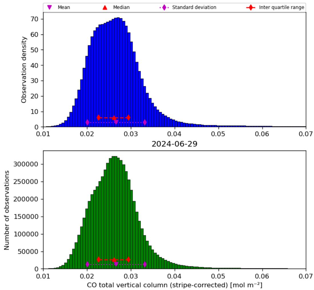
Figure 19: Histogram of “CO total vertical column (stripe-corrected)” for 2024-06-29 to 2024-06-30
