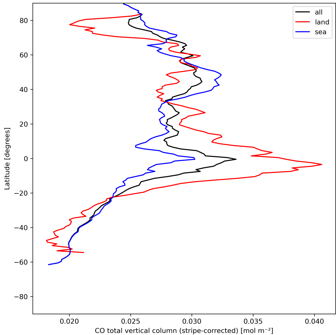
Figure 11: Zonal average of “CO total vertical column (stripe-corrected)” for 2024-06-29 to 2024-06-30.
