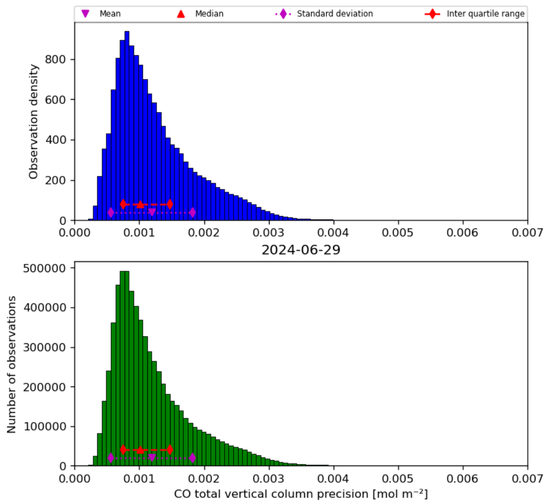
Figure 20: Histogram of “CO total vertical column precision” for 2024-06-29 to 2024-06-30
