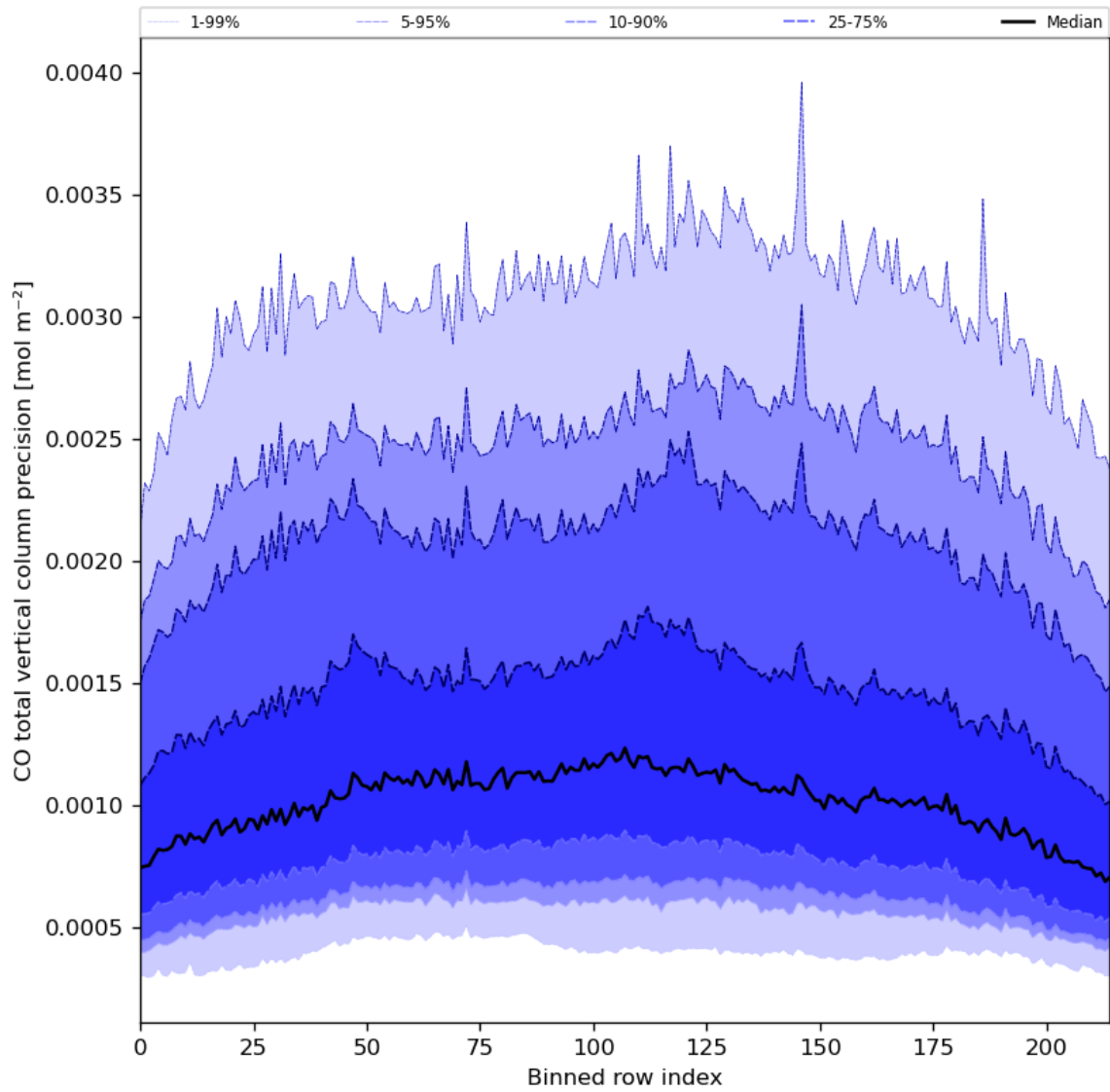
Figure 28: Along track statistics of “CO total vertical column precision” for 2024-06-29 to 2024-06-30
