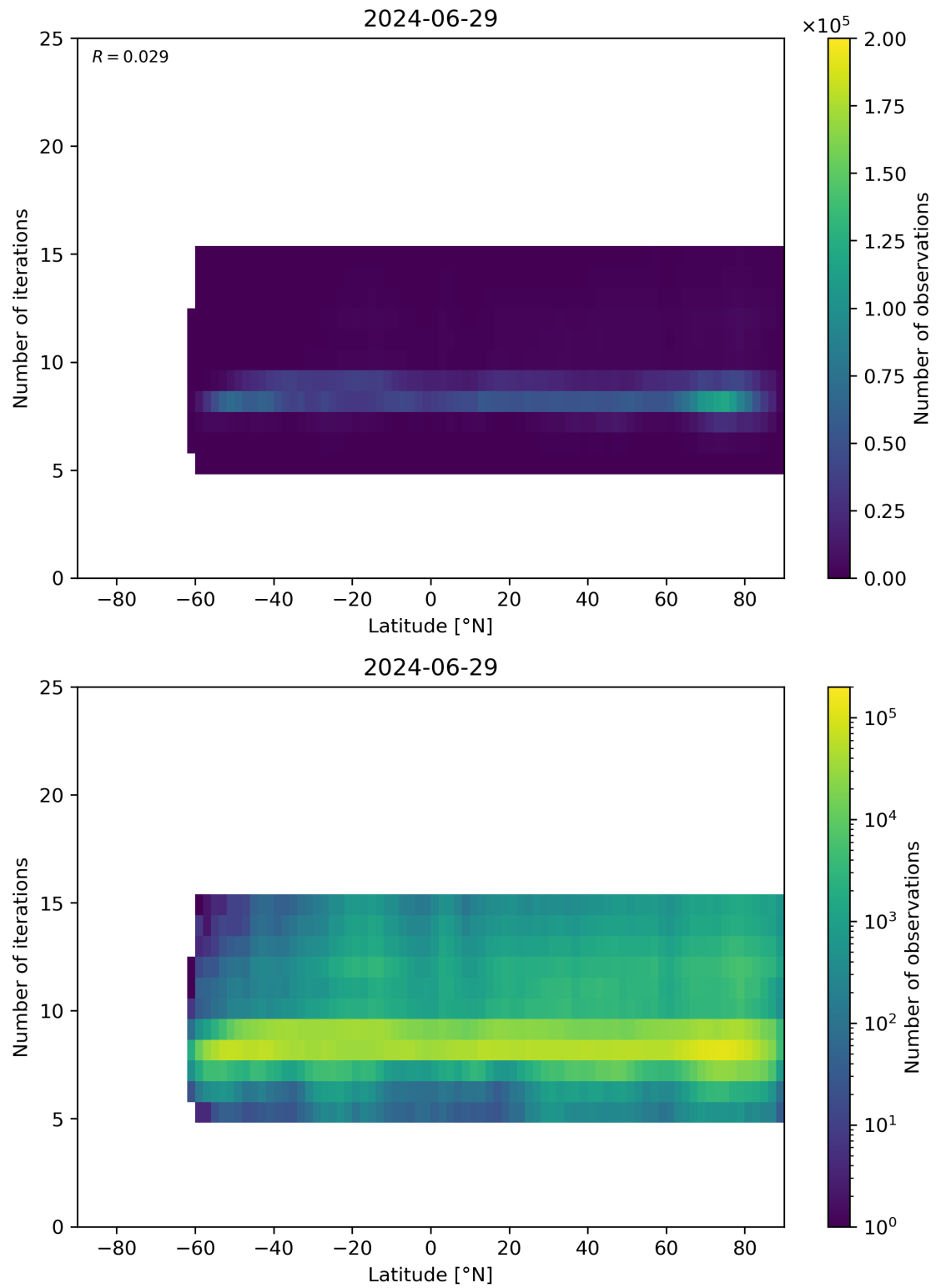
Figure 56: Scatter density plot of “Latitude” against “Number of iterations” for 2024-06-29 to 2024-06-30.
