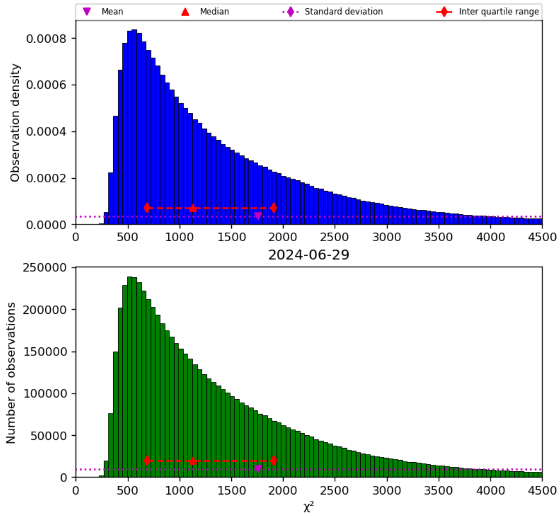
Figure 22: Histogram of “ \chi^2 ” for 2024-06-29 to 2024-06-30
