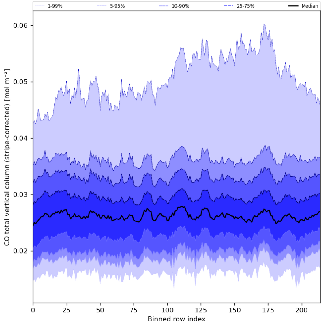
Figure 27: Along track statistics of “CO total vertical column (stripe-corrected)” for 2024-06-29 to 2024-06-30
