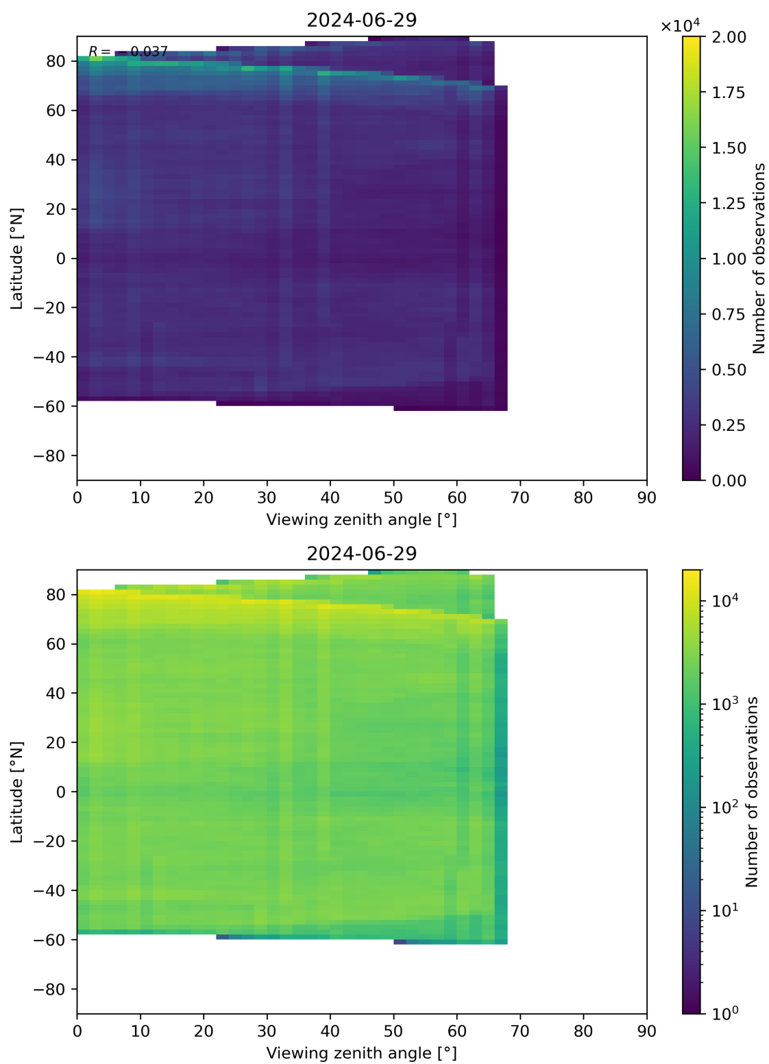
Figure 74: Scatter density plot of “Viewing zenith angle” against “Latitude” for 2024-06-29 to 2024-06-30.
