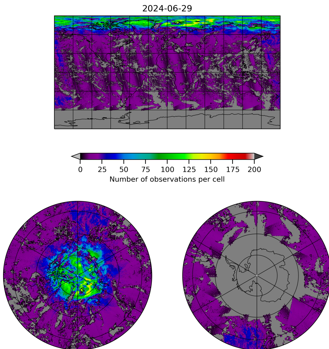
Figure 8: Map of the number of observations for 2024-06-29 to 2024-06-30
