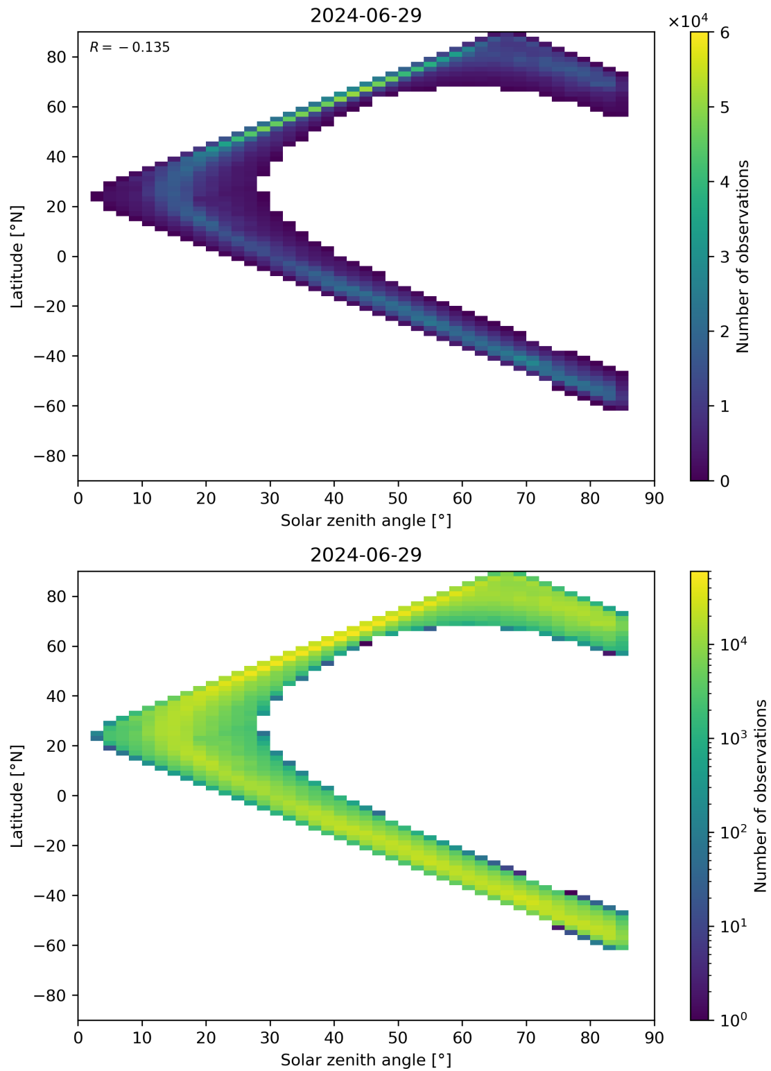
Figure 66: Scatter density plot of “Solar zenith angle” against “Latitude” for 2024-06-29 to 2024-06-30.
