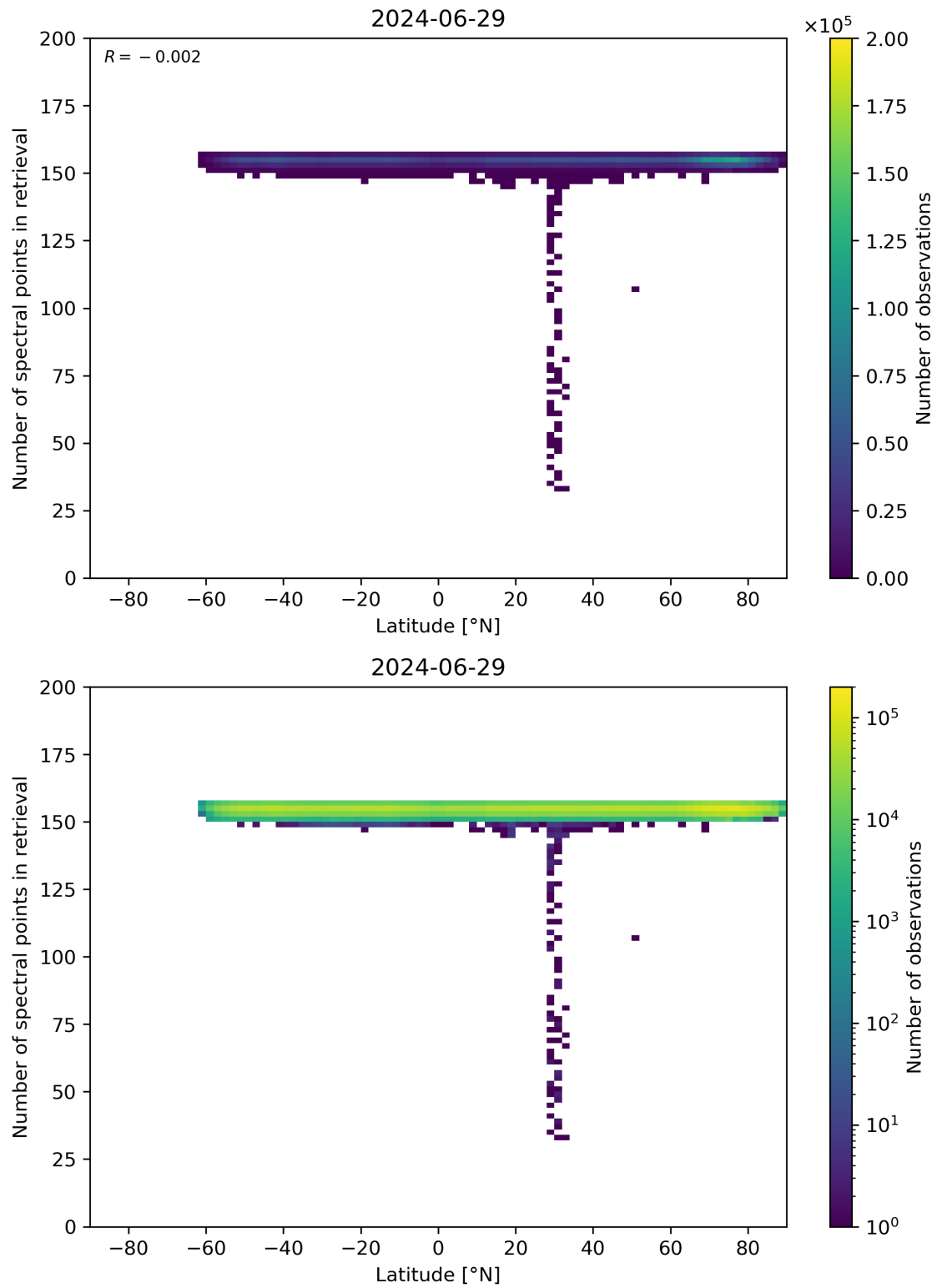
Figure 57: Scatter density plot of “Latitude” against “Number of spectral points in retrieval” for 2024-06-29 to 2024-06-30.
