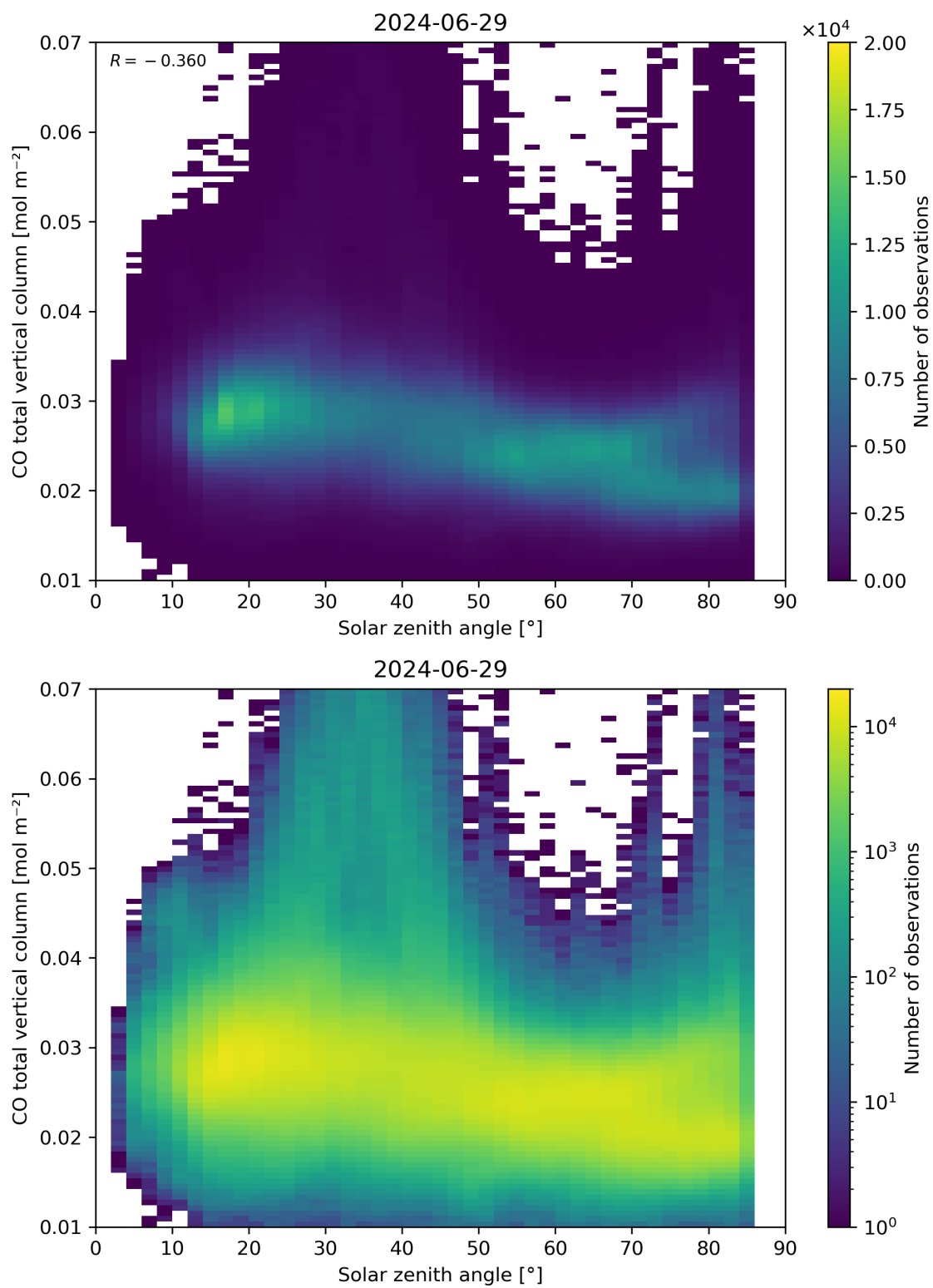
Figure 61: Scatter density plot of “Solar zenith angle” against “CO total vertical column” for 2024-06-29 to 2024-06-30.
