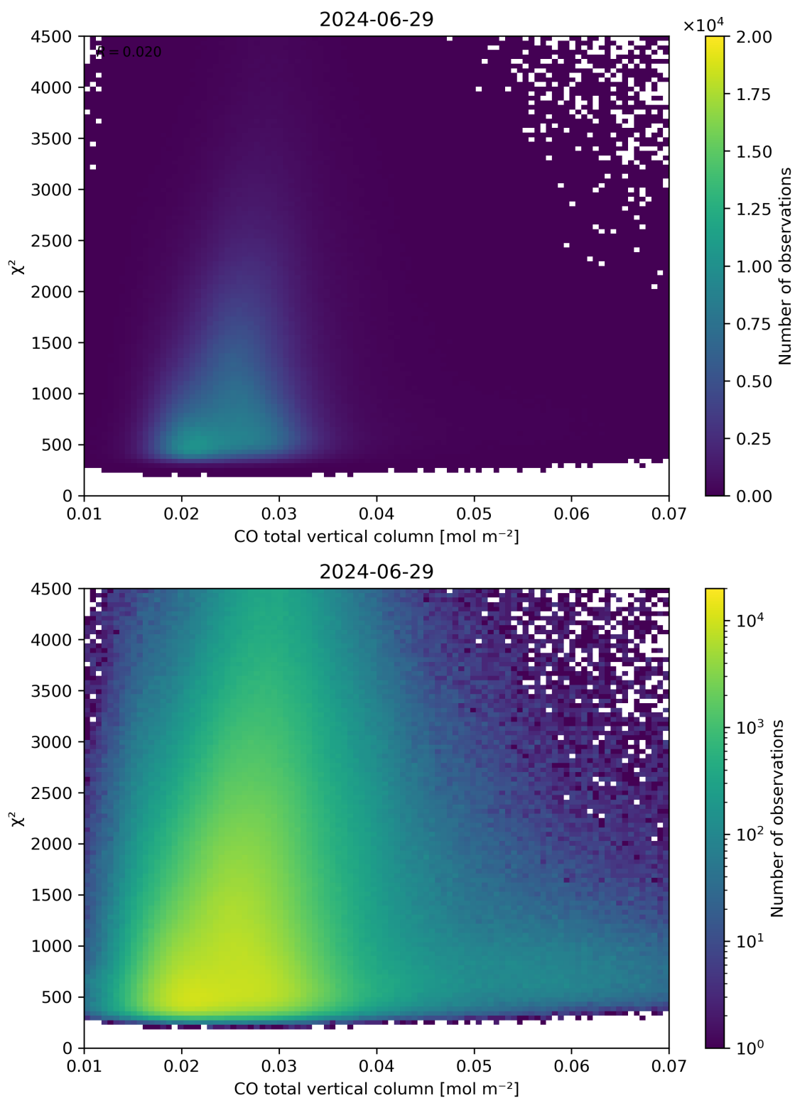
Figure 35: Scatter density plot of “CO total vertical column” against “ \chi^2 ” for 2024-06-29 to 2024-06-30.
