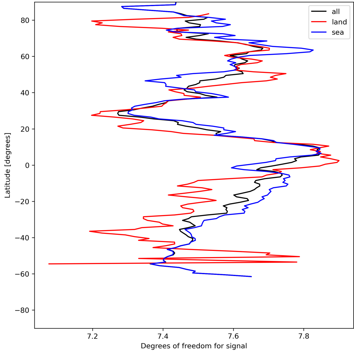
Figure 15: Zonal average of “Degrees of freedom for signal” for 2024-06-29 to 2024-06-30.
