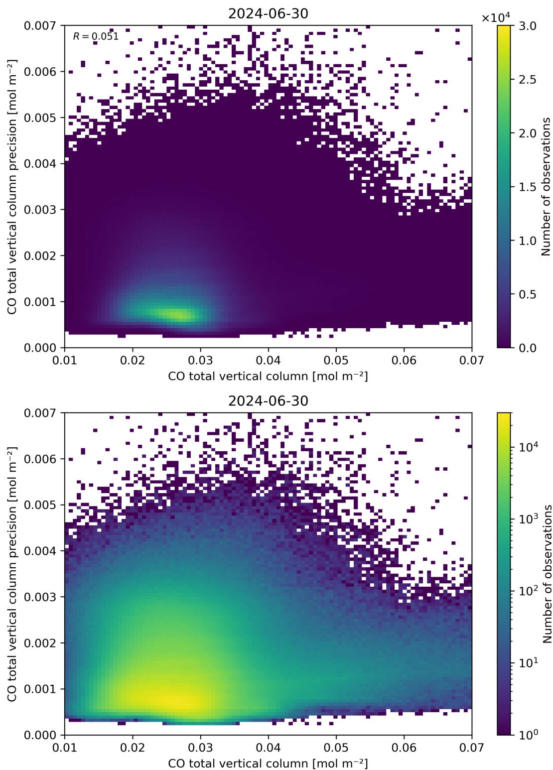
Figure 34: Scatter density plot of “CO total vertical column” against “CO total vertical column precision” for 2024-06-29 to 2024-07-01.
