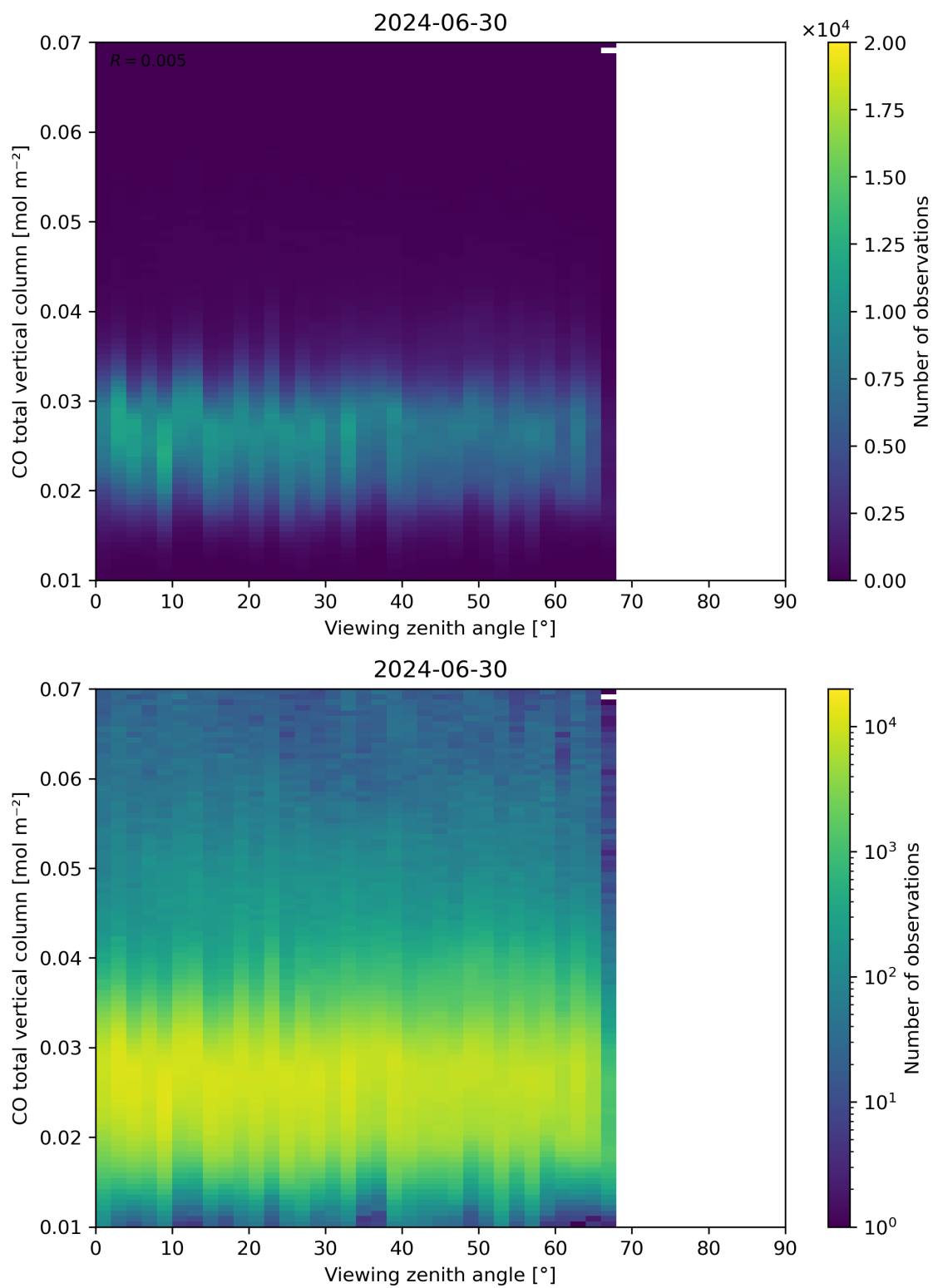
Figure 69: Scatter density plot of “Viewing zenith angle” against “CO total vertical column” for 2024-06-29 to 2024-07-01.
