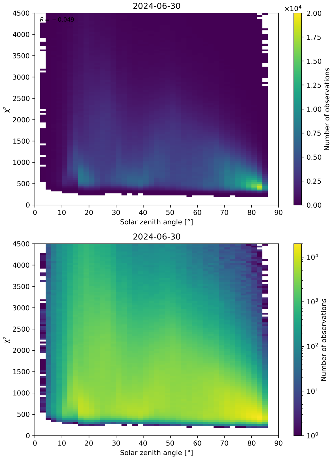
Figure 64: Scatter density plot of “Solar zenith angle” against “ \chi^2 ” for 2024-06-29 to 2024-07-01.
