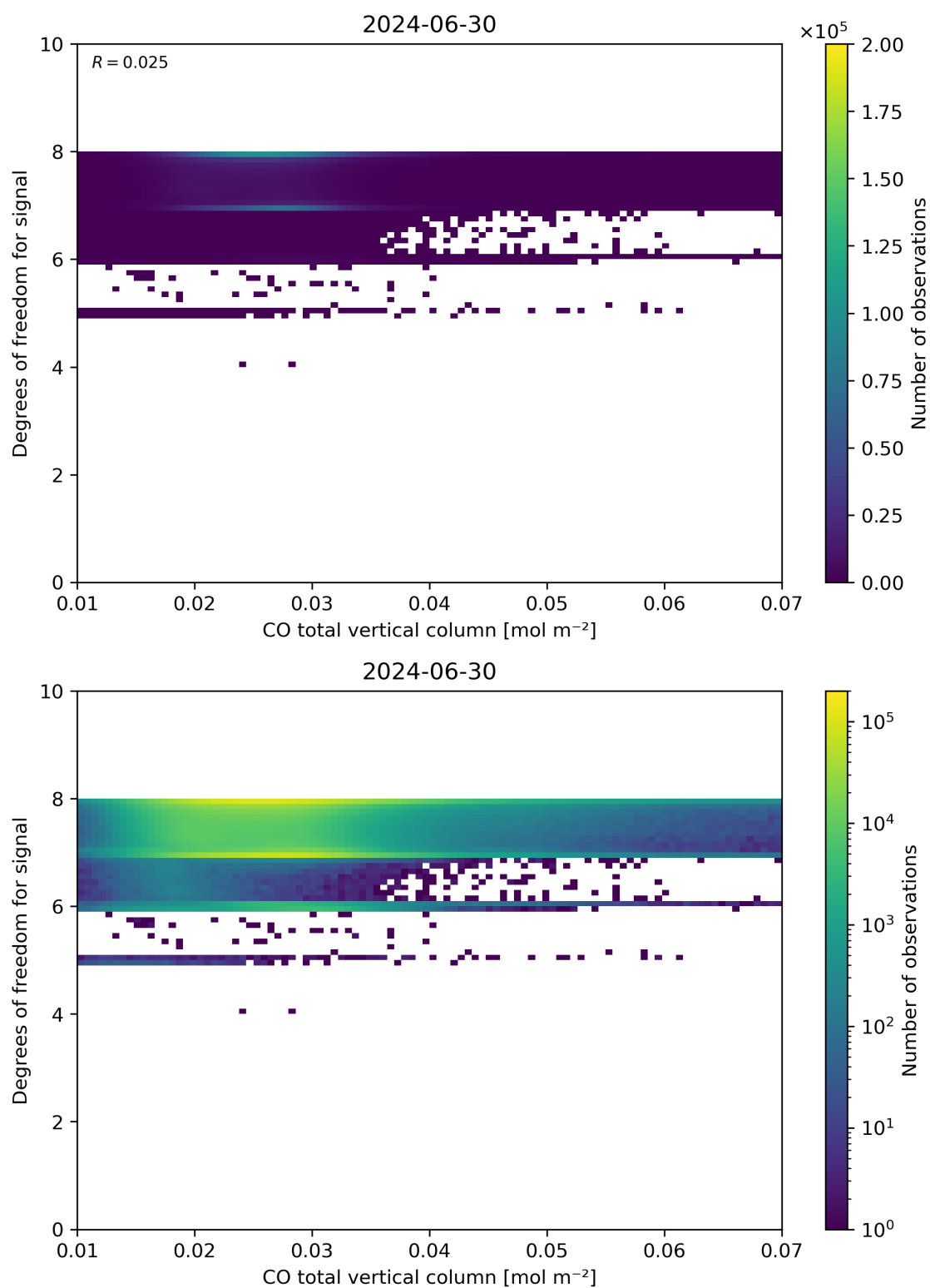
Figure 41: Scatter density plot of “CO total vertical column” against “Degrees of freedom for signal” for 2024-06-29 to 2024-07-01.
