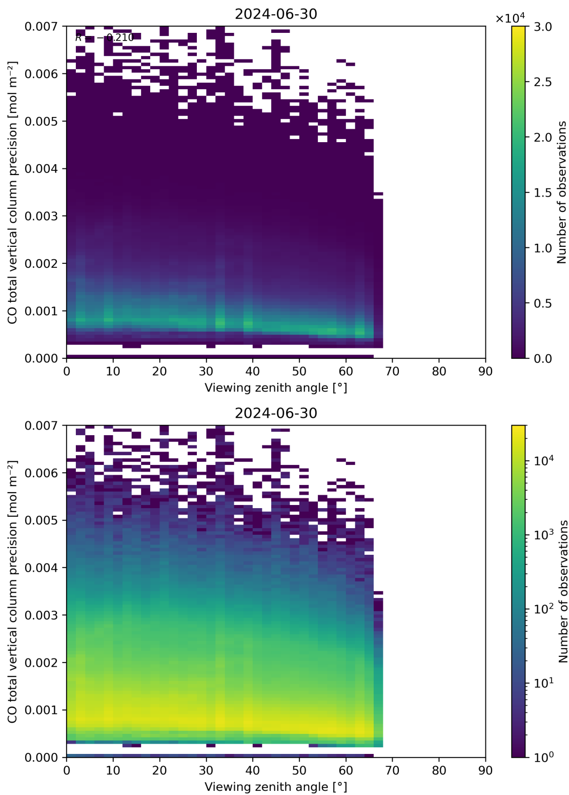
Figure 71: Scatter density plot of “Viewing zenith angle” against “CO total vertical column precision” for 2024-06-29 to 2024-07-01.
