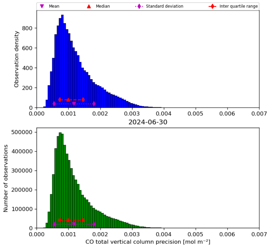
Figure 20: Histogram of “CO total vertical column precision” for 2024-06-29 to 2024-07-01
