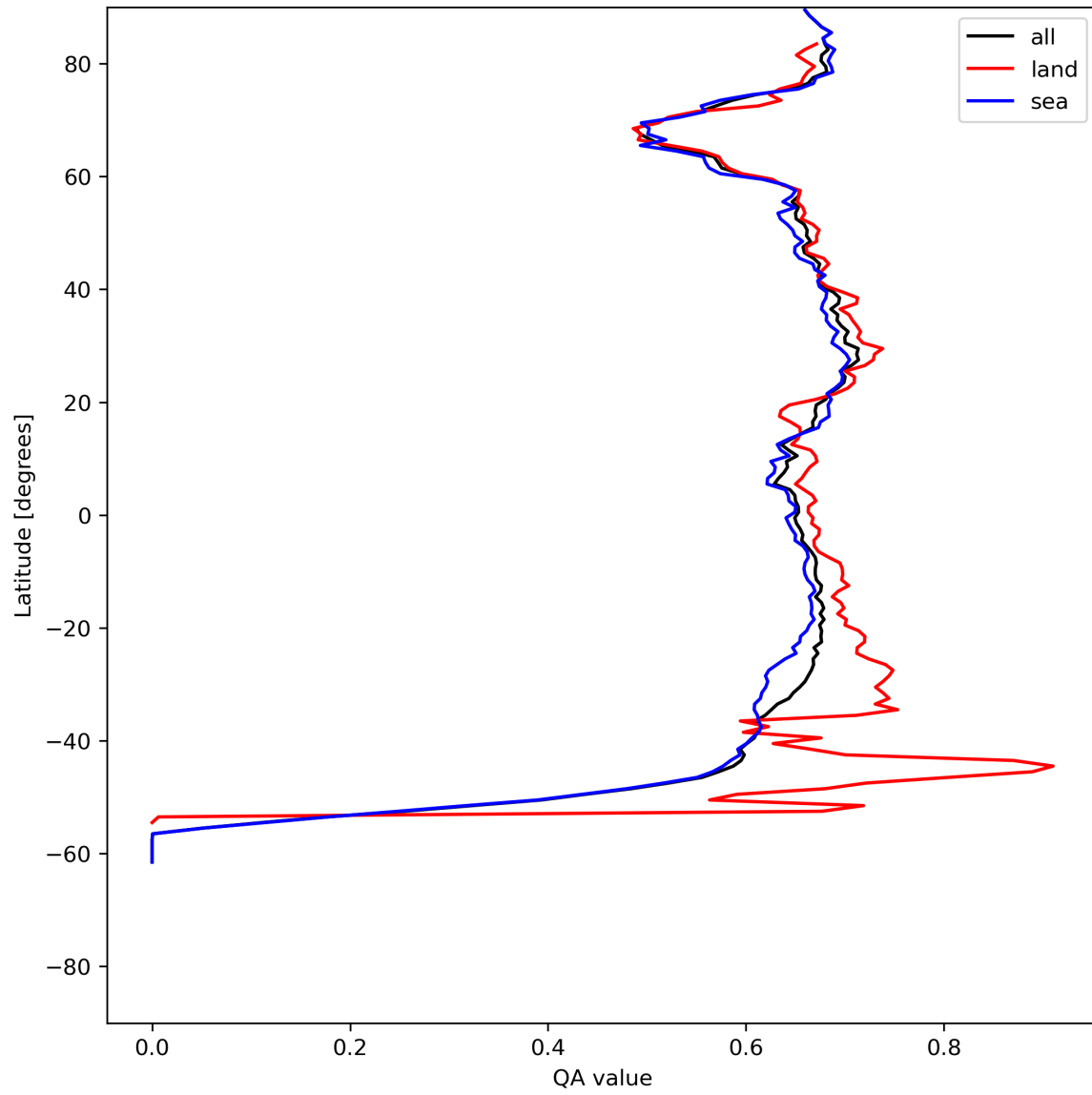
Figure 9: Zonal average of “QA value” for 2024-06-29 to 2024-07-01.
