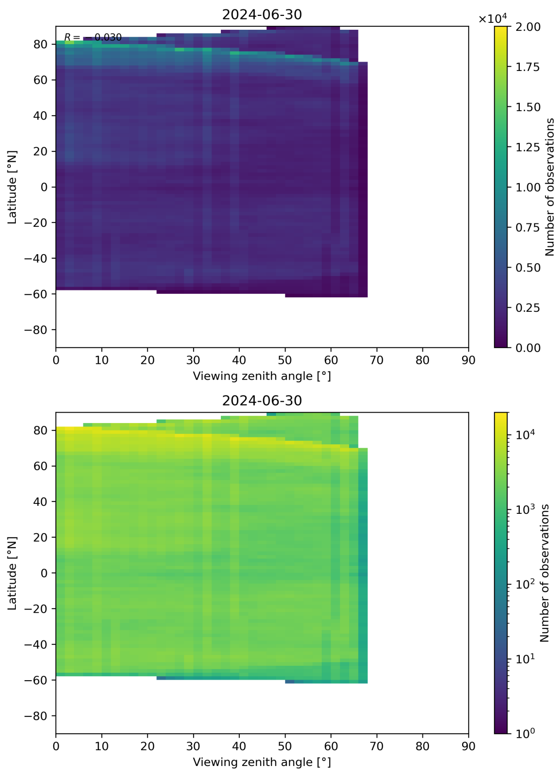
Figure 74: Scatter density plot of “Viewing zenith angle” against “Latitude” for 2024-06-29 to 2024-07-01.
