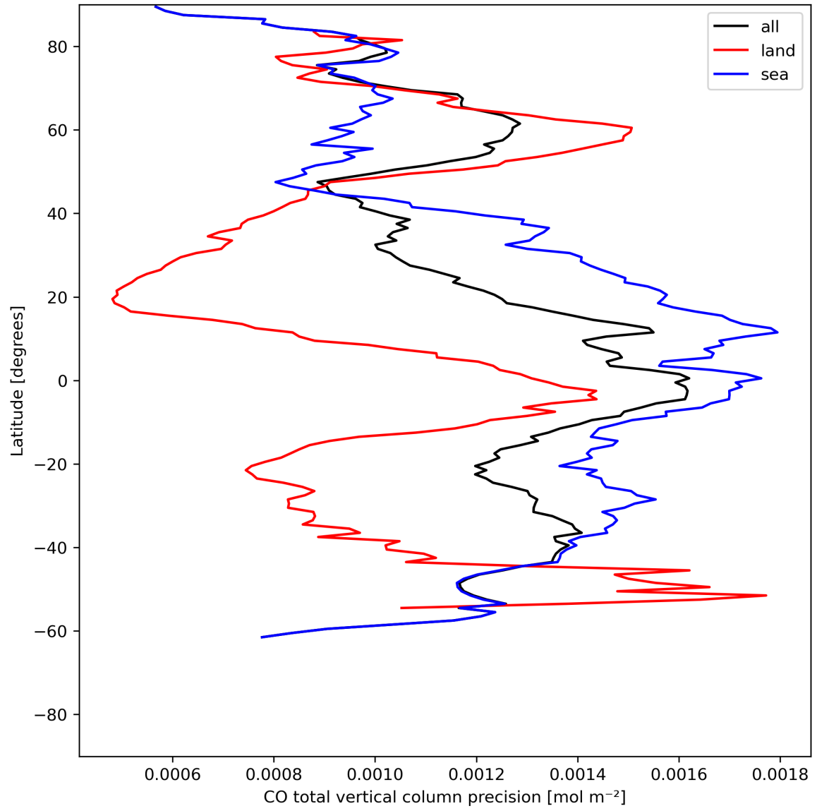
Figure 12: Zonal average of “CO total vertical column precision” for 2024-06-29 to 2024-07-01.
