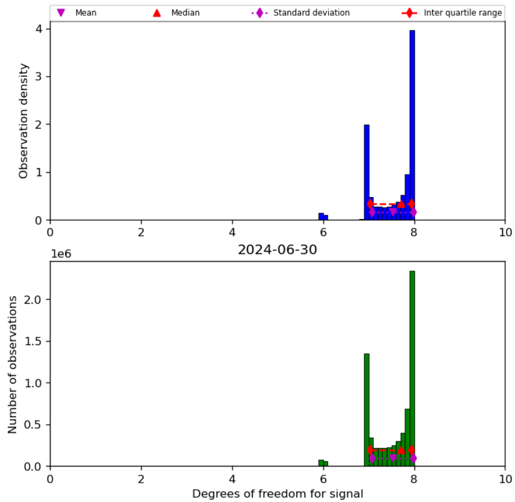
Figure 23: Histogram of “Degrees of freedom for signal” for 2024-06-29 to 2024-07-01
