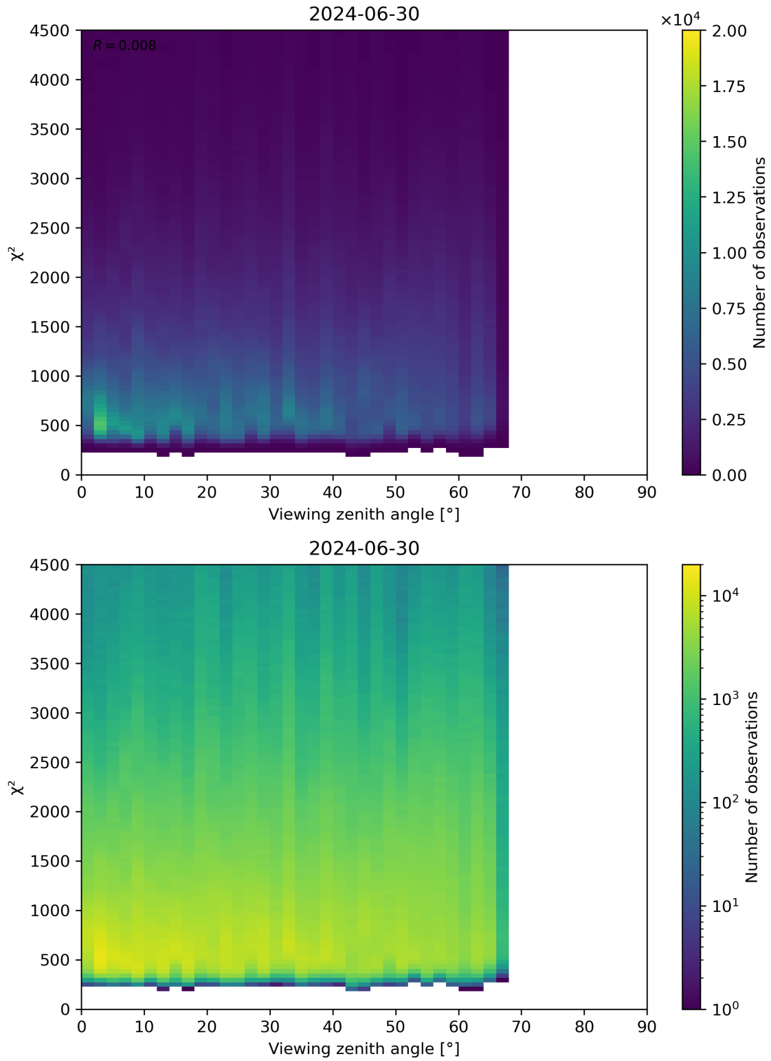
Figure 72: Scatter density plot of “Viewing zenith angle” against “ \chi^2 ” for 2024-06-29 to 2024-07-01.
