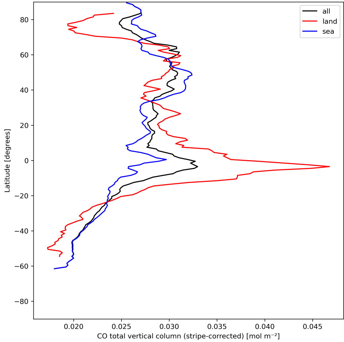
Figure 11: Zonal average of “CO total vertical column (stripe-corrected)” for 2024-06-29 to 2024-07-01.
