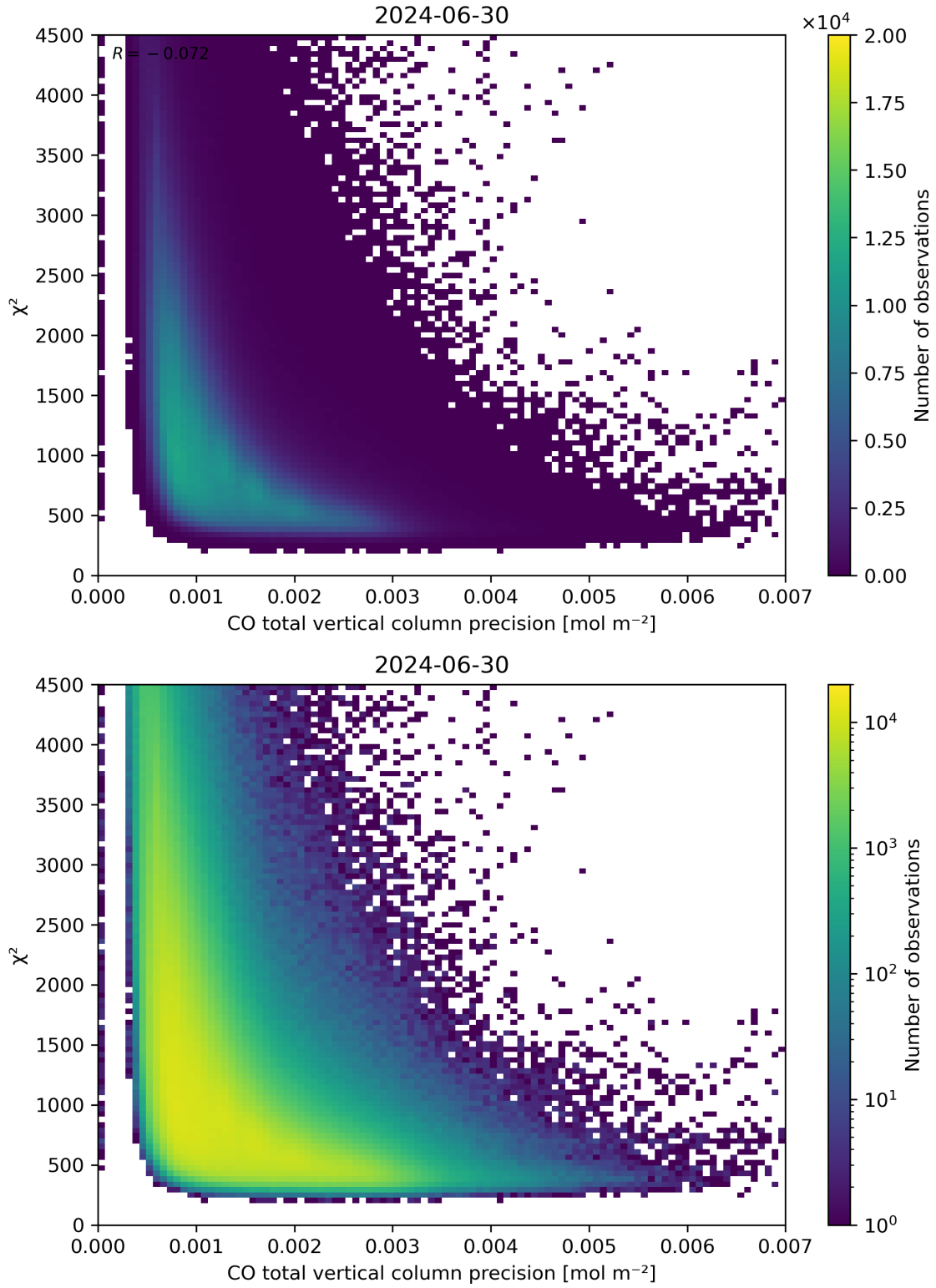
Figure 44: Scatter density plot of “CO total vertical column precision” against “ \chi^2 ” for 2024-06-29 to 2024-07-01.
