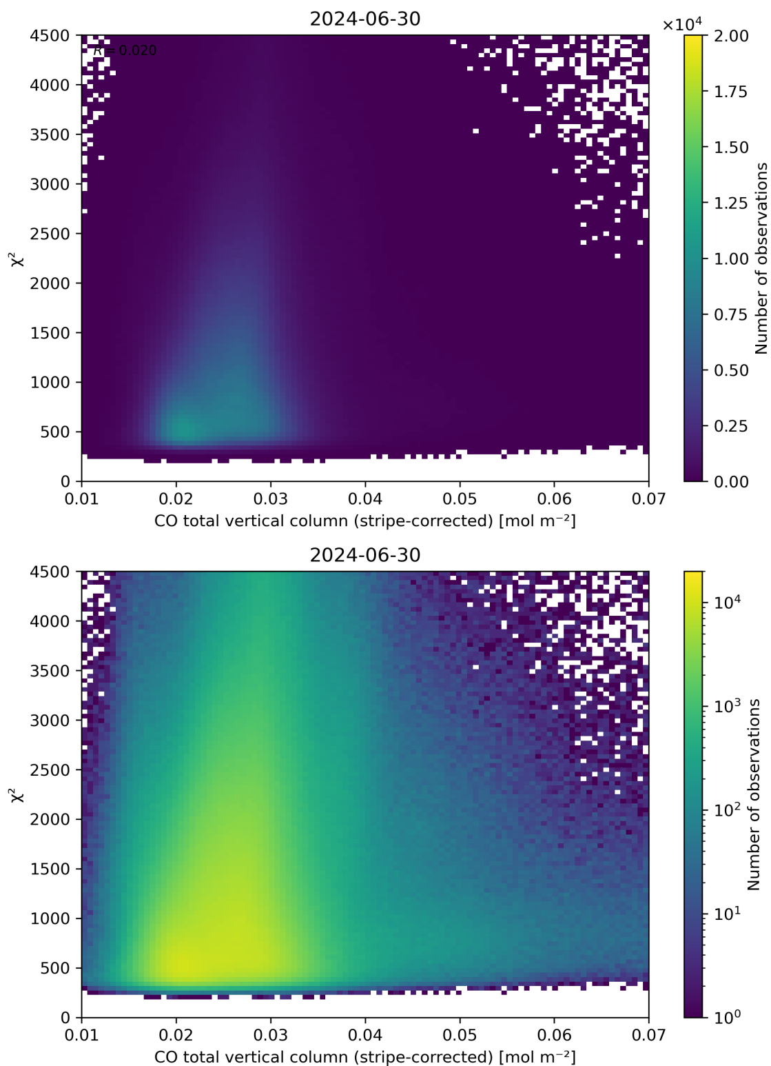
Figure 37: Scatter density plot of “CO total vertical column (stripe-corrected)” against “ \chi^2 ” for 2024-06-29 to 2024-07-01.
