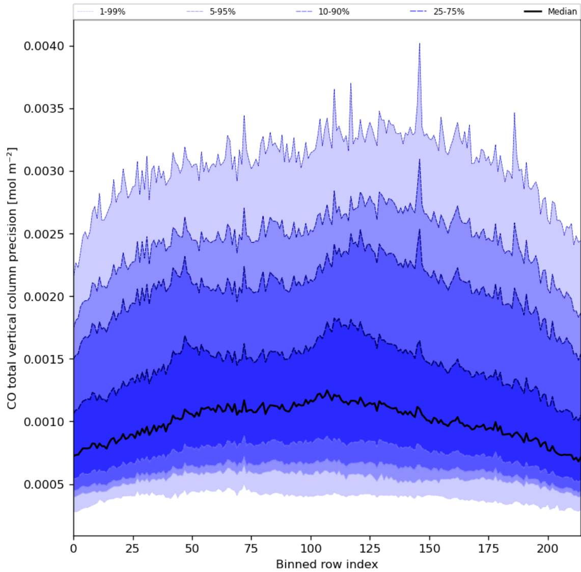
Figure 28: Along track statistics of “CO total vertical column precision” for 2024-06-29 to 2024-07-01
