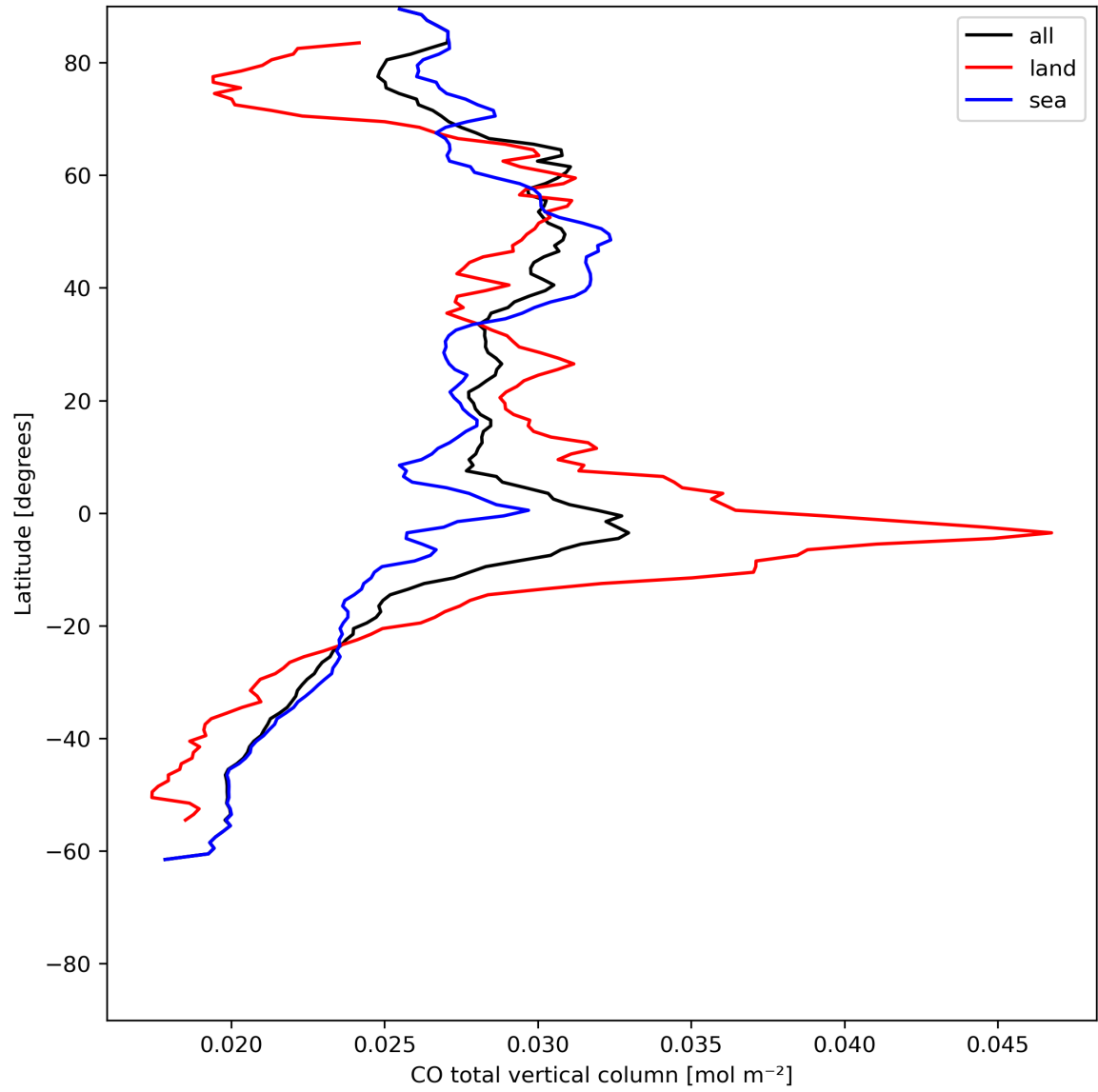
Figure 10: Zonal average of “CO total vertical column” for 2024-06-29 to 2024-07-01.
