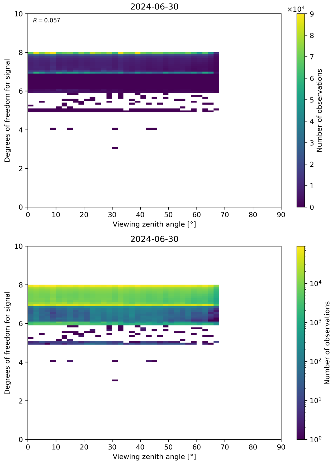
Figure 73: Scatter density plot of “Viewing zenith angle” against “Degrees of freedom for signal” for 2024-06-29 to 2024-07-01.
