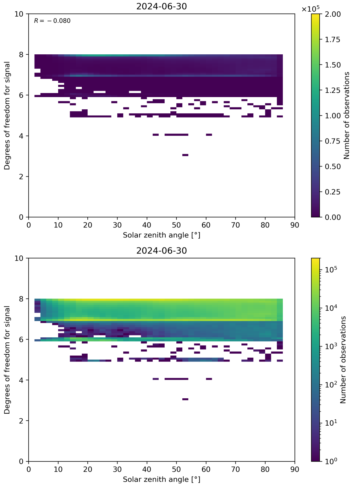
Figure 65: Scatter density plot of “Solar zenith angle” against “Degrees of freedom for signal” for 2024-06-29 to 2024-07-01.
