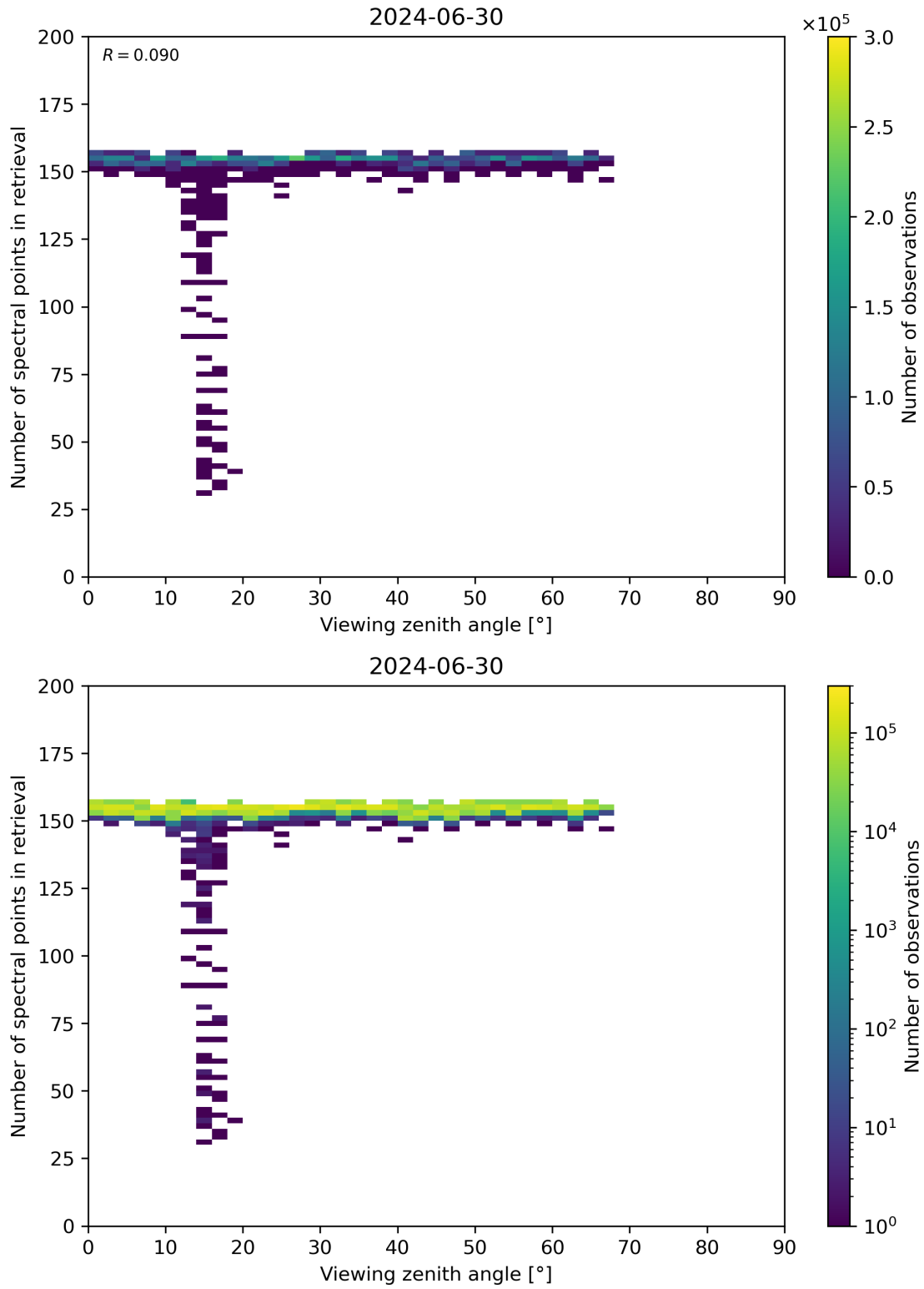
Figure 76: Scatter density plot of “Viewing zenith angle” against “Number of spectral points in retrieval” for 2024-06-29 to 2024-07-01.
