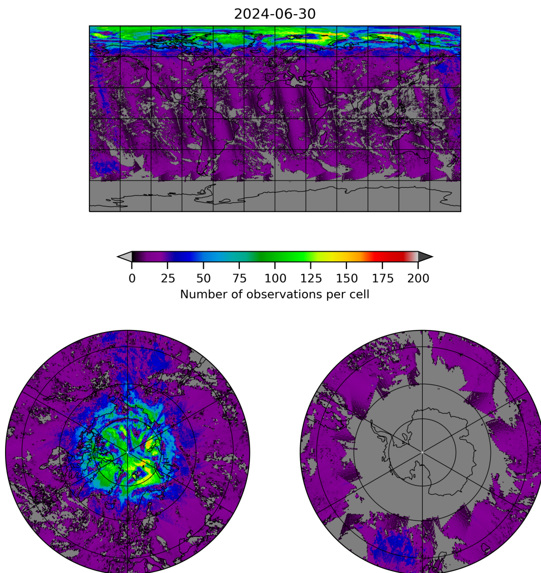
Figure 8: Map of the number of observations for 2024-06-29 to 2024-07-01
