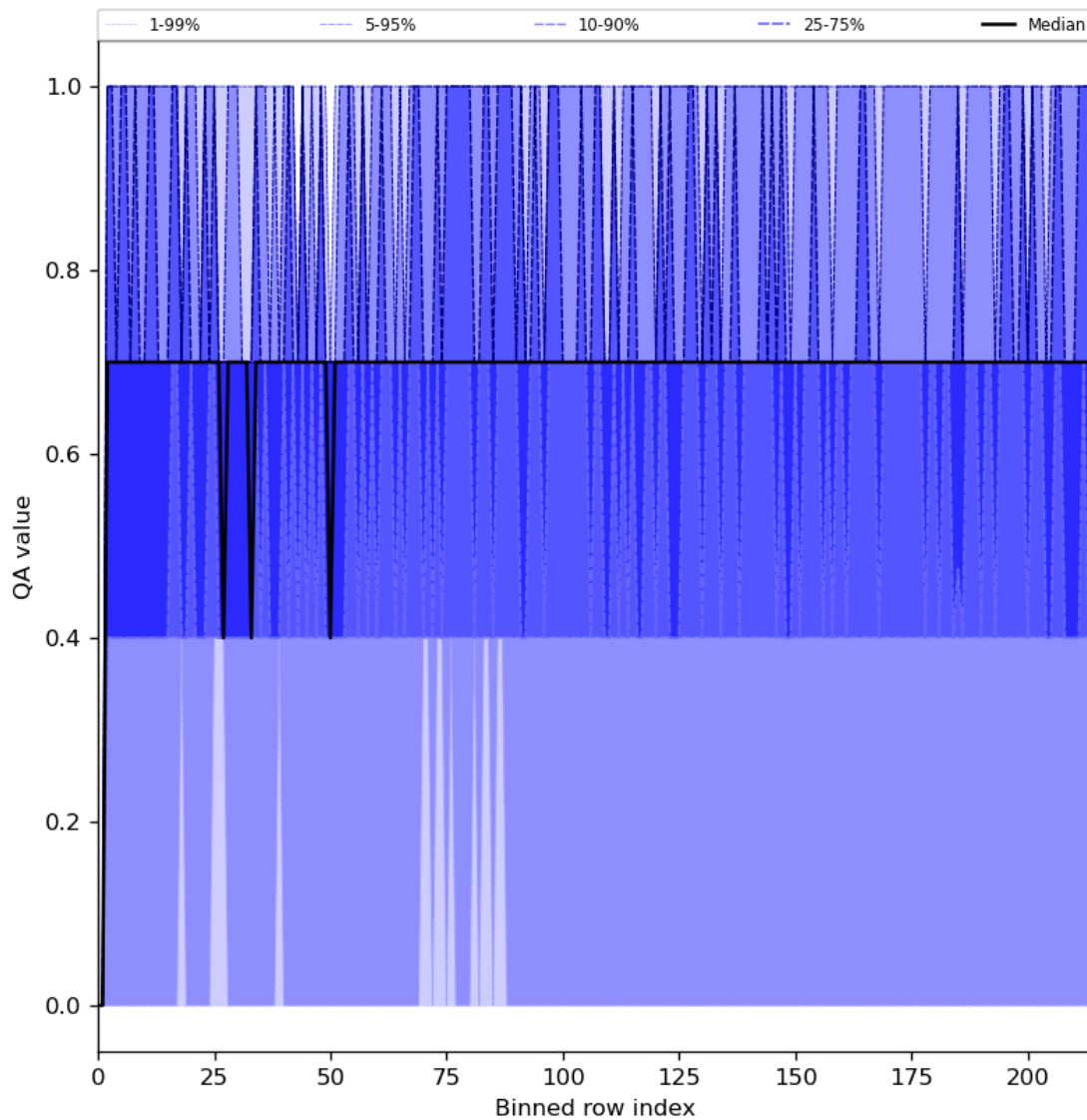
Figure 25: Along track statistics of “QA value” for 2024-06-29 to 2024-07-01
