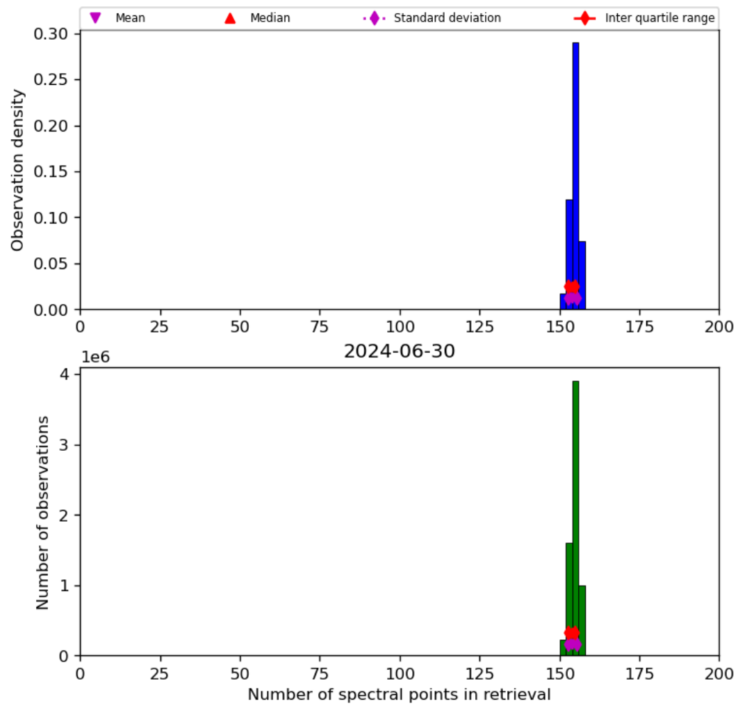
Figure 21: Histogram of “Number of spectral points in retrieval” for 2024-06-29 to 2024-07-01
