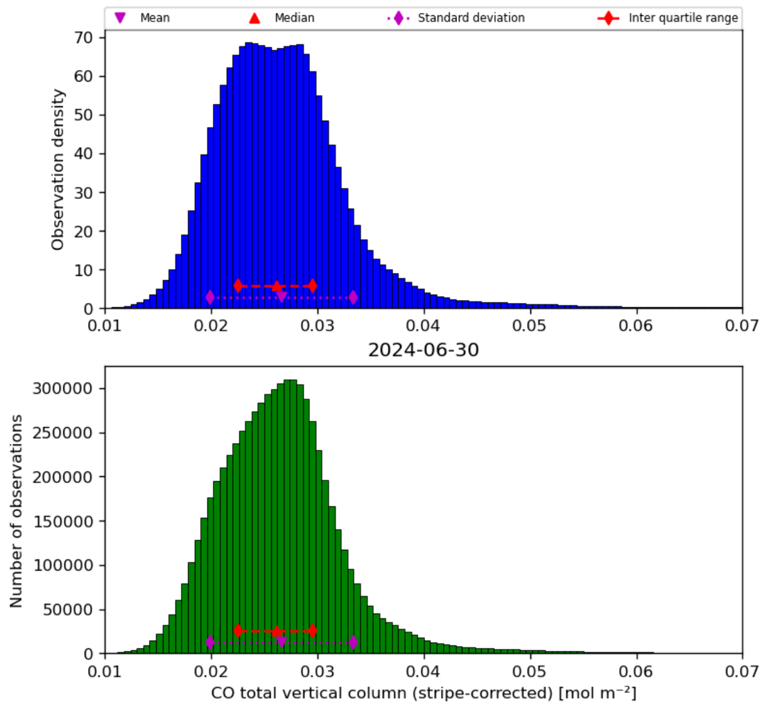
Figure 19: Histogram of “CO total vertical column (stripe-corrected)” for 2024-06-29 to 2024-07-01
