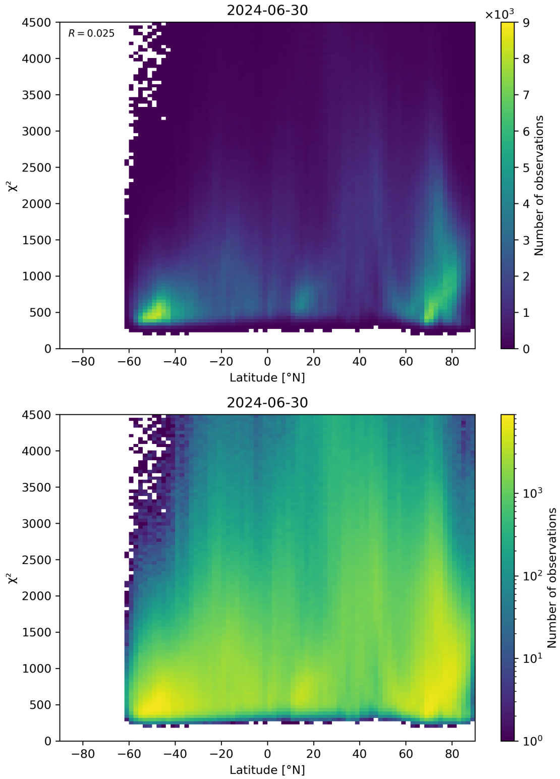
Figure 54: Scatter density plot of “Latitude” against “ \chi^2 ” for 2024-06-29 to 2024-07-01.
