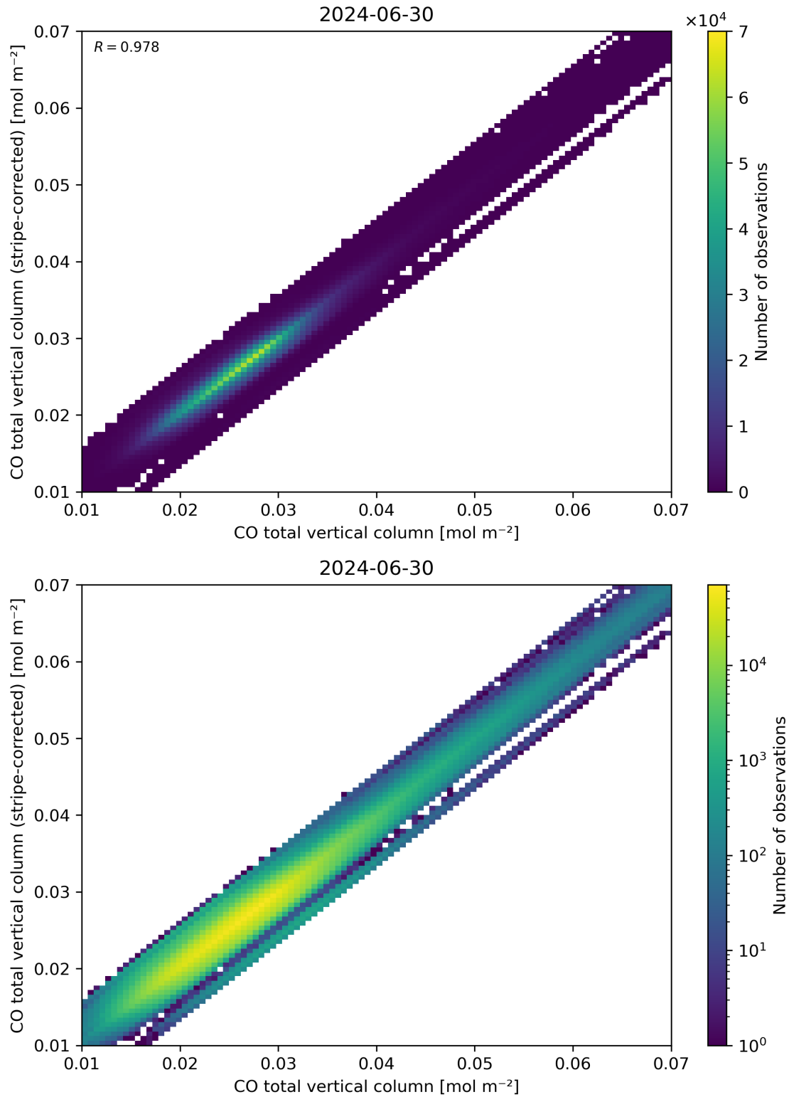
Figure 33: Scatter density plot of “CO total vertical column” against “CO total vertical column (stripe-corrected)” for 2024-06-29 to 2024-07-01.
