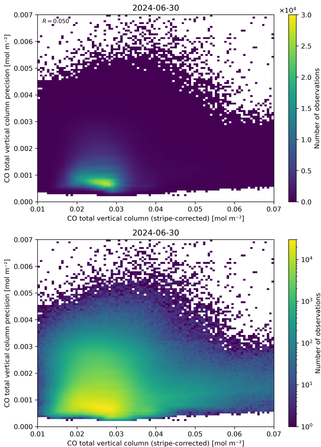
Figure 36: Scatter density plot of “CO total vertical column (stripe-corrected)” against “CO total vertical column precision” for 2024-06-29 to 2024-07-01.
