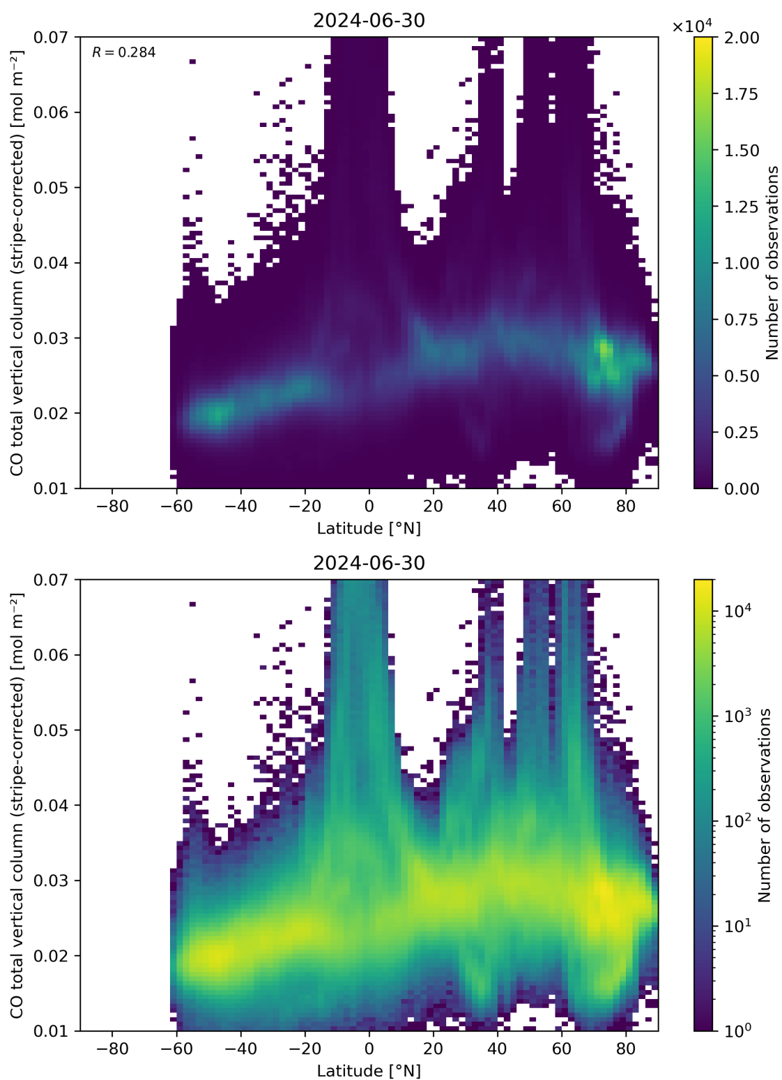
Figure 52: Scatter density plot of “Latitude” against “CO total vertical column (stripe-corrected)” for 2024-06-29 to 2024-07-01.
