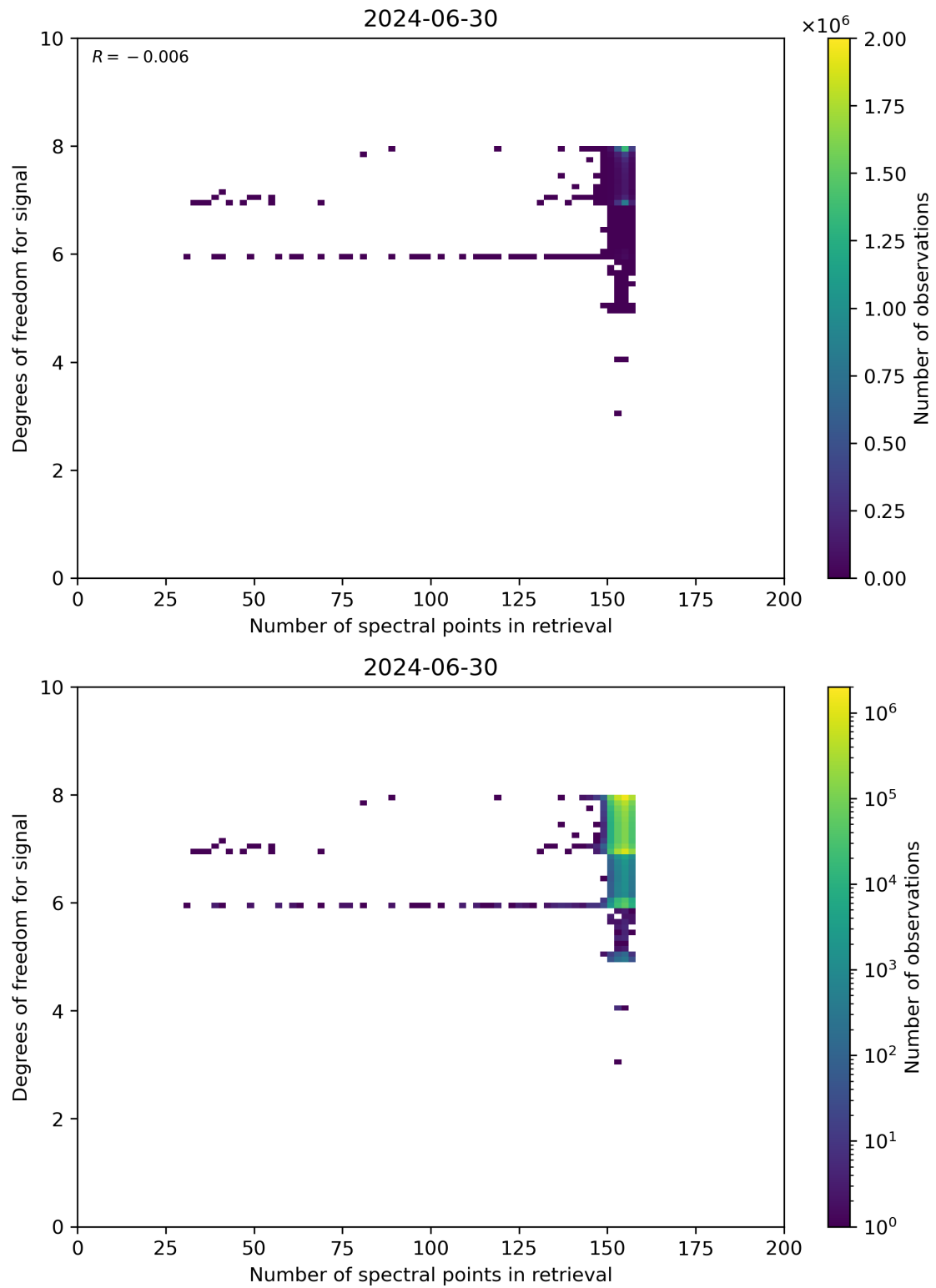
Figure 59: Scatter density plot of “Number of spectral points in retrieval” against “Degrees of freedom for signal” for 2024-06-29 to 2024-07-01.
