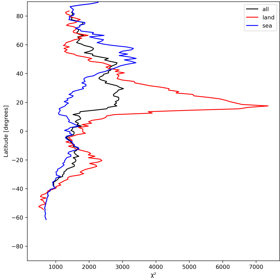
Figure 14: Zonal average of “ \chi^2 ” for 2024-06-29 to 2024-07-01.
