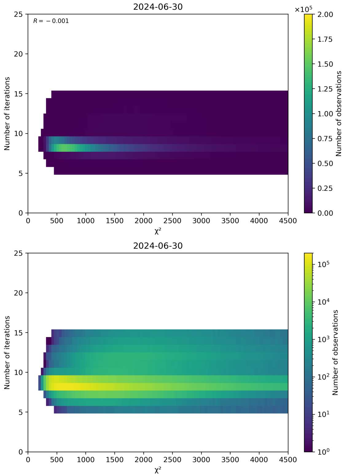
Figure 49: Scatter density plot of “ \chi^2 ” against “Number of iterations” for 2024-06-29 to 2024-07-01.
