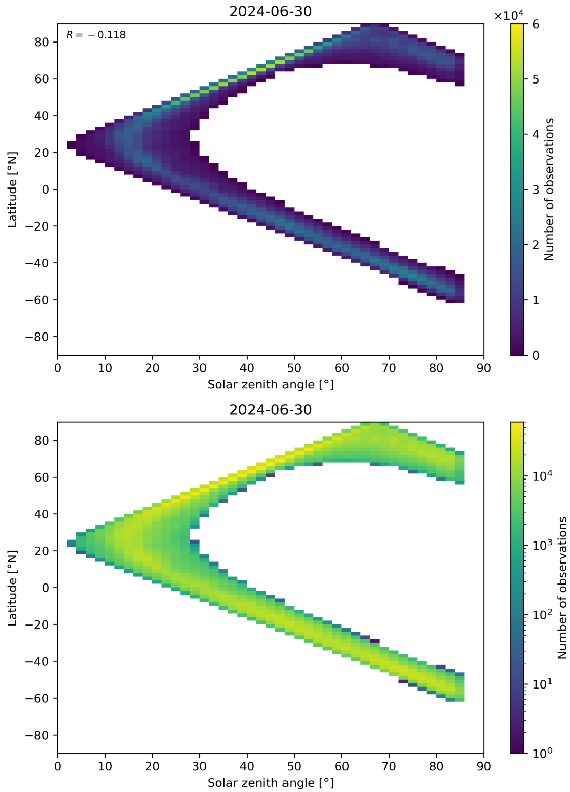
Figure 66: Scatter density plot of “Solar zenith angle” against “Latitude” for 2024-06-29 to 2024-07-01.
