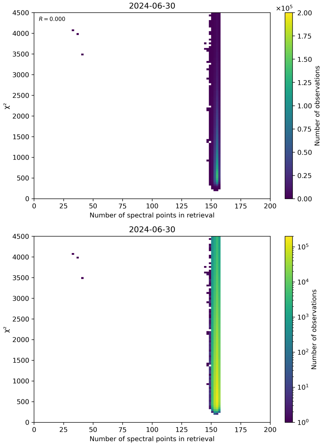
Figure 58: Scatter density plot of “Number of spectral points in retrieval” against “ \chi^2 ” for 2024-06-29 to 2024-07-01.
