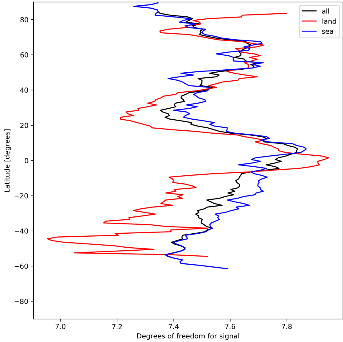
Figure 15: Zonal average of “Degrees of freedom for signal” for 2024-06-29 to 2024-07-01.
