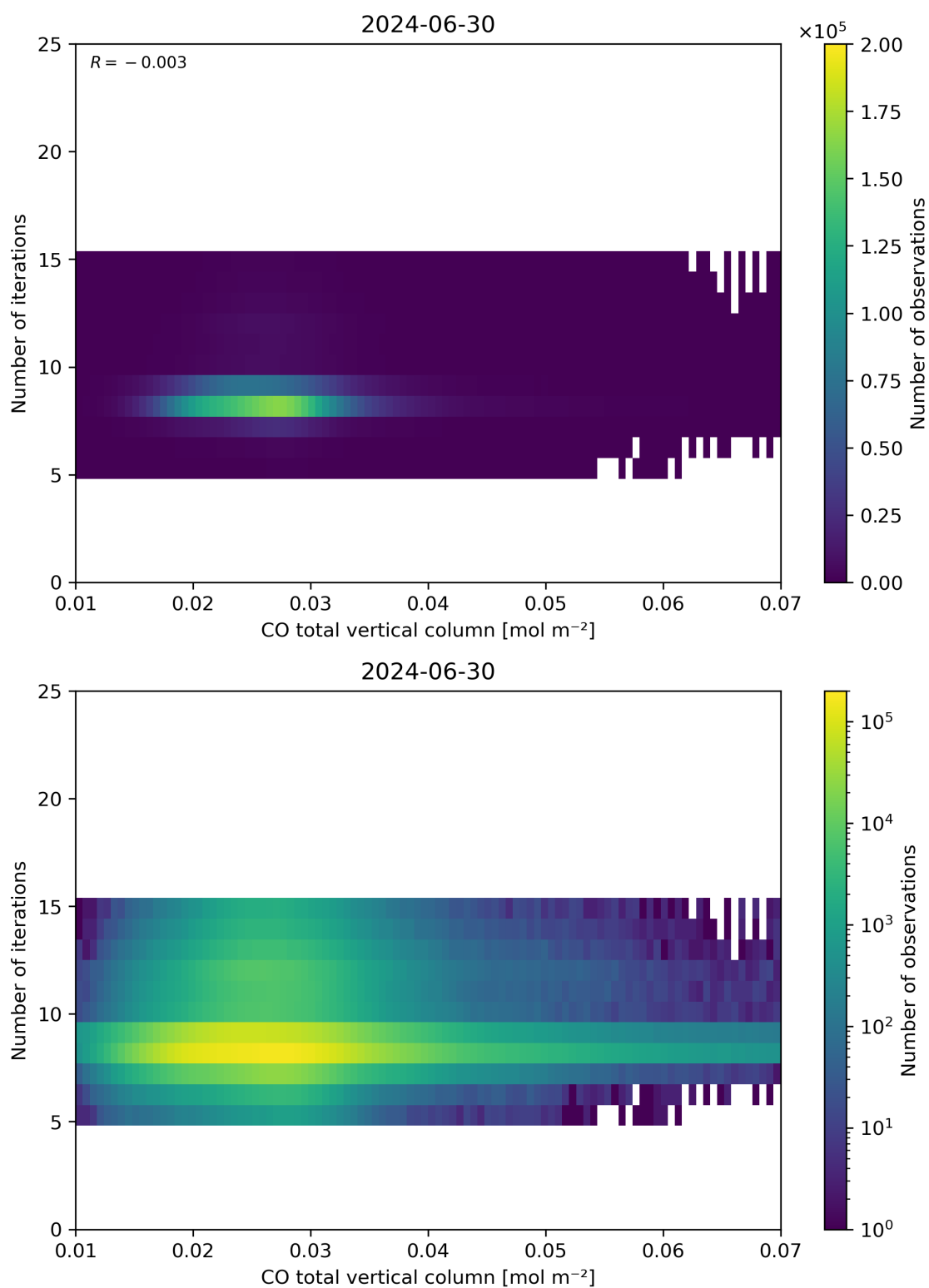
Figure 42: Scatter density plot of “CO total vertical column” against “Number of iterations” for 2024-06-29 to 2024-07-01.
