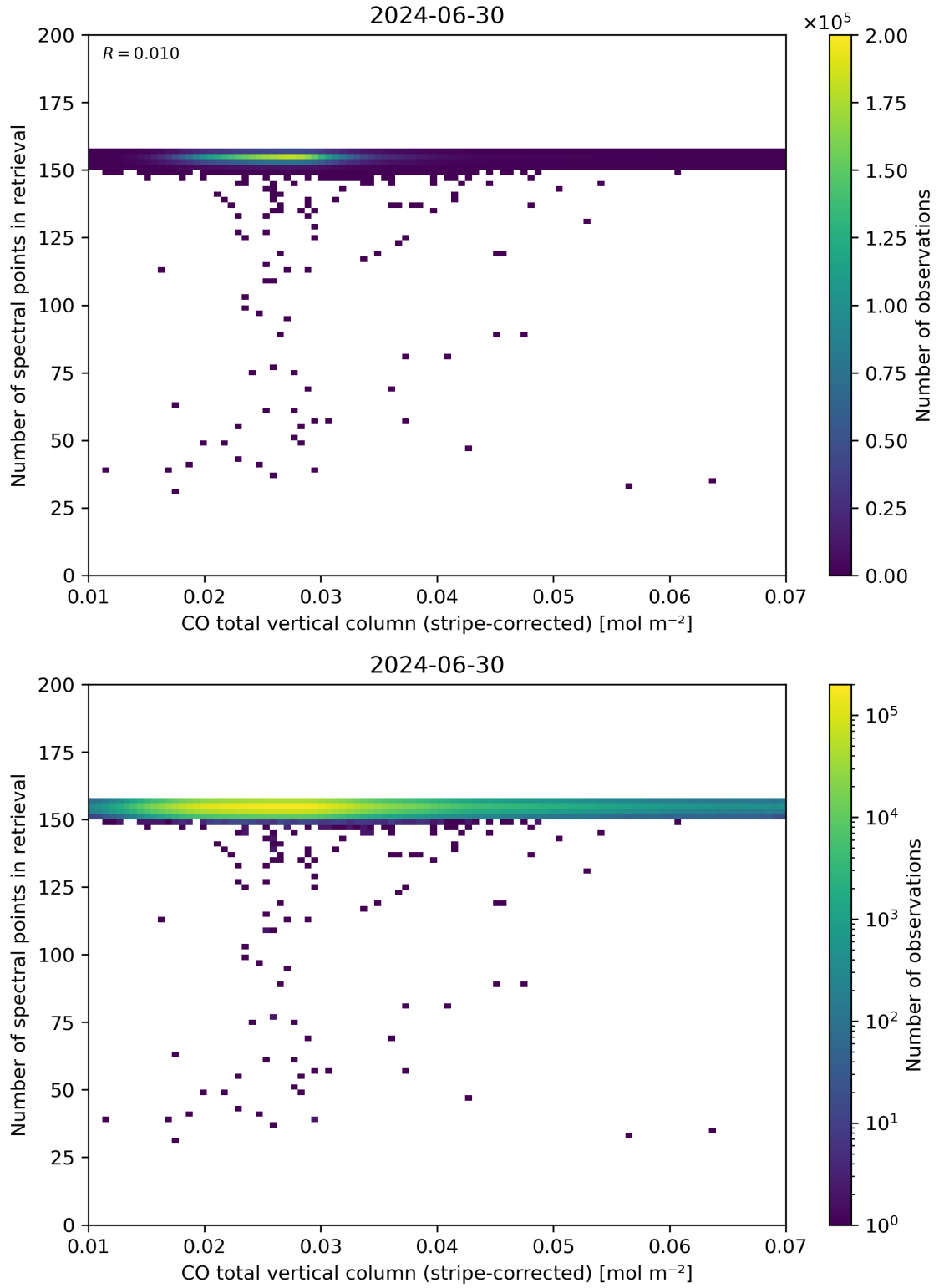
Figure 40: Scatter density plot of “CO total vertical column (stripe-corrected)” against “Number of spectral points in retrieval” for 2024-06-29 to 2024-07-01.
