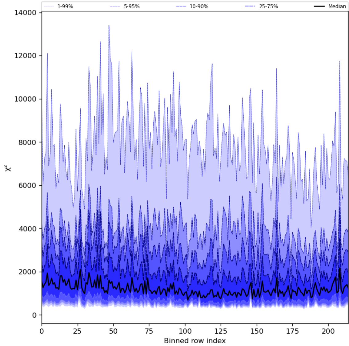
Figure 30: Along track statistics of “ \chi^2 ” for 2024-06-29 to 2024-07-01
