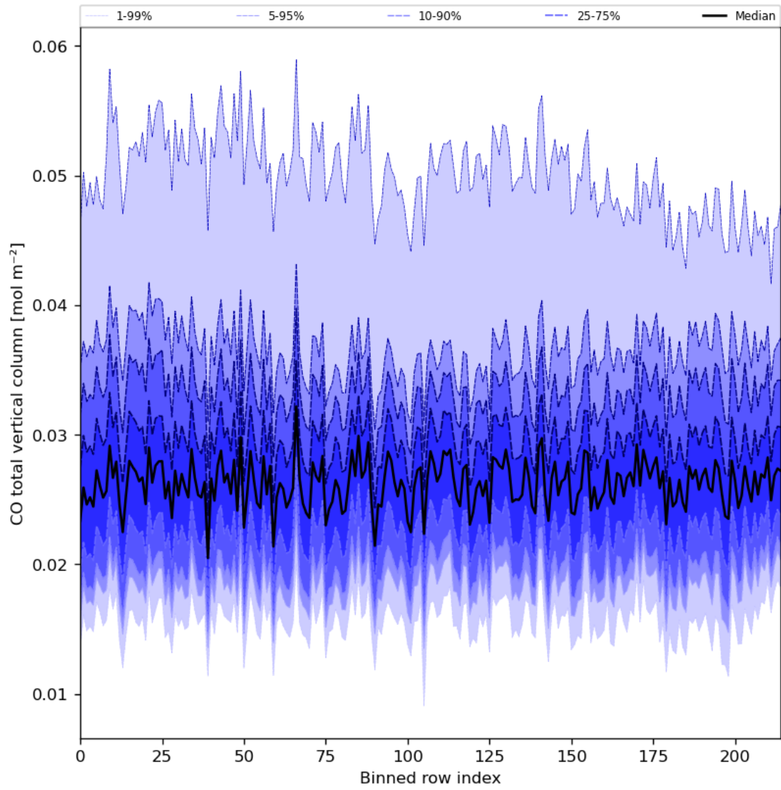
Figure 26: Along track statistics of “CO total vertical column” for 2024-06-29 to 2024-07-01
