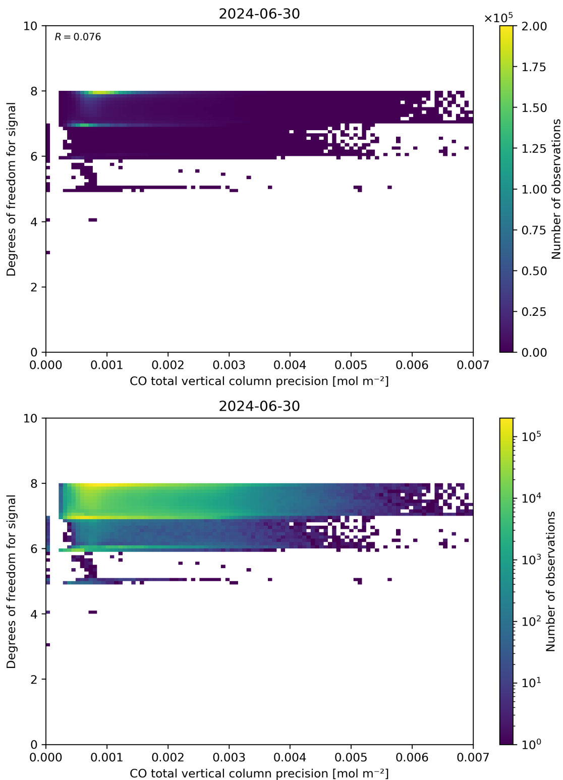
Figure 45: Scatter density plot of “CO total vertical column precision” against “Degrees of freedom for signal” for 2024-06-29 to 2024-07-01.
