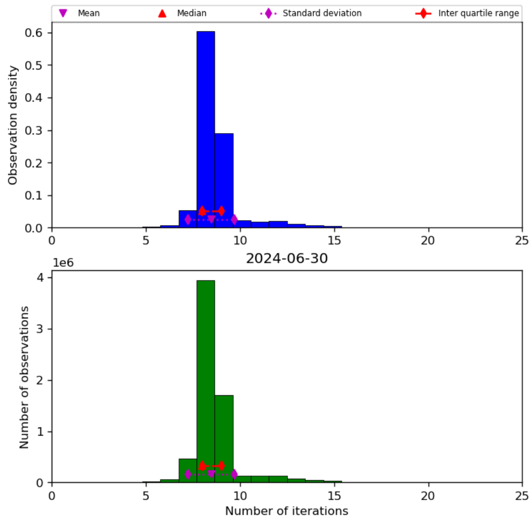
Figure 24: Histogram of “Number of iterations” for 2024-06-29 to 2024-07-01
