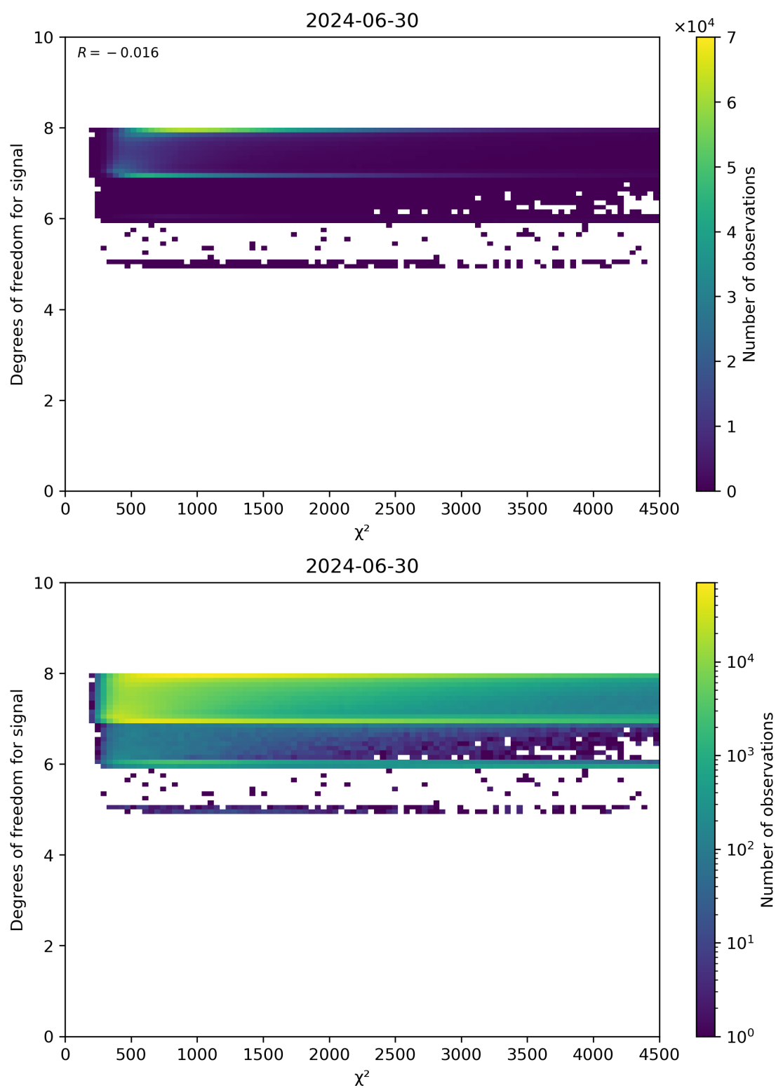
Figure 48: Scatter density plot of “ \chi^2 ” against “Degrees of freedom for signal” for 2024-06-29 to 2024-07-01.
