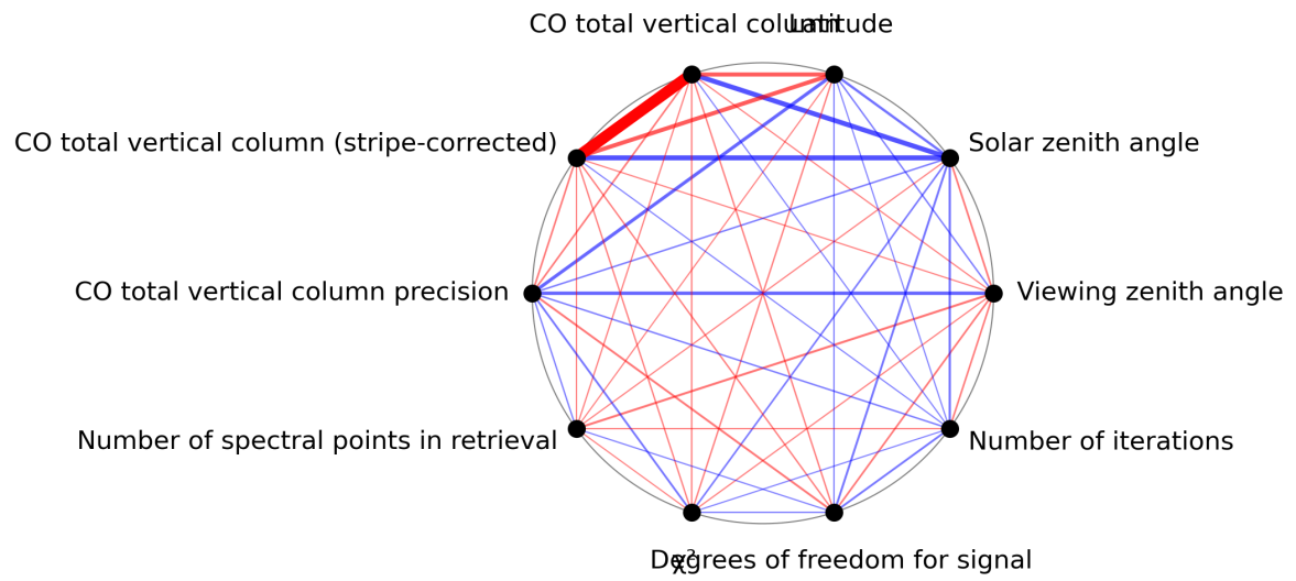
Figure 1: Map of correlation graph for 2024-06-29 to 2024-07-01.
