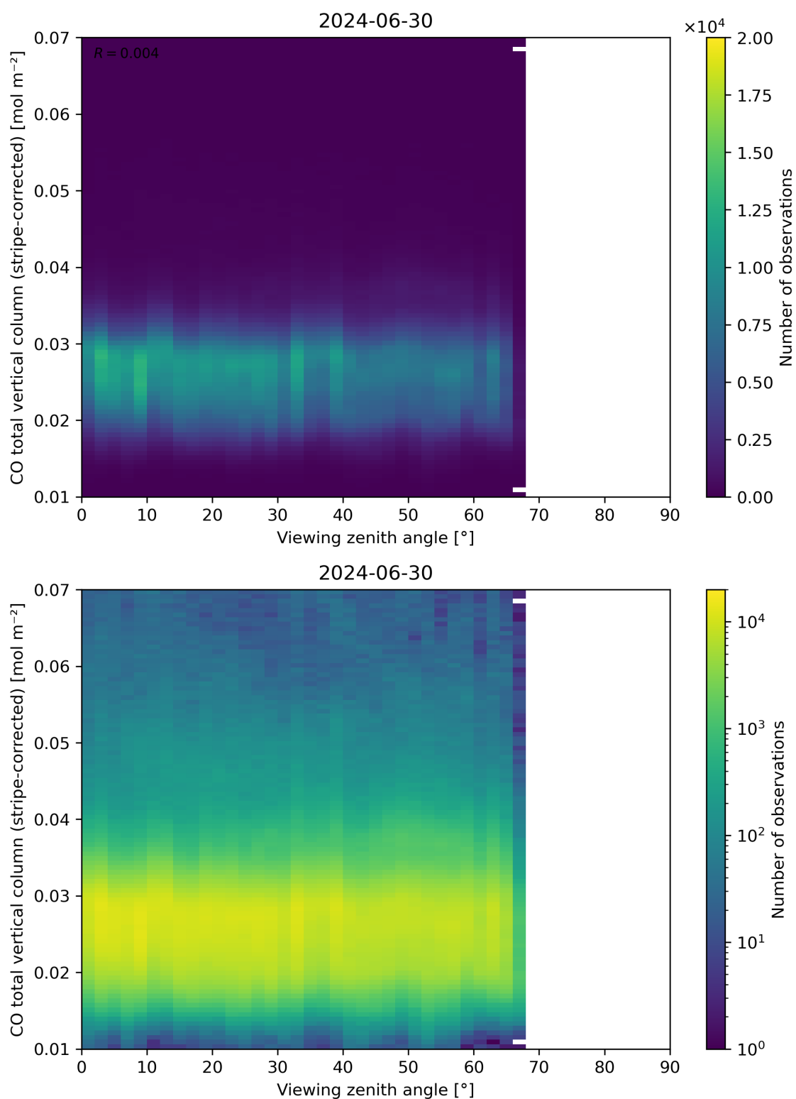
Figure 70: Scatter density plot of “Viewing zenith angle” against “CO total vertical column (stripe-corrected)” for 2024-06-29 to 2024-07-01.
