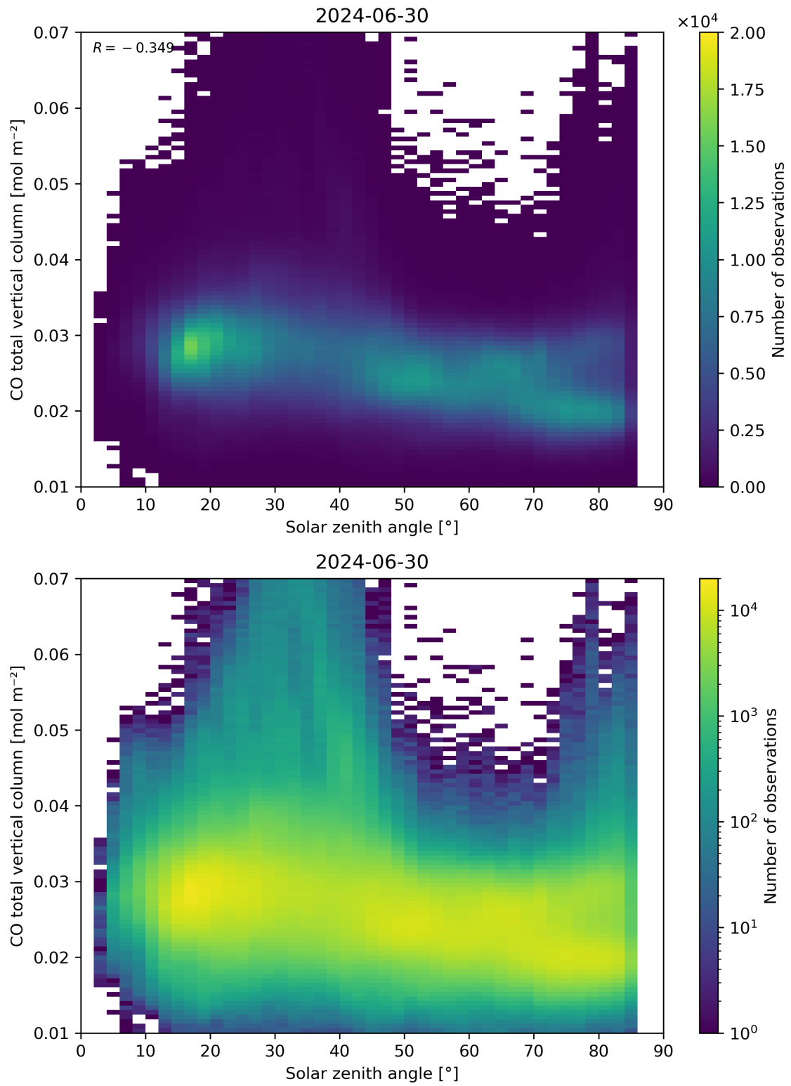
Figure 61: Scatter density plot of “Solar zenith angle” against “CO total vertical column” for 2024-06-29 to 2024-07-01.
