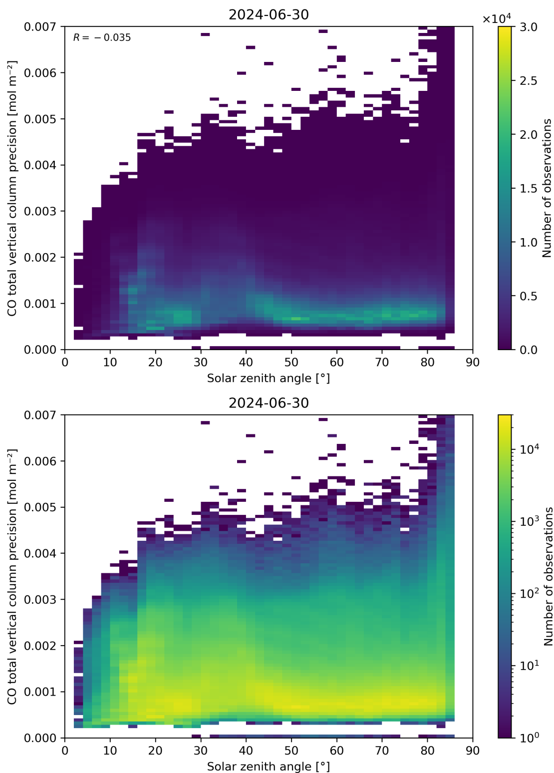
Figure 63: Scatter density plot of “Solar zenith angle” against “CO total vertical column precision” for 2024-06-29 to 2024-07-01.
