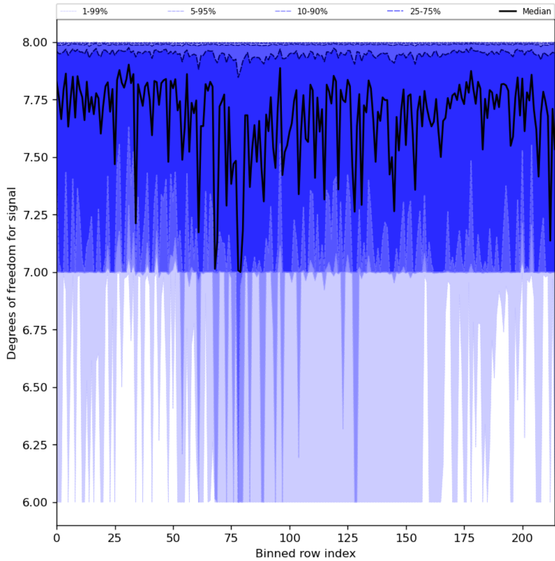
Figure 31: Along track statistics of “Degrees of freedom for signal” for 2024-06-29 to 2024-07-01
