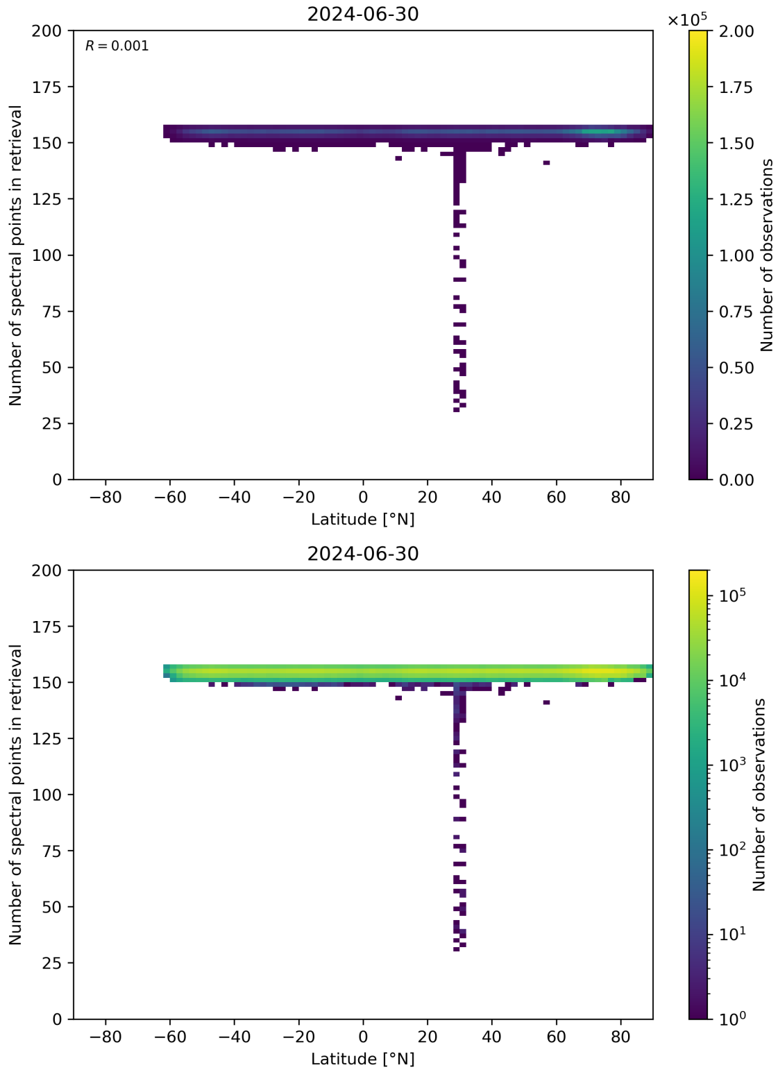
Figure 57: Scatter density plot of “Latitude” against “Number of spectral points in retrieval” for 2024-06-29 to 2024-07-01.
