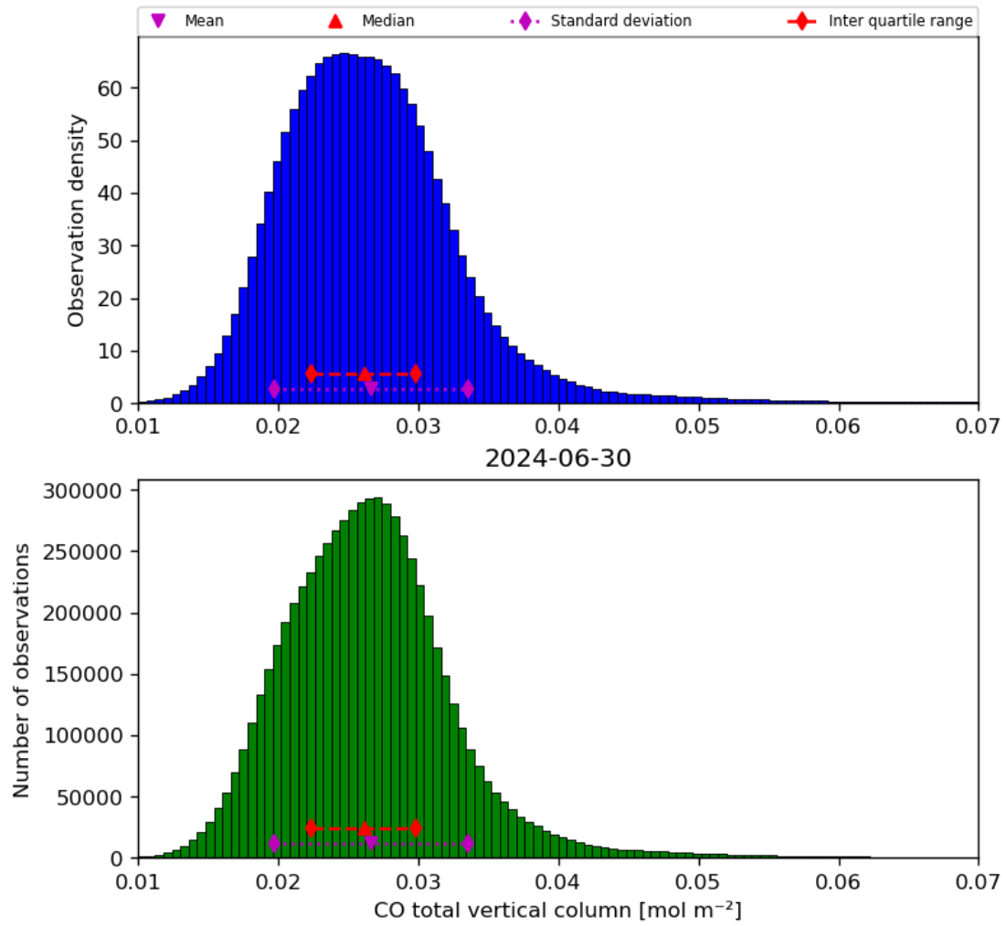
Figure 18: Histogram of “CO total vertical column” for 2024-06-29 to 2024-07-01
