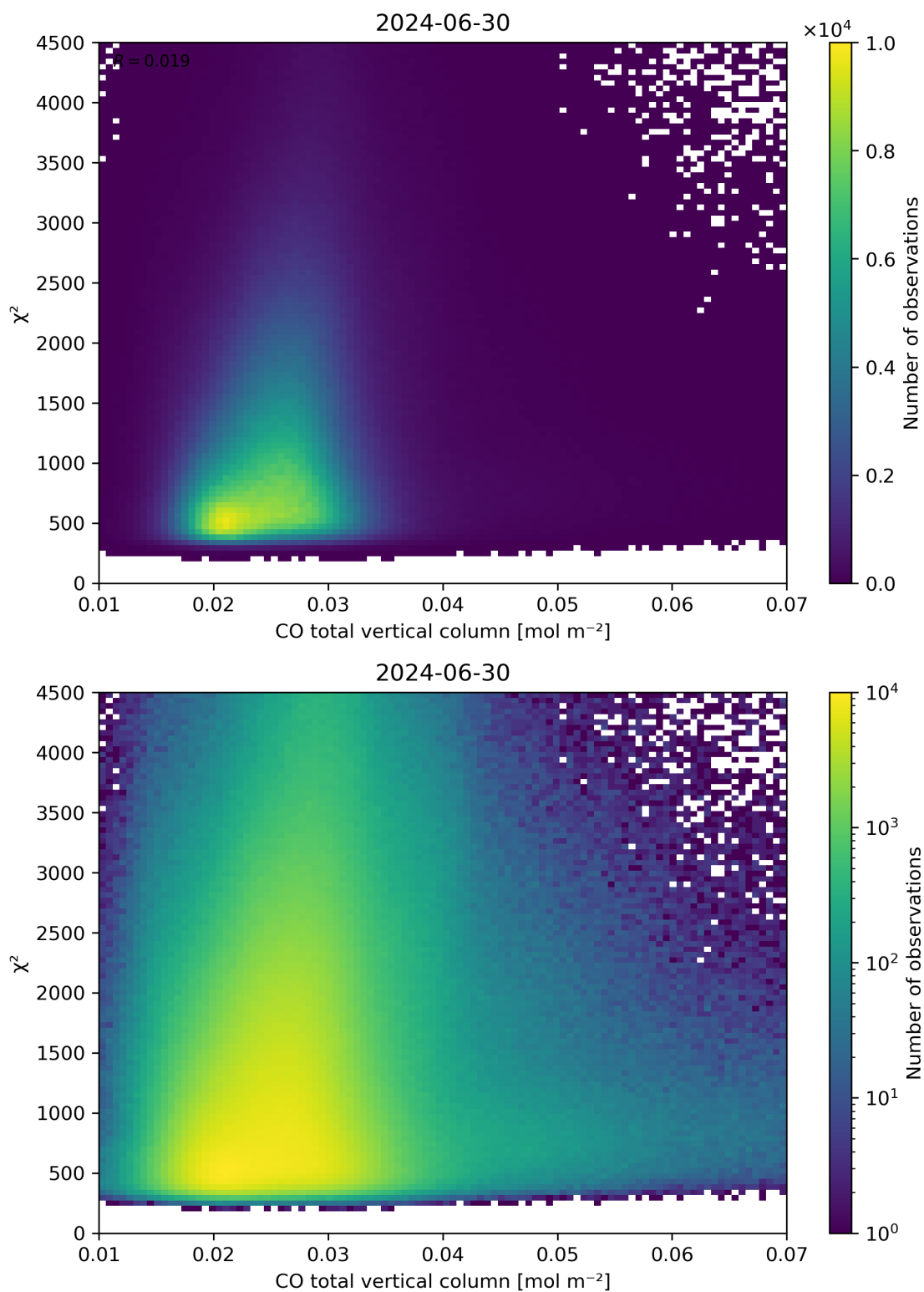
Figure 35: Scatter density plot of “CO total vertical column” against “ \chi^2 ” for 2024-06-29 to 2024-07-01.
