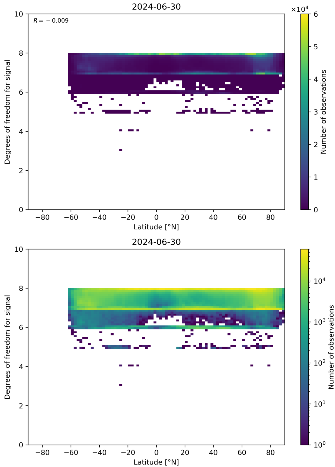
Figure 55: Scatter density plot of “Latitude” against “Degrees of freedom for signal” for 2024-06-29 to 2024-07-01.
