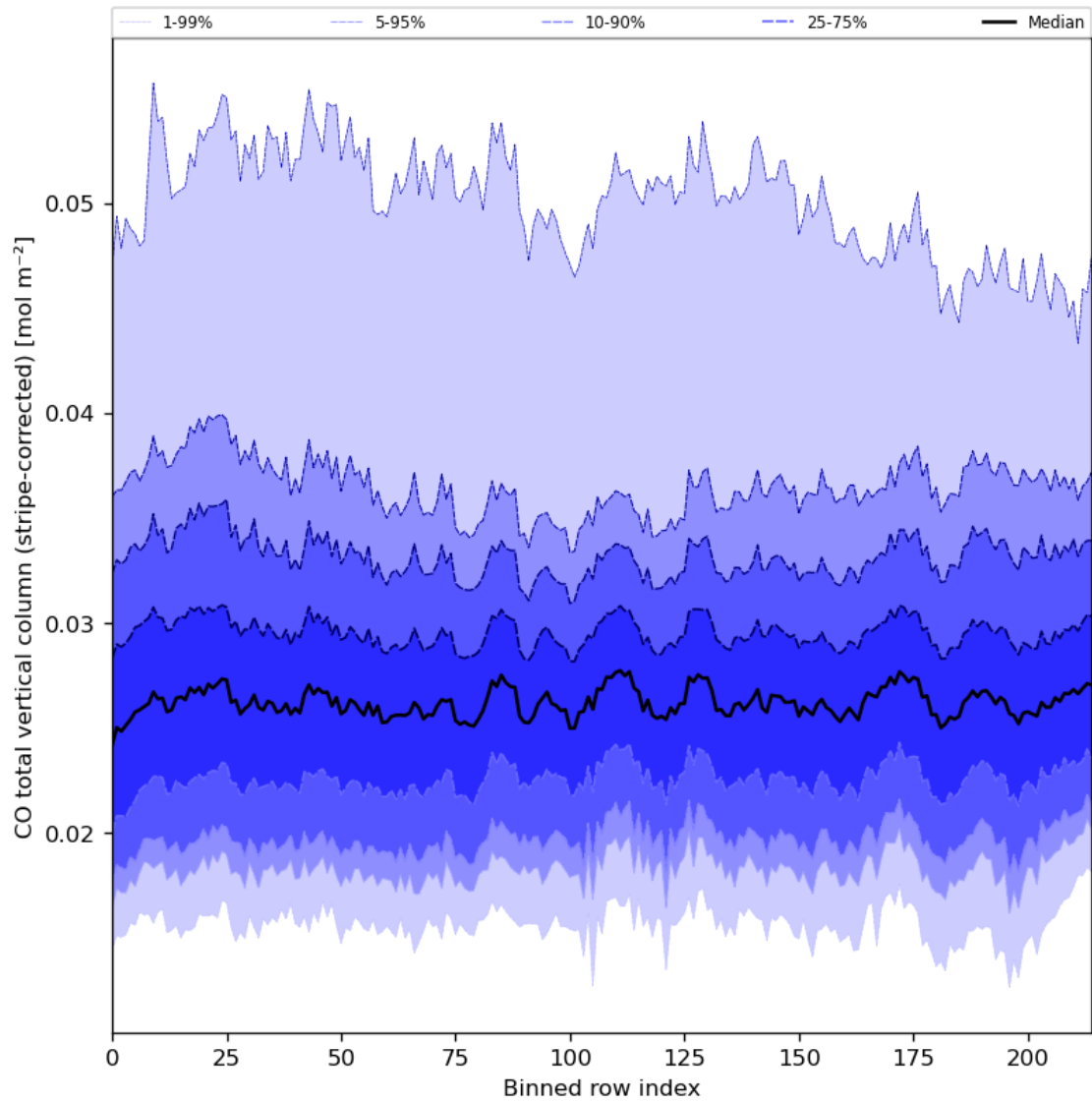
Figure 27: Along track statistics of “CO total vertical column (stripe-corrected)” for 2024-06-29 to 2024-07-01
