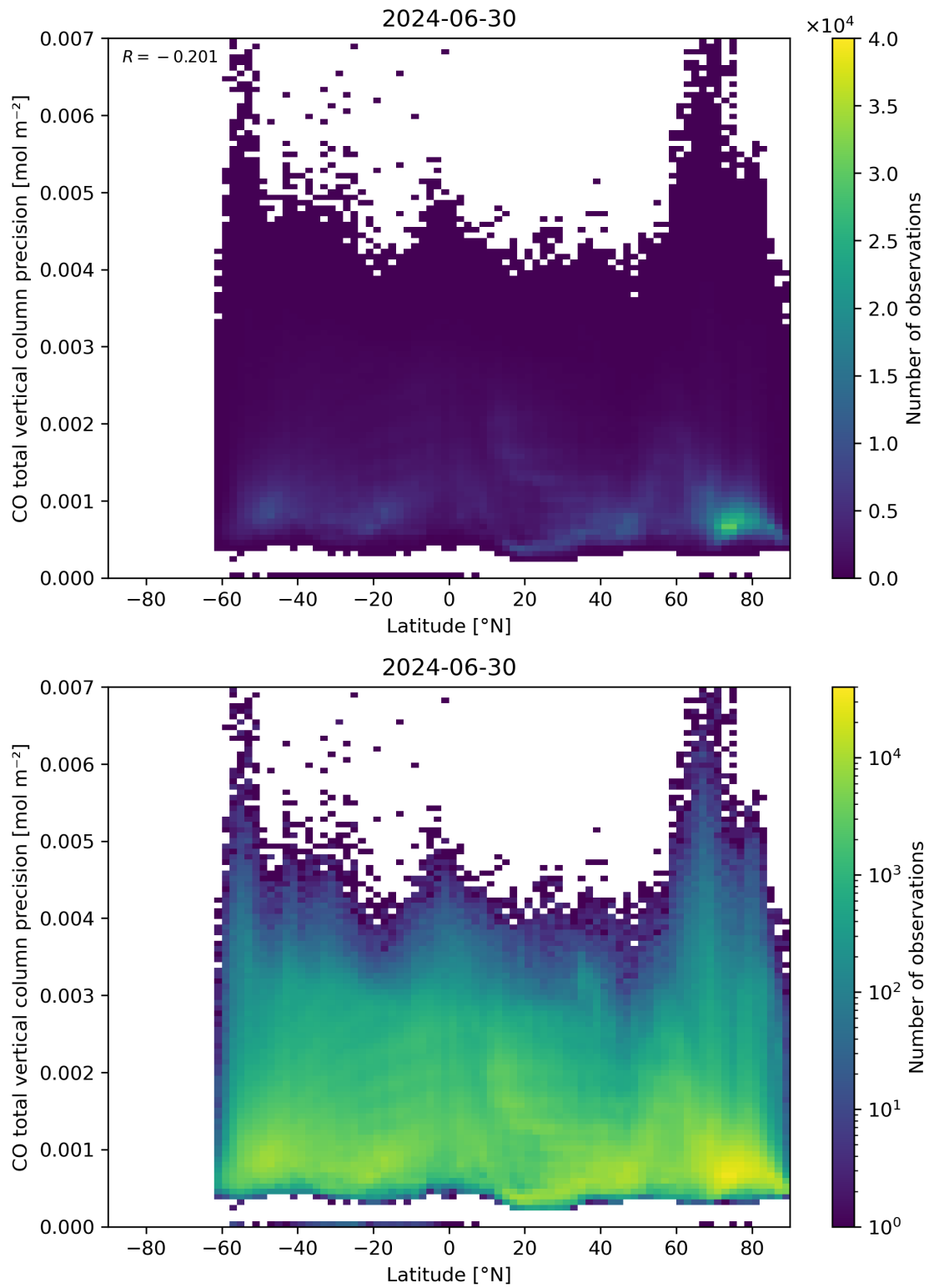
Figure 53: Scatter density plot of “Latitude” against “CO total vertical column precision” for 2024-06-29 to 2024-07-01.
