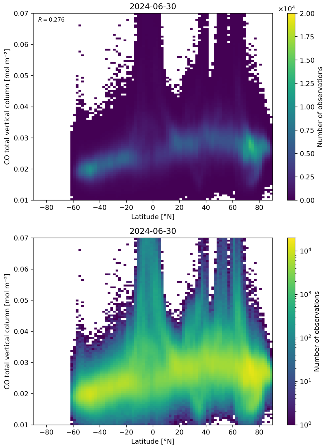
Figure 51: Scatter density plot of “Latitude” against “CO total vertical column” for 2024-06-29 to 2024-07-01.
