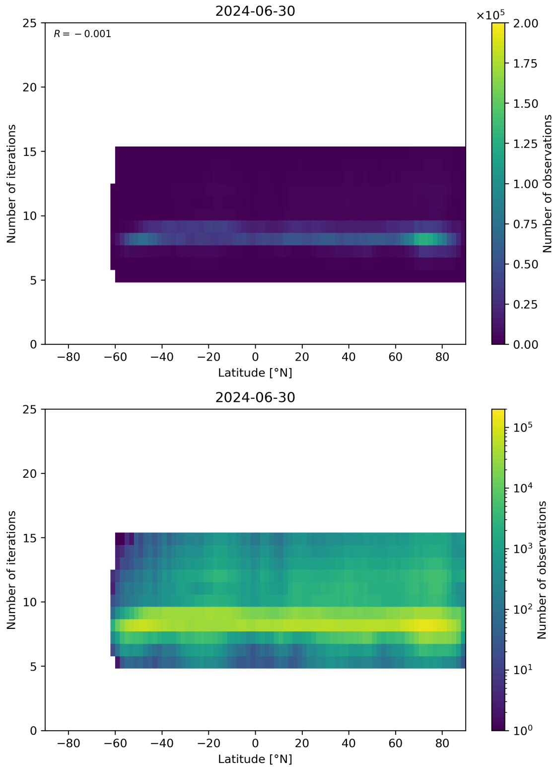
Figure 56: Scatter density plot of “Latitude” against “Number of iterations” for 2024-06-29 to 2024-07-01.
