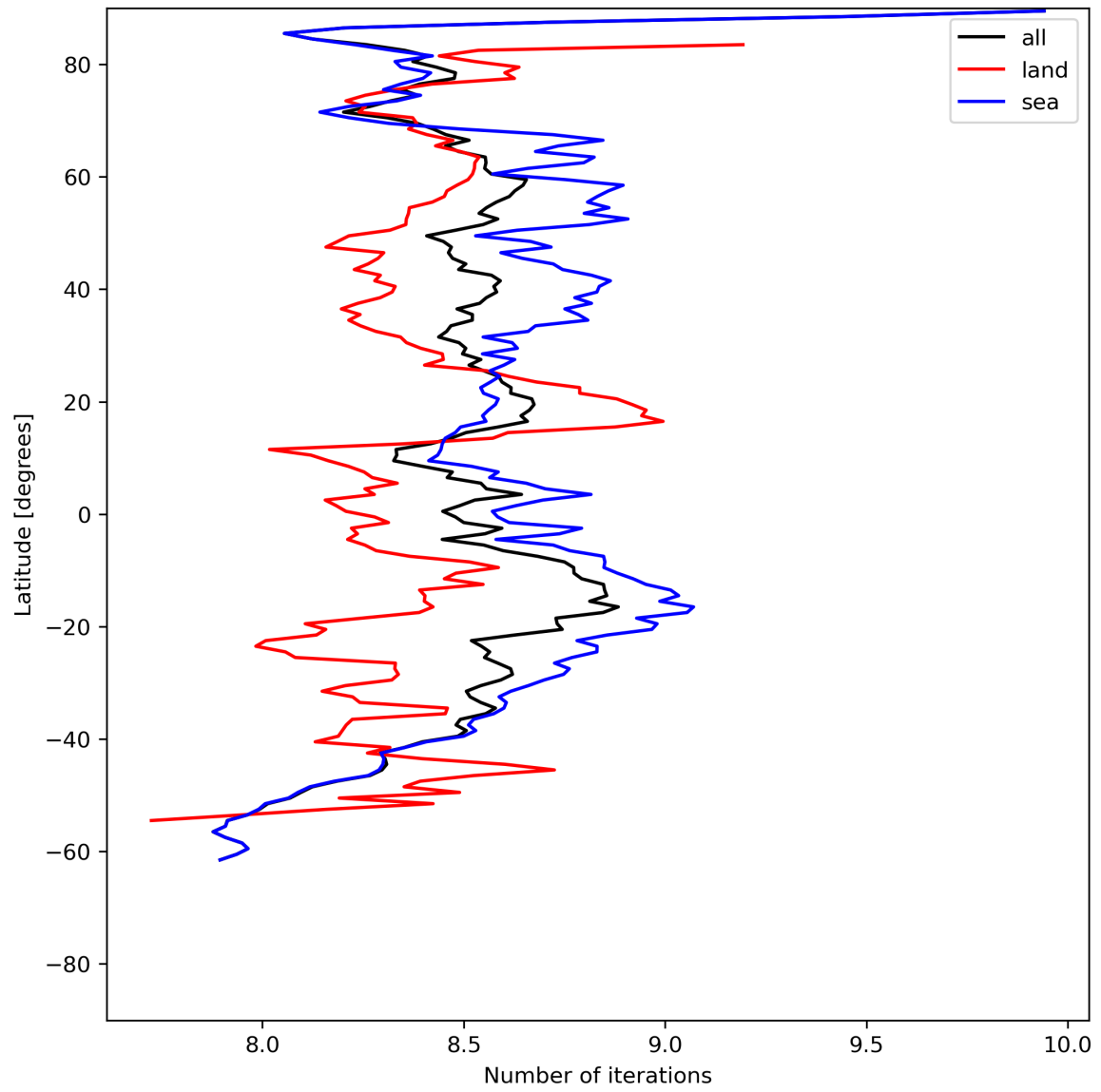
Figure 16: Zonal average of “Number of iterations” for 2024-06-29 to 2024-07-01.
