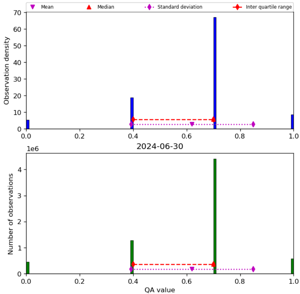
Figure 17: Histogram of “QA value” for 2024-06-29 to 2024-07-01
