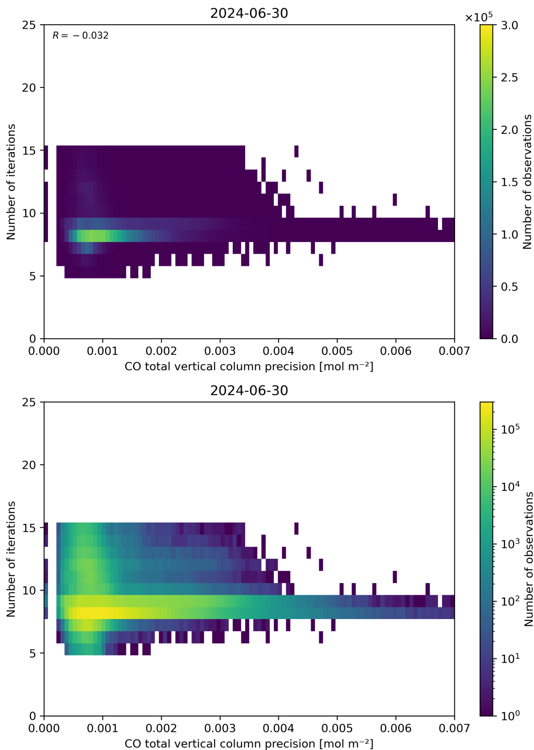
Figure 46: Scatter density plot of “CO total vertical column precision” against “Number of iterations” for 2024-06-29 to 2024-07-01.
