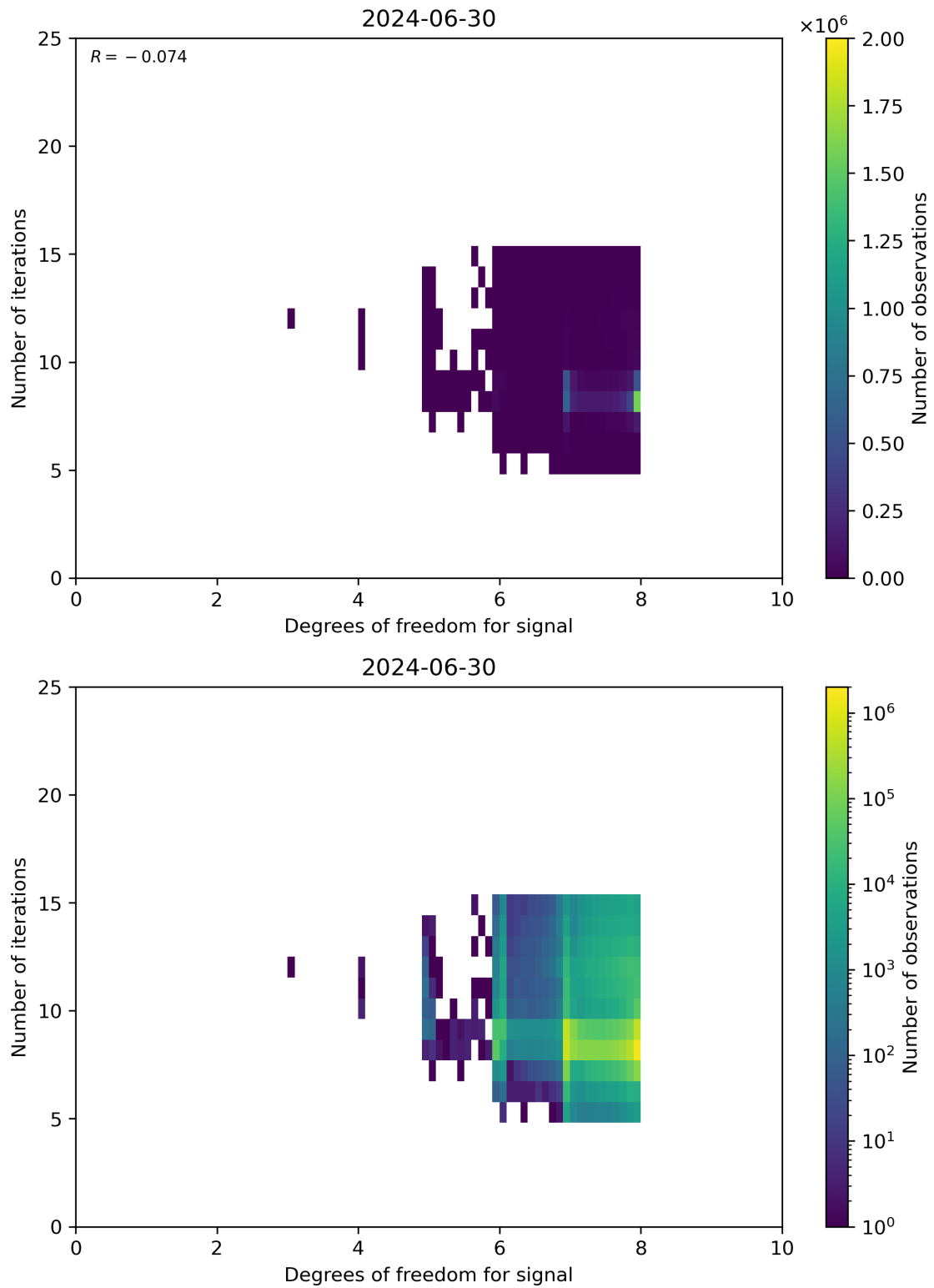
Figure 50: Scatter density plot of “Degrees of freedom for signal” against “Number of iterations” for 2024-06-29 to 2024-07-01.
