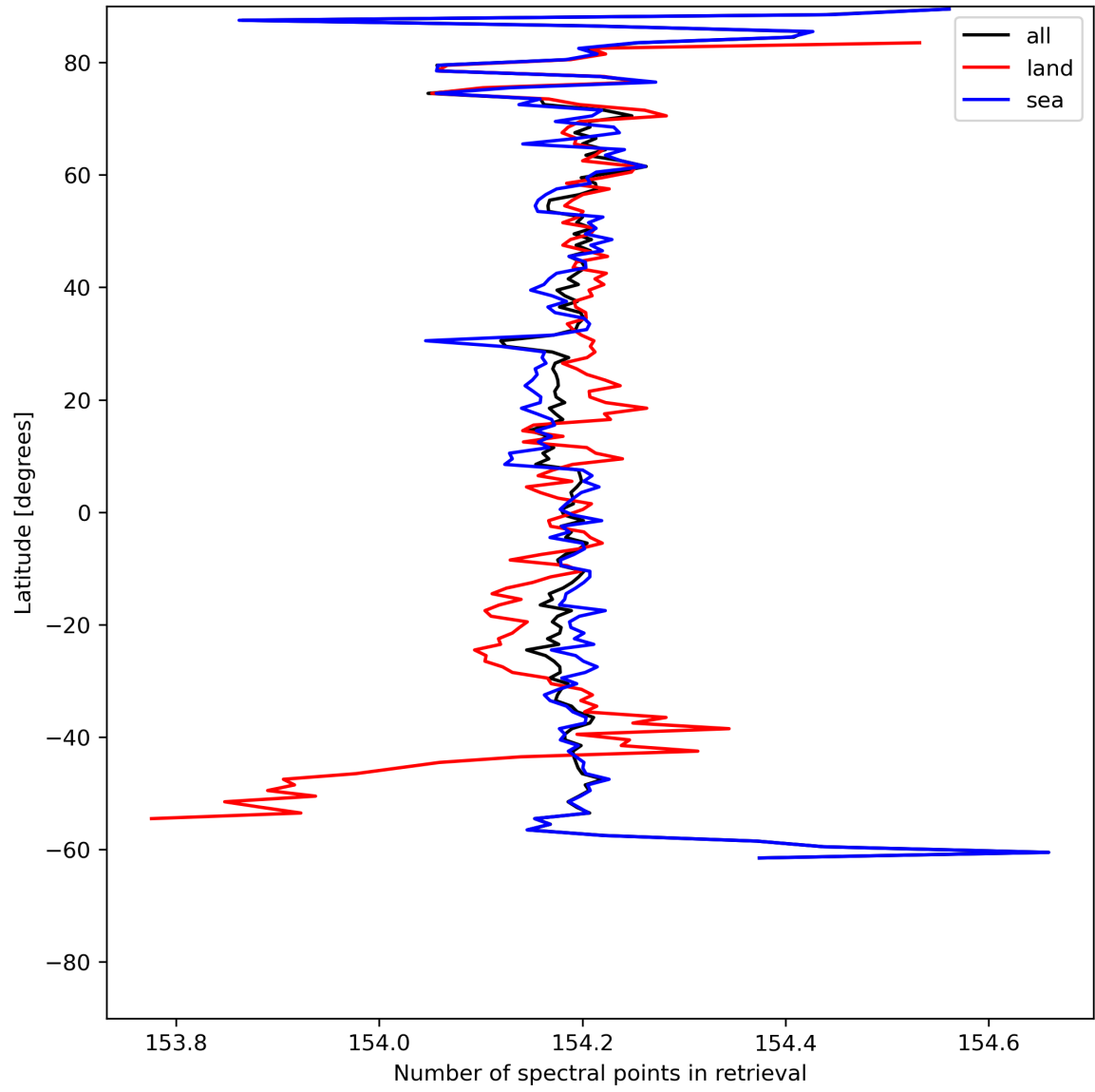
Figure 13: Zonal average of “Number of spectral points in retrieval” for 2024-06-29 to 2024-07-01.
