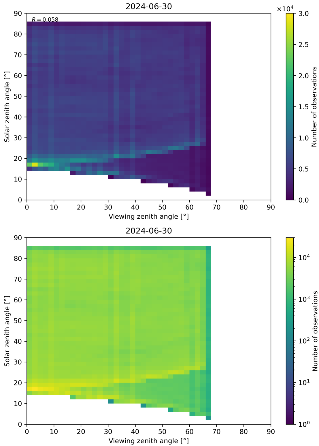
Figure 77: Scatter density plot of “Viewing zenith angle” against “Solar zenith angle” for 2024-06-29 to 2024-07-01.
