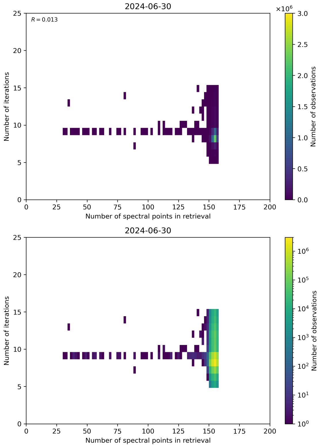
Figure 60: Scatter density plot of “Number of spectral points in retrieval” against “Number of iterations” for 2024-06-29 to 2024-07-01.
