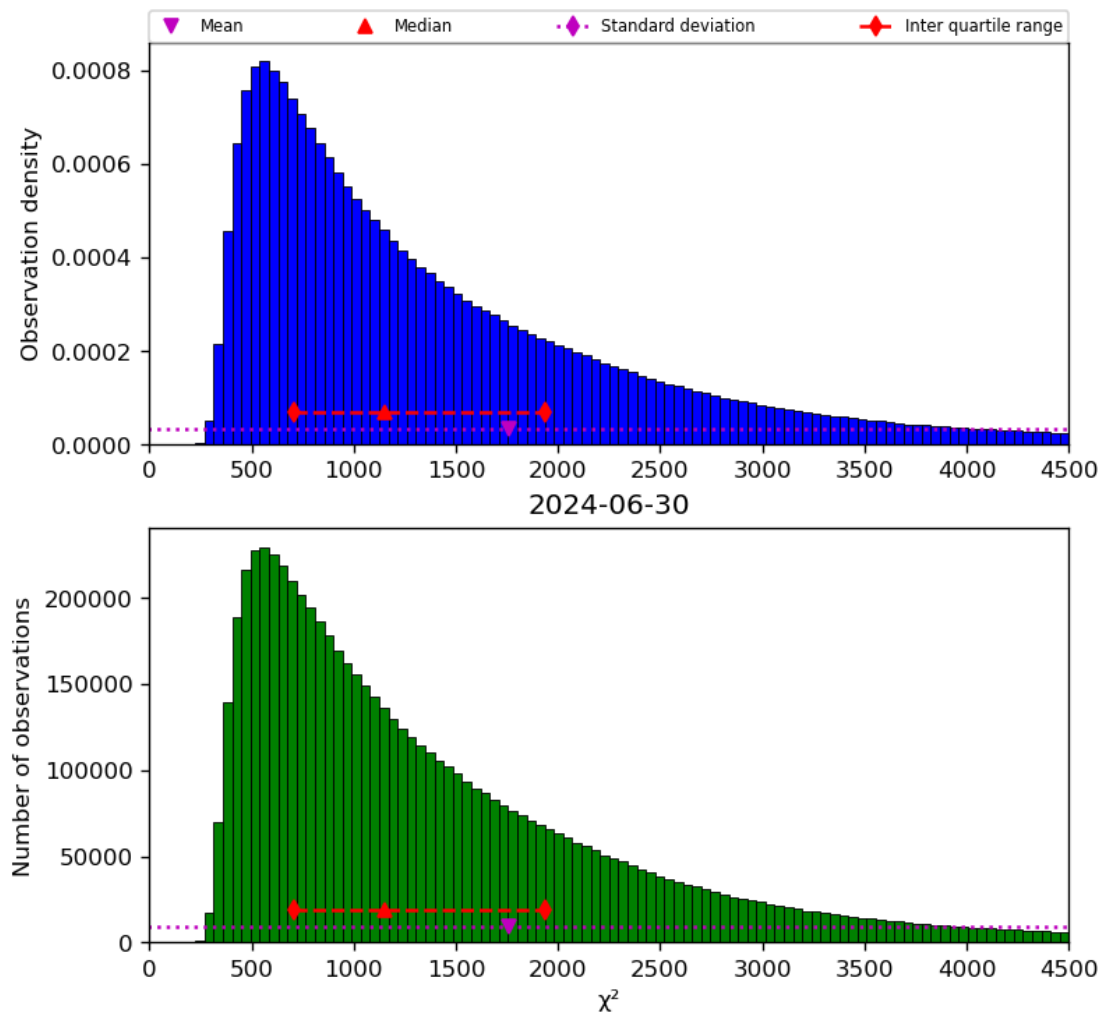
Figure 22: Histogram of “ \chi^2 ” for 2024-06-29 to 2024-07-01
