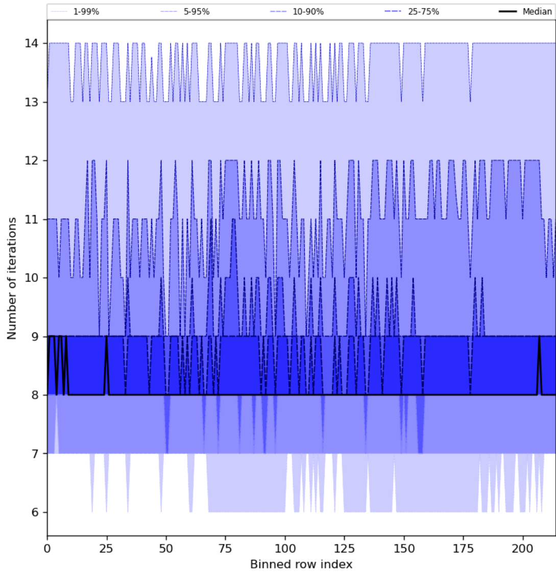
Figure 32: Along track statistics of “Number of iterations” for 2024-06-29 to 2024-07-01
