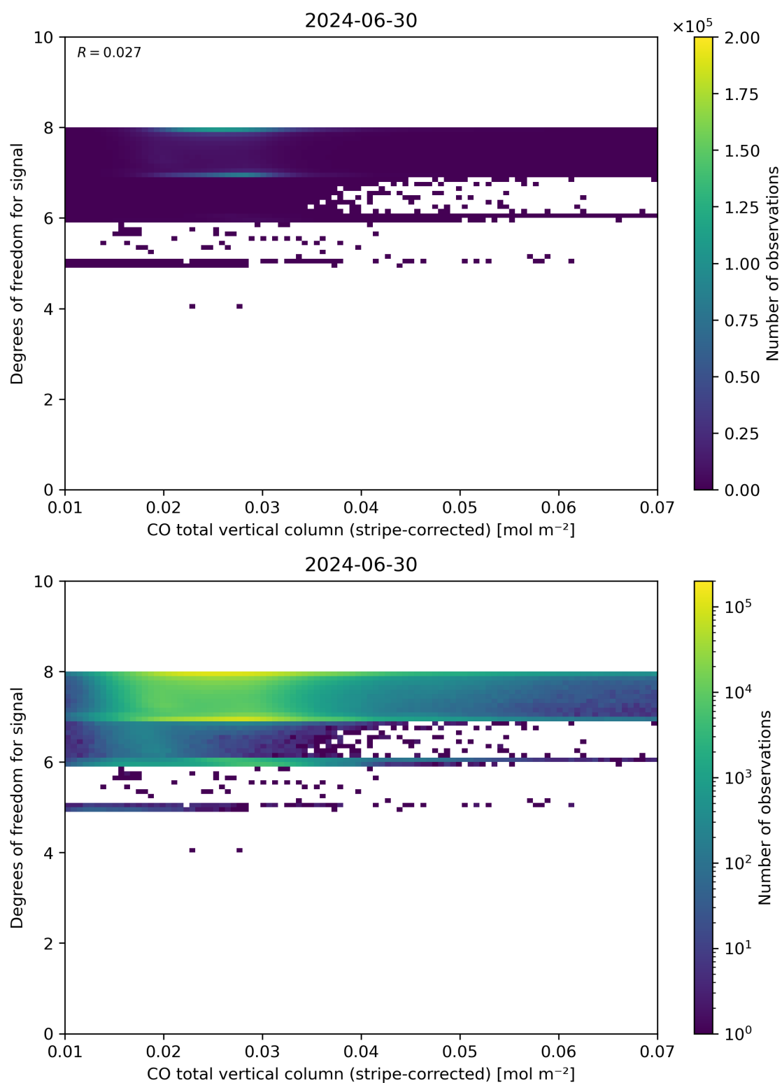
Figure 38: Scatter density plot of “CO total vertical column (stripe-corrected)” against “Degrees of freedom for signal” for 2024-06-29 to 2024-07-01.
