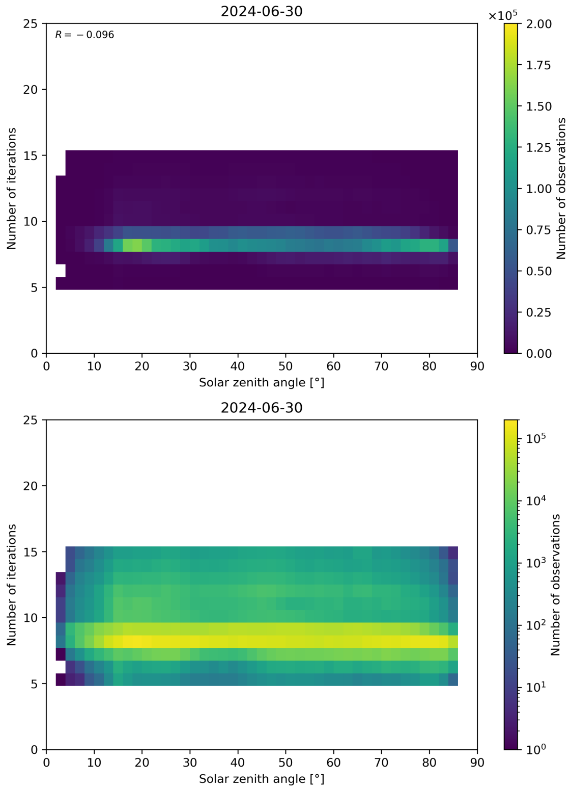
Figure 67: Scatter density plot of “Solar zenith angle” against “Number of iterations” for 2024-06-29 to 2024-07-01.
