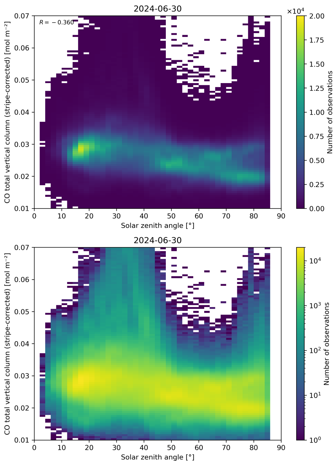
Figure 62: Scatter density plot of “Solar zenith angle” against “CO total vertical column (stripe-corrected)” for 2024-06-29 to 2024-07-01.
