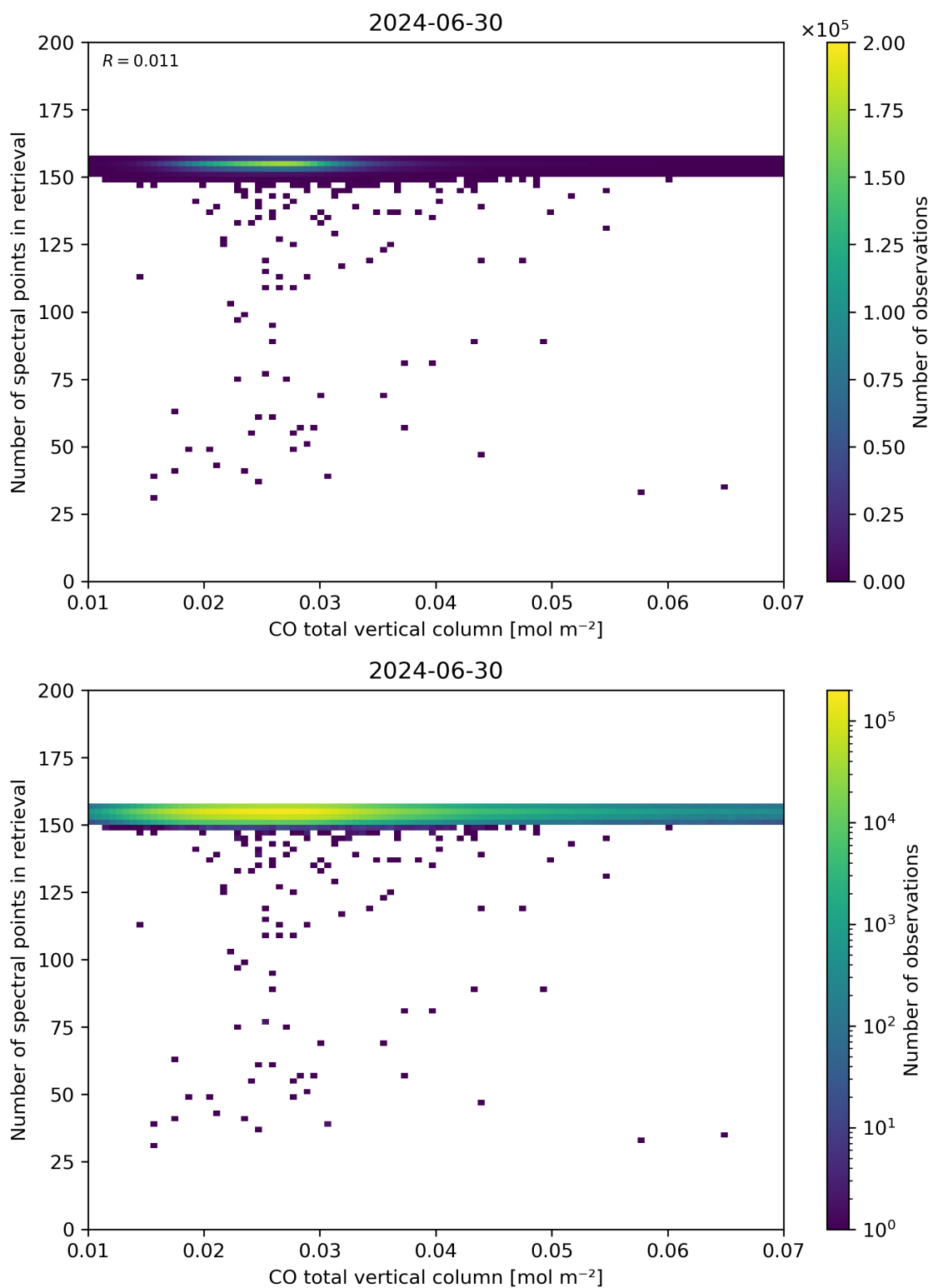
Figure 43: Scatter density plot of “CO total vertical column” against “Number of spectral points in retrieval” for 2024-06-29 to 2024-07-01.
