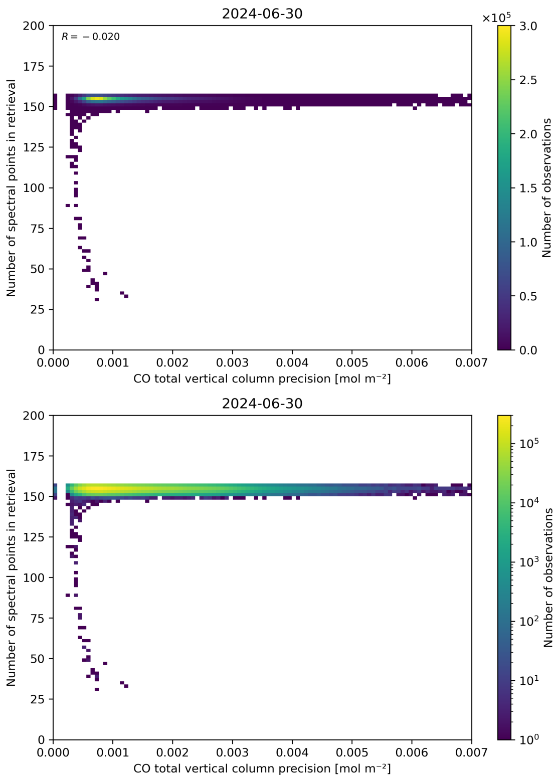
Figure 47: Scatter density plot of “CO total vertical column precision” against “Number of spectral points in retrieval” for 2024-06-29 to 2024-07-01.
