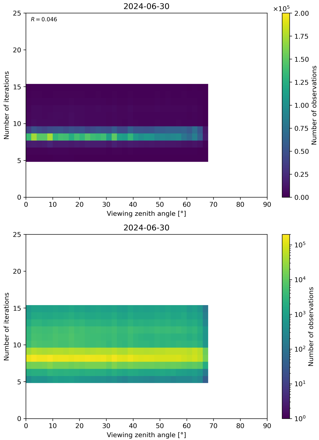
Figure 75: Scatter density plot of “Viewing zenith angle” against “Number of iterations” for 2024-06-29 to 2024-07-01.
