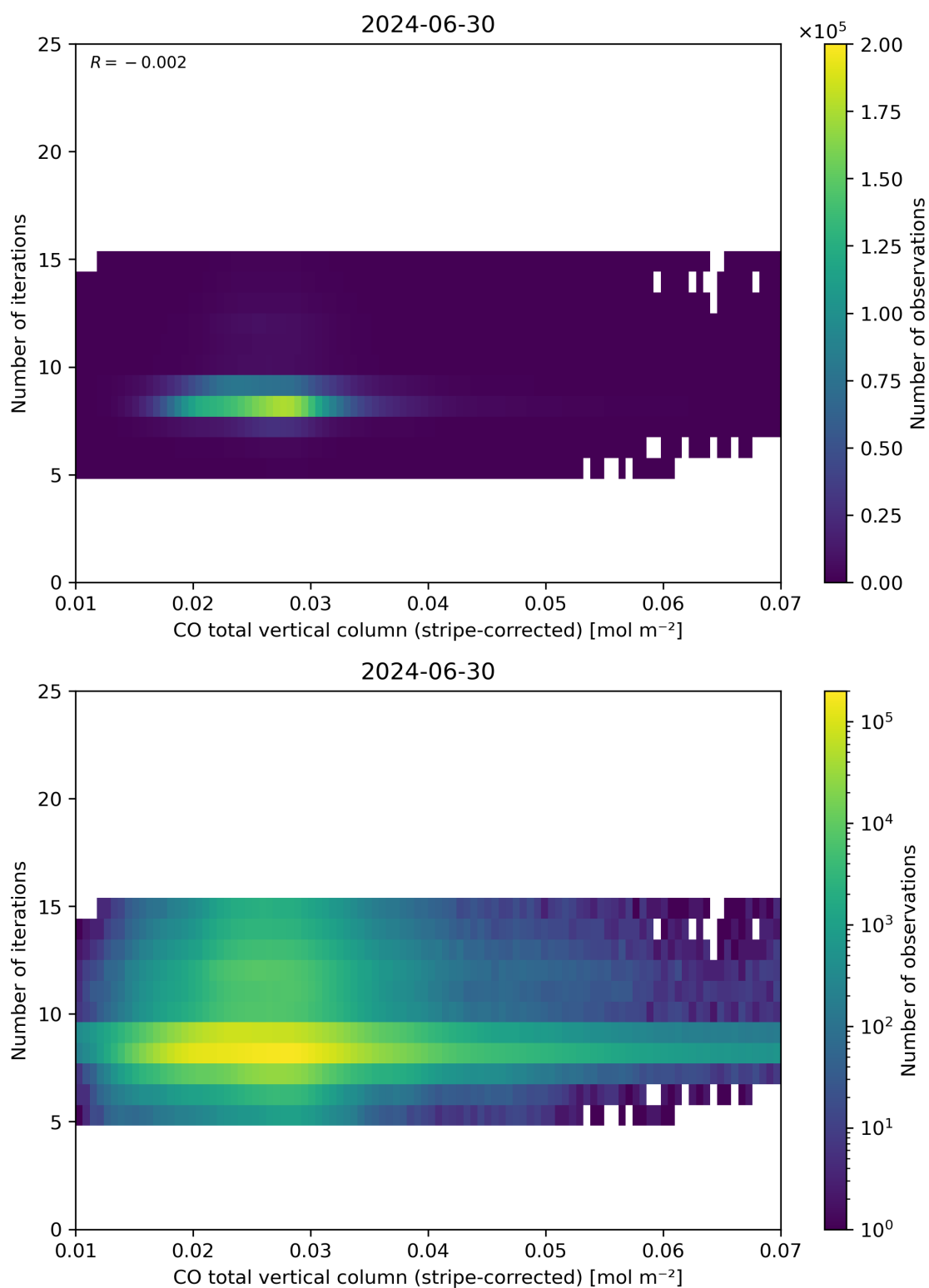
Figure 39: Scatter density plot of “CO total vertical column (stripe-corrected)” against “Number of iterations” for 2024-06-29 to 2024-07-01.
