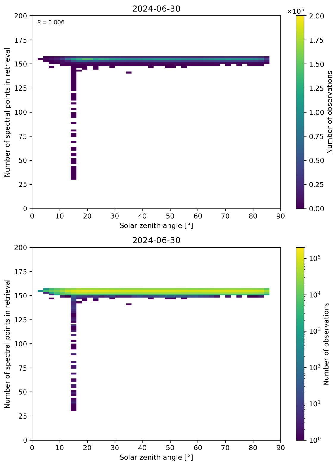
Figure 68: Scatter density plot of “Solar zenith angle” against “Number of spectral points in retrieval” for 2024-06-29 to 2024-07-01.
