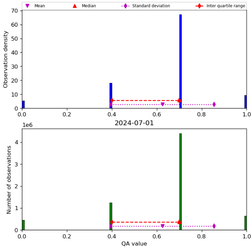
Figure 17: Histogram of “QA value” for 2024-06-30 to 2024-07-02
