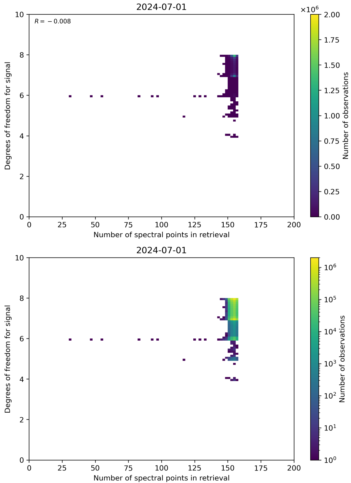
Figure 59: Scatter density plot of “Number of spectral points in retrieval” against “Degrees of freedom for signal” for 2024-06-30 to 2024-07-02.
