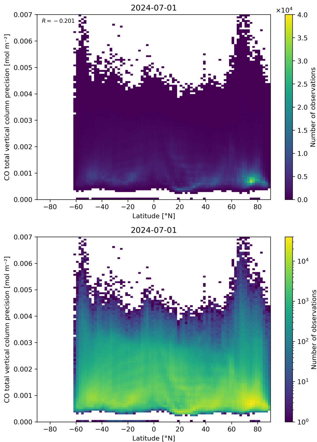
Figure 53: Scatter density plot of “Latitude” against “CO total vertical column precision” for 2024-06-30 to 2024-07-02.
