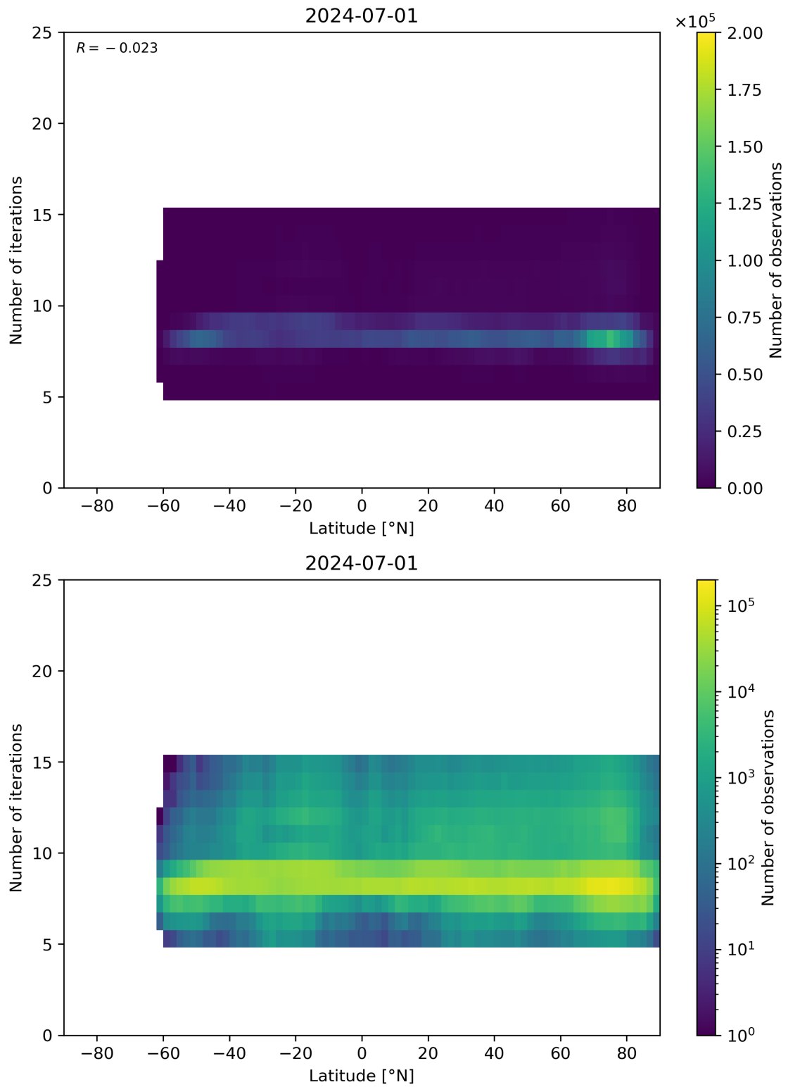
Figure 56: Scatter density plot of “Latitude” against “Number of iterations” for 2024-06-30 to 2024-07-02.
