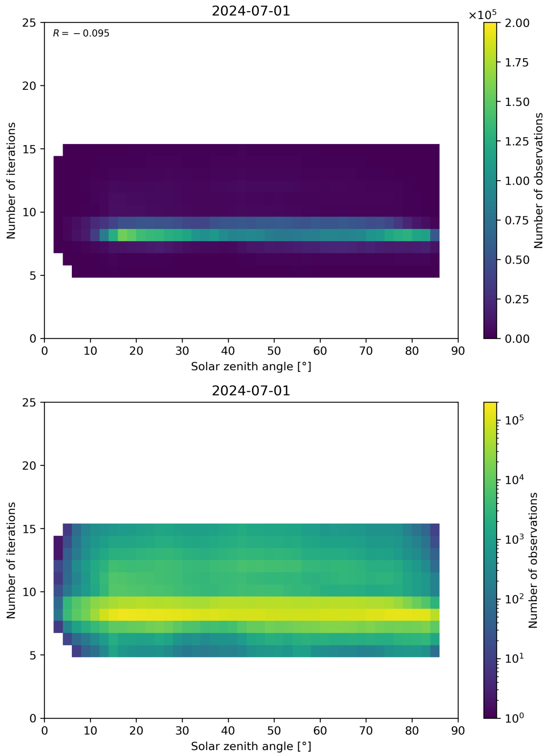
Figure 67: Scatter density plot of “Solar zenith angle” against “Number of iterations” for 2024-06-30 to 2024-07-02.
