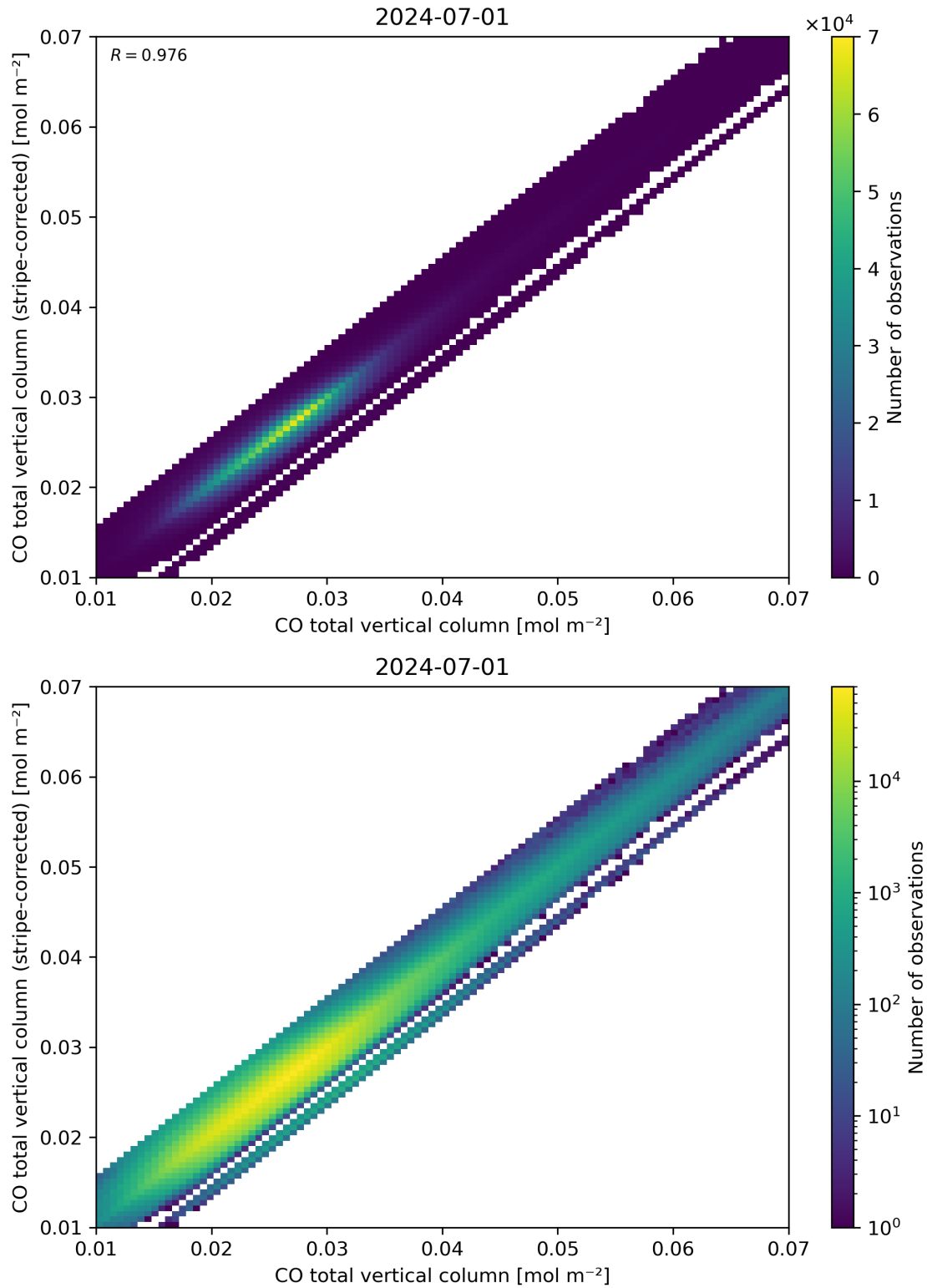
Figure 33: Scatter density plot of “CO total vertical column” against “CO total vertical column (stripe-corrected)” for 2024-06-30 to 2024-07-02.
