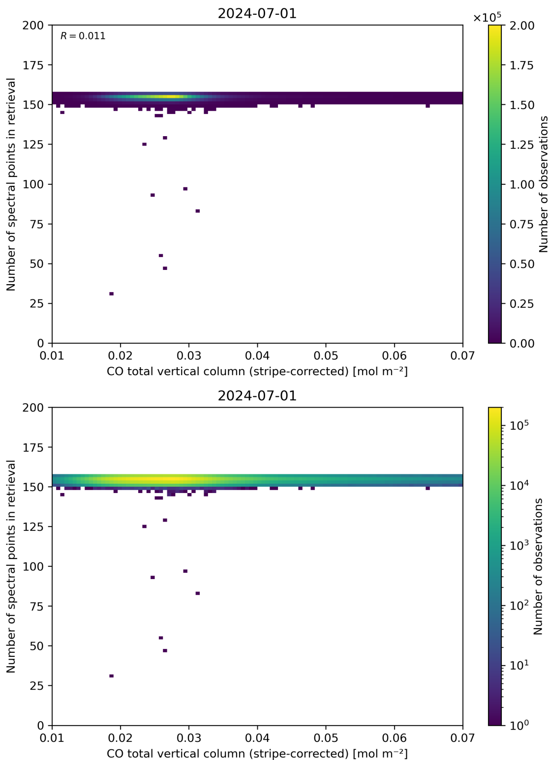
Figure 40: Scatter density plot of “CO total vertical column (stripe-corrected)” against “Number of spectral points in retrieval” for 2024-06-30 to 2024-07-02.
