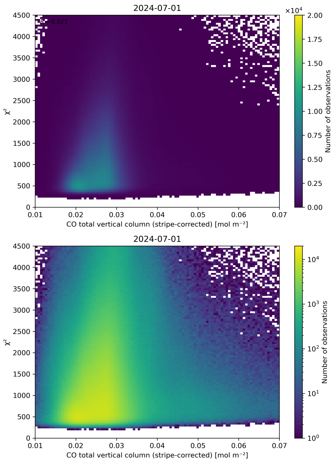
Figure 37: Scatter density plot of “CO total vertical column (stripe-corrected)” against “ \chi^2 ” for 2024-06-30 to 2024-07-02.
