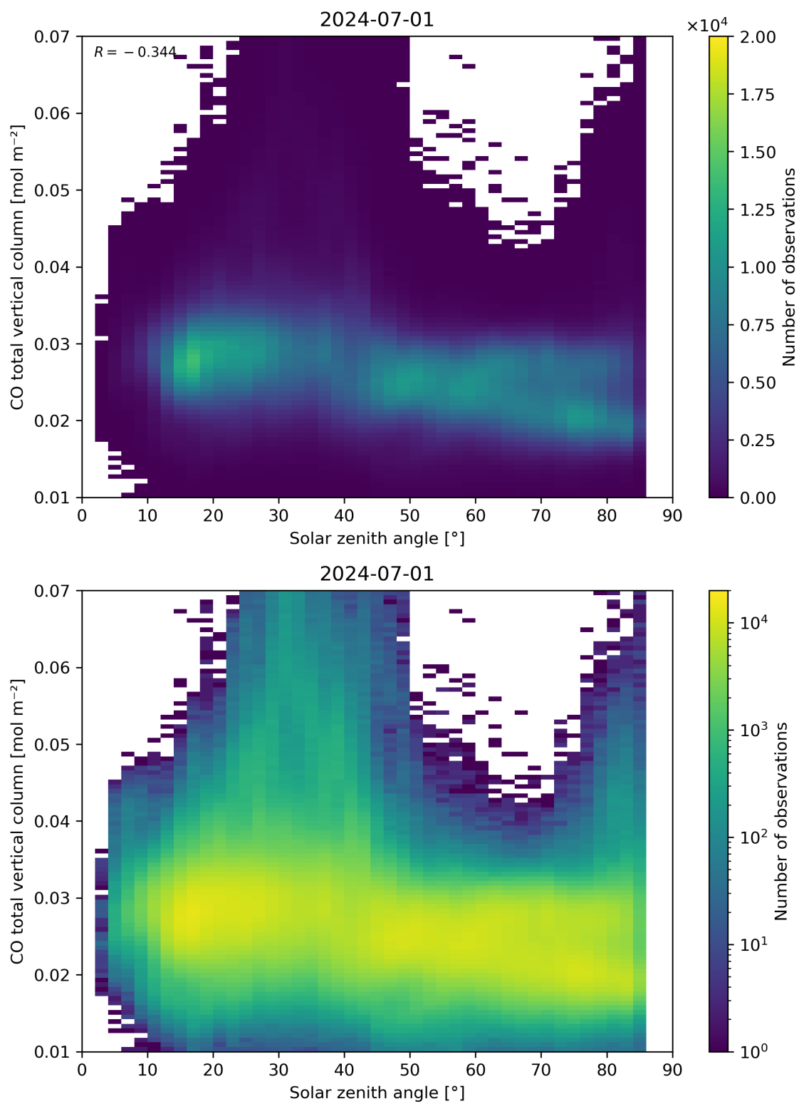
Figure 61: Scatter density plot of “Solar zenith angle” against “CO total vertical column” for 2024-06-30 to 2024-07-02.
