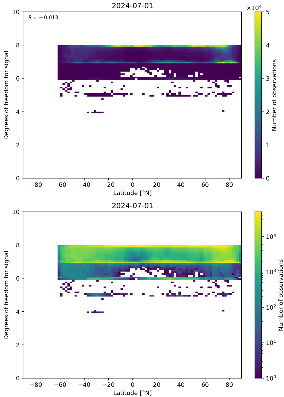
Figure 55: Scatter density plot of “Latitude” against “Degrees of freedom for signal” for 2024-06-30 to 2024-07-02.
