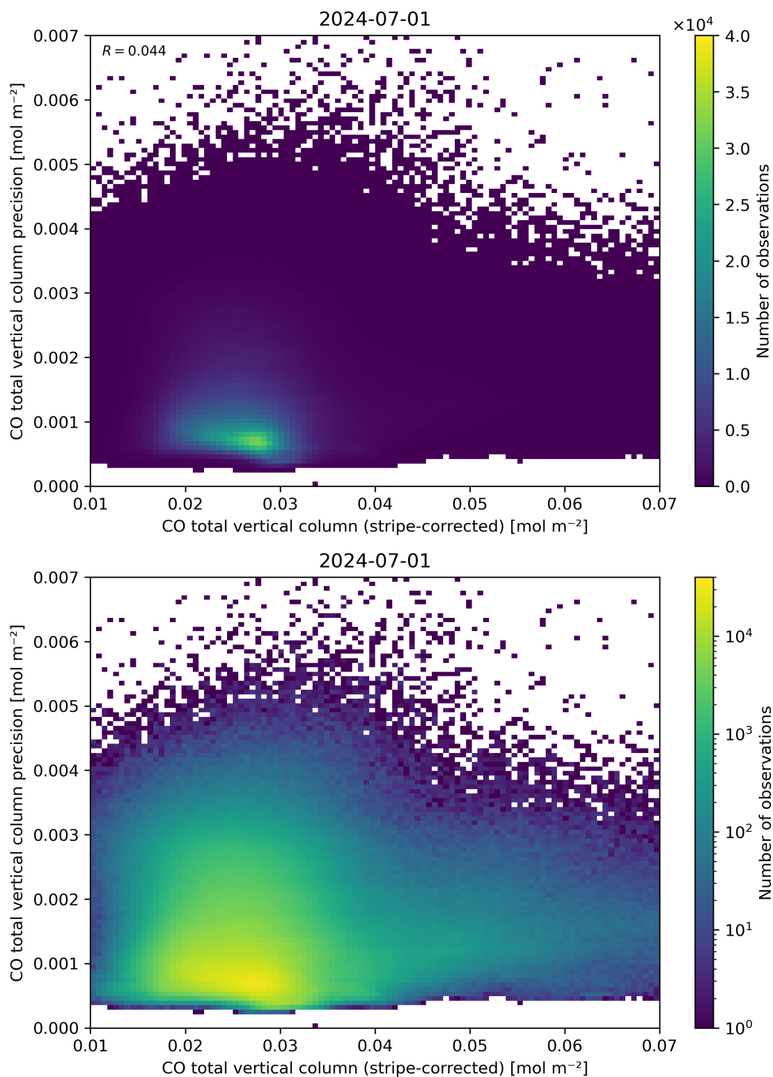
Figure 36: Scatter density plot of “CO total vertical column (stripe-corrected)” against “CO total vertical column precision” for 2024-06-30 to 2024-07-02.
