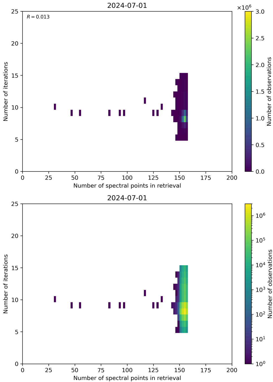
Figure 60: Scatter density plot of “Number of spectral points in retrieval” against “Number of iterations” for 2024-06-30 to 2024-07-02.
