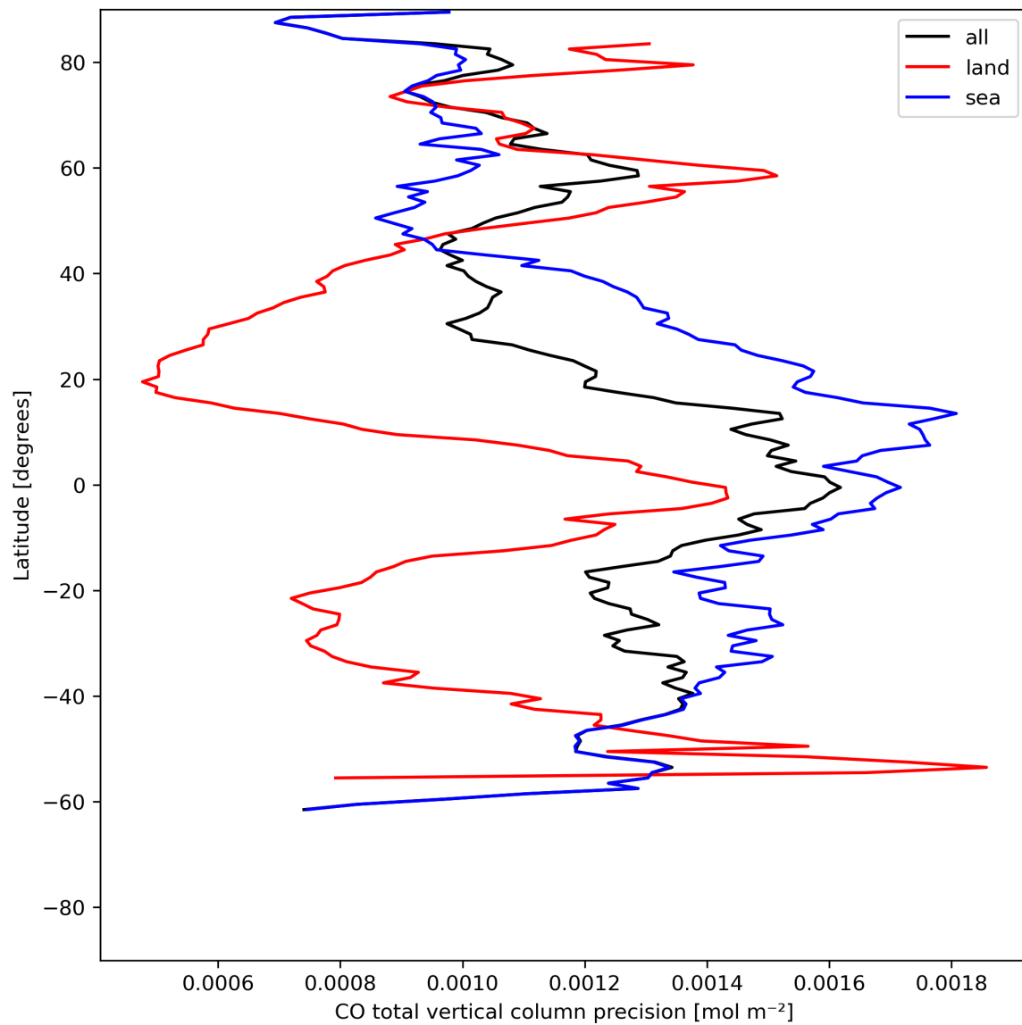
Figure 12: Zonal average of “CO total vertical column precision” for 2024-06-30 to 2024-07-02.
