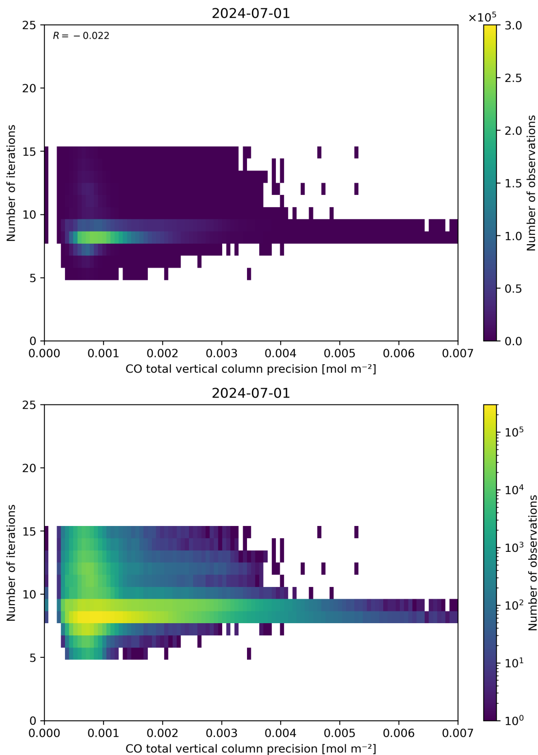
Figure 46: Scatter density plot of “CO total vertical column precision” against “Number of iterations” for 2024-06-30 to 2024-07-02.
