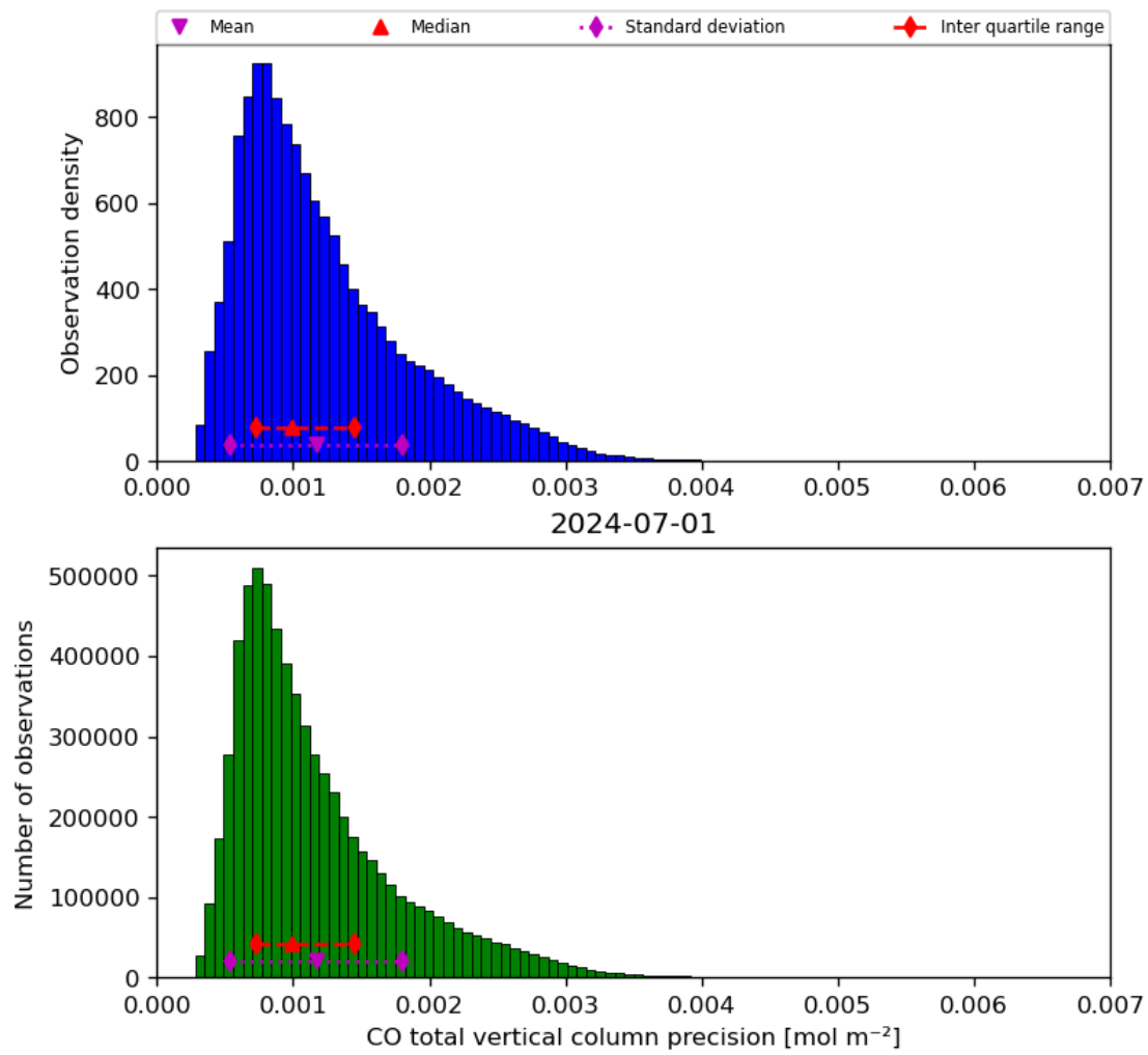
Figure 20: Histogram of “CO total vertical column precision” for 2024-06-30 to 2024-07-02
