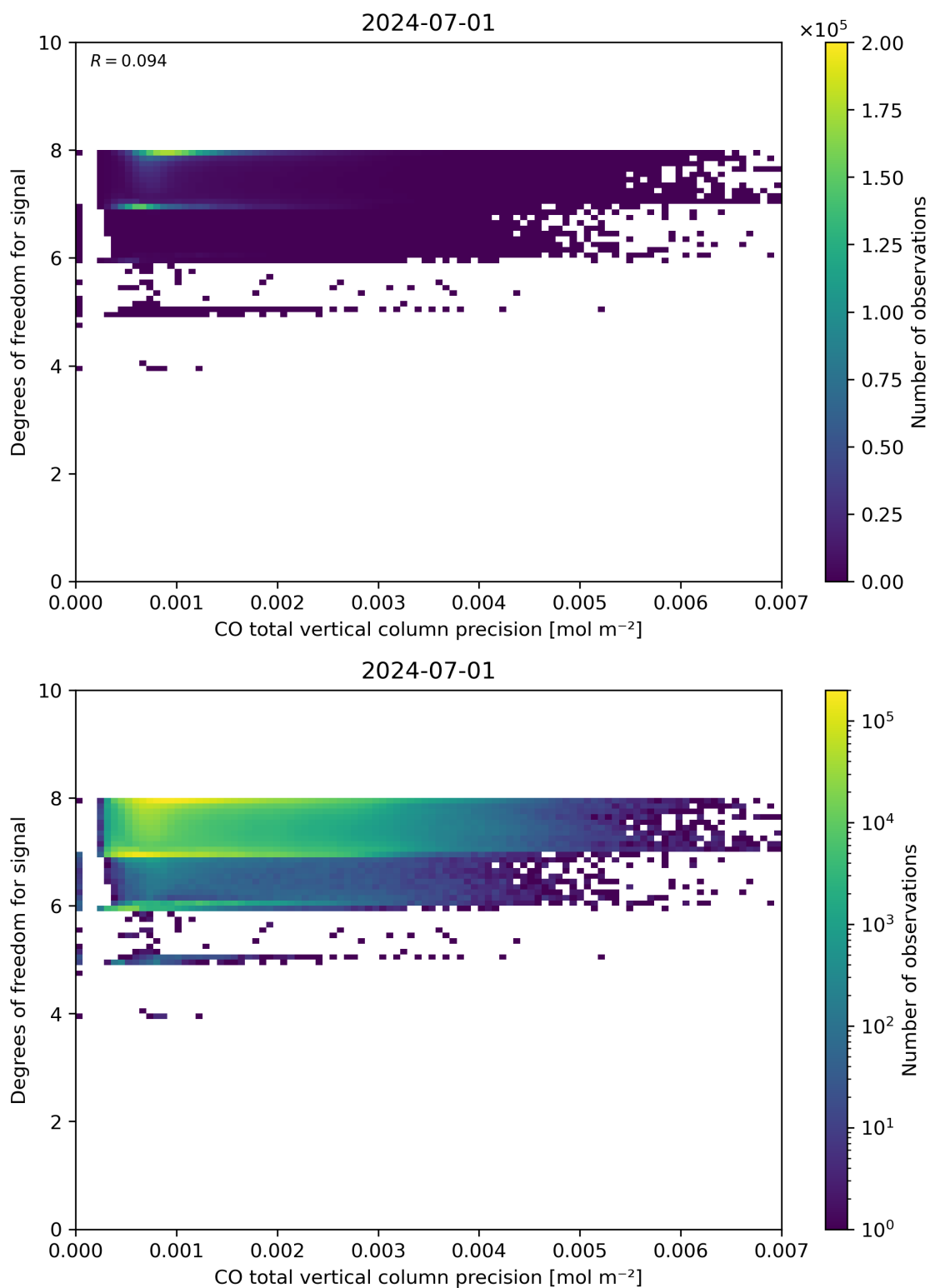
Figure 45: Scatter density plot of “CO total vertical column precision” against “Degrees of freedom for signal” for 2024-06-30 to 2024-07-02.
