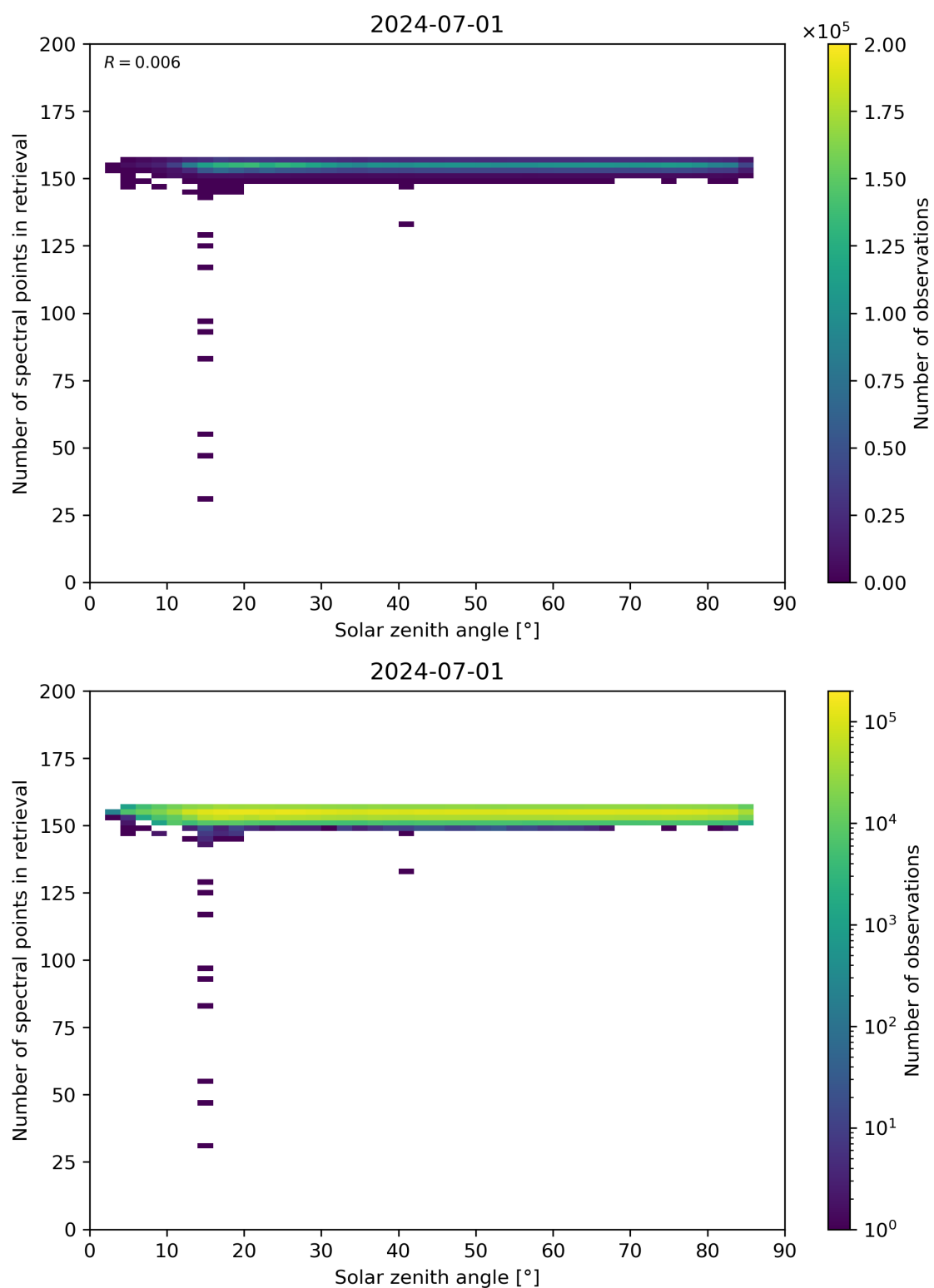
Figure 68: Scatter density plot of “Solar zenith angle” against “Number of spectral points in retrieval” for 2024-06-30 to 2024-07-02.
