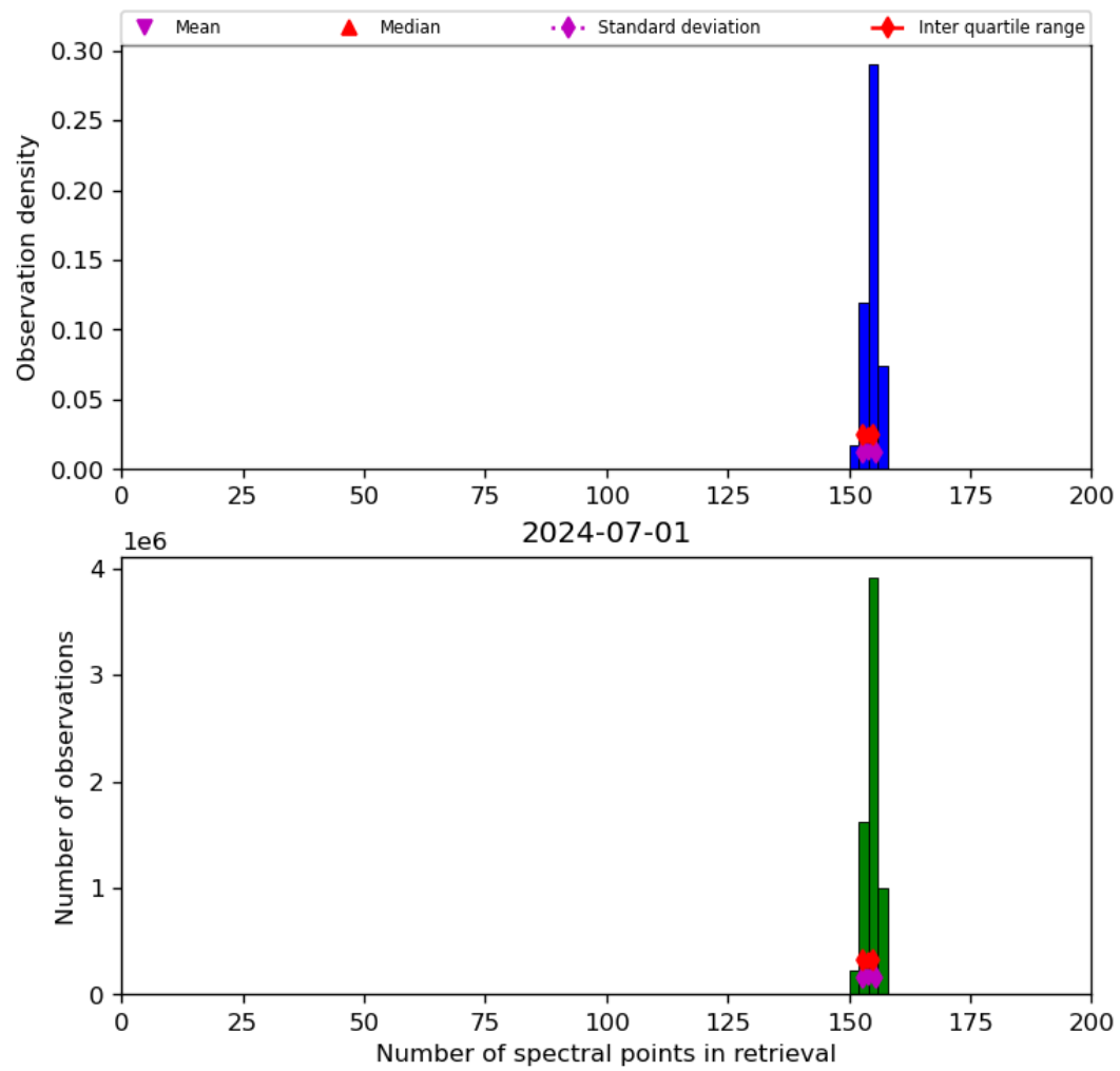
Figure 21: Histogram of “Number of spectral points in retrieval” for 2024-06-30 to 2024-07-02
