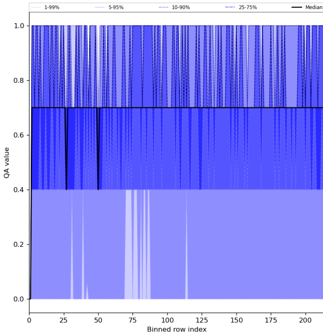
Figure 25: Along track statistics of “QA value” for 2024-06-30 to 2024-07-02
