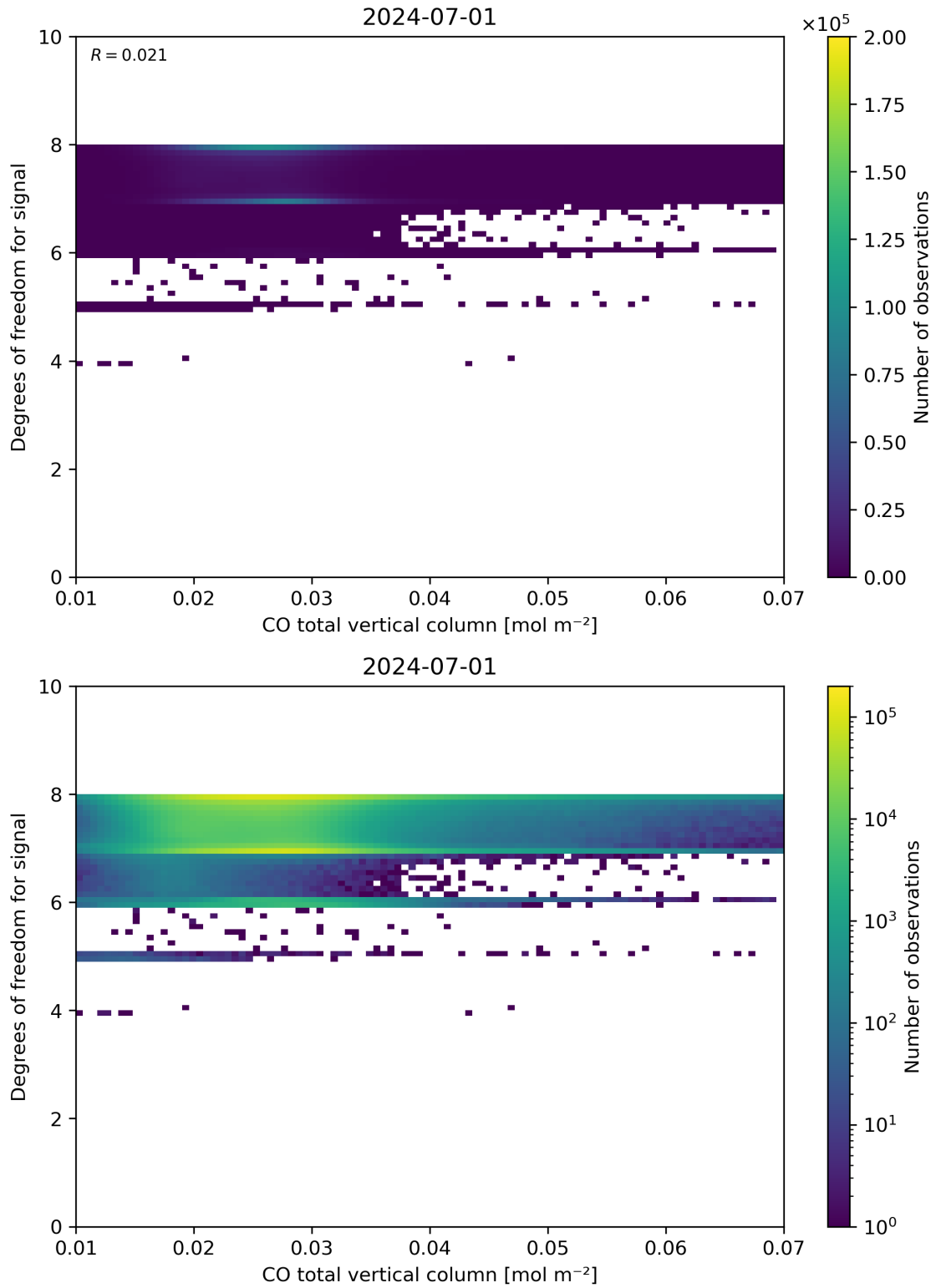
Figure 41: Scatter density plot of “CO total vertical column” against “Degrees of freedom for signal” for 2024-06-30 to 2024-07-02.
