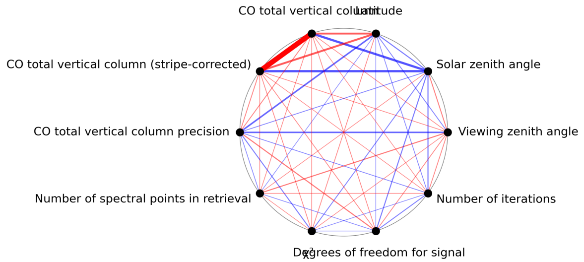
Figure 1: Map of correlation graph for 2024-06-30 to 2024-07-02.
