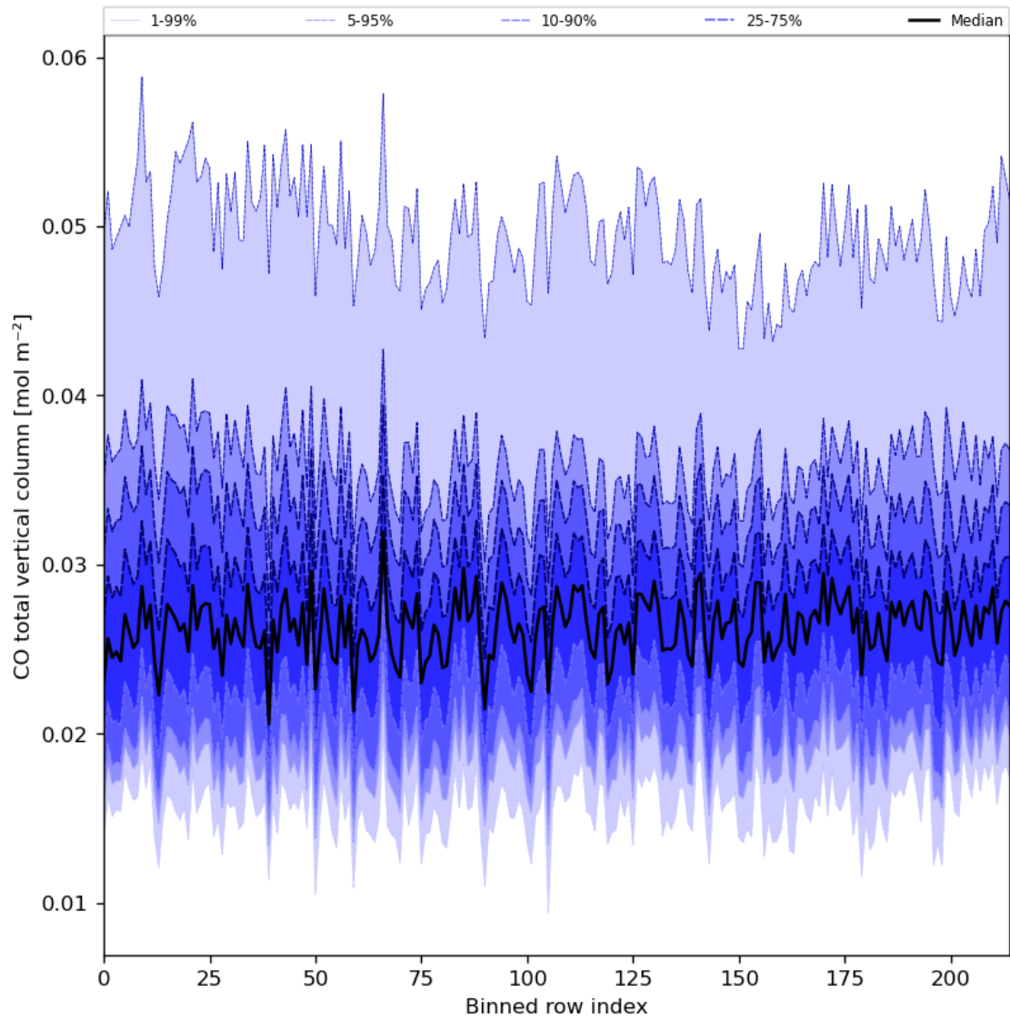
Figure 26: Along track statistics of “CO total vertical column” for 2024-06-30 to 2024-07-02
