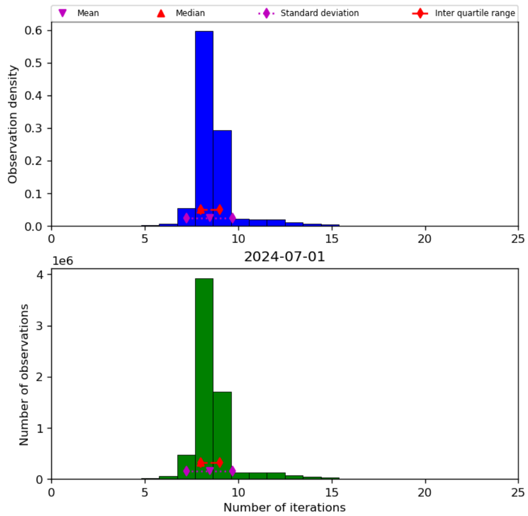
Figure 24: Histogram of “Number of iterations” for 2024-06-30 to 2024-07-02
