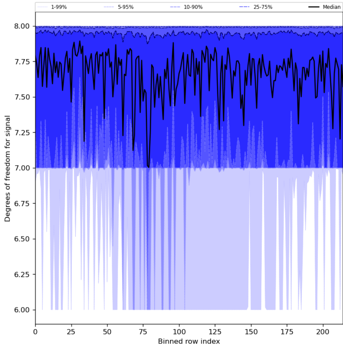
Figure 31: Along track statistics of “Degrees of freedom for signal” for 2024-06-30 to 2024-07-02
