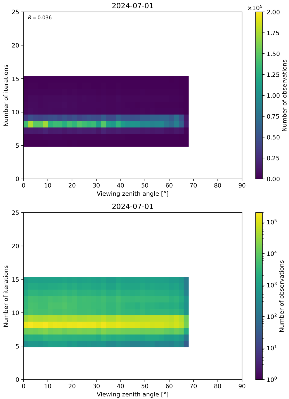
Figure 75: Scatter density plot of “Viewing zenith angle” against “Number of iterations” for 2024-06-30 to 2024-07-02.
