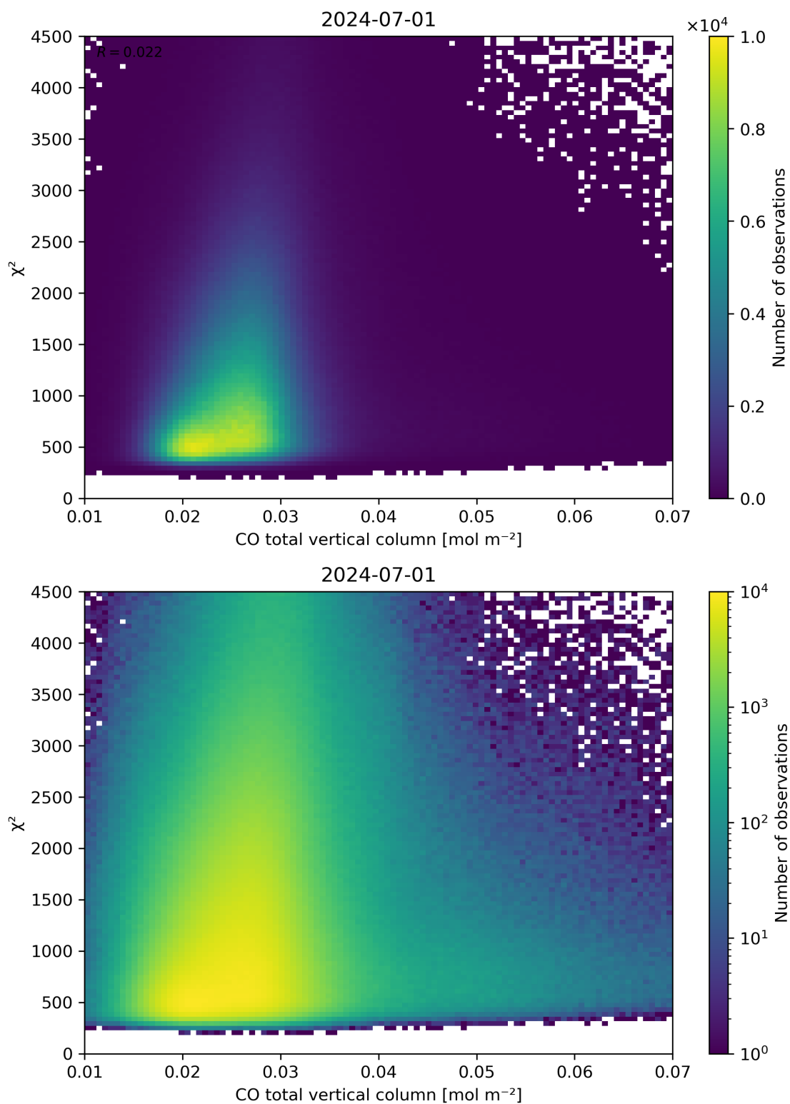
Figure 35: Scatter density plot of “CO total vertical column” against “ \chi^2 ” for 2024-06-30 to 2024-07-02.
