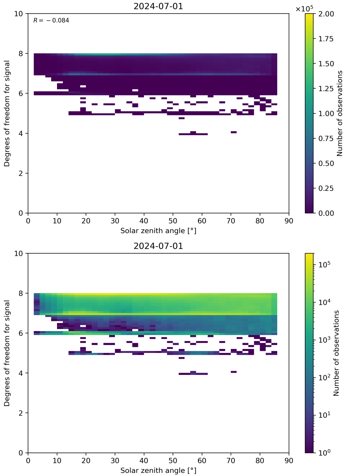
Figure 65: Scatter density plot of “Solar zenith angle” against “Degrees of freedom for signal” for 2024-06-30 to 2024-07-02.
