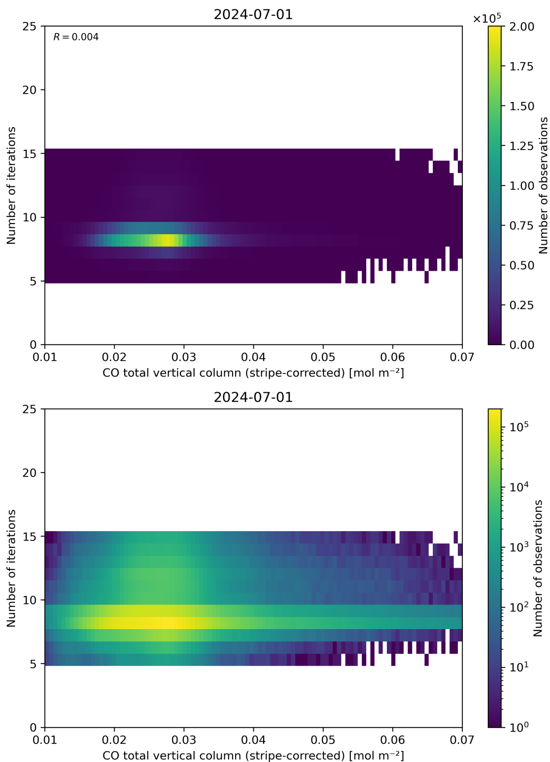
Figure 39: Scatter density plot of “CO total vertical column (stripe-corrected)” against “Number of iterations” for 2024-06-30 to 2024-07-02.
