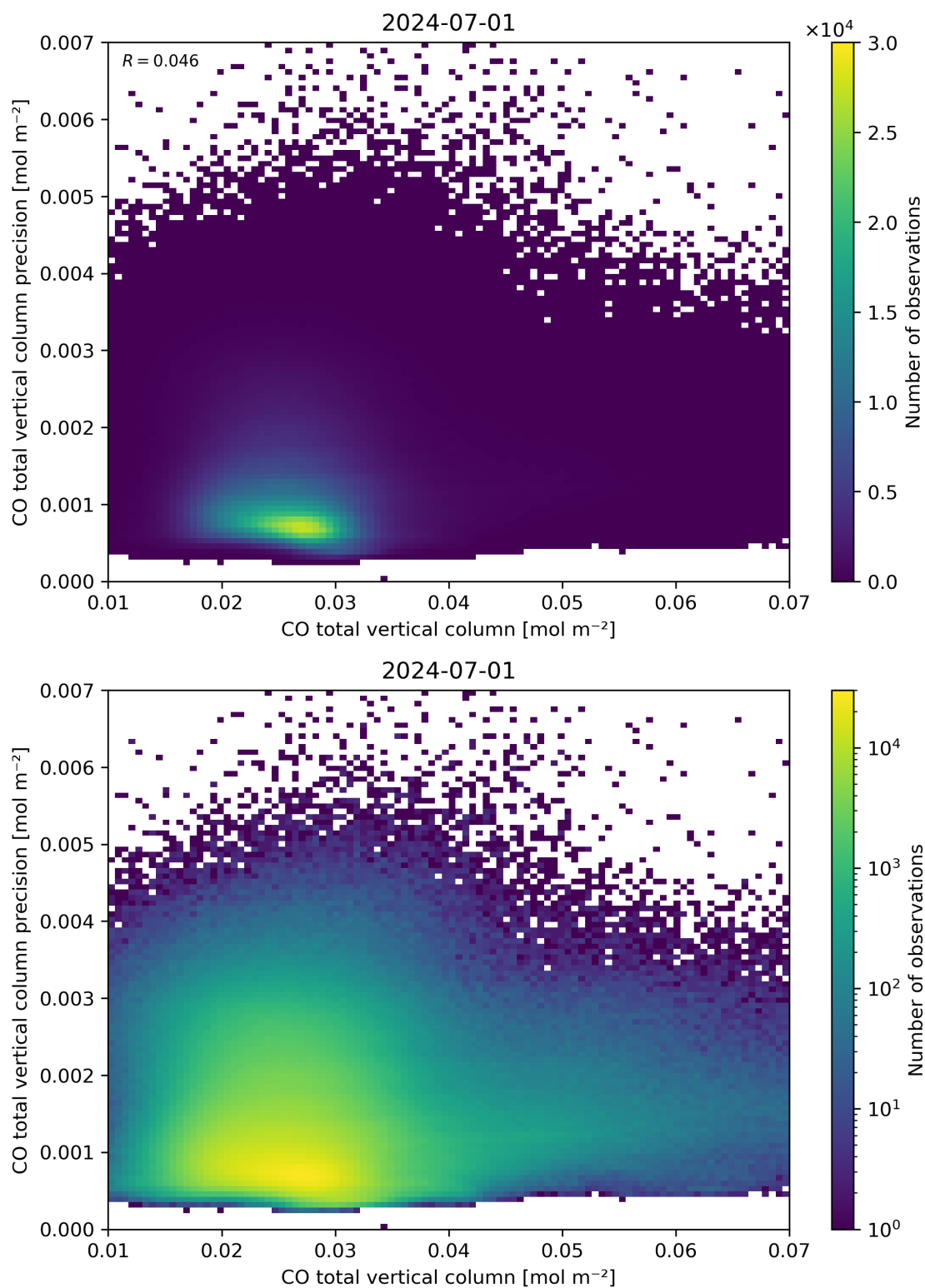
Figure 34: Scatter density plot of “CO total vertical column” against “CO total vertical column precision” for 2024-06-30 to 2024-07-02.
