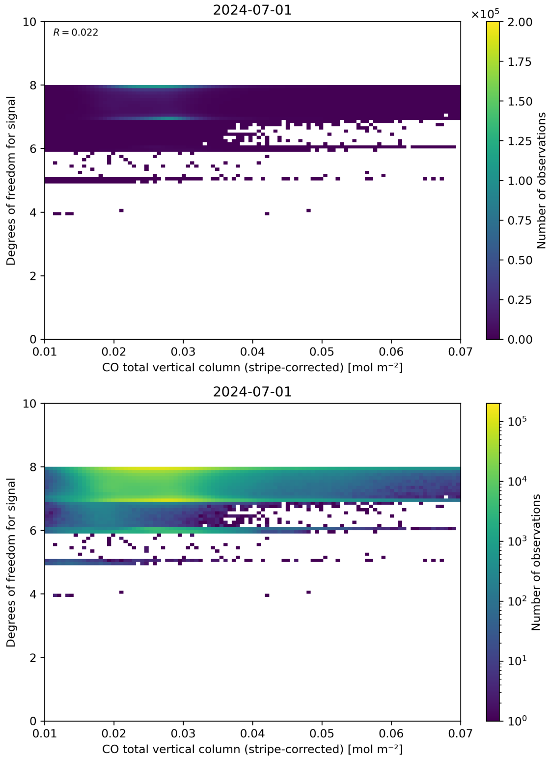
Figure 38: Scatter density plot of “CO total vertical column (stripe-corrected)” against “Degrees of freedom for signal” for 2024-06-30 to 2024-07-02.
