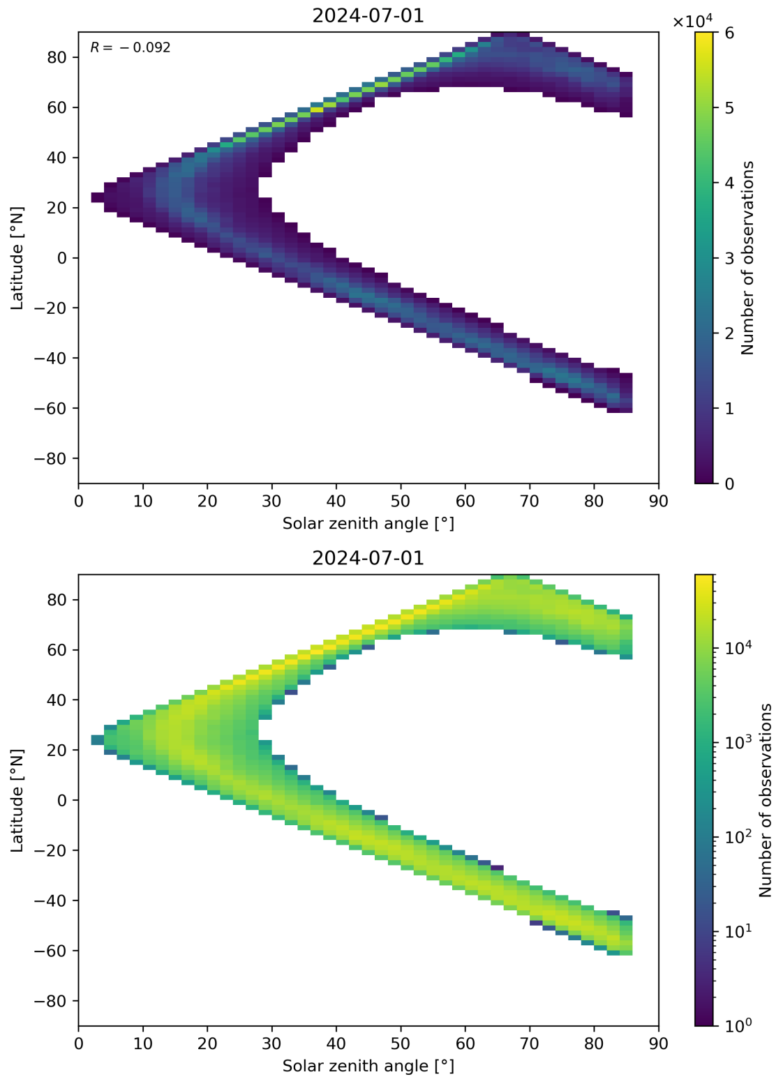
Figure 66: Scatter density plot of “Solar zenith angle” against “Latitude” for 2024-06-30 to 2024-07-02.
