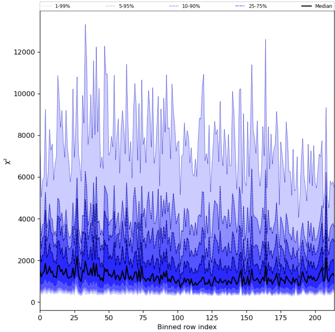
Figure 30: Along track statistics of “ \chi^2 ” for 2024-06-30 to 2024-07-02
