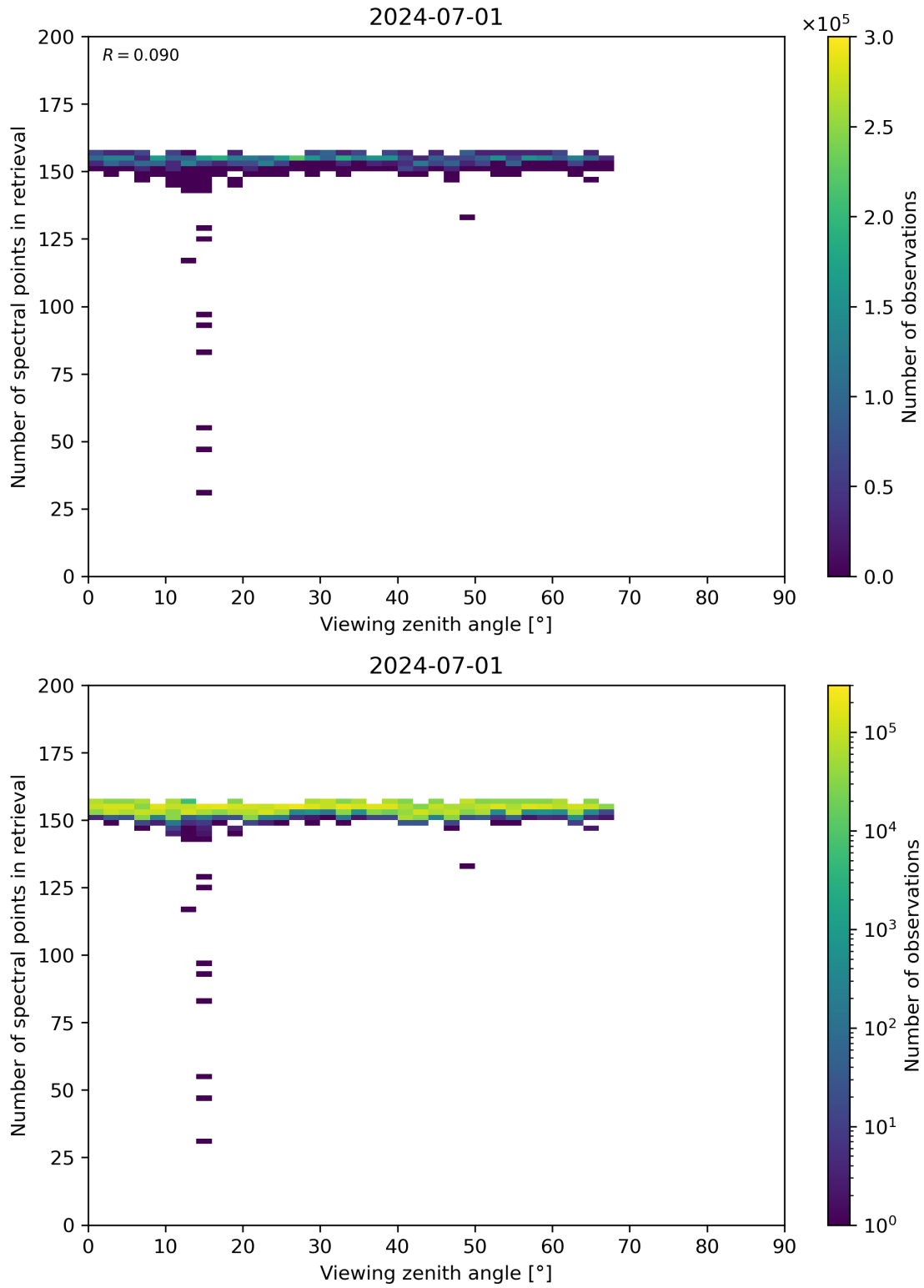
Figure 76: Scatter density plot of “Viewing zenith angle” against “Number of spectral points in retrieval” for 2024-06-30 to 2024-07-02.
