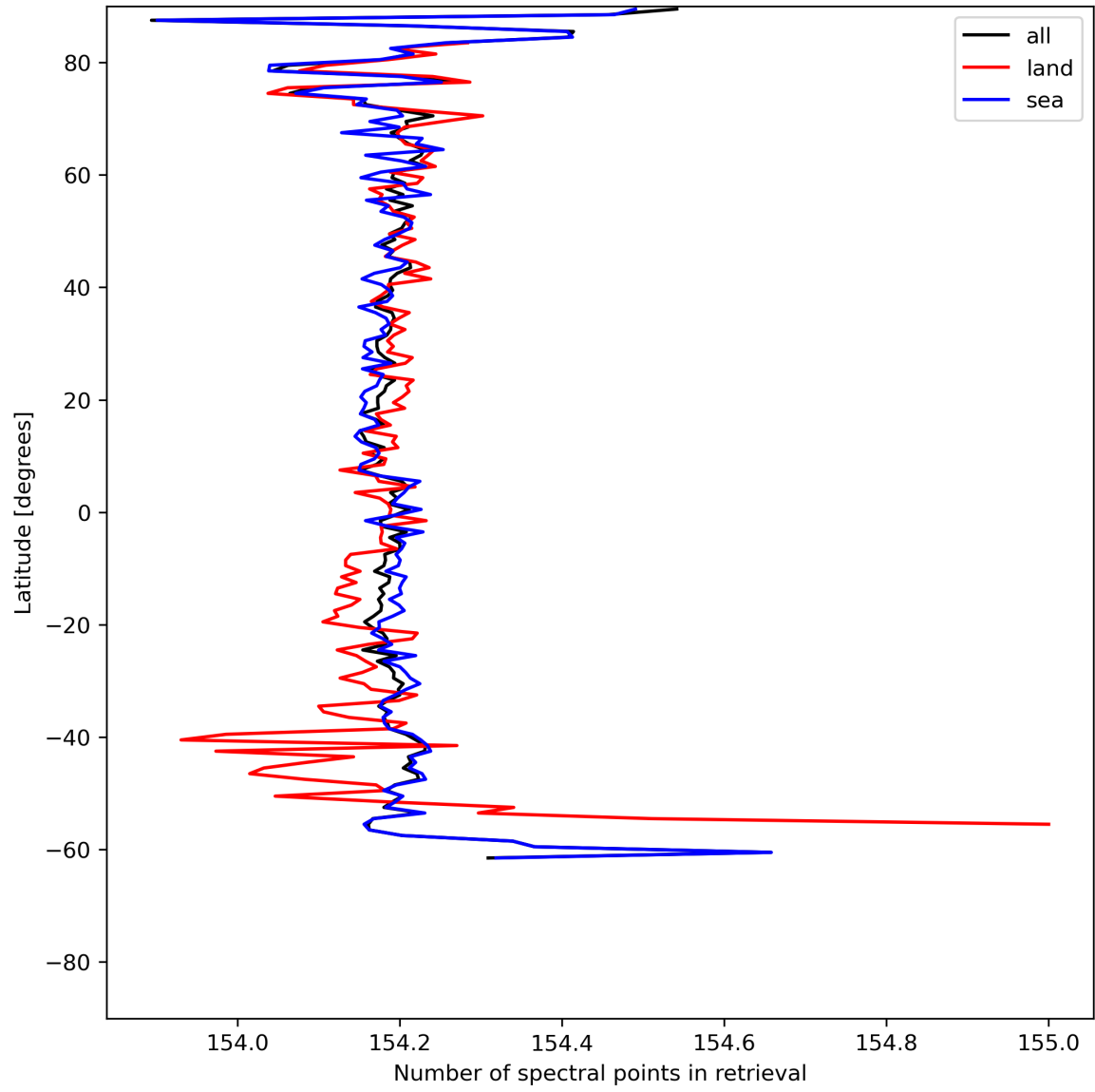
Figure 13: Zonal average of “Number of spectral points in retrieval” for 2024-06-30 to 2024-07-02.
