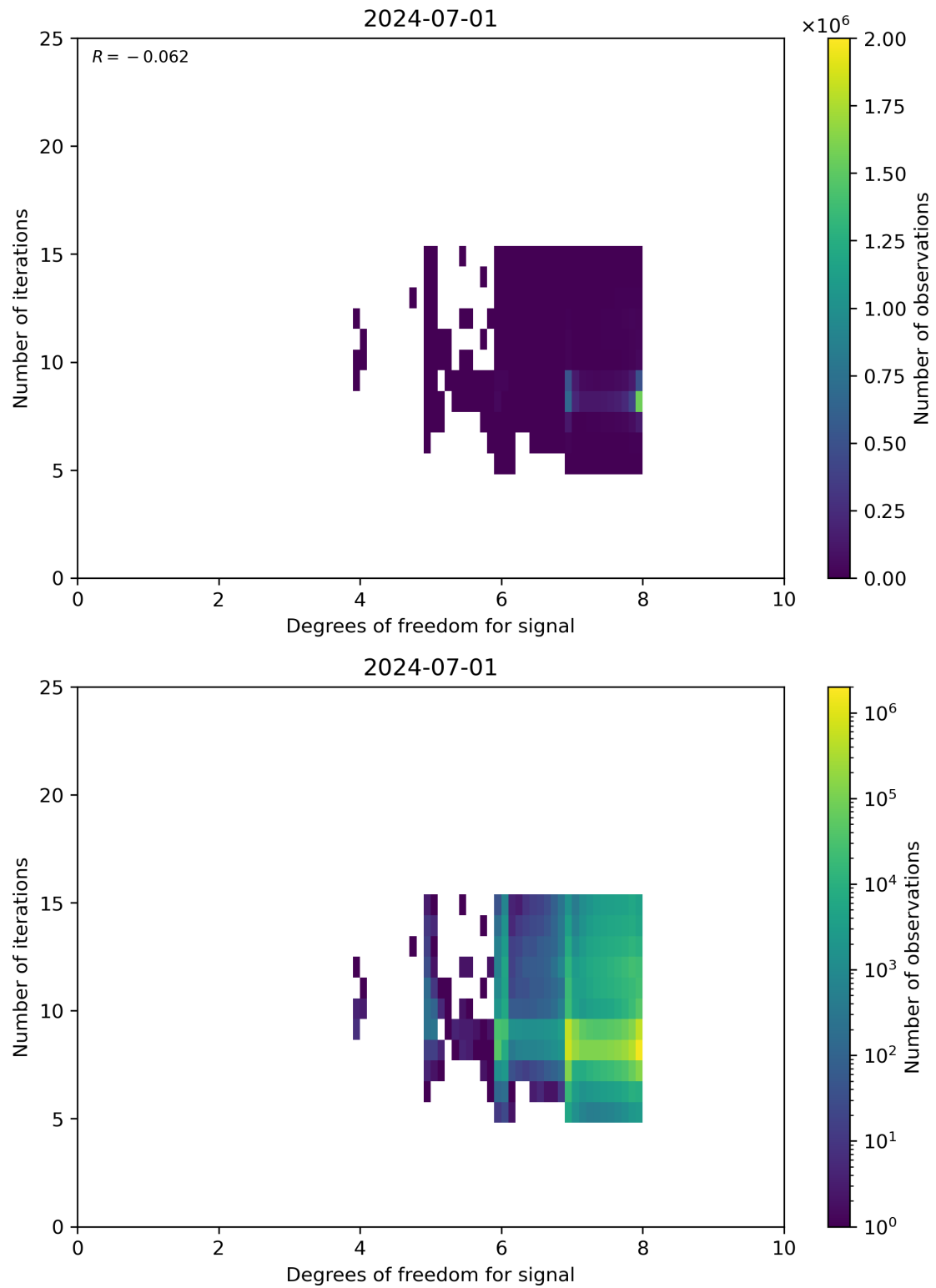
Figure 50: Scatter density plot of “Degrees of freedom for signal” against “Number of iterations” for 2024-06-30 to 2024-07-02.
