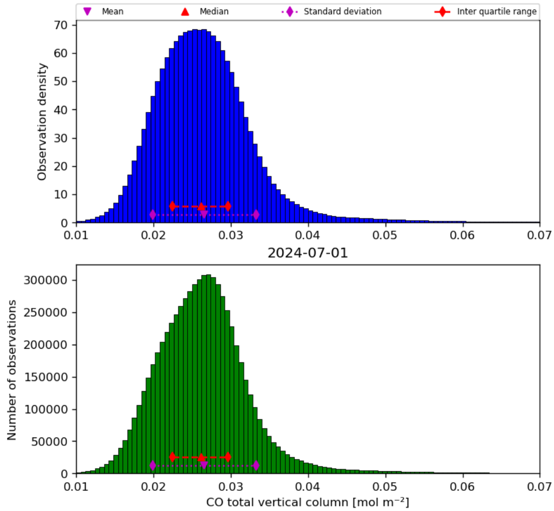
Figure 18: Histogram of “CO total vertical column” for 2024-06-30 to 2024-07-02
