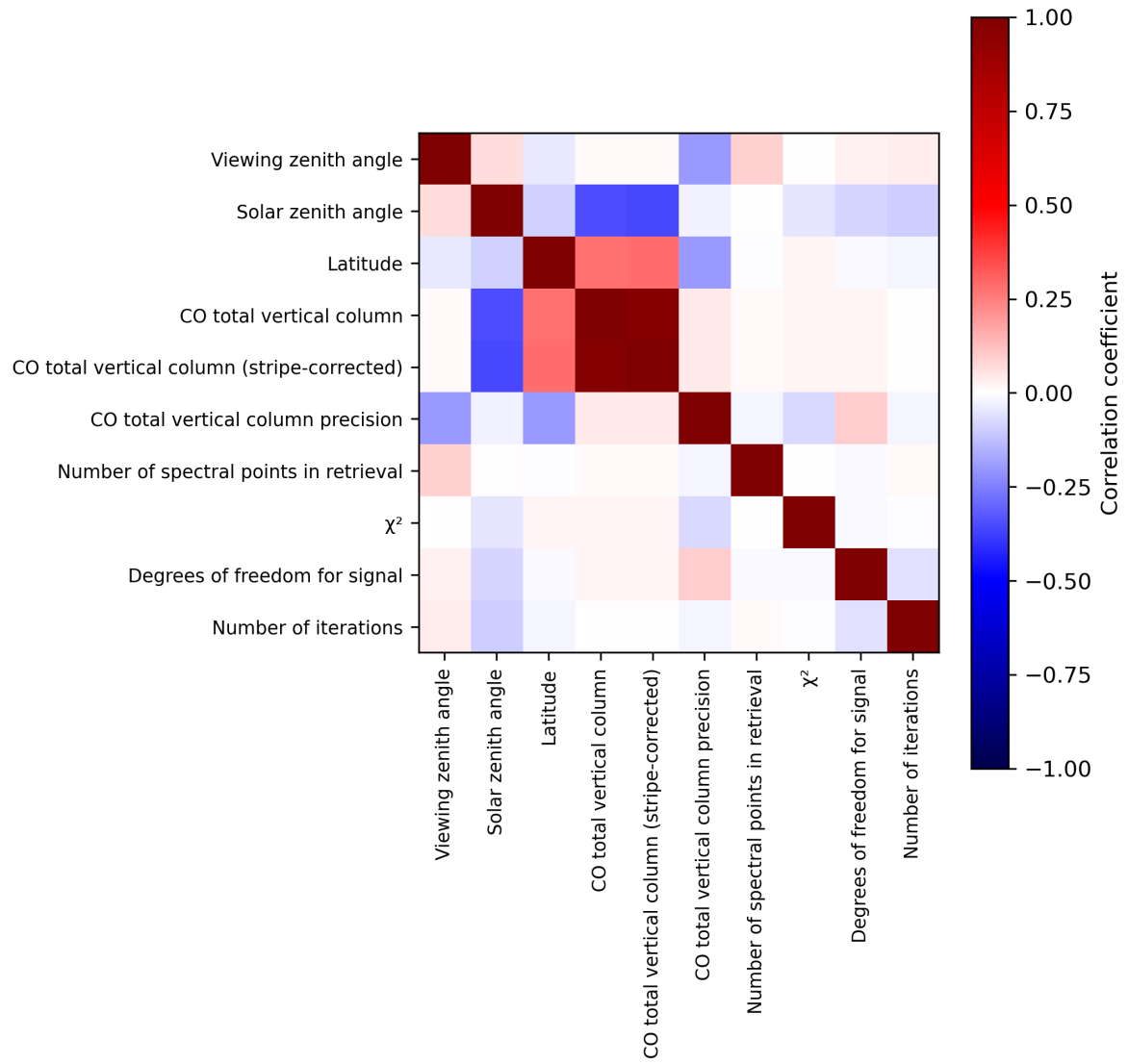
Figure 2: Map of correlation matrix for 2024-06-30 to 2024-07-02.
