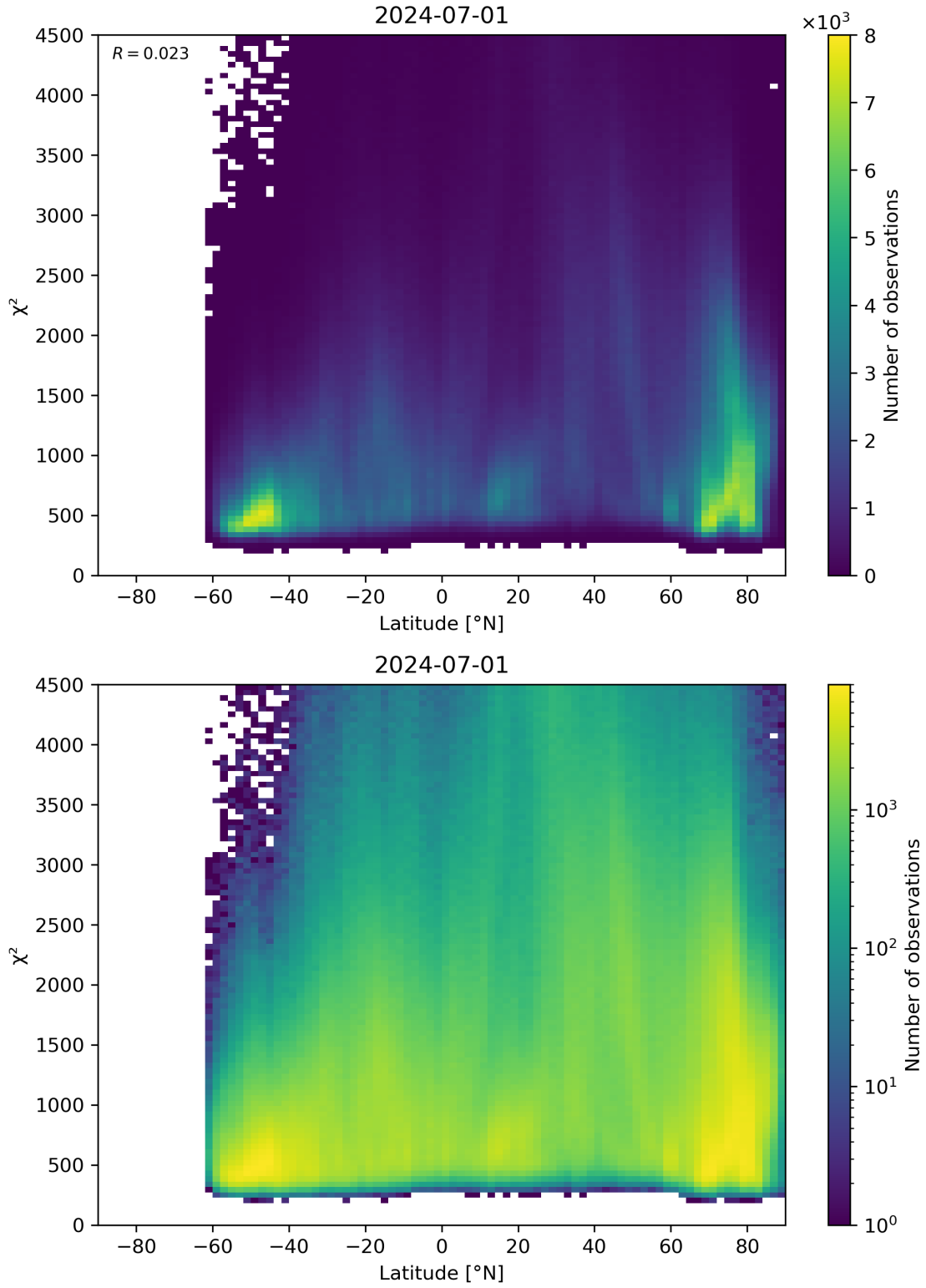
Figure 54: Scatter density plot of “Latitude” against “ \chi^2 ” for 2024-06-30 to 2024-07-02.
