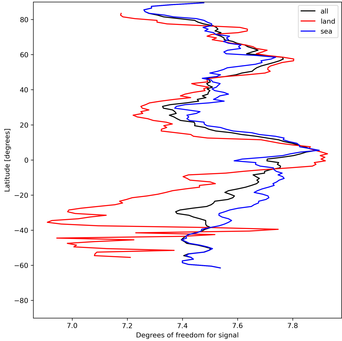
Figure 15: Zonal average of “Degrees of freedom for signal” for 2024-06-30 to 2024-07-02.
