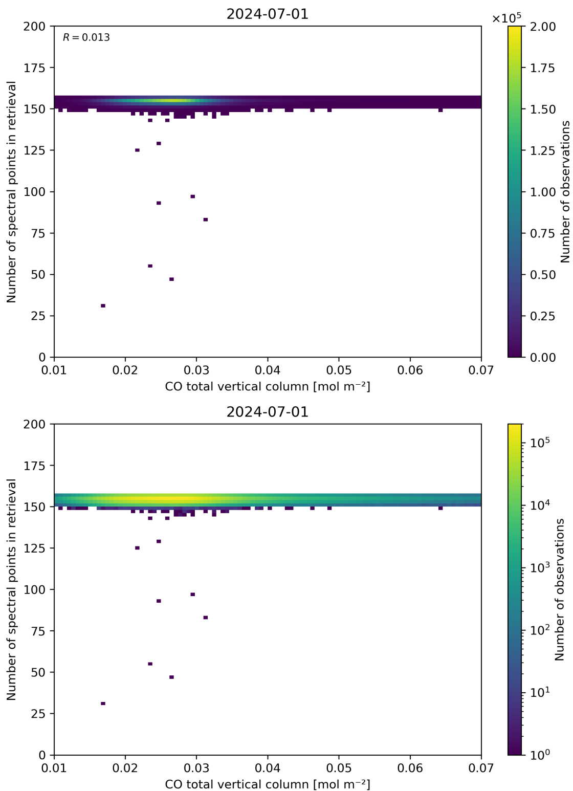
Figure 43: Scatter density plot of “CO total vertical column” against “Number of spectral points in retrieval” for 2024-06-30 to 2024-07-02.
