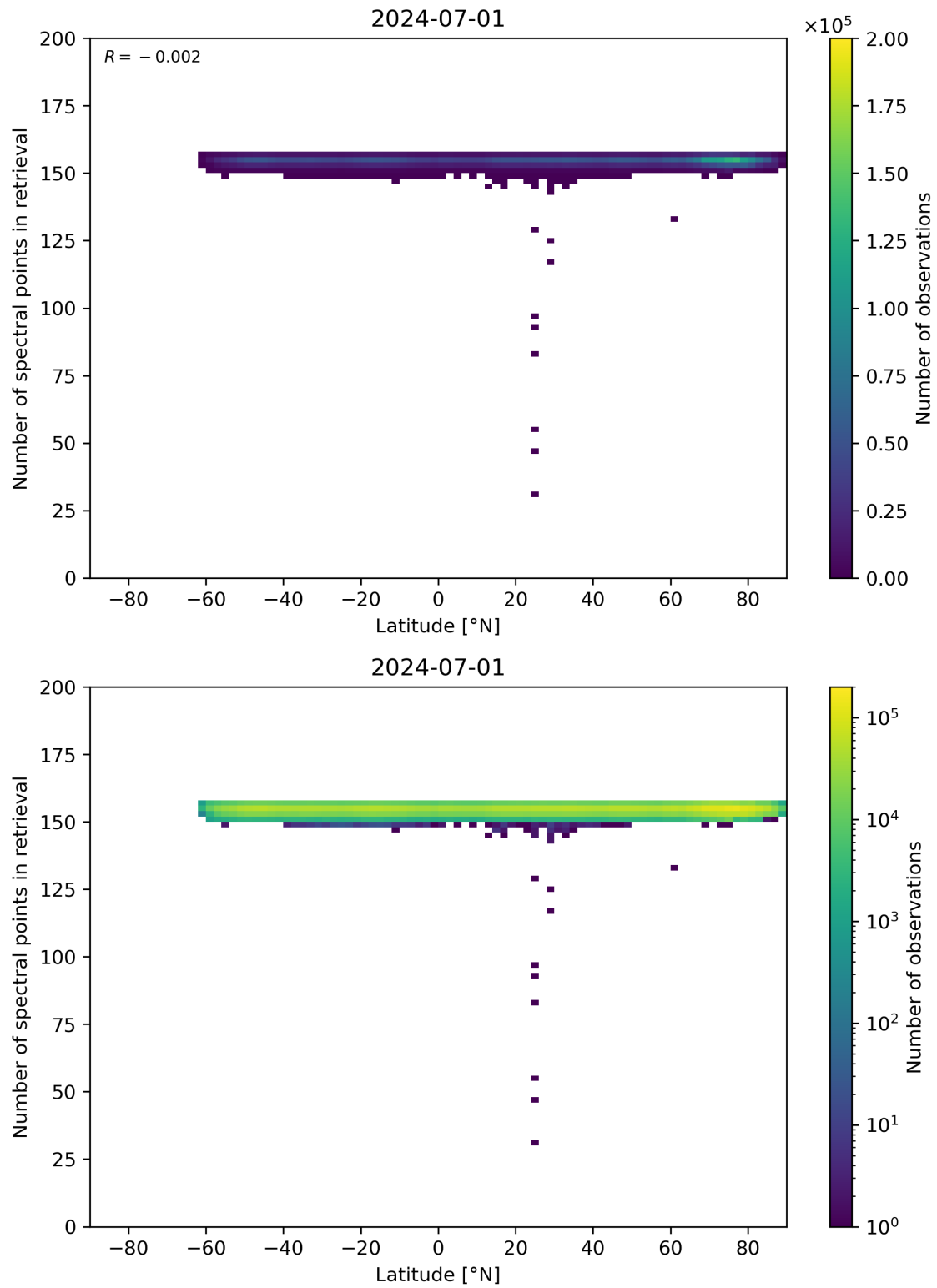
Figure 57: Scatter density plot of “Latitude” against “Number of spectral points in retrieval” for 2024-06-30 to 2024-07-02.
