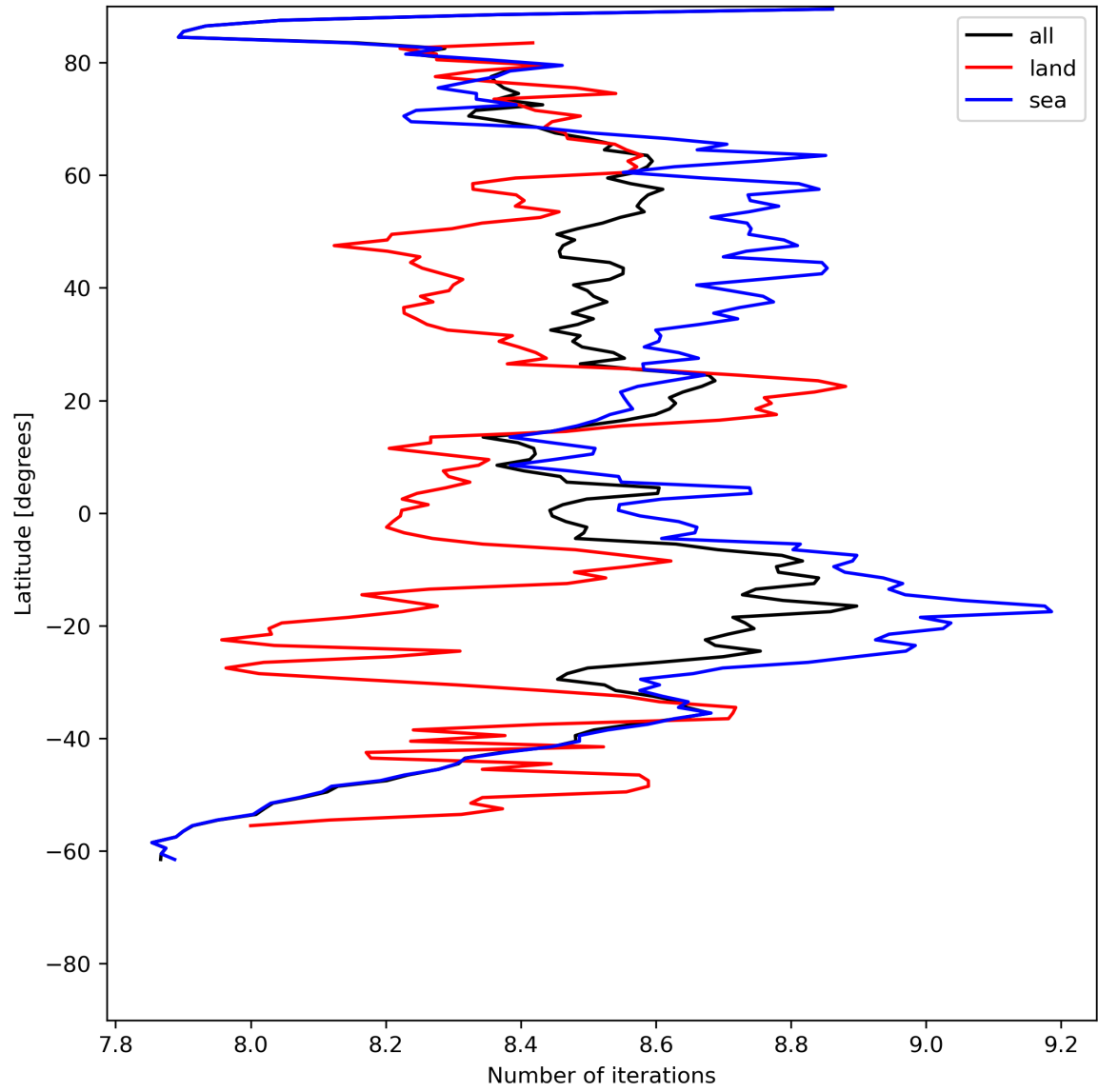
Figure 16: Zonal average of “Number of iterations” for 2024-06-30 to 2024-07-02.
