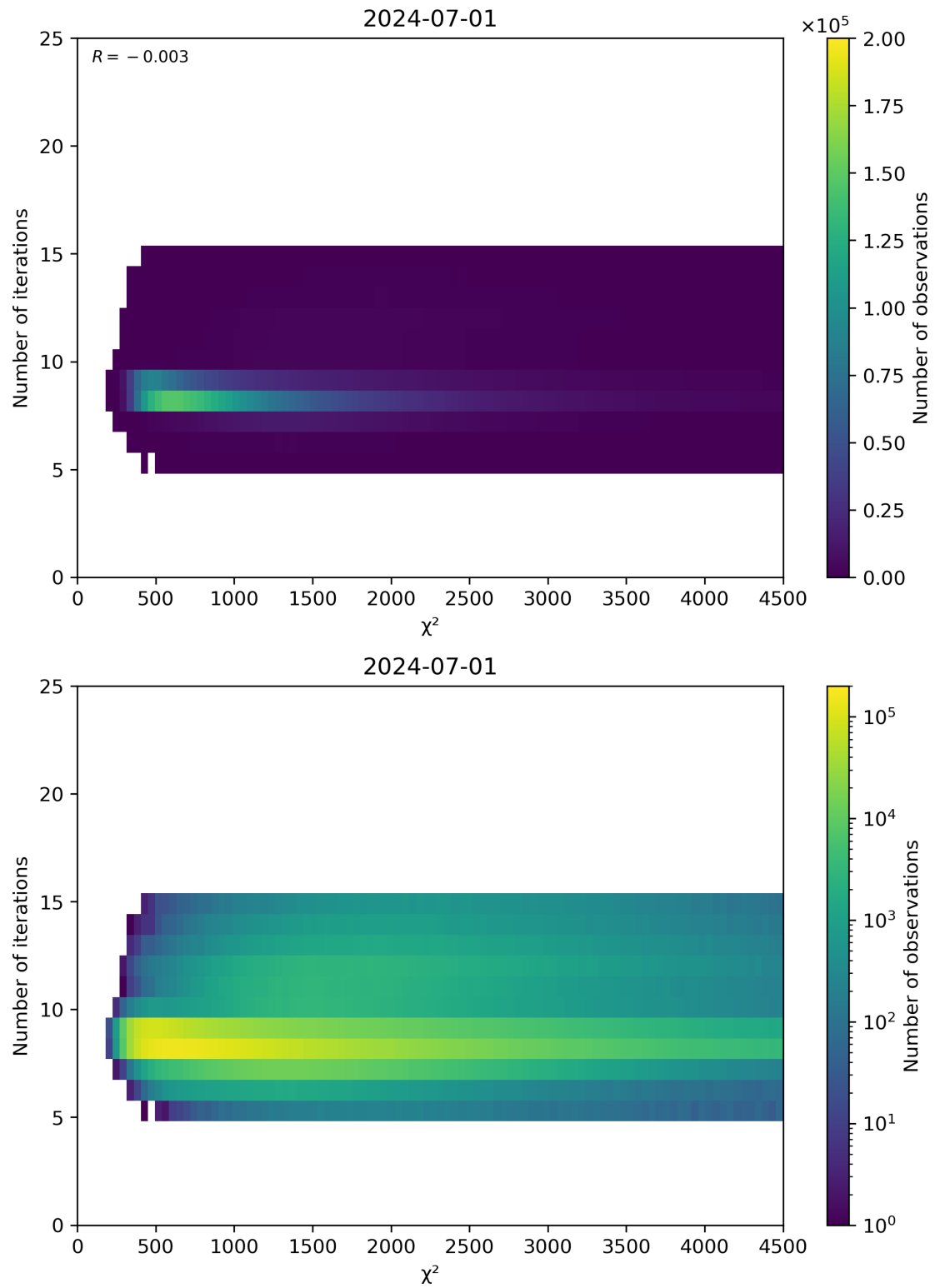
Figure 49: Scatter density plot of “ \chi^2 ” against “Number of iterations” for 2024-06-30 to 2024-07-02.
