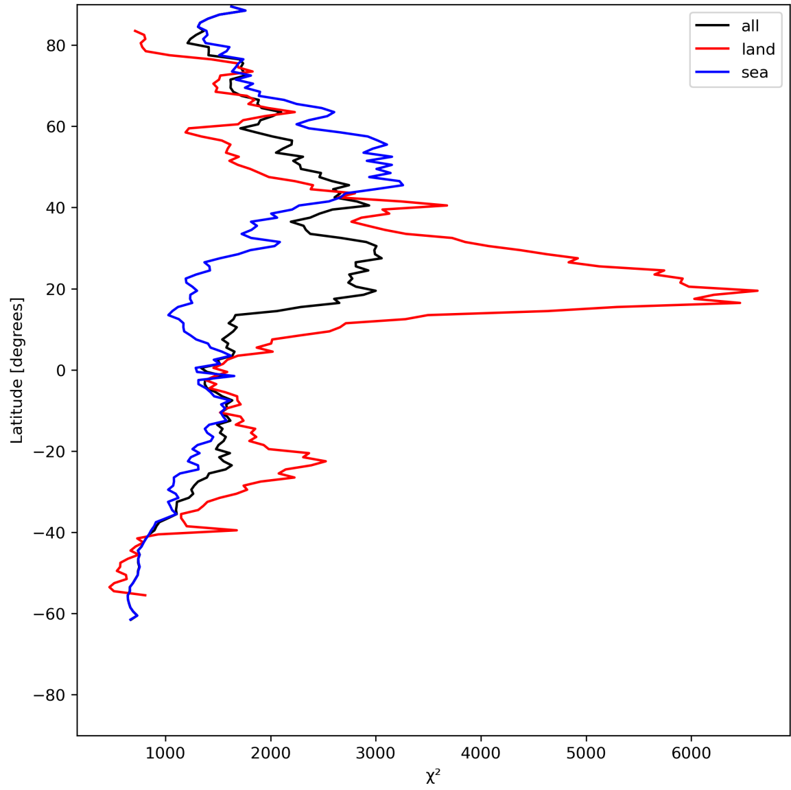
Figure 14: Zonal average of “ \chi^2 ” for 2024-06-30 to 2024-07-02.
