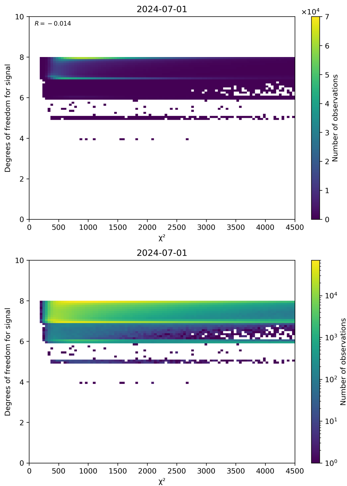
Figure 48: Scatter density plot of “ \chi^2 ” against “Degrees of freedom for signal” for 2024-06-30 to 2024-07-02.
