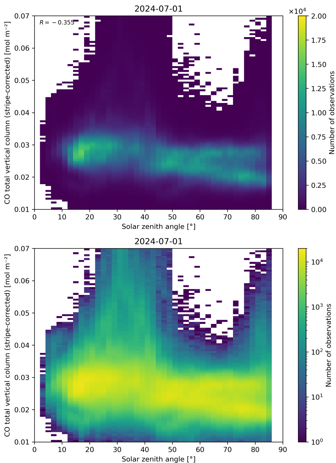
Figure 62: Scatter density plot of “Solar zenith angle” against “CO total vertical column (stripe-corrected)” for 2024-06-30 to 2024-07-02.
