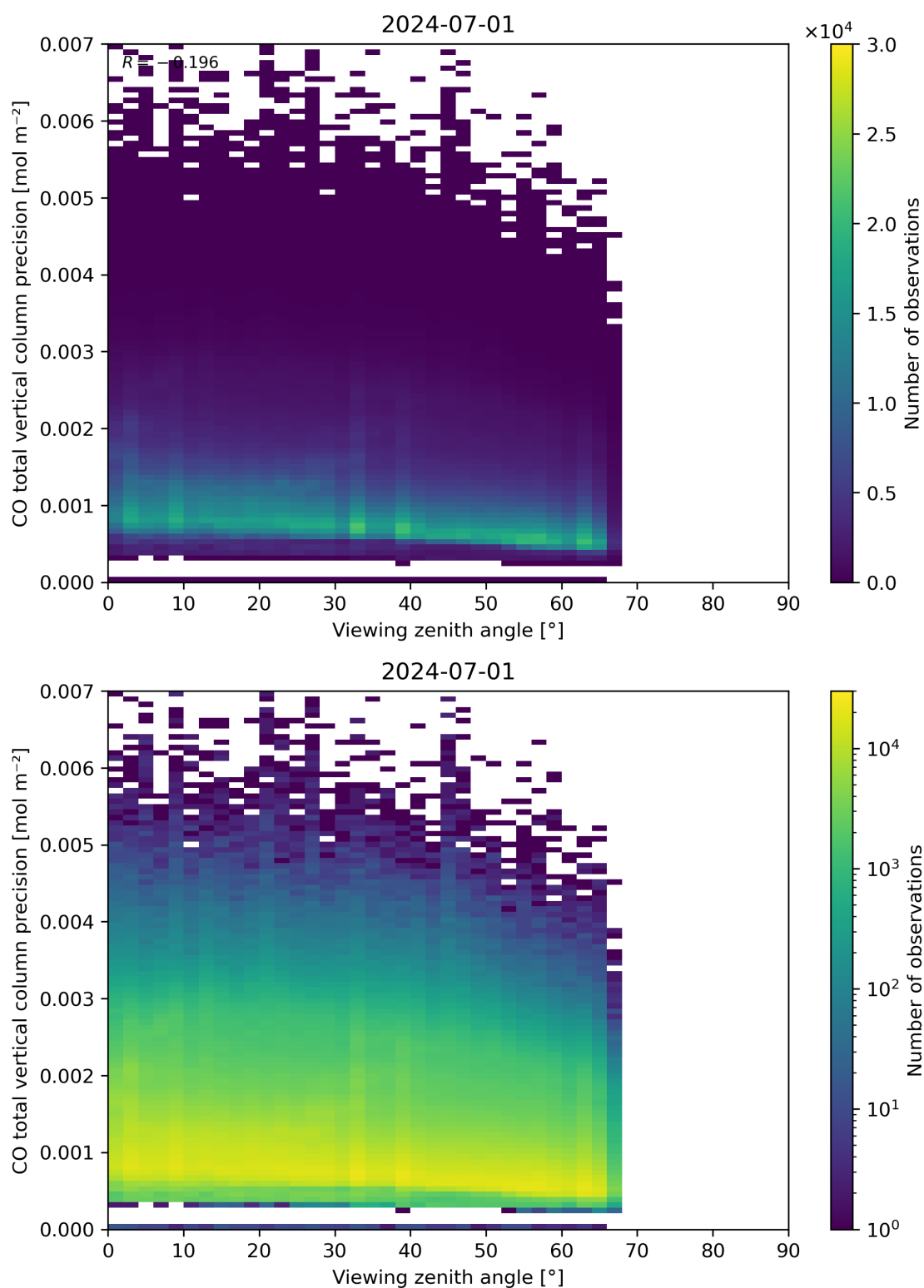
Figure 71: Scatter density plot of “Viewing zenith angle” against “CO total vertical column precision” for 2024-06-30 to 2024-07-02.
