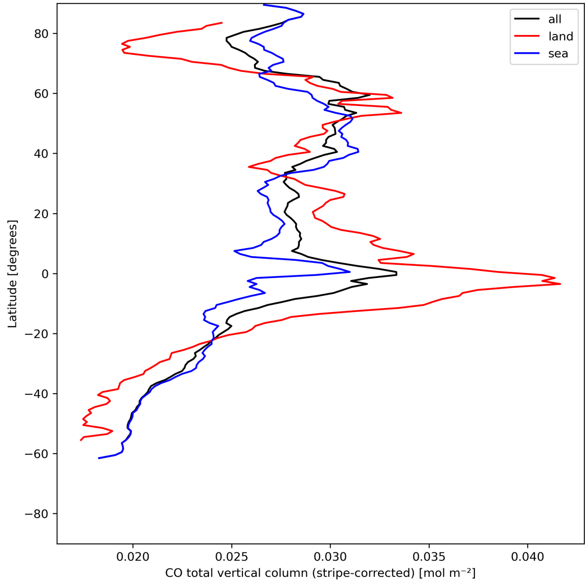
Figure 11: Zonal average of “CO total vertical column (stripe-corrected)” for 2024-06-30 to 2024-07-02.
