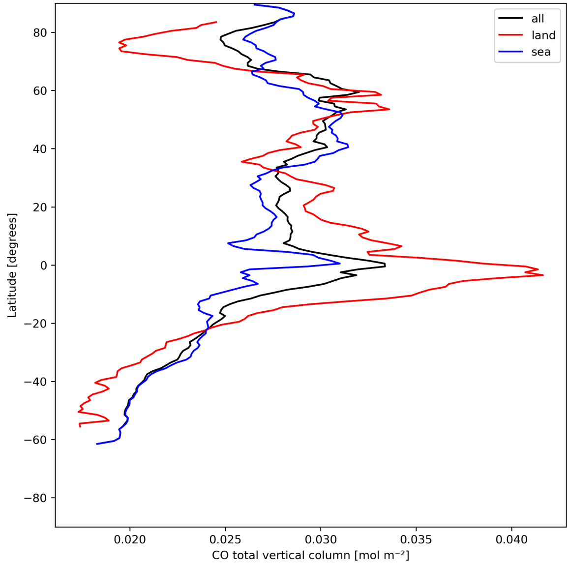
Figure 10: Zonal average of “CO total vertical column” for 2024-06-30 to 2024-07-02.
