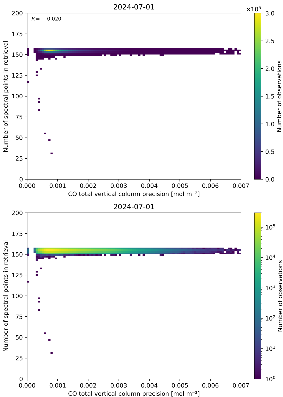
Figure 47: Scatter density plot of “CO total vertical column precision” against “Number of spectral points in retrieval” for 2024-06-30 to 2024-07-02.
