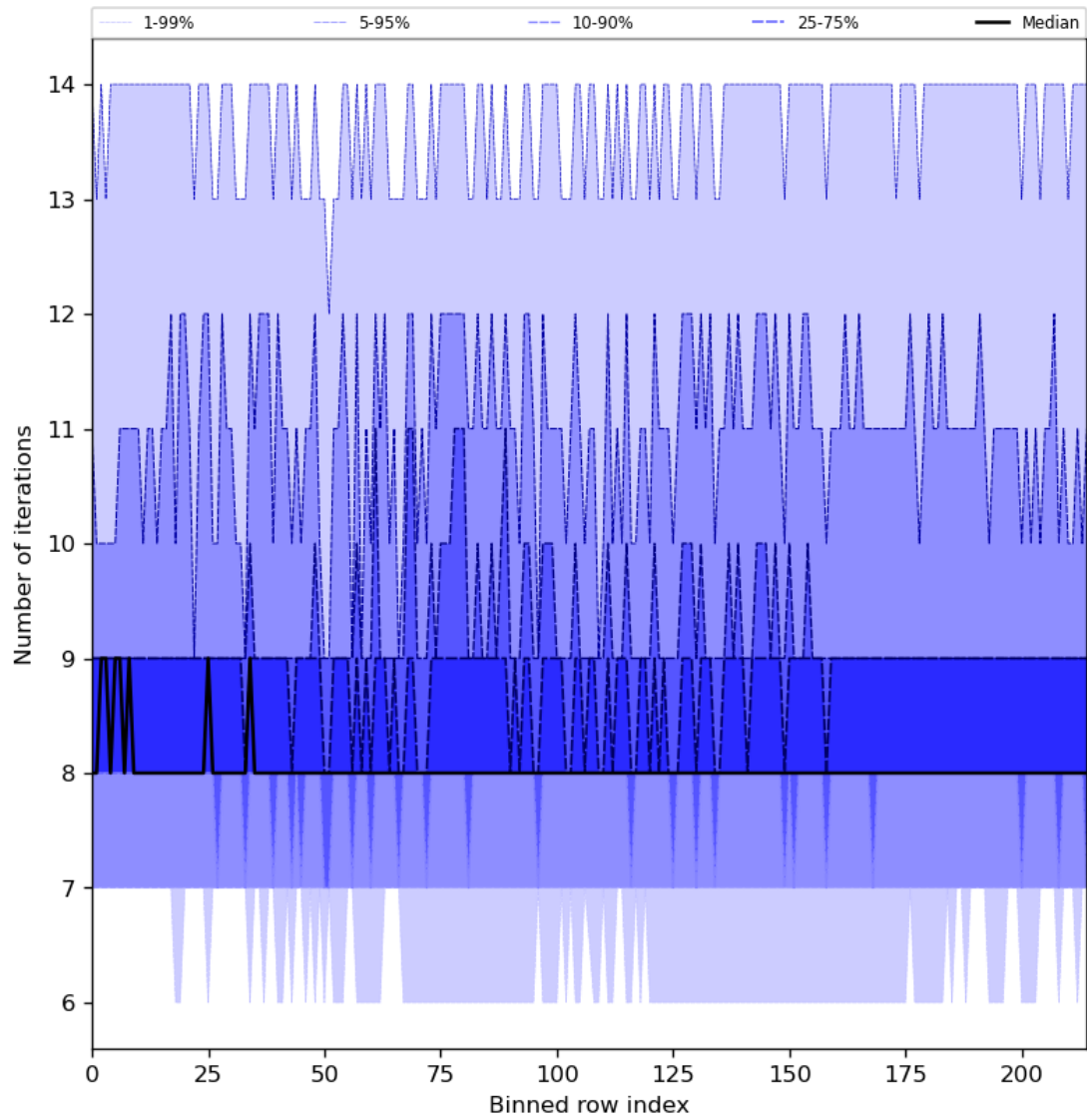
Figure 32: Along track statistics of “Number of iterations” for 2024-06-30 to 2024-07-02
