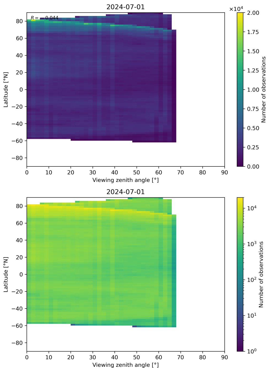
Figure 74: Scatter density plot of “Viewing zenith angle” against “Latitude” for 2024-06-30 to 2024-07-02.
