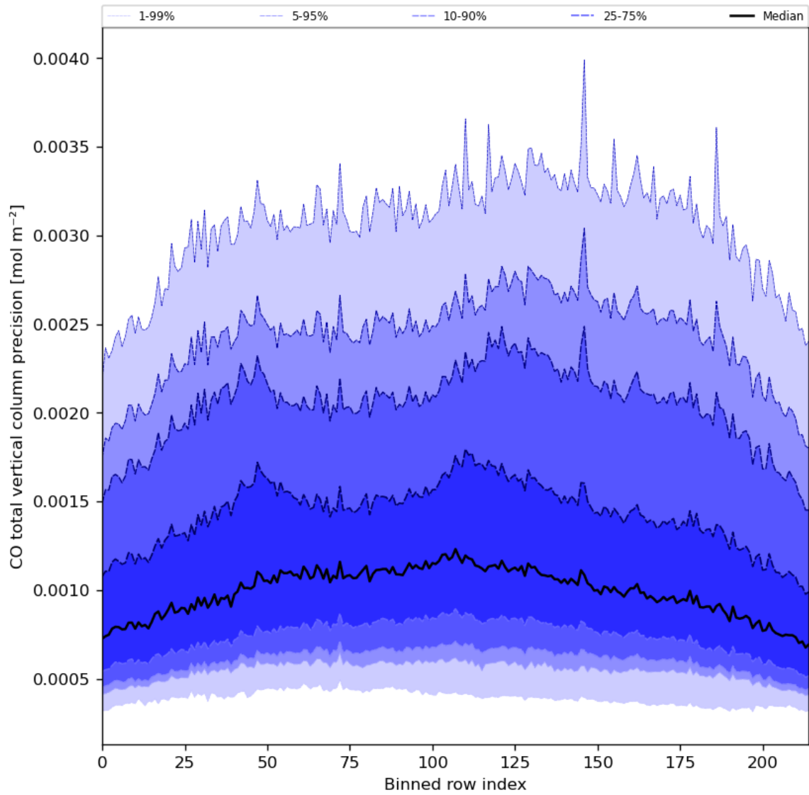
Figure 28: Along track statistics of “CO total vertical column precision” for 2024-06-30 to 2024-07-02
