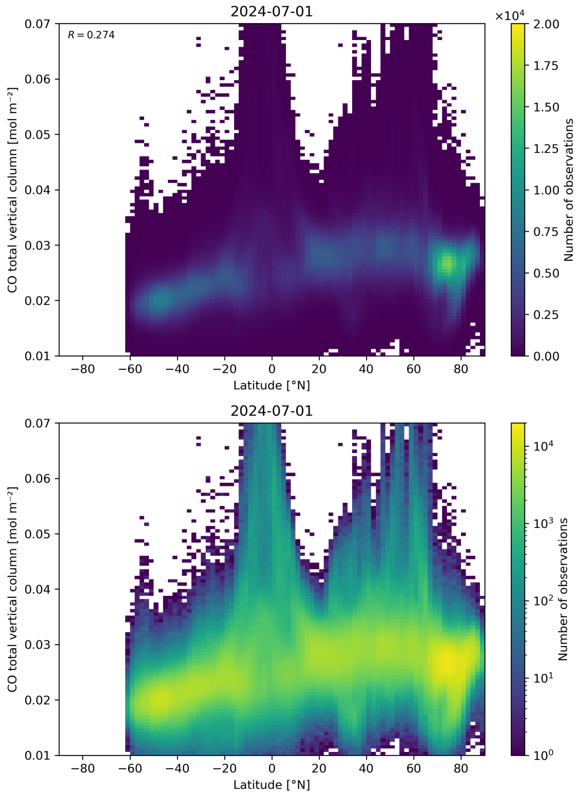
Figure 51: Scatter density plot of “Latitude” against “CO total vertical column” for 2024-06-30 to 2024-07-02.
