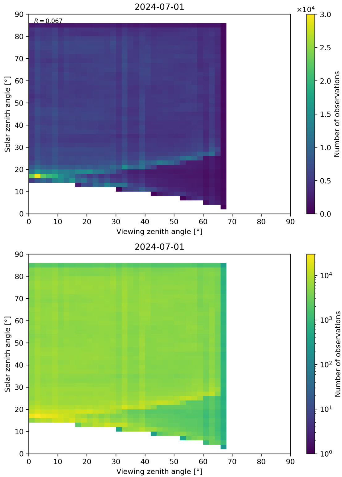
Figure 77: Scatter density plot of “Viewing zenith angle” against “Solar zenith angle” for 2024-06-30 to 2024-07-02.
