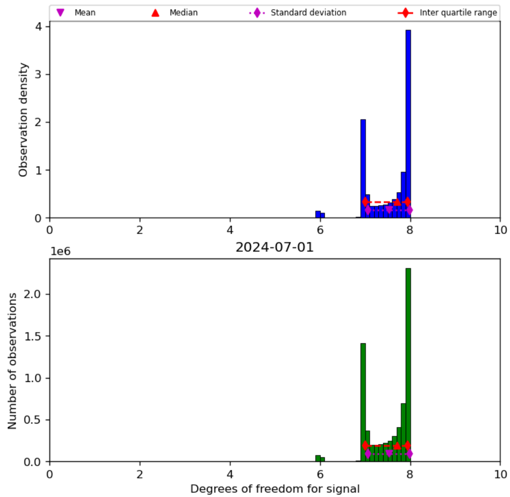
Figure 23: Histogram of “Degrees of freedom for signal” for 2024-06-30 to 2024-07-02
