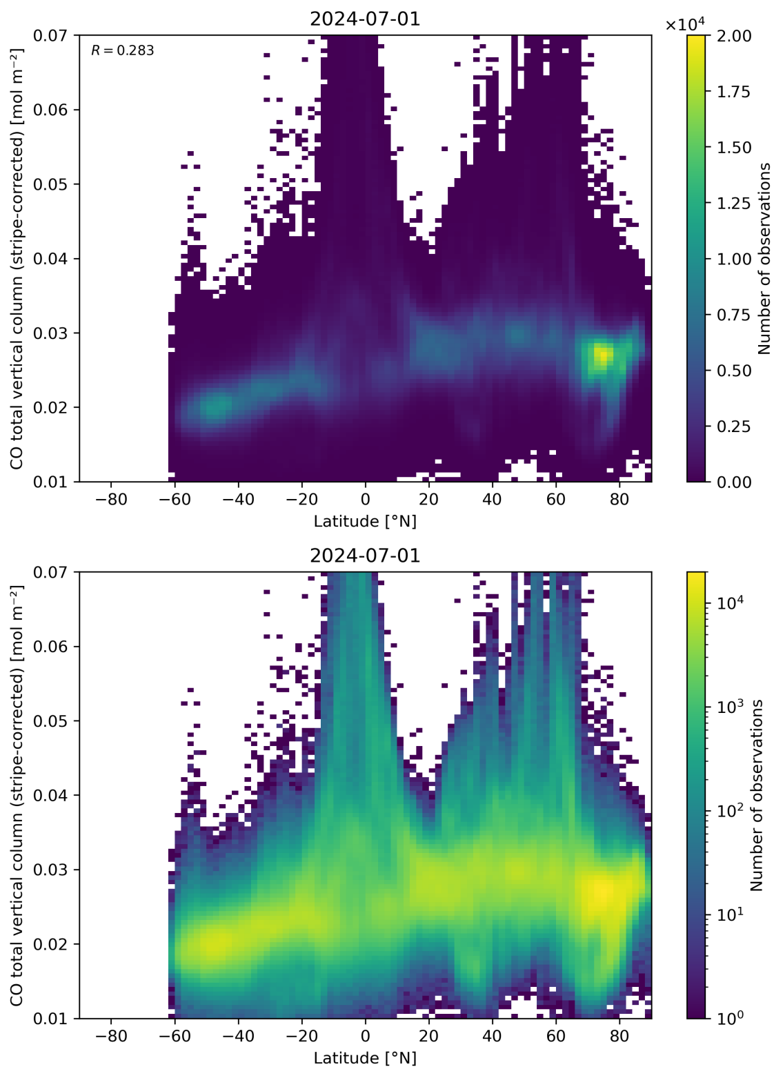
Figure 52: Scatter density plot of “Latitude” against “CO total vertical column (stripe-corrected)” for 2024-06-30 to 2024-07-02.
