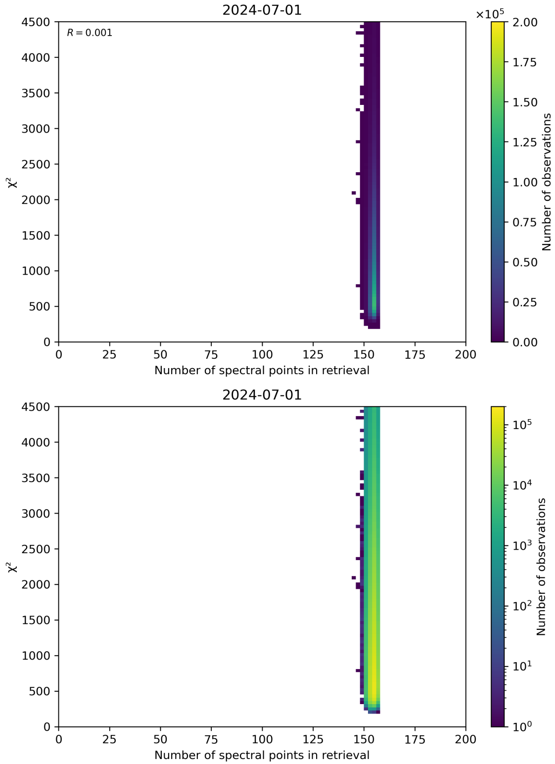
Figure 58: Scatter density plot of “Number of spectral points in retrieval” against “ \chi^2 ” for 2024-06-30 to 2024-07-02.
