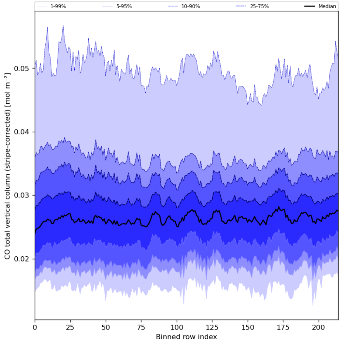
Figure 27: Along track statistics of “CO total vertical column (stripe-corrected)” for 2024-06-30 to 2024-07-02
