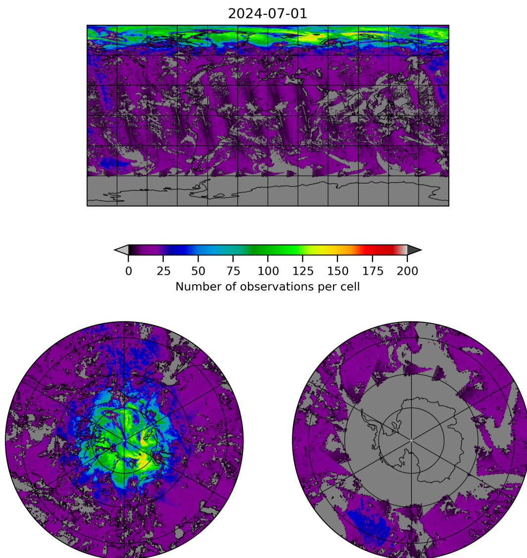
Figure 8: Map of the number of observations for 2024-06-30 to 2024-07-02
