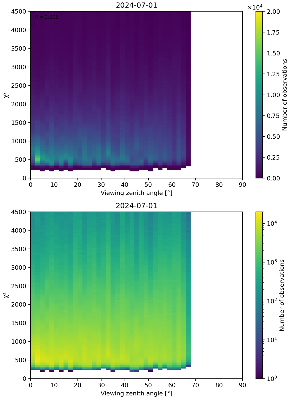
Figure 72: Scatter density plot of “Viewing zenith angle” against “ \chi^2 ” for 2024-06-30 to 2024-07-02.
