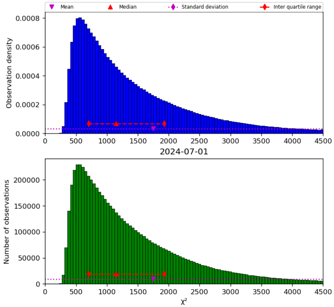
Figure 22: Histogram of “ \chi^2 ” for 2024-06-30 to 2024-07-02
