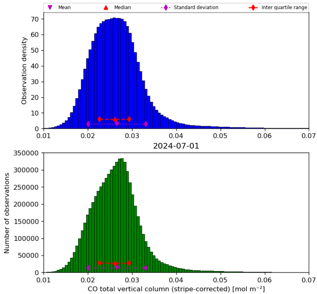
Figure 19: Histogram of “CO total vertical column (stripe-corrected)” for 2024-06-30 to 2024-07-02
