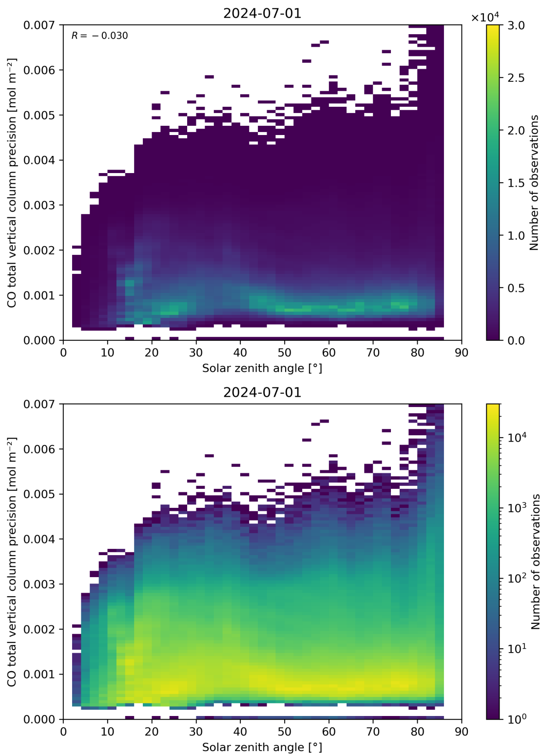
Figure 63: Scatter density plot of “Solar zenith angle” against “CO total vertical column precision” for 2024-06-30 to 2024-07-02.
