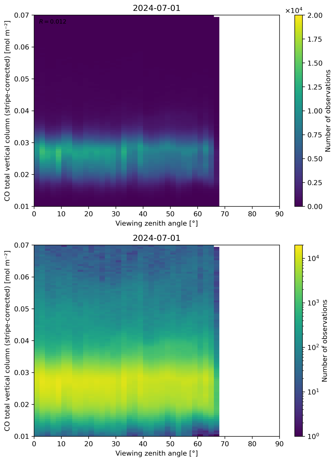
Figure 70: Scatter density plot of “Viewing zenith angle” against “CO total vertical column (stripe-corrected)” for 2024-06-30 to 2024-07-02.
