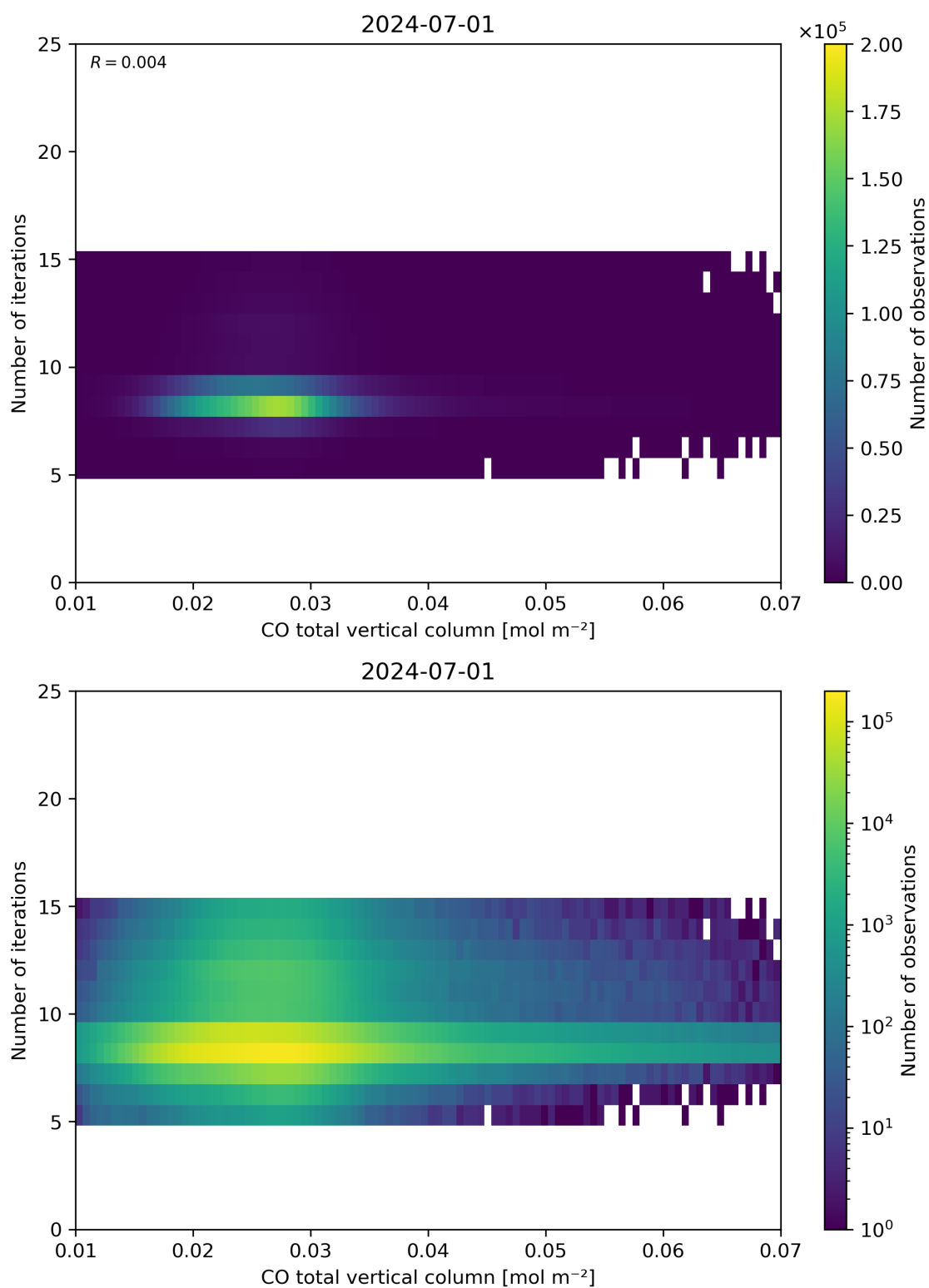
Figure 42: Scatter density plot of “CO total vertical column” against “Number of iterations” for 2024-06-30 to 2024-07-02.
