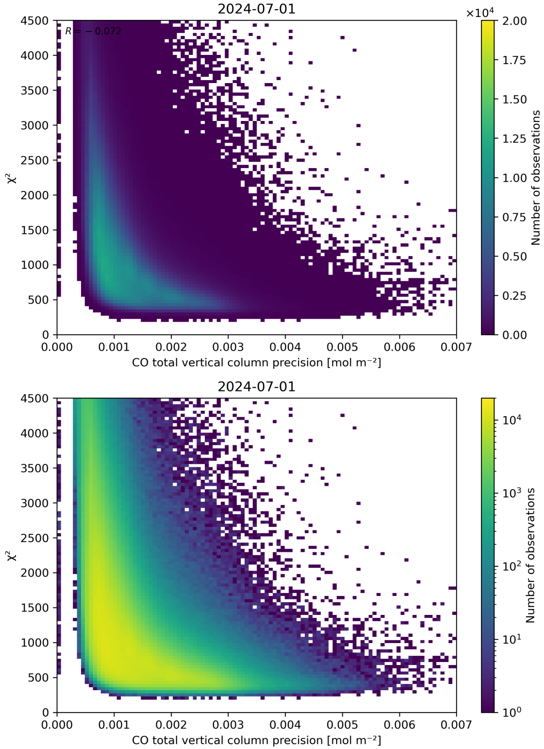
Figure 44: Scatter density plot of “CO total vertical column precision” against “ \chi^2 ” for 2024-06-30 to 2024-07-02.
