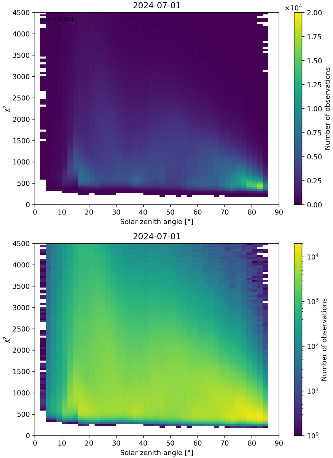
Figure 64: Scatter density plot of “Solar zenith angle” against “ \chi^2 ” for 2024-06-30 to 2024-07-02.
