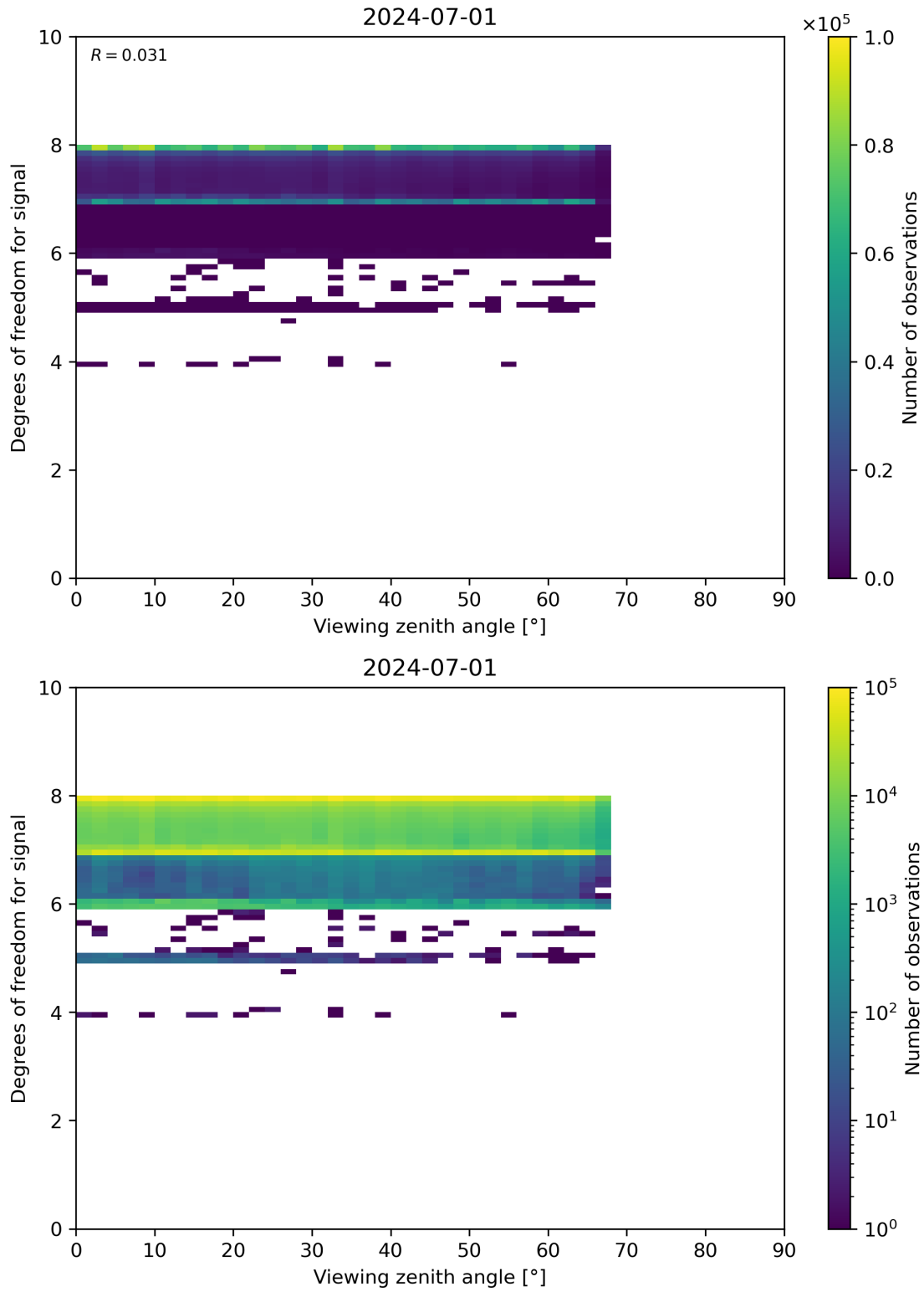
Figure 73: Scatter density plot of “Viewing zenith angle” against “Degrees of freedom for signal” for 2024-06-30 to 2024-07-02.
