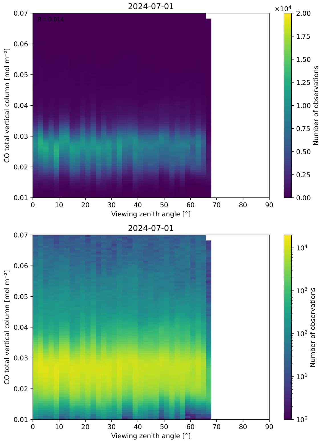
Figure 69: Scatter density plot of “Viewing zenith angle” against “CO total vertical column” for 2024-06-30 to 2024-07-02.
