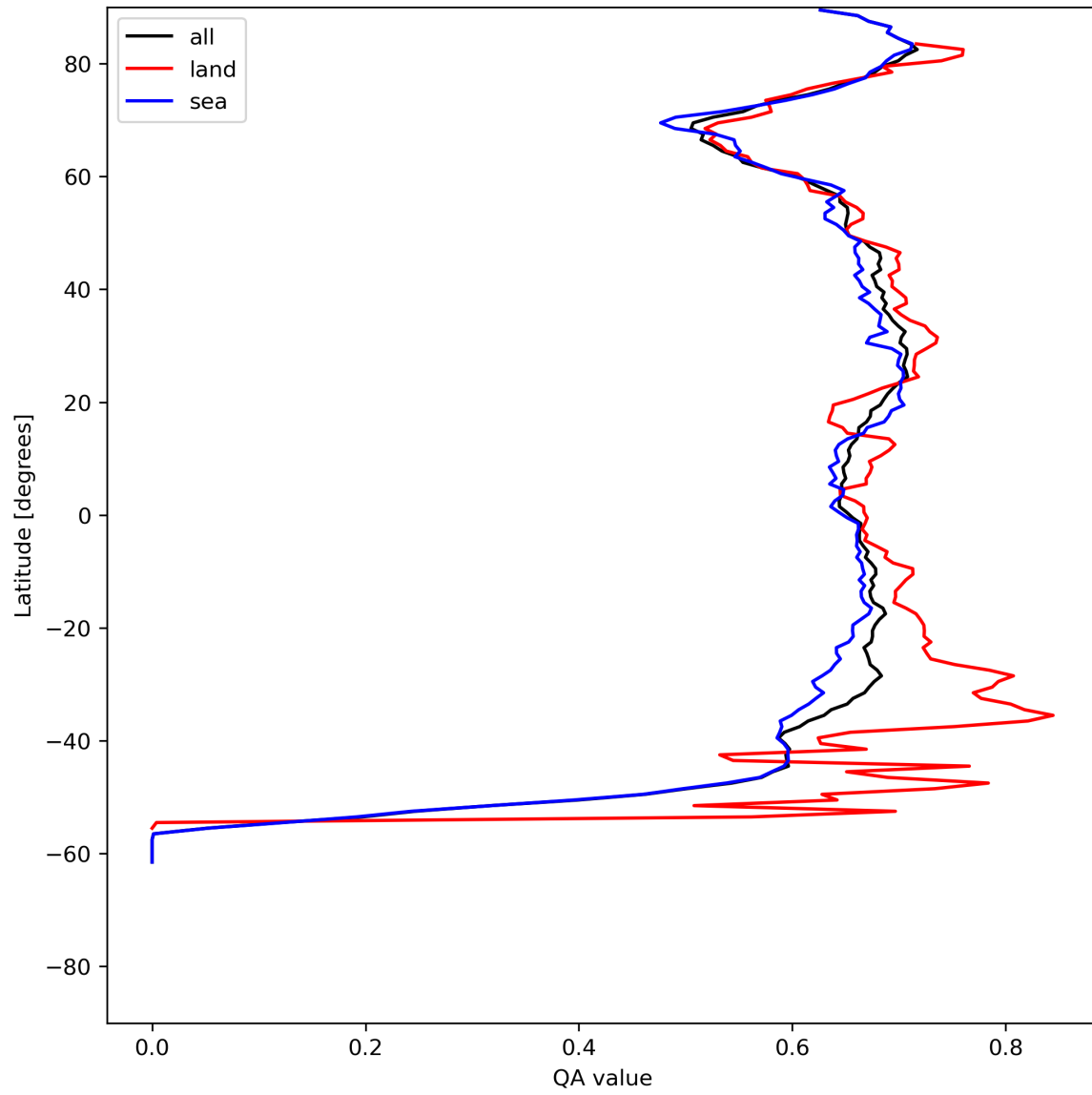
Figure 9: Zonal average of “QA value” for 2024-06-30 to 2024-07-02.
