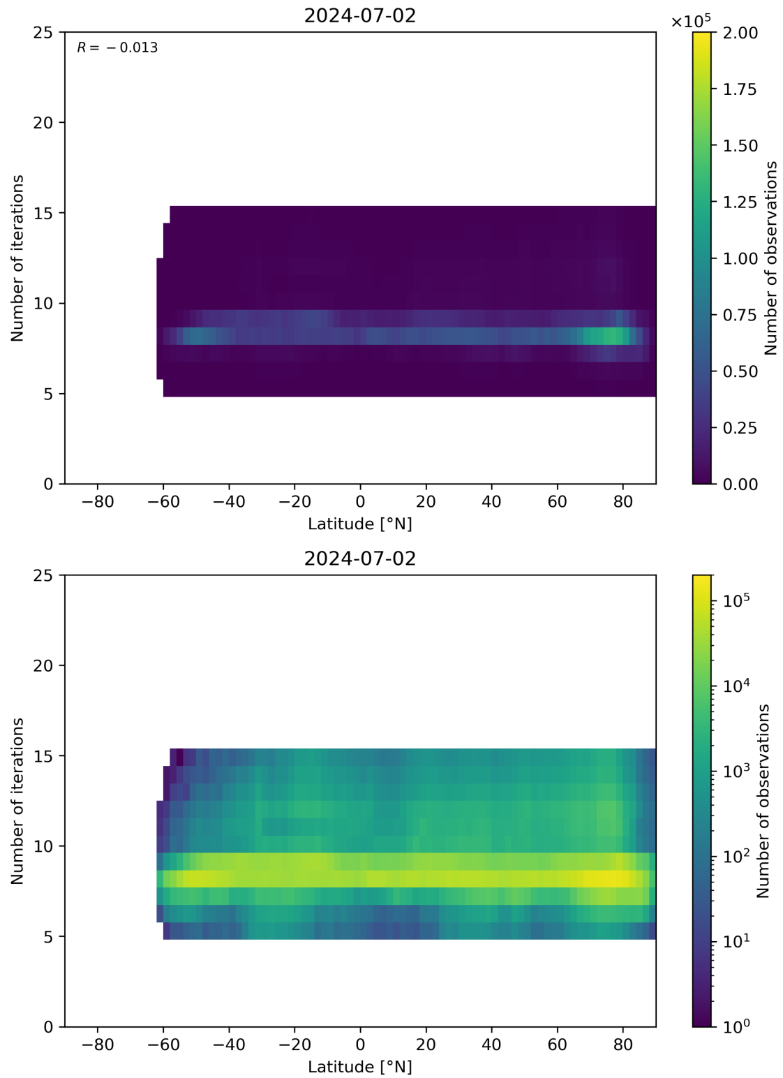
Figure 56: Scatter density plot of “Latitude” against “Number of iterations” for 2024-07-01 to 2024-07-03.
