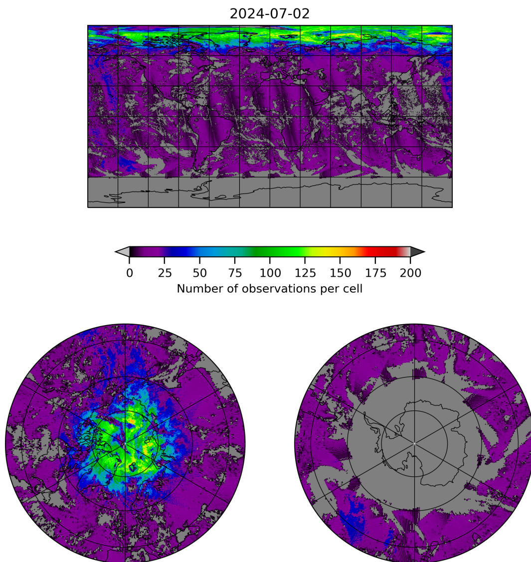
Figure 8: Map of the number of observations for 2024-07-01 to 2024-07-03
