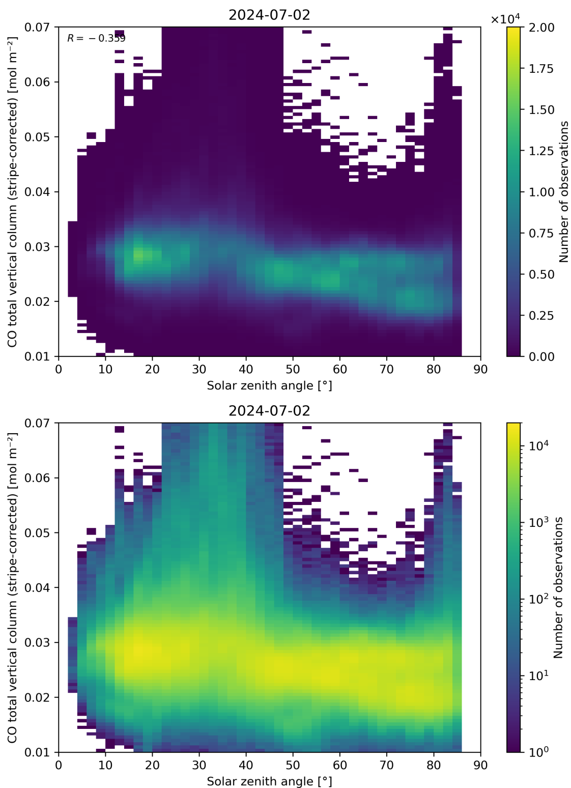
Figure 62: Scatter density plot of “Solar zenith angle” against “CO total vertical column (stripe-corrected)” for 2024-07-01 to 2024-07-03.
