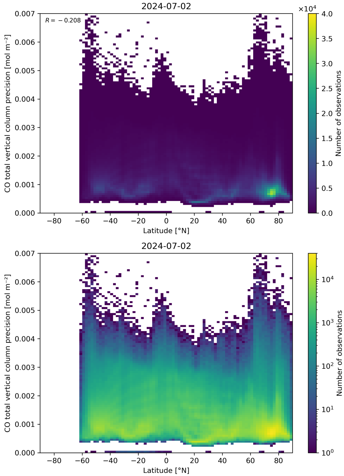
Figure 53: Scatter density plot of “Latitude” against “CO total vertical column precision” for 2024-07-01 to 2024-07-03.
