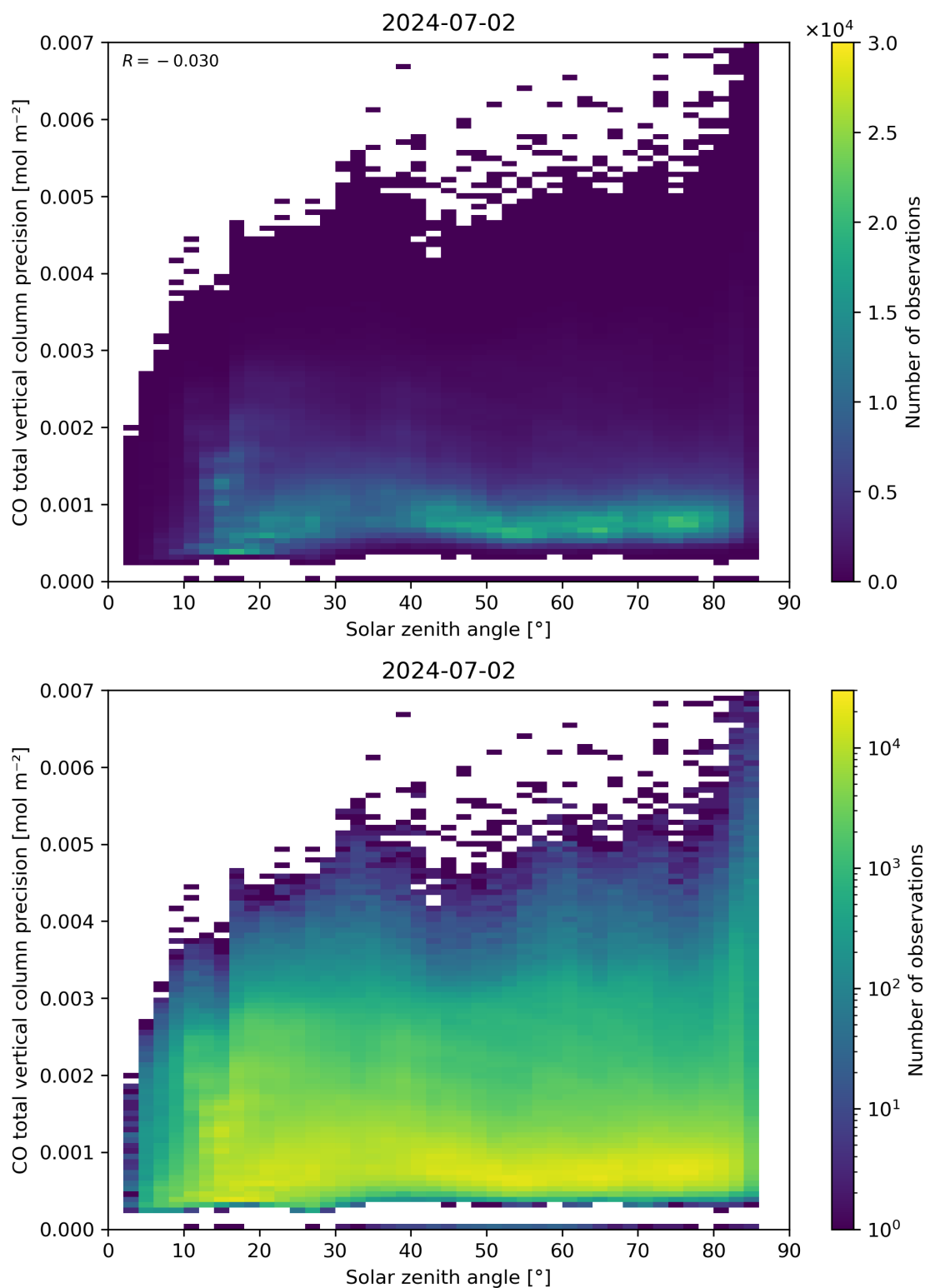
Figure 63: Scatter density plot of “Solar zenith angle” against “CO total vertical column precision” for 2024-07-01 to 2024-07-03.
