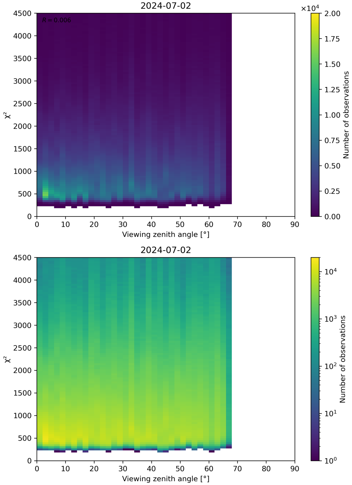
Figure 72: Scatter density plot of “Viewing zenith angle” against “ \chi^2 ” for 2024-07-01 to 2024-07-03.
