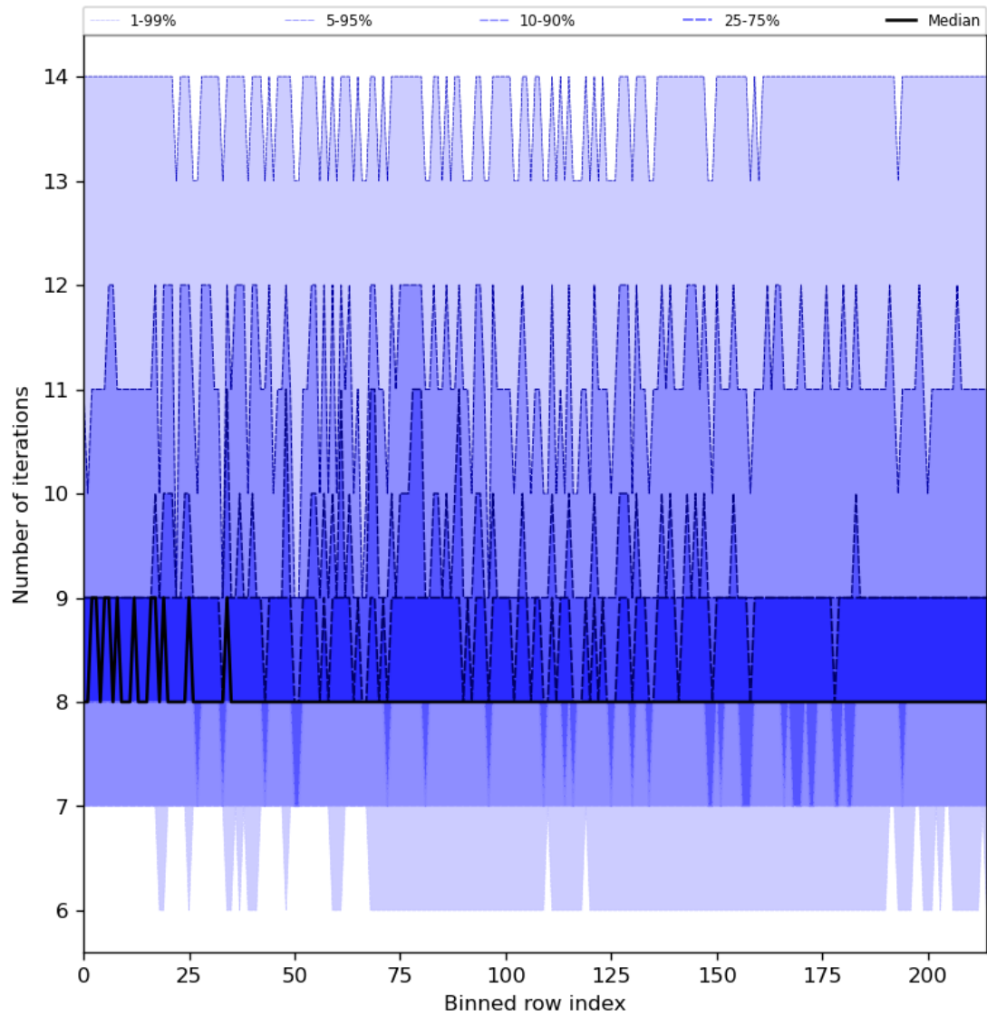
Figure 32: Along track statistics of “Number of iterations” for 2024-07-01 to 2024-07-03
