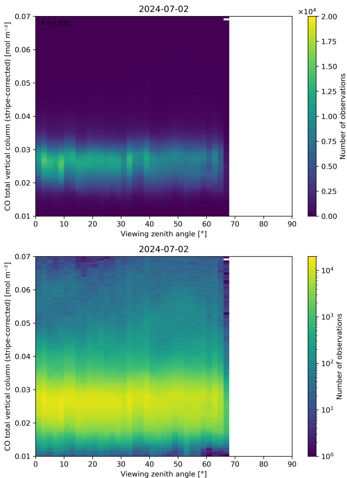
Figure 70: Scatter density plot of “Viewing zenith angle” against “CO total vertical column (stripe-corrected)” for 2024-07-01 to 2024-07-03.
