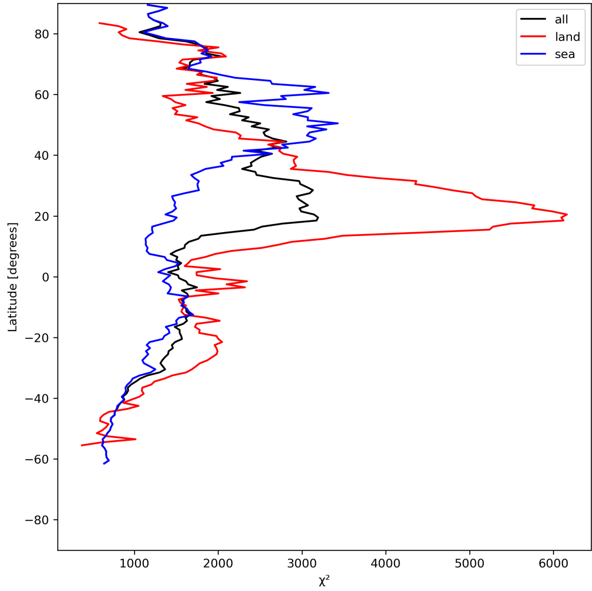
Figure 14: Zonal average of “ \chi^2 ” for 2024-07-01 to 2024-07-03.
