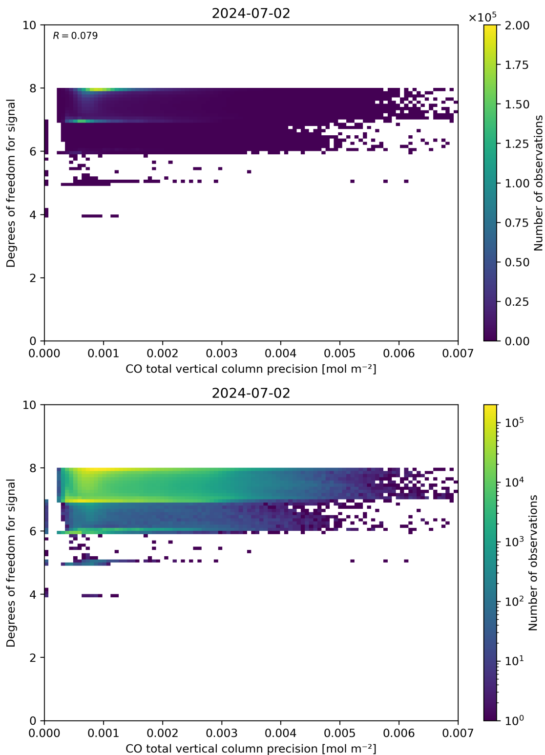
Figure 45: Scatter density plot of “CO total vertical column precision” against “Degrees of freedom for signal” for 2024-07-01 to 2024-07-03.
