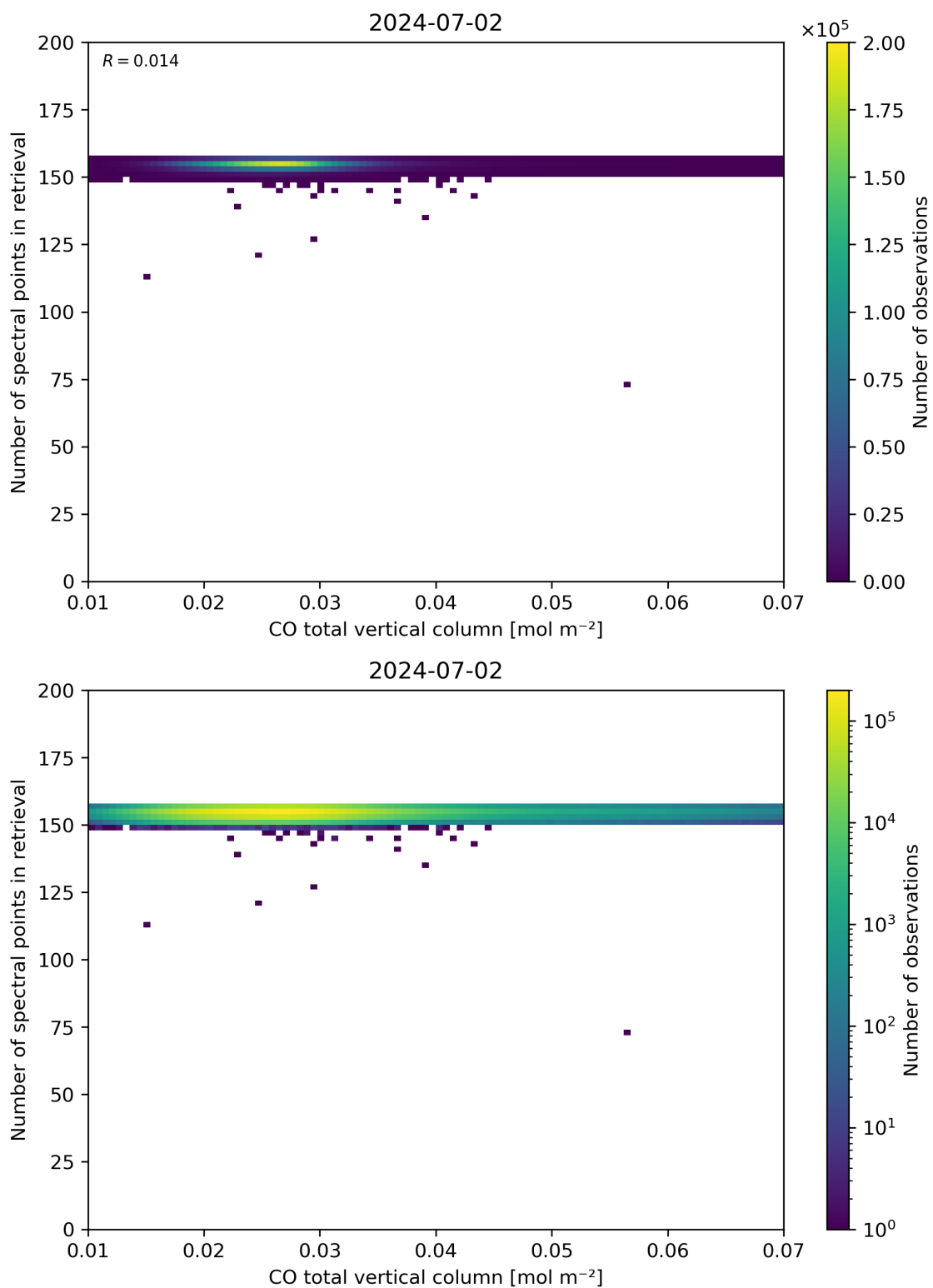
Figure 43: Scatter density plot of “CO total vertical column” against “Number of spectral points in retrieval” for 2024-07-01 to 2024-07-03.
