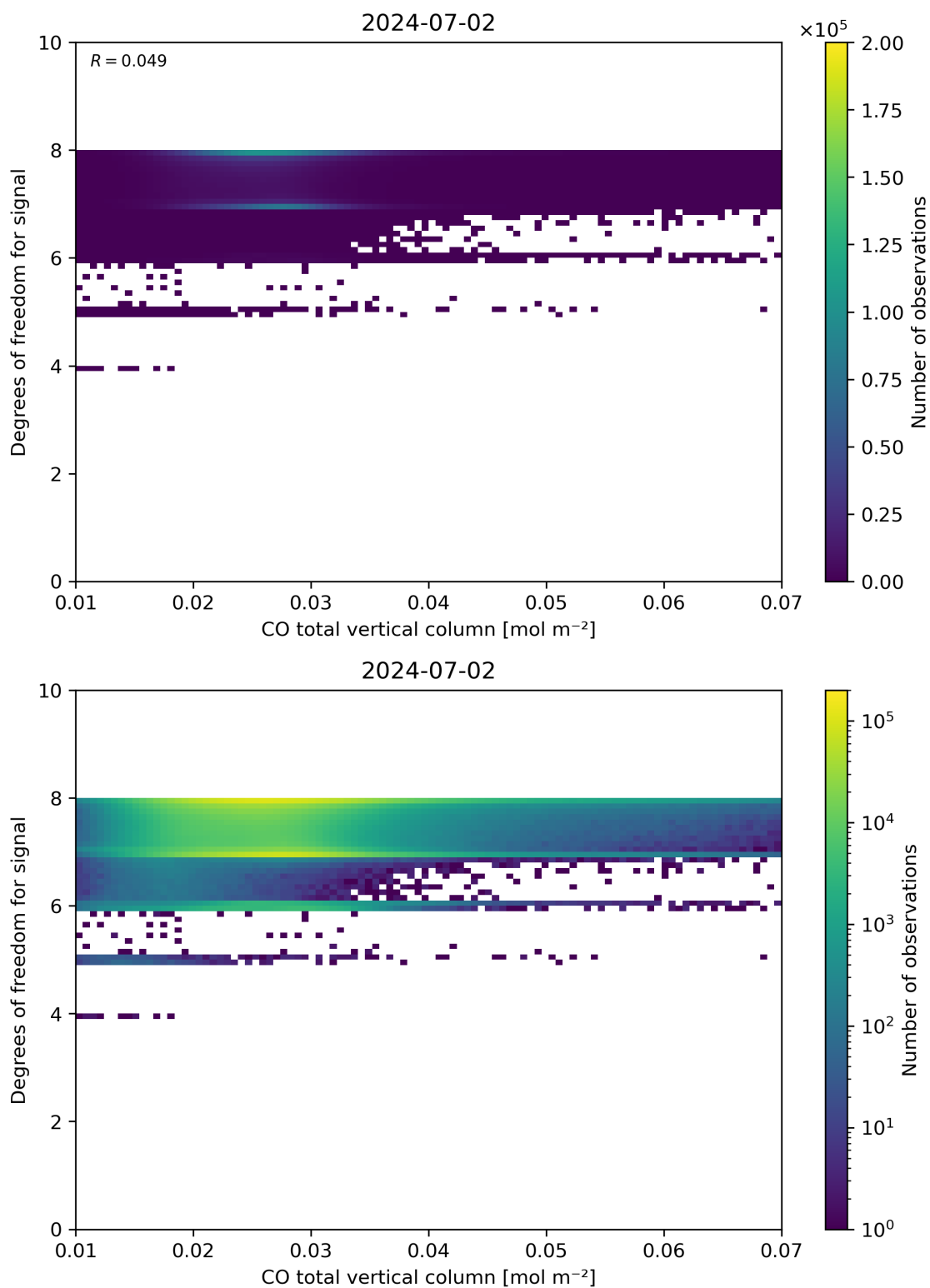
Figure 41: Scatter density plot of “CO total vertical column” against “Degrees of freedom for signal” for 2024-07-01 to 2024-07-03.
