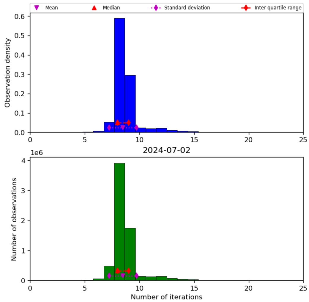
Figure 24: Histogram of “Number of iterations” for 2024-07-01 to 2024-07-03
