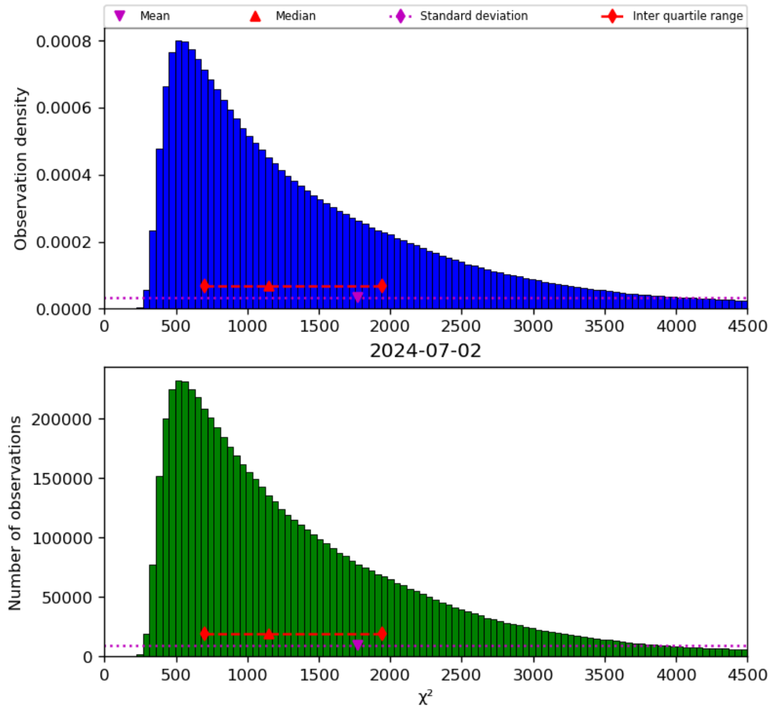
Figure 22: Histogram of “ \chi^2 ” for 2024-07-01 to 2024-07-03
