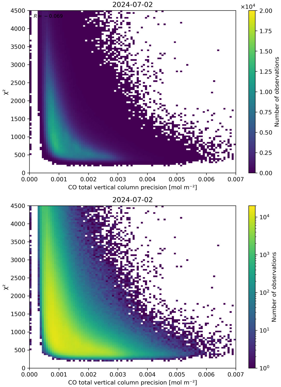
Figure 44: Scatter density plot of “CO total vertical column precision” against “ \chi^2 ” for 2024-07-01 to 2024-07-03.
