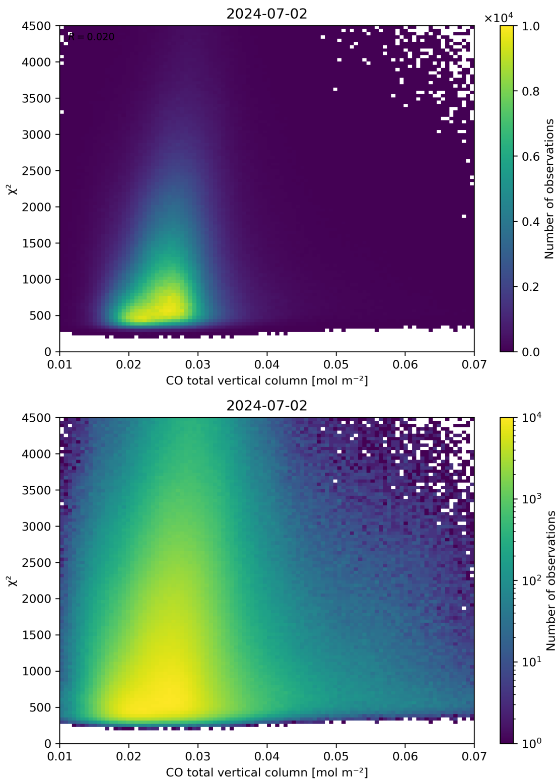
Figure 35: Scatter density plot of “CO total vertical column” against “ \chi^2 ” for 2024-07-01 to 2024-07-03.
