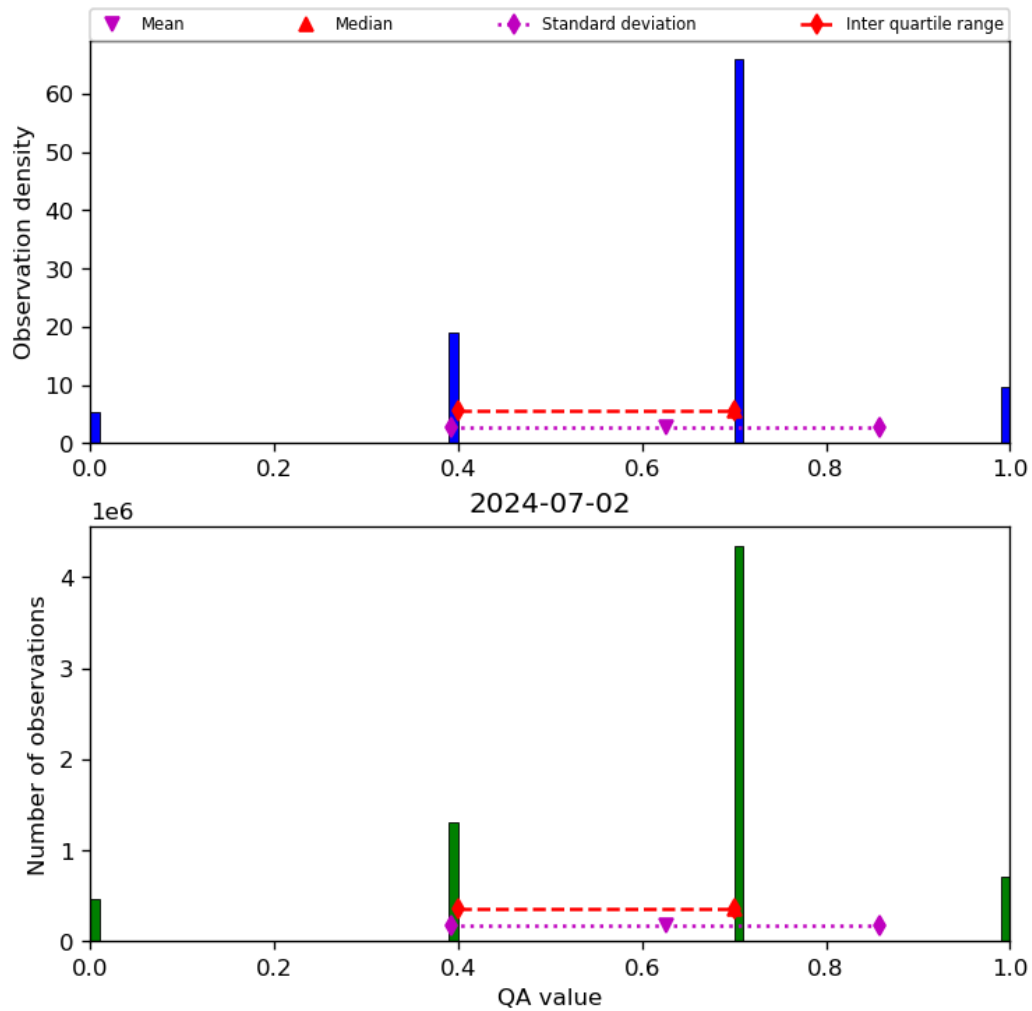
Figure 17: Histogram of “QA value” for 2024-07-01 to 2024-07-03
