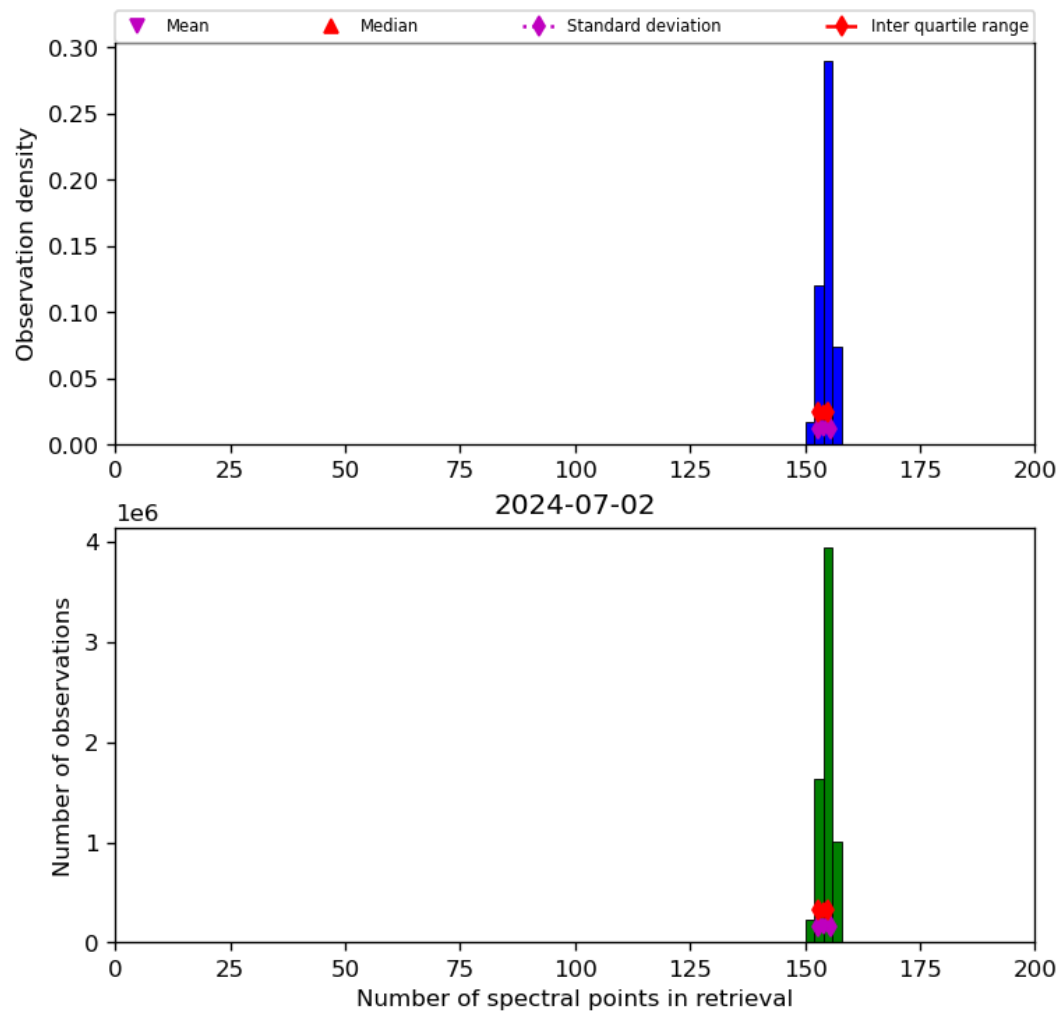
Figure 21: Histogram of “Number of spectral points in retrieval” for 2024-07-01 to 2024-07-03
