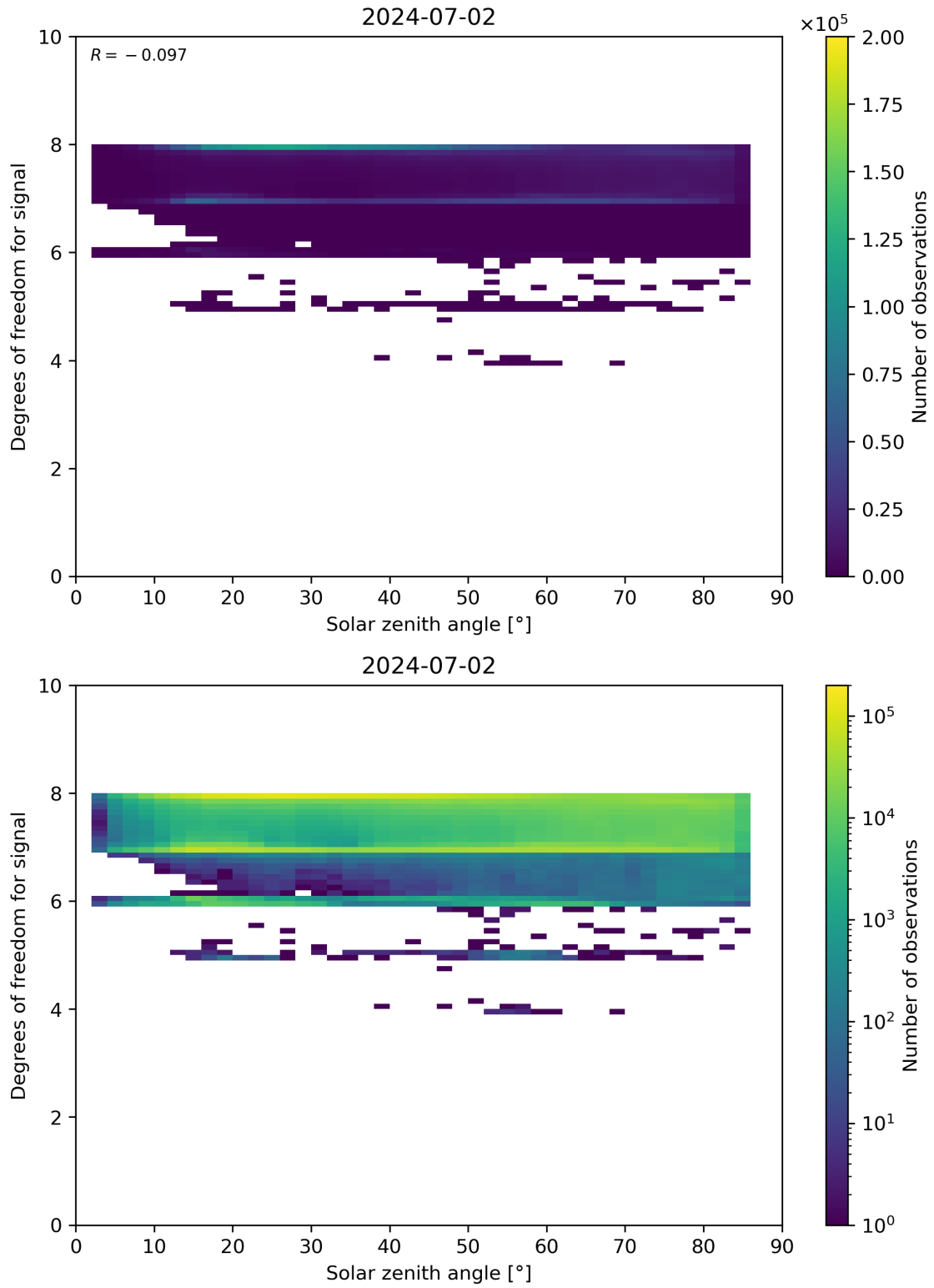
Figure 65: Scatter density plot of “Solar zenith angle” against “Degrees of freedom for signal” for 2024-07-01 to 2024-07-03.
