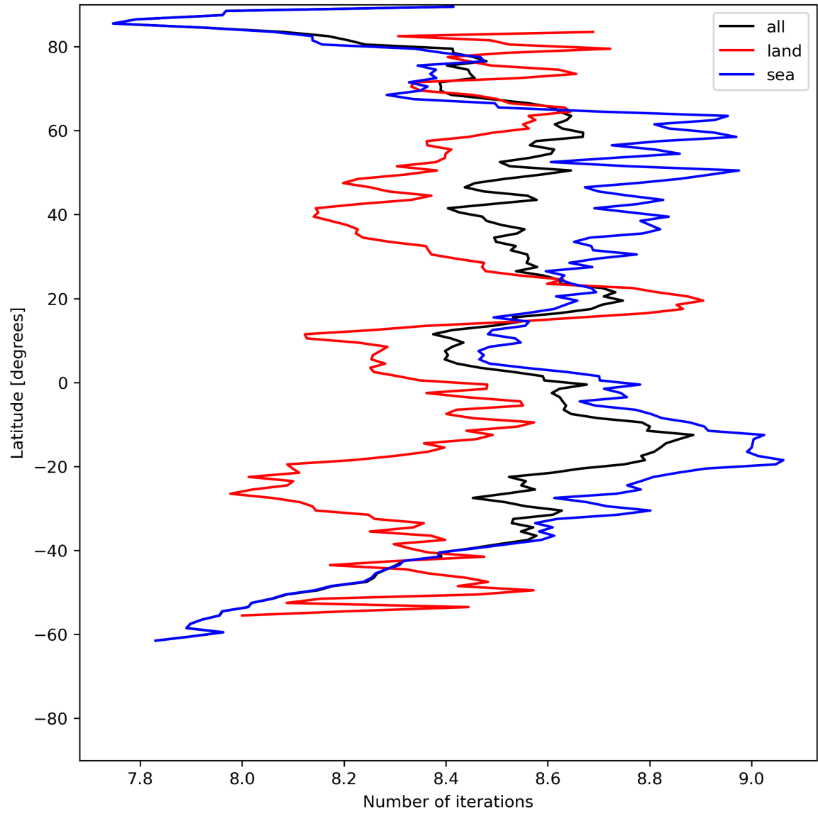
Figure 16: Zonal average of “Number of iterations” for 2024-07-01 to 2024-07-03.
