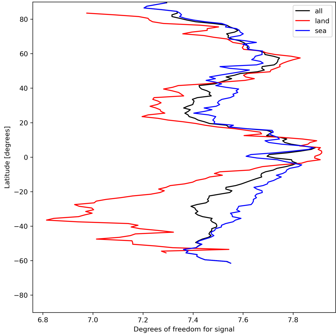
Figure 15: Zonal average of “Degrees of freedom for signal” for 2024-07-01 to 2024-07-03.
