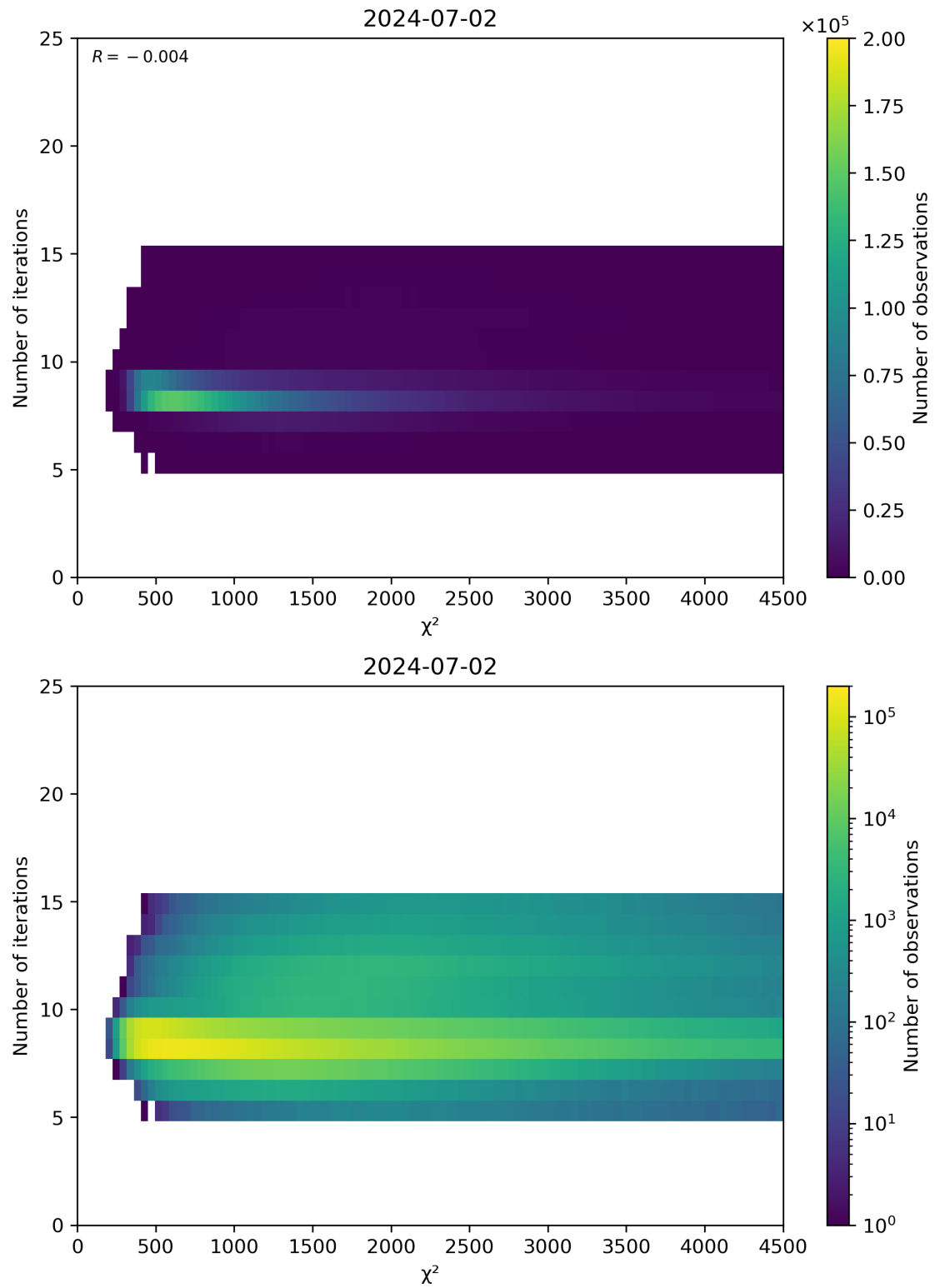
Figure 49: Scatter density plot of “ \chi^2 ” against “Number of iterations” for 2024-07-01 to 2024-07-03.
