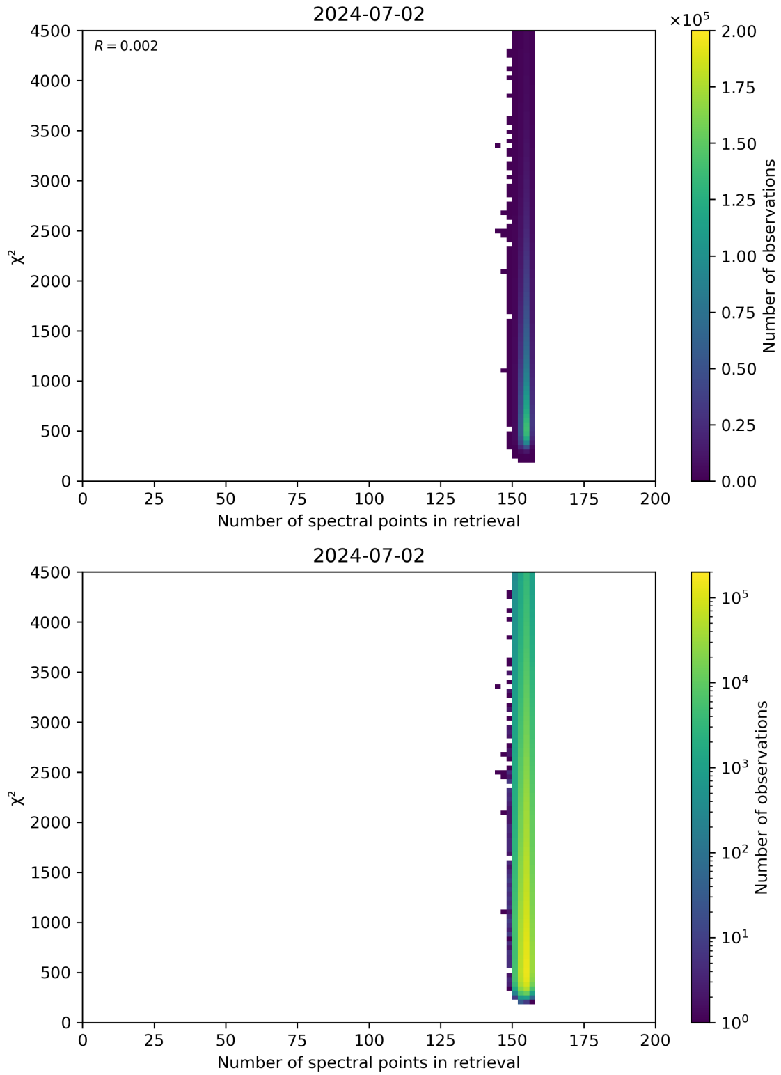
Figure 58: Scatter density plot of “Number of spectral points in retrieval” against “ \chi^2 ” for 2024-07-01 to 2024-07-03.
