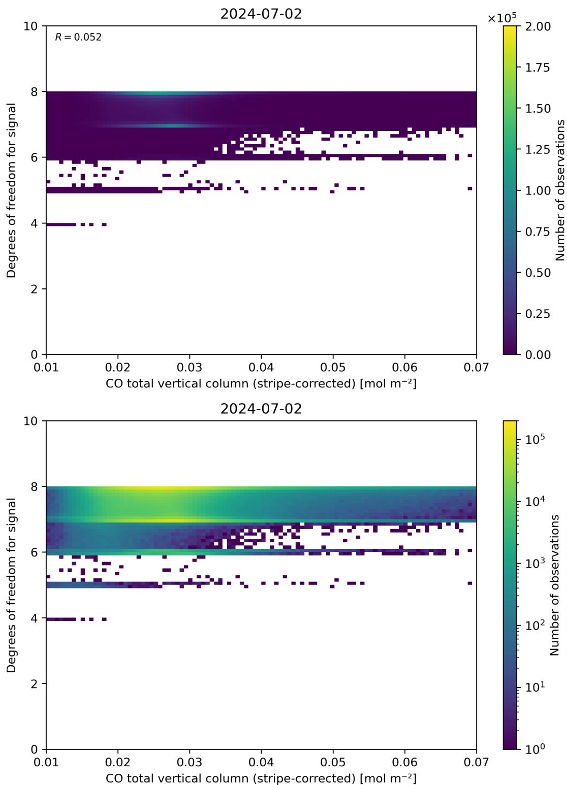
Figure 38: Scatter density plot of “CO total vertical column (stripe-corrected)” against “Degrees of freedom for signal” for 2024-07-01 to 2024-07-03.
