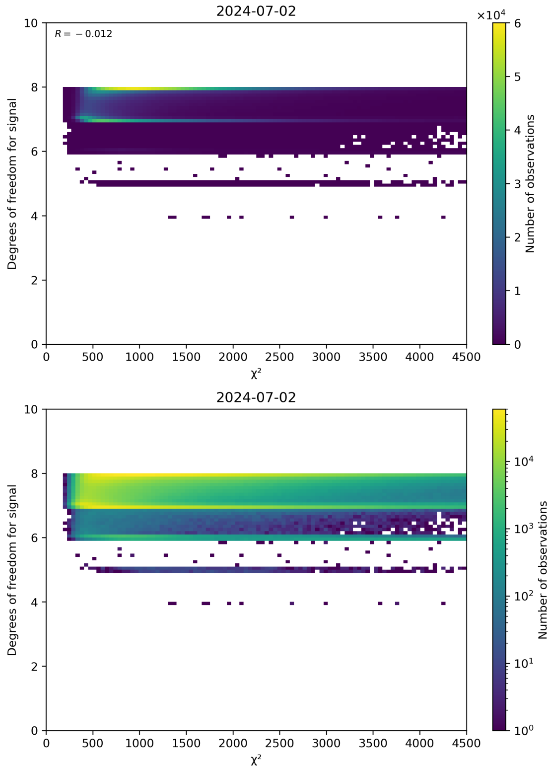
Figure 48: Scatter density plot of “ \chi^2 ” against “Degrees of freedom for signal” for 2024-07-01 to 2024-07-03.
