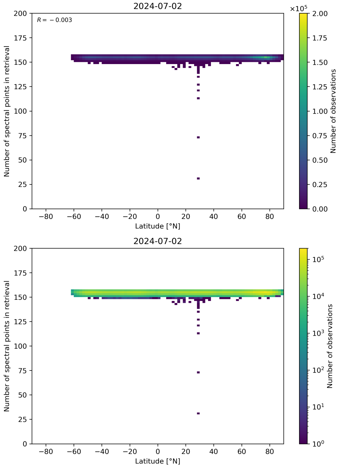
Figure 57: Scatter density plot of “Latitude” against “Number of spectral points in retrieval” for 2024-07-01 to 2024-07-03.
