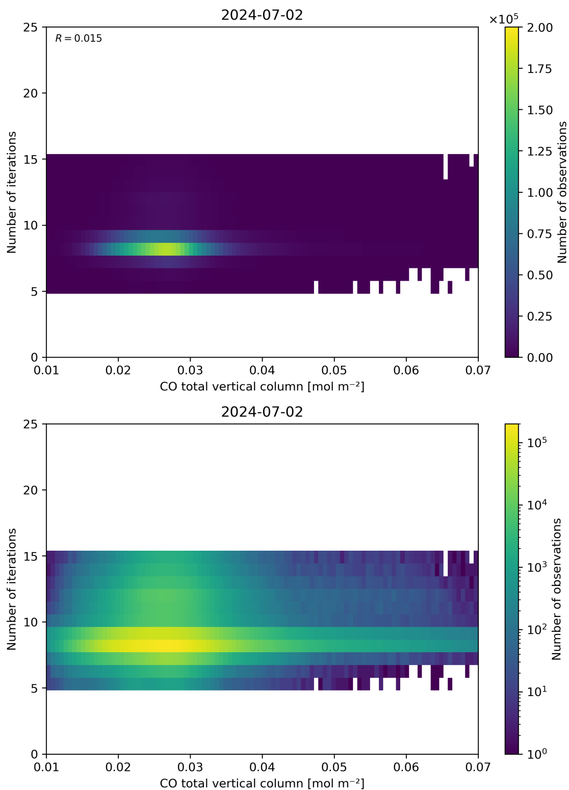
Figure 42: Scatter density plot of “CO total vertical column” against “Number of iterations” for 2024-07-01 to 2024-07-03.
