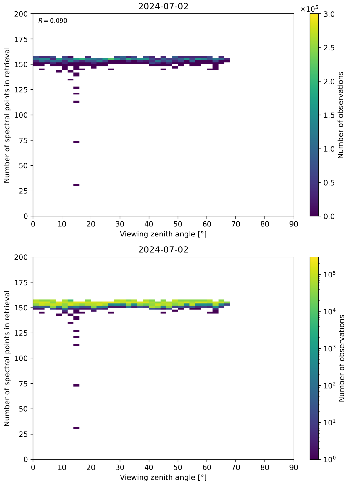
Figure 76: Scatter density plot of “Viewing zenith angle” against “Number of spectral points in retrieval” for 2024-07-01 to 2024-07-03.
