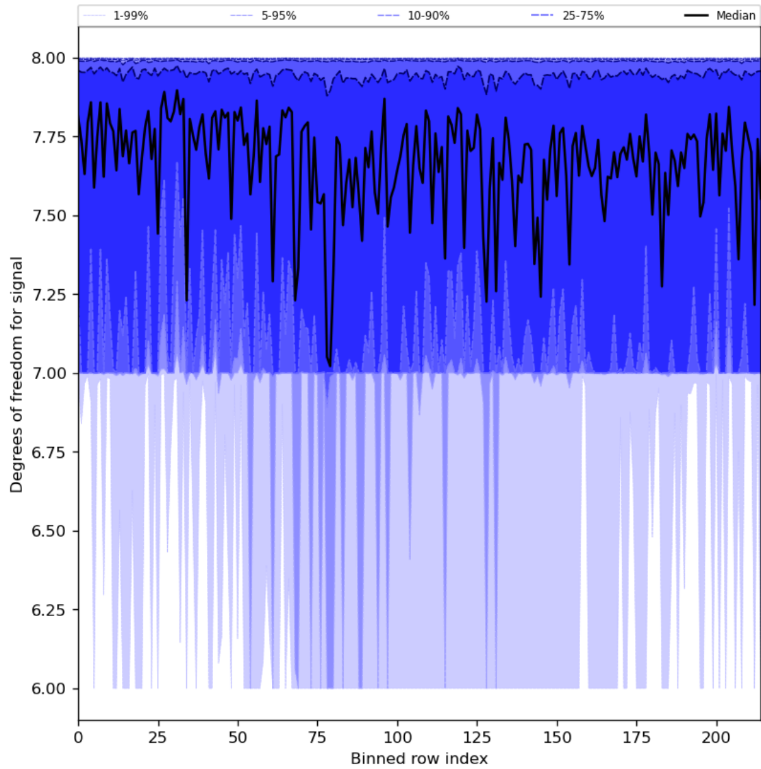
Figure 31: Along track statistics of “Degrees of freedom for signal” for 2024-07-01 to 2024-07-03
