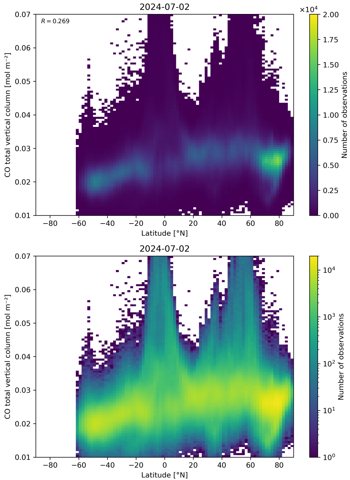
Figure 51: Scatter density plot of “Latitude” against “CO total vertical column” for 2024-07-01 to 2024-07-03.
