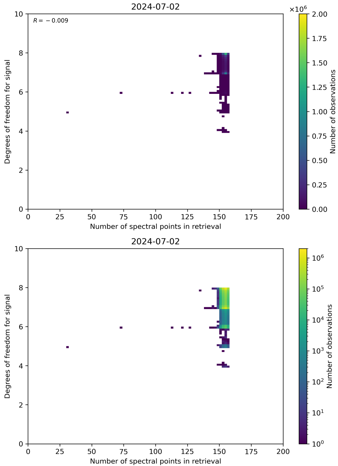
Figure 59: Scatter density plot of “Number of spectral points in retrieval” against “Degrees of freedom for signal” for 2024-07-01 to 2024-07-03.
