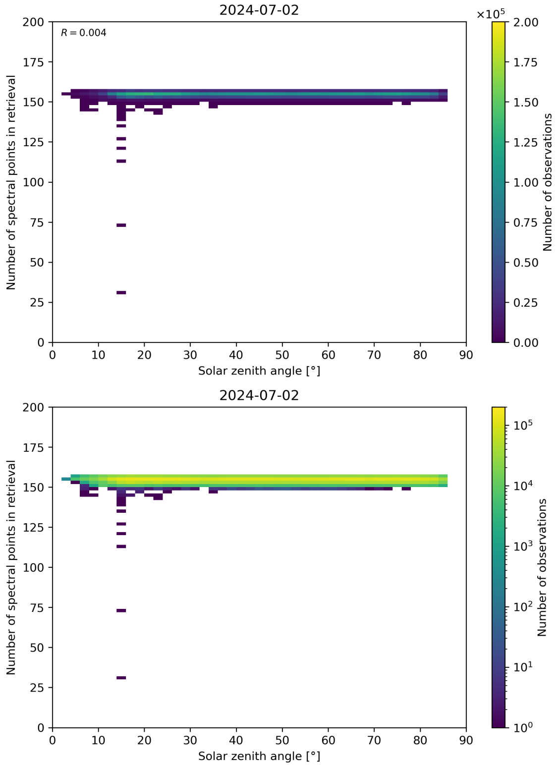
Figure 68: Scatter density plot of “Solar zenith angle” against “Number of spectral points in retrieval” for 2024-07-01 to 2024-07-03.
