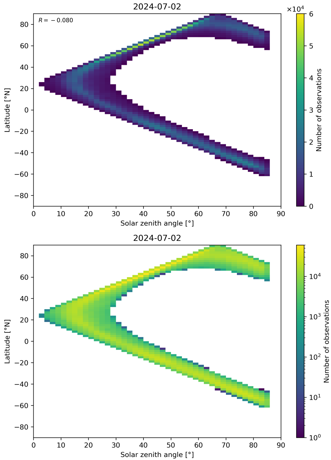
Figure 66: Scatter density plot of “Solar zenith angle” against “Latitude” for 2024-07-01 to 2024-07-03.
