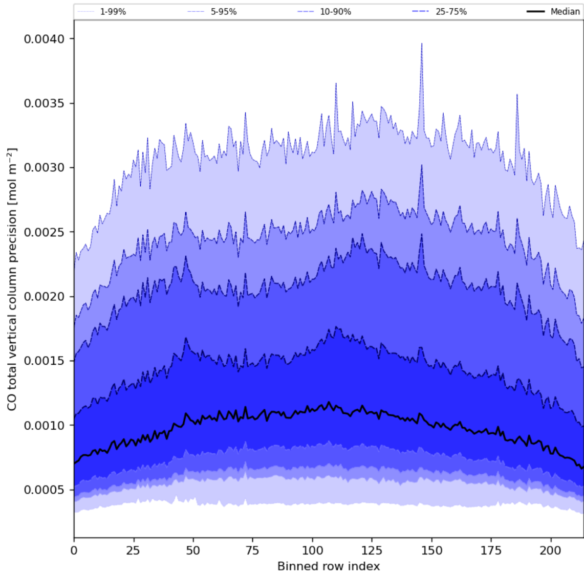
Figure 28: Along track statistics of “CO total vertical column precision” for 2024-07-01 to 2024-07-03
