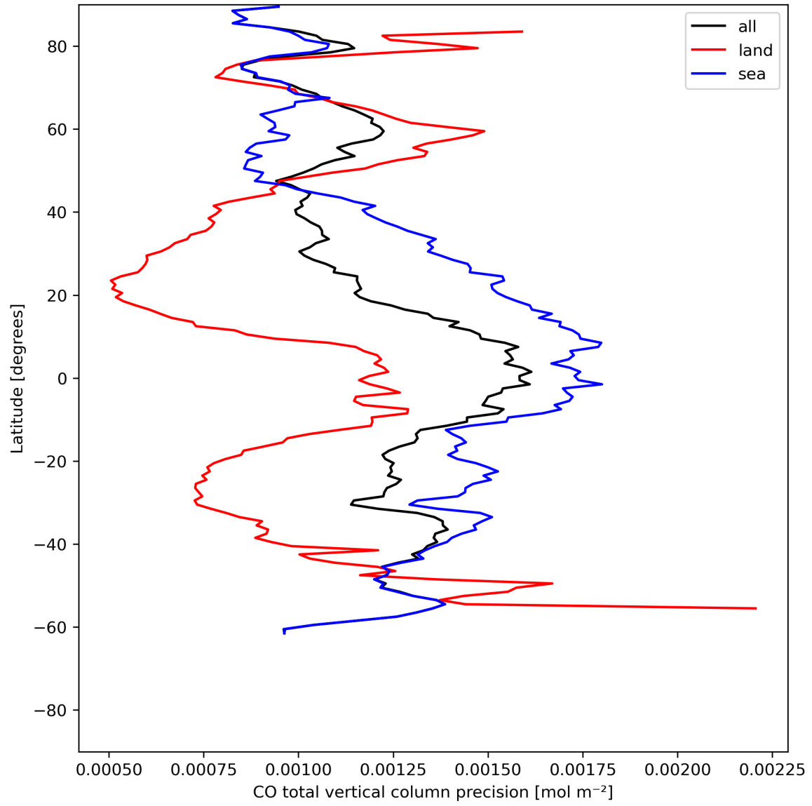
Figure 12: Zonal average of “CO total vertical column precision” for 2024-07-01 to 2024-07-03.
