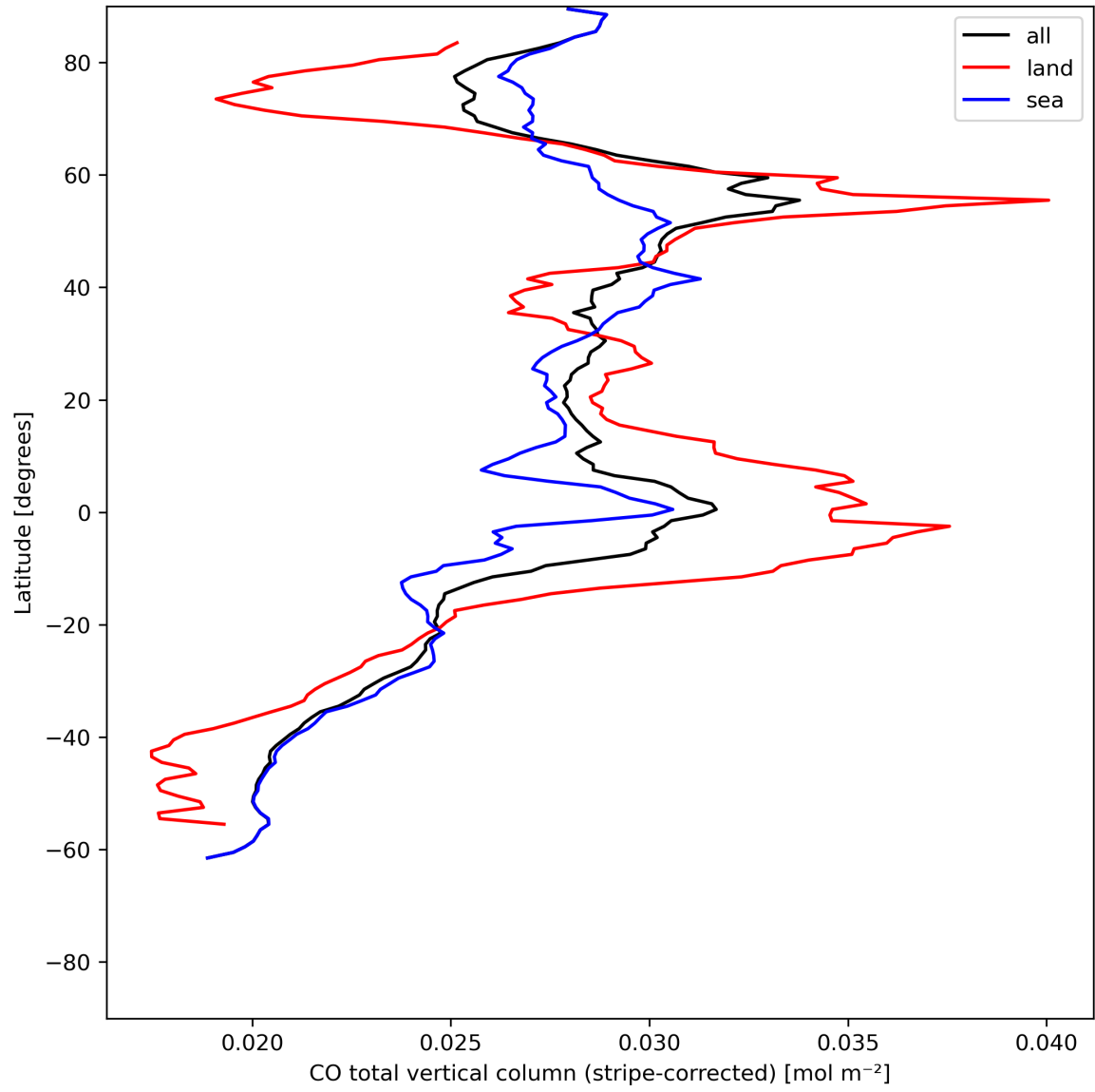
Figure 11: Zonal average of “CO total vertical column (stripe-corrected)” for 2024-07-01 to 2024-07-03.
