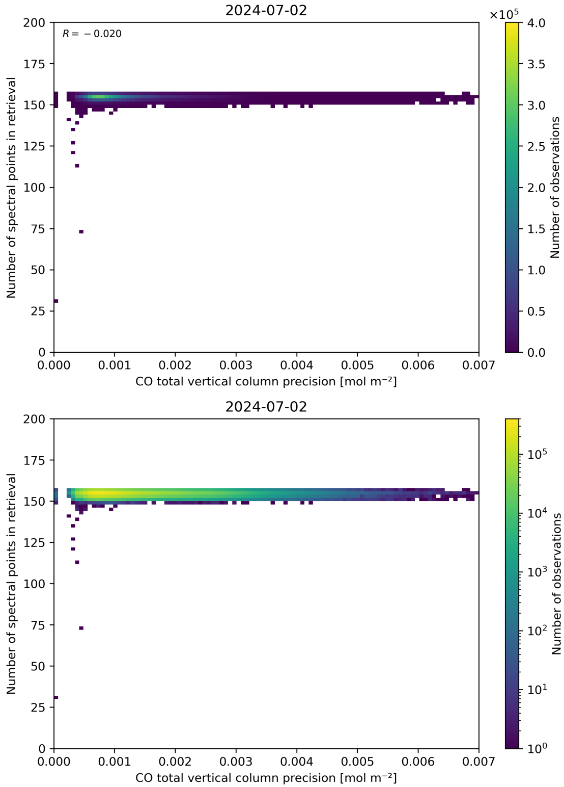
Figure 47: Scatter density plot of “CO total vertical column precision” against “Number of spectral points in retrieval” for 2024-07-01 to 2024-07-03.
