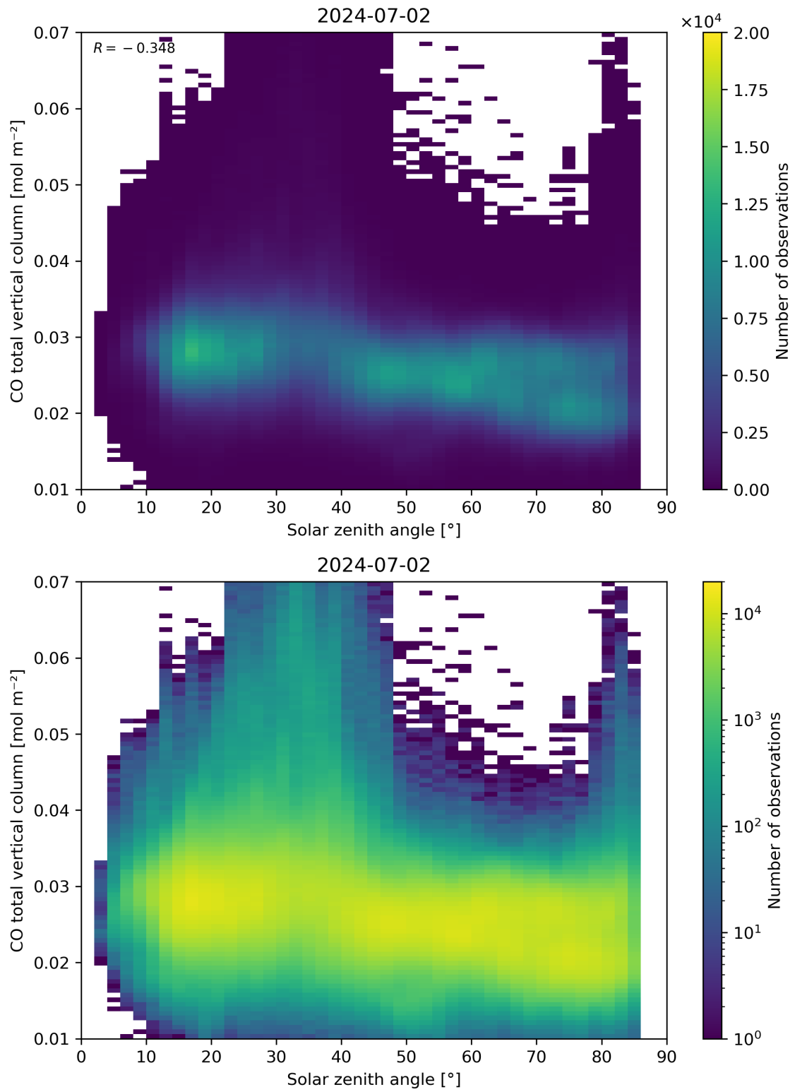
Figure 61: Scatter density plot of “Solar zenith angle” against “CO total vertical column” for 2024-07-01 to 2024-07-03.
