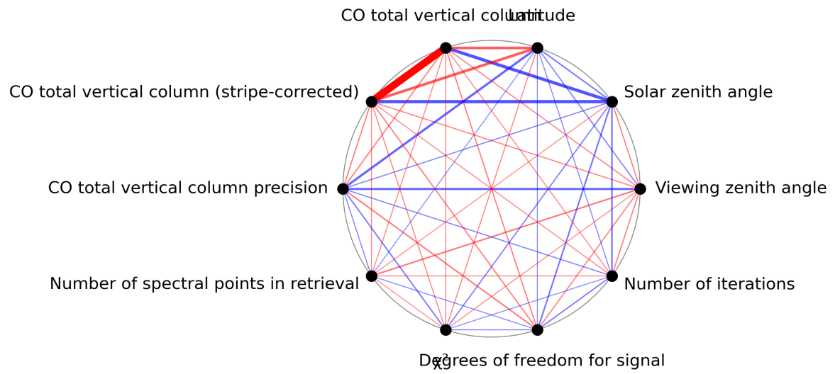
Figure 1: Map of correlation graph for 2024-07-01 to 2024-07-03.
