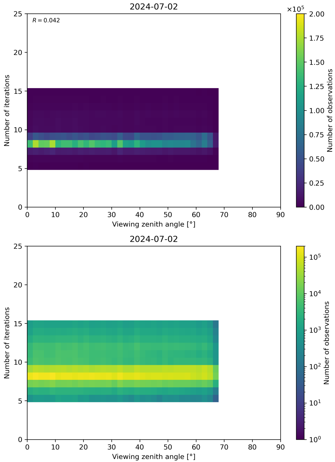
Figure 75: Scatter density plot of “Viewing zenith angle” against “Number of iterations” for 2024-07-01 to 2024-07-03.
