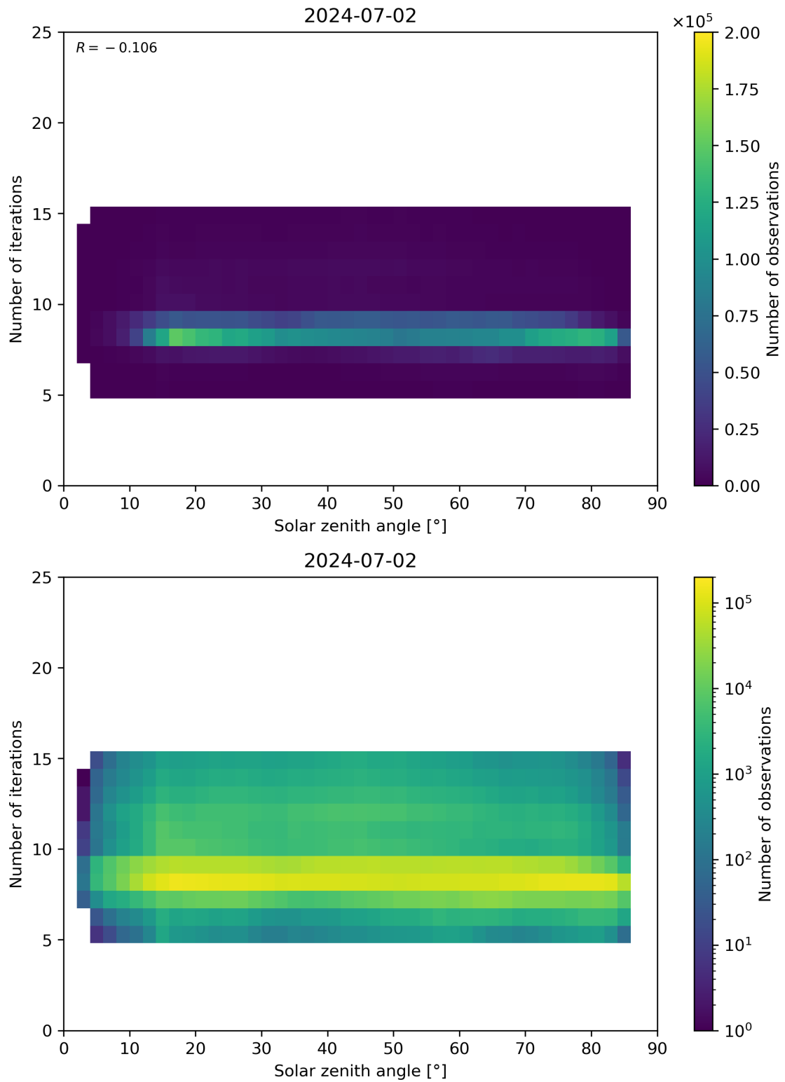
Figure 67: Scatter density plot of “Solar zenith angle” against “Number of iterations” for 2024-07-01 to 2024-07-03.
