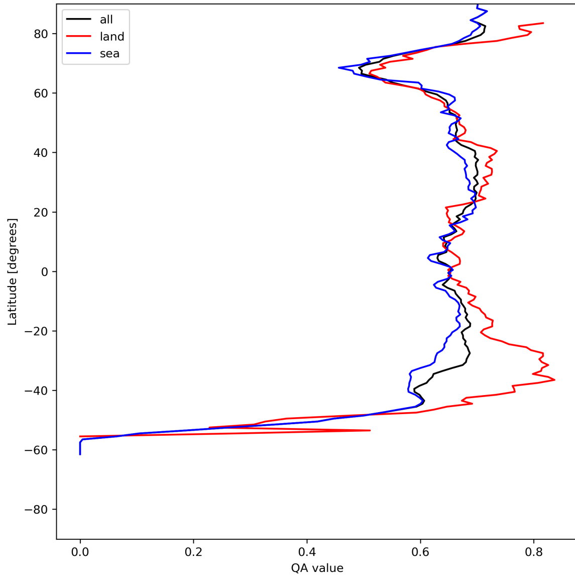
Figure 9: Zonal average of “QA value” for 2024-07-01 to 2024-07-03.
