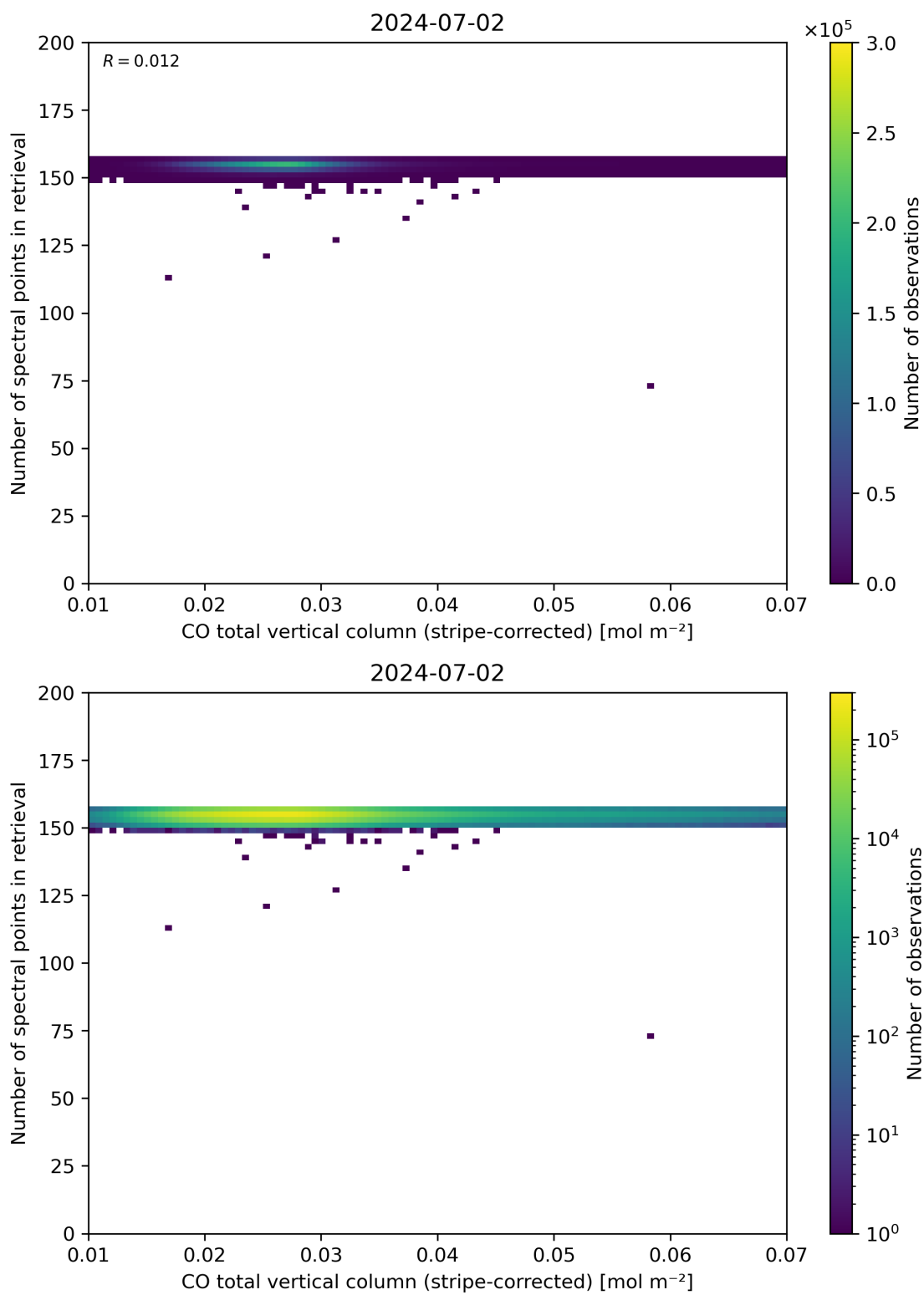
Figure 40: Scatter density plot of “CO total vertical column (stripe-corrected)” against “Number of spectral points in retrieval” for 2024-07-01 to 2024-07-03.
