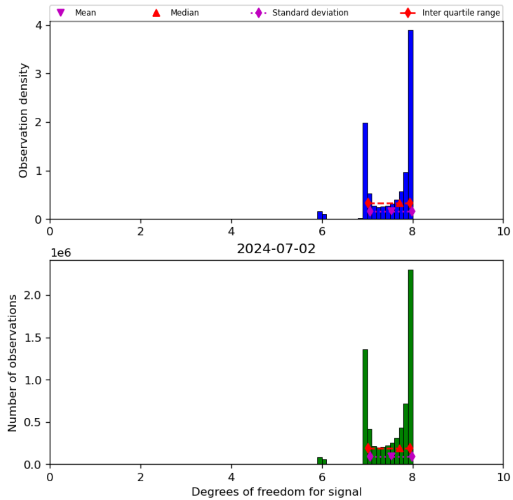
Figure 23: Histogram of “Degrees of freedom for signal” for 2024-07-01 to 2024-07-03
