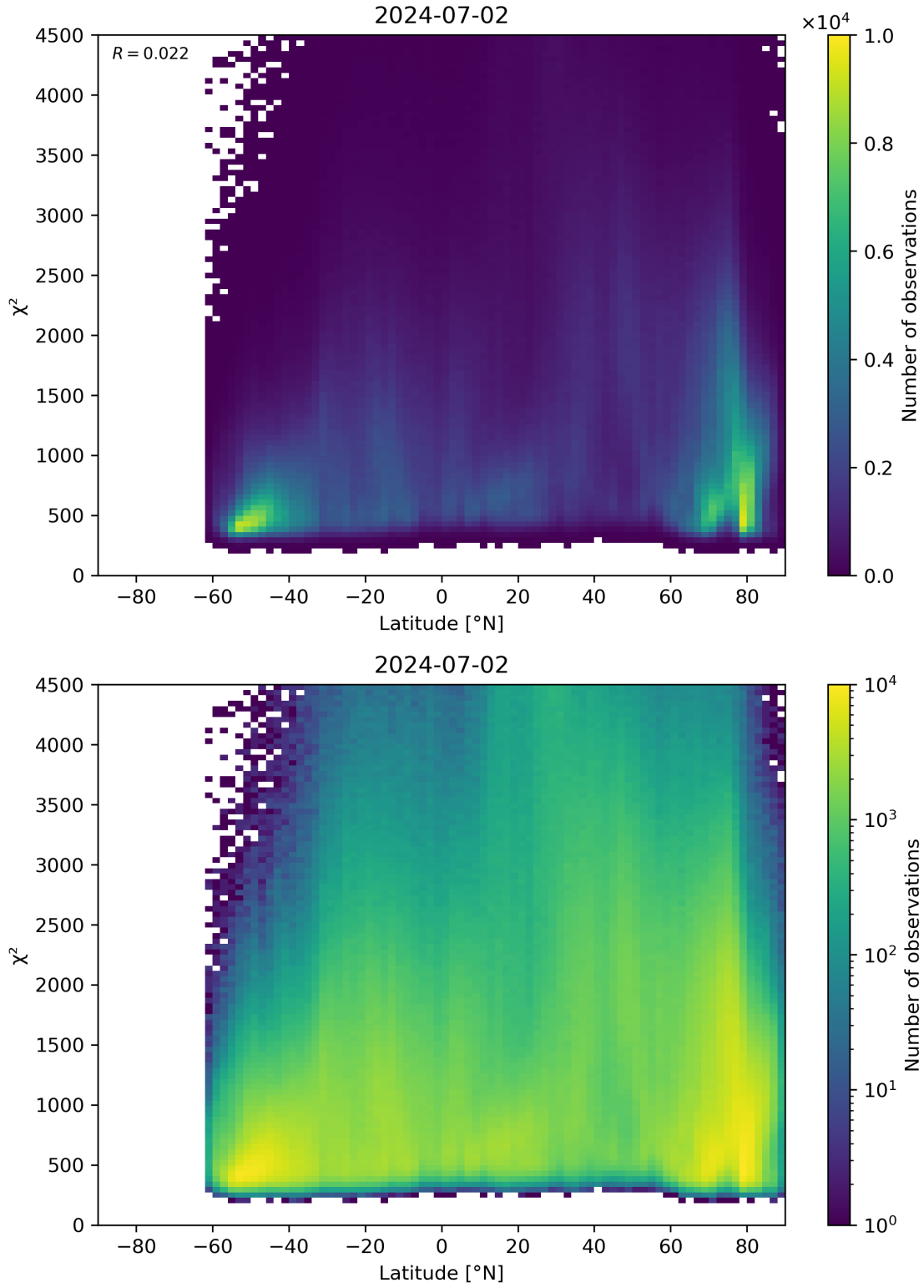
Figure 54: Scatter density plot of “Latitude” against “ \chi^2 ” for 2024-07-01 to 2024-07-03.
