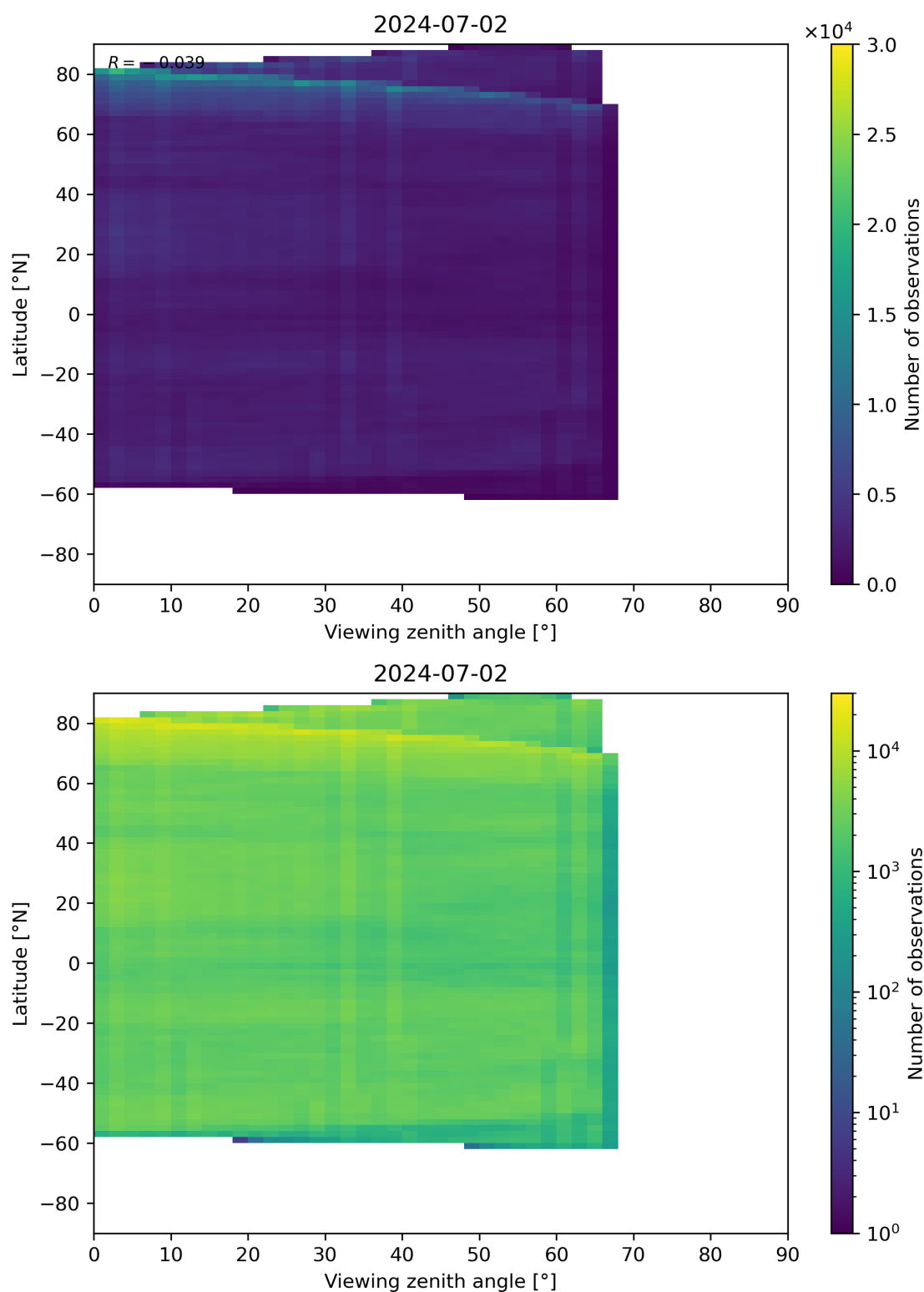
Figure 74: Scatter density plot of “Viewing zenith angle” against “Latitude” for 2024-07-01 to 2024-07-03.
