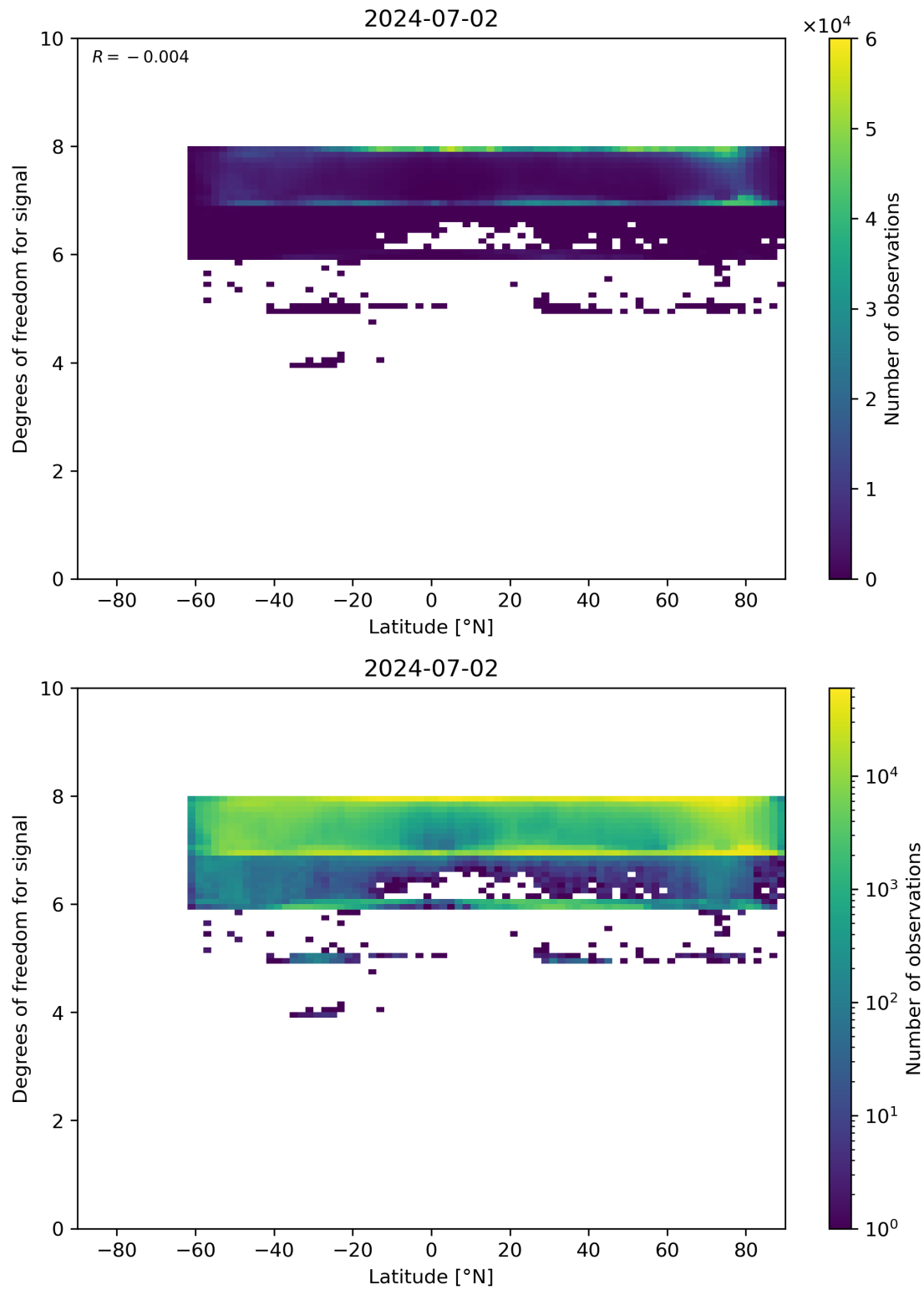
Figure 55: Scatter density plot of “Latitude” against “Degrees of freedom for signal” for 2024-07-01 to 2024-07-03.
