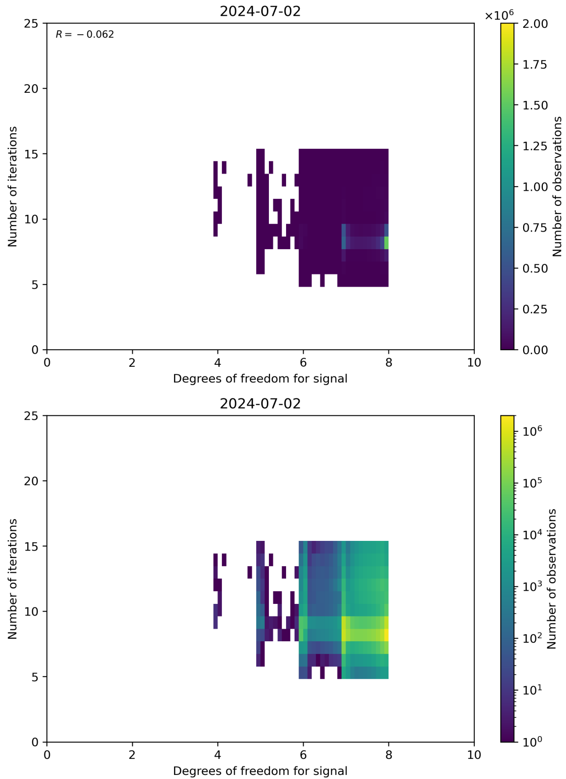
Figure 50: Scatter density plot of “Degrees of freedom for signal” against “Number of iterations” for 2024-07-01 to 2024-07-03.
