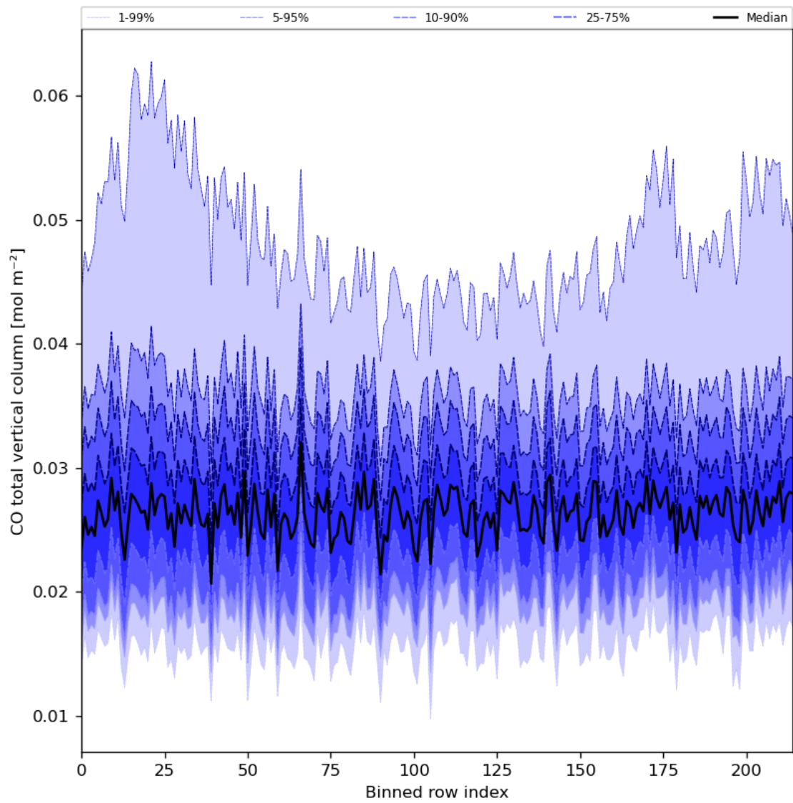
Figure 26: Along track statistics of “CO total vertical column” for 2024-07-01 to 2024-07-03
