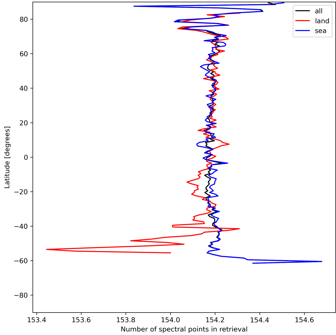
Figure 13: Zonal average of “Number of spectral points in retrieval” for 2024-07-01 to 2024-07-03.
