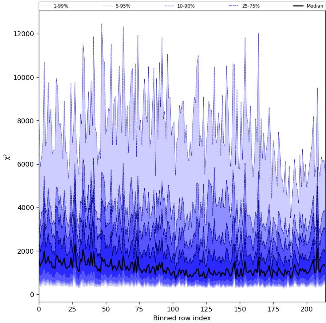
Figure 30: Along track statistics of “ \chi^2 ” for 2024-07-01 to 2024-07-03
