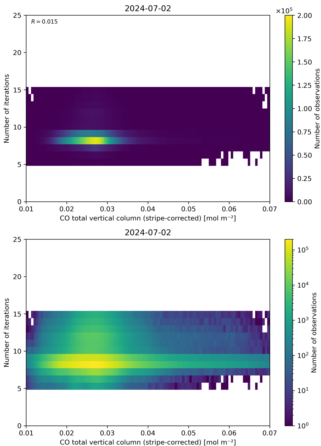
Figure 39: Scatter density plot of “CO total vertical column (stripe-corrected)” against “Number of iterations” for 2024-07-01 to 2024-07-03.
