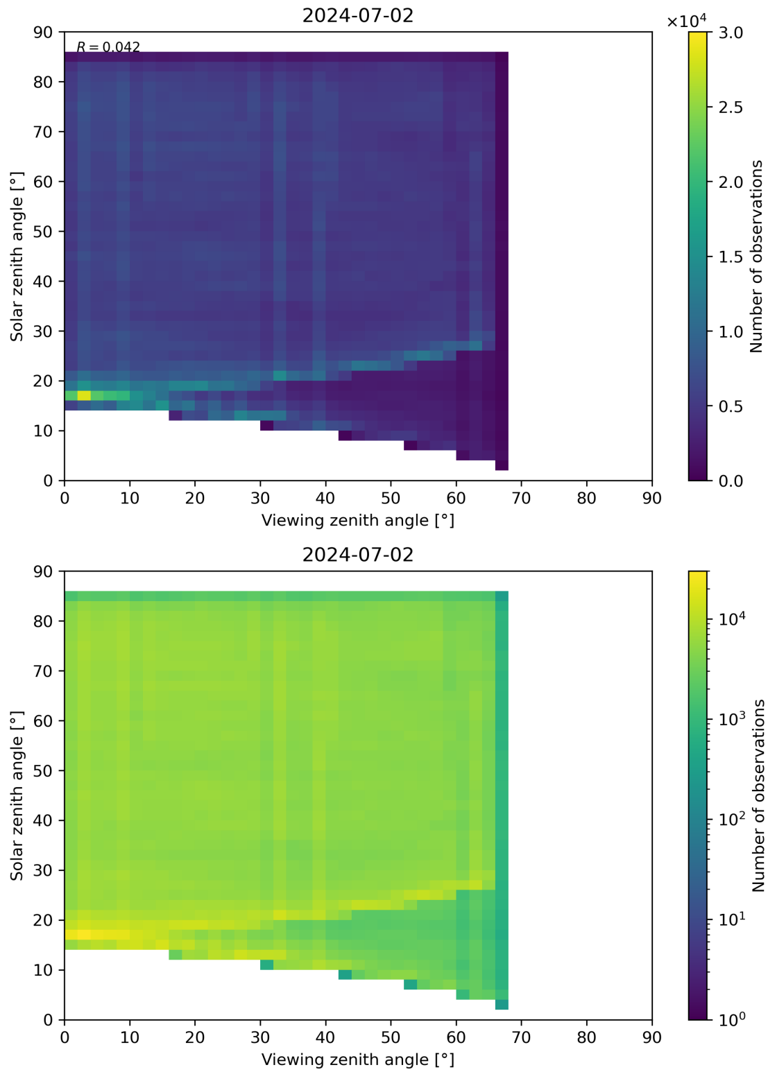
Figure 77: Scatter density plot of “Viewing zenith angle” against “Solar zenith angle” for 2024-07-01 to 2024-07-03.
