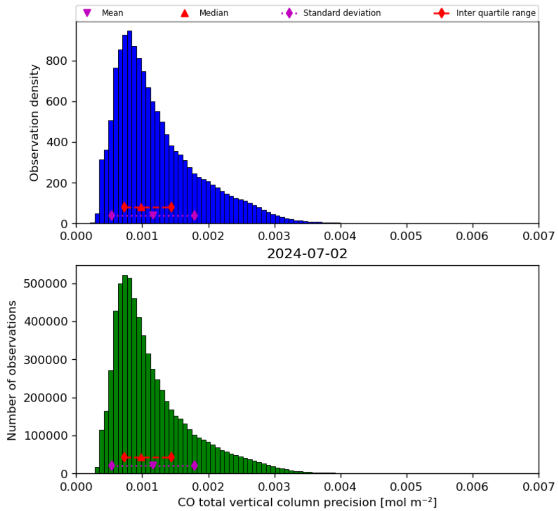
Figure 20: Histogram of “CO total vertical column precision” for 2024-07-01 to 2024-07-03
