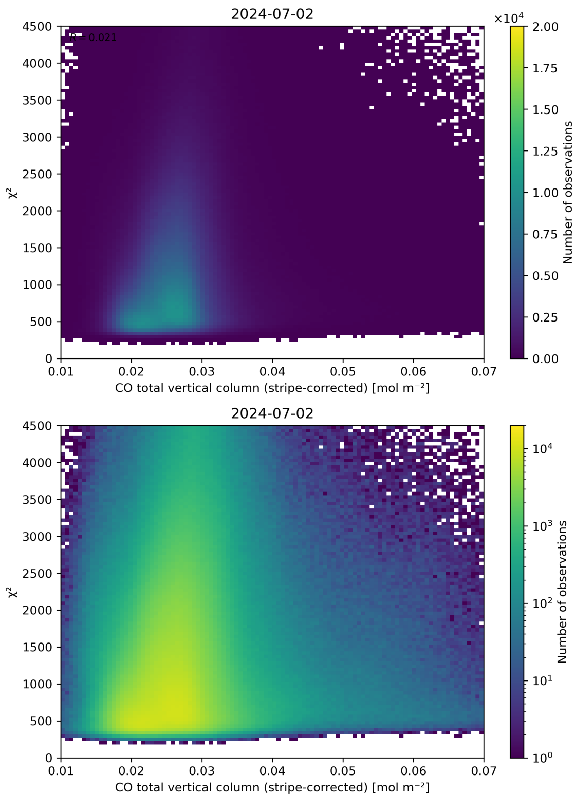
Figure 37: Scatter density plot of “CO total vertical column (stripe-corrected)” against “ \chi^2 ” for 2024-07-01 to 2024-07-03.
