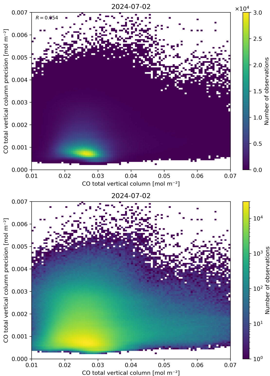
Figure 34: Scatter density plot of “CO total vertical column” against “CO total vertical column precision” for 2024-07-01 to 2024-07-03.
