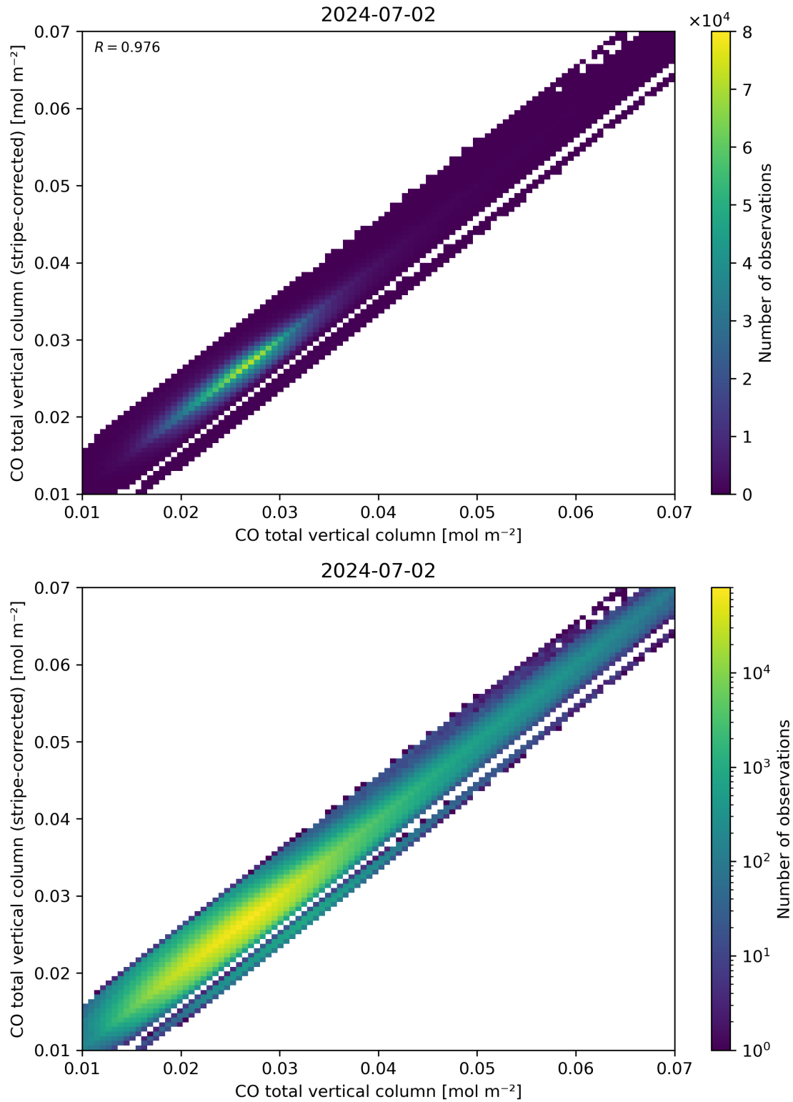
Figure 33: Scatter density plot of “CO total vertical column” against “CO total vertical column (stripe-corrected)” for 2024-07-01 to 2024-07-03.
