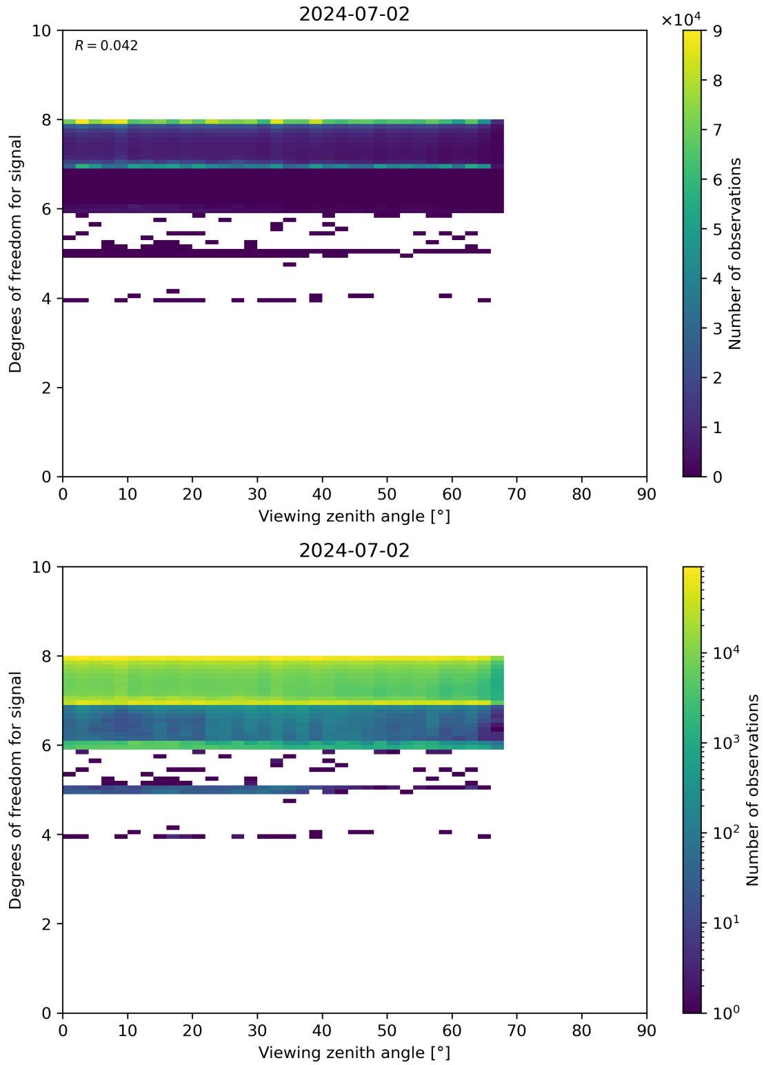
Figure 73: Scatter density plot of “Viewing zenith angle” against “Degrees of freedom for signal” for 2024-07-01 to 2024-07-03.
