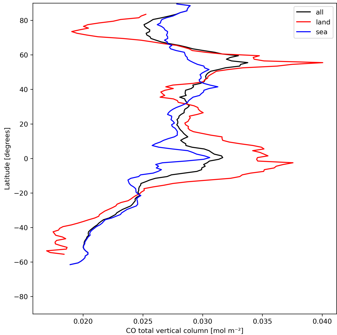
Figure 10: Zonal average of “CO total vertical column” for 2024-07-01 to 2024-07-03.
