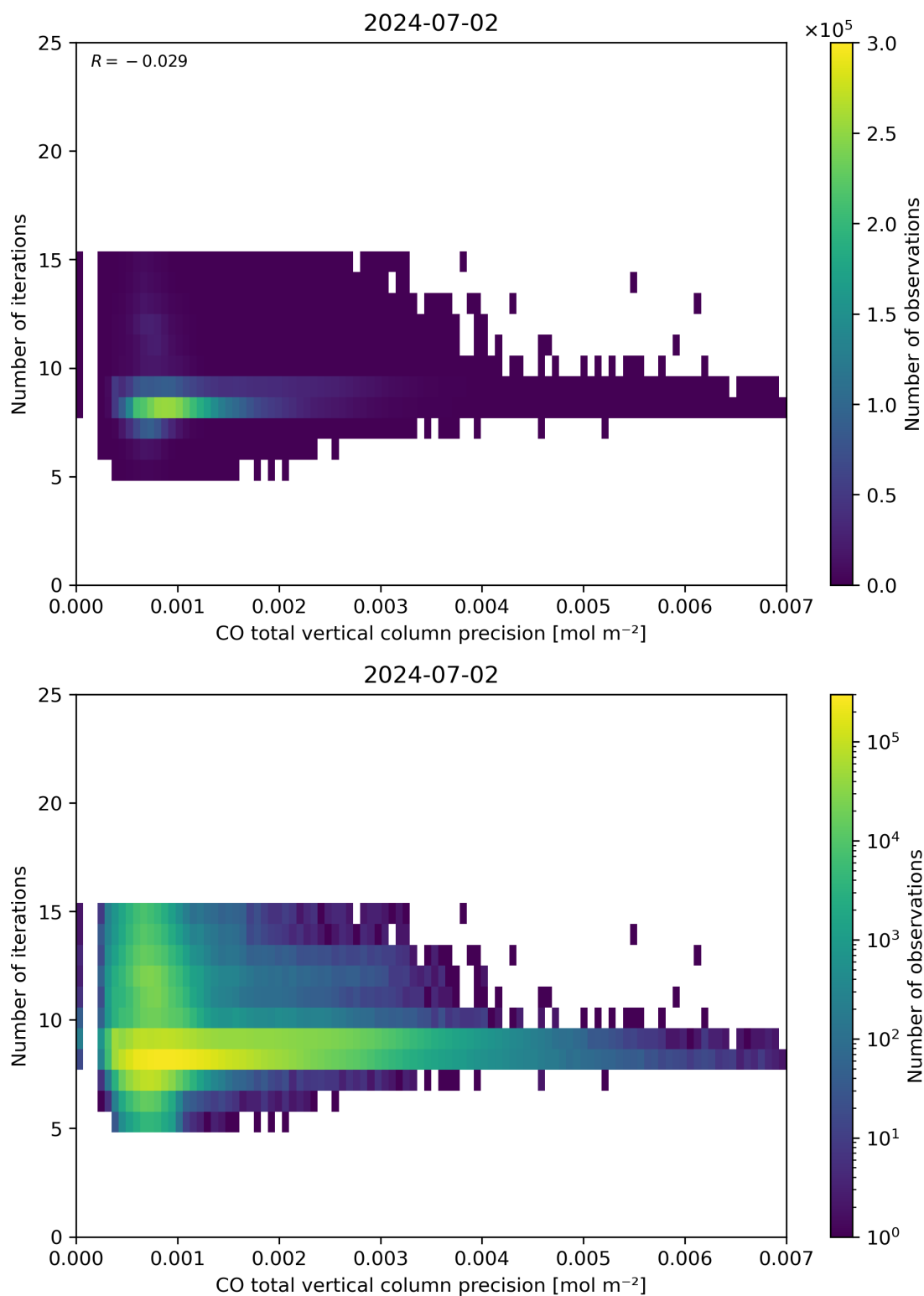
Figure 46: Scatter density plot of “CO total vertical column precision” against “Number of iterations” for 2024-07-01 to 2024-07-03.
