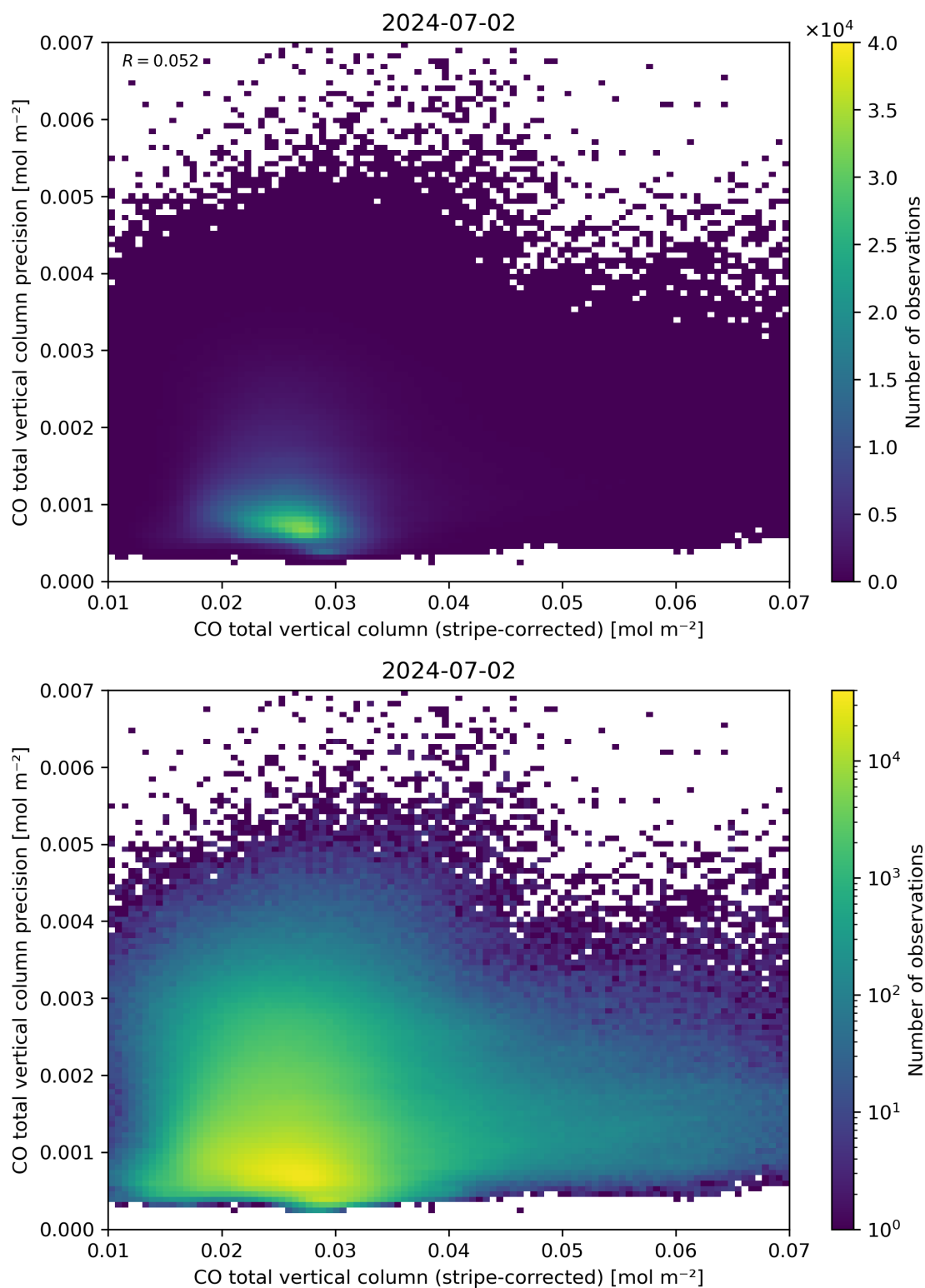
Figure 36: Scatter density plot of “CO total vertical column (stripe-corrected)” against “CO total vertical column precision” for 2024-07-01 to 2024-07-03.
