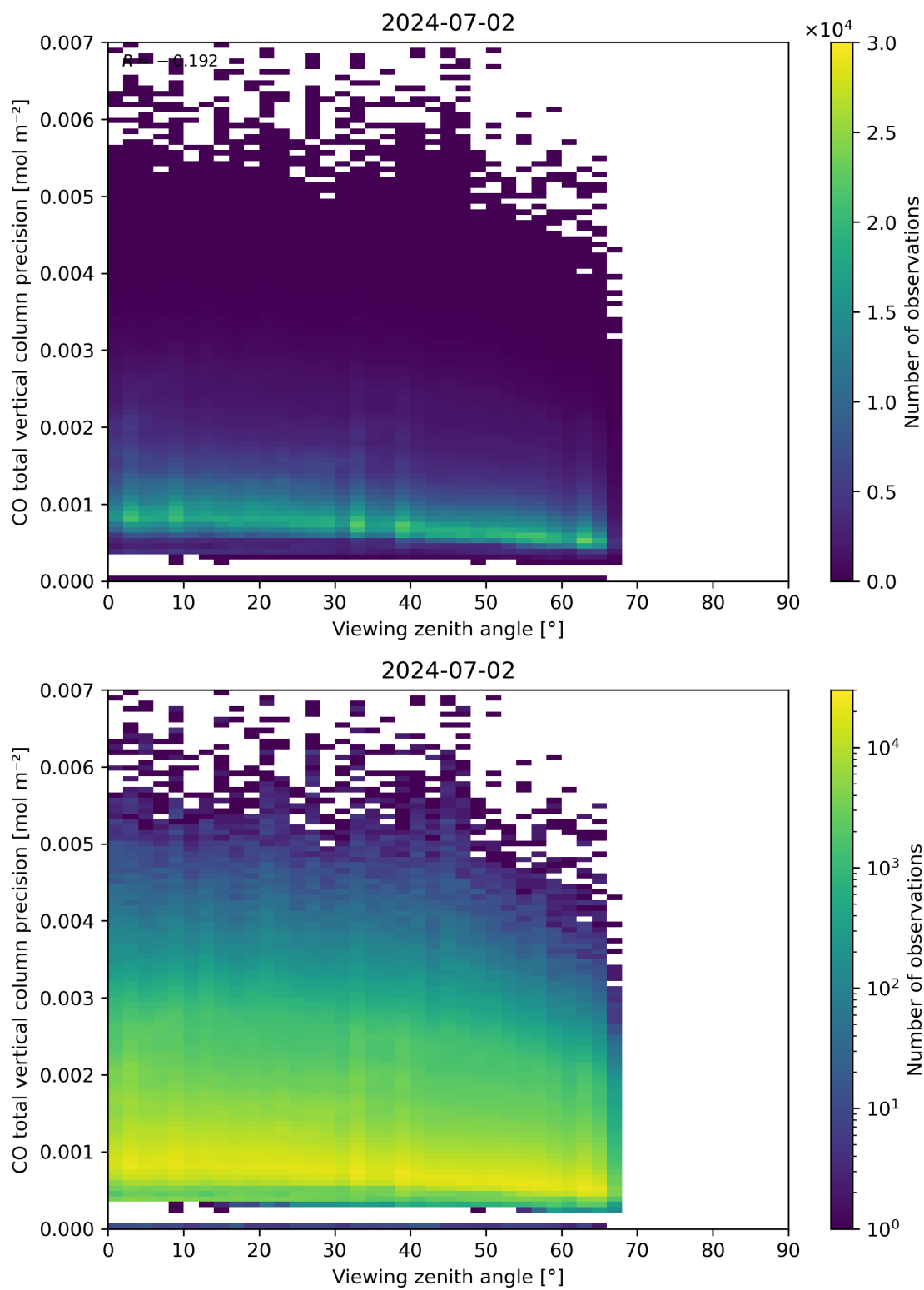
Figure 71: Scatter density plot of “Viewing zenith angle” against “CO total vertical column precision” for 2024-07-01 to 2024-07-03.
