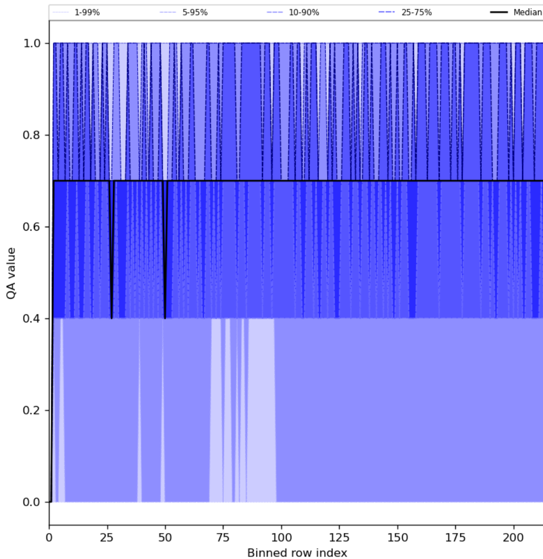
Figure 25: Along track statistics of “QA value” for 2024-07-01 to 2024-07-03
