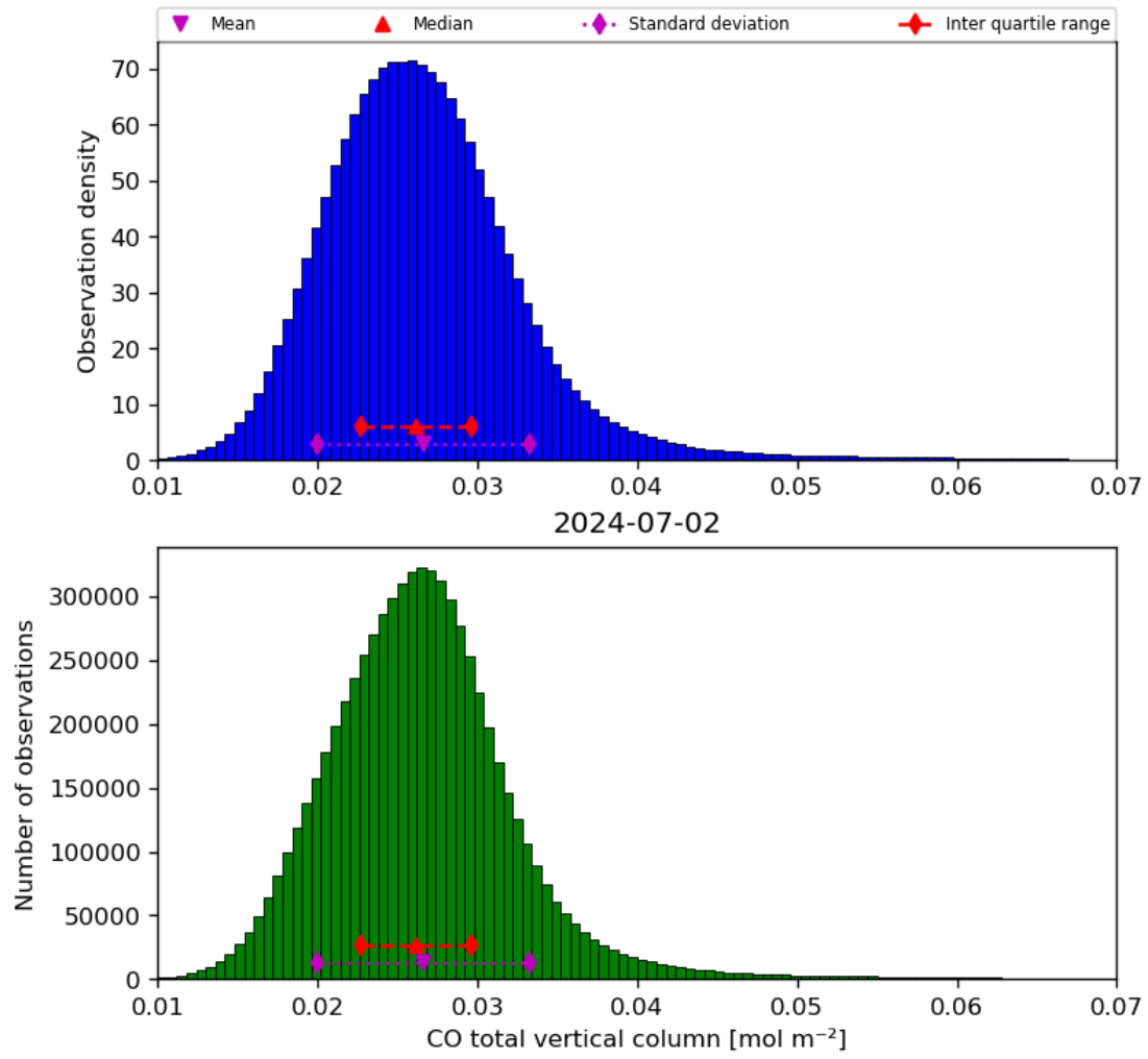
Figure 18: Histogram of “CO total vertical column” for 2024-07-01 to 2024-07-03
