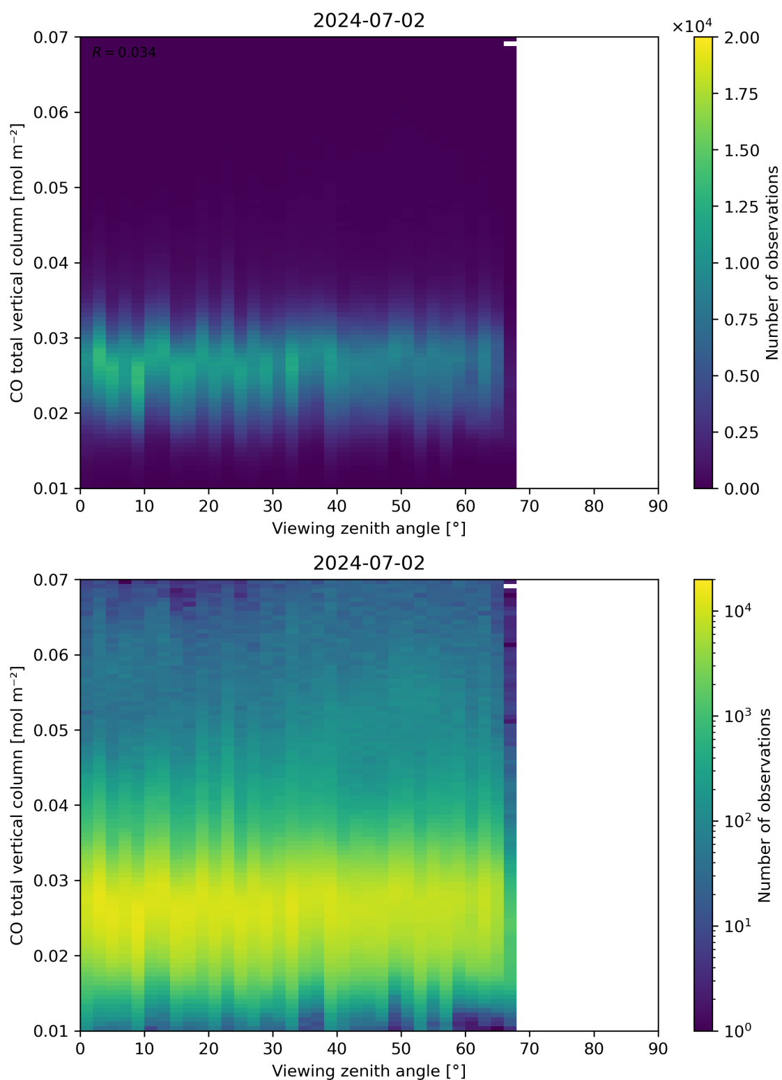
Figure 69: Scatter density plot of “Viewing zenith angle” against “CO total vertical column” for 2024-07-01 to 2024-07-03.
