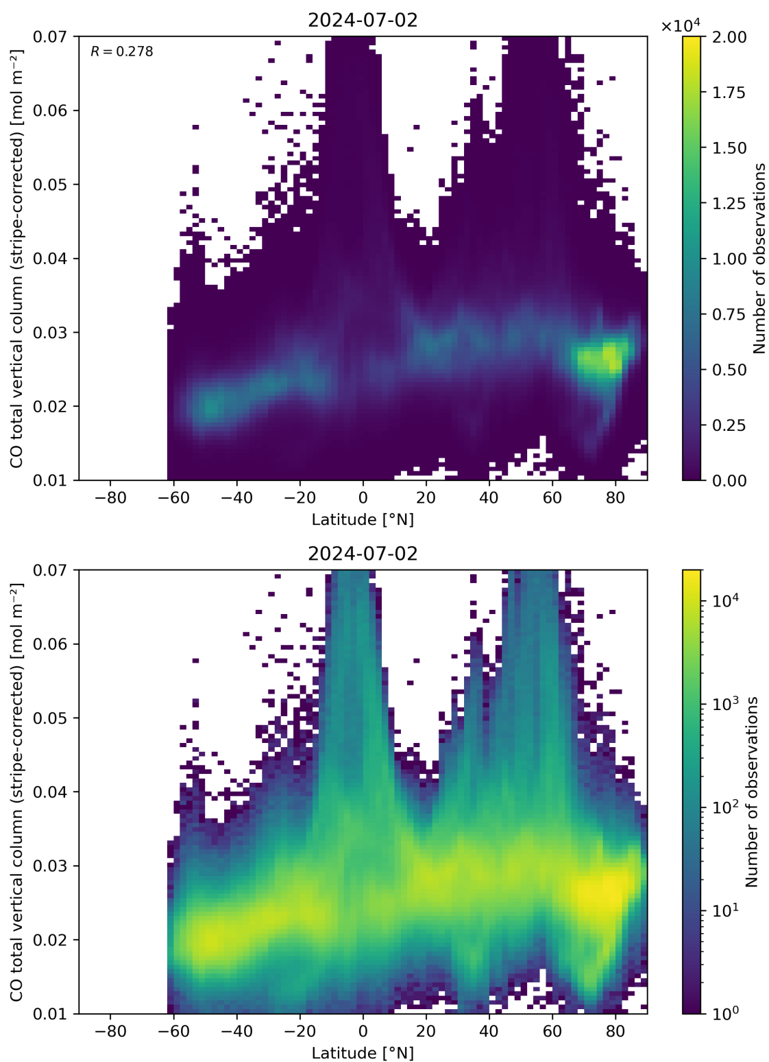
Figure 52: Scatter density plot of “Latitude” against “CO total vertical column (stripe-corrected)” for 2024-07-01 to 2024-07-03.
