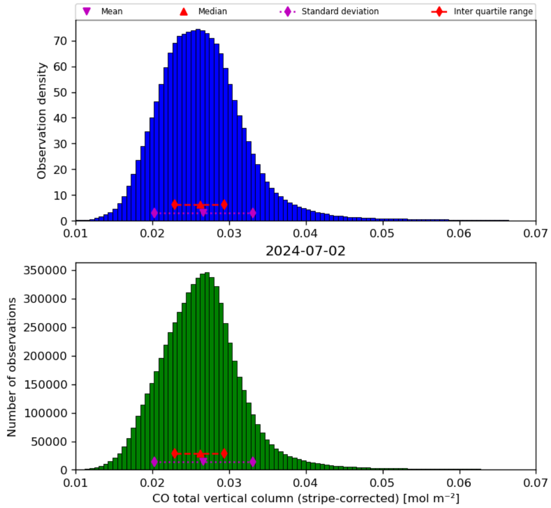
Figure 19: Histogram of “CO total vertical column (stripe-corrected)” for 2024-07-01 to 2024-07-03
