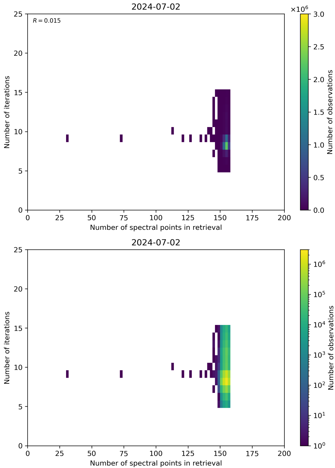
Figure 60: Scatter density plot of “Number of spectral points in retrieval” against “Number of iterations” for 2024-07-01 to 2024-07-03.
