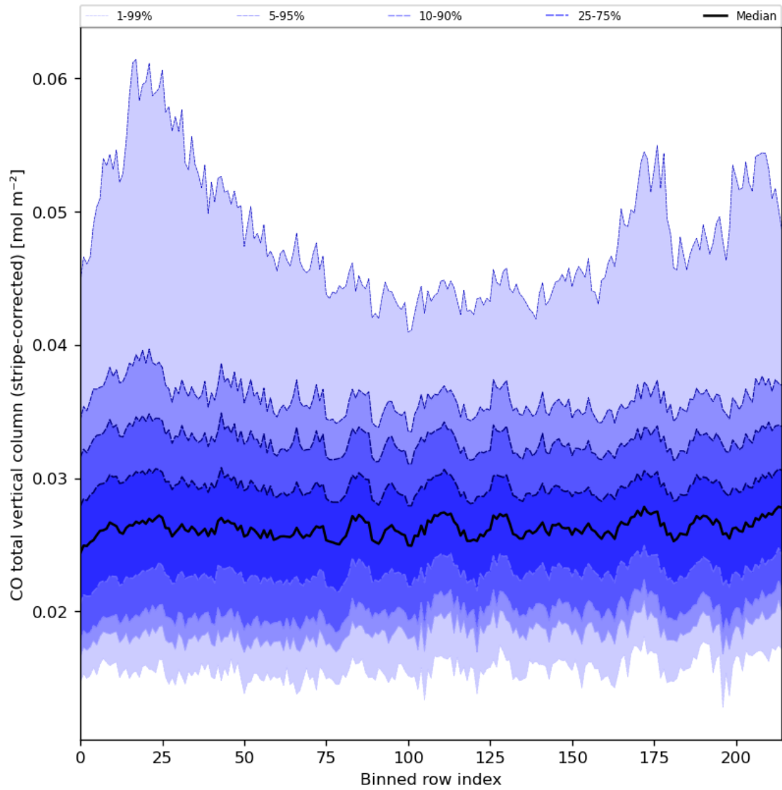
Figure 27: Along track statistics of “CO total vertical column (stripe-corrected)” for 2024-07-01 to 2024-07-03
