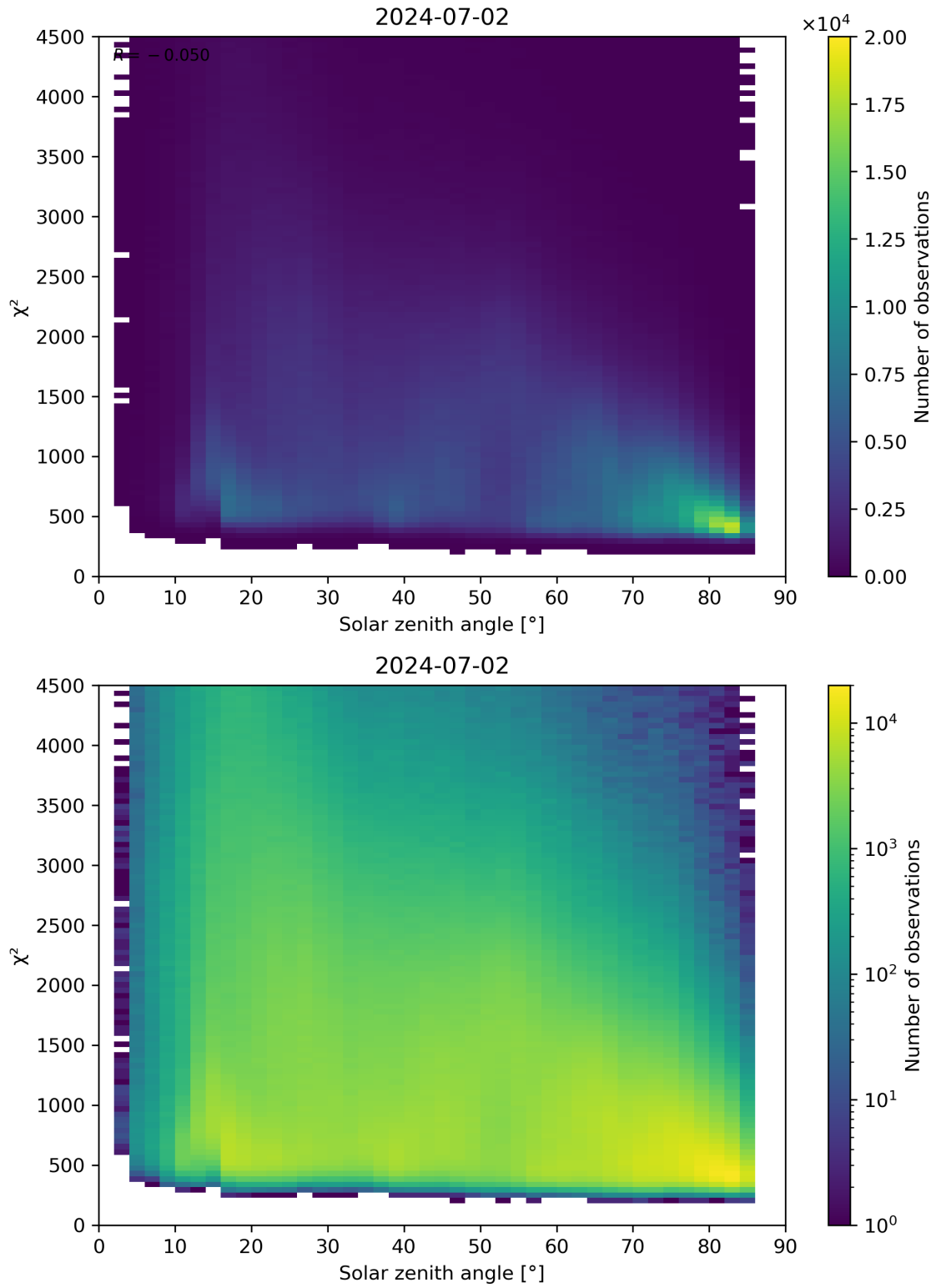
Figure 64: Scatter density plot of “Solar zenith angle” against “ \chi^2 ” for 2024-07-01 to 2024-07-03.
