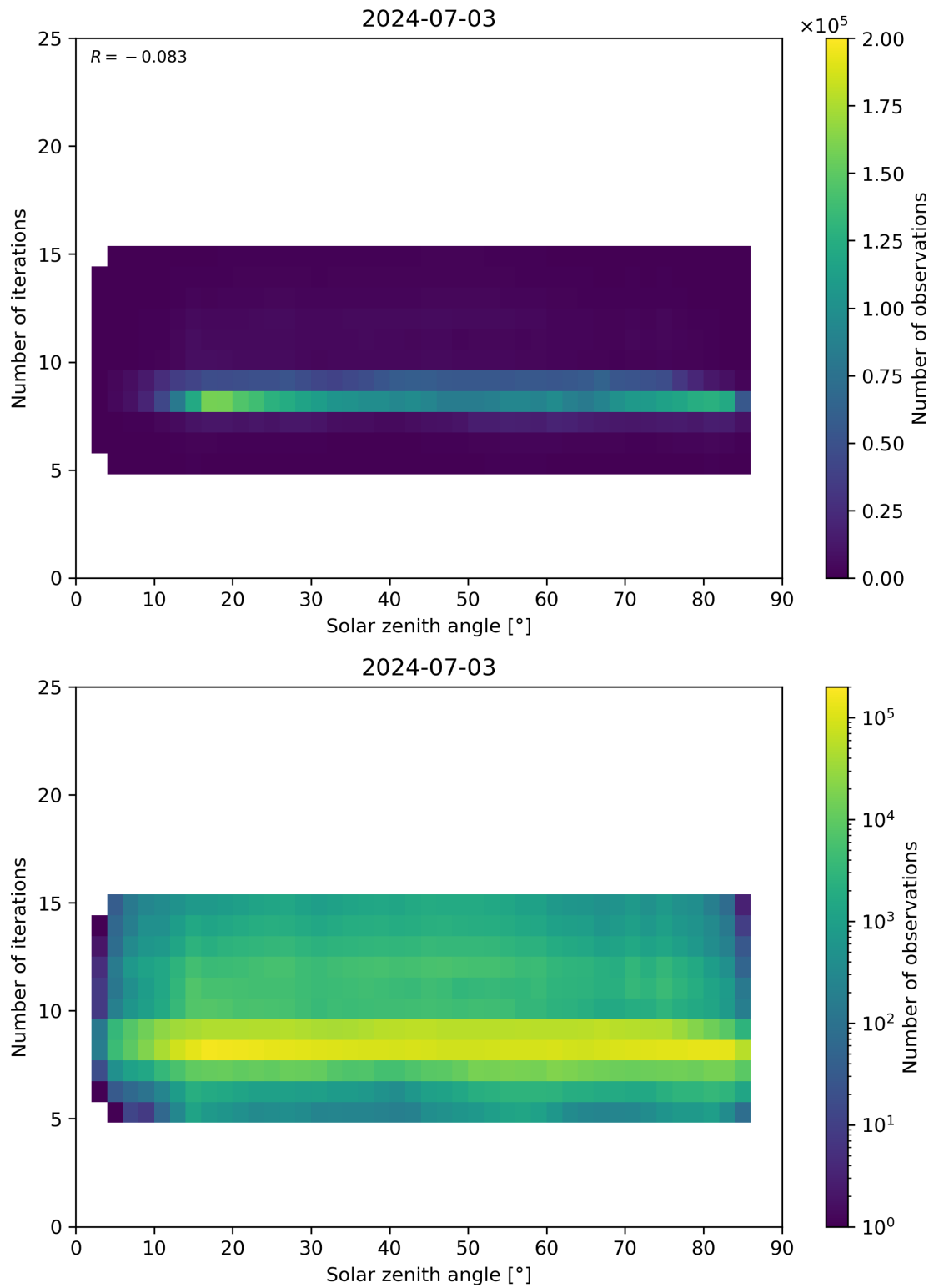
Figure 67: Scatter density plot of “Solar zenith angle” against “Number of iterations” for 2024-07-02 to 2024-07-04.
