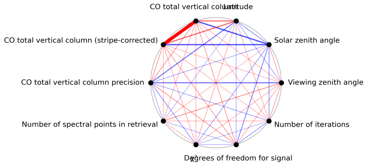
Figure 1: Map of correlation graph for 2024-07-02 to 2024-07-04.
