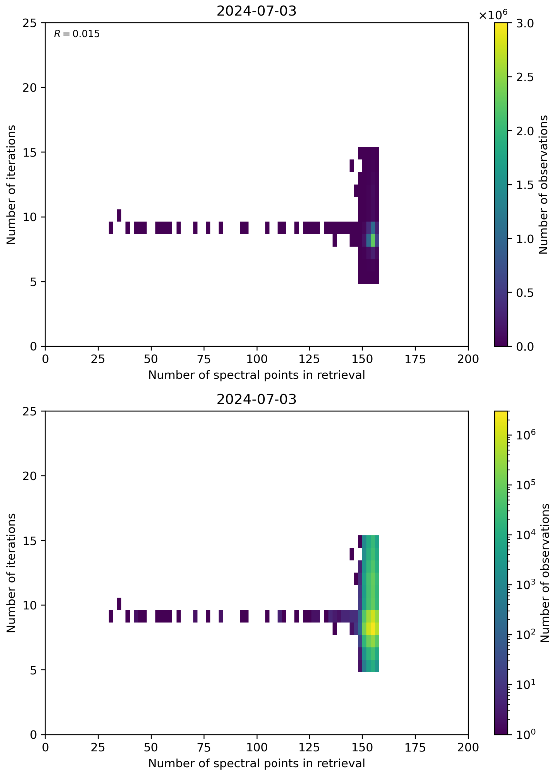
Figure 60: Scatter density plot of “Number of spectral points in retrieval” against “Number of iterations” for 2024-07-02 to 2024-07-04.
