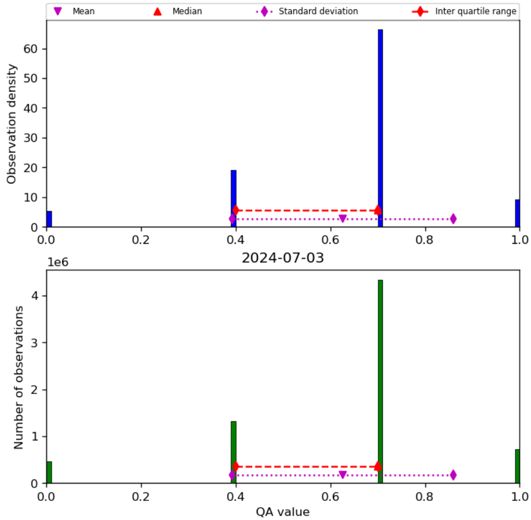
Figure 17: Histogram of “QA value” for 2024-07-02 to 2024-07-04
