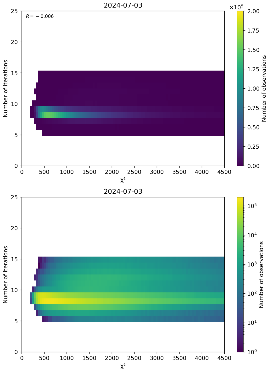
Figure 49: Scatter density plot of “ \chi^2 ” against “Number of iterations” for 2024-07-02 to 2024-07-04.
