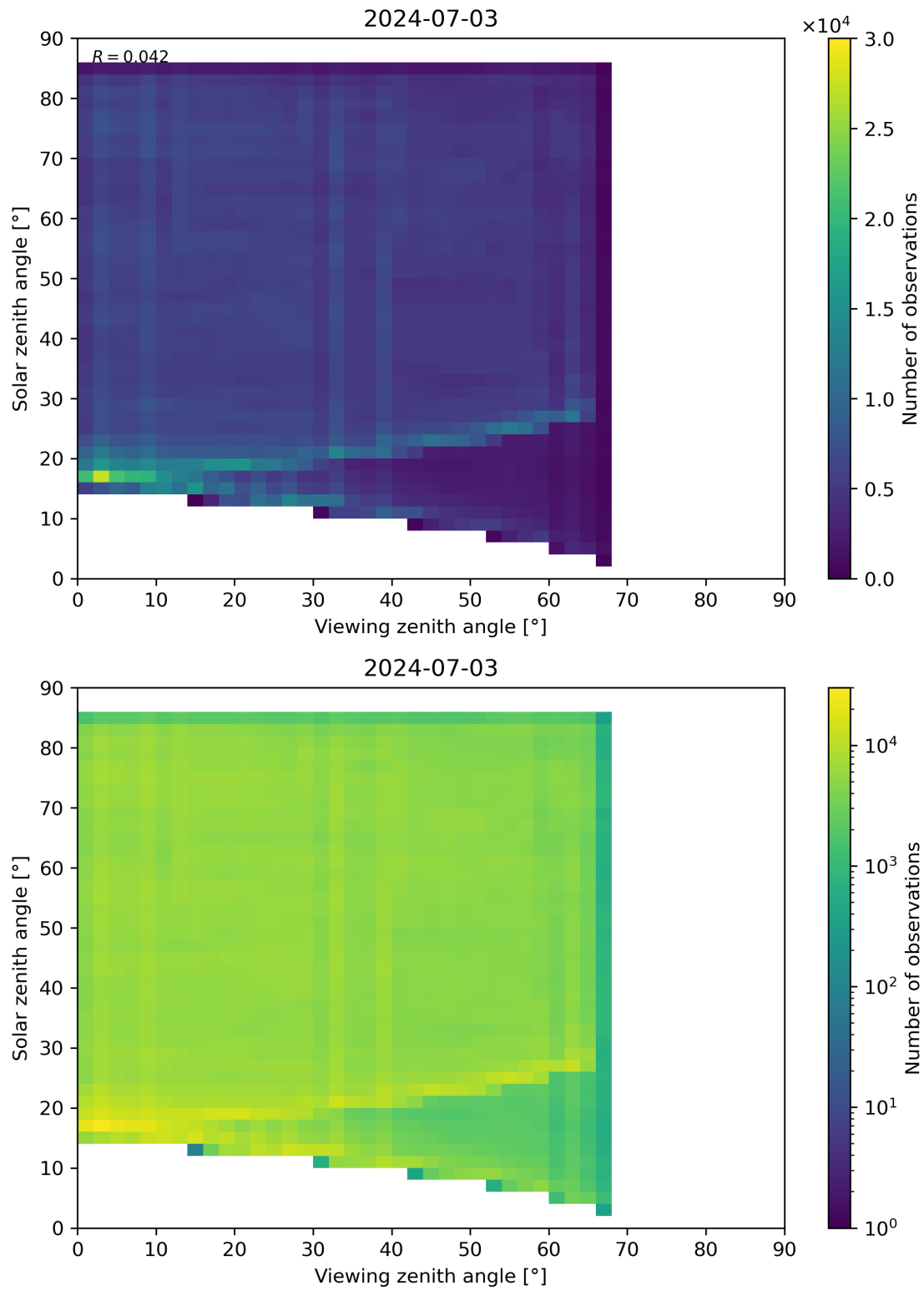
Figure 77: Scatter density plot of “Viewing zenith angle” against “Solar zenith angle” for 2024-07-02 to 2024-07-04.
