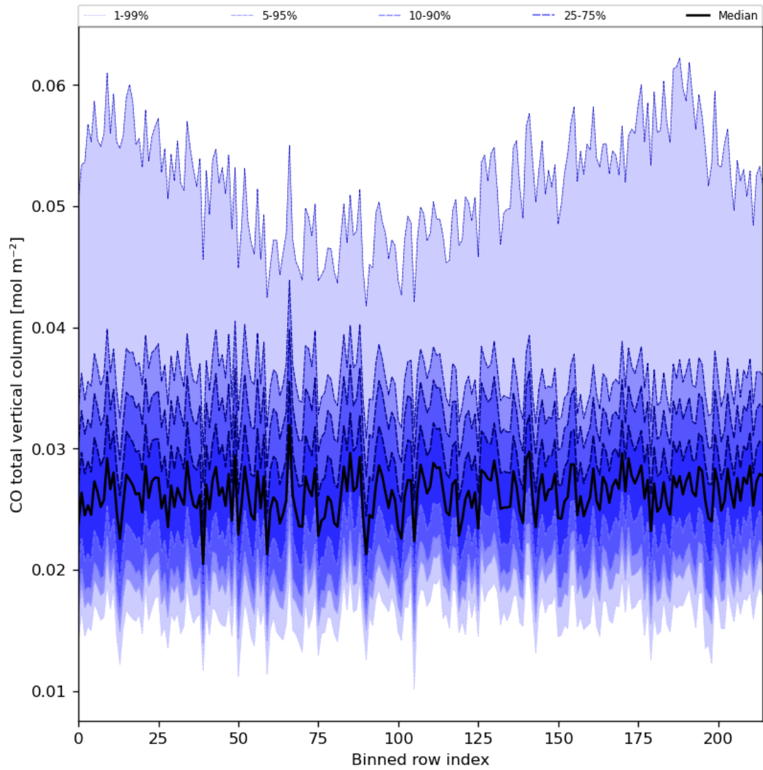
Figure 26: Along track statistics of “CO total vertical column” for 2024-07-02 to 2024-07-04
