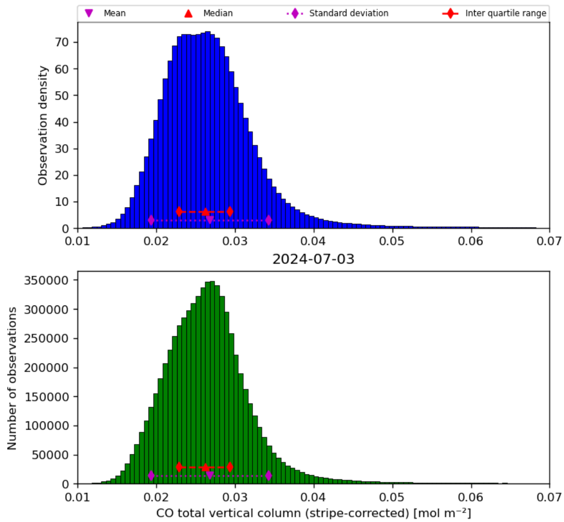
Figure 19: Histogram of “CO total vertical column (stripe-corrected)” for 2024-07-02 to 2024-07-04
