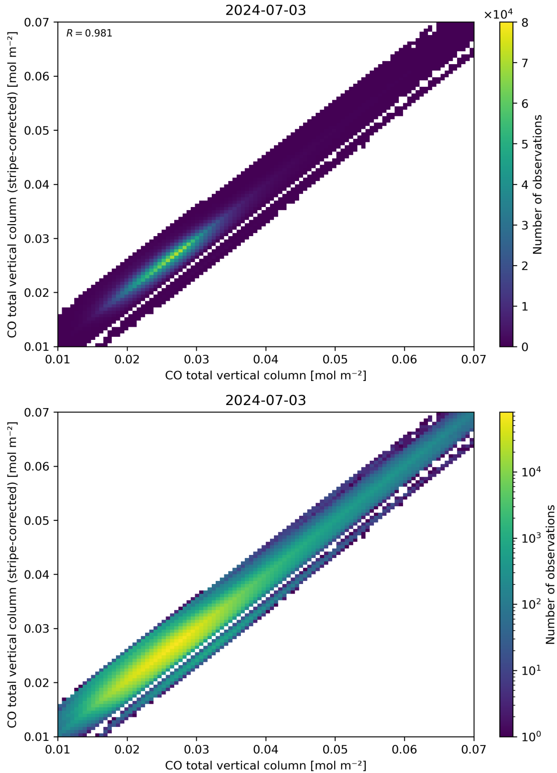
Figure 33: Scatter density plot of “CO total vertical column” against “CO total vertical column (stripe-corrected)” for 2024-07-02 to 2024-07-04.
