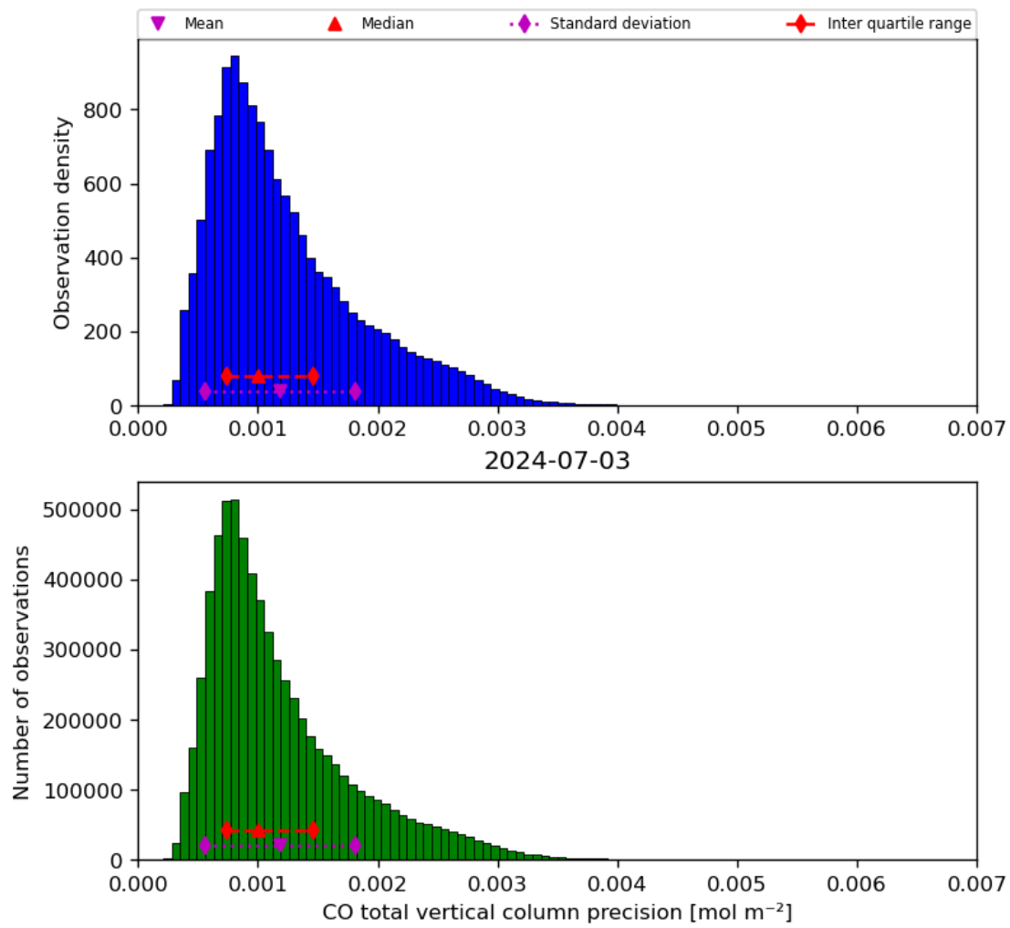
Figure 20: Histogram of “CO total vertical column precision” for 2024-07-02 to 2024-07-04
