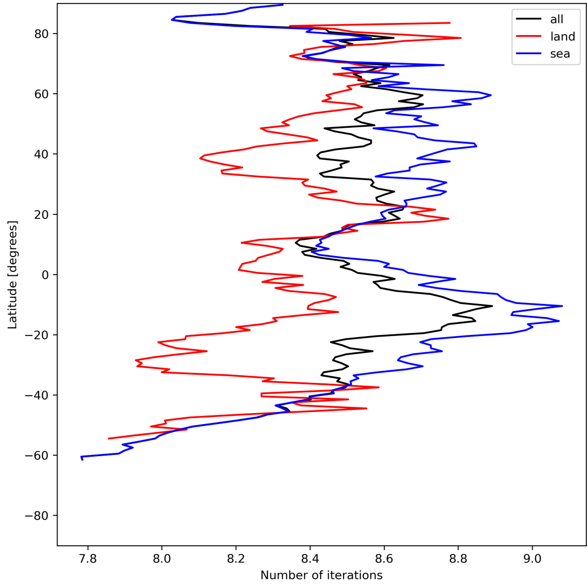
Figure 16: Zonal average of “Number of iterations” for 2024-07-02 to 2024-07-04.
