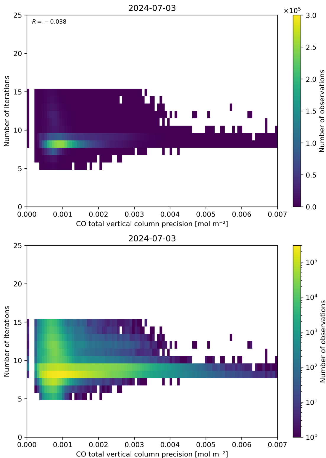
Figure 46: Scatter density plot of “CO total vertical column precision” against “Number of iterations” for 2024-07-02 to 2024-07-04.
