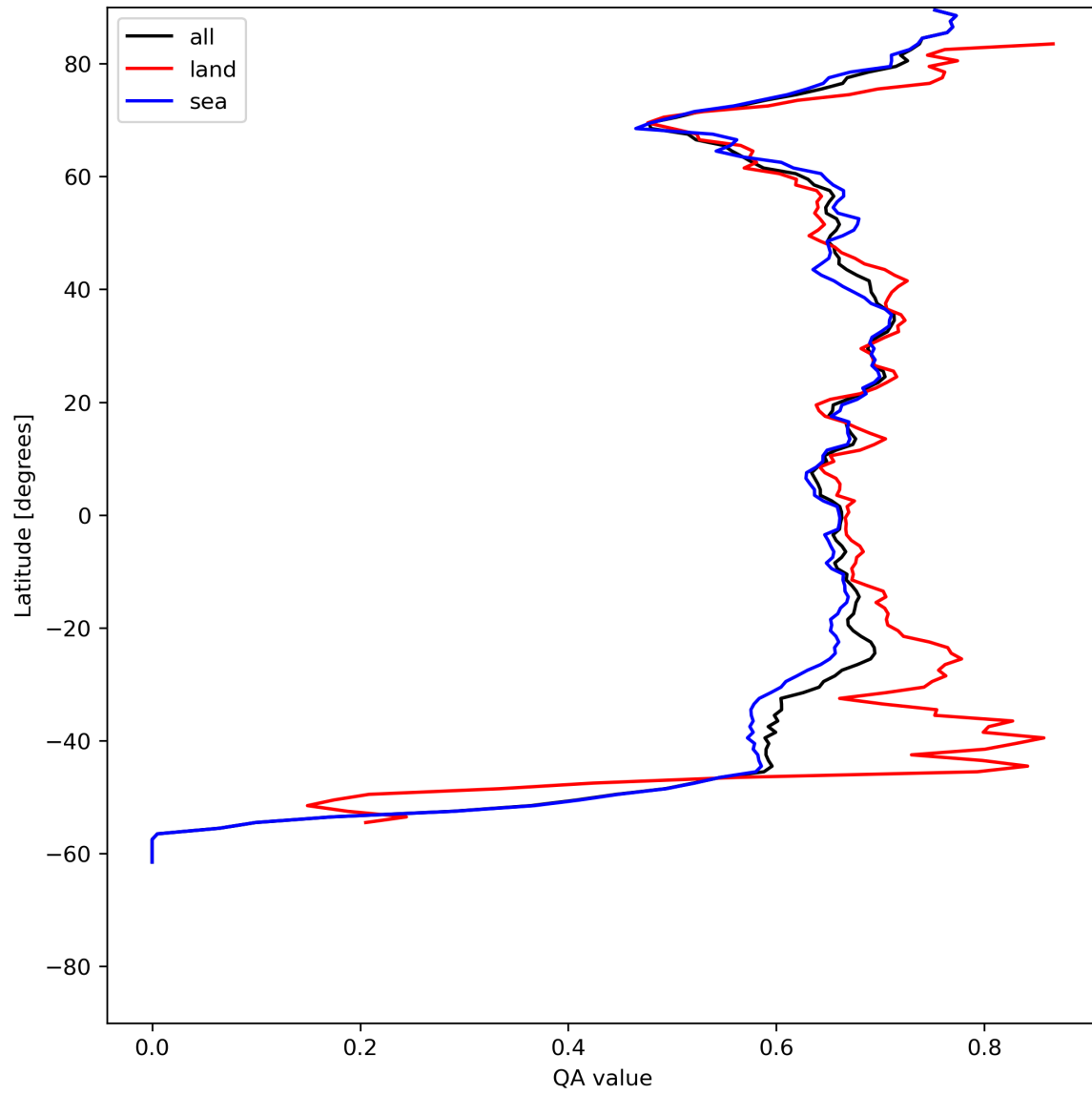
Figure 9: Zonal average of “QA value” for 2024-07-02 to 2024-07-04.
