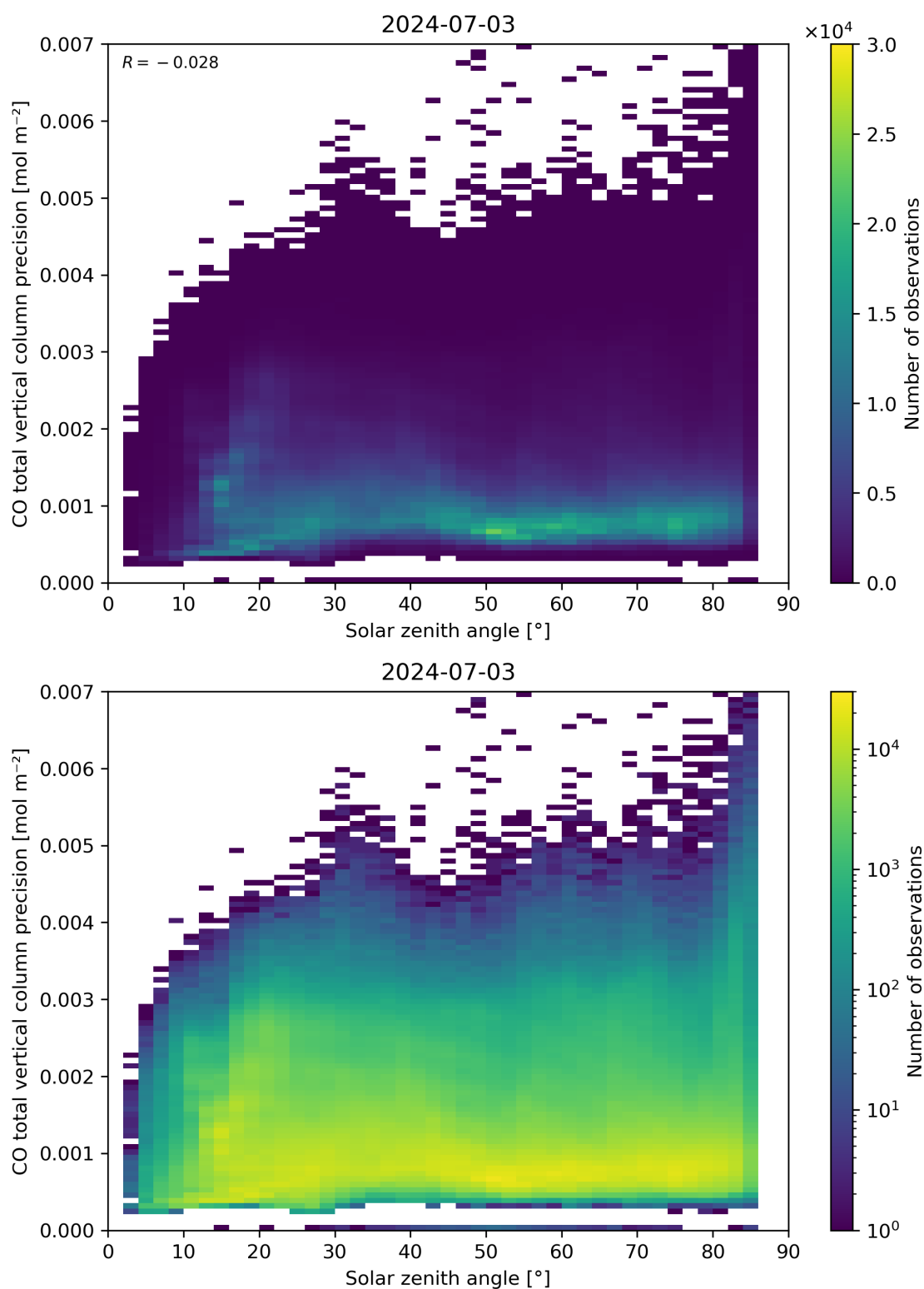
Figure 63: Scatter density plot of “Solar zenith angle” against “CO total vertical column precision” for 2024-07-02 to 2024-07-04.
