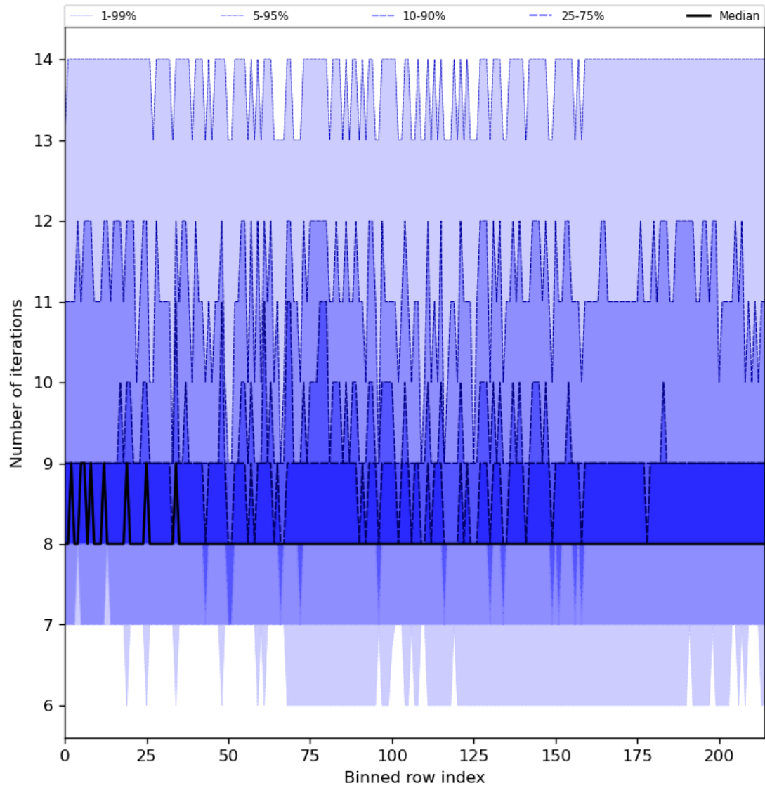
Figure 32: Along track statistics of “Number of iterations” for 2024-07-02 to 2024-07-04
