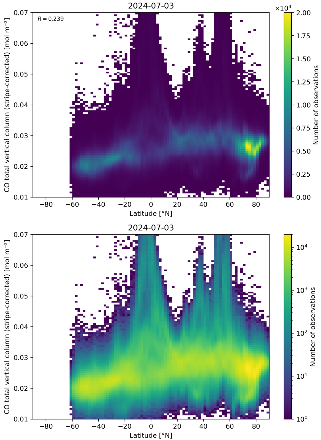
Figure 52: Scatter density plot of “Latitude” against “CO total vertical column (stripe-corrected)” for 2024-07-02 to 2024-07-04.
