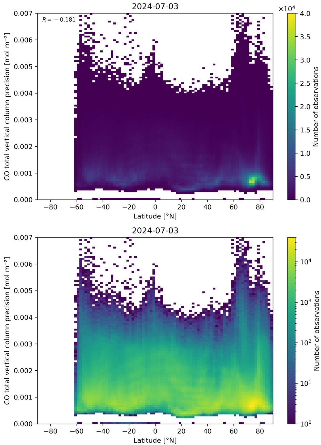
Figure 53: Scatter density plot of “Latitude” against “CO total vertical column precision” for 2024-07-02 to 2024-07-04.
