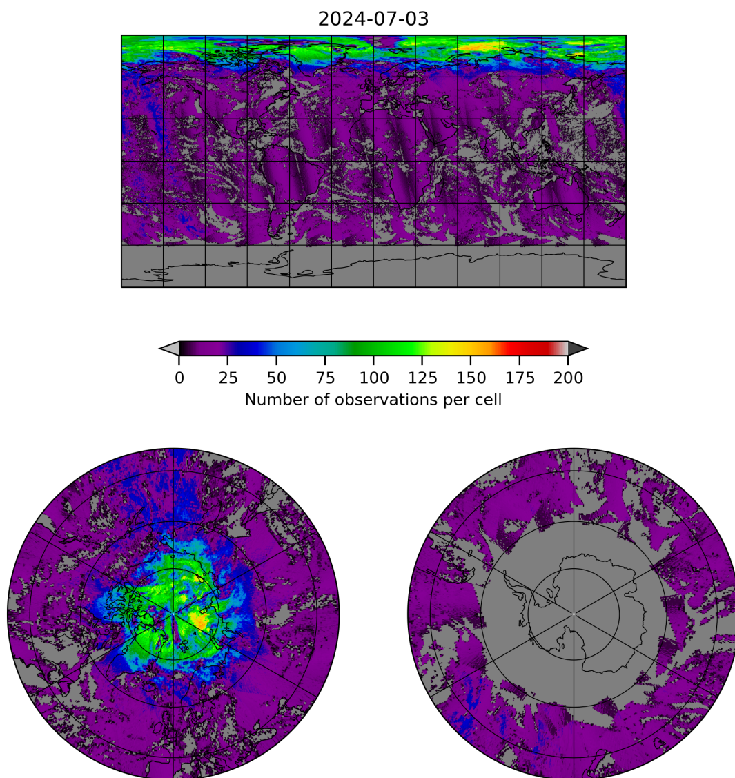
Figure 8: Map of the number of observations for 2024-07-02 to 2024-07-04
