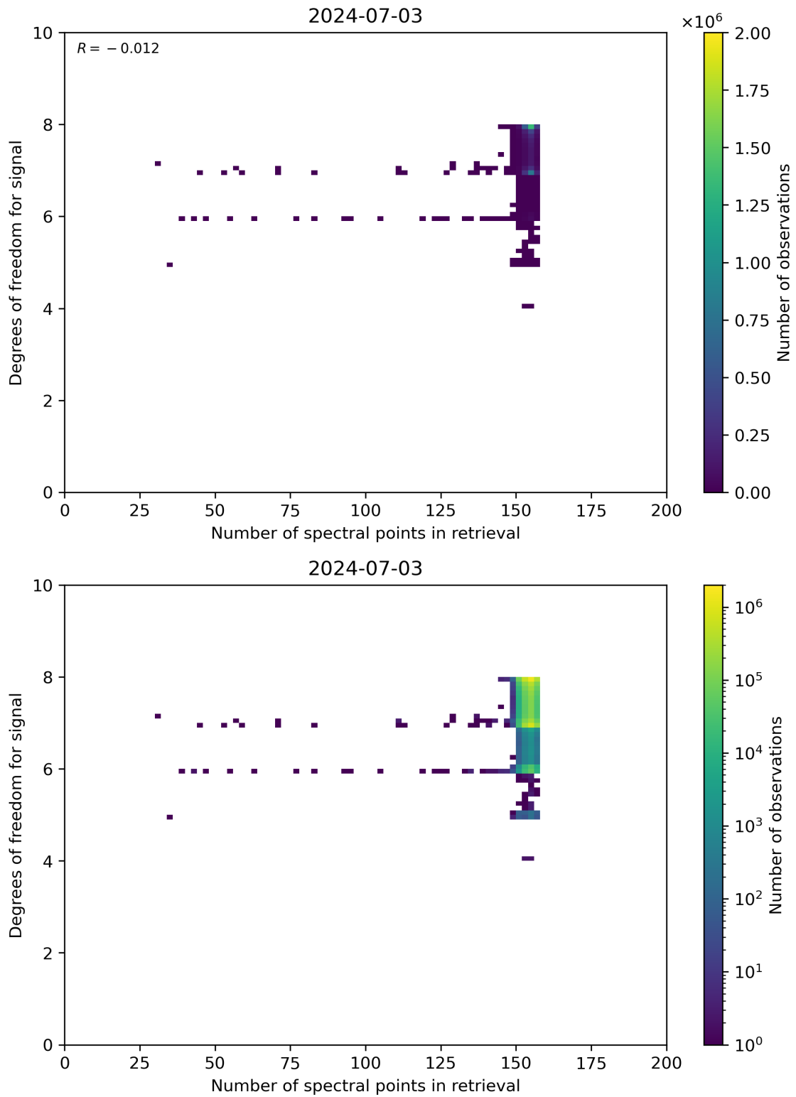
Figure 59: Scatter density plot of “Number of spectral points in retrieval” against “Degrees of freedom for signal” for 2024-07-02 to 2024-07-04.
