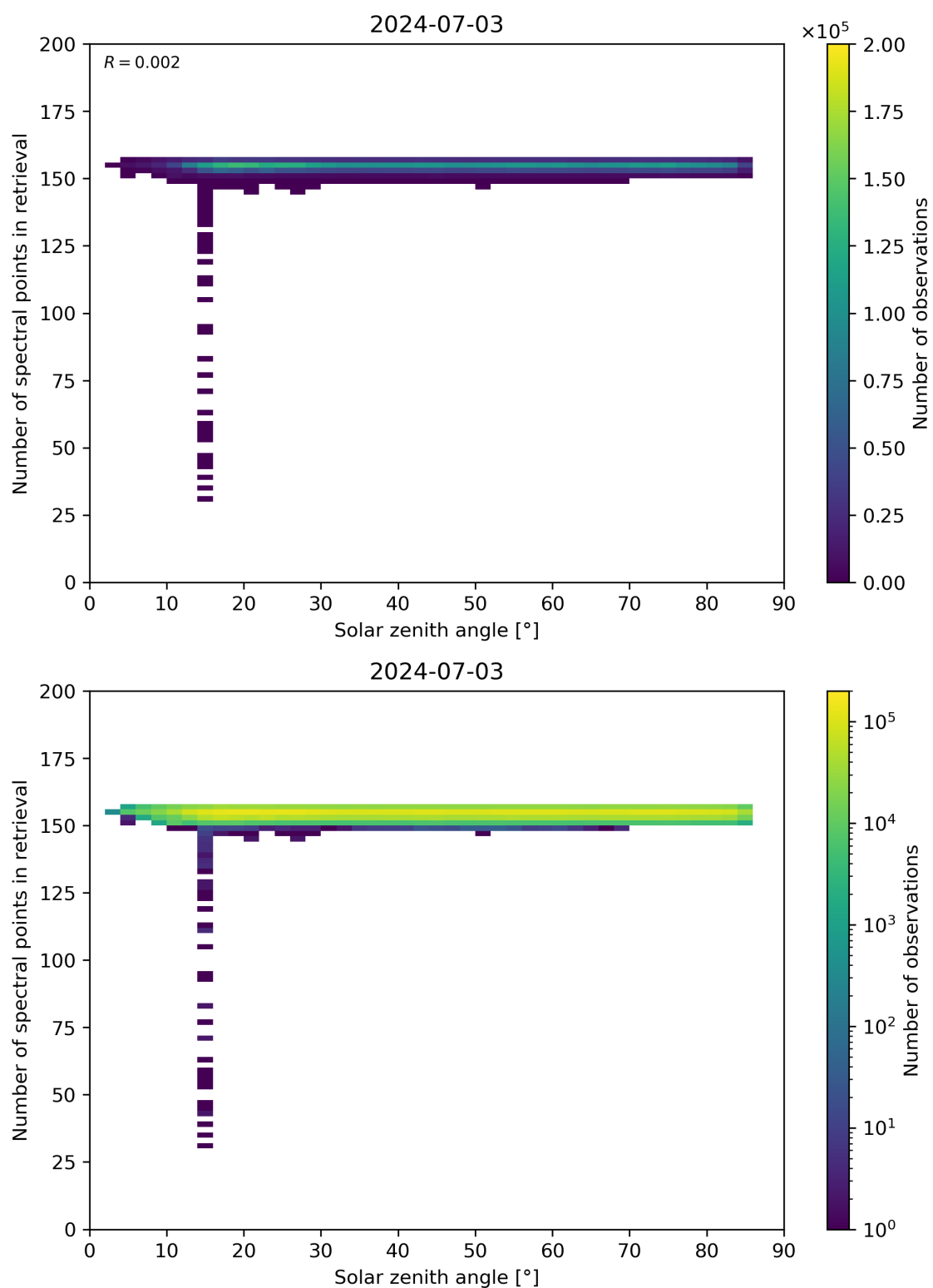
Figure 68: Scatter density plot of “Solar zenith angle” against “Number of spectral points in retrieval” for 2024-07-02 to 2024-07-04.
