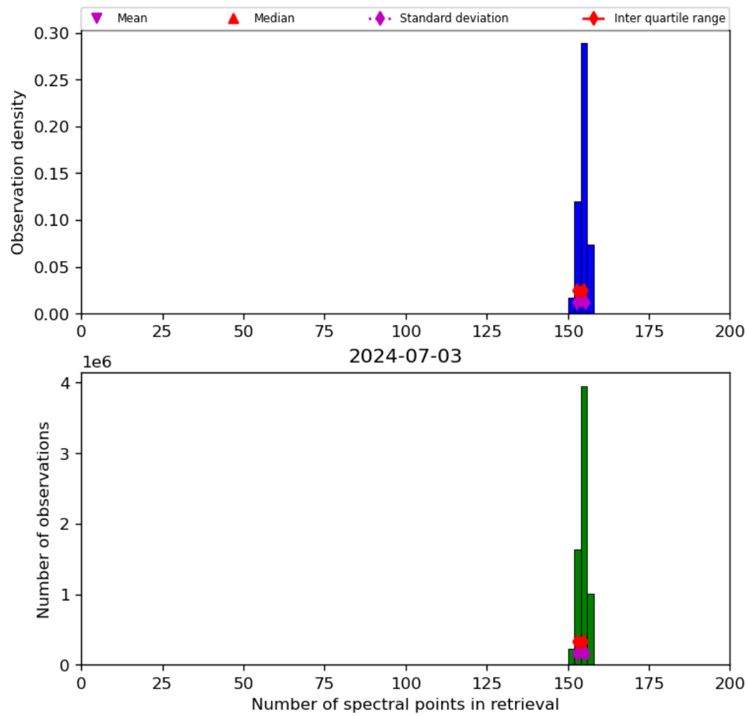
Figure 21: Histogram of “Number of spectral points in retrieval” for 2024-07-02 to 2024-07-04
