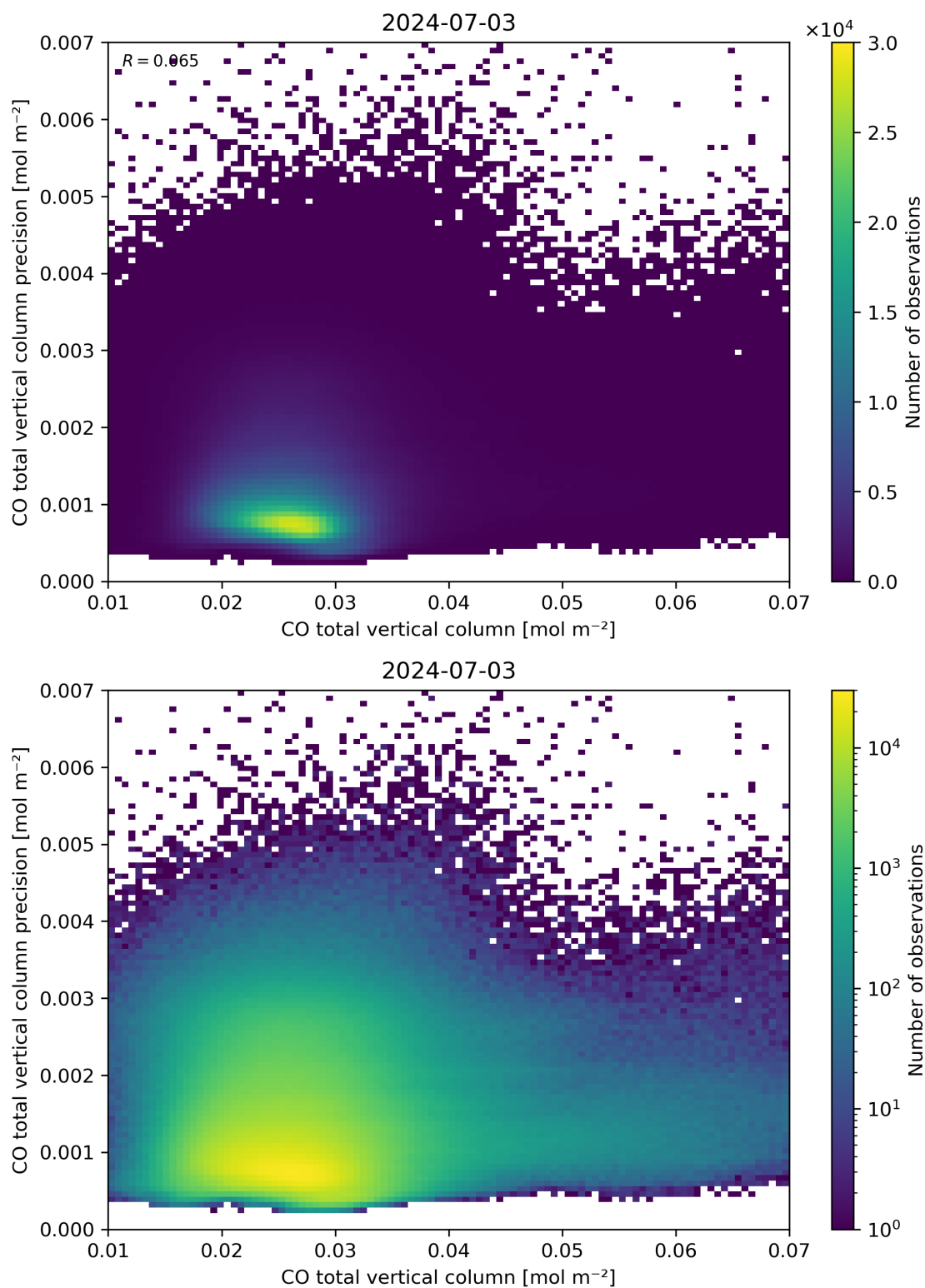
Figure 34: Scatter density plot of “CO total vertical column” against “CO total vertical column precision” for 2024-07-02 to 2024-07-04.
