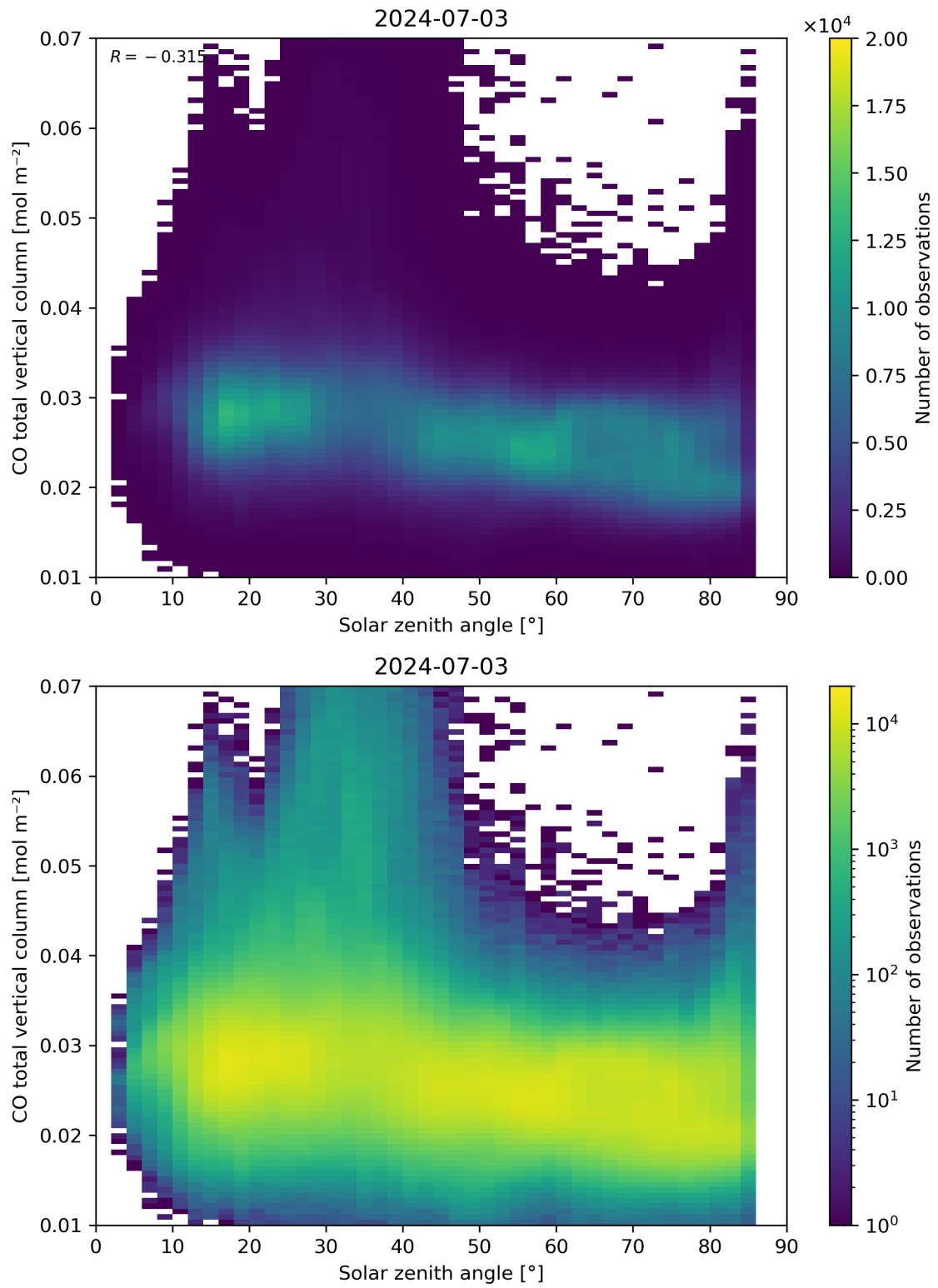
Figure 61: Scatter density plot of “Solar zenith angle” against “CO total vertical column” for 2024-07-02 to 2024-07-04.
