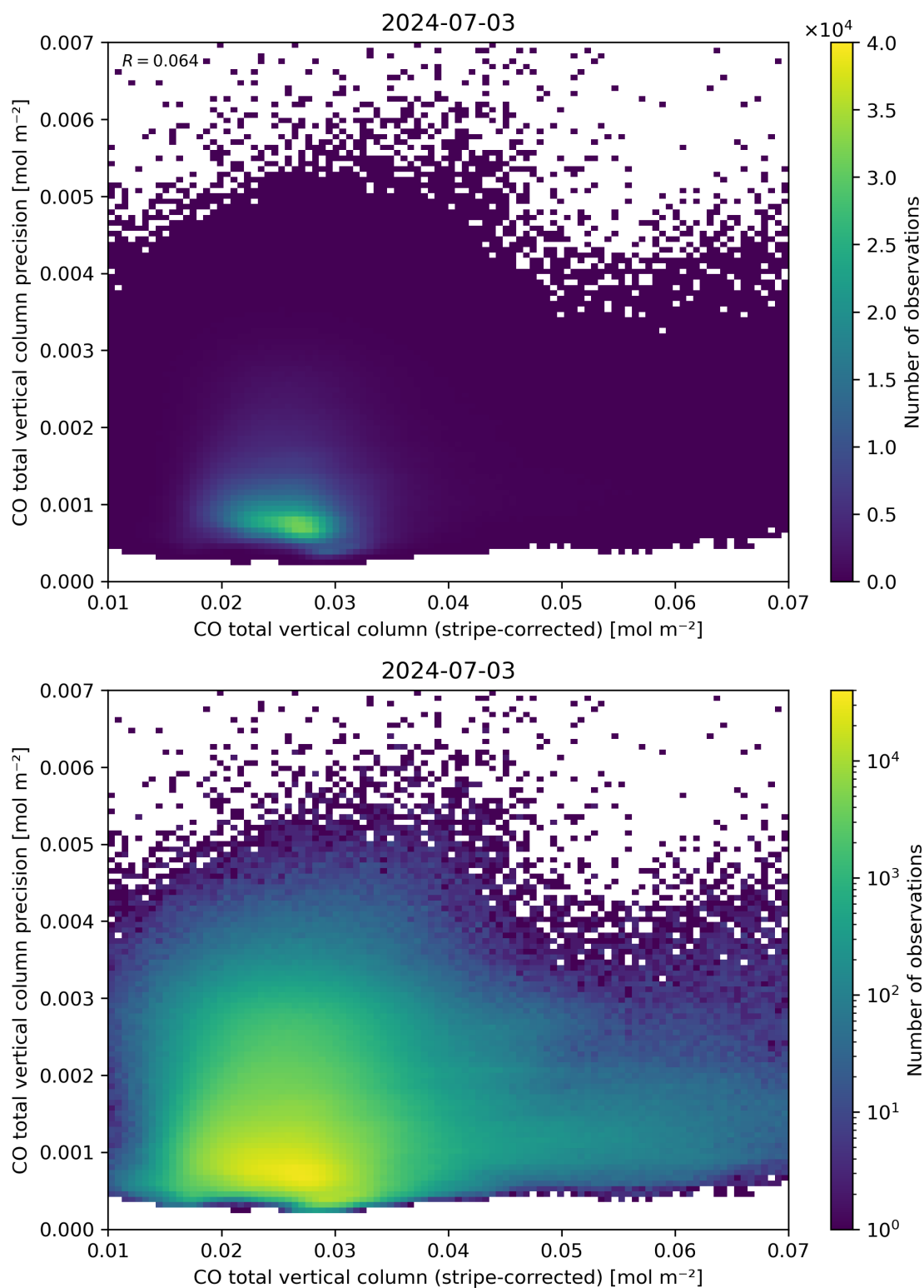
Figure 36: Scatter density plot of “CO total vertical column (stripe-corrected)” against “CO total vertical column precision” for 2024-07-02 to 2024-07-04.
