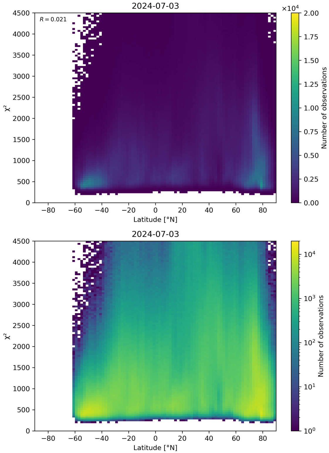
Figure 54: Scatter density plot of “Latitude” against “ \chi^2 ” for 2024-07-02 to 2024-07-04.
