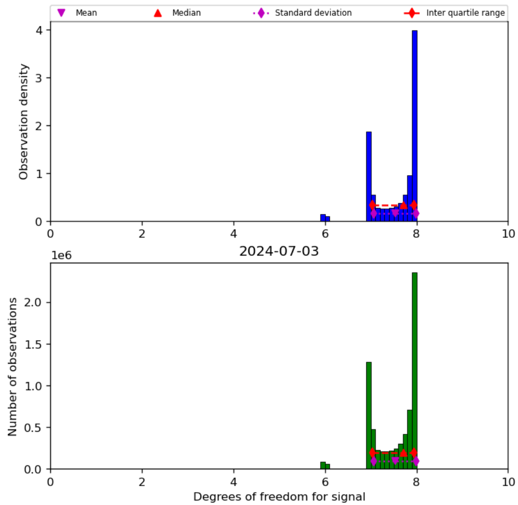
Figure 23: Histogram of “Degrees of freedom for signal” for 2024-07-02 to 2024-07-04
