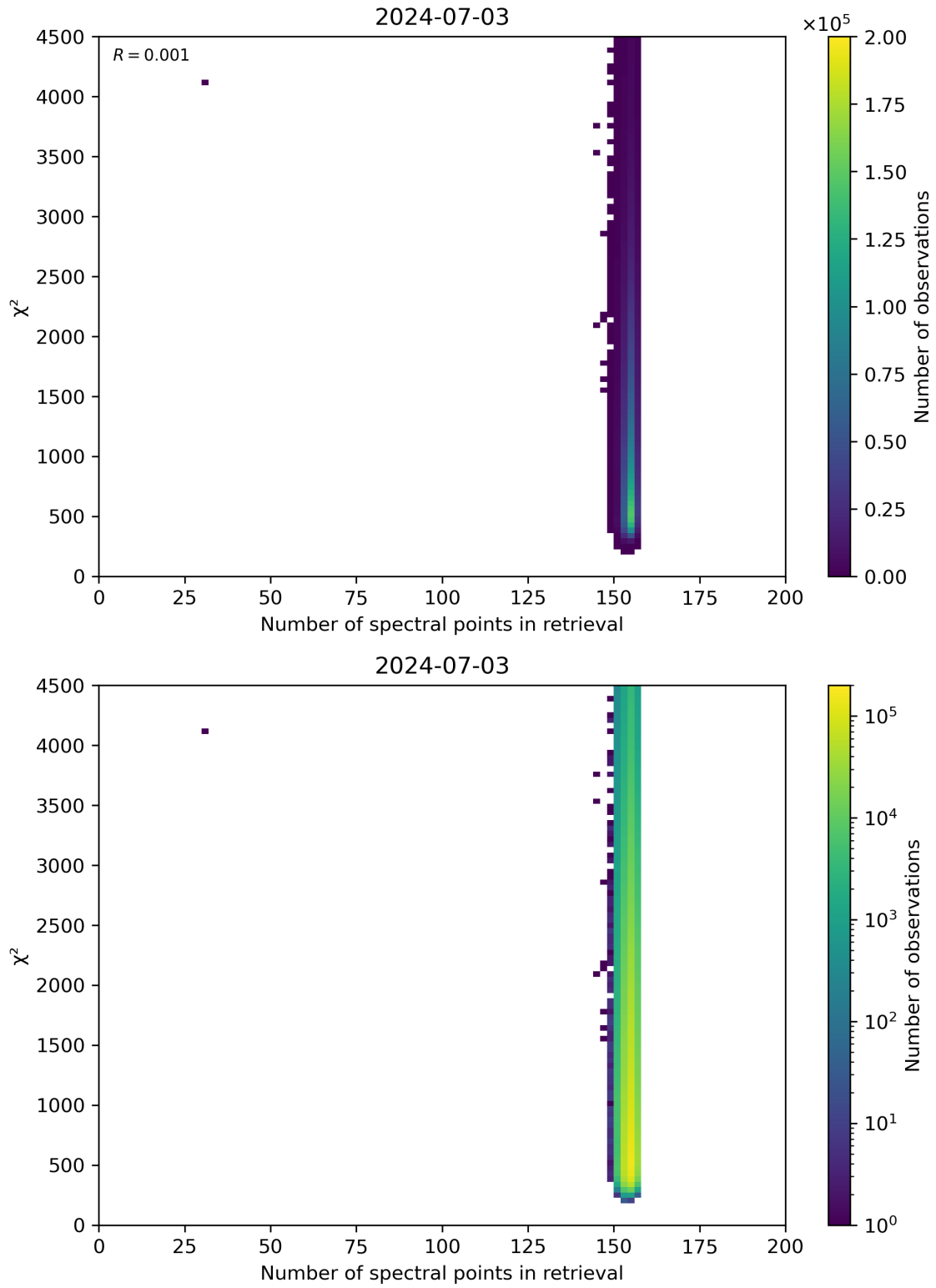
Figure 58: Scatter density plot of “Number of spectral points in retrieval” against “ \chi^2 ” for 2024-07-02 to 2024-07-04.
