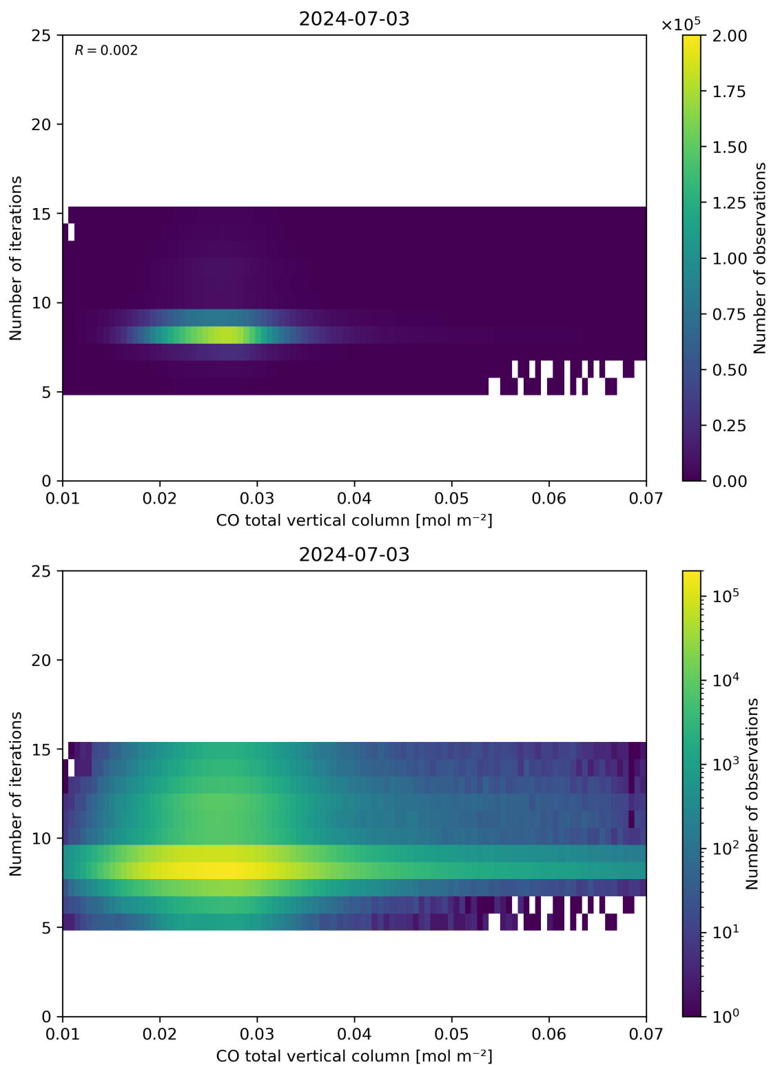
Figure 42: Scatter density plot of “CO total vertical column” against “Number of iterations” for 2024-07-02 to 2024-07-04.
