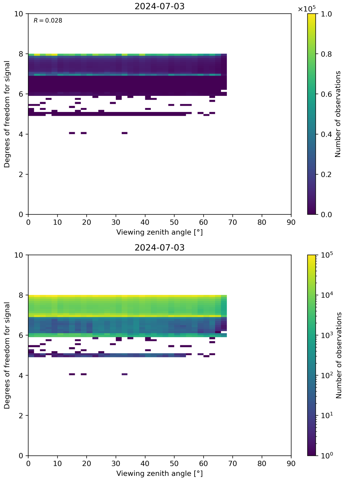
Figure 73: Scatter density plot of “Viewing zenith angle” against “Degrees of freedom for signal” for 2024-07-02 to 2024-07-04.
