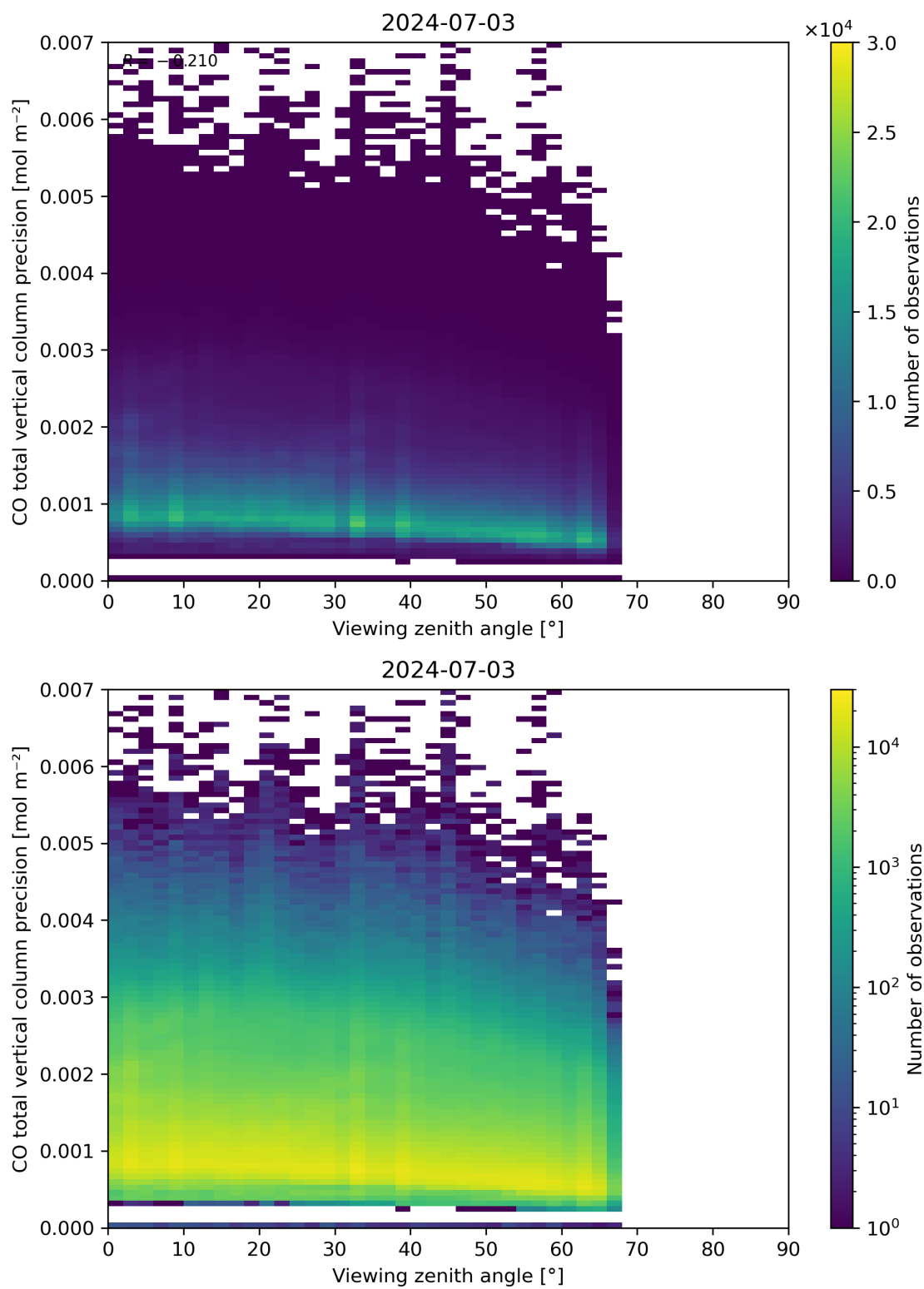
Figure 71: Scatter density plot of “Viewing zenith angle” against “CO total vertical column precision” for 2024-07-02 to 2024-07-04.
