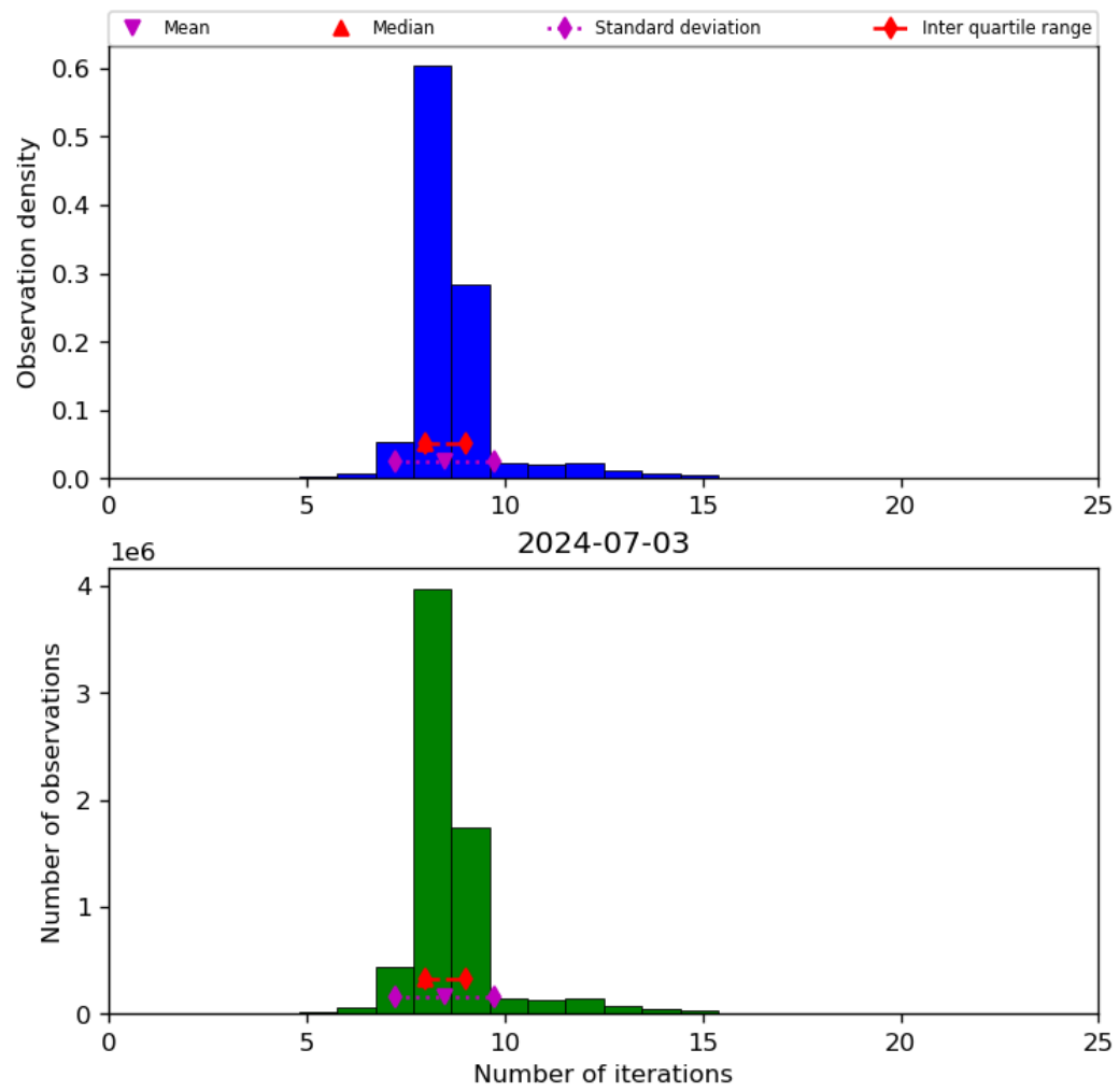
Figure 24: Histogram of “Number of iterations” for 2024-07-02 to 2024-07-04
