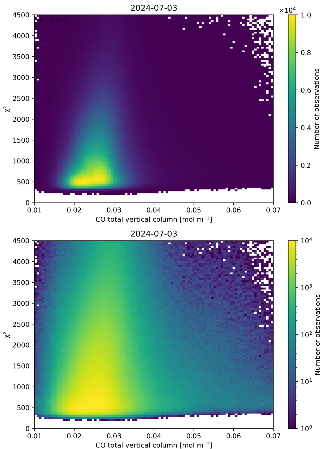
Figure 35: Scatter density plot of “CO total vertical column” against “ \chi^2 ” for 2024-07-02 to 2024-07-04.
