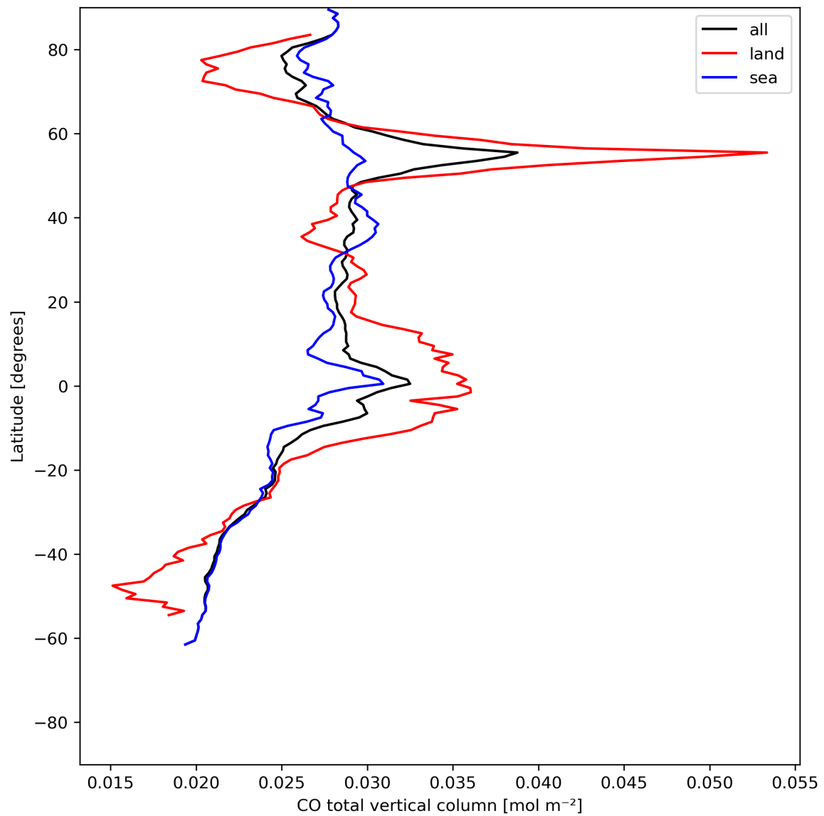
Figure 10: Zonal average of “CO total vertical column” for 2024-07-02 to 2024-07-04.
