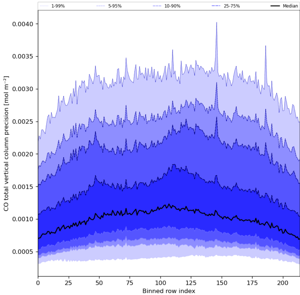
Figure 28: Along track statistics of “CO total vertical column precision” for 2024-07-02 to 2024-07-04
