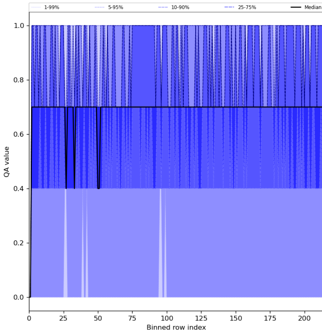
Figure 25: Along track statistics of “QA value” for 2024-07-02 to 2024-07-04
