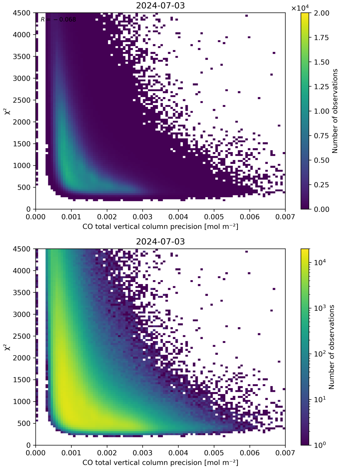
Figure 44: Scatter density plot of “CO total vertical column precision” against “ \chi^2 ” for 2024-07-02 to 2024-07-04.
