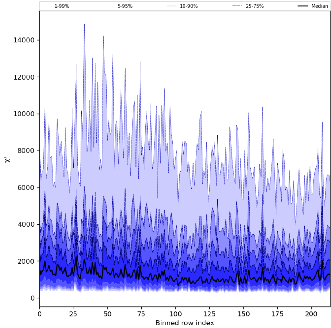
Figure 30: Along track statistics of “ \chi^2 ” for 2024-07-02 to 2024-07-04
