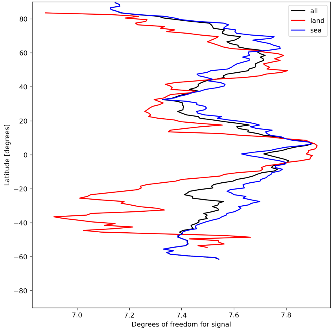
Figure 15: Zonal average of “Degrees of freedom for signal” for 2024-07-02 to 2024-07-04.
