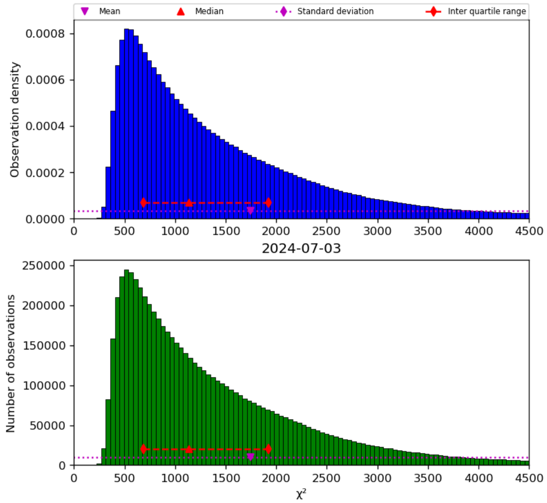
Figure 22: Histogram of “ \chi^2 ” for 2024-07-02 to 2024-07-04
