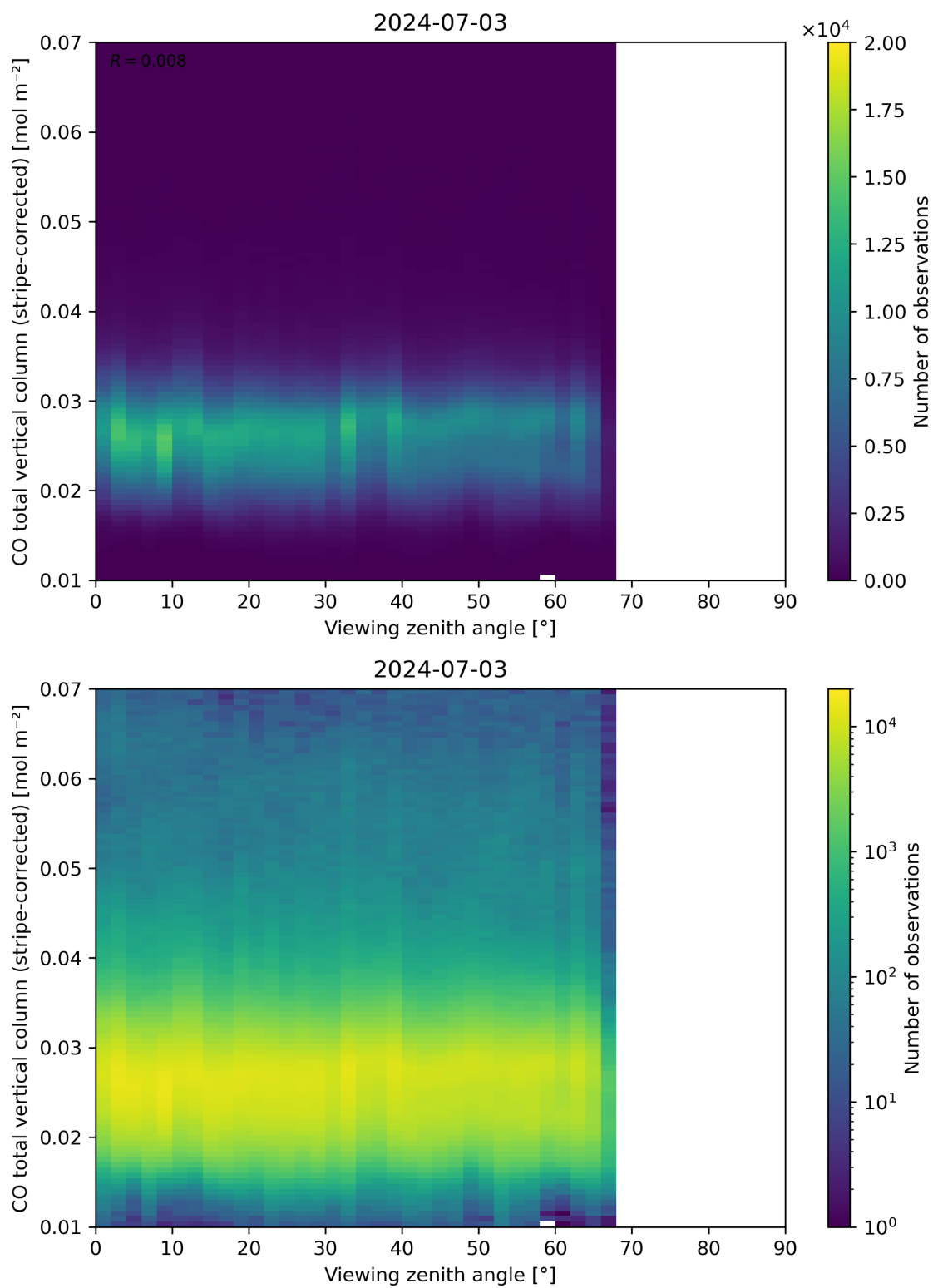
Figure 70: Scatter density plot of “Viewing zenith angle” against “CO total vertical column (stripe-corrected)” for 2024-07-02 to 2024-07-04.
