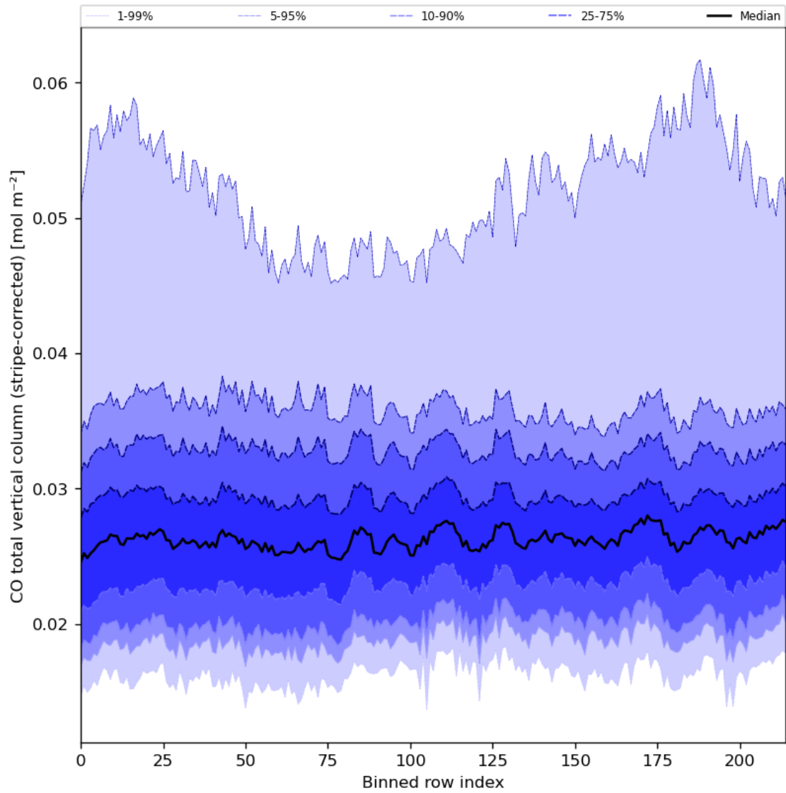
Figure 27: Along track statistics of “CO total vertical column (stripe-corrected)” for 2024-07-02 to 2024-07-04
