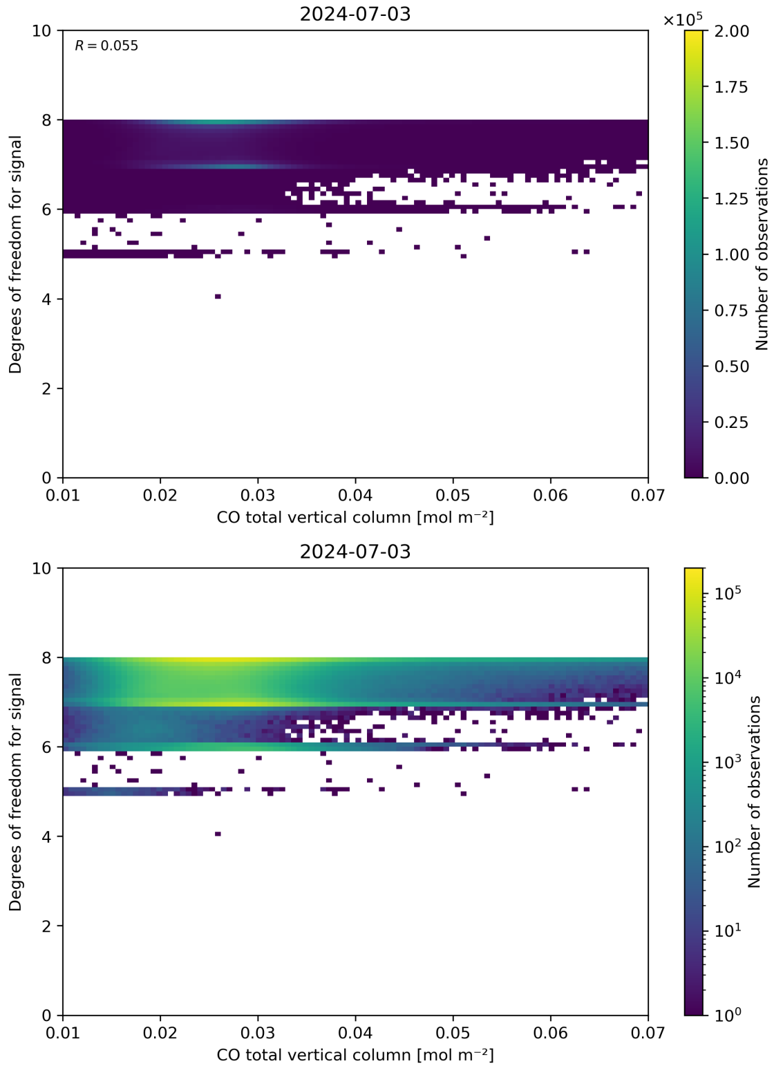
Figure 41: Scatter density plot of “CO total vertical column” against “Degrees of freedom for signal” for 2024-07-02 to 2024-07-04.
