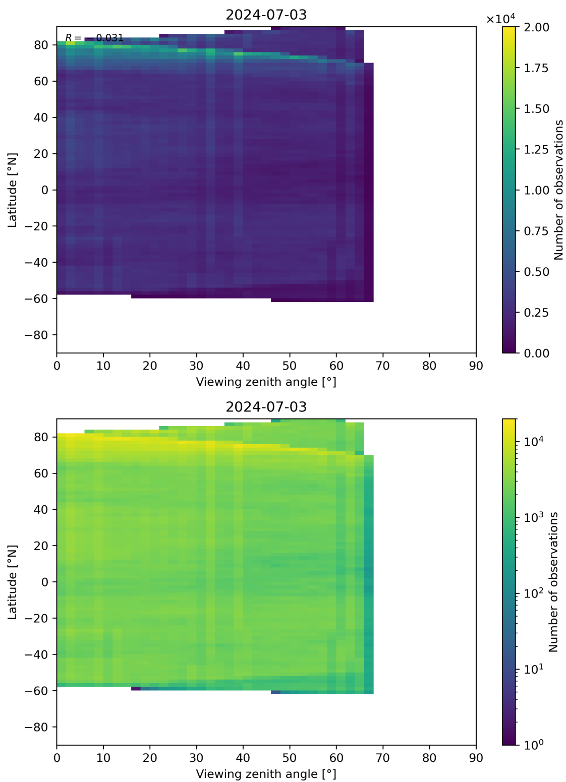
Figure 74: Scatter density plot of “Viewing zenith angle” against “Latitude” for 2024-07-02 to 2024-07-04.
