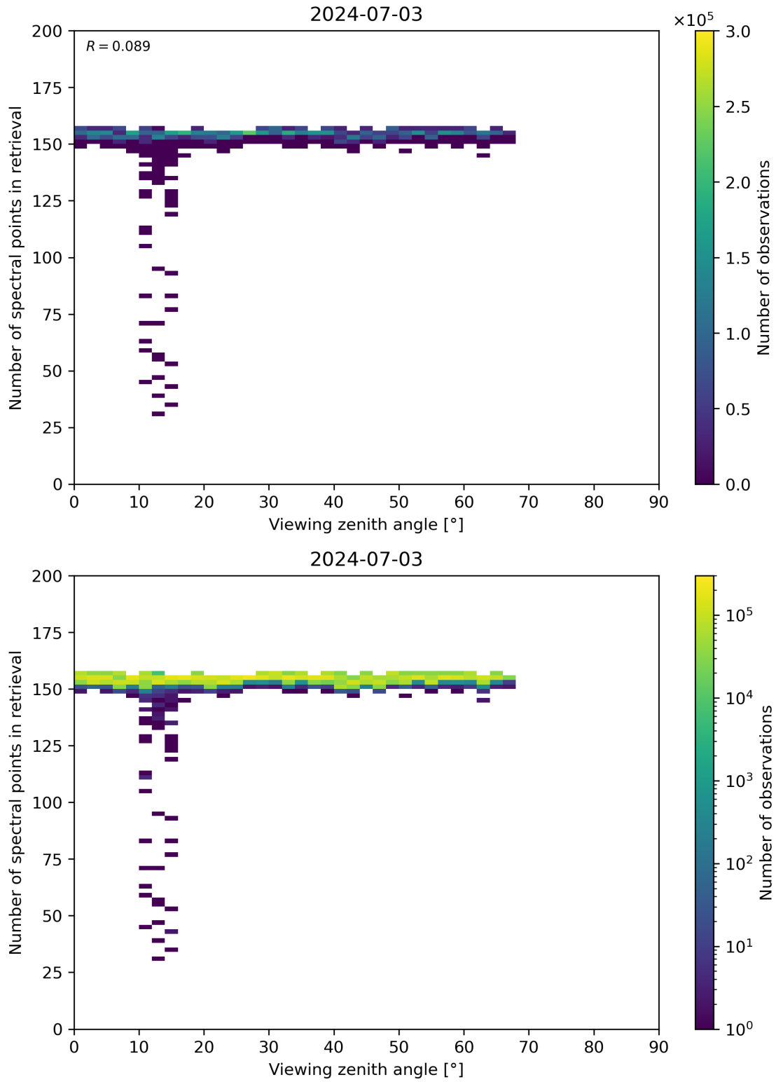
Figure 76: Scatter density plot of “Viewing zenith angle” against “Number of spectral points in retrieval” for 2024-07-02 to 2024-07-04.
