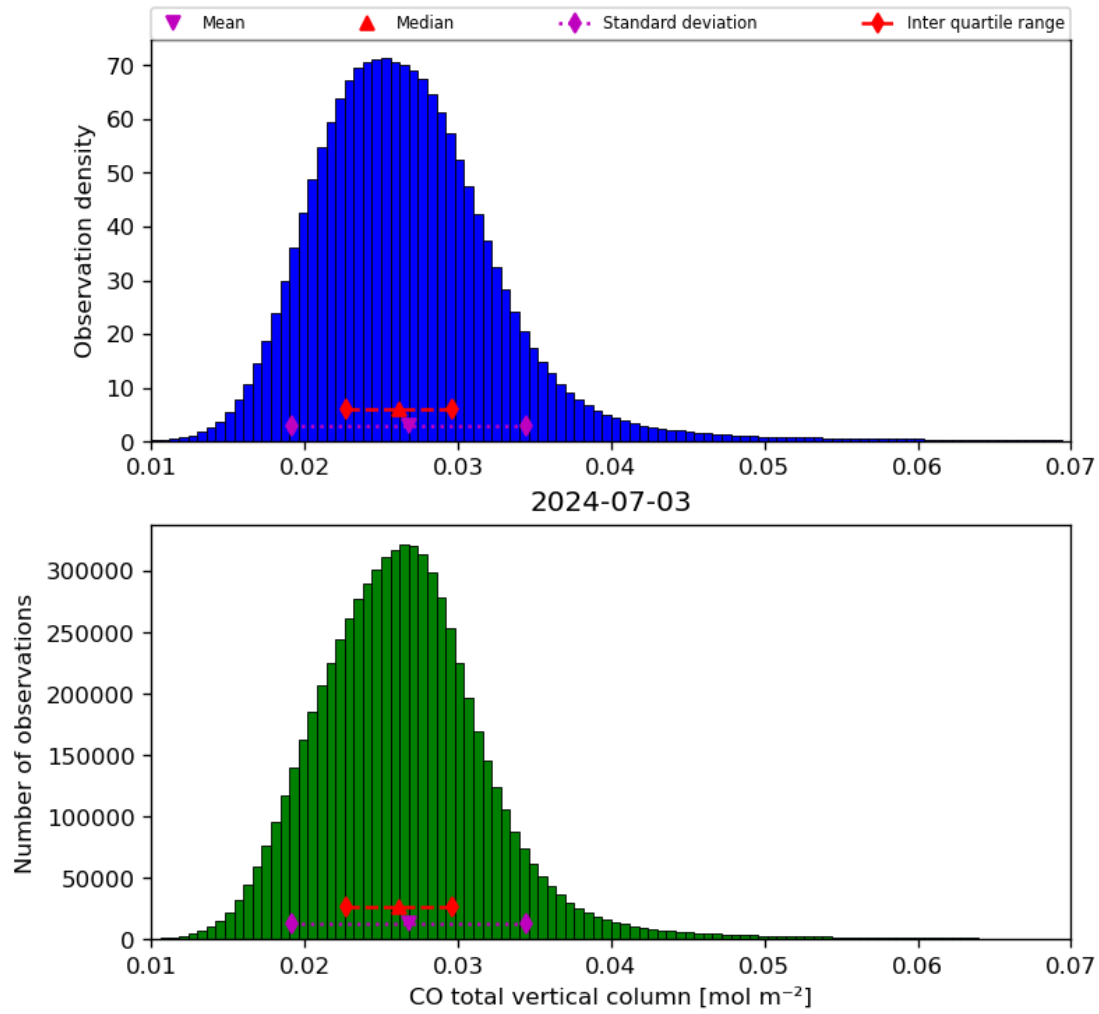
Figure 18: Histogram of “CO total vertical column” for 2024-07-02 to 2024-07-04
