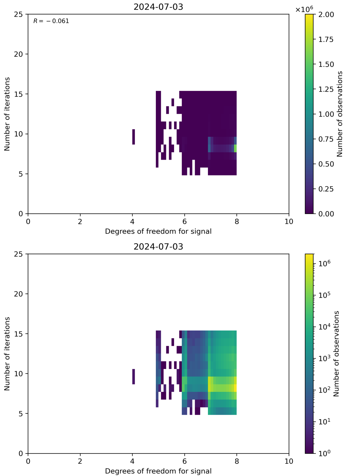
Figure 50: Scatter density plot of “Degrees of freedom for signal” against “Number of iterations” for 2024-07-02 to 2024-07-04.
