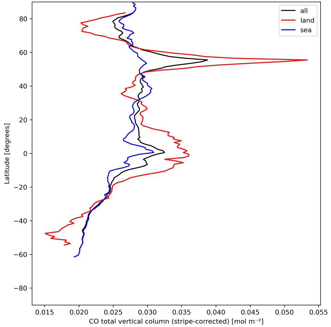
Figure 11: Zonal average of “CO total vertical column (stripe-corrected)” for 2024-07-02 to 2024-07-04.
