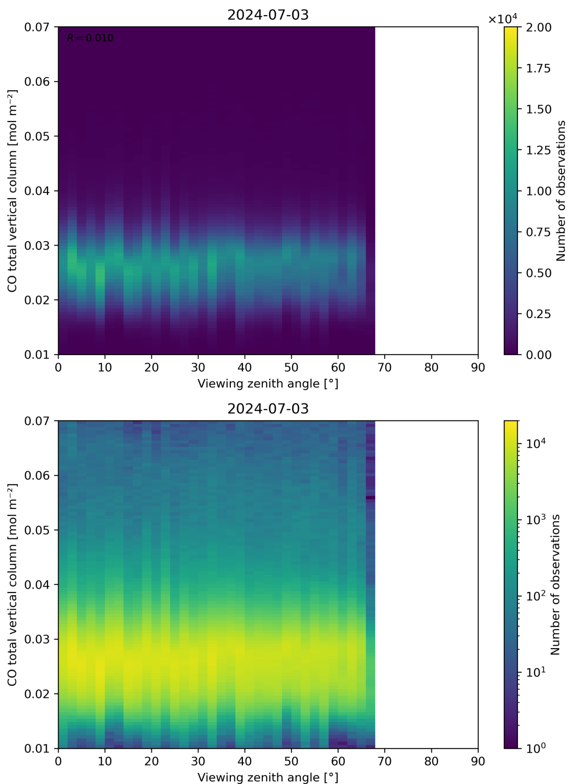
Figure 69: Scatter density plot of “Viewing zenith angle” against “CO total vertical column” for 2024-07-02 to 2024-07-04.
