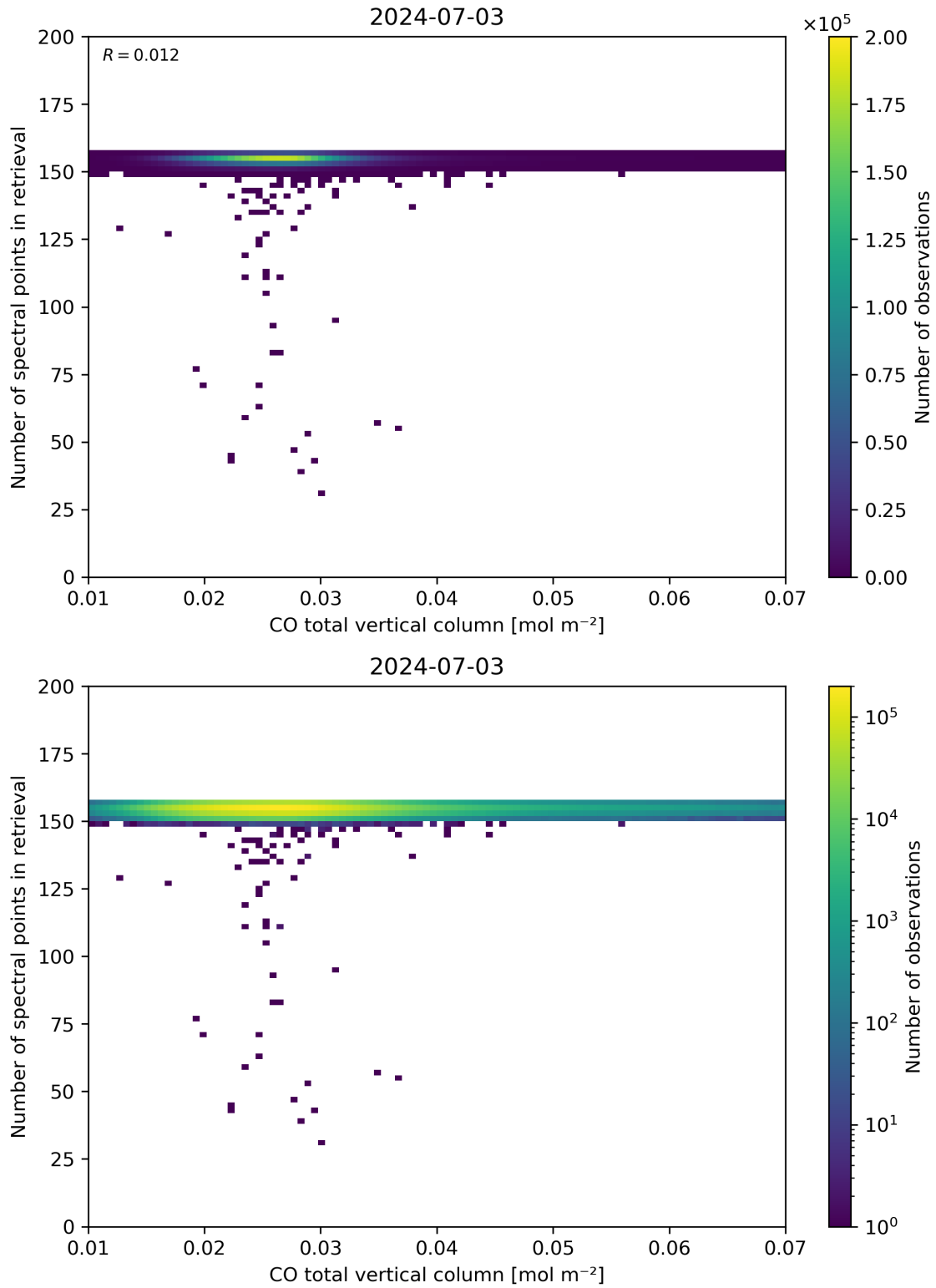
Figure 43: Scatter density plot of “CO total vertical column” against “Number of spectral points in retrieval” for 2024-07-02 to 2024-07-04.
