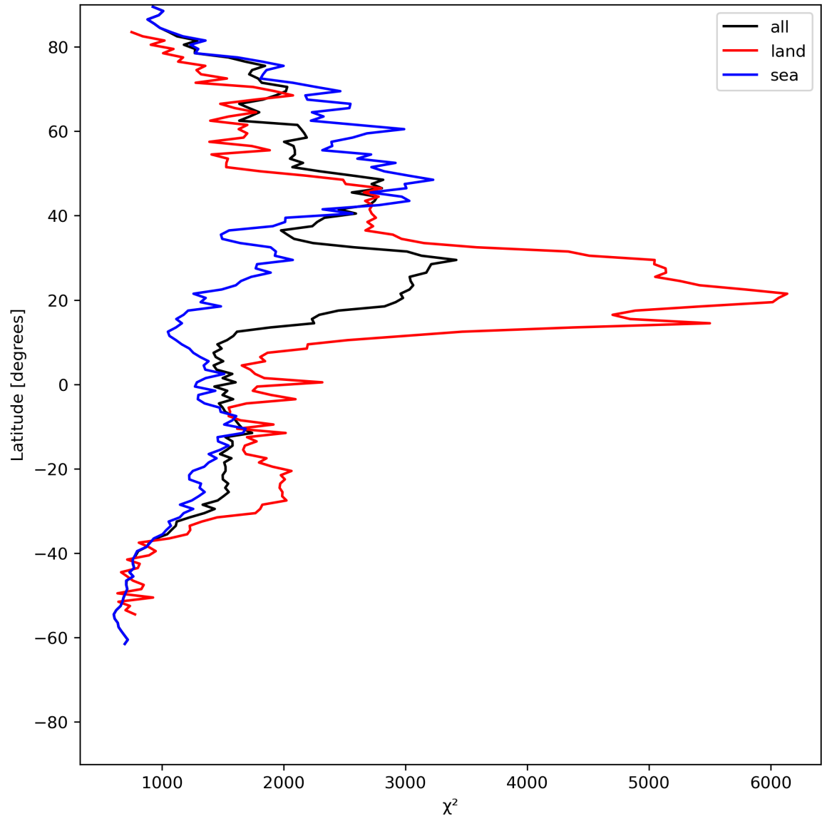
Figure 14: Zonal average of “ \chi^2 ” for 2024-07-02 to 2024-07-04.
