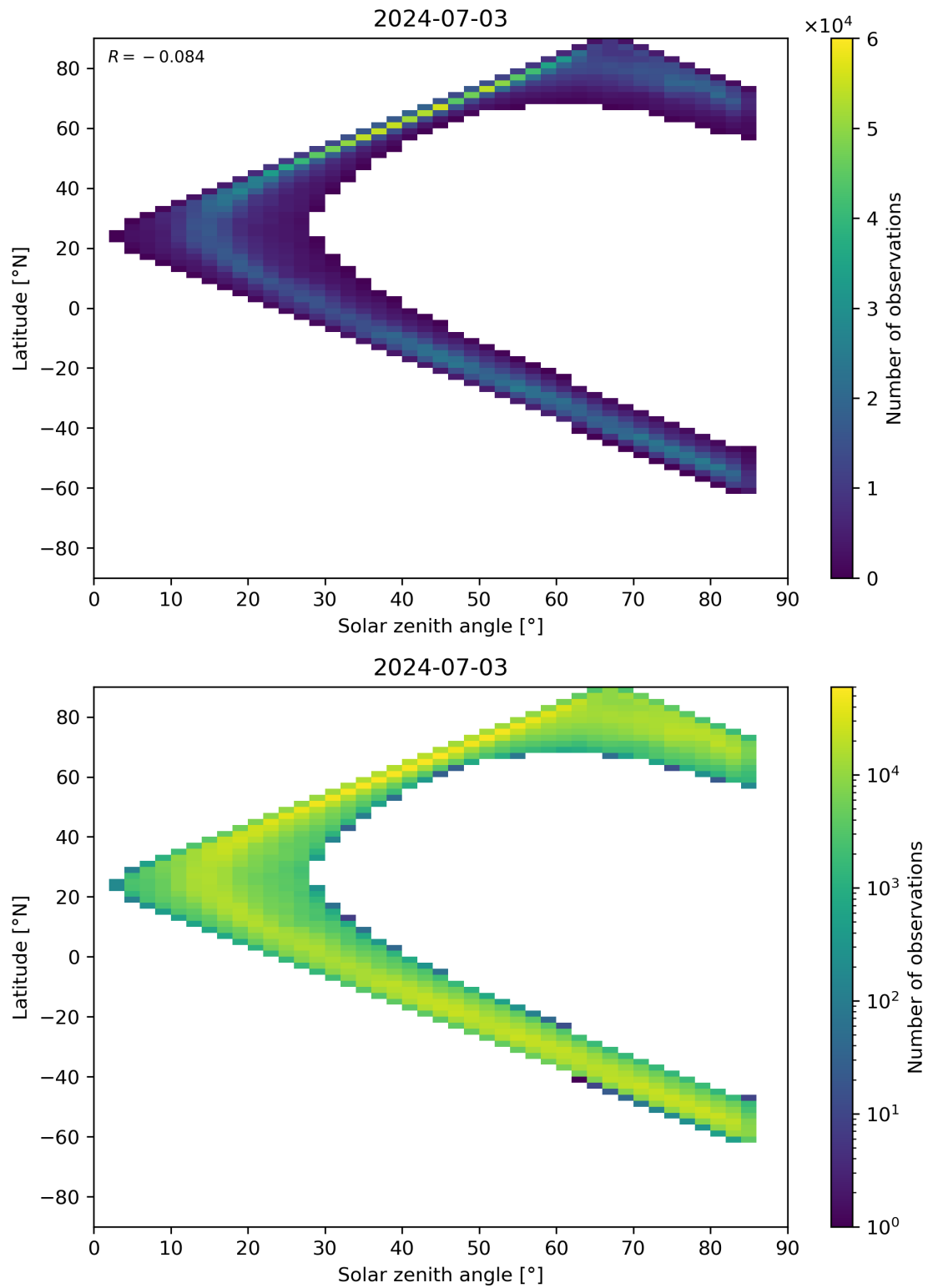
Figure 66: Scatter density plot of “Solar zenith angle” against “Latitude” for 2024-07-02 to 2024-07-04.
