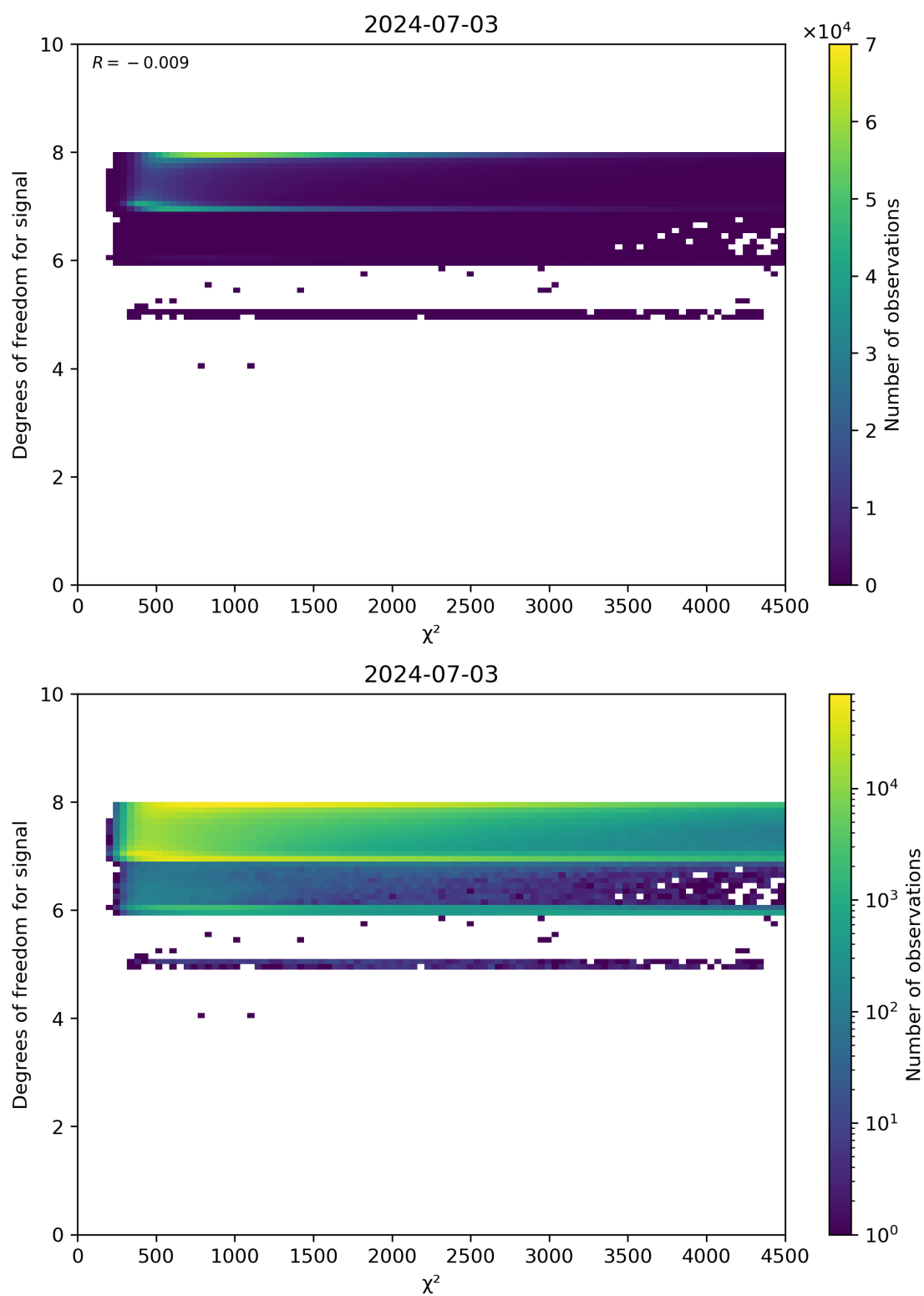
Figure 48: Scatter density plot of “ \chi^2 ” against “Degrees of freedom for signal” for 2024-07-02 to 2024-07-04.
