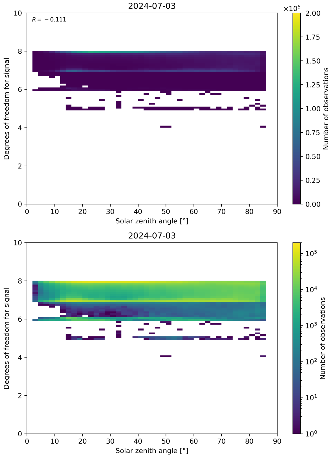
Figure 65: Scatter density plot of “Solar zenith angle” against “Degrees of freedom for signal” for 2024-07-02 to 2024-07-04.
