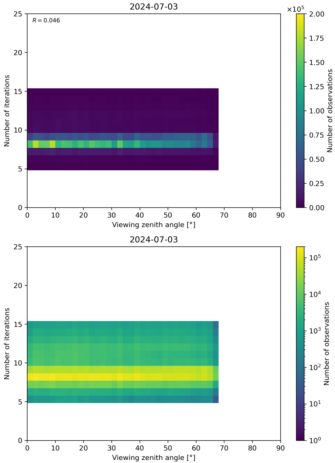
Figure 75: Scatter density plot of “Viewing zenith angle” against “Number of iterations” for 2024-07-02 to 2024-07-04.
