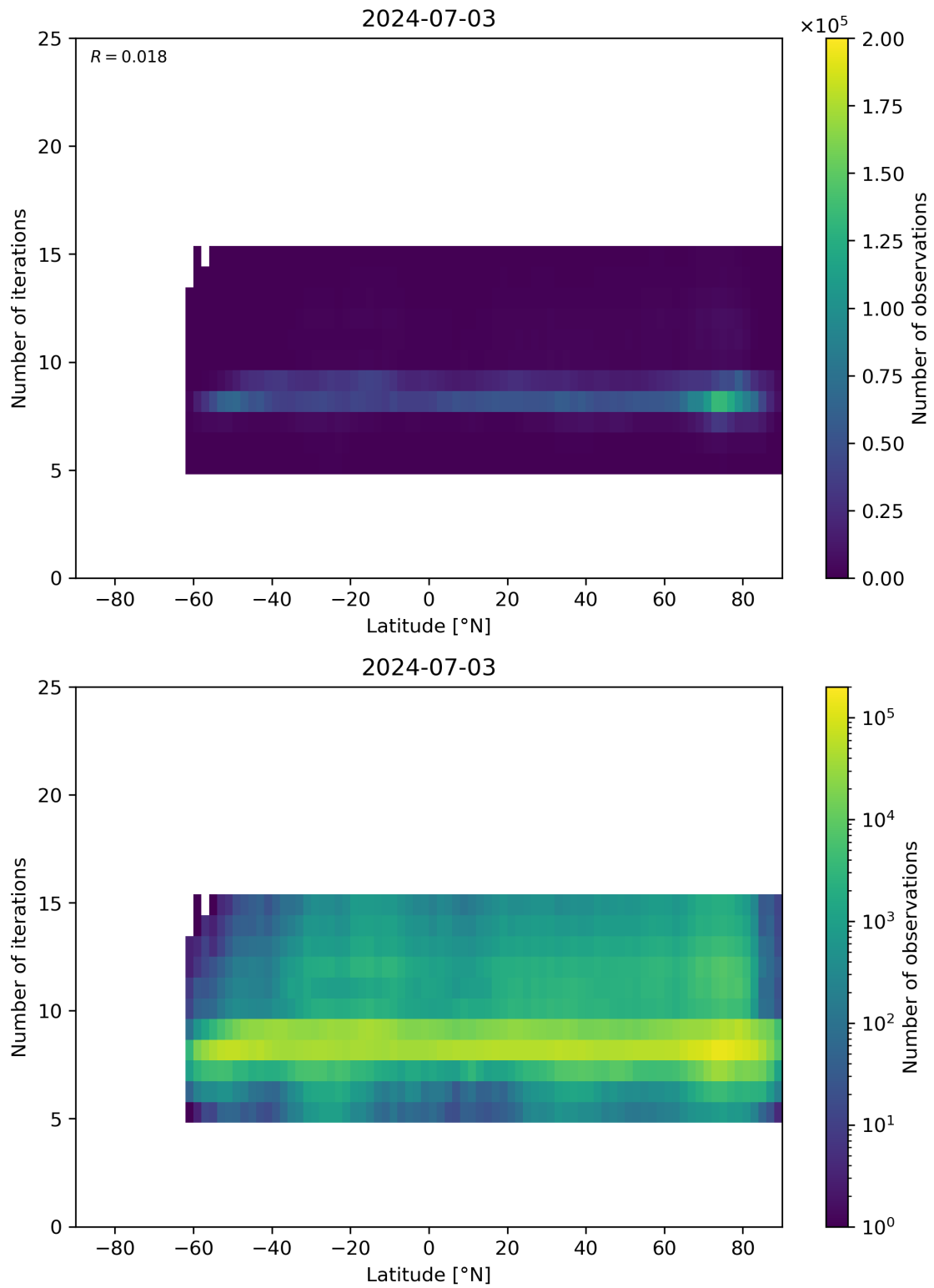
Figure 56: Scatter density plot of “Latitude” against “Number of iterations” for 2024-07-02 to 2024-07-04.
