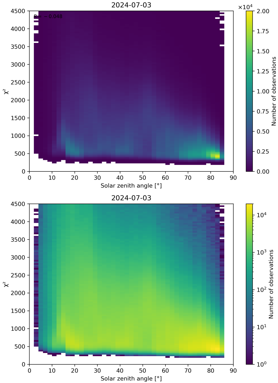
Figure 64: Scatter density plot of “Solar zenith angle” against “ \chi^2 ” for 2024-07-02 to 2024-07-04.
