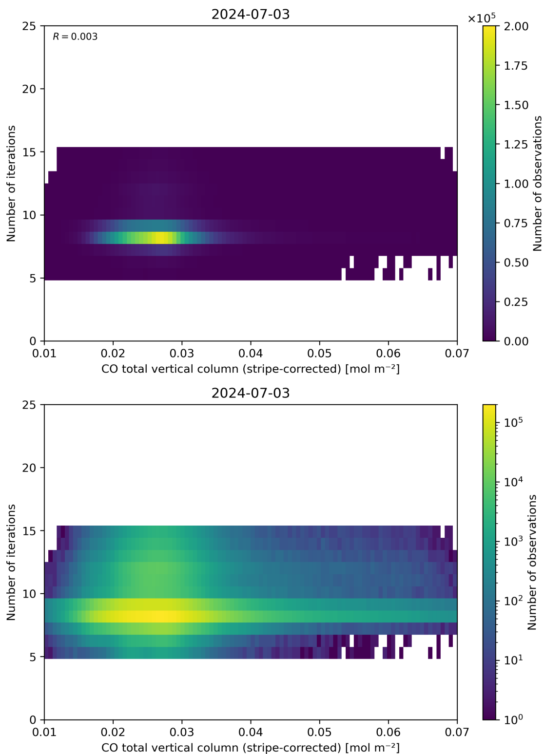
Figure 39: Scatter density plot of “CO total vertical column (stripe-corrected)” against “Number of iterations” for 2024-07-02 to 2024-07-04.
