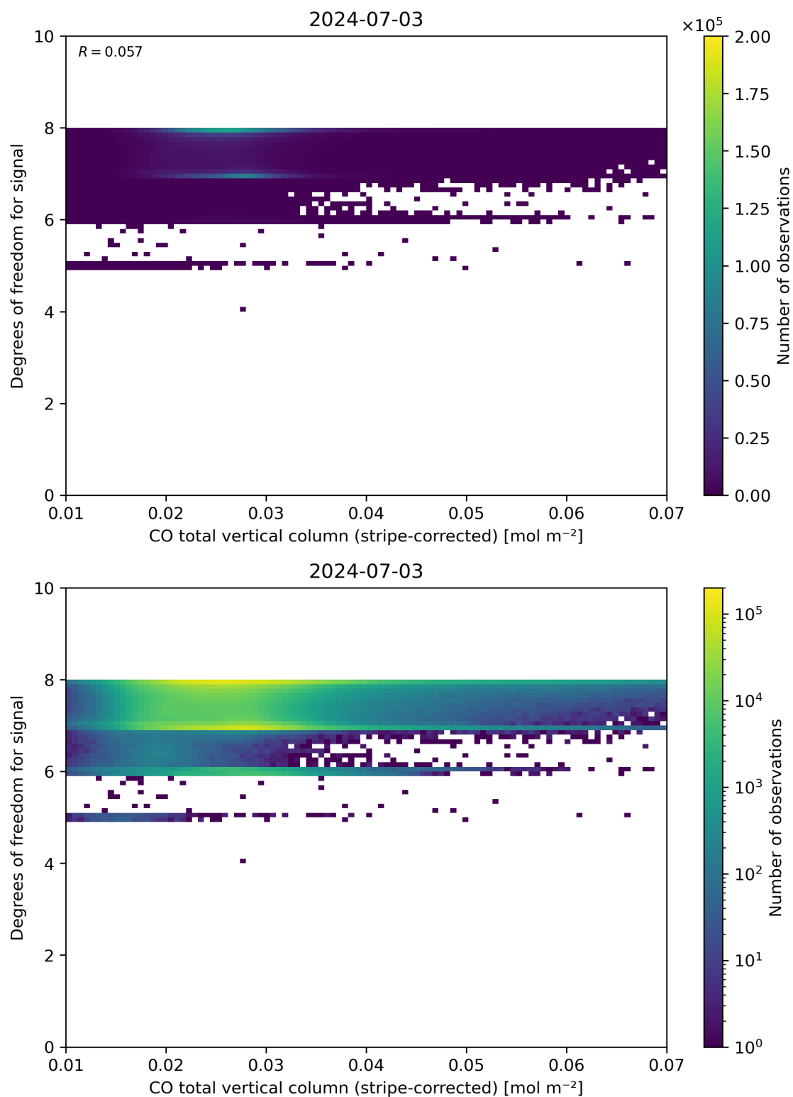
Figure 38: Scatter density plot of “CO total vertical column (stripe-corrected)” against “Degrees of freedom for signal” for 2024-07-02 to 2024-07-04.
