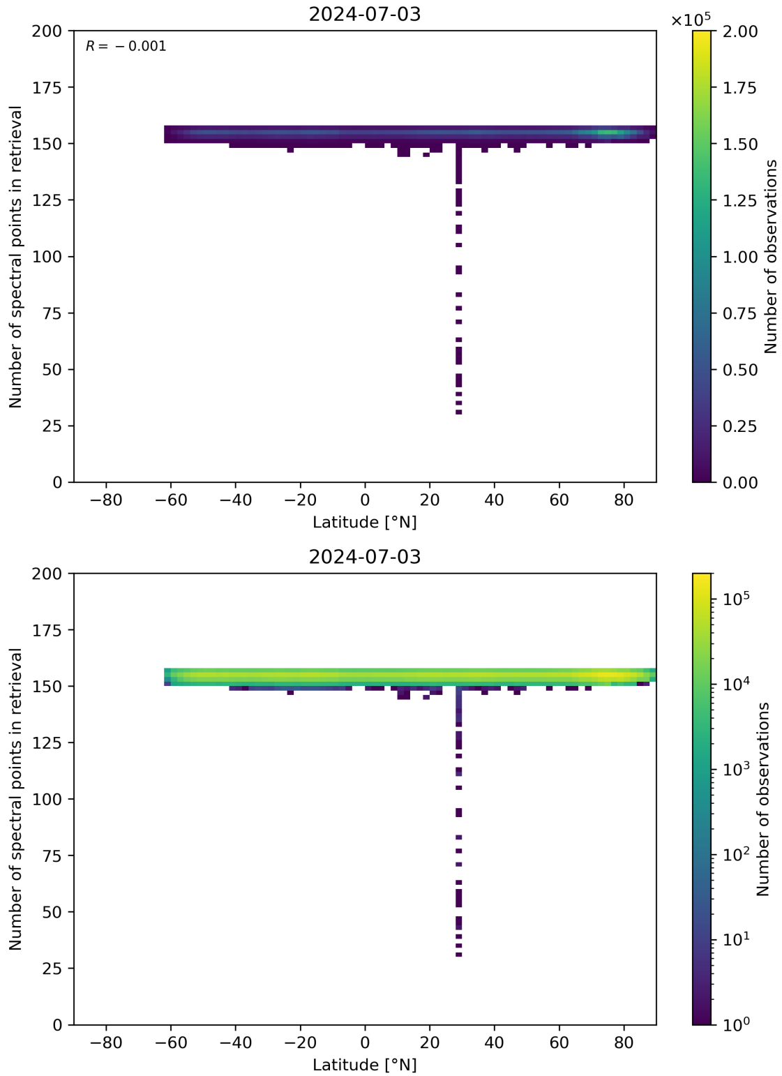
Figure 57: Scatter density plot of “Latitude” against “Number of spectral points in retrieval” for 2024-07-02 to 2024-07-04.
