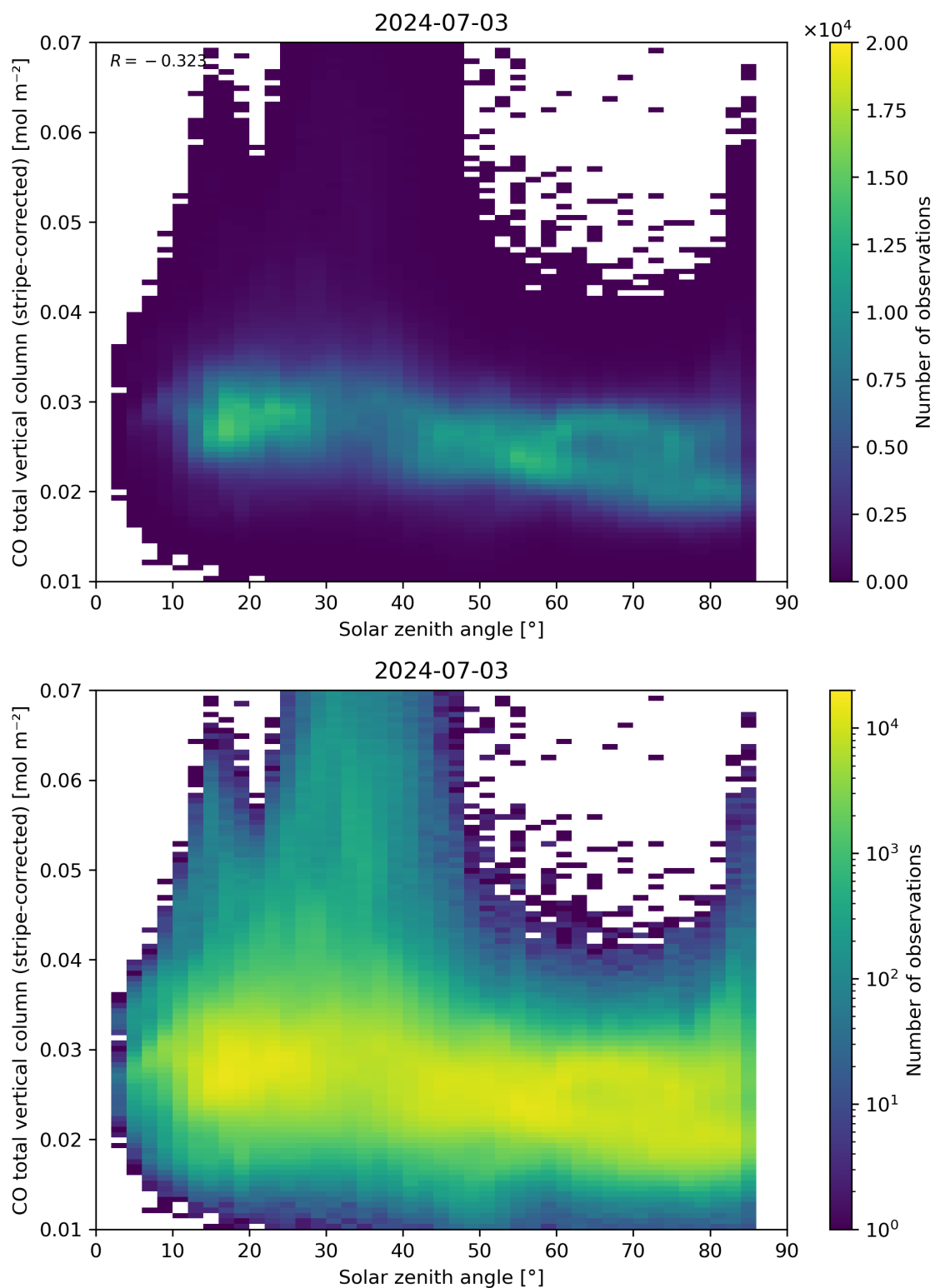
Figure 62: Scatter density plot of “Solar zenith angle” against “CO total vertical column (stripe-corrected)” for 2024-07-02 to 2024-07-04.
