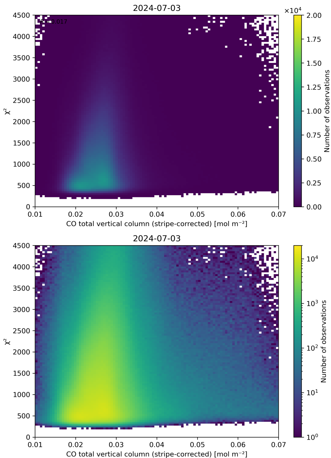
Figure 37: Scatter density plot of “CO total vertical column (stripe-corrected)” against “ \chi^2 ” for 2024-07-02 to 2024-07-04.
