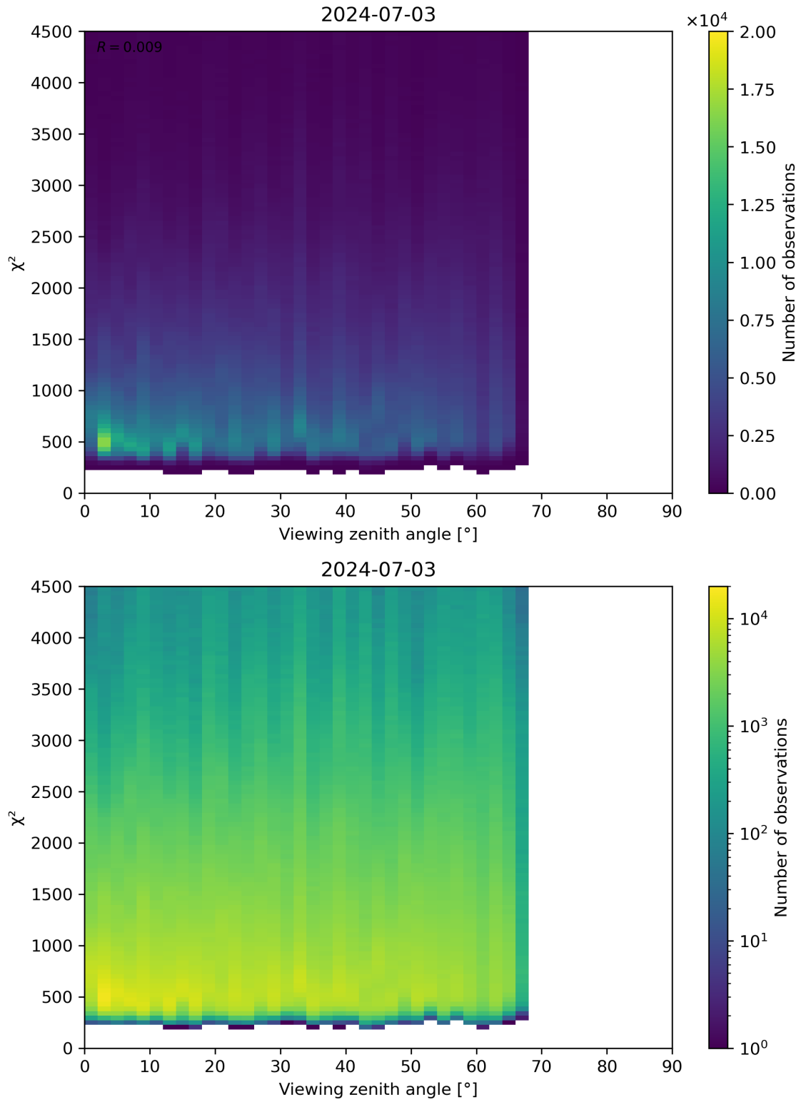
Figure 72: Scatter density plot of “Viewing zenith angle” against “ \chi^2 ” for 2024-07-02 to 2024-07-04.
