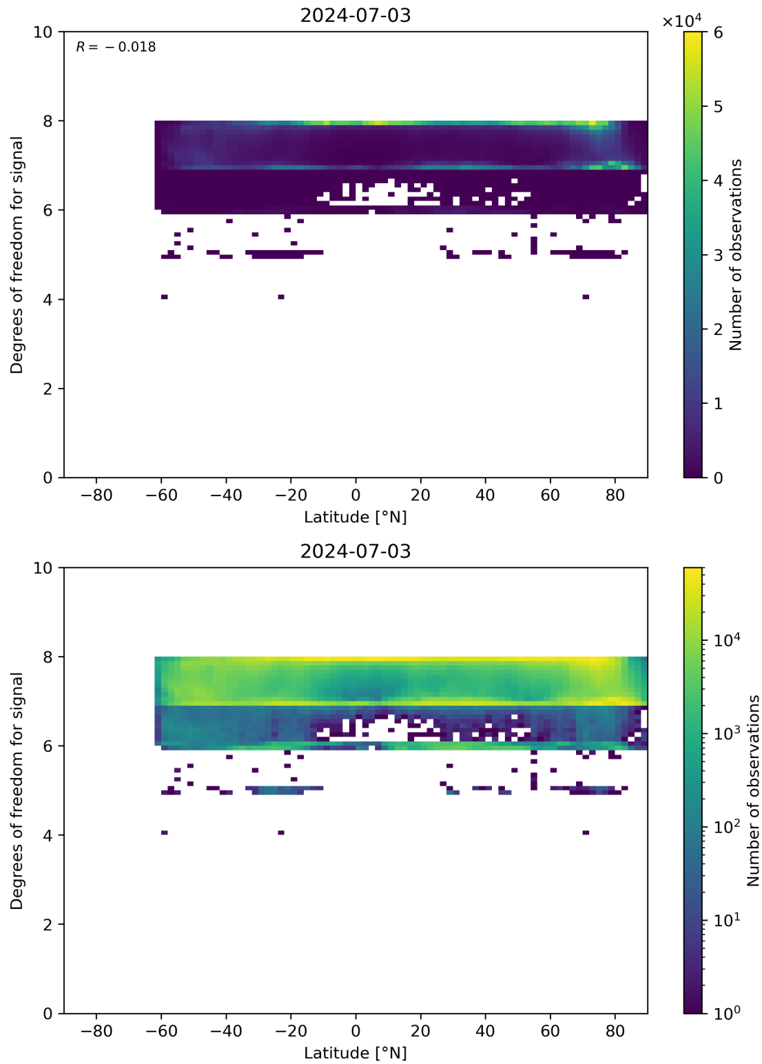
Figure 55: Scatter density plot of “Latitude” against “Degrees of freedom for signal” for 2024-07-02 to 2024-07-04.
