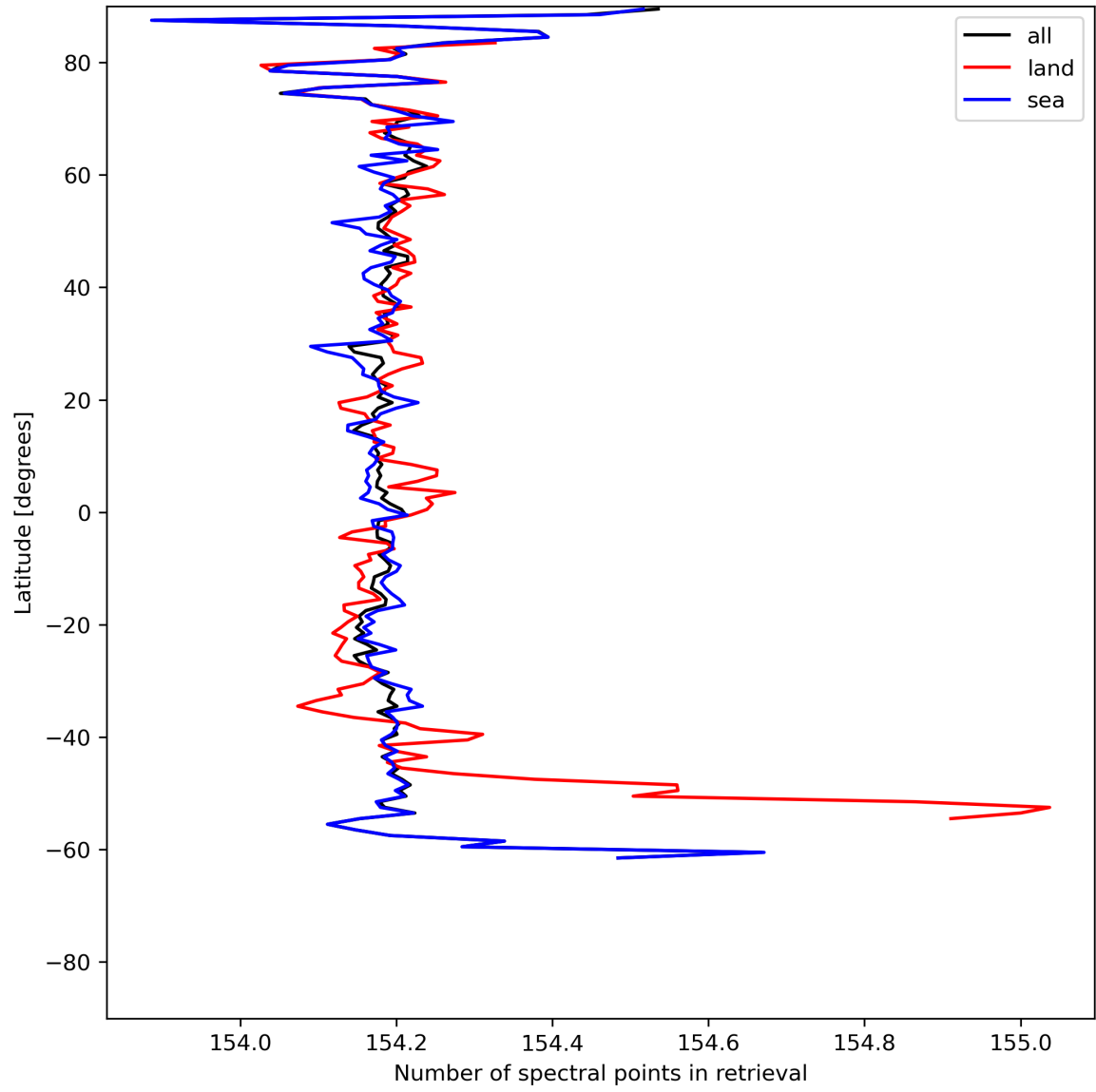
Figure 13: Zonal average of “Number of spectral points in retrieval” for 2024-07-02 to 2024-07-04.
