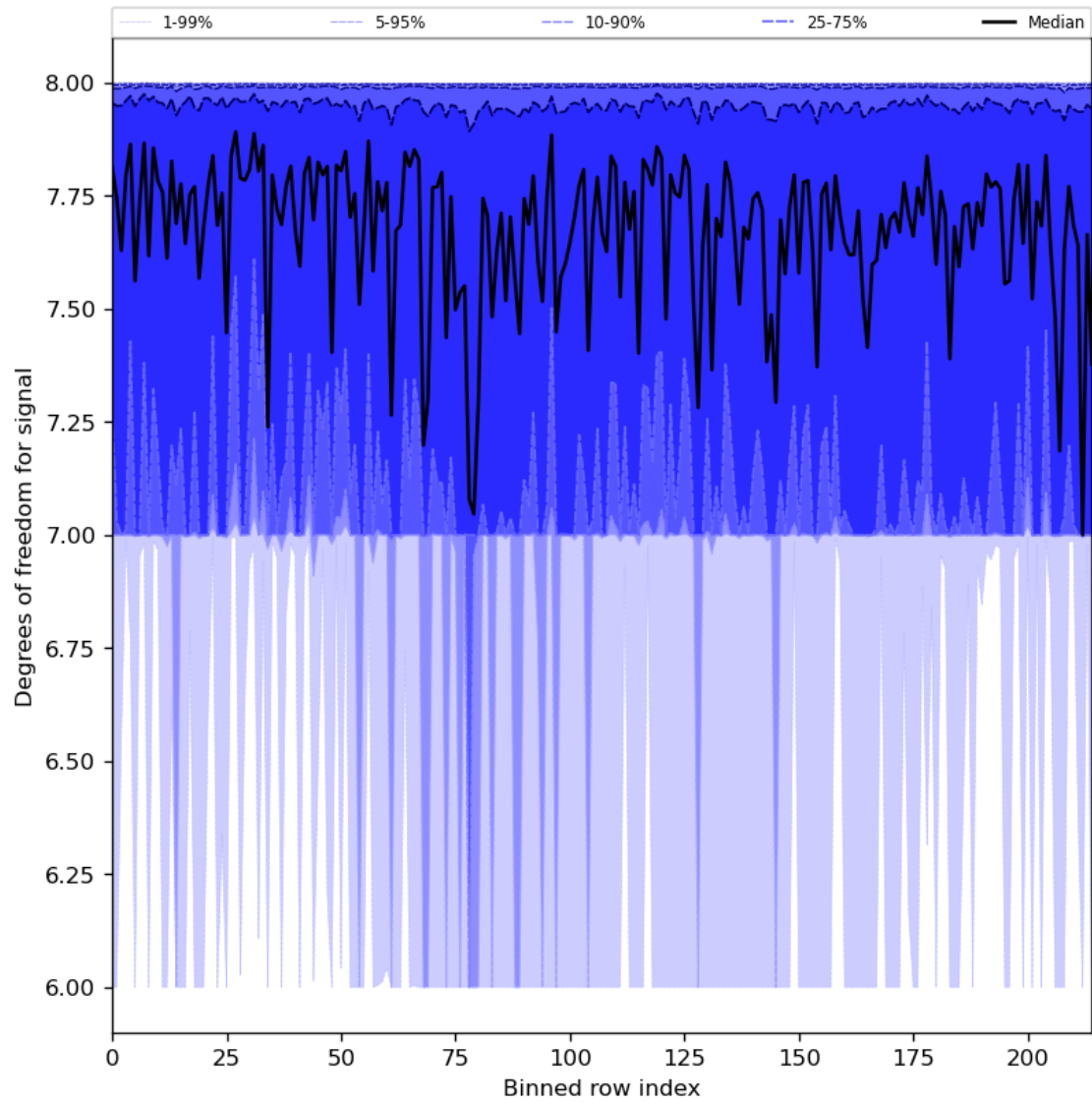
Figure 31: Along track statistics of “Degrees of freedom for signal” for 2024-07-02 to 2024-07-04
