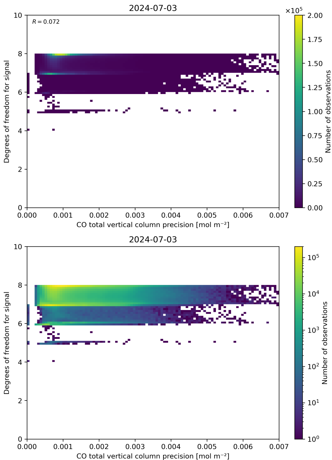
Figure 45: Scatter density plot of “CO total vertical column precision” against “Degrees of freedom for signal” for 2024-07-02 to 2024-07-04.
