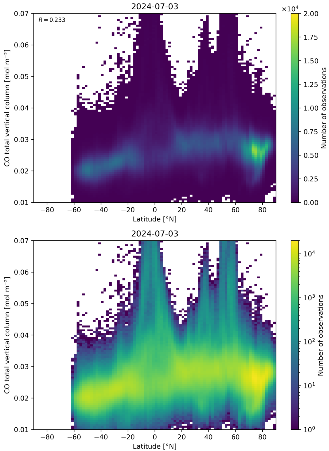
Figure 51: Scatter density plot of “Latitude” against “CO total vertical column” for 2024-07-02 to 2024-07-04.
