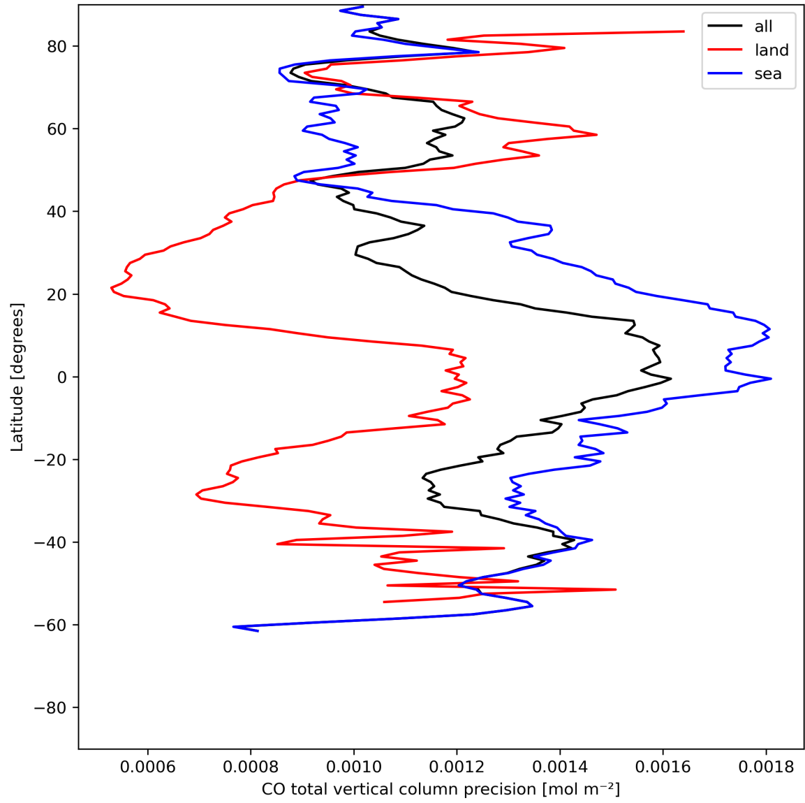
Figure 12: Zonal average of “CO total vertical column precision” for 2024-07-02 to 2024-07-04.
