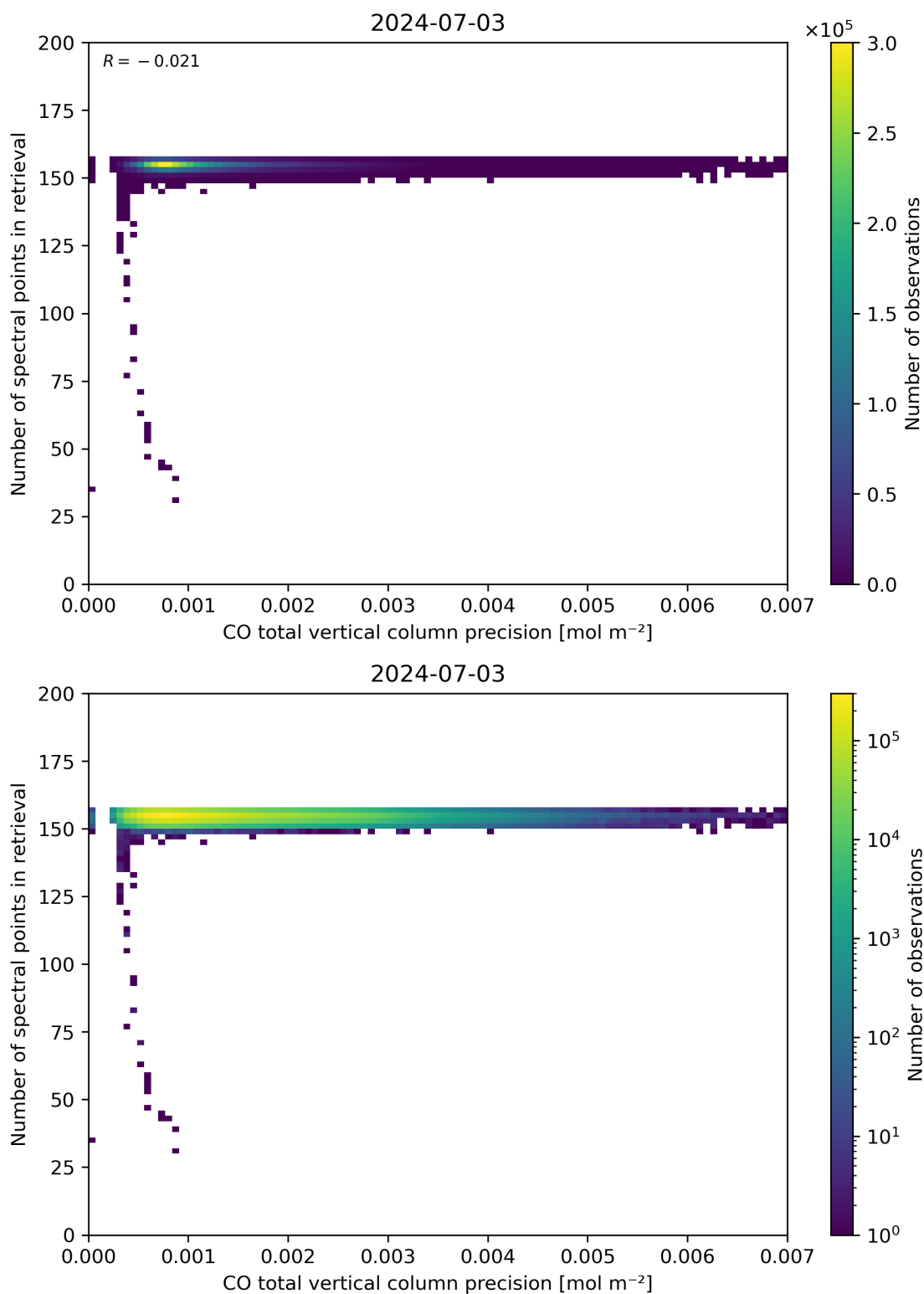
Figure 47: Scatter density plot of “CO total vertical column precision” against “Number of spectral points in retrieval” for 2024-07-02 to 2024-07-04.
