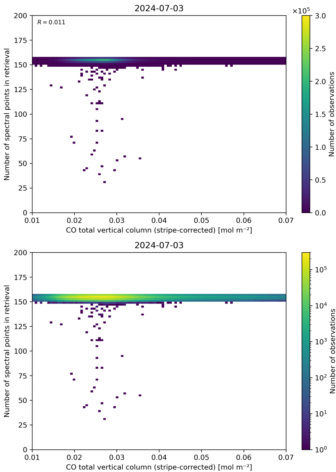
Figure 40: Scatter density plot of “CO total vertical column (stripe-corrected)” against “Number of spectral points in retrieval” for 2024-07-02 to 2024-07-04.
