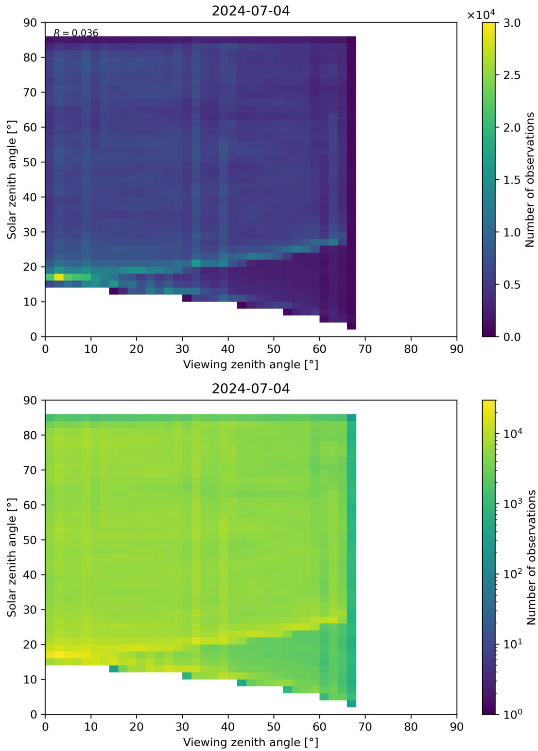
Figure 77: Scatter density plot of “Viewing zenith angle” against “Solar zenith angle” for 2024-07-03 to 2024-07-05.
