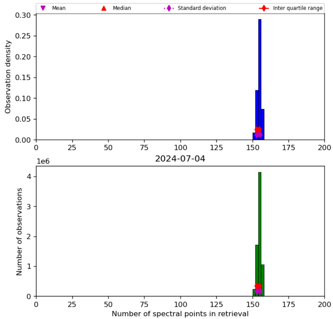
Figure 21: Histogram of “Number of spectral points in retrieval” for 2024-07-03 to 2024-07-05
