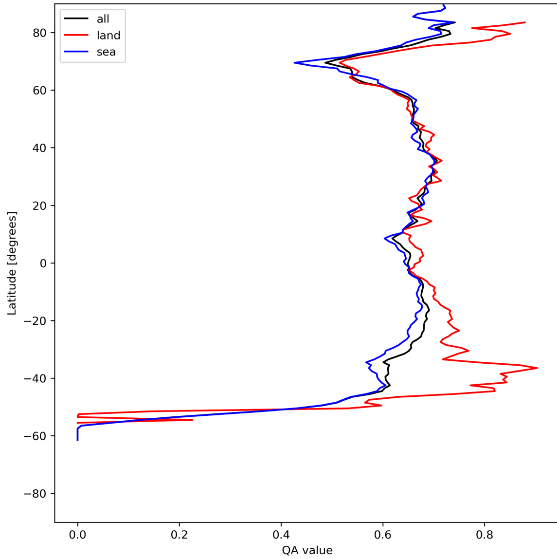
Figure 9: Zonal average of “QA value” for 2024-07-03 to 2024-07-05.
