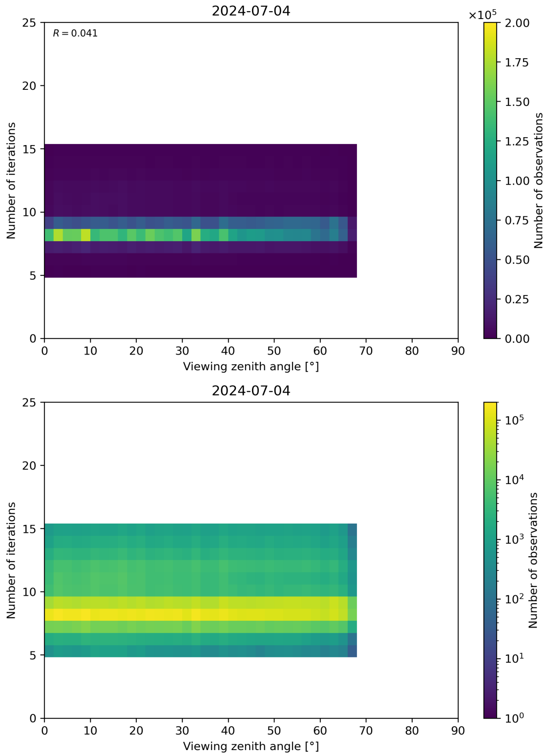
Figure 75: Scatter density plot of “Viewing zenith angle” against “Number of iterations” for 2024-07-03 to 2024-07-05.
