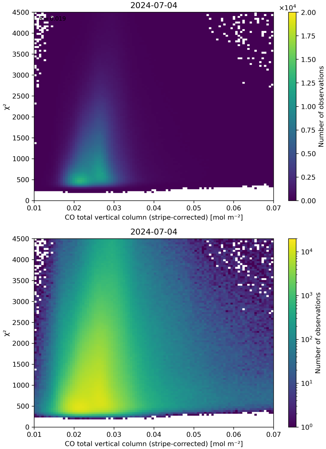
Figure 37: Scatter density plot of “CO total vertical column (stripe-corrected)” against “ \chi^2 ” for 2024-07-03 to 2024-07-05.
