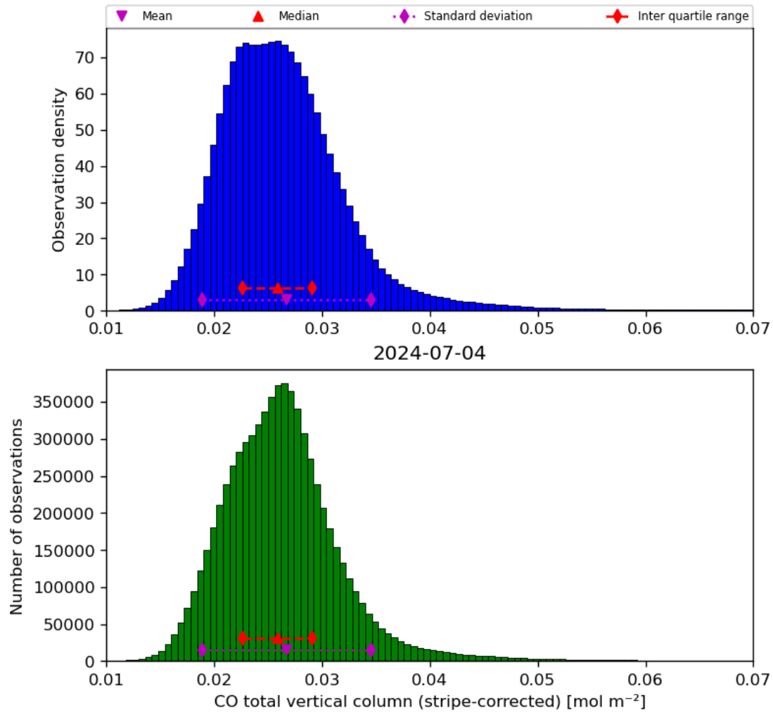
Figure 19: Histogram of “CO total vertical column (stripe-corrected)” for 2024-07-03 to 2024-07-05
