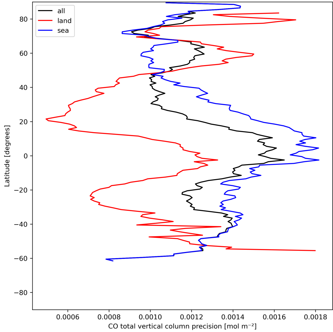
Figure 12: Zonal average of “CO total vertical column precision” for 2024-07-03 to 2024-07-05.
