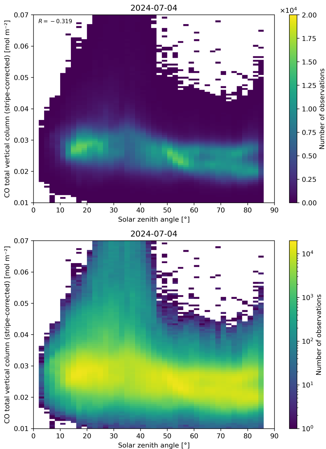
Figure 62: Scatter density plot of “Solar zenith angle” against “CO total vertical column (stripe-corrected)” for 2024-07-03 to 2024-07-05.
