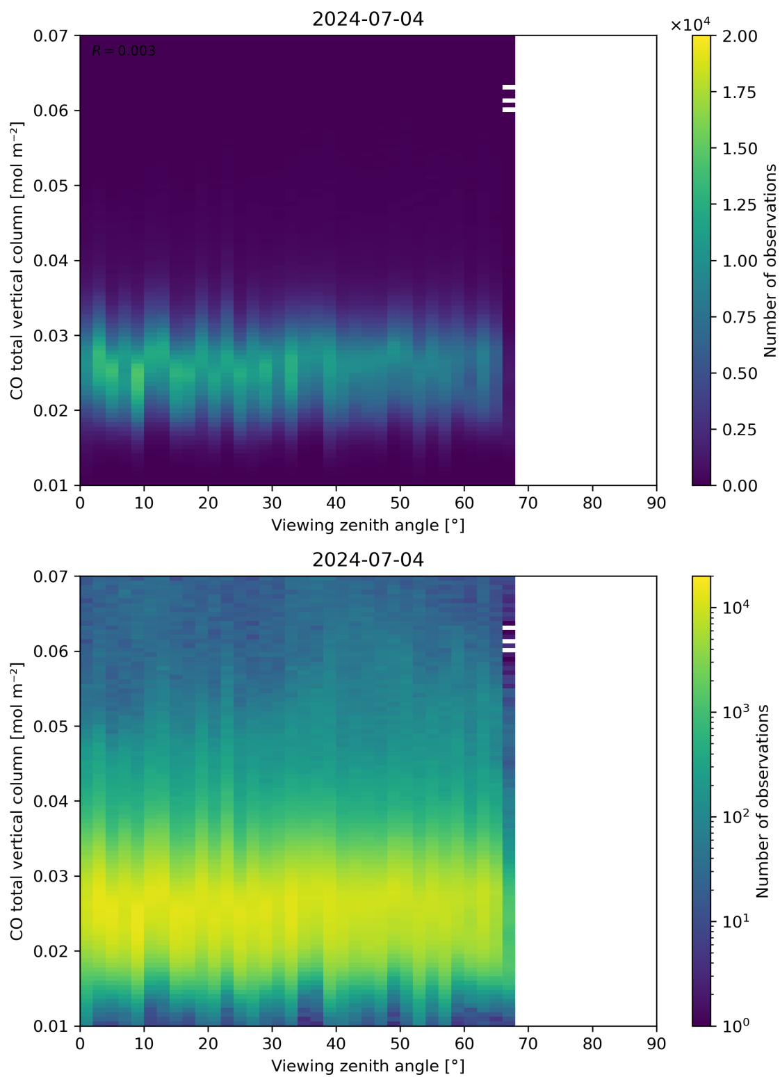
Figure 69: Scatter density plot of “Viewing zenith angle” against “CO total vertical column” for 2024-07-03 to 2024-07-05.
