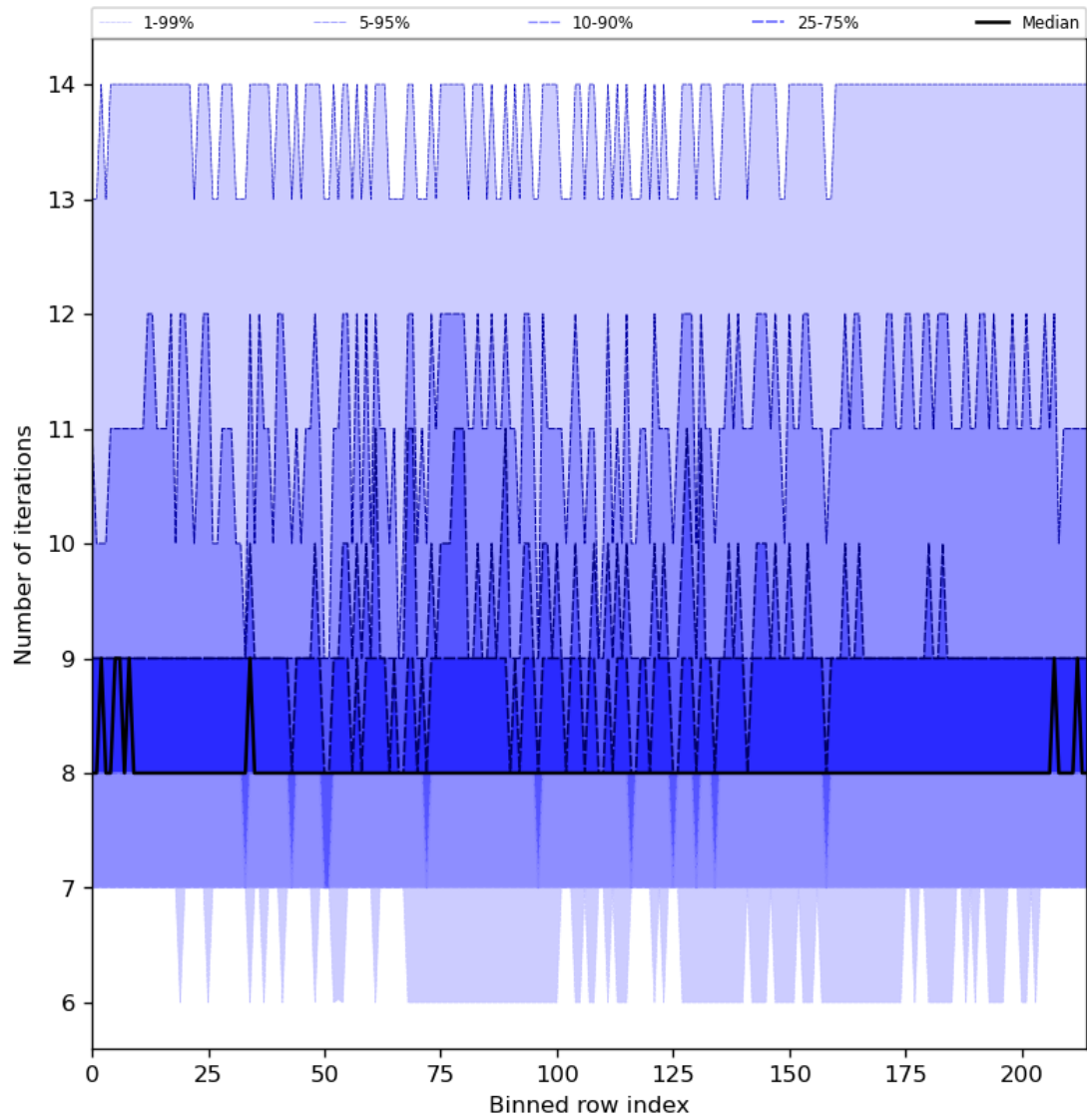
Figure 32: Along track statistics of “Number of iterations” for 2024-07-03 to 2024-07-05
