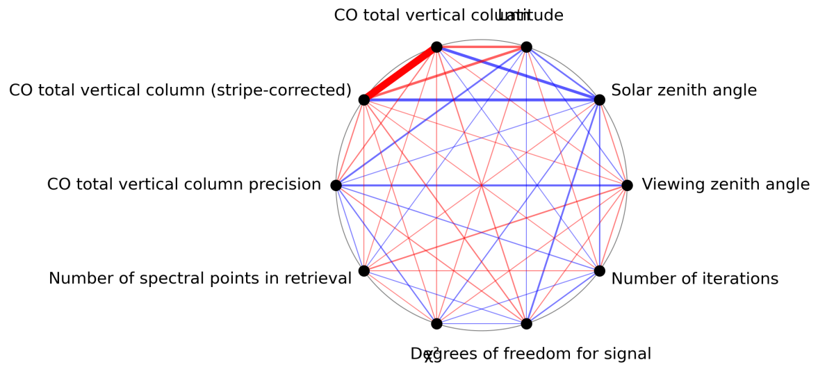
Figure 1: Map of correlation graph for 2024-07-03 to 2024-07-05.
