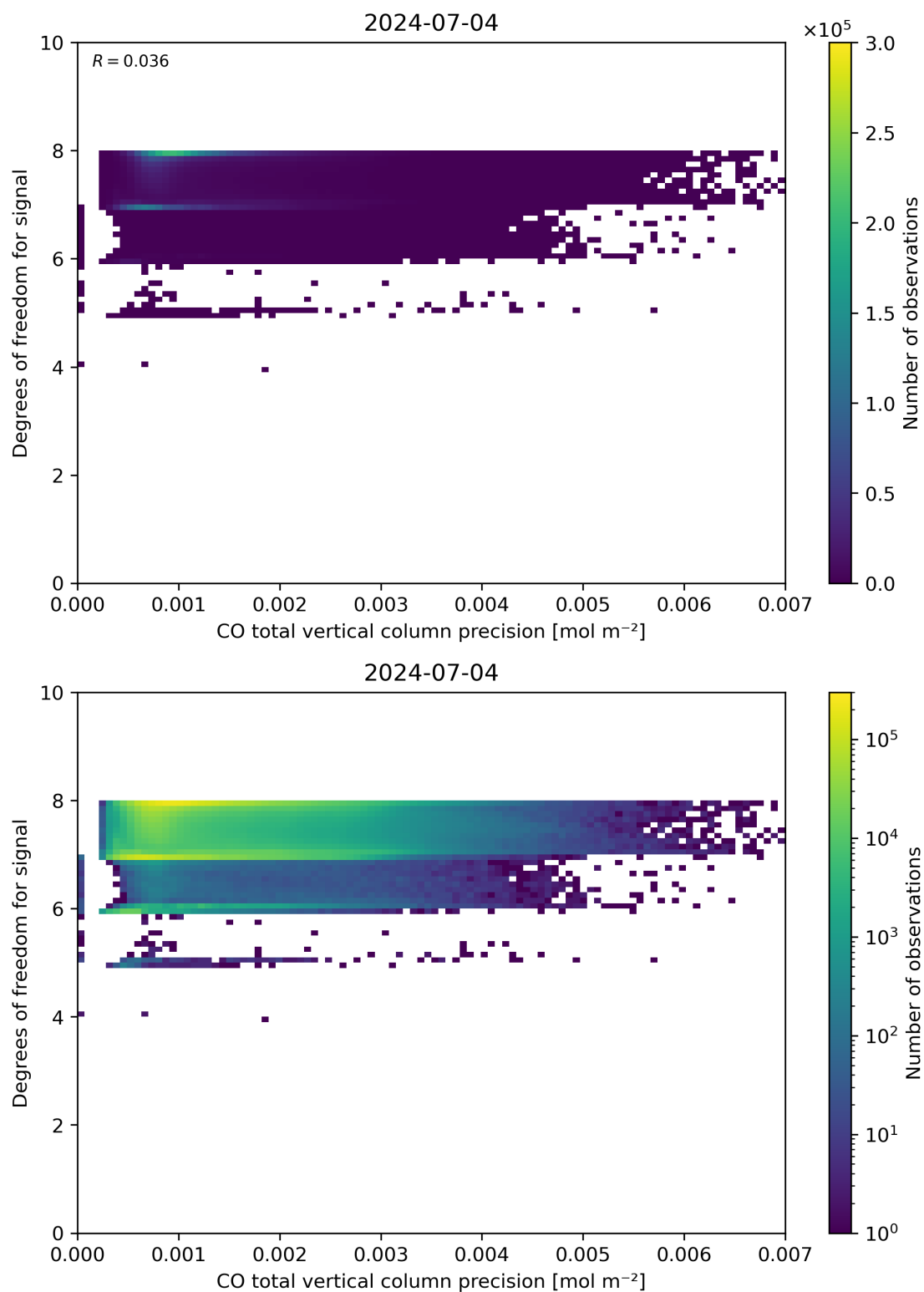
Figure 45: Scatter density plot of “CO total vertical column precision” against “Degrees of freedom for signal” for 2024-07-03 to 2024-07-05.
