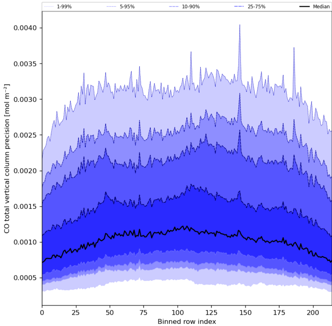
Figure 28: Along track statistics of "CO total vertical column precision" for 2024-07-03 to 2024-07-05
