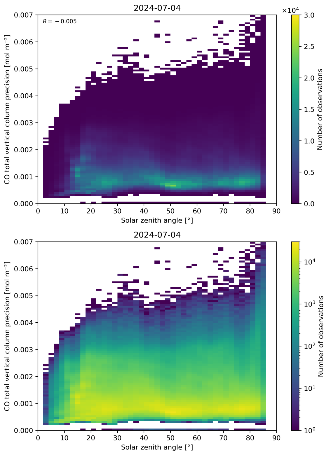
Figure 63: Scatter density plot of “Solar zenith angle” against “CO total vertical column precision” for 2024-07-03 to 2024-07-05.
