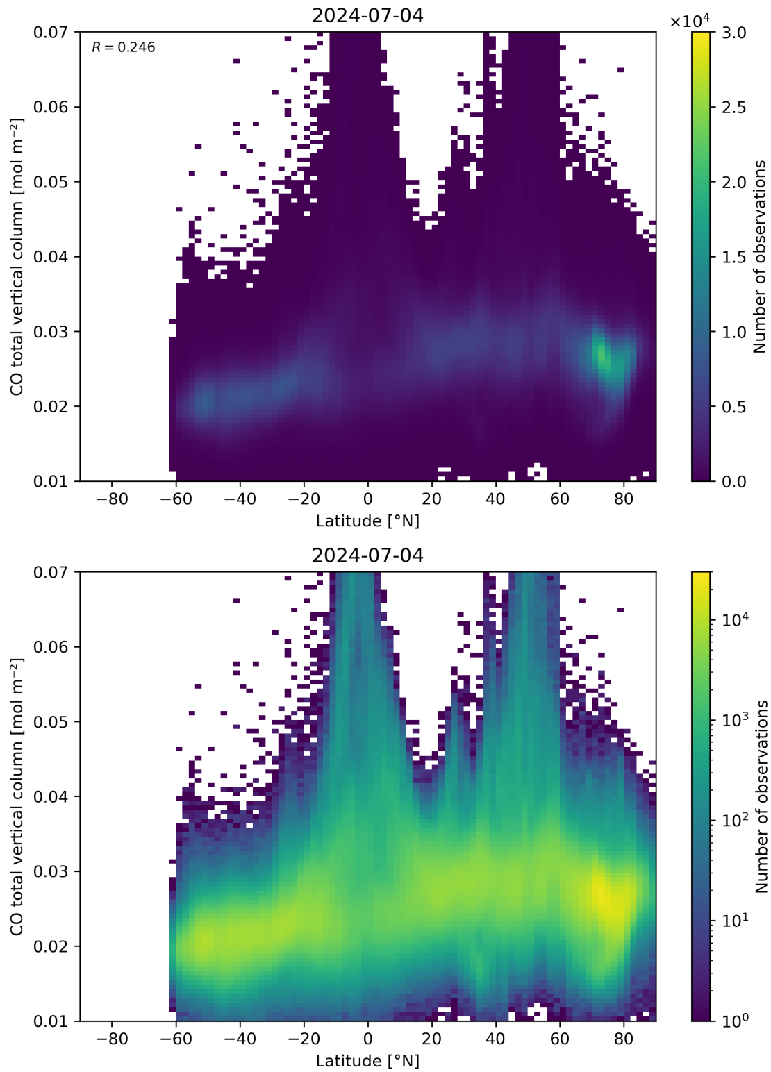
Figure 51: Scatter density plot of “Latitude” against “CO total vertical column” for 2024-07-03 to 2024-07-05.
