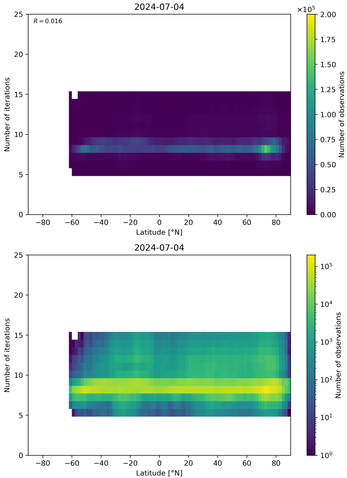
Figure 56: Scatter density plot of “Latitude” against “Number of iterations” for 2024-07-03 to 2024-07-05.
