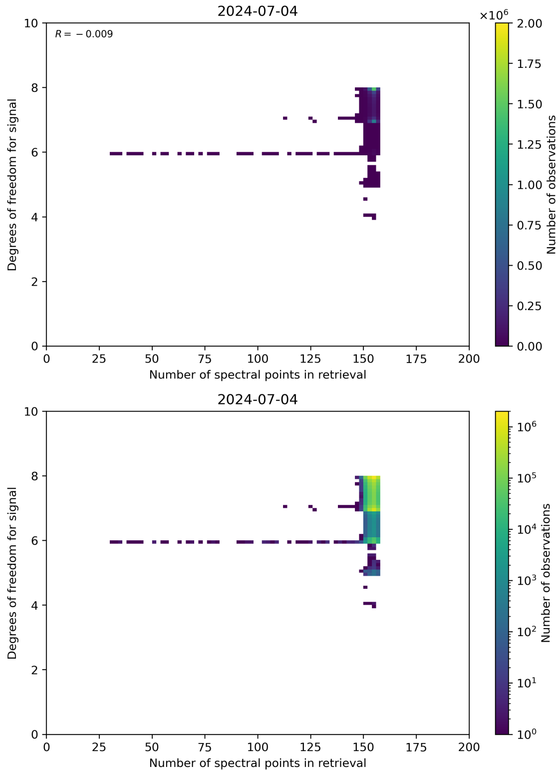
Figure 59: Scatter density plot of “Number of spectral points in retrieval” against “Degrees of freedom for signal” for 2024-07-03 to 2024-07-05.
