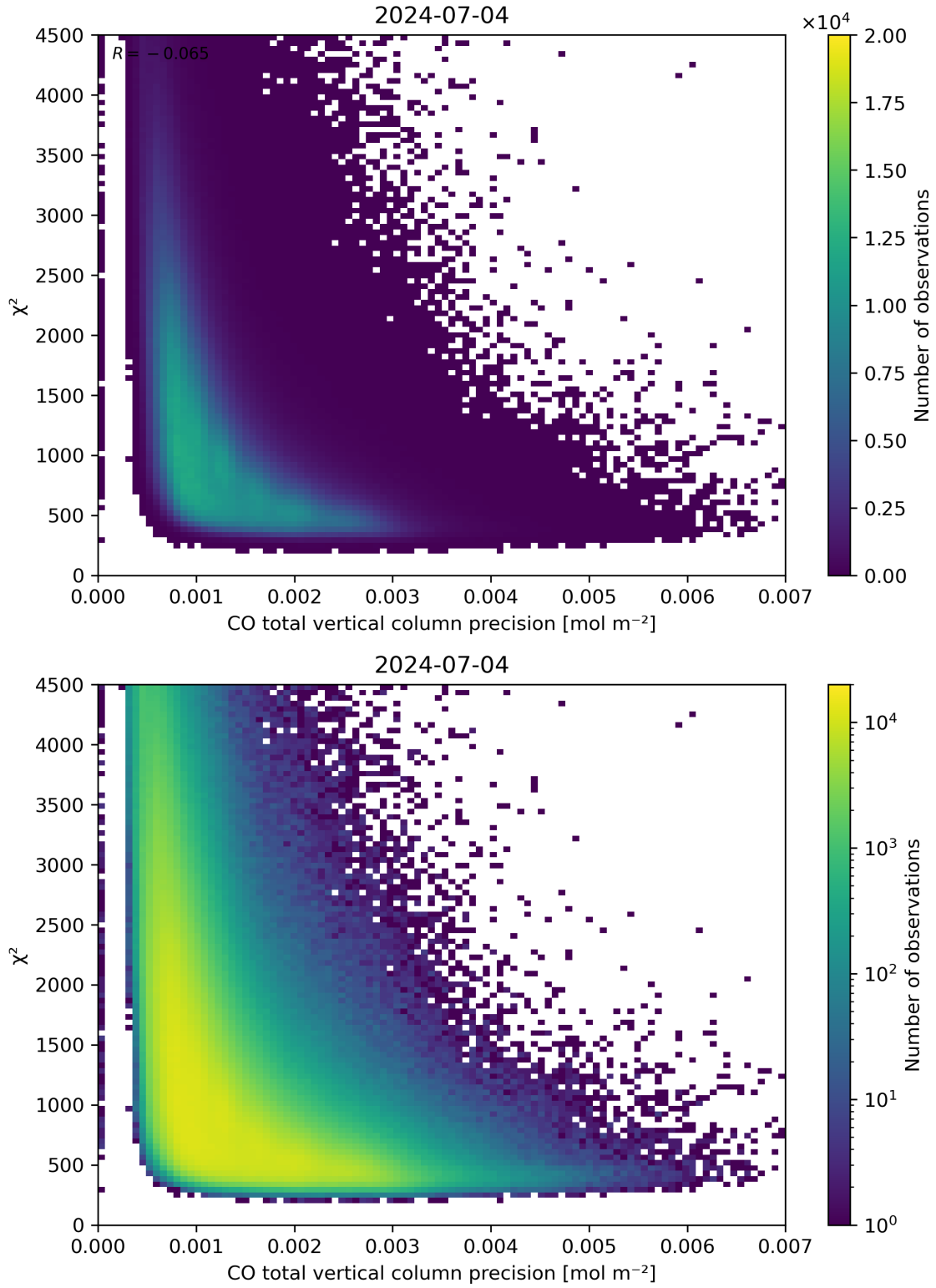
Figure 44: Scatter density plot of “CO total vertical column precision” against “ \chi^2 ” for 2024-07-03 to 2024-07-05.
