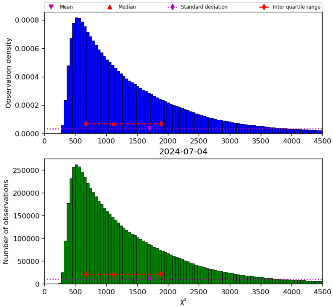
Figure 22: Histogram of “ \chi^2 ” for 2024-07-03 to 2024-07-05
