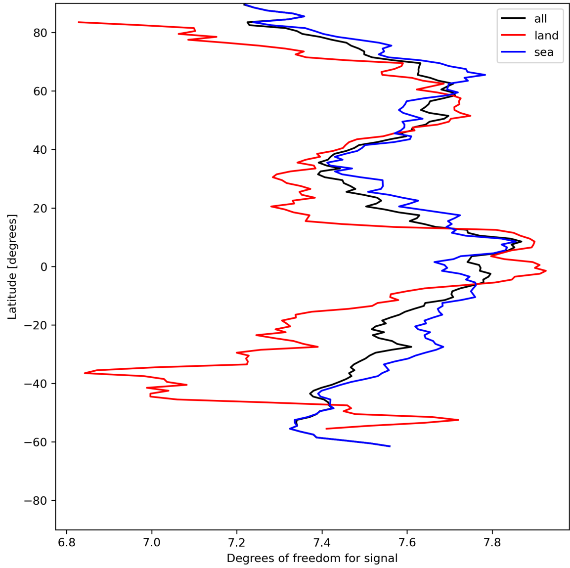
Figure 15: Zonal average of “Degrees of freedom for signal” for 2024-07-03 to 2024-07-05.
