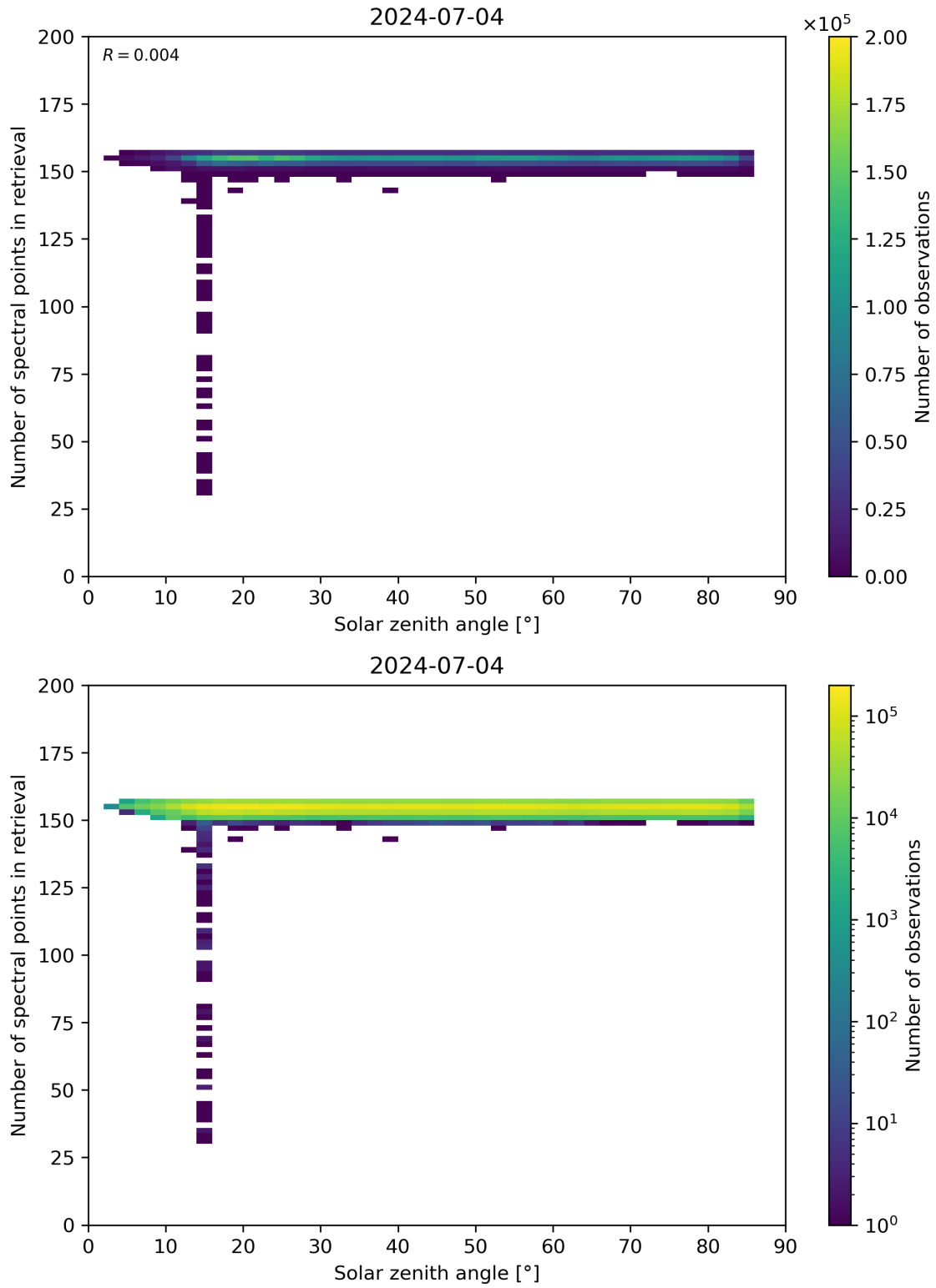
Figure 68: Scatter density plot of “Solar zenith angle” against “Number of spectral points in retrieval” for 2024-07-03 to 2024-07-05.
