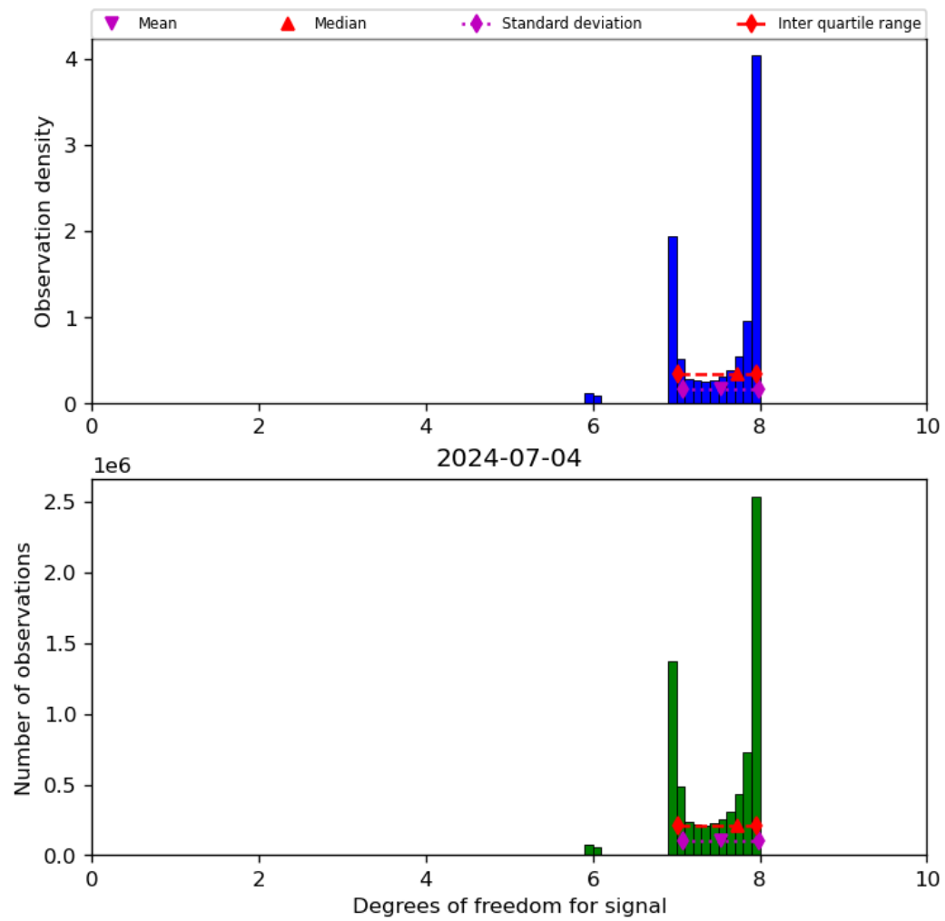
Figure 23: Histogram of “Degrees of freedom for signal” for 2024-07-03 to 2024-07-05
