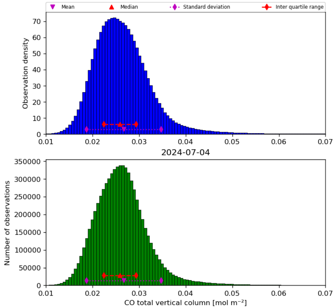
Figure 18: Histogram of “CO total vertical column” for 2024-07-03 to 2024-07-05
