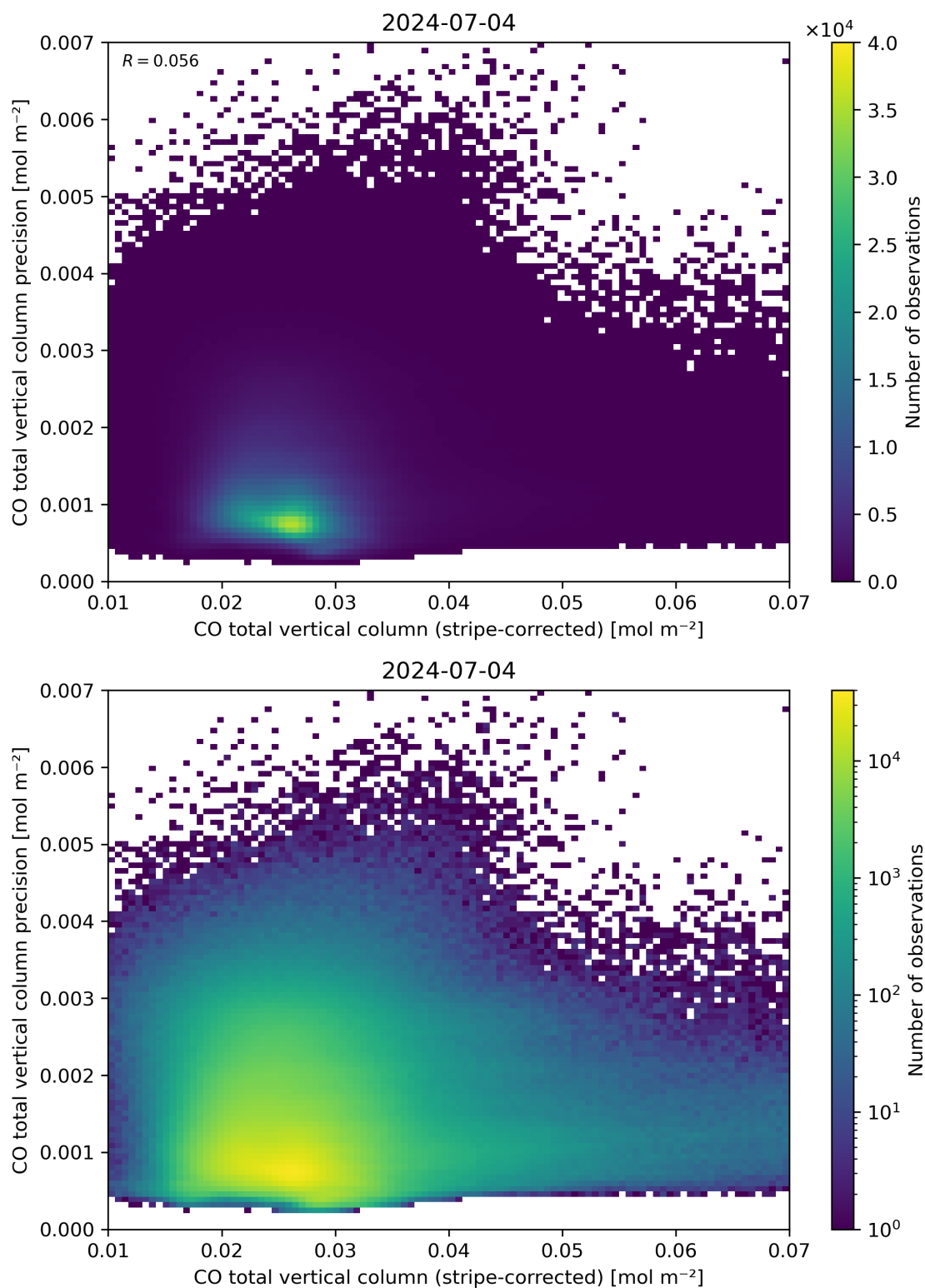
Figure 36: Scatter density plot of “CO total vertical column (stripe-corrected)” against “CO total vertical column precision” for 2024-07-03 to 2024-07-05.
