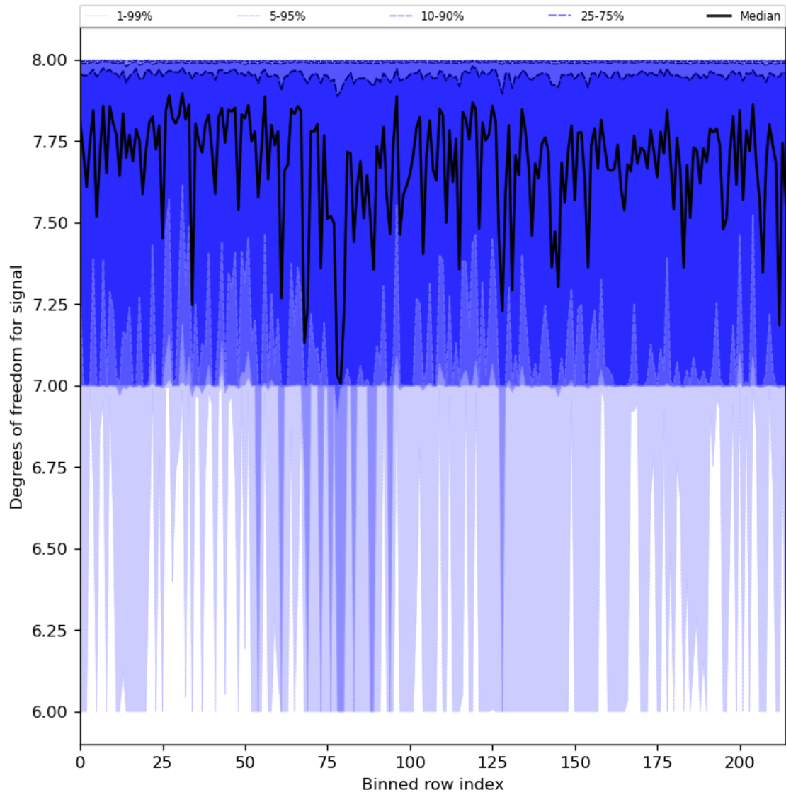
Figure 31: Along track statistics of “Degrees of freedom for signal” for 2024-07-03 to 2024-07-05
