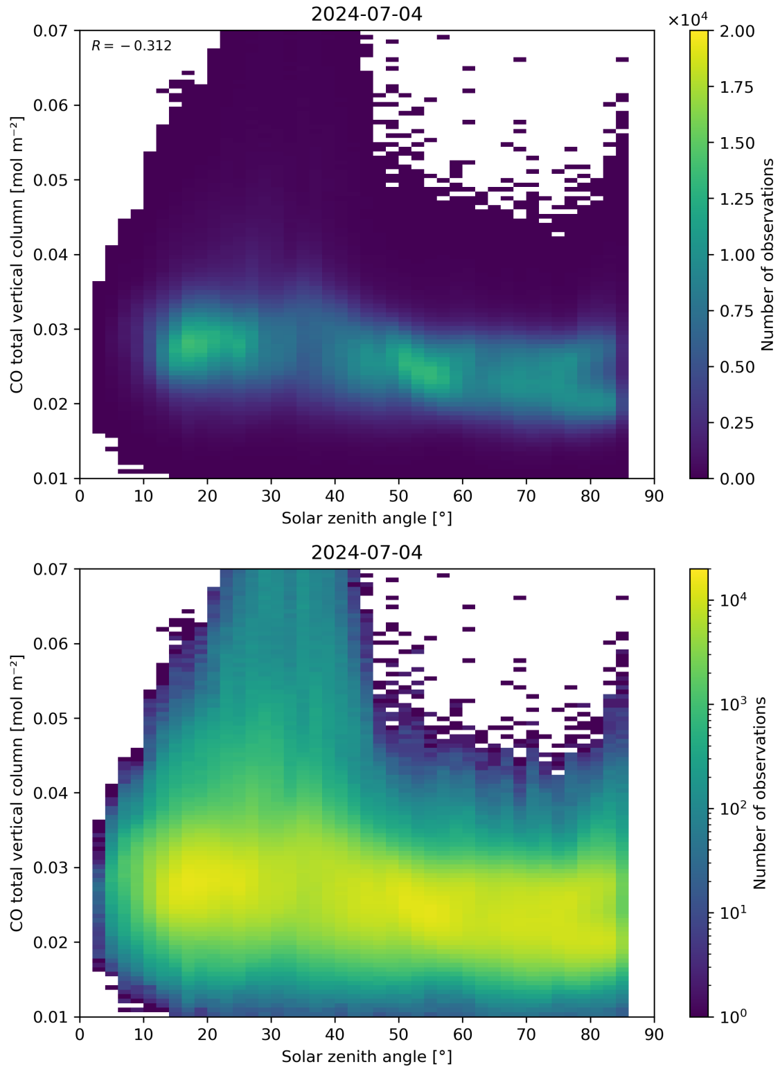
Figure 61: Scatter density plot of “Solar zenith angle” against “CO total vertical column” for 2024-07-03 to 2024-07-05.
