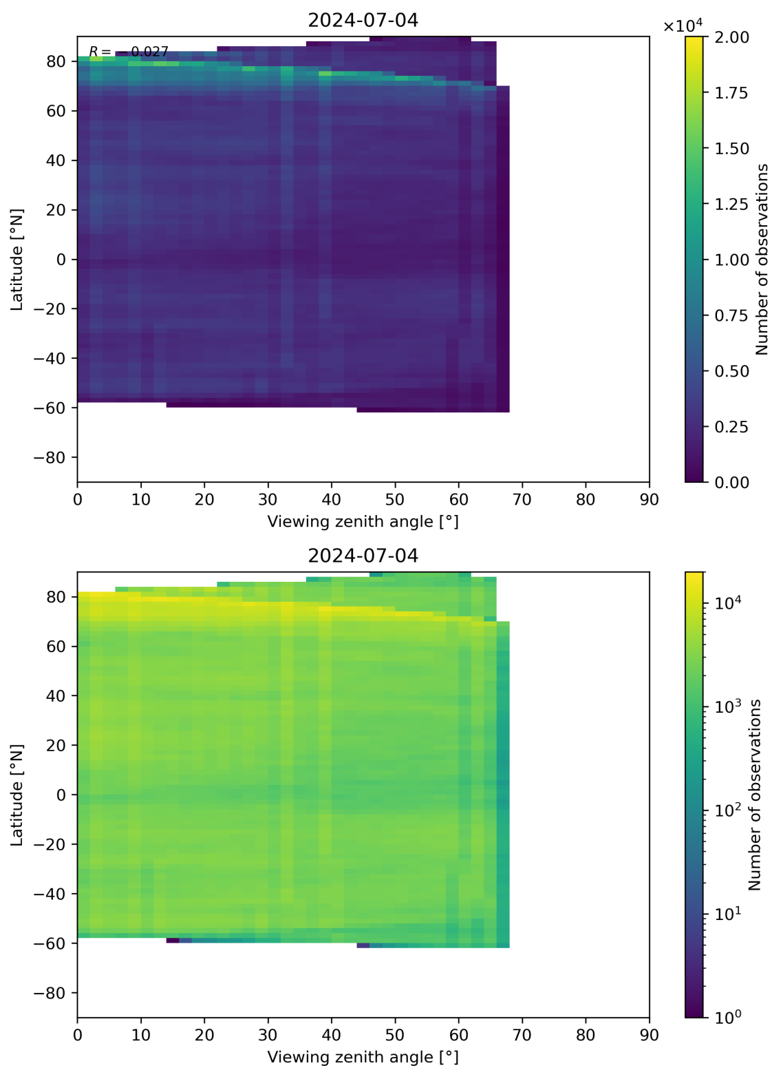
Figure 74: Scatter density plot of “Viewing zenith angle” against “Latitude” for 2024-07-03 to 2024-07-05.
