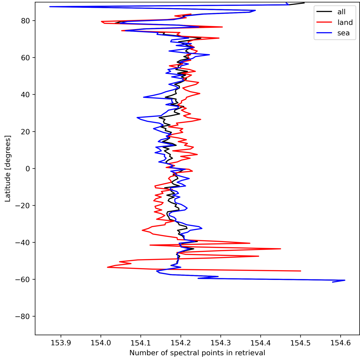
Figure 13: Zonal average of “Number of spectral points in retrieval” for 2024-07-03 to 2024-07-05.
