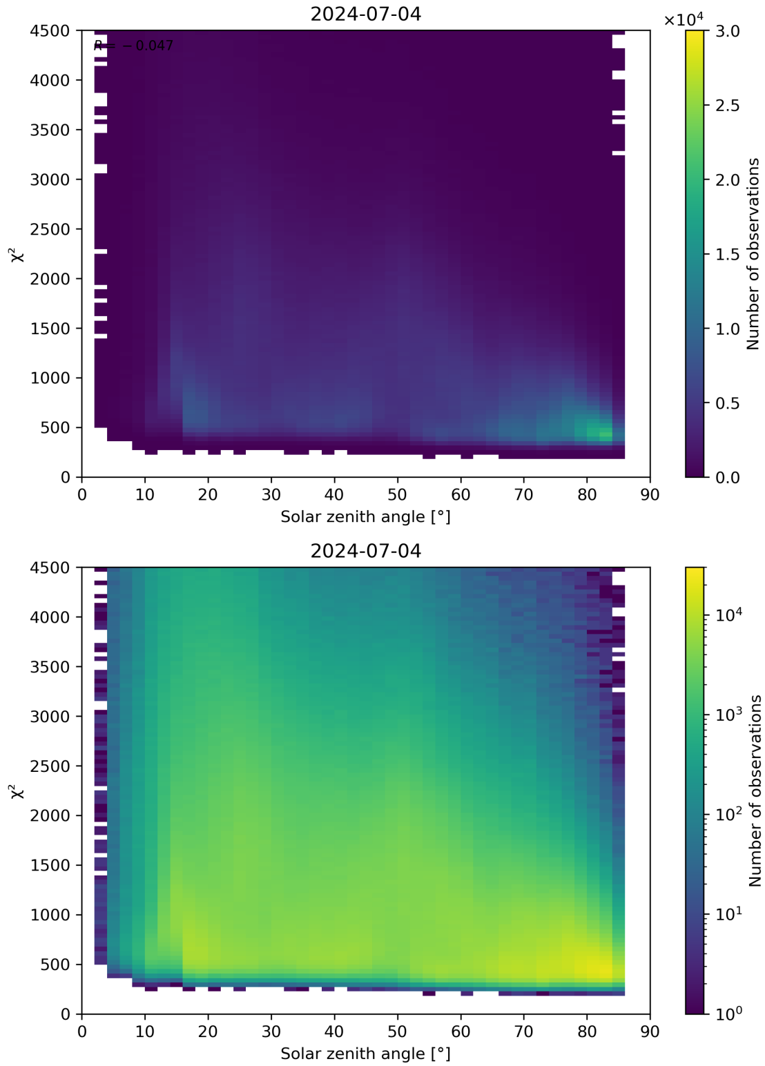
Figure 64: Scatter density plot of “Solar zenith angle” against “ \chi^2 ” for 2024-07-03 to 2024-07-05.
