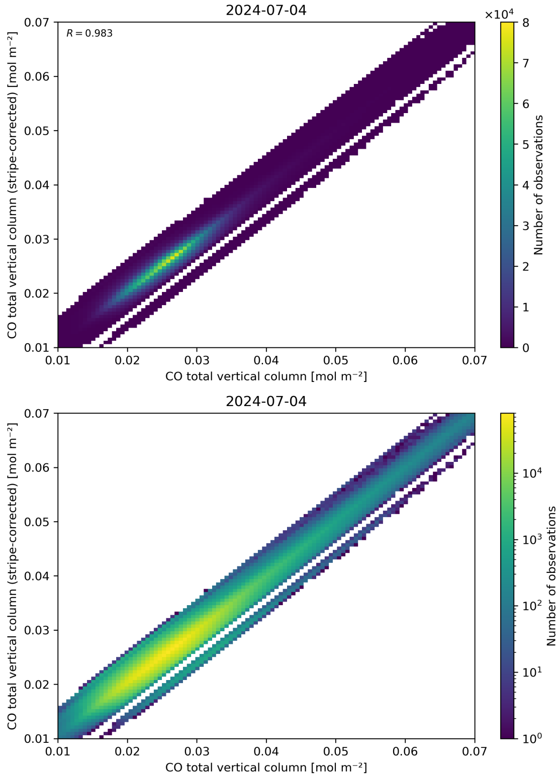
Figure 33: Scatter density plot of “CO total vertical column” against “CO total vertical column (stripe-corrected)” for 2024-07-03 to 2024-07-05.
