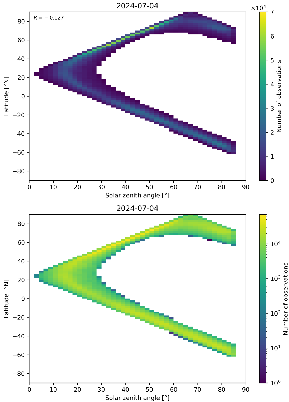
Figure 66: Scatter density plot of “Solar zenith angle” against “Latitude” for 2024-07-03 to 2024-07-05.
