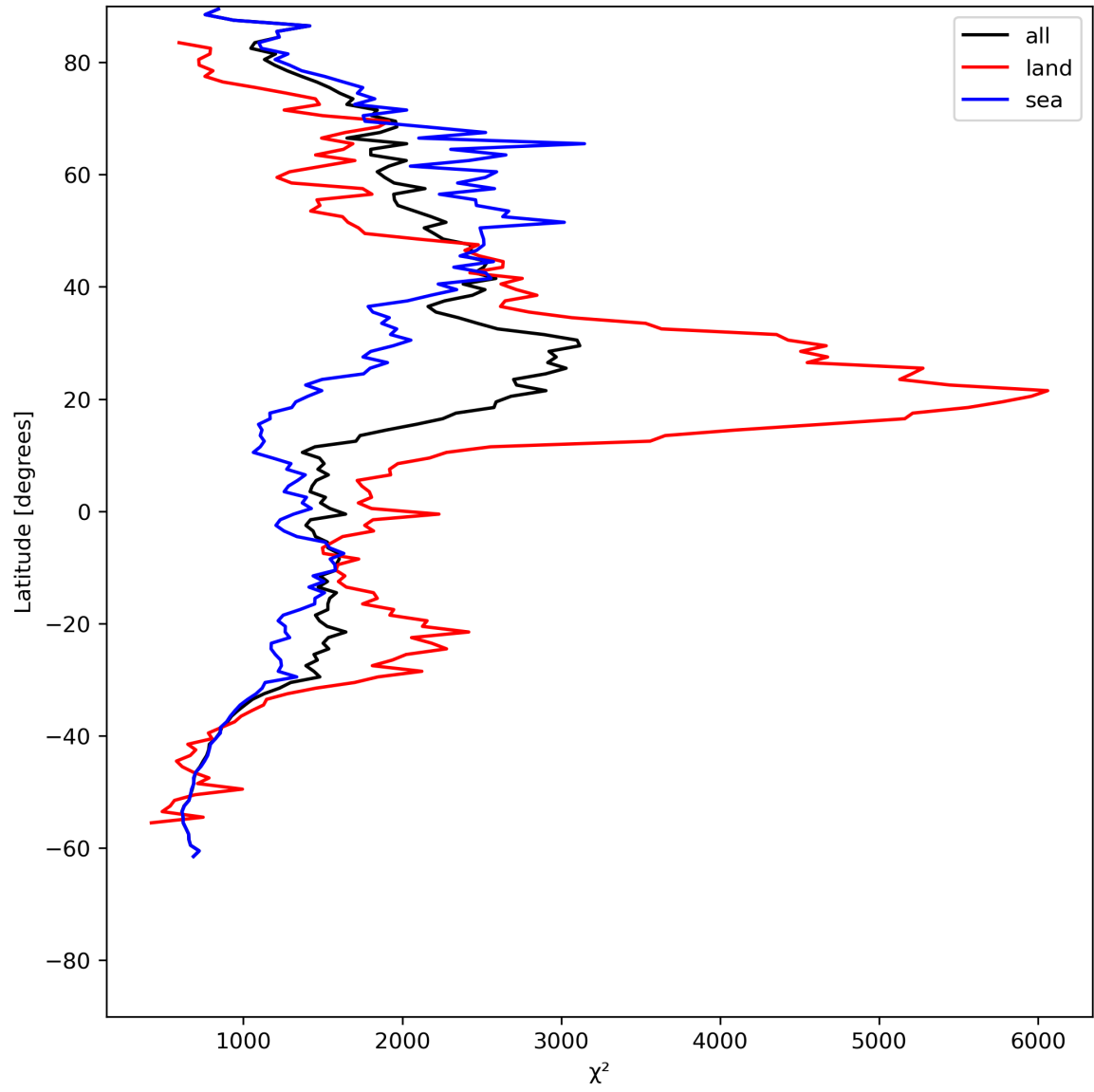
Figure 14: Zonal average of “ \chi^2 ” for 2024-07-03 to 2024-07-05.
