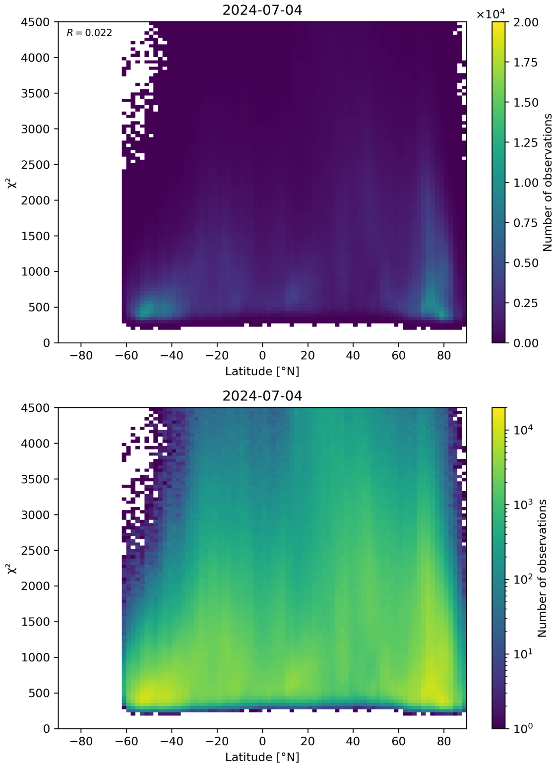
Figure 54: Scatter density plot of “Latitude” against “ \chi^2 ” for 2024-07-03 to 2024-07-05.
