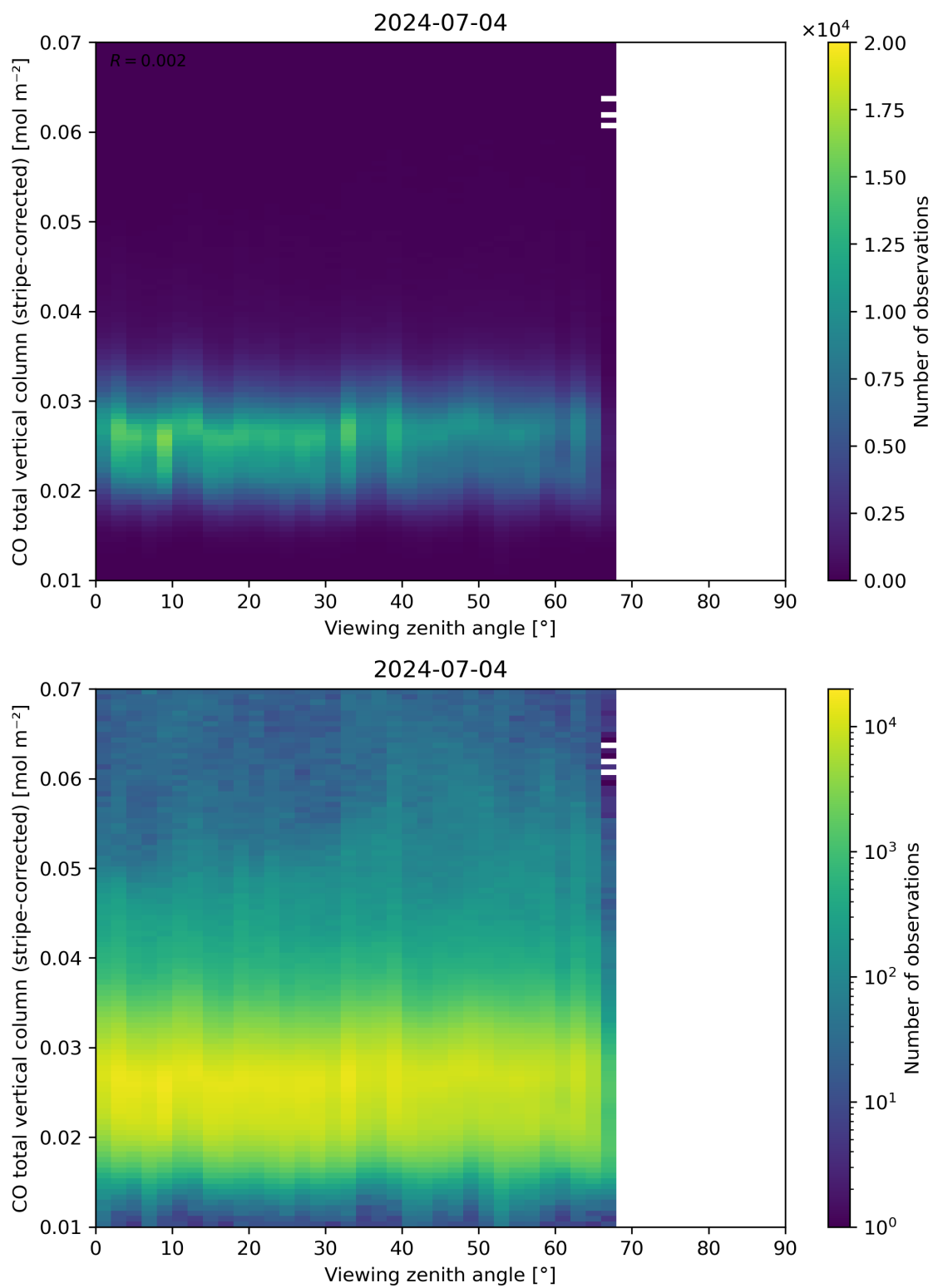
Figure 70: Scatter density plot of “Viewing zenith angle” against “CO total vertical column (stripe-corrected)” for 2024-07-03 to 2024-07-05.
