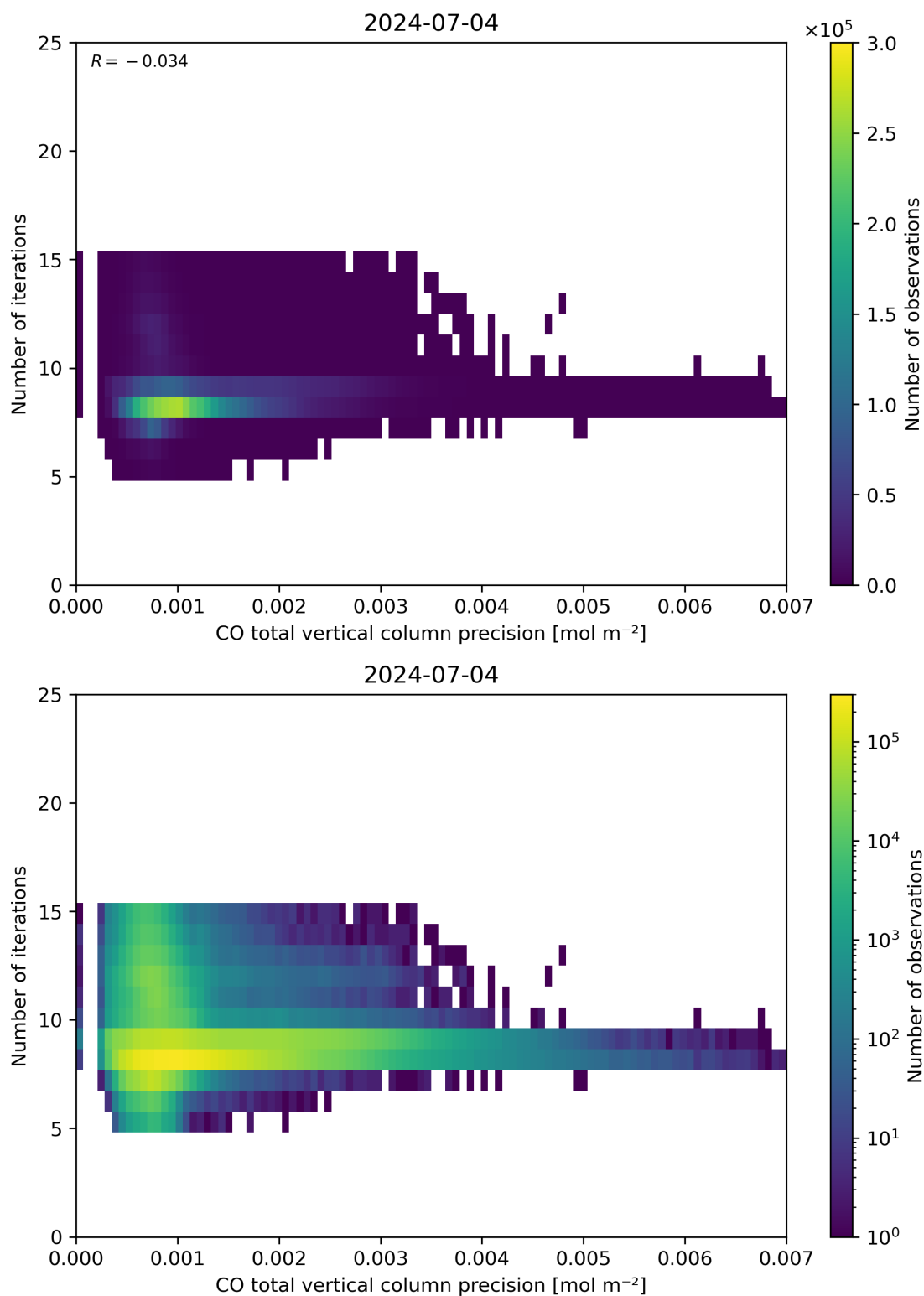
Figure 46: Scatter density plot of “CO total vertical column precision” against “Number of iterations” for 2024-07-03 to 2024-07-05.
