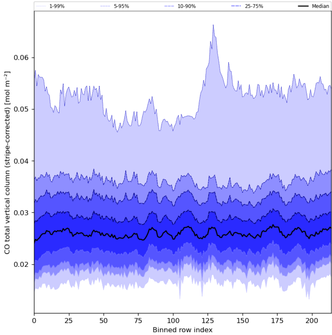
Figure 27: Along track statistics of “CO total vertical column (stripe-corrected)” for 2024-07-03 to 2024-07-05
