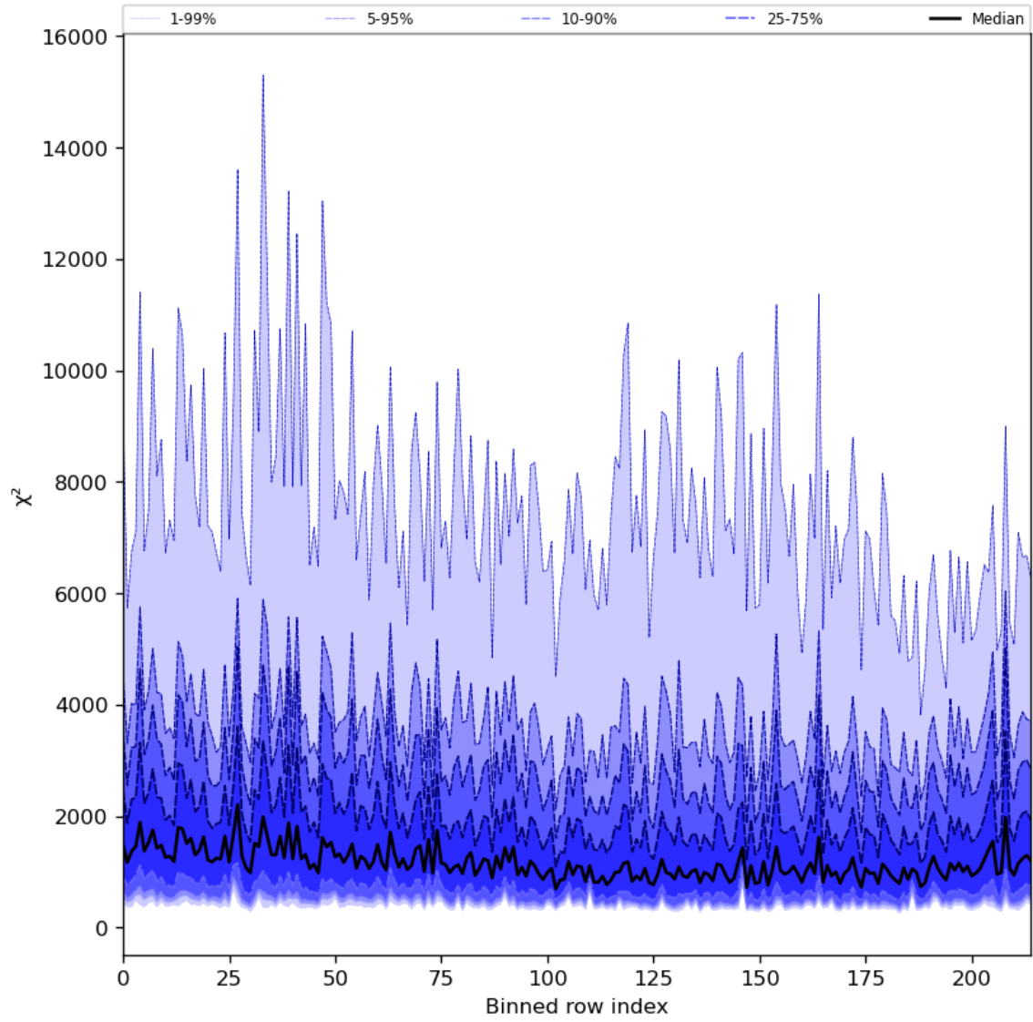
Figure 30: Along track statistics of “ \chi^2 ” for 2024-07-03 to 2024-07-05
