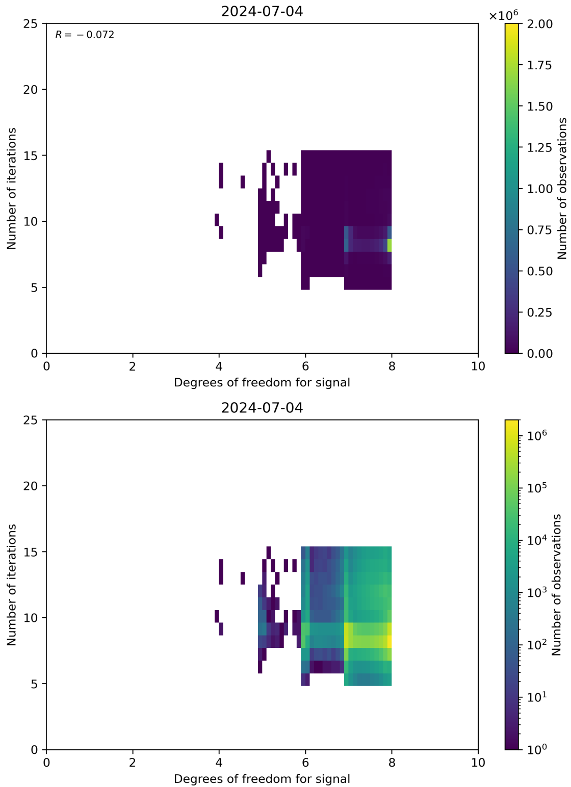
Figure 50: Scatter density plot of “Degrees of freedom for signal” against “Number of iterations” for 2024-07-03 to 2024-07-05.
