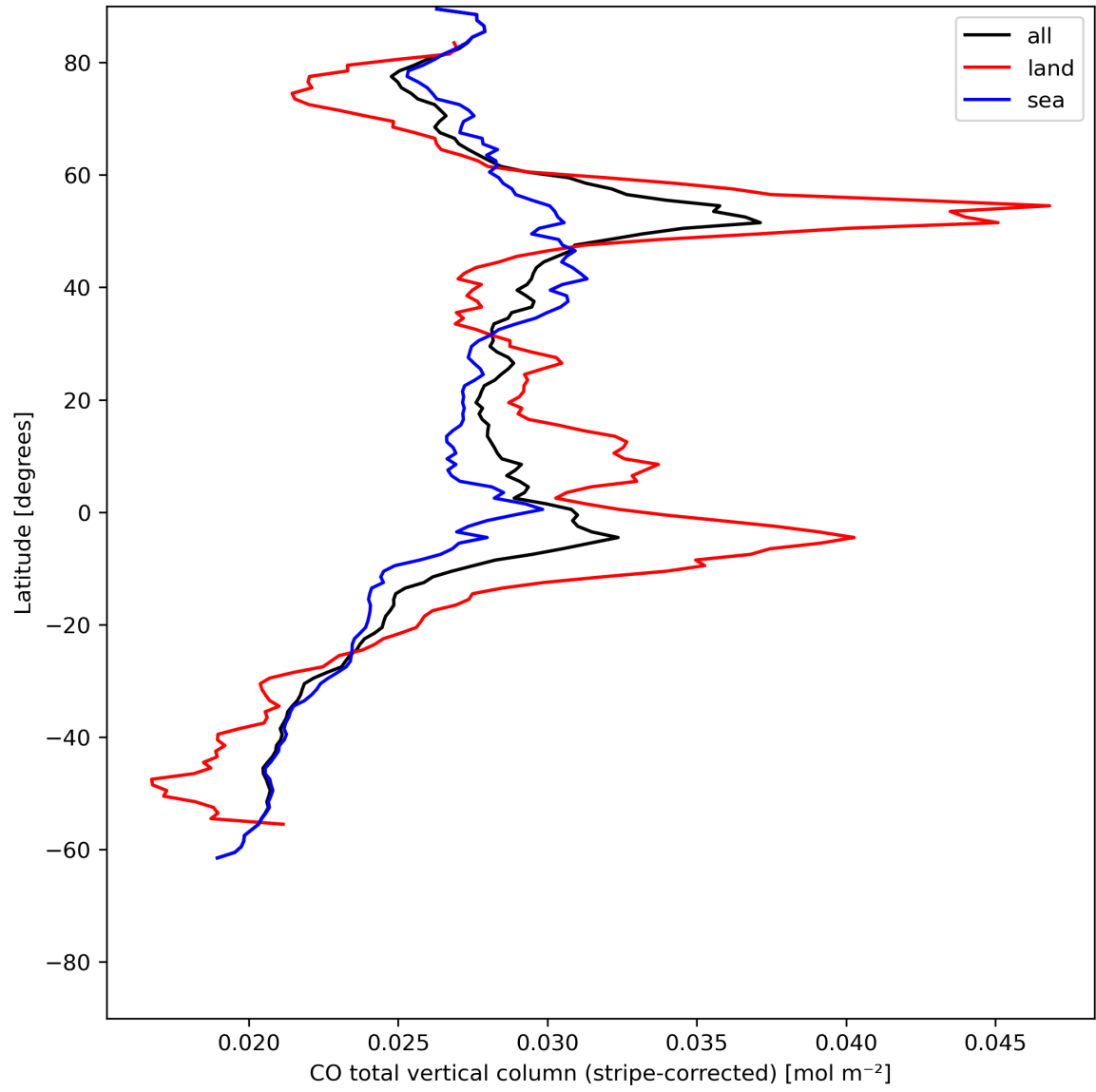
Figure 11: Zonal average of “CO total vertical column (stripe-corrected)” for 2024-07-03 to 2024-07-05.
