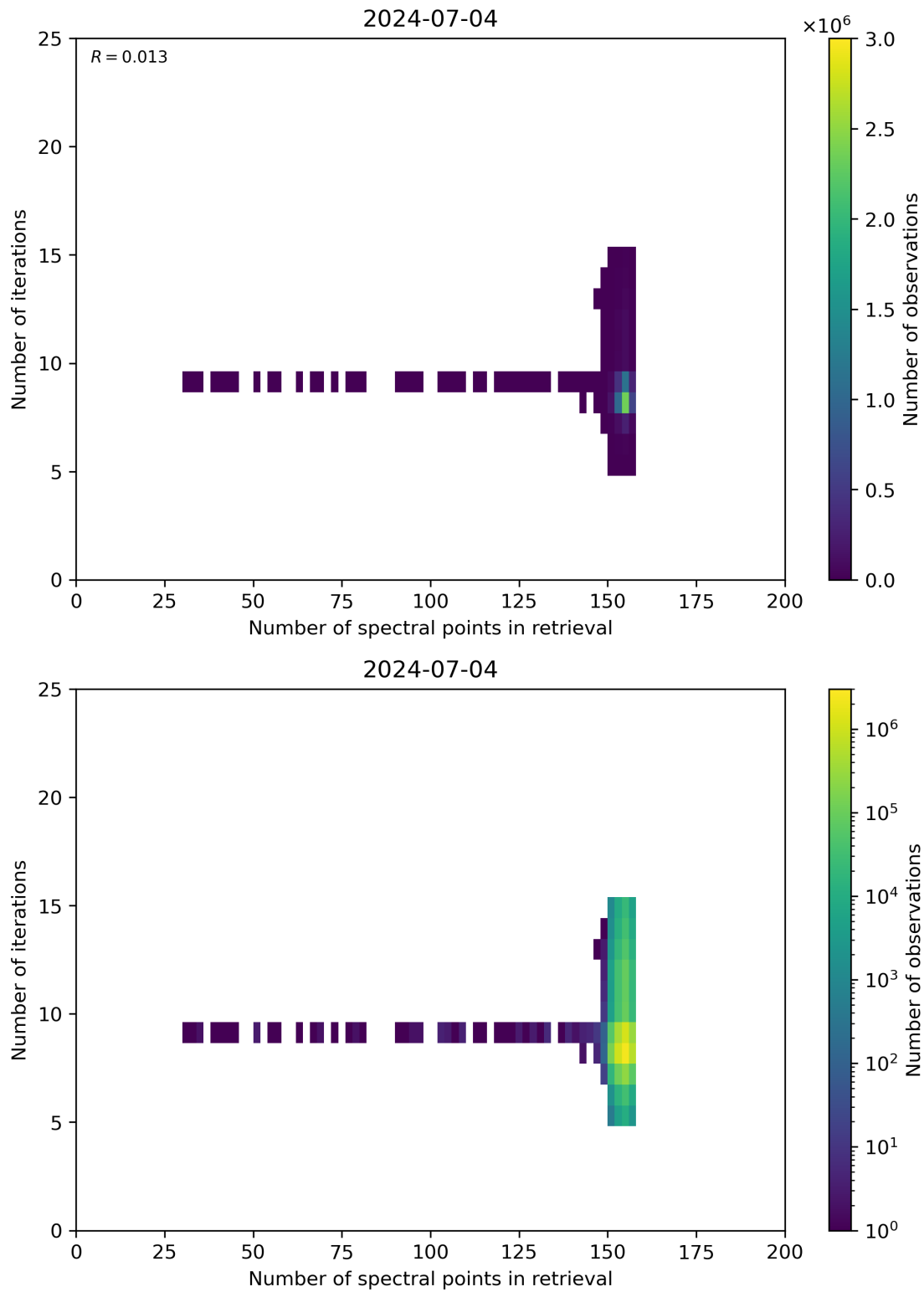
Figure 60: Scatter density plot of “Number of spectral points in retrieval” against “Number of iterations” for 2024-07-03 to 2024-07-05.
