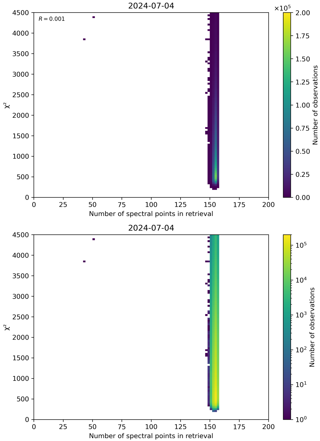
Figure 58: Scatter density plot of “Number of spectral points in retrieval” against “ \chi^2 ” for 2024-07-03 to 2024-07-05.
