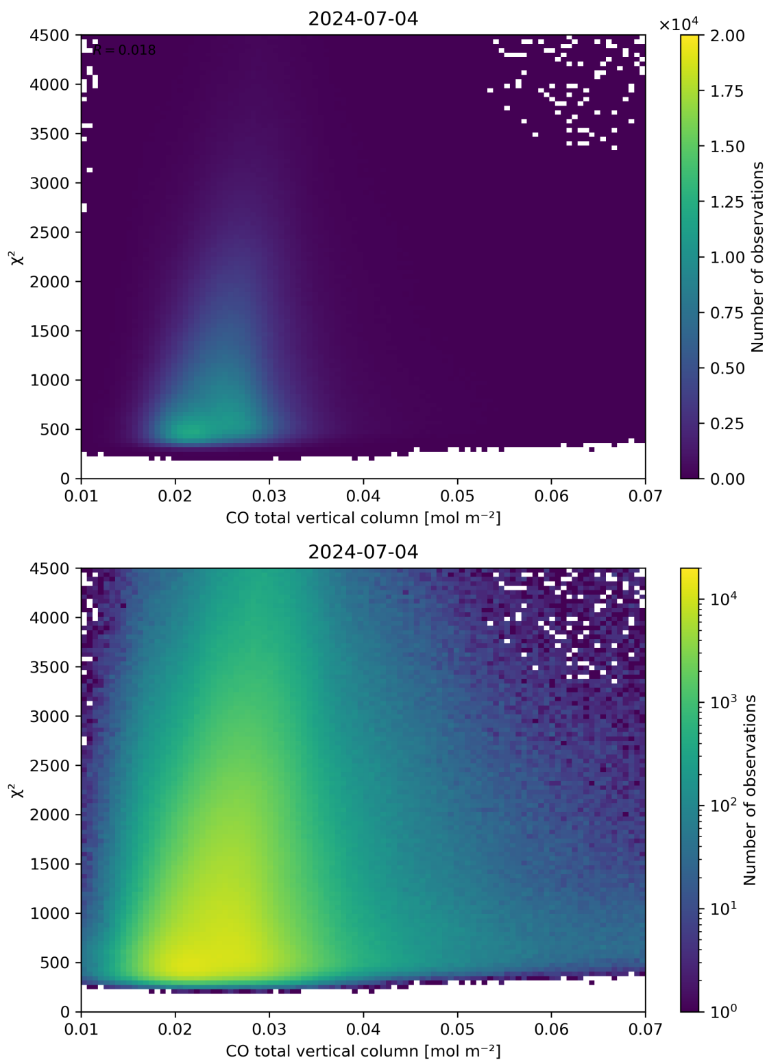
Figure 35: Scatter density plot of “CO total vertical column” against “ \chi^2 ” for 2024-07-03 to 2024-07-05.
