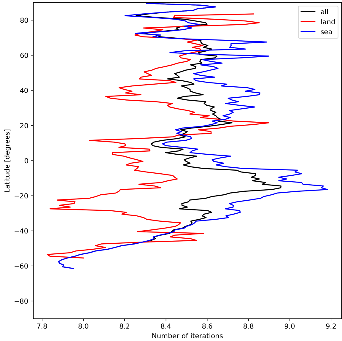
Figure 16: Zonal average of “Number of iterations” for 2024-07-03 to 2024-07-05.
