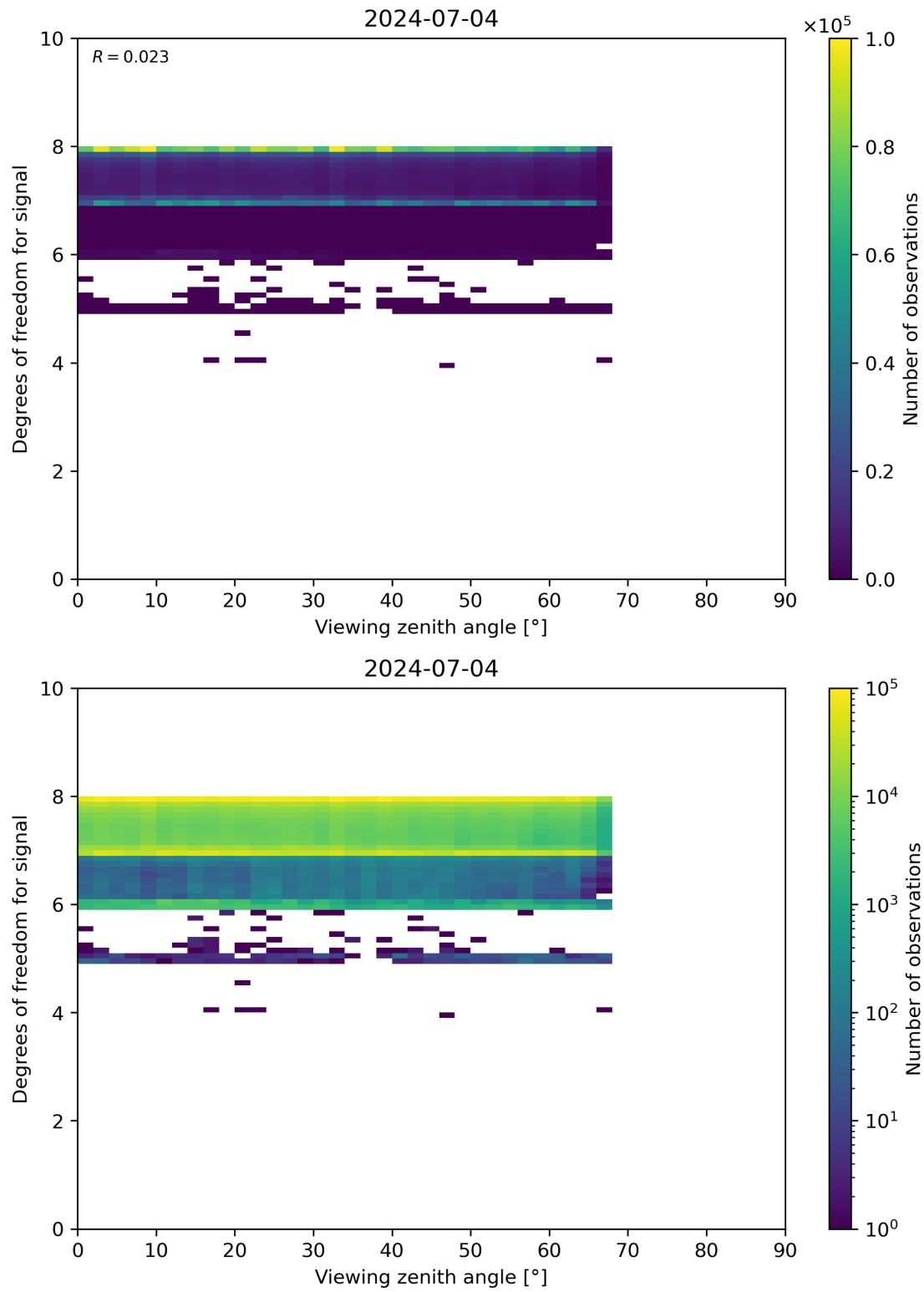
Figure 73: Scatter density plot of “Viewing zenith angle” against “Degrees of freedom for signal” for 2024-07-03 to 2024-07-05.
