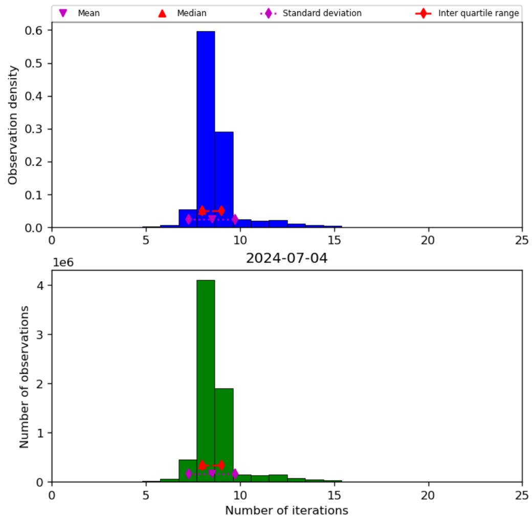
Figure 24: Histogram of “Number of iterations” for 2024-07-03 to 2024-07-05
