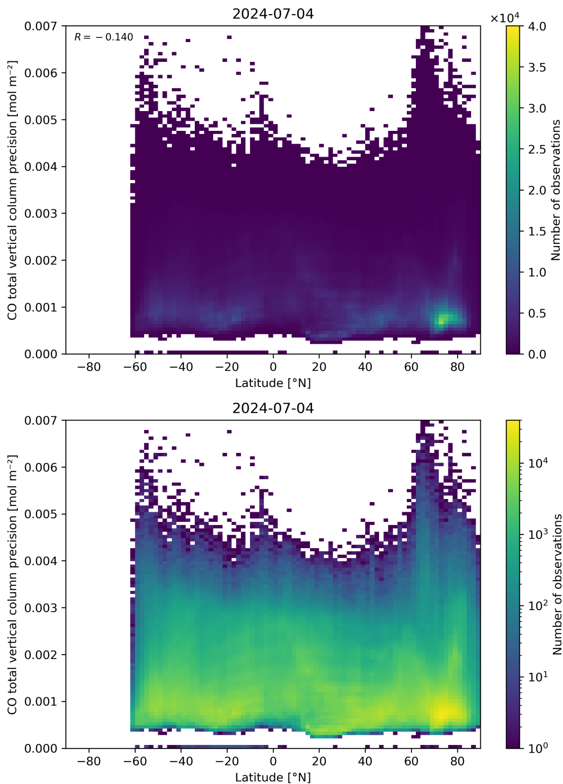
Figure 53: Scatter density plot of “Latitude” against “CO total vertical column precision” for 2024-07-03 to 2024-07-05.
