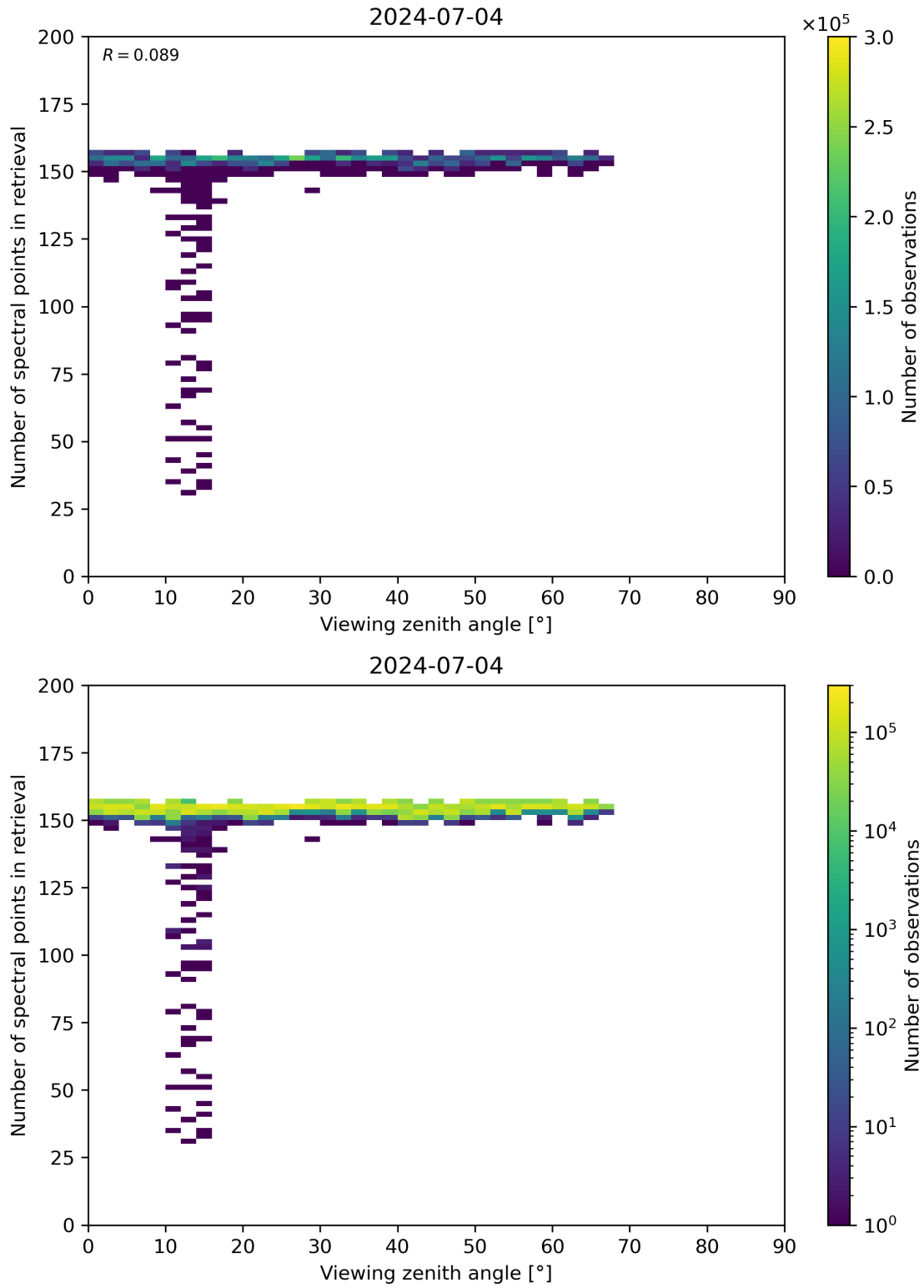
Figure 76: Scatter density plot of “Viewing zenith angle” against “Number of spectral points in retrieval” for 2024-07-03 to 2024-07-05.
