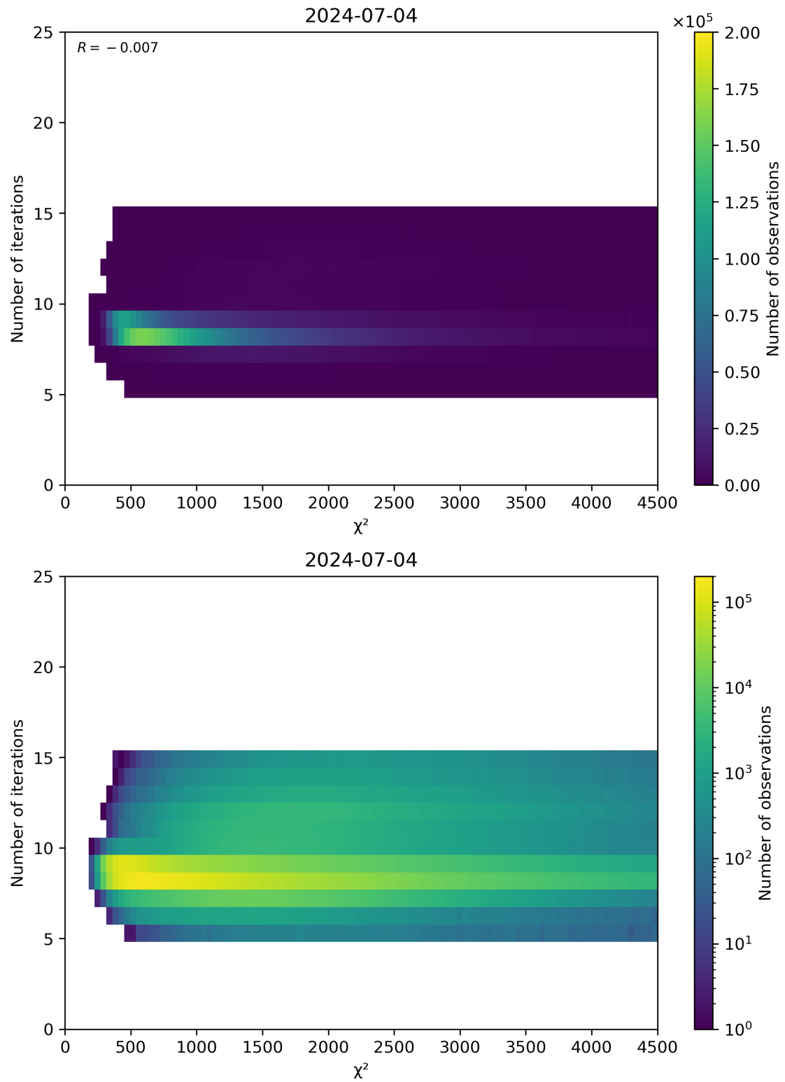
Figure 49: Scatter density plot of “ \chi^2 ” against “Number of iterations” for 2024-07-03 to 2024-07-05.
