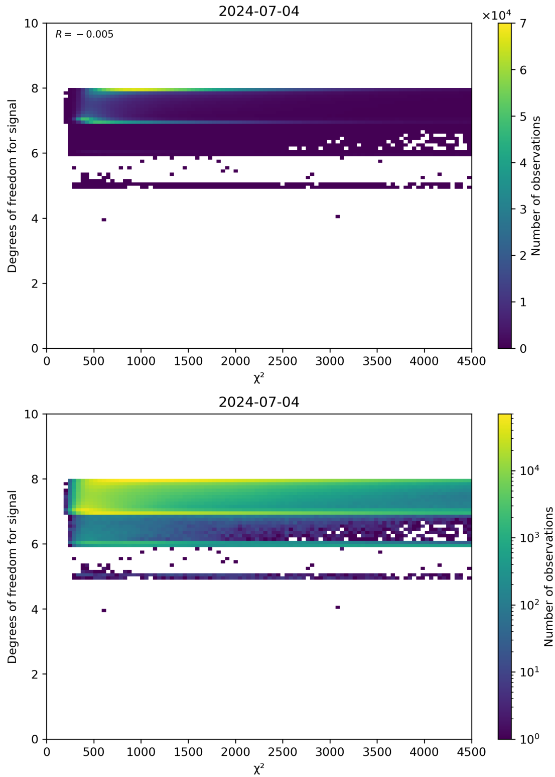
Figure 48: Scatter density plot of “ \chi^2 ” against “Degrees of freedom for signal” for 2024-07-03 to 2024-07-05.
