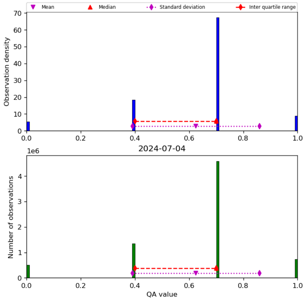
Figure 17: Histogram of “QA value” for 2024-07-03 to 2024-07-05
