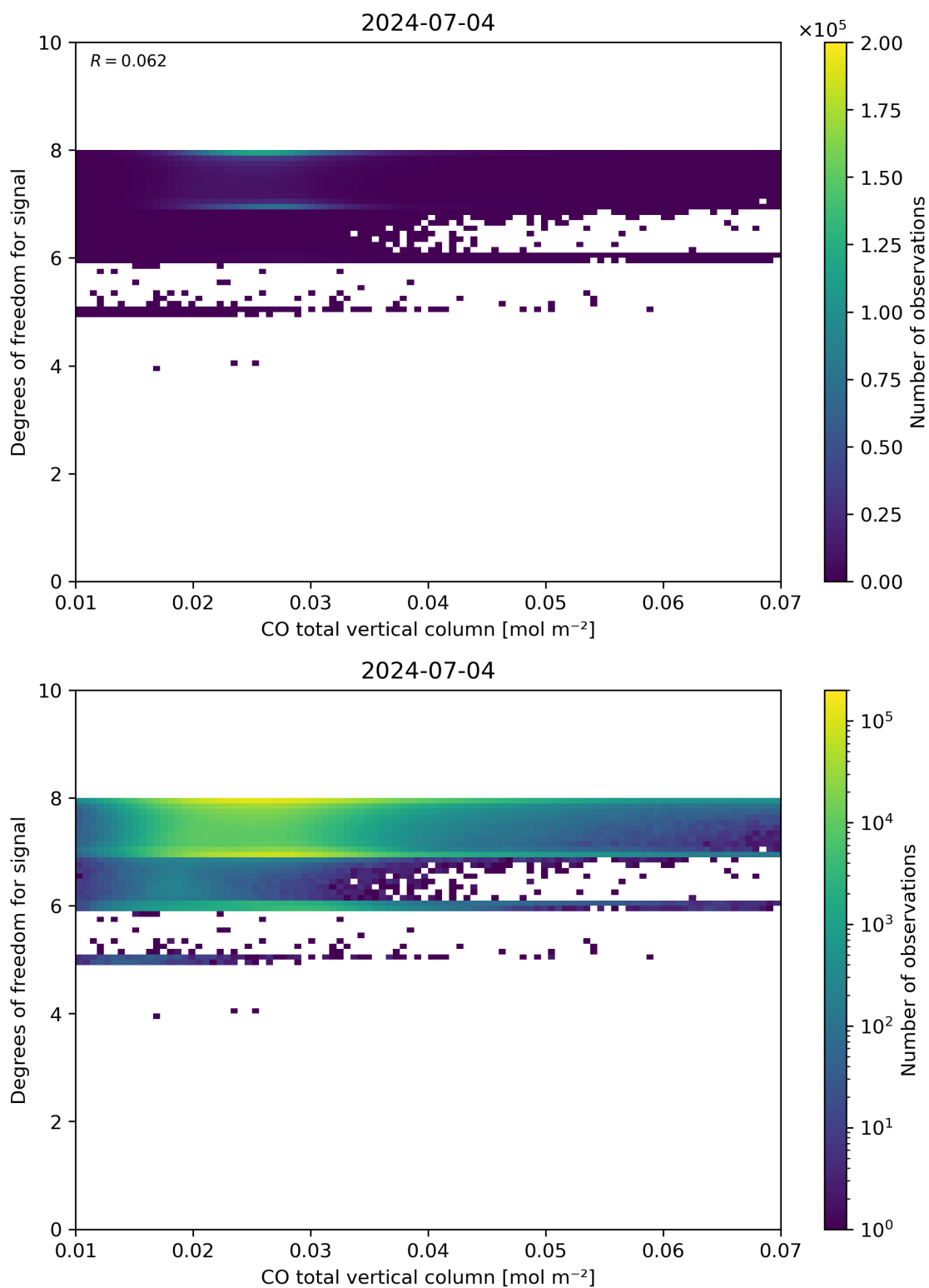
Figure 41: Scatter density plot of “CO total vertical column” against “Degrees of freedom for signal” for 2024-07-03 to 2024-07-05.
