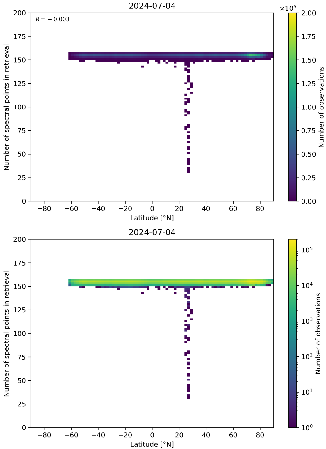
Figure 57: Scatter density plot of “Latitude” against “Number of spectral points in retrieval” for 2024-07-03 to 2024-07-05.
