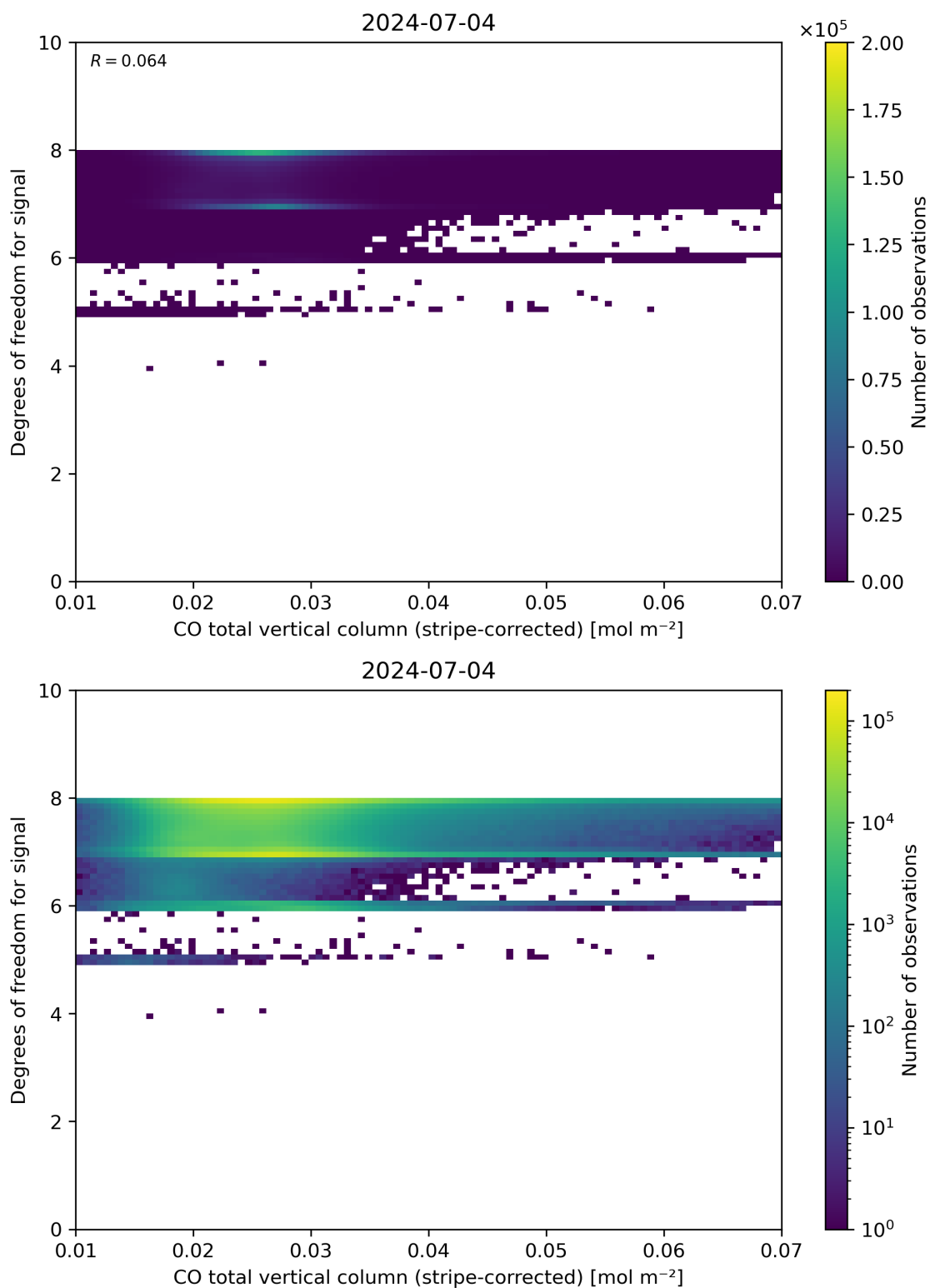
Figure 38: Scatter density plot of “CO total vertical column (stripe-corrected)” against “Degrees of freedom for signal” for 2024-07-03 to 2024-07-05.
