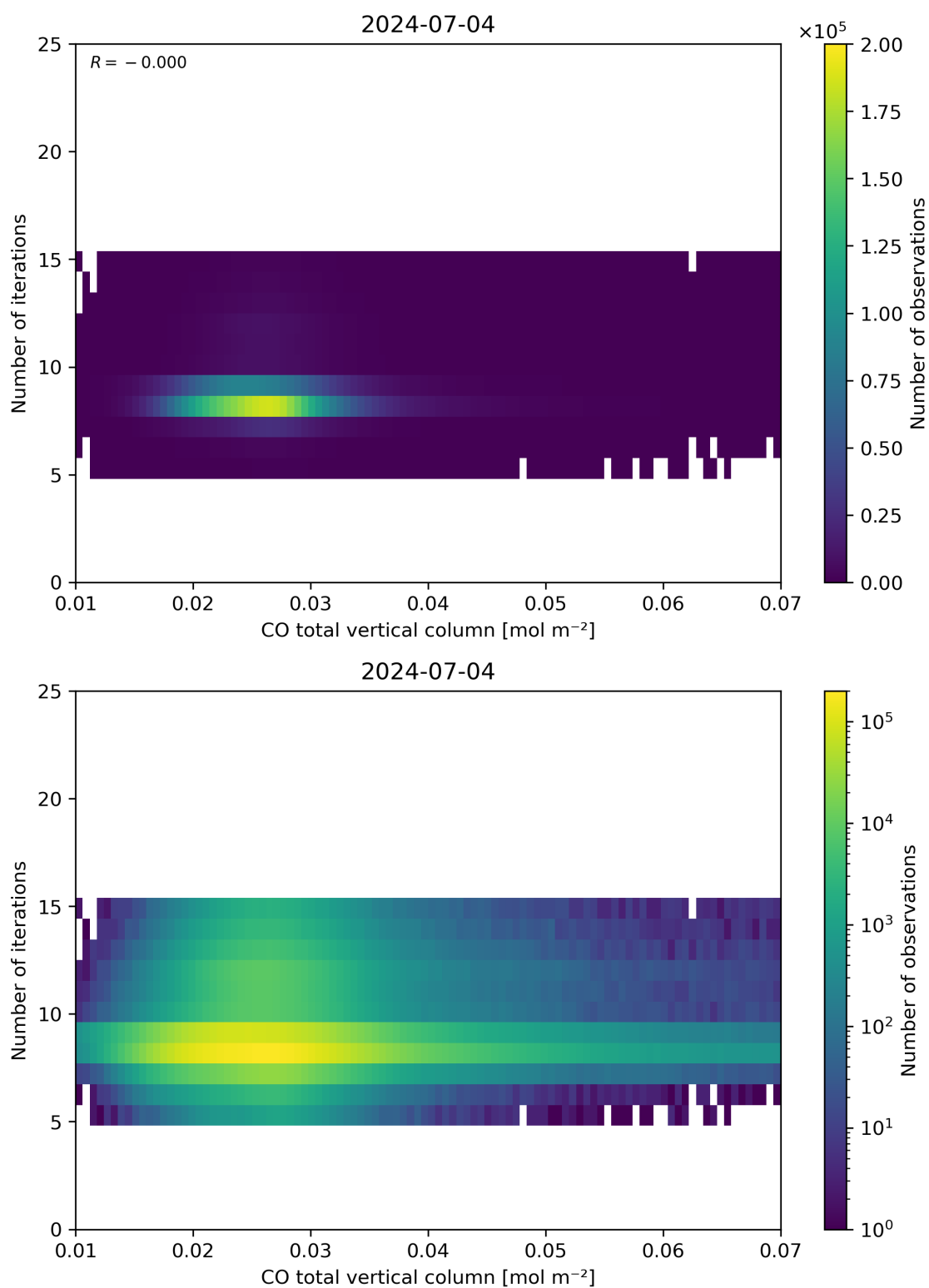
Figure 42: Scatter density plot of “CO total vertical column” against “Number of iterations” for 2024-07-03 to 2024-07-05.
