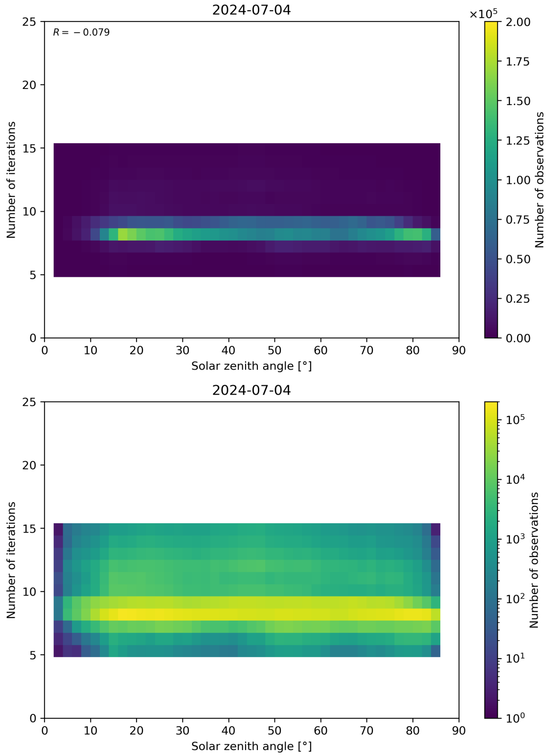
Figure 67: Scatter density plot of “Solar zenith angle” against “Number of iterations” for 2024-07-03 to 2024-07-05.
