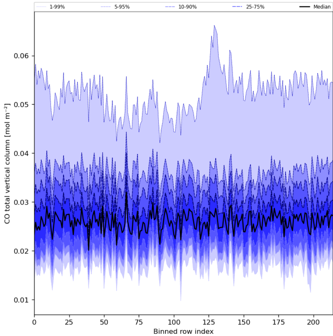
Figure 26: Along track statistics of “CO total vertical column” for 2024-07-03 to 2024-07-05
