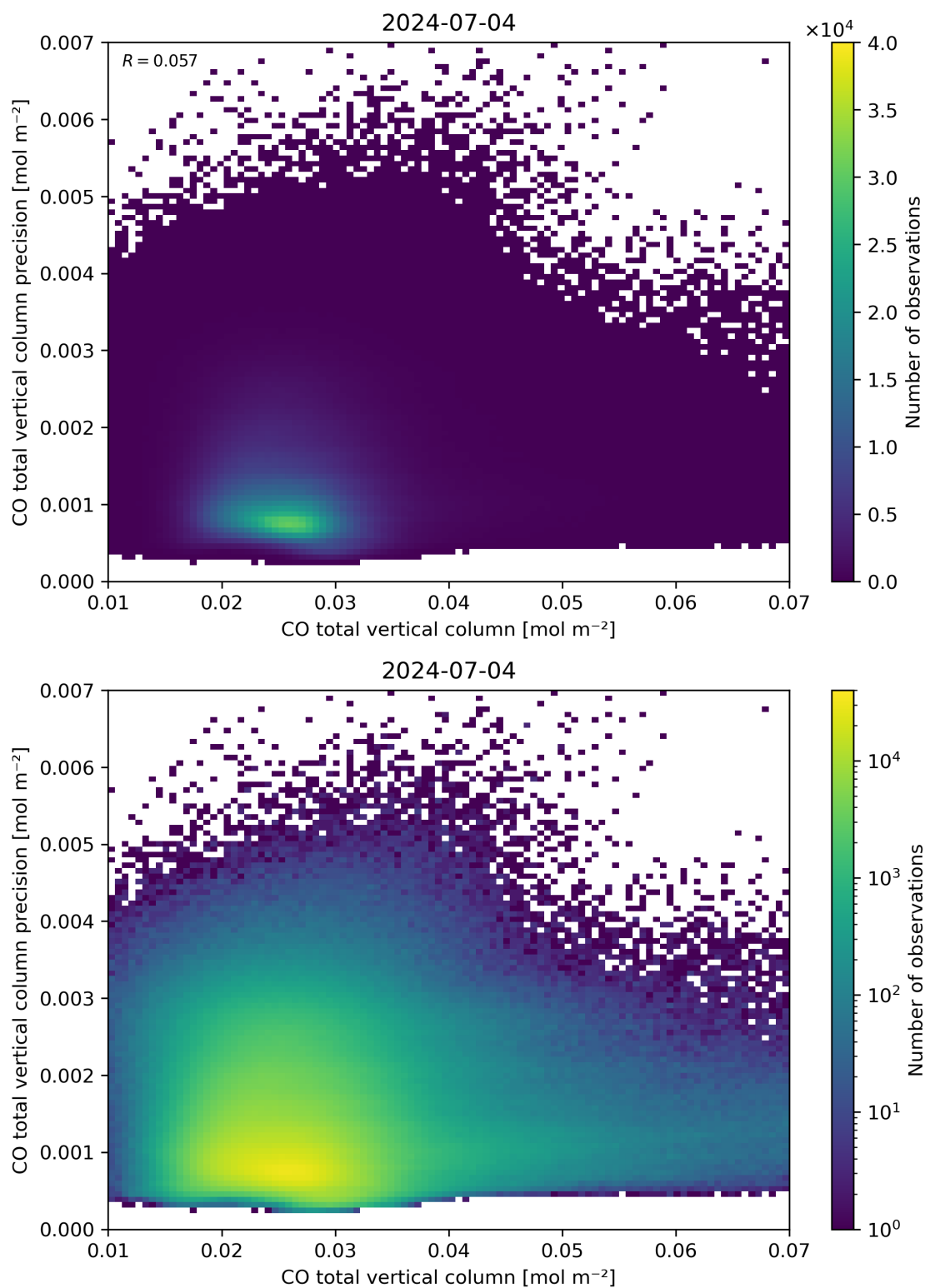
Figure 34: Scatter density plot of “CO total vertical column” against “CO total vertical column precision” for 2024-07-03 to 2024-07-05.
