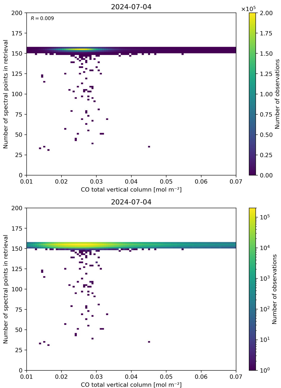
Figure 43: Scatter density plot of “CO total vertical column” against “Number of spectral points in retrieval” for 2024-07-03 to 2024-07-05.
