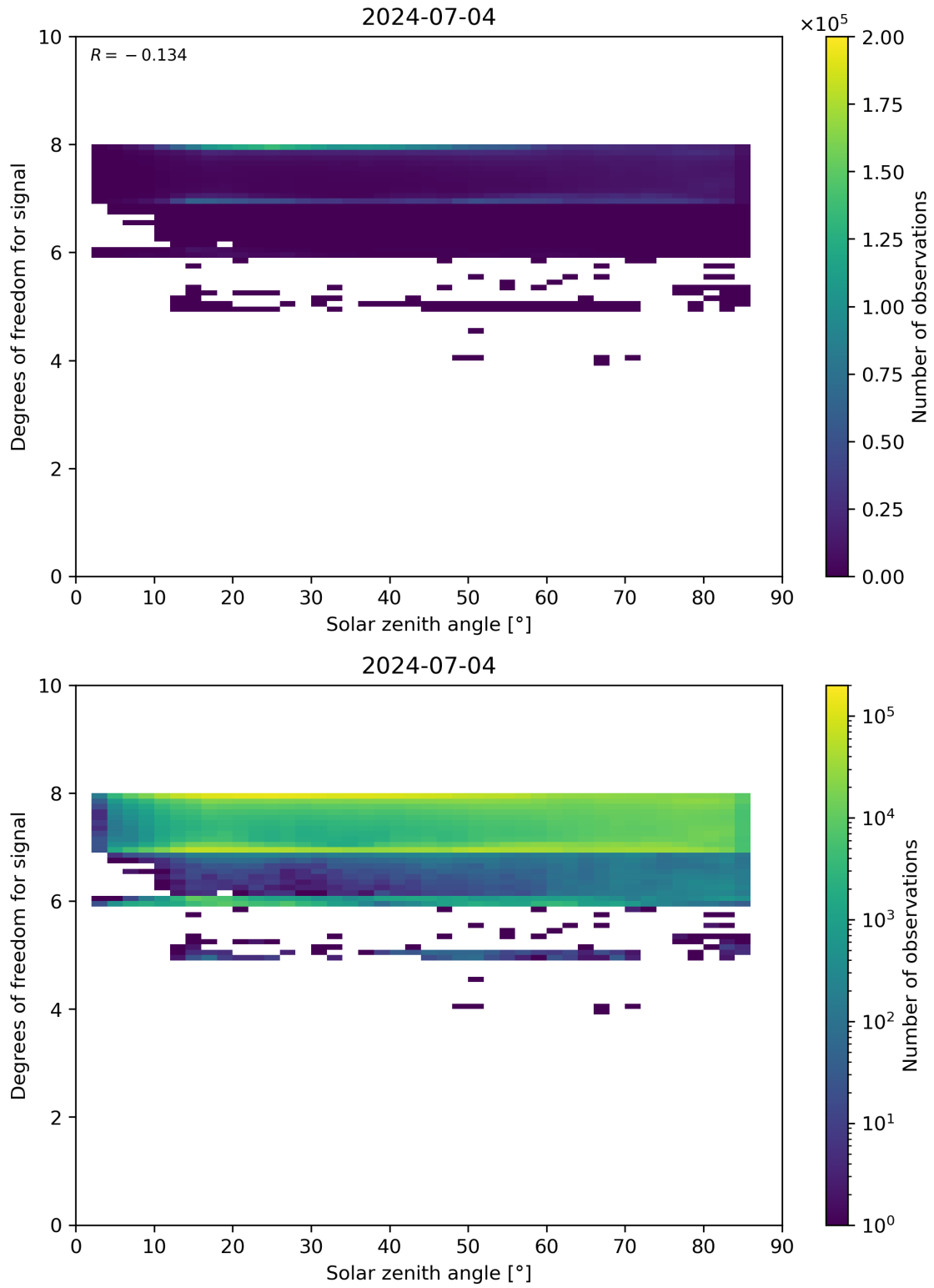
Figure 65: Scatter density plot of “Solar zenith angle” against “Degrees of freedom for signal” for 2024-07-03 to 2024-07-05.
