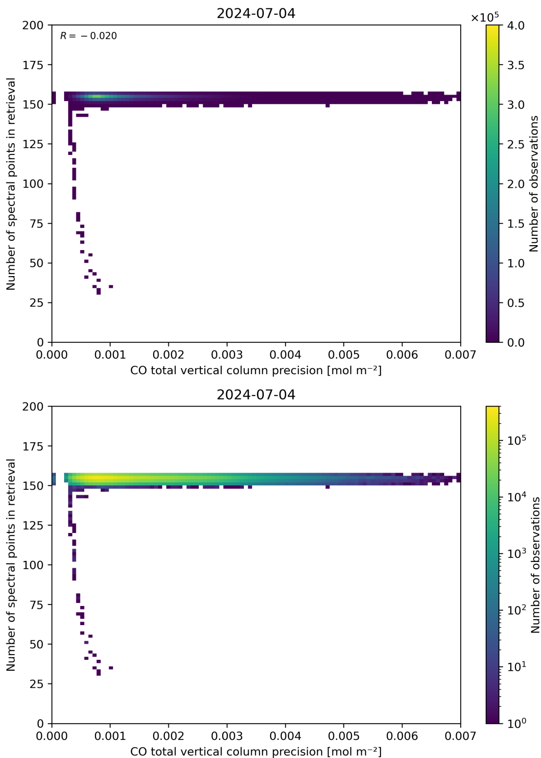
Figure 47: Scatter density plot of “CO total vertical column precision” against “Number of spectral points in retrieval” for 2024-07-03 to 2024-07-05.
