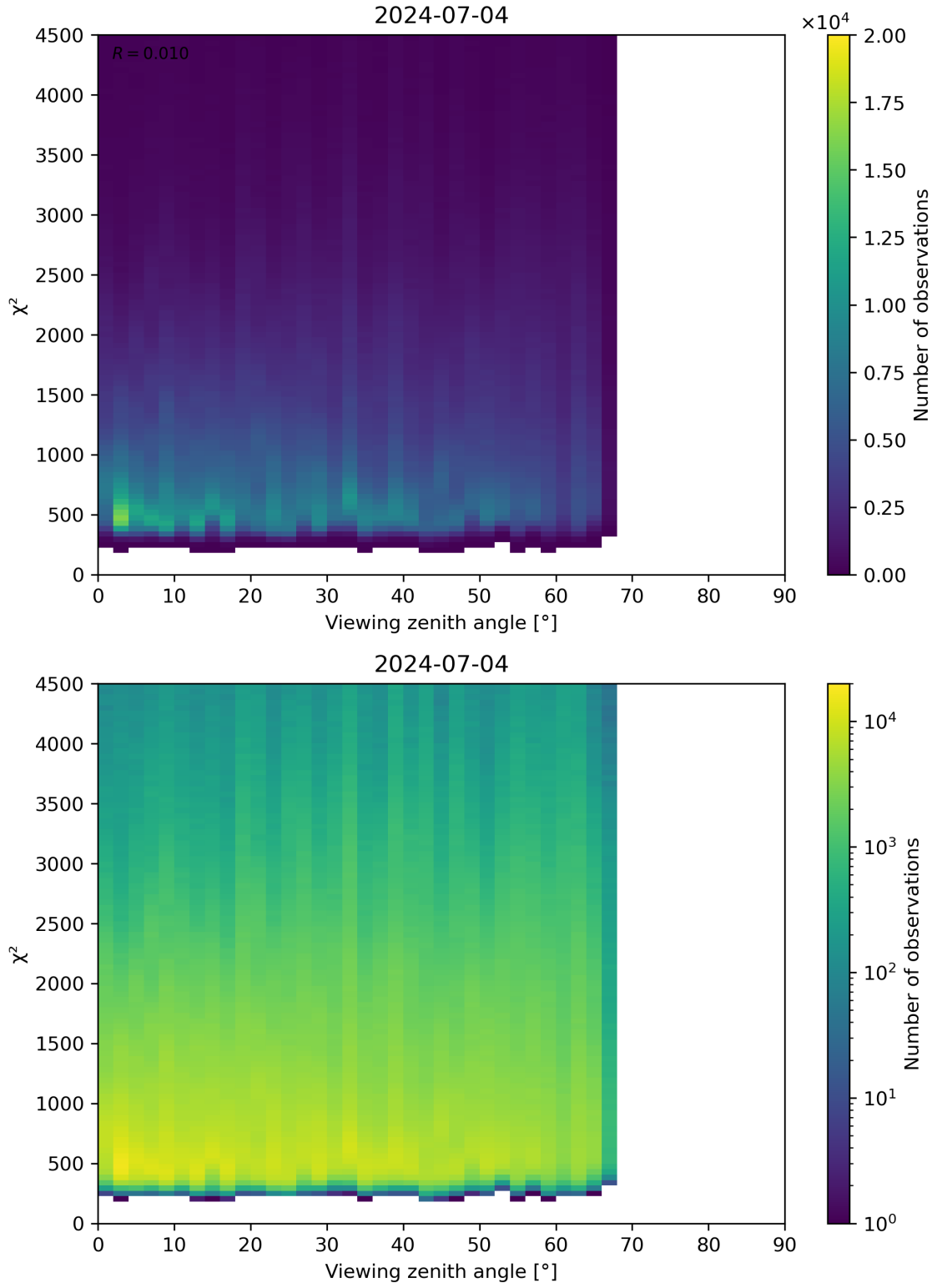
Figure 72: Scatter density plot of “Viewing zenith angle” against “ \chi^2 ” for 2024-07-03 to 2024-07-05.
