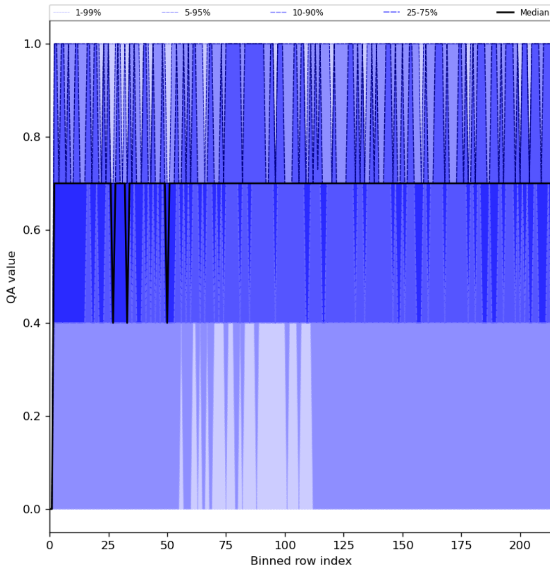
Figure 25: Along track statistics of “QA value” for 2024-07-03 to 2024-07-05
