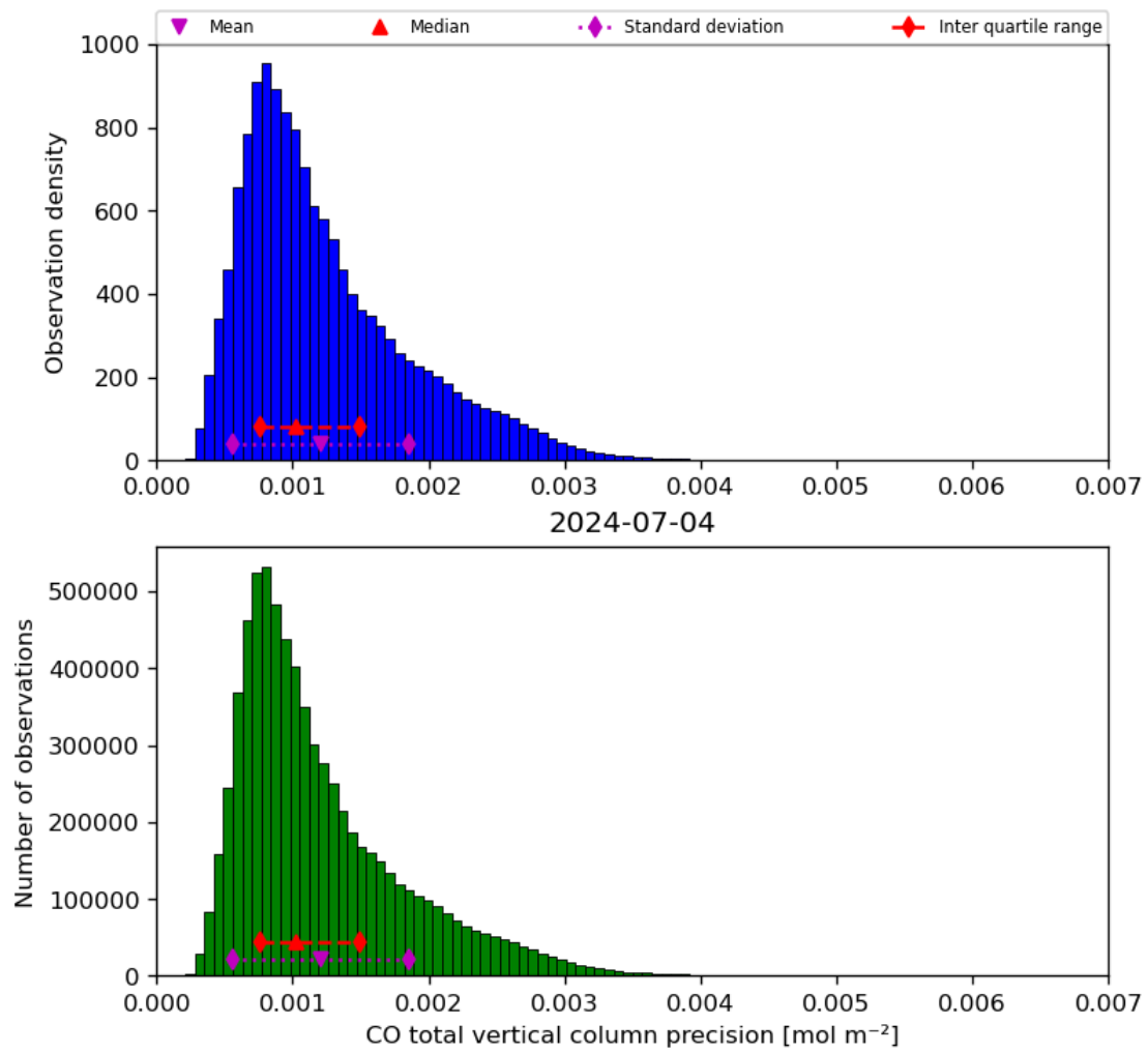
Figure 20: Histogram of “CO total vertical column precision” for 2024-07-03 to 2024-07-05
