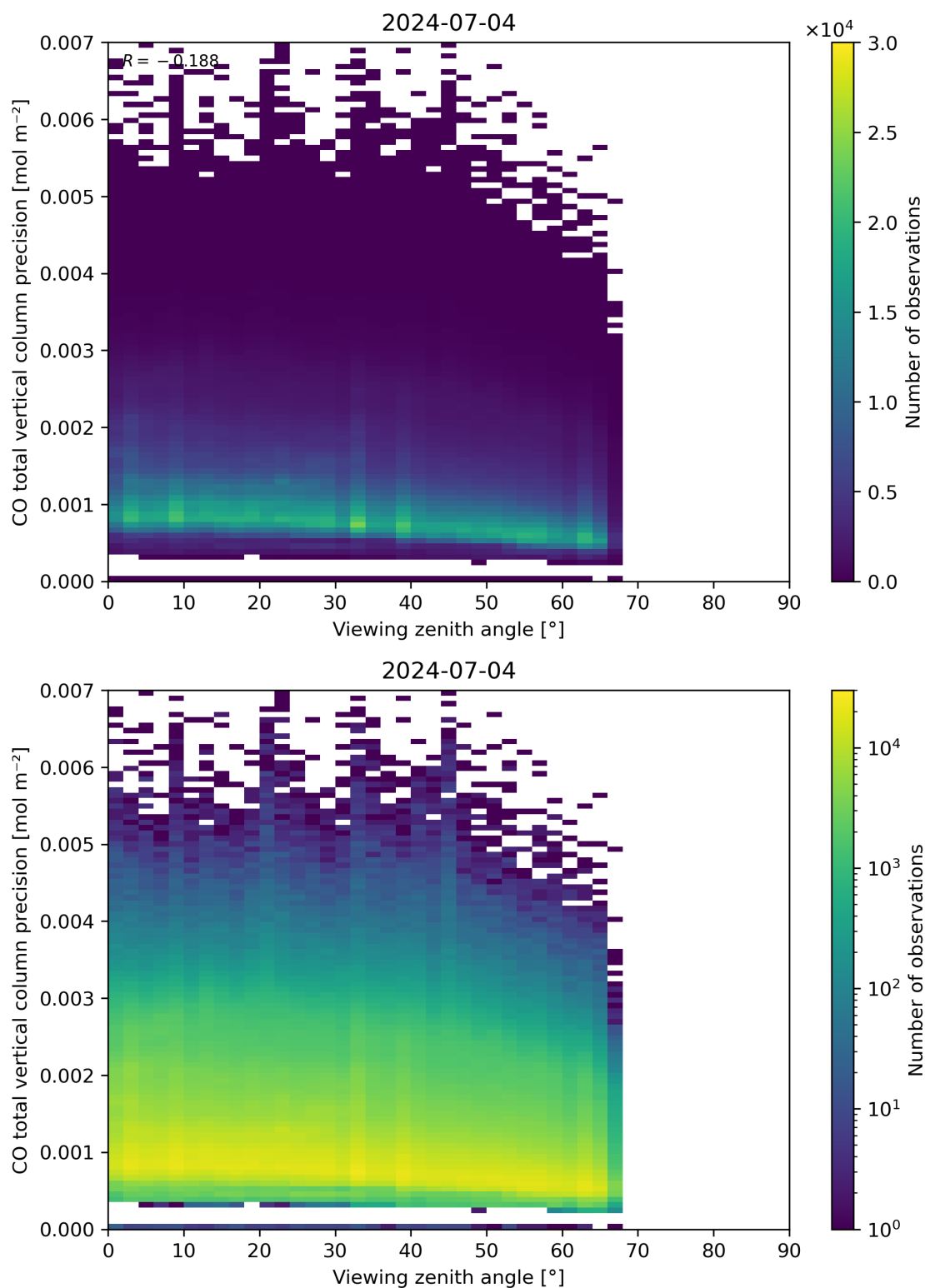
Figure 71: Scatter density plot of “Viewing zenith angle” against “CO total vertical column precision” for 2024-07-03 to 2024-07-05.
