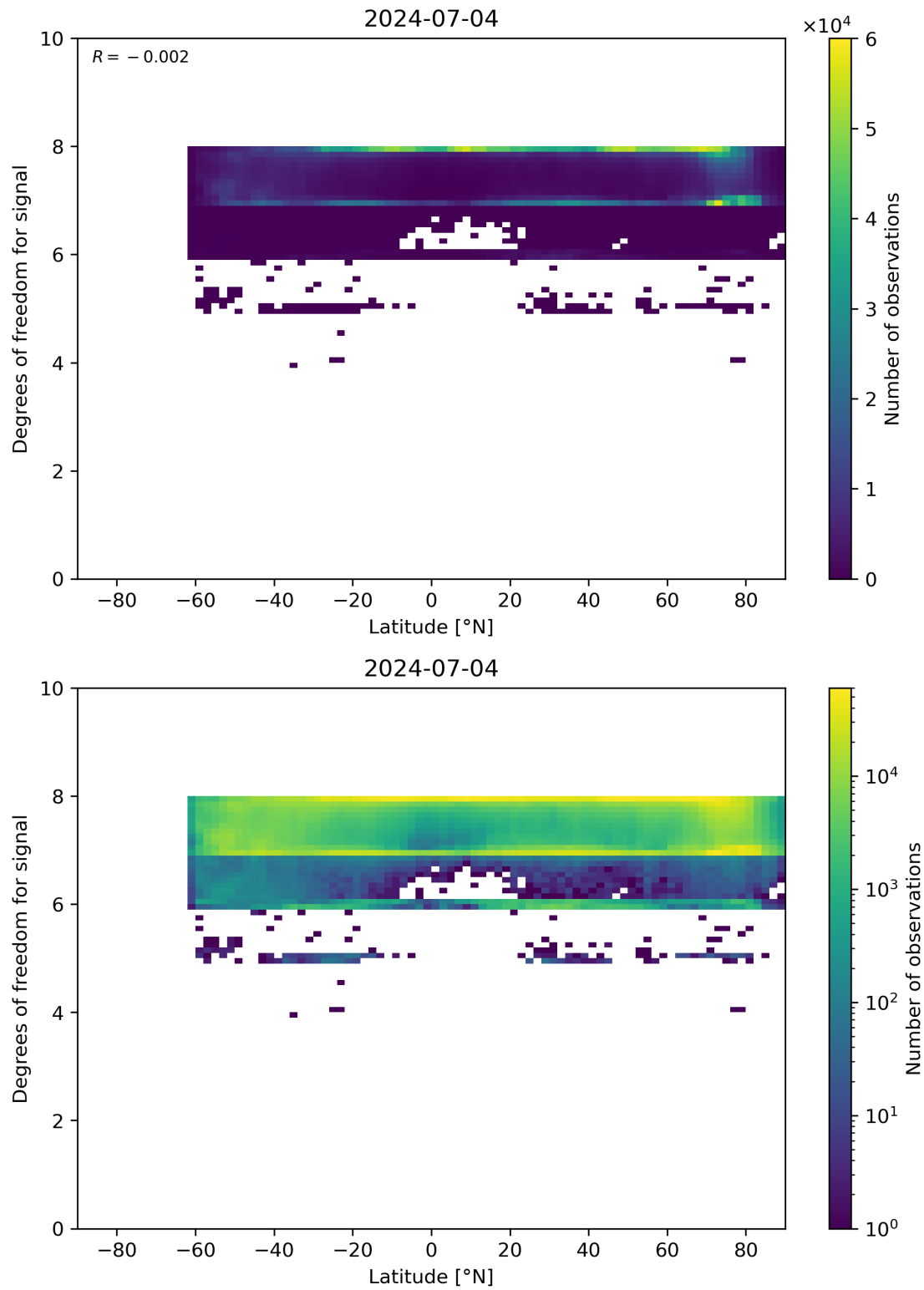
Figure 55: Scatter density plot of “Latitude” against “Degrees of freedom for signal” for 2024-07-03 to 2024-07-05.
