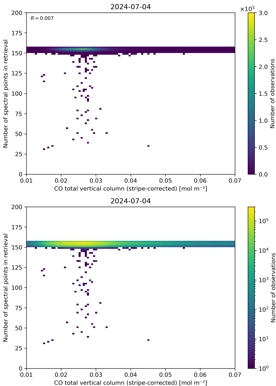
Figure 40: Scatter density plot of “CO total vertical column (stripe-corrected)” against “Number of spectral points in retrieval” for 2024-07-03 to 2024-07-05.
