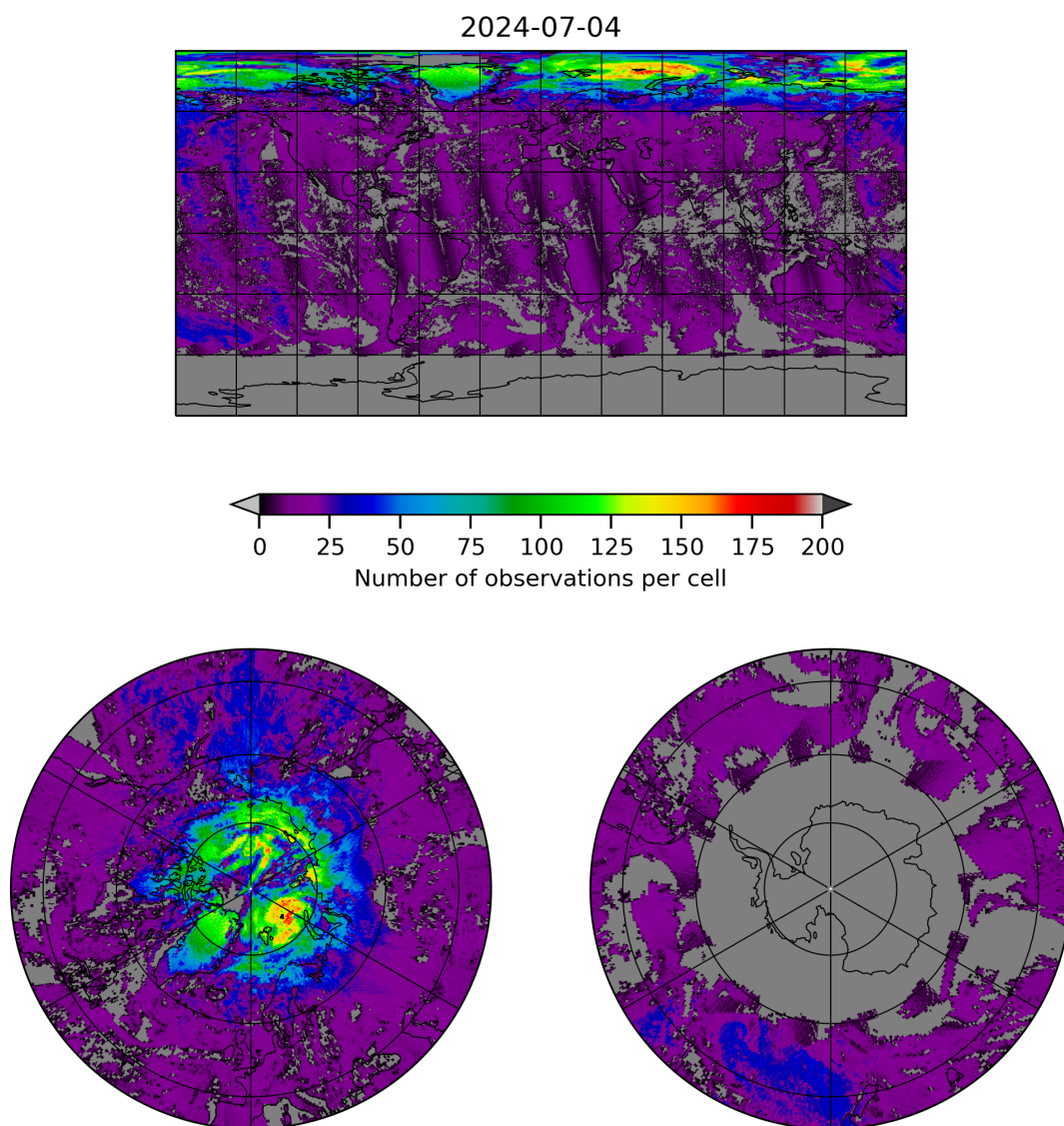
Figure 8: Map of the number of observations for 2024-07-03 to 2024-07-05
