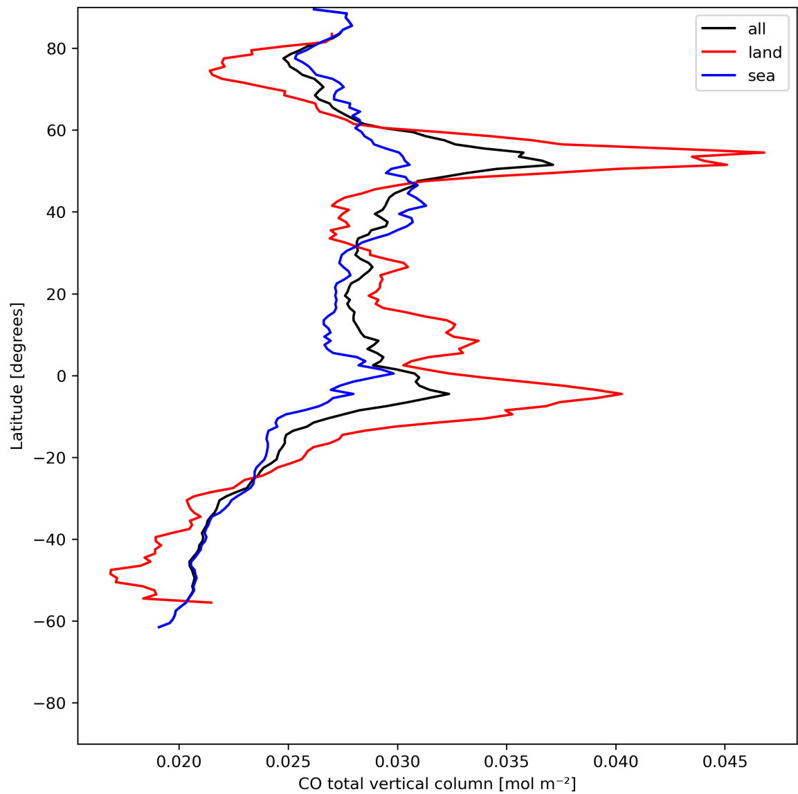
Figure 10: Zonal average of “CO total vertical column” for 2024-07-03 to 2024-07-05.
