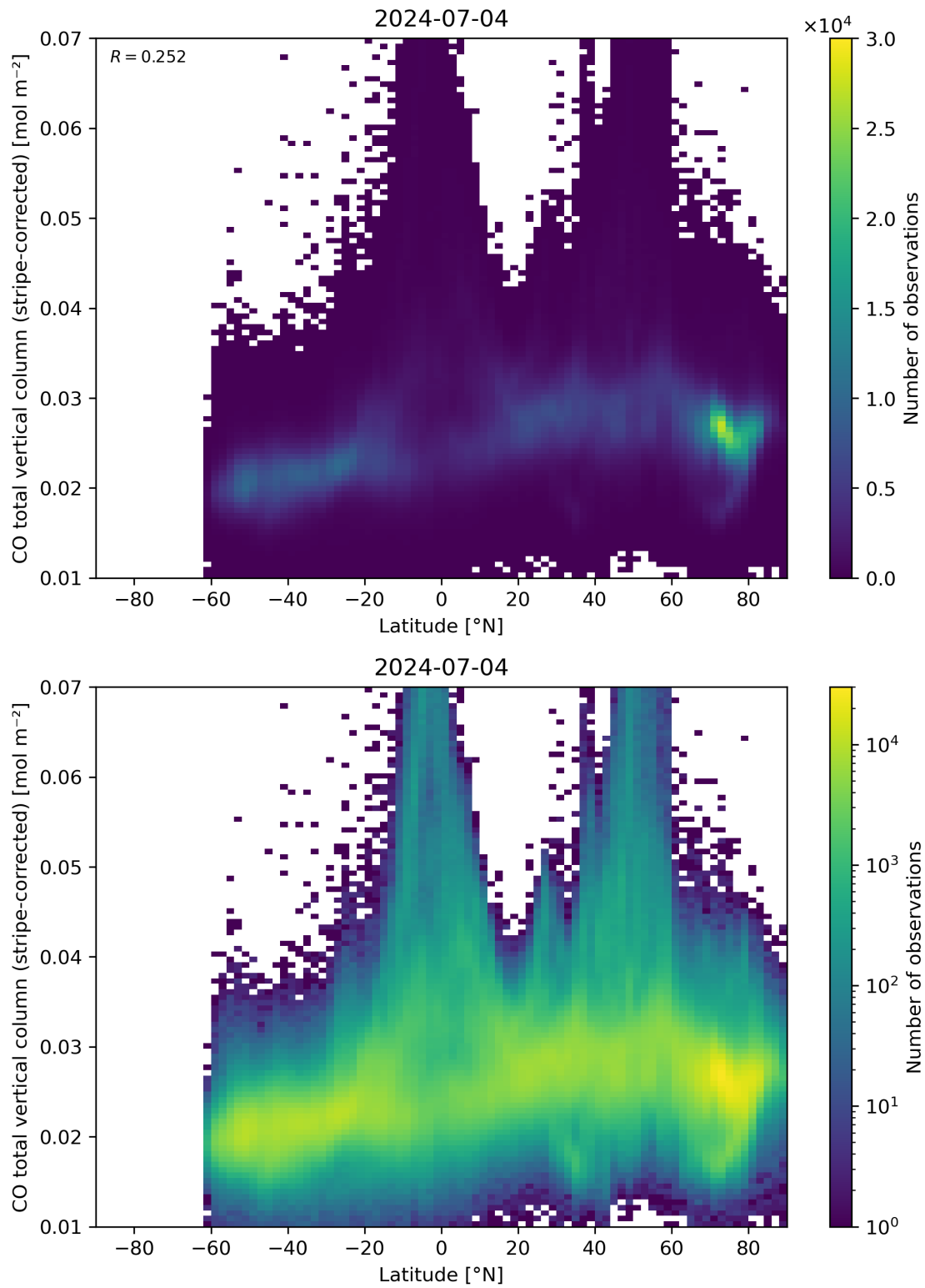
Figure 52: Scatter density plot of “Latitude” against “CO total vertical column (stripe-corrected)” for 2024-07-03 to 2024-07-05.
