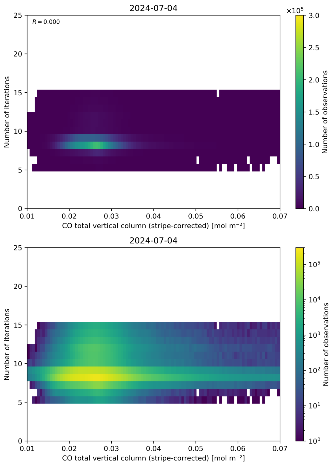
Figure 39: Scatter density plot of “CO total vertical column (stripe-corrected)” against “Number of iterations” for 2024-07-03 to 2024-07-05.
