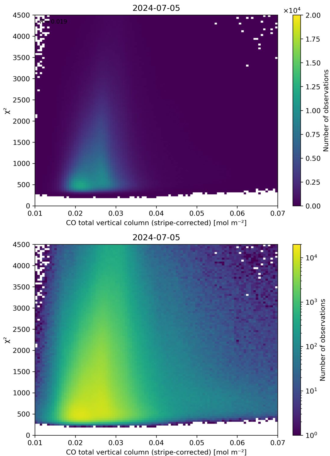
Figure 37: Scatter density plot of “CO total vertical column (stripe-corrected)” against “ \chi^2 ” for 2024-07-05 to 2024-07-06.
