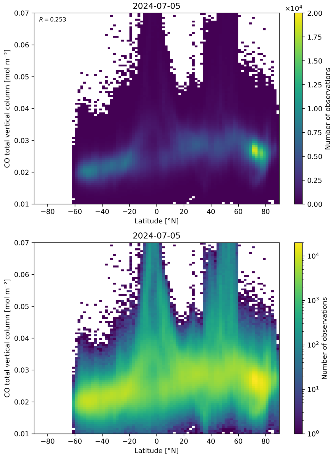
Figure 51: Scatter density plot of “Latitude” against “CO total vertical column” for 2024-07-05 to 2024-07-06.
