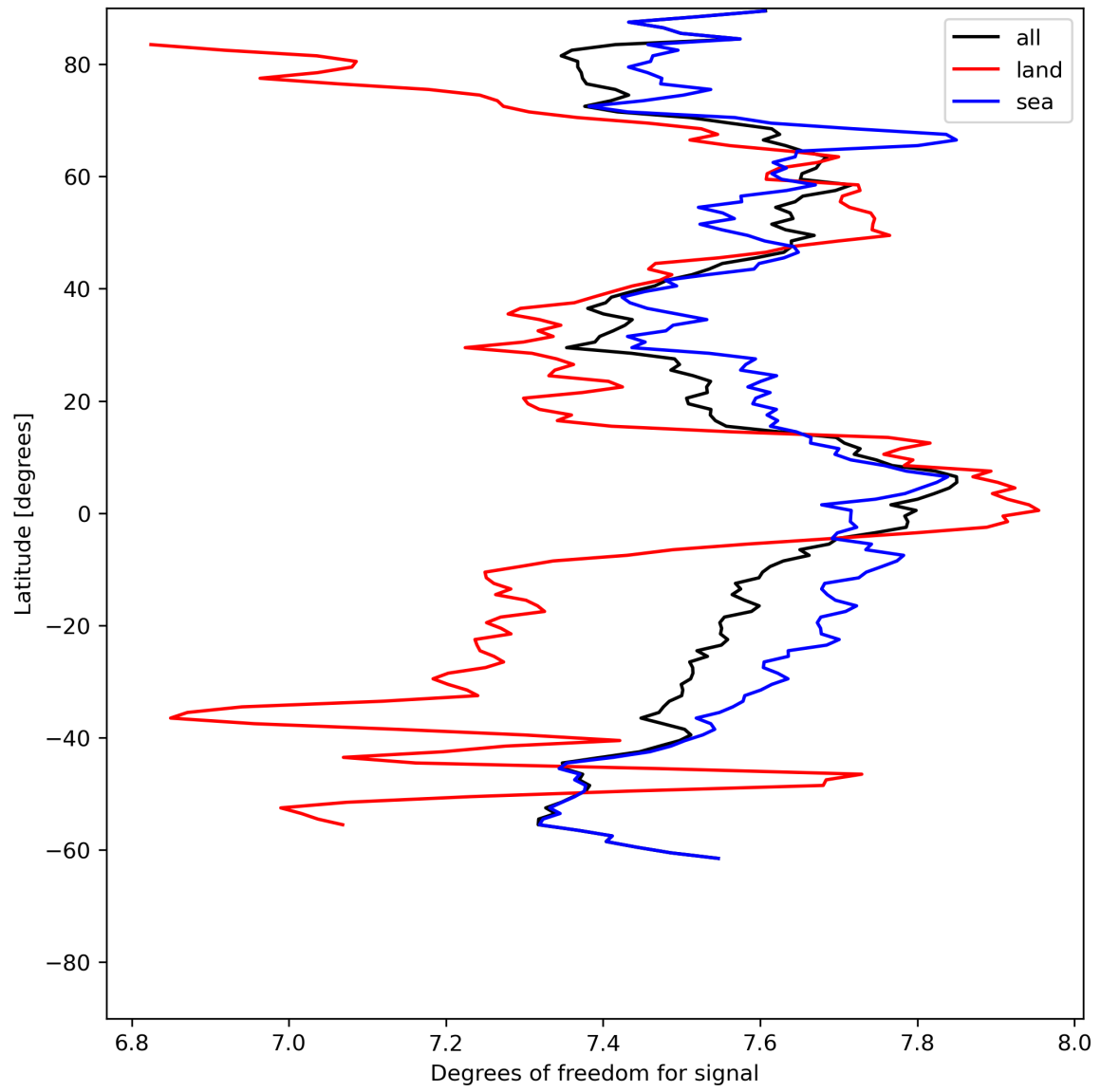
Figure 15: Zonal average of “Degrees of freedom for signal” for 2024-07-05 to 2024-07-06.
