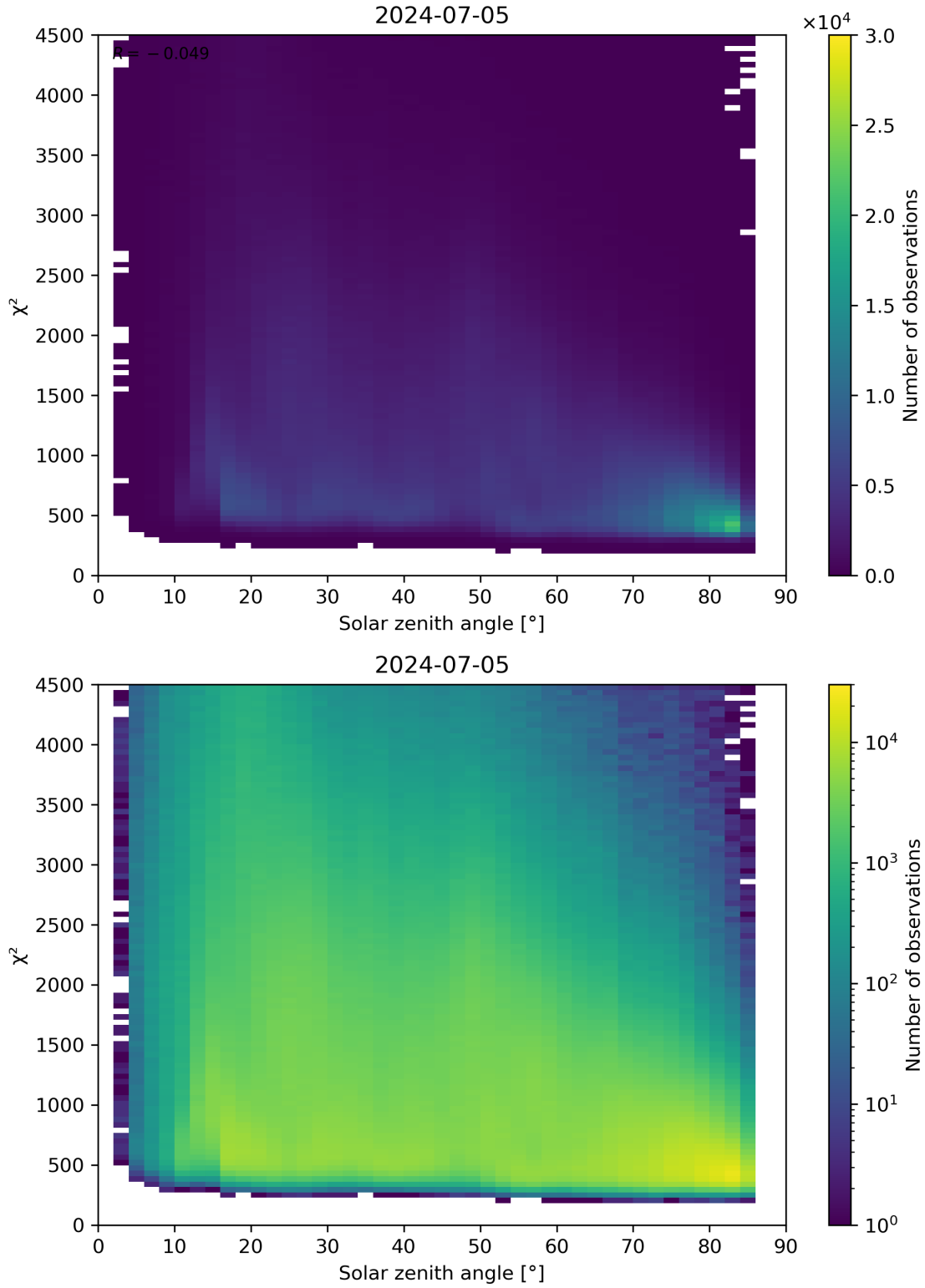
Figure 64: Scatter density plot of “Solar zenith angle” against “ \chi^2 ” for 2024-07-05 to 2024-07-06.
