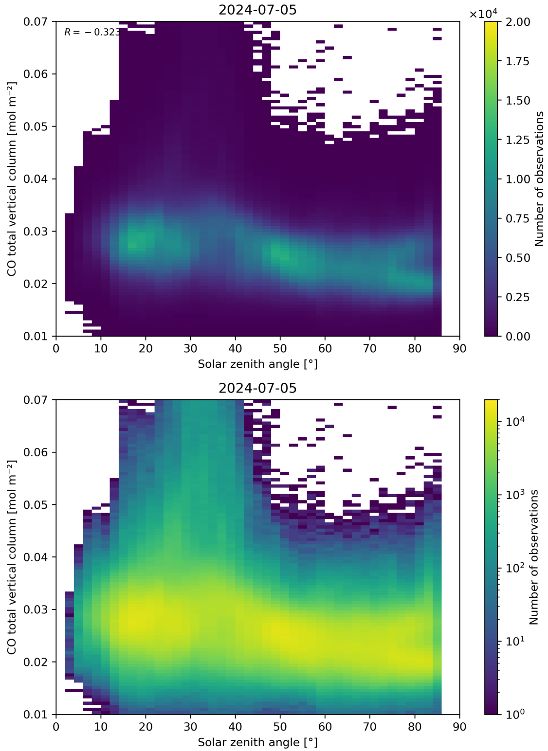
Figure 61: Scatter density plot of “Solar zenith angle” against “CO total vertical column” for 2024-07-05 to 2024-07-06.
