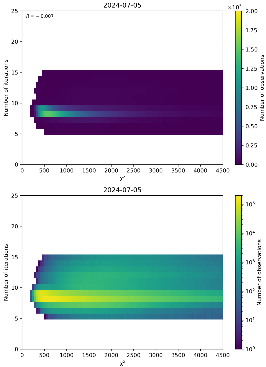
Figure 49: Scatter density plot of “ \chi^2 ” against “Number of iterations” for 2024-07-05 to 2024-07-06.
