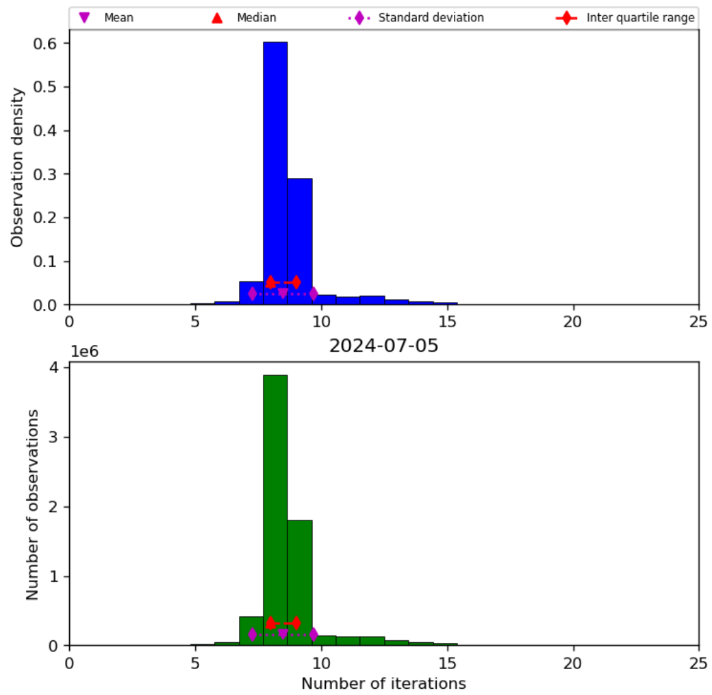
Figure 24: Histogram of “Number of iterations” for 2024-07-05 to 2024-07-06
