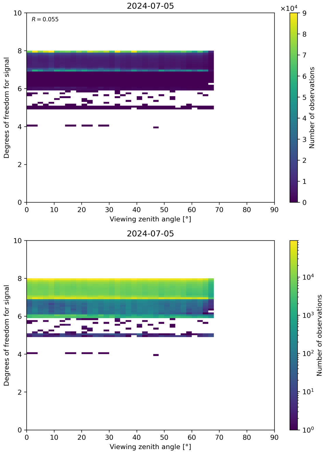
Figure 73: Scatter density plot of “Viewing zenith angle” against “Degrees of freedom for signal” for 2024-07-05 to 2024-07-06.
