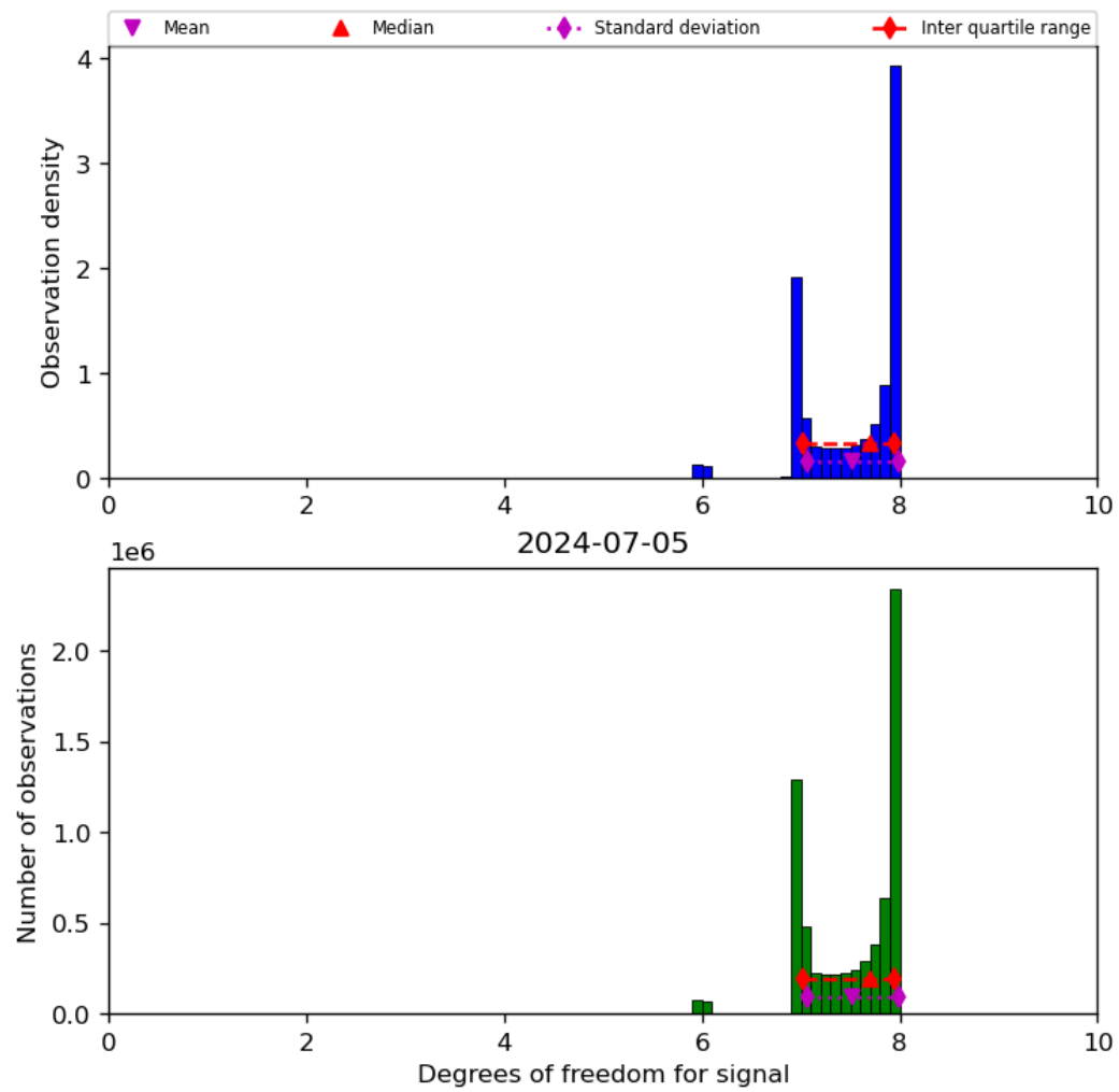
Figure 23: Histogram of “Degrees of freedom for signal” for 2024-07-05 to 2024-07-06
