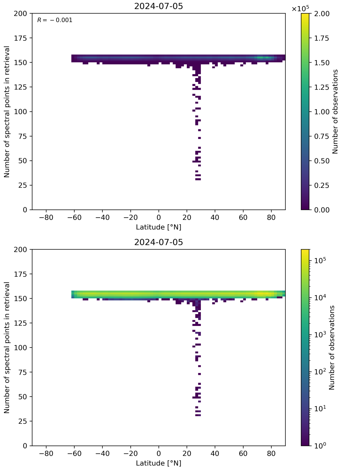
Figure 57: Scatter density plot of “Latitude” against “Number of spectral points in retrieval” for 2024-07-05 to 2024-07-06.
