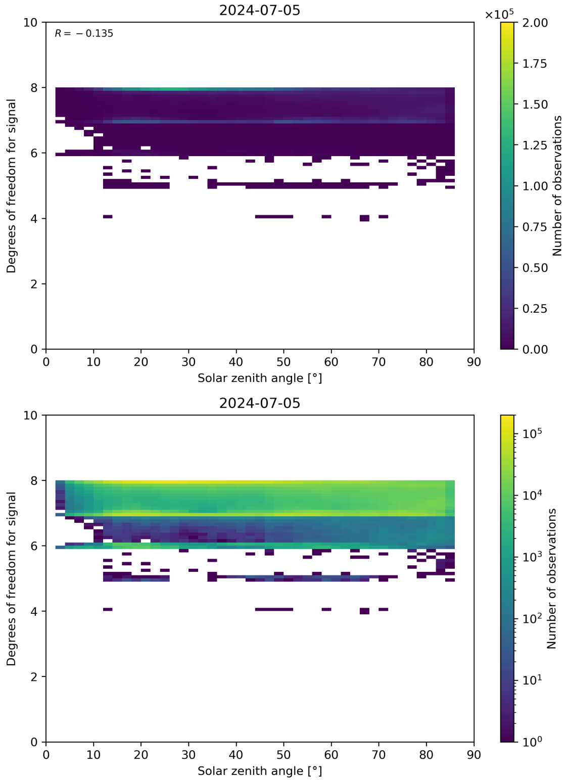
Figure 65: Scatter density plot of “Solar zenith angle” against “Degrees of freedom for signal” for 2024-07-05 to 2024-07-06.
