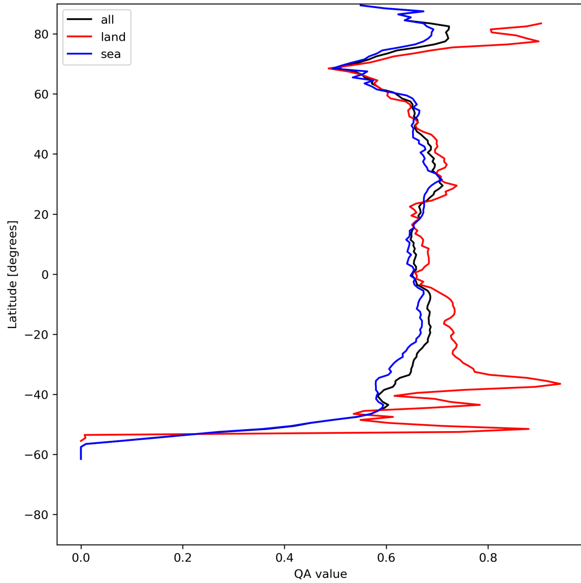
Figure 9: Zonal average of “QA value” for 2024-07-05 to 2024-07-06.
