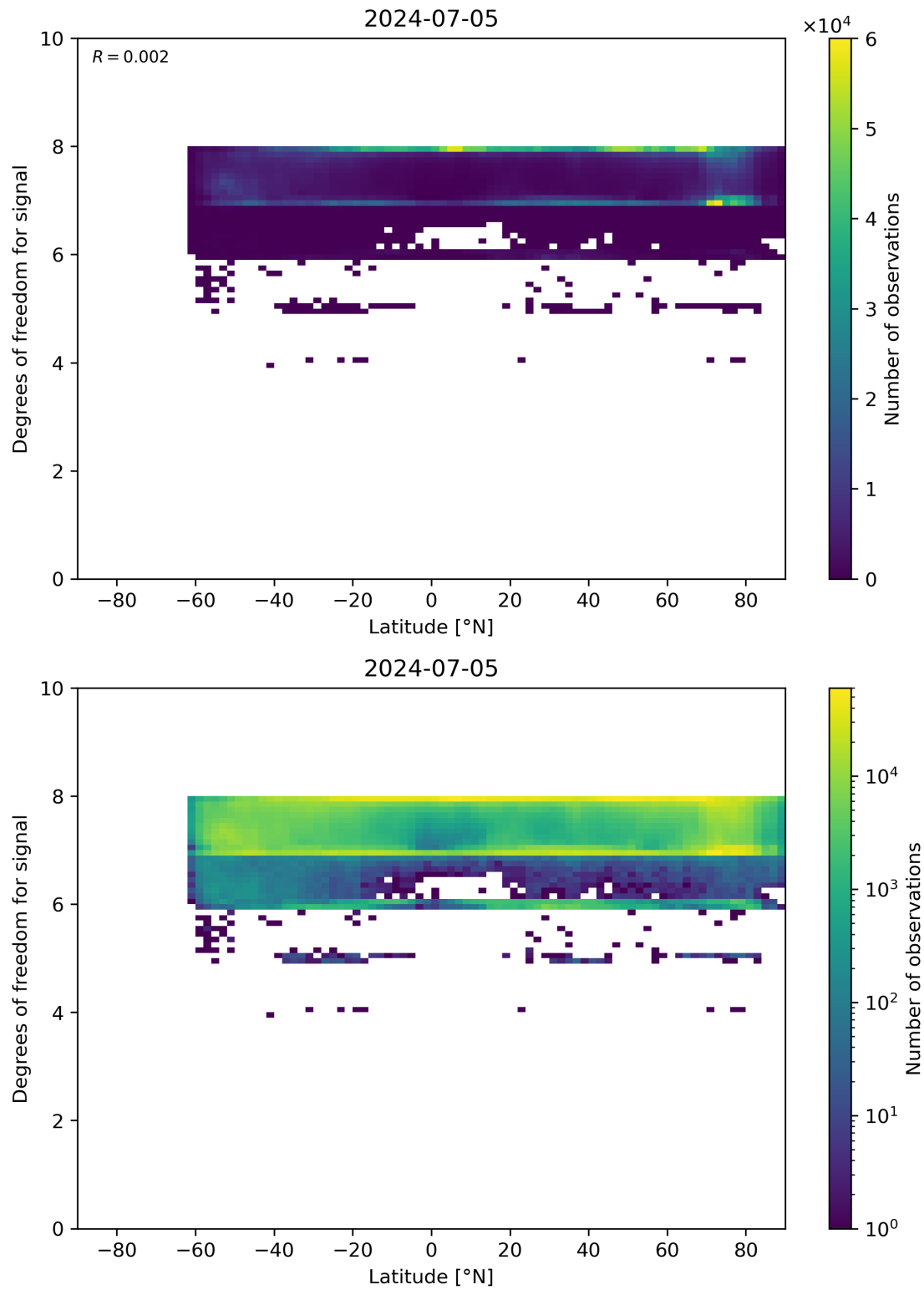
Figure 55: Scatter density plot of “Latitude” against “Degrees of freedom for signal” for 2024-07-05 to 2024-07-06.
