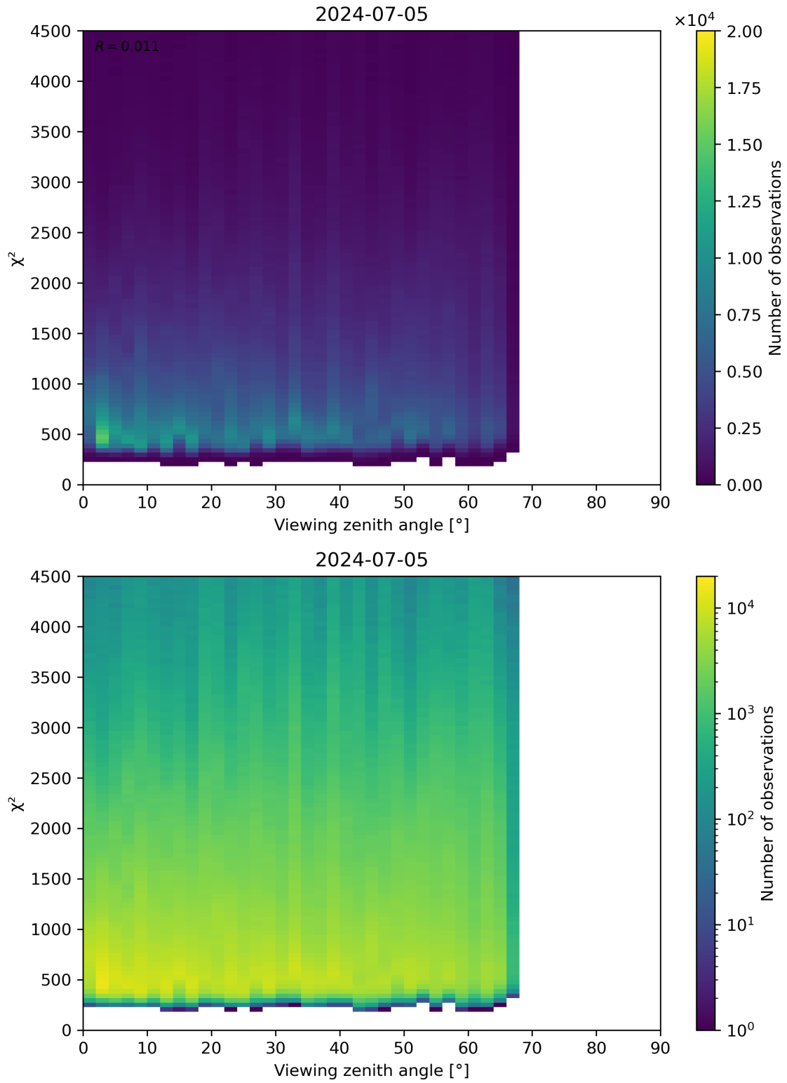
Figure 72: Scatter density plot of “Viewing zenith angle” against “ \chi^2 ” for 2024-07-05 to 2024-07-06.
