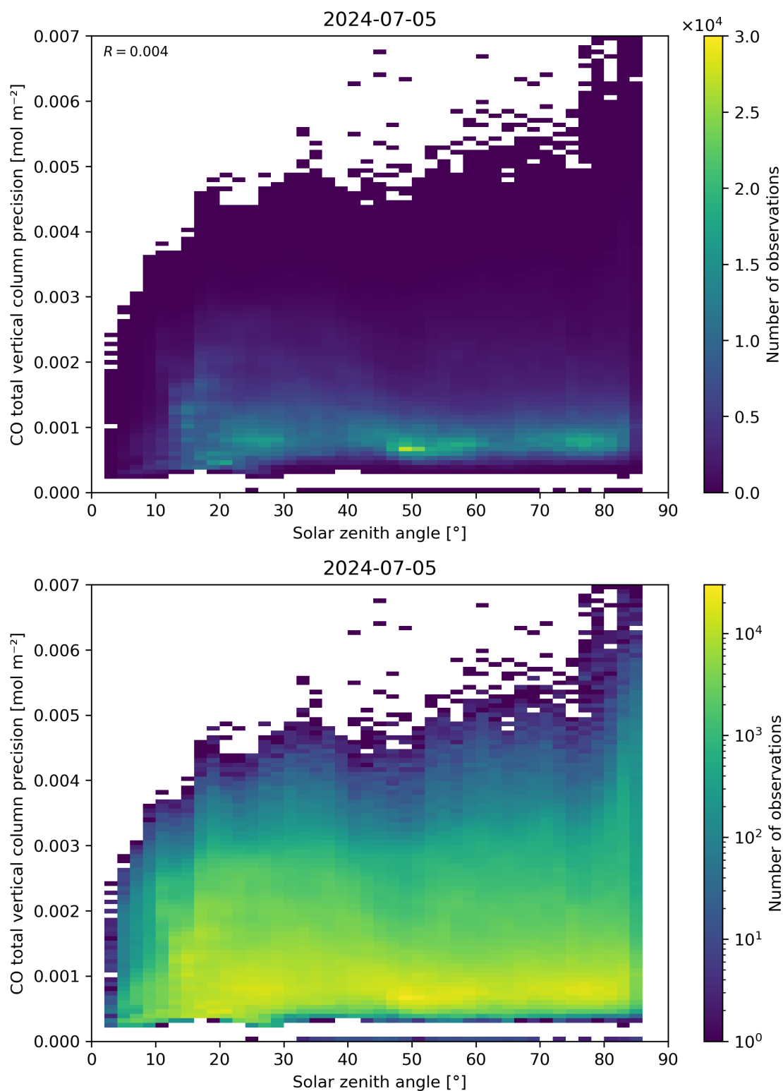
Figure 63: Scatter density plot of “Solar zenith angle” against “CO total vertical column precision” for 2024-07-05 to 2024-07-06.
