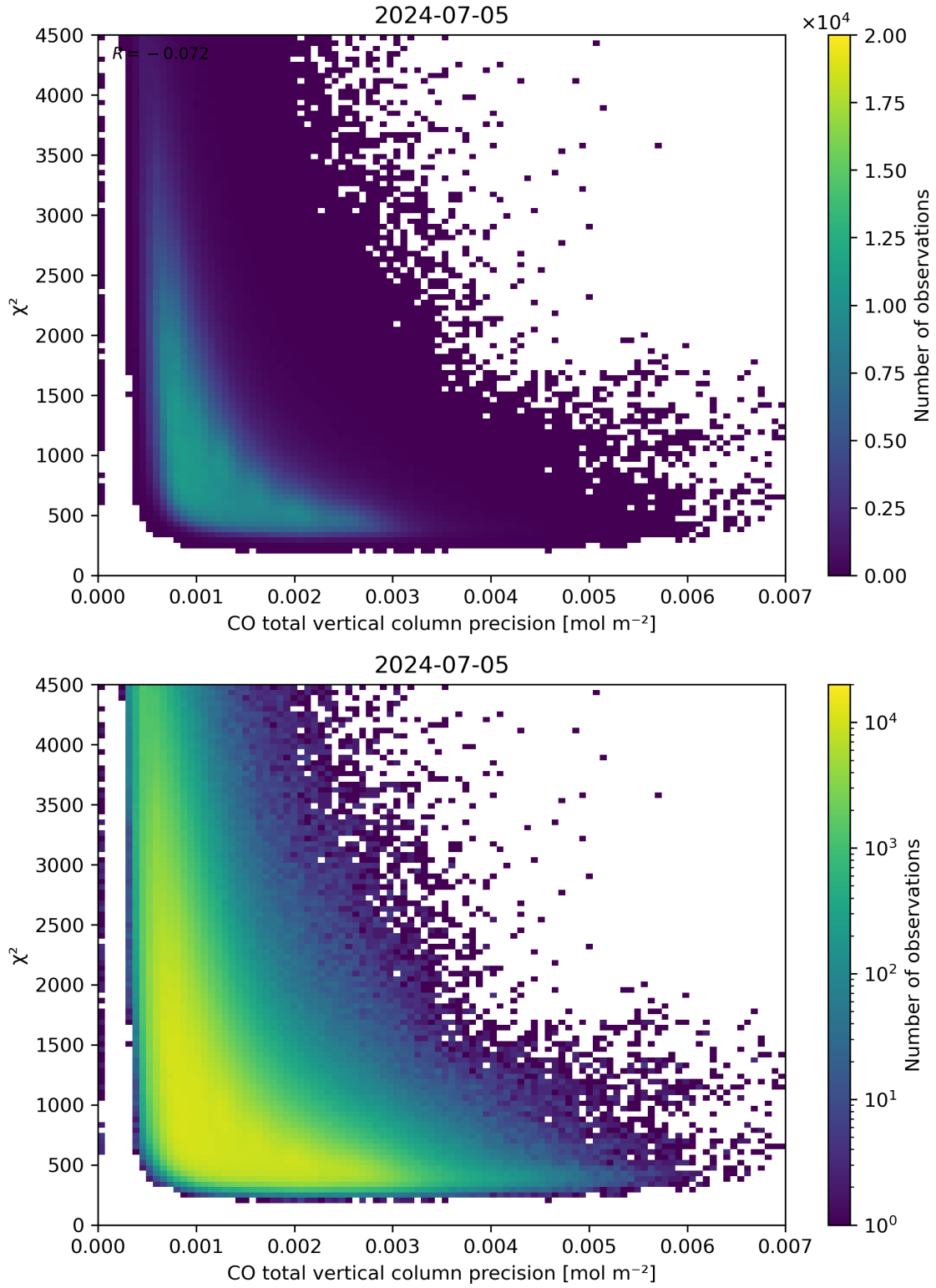
Figure 44: Scatter density plot of “CO total vertical column precision” against “ \chi^2 ” for 2024-07-05 to 2024-07-06.
