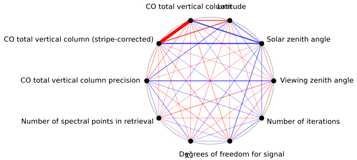
Figure 1: Map of correlation graph for 2024-07-05 to 2024-07-06.
