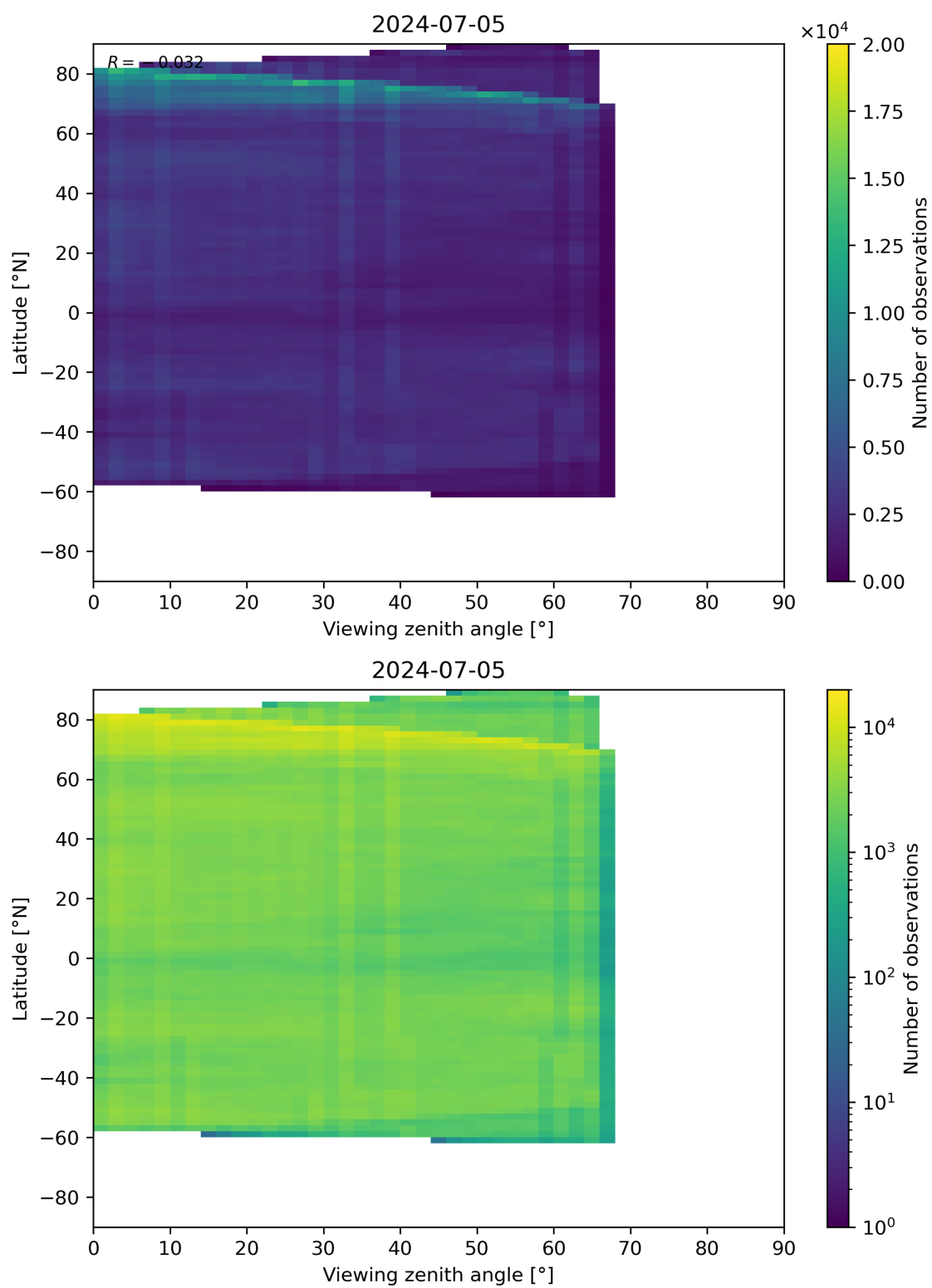
Figure 74: Scatter density plot of “Viewing zenith angle” against “Latitude” for 2024-07-05 to 2024-07-06.
