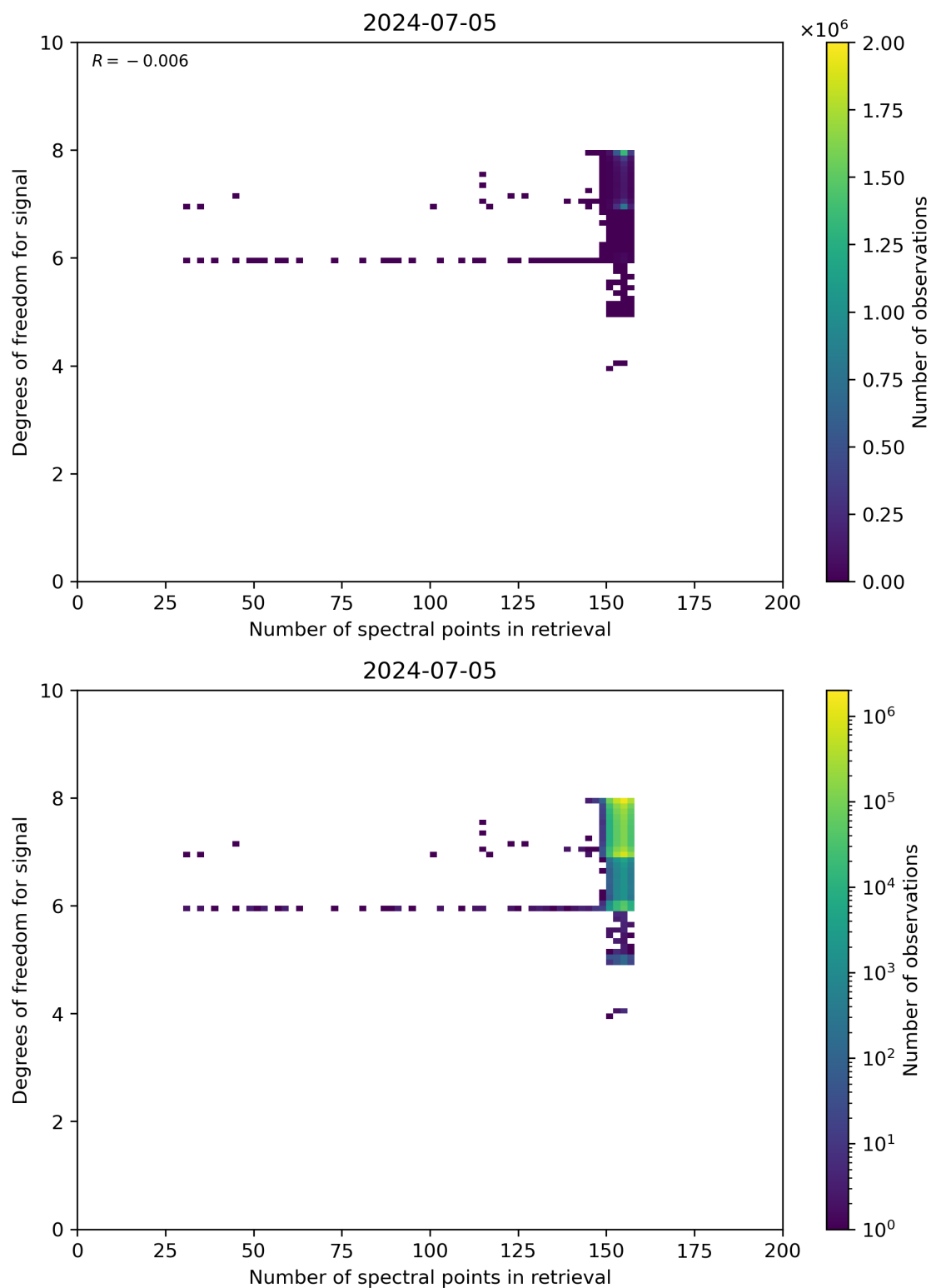
Figure 59: Scatter density plot of “Number of spectral points in retrieval” against “Degrees of freedom for signal” for 2024-07-05 to 2024-07-06.
