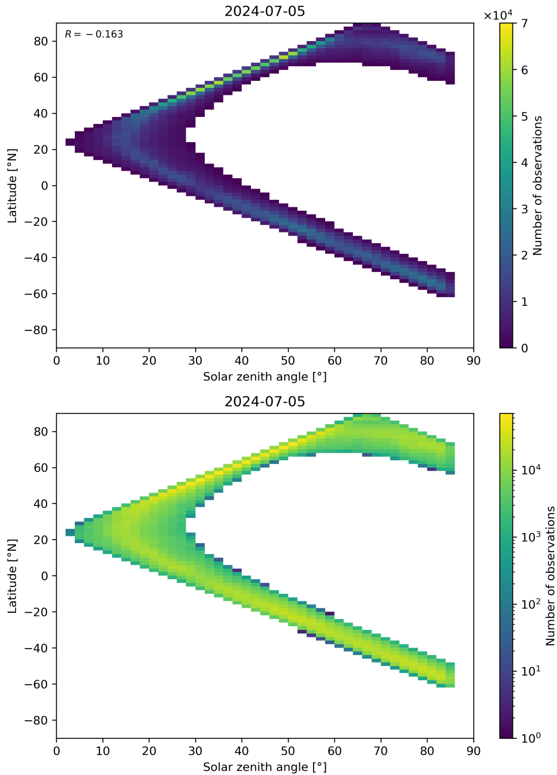
Figure 66: Scatter density plot of “Solar zenith angle” against “Latitude” for 2024-07-05 to 2024-07-06.
