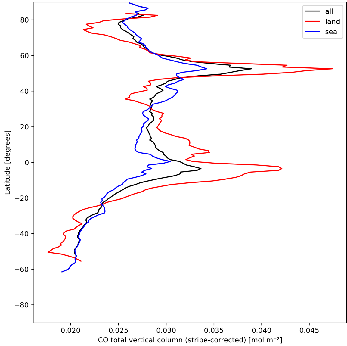
Figure 11: Zonal average of “CO total vertical column (stripe-corrected)” for 2024-07-05 to 2024-07-06.
