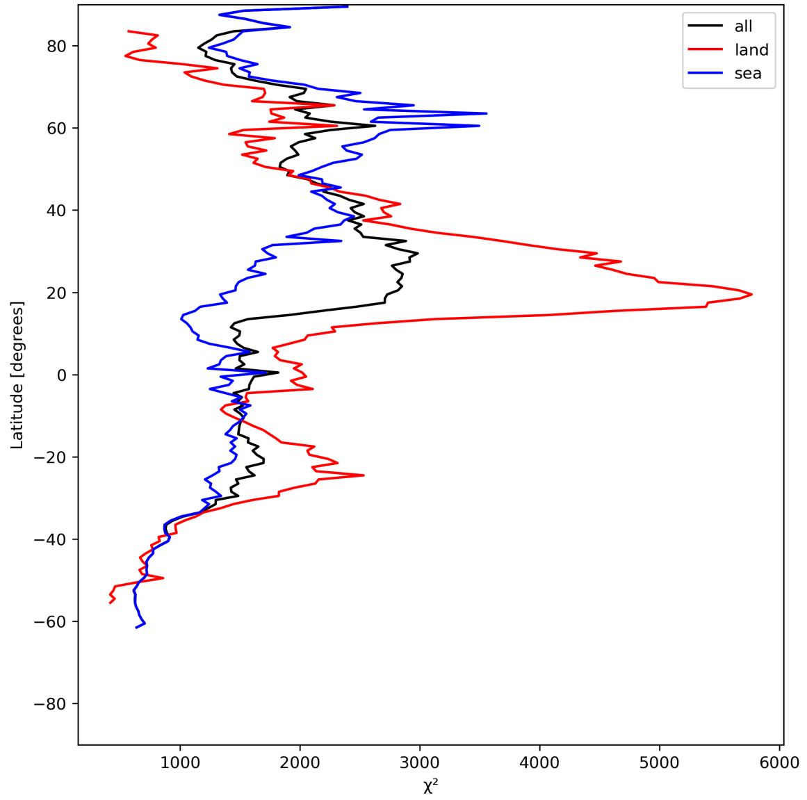
Figure 14: Zonal average of “ \chi^2 ” for 2024-07-05 to 2024-07-06.
