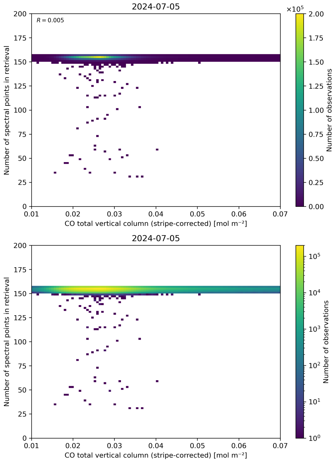
Figure 40: Scatter density plot of “CO total vertical column (stripe-corrected)” against “Number of spectral points in retrieval” for 2024-07-05 to 2024-07-06.
