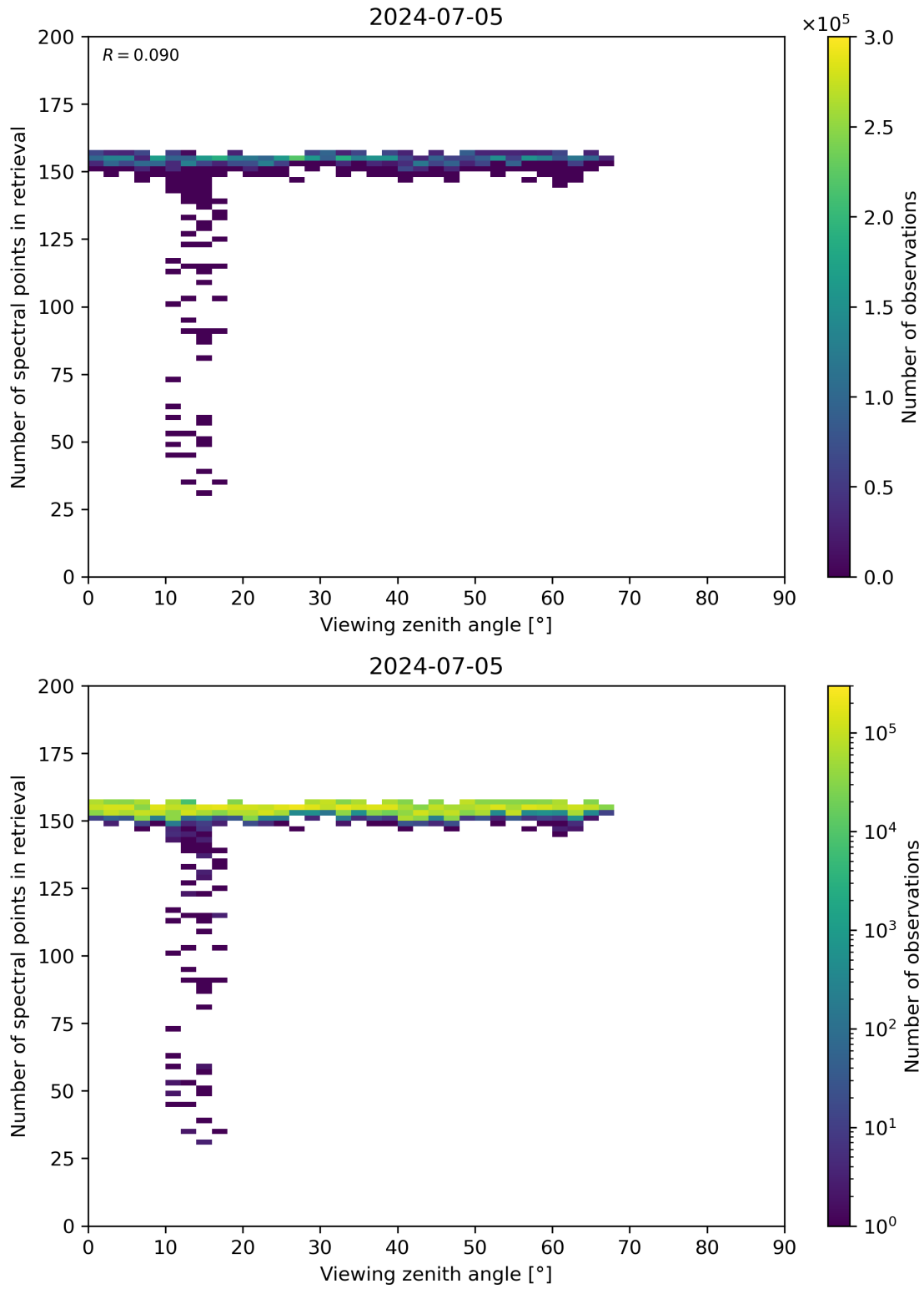
Figure 76: Scatter density plot of “Viewing zenith angle” against “Number of spectral points in retrieval” for 2024-07-05 to 2024-07-06.
