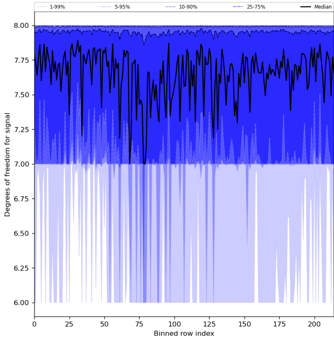
Figure 31: Along track statistics of “Degrees of freedom for signal” for 2024-07-05 to 2024-07-06
