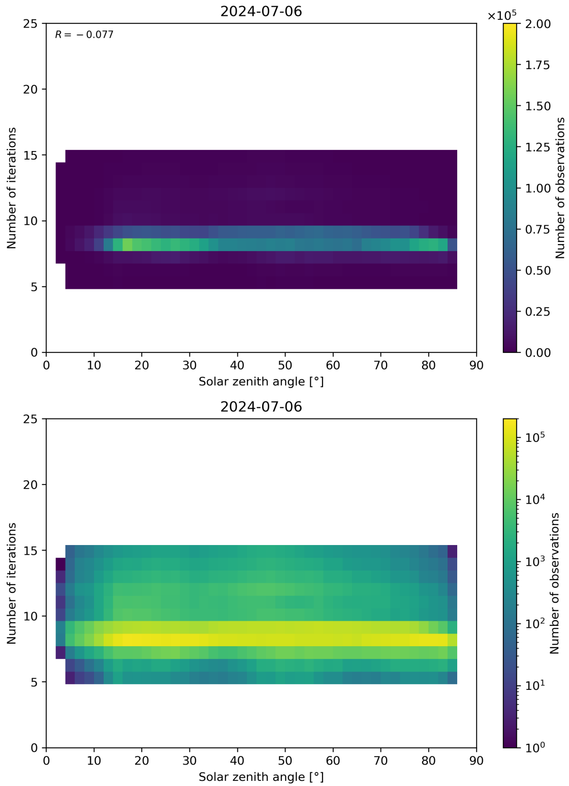
Figure 67: Scatter density plot of “Solar zenith angle” against “Number of iterations” for 2024-07-05 to 2024-07-07.
