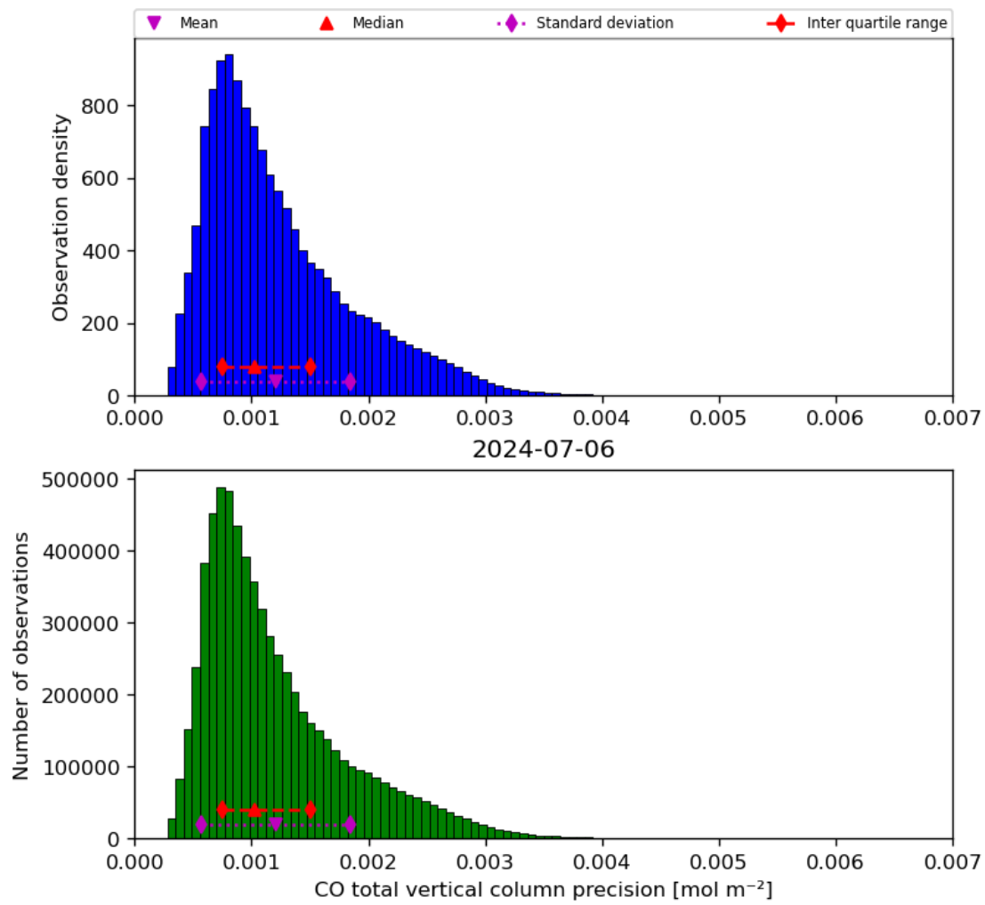
Figure 20: Histogram of “CO total vertical column precision” for 2024-07-05 to 2024-07-07
