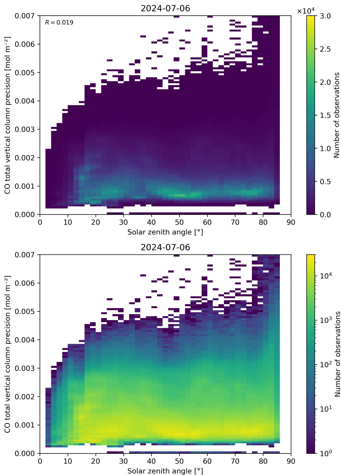
Figure 63: Scatter density plot of “Solar zenith angle” against “CO total vertical column precision” for 2024-07-05 to 2024-07-07.
