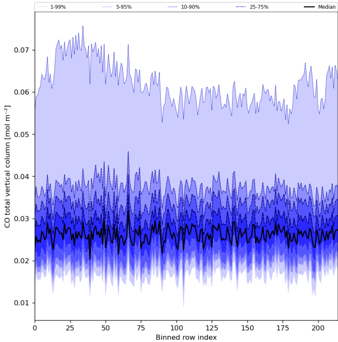
Figure 26: Along track statistics of “CO total vertical column” for 2024-07-05 to 2024-07-07
