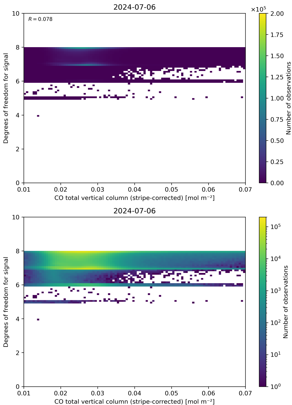
Figure 38: Scatter density plot of “CO total vertical column (stripe-corrected)” against “Degrees of freedom for signal” for 2024-07-05 to 2024-07-07.
