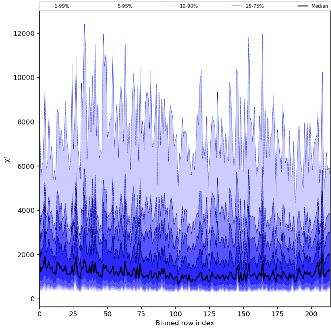
Figure 30: Along track statistics of “ \chi^2 ” for 2024-07-05 to 2024-07-07
