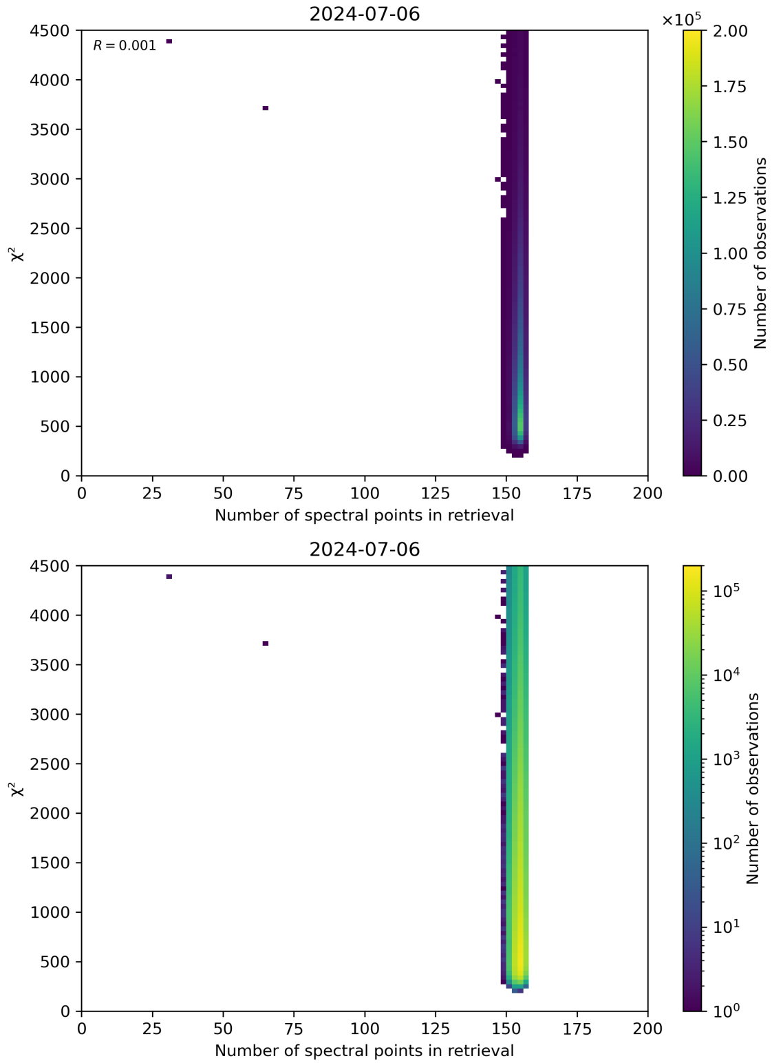
Figure 58: Scatter density plot of “Number of spectral points in retrieval” against “ \chi^2 ” for 2024-07-05 to 2024-07-07.
