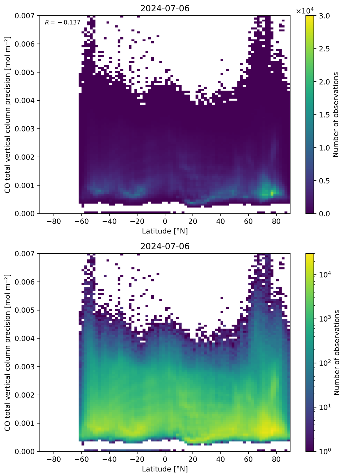
Figure 53: Scatter density plot of “Latitude” against “CO total vertical column precision” for 2024-07-05 to 2024-07-07.
