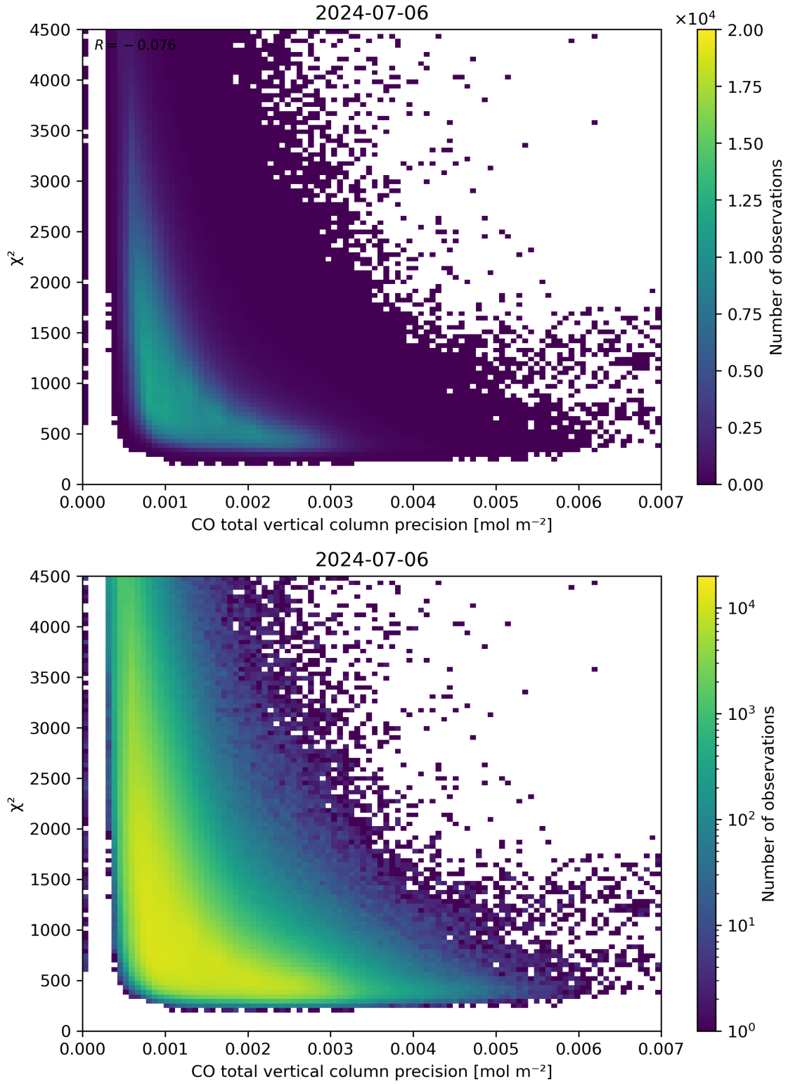
Figure 44: Scatter density plot of “CO total vertical column precision” against “ \chi^2 ” for 2024-07-05 to 2024-07-07.
