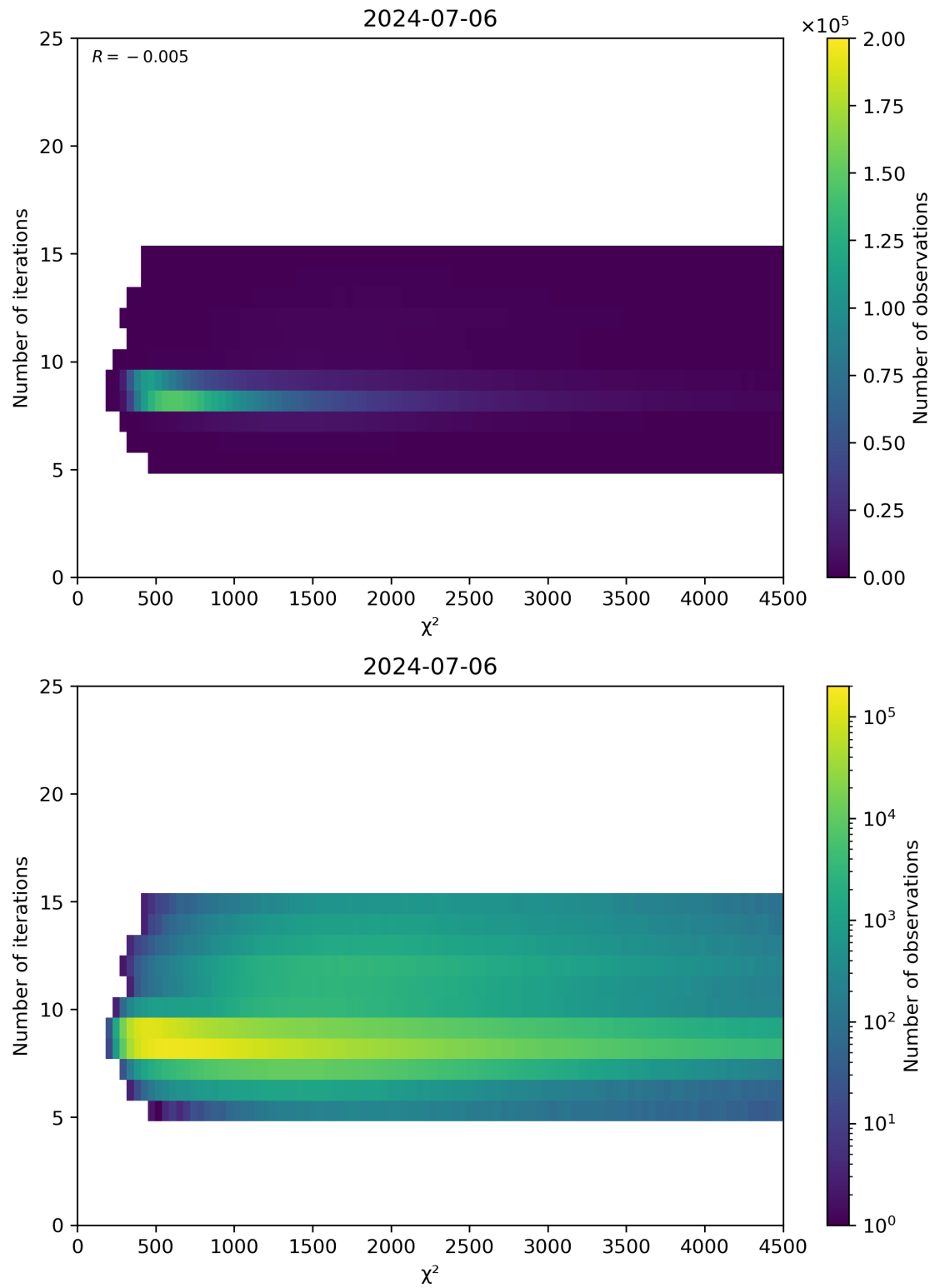
Figure 49: Scatter density plot of “ \chi^2 ” against “Number of iterations” for 2024-07-05 to 2024-07-07.
