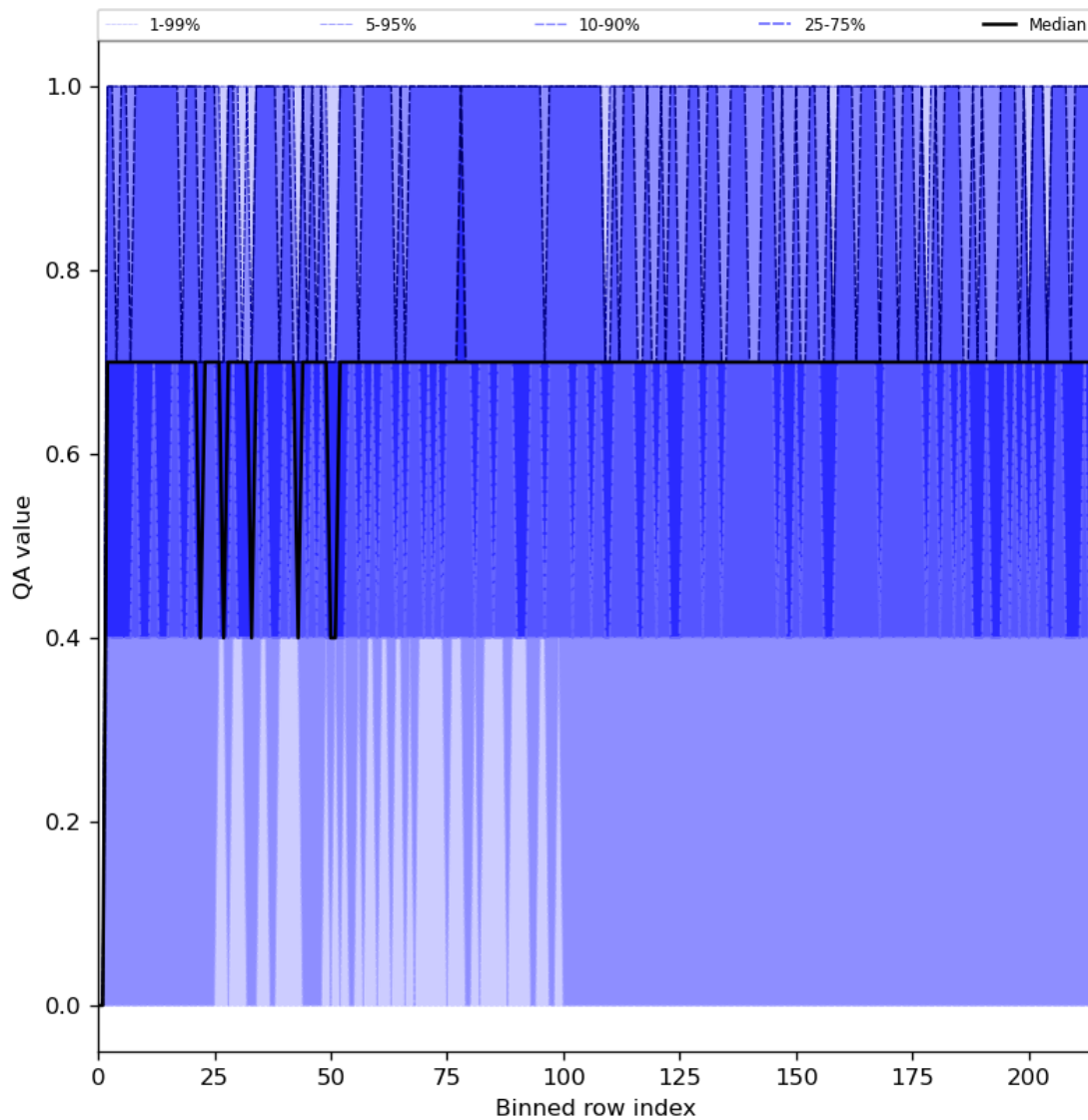
Figure 25: Along track statistics of “QA value” for 2024-07-05 to 2024-07-07
