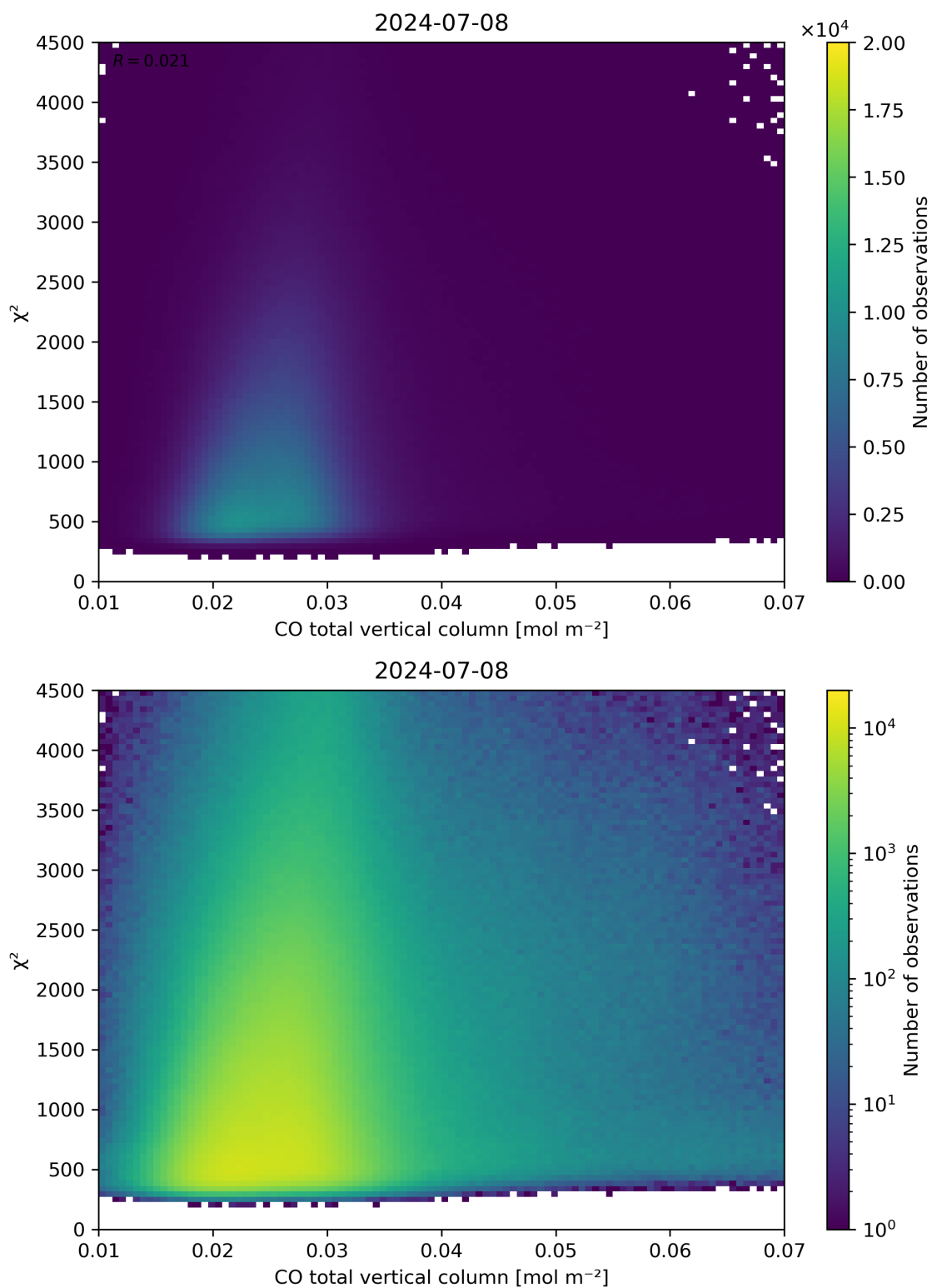
Figure 35: Scatter density plot of “CO total vertical column” against “ \chi^2 ” for 2024-07-07 to 2024-07-09.
