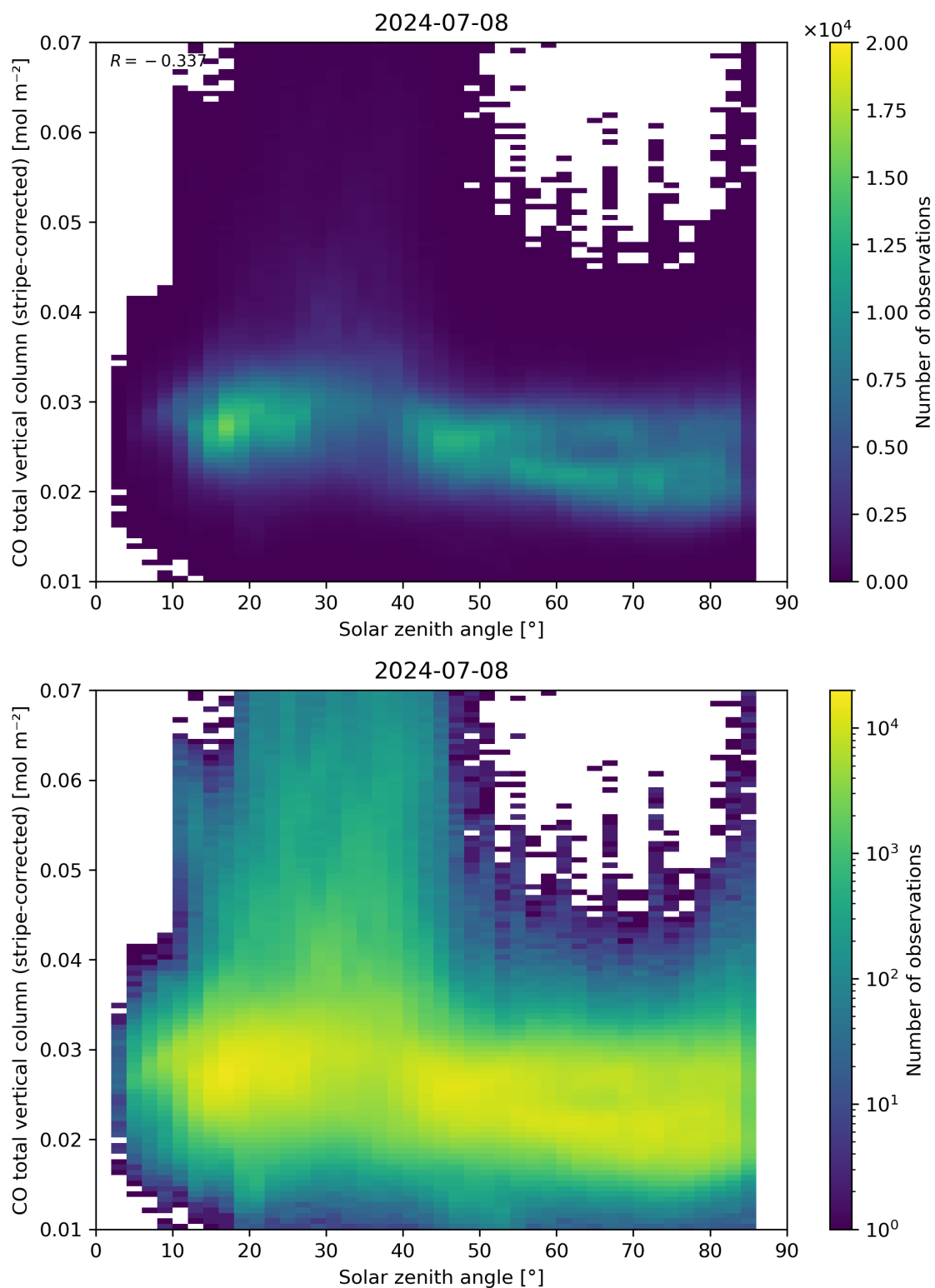
Figure 62: Scatter density plot of “Solar zenith angle” against “CO total vertical column (stripe-corrected)” for 2024-07-07 to 2024-07-09.
