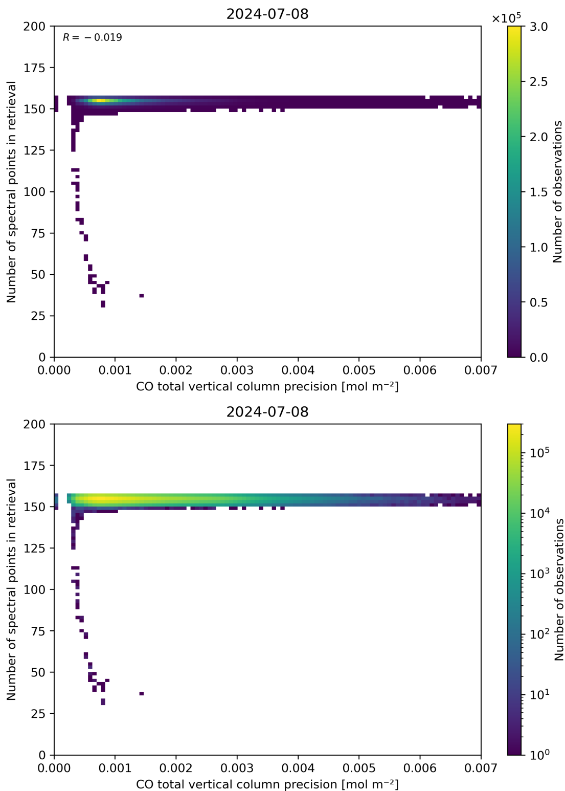
Figure 47: Scatter density plot of “CO total vertical column precision” against “Number of spectral points in retrieval” for 2024-07-07 to 2024-07-09.
