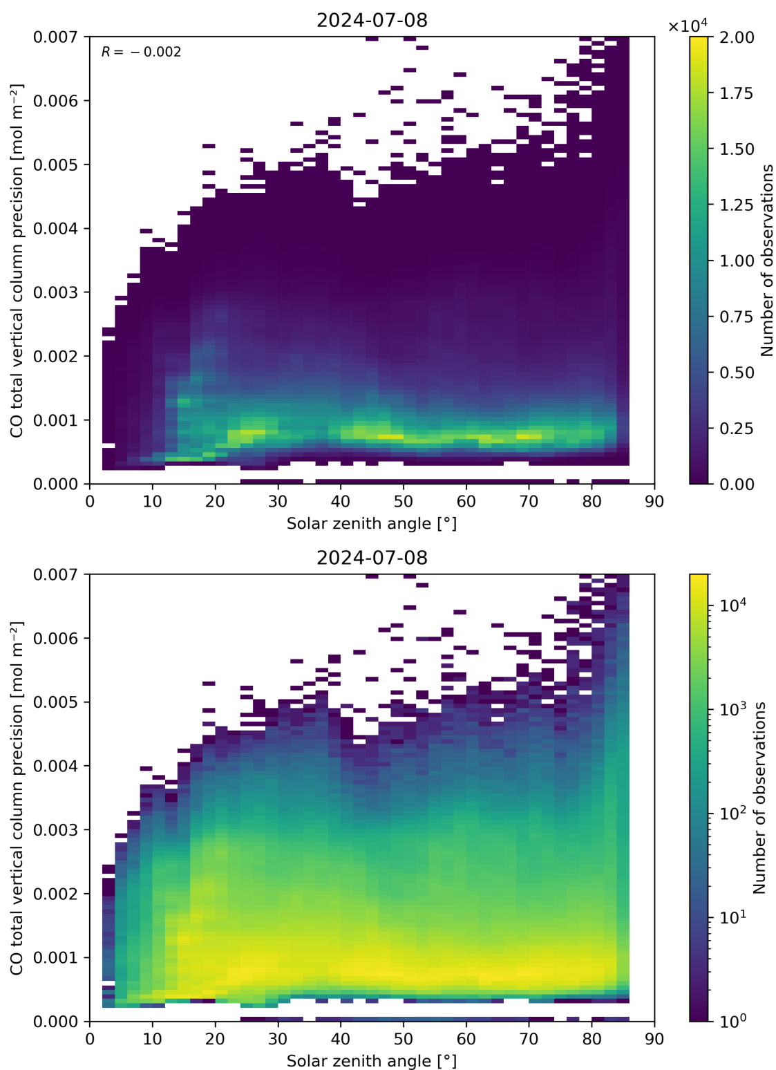
Figure 63: Scatter density plot of “Solar zenith angle” against “CO total vertical column precision” for 2024-07-07 to 2024-07-09.
