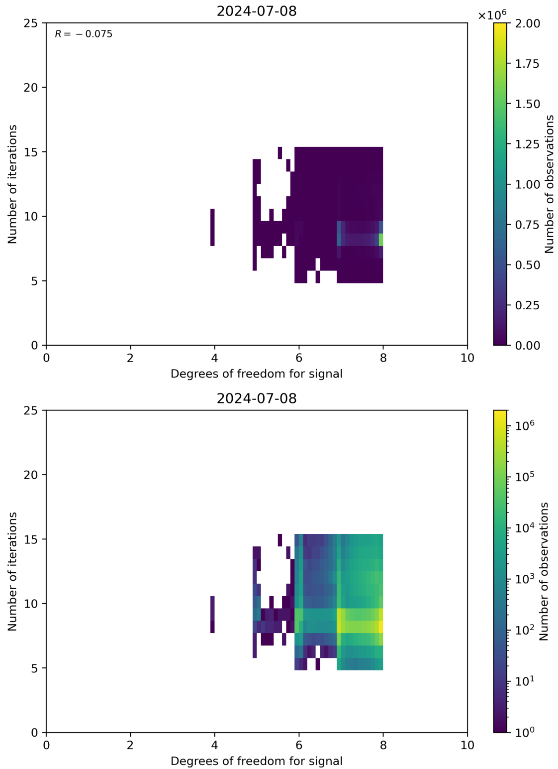
Figure 50: Scatter density plot of “Degrees of freedom for signal” against “Number of iterations” for 2024-07-07 to 2024-07-09.
