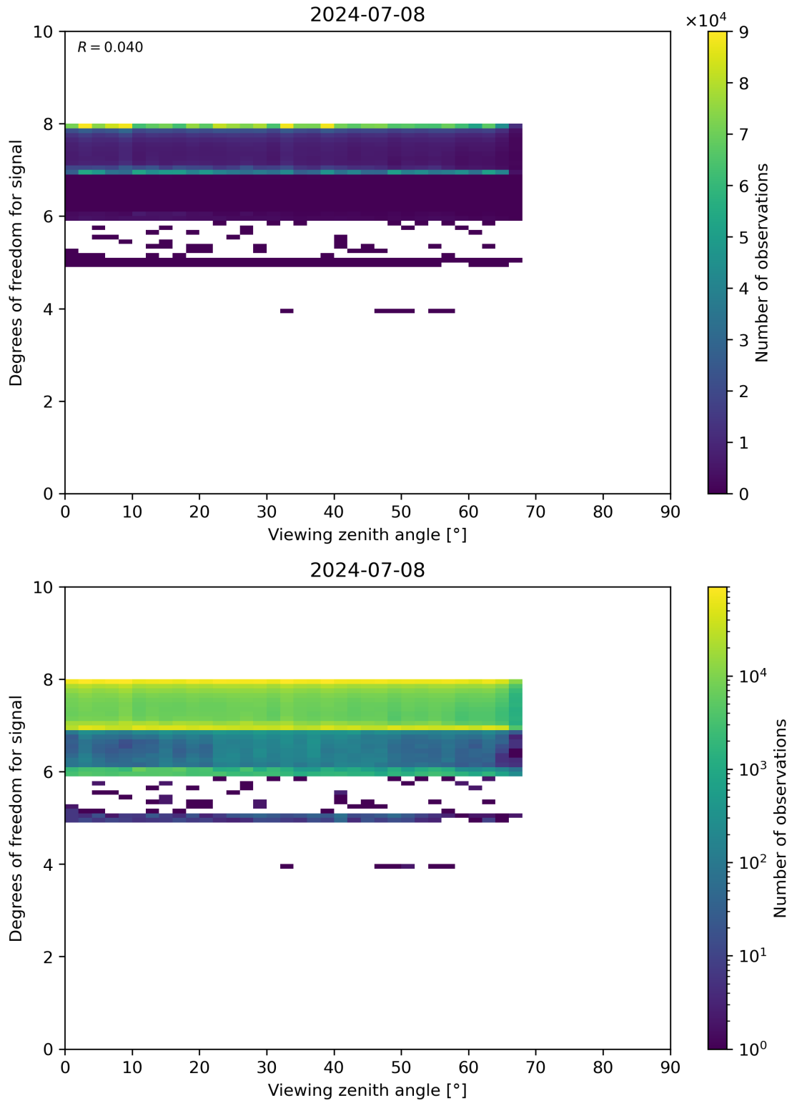
Figure 73: Scatter density plot of “Viewing zenith angle” against “Degrees of freedom for signal” for 2024-07-07 to 2024-07-09.
