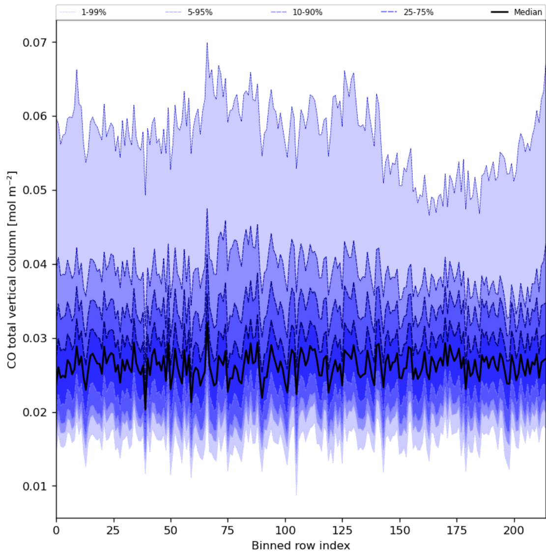
Figure 26: Along track statistics of “CO total vertical column” for 2024-07-07 to 2024-07-09
