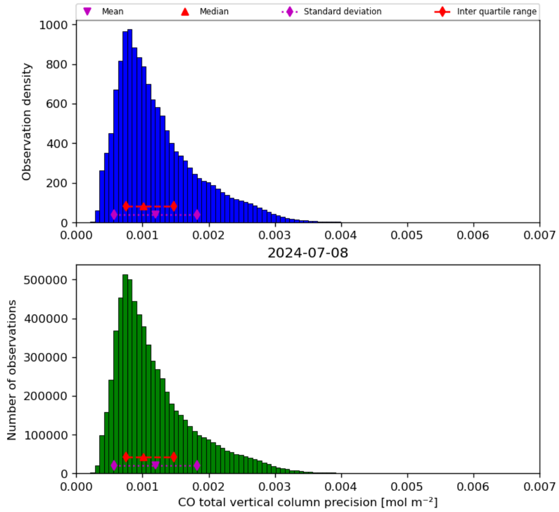
Figure 20: Histogram of “CO total vertical column precision” for 2024-07-07 to 2024-07-09
