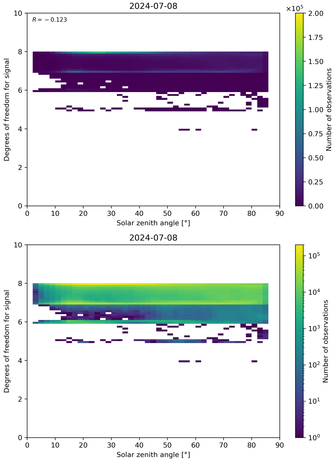
Figure 65: Scatter density plot of “Solar zenith angle” against “Degrees of freedom for signal” for 2024-07-07 to 2024-07-09.
