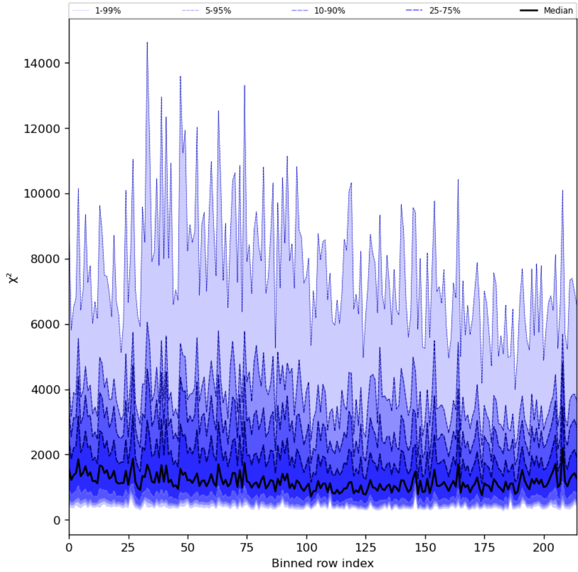
Figure 30: Along track statistics of “ \chi^2 ” for 2024-07-07 to 2024-07-09
