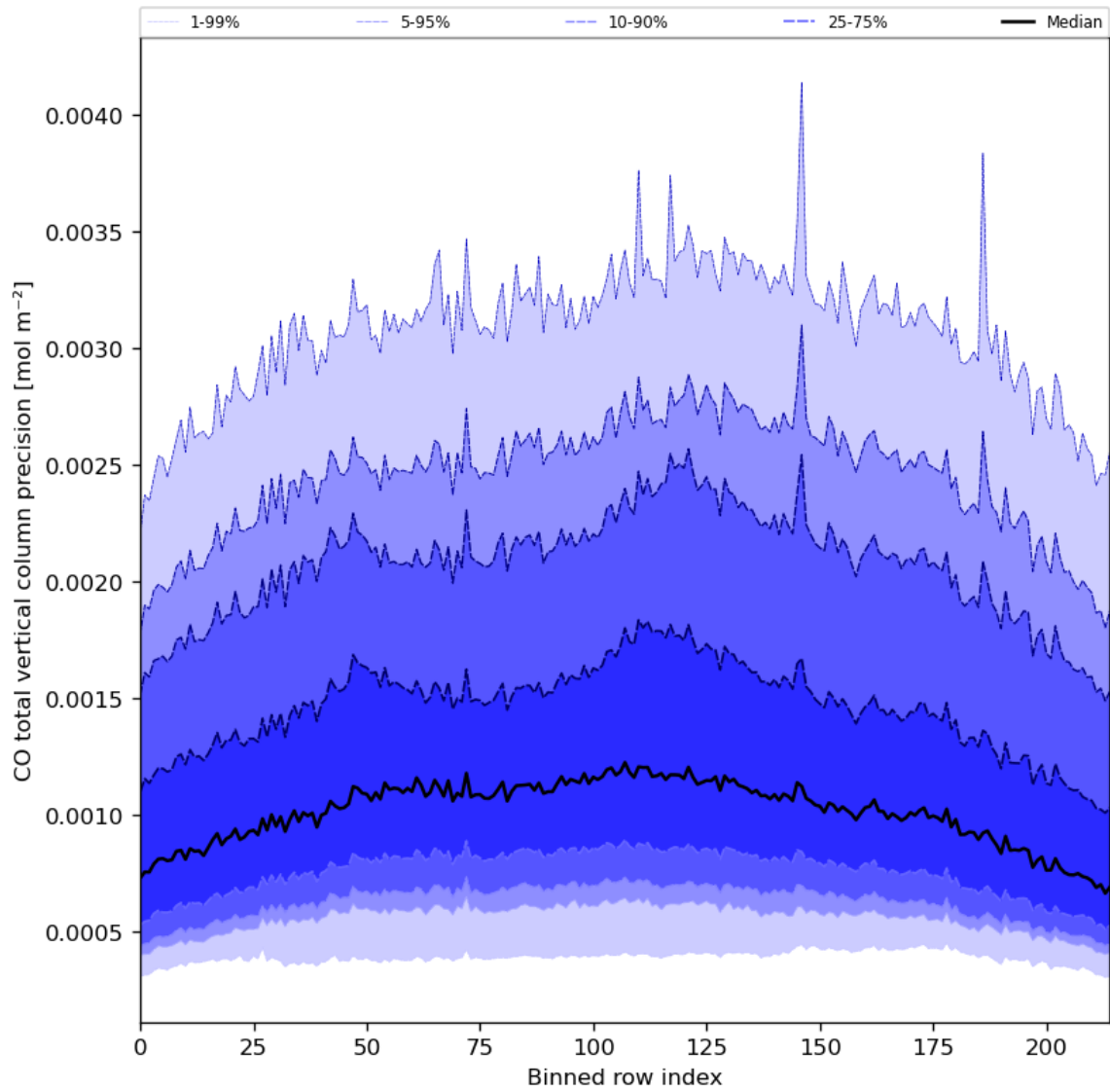
Figure 28: Along track statistics of “CO total vertical column precision” for 2024-07-07 to 2024-07-09
