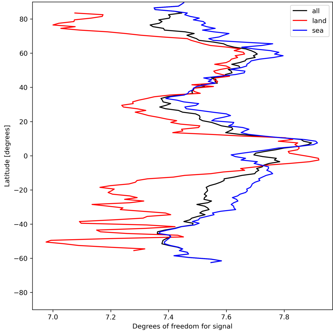
Figure 15: Zonal average of “Degrees of freedom for signal” for 2024-07-07 to 2024-07-09.
