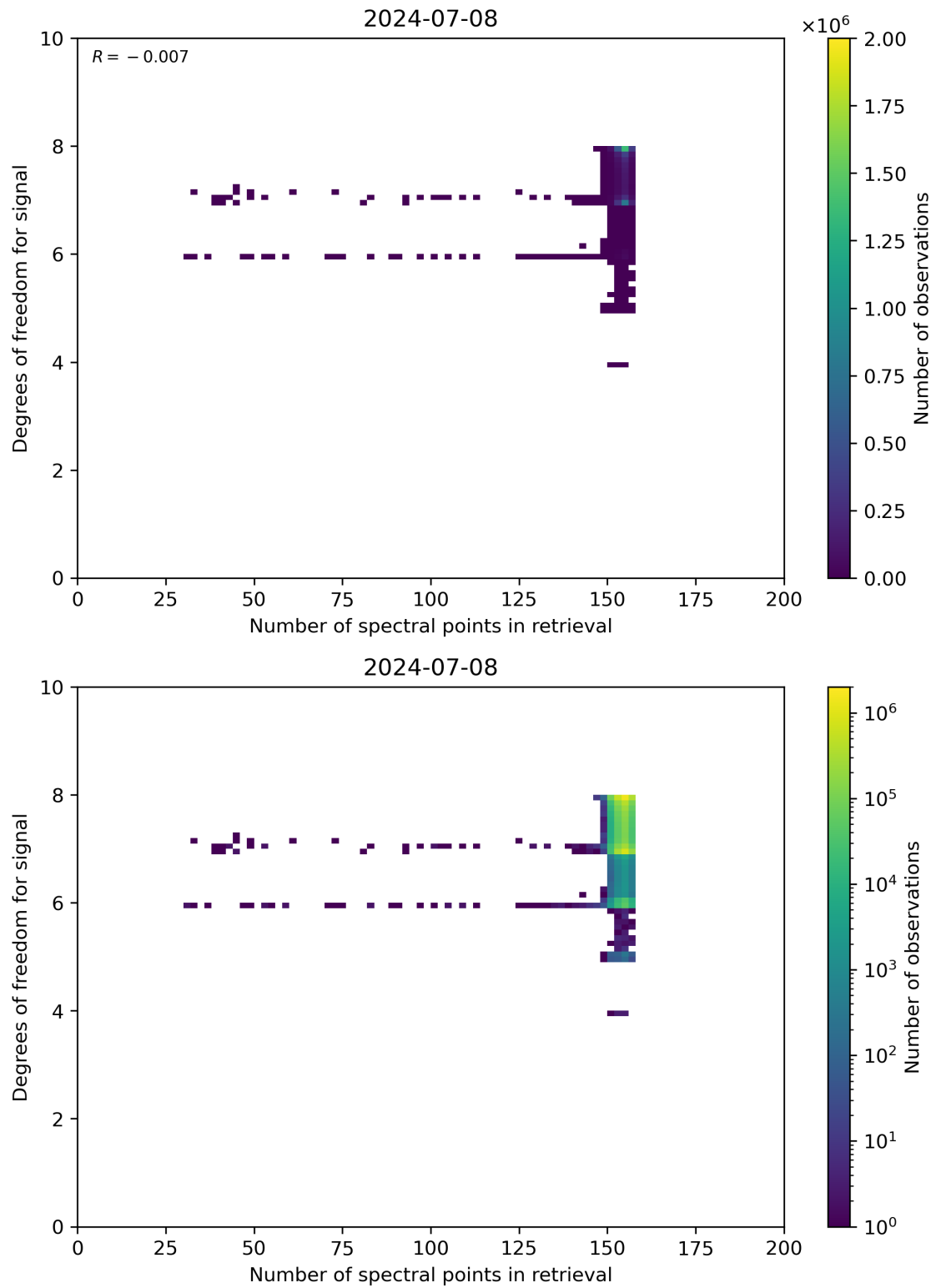
Figure 59: Scatter density plot of “Number of spectral points in retrieval” against “Degrees of freedom for signal” for 2024-07-07 to 2024-07-09.
