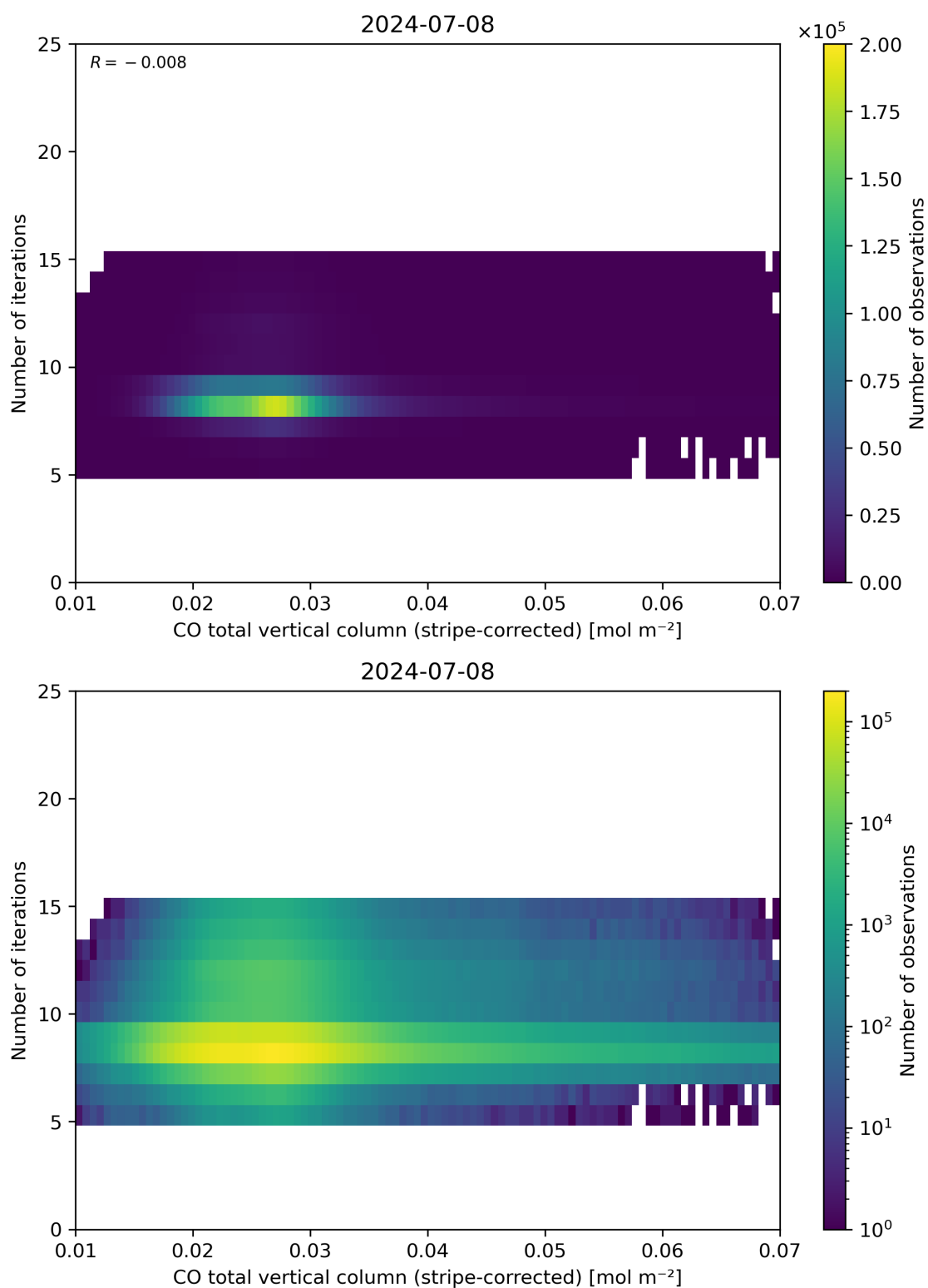
Figure 39: Scatter density plot of “CO total vertical column (stripe-corrected)” against “Number of iterations” for 2024-07-07 to 2024-07-09.
