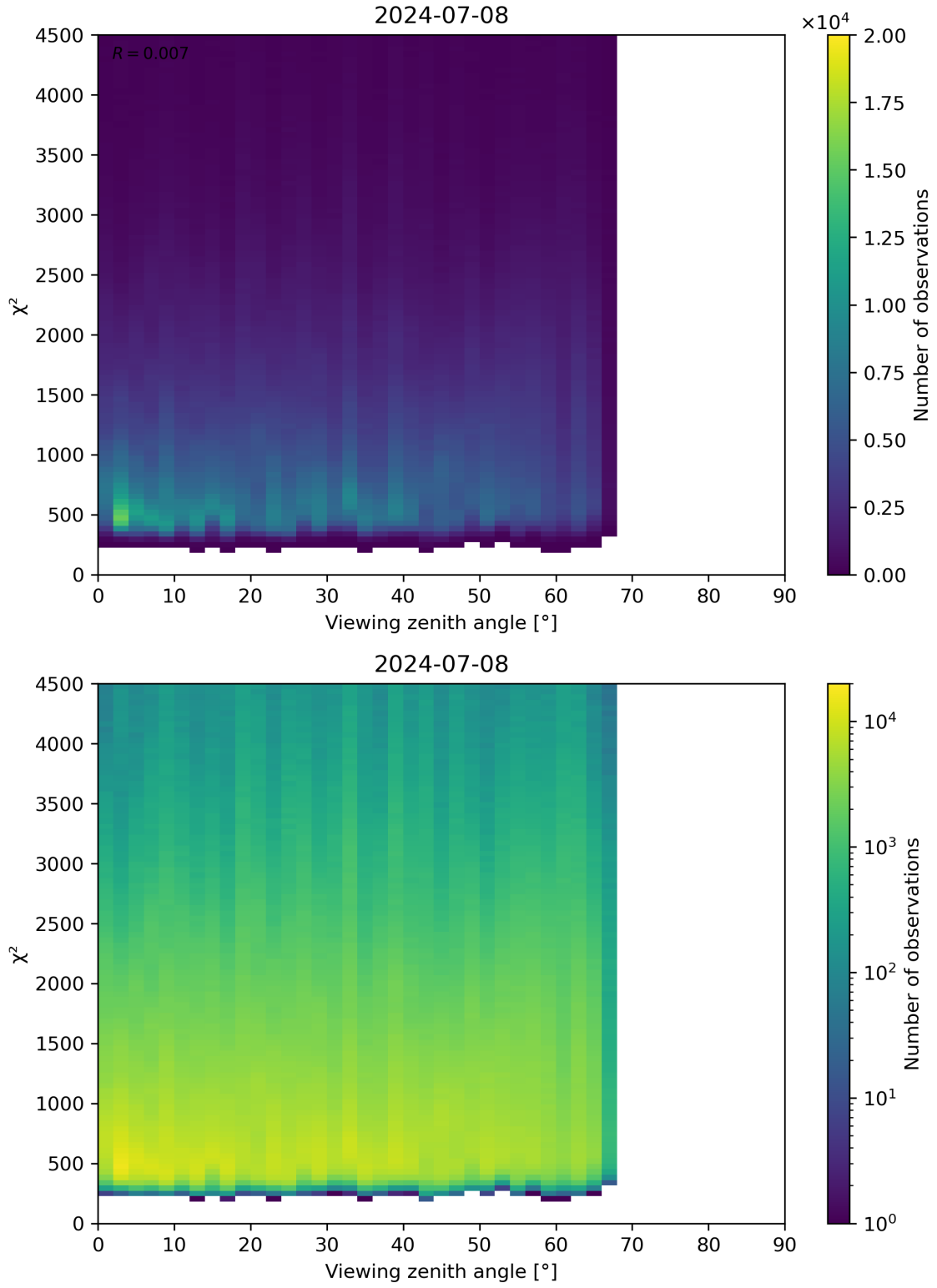
Figure 72: Scatter density plot of “Viewing zenith angle” against “ \chi^2 ” for 2024-07-07 to 2024-07-09.
