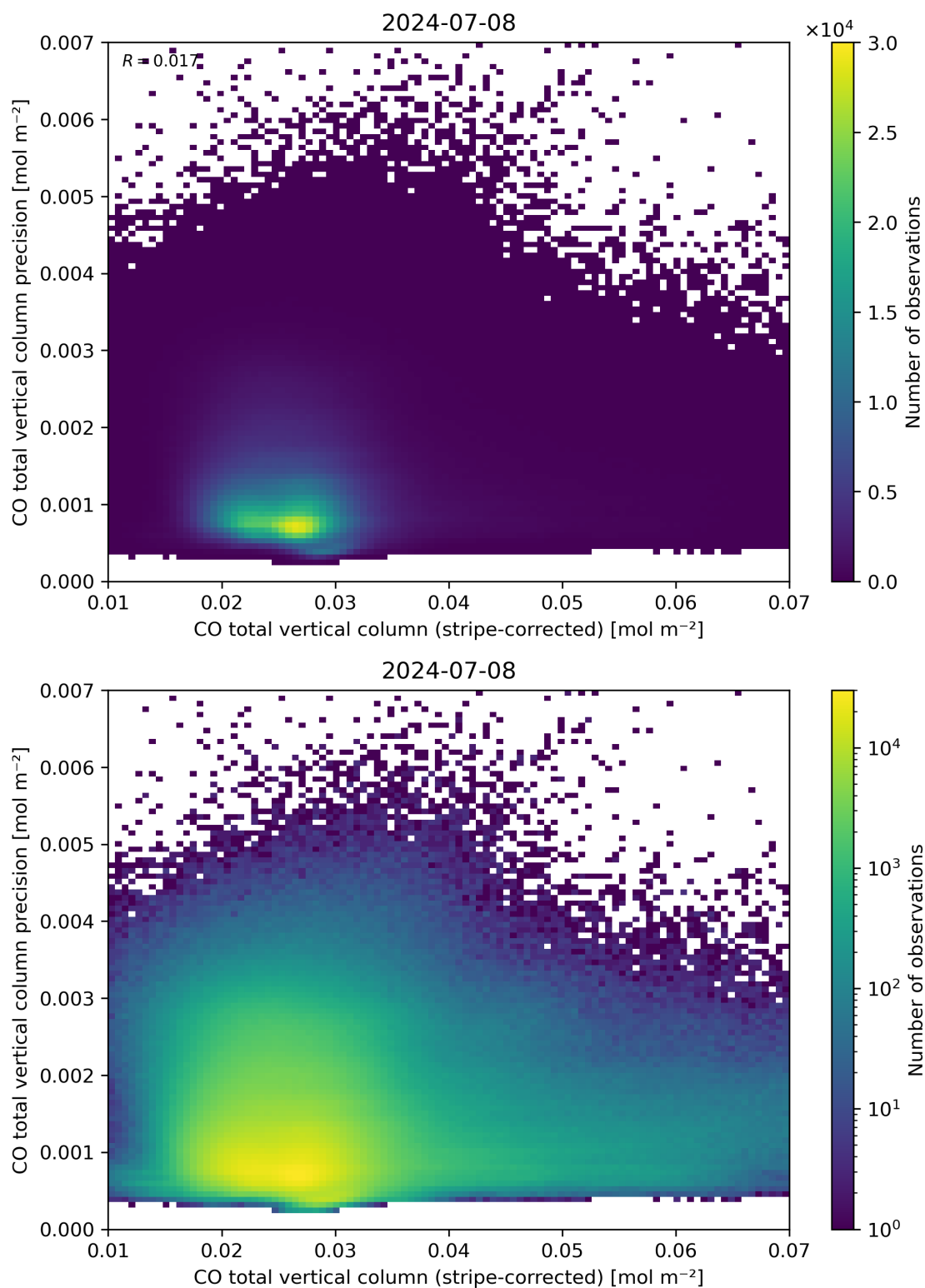
Figure 36: Scatter density plot of “CO total vertical column (stripe-corrected)” against “CO total vertical column precision” for 2024-07-07 to 2024-07-09.
