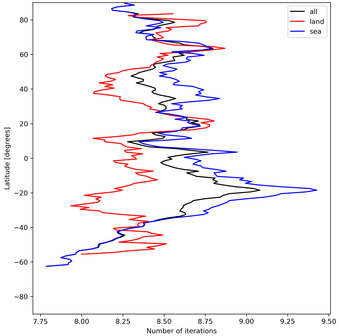
Figure 16: Zonal average of “Number of iterations” for 2024-07-07 to 2024-07-09.
