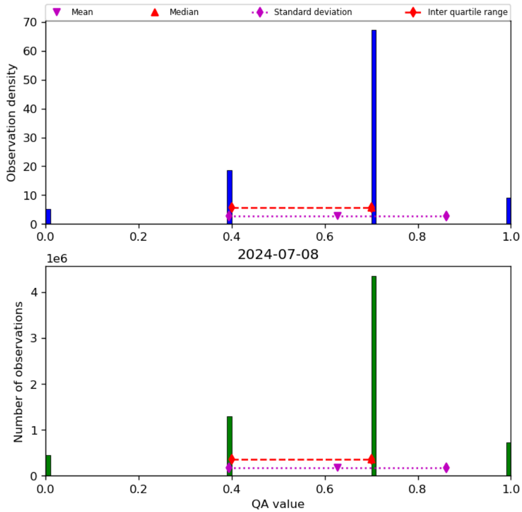
Figure 17: Histogram of “QA value” for 2024-07-07 to 2024-07-09
