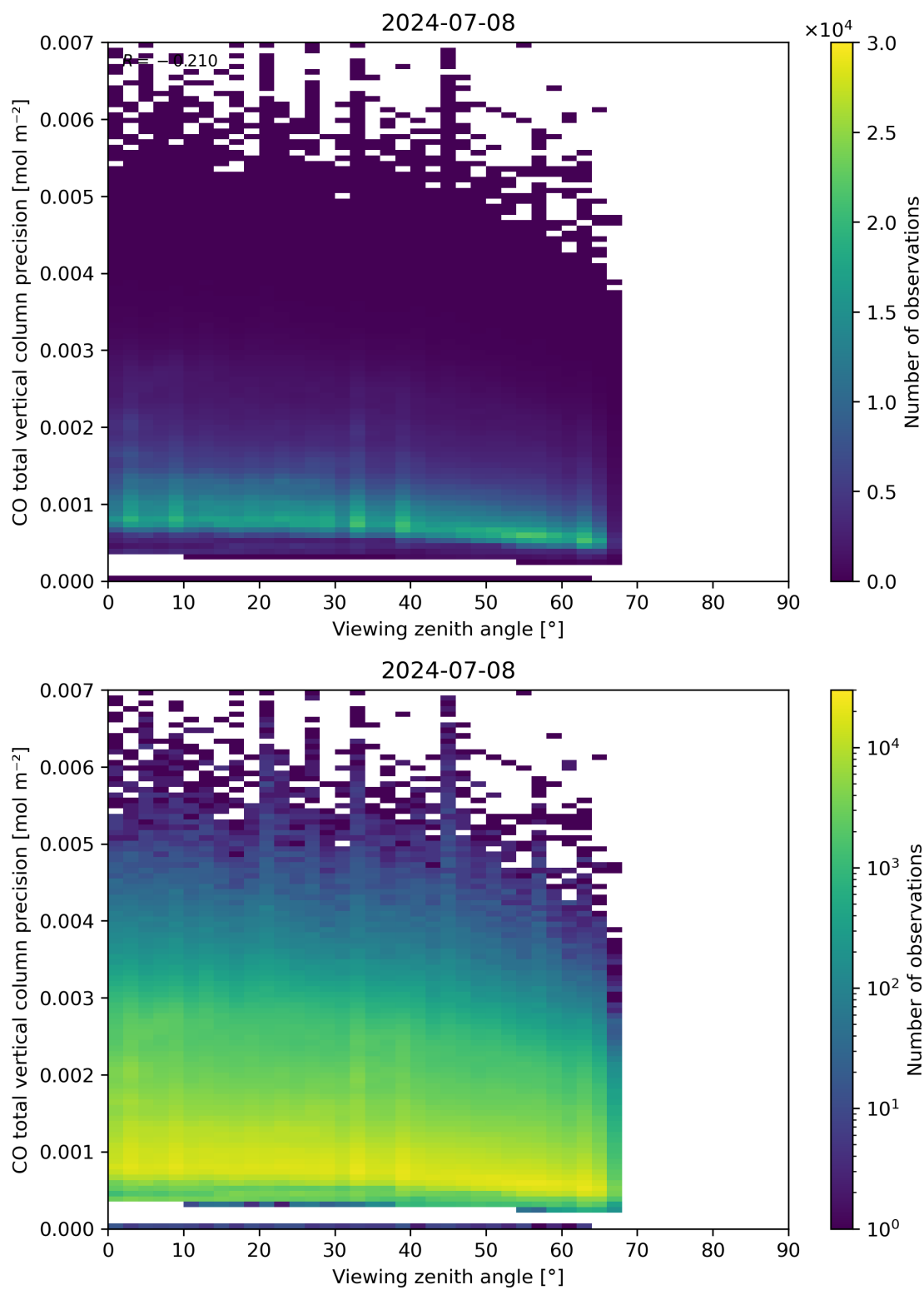
Figure 71: Scatter density plot of “Viewing zenith angle” against “CO total vertical column precision” for 2024-07-07 to 2024-07-09.
