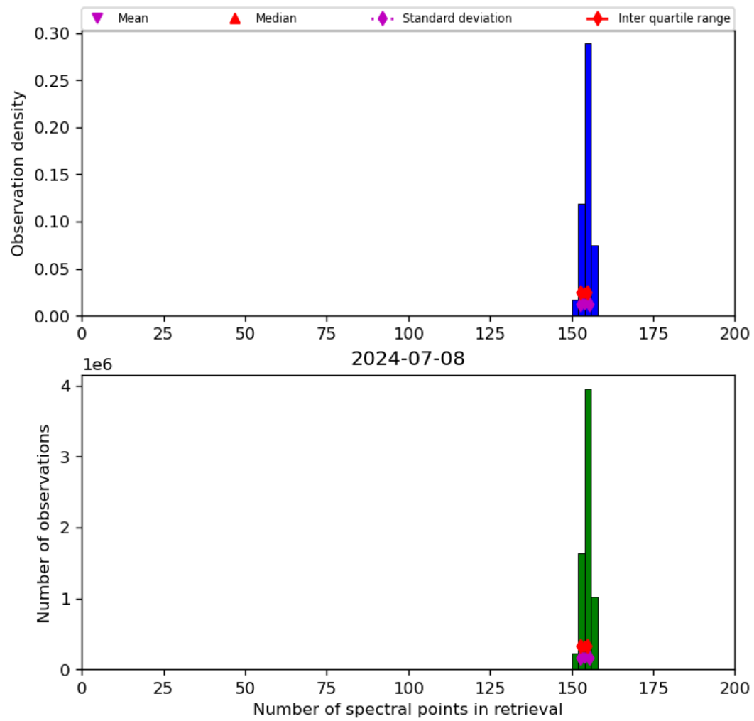
Figure 21: Histogram of “Number of spectral points in retrieval” for 2024-07-07 to 2024-07-09
