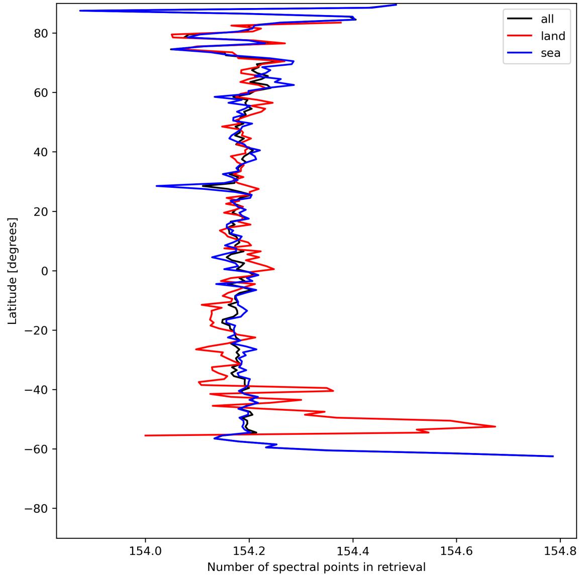
Figure 13: Zonal average of “Number of spectral points in retrieval” for 2024-07-07 to 2024-07-09.
