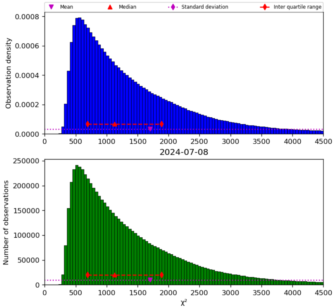
Figure 22: Histogram of “ \chi^2 ” for 2024-07-07 to 2024-07-09
