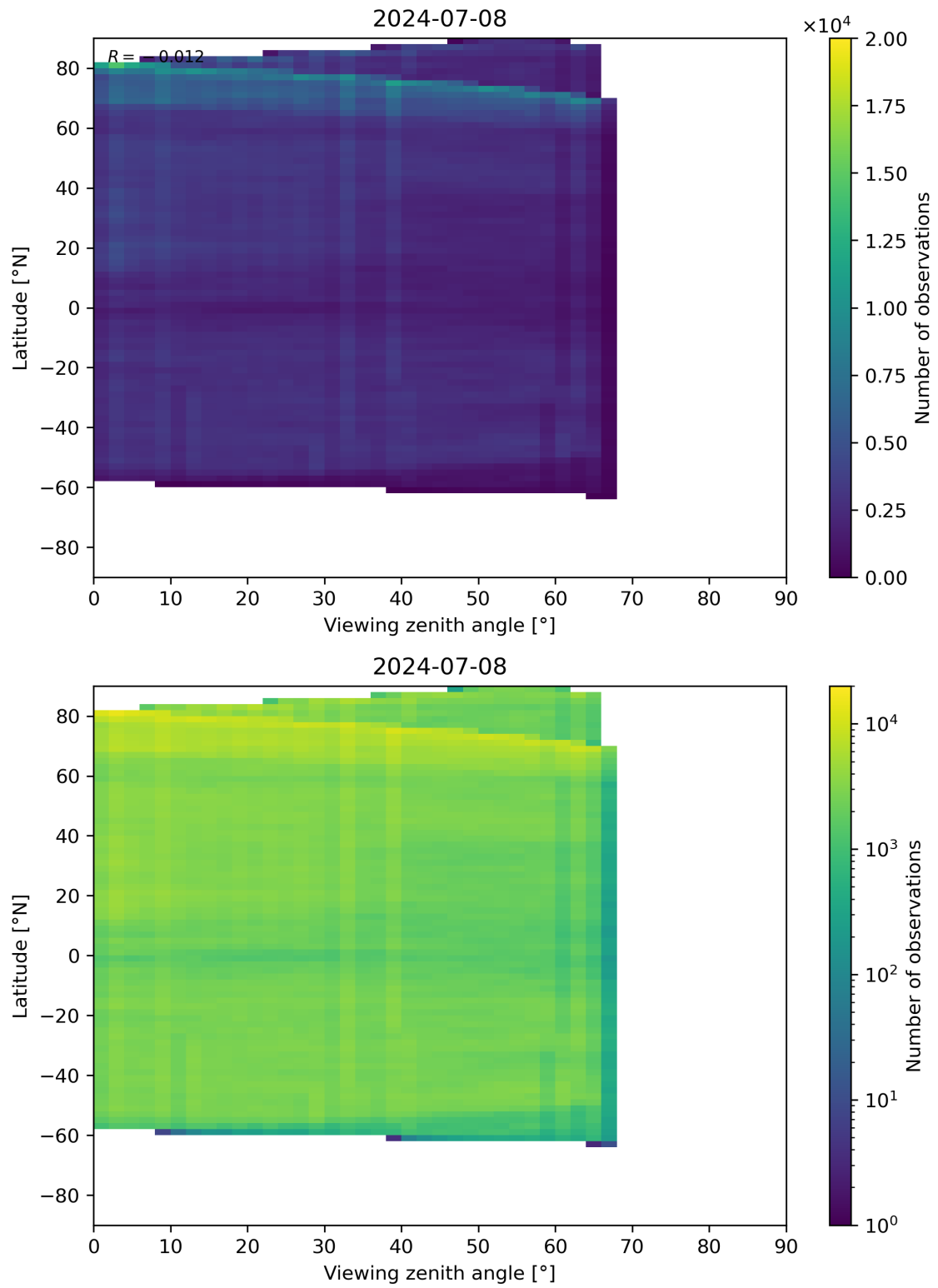
Figure 74: Scatter density plot of “Viewing zenith angle” against “Latitude” for 2024-07-07 to 2024-07-09.
