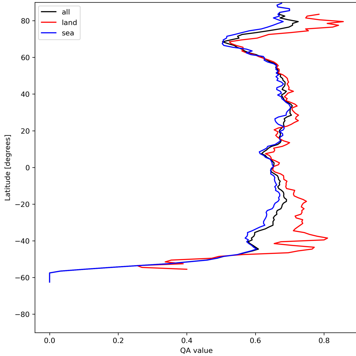
Figure 9: Zonal average of “QA value” for 2024-07-07 to 2024-07-09.
