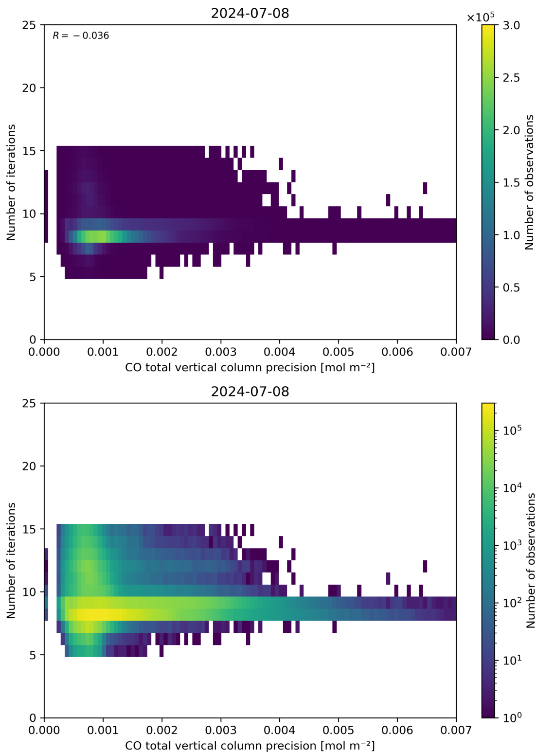
Figure 46: Scatter density plot of “CO total vertical column precision” against “Number of iterations” for 2024-07-07 to 2024-07-09.
