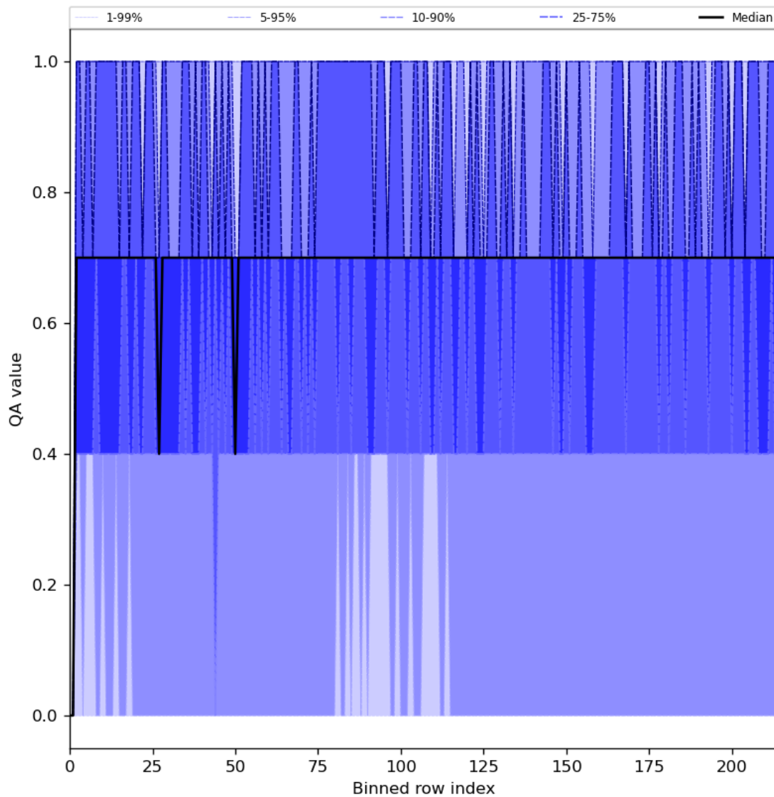
Figure 25: Along track statistics of “QA value” for 2024-07-07 to 2024-07-09
