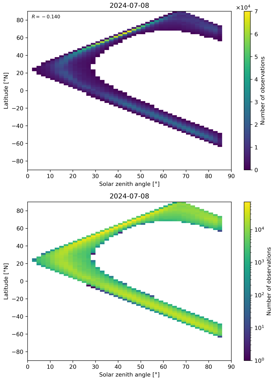
Figure 66: Scatter density plot of “Solar zenith angle” against “Latitude” for 2024-07-07 to 2024-07-09.
