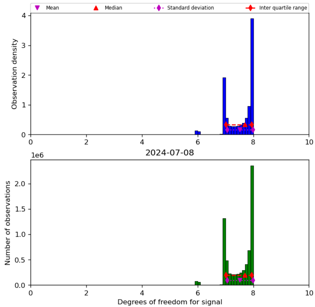
Figure 23: Histogram of “Degrees of freedom for signal” for 2024-07-07 to 2024-07-09
