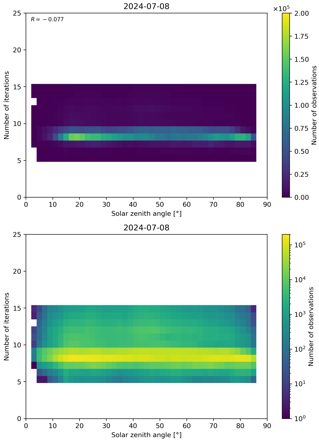
Figure 67: Scatter density plot of “Solar zenith angle” against “Number of iterations” for 2024-07-07 to 2024-07-09.
