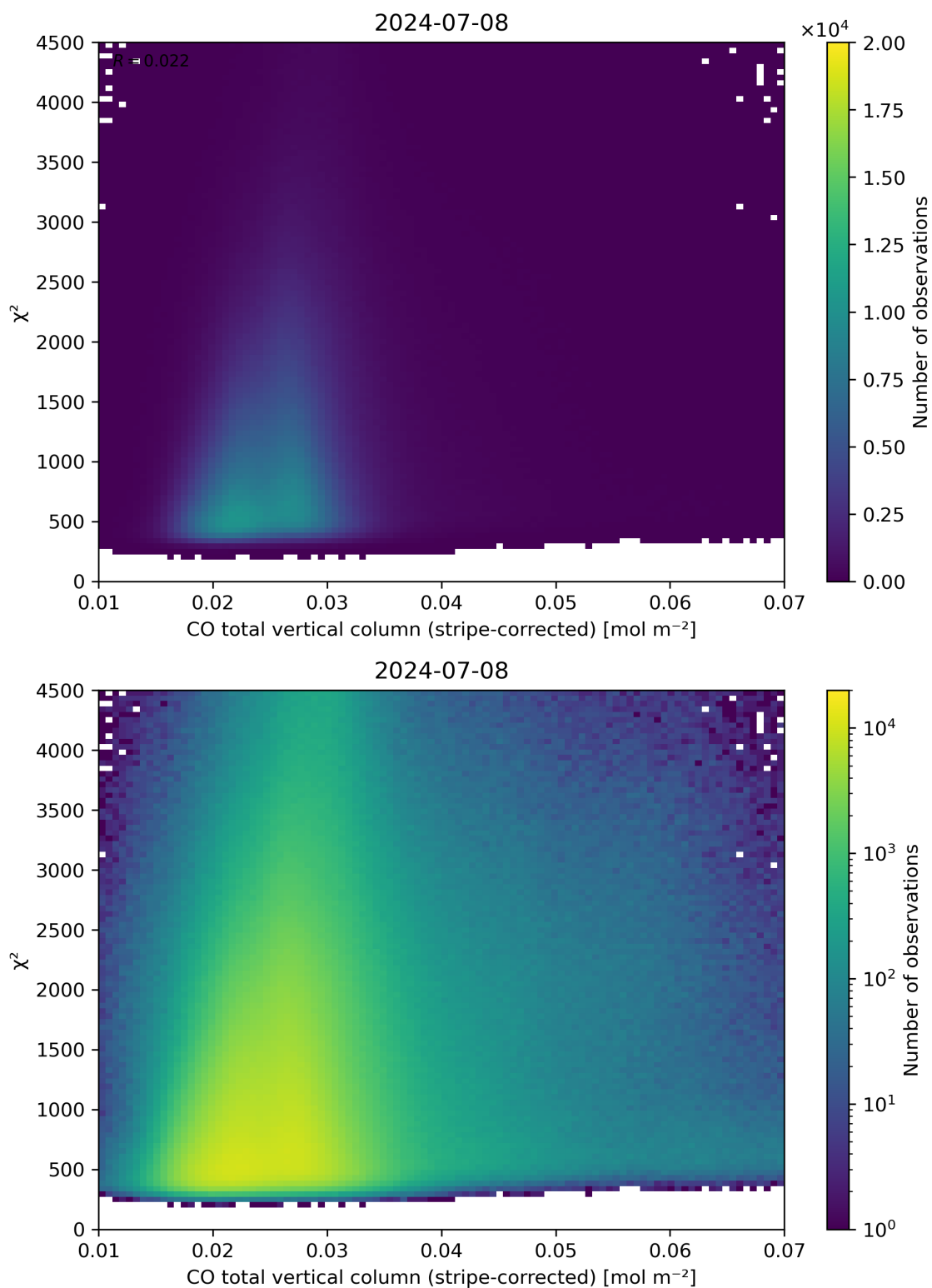
Figure 37: Scatter density plot of “CO total vertical column (stripe-corrected)” against “ \chi^2 ” for 2024-07-07 to 2024-07-09.
