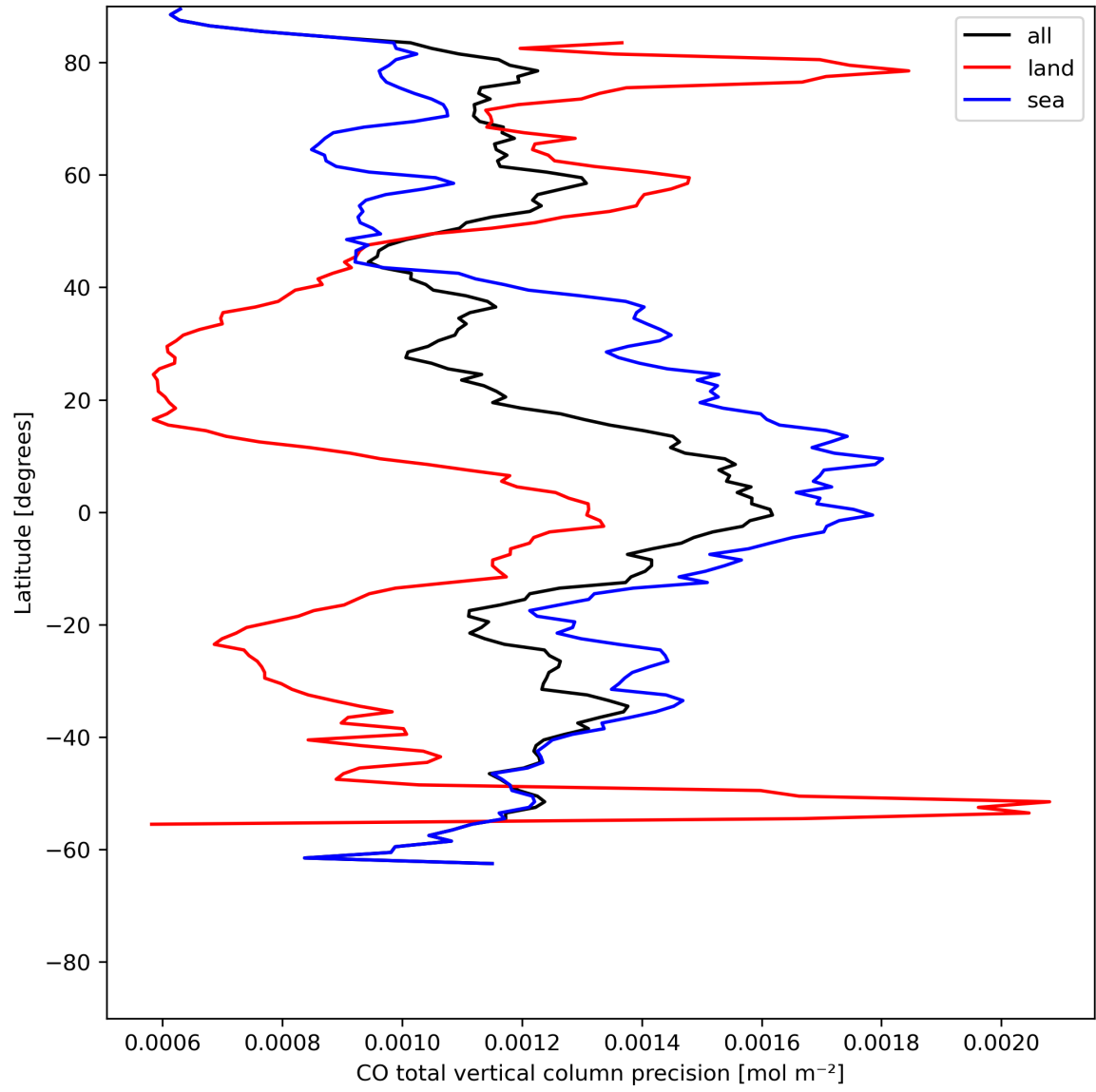
Figure 12: Zonal average of “CO total vertical column precision” for 2024-07-07 to 2024-07-09.
