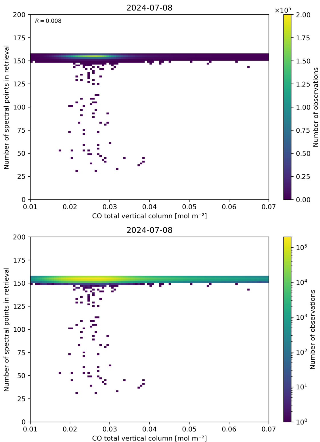
Figure 43: Scatter density plot of “CO total vertical column” against “Number of spectral points in retrieval” for 2024-07-07 to 2024-07-09.
