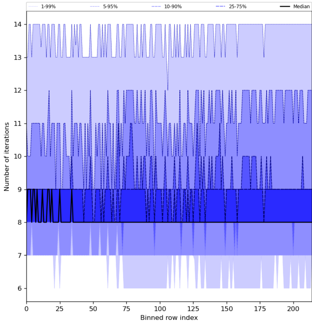
Figure 32: Along track statistics of “Number of iterations” for 2024-07-07 to 2024-07-09
