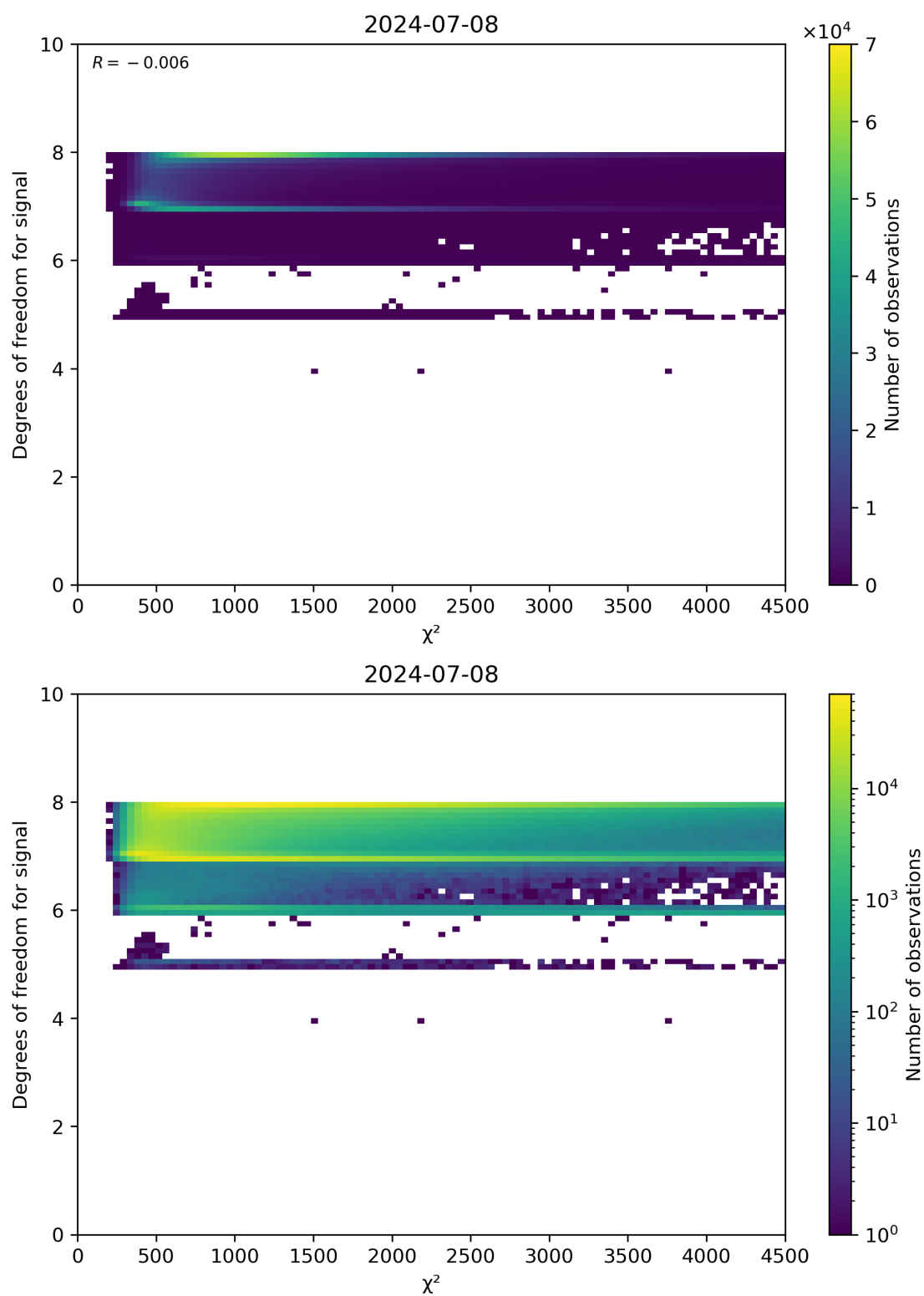
Figure 48: Scatter density plot of “ \chi^2 ” against “Degrees of freedom for signal” for 2024-07-07 to 2024-07-09.
