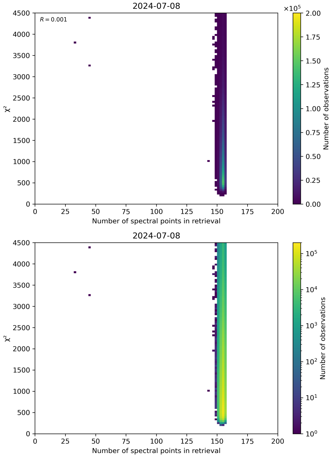
Figure 58: Scatter density plot of “Number of spectral points in retrieval” against “ \chi^2 ” for 2024-07-07 to 2024-07-09.
