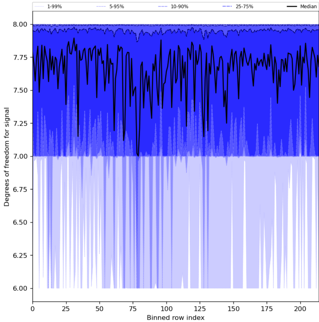
Figure 31: Along track statistics of “Degrees of freedom for signal” for 2024-07-07 to 2024-07-09
