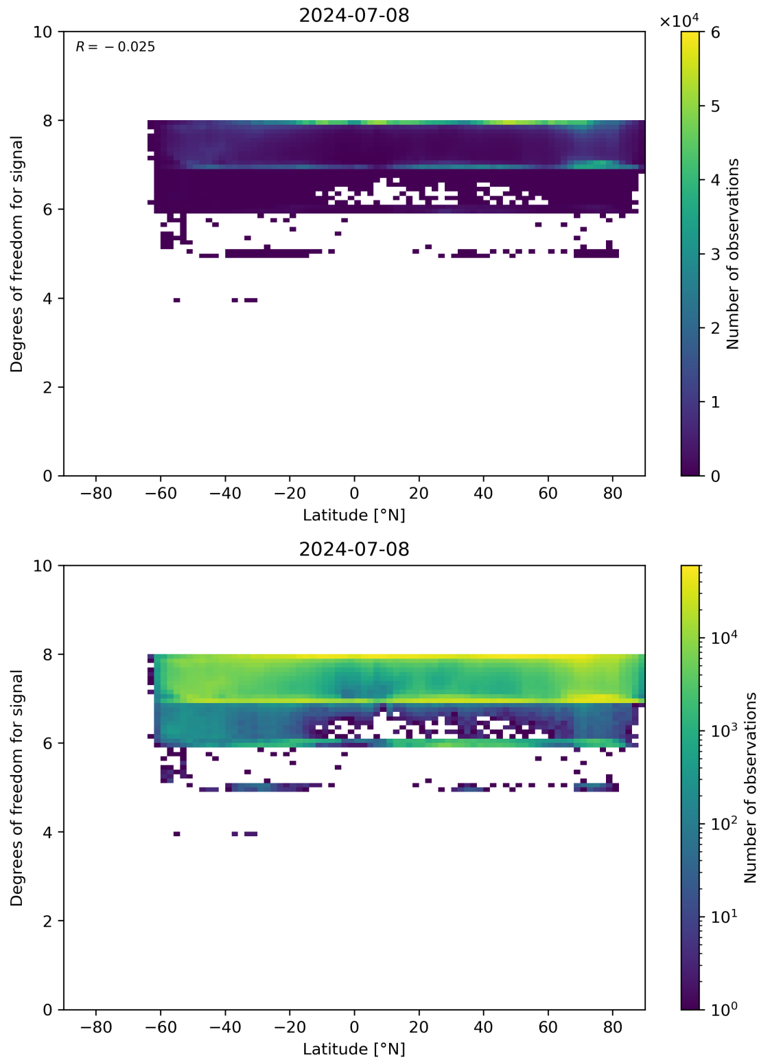
Figure 55: Scatter density plot of “Latitude” against “Degrees of freedom for signal” for 2024-07-07 to 2024-07-09.
