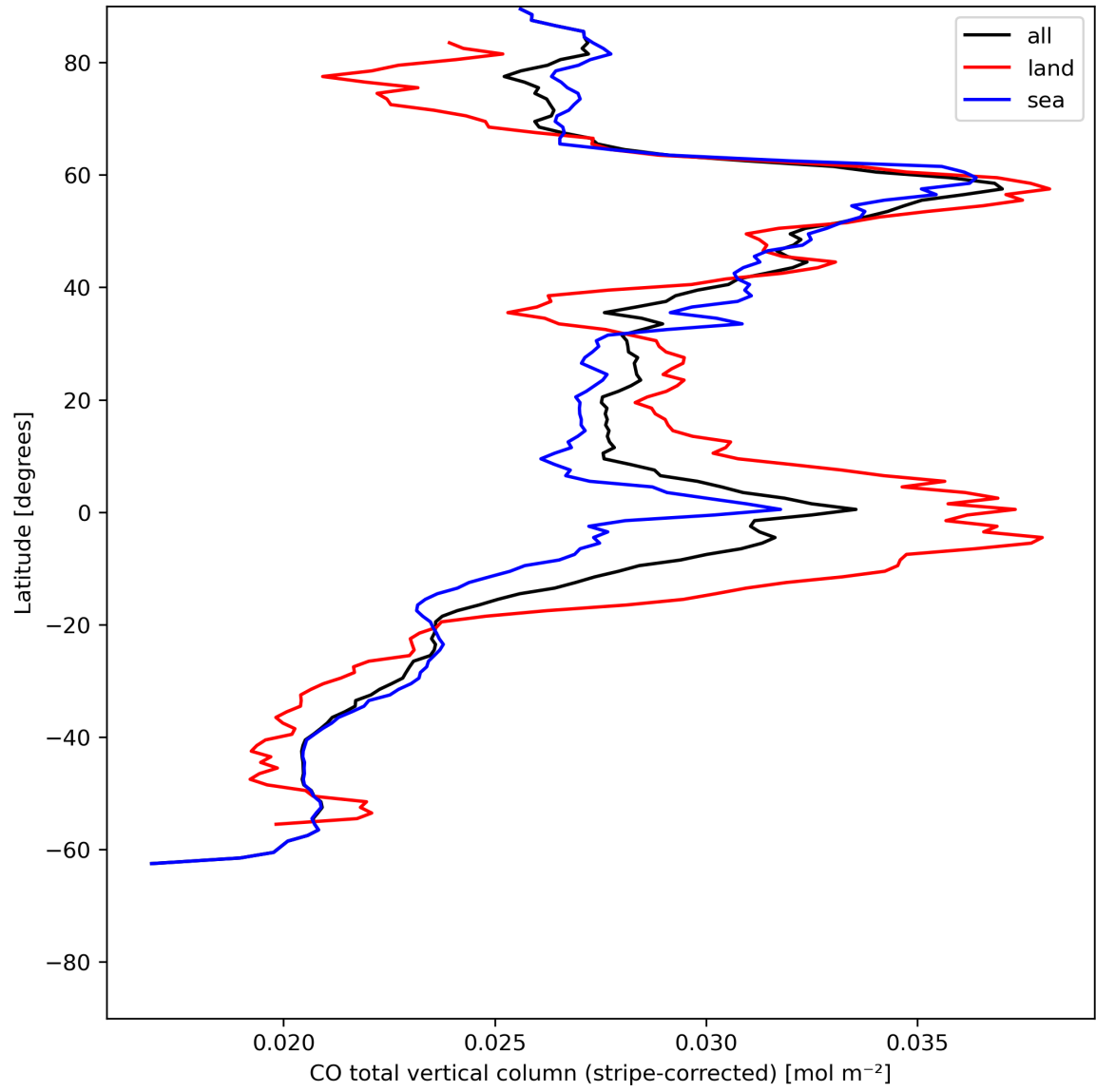
Figure 11: Zonal average of “CO total vertical column (stripe-corrected)” for 2024-07-07 to 2024-07-09.
