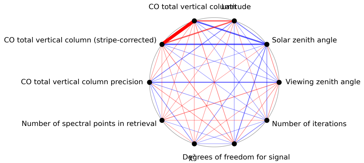
Figure 1: Map of correlation graph for 2024-07-07 to 2024-07-09.
