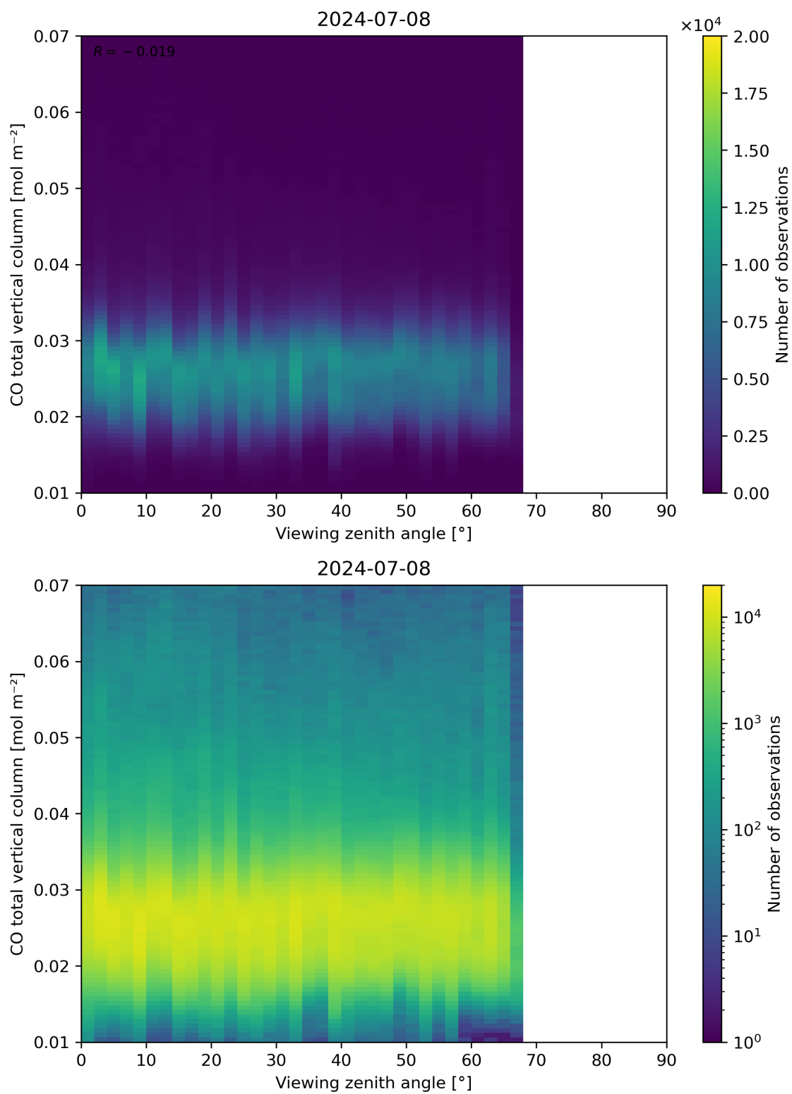
Figure 69: Scatter density plot of “Viewing zenith angle” against “CO total vertical column” for 2024-07-07 to 2024-07-09.
