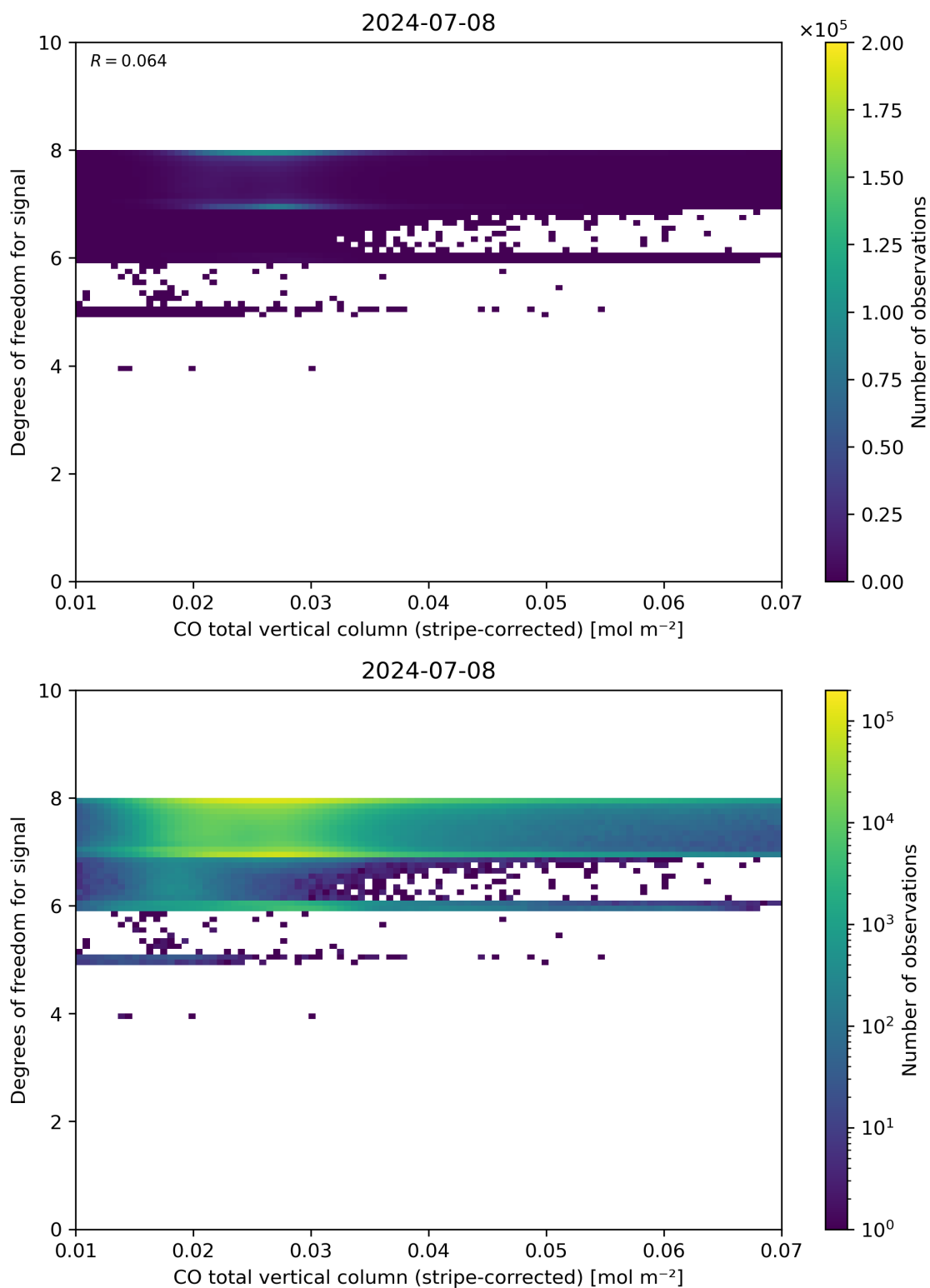
Figure 38: Scatter density plot of “CO total vertical column (stripe-corrected)” against “Degrees of freedom for signal” for 2024-07-07 to 2024-07-09.
