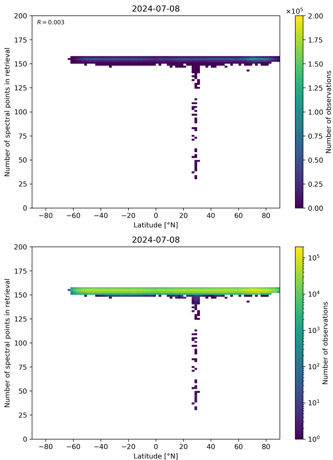
Figure 57: Scatter density plot of “Latitude” against “Number of spectral points in retrieval” for 2024-07-07 to 2024-07-09.
