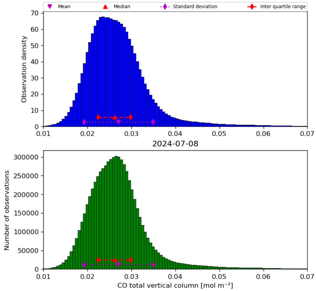
Figure 18: Histogram of “CO total vertical column” for 2024-07-07 to 2024-07-09
