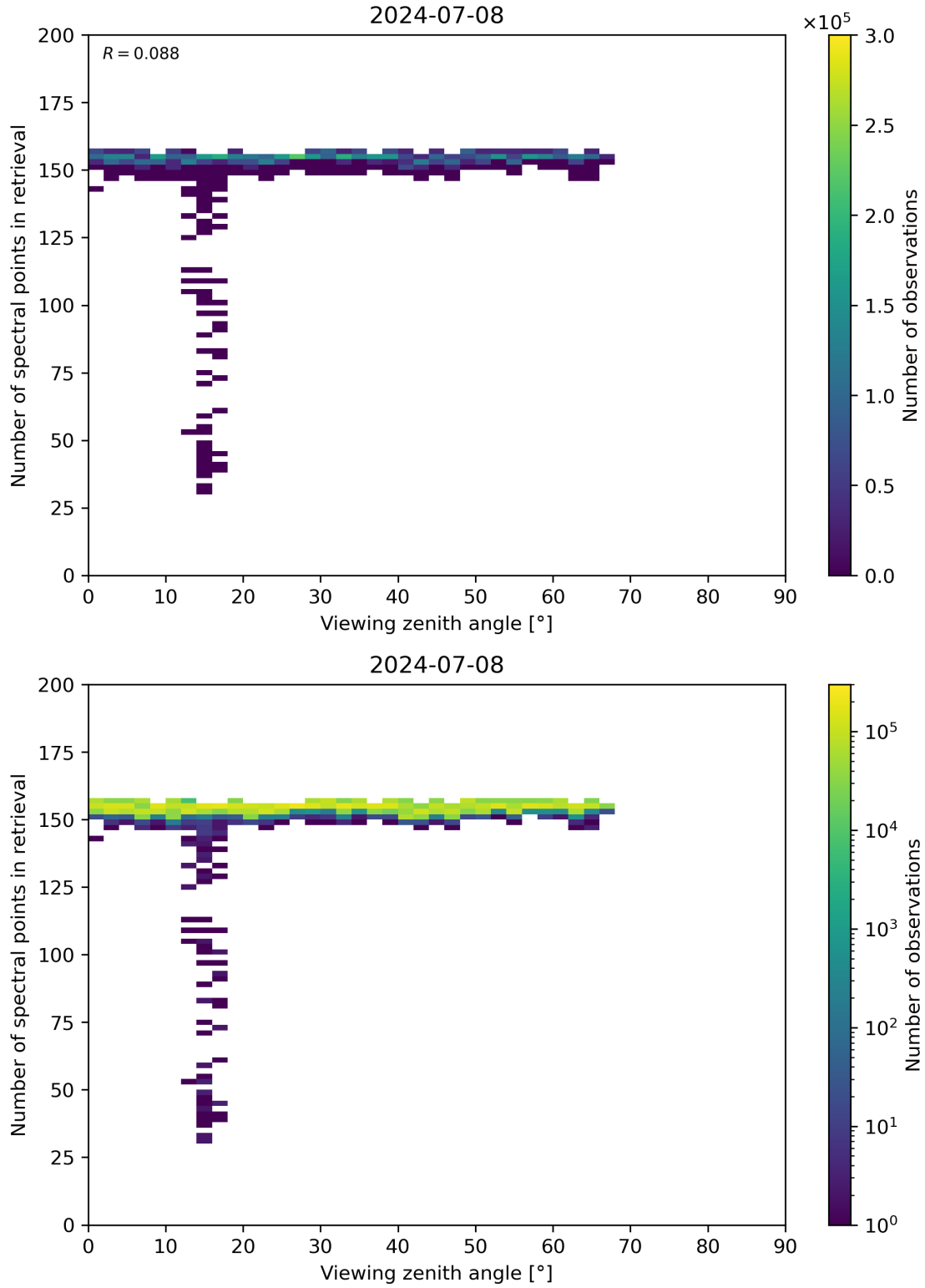
Figure 76: Scatter density plot of “Viewing zenith angle” against “Number of spectral points in retrieval” for 2024-07-07 to 2024-07-09.
