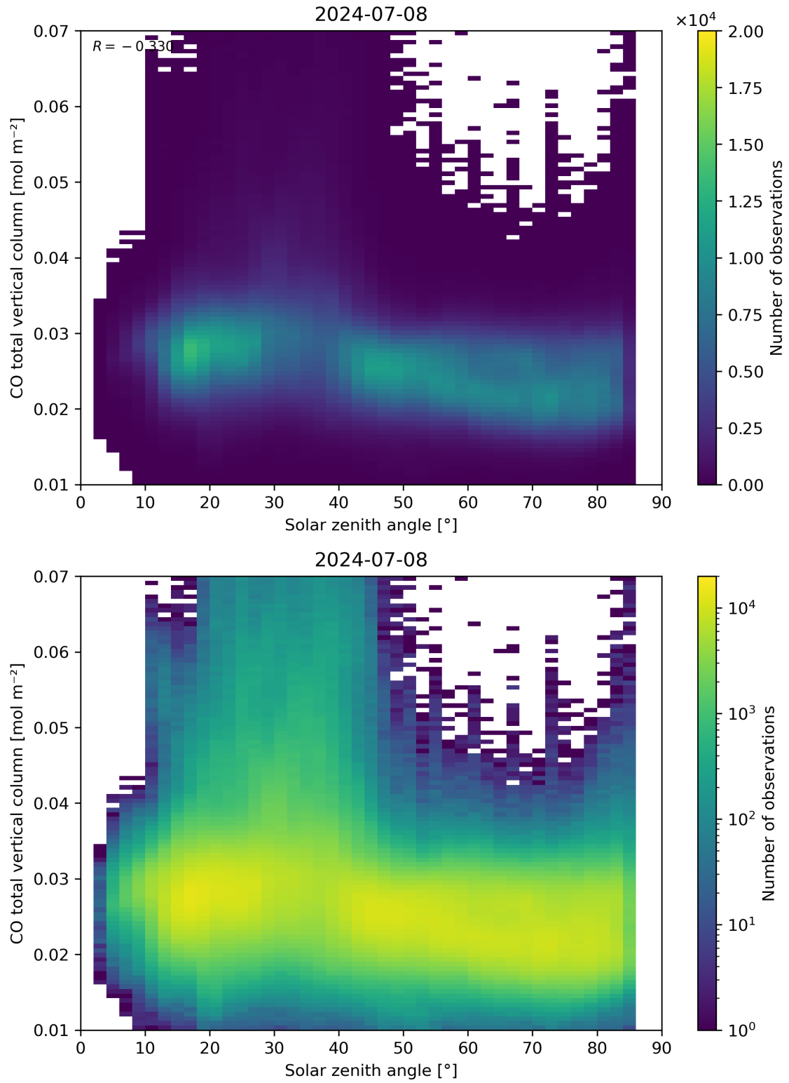
Figure 61: Scatter density plot of “Solar zenith angle” against “CO total vertical column” for 2024-07-07 to 2024-07-09.
