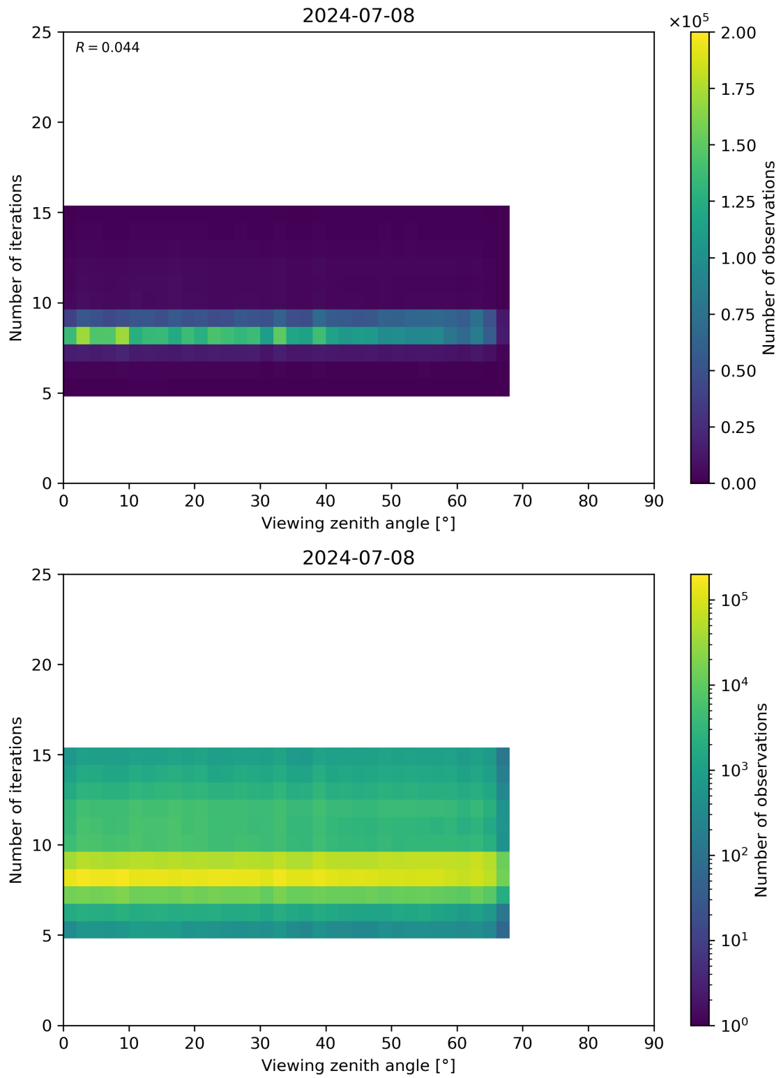
Figure 75: Scatter density plot of “Viewing zenith angle” against “Number of iterations” for 2024-07-07 to 2024-07-09.
