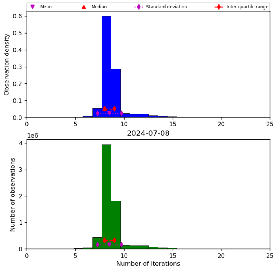
Figure 24: Histogram of “Number of iterations” for 2024-07-07 to 2024-07-09
