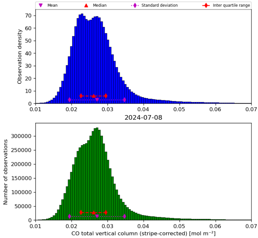
Figure 19: Histogram of “CO total vertical column (stripe-corrected)” for 2024-07-07 to 2024-07-09
