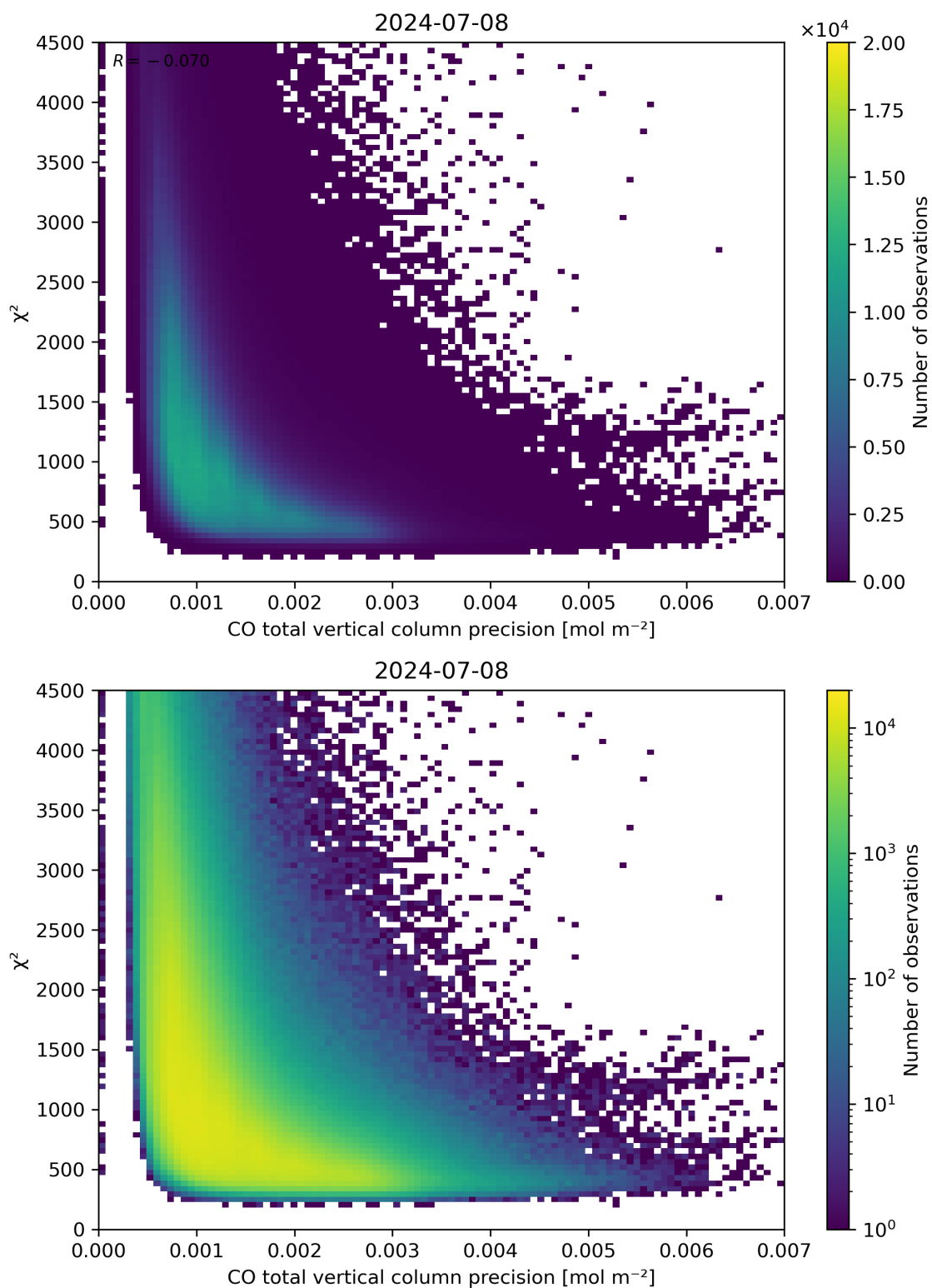
Figure 44: Scatter density plot of “CO total vertical column precision” against “ \chi^2 ” for 2024-07-07 to 2024-07-09.
