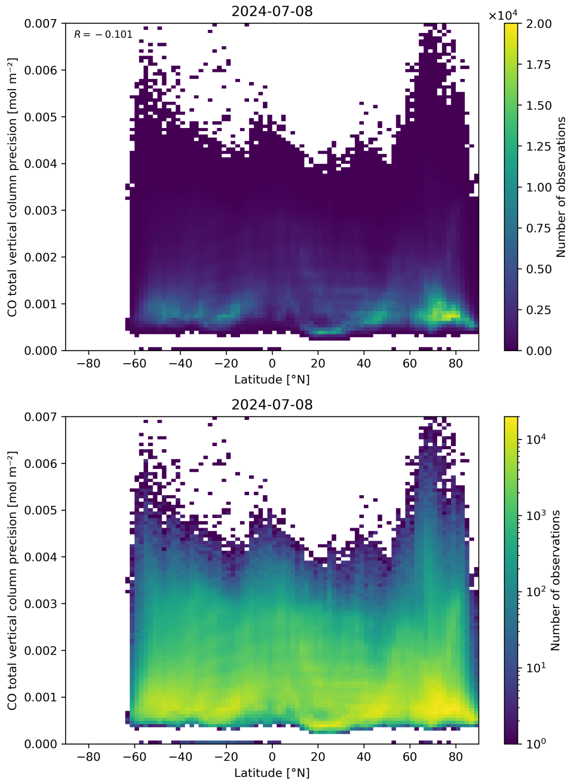
Figure 53: Scatter density plot of “Latitude” against “CO total vertical column precision” for 2024-07-07 to 2024-07-09.
