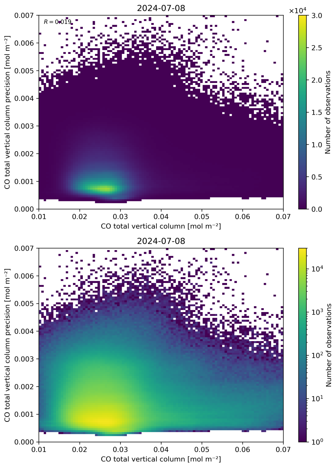
Figure 34: Scatter density plot of “CO total vertical column” against “CO total vertical column precision” for 2024-07-07 to 2024-07-09.
