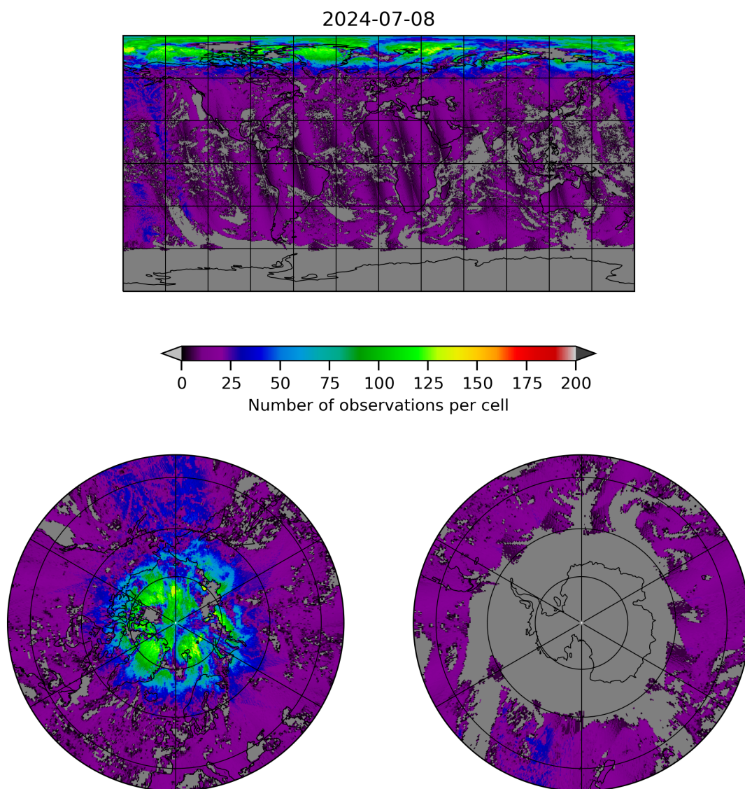
Figure 8: Map of the number of observations for 2024-07-07 to 2024-07-09
