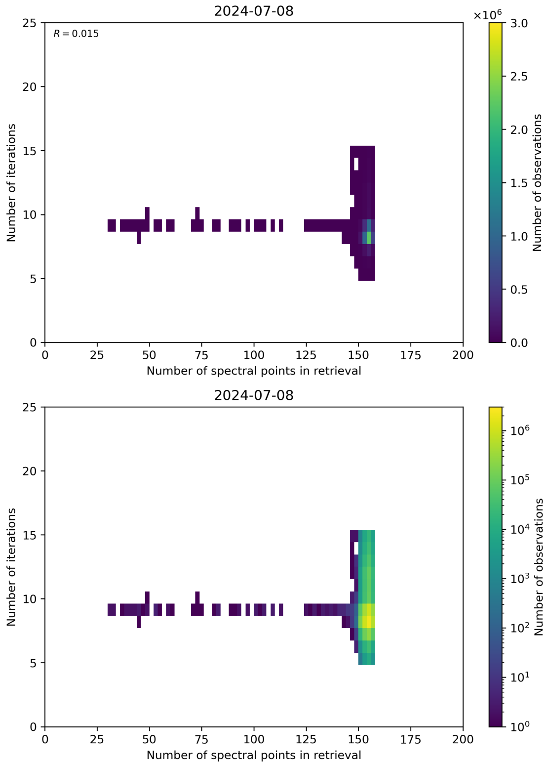
Figure 60: Scatter density plot of “Number of spectral points in retrieval” against “Number of iterations” for 2024-07-07 to 2024-07-09.
