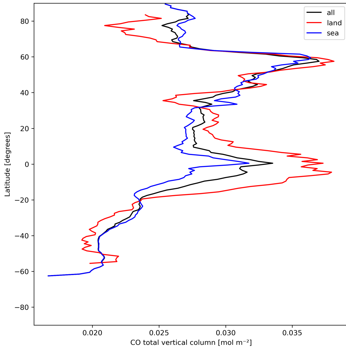
Figure 10: Zonal average of “CO total vertical column” for 2024-07-07 to 2024-07-09.
