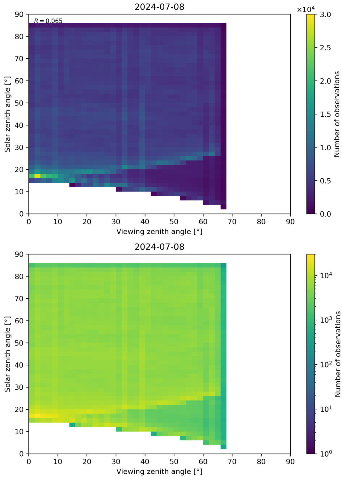
Figure 77: Scatter density plot of “Viewing zenith angle” against “Solar zenith angle” for 2024-07-07 to 2024-07-09.
