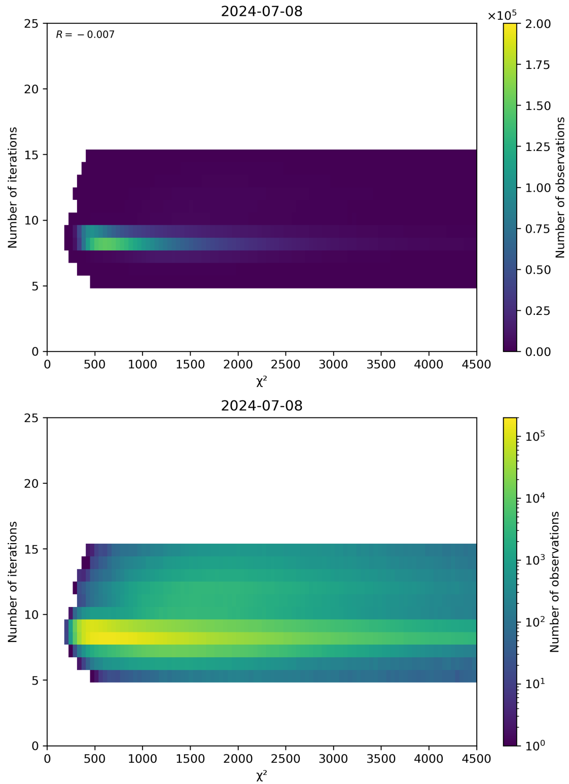
Figure 49: Scatter density plot of “ \chi^2 ” against “Number of iterations” for 2024-07-07 to 2024-07-09.
