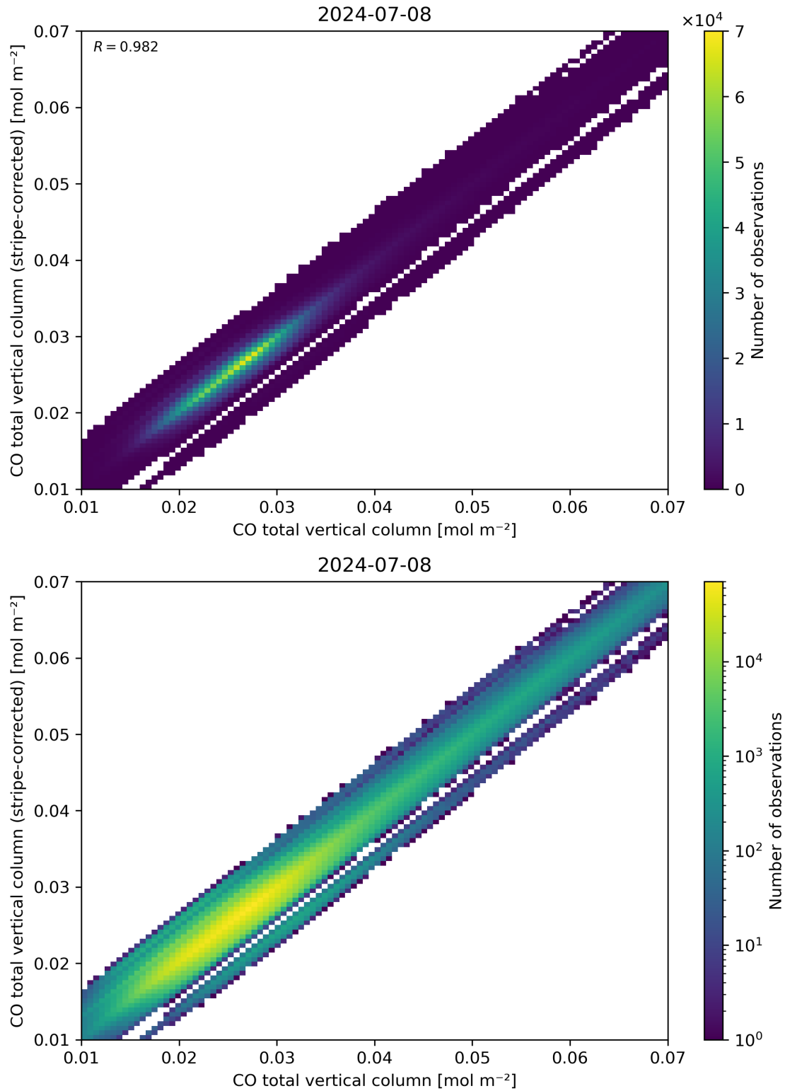
Figure 33: Scatter density plot of “CO total vertical column” against “CO total vertical column (stripe-corrected)” for 2024-07-07 to 2024-07-09.
