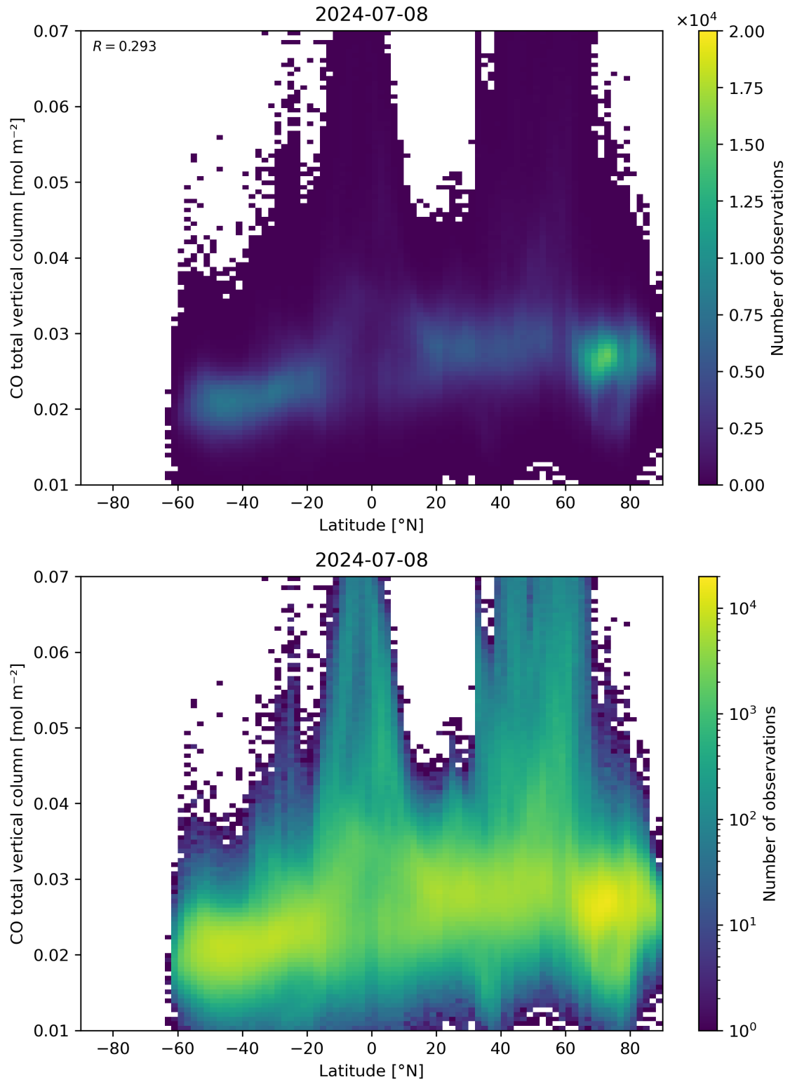
Figure 51: Scatter density plot of “Latitude” against “CO total vertical column” for 2024-07-07 to 2024-07-09.
