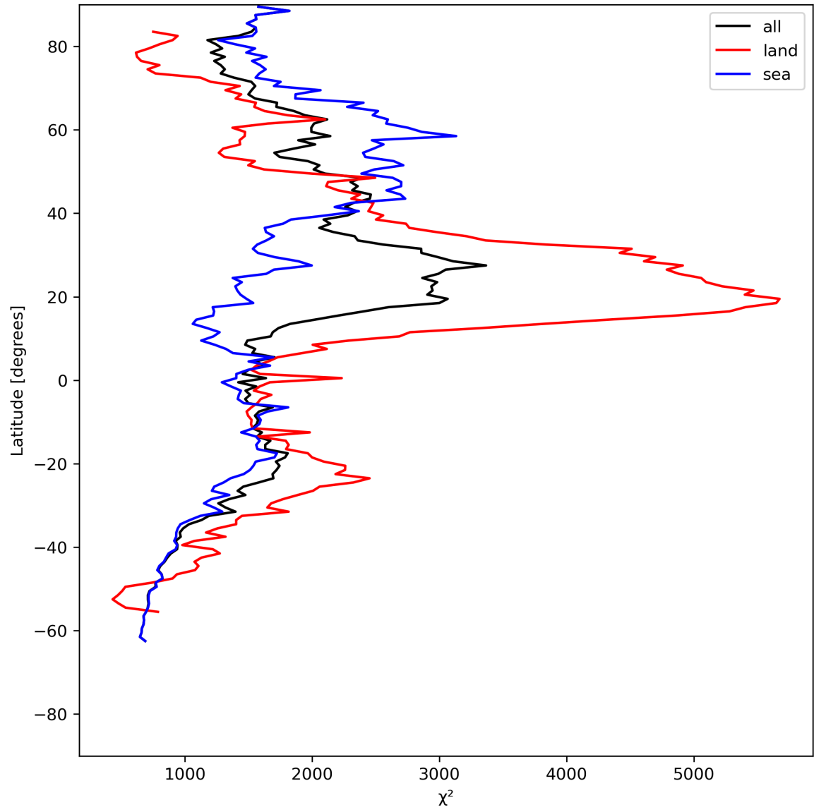
Figure 14: Zonal average of “ \chi^2 ” for 2024-07-07 to 2024-07-09.
