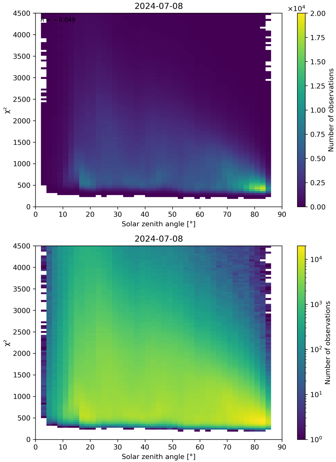
Figure 64: Scatter density plot of “Solar zenith angle” against “ \chi^2 ” for 2024-07-07 to 2024-07-09.
