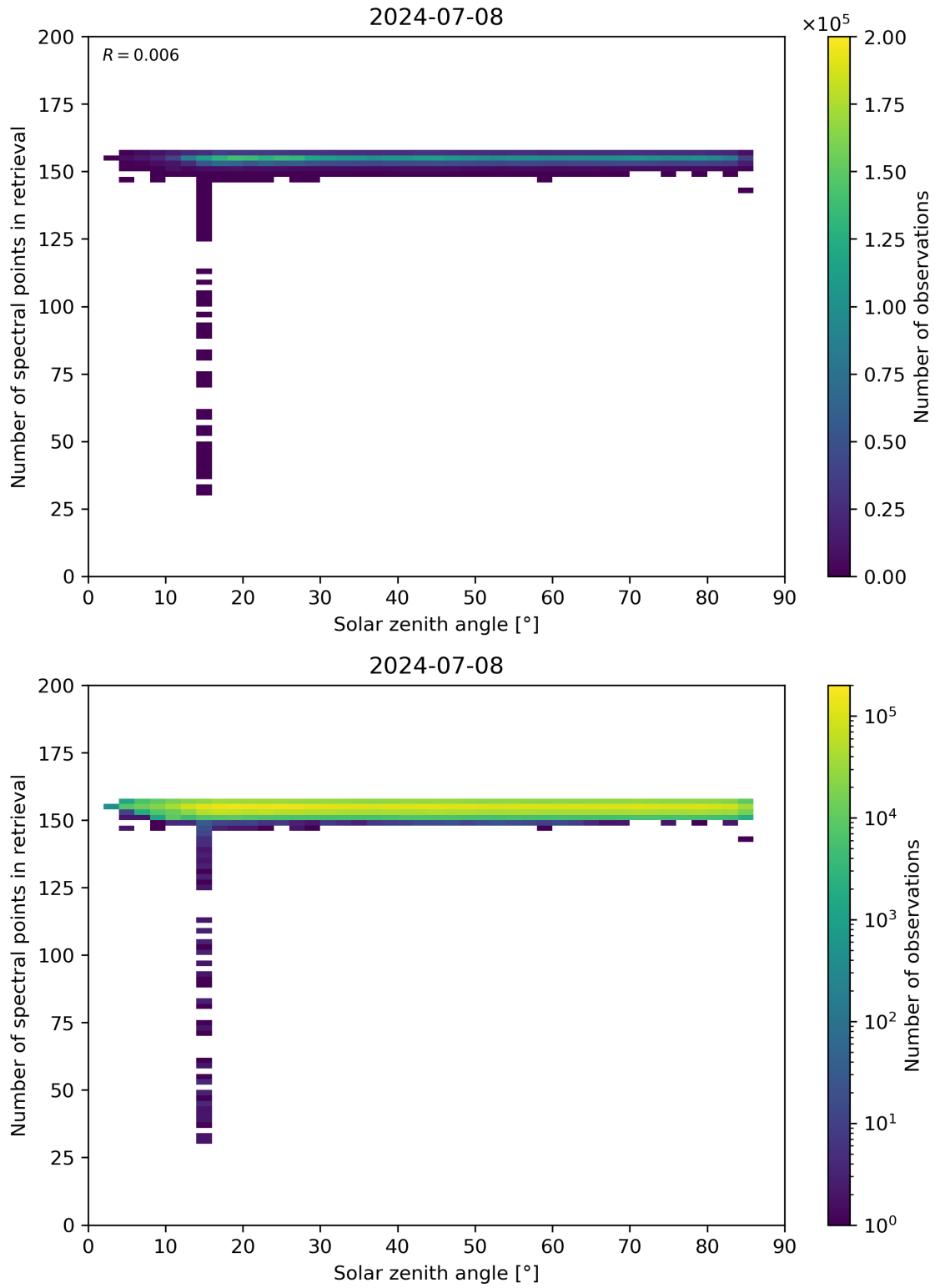
Figure 68: Scatter density plot of “Solar zenith angle” against “Number of spectral points in retrieval” for 2024-07-07 to 2024-07-09.
