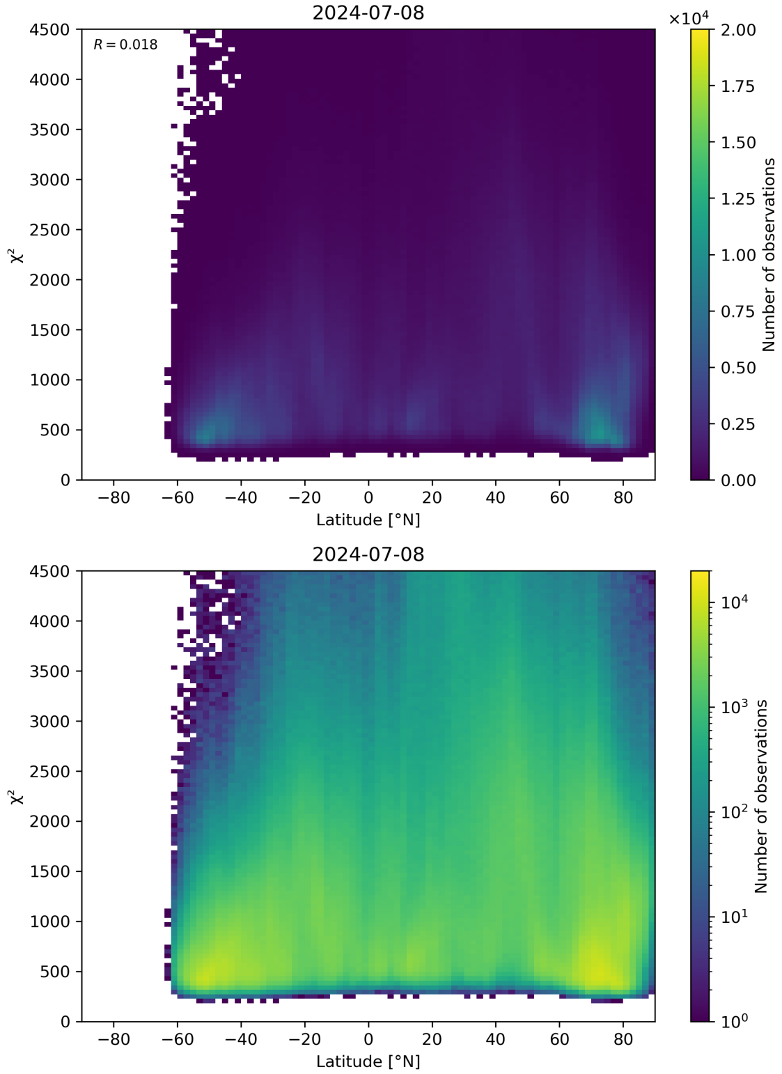
Figure 54: Scatter density plot of “Latitude” against “ \chi^2 ” for 2024-07-07 to 2024-07-09.
