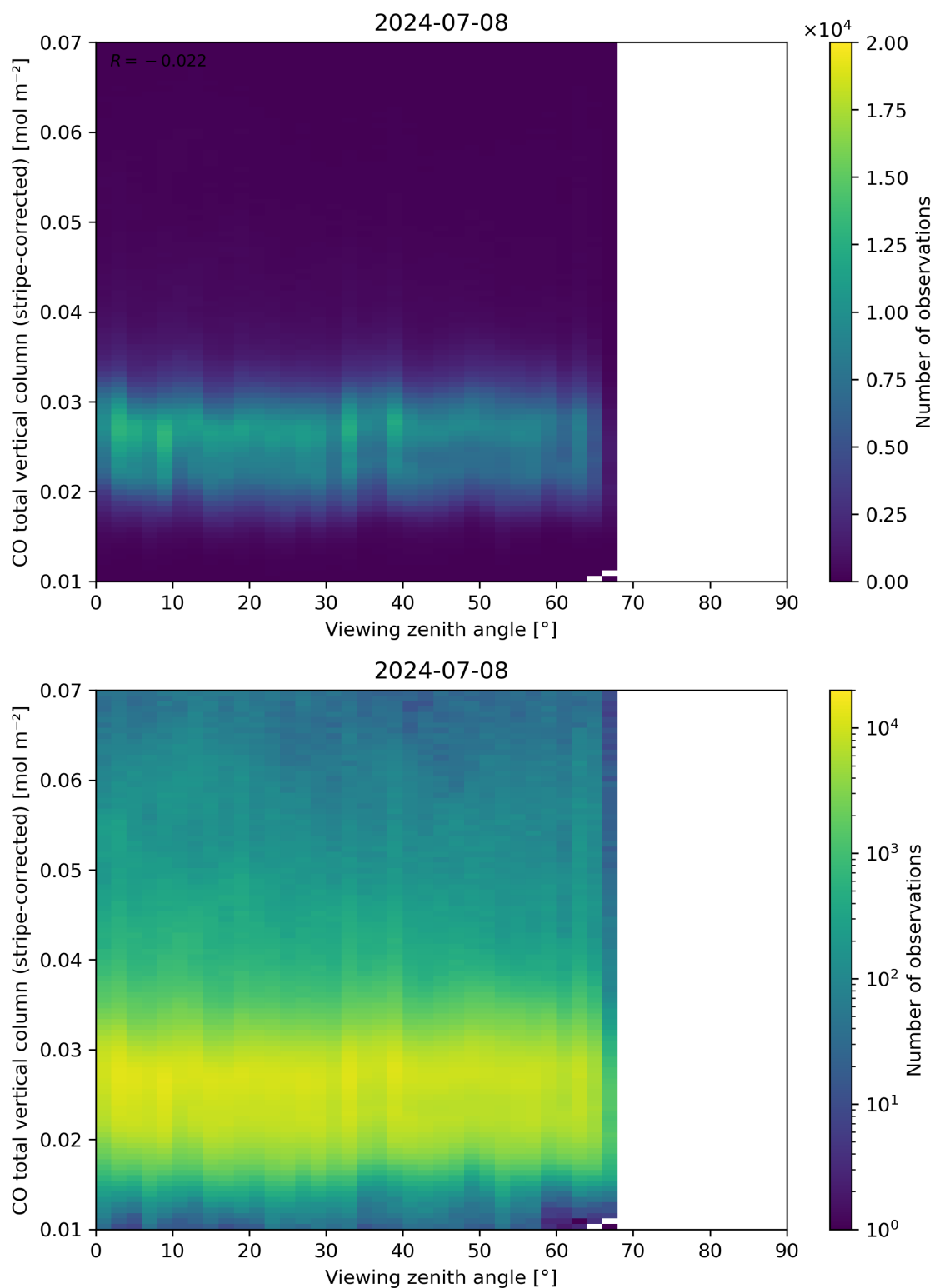
Figure 70: Scatter density plot of “Viewing zenith angle” against “CO total vertical column (stripe-corrected)” for 2024-07-07 to 2024-07-09.
