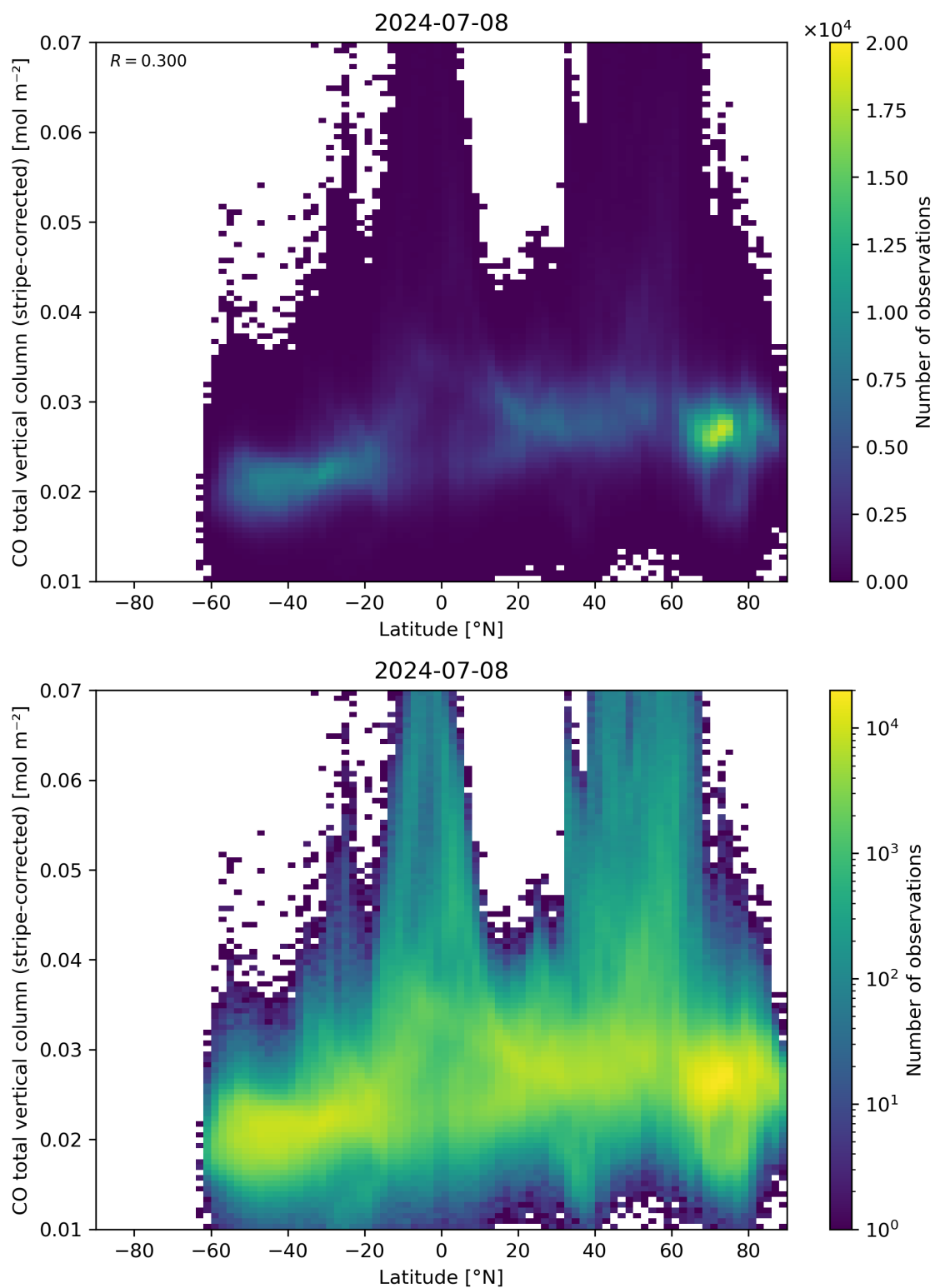
Figure 52: Scatter density plot of “Latitude” against “CO total vertical column (stripe-corrected)” for 2024-07-07 to 2024-07-09.
