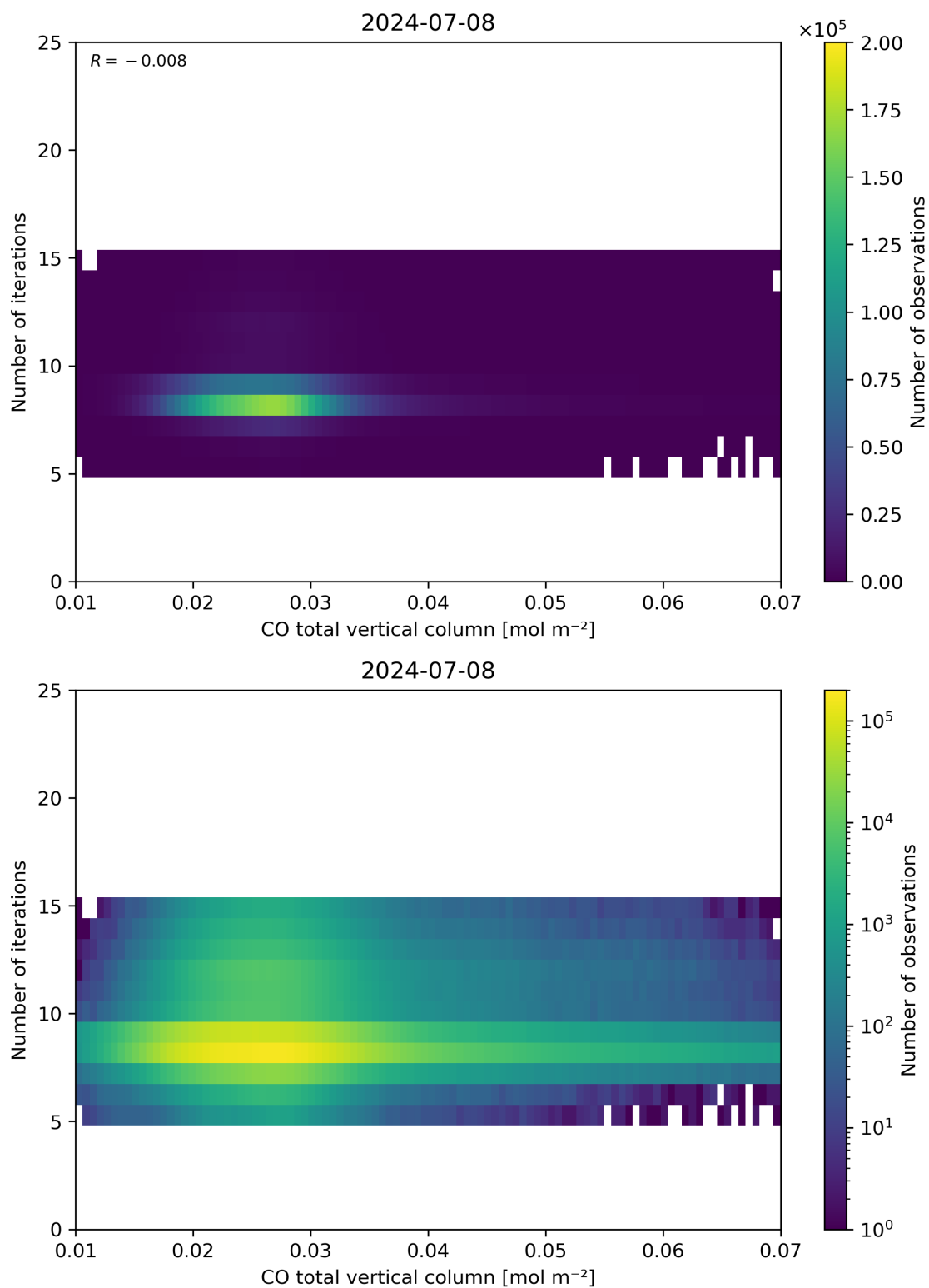
Figure 42: Scatter density plot of “CO total vertical column” against “Number of iterations” for 2024-07-07 to 2024-07-09.
