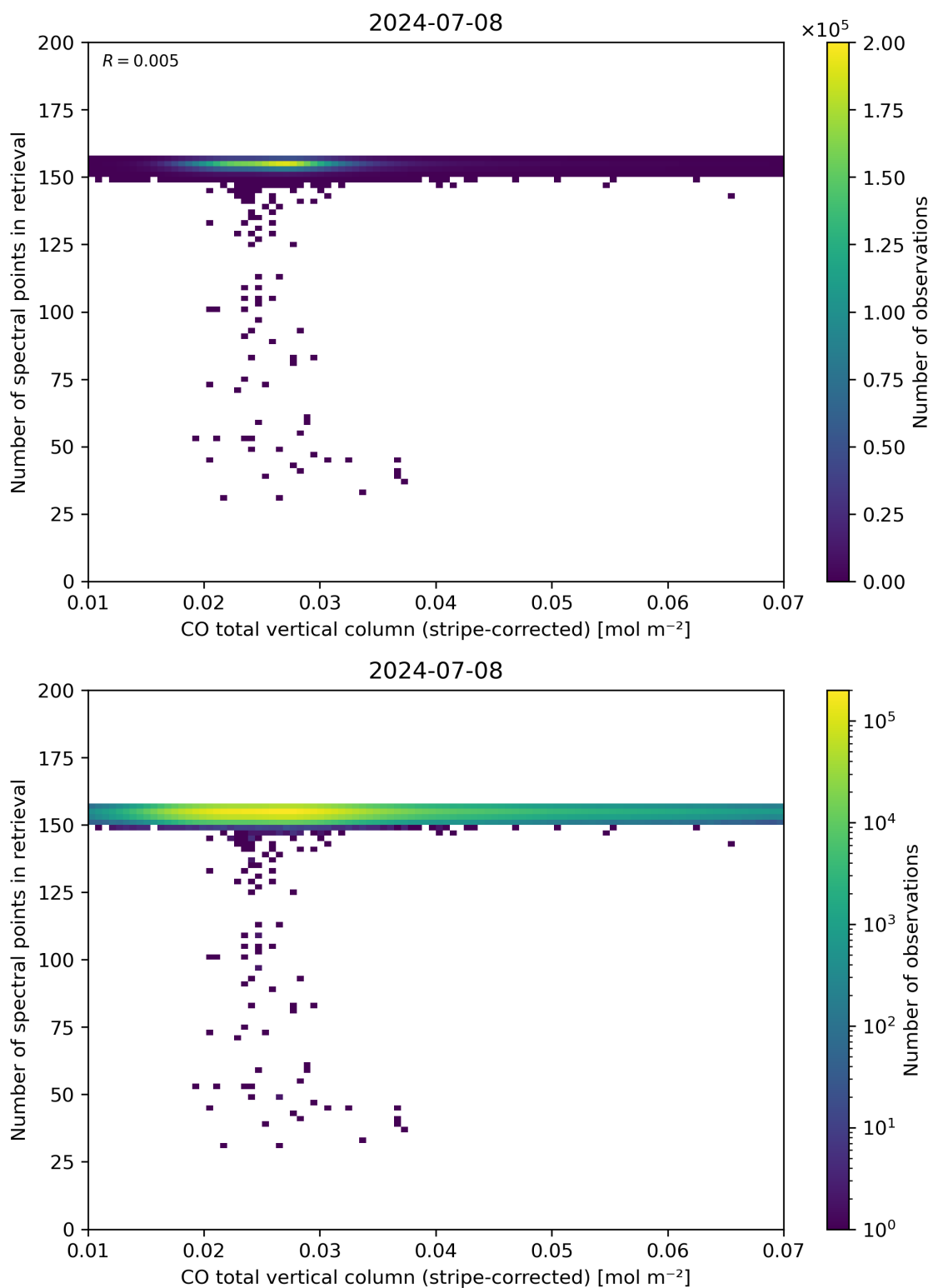
Figure 40: Scatter density plot of “CO total vertical column (stripe-corrected)” against “Number of spectral points in retrieval” for 2024-07-07 to 2024-07-09.
