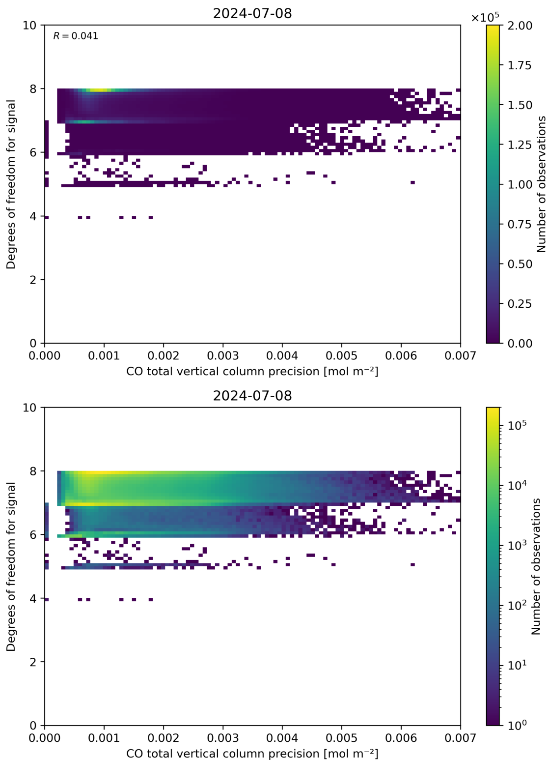
Figure 45: Scatter density plot of “CO total vertical column precision” against “Degrees of freedom for signal” for 2024-07-07 to 2024-07-09.
