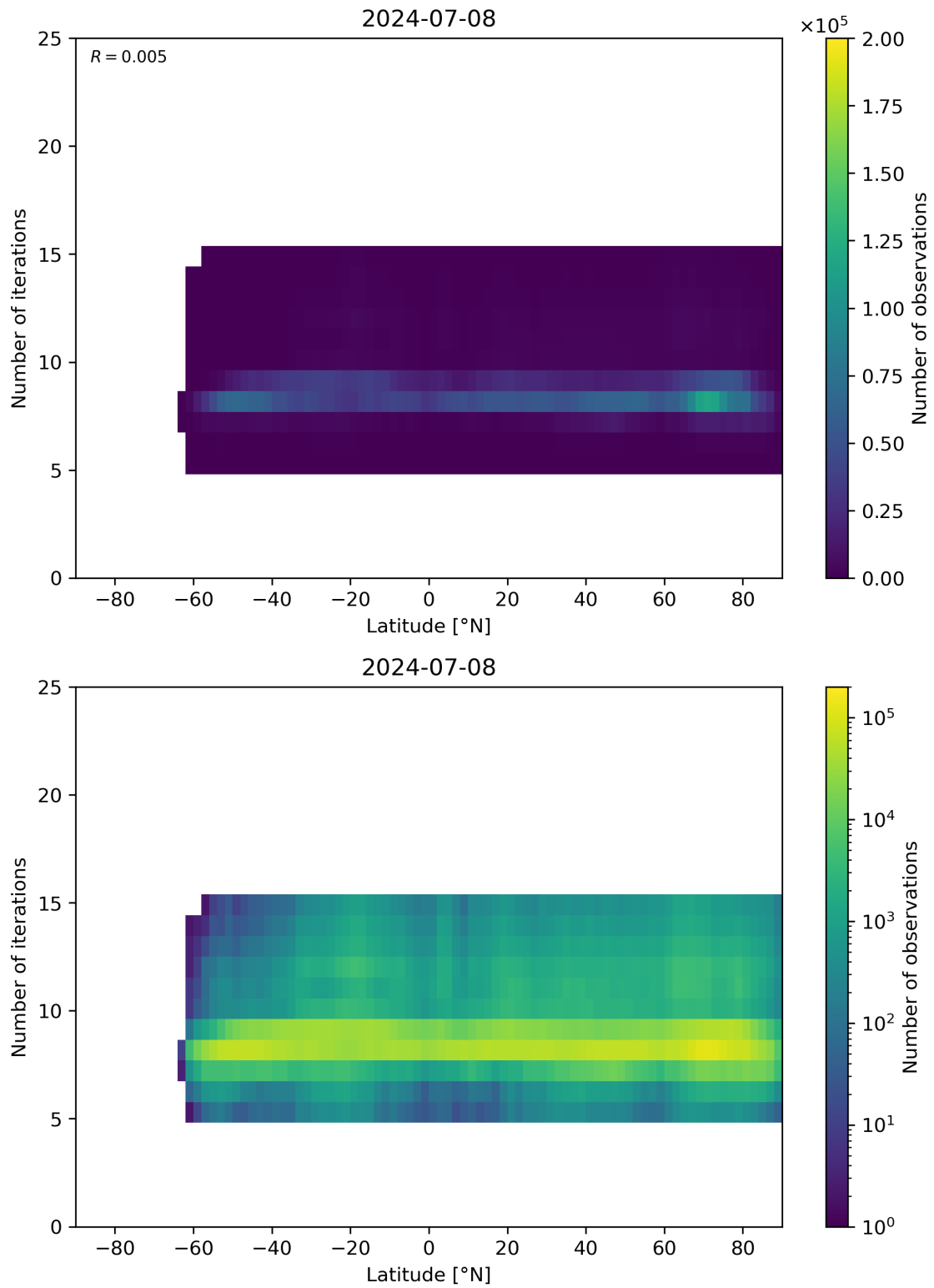
Figure 56: Scatter density plot of “Latitude” against “Number of iterations” for 2024-07-07 to 2024-07-09.
