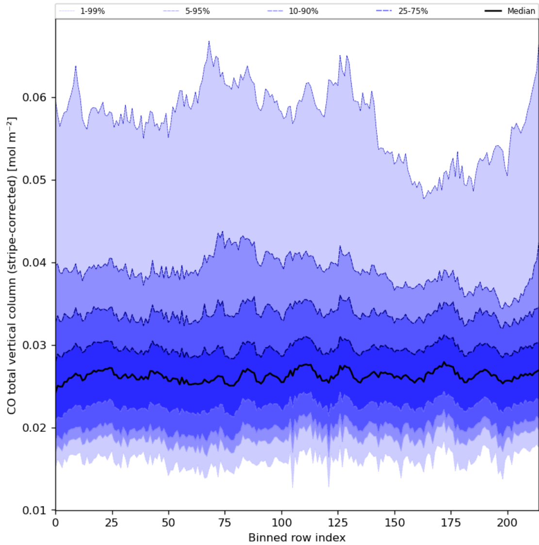
Figure 27: Along track statistics of “CO total vertical column (stripe-corrected)” for 2024-07-07 to 2024-07-09
