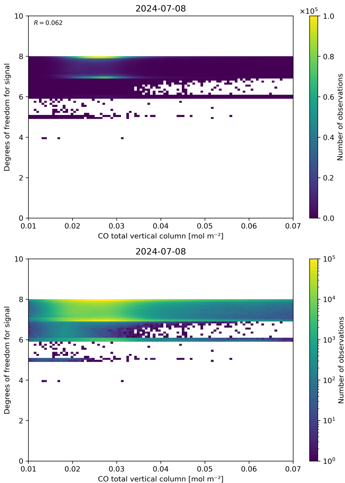
Figure 41: Scatter density plot of “CO total vertical column” against “Degrees of freedom for signal” for 2024-07-07 to 2024-07-09.
