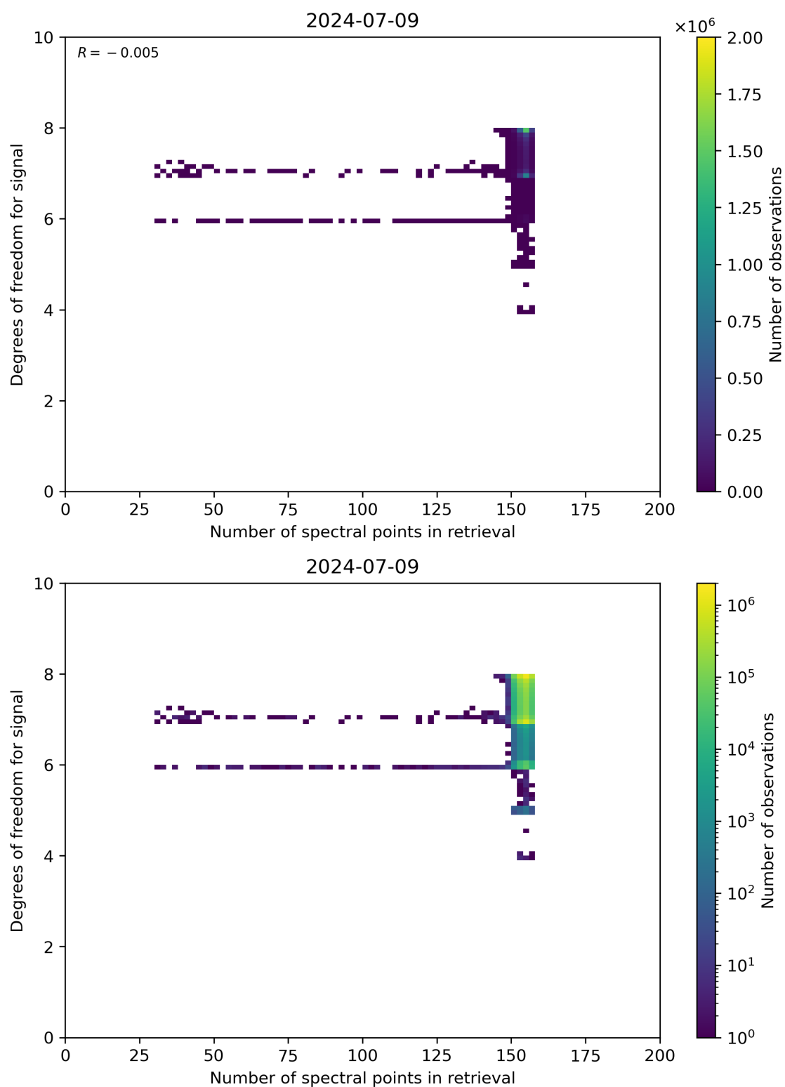
Figure 59: Scatter density plot of “Number of spectral points in retrieval” against “Degrees of freedom for signal” for 2024-07-08 to 2024-07-10.
