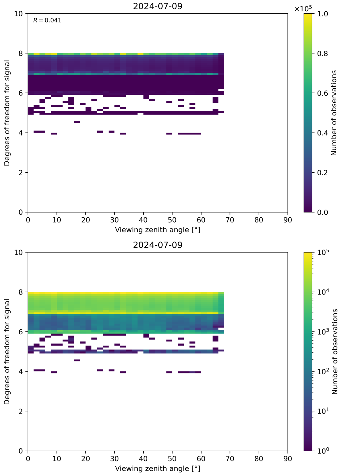
Figure 73: Scatter density plot of “Viewing zenith angle” against “Degrees of freedom for signal” for 2024-07-08 to 2024-07-10.
