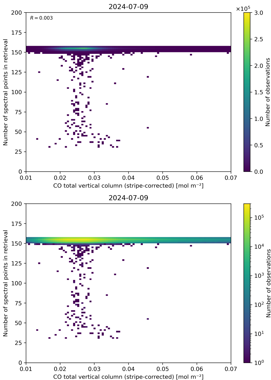
Figure 40: Scatter density plot of “CO total vertical column (stripe-corrected)” against “Number of spectral points in retrieval” for 2024-07-08 to 2024-07-10.
