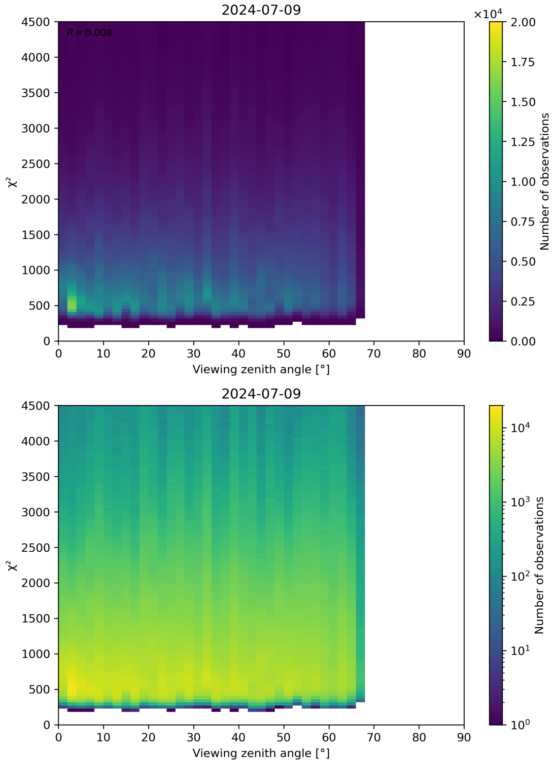
Figure 72: Scatter density plot of “Viewing zenith angle” against “ \chi^2 ” for 2024-07-08 to 2024-07-10.
