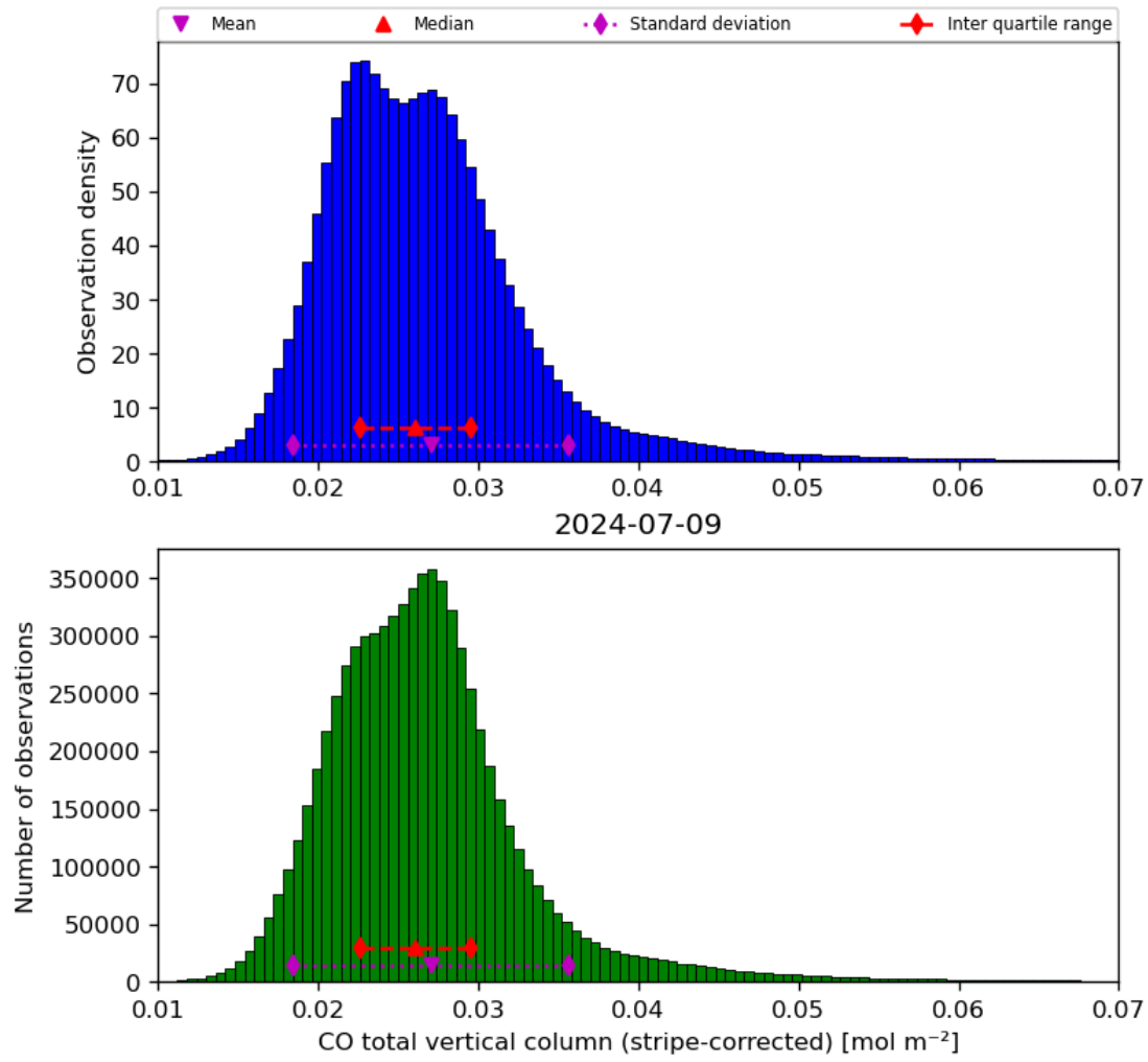
Figure 19: Histogram of “CO total vertical column (stripe-corrected)” for 2024-07-08 to 2024-07-10
