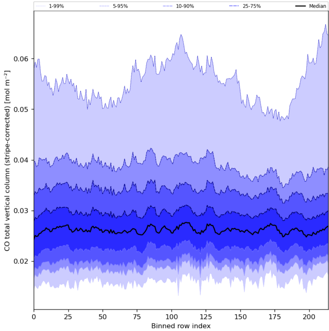
Figure 27: Along track statistics of “CO total vertical column (stripe-corrected)” for 2024-07-08 to 2024-07-10
