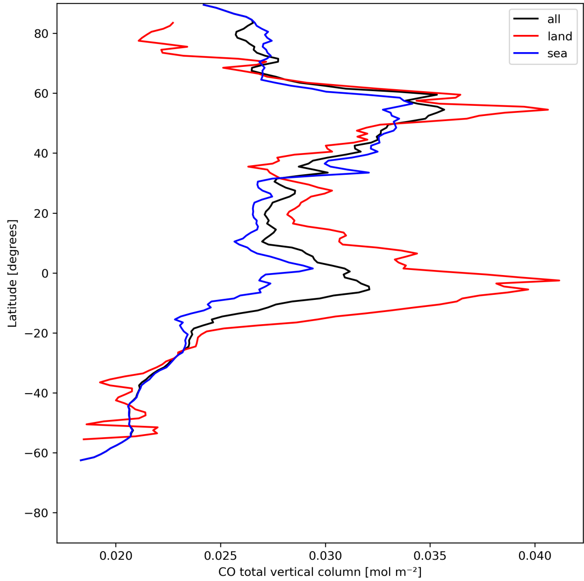
Figure 10: Zonal average of “CO total vertical column” for 2024-07-08 to 2024-07-10.
