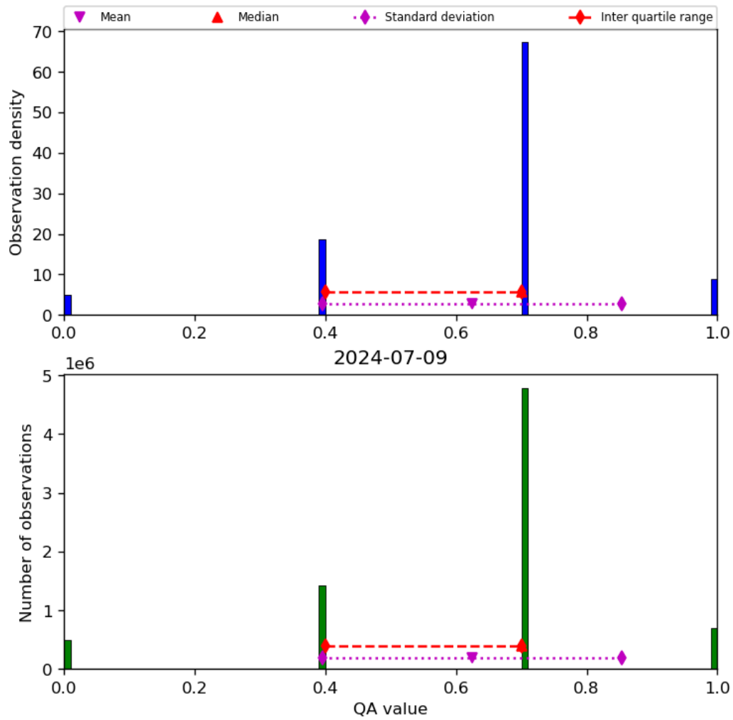
Figure 17: Histogram of “QA value” for 2024-07-08 to 2024-07-10
