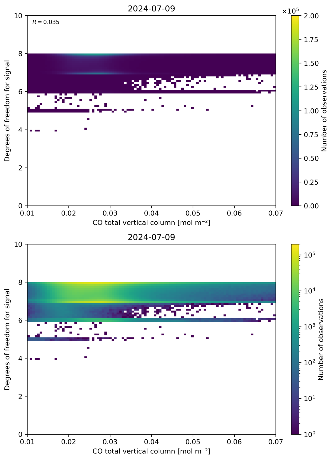
Figure 41: Scatter density plot of “CO total vertical column” against “Degrees of freedom for signal” for 2024-07-08 to 2024-07-10.
