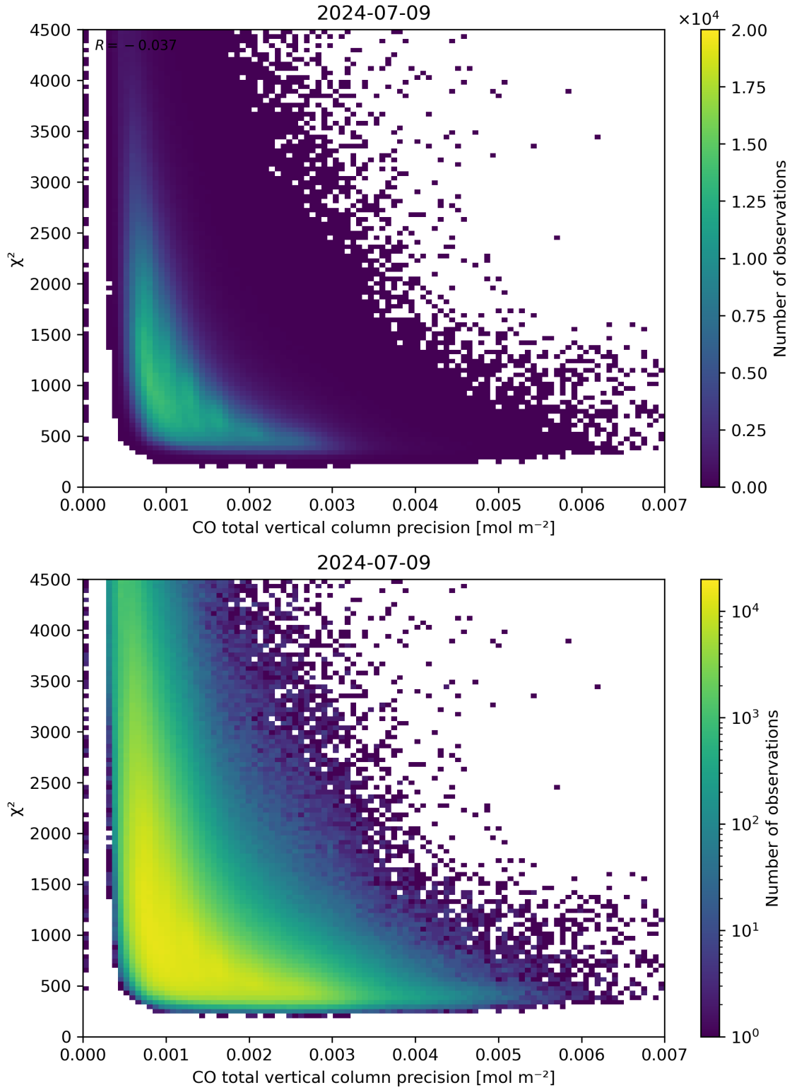
Figure 44: Scatter density plot of “CO total vertical column precision” against “ \chi^2 ” for 2024-07-08 to 2024-07-10.
