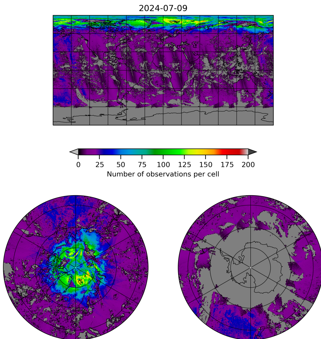
Figure 8: Map of the number of observations for 2024-07-08 to 2024-07-10
