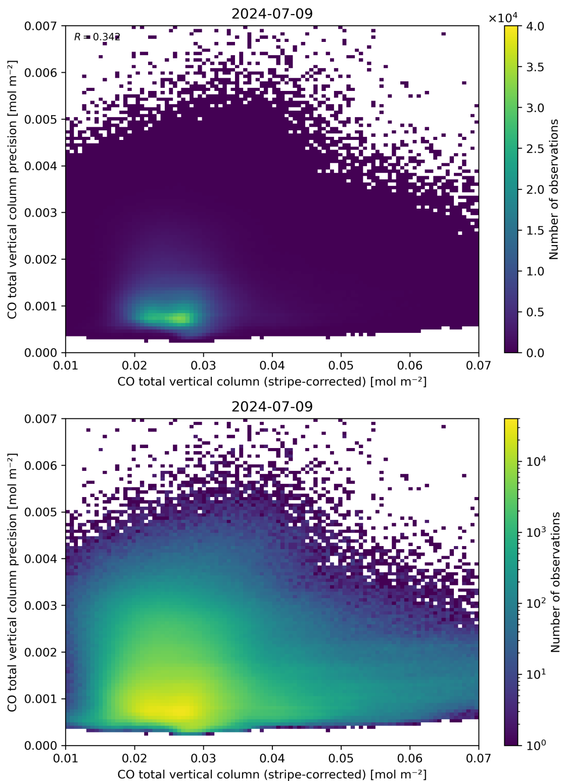
Figure 36: Scatter density plot of “CO total vertical column (stripe-corrected)” against “CO total vertical column precision” for 2024-07-08 to 2024-07-10.
