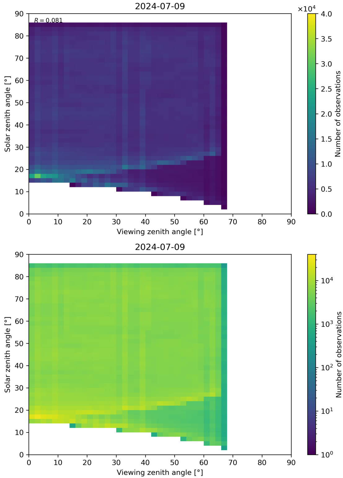
Figure 77: Scatter density plot of “Viewing zenith angle” against “Solar zenith angle” for 2024-07-08 to 2024-07-10.
