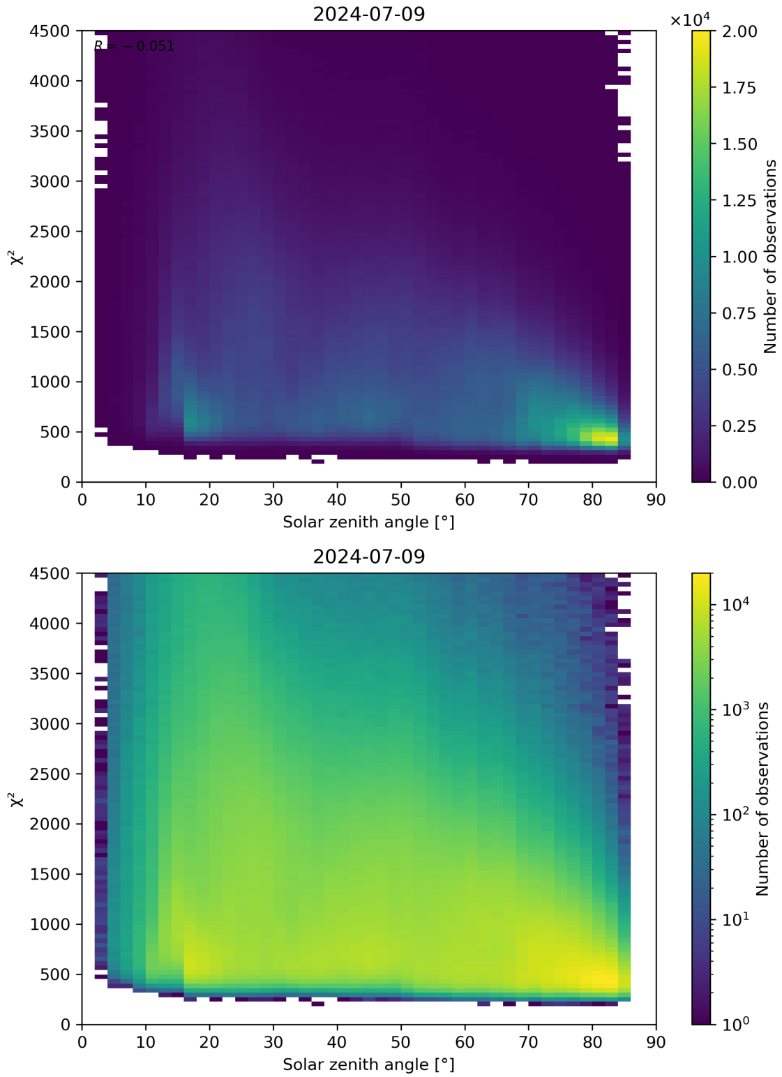
Figure 64: Scatter density plot of “Solar zenith angle” against “ \chi^2 ” for 2024-07-08 to 2024-07-10.
