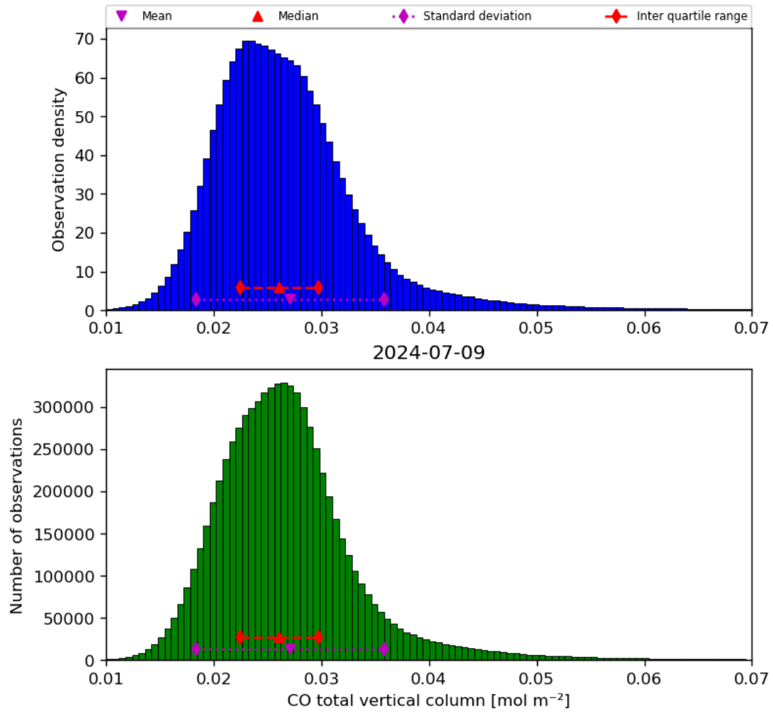
Figure 18: Histogram of “CO total vertical column” for 2024-07-08 to 2024-07-10
