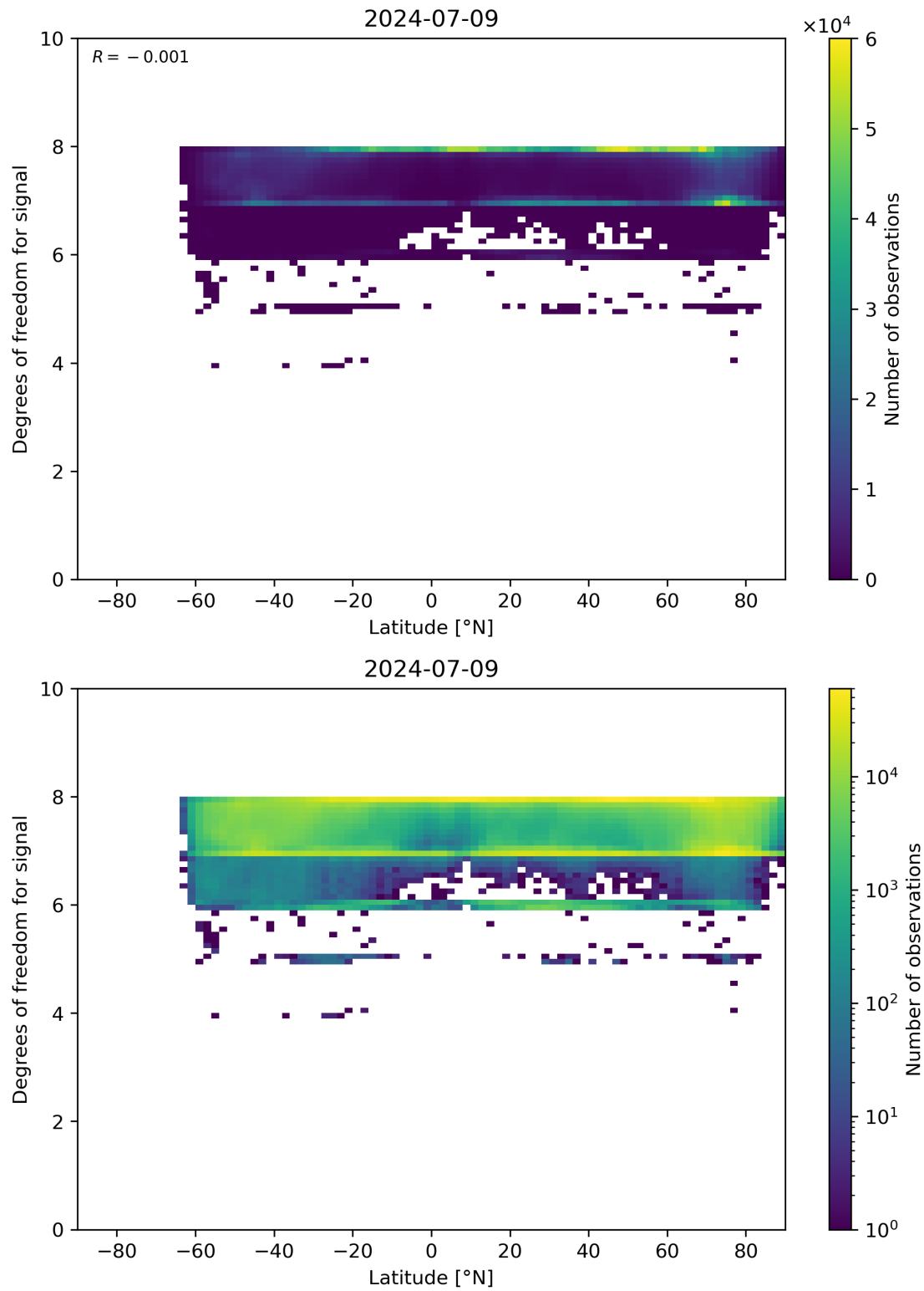
Figure 55: Scatter density plot of “Latitude” against “Degrees of freedom for signal” for 2024-07-08 to 2024-07-10.
