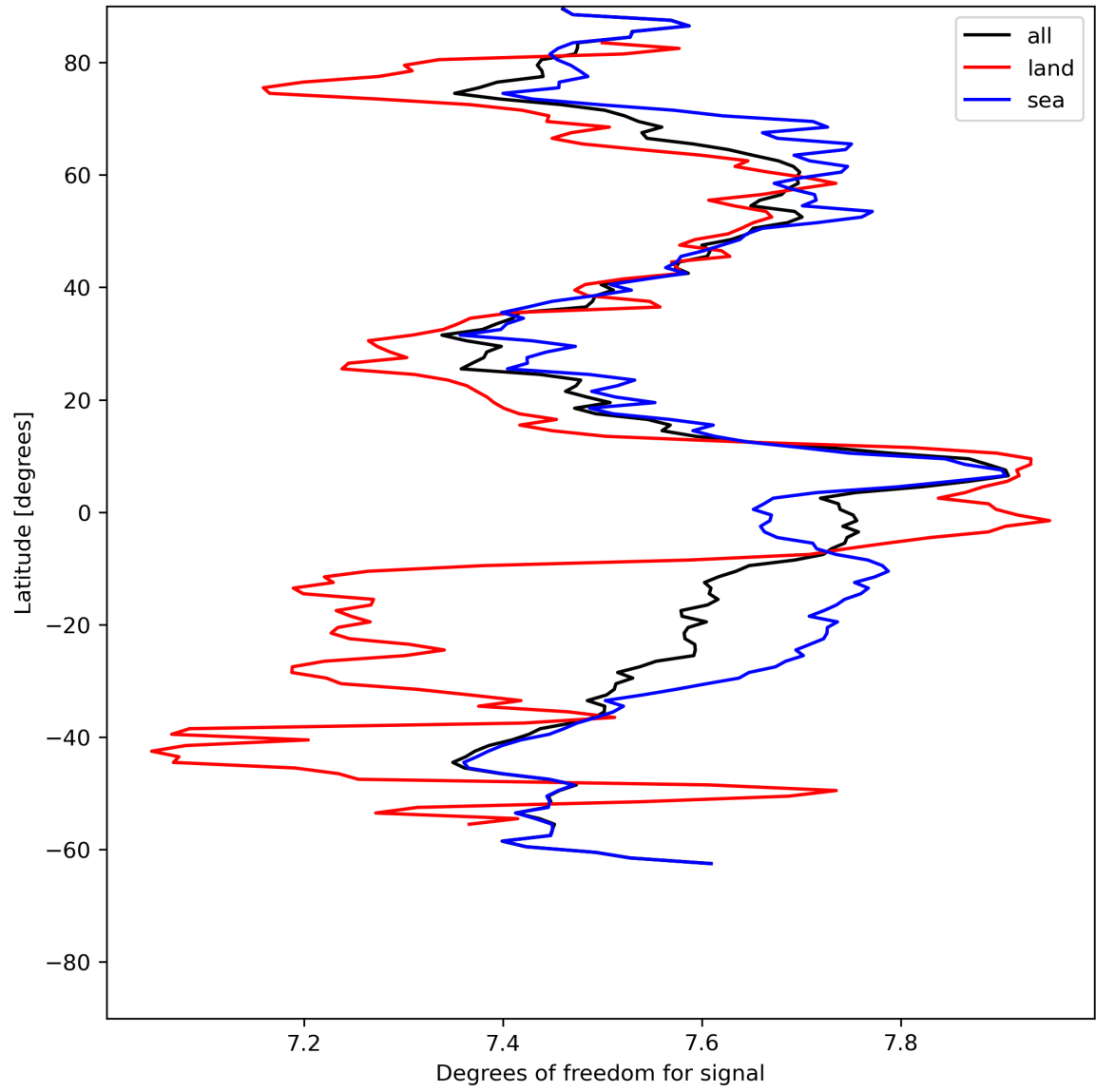
Figure 15: Zonal average of “Degrees of freedom for signal” for 2024-07-08 to 2024-07-10.
