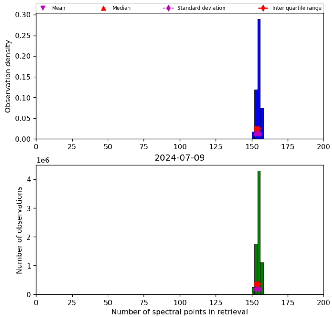
Figure 21: Histogram of “Number of spectral points in retrieval” for 2024-07-08 to 2024-07-10
