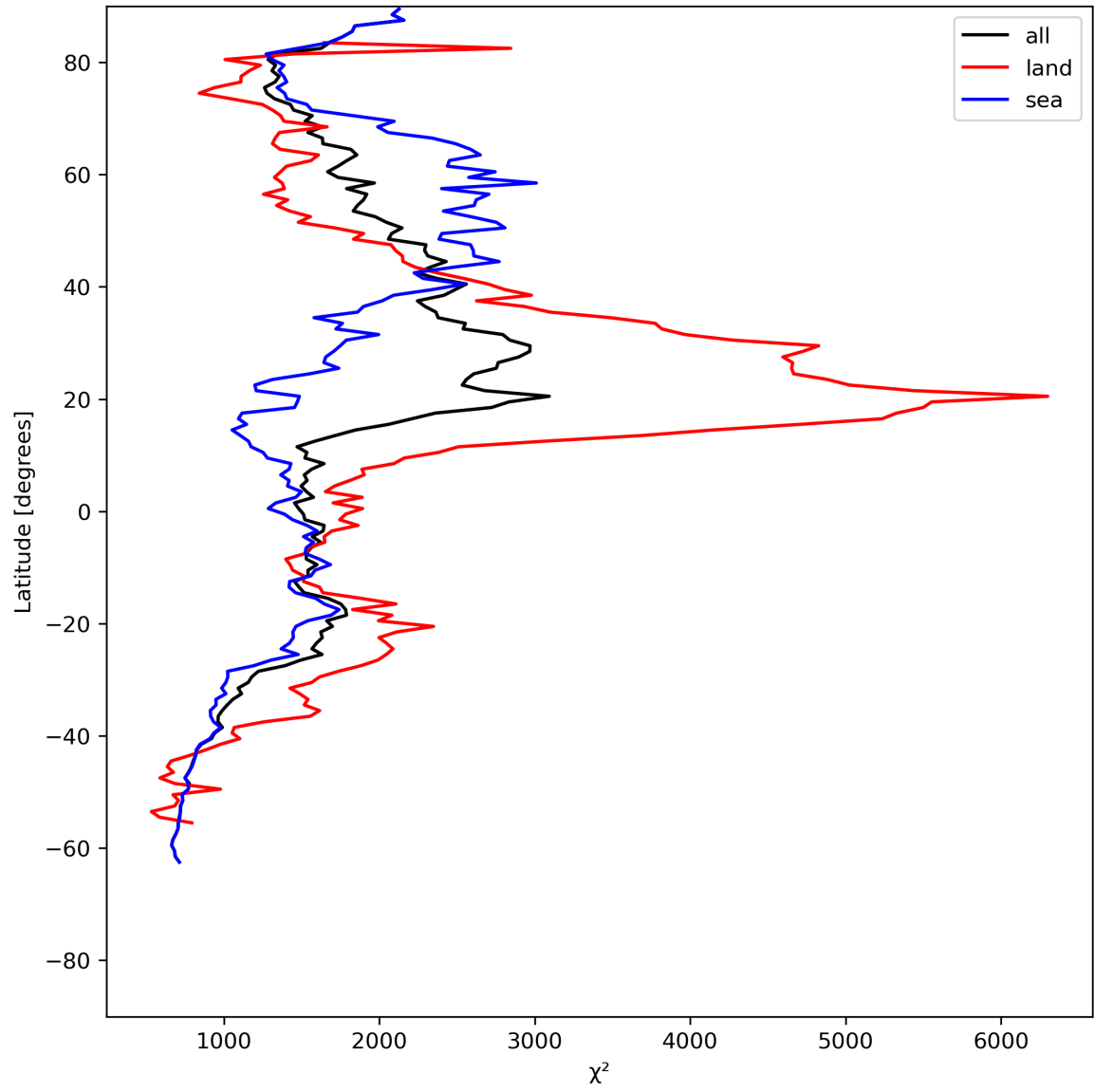
Figure 14: Zonal average of “ \chi^2 ” for 2024-07-08 to 2024-07-10.
