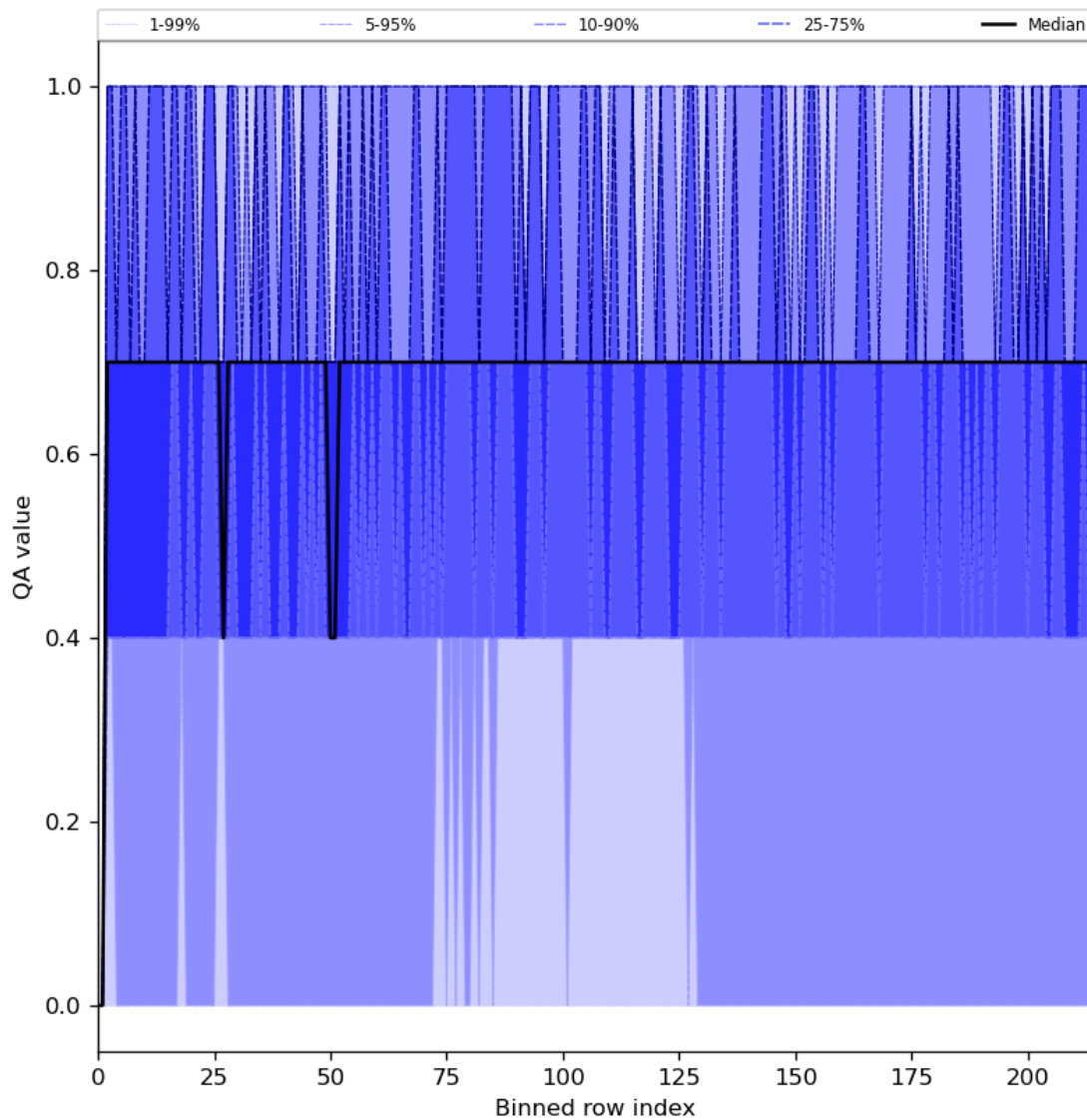
Figure 25: Along track statistics of “QA value” for 2024-07-08 to 2024-07-10
