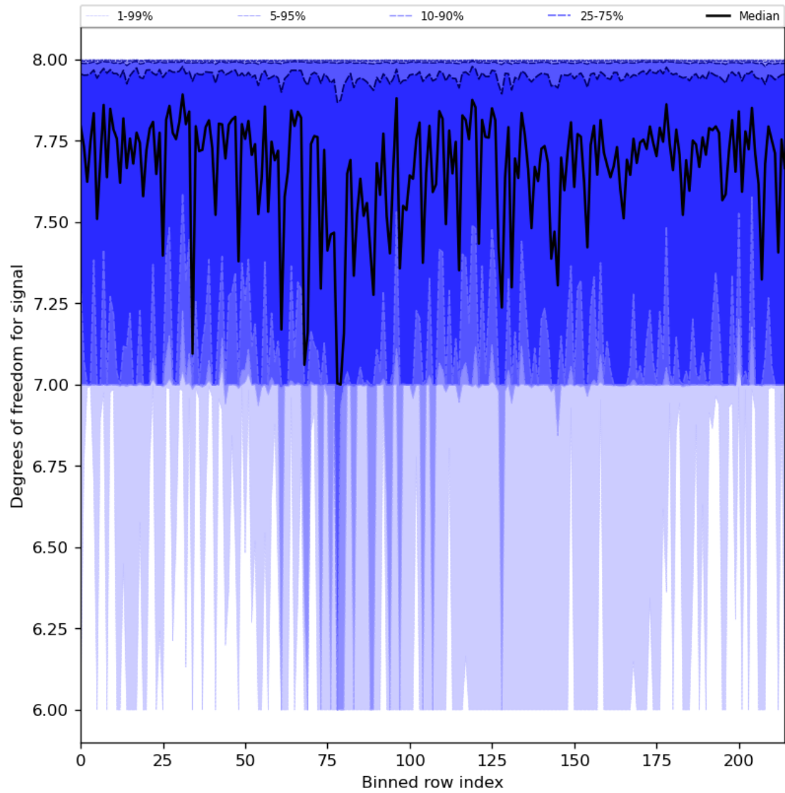
Figure 31: Along track statistics of “Degrees of freedom for signal” for 2024-07-08 to 2024-07-10
