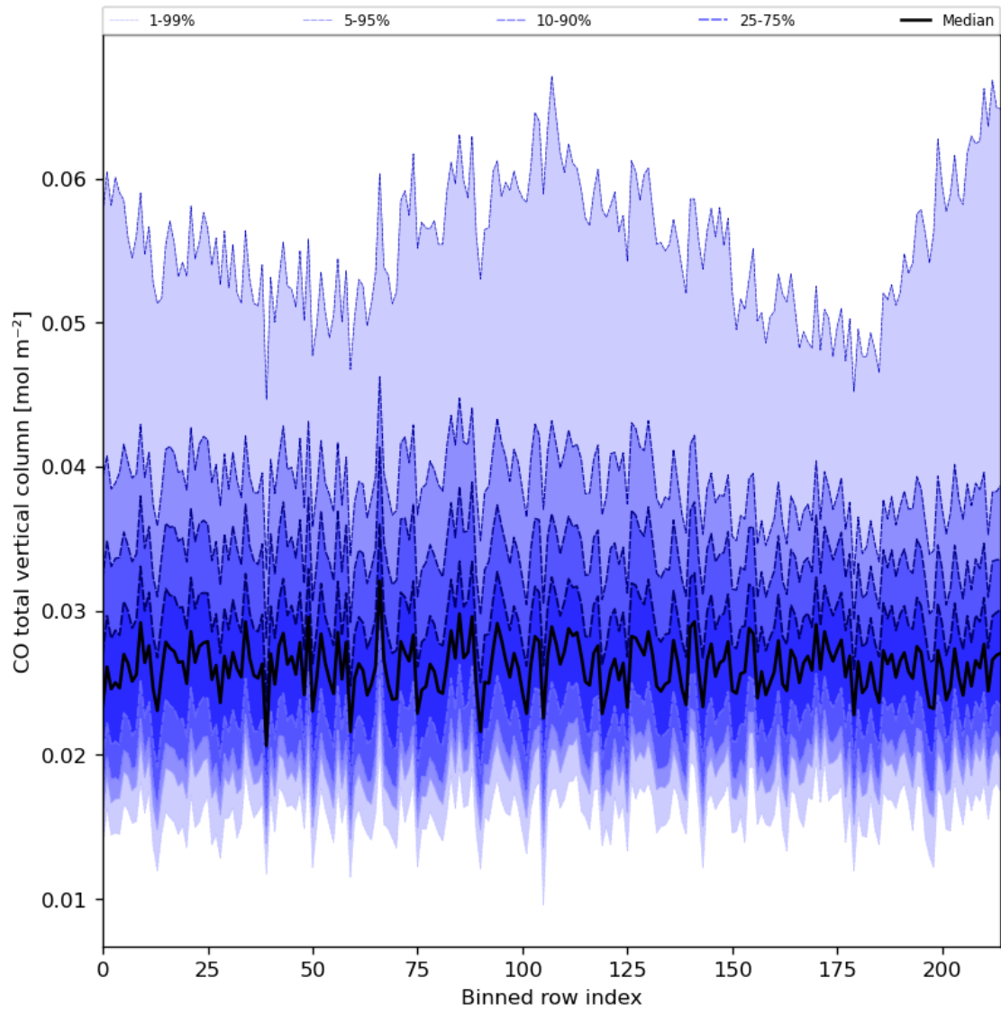
Figure 26: Along track statistics of “CO total vertical column” for 2024-07-08 to 2024-07-10
