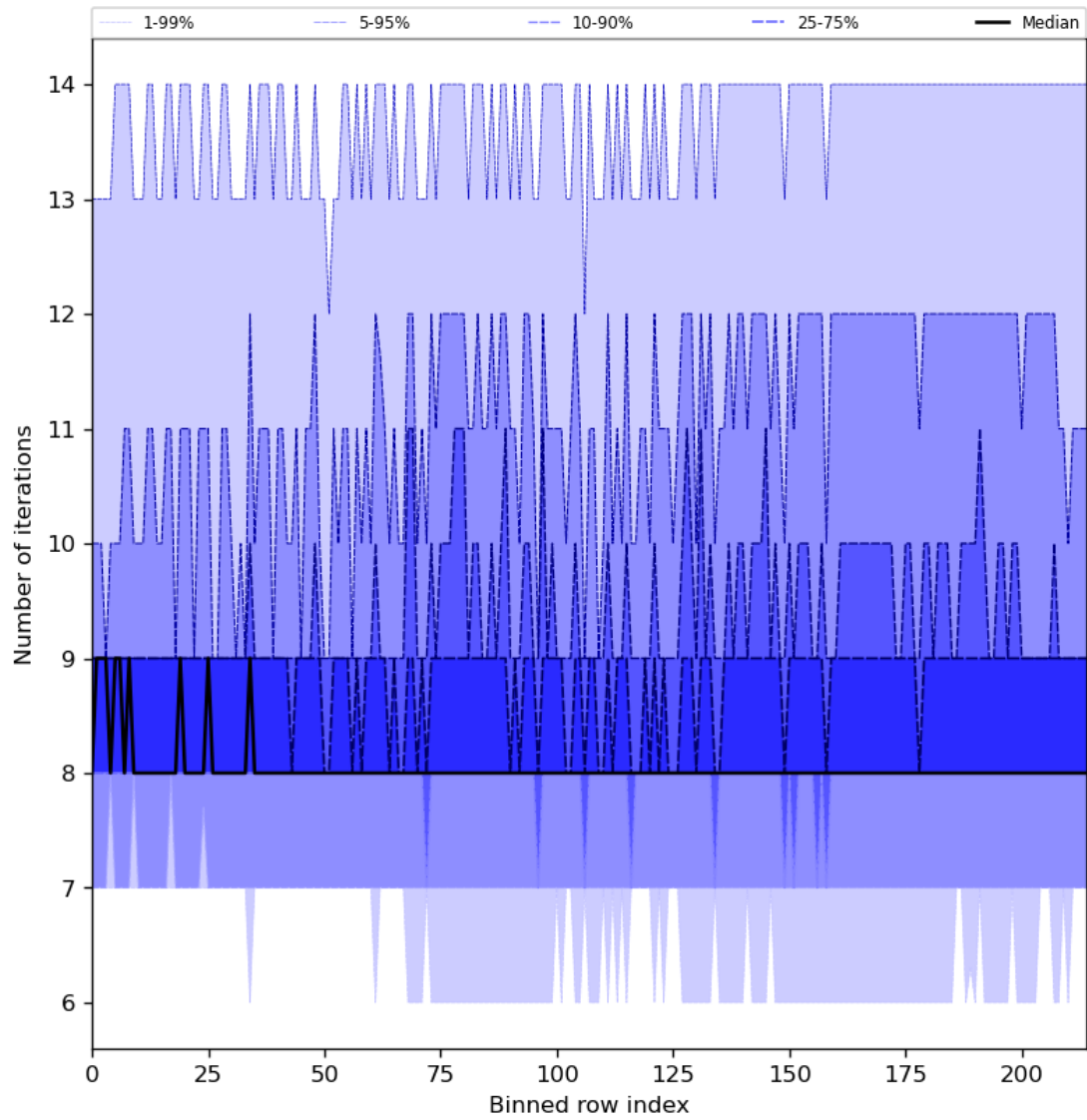
Figure 32: Along track statistics of “Number of iterations” for 2024-07-08 to 2024-07-10
