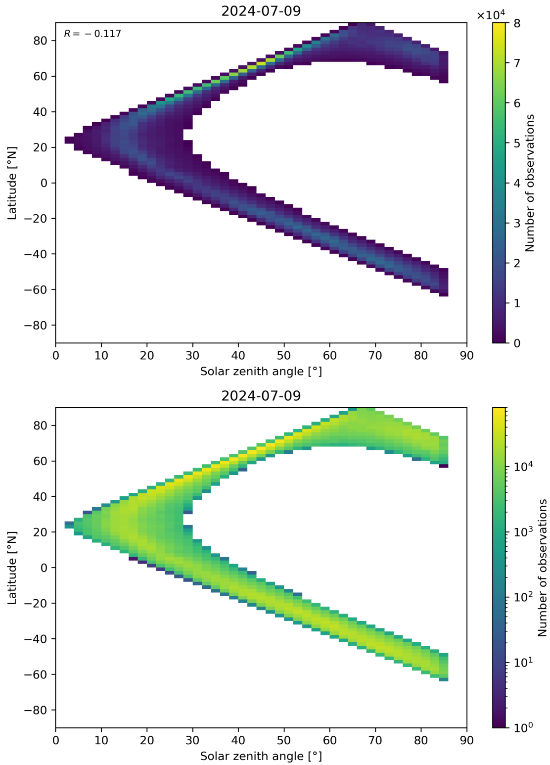
Figure 66: Scatter density plot of “Solar zenith angle” against “Latitude” for 2024-07-08 to 2024-07-10.
