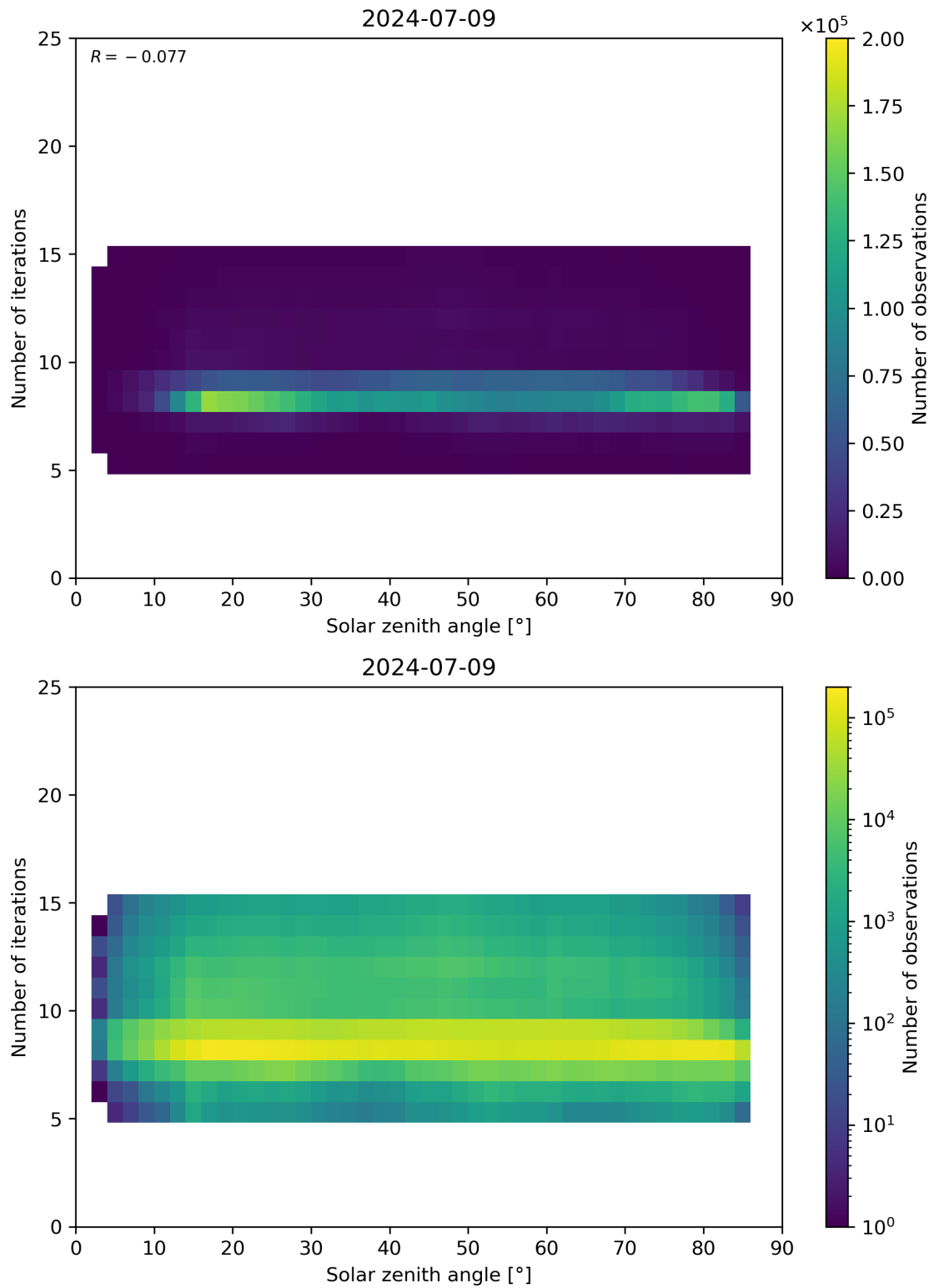
Figure 67: Scatter density plot of “Solar zenith angle” against “Number of iterations” for 2024-07-08 to 2024-07-10.
