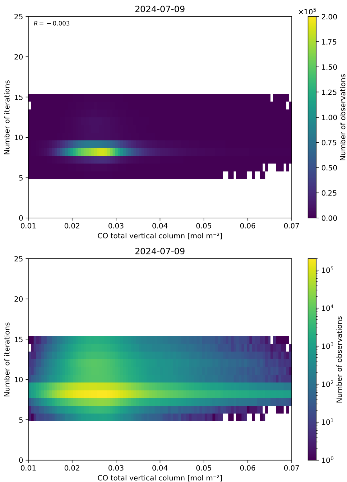
Figure 42: Scatter density plot of “CO total vertical column” against “Number of iterations” for 2024-07-08 to 2024-07-10.
