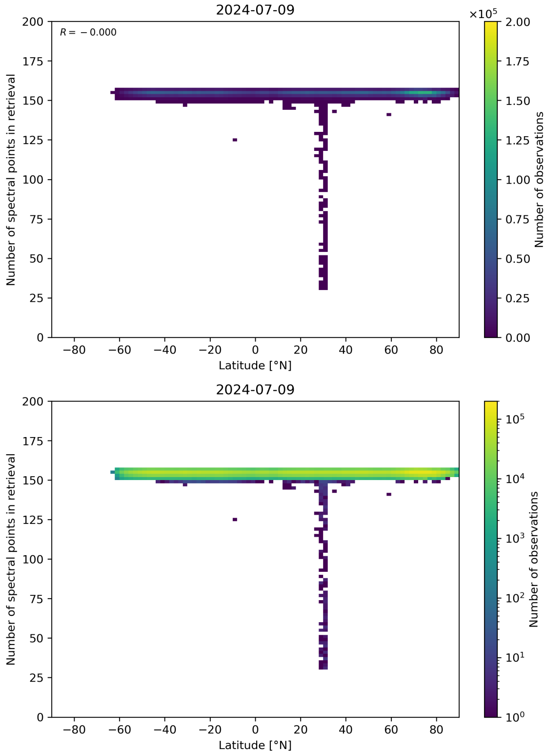
Figure 57: Scatter density plot of “Latitude” against “Number of spectral points in retrieval” for 2024-07-08 to 2024-07-10.
