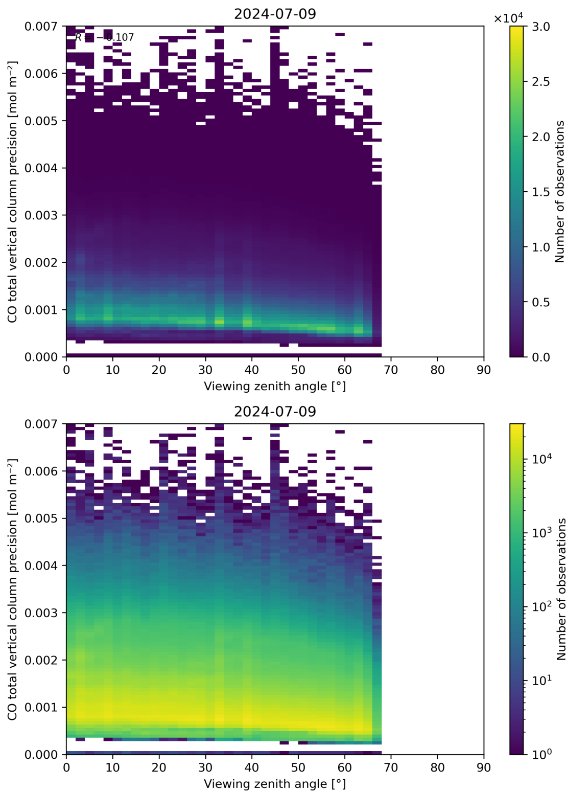
Figure 71: Scatter density plot of “Viewing zenith angle” against “CO total vertical column precision” for 2024-07-08 to 2024-07-10.
