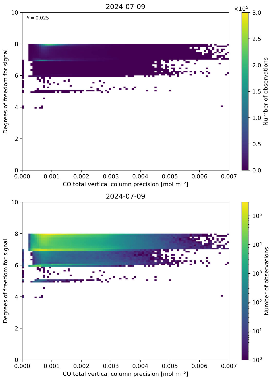
Figure 45: Scatter density plot of “CO total vertical column precision” against “Degrees of freedom for signal” for 2024-07-08 to 2024-07-10.
