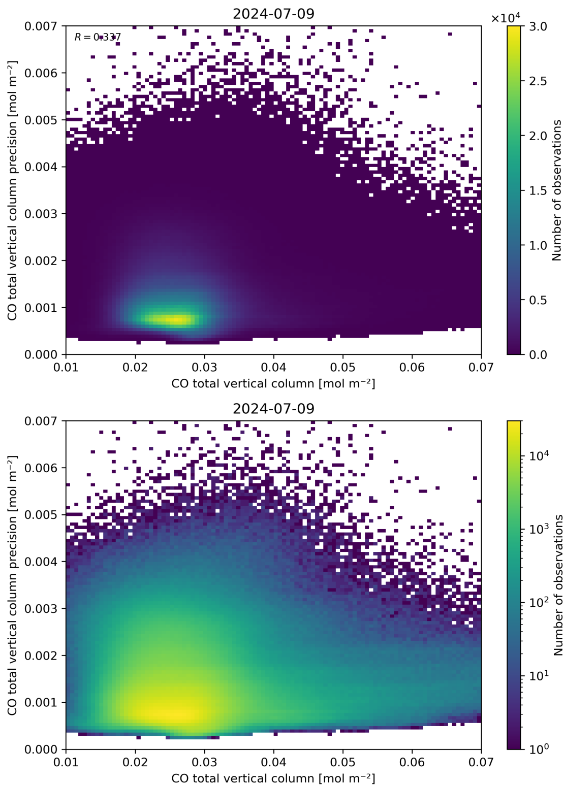
Figure 34: Scatter density plot of “CO total vertical column” against “CO total vertical column precision” for 2024-07-08 to 2024-07-10.
