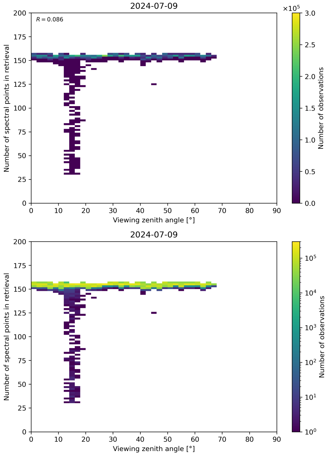
Figure 76: Scatter density plot of “Viewing zenith angle” against “Number of spectral points in retrieval” for 2024-07-08 to 2024-07-10.
