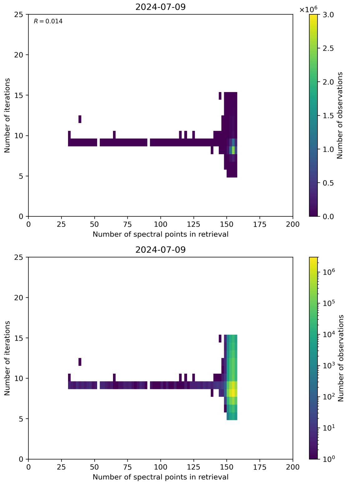
Figure 60: Scatter density plot of “Number of spectral points in retrieval” against “Number of iterations” for 2024-07-08 to 2024-07-10.
