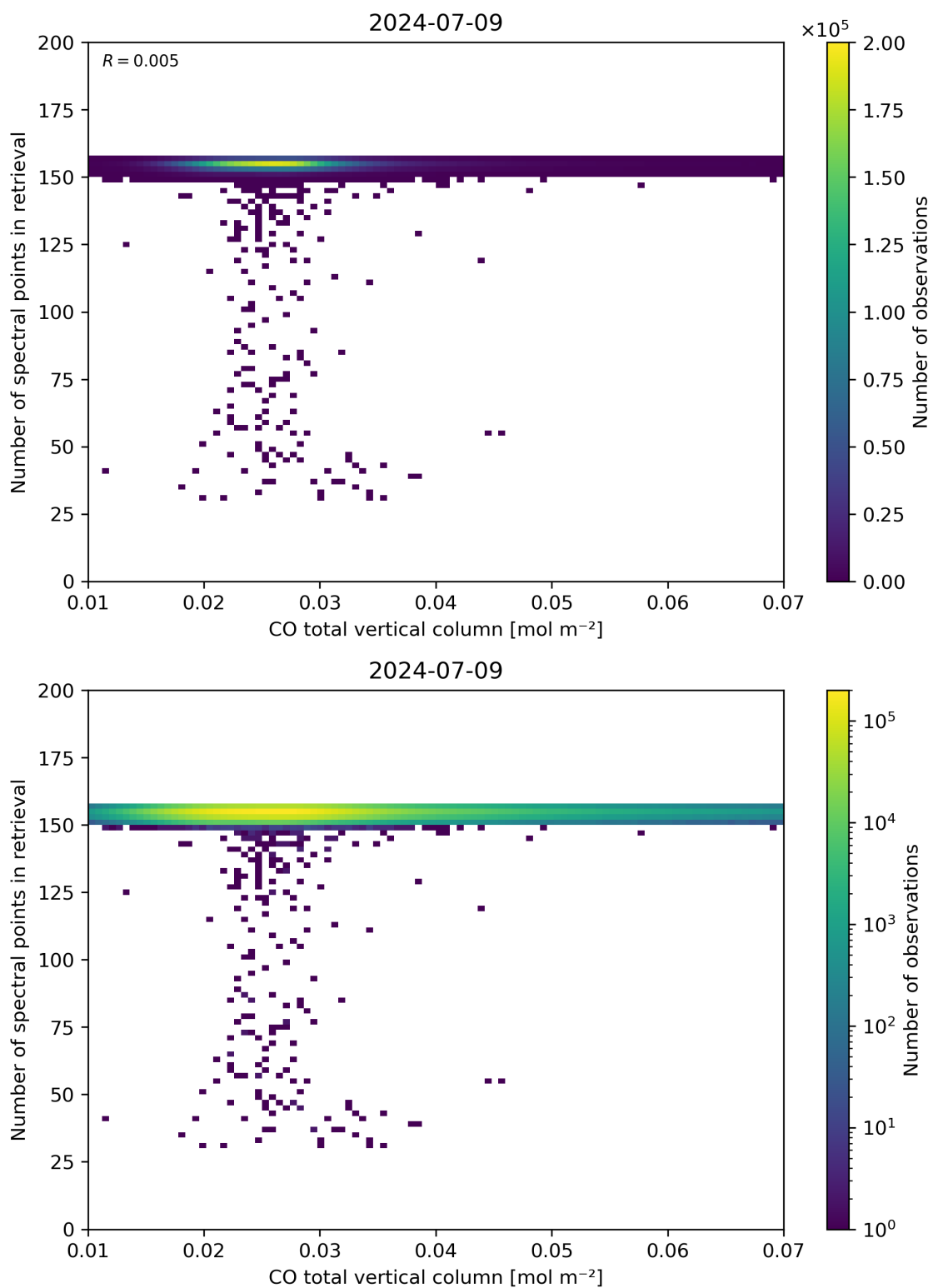
Figure 43: Scatter density plot of “CO total vertical column” against “Number of spectral points in retrieval” for 2024-07-08 to 2024-07-10.
