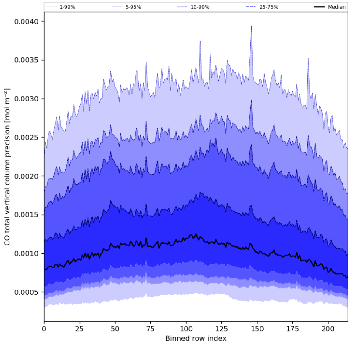
Figure 28: Along track statistics of “CO total vertical column precision” for 2024-07-08 to 2024-07-10
