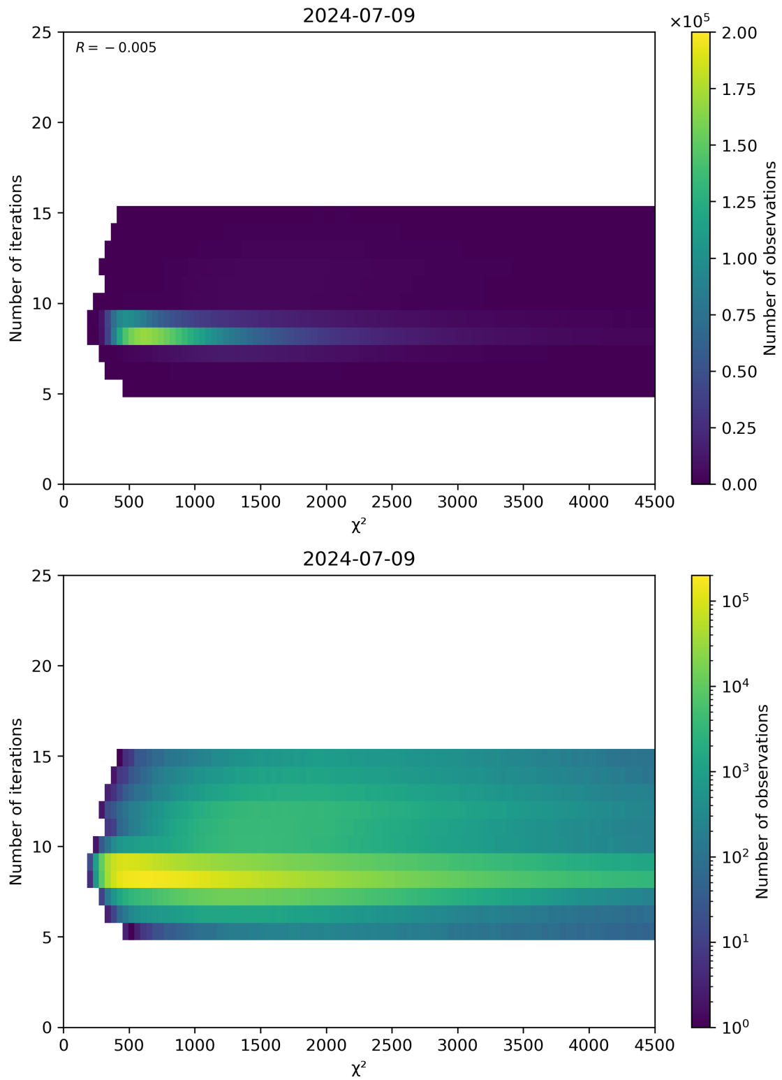
Figure 49: Scatter density plot of “ \chi^2 ” against “Number of iterations” for 2024-07-08 to 2024-07-10.
