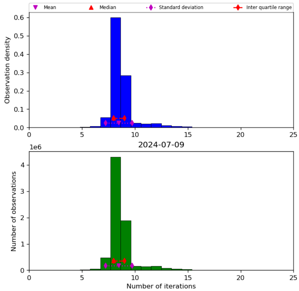
Figure 24: Histogram of “Number of iterations” for 2024-07-08 to 2024-07-10
