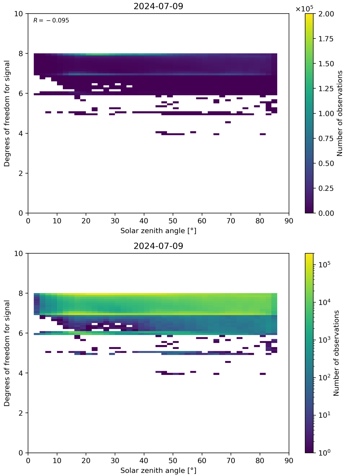
Figure 65: Scatter density plot of “Solar zenith angle” against “Degrees of freedom for signal” for 2024-07-08 to 2024-07-10.
