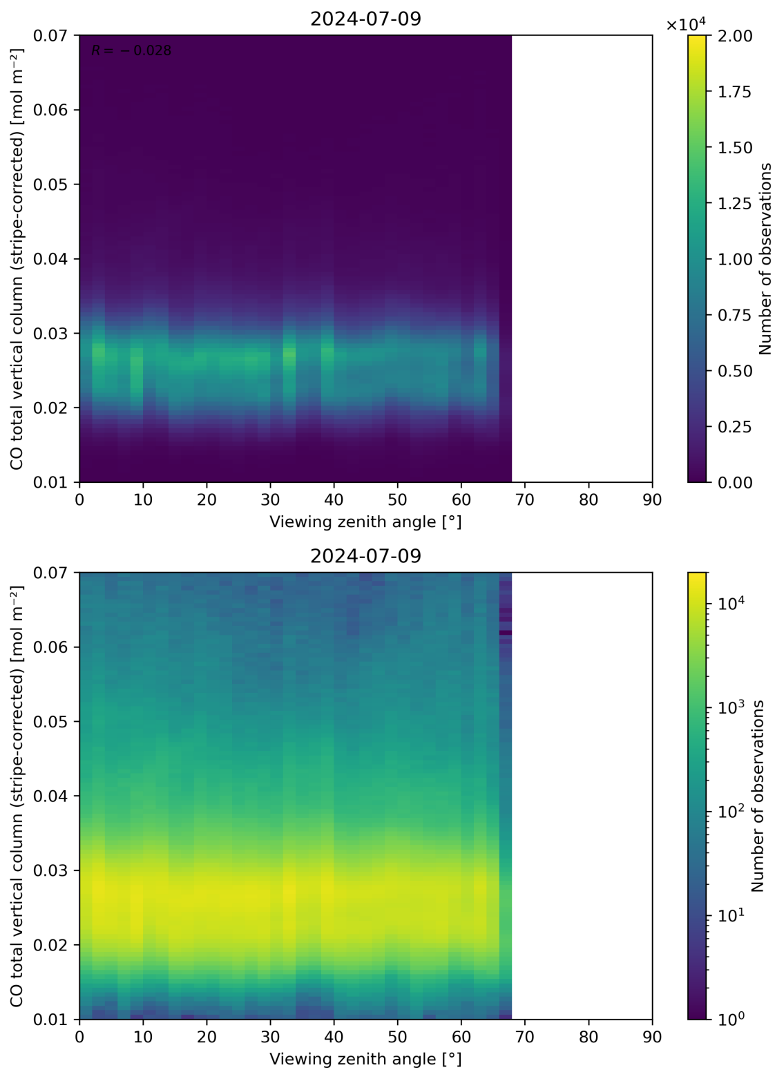
Figure 70: Scatter density plot of “Viewing zenith angle” against “CO total vertical column (stripe-corrected)” for 2024-07-08 to 2024-07-10.
