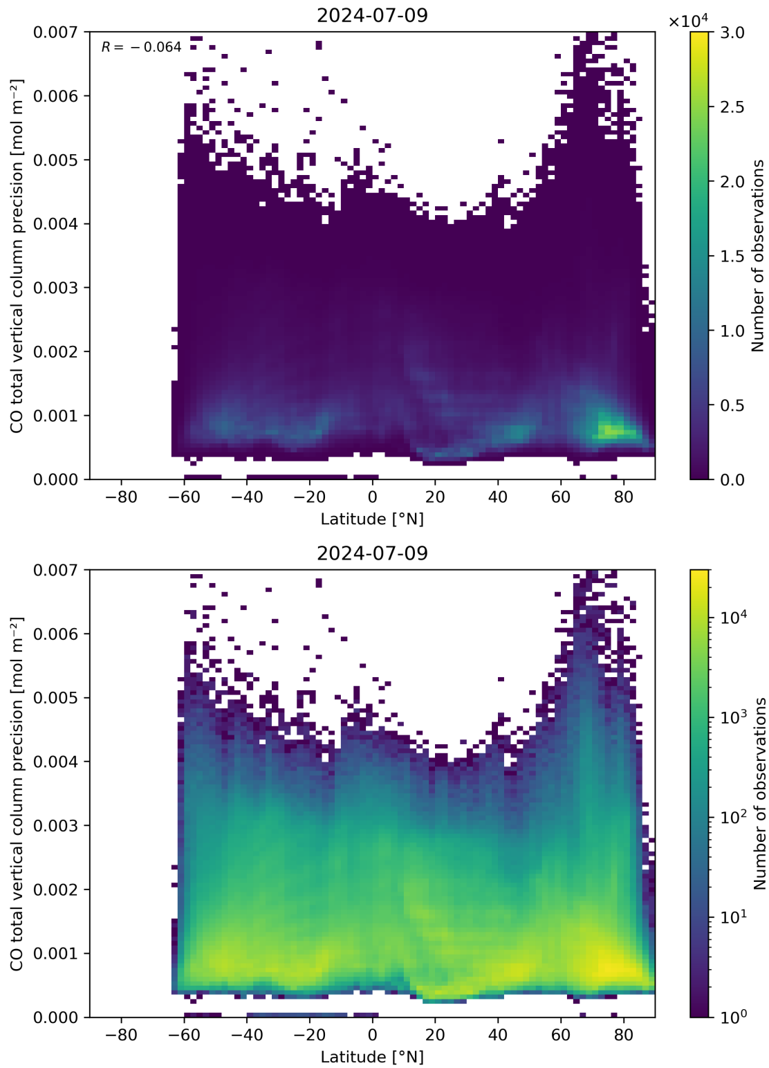
Figure 53: Scatter density plot of “Latitude” against “CO total vertical column precision” for 2024-07-08 to 2024-07-10.
