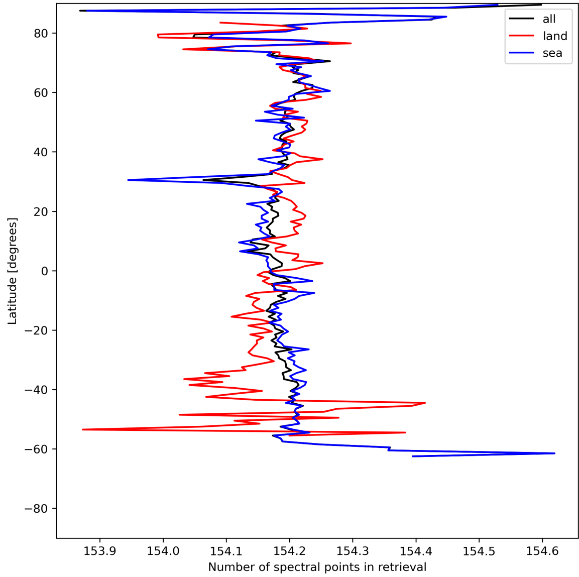
Figure 13: Zonal average of “Number of spectral points in retrieval” for 2024-07-08 to 2024-07-10.
