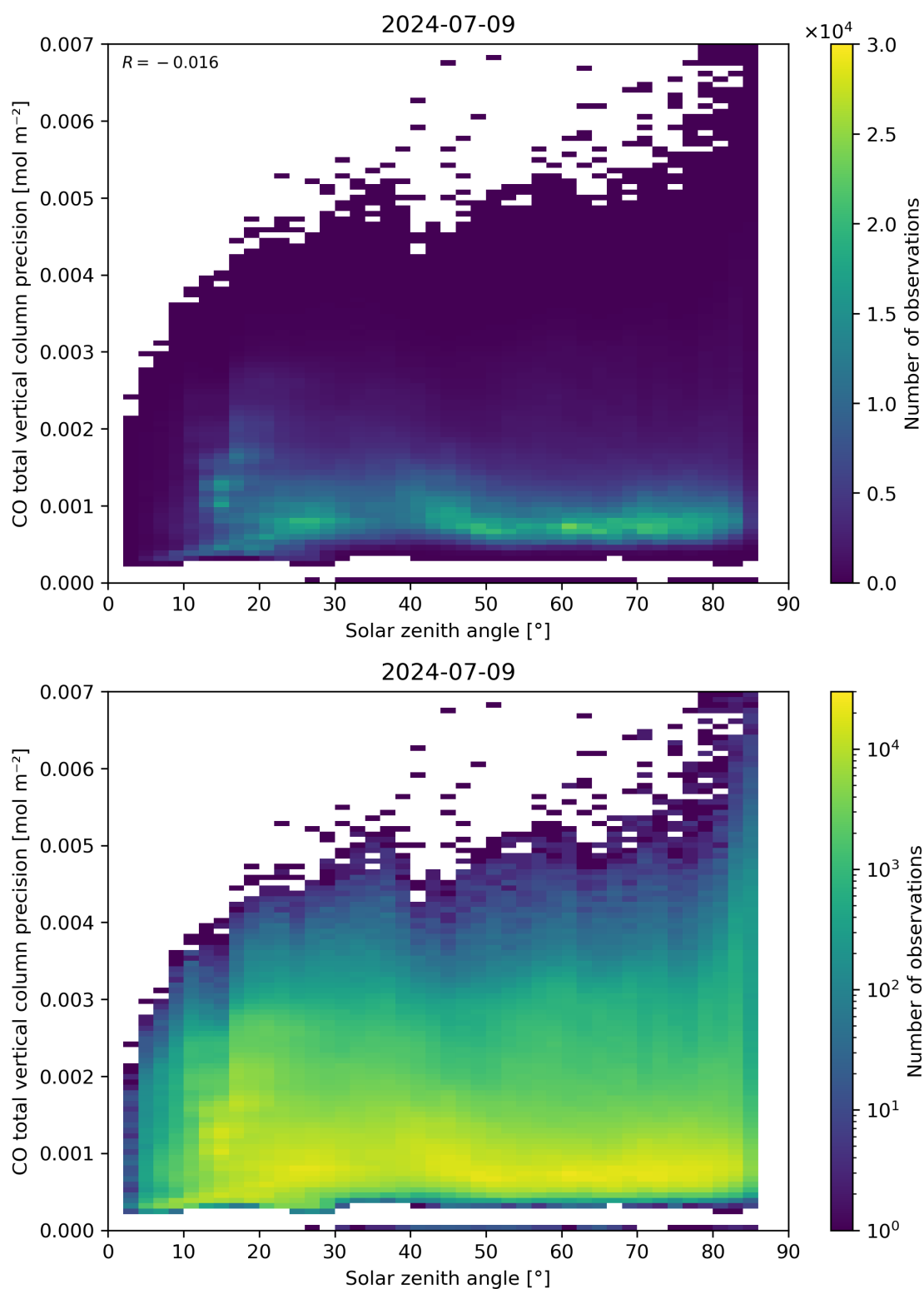
Figure 63: Scatter density plot of “Solar zenith angle” against “CO total vertical column precision” for 2024-07-08 to 2024-07-10.
