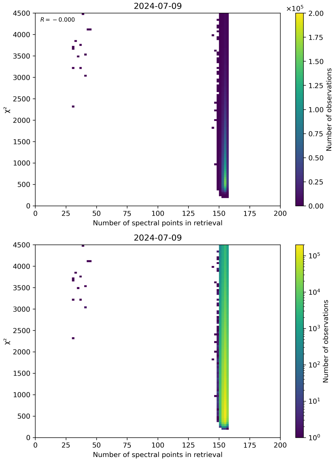
Figure 58: Scatter density plot of “Number of spectral points in retrieval” against “ \chi^2 ” for 2024-07-08 to 2024-07-10.
