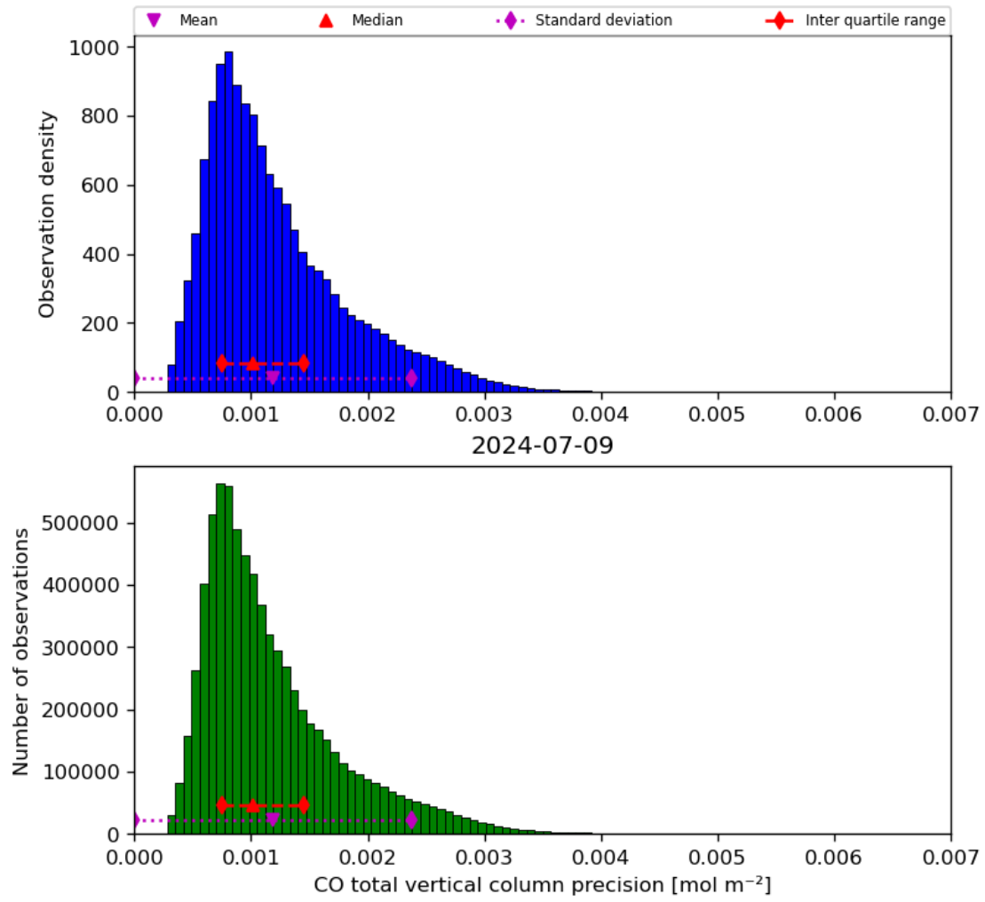
Figure 20: Histogram of “CO total vertical column precision” for 2024-07-08 to 2024-07-10
