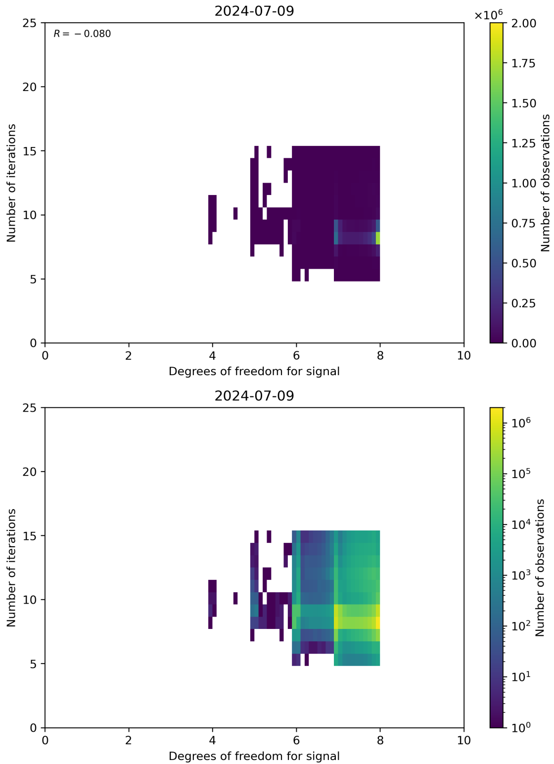
Figure 50: Scatter density plot of “Degrees of freedom for signal” against “Number of iterations” for 2024-07-08 to 2024-07-10.
