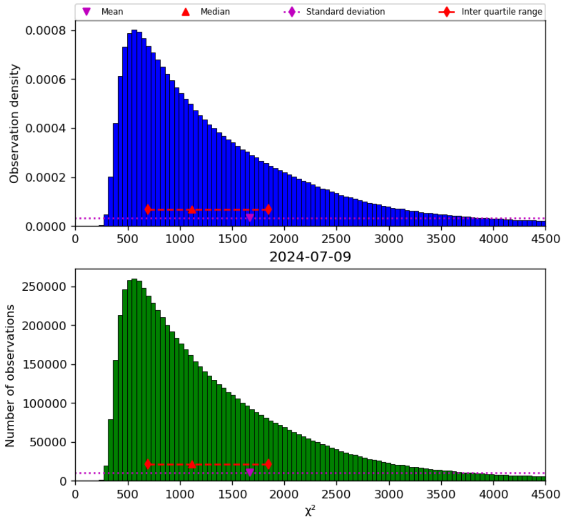
Figure 22: Histogram of “ \chi^2 ” for 2024-07-08 to 2024-07-10
