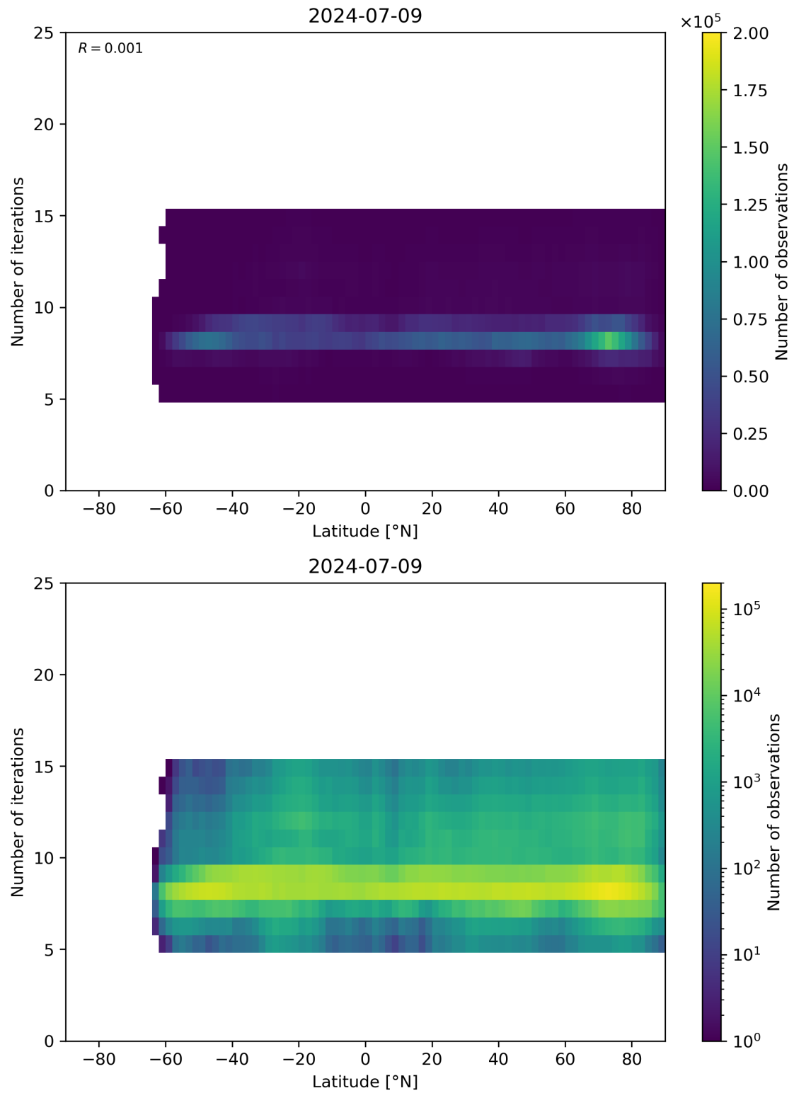
Figure 56: Scatter density plot of “Latitude” against “Number of iterations” for 2024-07-08 to 2024-07-10.
