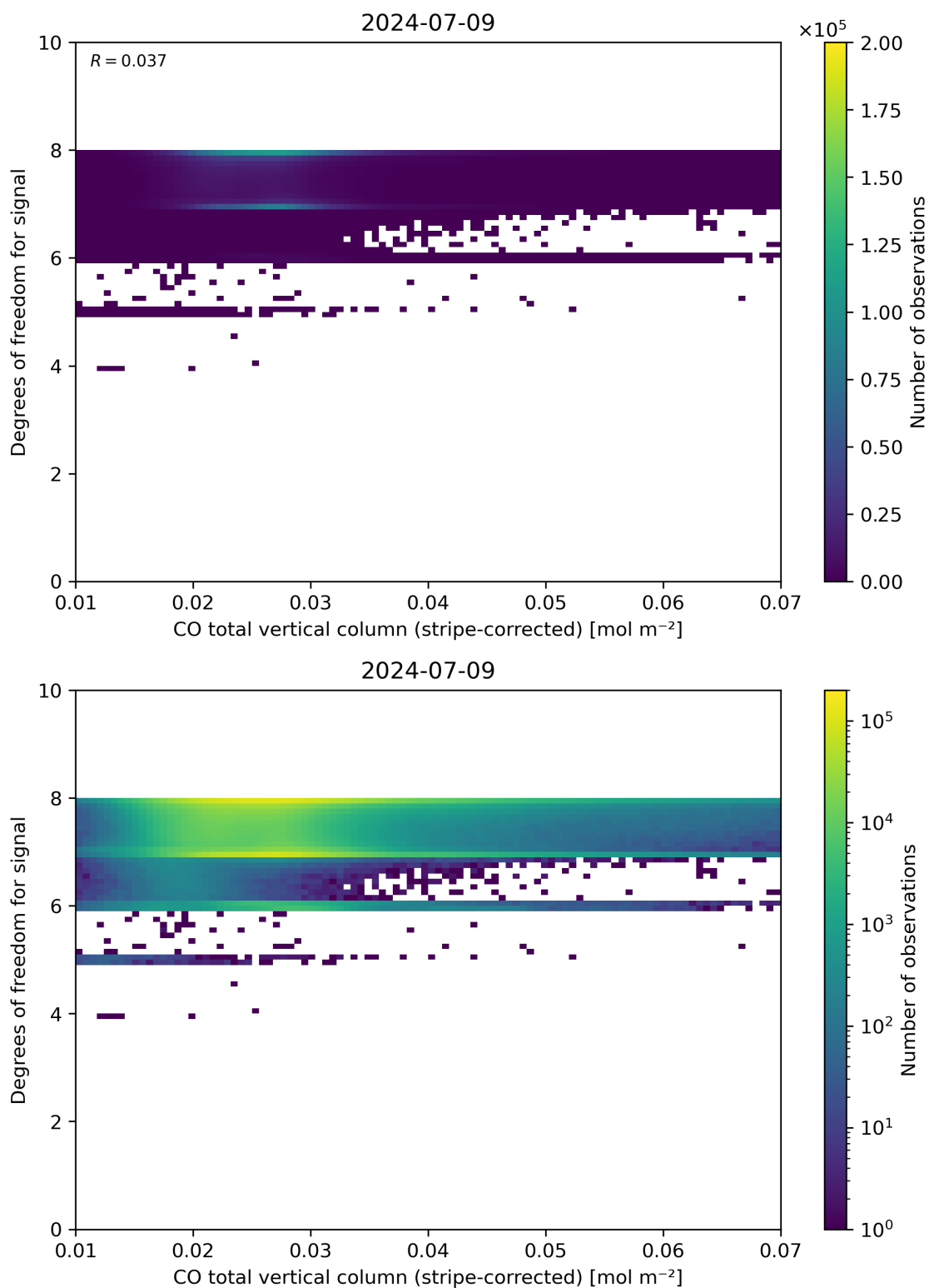
Figure 38: Scatter density plot of “CO total vertical column (stripe-corrected)” against “Degrees of freedom for signal” for 2024-07-08 to 2024-07-10.
