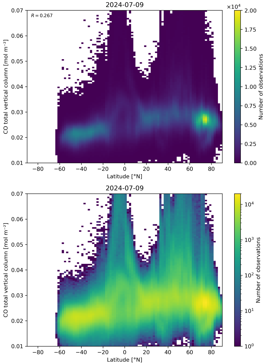
Figure 51: Scatter density plot of “Latitude” against “CO total vertical column” for 2024-07-08 to 2024-07-10.
