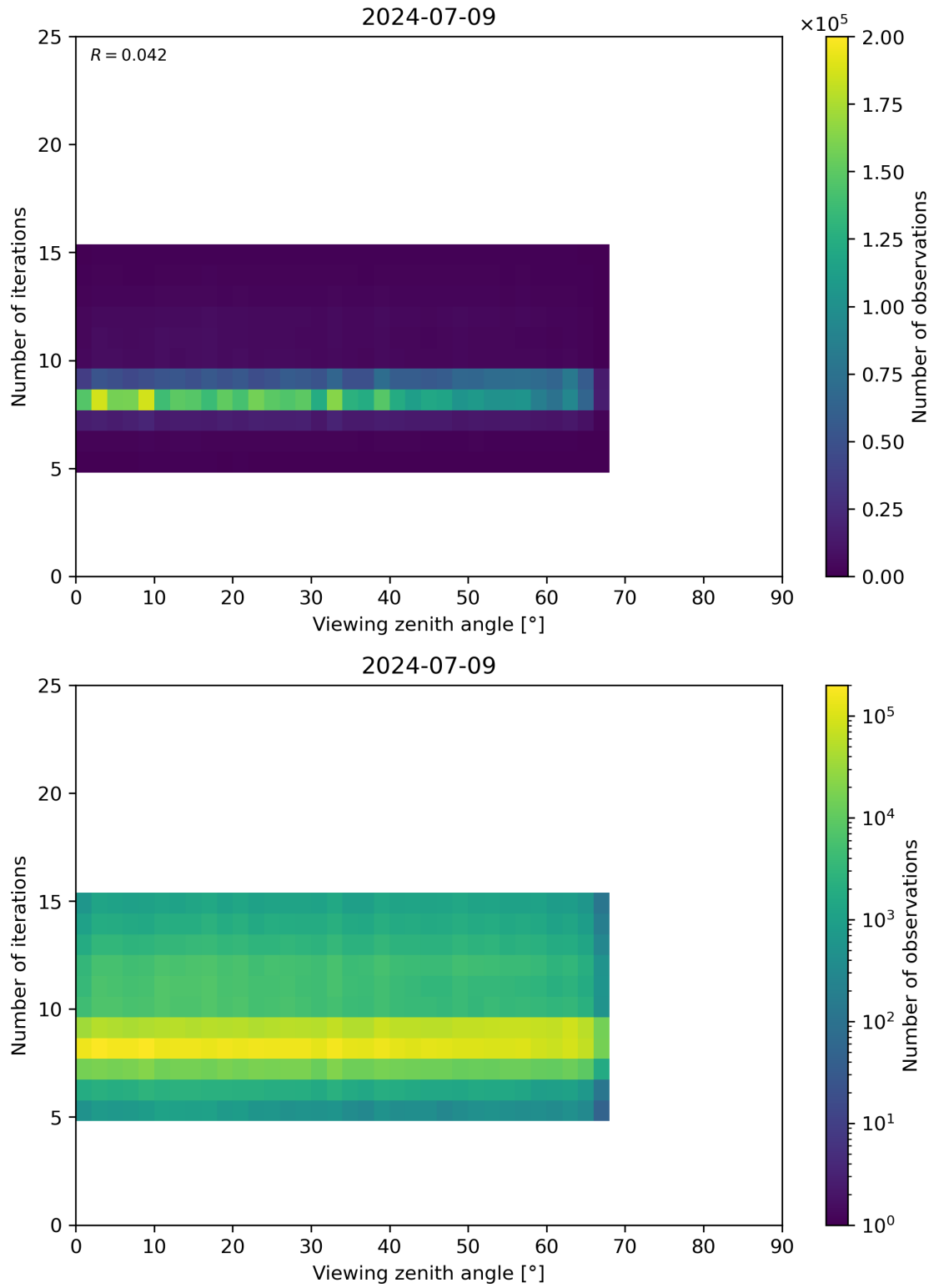
Figure 75: Scatter density plot of “Viewing zenith angle” against “Number of iterations” for 2024-07-08 to 2024-07-10.
