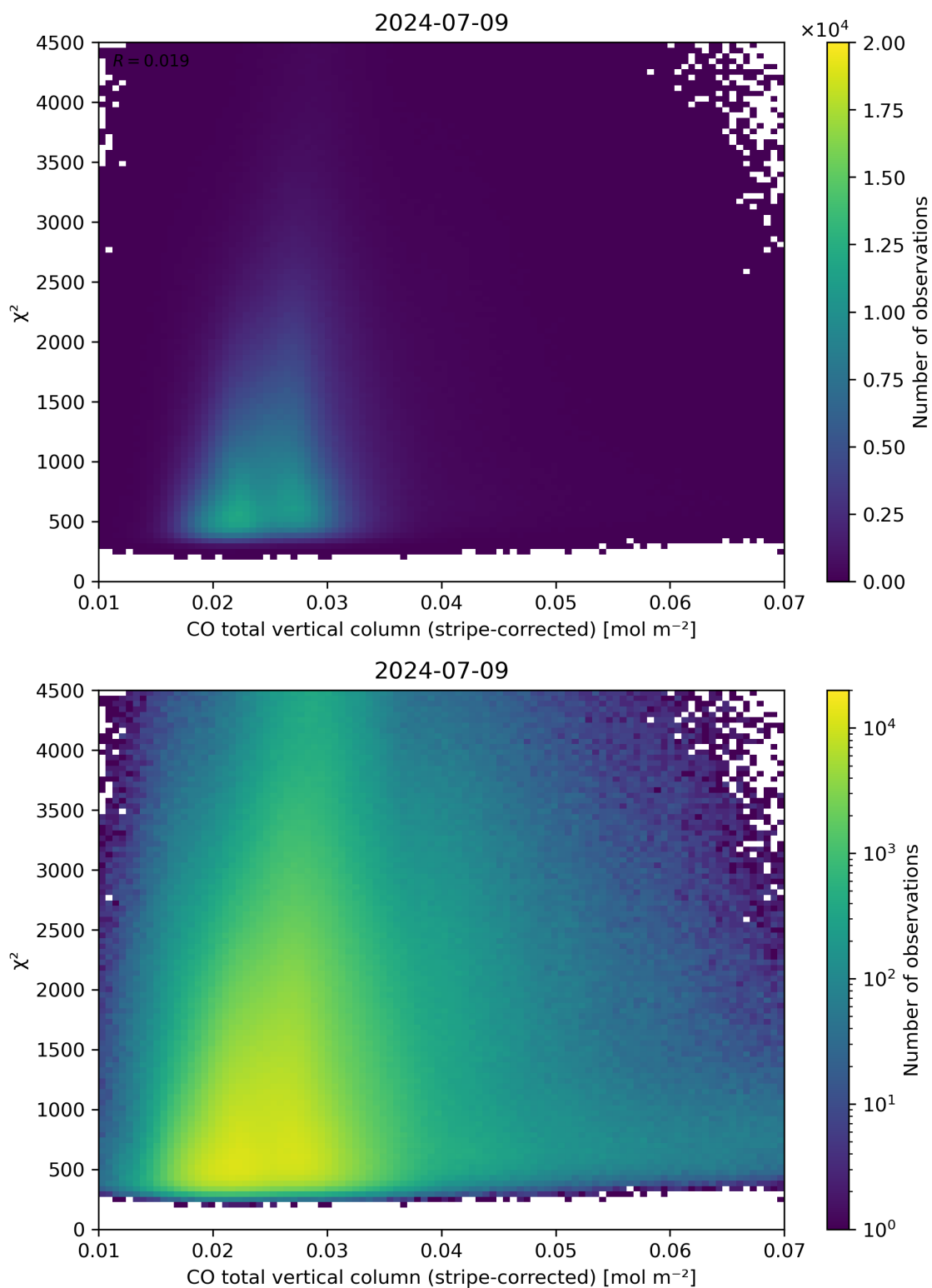
Figure 37: Scatter density plot of “CO total vertical column (stripe-corrected)” against “ \chi^2 ” for 2024-07-08 to 2024-07-10.
