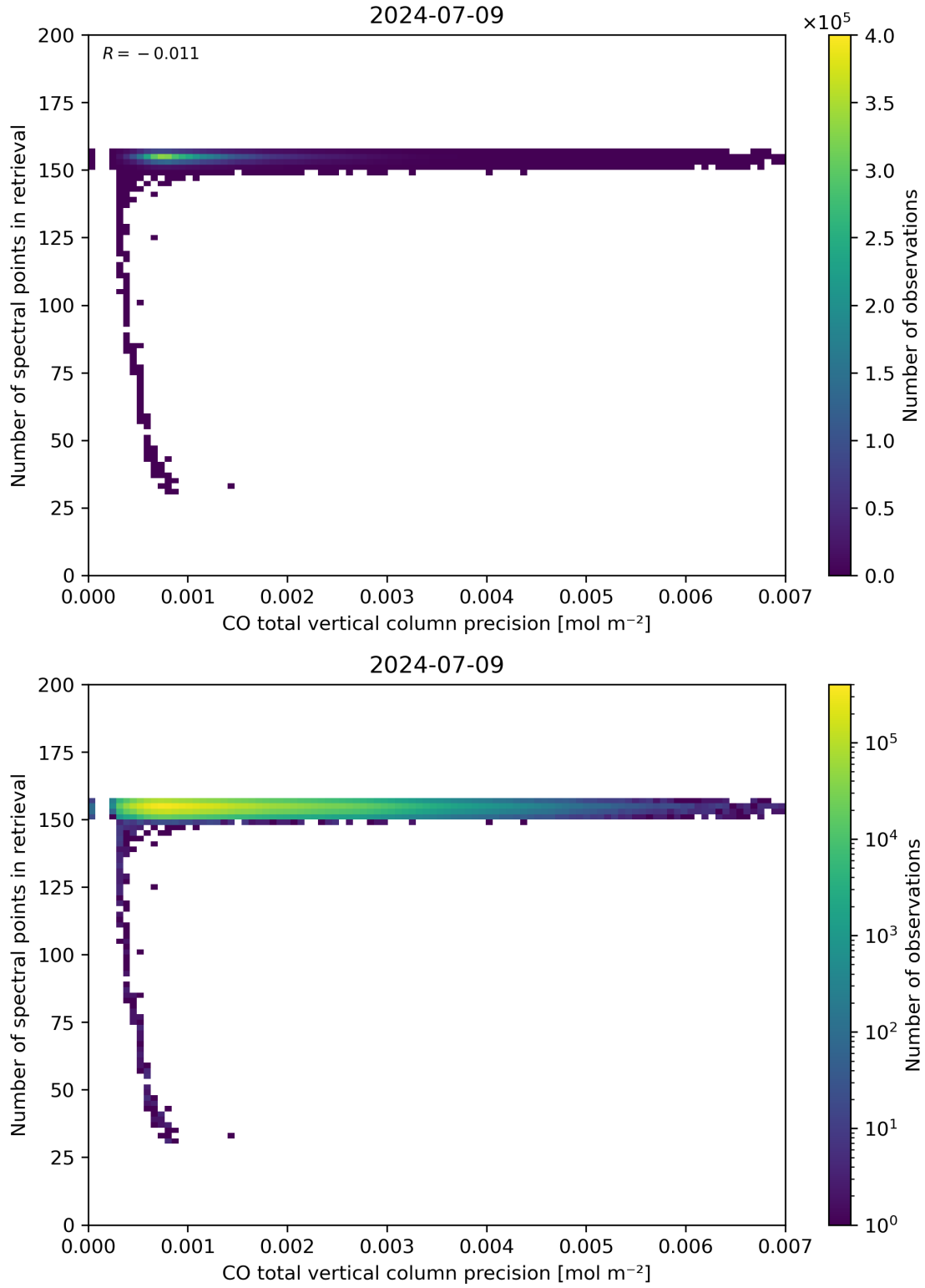
Figure 47: Scatter density plot of “CO total vertical column precision” against “Number of spectral points in retrieval” for 2024-07-08 to 2024-07-10.
