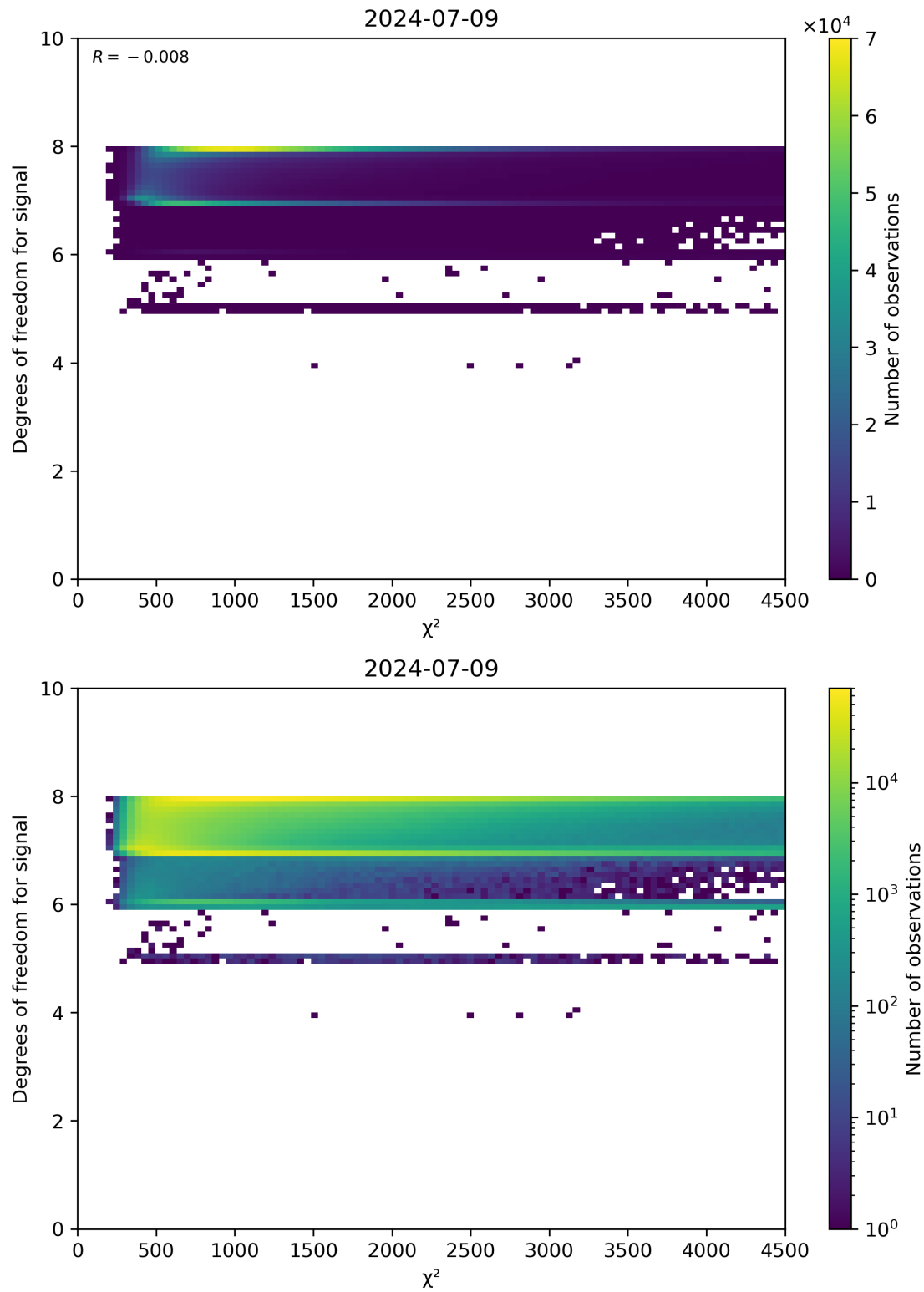
Figure 48: Scatter density plot of “ \chi^2 ” against “Degrees of freedom for signal” for 2024-07-08 to 2024-07-10.
