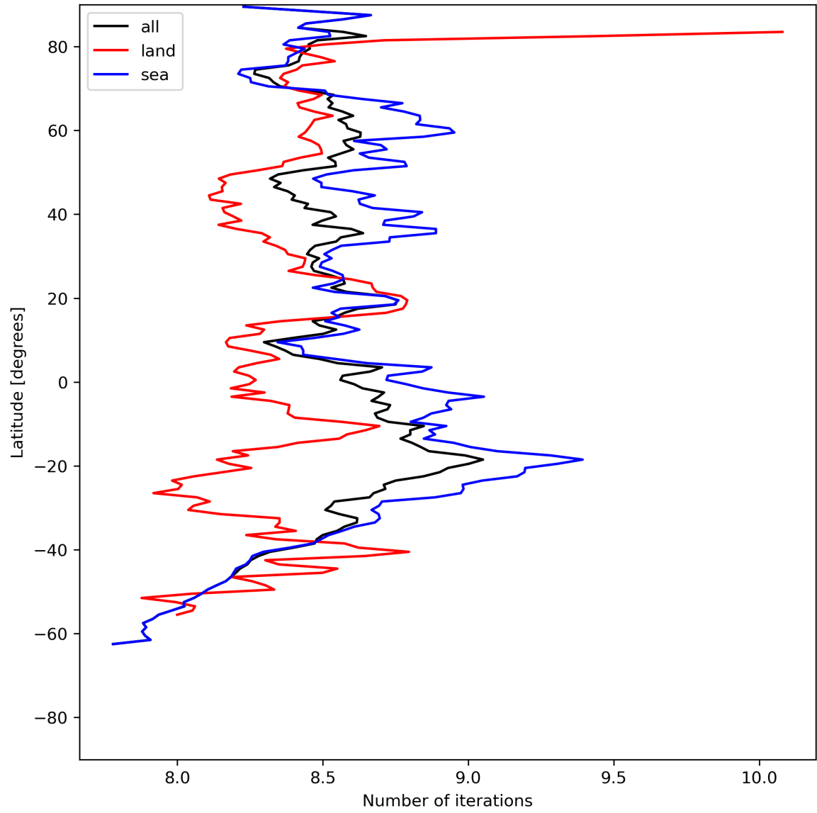
Figure 16: Zonal average of “Number of iterations” for 2024-07-08 to 2024-07-10.
