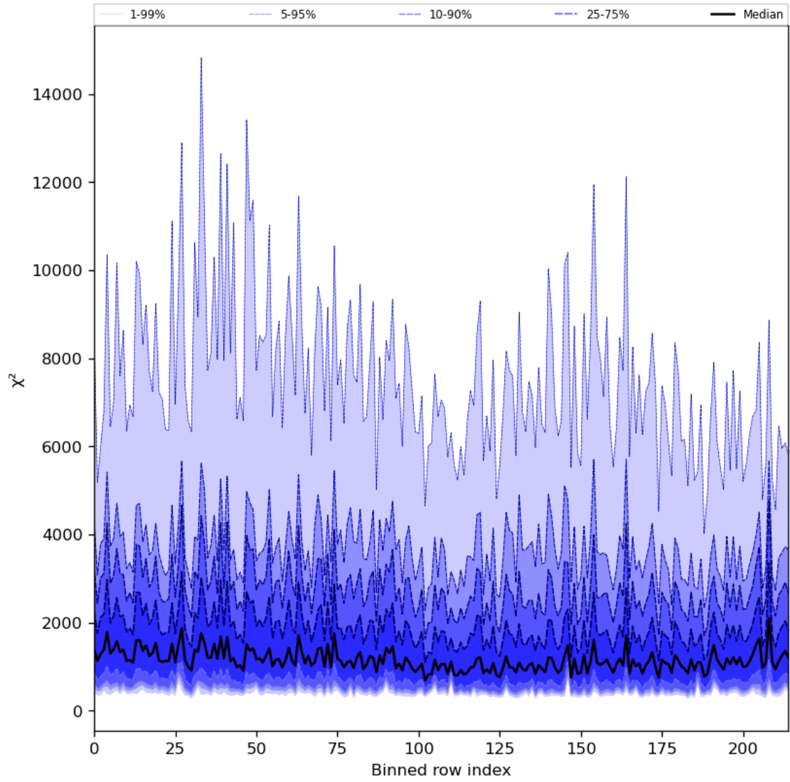
Figure 30: Along track statistics of “ \chi^2 ” for 2024-07-08 to 2024-07-10
