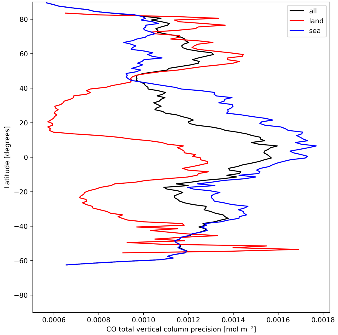
Figure 12: Zonal average of “CO total vertical column precision” for 2024-07-08 to 2024-07-10.
