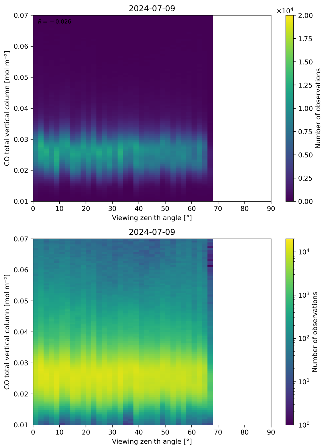
Figure 69: Scatter density plot of “Viewing zenith angle” against “CO total vertical column” for 2024-07-08 to 2024-07-10.
