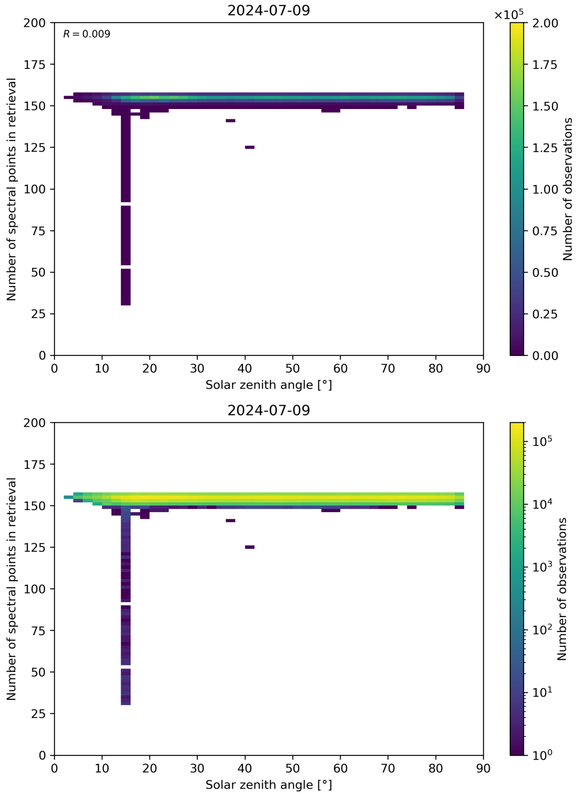
Figure 68: Scatter density plot of “Solar zenith angle” against “Number of spectral points in retrieval” for 2024-07-08 to 2024-07-10.
