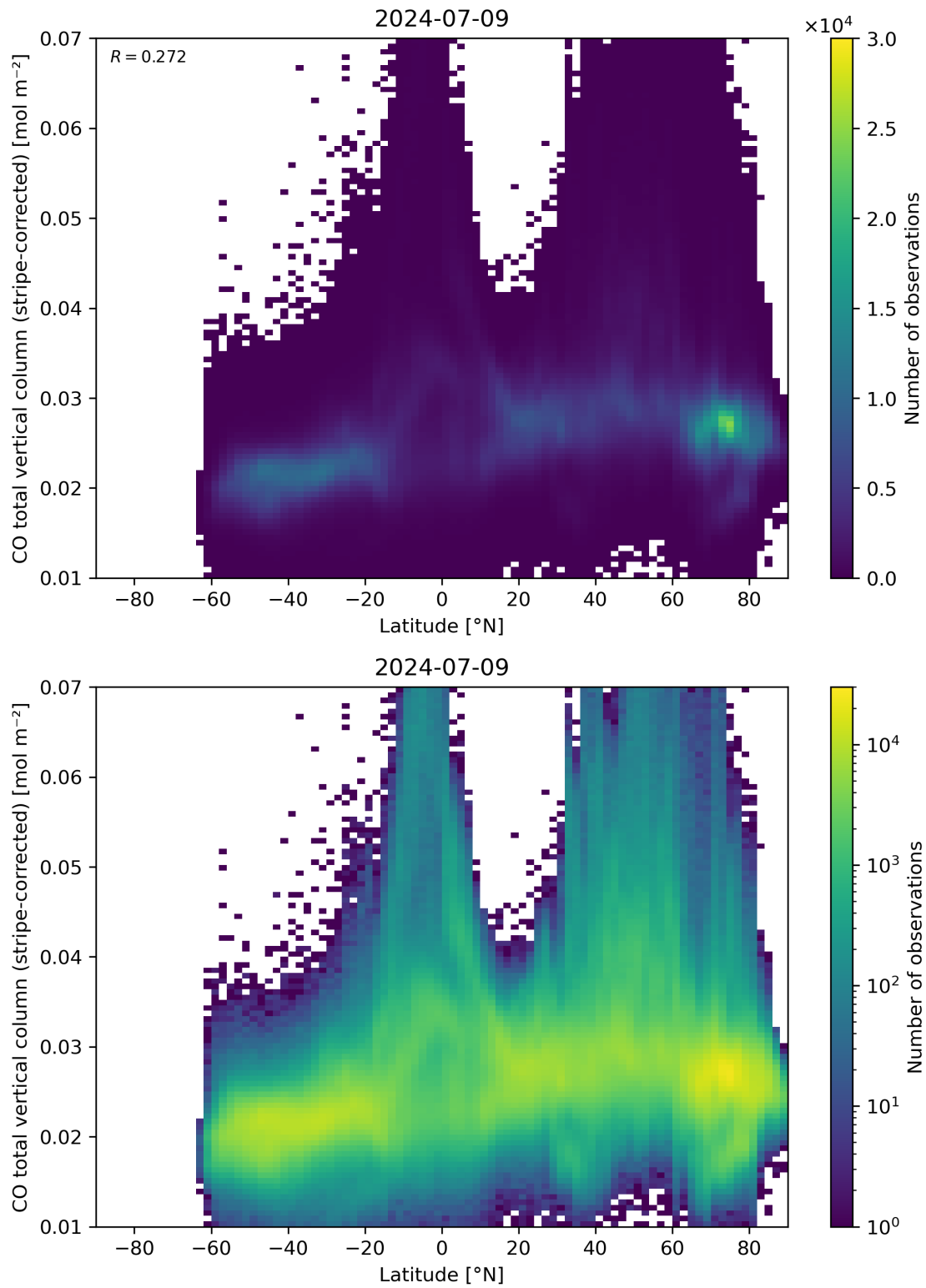
Figure 52: Scatter density plot of “Latitude” against “CO total vertical column (stripe-corrected)” for 2024-07-08 to 2024-07-10.
