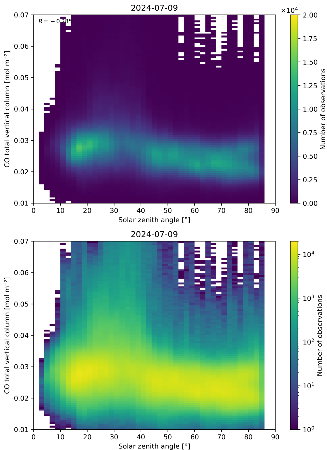
Figure 61: Scatter density plot of “Solar zenith angle” against “CO total vertical column” for 2024-07-08 to 2024-07-10.
