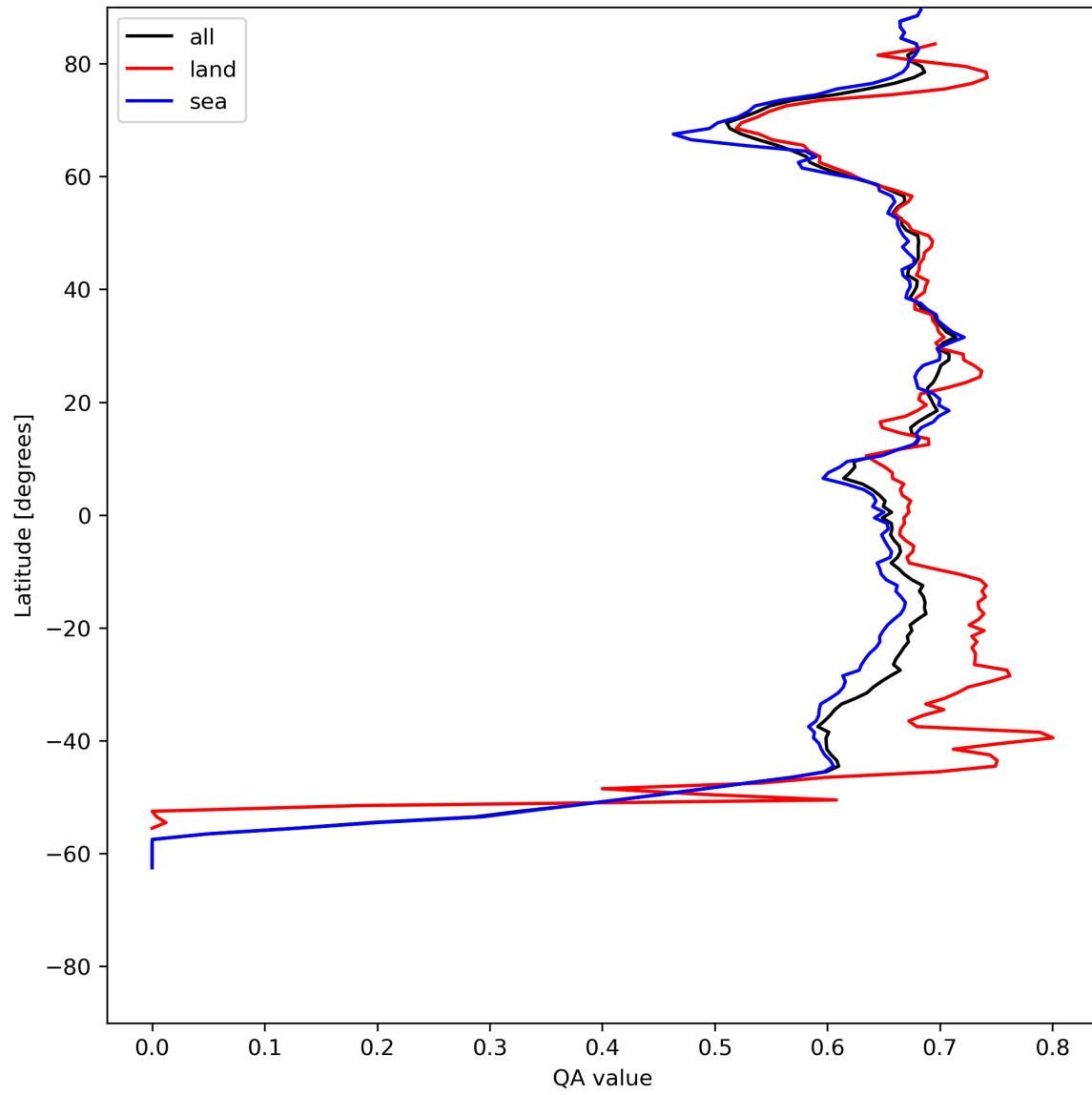
Figure 9: Zonal average of “QA value” for 2024-07-08 to 2024-07-10.
