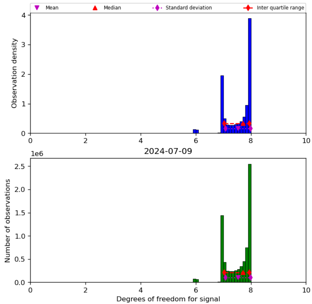
Figure 23: Histogram of “Degrees of freedom for signal” for 2024-07-08 to 2024-07-10
