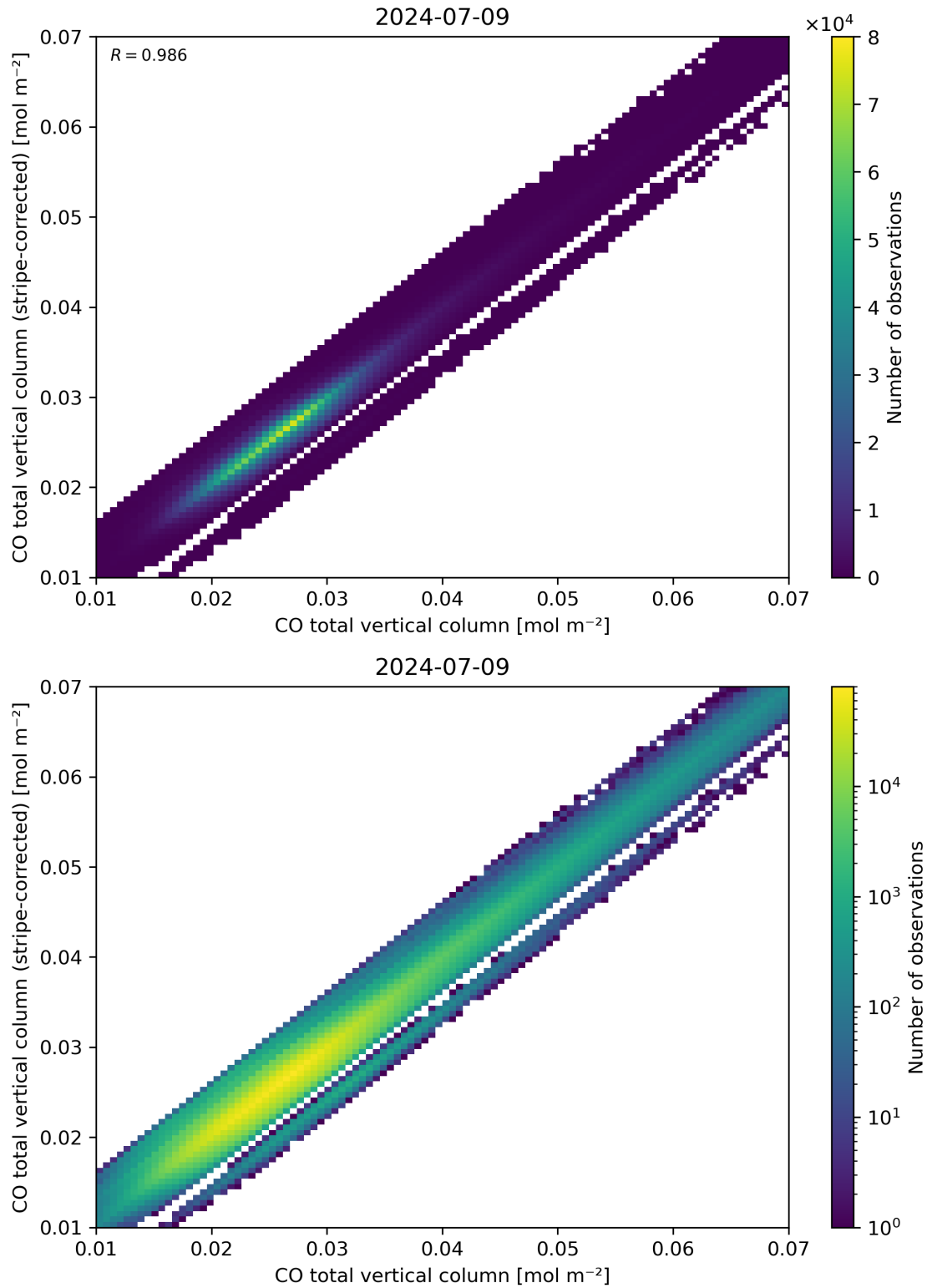
Figure 33: Scatter density plot of “CO total vertical column” against “CO total vertical column (stripe-corrected)” for 2024-07-08 to 2024-07-10.
