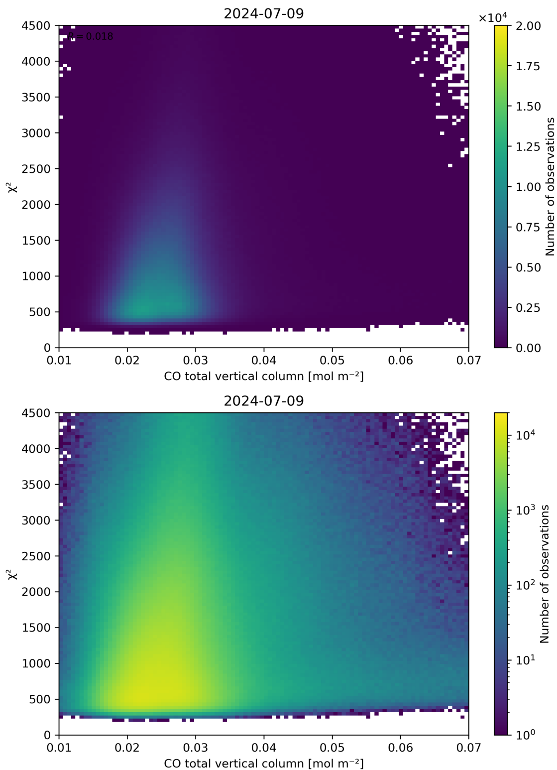
Figure 35: Scatter density plot of “CO total vertical column” against “ \chi^2 ” for 2024-07-08 to 2024-07-10.
