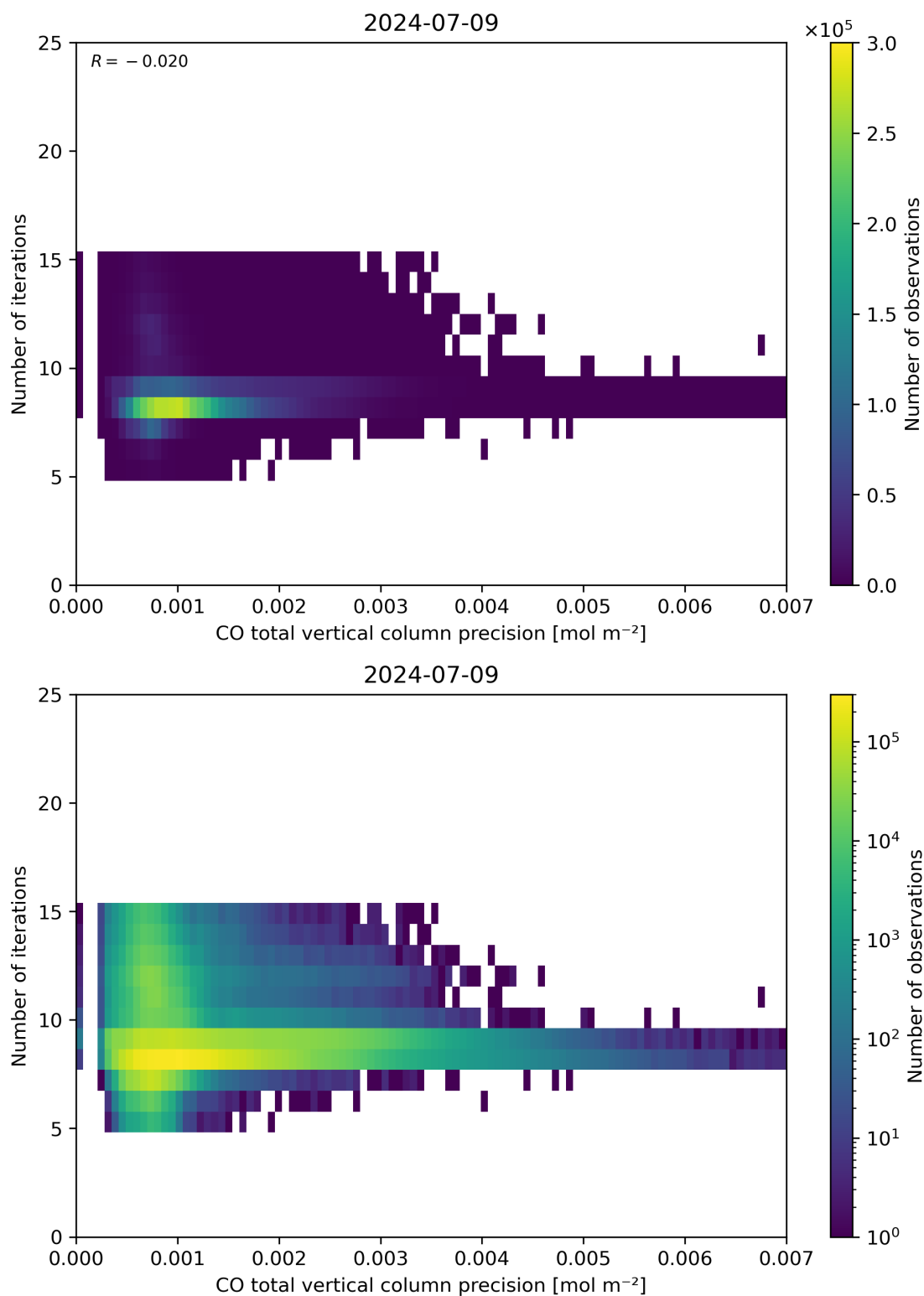
Figure 46: Scatter density plot of “CO total vertical column precision” against “Number of iterations” for 2024-07-08 to 2024-07-10.
