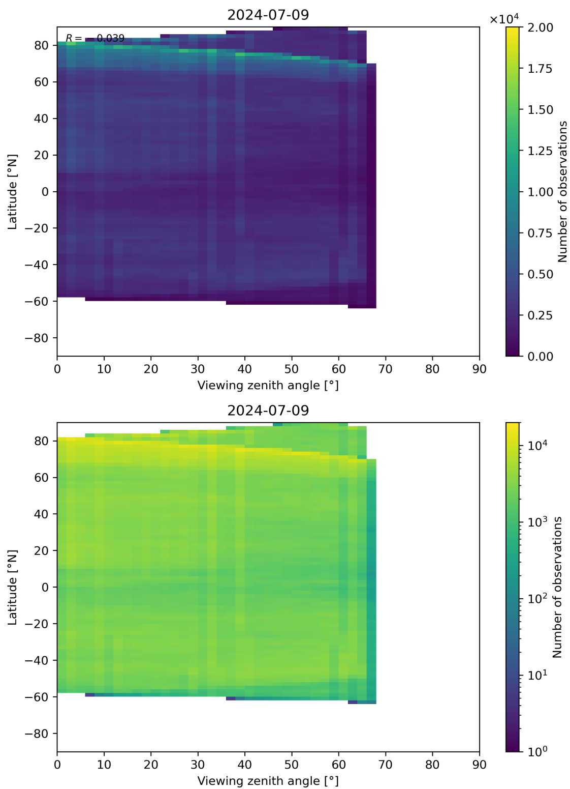
Figure 74: Scatter density plot of “Viewing zenith angle” against “Latitude” for 2024-07-08 to 2024-07-10.
