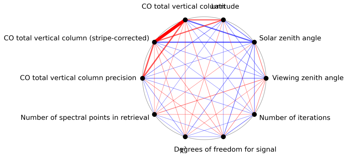
Figure 1: Map of correlation graph for 2024-07-08 to 2024-07-10.
