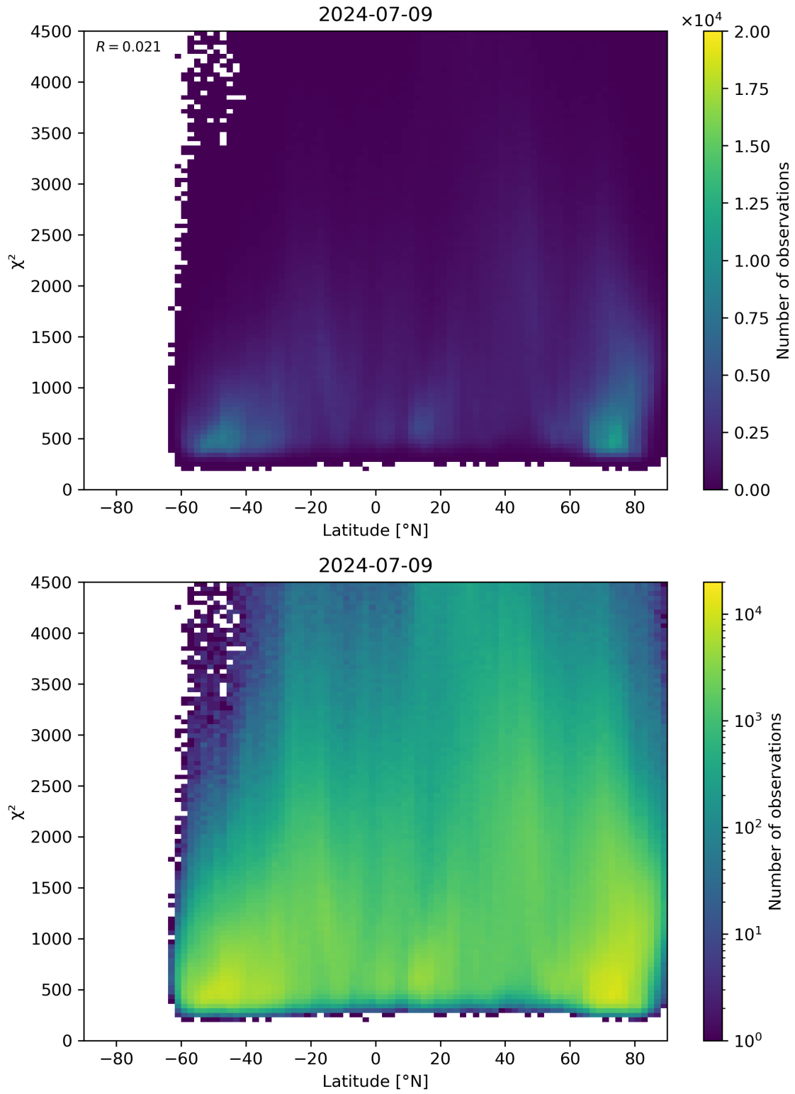
Figure 54: Scatter density plot of “Latitude” against “ \chi^2 ” for 2024-07-08 to 2024-07-10.
