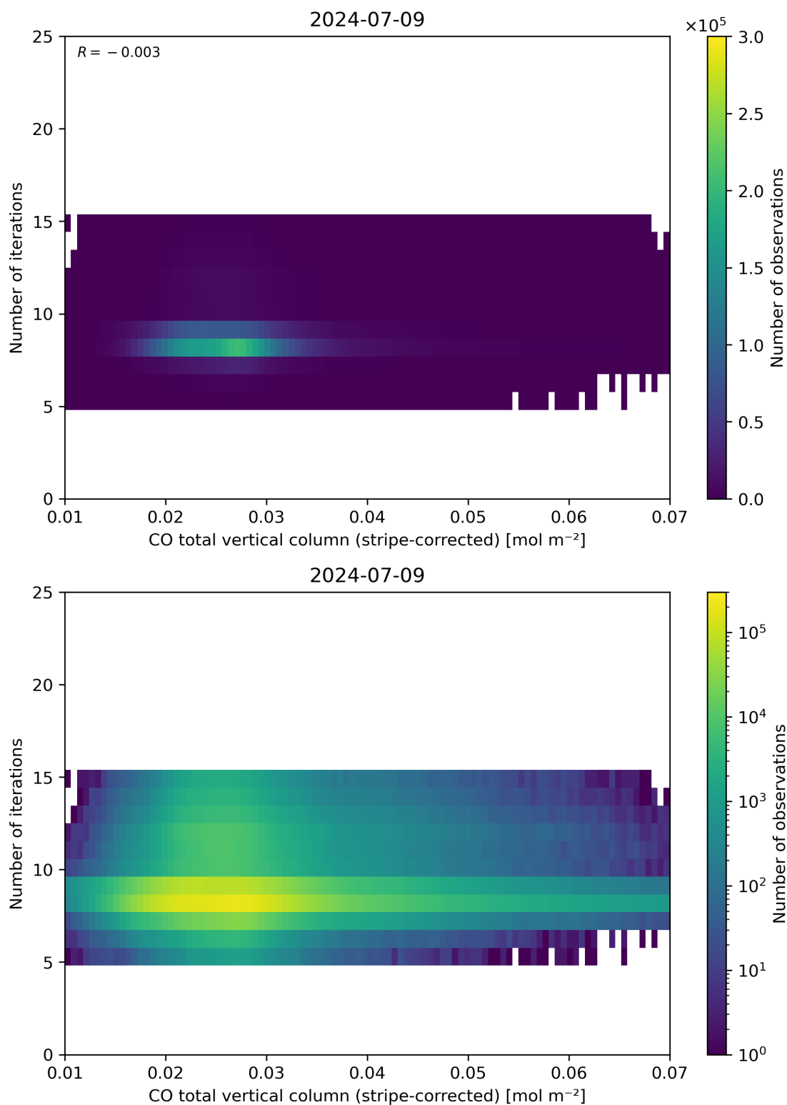
Figure 39: Scatter density plot of “CO total vertical column (stripe-corrected)” against “Number of iterations” for 2024-07-08 to 2024-07-10.
