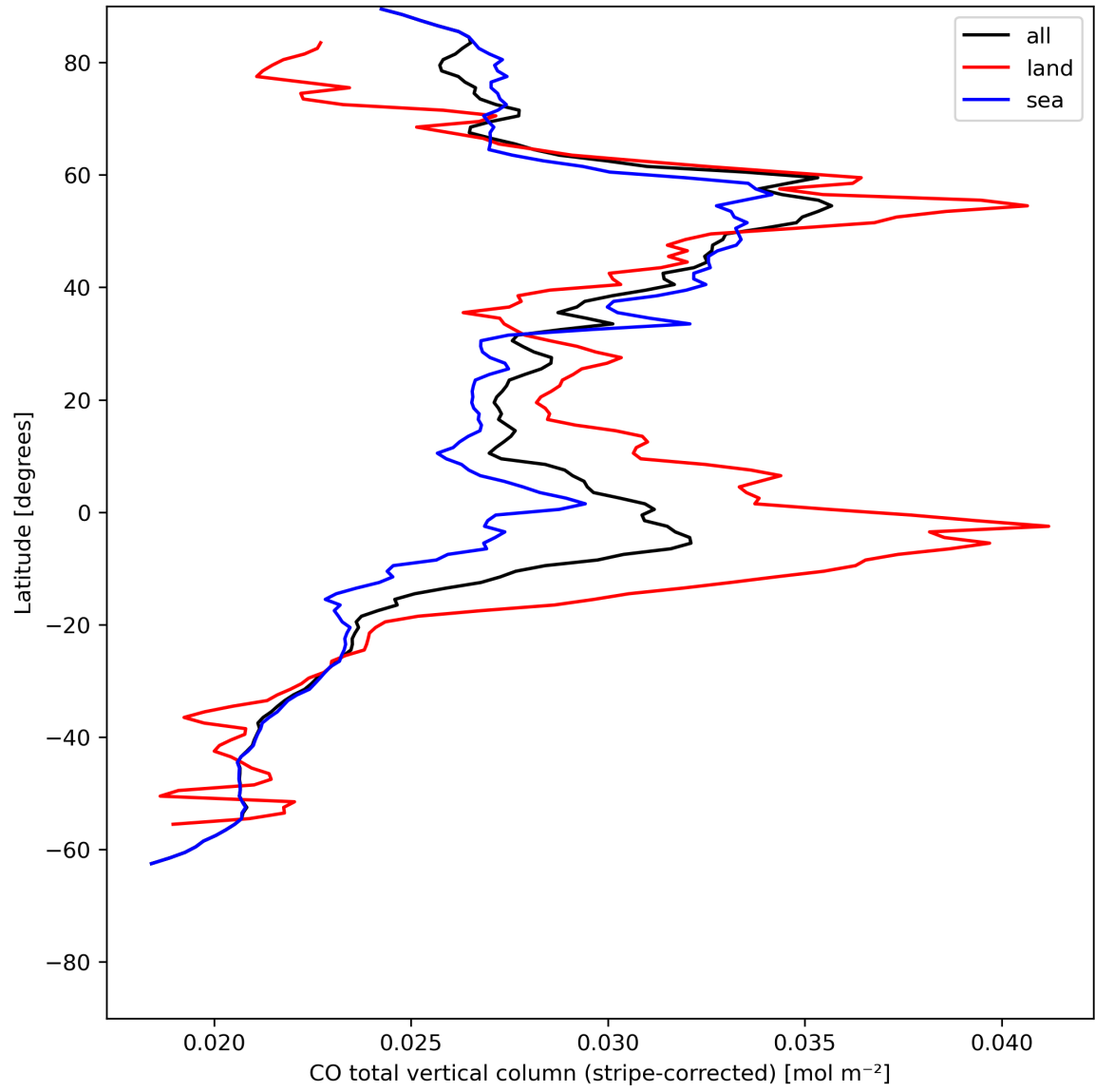
Figure 11: Zonal average of “CO total vertical column (stripe-corrected)” for 2024-07-08 to 2024-07-10.
