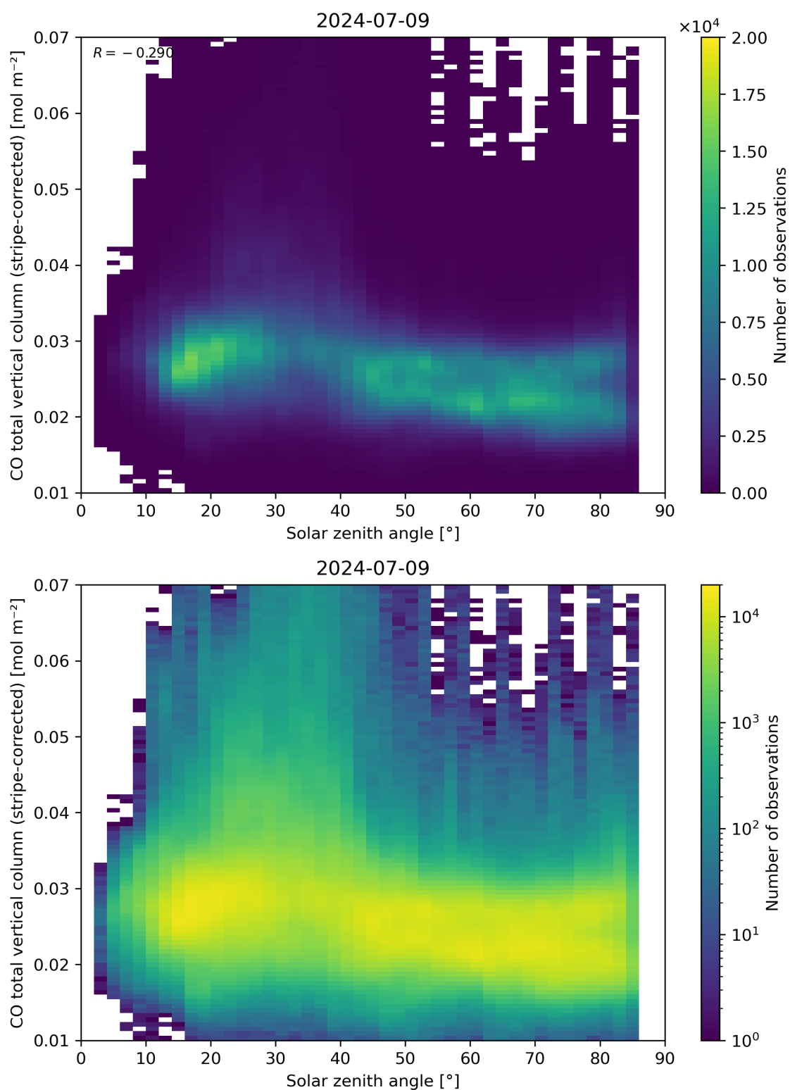
Figure 62: Scatter density plot of “Solar zenith angle” against “CO total vertical column (stripe-corrected)” for 2024-07-08 to 2024-07-10.
