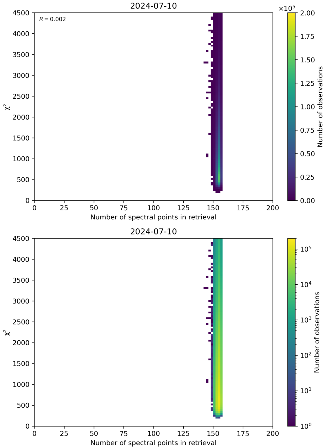
Figure 58: Scatter density plot of “Number of spectral points in retrieval” against “ \chi^2 ” for 2024-07-10 to 2024-07-11.
