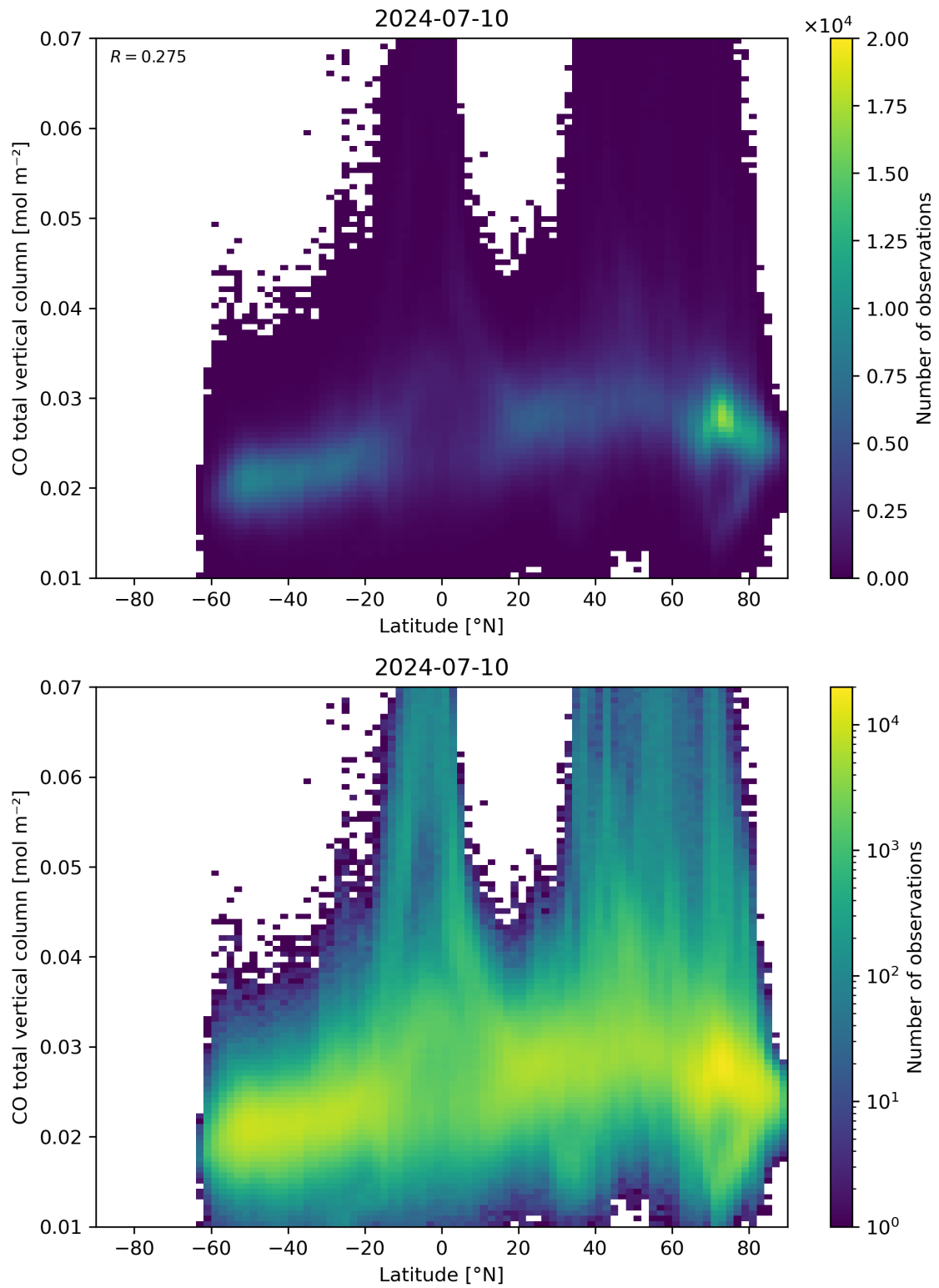
Figure 51: Scatter density plot of “Latitude” against “CO total vertical column” for 2024-07-10 to 2024-07-11.
