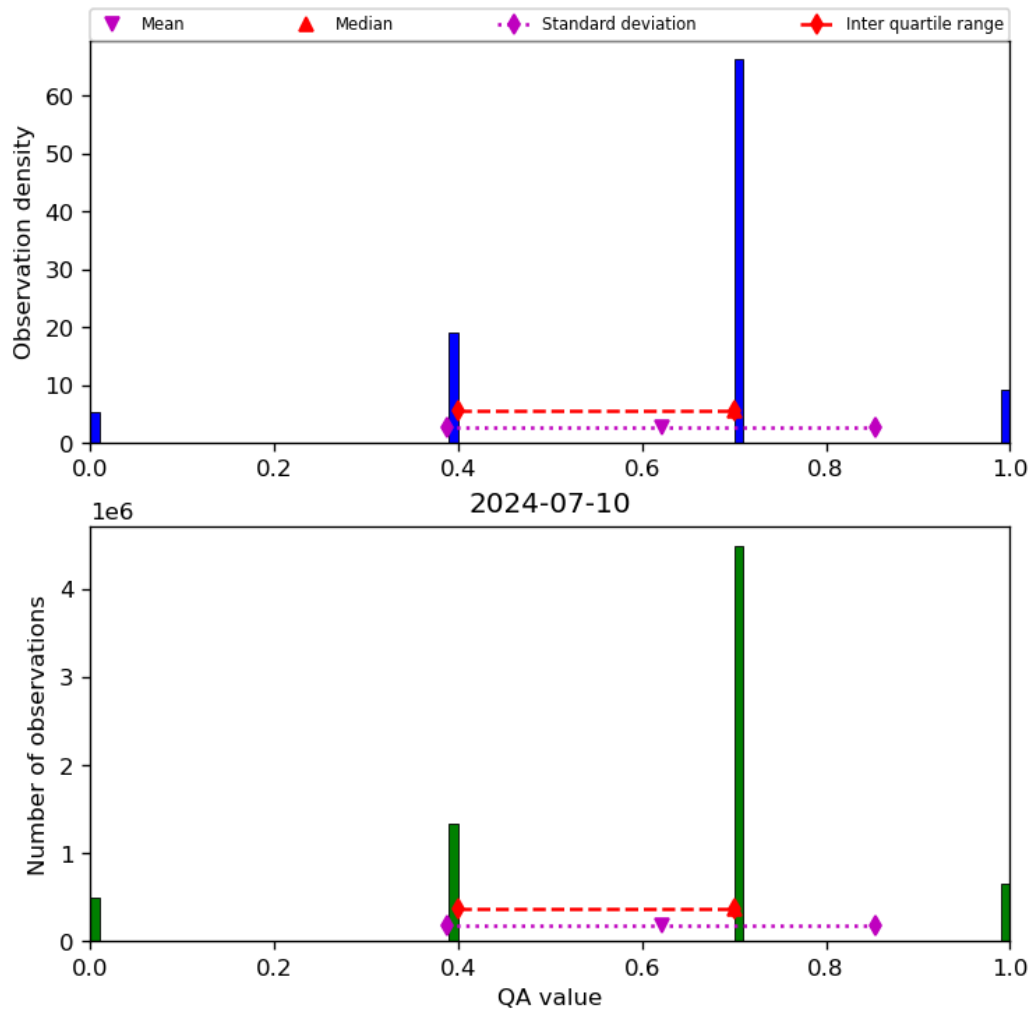
Figure 17: Histogram of “QA value” for 2024-07-10 to 2024-07-11
