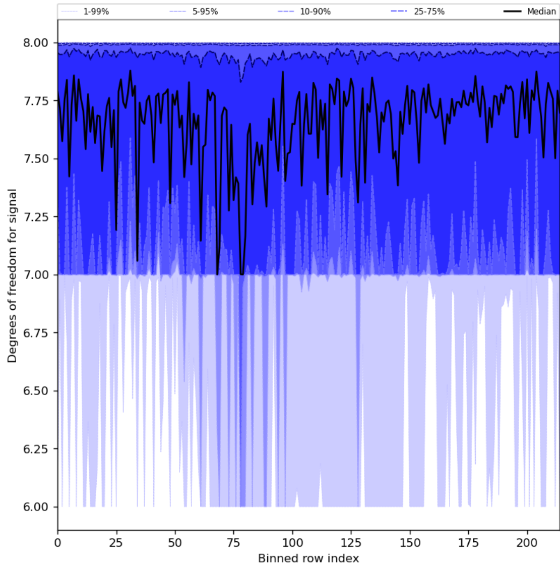
Figure 31: Along track statistics of “Degrees of freedom for signal” for 2024-07-10 to 2024-07-11
