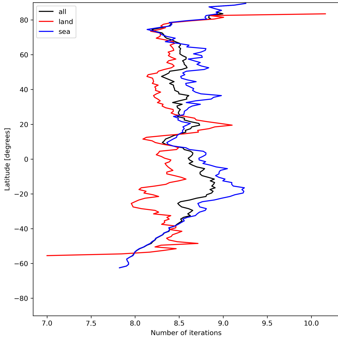
Figure 16: Zonal average of “Number of iterations” for 2024-07-10 to 2024-07-11.
