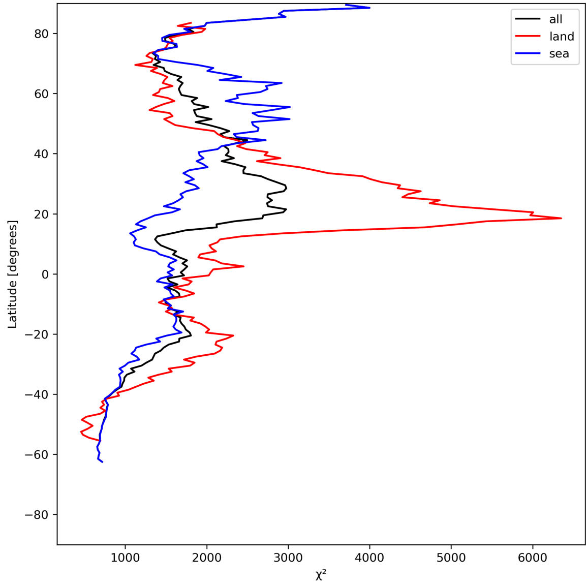
Figure 14: Zonal average of “ \chi^2 ” for 2024-07-10 to 2024-07-11.
