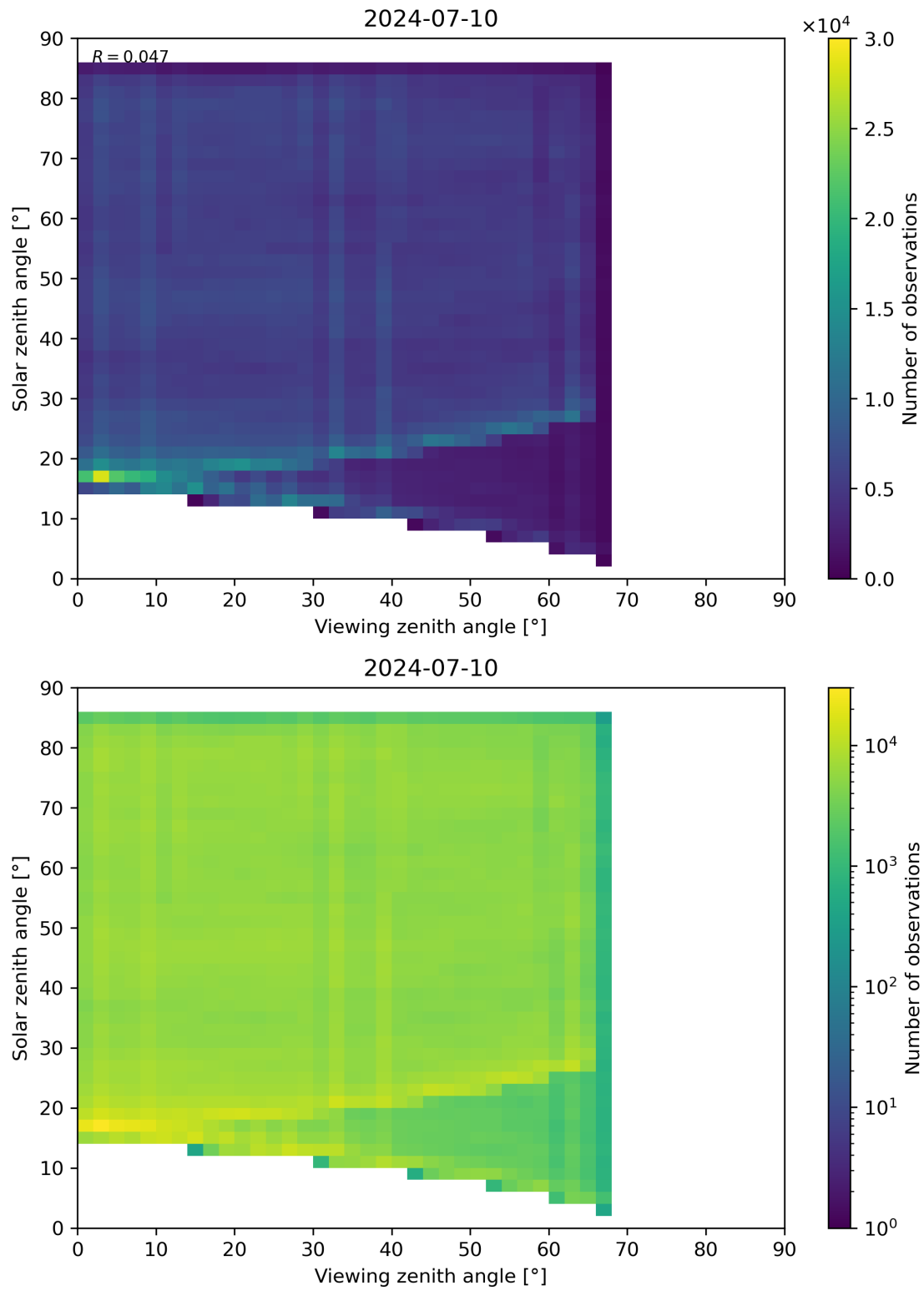
Figure 77: Scatter density plot of “Viewing zenith angle” against “Solar zenith angle” for 2024-07-10 to 2024-07-11.
