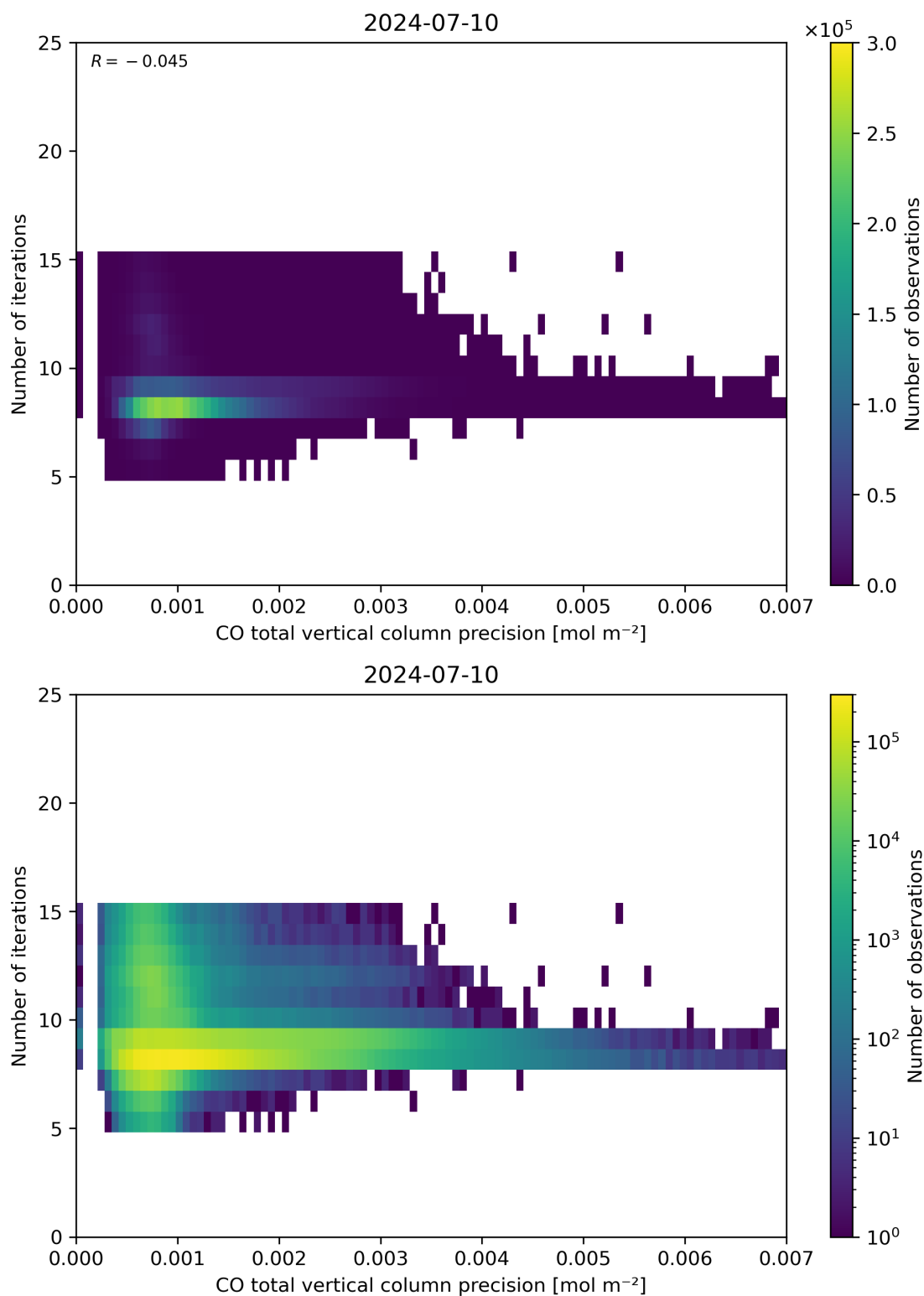
Figure 46: Scatter density plot of “CO total vertical column precision” against “Number of iterations” for 2024-07-10 to 2024-07-11.
