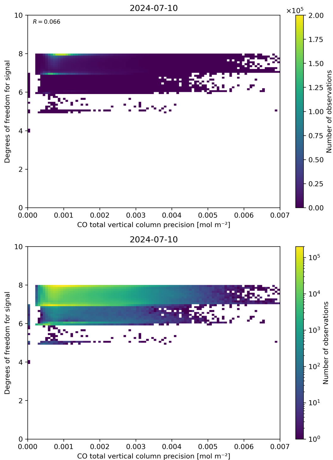
Figure 45: Scatter density plot of “CO total vertical column precision” against “Degrees of freedom for signal” for 2024-07-10 to 2024-07-11.
