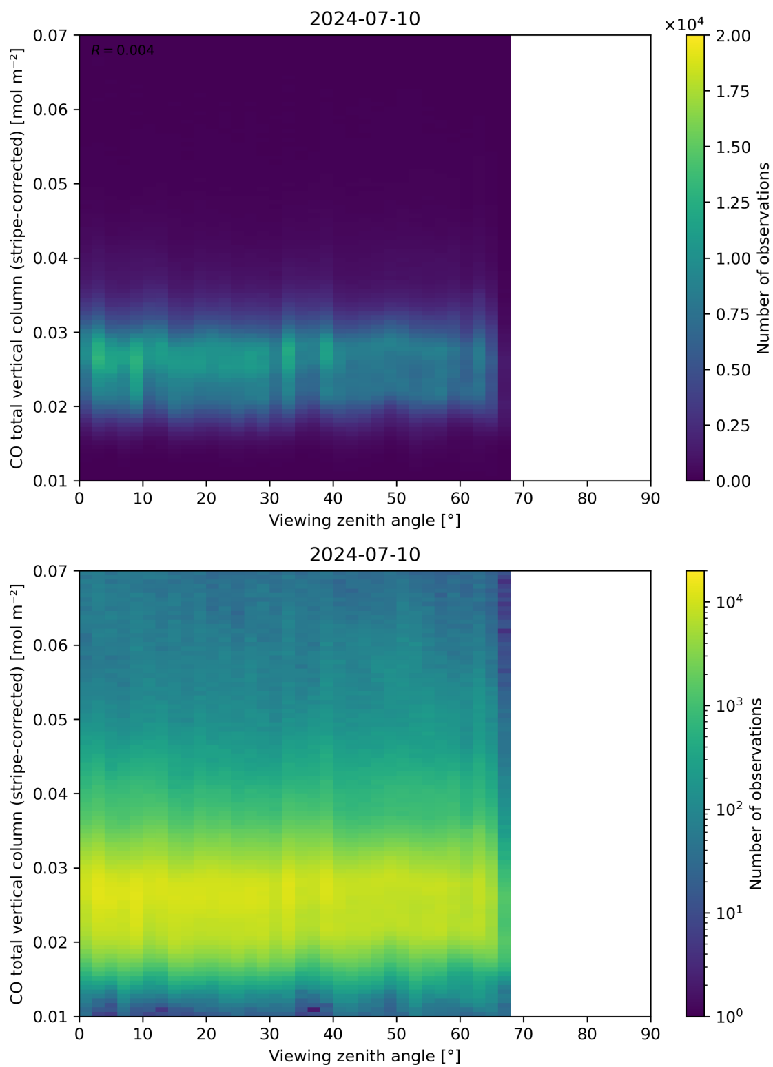
Figure 70: Scatter density plot of “Viewing zenith angle” against “CO total vertical column (stripe-corrected)” for 2024-07-10 to 2024-07-11.
