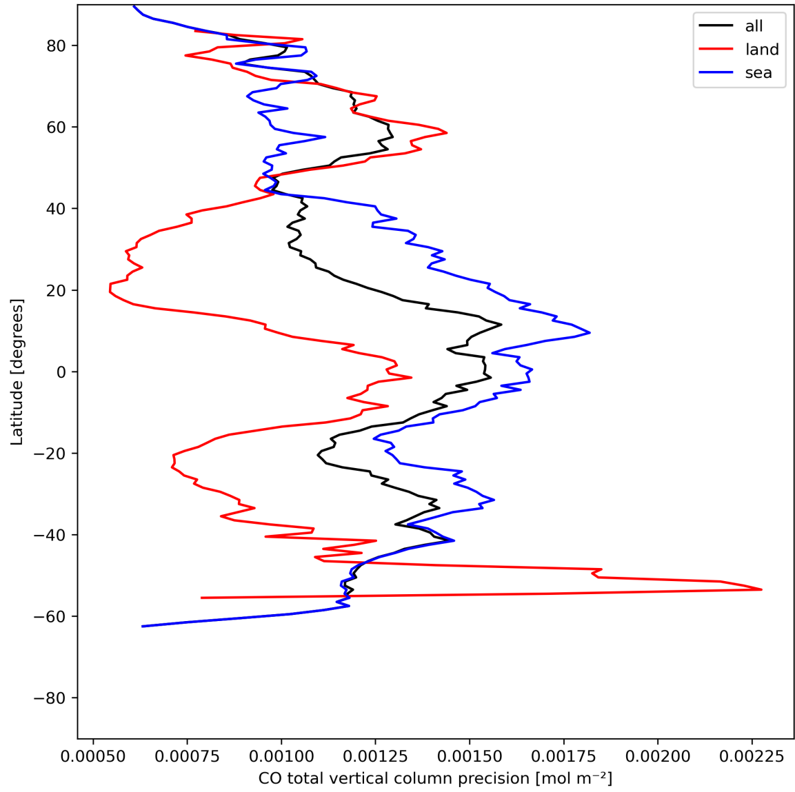
Figure 12: Zonal average of “CO total vertical column precision” for 2024-07-10 to 2024-07-11.
