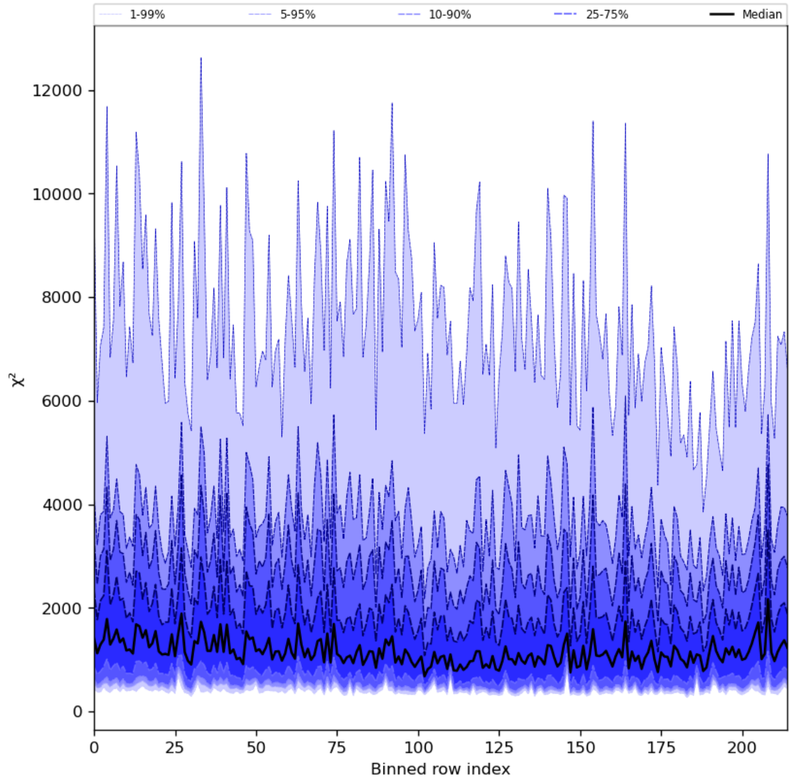
Figure 30: Along track statistics of “ \chi^2 ” for 2024-07-10 to 2024-07-11
