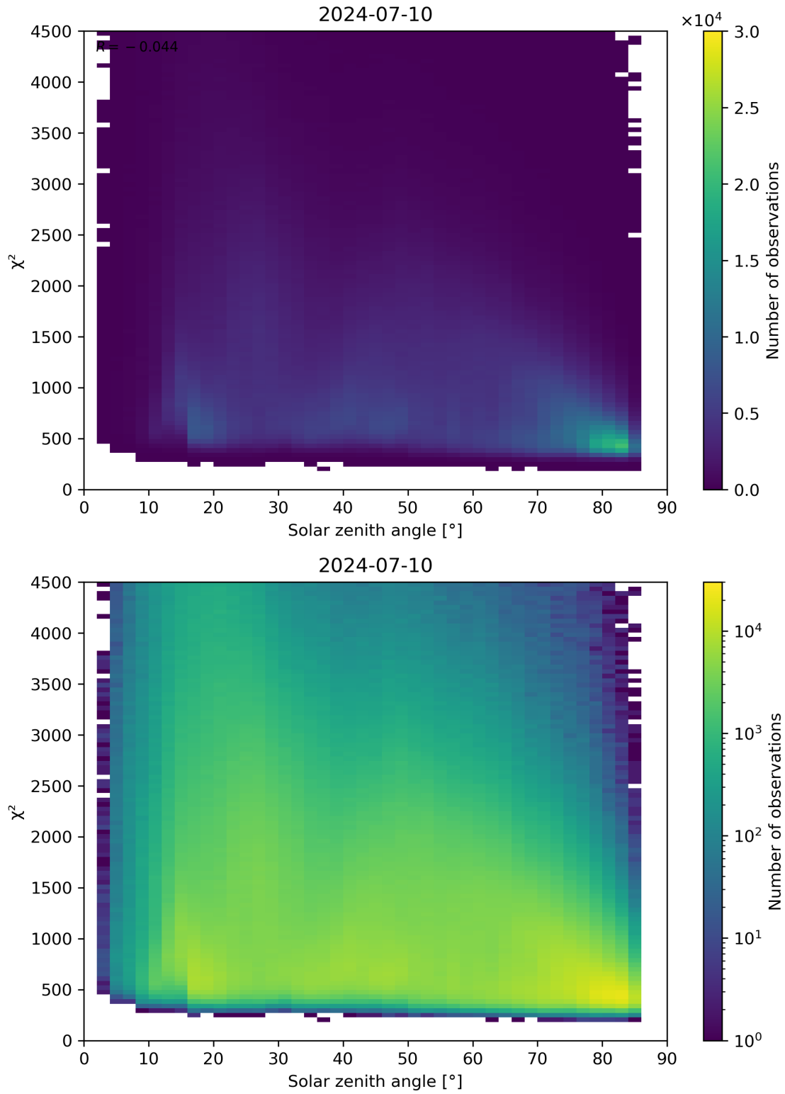
Figure 64: Scatter density plot of “Solar zenith angle” against “ \chi^2 ” for 2024-07-10 to 2024-07-11.
