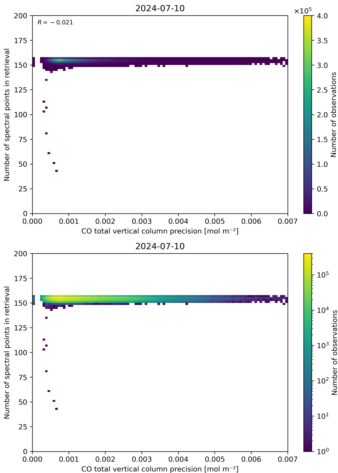
Figure 47: Scatter density plot of “CO total vertical column precision” against “Number of spectral points in retrieval” for 2024-07-10 to 2024-07-11.
