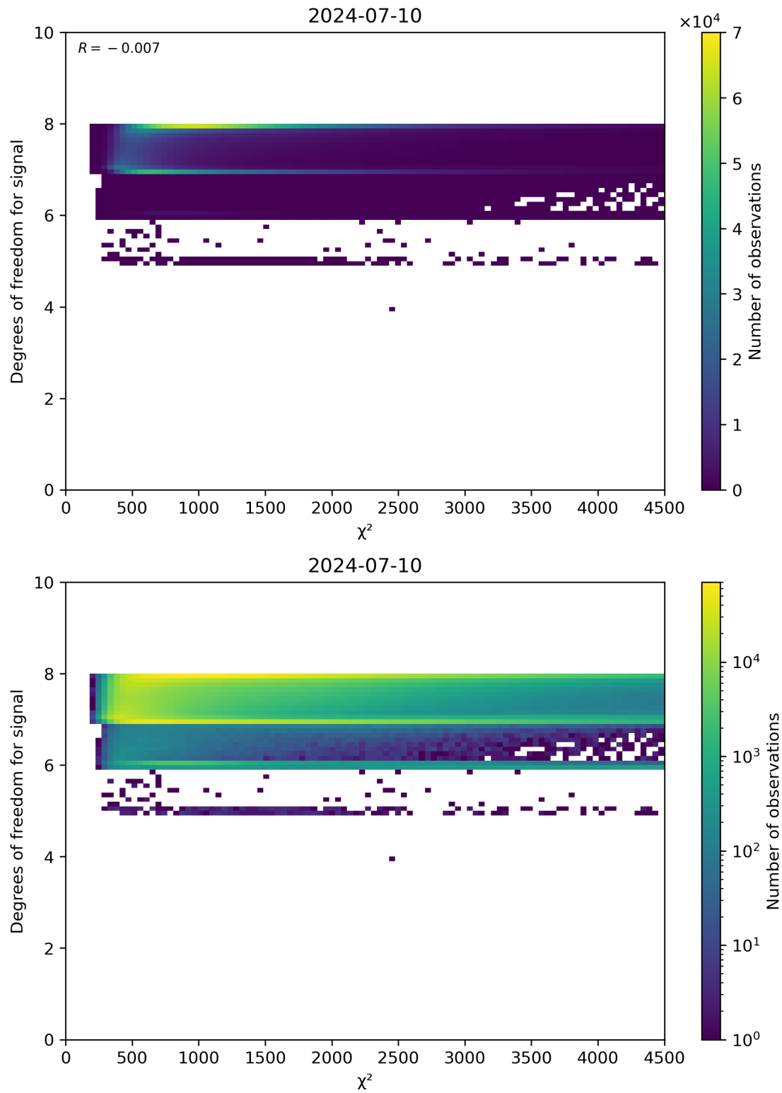
Figure 48: Scatter density plot of “ \chi^2 ” against “Degrees of freedom for signal” for 2024-07-10 to 2024-07-11.
