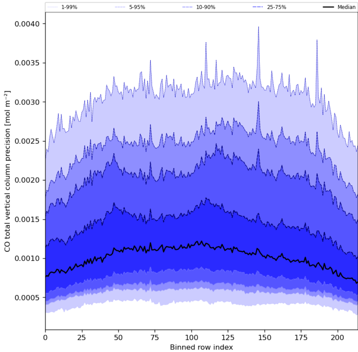
Figure 28: Along track statistics of “CO total vertical column precision” for 2024-07-10 to 2024-07-11
