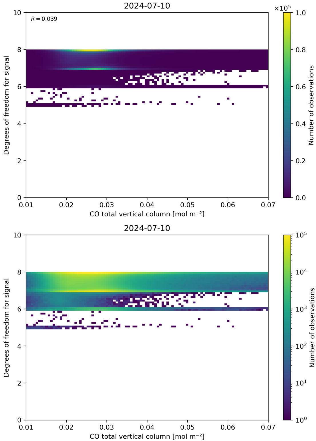
Figure 41: Scatter density plot of “CO total vertical column” against “Degrees of freedom for signal” for 2024-07-10 to 2024-07-11.
