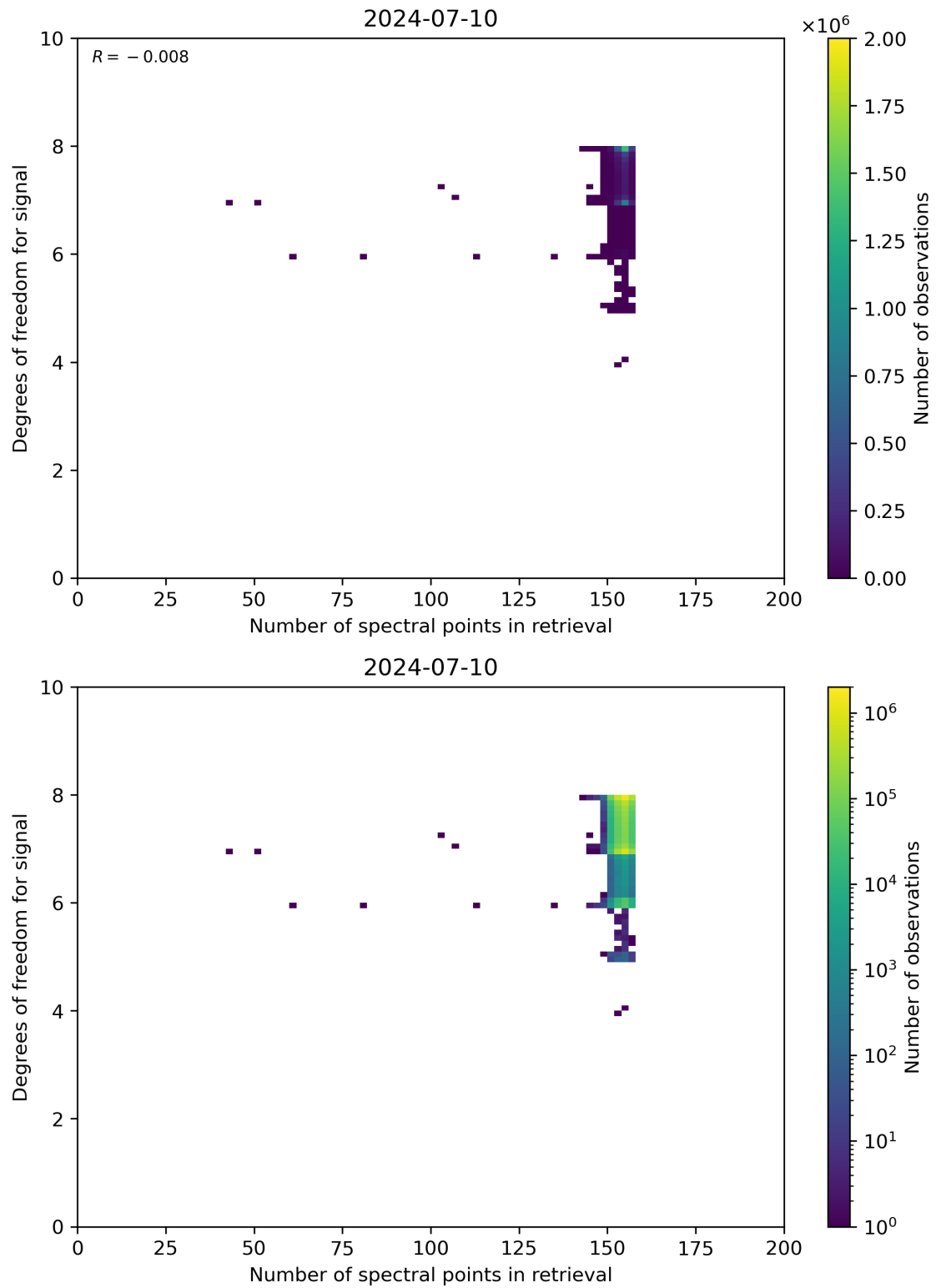
Figure 59: Scatter density plot of “Number of spectral points in retrieval” against “Degrees of freedom for signal” for 2024-07-10 to 2024-07-11.
