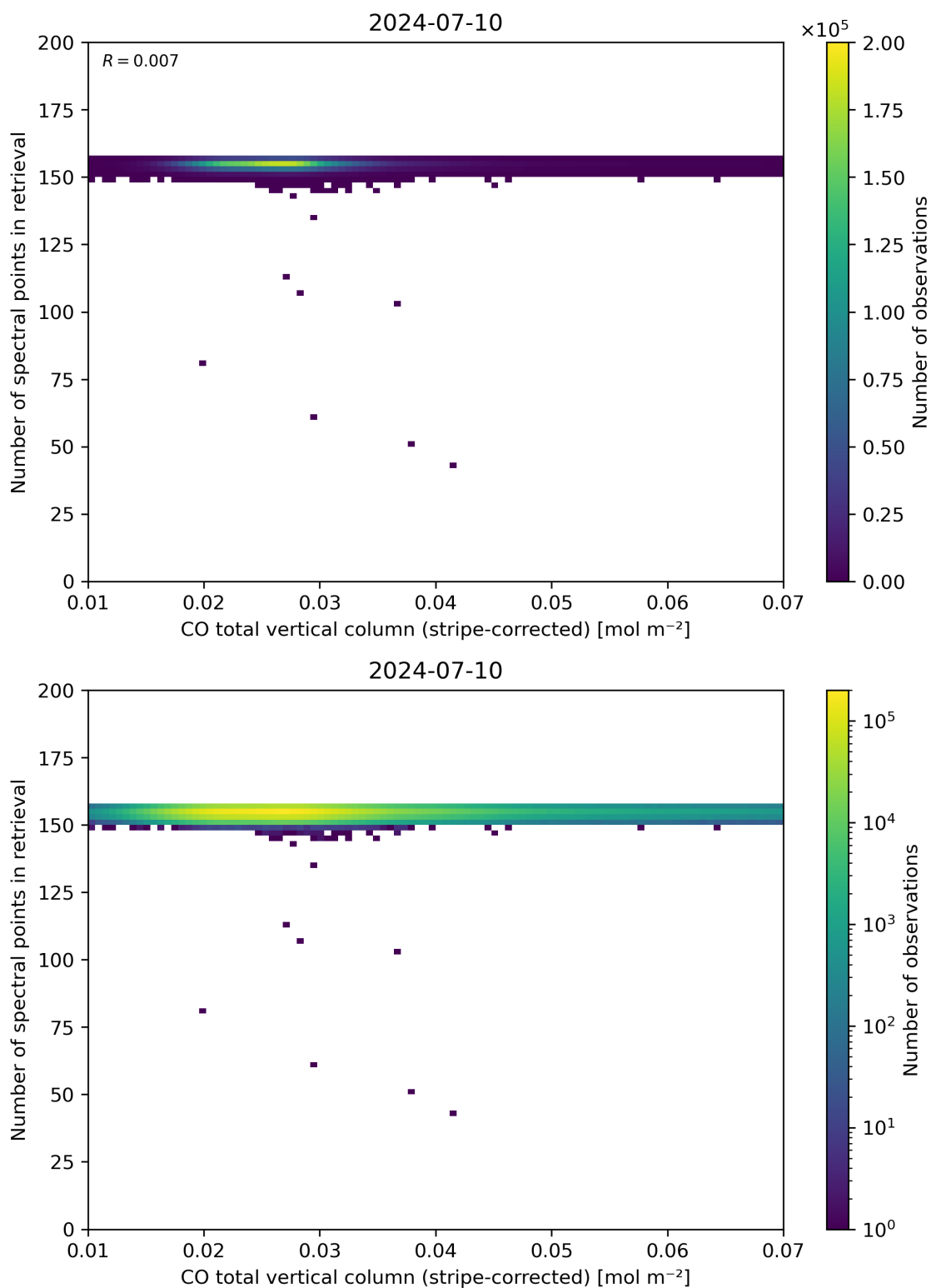
Figure 40: Scatter density plot of “CO total vertical column (stripe-corrected)” against “Number of spectral points in retrieval” for 2024-07-10 to 2024-07-11.
