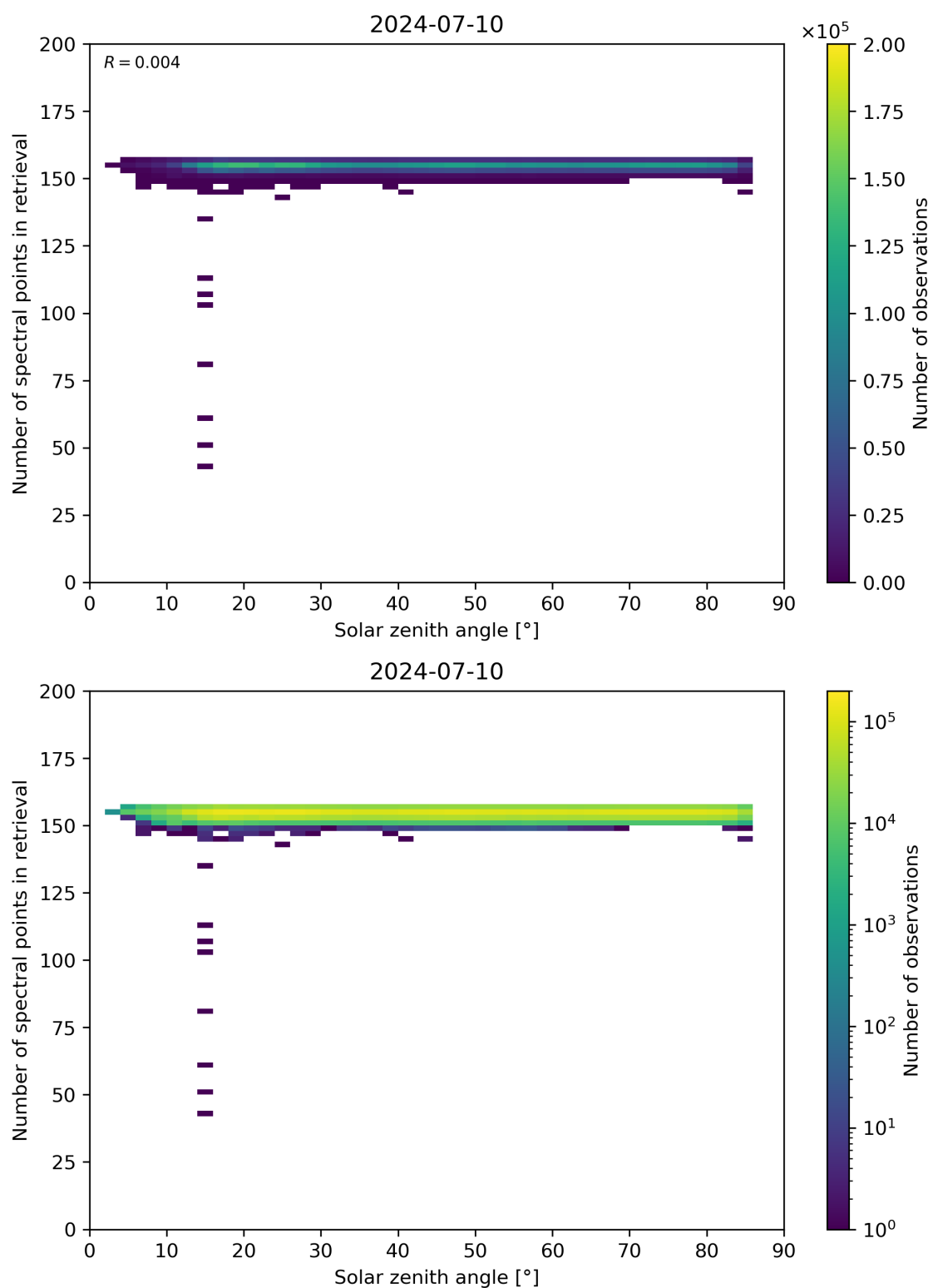
Figure 68: Scatter density plot of “Solar zenith angle” against “Number of spectral points in retrieval” for 2024-07-10 to 2024-07-11.
