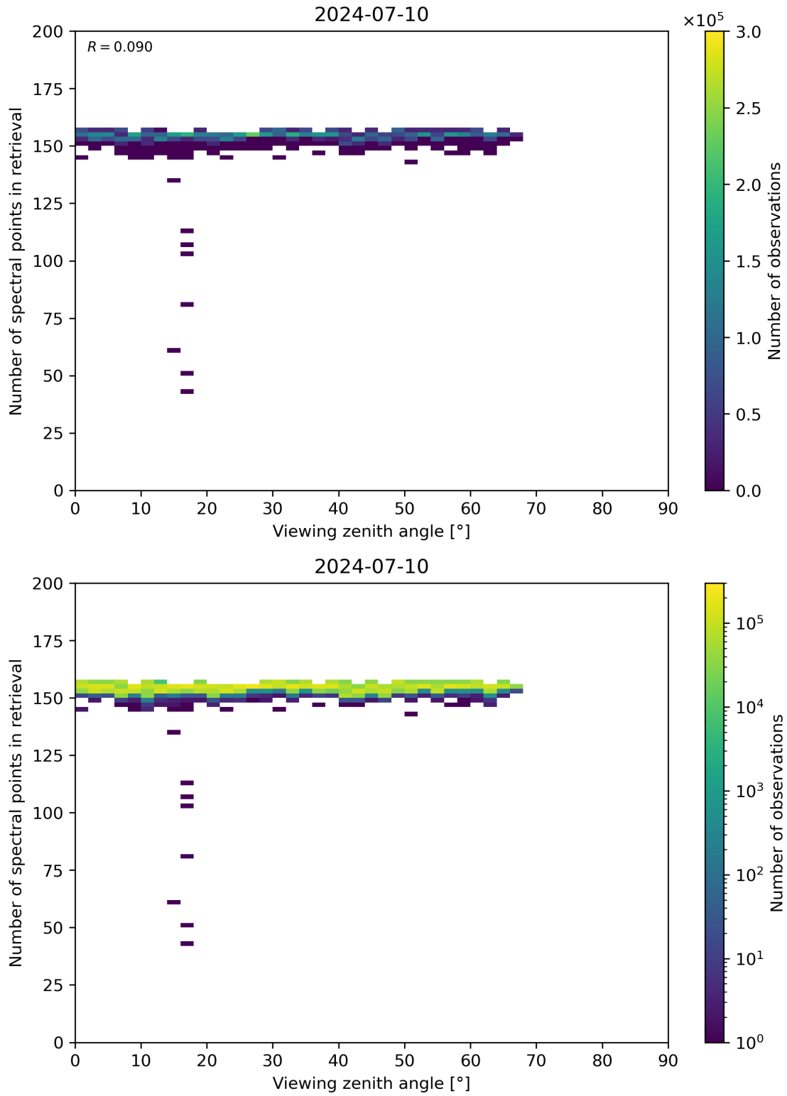
Figure 76: Scatter density plot of “Viewing zenith angle” against “Number of spectral points in retrieval” for 2024-07-10 to 2024-07-11.
