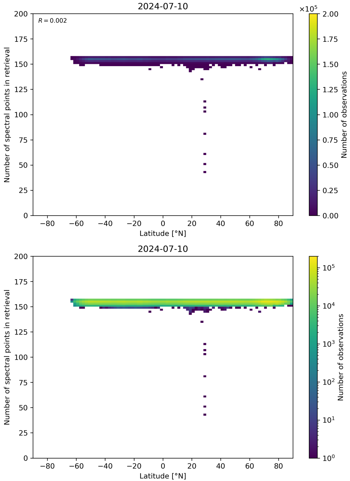
Figure 57: Scatter density plot of “Latitude” against “Number of spectral points in retrieval” for 2024-07-10 to 2024-07-11.
