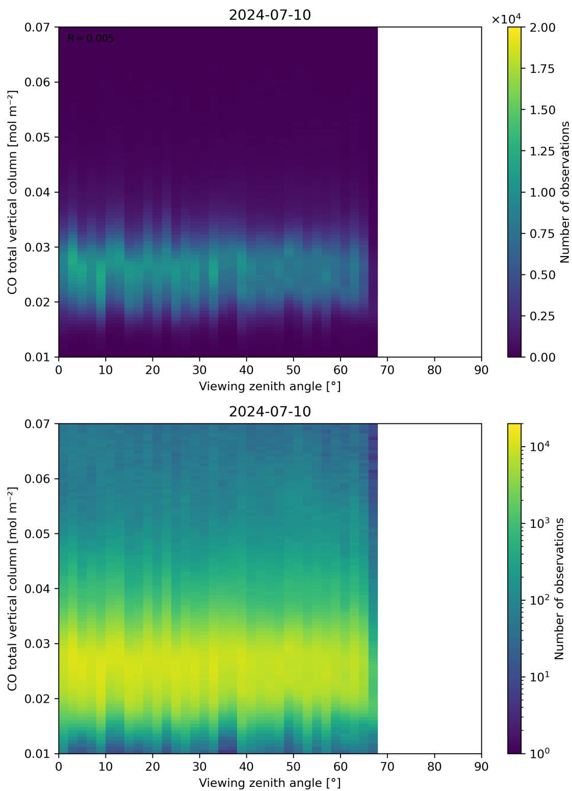
Figure 69: Scatter density plot of “Viewing zenith angle” against “CO total vertical column” for 2024-07-10 to 2024-07-11.
