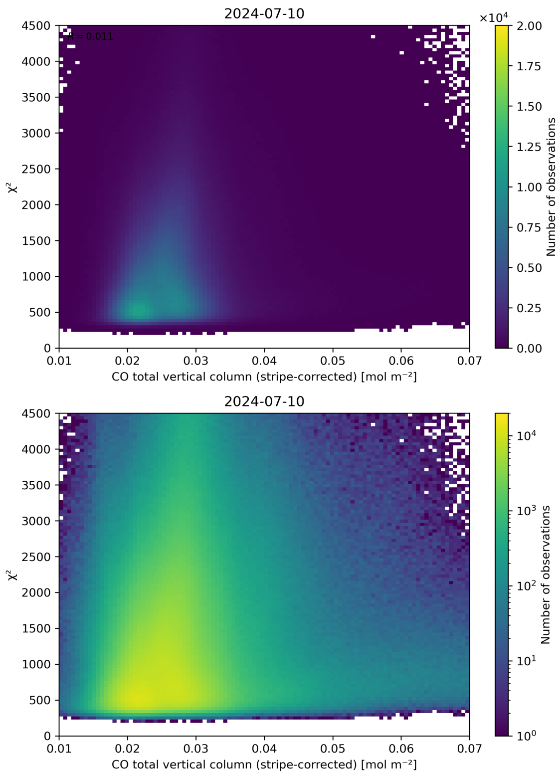
Figure 37: Scatter density plot of “CO total vertical column (stripe-corrected)” against “ \chi^2 ” for 2024-07-10 to 2024-07-11.
