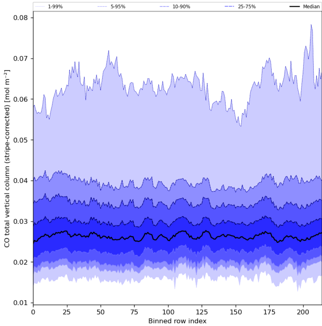
Figure 27: Along track statistics of “CO total vertical column (stripe-corrected)” for 2024-07-10 to 2024-07-11
