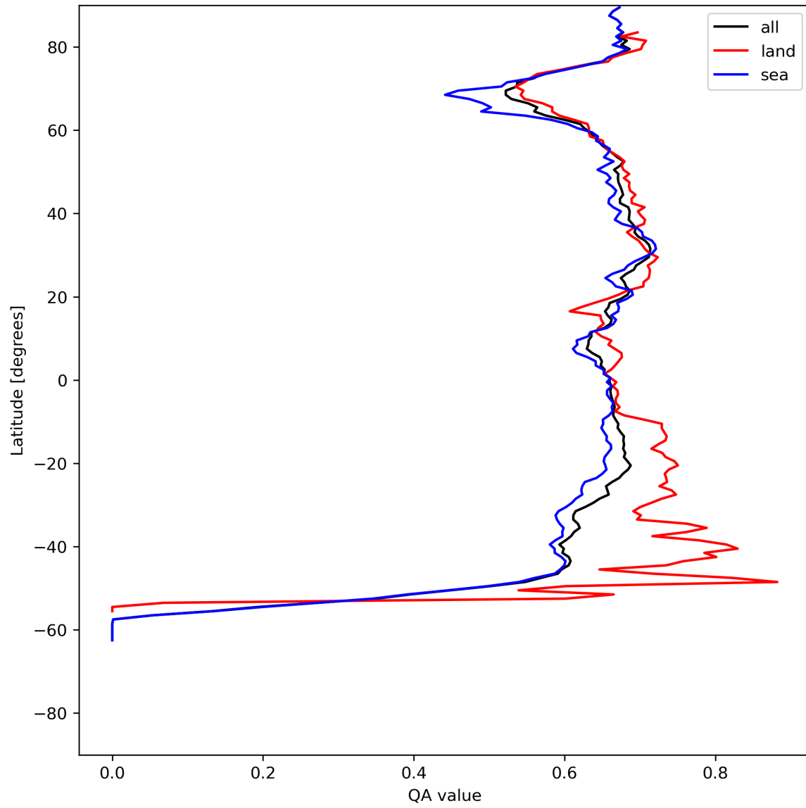
Figure 9: Zonal average of “QA value” for 2024-07-10 to 2024-07-11.
