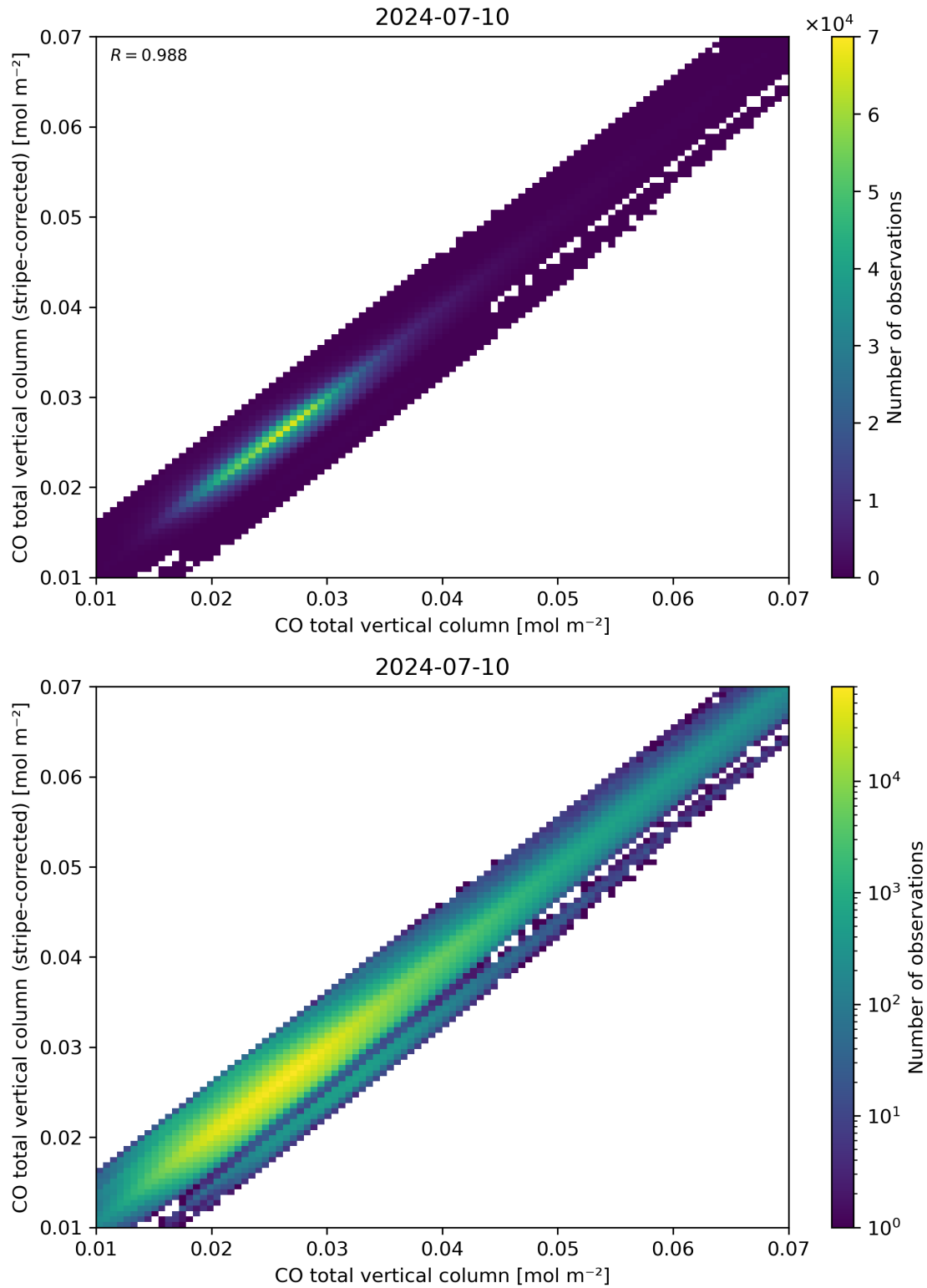
Figure 33: Scatter density plot of “CO total vertical column” against “CO total vertical column (stripe-corrected)” for 2024-07-10 to 2024-07-11.
