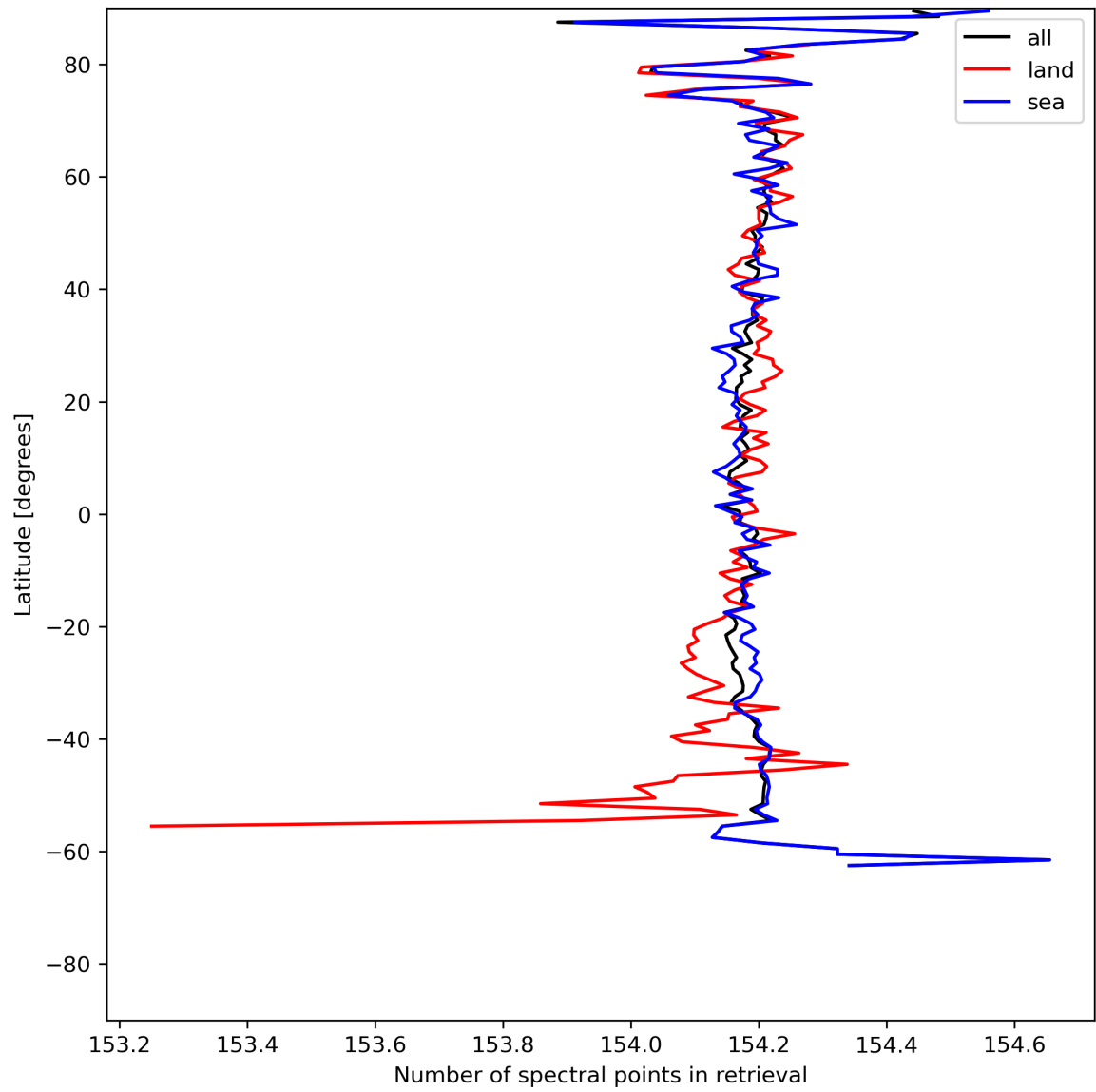
Figure 13: Zonal average of “Number of spectral points in retrieval” for 2024-07-10 to 2024-07-11.
