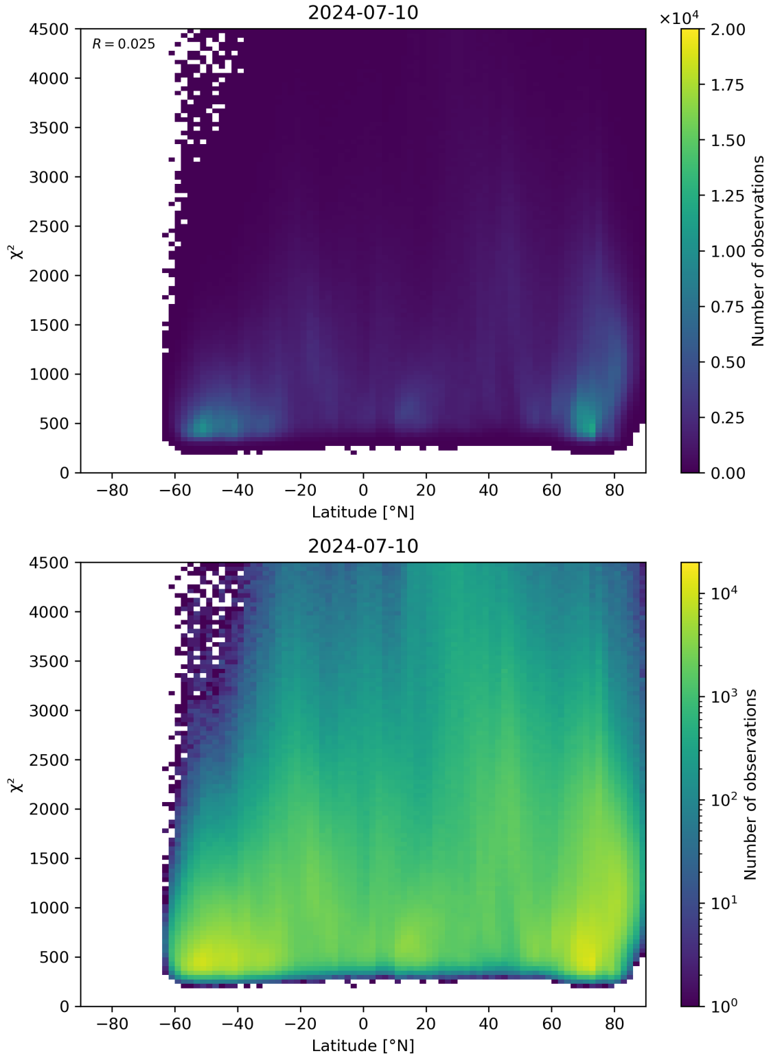
Figure 54: Scatter density plot of “Latitude” against “ \chi^2 ” for 2024-07-10 to 2024-07-11.
