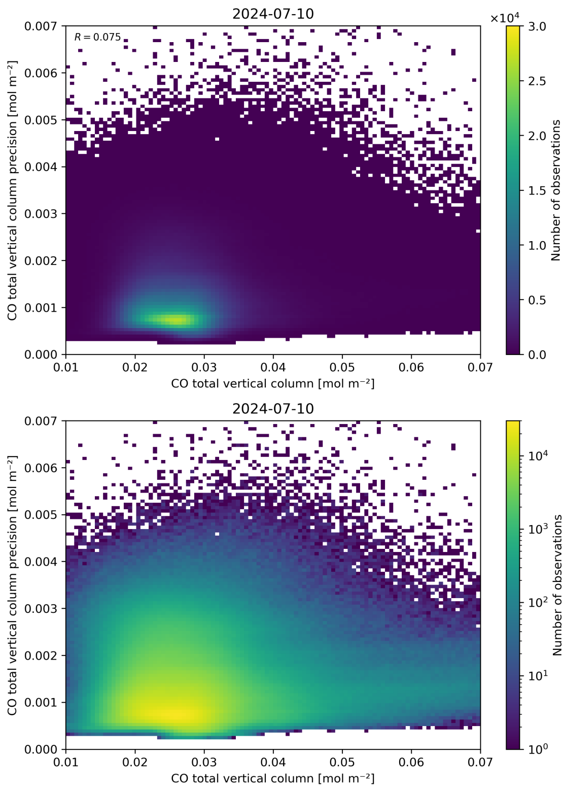
Figure 34: Scatter density plot of “CO total vertical column” against “CO total vertical column precision” for 2024-07-10 to 2024-07-11.
