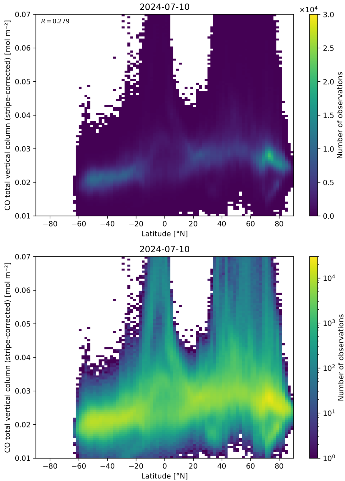
Figure 52: Scatter density plot of “Latitude” against “CO total vertical column (stripe-corrected)” for 2024-07-10 to 2024-07-11.
