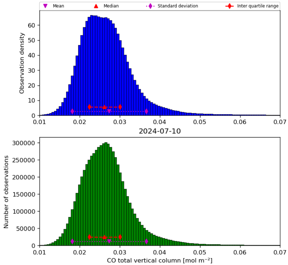
Figure 18: Histogram of “CO total vertical column” for 2024-07-10 to 2024-07-11
