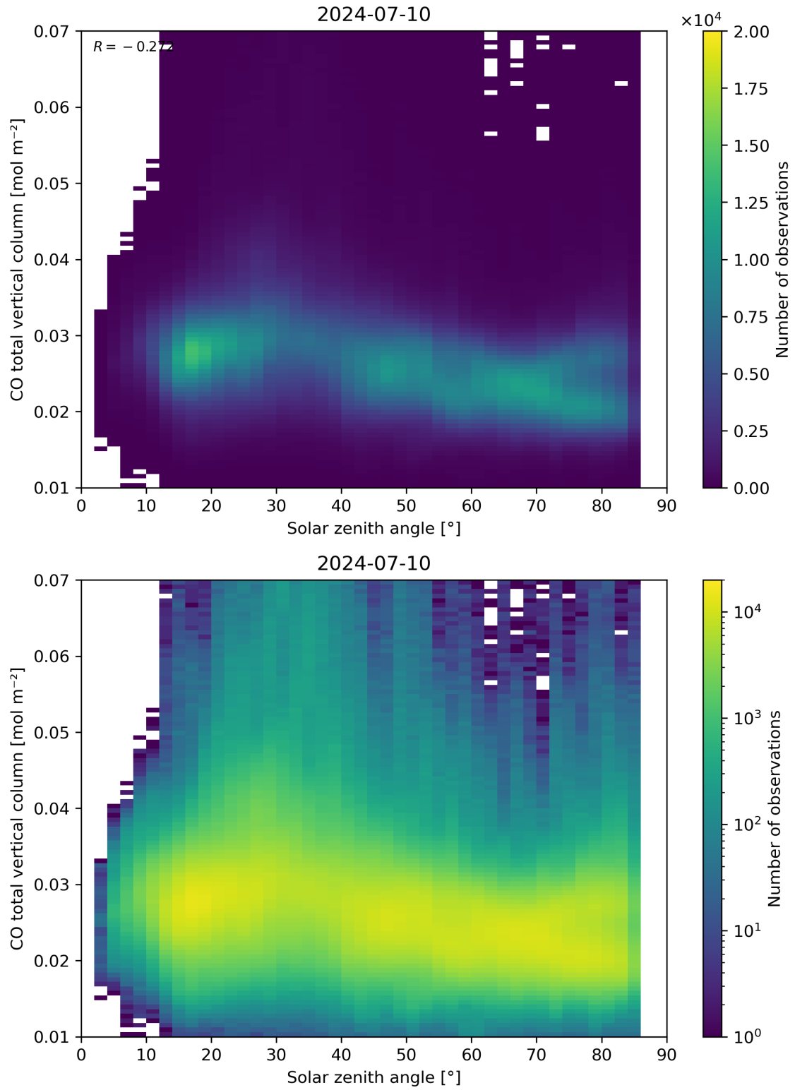
Figure 61: Scatter density plot of “Solar zenith angle” against “CO total vertical column” for 2024-07-10 to 2024-07-11.
