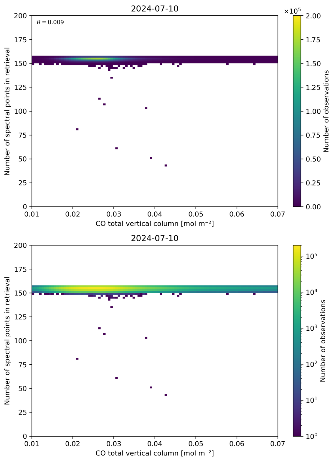
Figure 43: Scatter density plot of “CO total vertical column” against “Number of spectral points in retrieval” for 2024-07-10 to 2024-07-11.
