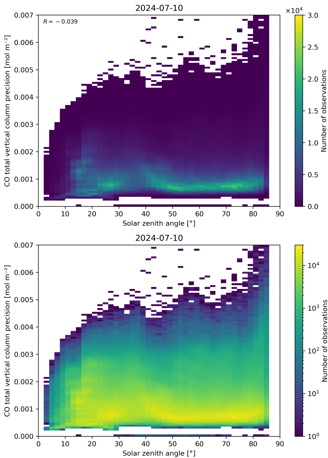
Figure 63: Scatter density plot of “Solar zenith angle” against “CO total vertical column precision” for 2024-07-10 to 2024-07-11.
