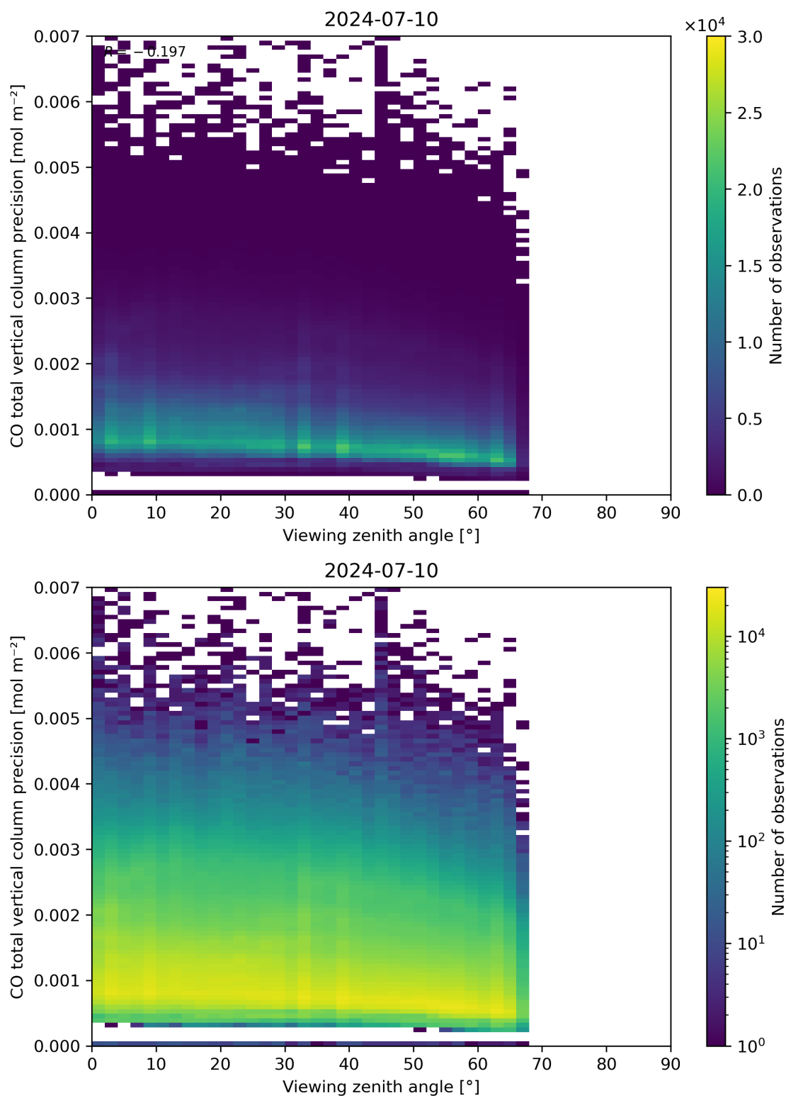
Figure 71: Scatter density plot of “Viewing zenith angle” against “CO total vertical column precision” for 2024-07-10 to 2024-07-11.
