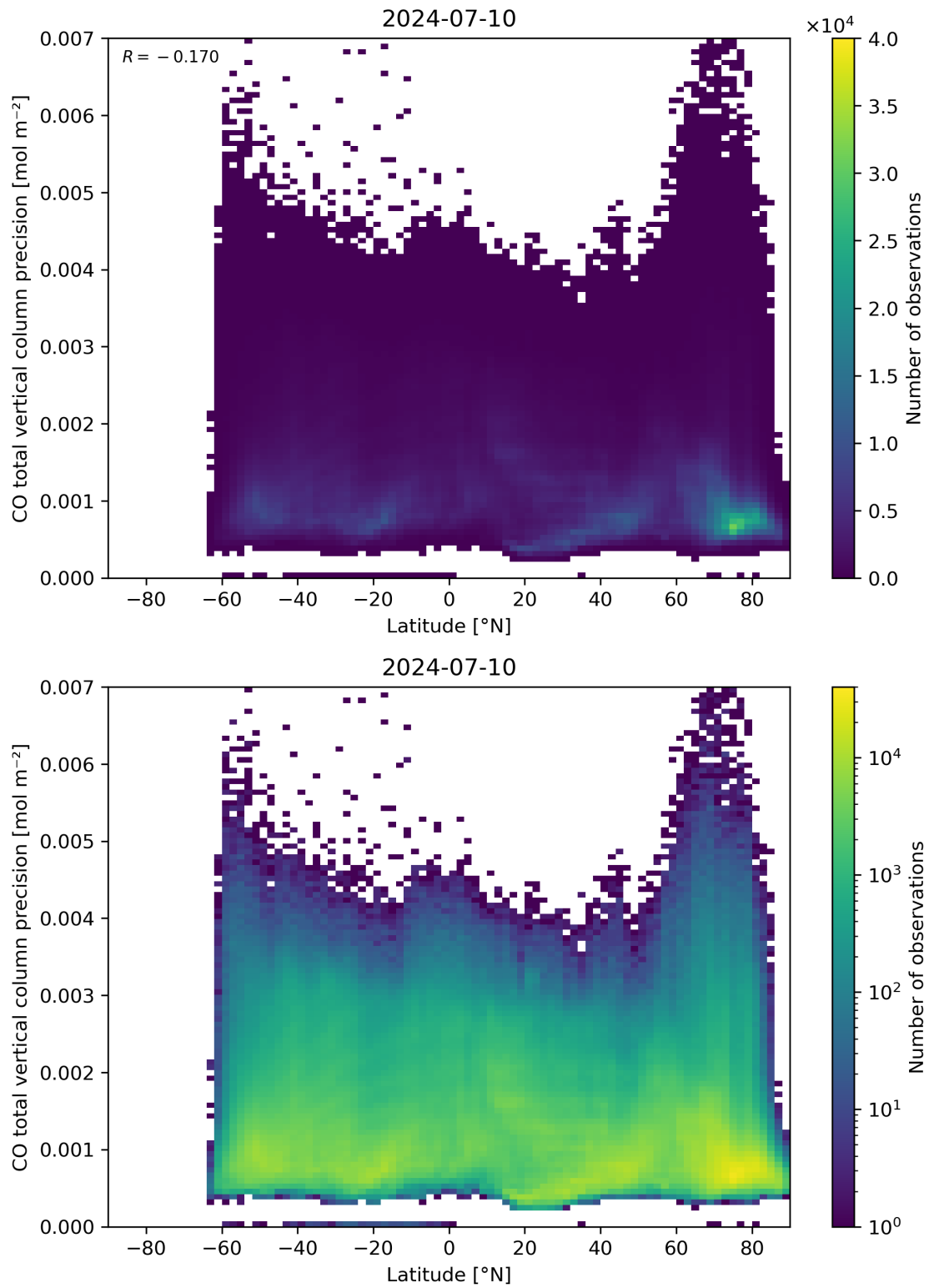
Figure 53: Scatter density plot of “Latitude” against “CO total vertical column precision” for 2024-07-10 to 2024-07-11.
