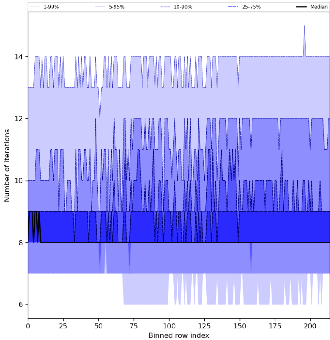
Figure 32: Along track statistics of “Number of iterations” for 2024-07-10 to 2024-07-11
