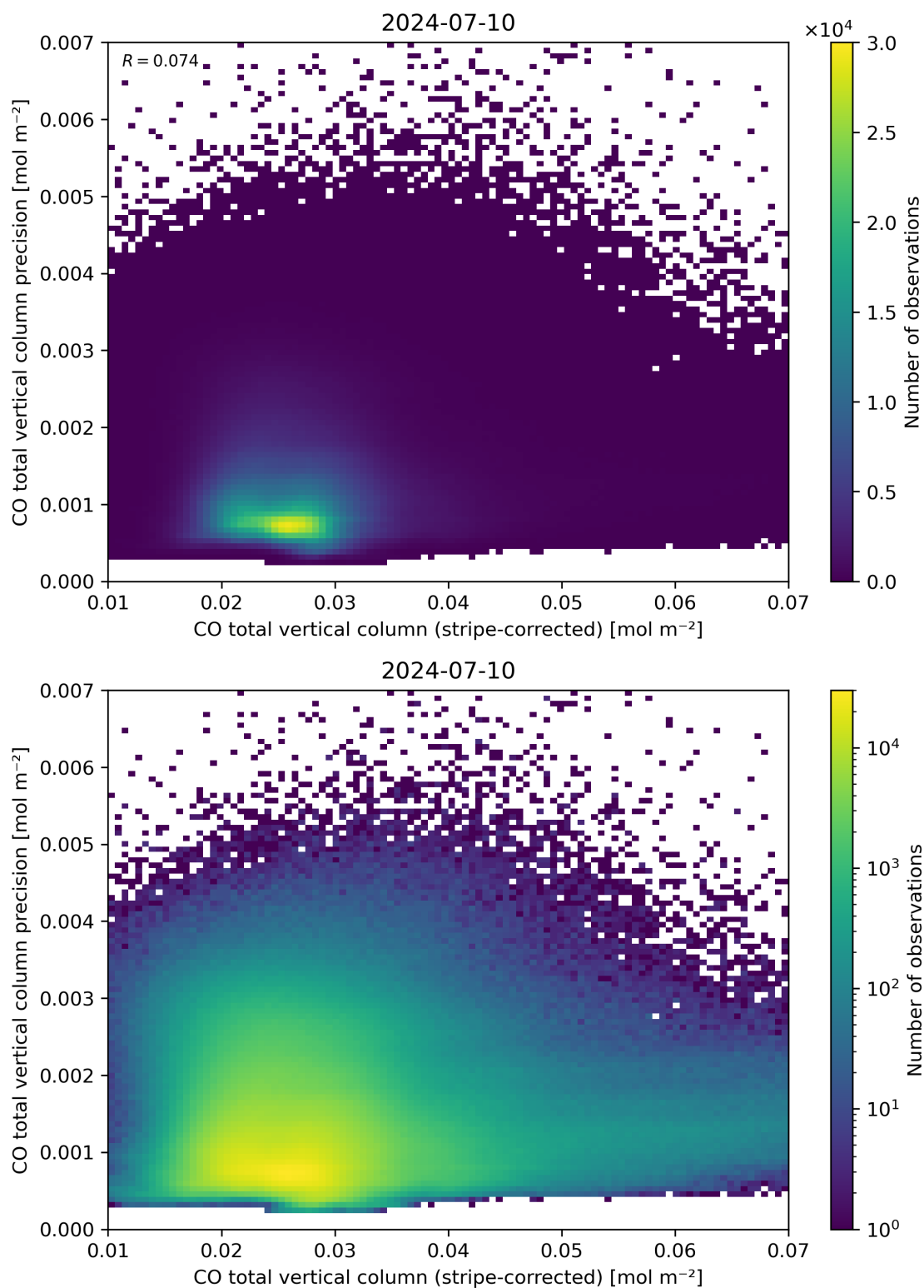
Figure 36: Scatter density plot of “CO total vertical column (stripe-corrected)” against “CO total vertical column precision” for 2024-07-10 to 2024-07-11.
