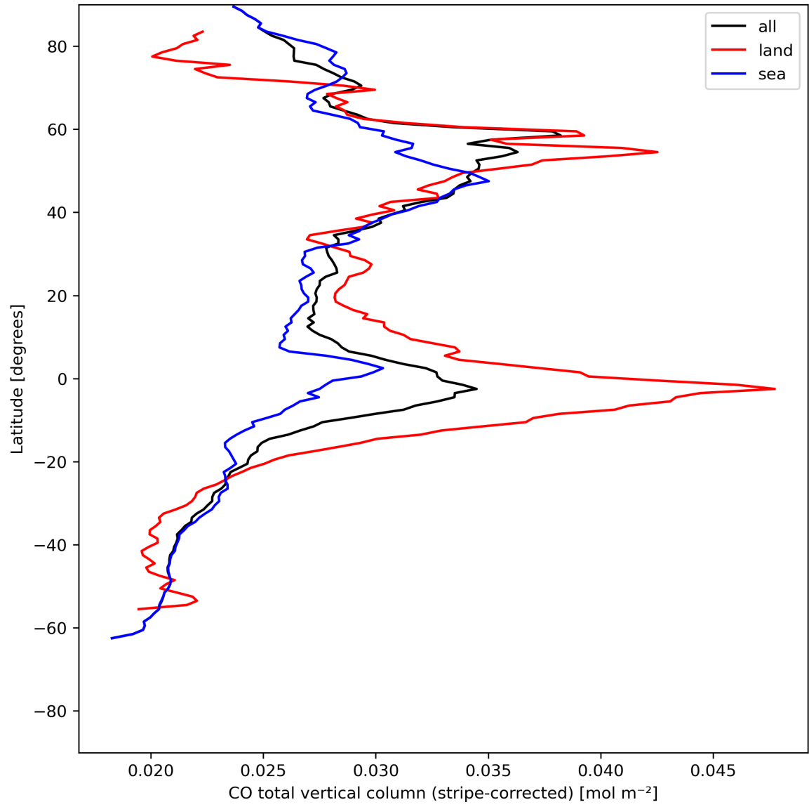
Figure 11: Zonal average of “CO total vertical column (stripe-corrected)” for 2024-07-10 to 2024-07-11.
