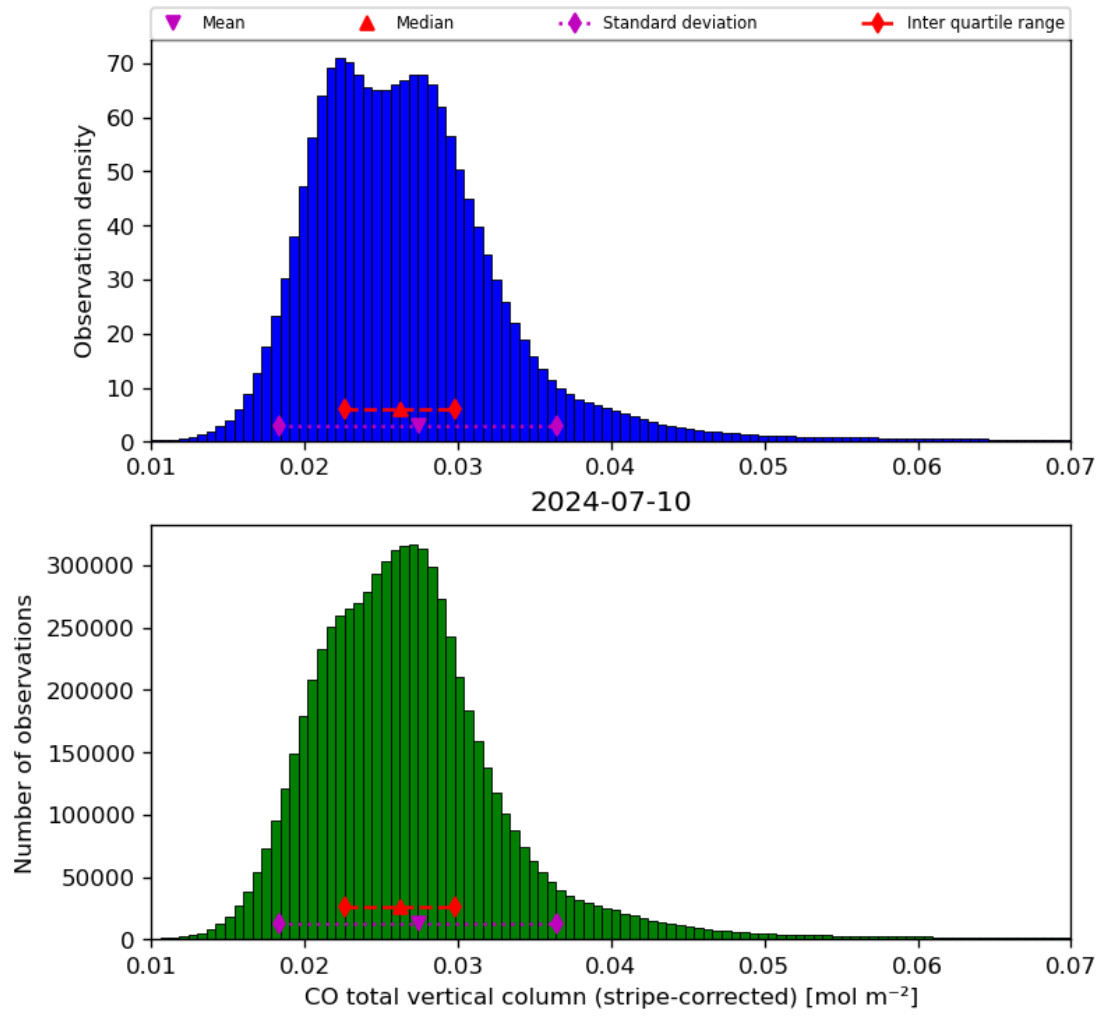
Figure 19: Histogram of “CO total vertical column (stripe-corrected)” for 2024-07-10 to 2024-07-11
