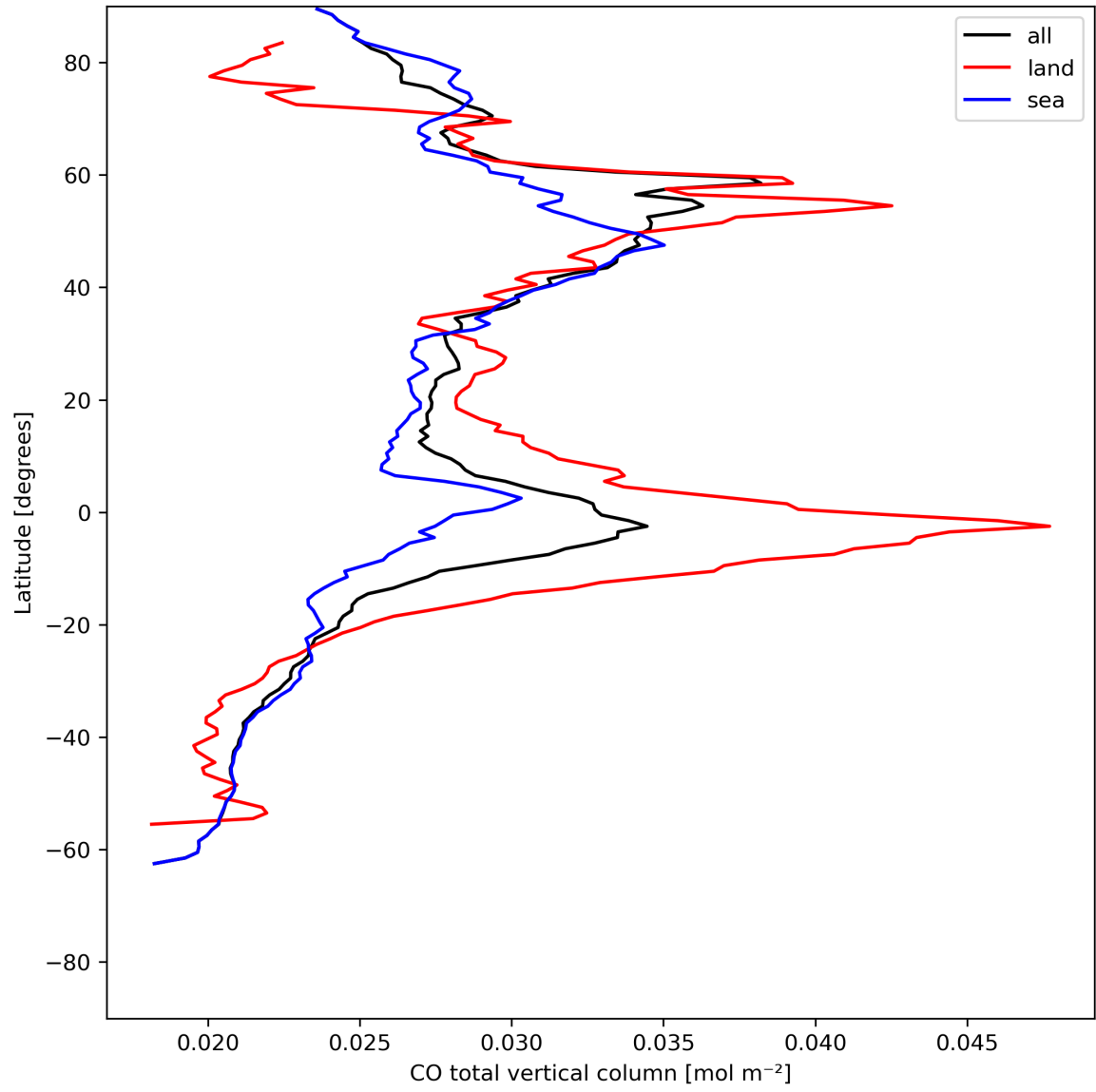
Figure 10: Zonal average of “CO total vertical column” for 2024-07-10 to 2024-07-11.
