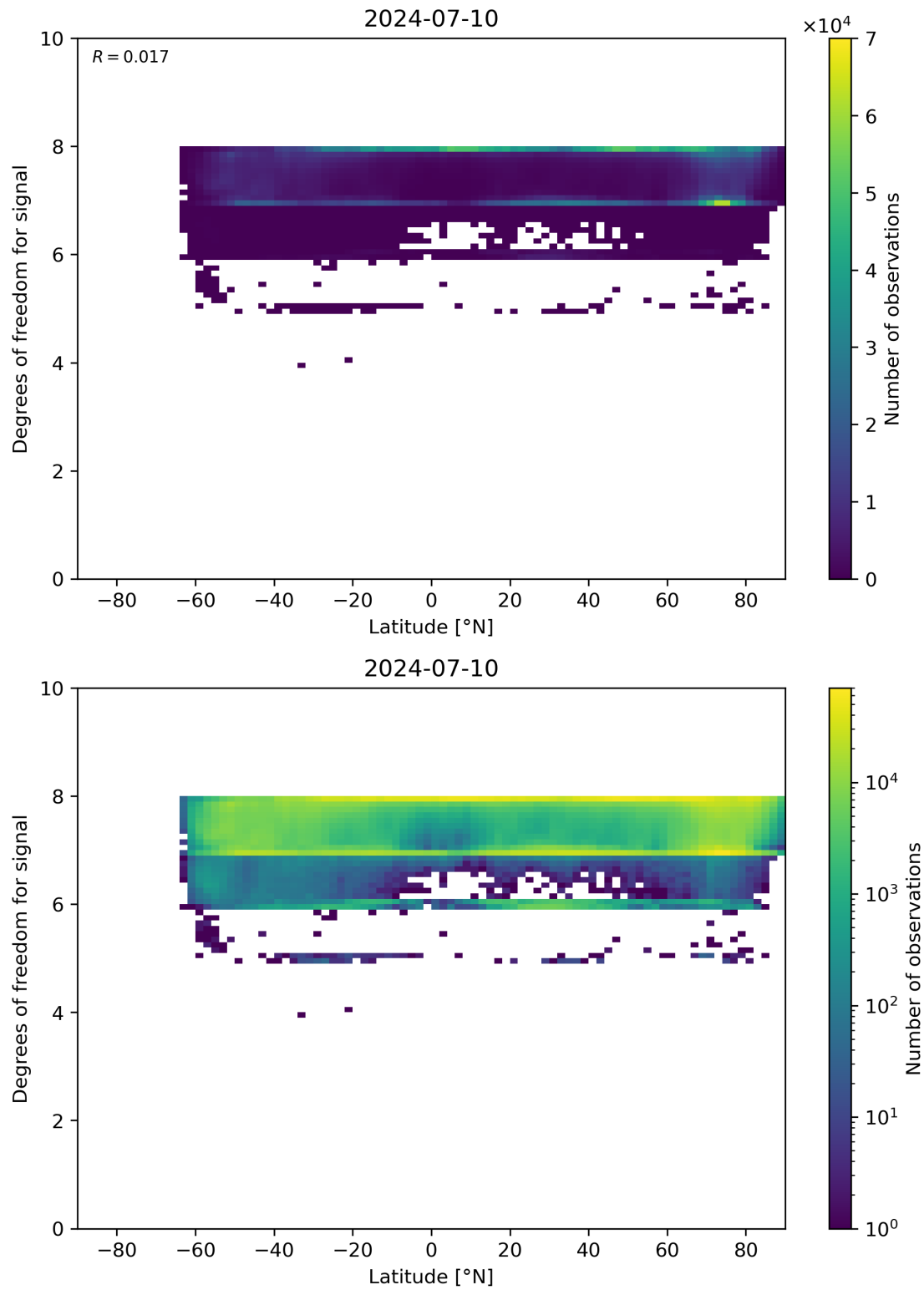
Figure 55: Scatter density plot of “Latitude” against “Degrees of freedom for signal” for 2024-07-10 to 2024-07-11.
