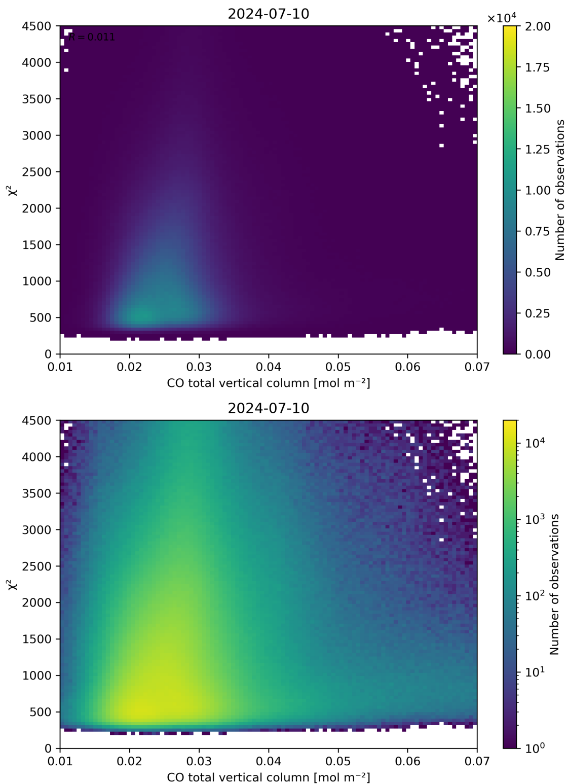
Figure 35: Scatter density plot of “CO total vertical column” against “ \chi^2 ” for 2024-07-10 to 2024-07-11.
