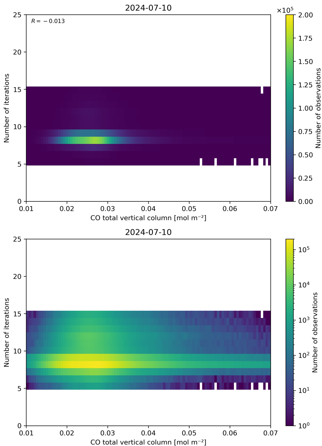
Figure 42: Scatter density plot of “CO total vertical column” against “Number of iterations” for 2024-07-10 to 2024-07-11.
