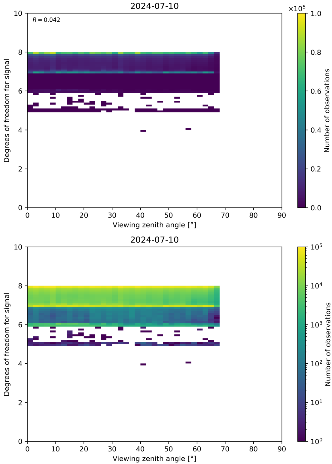
Figure 73: Scatter density plot of “Viewing zenith angle” against “Degrees of freedom for signal” for 2024-07-10 to 2024-07-11.
