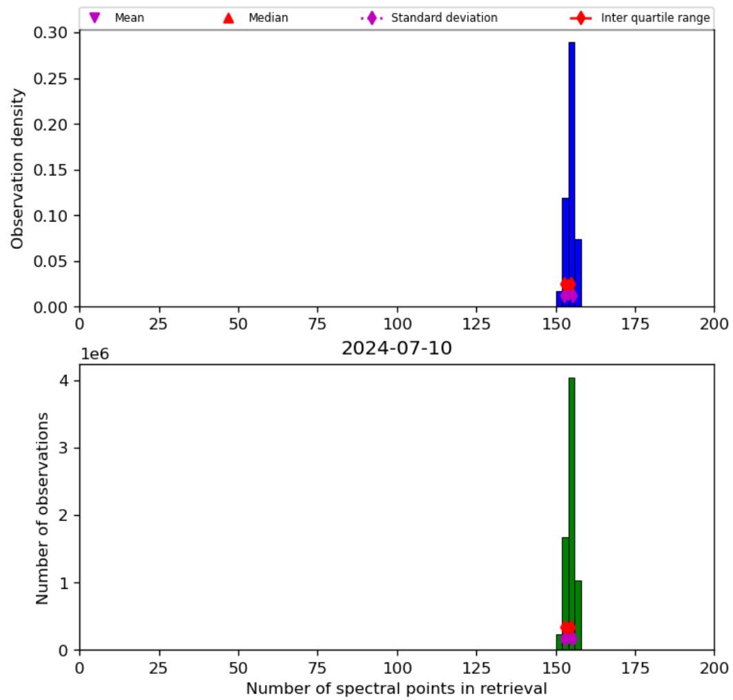
Figure 21: Histogram of “Number of spectral points in retrieval” for 2024-07-10 to 2024-07-11
