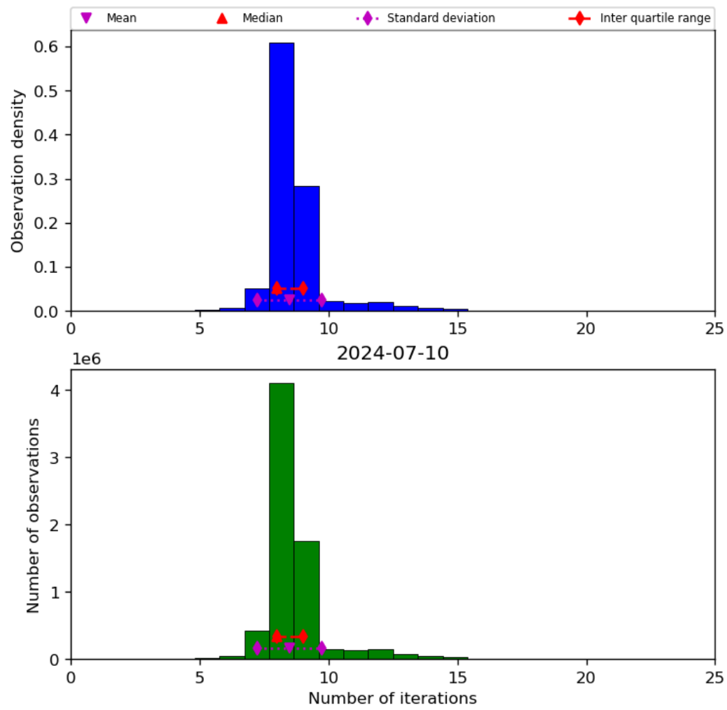
Figure 24: Histogram of “Number of iterations” for 2024-07-10 to 2024-07-11
