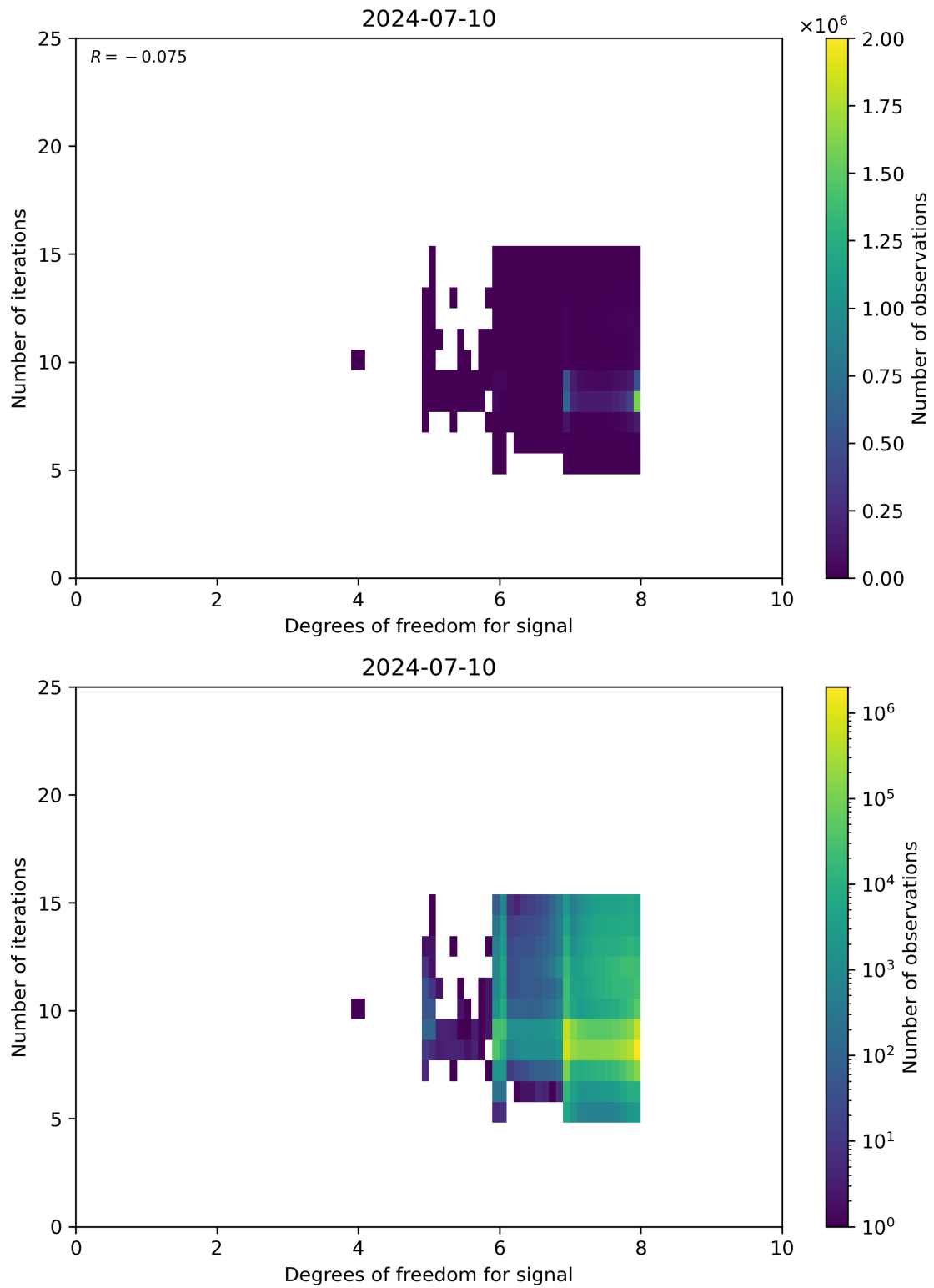
Figure 50: Scatter density plot of “Degrees of freedom for signal” against “Number of iterations” for 2024-07-10 to 2024-07-11.
