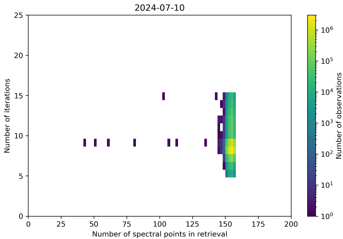
Figure 60: Scatter density plot of “Number of spectral points in retrieval” against “Number of iterations” for 2024-07-10 to 2024-07-11.
