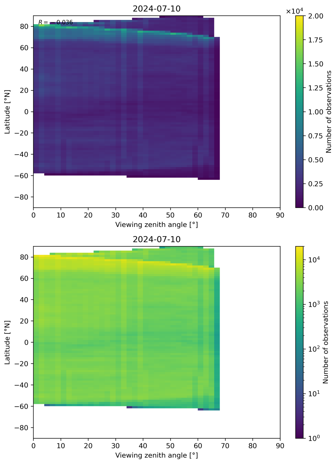
Figure 74: Scatter density plot of “Viewing zenith angle” against “Latitude” for 2024-07-10 to 2024-07-11.
