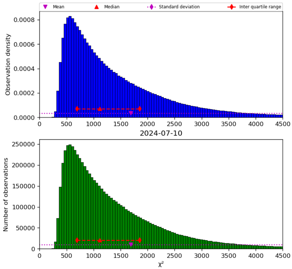
Figure 22: Histogram of “ \chi^2 ” for 2024-07-10 to 2024-07-11
