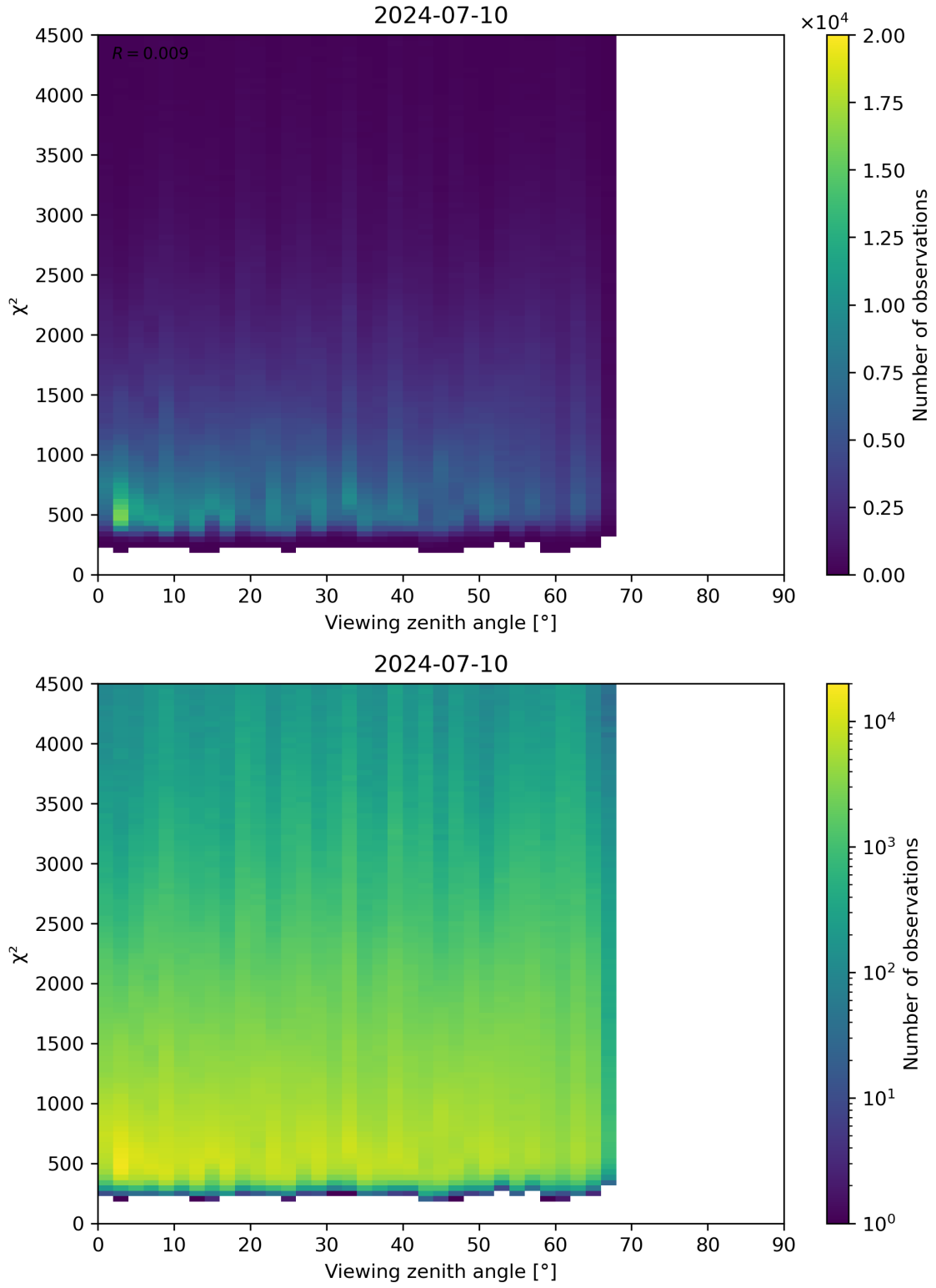
Figure 72: Scatter density plot of “Viewing zenith angle” against “ \chi^2 ” for 2024-07-10 to 2024-07-11.
