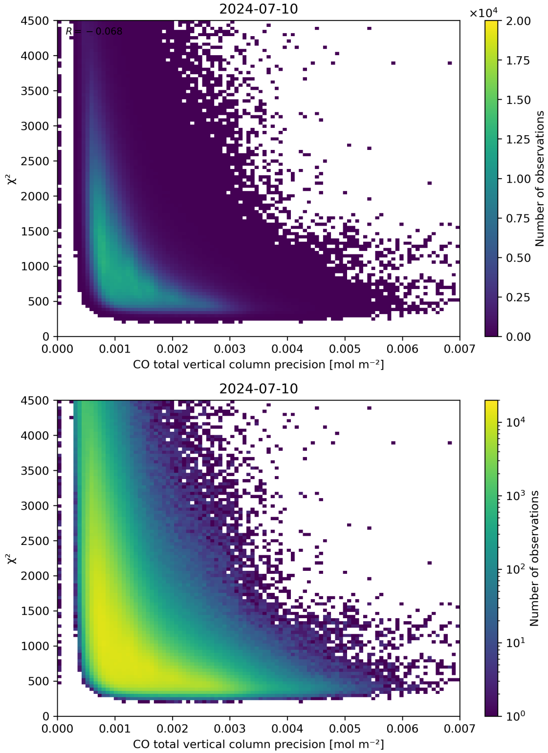
Figure 44: Scatter density plot of “CO total vertical column precision” against “ \chi^2 ” for 2024-07-10 to 2024-07-11.
