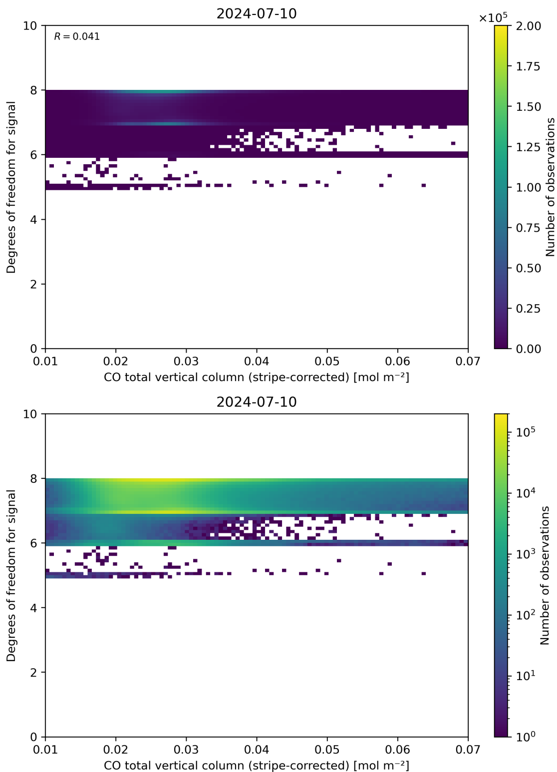
Figure 38: Scatter density plot of “CO total vertical column (stripe-corrected)” against “Degrees of freedom for signal” for 2024-07-10 to 2024-07-11.
