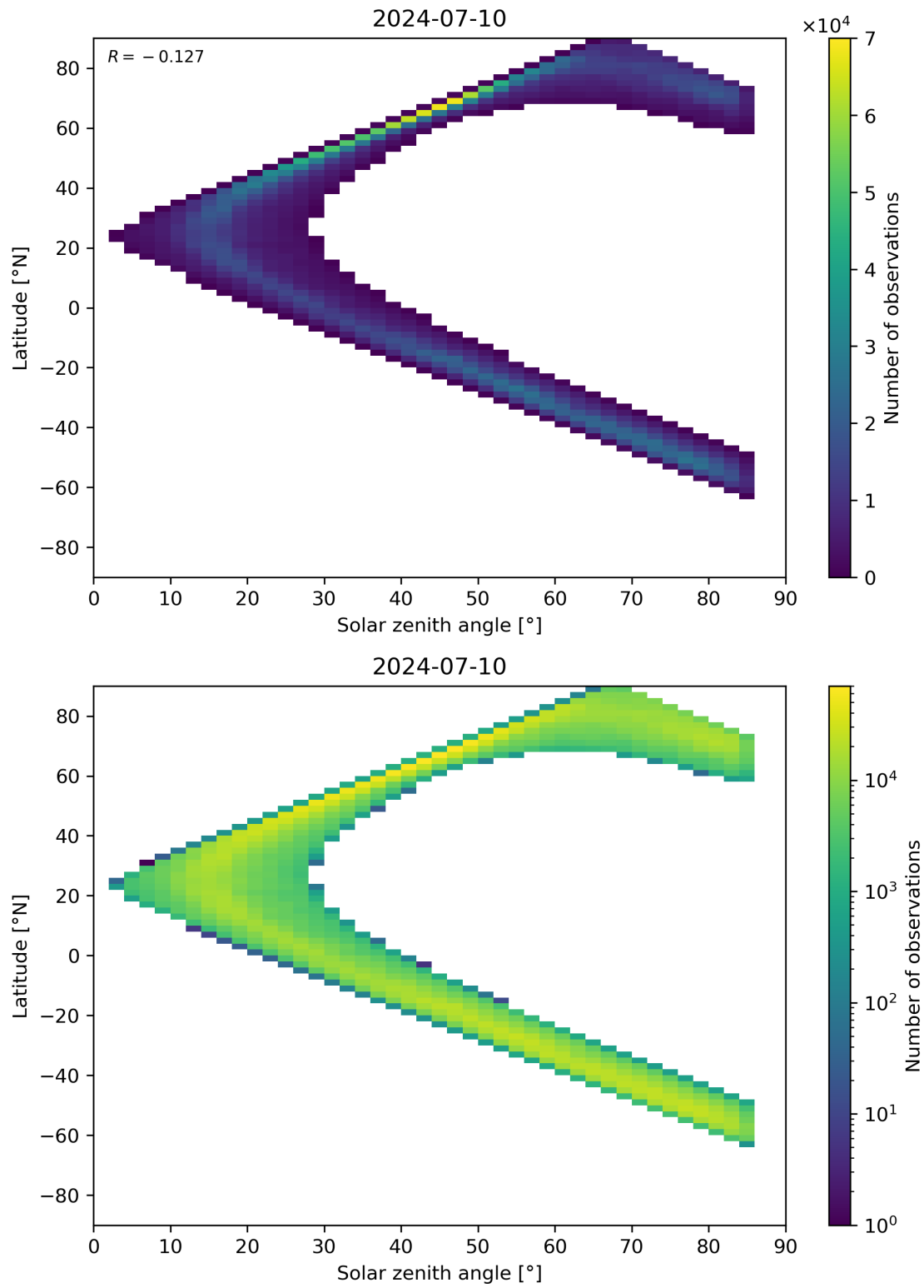
Figure 66: Scatter density plot of “Solar zenith angle” against “Latitude” for 2024-07-10 to 2024-07-11.
