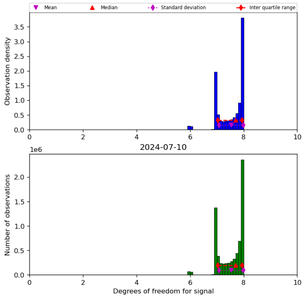
Figure 23: Histogram of “Degrees of freedom for signal” for 2024-07-10 to 2024-07-11
