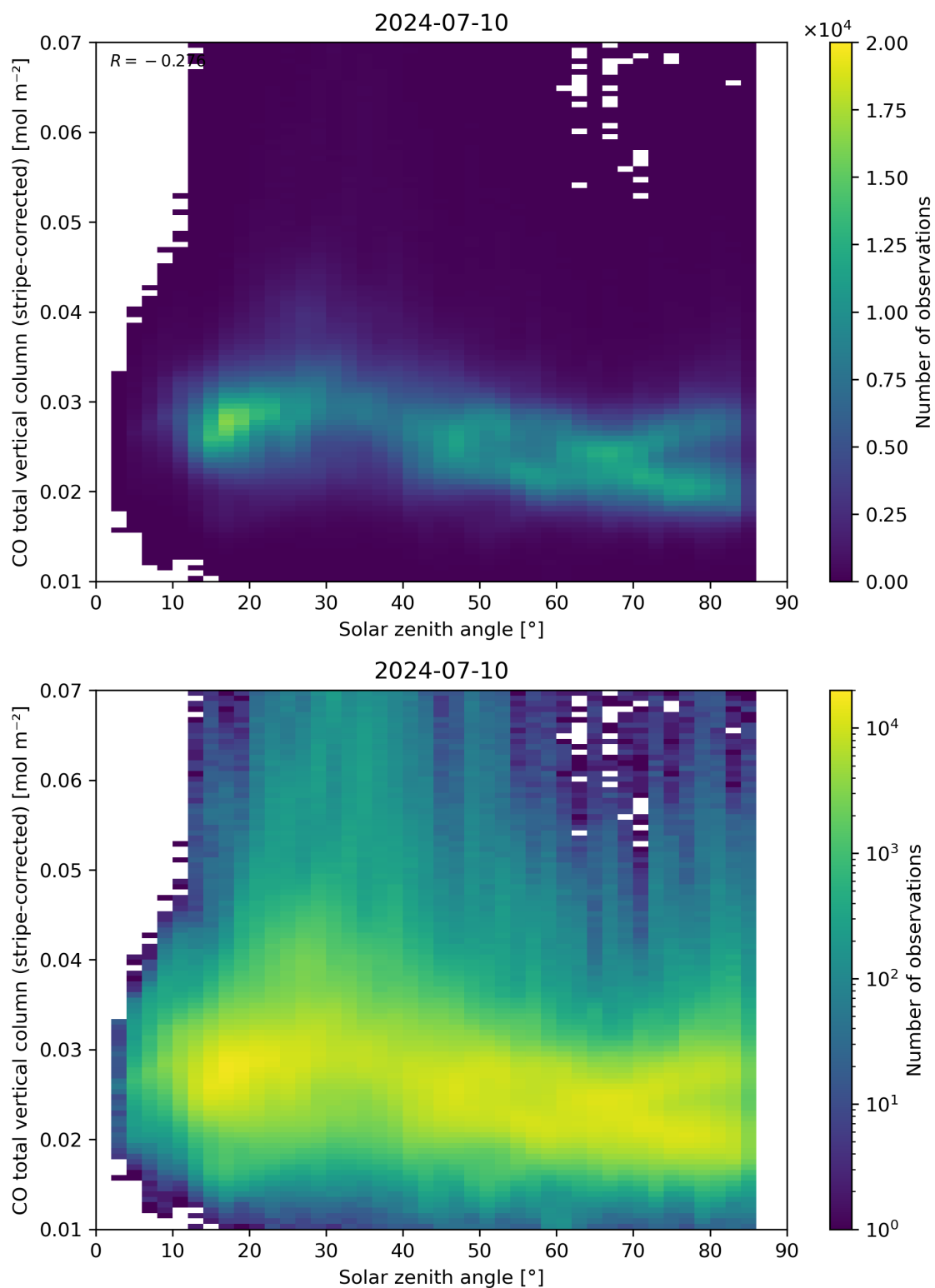
Figure 62: Scatter density plot of “Solar zenith angle” against “CO total vertical column (stripe-corrected)” for 2024-07-10 to 2024-07-11.
