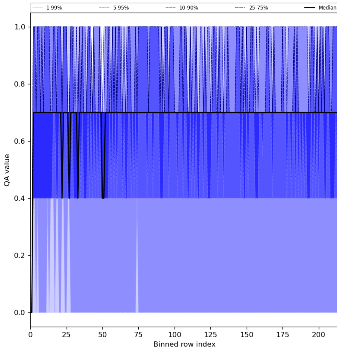
Figure 25: Along track statistics of “QA value” for 2024-07-10 to 2024-07-11
