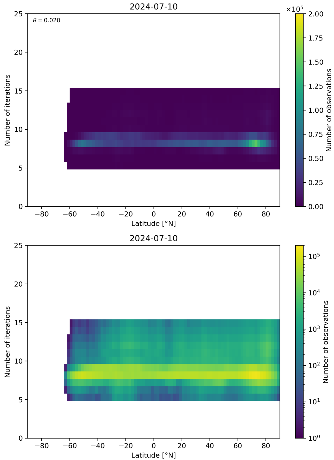
Figure 56: Scatter density plot of “Latitude” against “Number of iterations” for 2024-07-10 to 2024-07-11.
