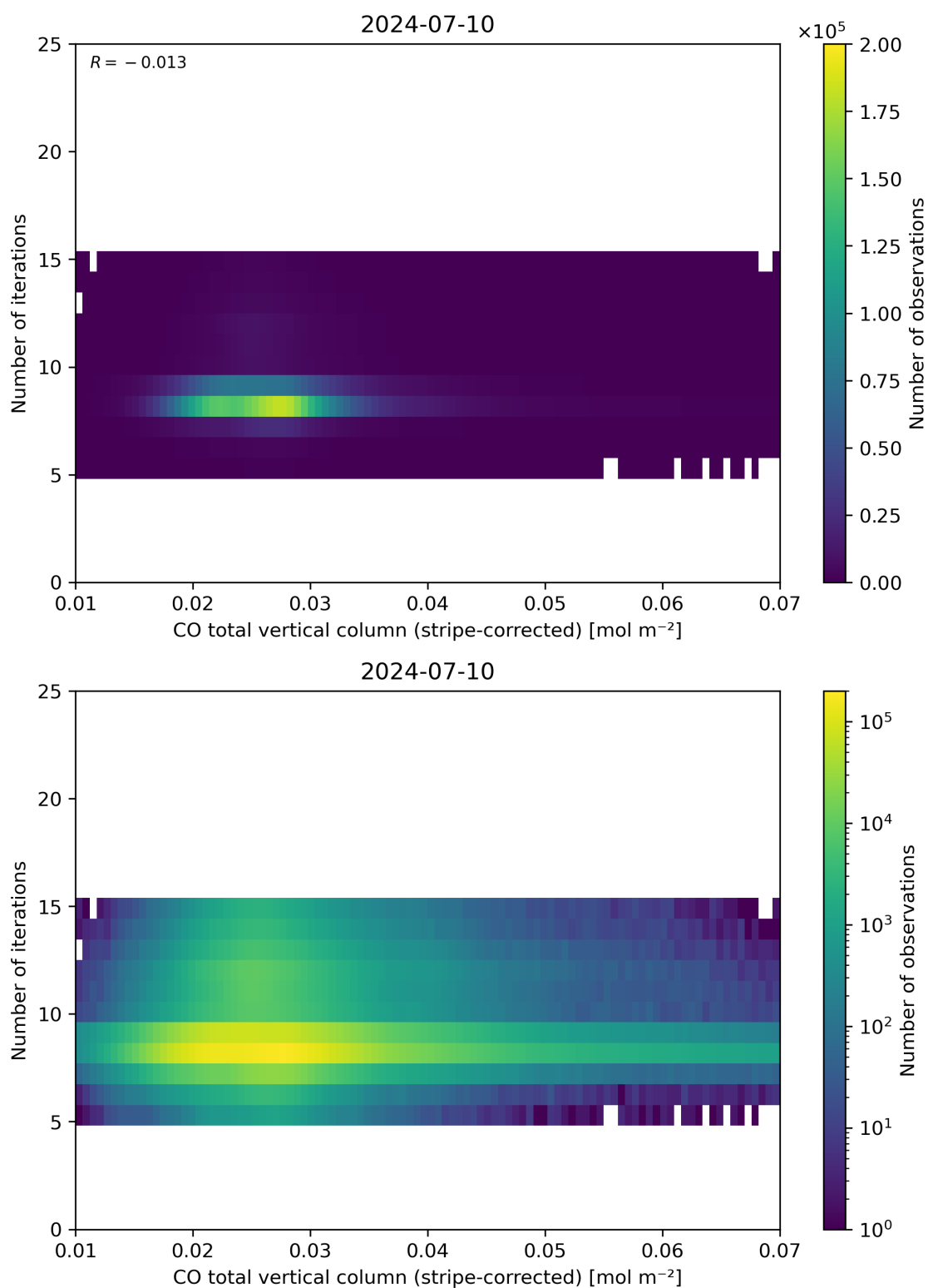
Figure 39: Scatter density plot of “CO total vertical column (stripe-corrected)” against “Number of iterations” for 2024-07-10 to 2024-07-11.
