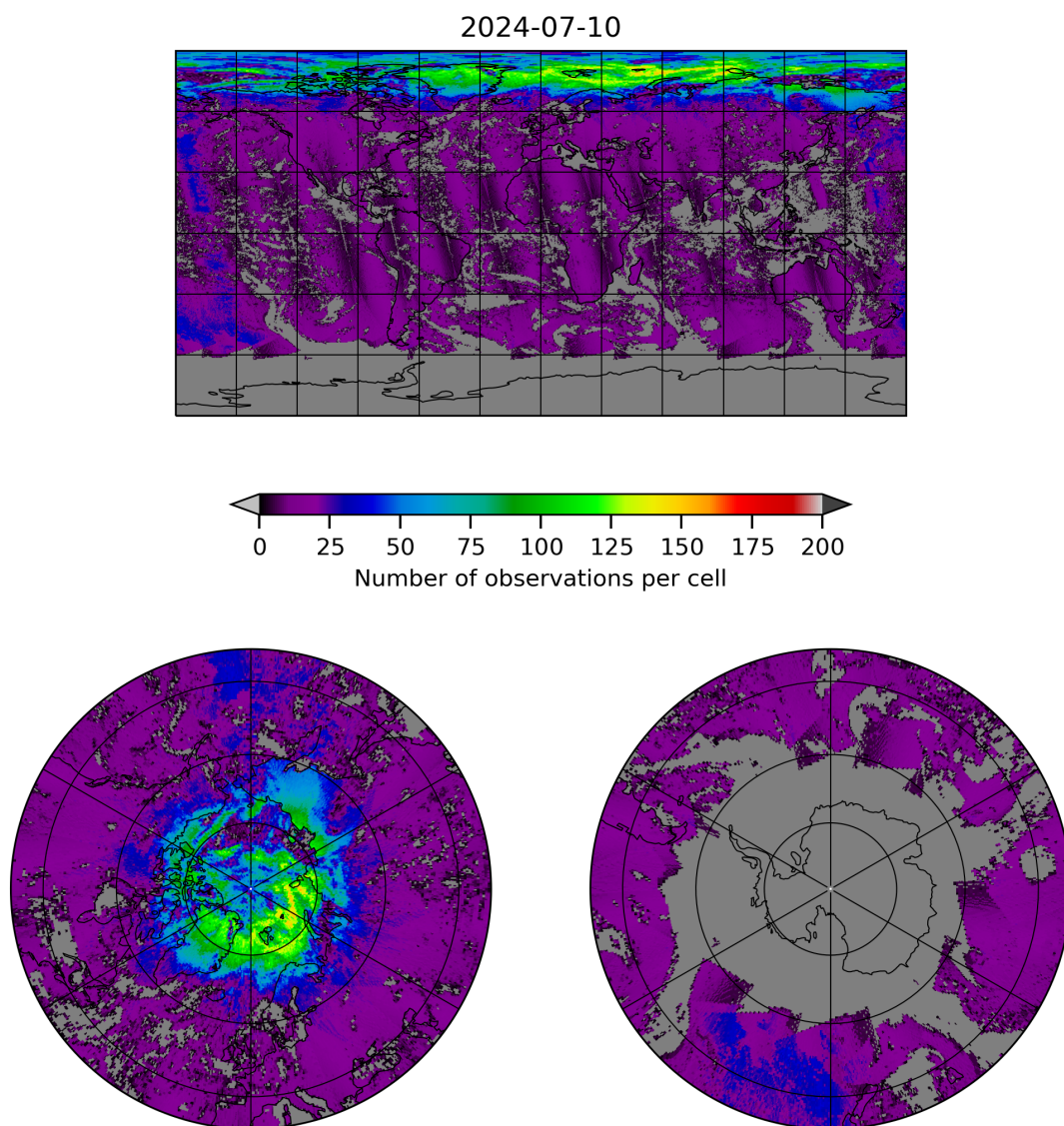
Figure 8: Map of the number of observations for 2024-07-10 to 2024-07-11
