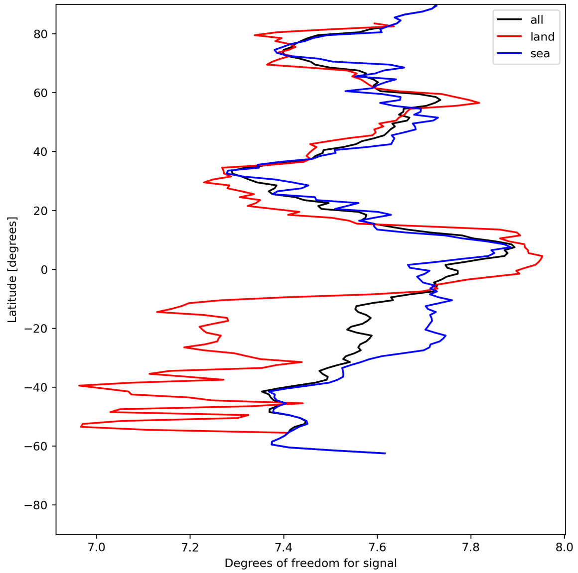
Figure 15: Zonal average of “Degrees of freedom for signal” for 2024-07-10 to 2024-07-11.
