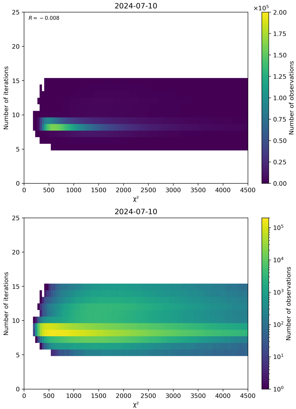
Figure 49: Scatter density plot of “ \chi^2 ” against “Number of iterations” for 2024-07-10 to 2024-07-11.
