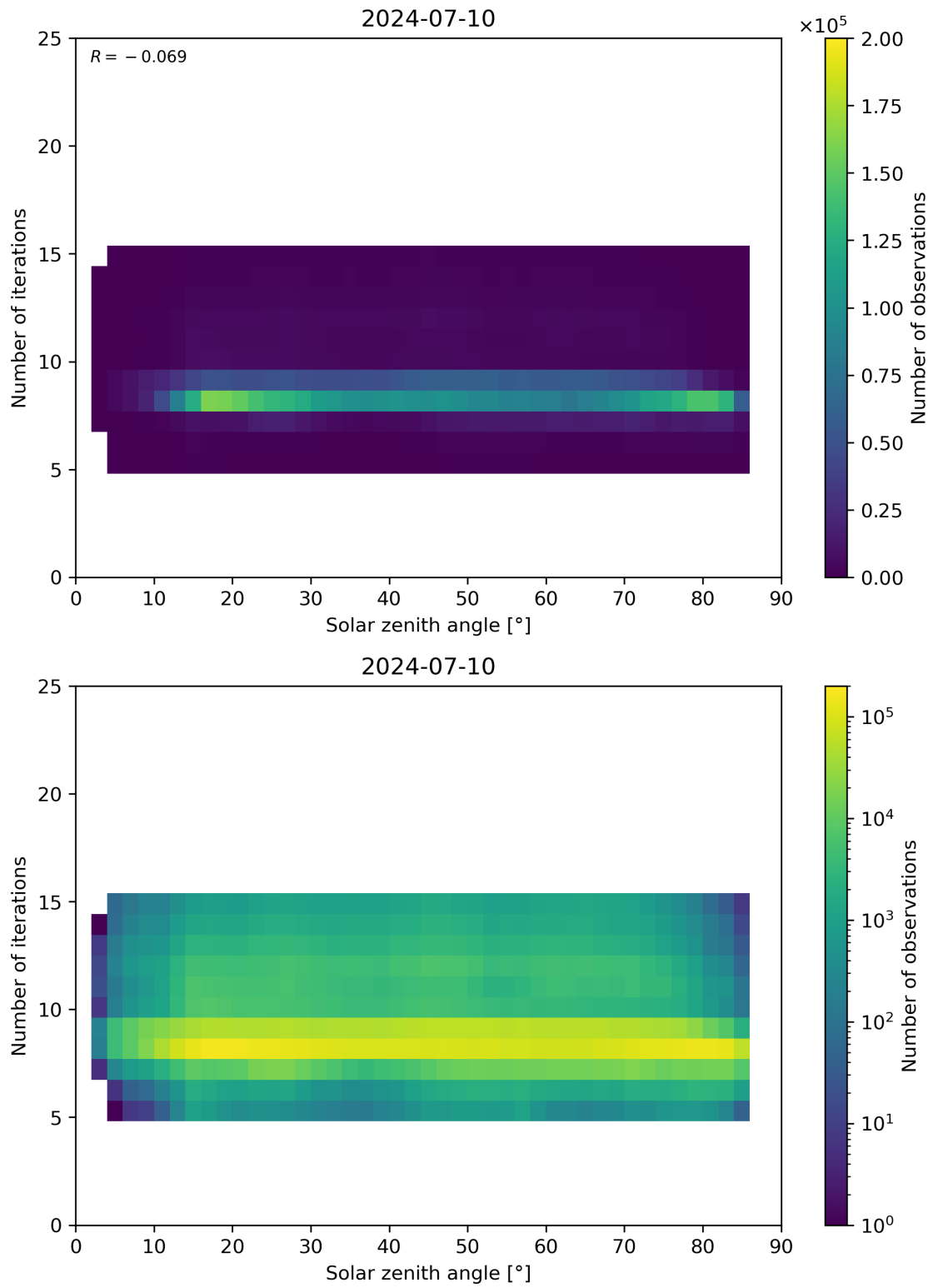
Figure 67: Scatter density plot of “Solar zenith angle” against “Number of iterations” for 2024-07-10 to 2024-07-11.
