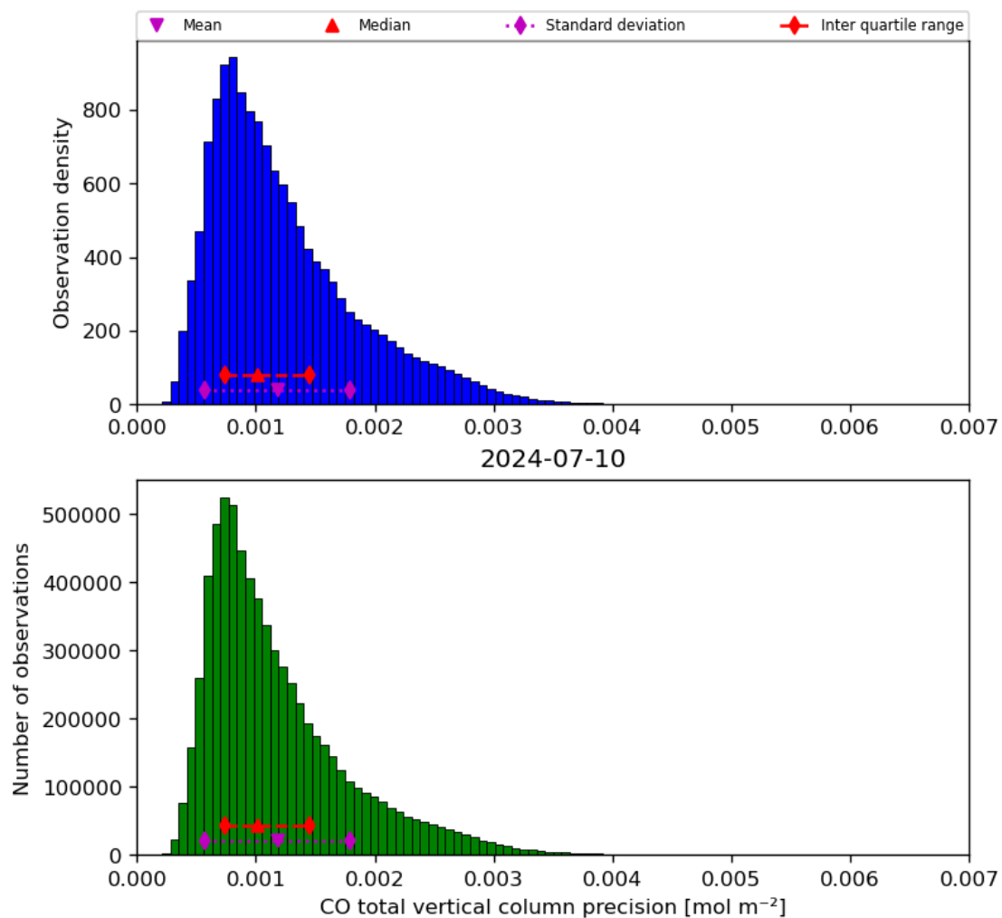
Figure 20: Histogram of “CO total vertical column precision” for 2024-07-10 to 2024-07-11
