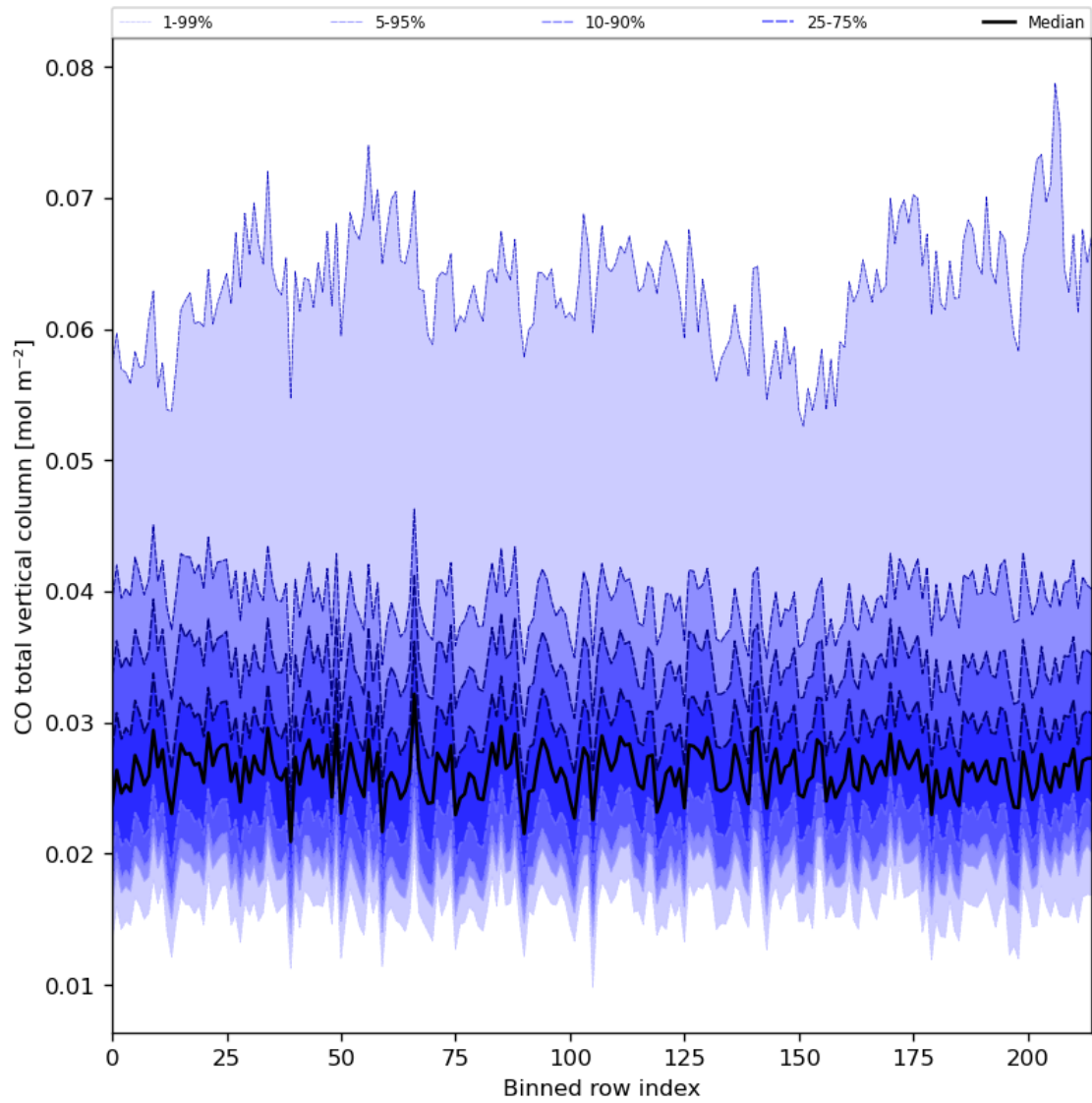
Figure 26: Along track statistics of “CO total vertical column” for 2024-07-10 to 2024-07-11
