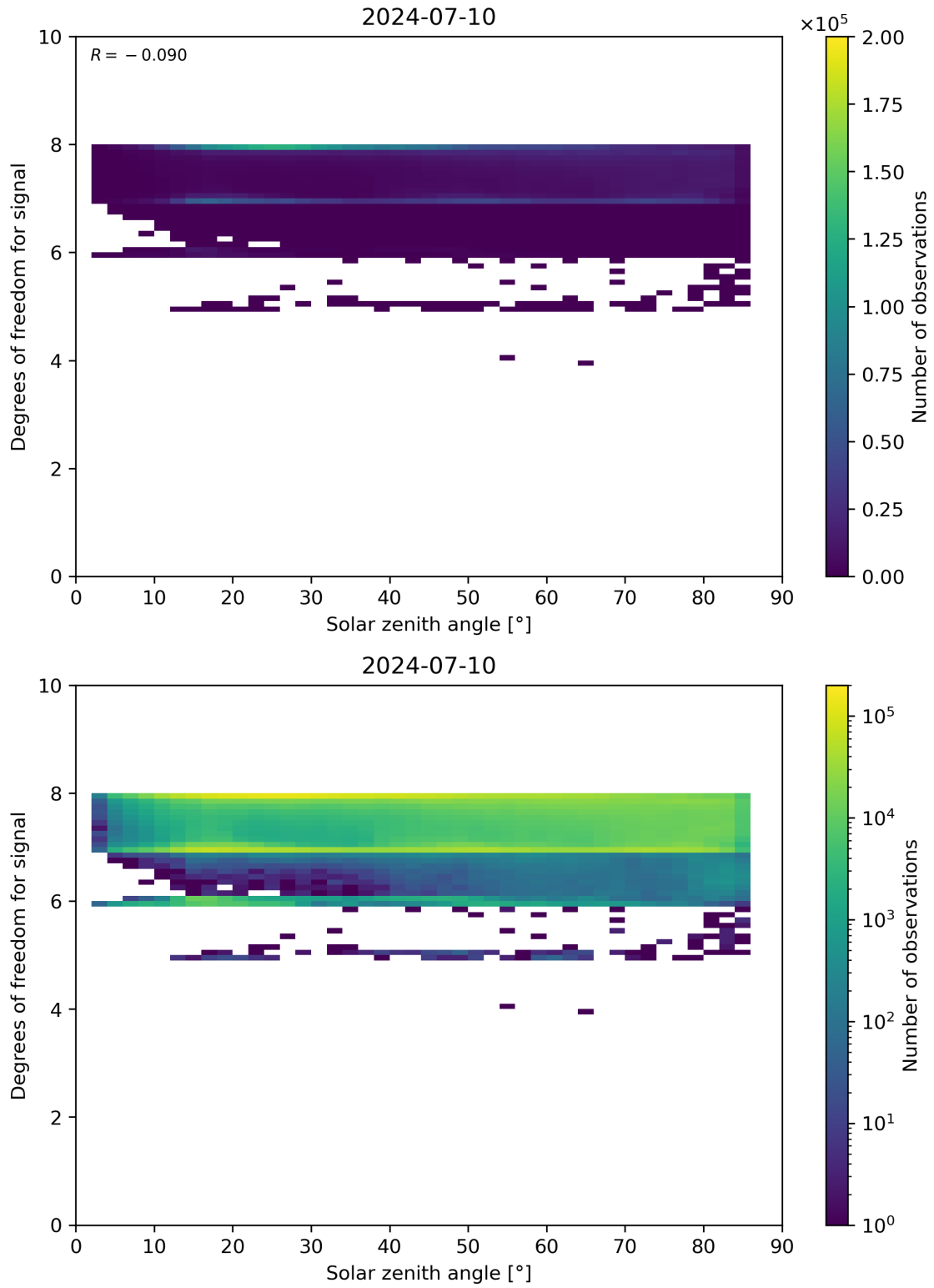
Figure 65: Scatter density plot of “Solar zenith angle” against “Degrees of freedom for signal” for 2024-07-10 to 2024-07-11.
