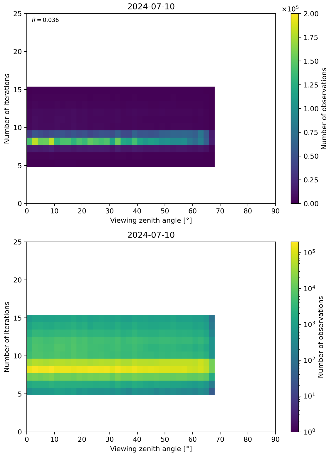
Figure 75: Scatter density plot of “Viewing zenith angle” against “Number of iterations” for 2024-07-10 to 2024-07-11.
