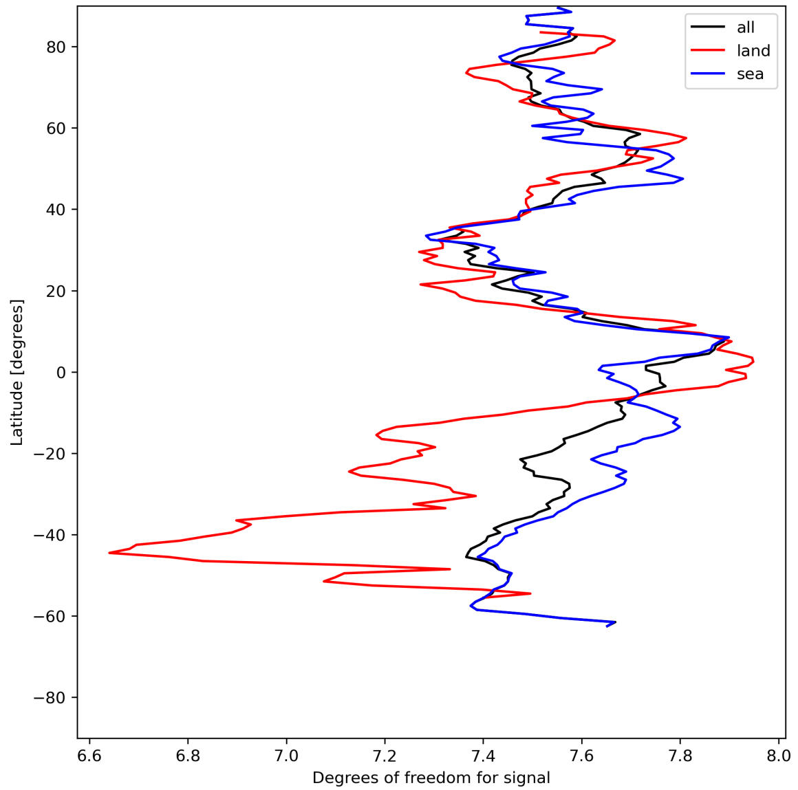
Figure 15: Zonal average of “Degrees of freedom for signal” for 2024-07-10 to 2024-07-12.
