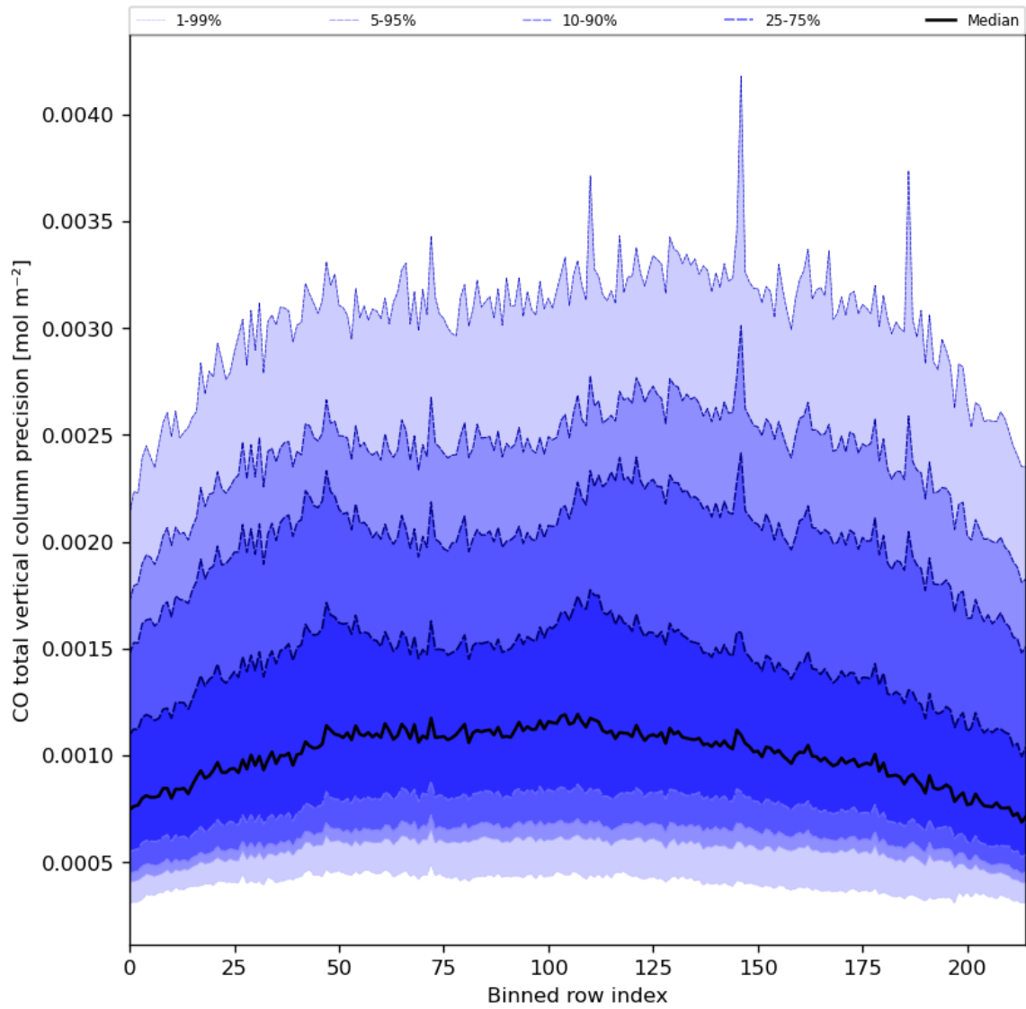
Figure 28: Along track statistics of “CO total vertical column precision” for 2024-07-10 to 2024-07-12
