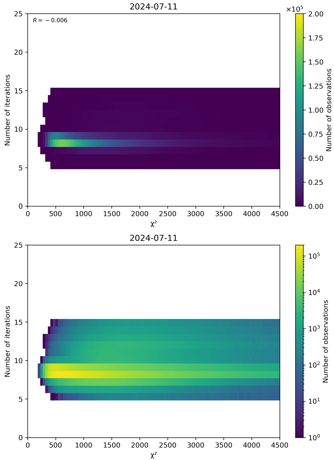
Figure 49: Scatter density plot of “ \chi^2 ” against “Number of iterations” for 2024-07-10 to 2024-07-12.
