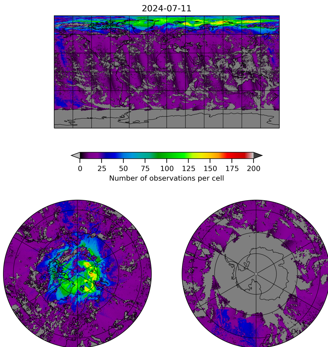
Figure 8: Map of the number of observations for 2024-07-10 to 2024-07-12
