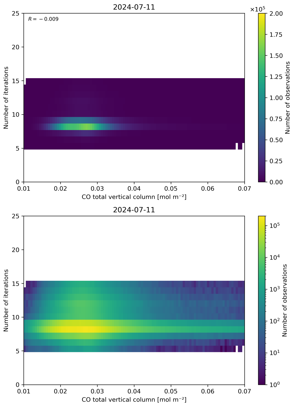
Figure 42: Scatter density plot of “CO total vertical column” against “Number of iterations” for 2024-07-10 to 2024-07-12.
