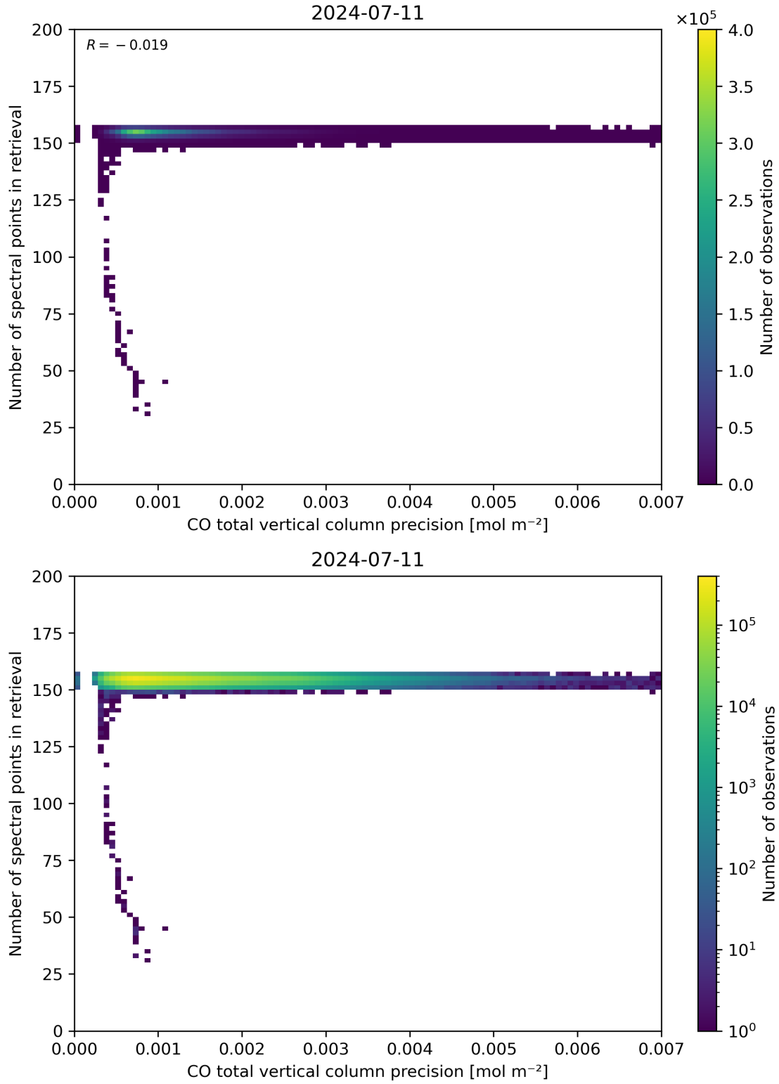
Figure 47: Scatter density plot of “CO total vertical column precision” against “Number of spectral points in retrieval” for 2024-07-10 to 2024-07-12.
