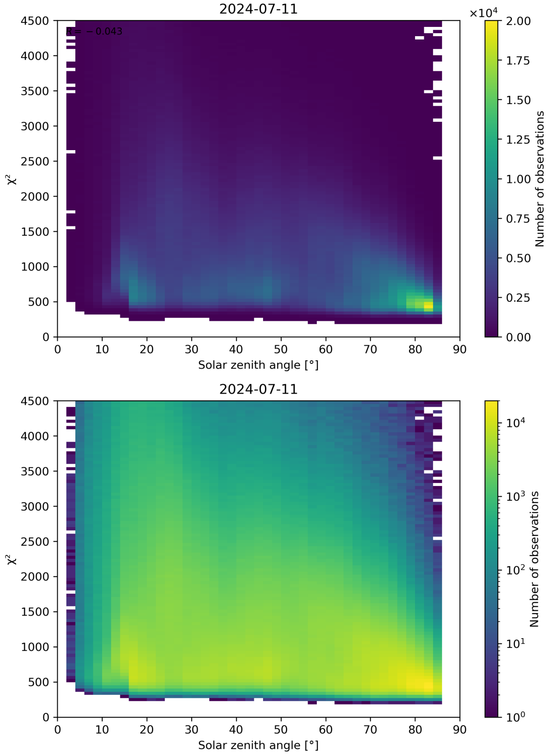
Figure 64: Scatter density plot of “Solar zenith angle” against “ \chi^2 ” for 2024-07-10 to 2024-07-12.
