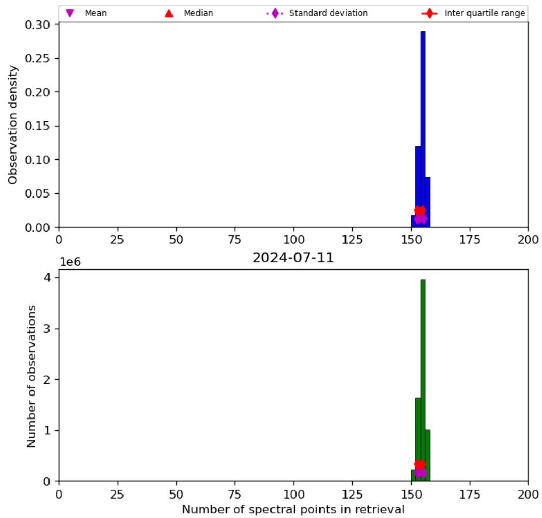
Figure 21: Histogram of “Number of spectral points in retrieval” for 2024-07-10 to 2024-07-12
