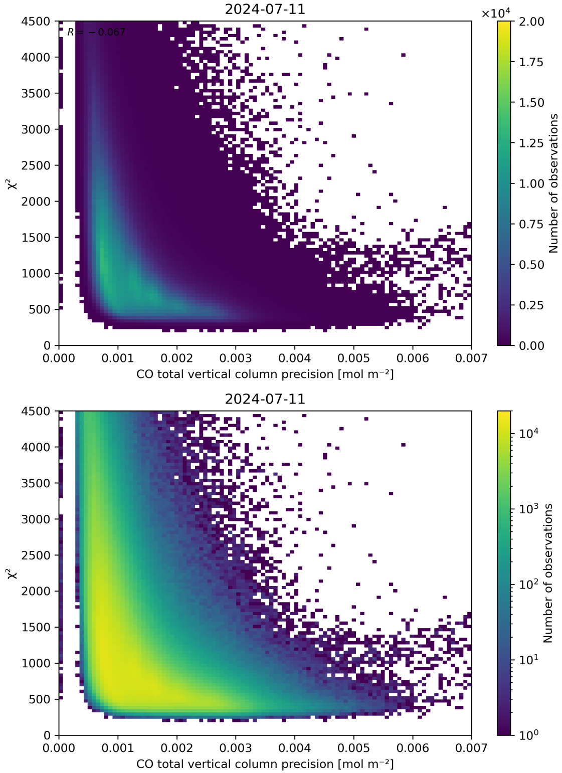
Figure 44: Scatter density plot of “CO total vertical column precision” against “ \chi^2 ” for 2024-07-10 to 2024-07-12.
