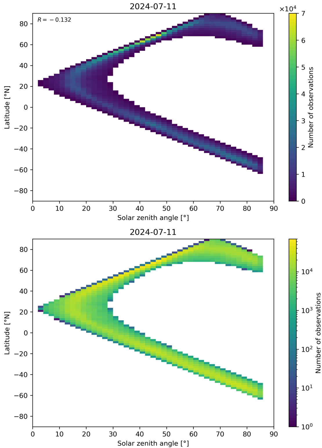
Figure 66: Scatter density plot of “Solar zenith angle” against “Latitude” for 2024-07-10 to 2024-07-12.
