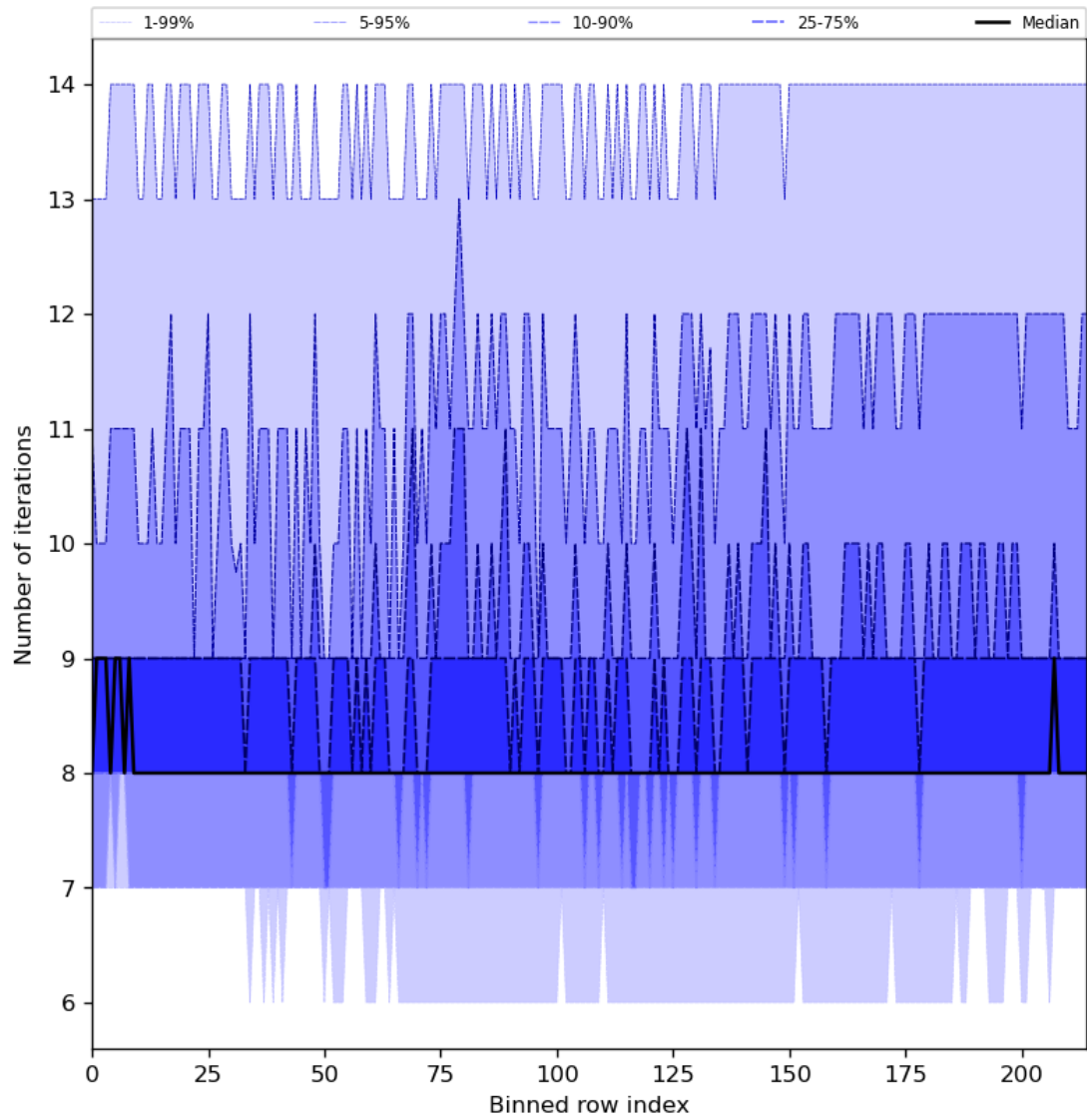
Figure 32: Along track statistics of “Number of iterations” for 2024-07-10 to 2024-07-12
