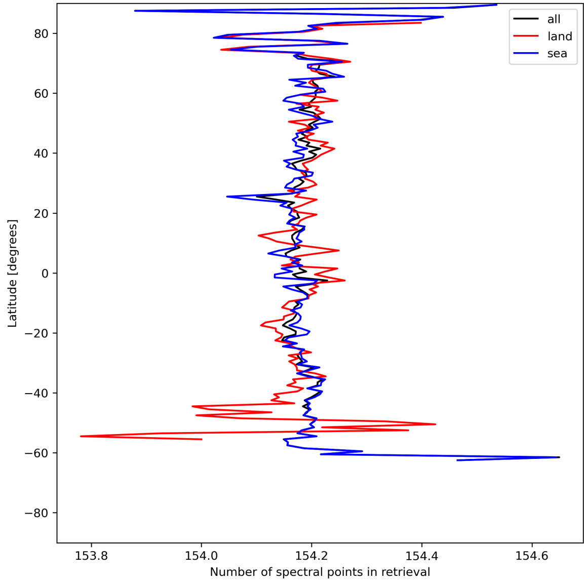
Figure 13: Zonal average of “Number of spectral points in retrieval” for 2024-07-10 to 2024-07-12.
