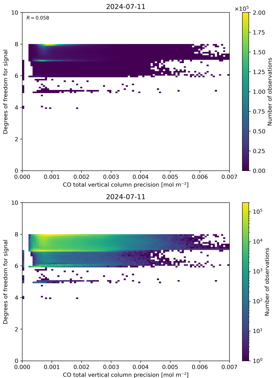
Figure 45: Scatter density plot of “CO total vertical column precision” against “Degrees of freedom for signal” for 2024-07-10 to 2024-07-12.
