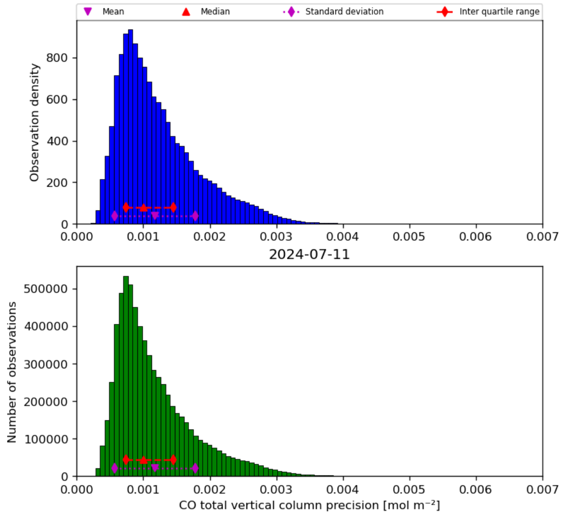
Figure 20: Histogram of “CO total vertical column precision” for 2024-07-10 to 2024-07-12
