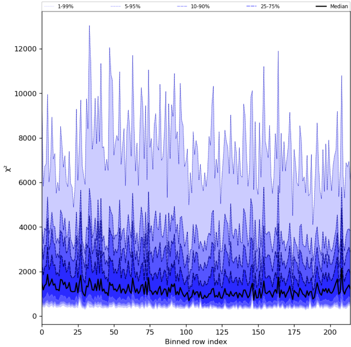
Figure 30: Along track statistics of “ \chi^2 ” for 2024-07-10 to 2024-07-12
