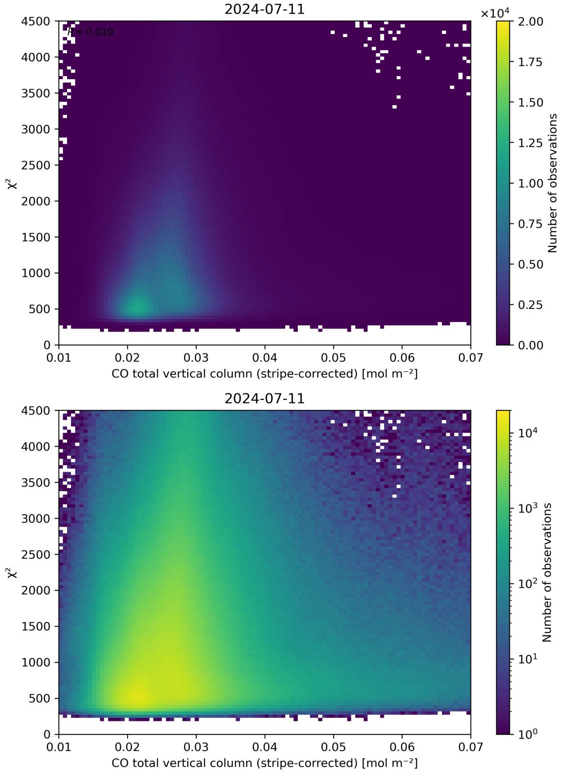
Figure 37: Scatter density plot of “CO total vertical column (stripe-corrected)” against “ \chi^2 ” for 2024-07-10 to 2024-07-12.
