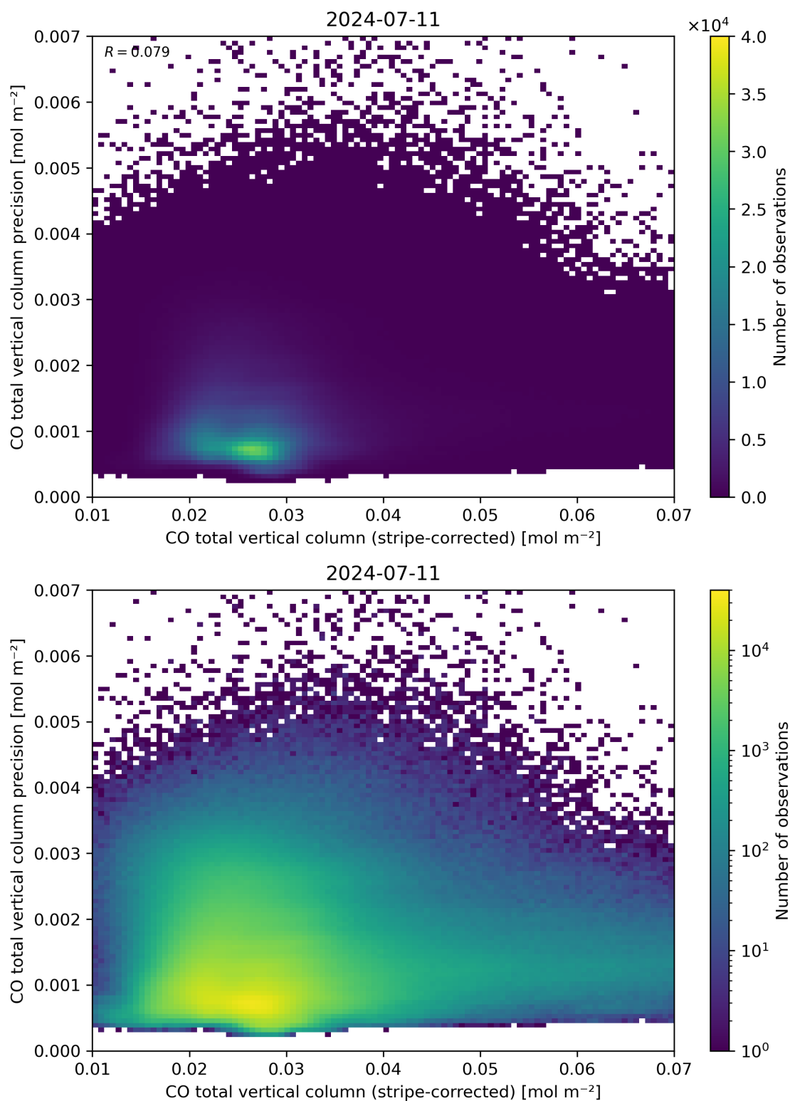
Figure 36: Scatter density plot of “CO total vertical column (stripe-corrected)” against “CO total vertical column precision” for 2024-07-10 to 2024-07-12.
