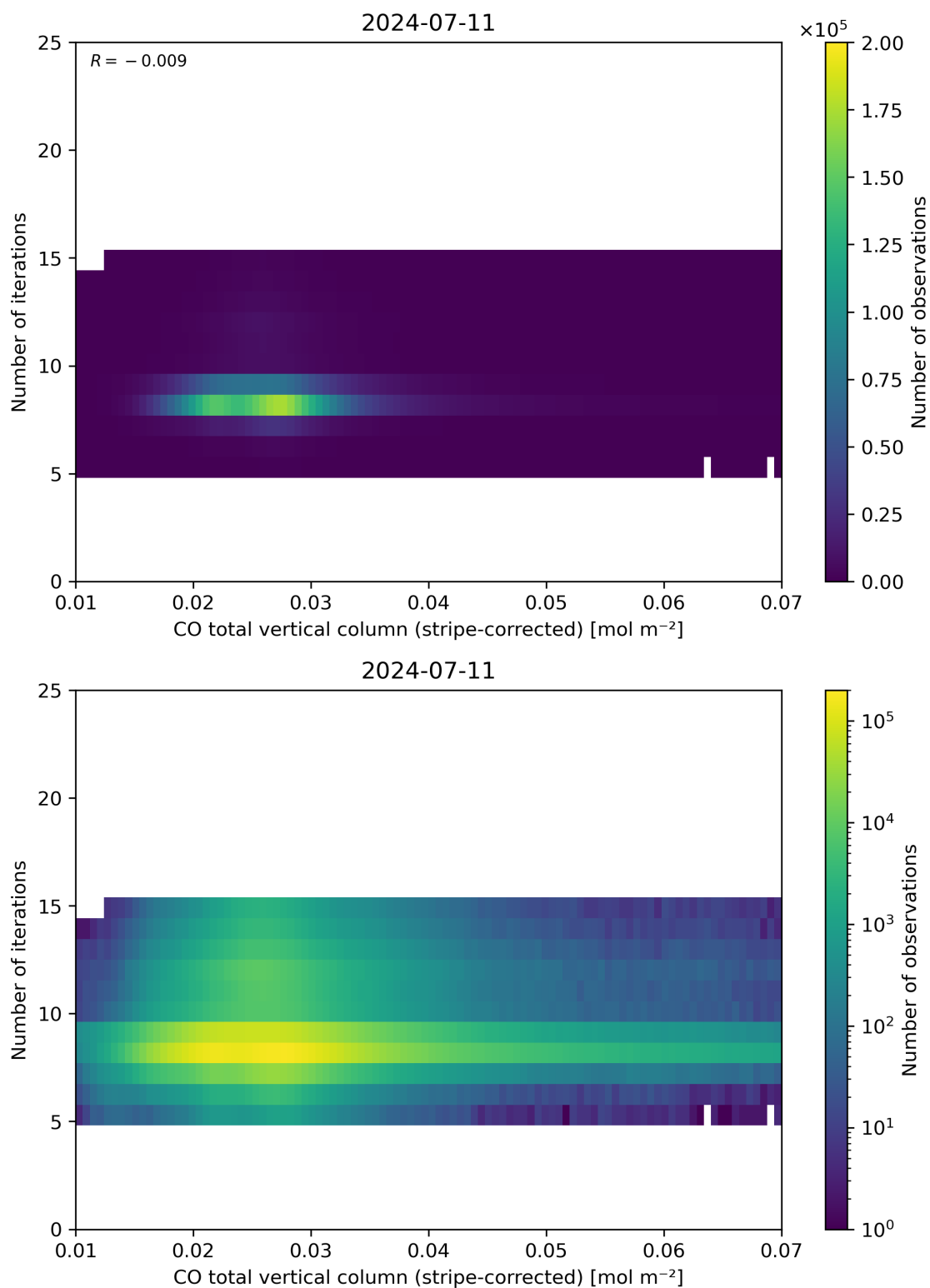
Figure 39: Scatter density plot of “CO total vertical column (stripe-corrected)” against “Number of iterations” for 2024-07-10 to 2024-07-12.
