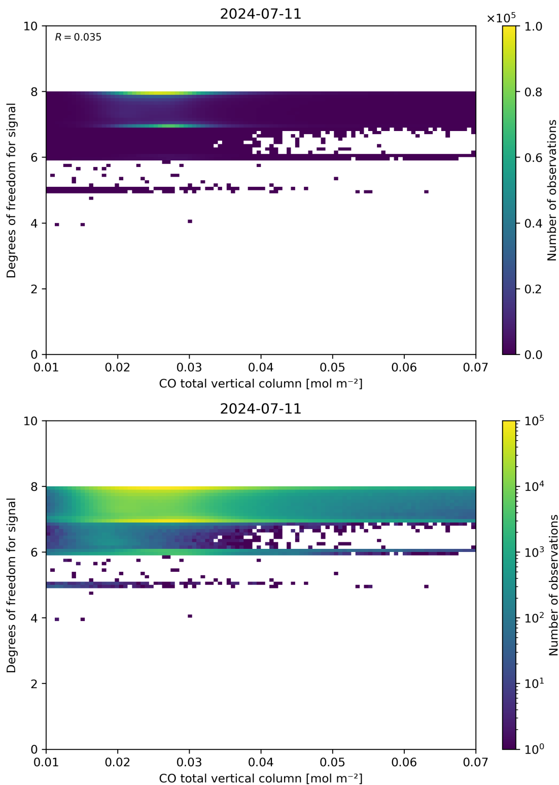
Figure 41: Scatter density plot of “CO total vertical column” against “Degrees of freedom for signal” for 2024-07-10 to 2024-07-12.
