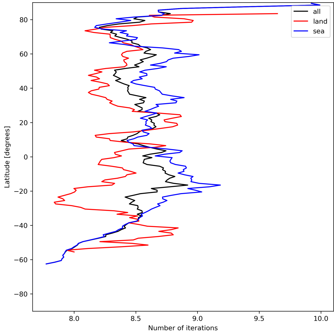
Figure 16: Zonal average of “Number of iterations” for 2024-07-10 to 2024-07-12.
