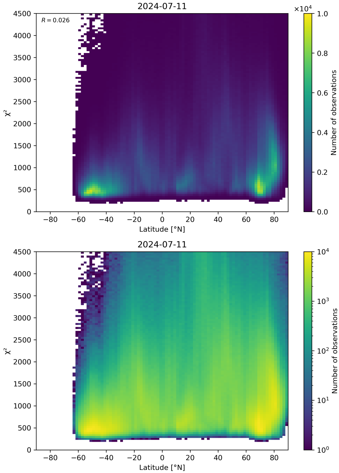
Figure 54: Scatter density plot of “Latitude” against “ \chi^2 ” for 2024-07-10 to 2024-07-12.
