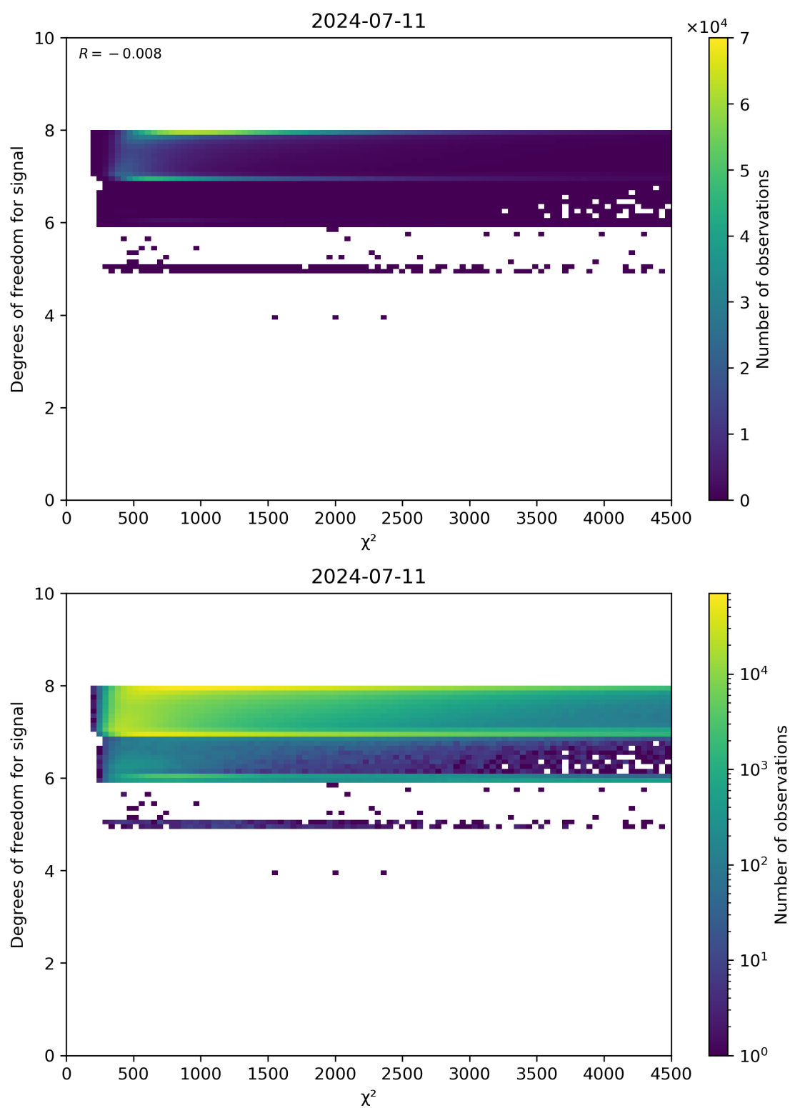
Figure 48: Scatter density plot of " \chi^2 " against "Degrees of freedom for signal" for 2024-07-10 to 2024-07-12.
