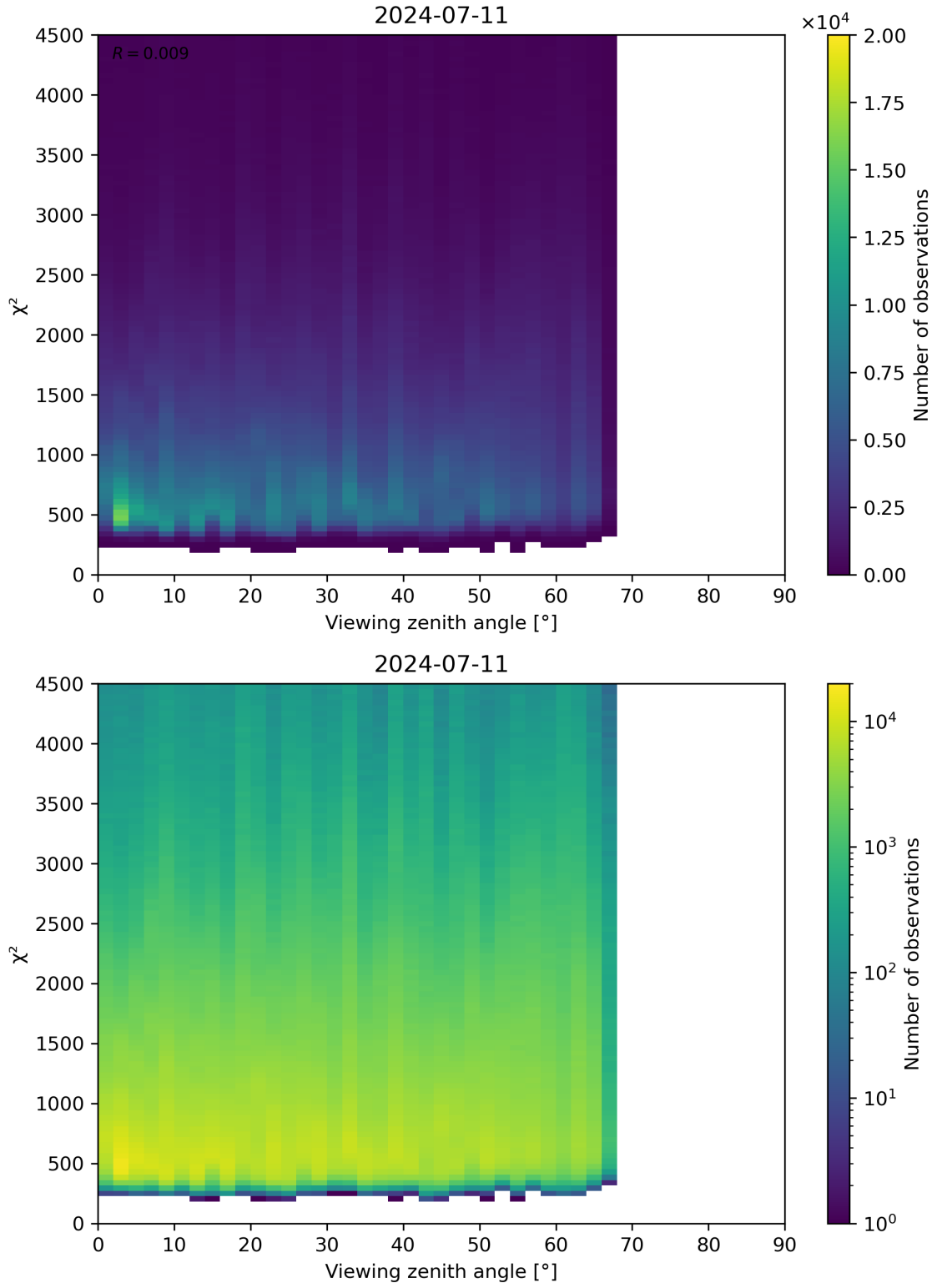
Figure 72: Scatter density plot of “Viewing zenith angle” against “ \chi^2 ” for 2024-07-10 to 2024-07-12.
