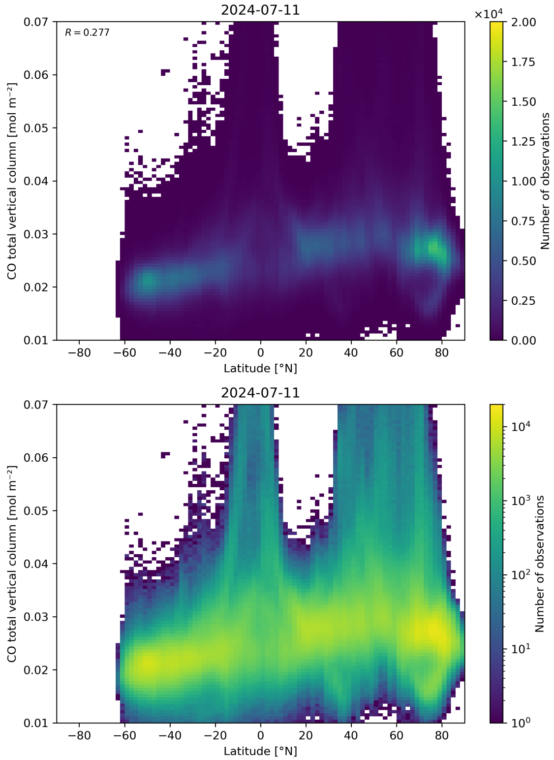
Figure 51: Scatter density plot of “Latitude” against “CO total vertical column” for 2024-07-10 to 2024-07-12.
