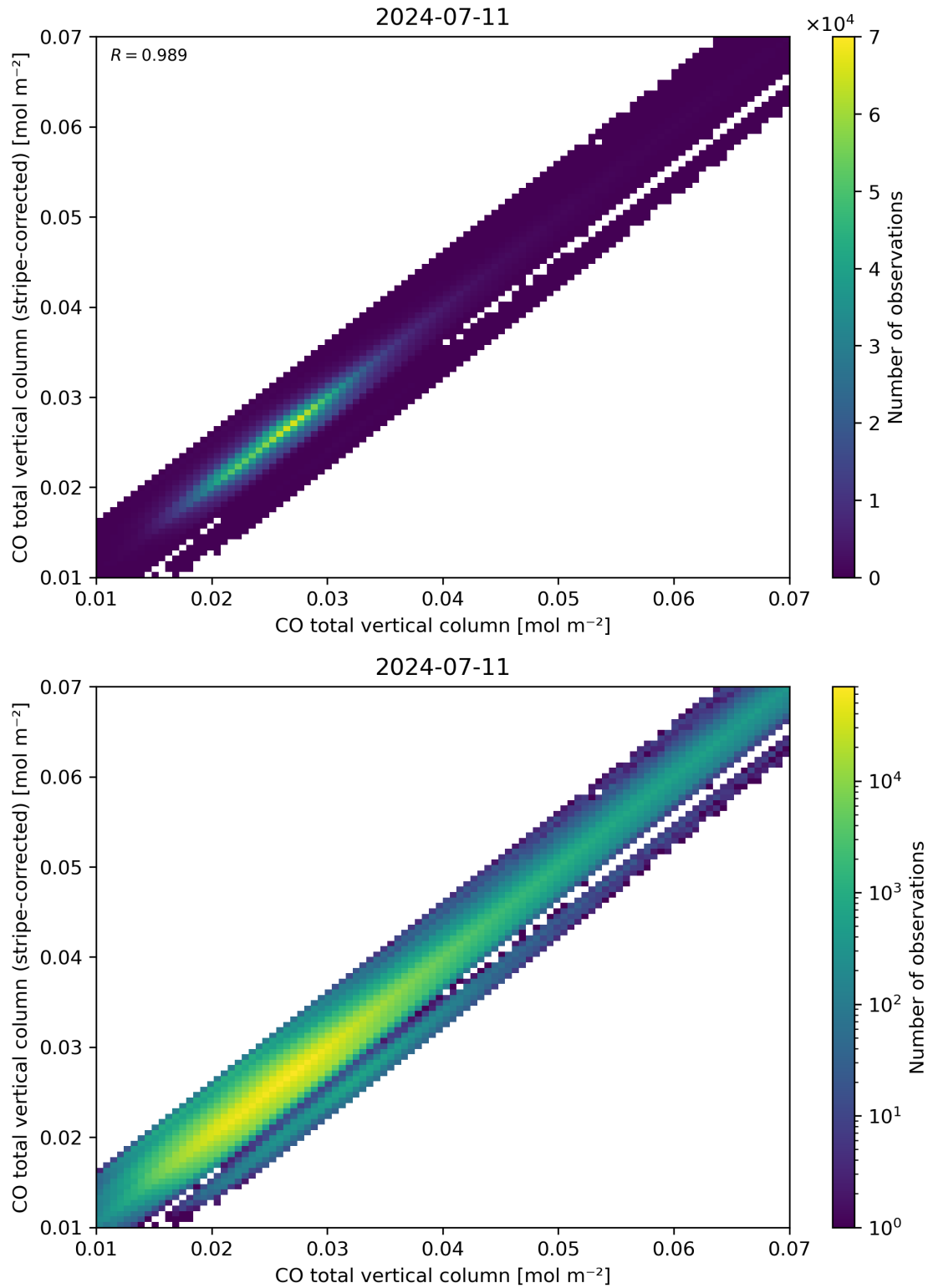
Figure 33: Scatter density plot of “CO total vertical column” against “CO total vertical column (stripe-corrected)” for 2024-07-10 to 2024-07-12.
