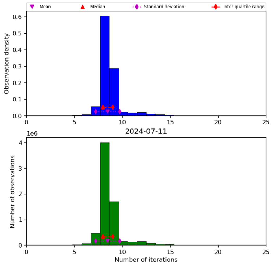
Figure 24: Histogram of “Number of iterations” for 2024-07-10 to 2024-07-12
