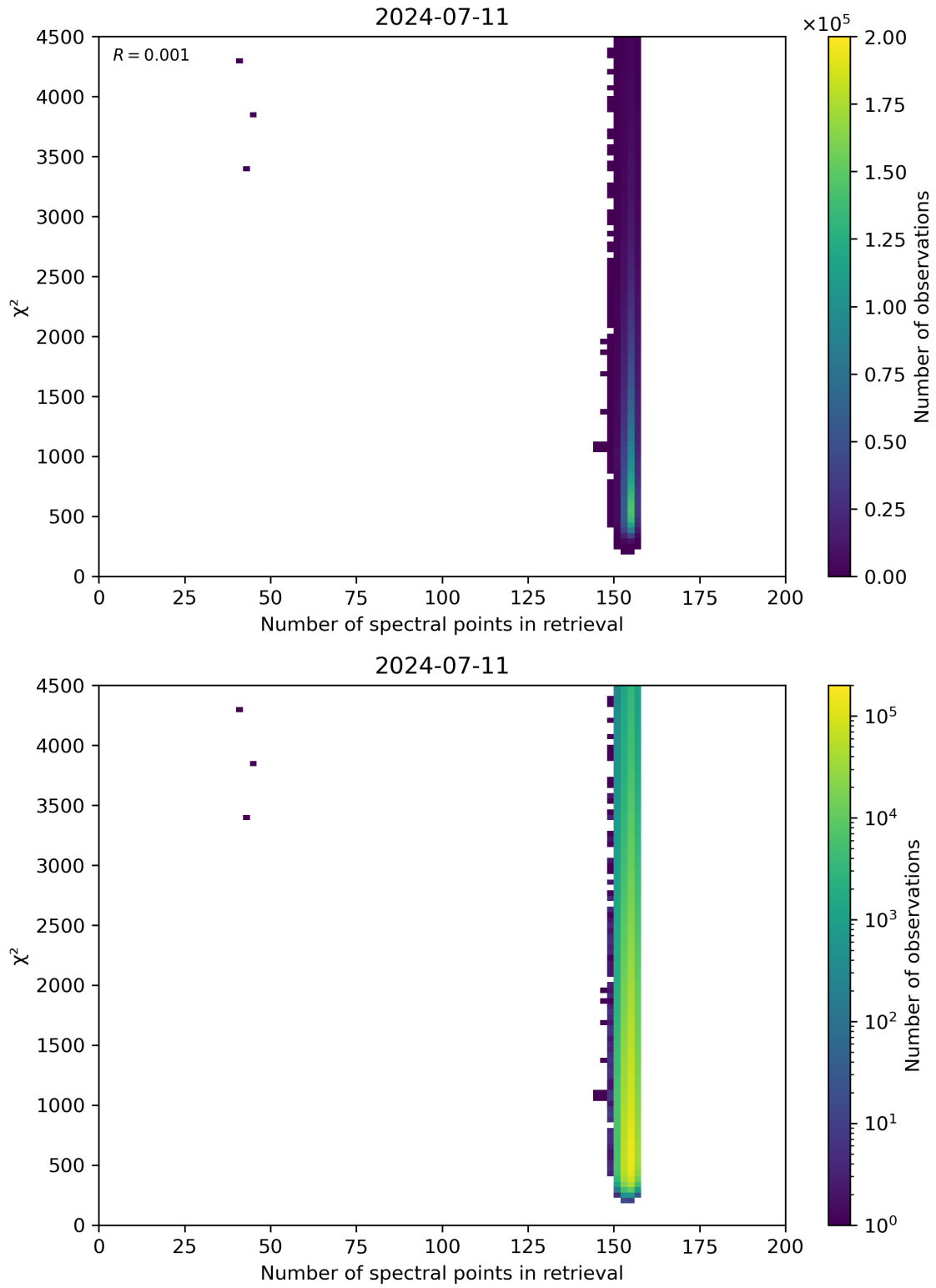
Figure 58: Scatter density plot of “Number of spectral points in retrieval” against “ \chi^2 ” for 2024-07-10 to 2024-07-12.
