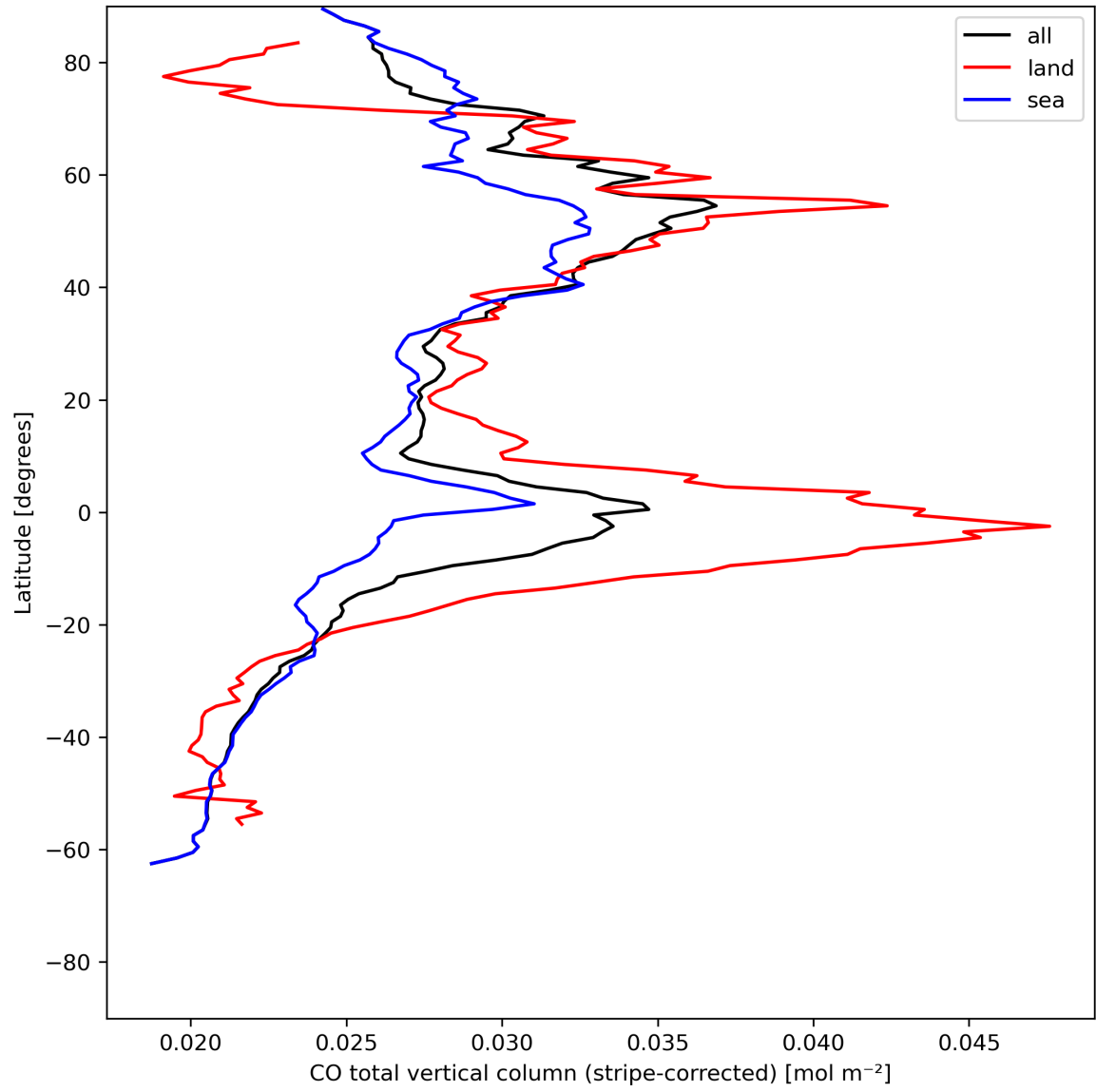
Figure 11: Zonal average of “CO total vertical column (stripe-corrected)” for 2024-07-10 to 2024-07-12.
