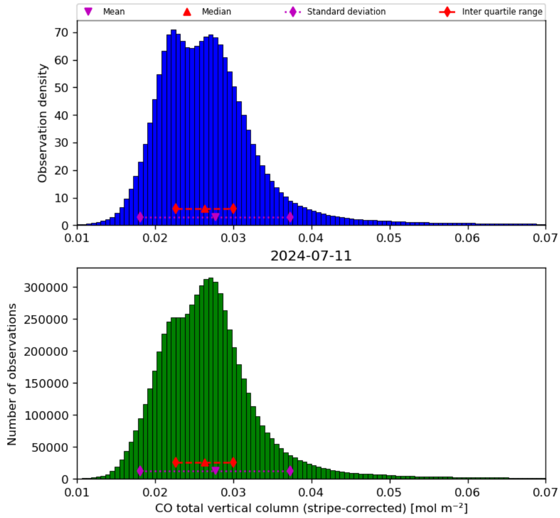
Figure 19: Histogram of “CO total vertical column (stripe-corrected)” for 2024-07-10 to 2024-07-12
