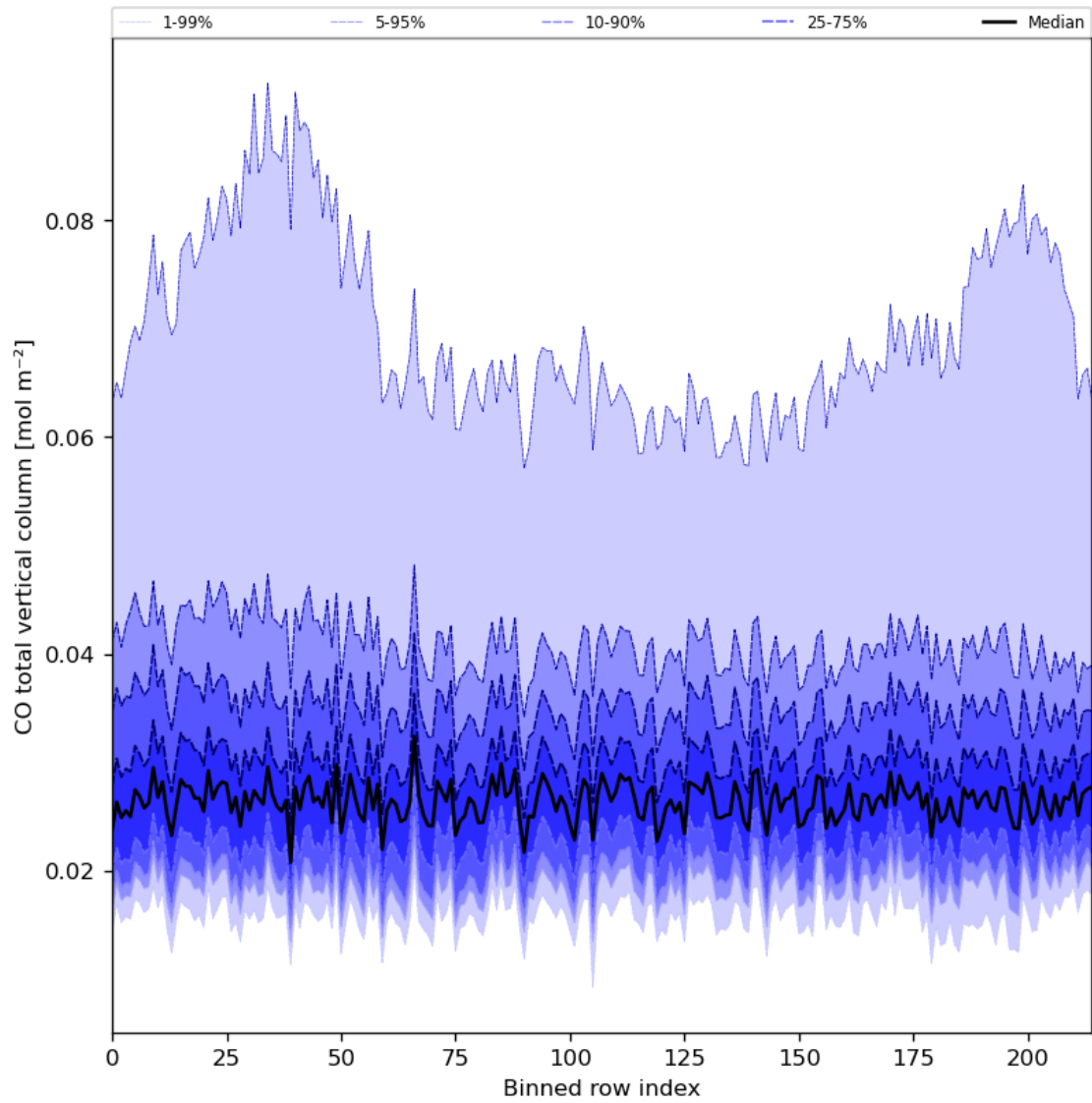
Figure 26: Along track statistics of “CO total vertical column” for 2024-07-10 to 2024-07-12
