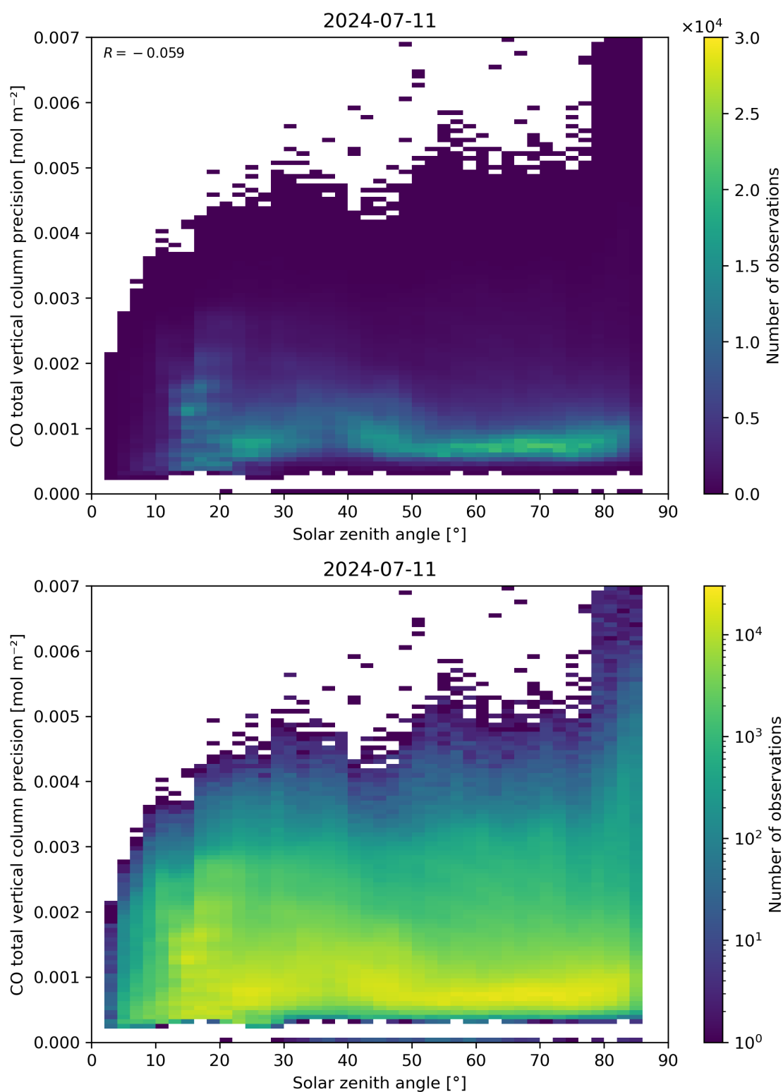
Figure 63: Scatter density plot of “Solar zenith angle” against “CO total vertical column precision” for 2024-07-10 to 2024-07-12.
