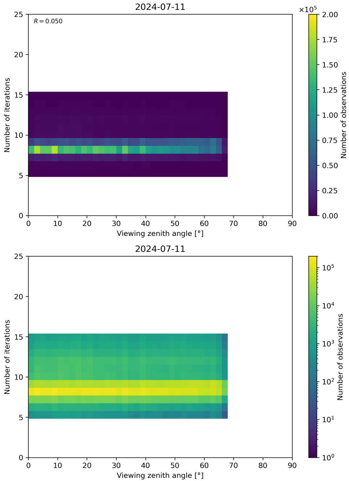
Figure 75: Scatter density plot of “Viewing zenith angle” against “Number of iterations” for 2024-07-10 to 2024-07-12.
