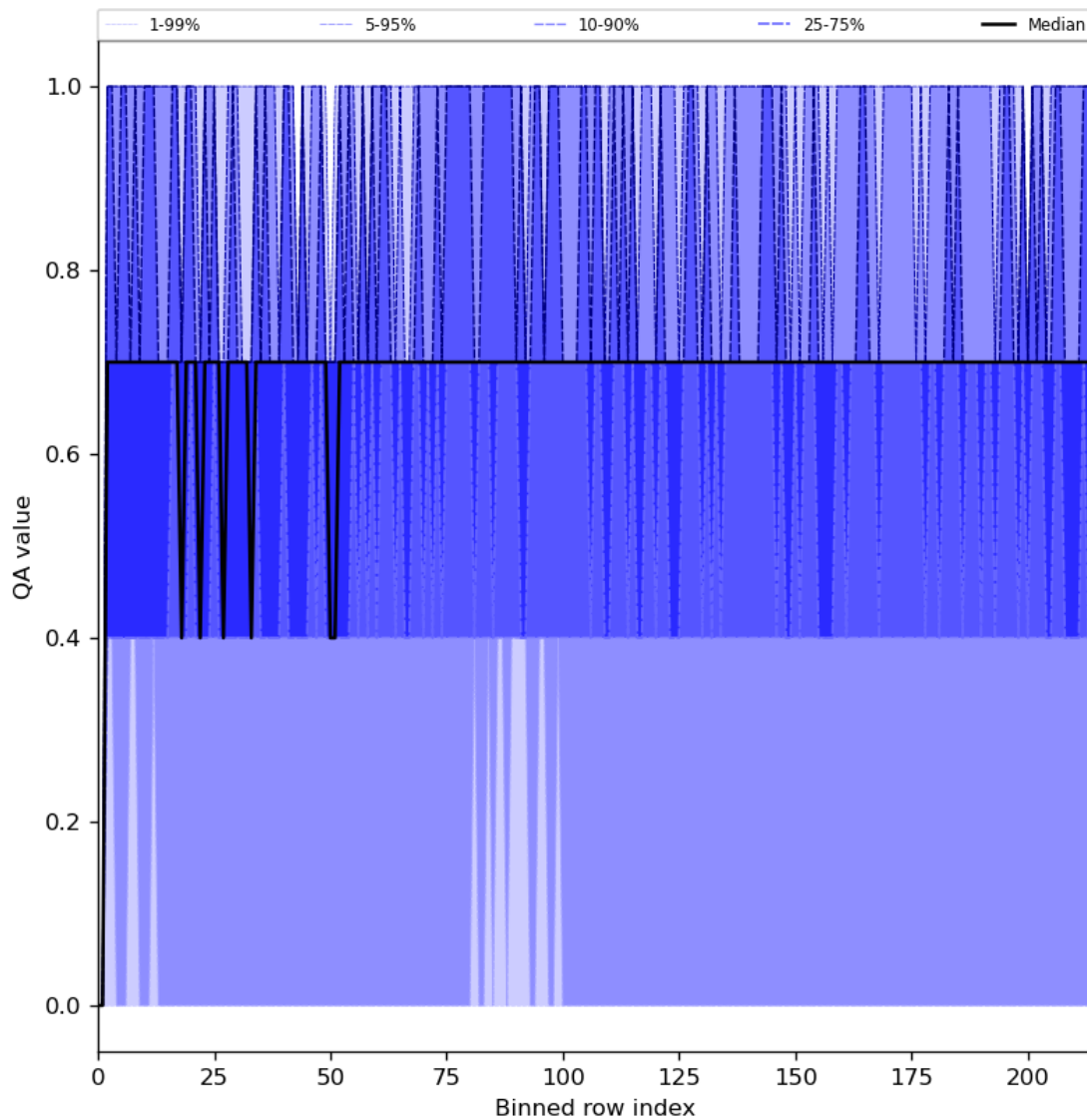
Figure 25: Along track statistics of “QA value” for 2024-07-10 to 2024-07-12
