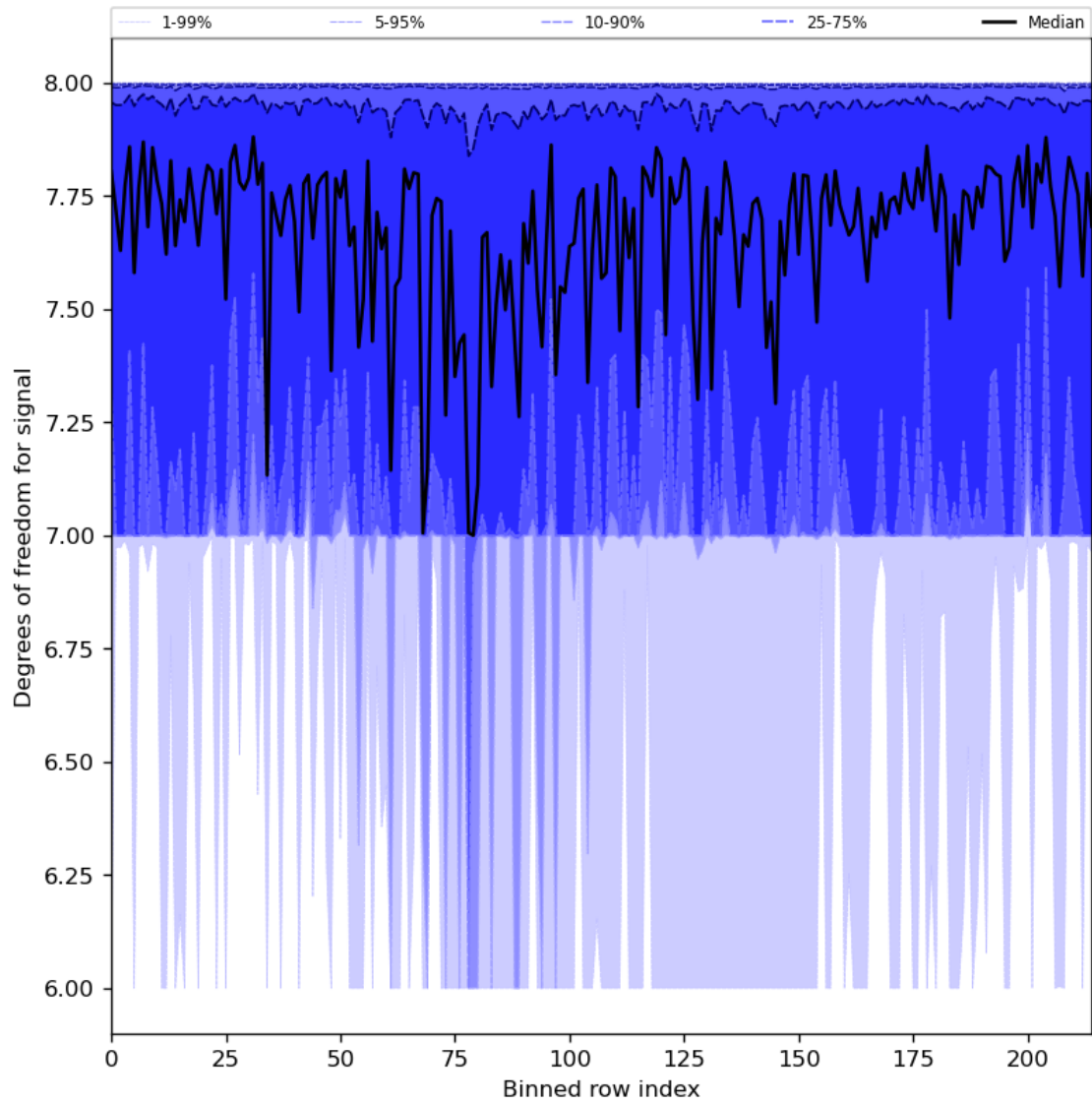
Figure 31: Along track statistics of “Degrees of freedom for signal” for 2024-07-10 to 2024-07-12
