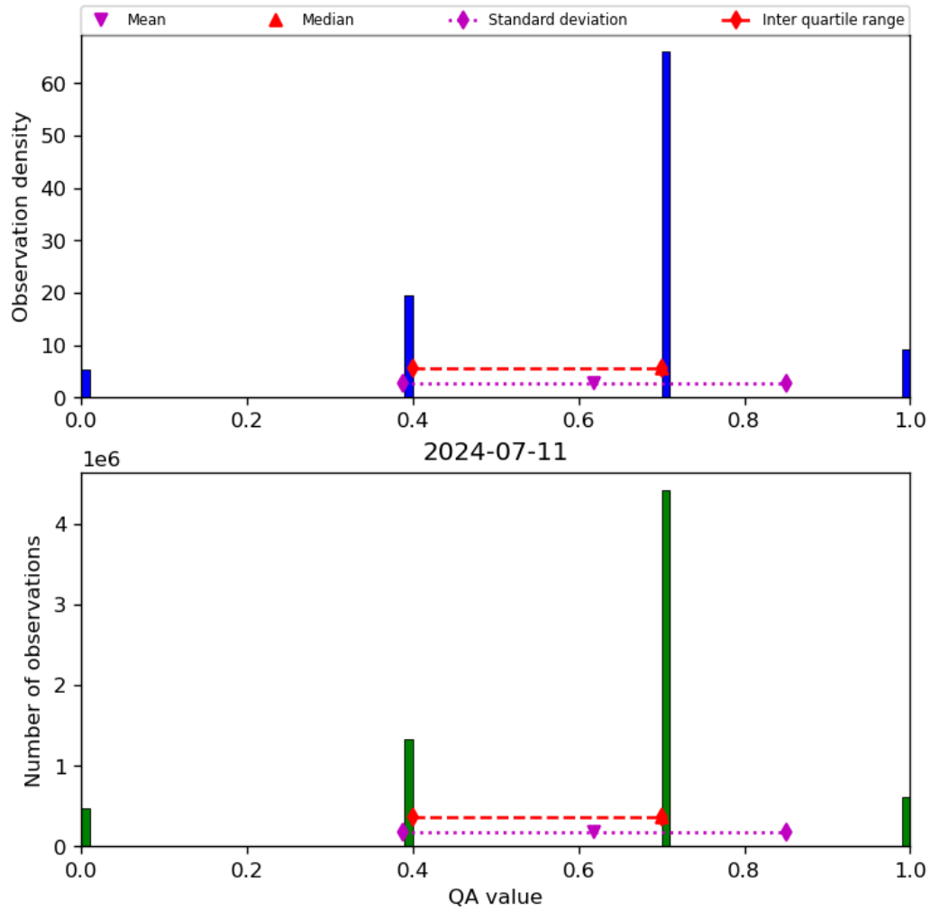
Figure 17: Histogram of “QA value” for 2024-07-10 to 2024-07-12
