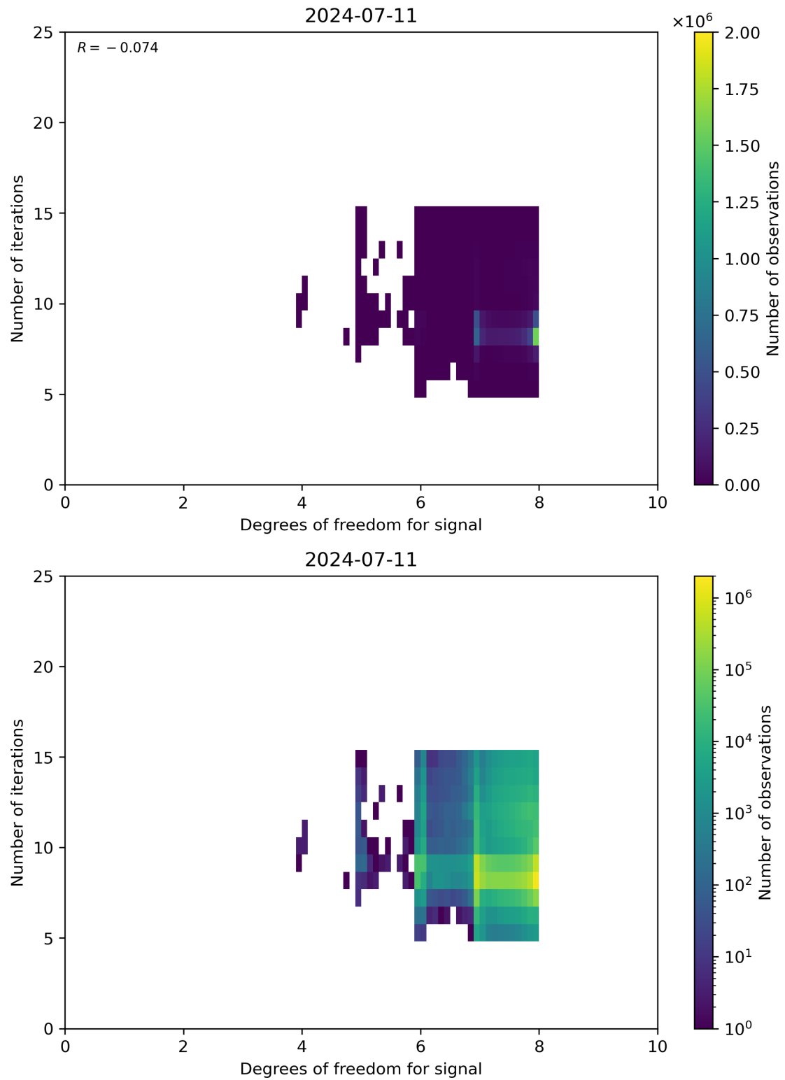
Figure 50: Scatter density plot of “Degrees of freedom for signal” against “Number of iterations” for 2024-07-10 to 2024-07-12.
