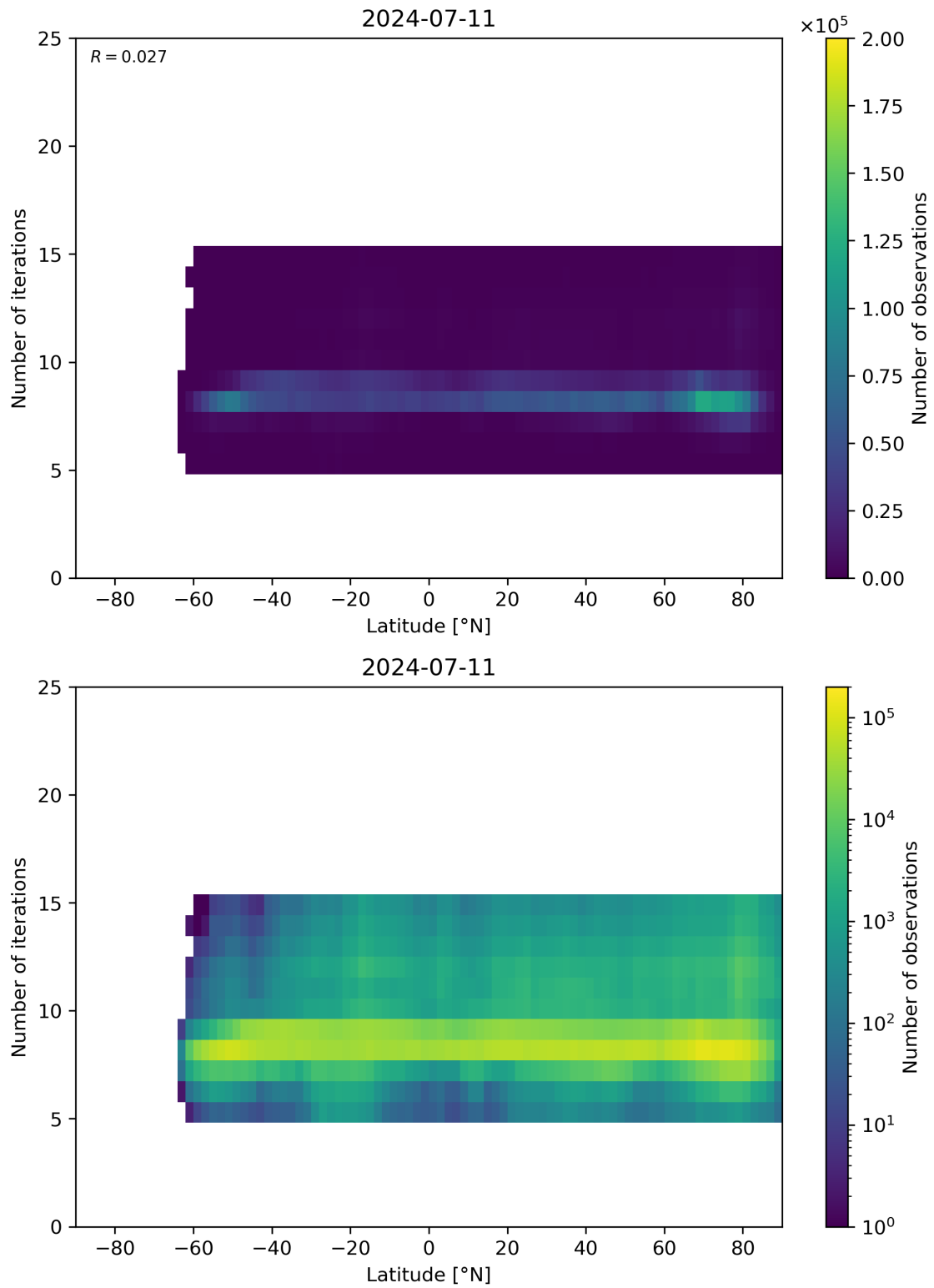
Figure 56: Scatter density plot of “Latitude” against “Number of iterations” for 2024-07-10 to 2024-07-12.
