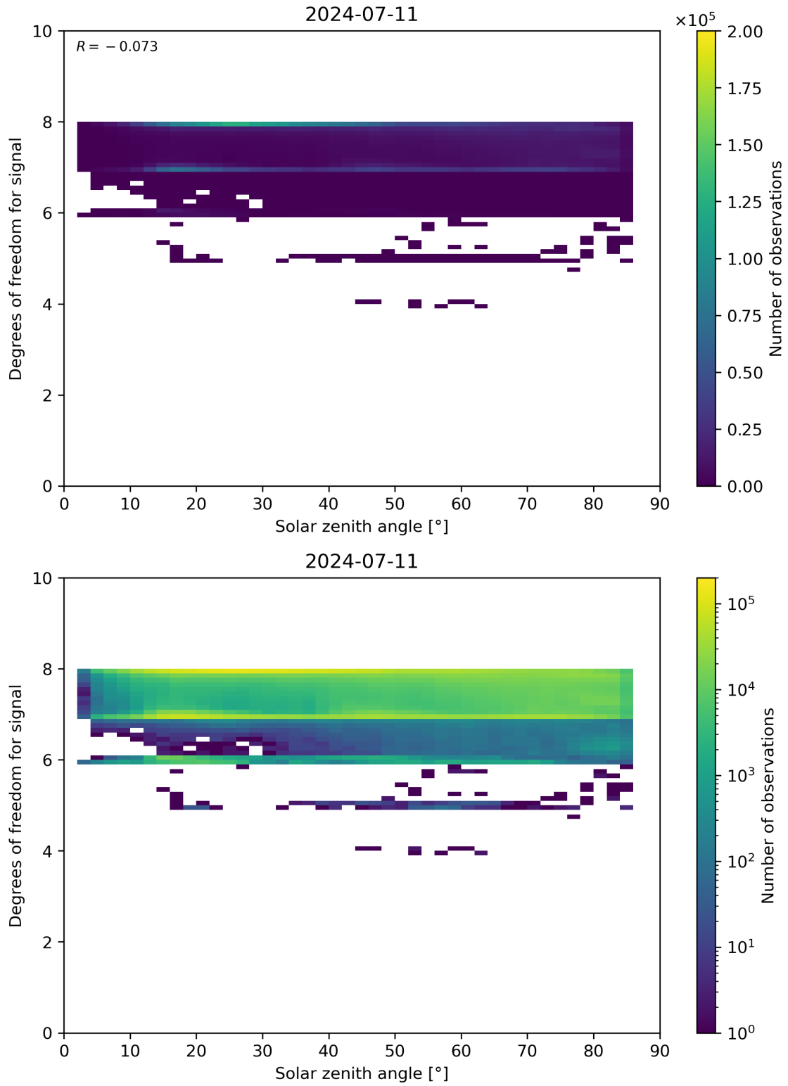
Figure 65: Scatter density plot of “Solar zenith angle” against “Degrees of freedom for signal” for 2024-07-10 to 2024-07-12.
