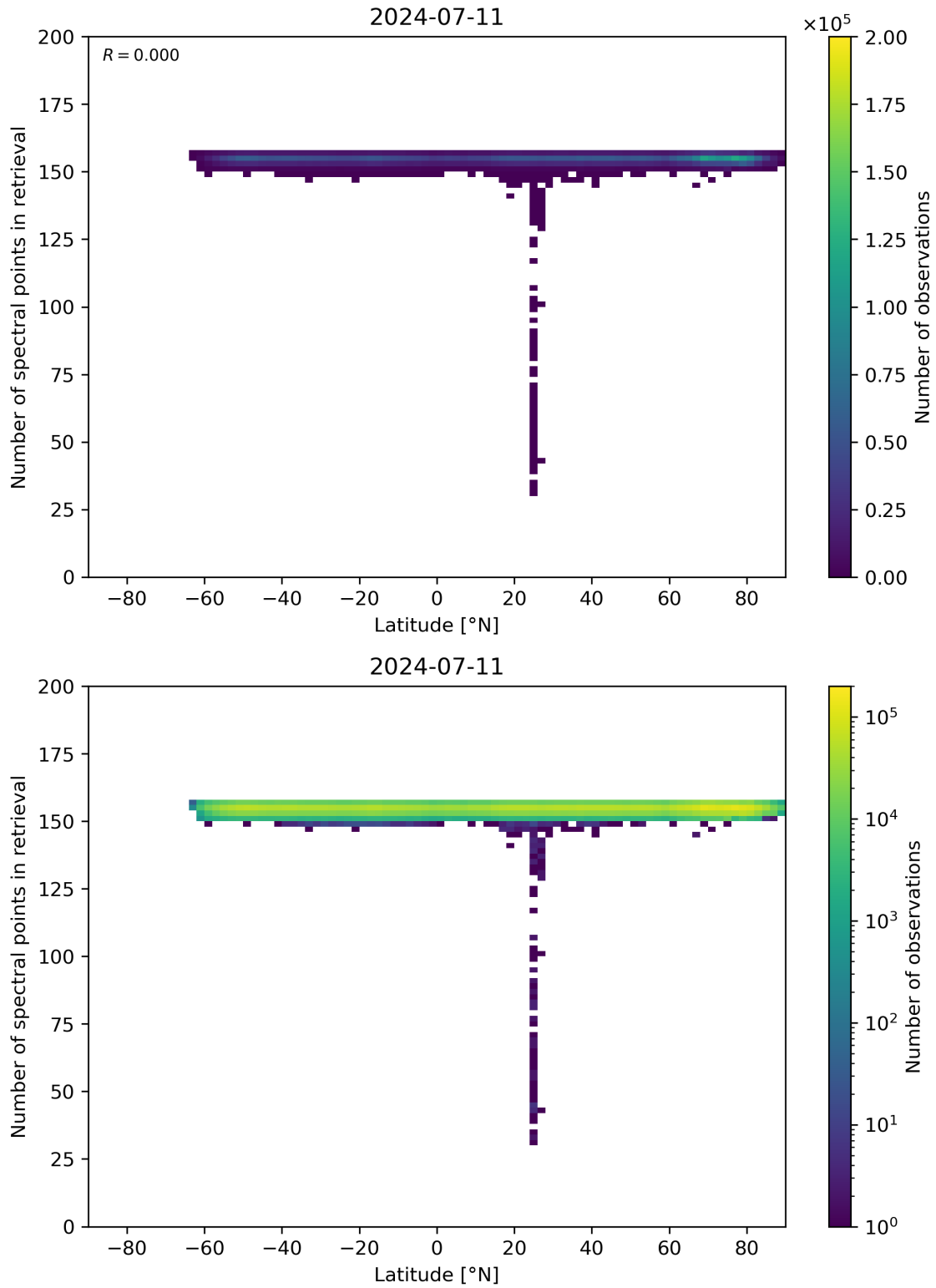
Figure 57: Scatter density plot of “Latitude” against “Number of spectral points in retrieval” for 2024-07-10 to 2024-07-12.
