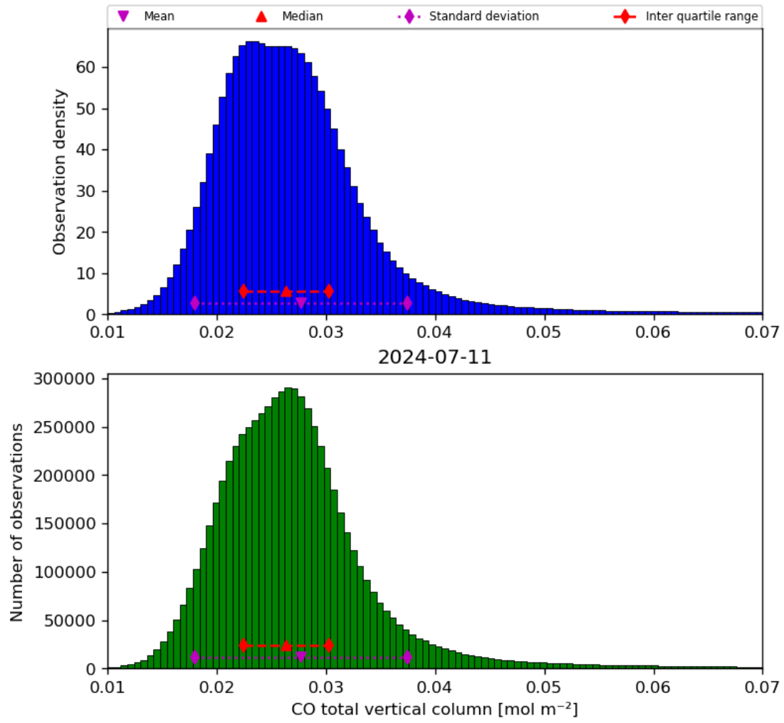
Figure 18: Histogram of “CO total vertical column” for 2024-07-10 to 2024-07-12
