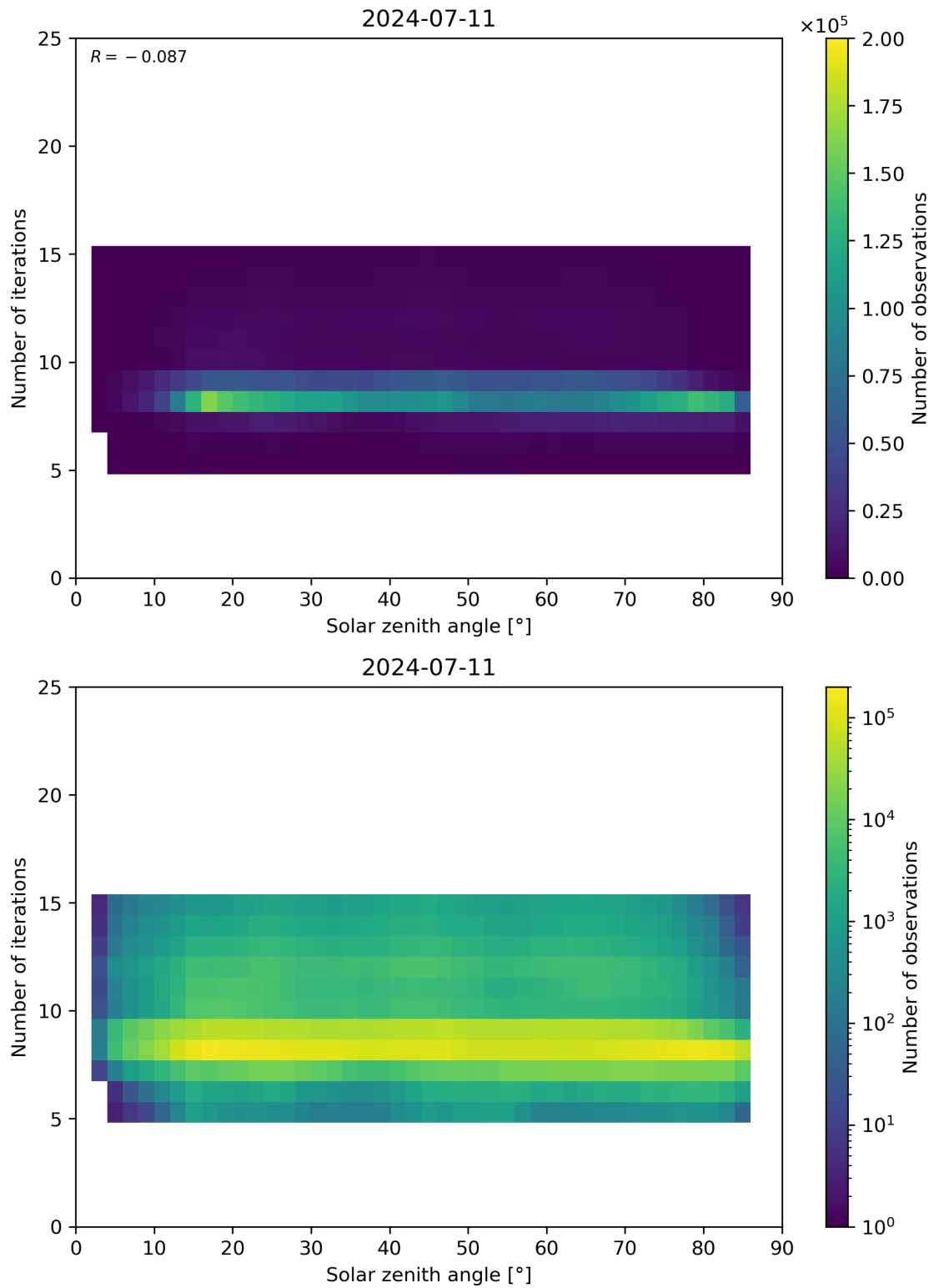
Figure 67: Scatter density plot of “Solar zenith angle” against “Number of iterations” for 2024-07-10 to 2024-07-12.
