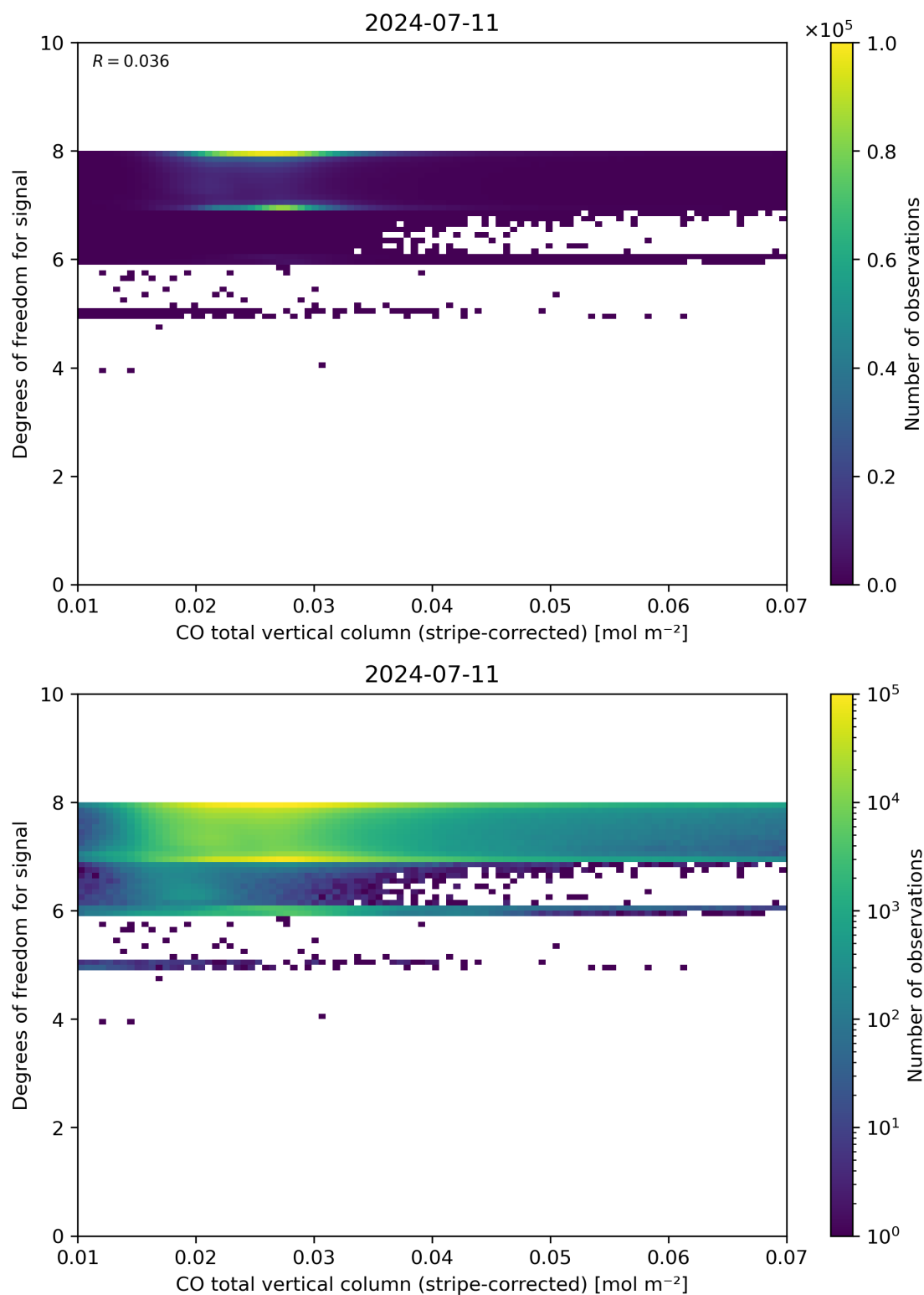
Figure 38: Scatter density plot of “CO total vertical column (stripe-corrected)” against “Degrees of freedom for signal” for 2024-07-10 to 2024-07-12.
