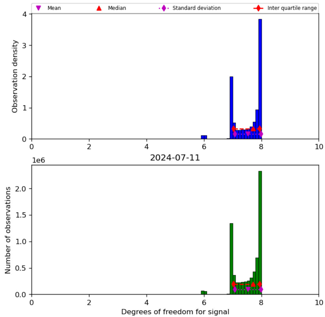
Figure 23: Histogram of “Degrees of freedom for signal” for 2024-07-10 to 2024-07-12
