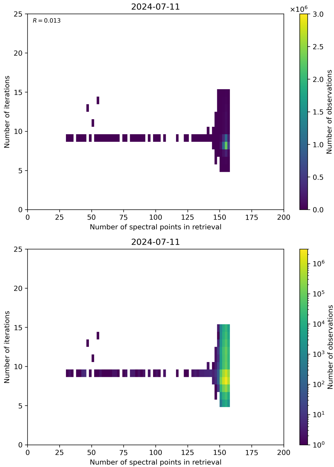
Figure 60: Scatter density plot of “Number of spectral points in retrieval” against “Number of iterations” for 2024-07-10 to 2024-07-12.
