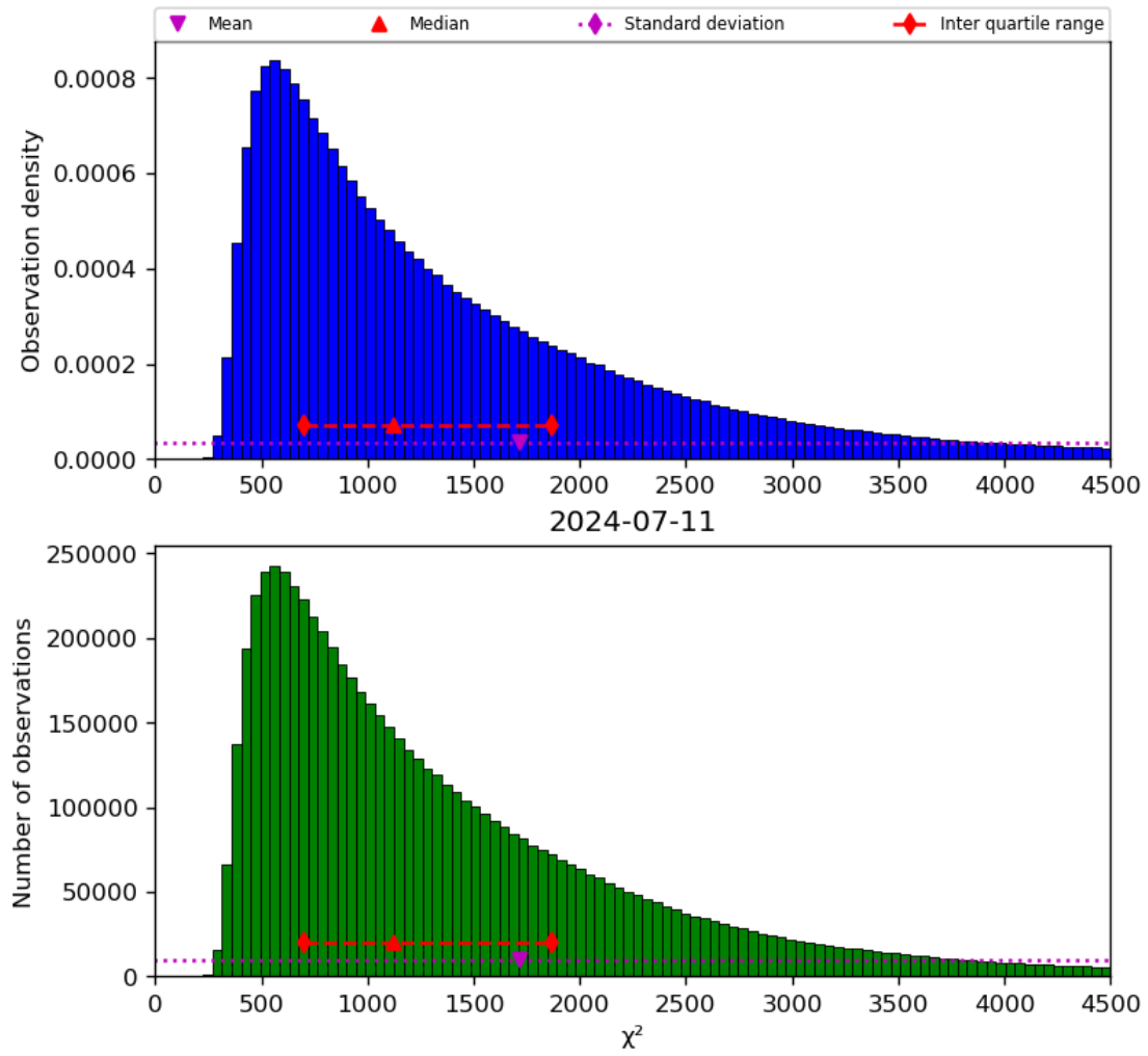
Figure 22: Histogram of “ \chi^2 ” for 2024-07-10 to 2024-07-12
