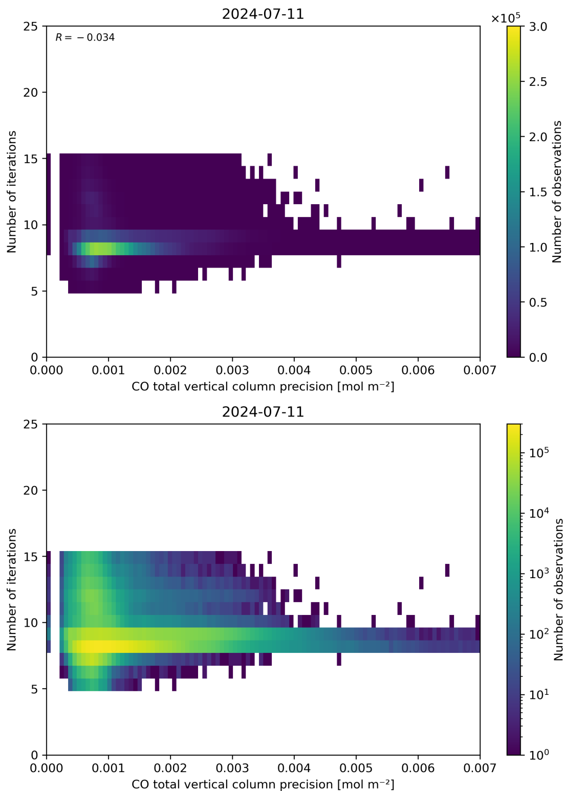
Figure 46: Scatter density plot of “CO total vertical column precision” against “Number of iterations” for 2024-07-10 to 2024-07-12.
