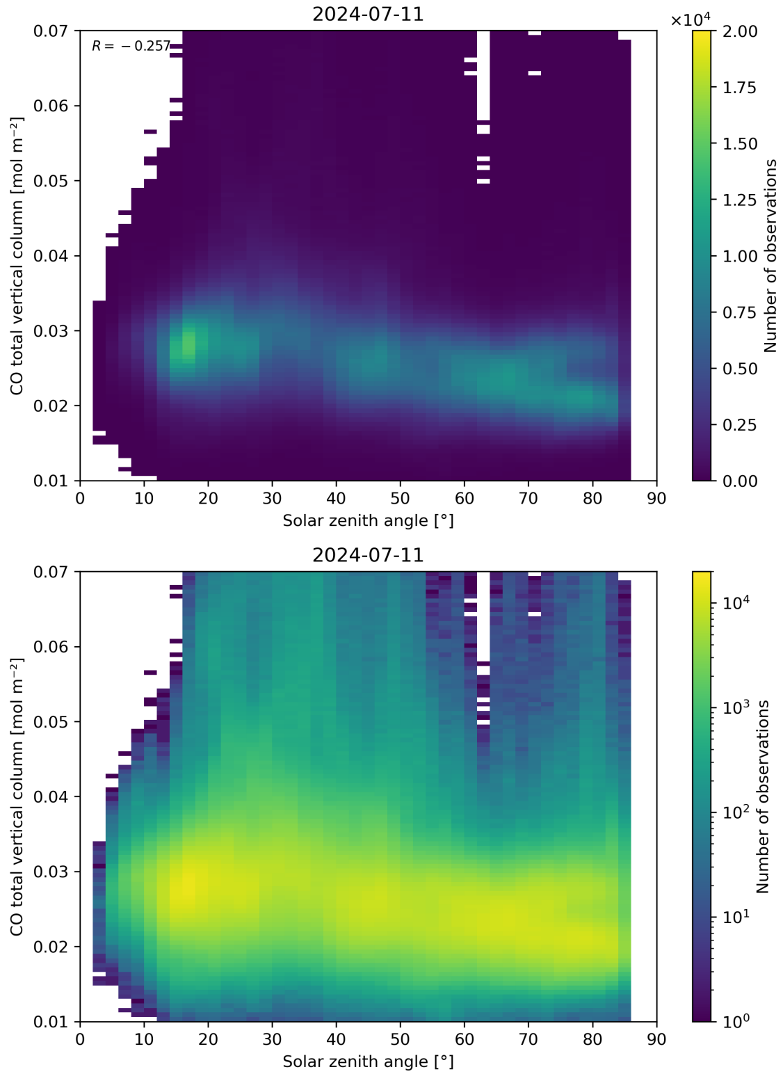
Figure 61: Scatter density plot of “Solar zenith angle” against “CO total vertical column” for 2024-07-10 to 2024-07-12.
