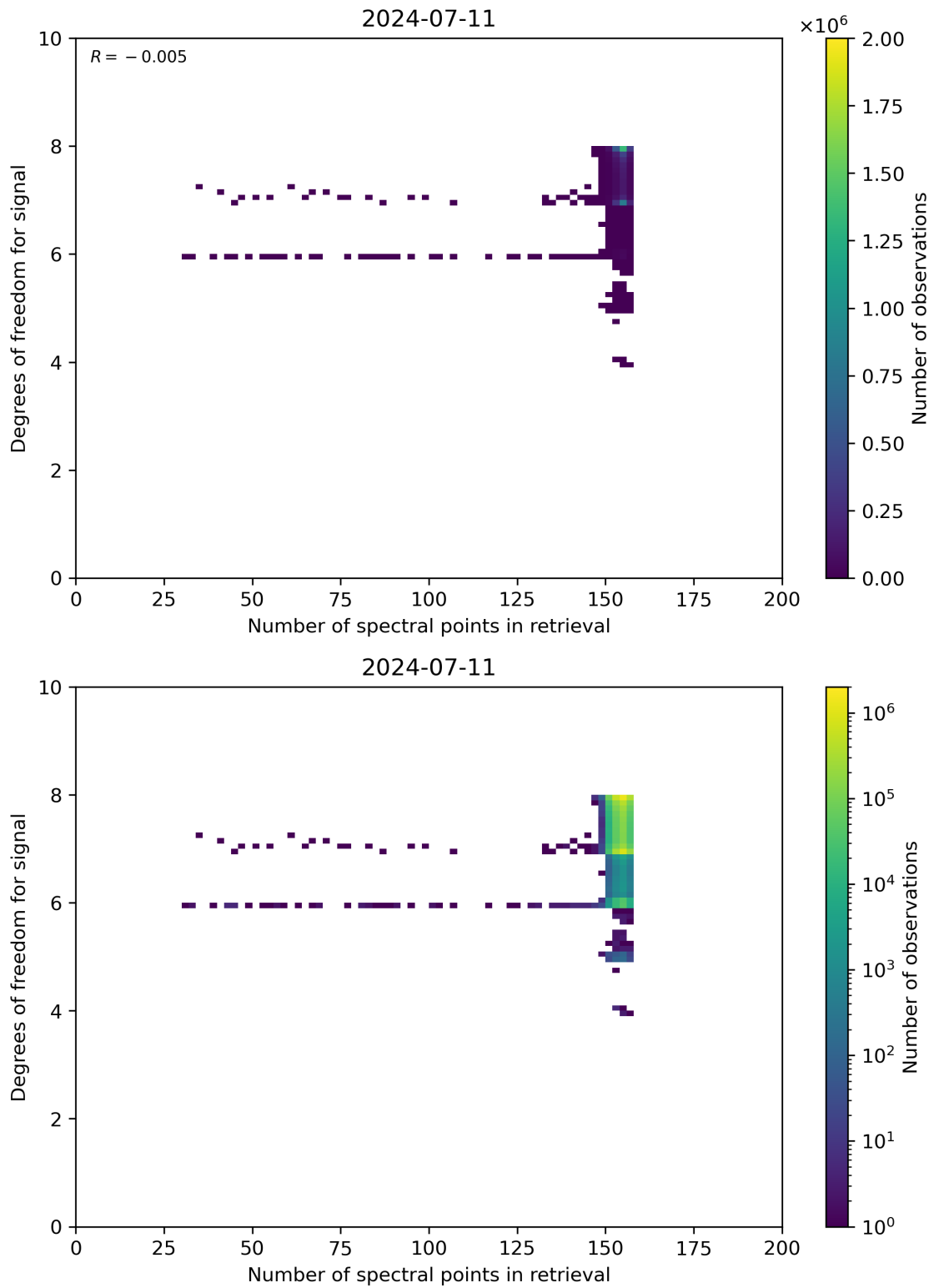
Figure 59: Scatter density plot of “Number of spectral points in retrieval” against “Degrees of freedom for signal” for 2024-07-10 to 2024-07-12.
