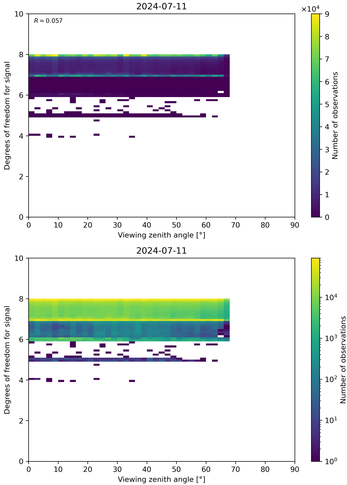
Figure 73: Scatter density plot of “Viewing zenith angle” against “Degrees of freedom for signal” for 2024-07-10 to 2024-07-12.
