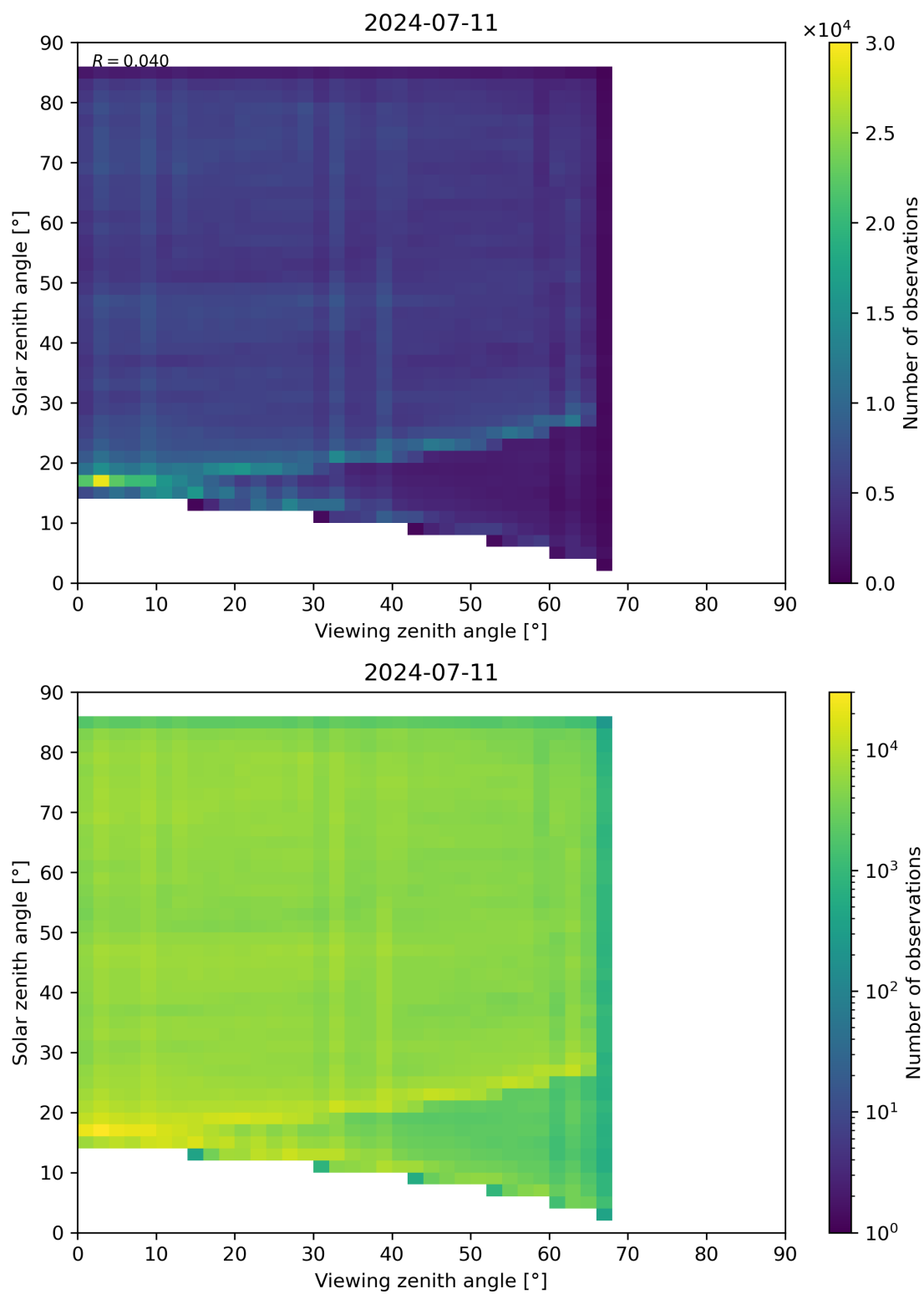
Figure 77: Scatter density plot of “Viewing zenith angle” against “Solar zenith angle” for 2024-07-10 to 2024-07-12.
