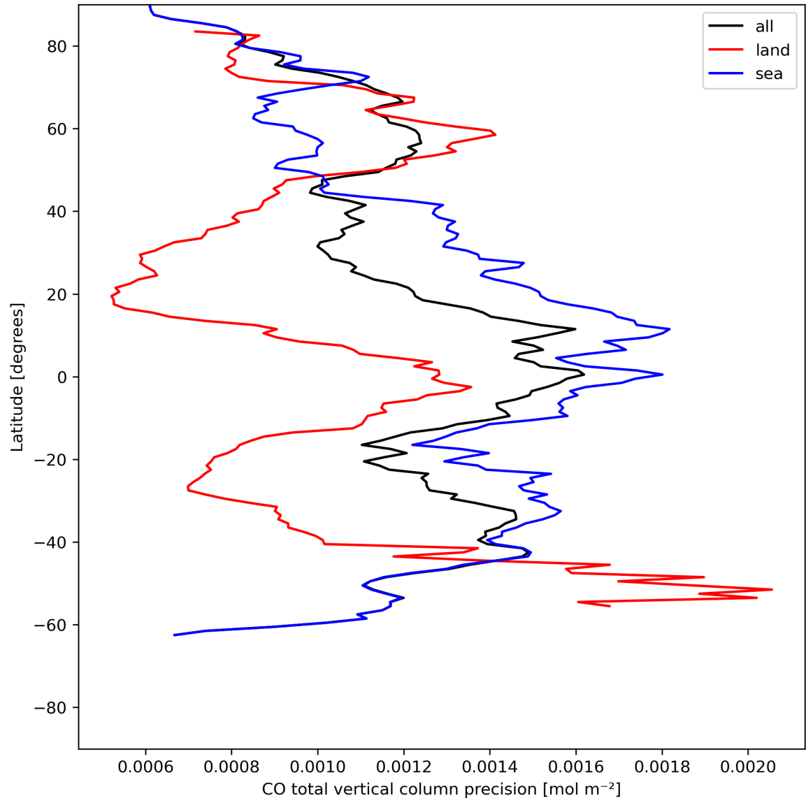
Figure 12: Zonal average of “CO total vertical column precision” for 2024-07-10 to 2024-07-12.
