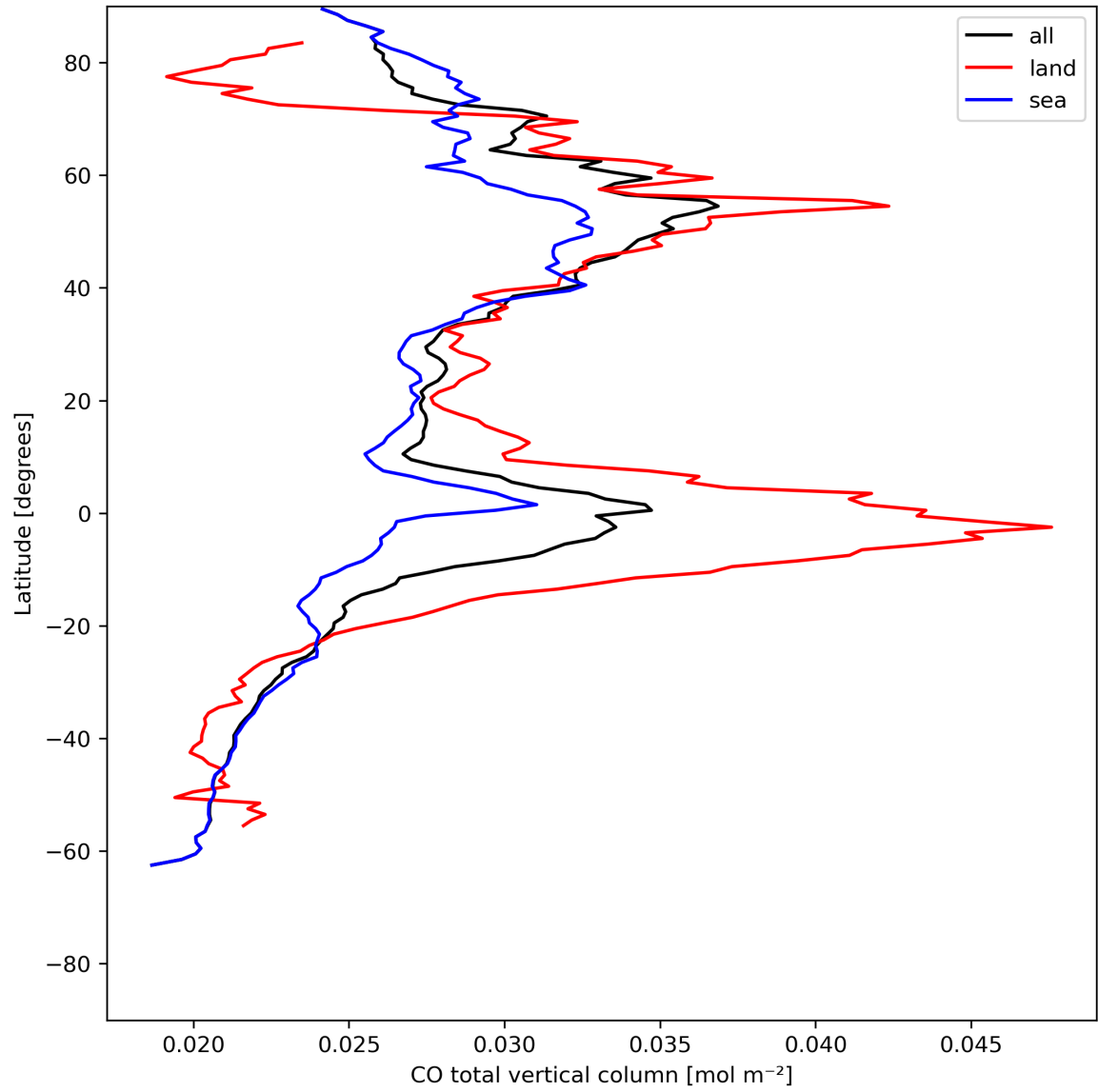
Figure 10: Zonal average of “CO total vertical column” for 2024-07-10 to 2024-07-12.
