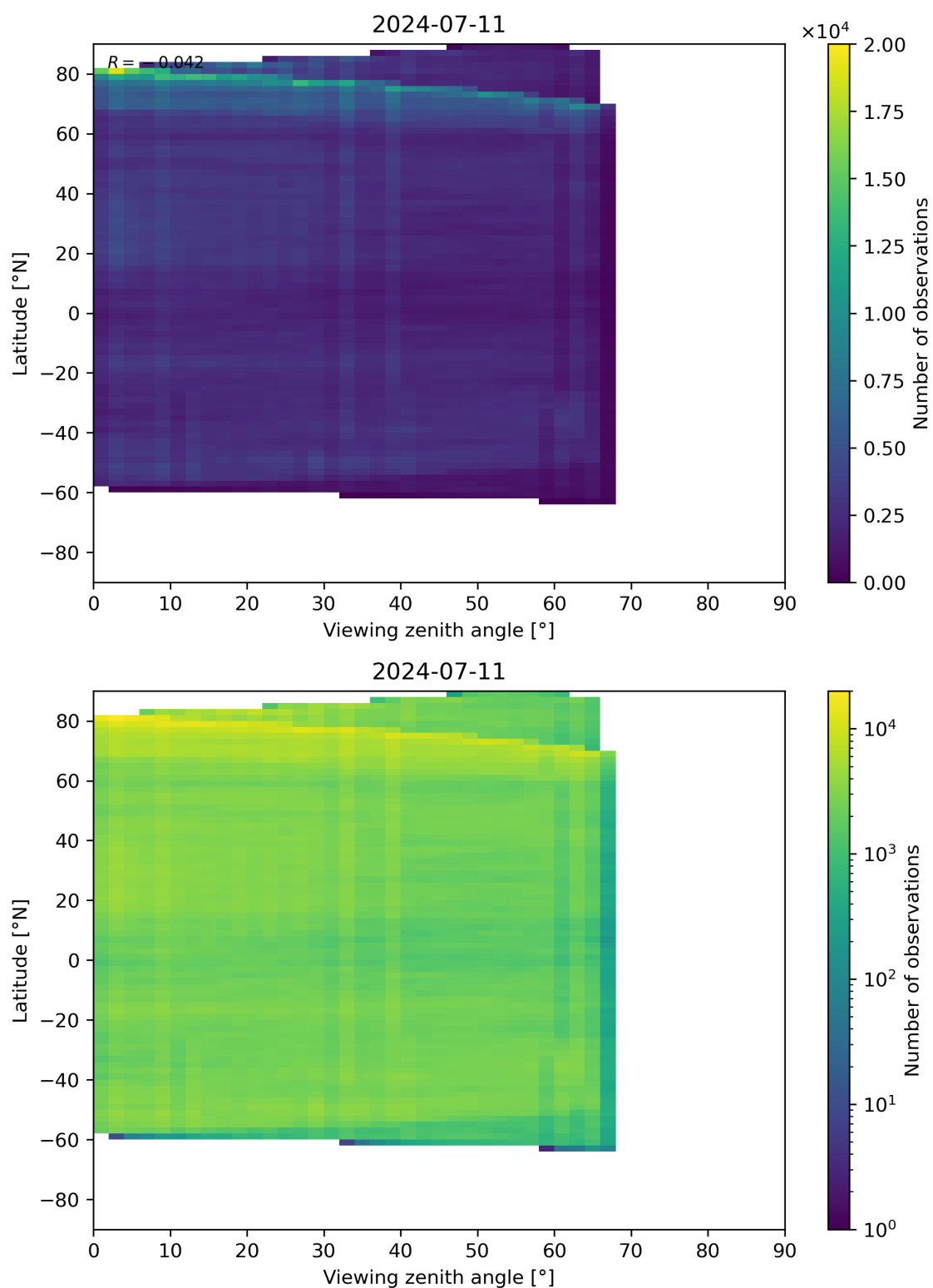
Figure 74: Scatter density plot of “Viewing zenith angle” against “Latitude” for 2024-07-10 to 2024-07-12.
