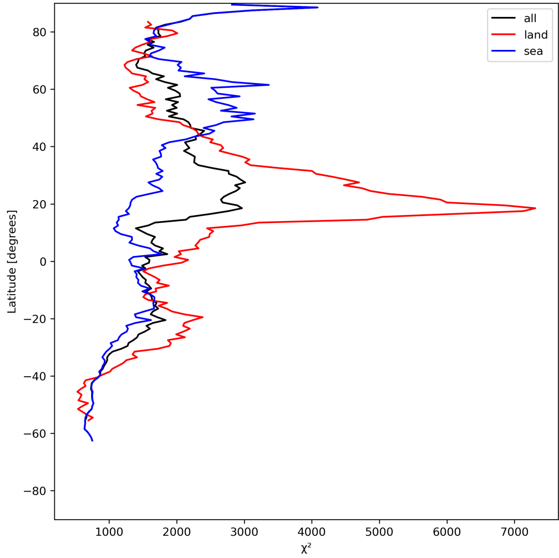
Figure 14: Zonal average of “ \chi^2 ” for 2024-07-10 to 2024-07-12.
