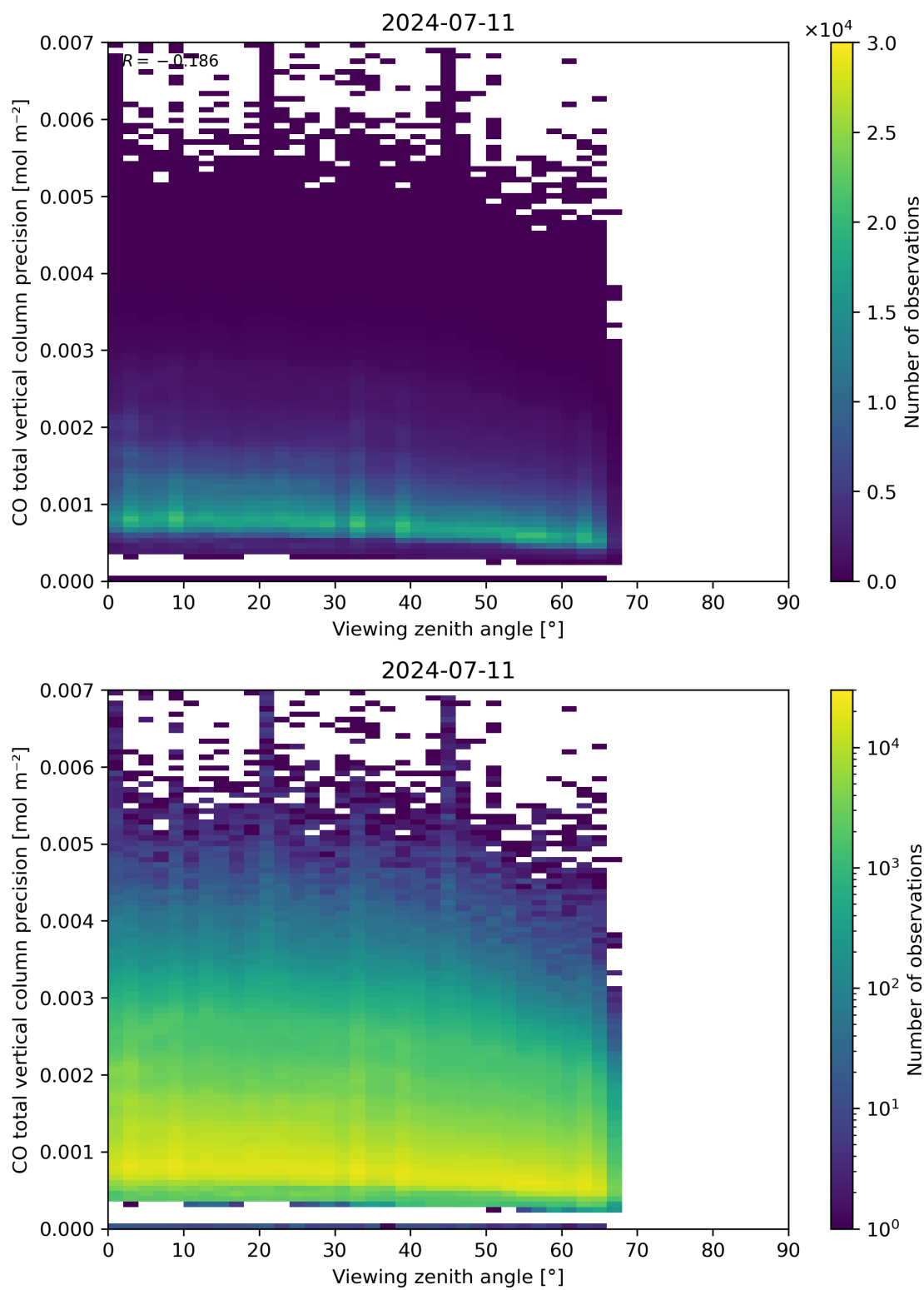
Figure 71: Scatter density plot of “Viewing zenith angle” against “CO total vertical column precision” for 2024-07-10 to 2024-07-12.
