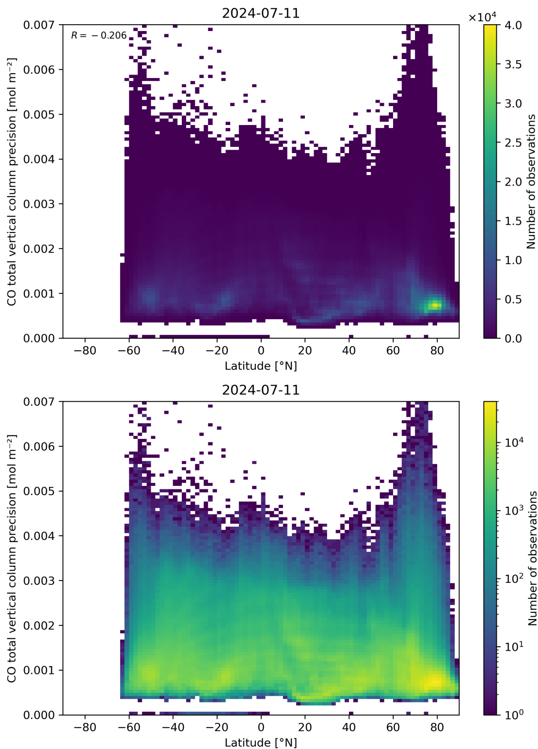
Figure 53: Scatter density plot of “Latitude” against “CO total vertical column precision” for 2024-07-10 to 2024-07-12.
