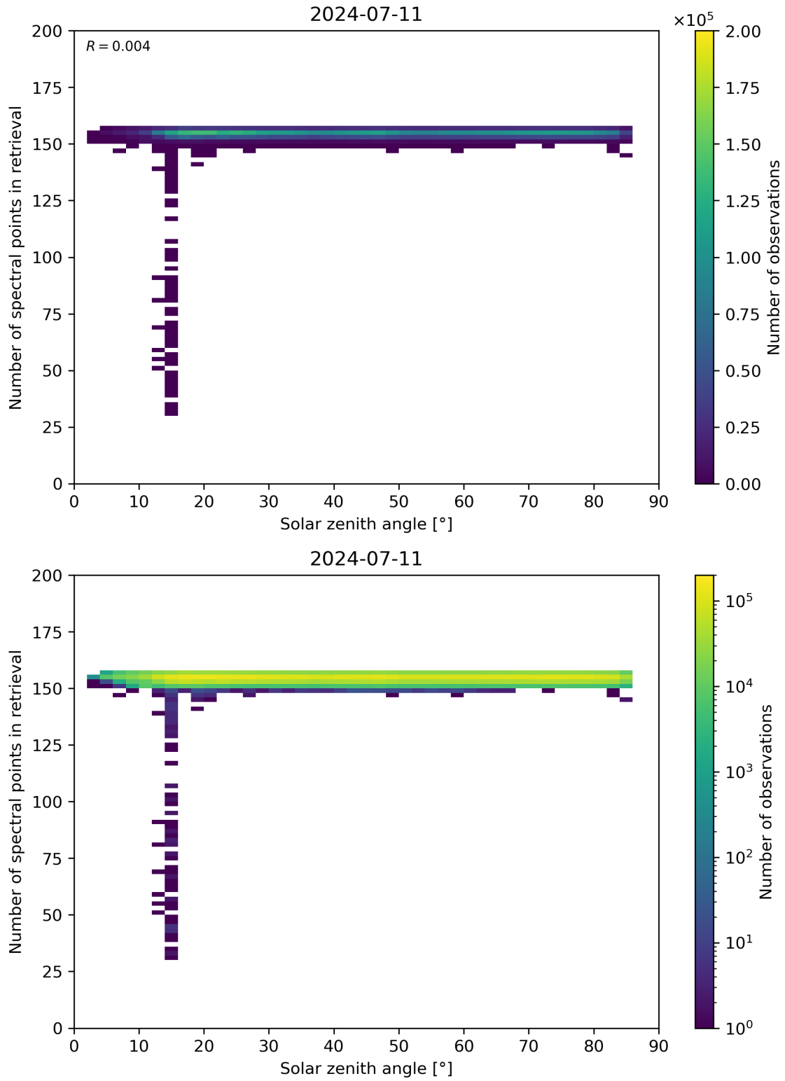
Figure 68: Scatter density plot of “Solar zenith angle” against “Number of spectral points in retrieval” for 2024-07-10 to 2024-07-12.
