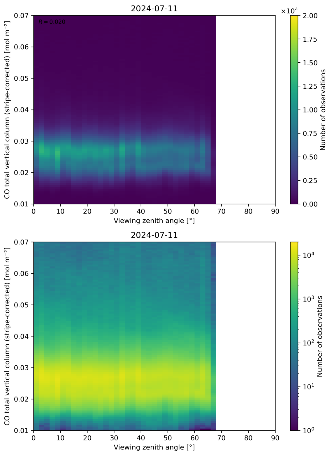
Figure 70: Scatter density plot of “Viewing zenith angle” against “CO total vertical column (stripe-corrected)” for 2024-07-10 to 2024-07-12.
