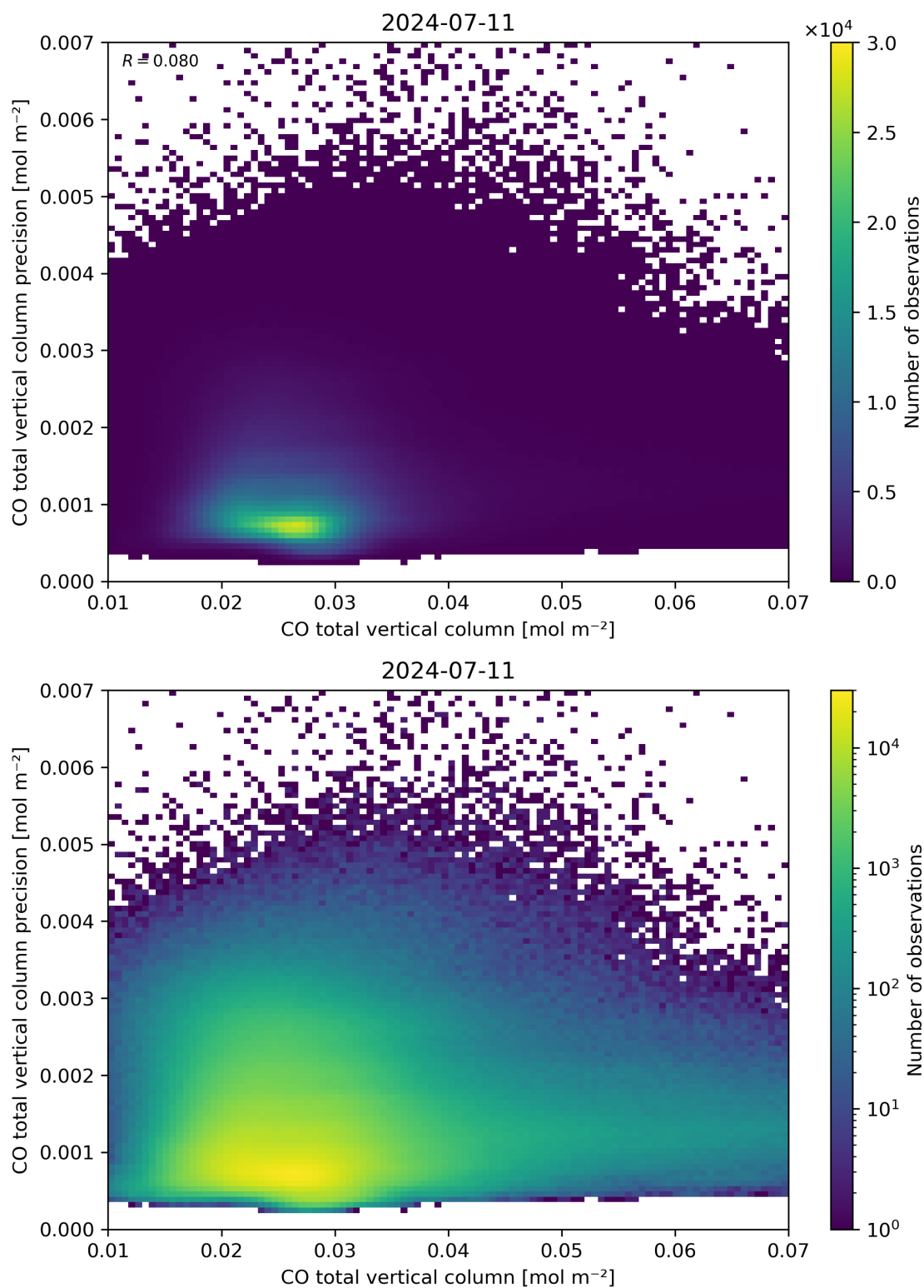
Figure 34: Scatter density plot of “CO total vertical column” against “CO total vertical column precision” for 2024-07-10 to 2024-07-12.
