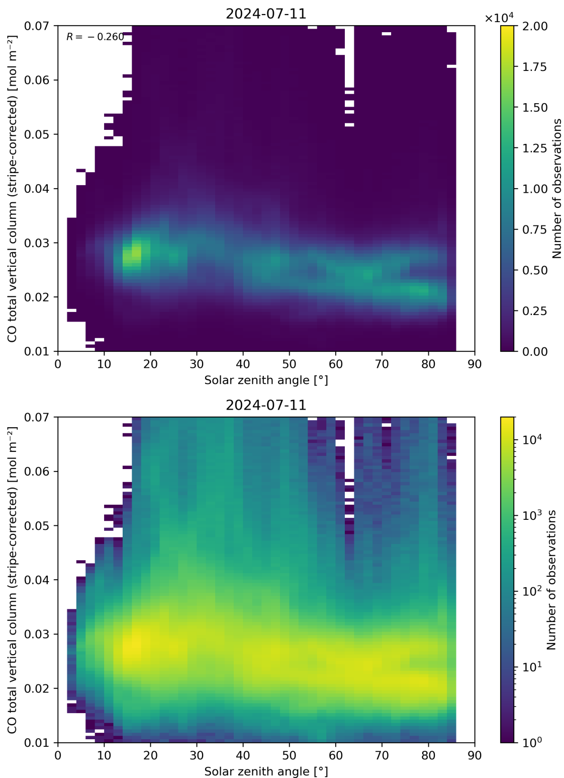
Figure 62: Scatter density plot of “Solar zenith angle” against “CO total vertical column (stripe-corrected)” for 2024-07-10 to 2024-07-12.
