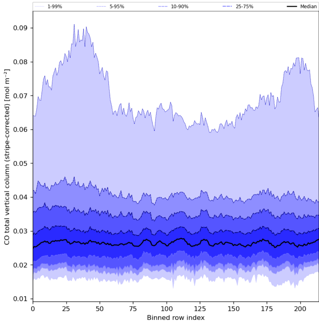
Figure 27: Along track statistics of “CO total vertical column (stripe-corrected)” for 2024-07-10 to 2024-07-12
