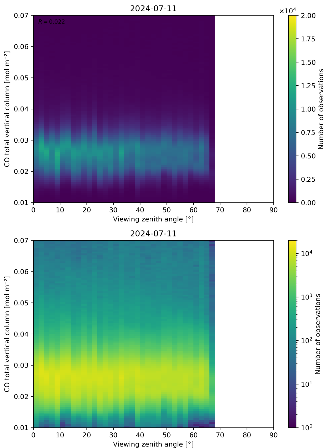
Figure 69: Scatter density plot of “Viewing zenith angle” against “CO total vertical column” for 2024-07-10 to 2024-07-12.
