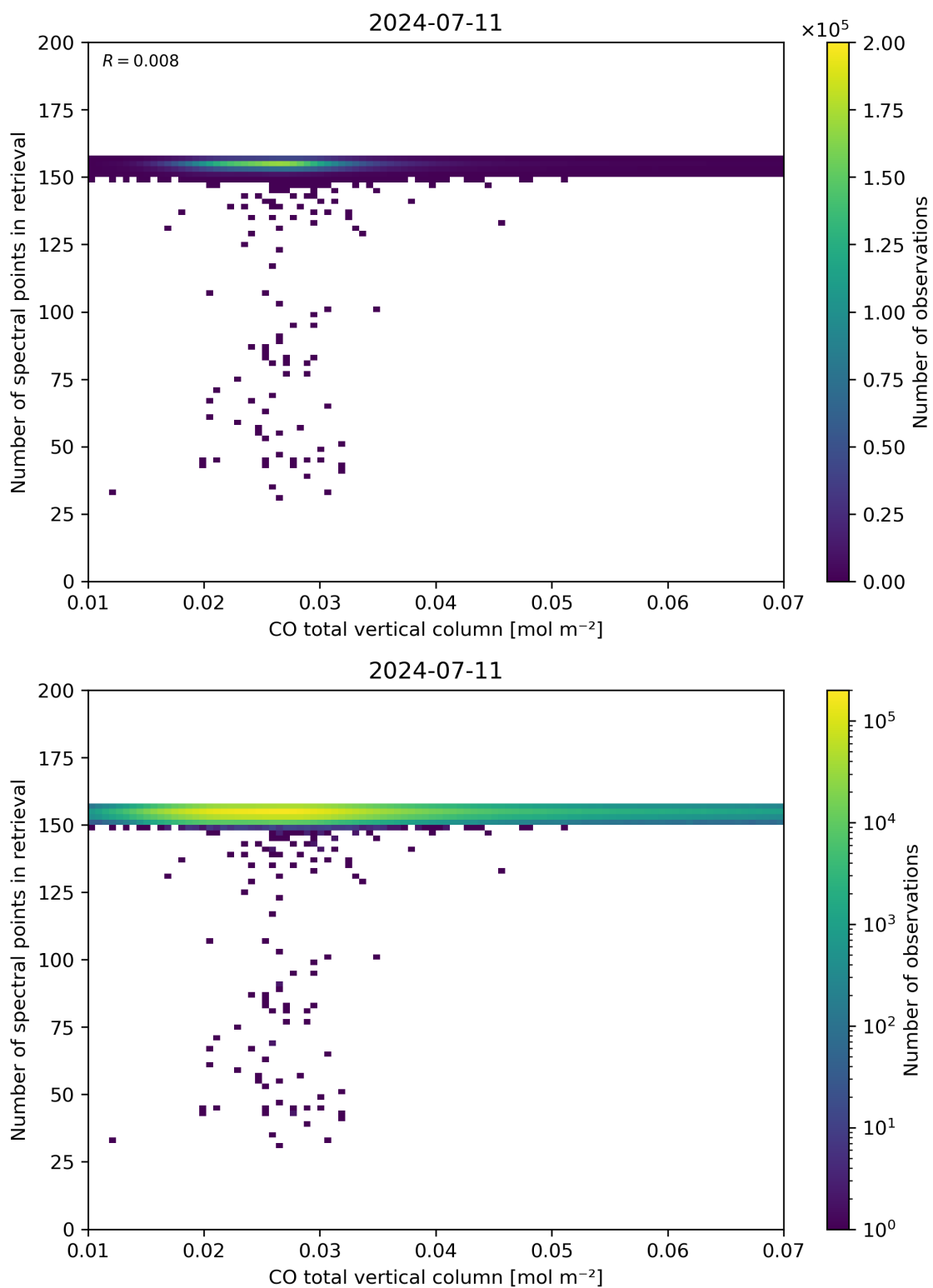
Figure 43: Scatter density plot of “CO total vertical column” against “Number of spectral points in retrieval” for 2024-07-10 to 2024-07-12.
