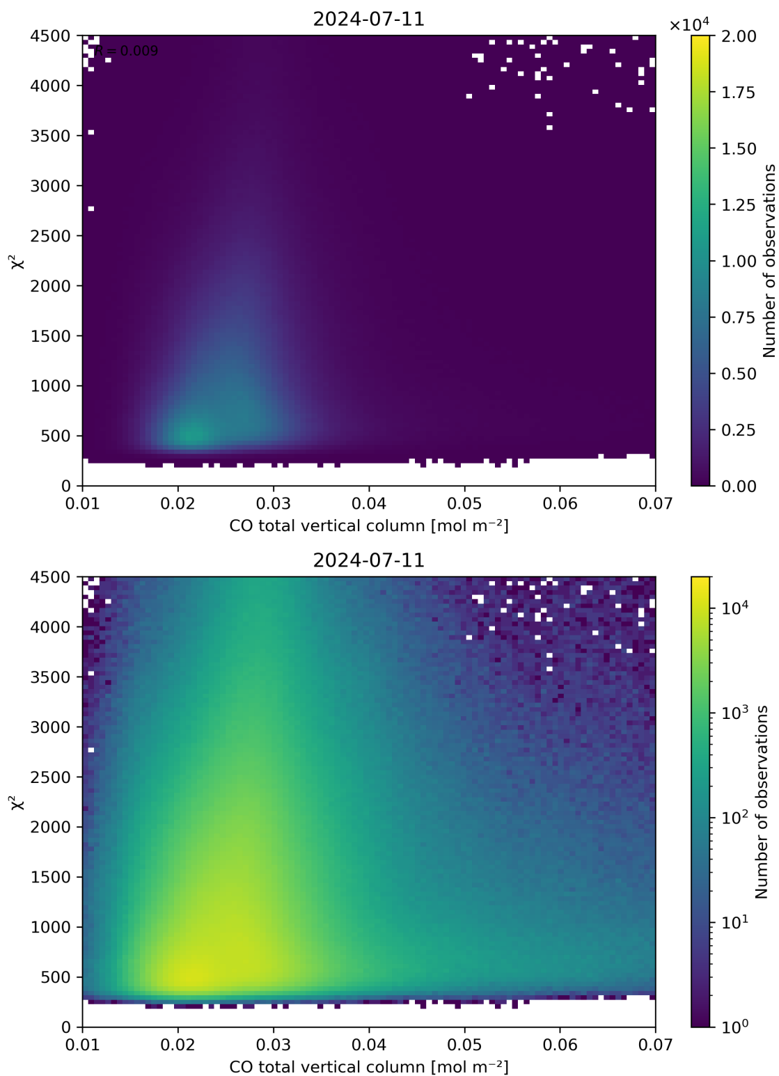
Figure 35: Scatter density plot of “CO total vertical column” against “ \chi^2 ” for 2024-07-10 to 2024-07-12.
