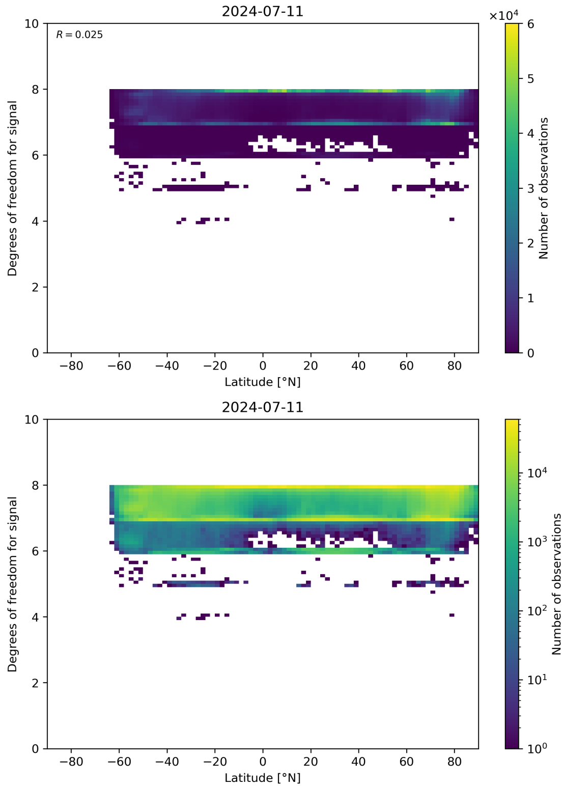
Figure 55: Scatter density plot of “Latitude” against “Degrees of freedom for signal” for 2024-07-10 to 2024-07-12.
