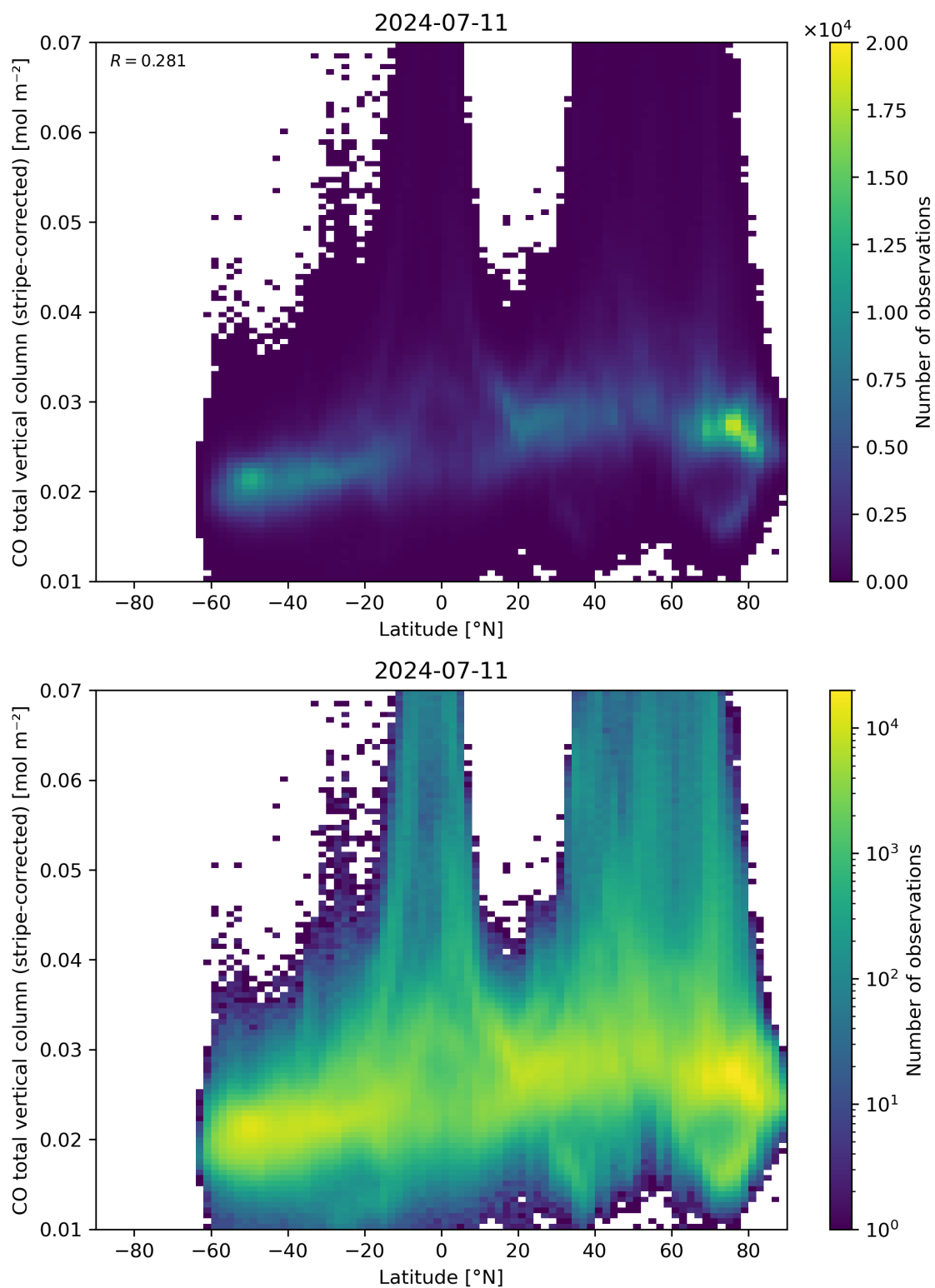
Figure 52: Scatter density plot of “Latitude” against “CO total vertical column (stripe-corrected)” for 2024-07-10 to 2024-07-12.
