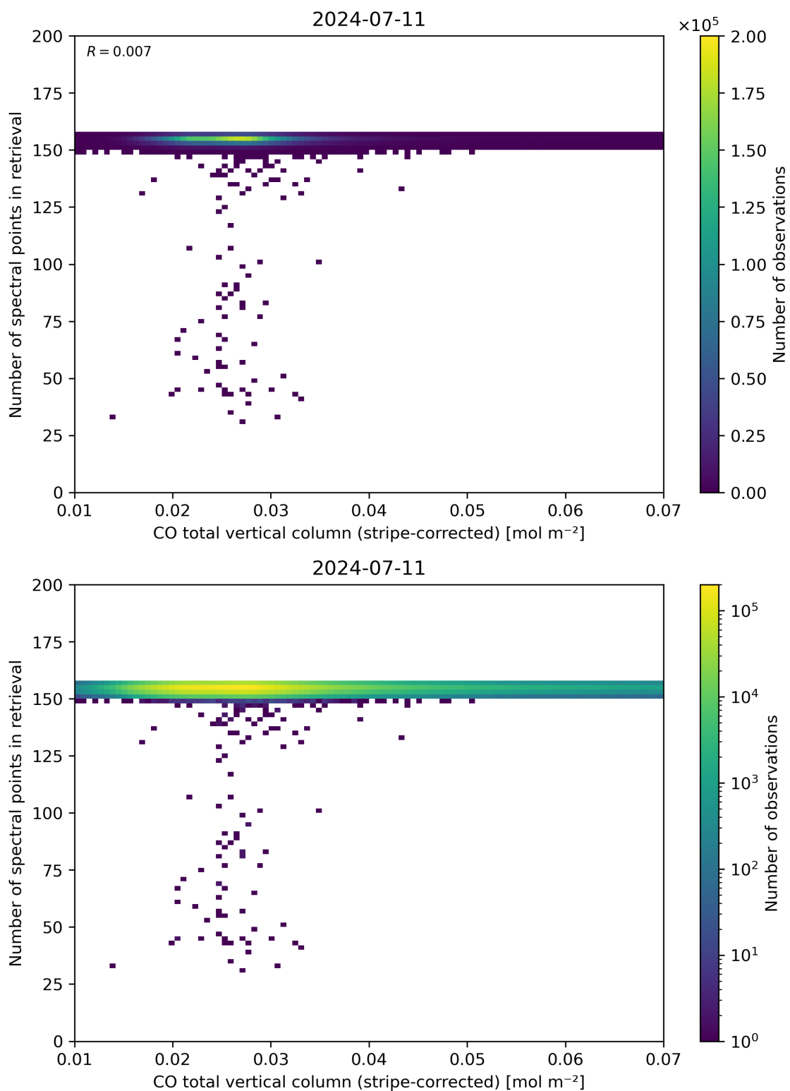
Figure 40: Scatter density plot of “CO total vertical column (stripe-corrected)” against “Number of spectral points in retrieval” for 2024-07-10 to 2024-07-12.
