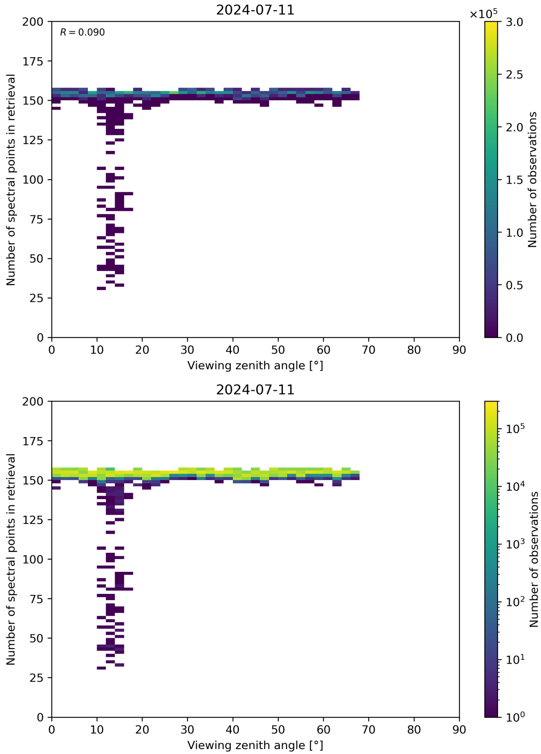
Figure 76: Scatter density plot of “Viewing zenith angle” against “Number of spectral points in retrieval” for 2024-07-10 to 2024-07-12.
