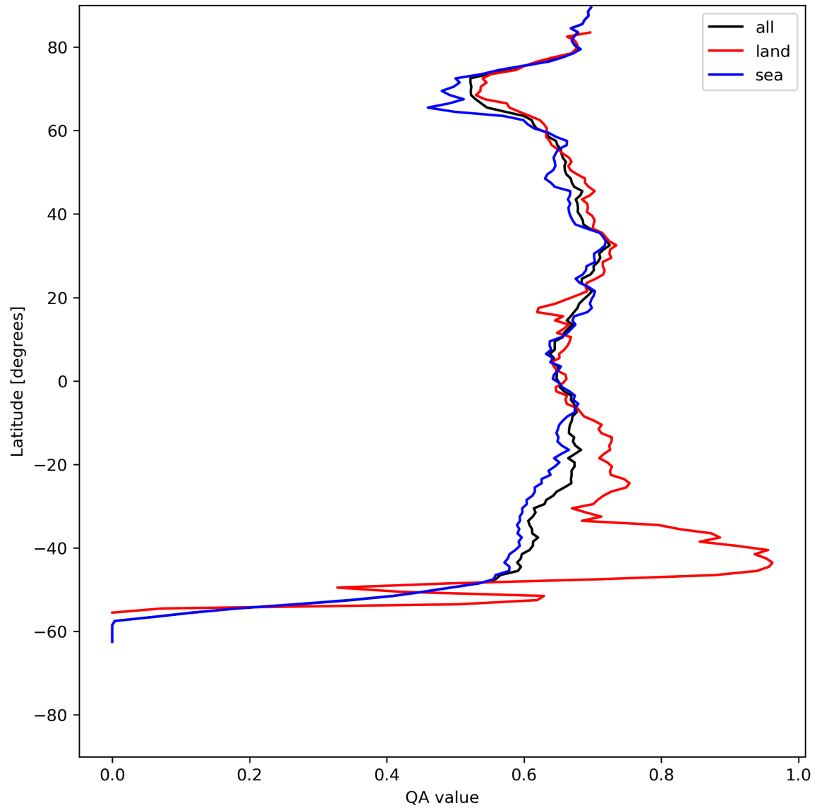
Figure 9: Zonal average of “QA value” for 2024-07-10 to 2024-07-12.
