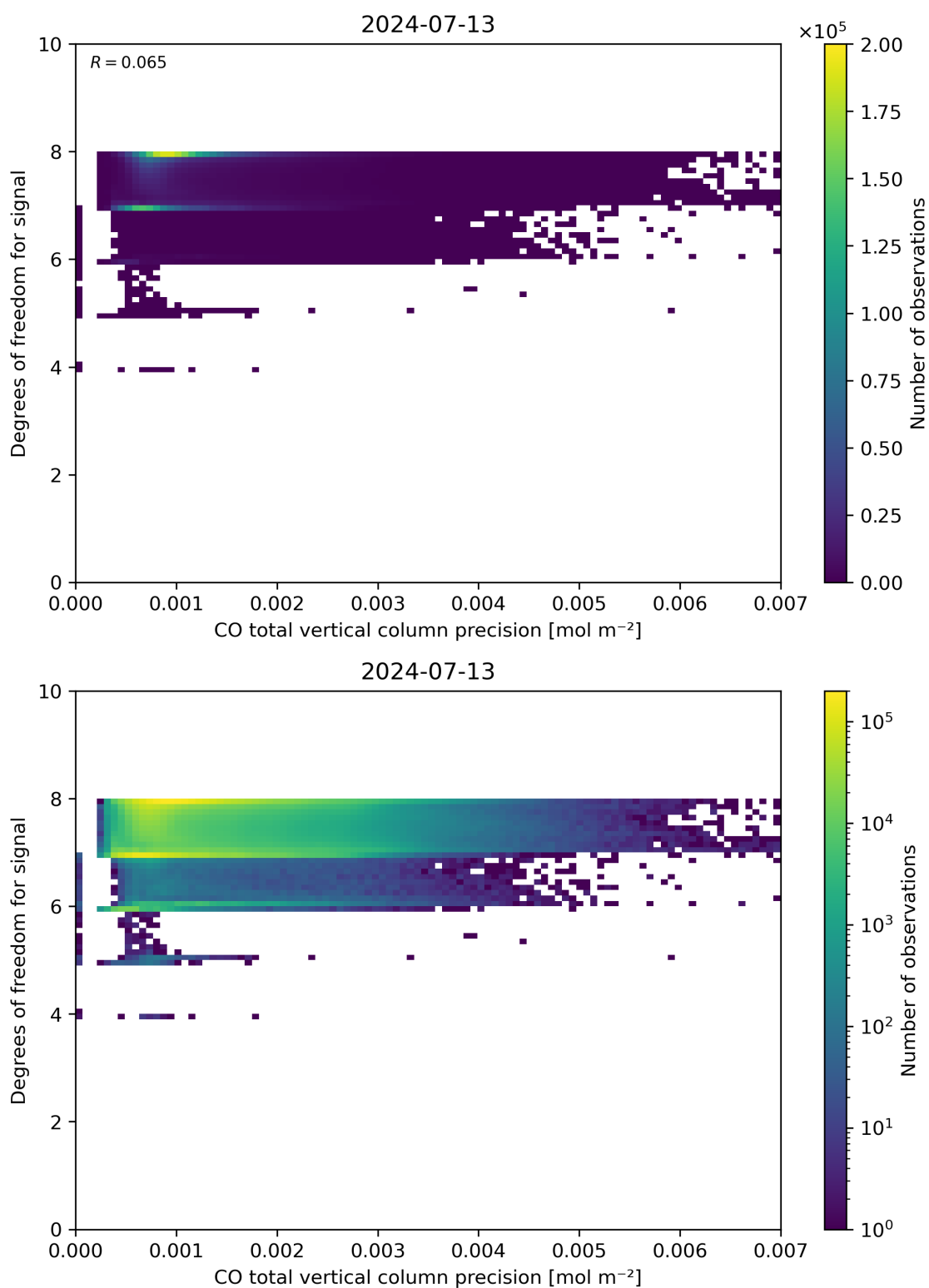
Figure 45: Scatter density plot of “CO total vertical column precision” against “Degrees of freedom for signal” for 2024-07-12 to 2024-07-14.
