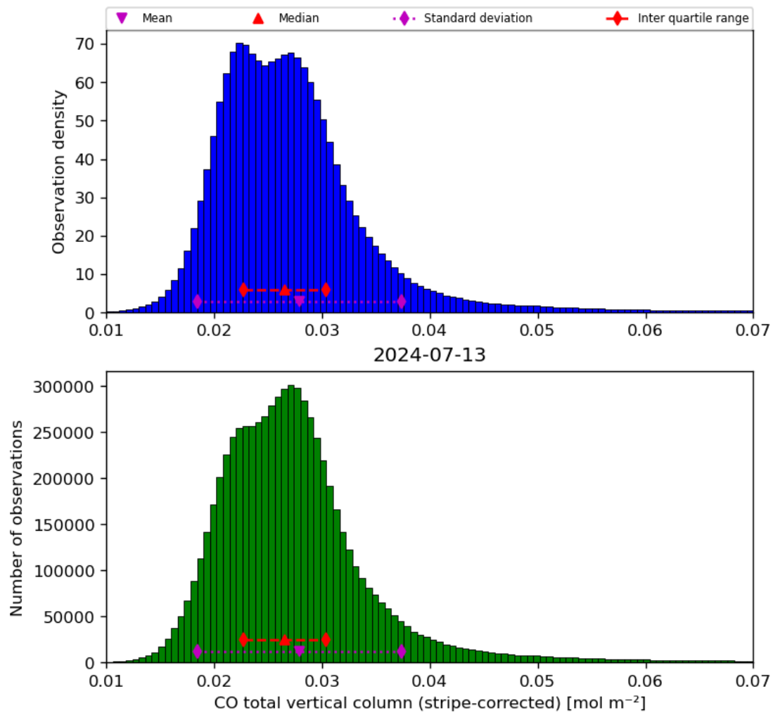
Figure 19: Histogram of “CO total vertical column (stripe-corrected)” for 2024-07-12 to 2024-07-14
