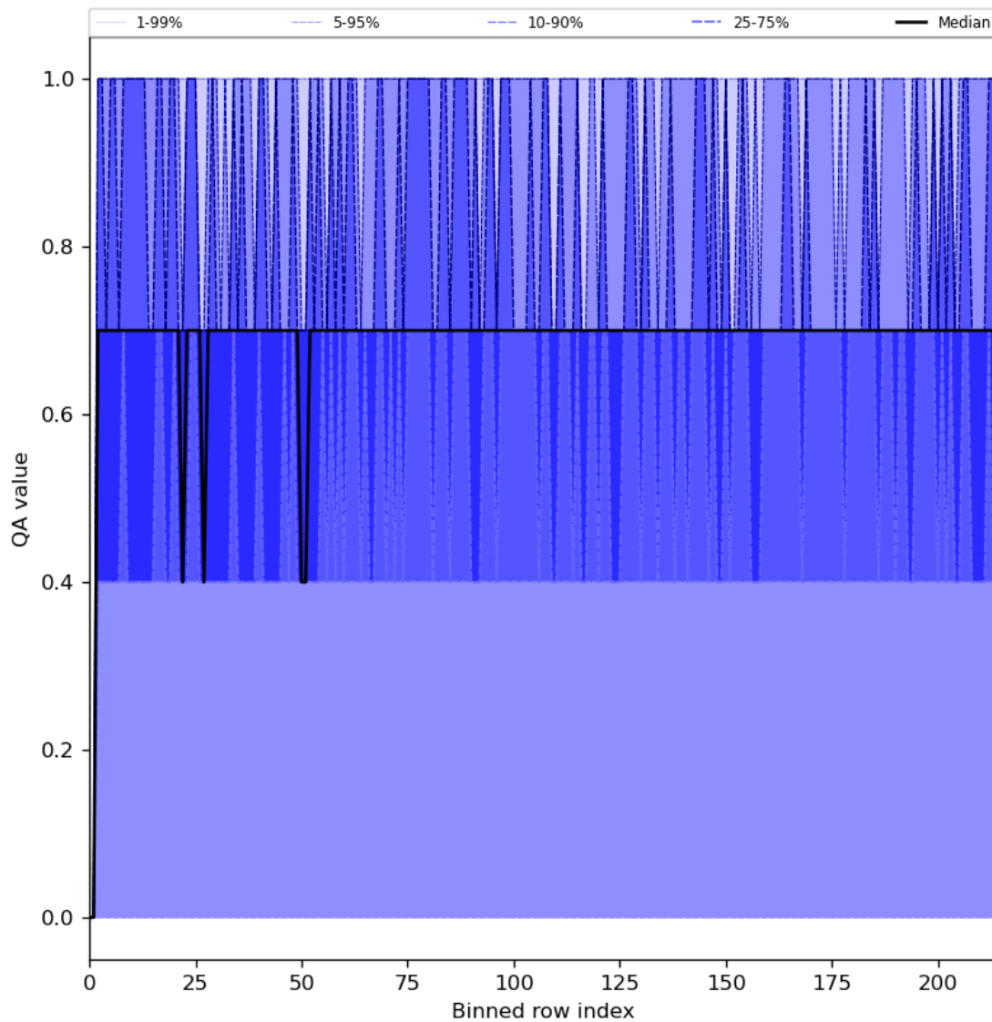
Figure 25: Along track statistics of “QA value” for 2024-07-12 to 2024-07-14
