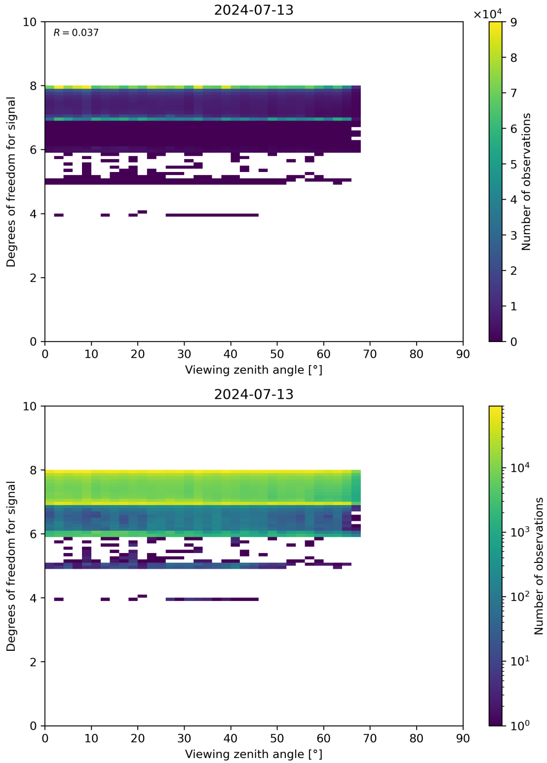
Figure 73: Scatter density plot of “Viewing zenith angle” against “Degrees of freedom for signal” for 2024-07-12 to 2024-07-14.
