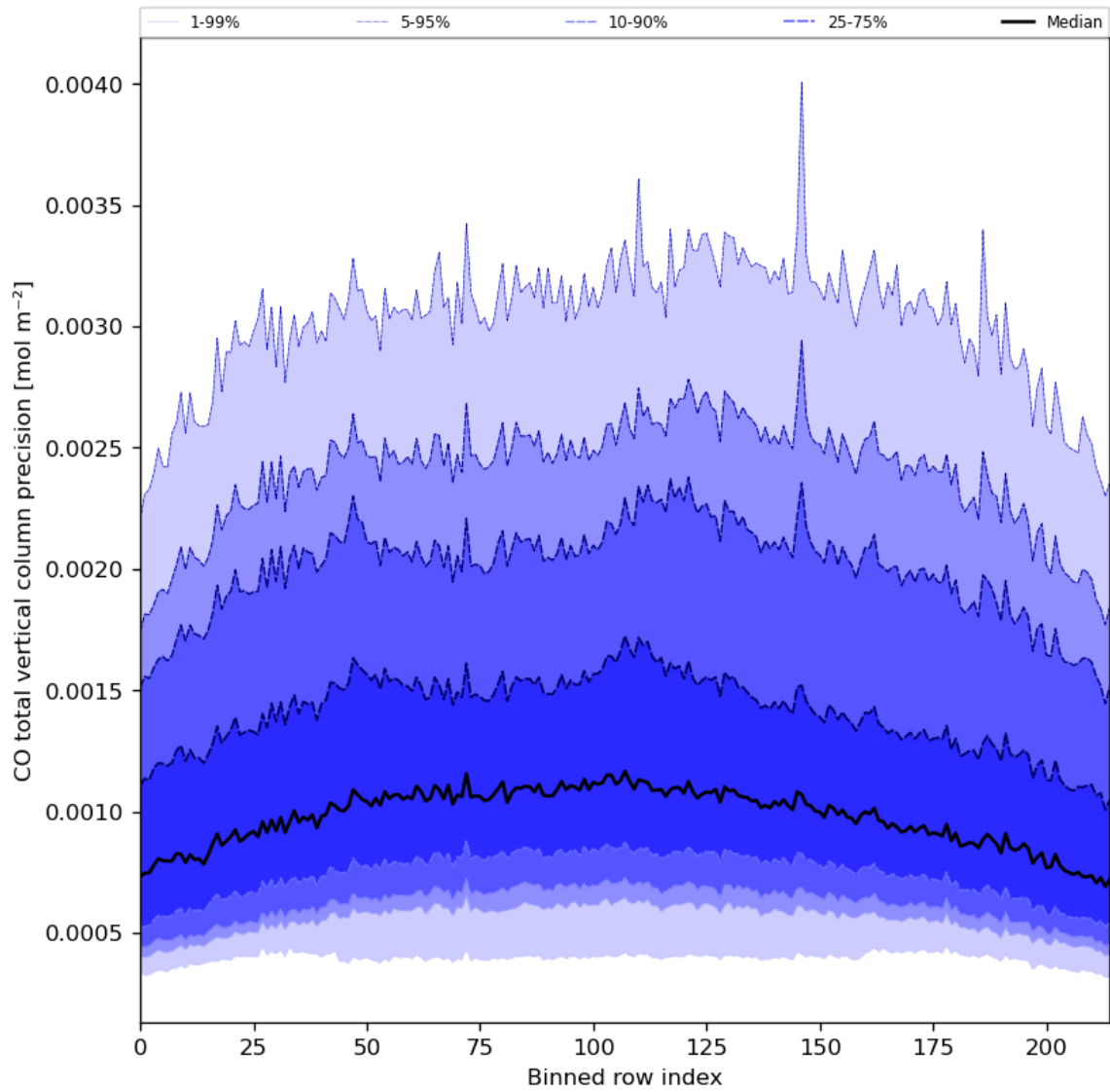
Figure 28: Along track statistics of “CO total vertical column precision” for 2024-07-12 to 2024-07-14
