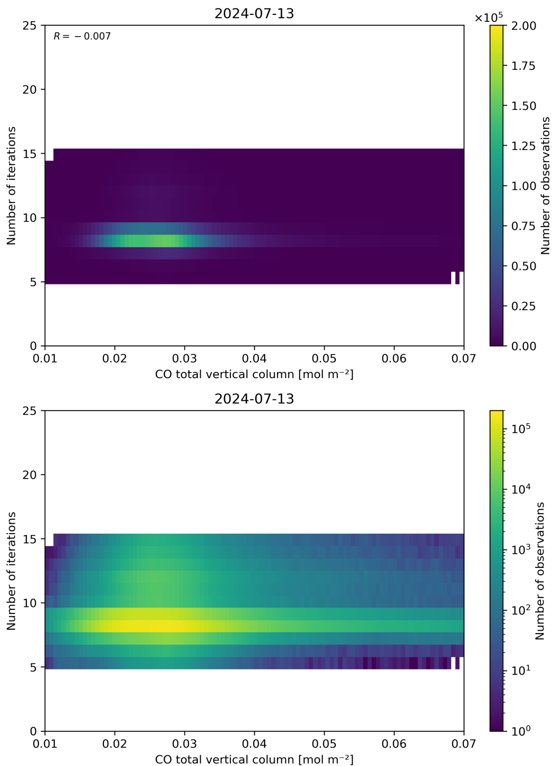
Figure 42: Scatter density plot of “CO total vertical column” against “Number of iterations” for 2024-07-12 to 2024-07-14.
