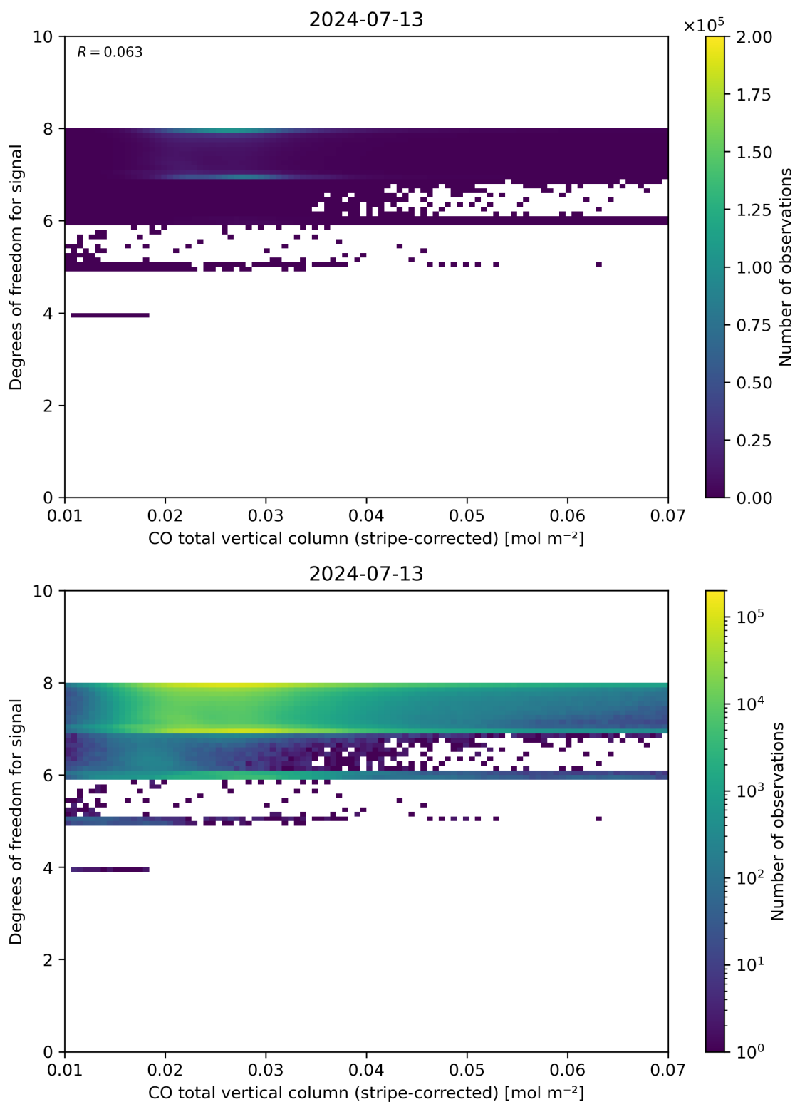
Figure 38: Scatter density plot of “CO total vertical column (stripe-corrected)” against “Degrees of freedom for signal” for 2024-07-12 to 2024-07-14.
