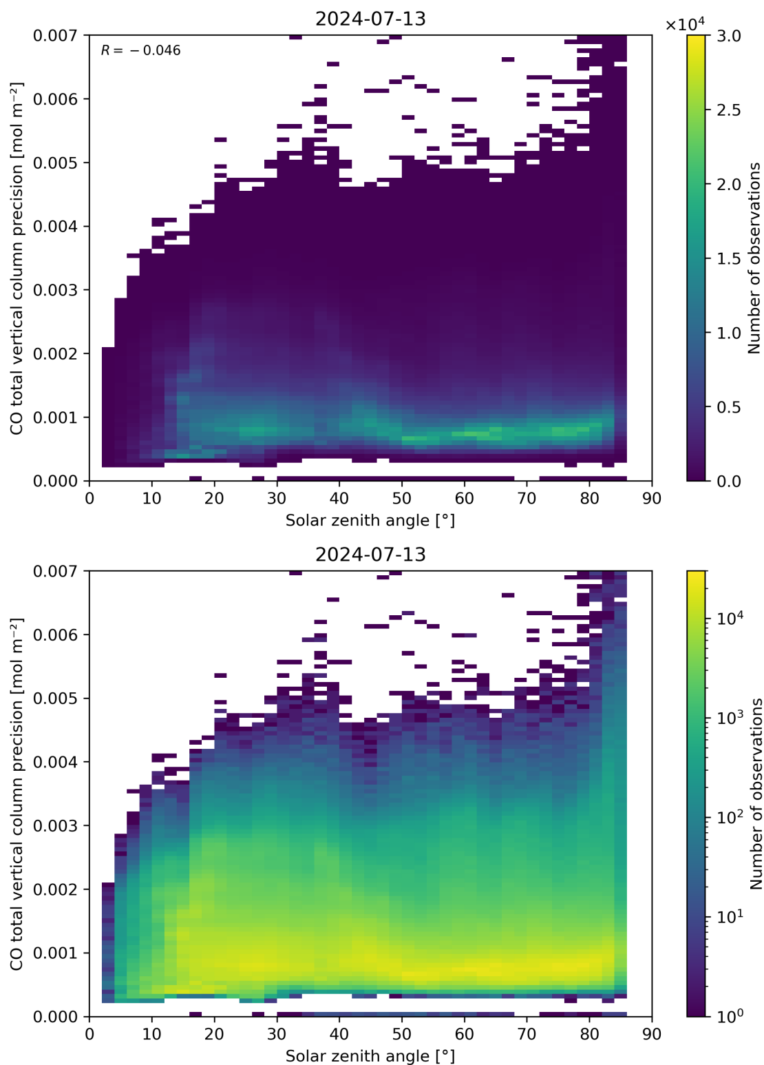
Figure 63: Scatter density plot of “Solar zenith angle” against “CO total vertical column precision” for 2024-07-12 to 2024-07-14.
