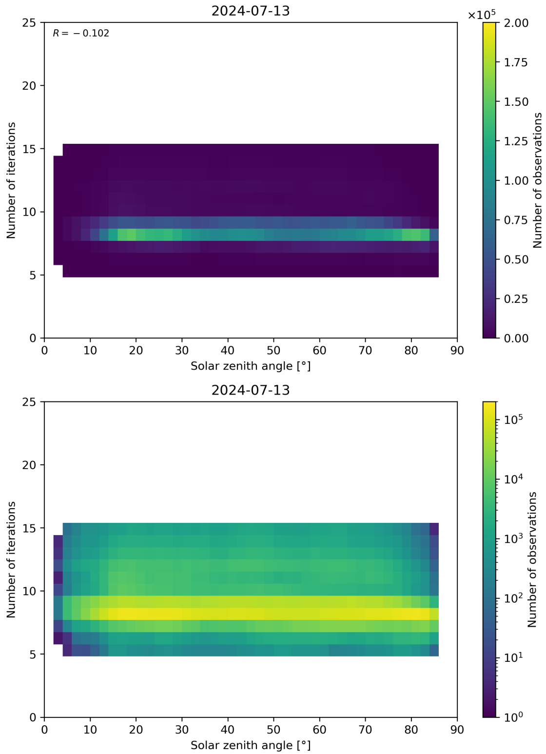
Figure 67: Scatter density plot of “Solar zenith angle” against “Number of iterations” for 2024-07-12 to 2024-07-14.
