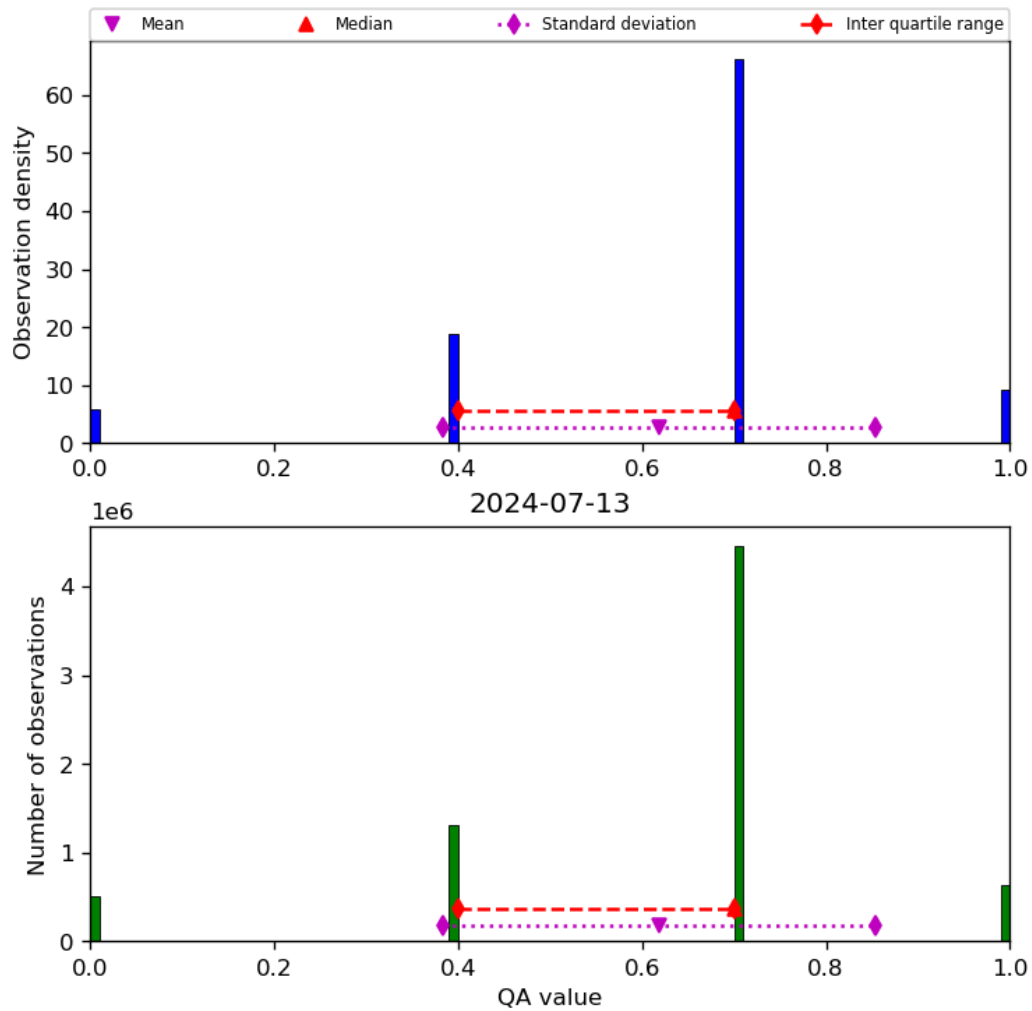
Figure 17: Histogram of “QA value” for 2024-07-12 to 2024-07-14
