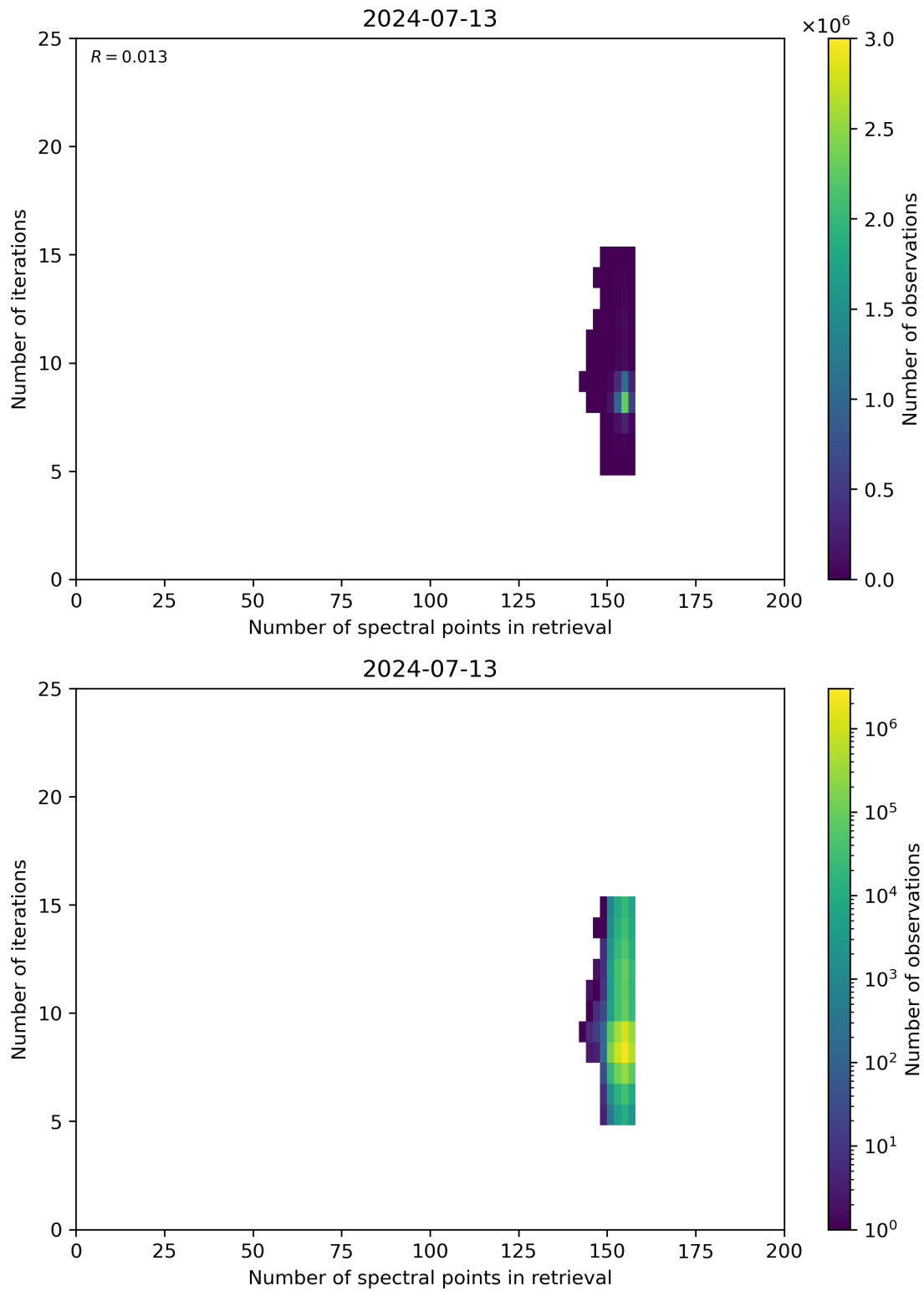
Figure 60: Scatter density plot of “Number of spectral points in retrieval” against “Number of iterations” for 2024-07-12 to 2024-07-14.
