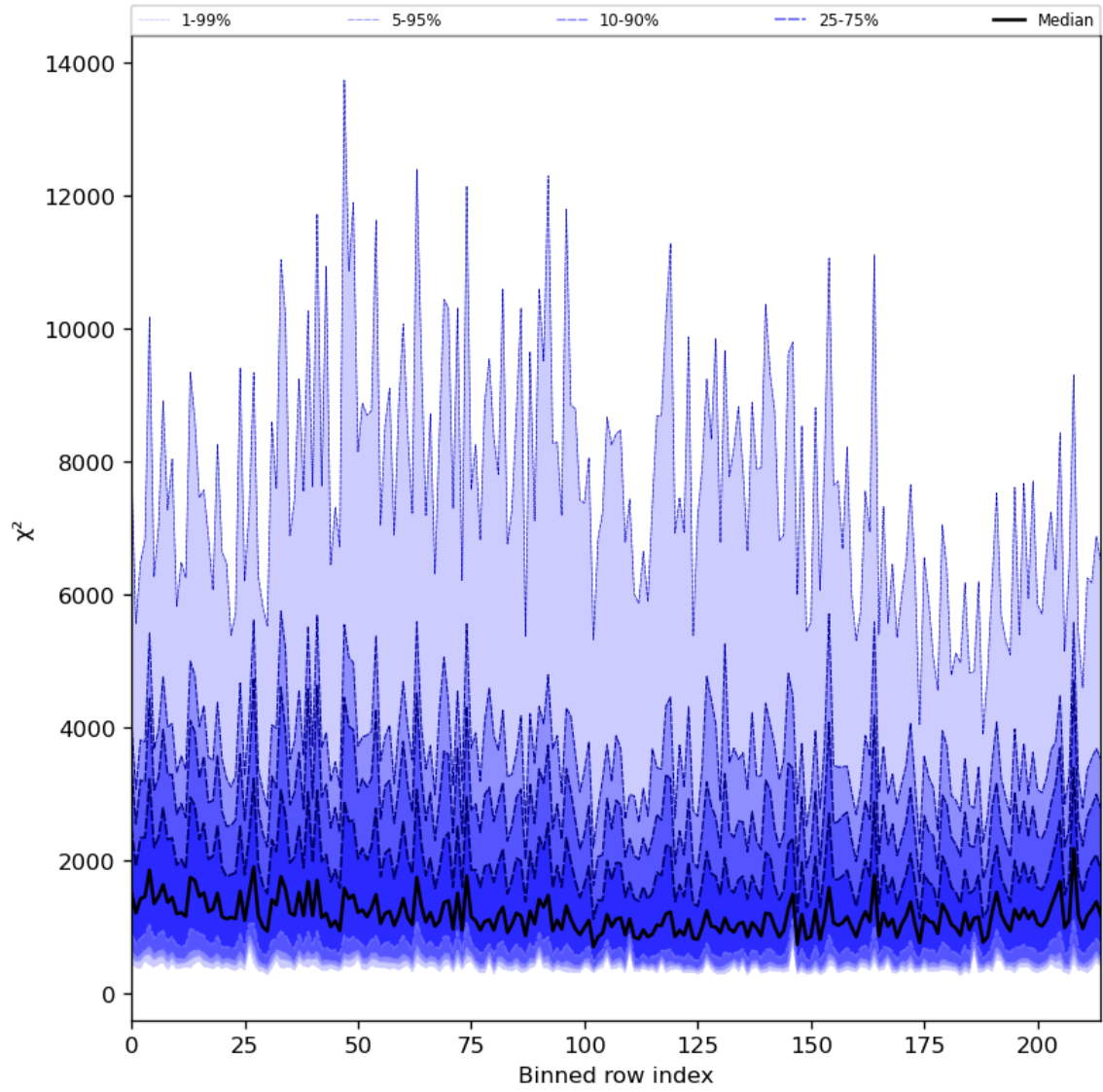
Figure 30: Along track statistics of “ \chi^2 ” for 2024-07-12 to 2024-07-14
