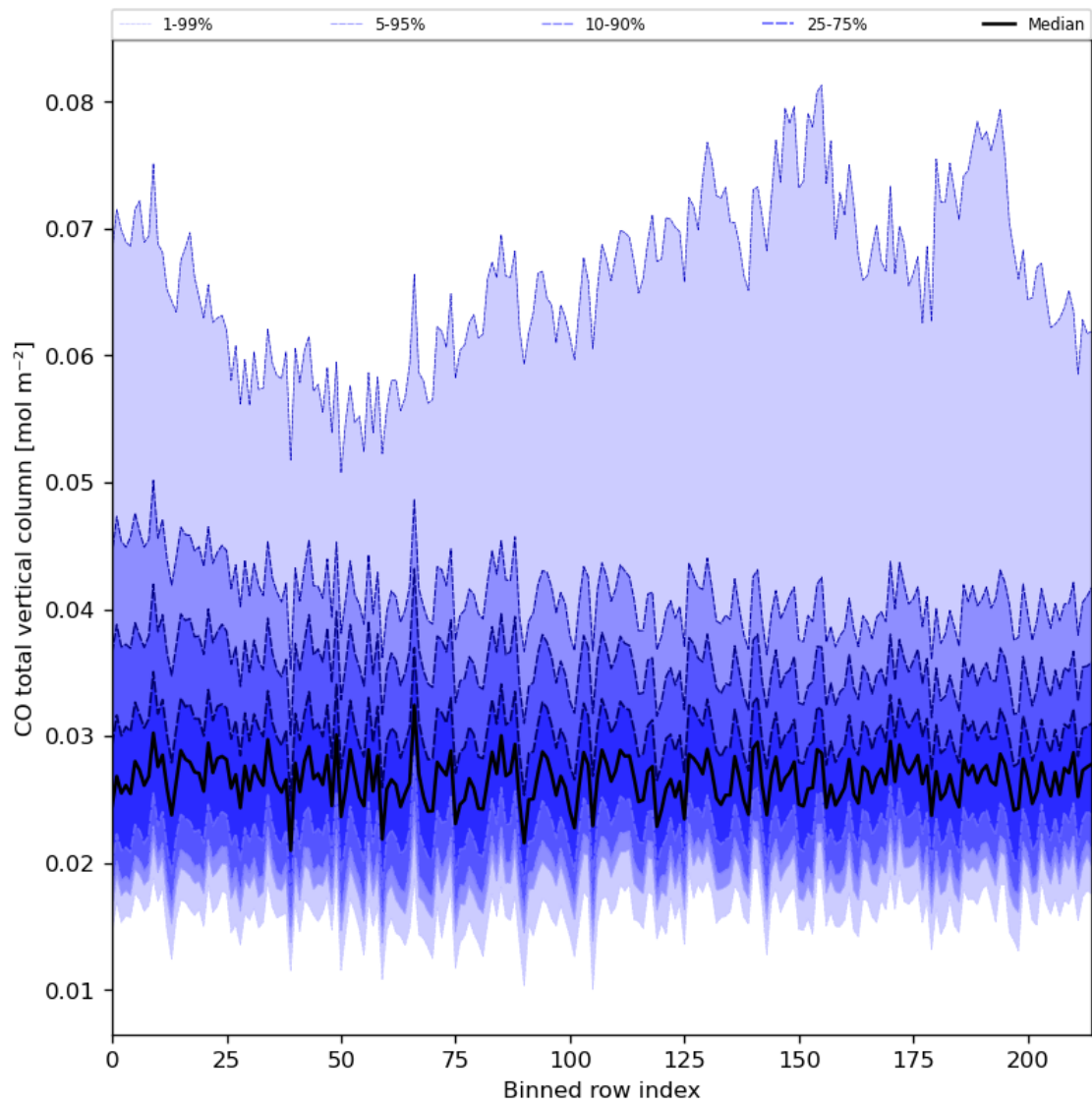
Figure 26: Along track statistics of “CO total vertical column” for 2024-07-12 to 2024-07-14
