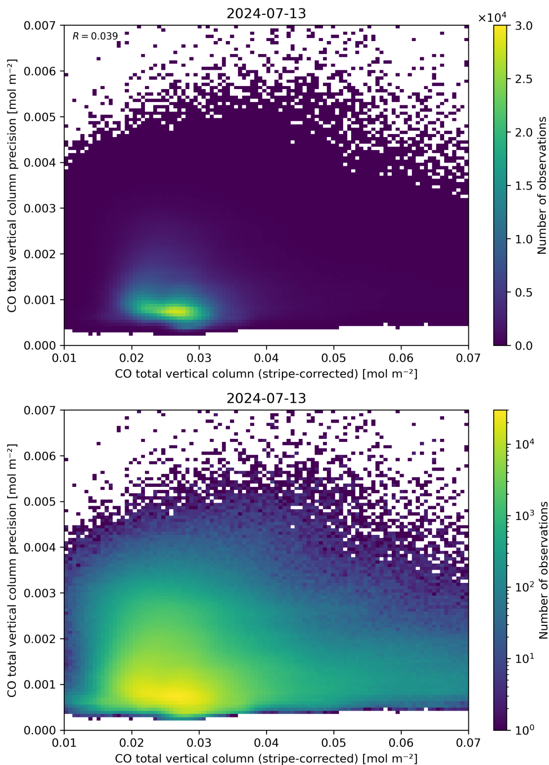
Figure 36: Scatter density plot of “CO total vertical column (stripe-corrected)” against “CO total vertical column precision” for 2024-07-12 to 2024-07-14.
