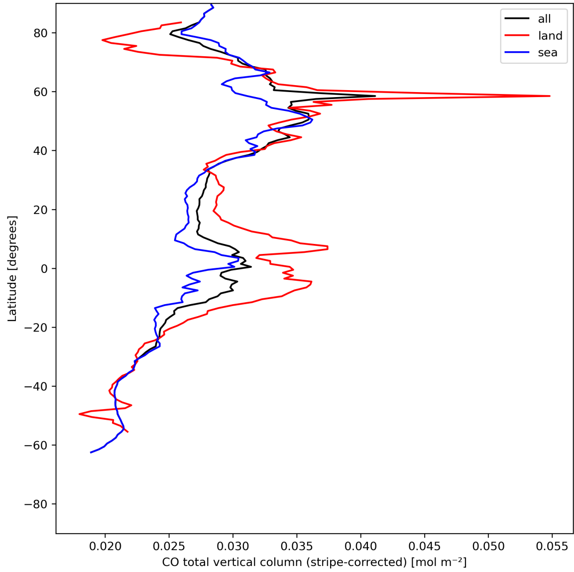
Figure 11: Zonal average of “CO total vertical column (stripe-corrected)” for 2024-07-12 to 2024-07-14.
