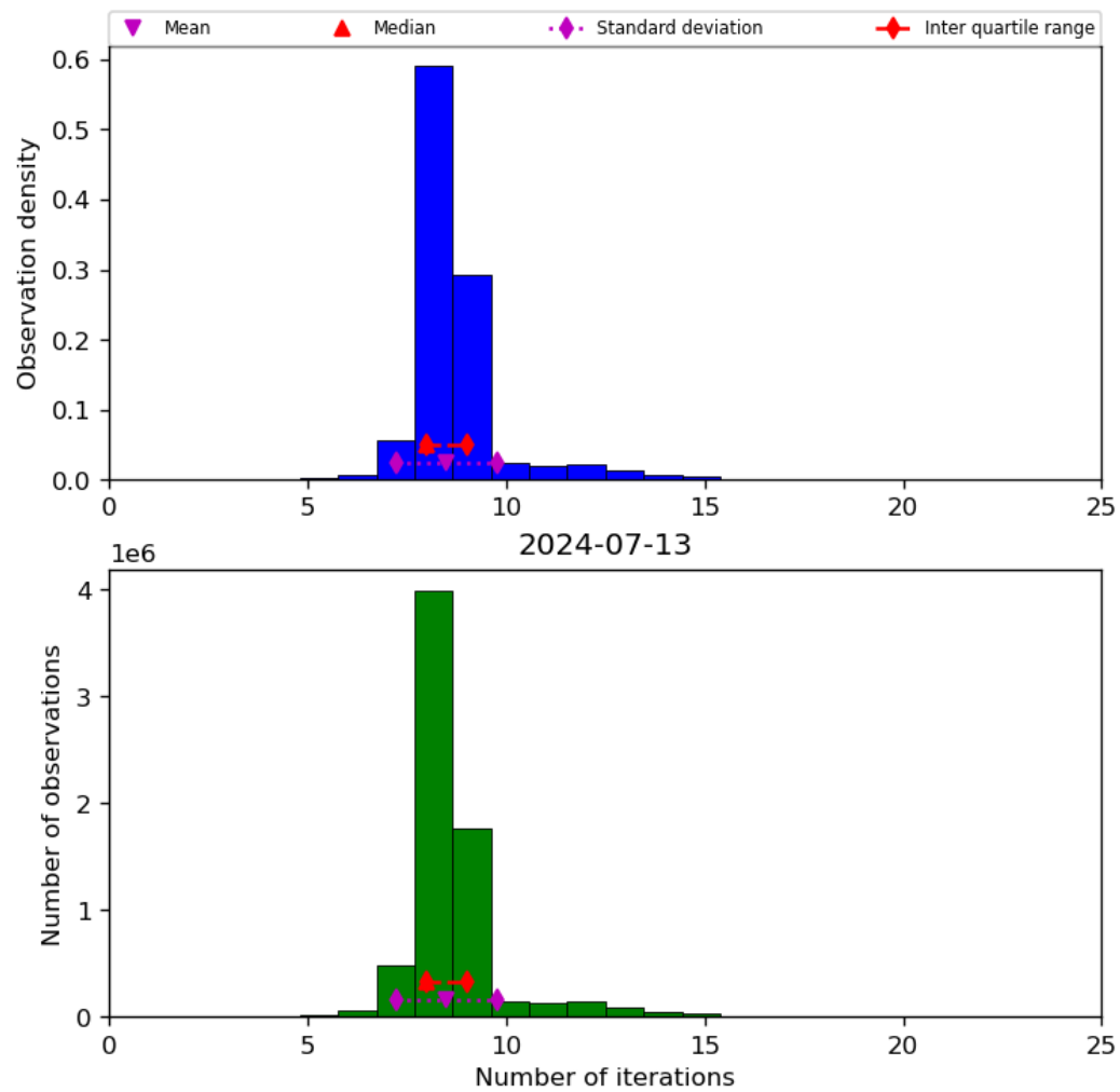
Figure 24: Histogram of “Number of iterations” for 2024-07-12 to 2024-07-14
