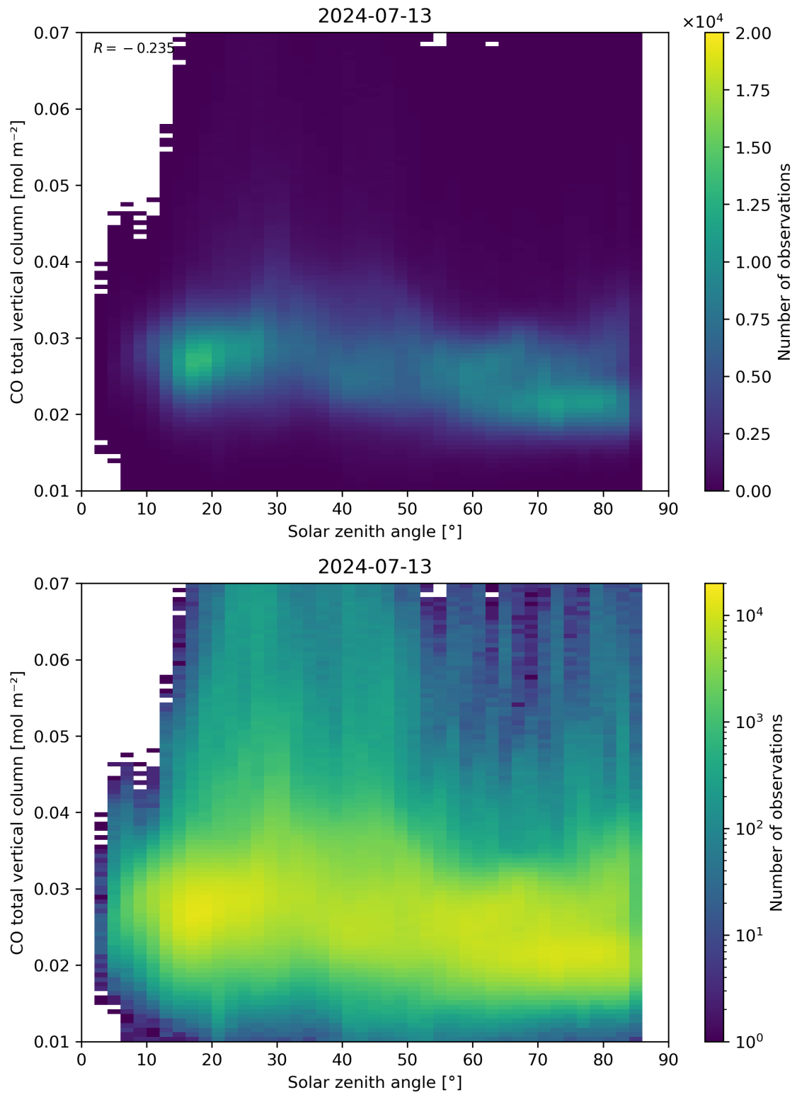
Figure 61: Scatter density plot of “Solar zenith angle” against “CO total vertical column” for 2024-07-12 to 2024-07-14.
