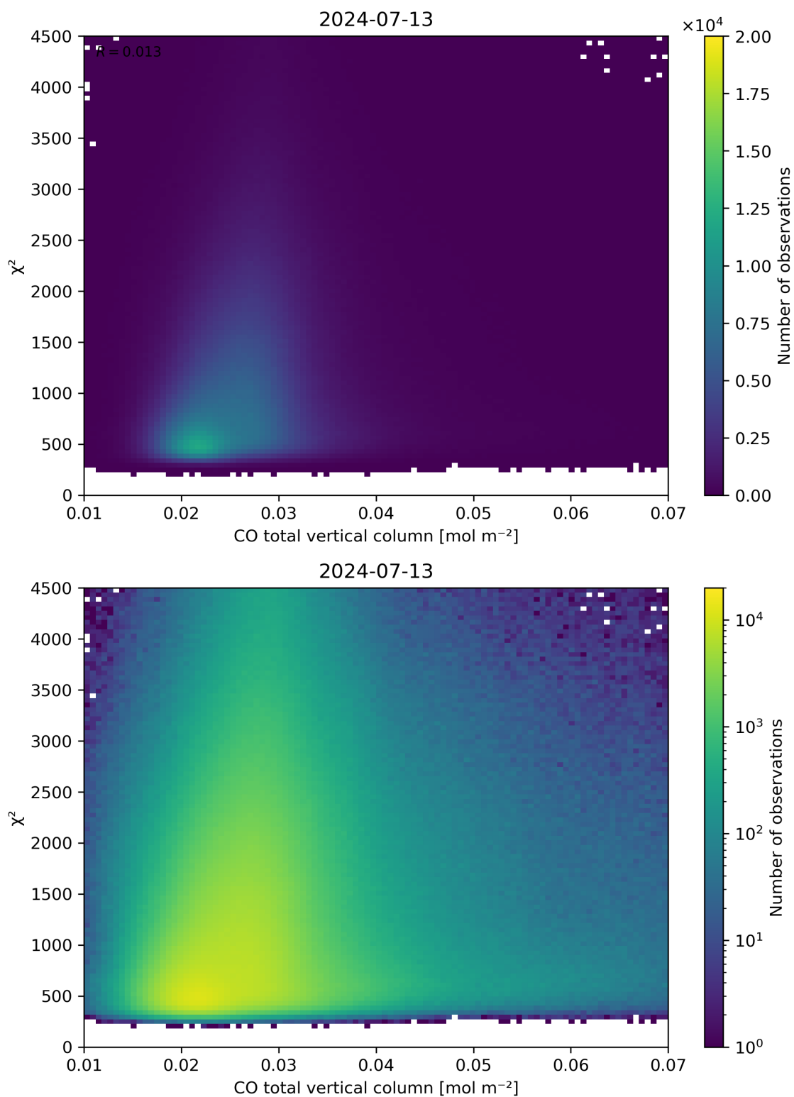
Figure 35: Scatter density plot of “CO total vertical column” against “ \chi^2 ” for 2024-07-12 to 2024-07-14.
