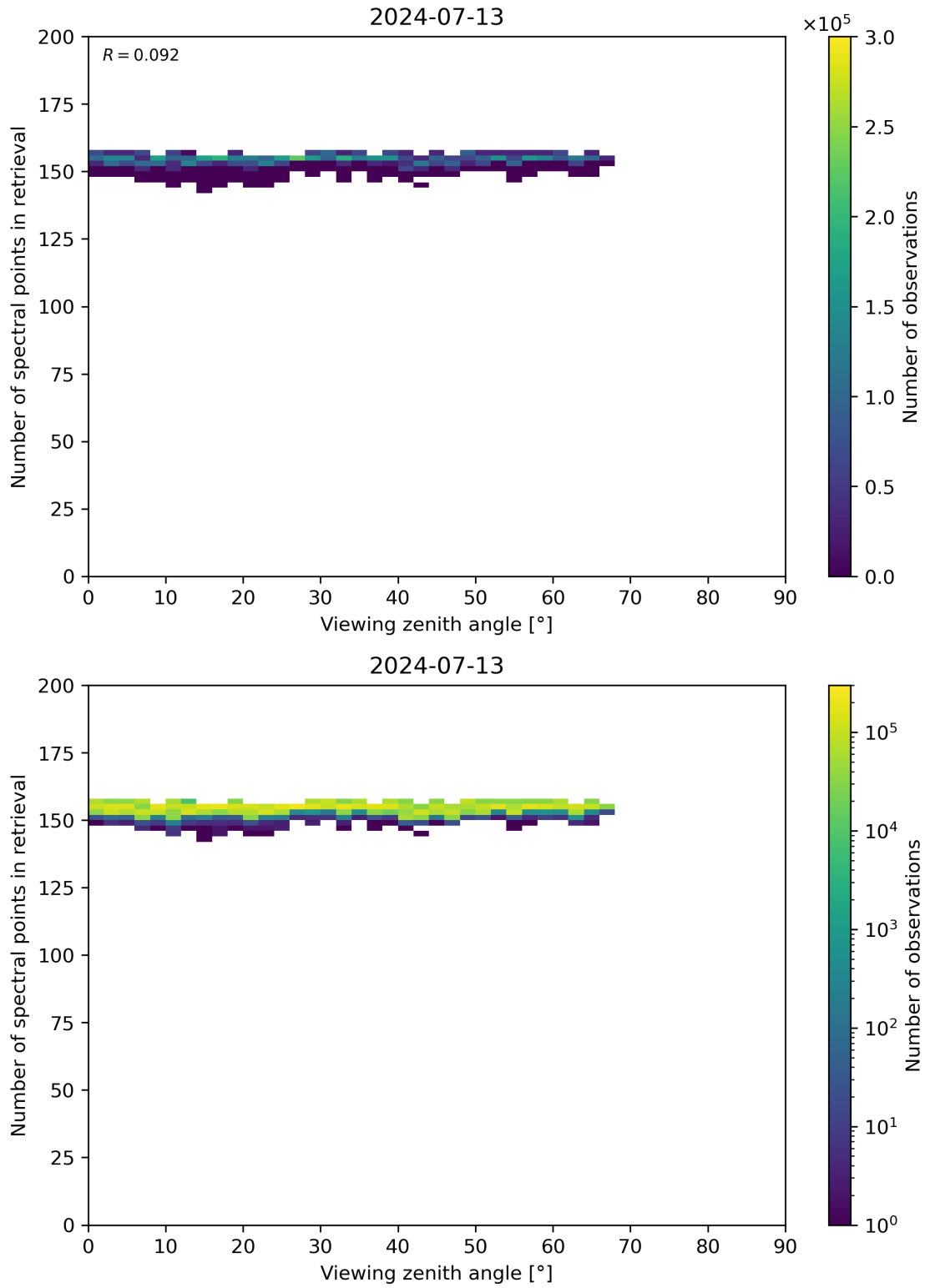
Figure 76: Scatter density plot of “Viewing zenith angle” against “Number of spectral points in retrieval” for 2024-07-12 to 2024-07-14.
