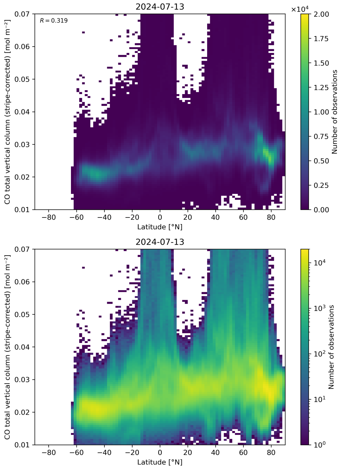
Figure 52: Scatter density plot of “Latitude” against “CO total vertical column (stripe-corrected)” for 2024-07-12 to 2024-07-14.
