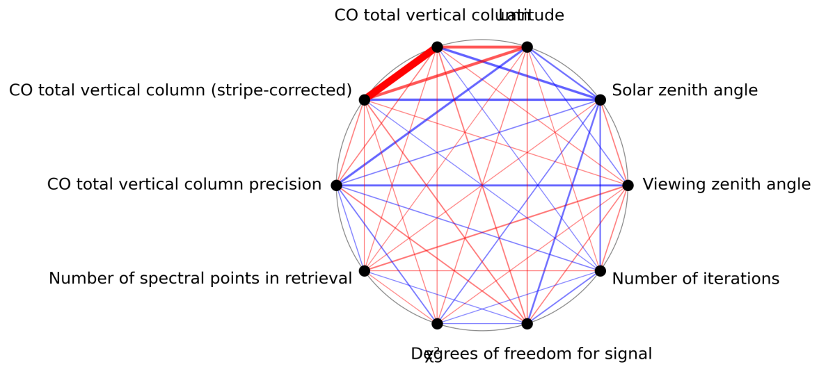
Figure 1: Map of correlation graph for 2024-07-12 to 2024-07-14.
