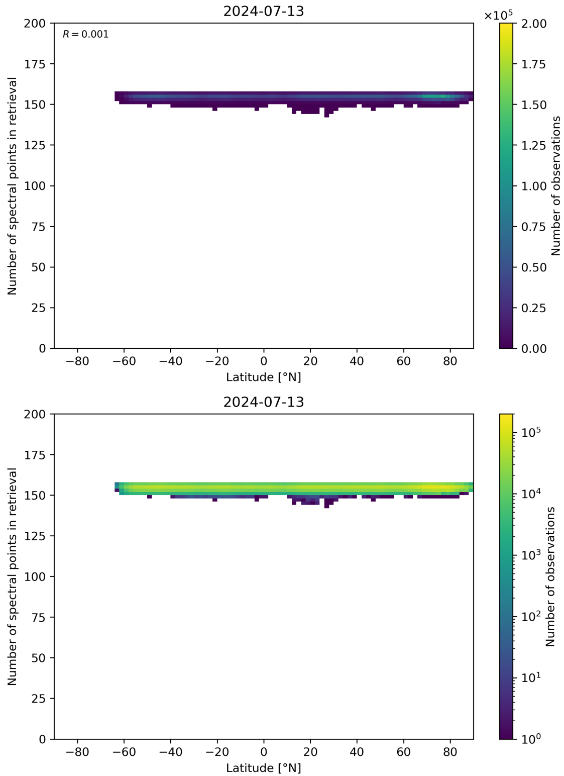
Figure 57: Scatter density plot of “Latitude” against “Number of spectral points in retrieval” for 2024-07-12 to 2024-07-14.
