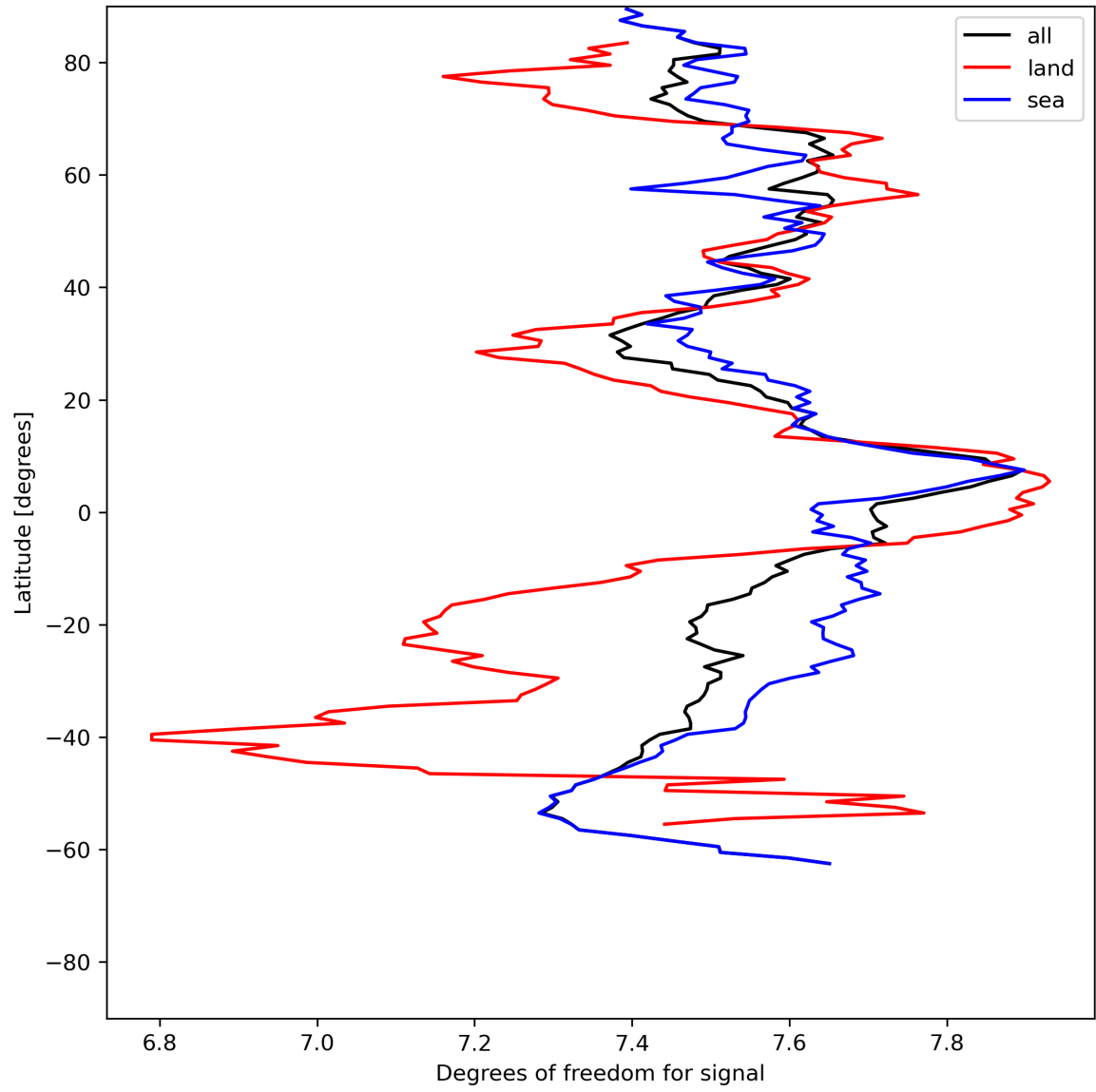
Figure 15: Zonal average of “Degrees of freedom for signal” for 2024-07-12 to 2024-07-14.
