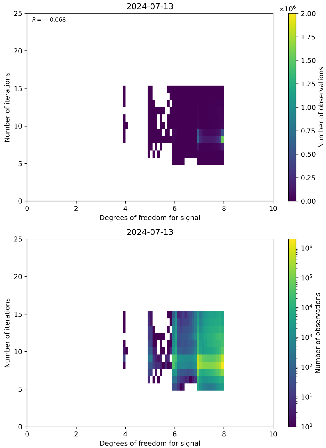
Figure 50: Scatter density plot of “Degrees of freedom for signal” against “Number of iterations” for 2024-07-12 to 2024-07-14.
