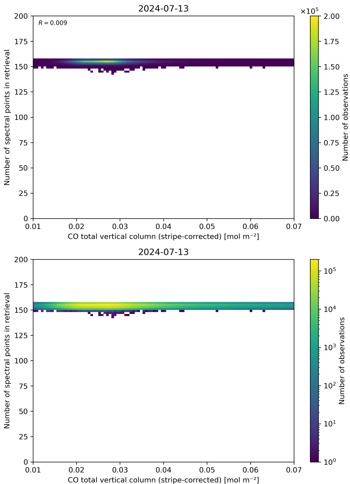
Figure 40: Scatter density plot of “CO total vertical column (stripe-corrected)” against “Number of spectral points in retrieval” for 2024-07-12 to 2024-07-14.
