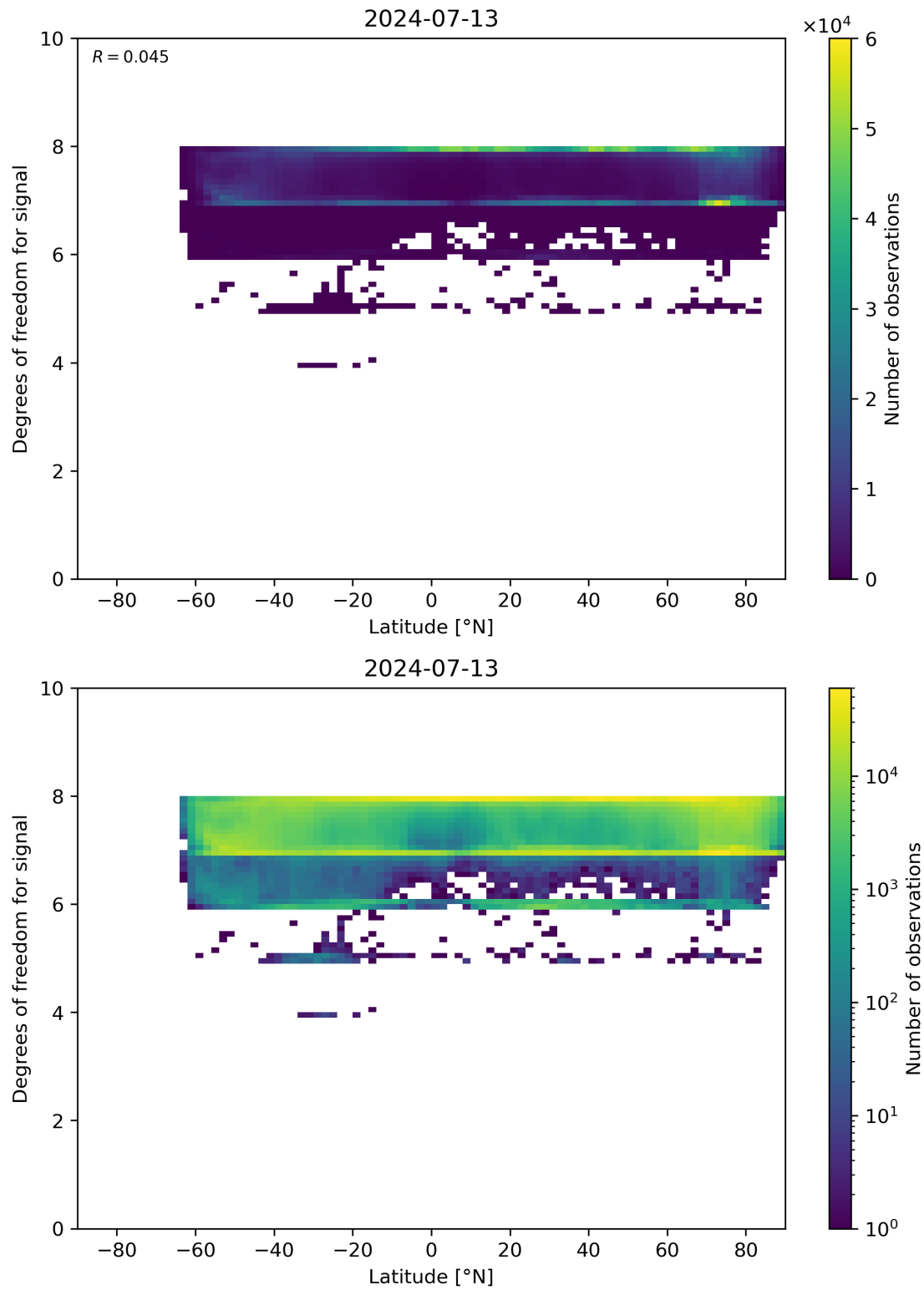
Figure 55: Scatter density plot of “Latitude” against “Degrees of freedom for signal” for 2024-07-12 to 2024-07-14.
