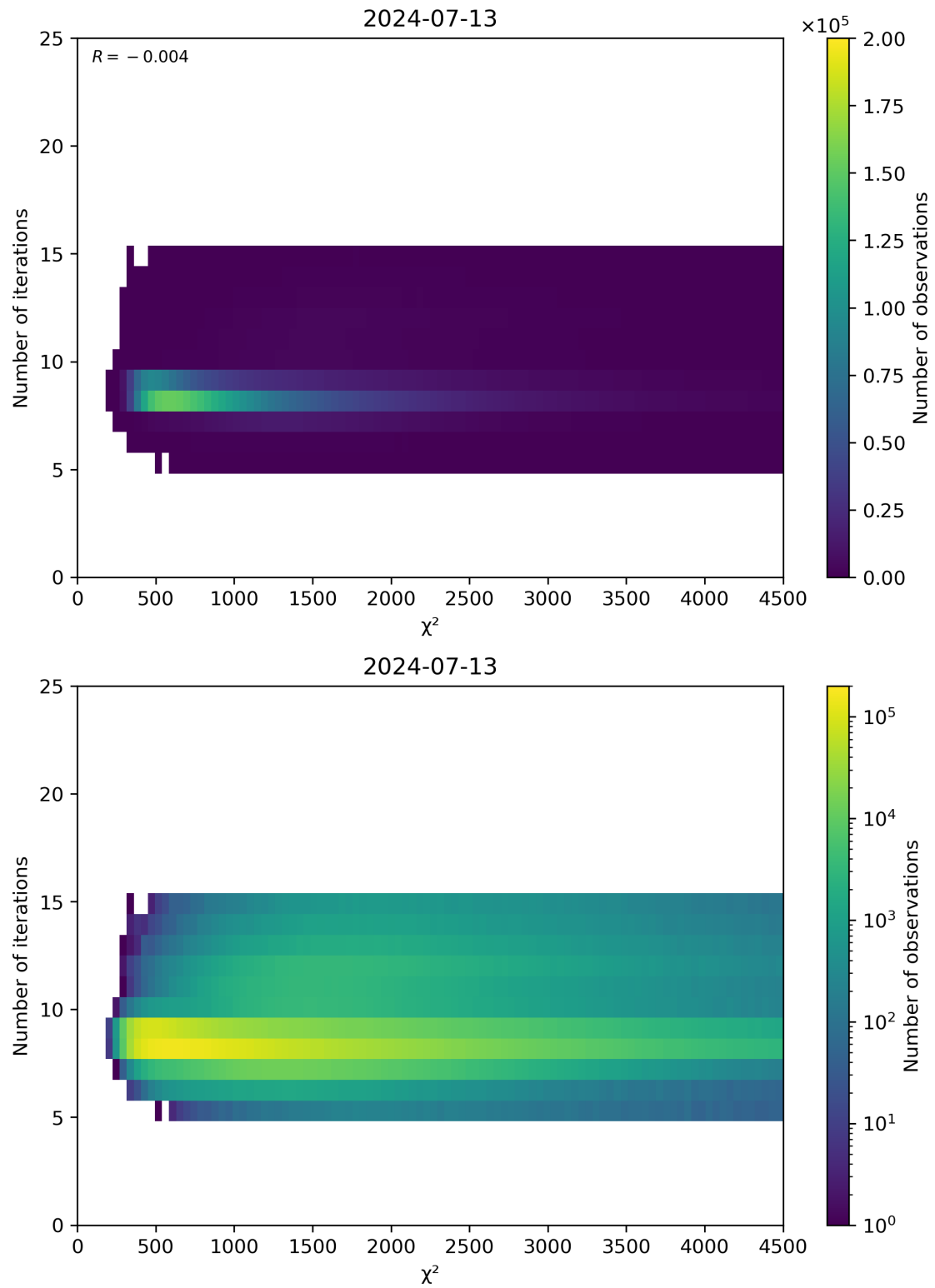
Figure 49: Scatter density plot of “ \chi^2 ” against “Number of iterations” for 2024-07-12 to 2024-07-14.
