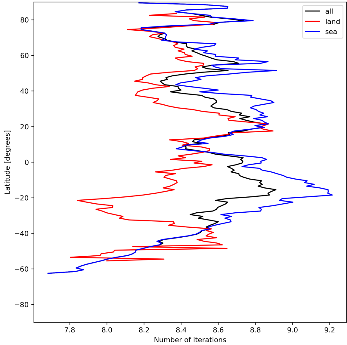
Figure 16: Zonal average of “Number of iterations” for 2024-07-12 to 2024-07-14.
