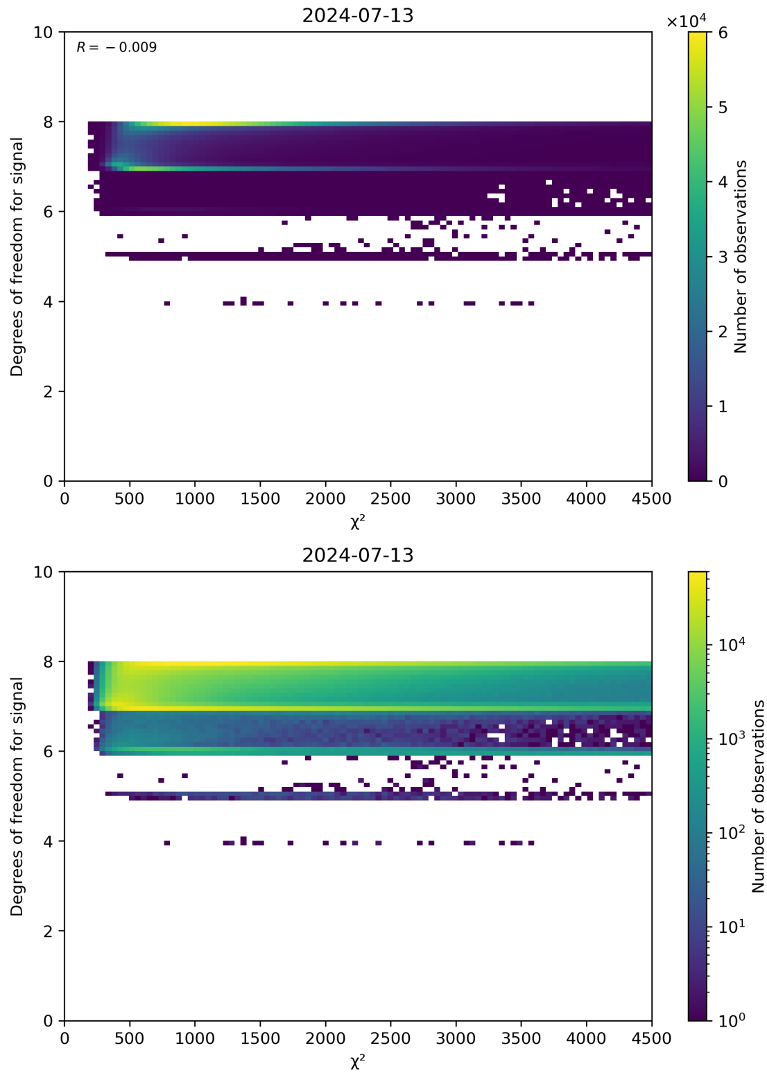
Figure 48: Scatter density plot of " \chi^2 " against "Degrees of freedom for signal" for 2024-07-12 to 2024-07-14.
