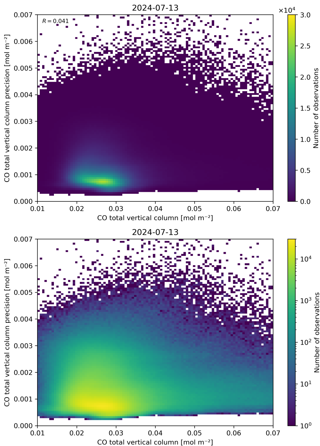
Figure 34: Scatter density plot of “CO total vertical column” against “CO total vertical column precision” for 2024-07-12 to 2024-07-14.
