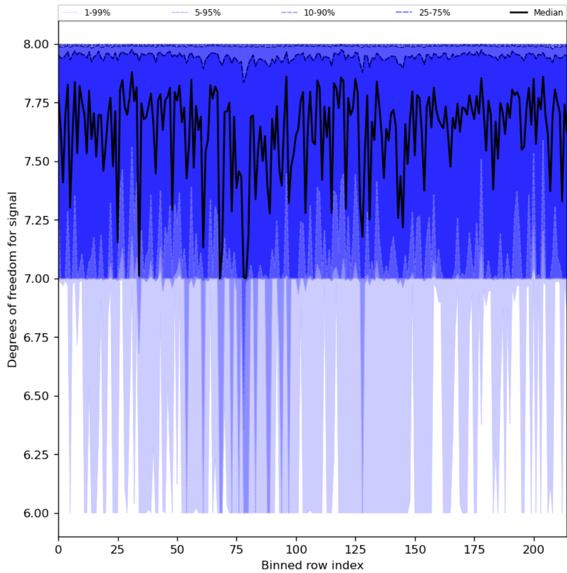
Figure 31: Along track statistics of “Degrees of freedom for signal” for 2024-07-12 to 2024-07-14
