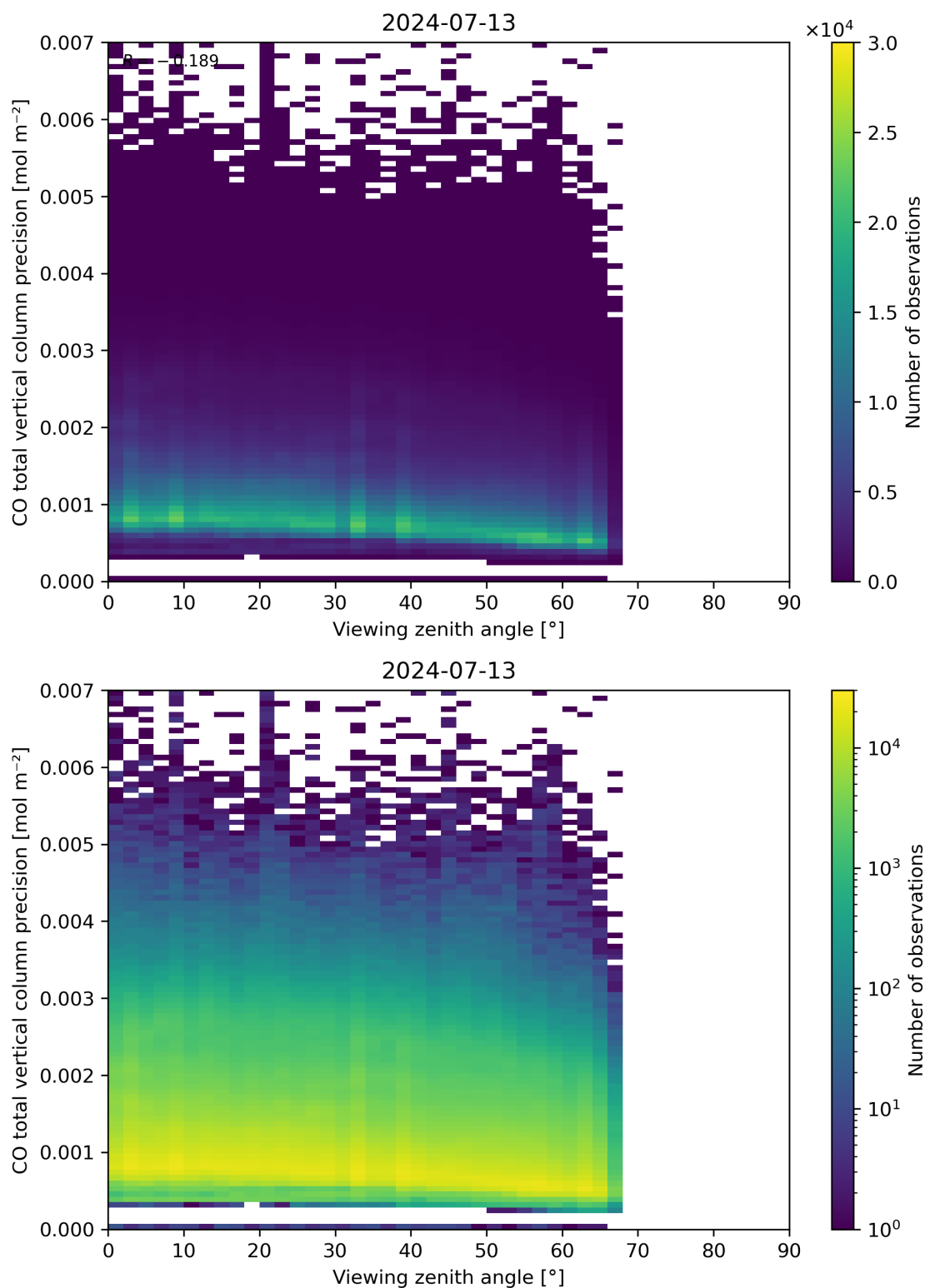
Figure 71: Scatter density plot of “Viewing zenith angle” against “CO total vertical column precision” for 2024-07-12 to 2024-07-14.
