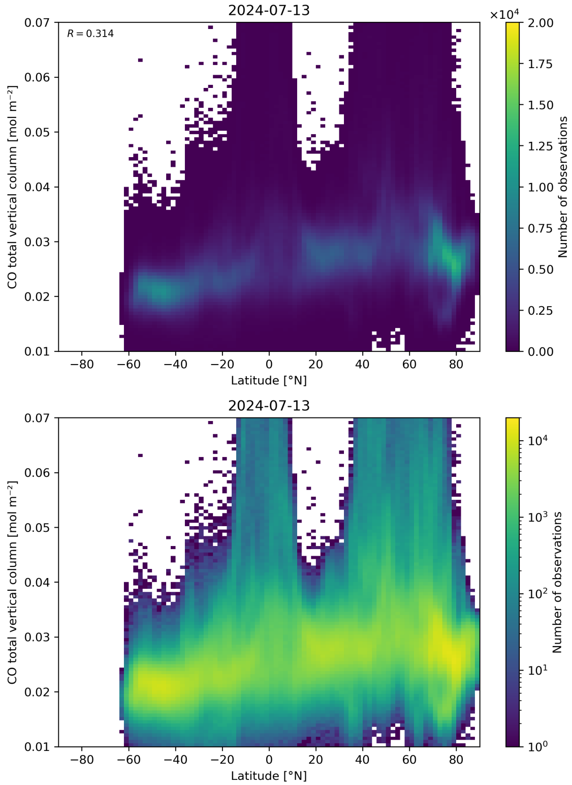
Figure 51: Scatter density plot of “Latitude” against “CO total vertical column” for 2024-07-12 to 2024-07-14.
