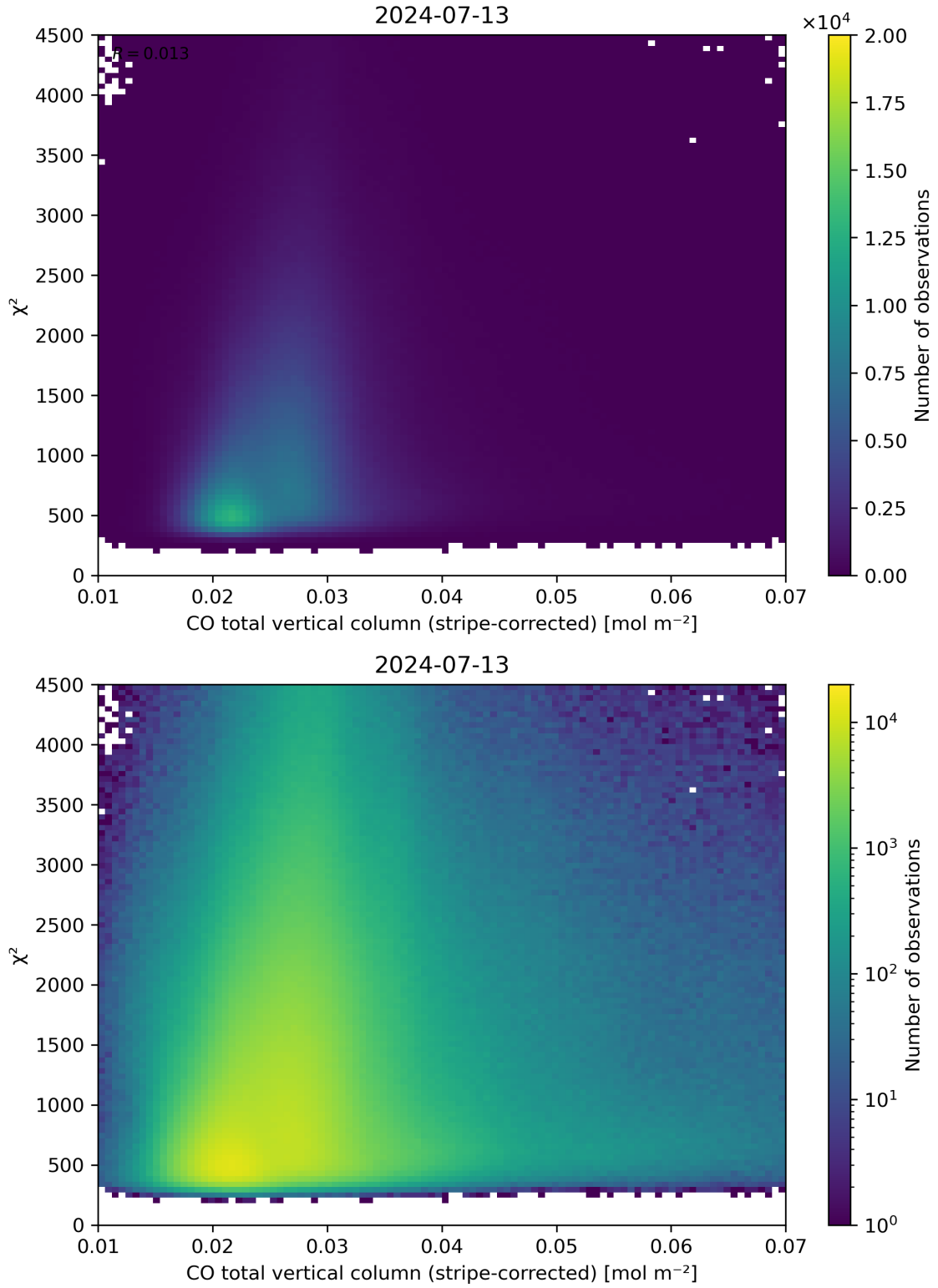
Figure 37: Scatter density plot of “CO total vertical column (stripe-corrected)” against “ \chi^2 ” for 2024-07-12 to 2024-07-14.
