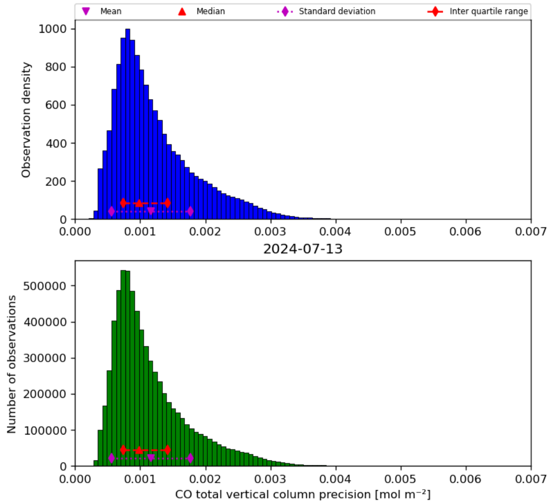
Figure 20: Histogram of “CO total vertical column precision” for 2024-07-12 to 2024-07-14
