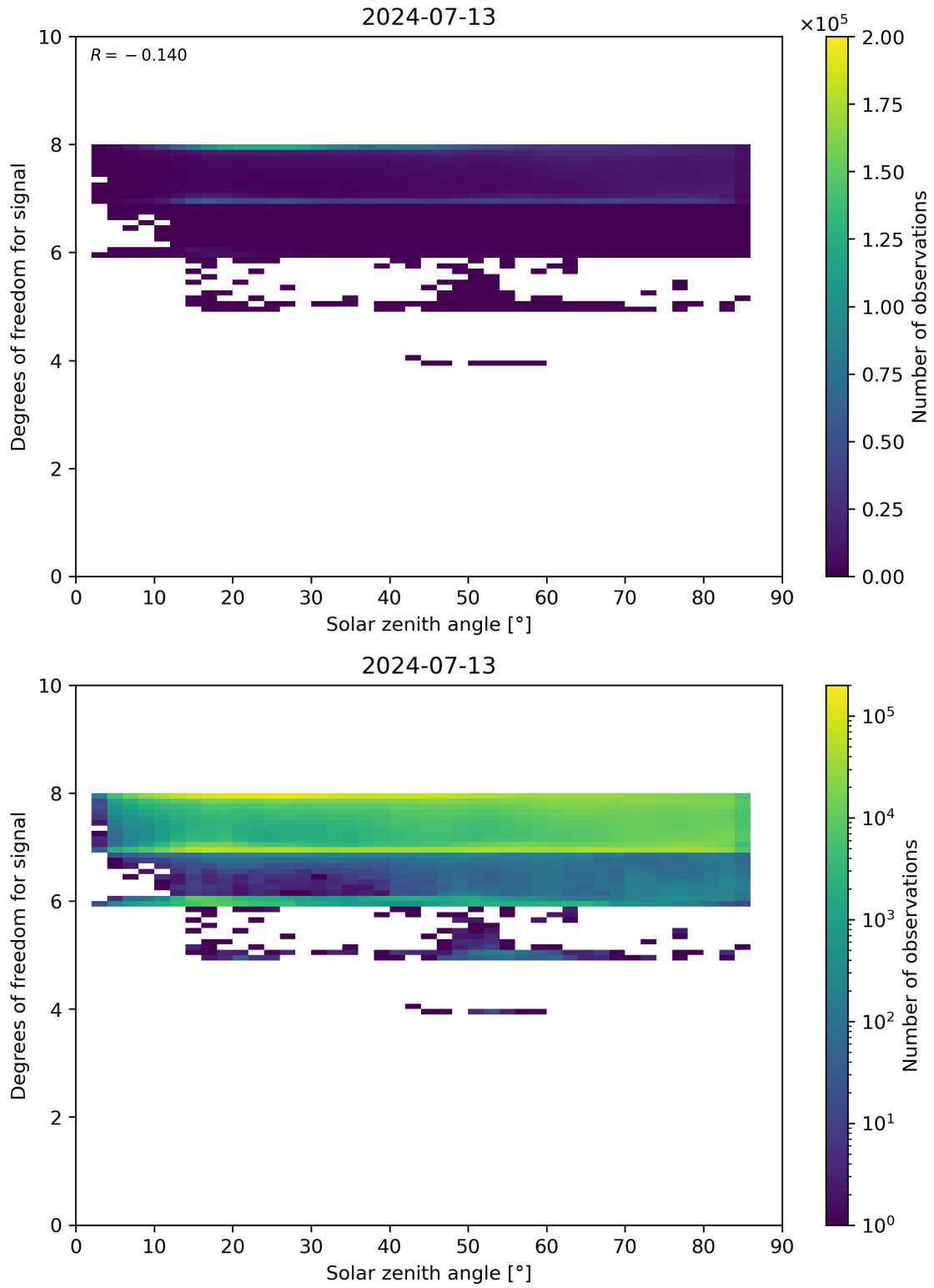
Figure 65: Scatter density plot of “Solar zenith angle” against “Degrees of freedom for signal” for 2024-07-12 to 2024-07-14.
