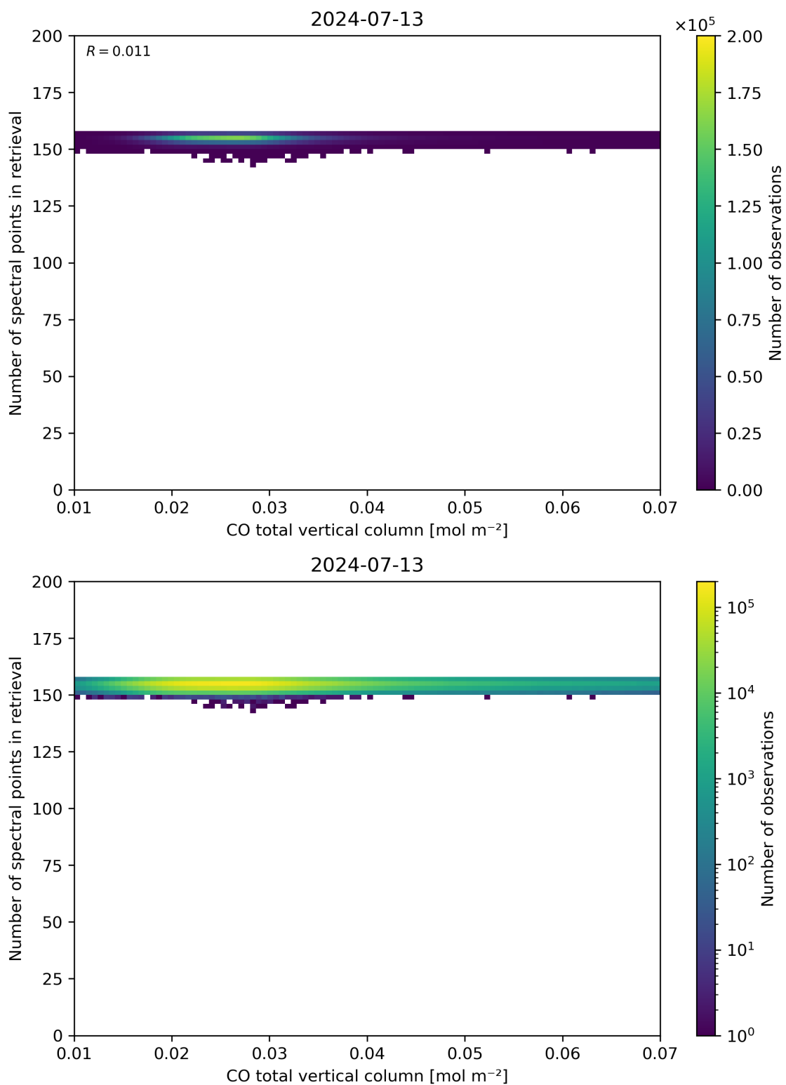
Figure 43: Scatter density plot of “CO total vertical column” against “Number of spectral points in retrieval” for 2024-07-12 to 2024-07-14.
