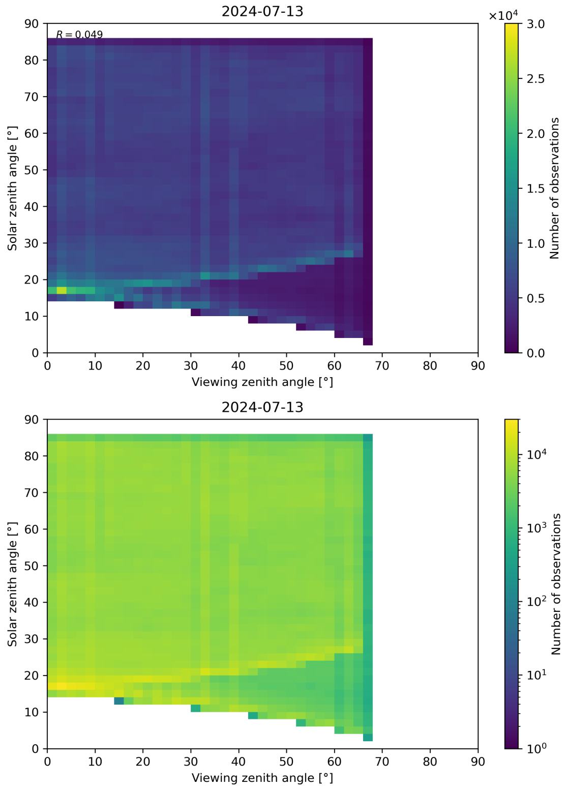
Figure 77: Scatter density plot of “Viewing zenith angle” against “Solar zenith angle” for 2024-07-12 to 2024-07-14.
