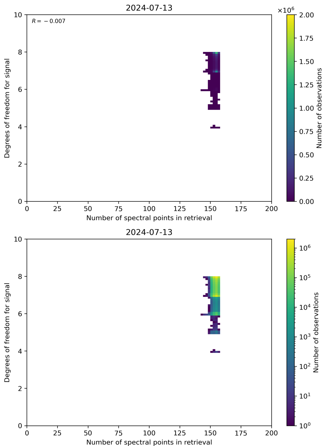
Figure 59: Scatter density plot of “Number of spectral points in retrieval” against “Degrees of freedom for signal” for 2024-07-12 to 2024-07-14.
