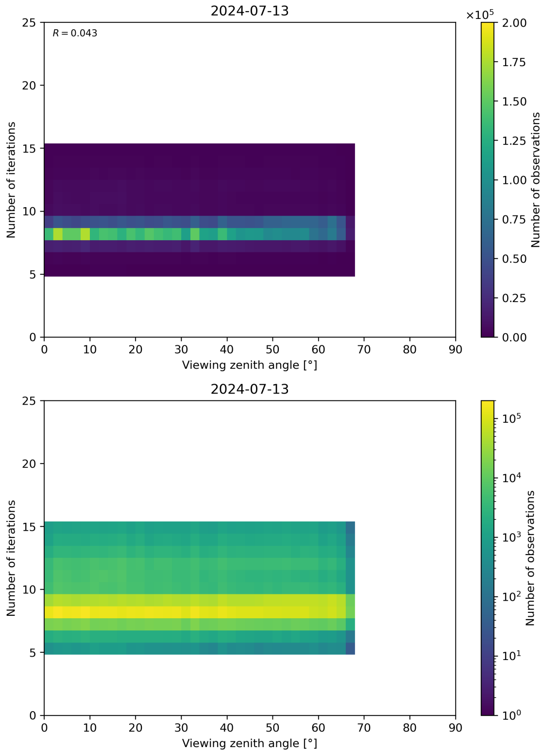
Figure 75: Scatter density plot of “Viewing zenith angle” against “Number of iterations” for 2024-07-12 to 2024-07-14.
