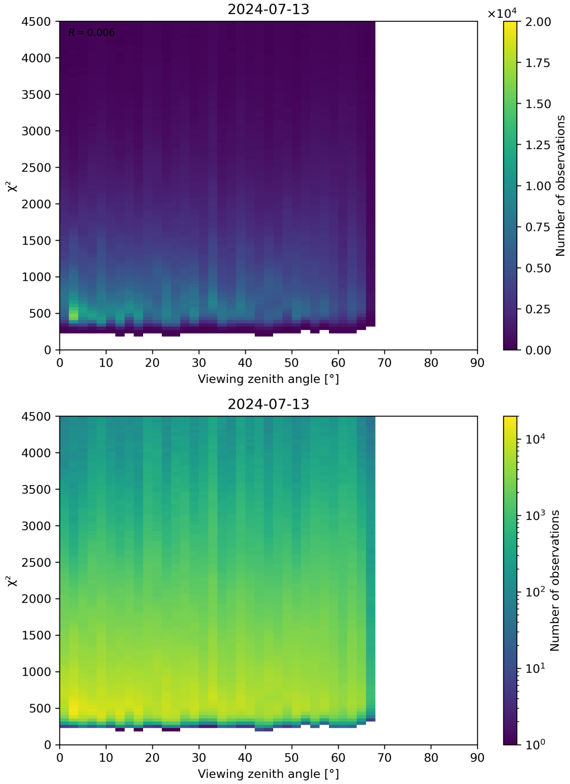
Figure 72: Scatter density plot of “Viewing zenith angle” against “ \chi^2 ” for 2024-07-12 to 2024-07-14.
