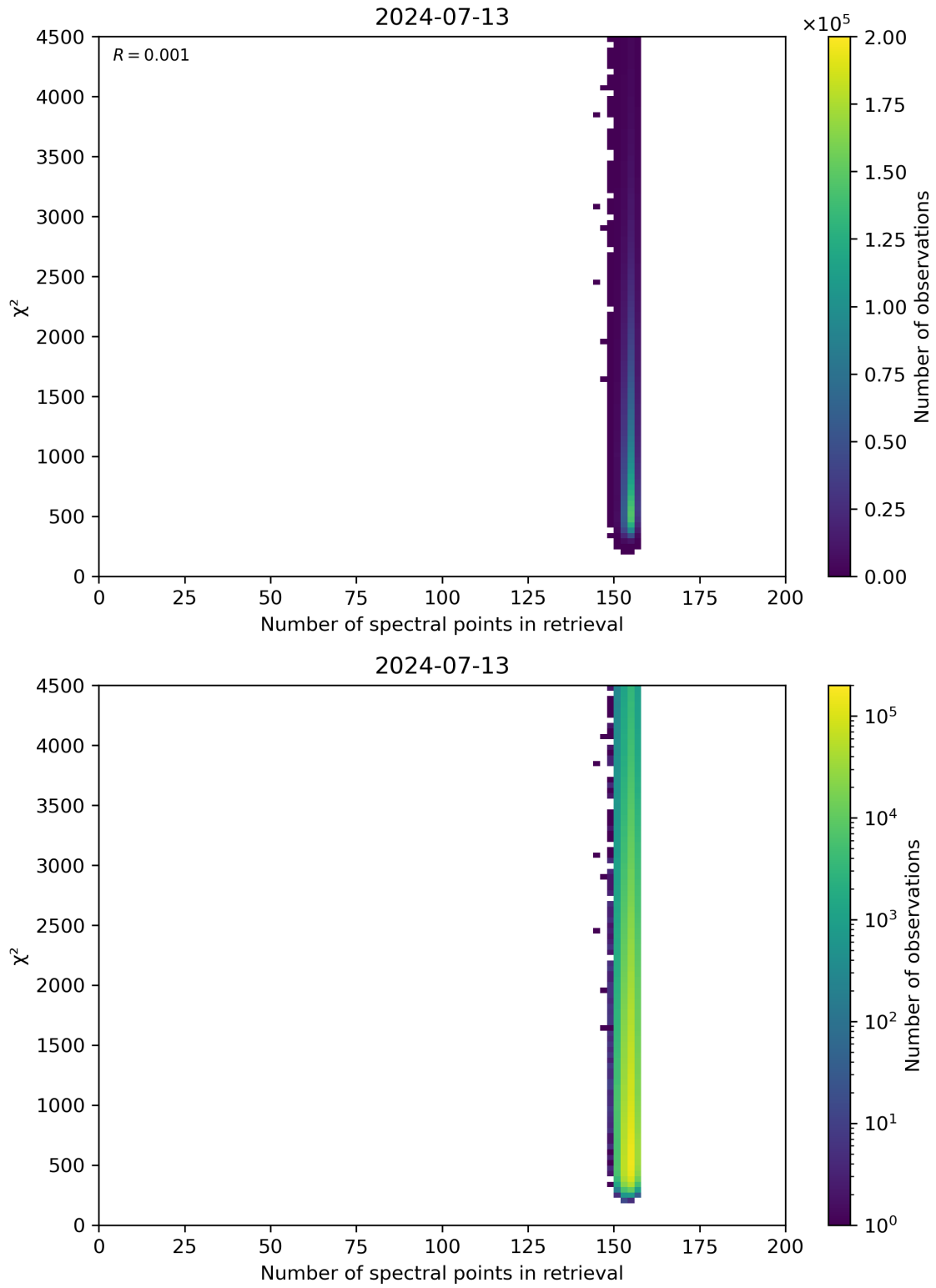
Figure 58: Scatter density plot of “Number of spectral points in retrieval” against “ \chi^2 ” for 2024-07-12 to 2024-07-14.
