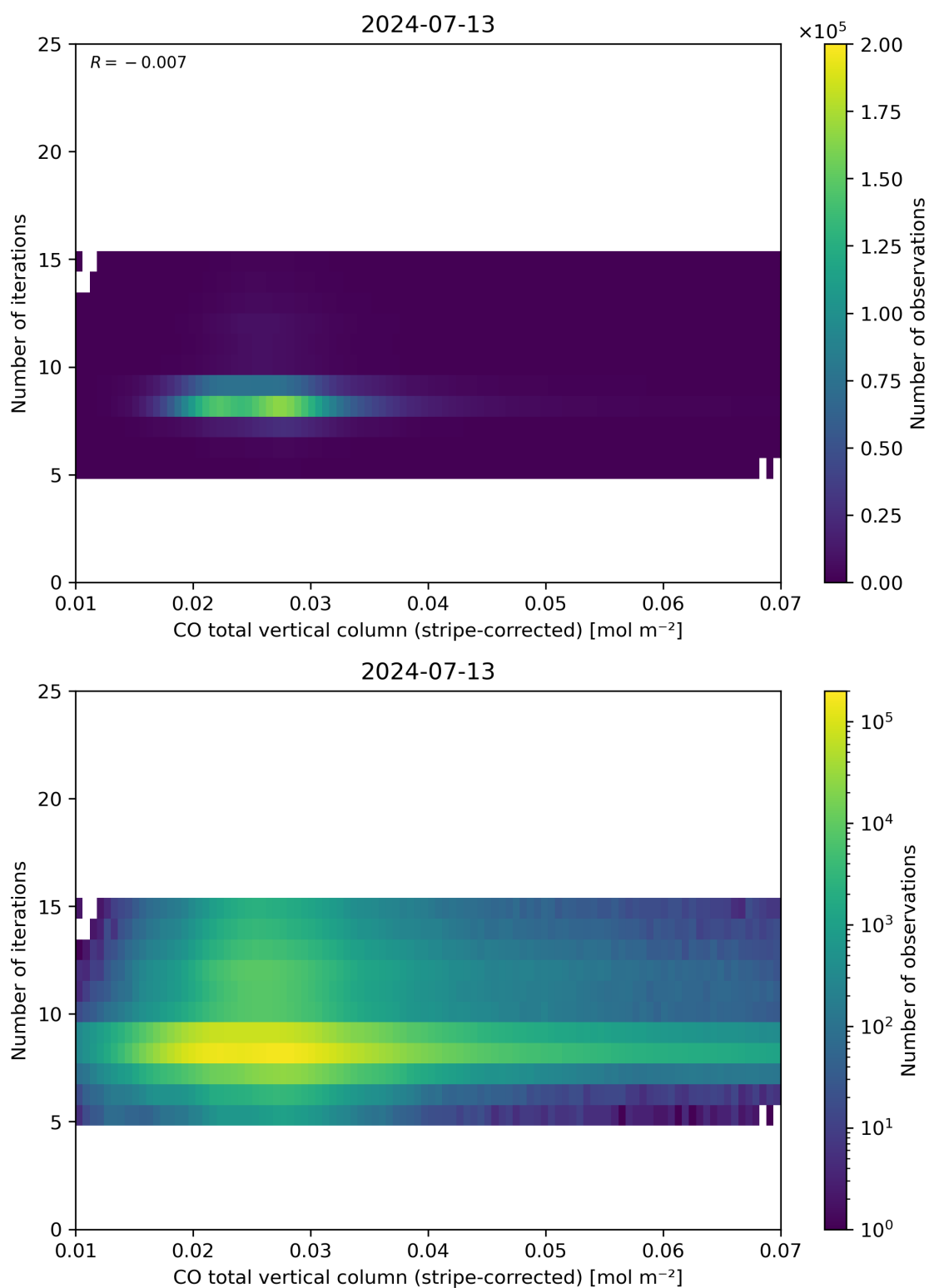
Figure 39: Scatter density plot of “CO total vertical column (stripe-corrected)” against “Number of iterations” for 2024-07-12 to 2024-07-14.
