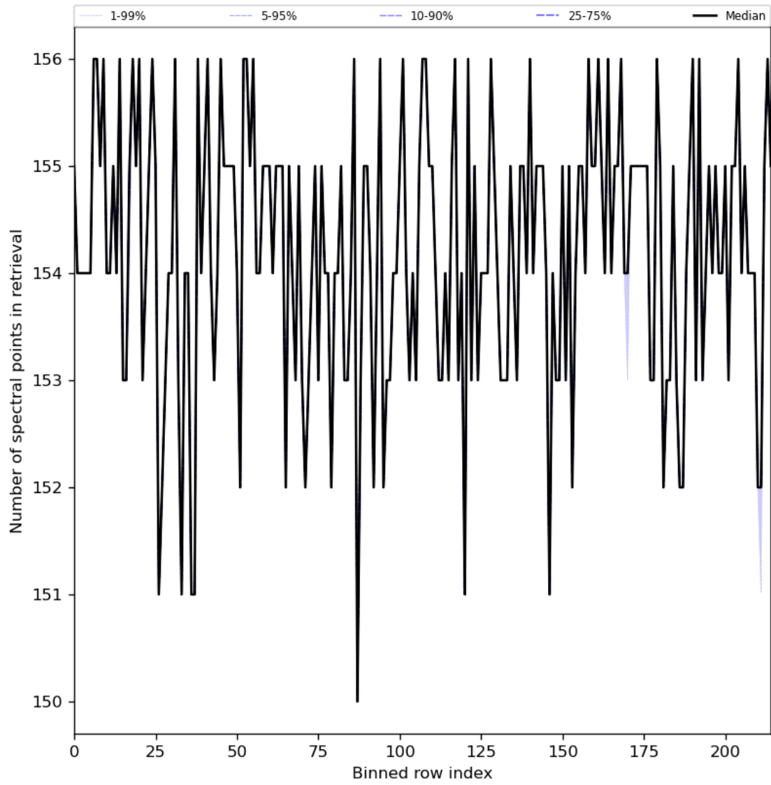
Figure 29: Along track statistics of “Number of spectral points in retrieval” for 2024-07-12 to 2024-07-14
