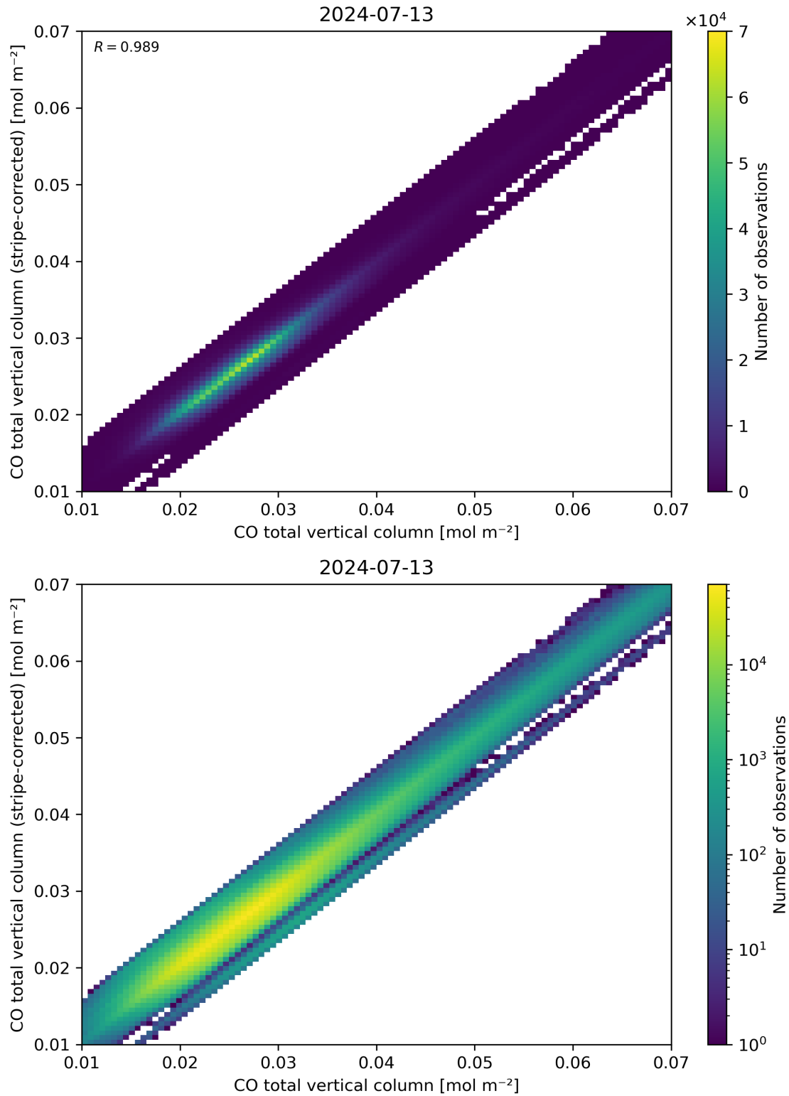
Figure 33: Scatter density plot of “CO total vertical column” against “CO total vertical column (stripe-corrected)” for 2024-07-12 to 2024-07-14.
