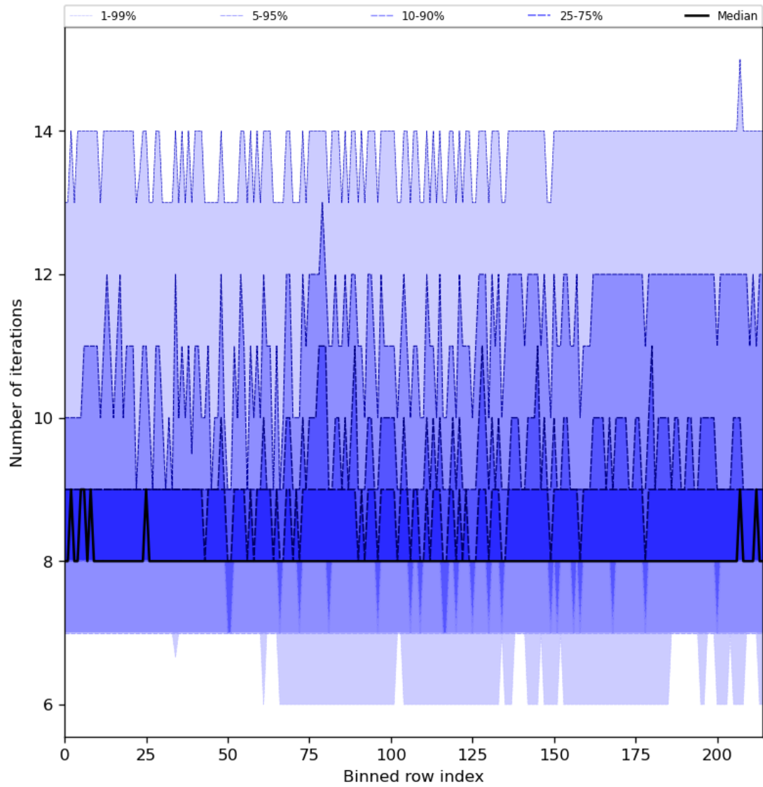
Figure 32: Along track statistics of “Number of iterations” for 2024-07-12 to 2024-07-14
