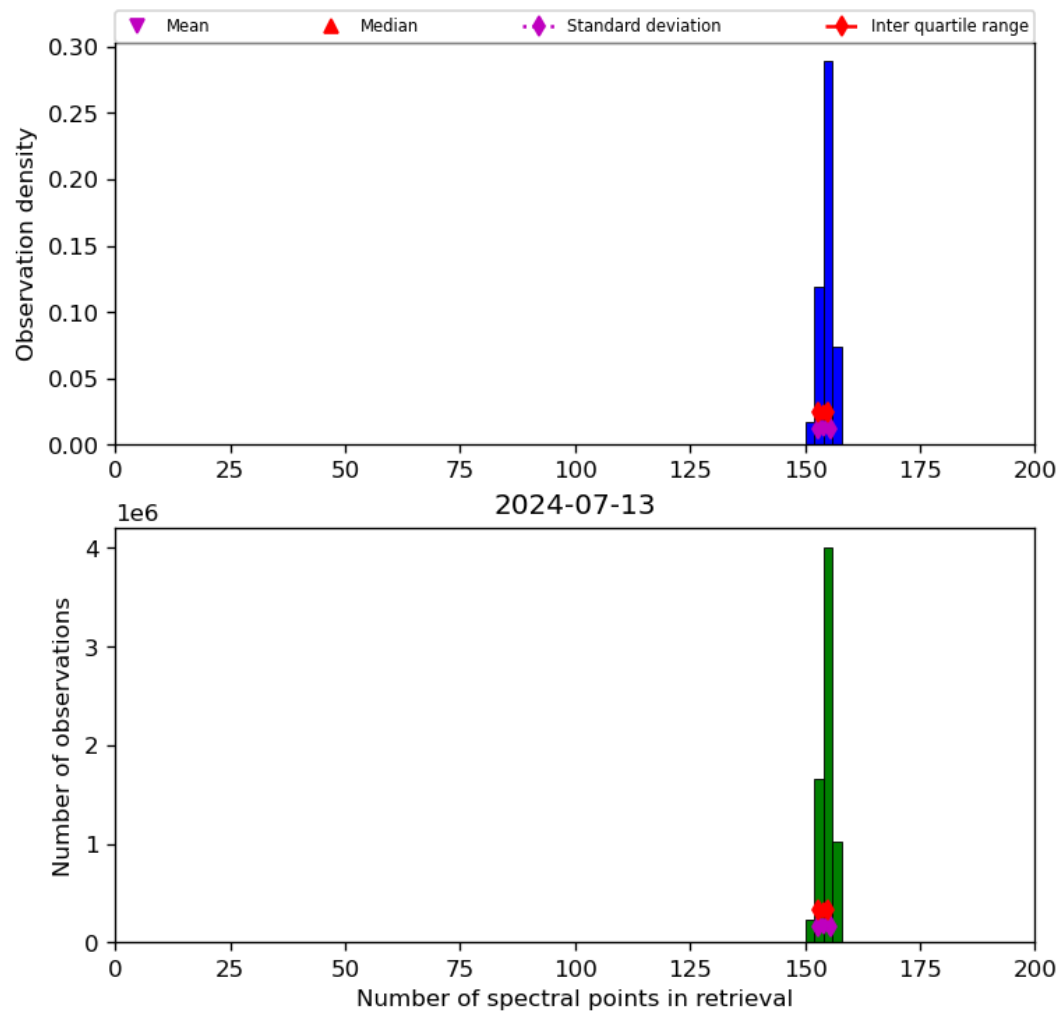
Figure 21: Histogram of “Number of spectral points in retrieval” for 2024-07-12 to 2024-07-14
