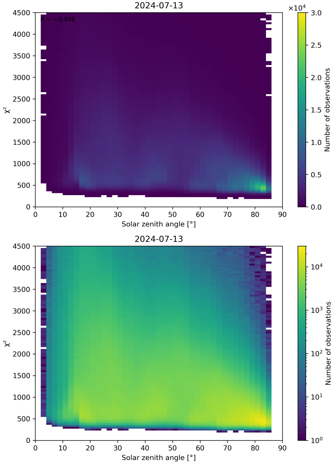
Figure 64: Scatter density plot of “Solar zenith angle” against “ \chi^2 ” for 2024-07-12 to 2024-07-14.
