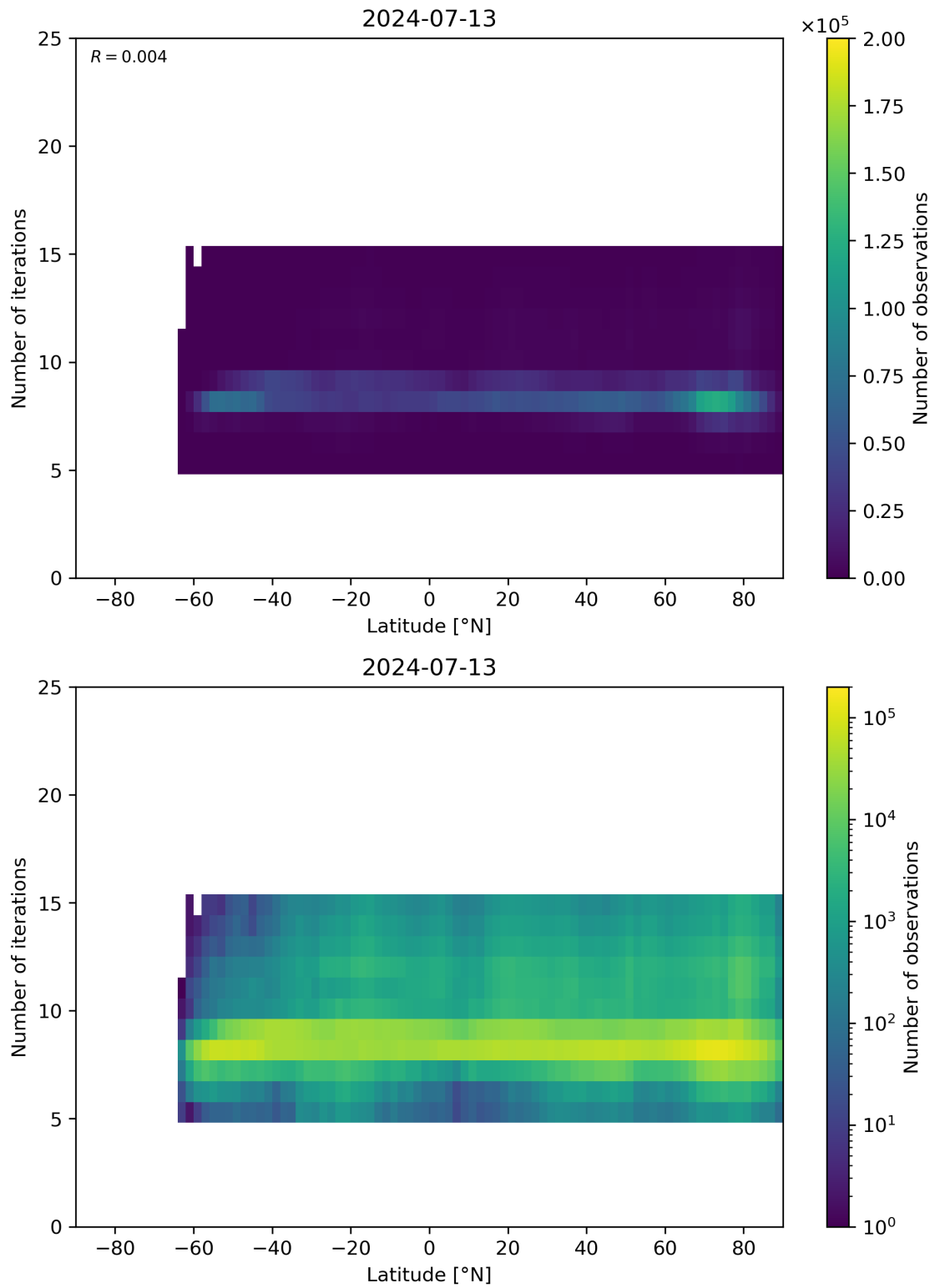
Figure 56: Scatter density plot of “Latitude” against “Number of iterations” for 2024-07-12 to 2024-07-14.
