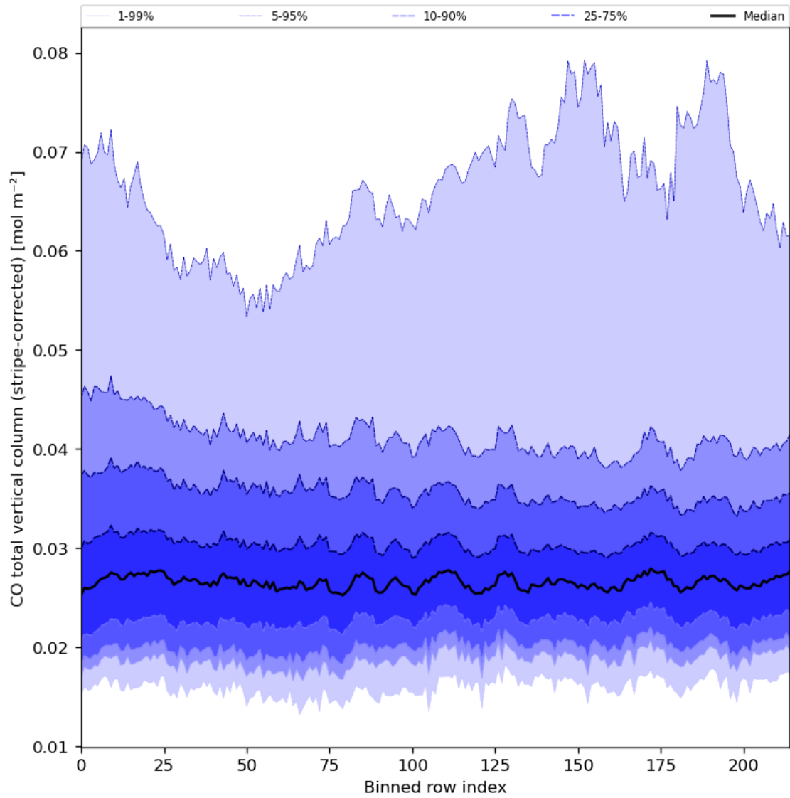
Figure 27: Along track statistics of “CO total vertical column (stripe-corrected)” for 2024-07-12 to 2024-07-14
