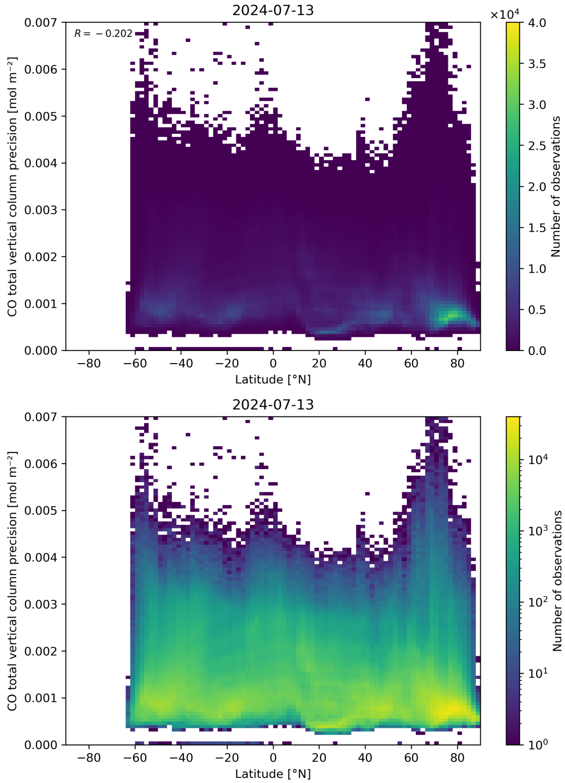
Figure 53: Scatter density plot of “Latitude” against “CO total vertical column precision” for 2024-07-12 to 2024-07-14.
