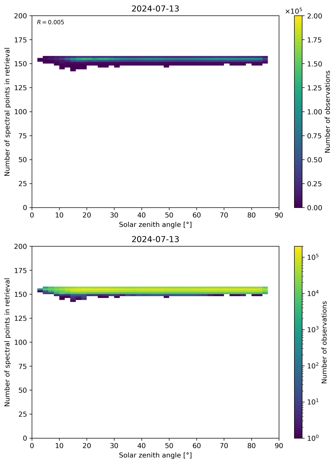
Figure 68: Scatter density plot of “Solar zenith angle” against “Number of spectral points in retrieval” for 2024-07-12 to 2024-07-14.
