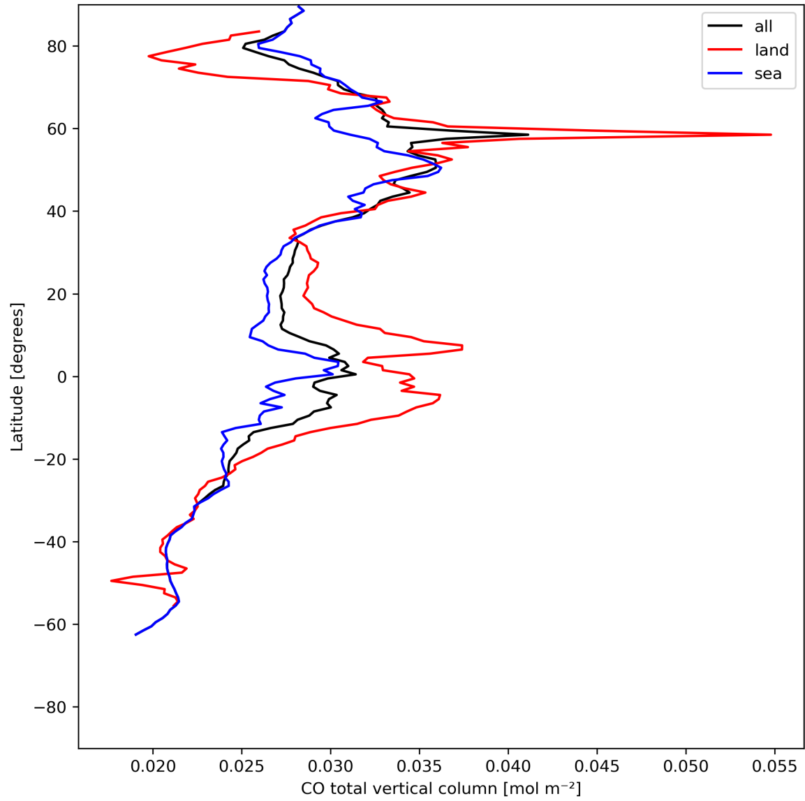
Figure 10: Zonal average of “CO total vertical column” for 2024-07-12 to 2024-07-14.
