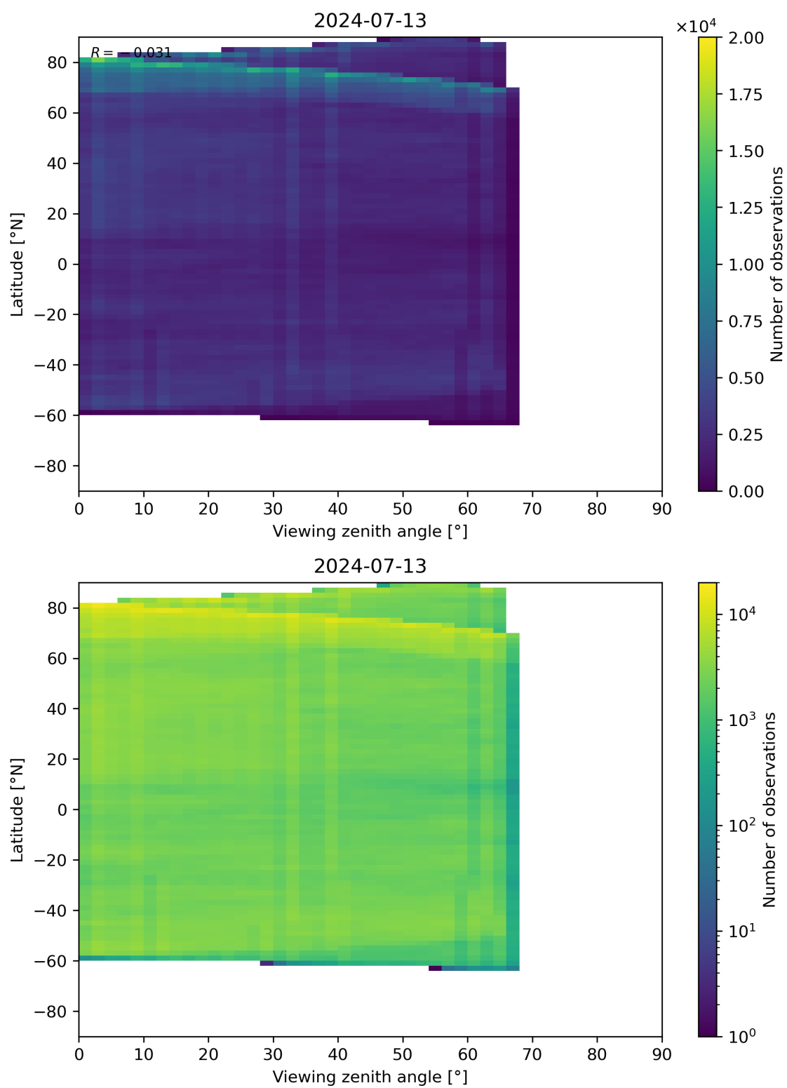
Figure 74: Scatter density plot of “Viewing zenith angle” against “Latitude” for 2024-07-12 to 2024-07-14.
