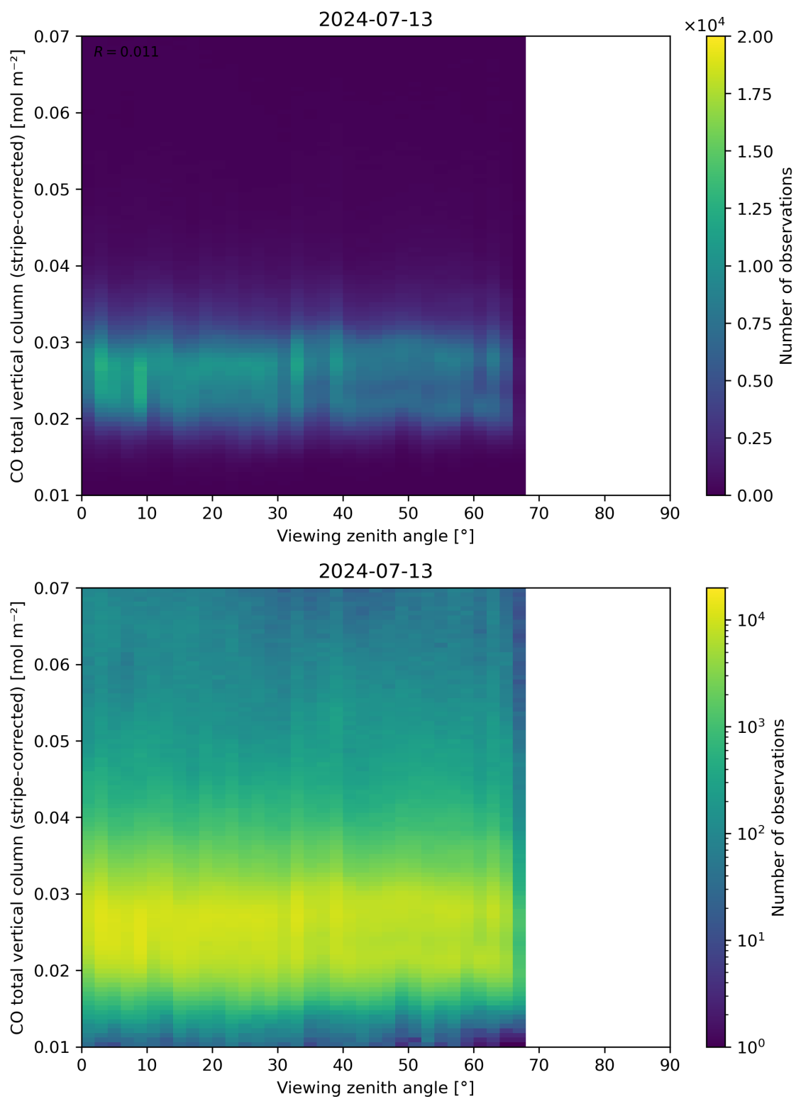
Figure 70: Scatter density plot of “Viewing zenith angle” against “CO total vertical column (stripe-corrected)” for 2024-07-12 to 2024-07-14.
