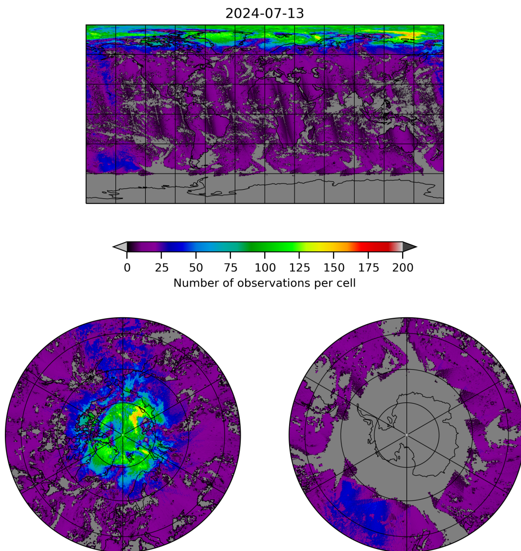
Figure 8: Map of the number of observations for 2024-07-12 to 2024-07-14
