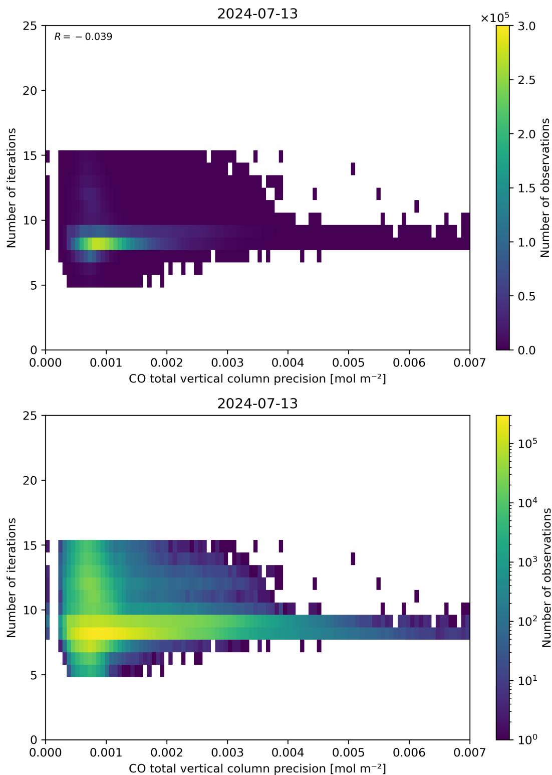
Figure 46: Scatter density plot of “CO total vertical column precision” against “Number of iterations” for 2024-07-12 to 2024-07-14.
