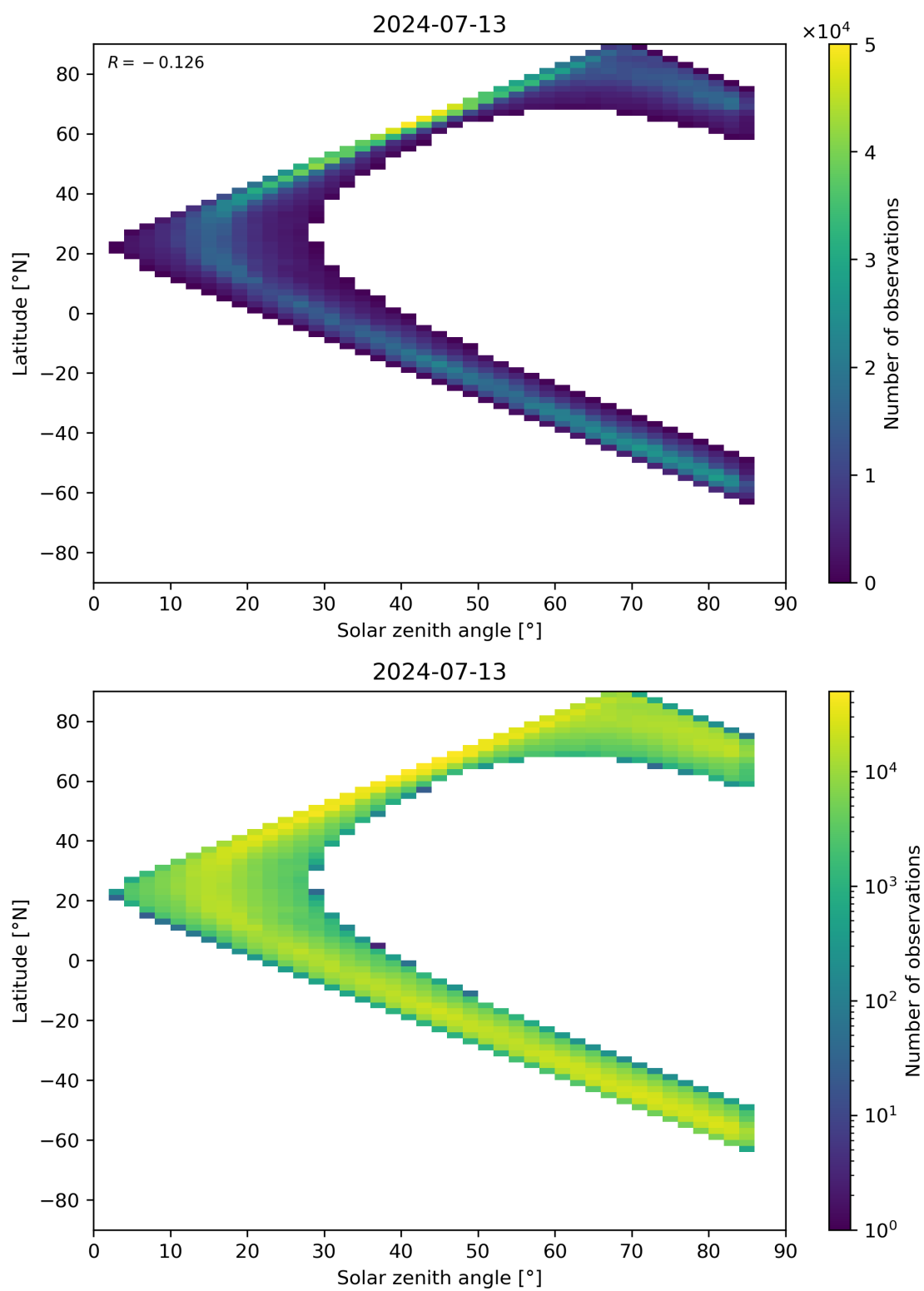
Figure 66: Scatter density plot of “Solar zenith angle” against “Latitude” for 2024-07-12 to 2024-07-14.
