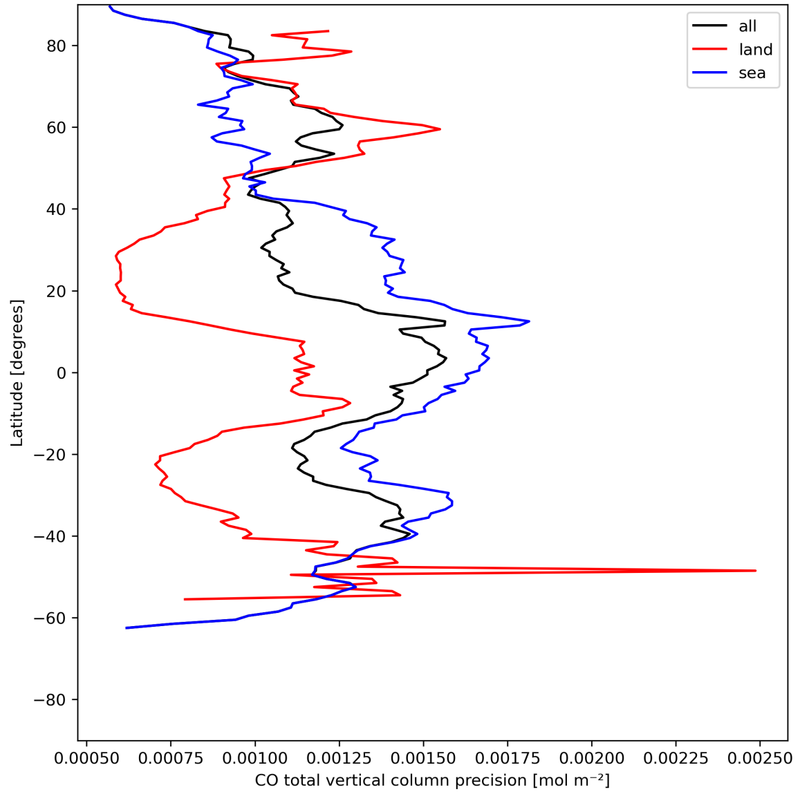
Figure 12: Zonal average of "CO total vertical column precision" for 2024-07-12 to 2024-07-14.
