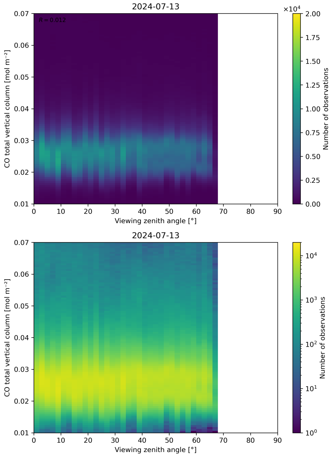
Figure 69: Scatter density plot of “Viewing zenith angle” against “CO total vertical column” for 2024-07-12 to 2024-07-14.
