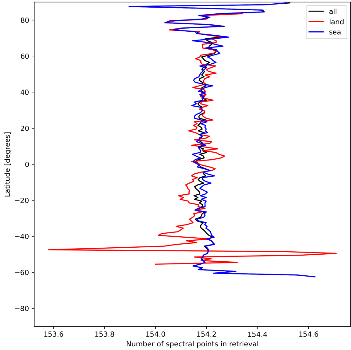
Figure 13: Zonal average of “Number of spectral points in retrieval” for 2024-07-12 to 2024-07-14.
