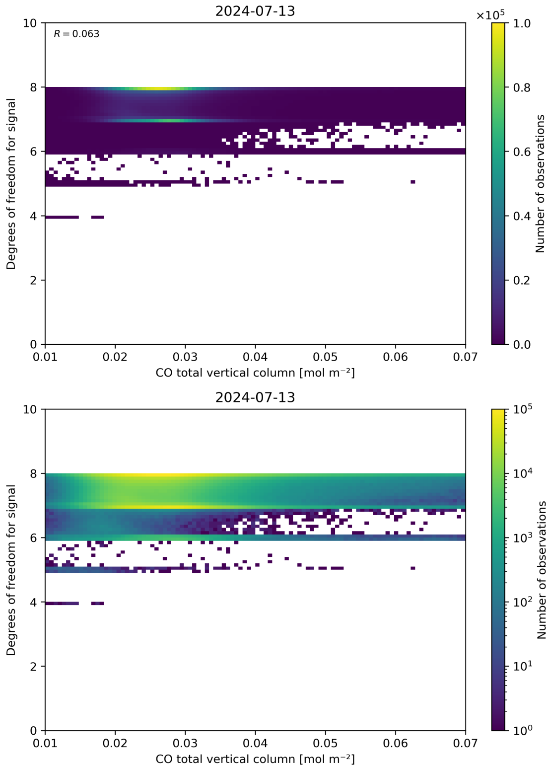
Figure 41: Scatter density plot of “CO total vertical column” against “Degrees of freedom for signal” for 2024-07-12 to 2024-07-14.
