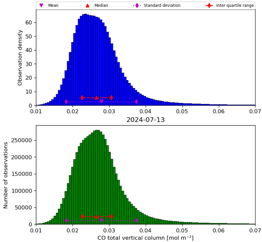
Figure 18: Histogram of “CO total vertical column” for 2024-07-12 to 2024-07-14
