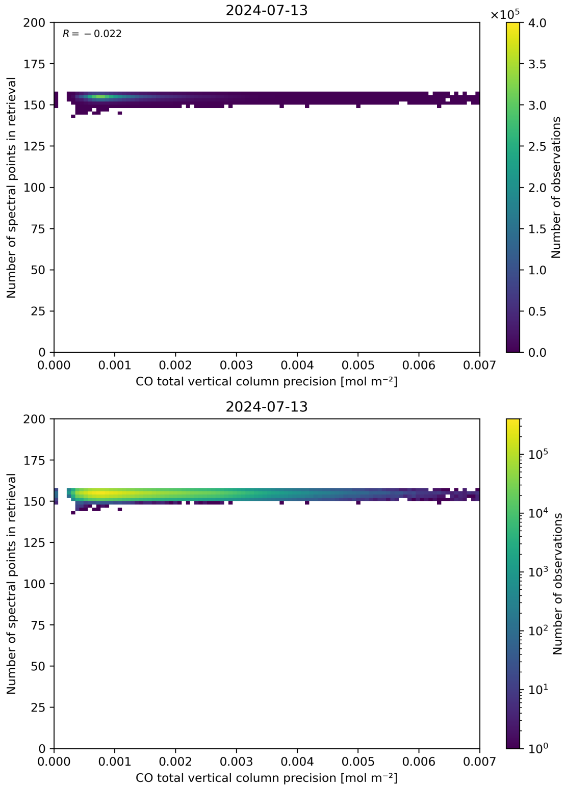
Figure 47: Scatter density plot of “CO total vertical column precision” against “Number of spectral points in retrieval” for 2024-07-12 to 2024-07-14.
