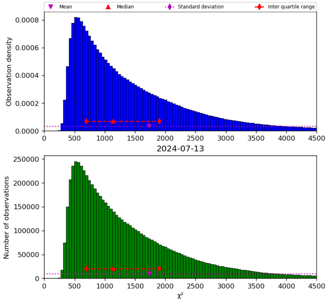
Figure 22: Histogram of “ \chi^2 ” for 2024-07-12 to 2024-07-14
