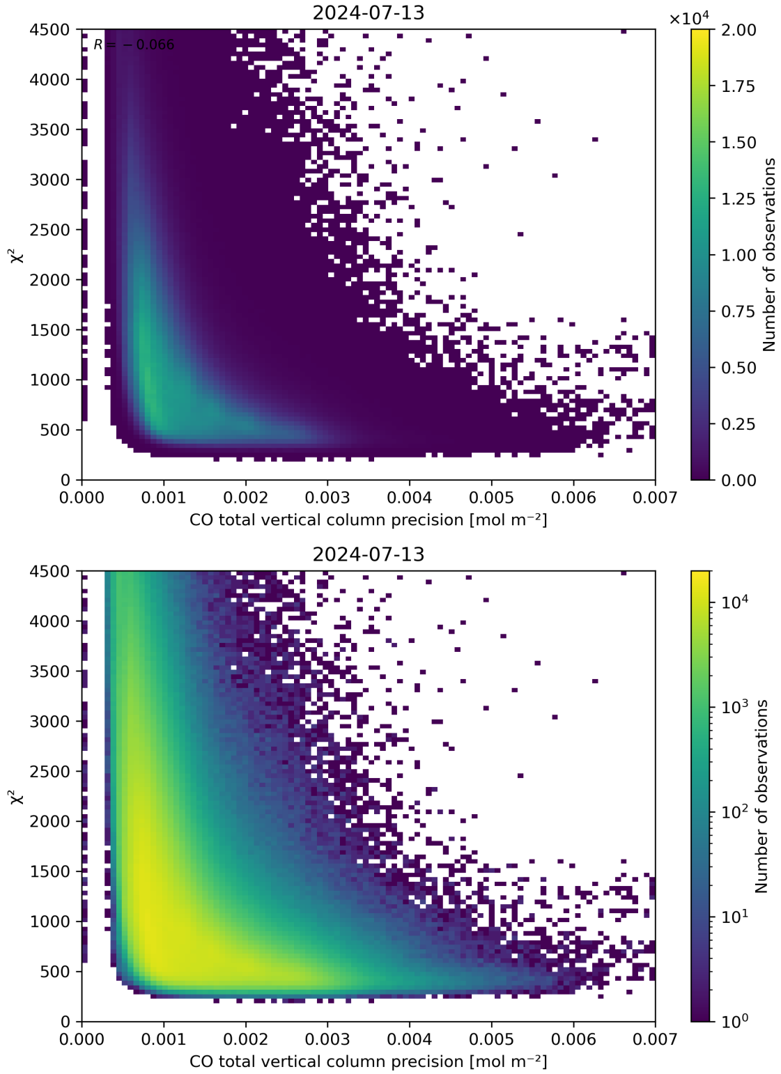
Figure 44: Scatter density plot of “CO total vertical column precision” against “ \chi^2 ” for 2024-07-12 to 2024-07-14.
