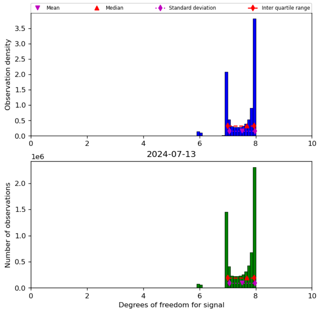
Figure 23: Histogram of “Degrees of freedom for signal” for 2024-07-12 to 2024-07-14
