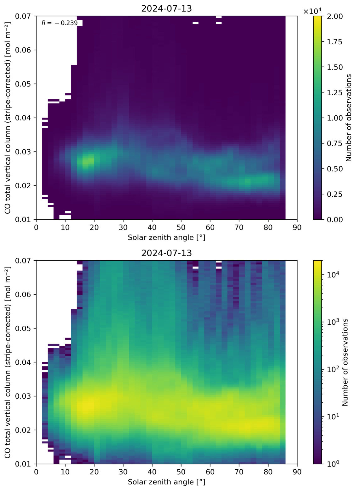
Figure 62: Scatter density plot of “Solar zenith angle” against “CO total vertical column (stripe-corrected)” for 2024-07-12 to 2024-07-14.
