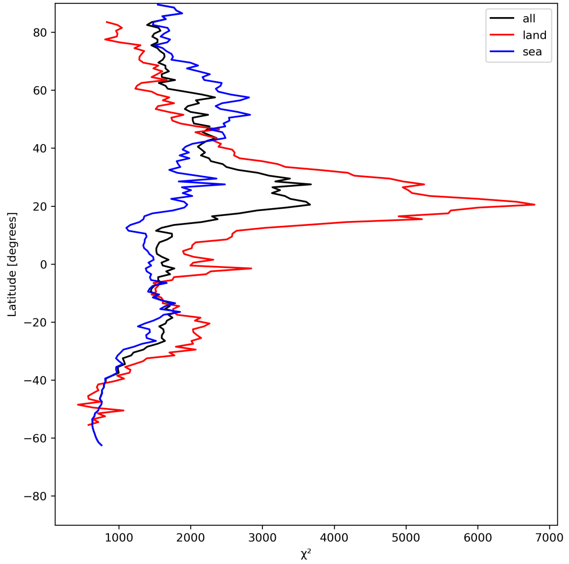
Figure 14: Zonal average of “ \chi^2 ” for 2024-07-12 to 2024-07-14.
