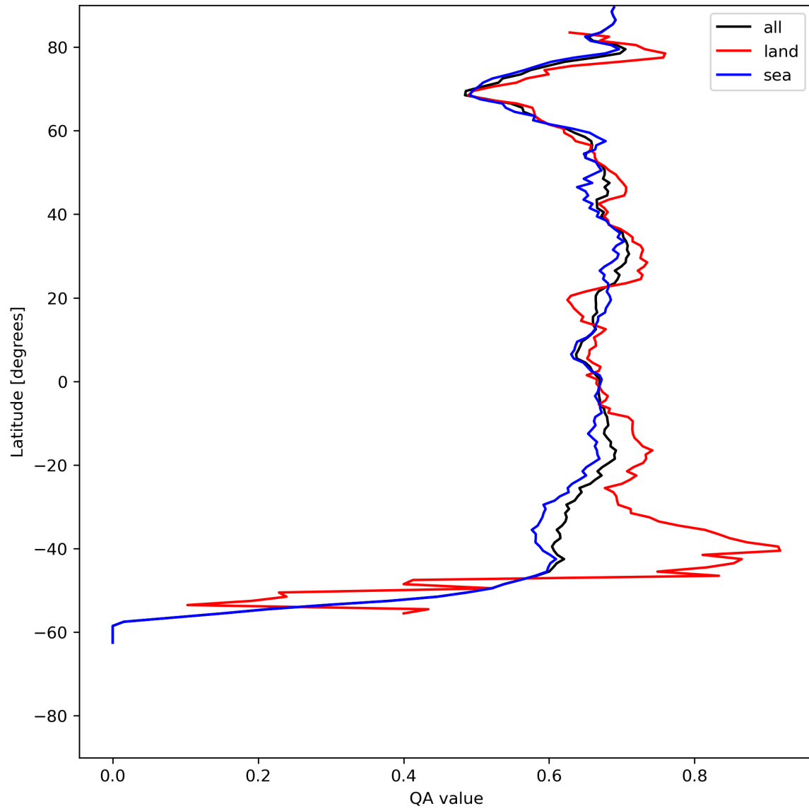
Figure 9: Zonal average of “QA value” for 2024-07-12 to 2024-07-14.
