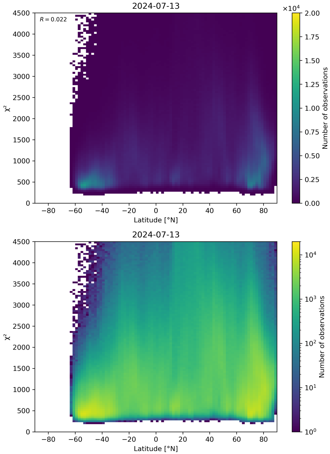
Figure 54: Scatter density plot of “Latitude” against “ \chi^2 ” for 2024-07-12 to 2024-07-14.
