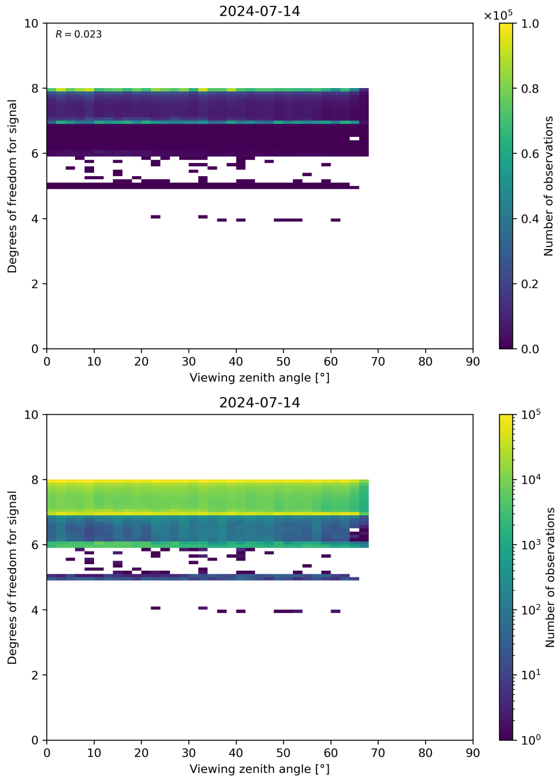
Figure 73: Scatter density plot of “Viewing zenith angle” against “Degrees of freedom for signal” for 2024-07-13 to 2024-07-15.
