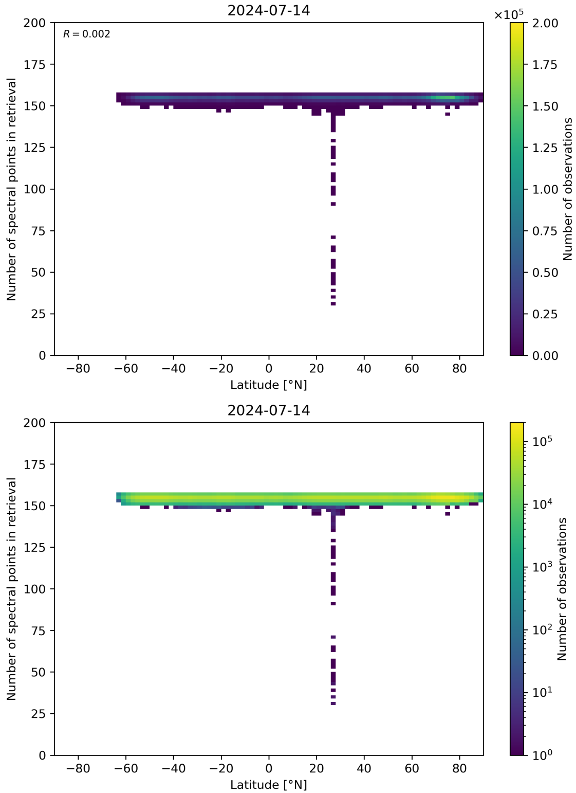
Figure 57: Scatter density plot of “Latitude” against “Number of spectral points in retrieval” for 2024-07-13 to 2024-07-15.
