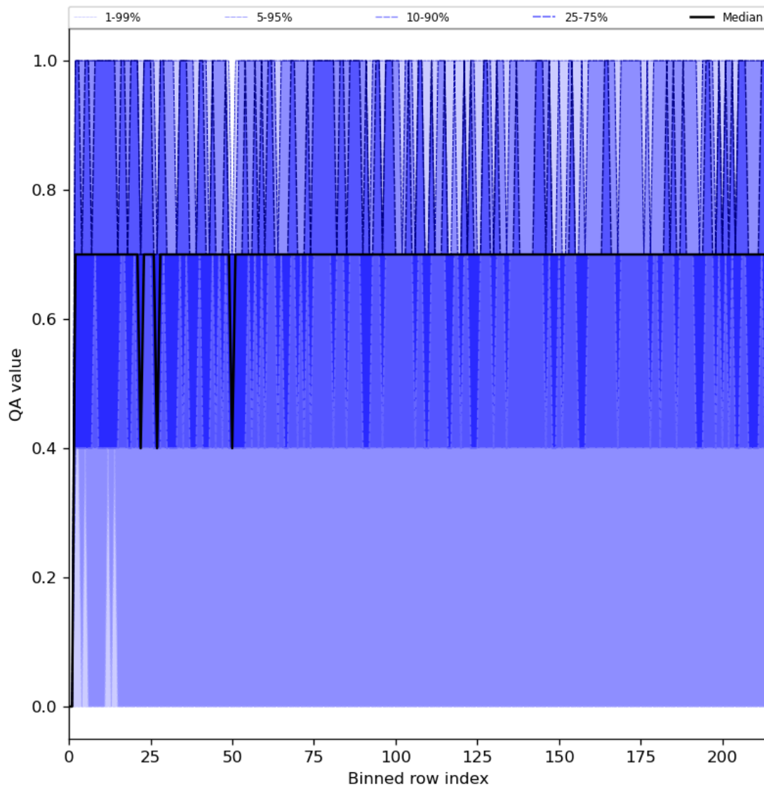
Figure 25: Along track statistics of “QA value” for 2024-07-13 to 2024-07-15
