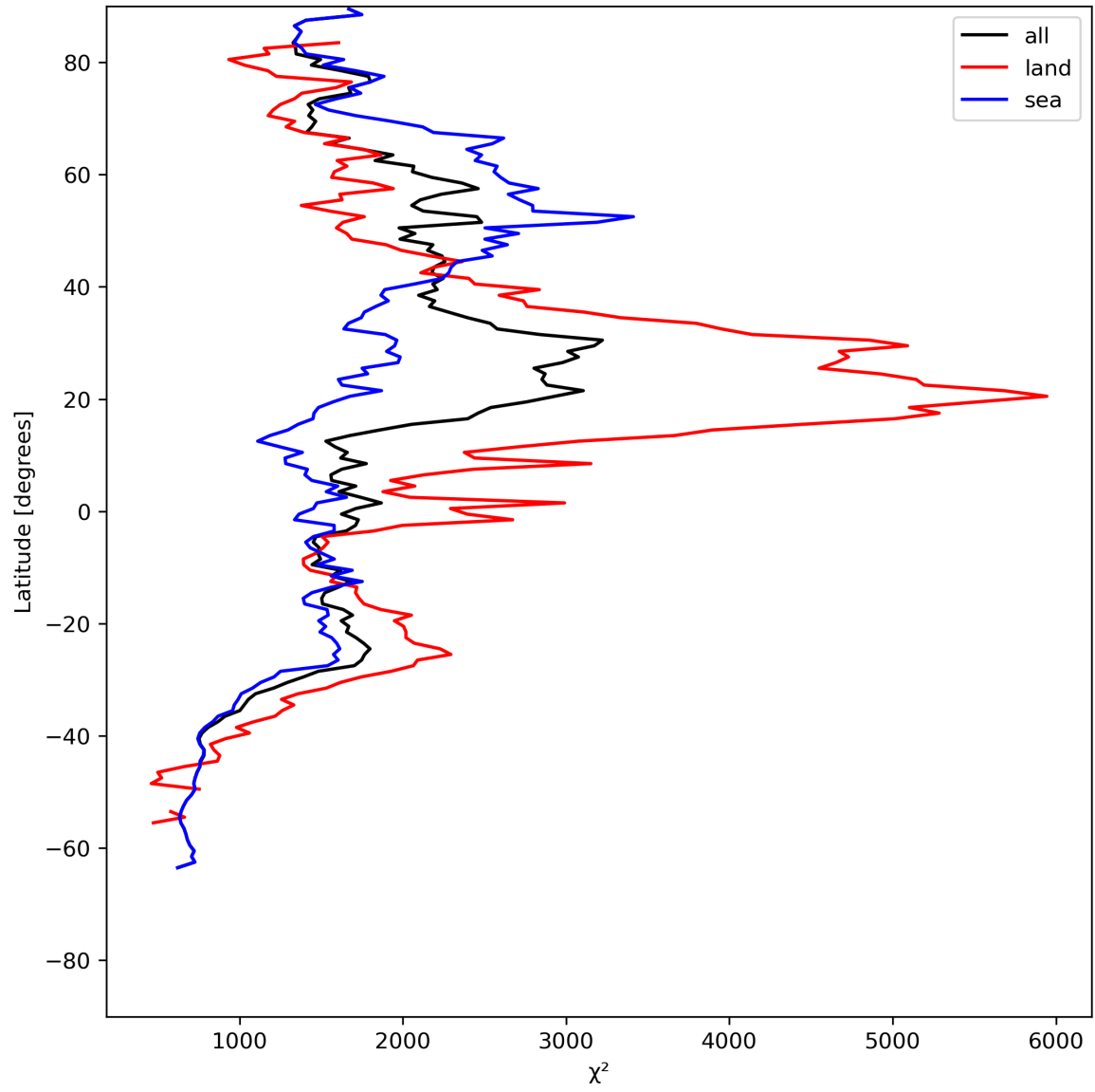
Figure 14: Zonal average of “ \chi^2 ” for 2024-07-13 to 2024-07-15.
