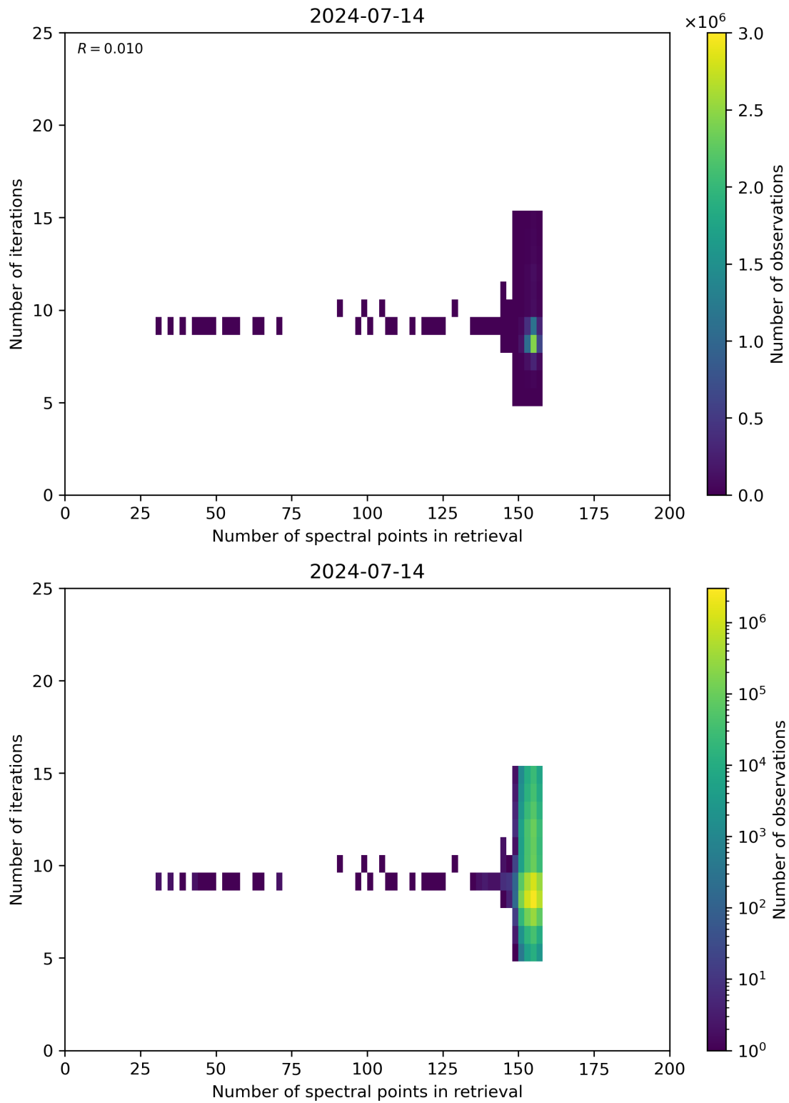
Figure 60: Scatter density plot of “Number of spectral points in retrieval” against “Number of iterations” for 2024-07-13 to 2024-07-15.
