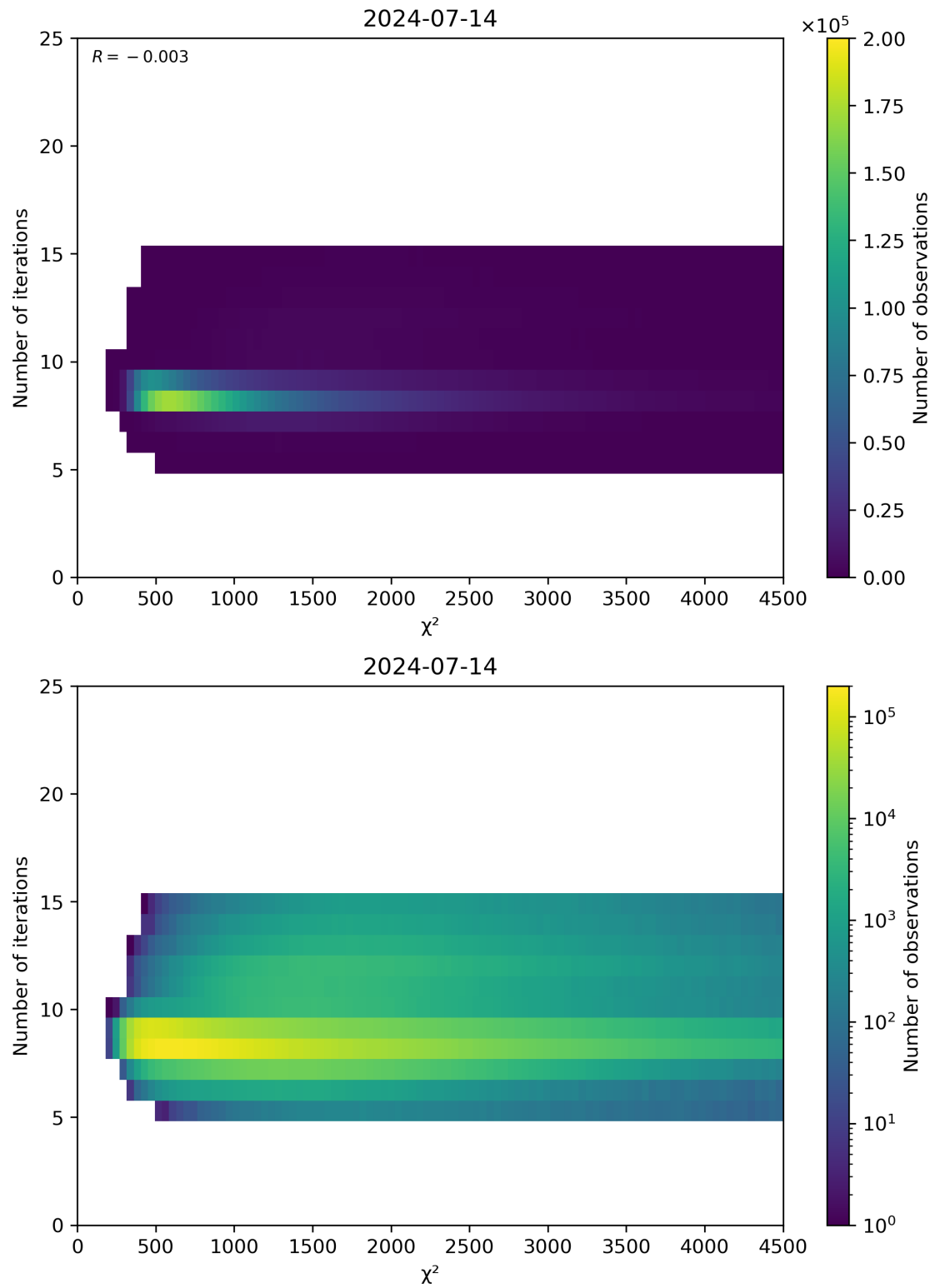
Figure 49: Scatter density plot of “ \chi^2 ” against “Number of iterations” for 2024-07-13 to 2024-07-15.
