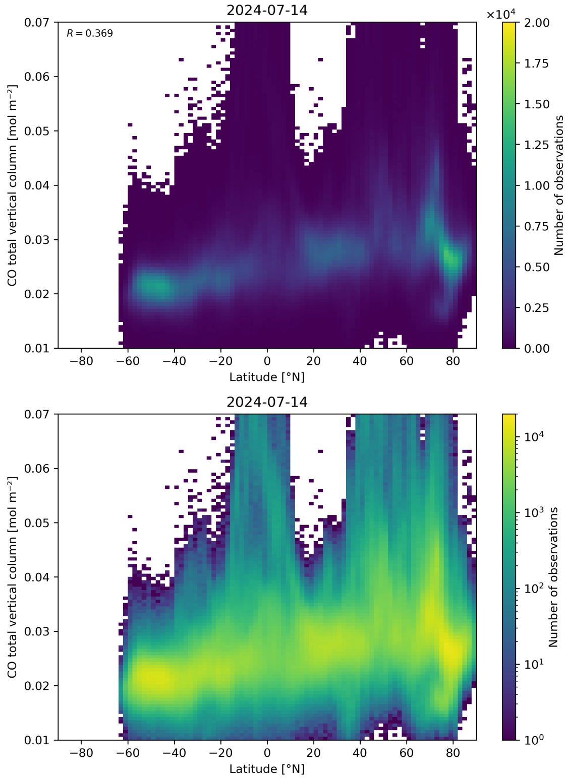
Figure 51: Scatter density plot of “Latitude” against “CO total vertical column” for 2024-07-13 to 2024-07-15.
