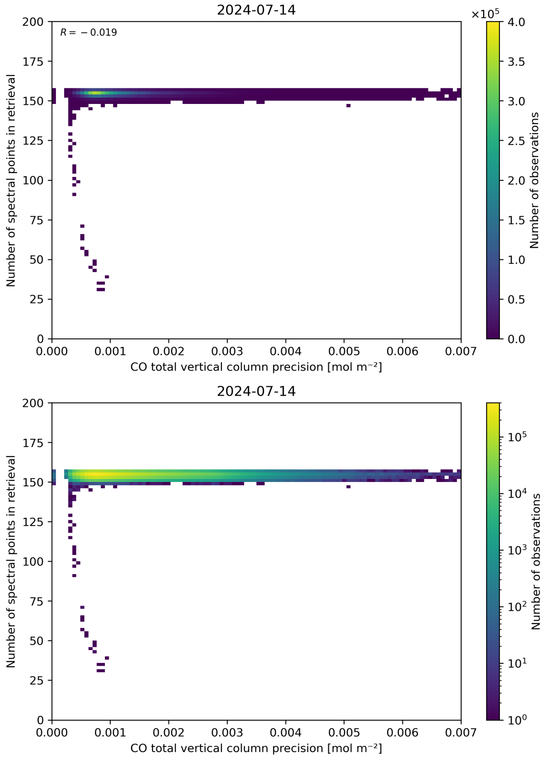
Figure 47: Scatter density plot of “CO total vertical column precision” against “Number of spectral points in retrieval” for 2024-07-13 to 2024-07-15.
