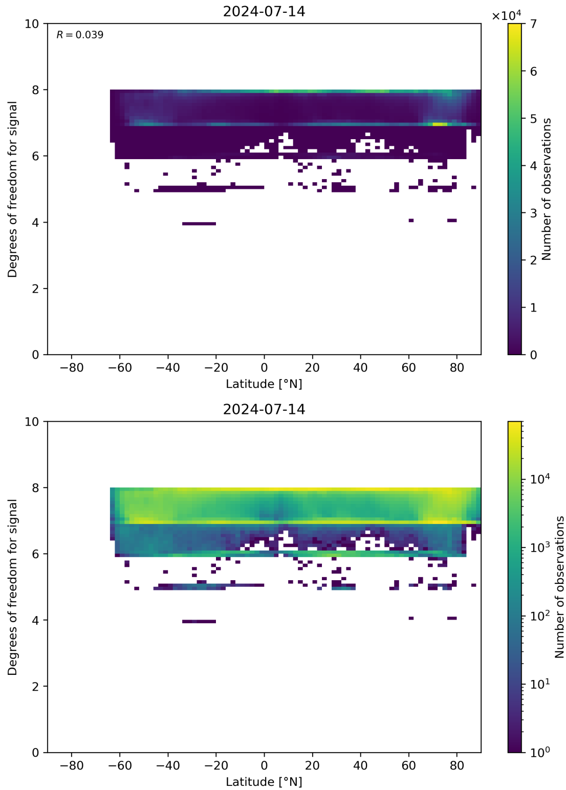
Figure 55: Scatter density plot of “Latitude” against “Degrees of freedom for signal” for 2024-07-13 to 2024-07-15.
