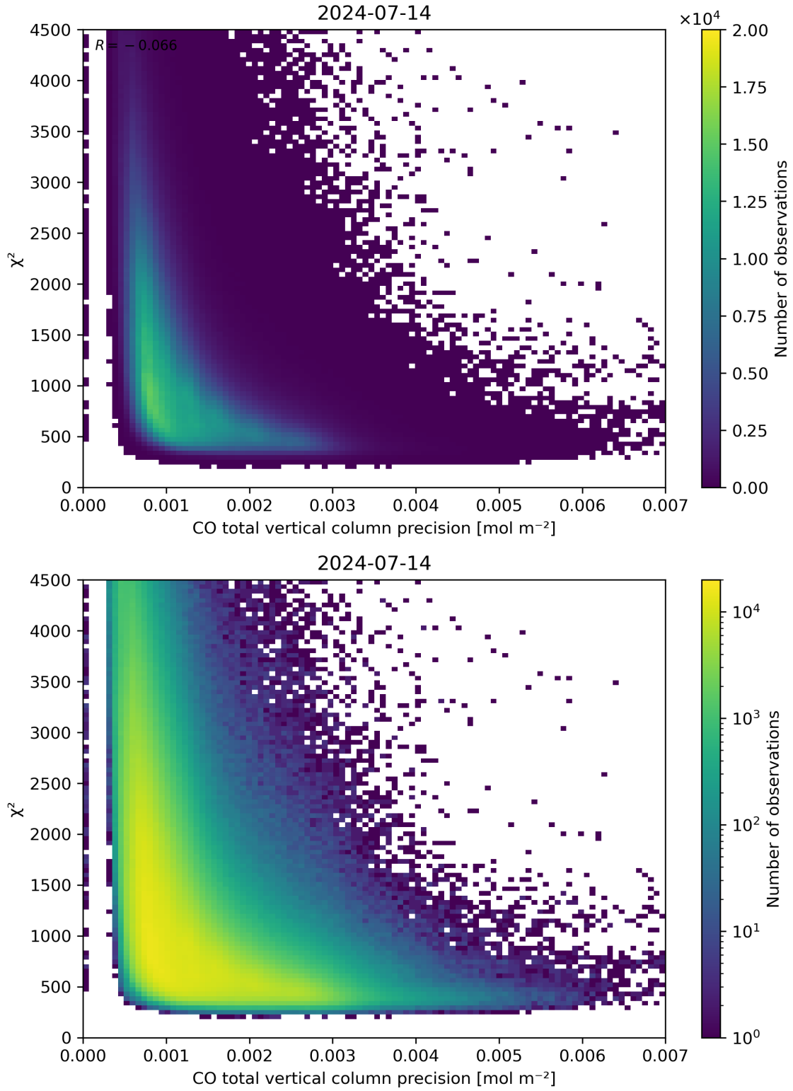
Figure 44: Scatter density plot of “CO total vertical column precision” against “ \chi^2 ” for 2024-07-13 to 2024-07-15.
