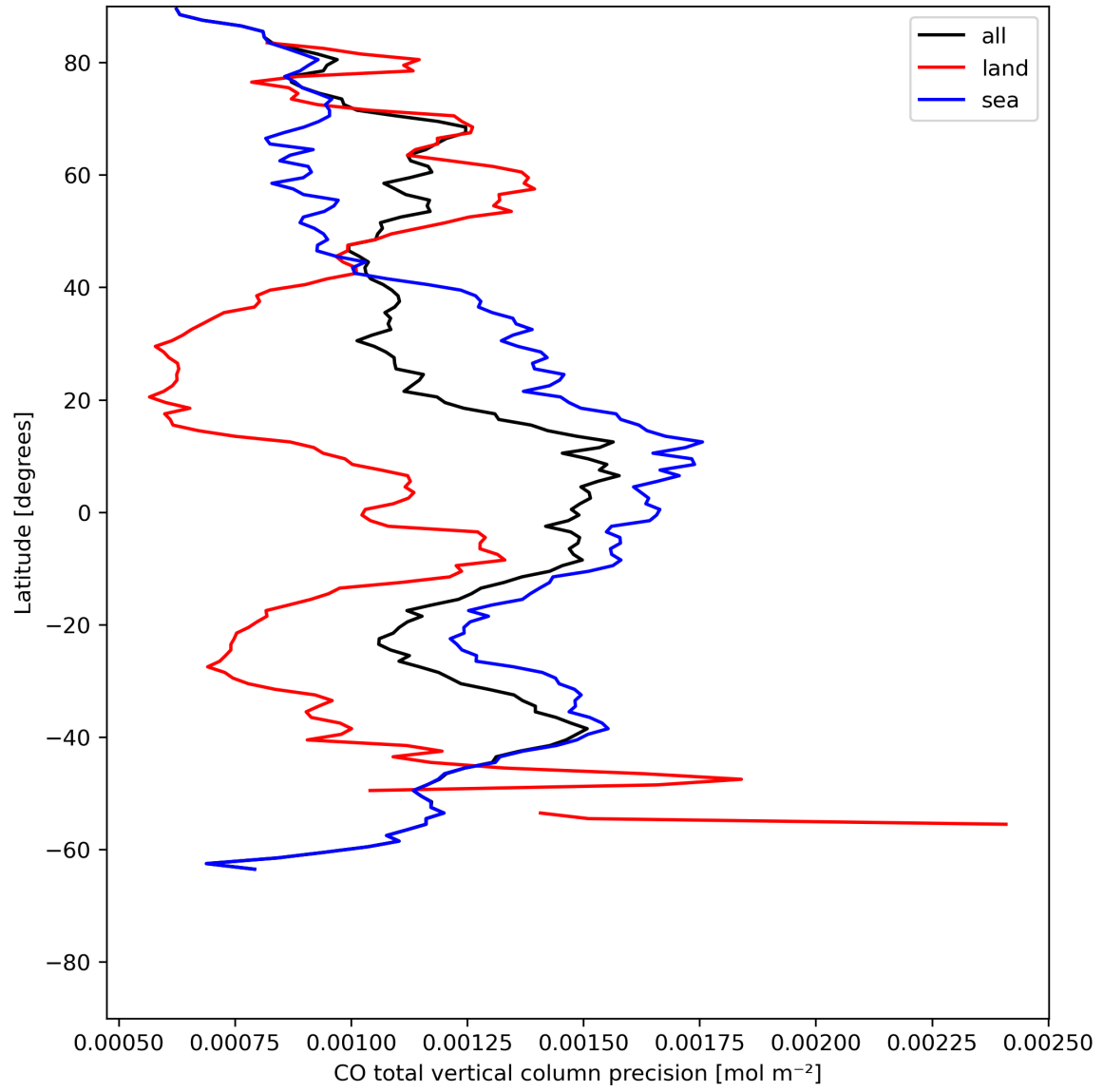
Figure 12: Zonal average of “CO total vertical column precision” for 2024-07-13 to 2024-07-15.
