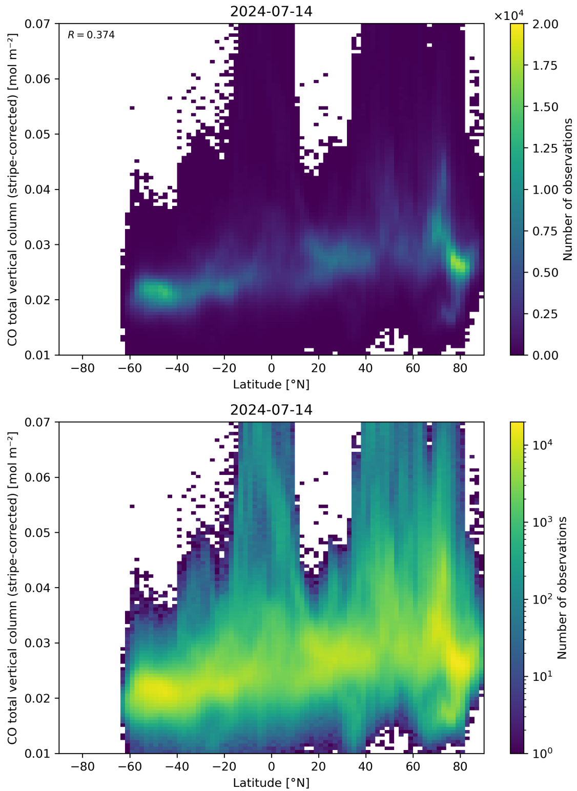
Figure 52: Scatter density plot of “Latitude” against “CO total vertical column (stripe-corrected)” for 2024-07-13 to 2024-07-15.
