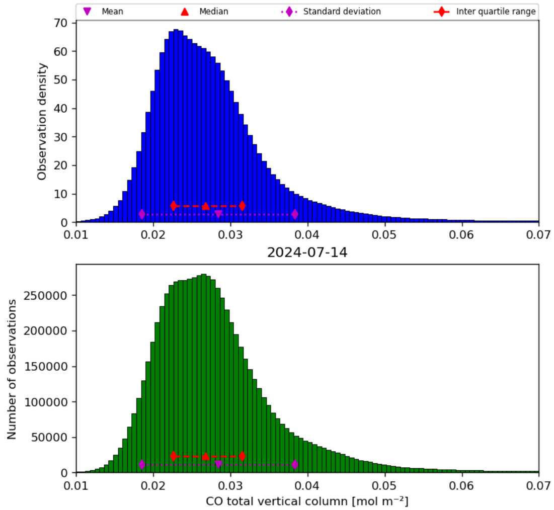
Figure 18: Histogram of “CO total vertical column” for 2024-07-13 to 2024-07-15
