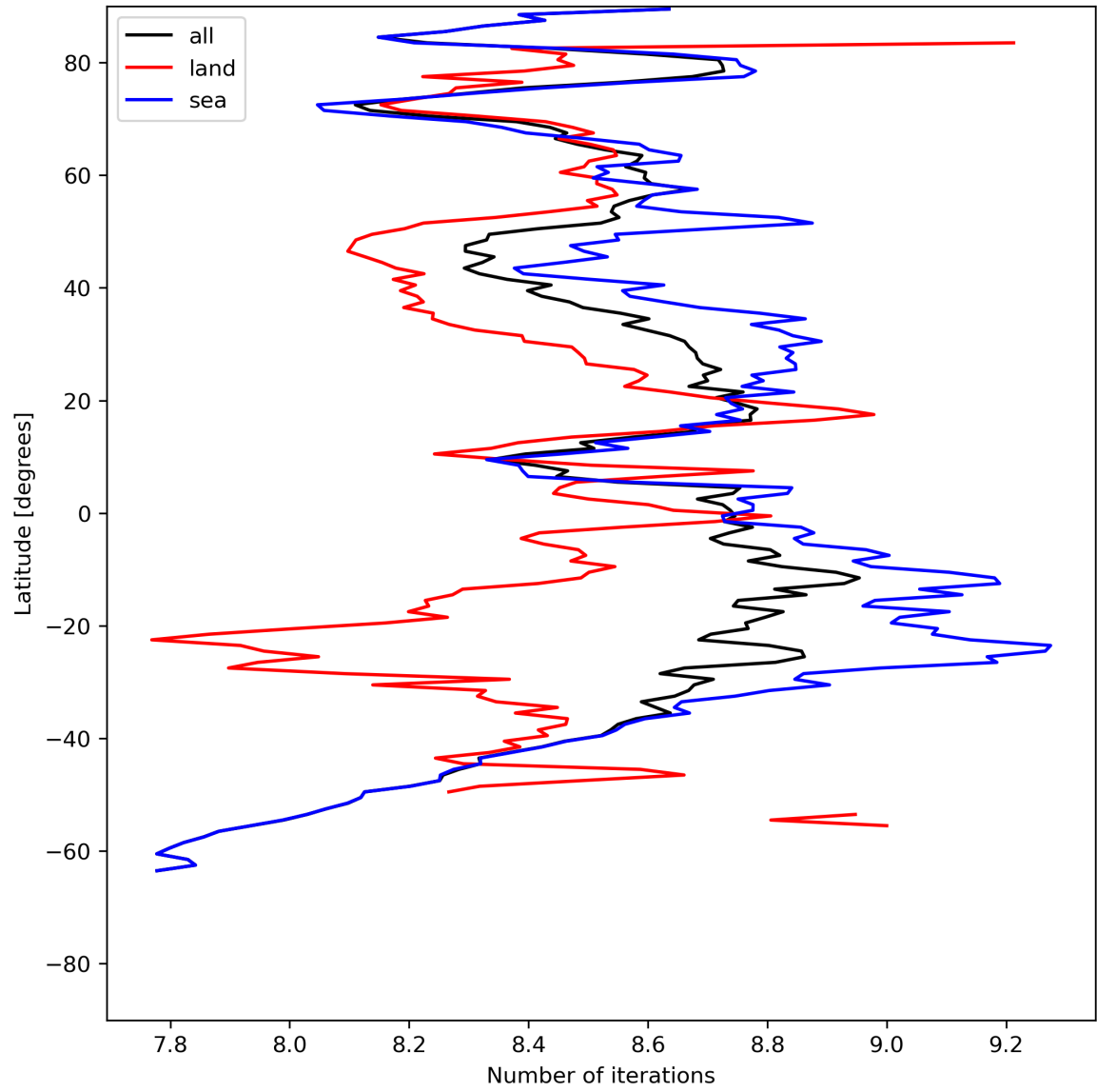
Figure 16: Zonal average of “Number of iterations” for 2024-07-13 to 2024-07-15.
