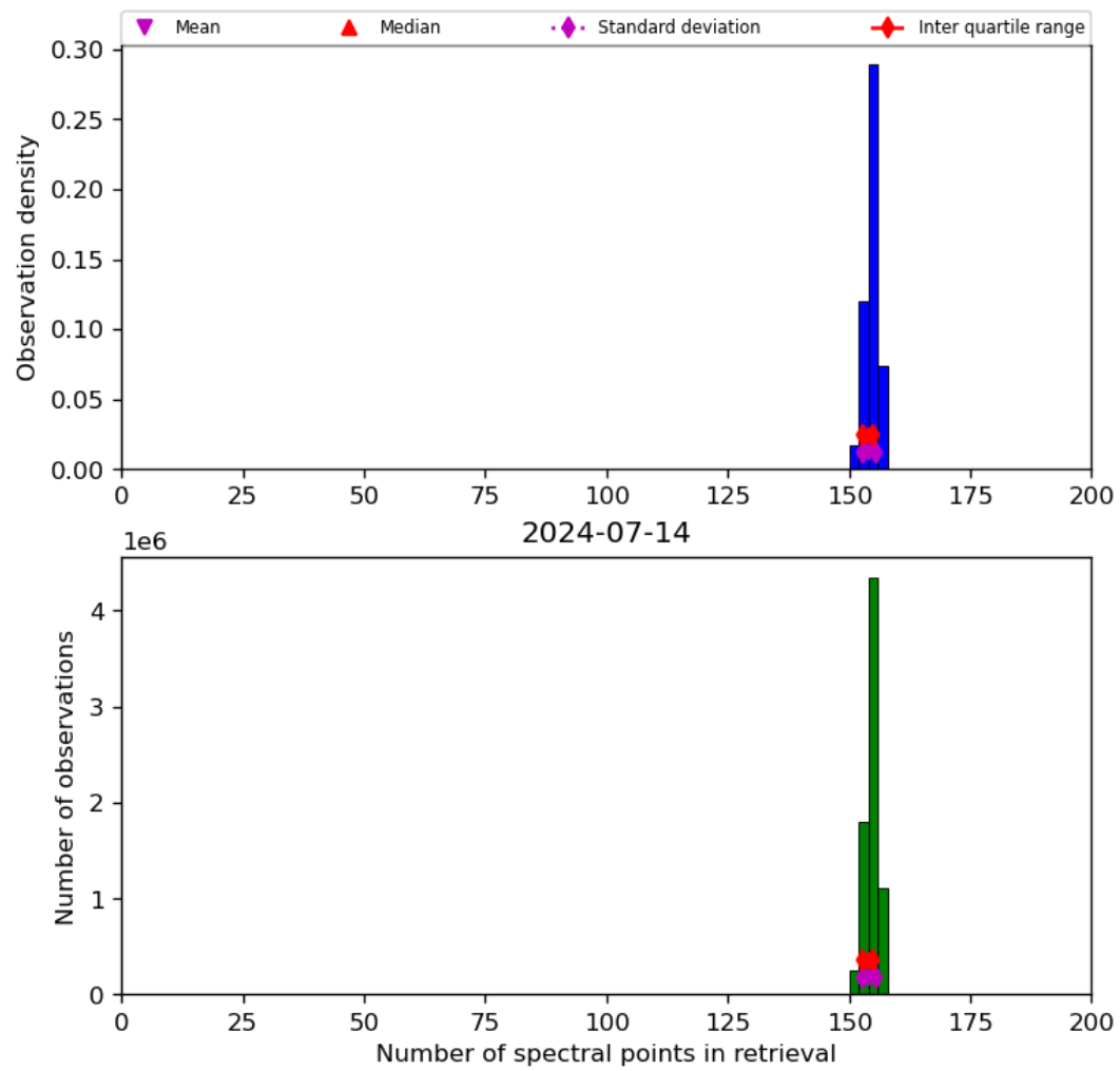
Figure 21: Histogram of “Number of spectral points in retrieval” for 2024-07-13 to 2024-07-15
