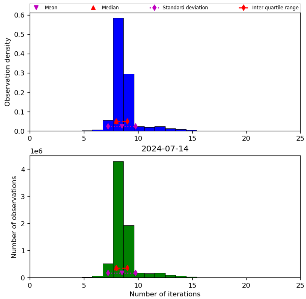
Figure 24: Histogram of “Number of iterations” for 2024-07-13 to 2024-07-15
