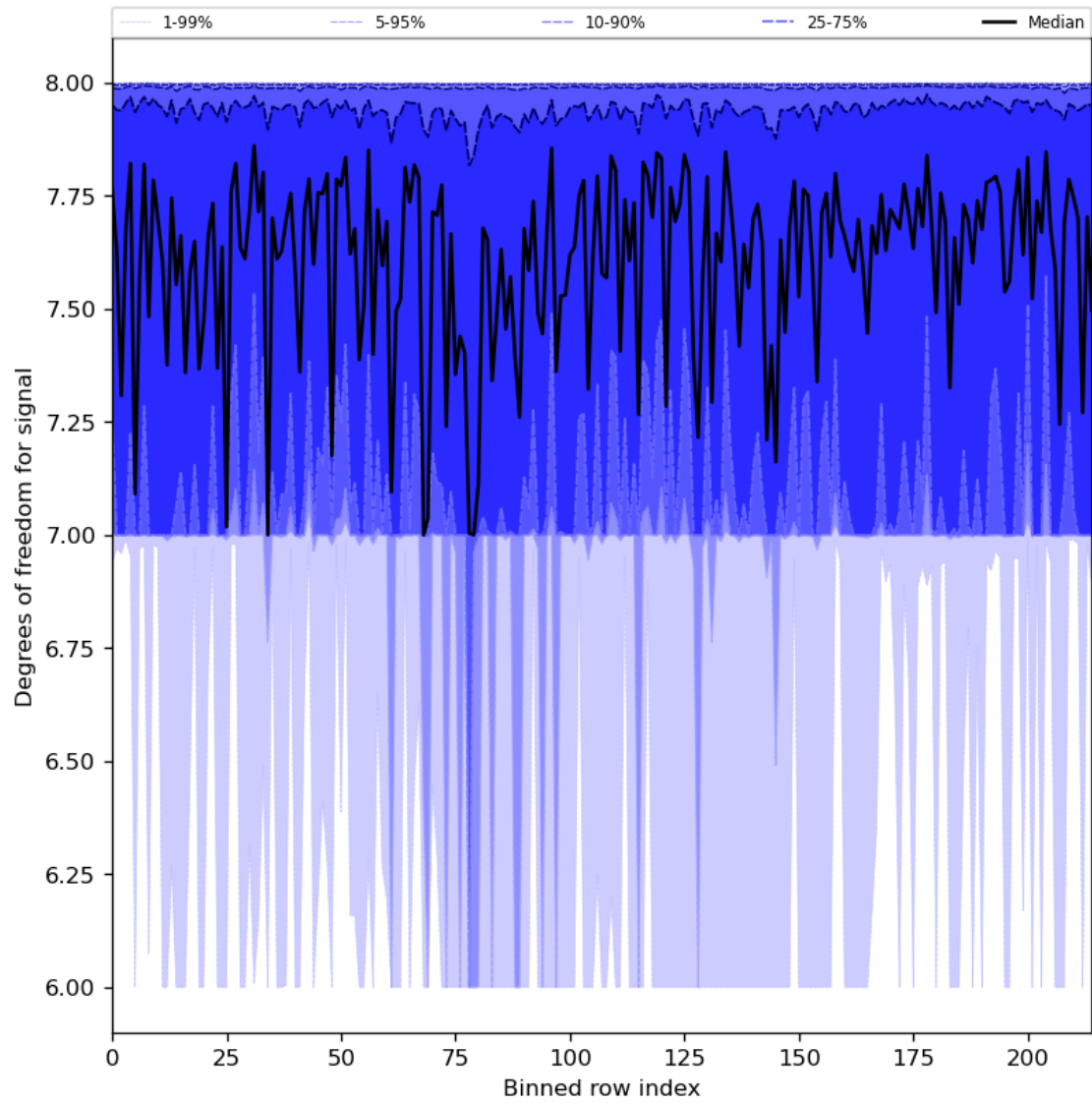
Figure 31: Along track statistics of “Degrees of freedom for signal” for 2024-07-13 to 2024-07-15
