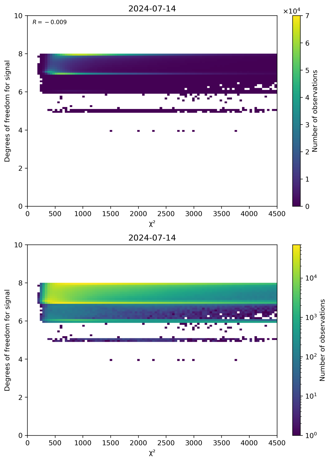
Figure 48: Scatter density plot of “ \chi^2 ” against “Degrees of freedom for signal” for 2024-07-13 to 2024-07-15.
