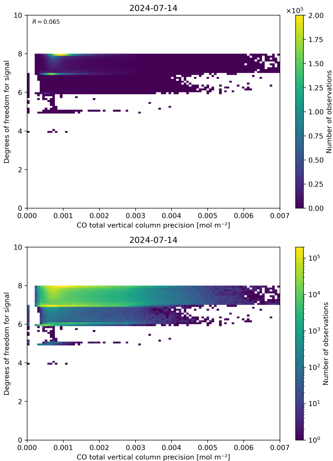
Figure 45: Scatter density plot of “CO total vertical column precision” against “Degrees of freedom for signal” for 2024-07-13 to 2024-07-15.
