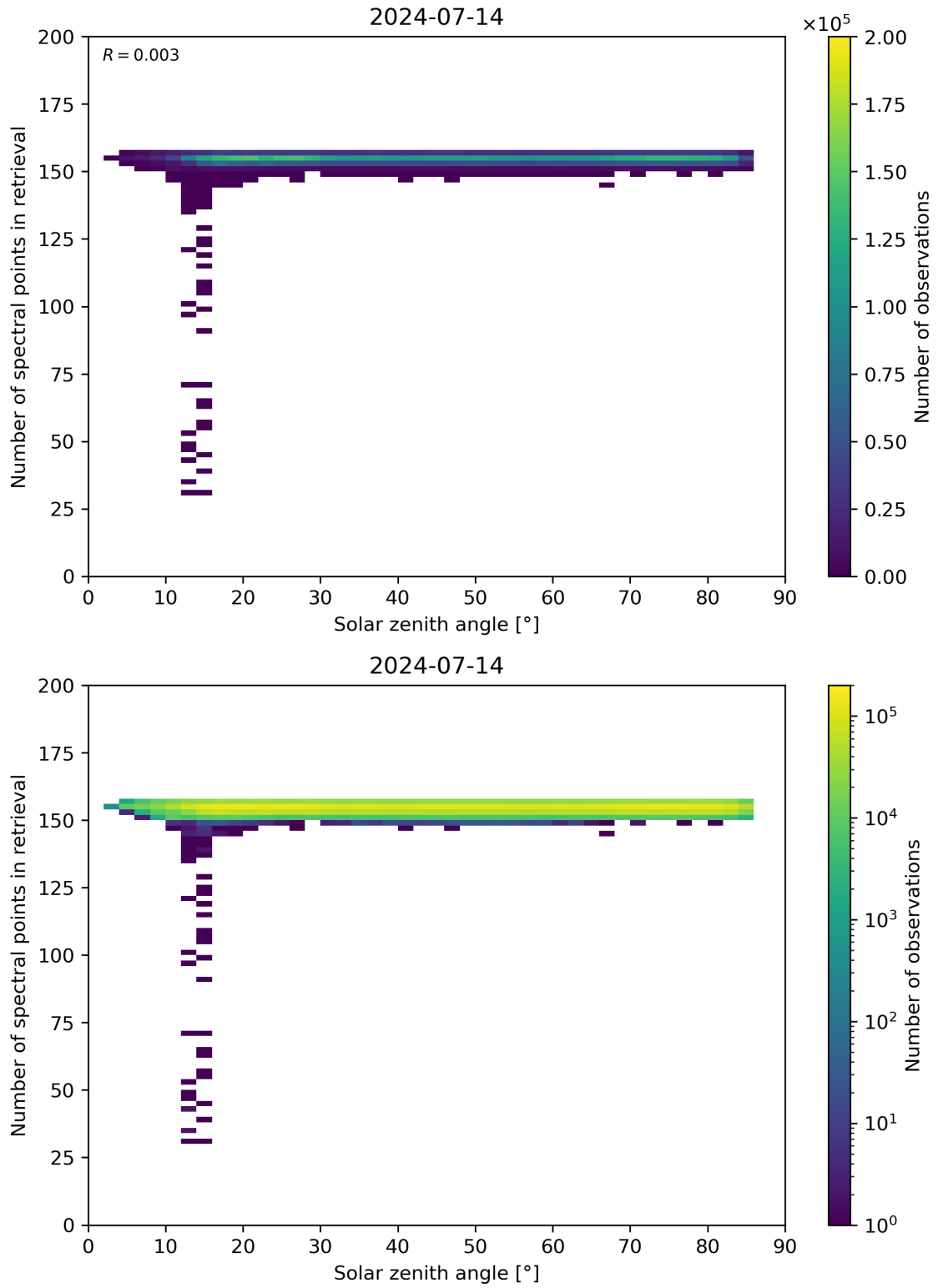
Figure 68: Scatter density plot of “Solar zenith angle” against “Number of spectral points in retrieval” for 2024-07-13 to 2024-07-15.
