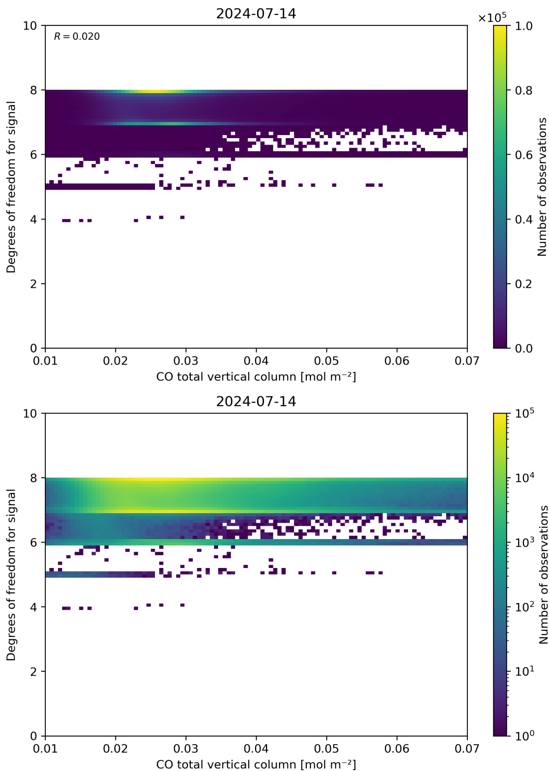
Figure 41: Scatter density plot of “CO total vertical column” against “Degrees of freedom for signal” for 2024-07-13 to 2024-07-15.
