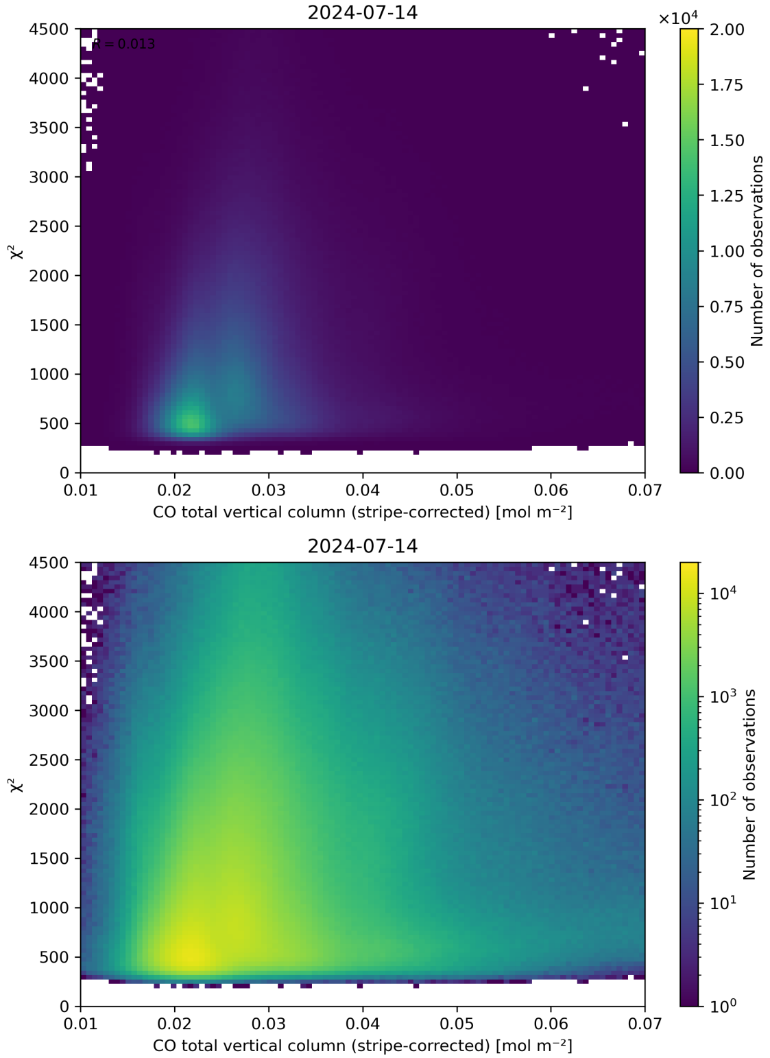
Figure 37: Scatter density plot of “CO total vertical column (stripe-corrected)” against “ \chi^2 ” for 2024-07-13 to 2024-07-15.
