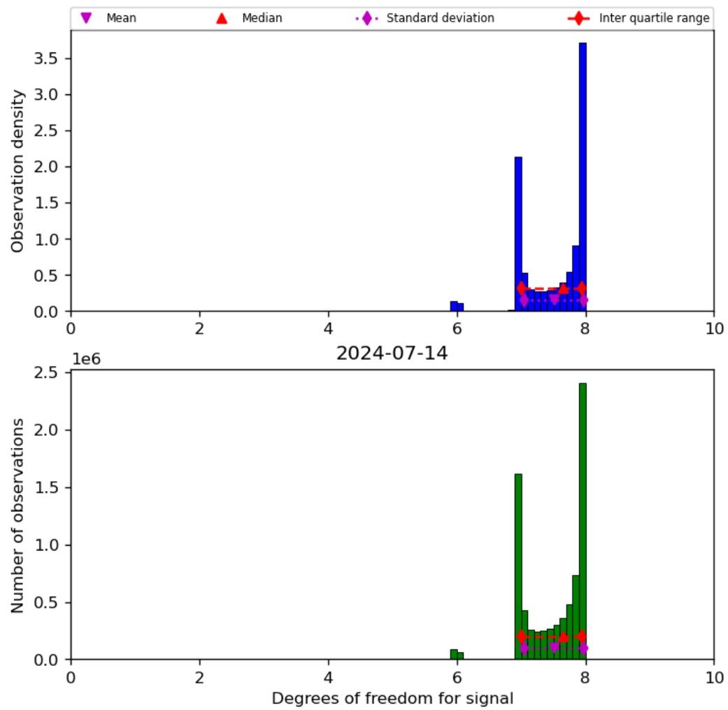
Figure 23: Histogram of “Degrees of freedom for signal” for 2024-07-13 to 2024-07-15
