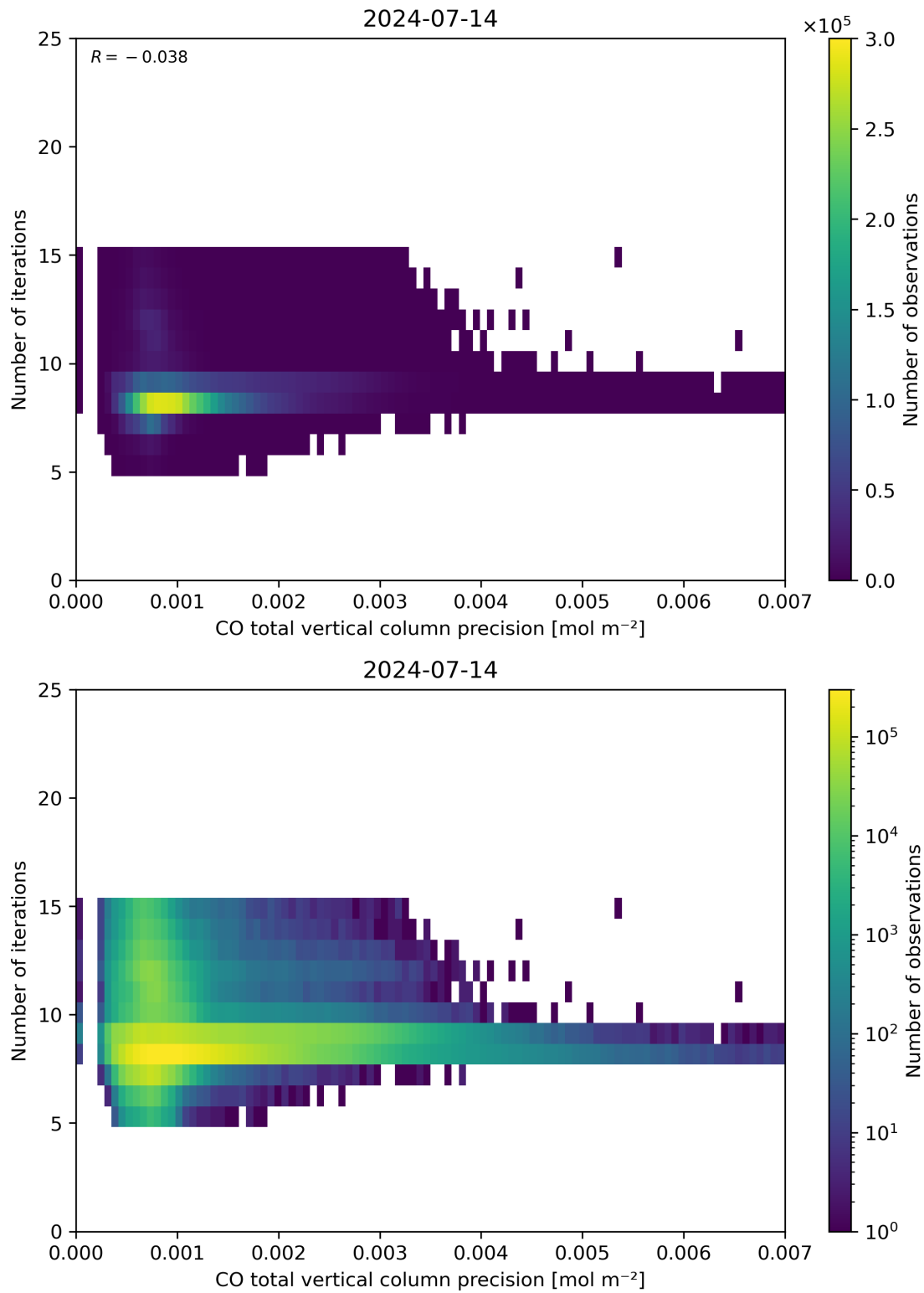
Figure 46: Scatter density plot of “CO total vertical column precision” against “Number of iterations” for 2024-07-13 to 2024-07-15.
