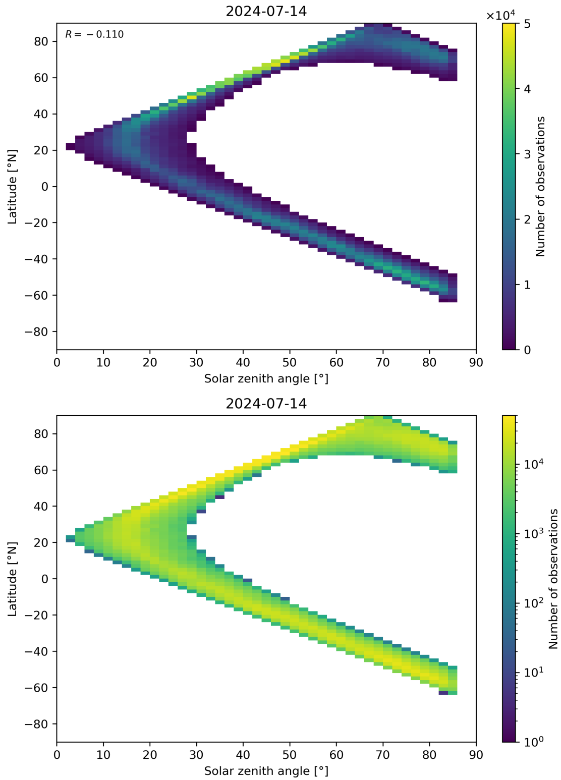
Figure 66: Scatter density plot of “Solar zenith angle” against “Latitude” for 2024-07-13 to 2024-07-15.
