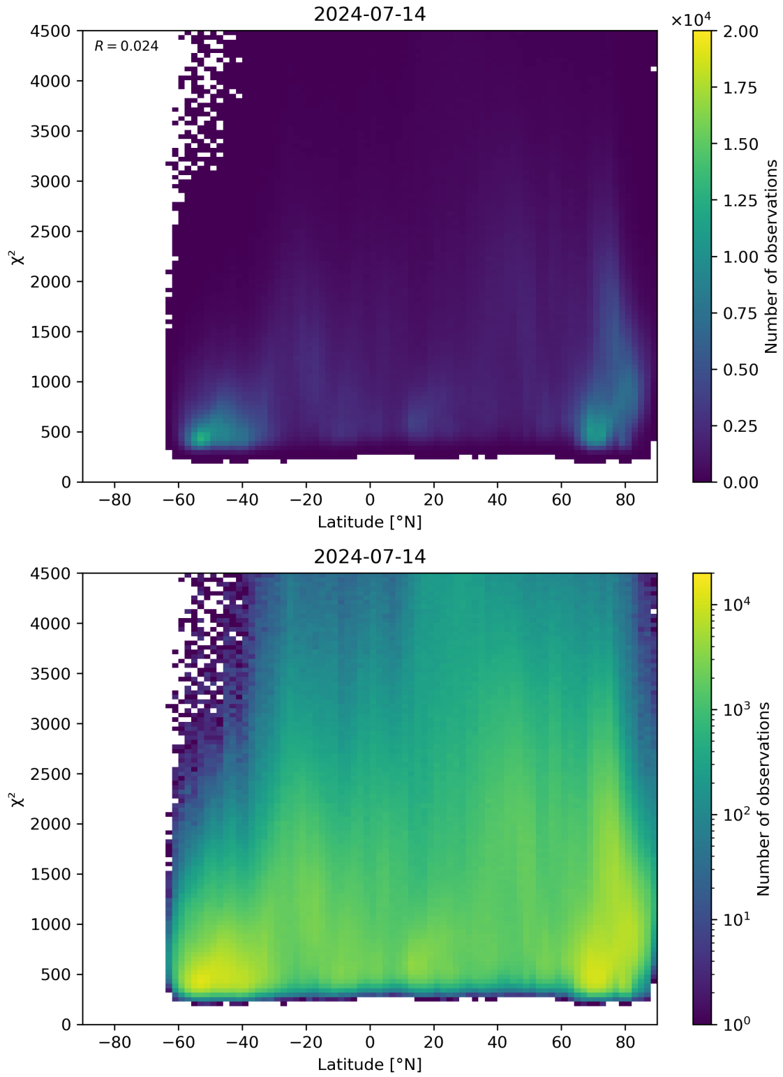
Figure 54: Scatter density plot of “Latitude” against “ \chi^2 ” for 2024-07-13 to 2024-07-15.
