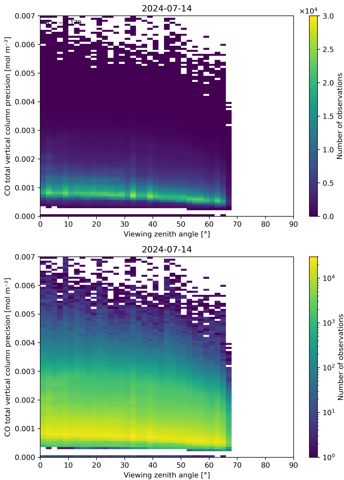
Figure 71: Scatter density plot of “Viewing zenith angle” against “CO total vertical column precision” for 2024-07-13 to 2024-07-15.
