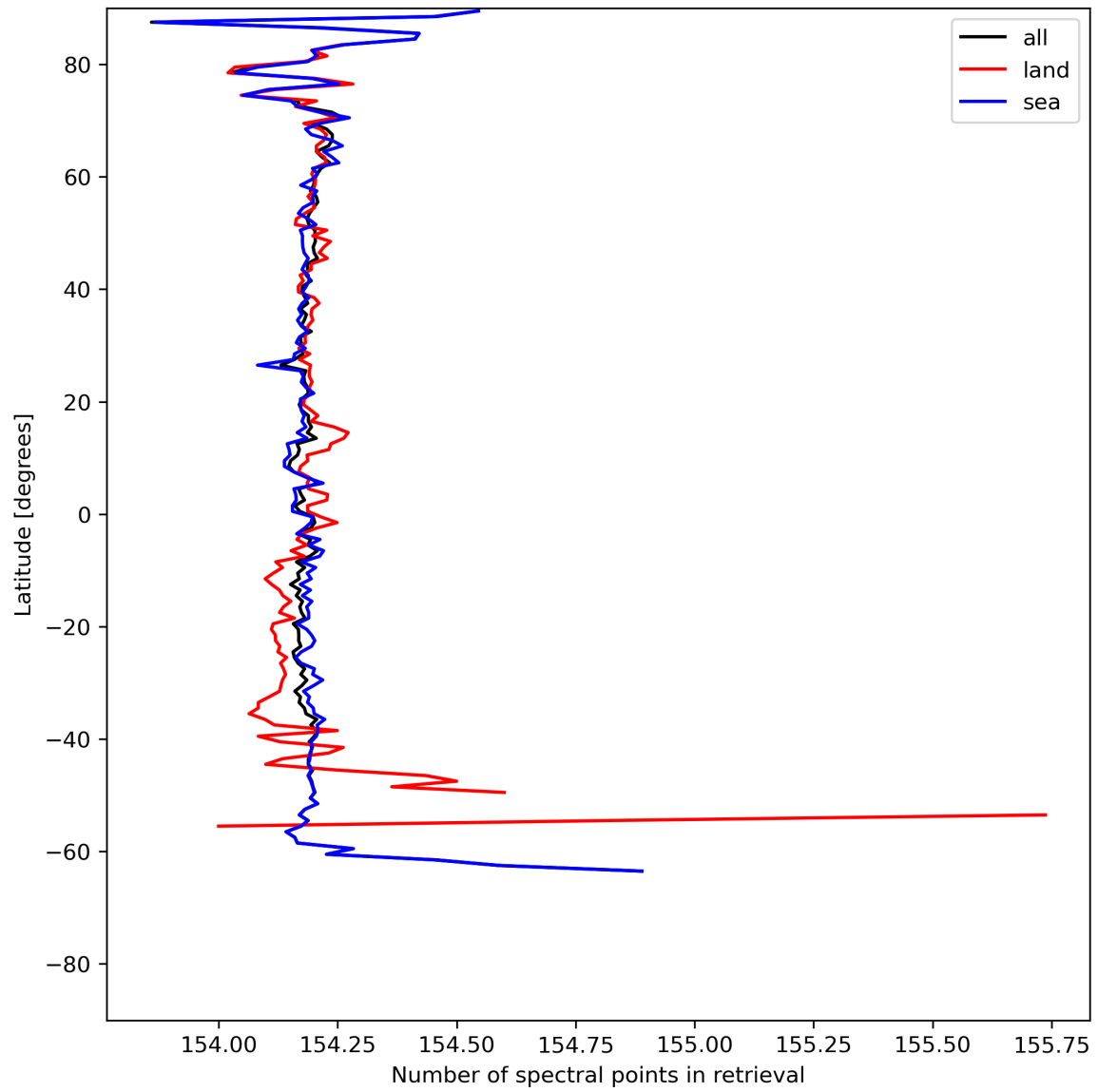
Figure 13: Zonal average of “Number of spectral points in retrieval” for 2024-07-13 to 2024-07-15.
