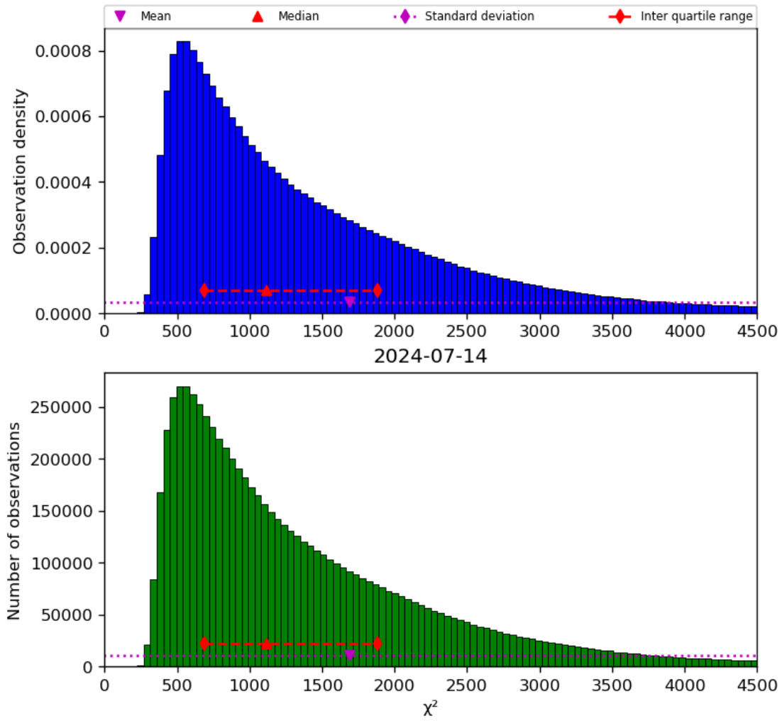
Figure 22: Histogram of “ \chi^2 ” for 2024-07-13 to 2024-07-15
