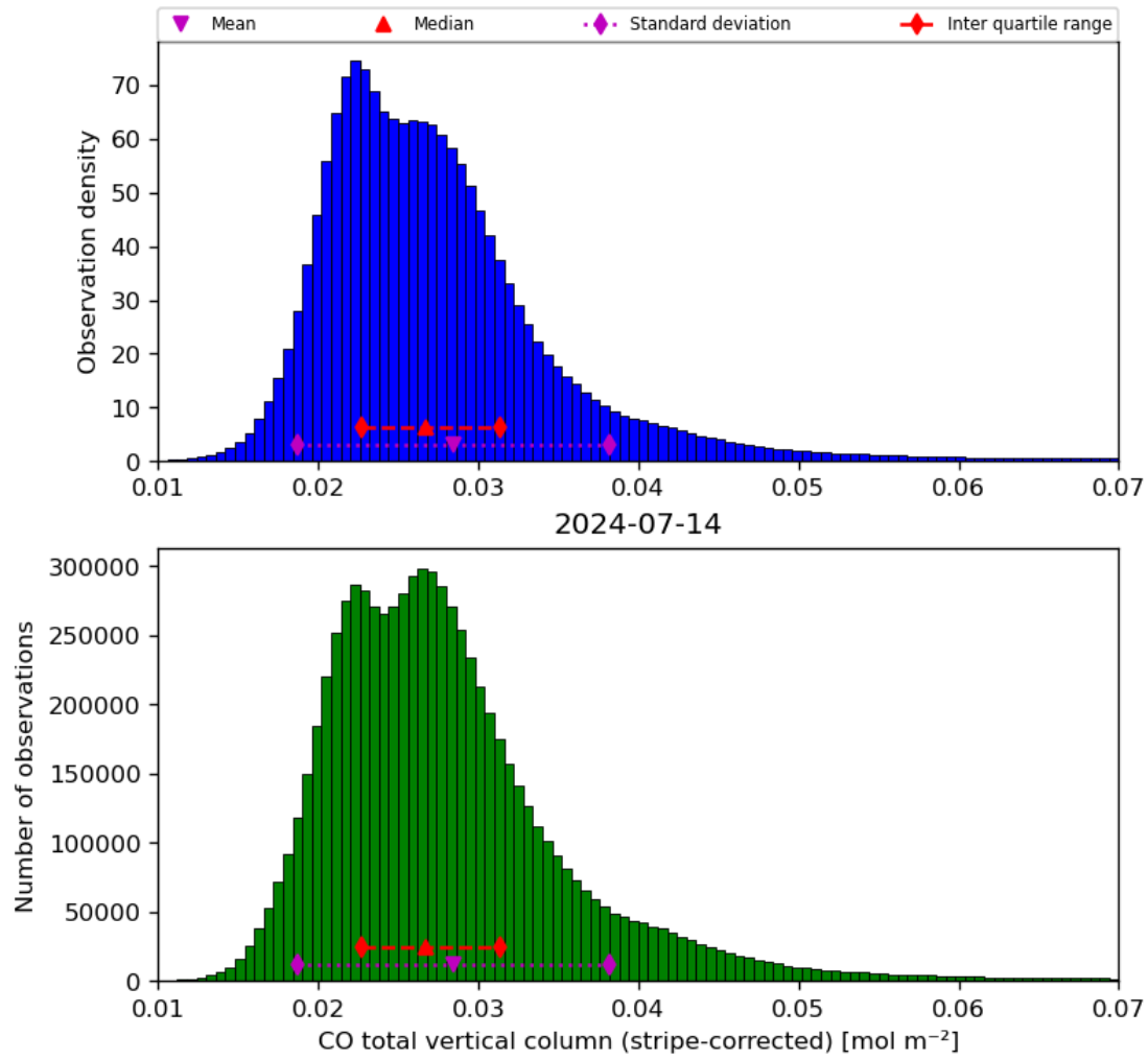
Figure 19: Histogram of “CO total vertical column (stripe-corrected)” for 2024-07-13 to 2024-07-15
