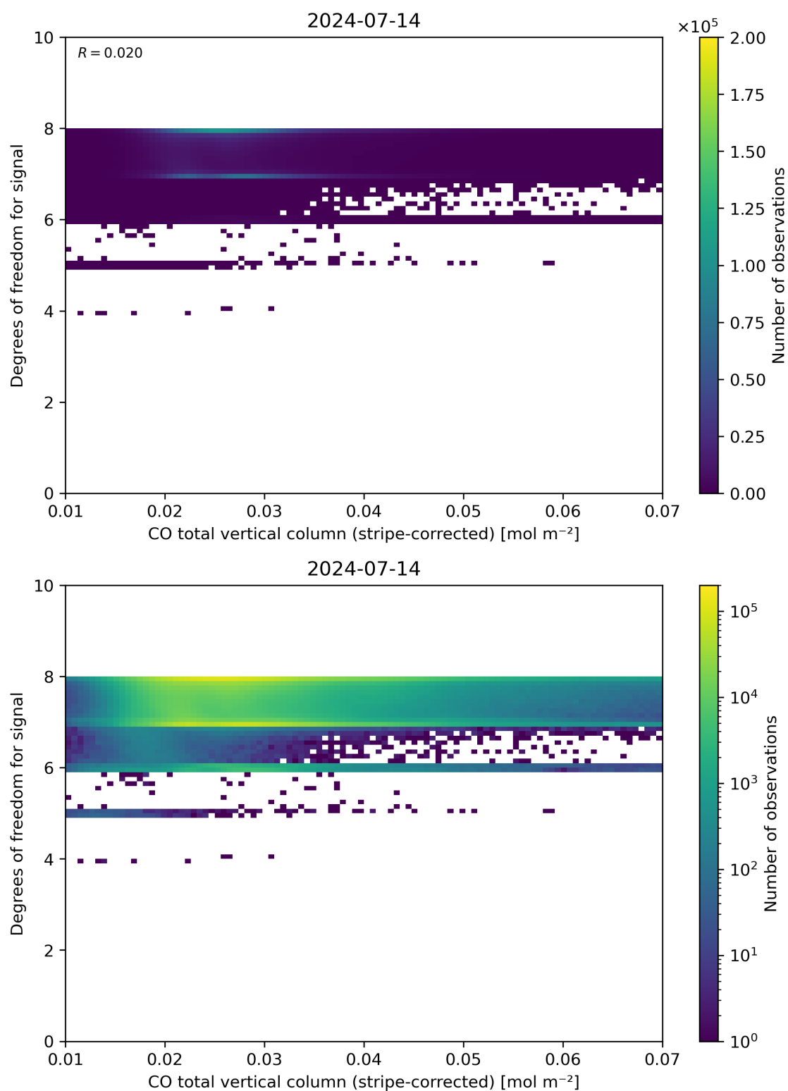
Figure 38: Scatter density plot of “CO total vertical column (stripe-corrected)” against “Degrees of freedom for signal” for 2024-07-13 to 2024-07-15.
