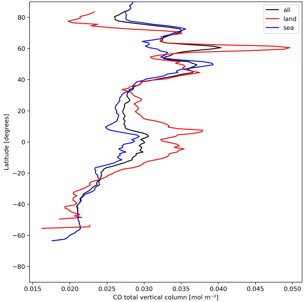
Figure 10: Zonal average of “CO total vertical column” for 2024-07-13 to 2024-07-15.
