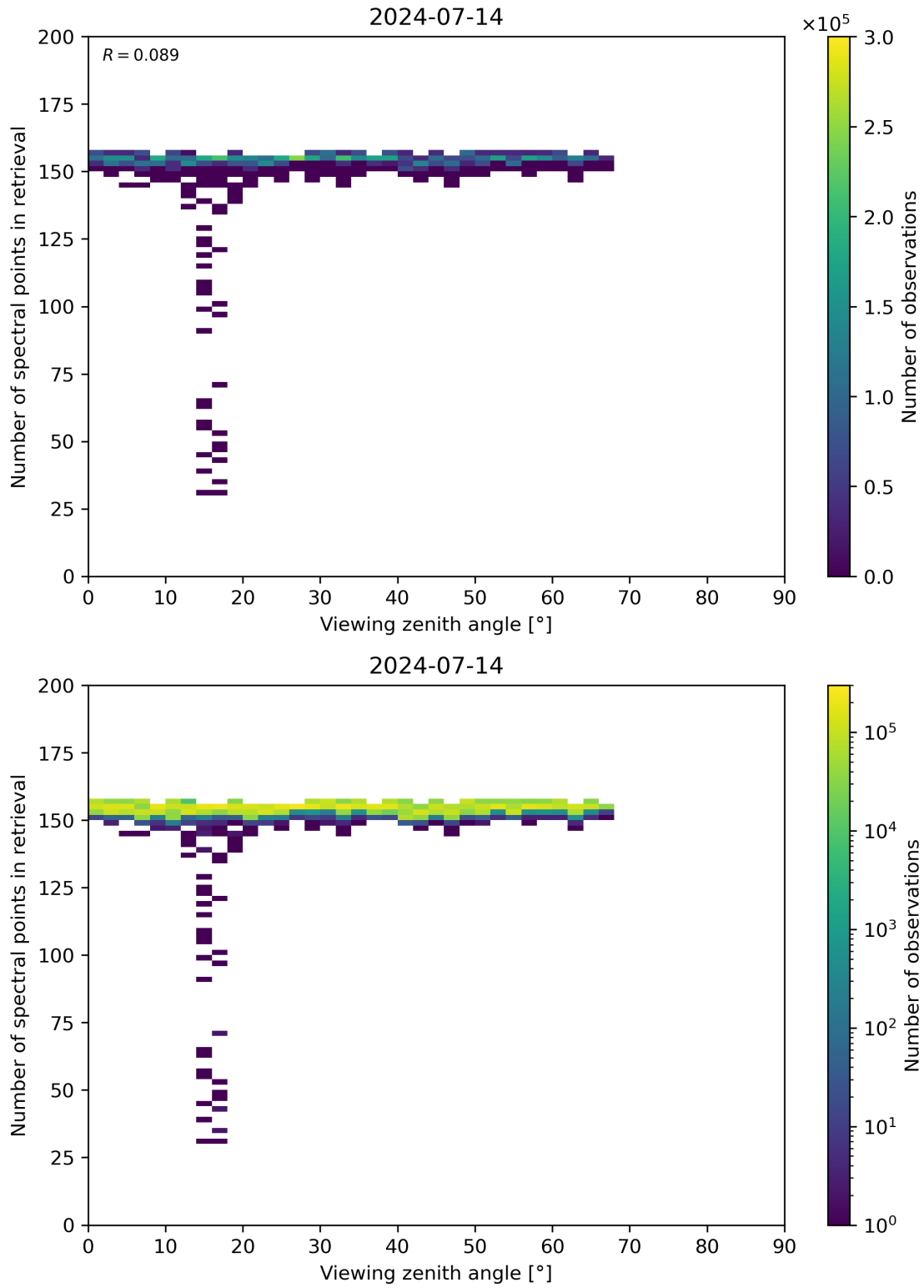
Figure 76: Scatter density plot of “Viewing zenith angle” against “Number of spectral points in retrieval” for 2024-07-13 to 2024-07-15.
