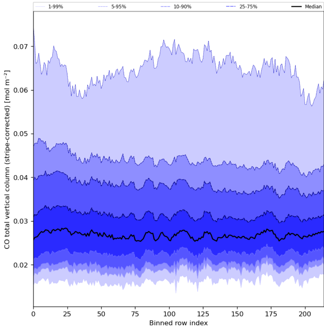
Figure 27: Along track statistics of “CO total vertical column (stripe-corrected)” for 2024-07-13 to 2024-07-15
