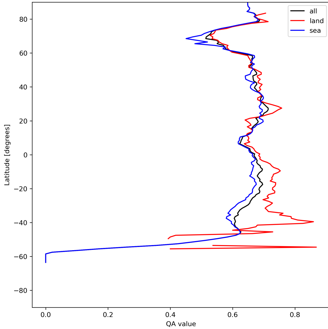
Figure 9: Zonal average of “QA value” for 2024-07-13 to 2024-07-15.
