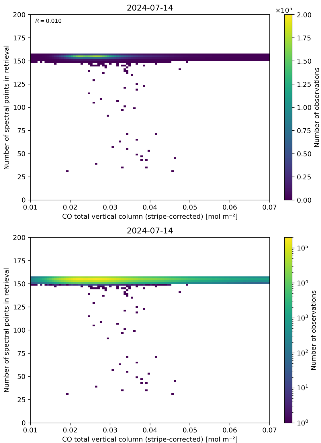
Figure 40: Scatter density plot of “CO total vertical column (stripe-corrected)” against “Number of spectral points in retrieval” for 2024-07-13 to 2024-07-15.
