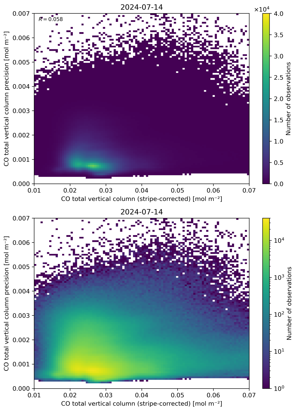
Figure 36: Scatter density plot of “CO total vertical column (stripe-corrected)” against “CO total vertical column precision” for 2024-07-13 to 2024-07-15.
