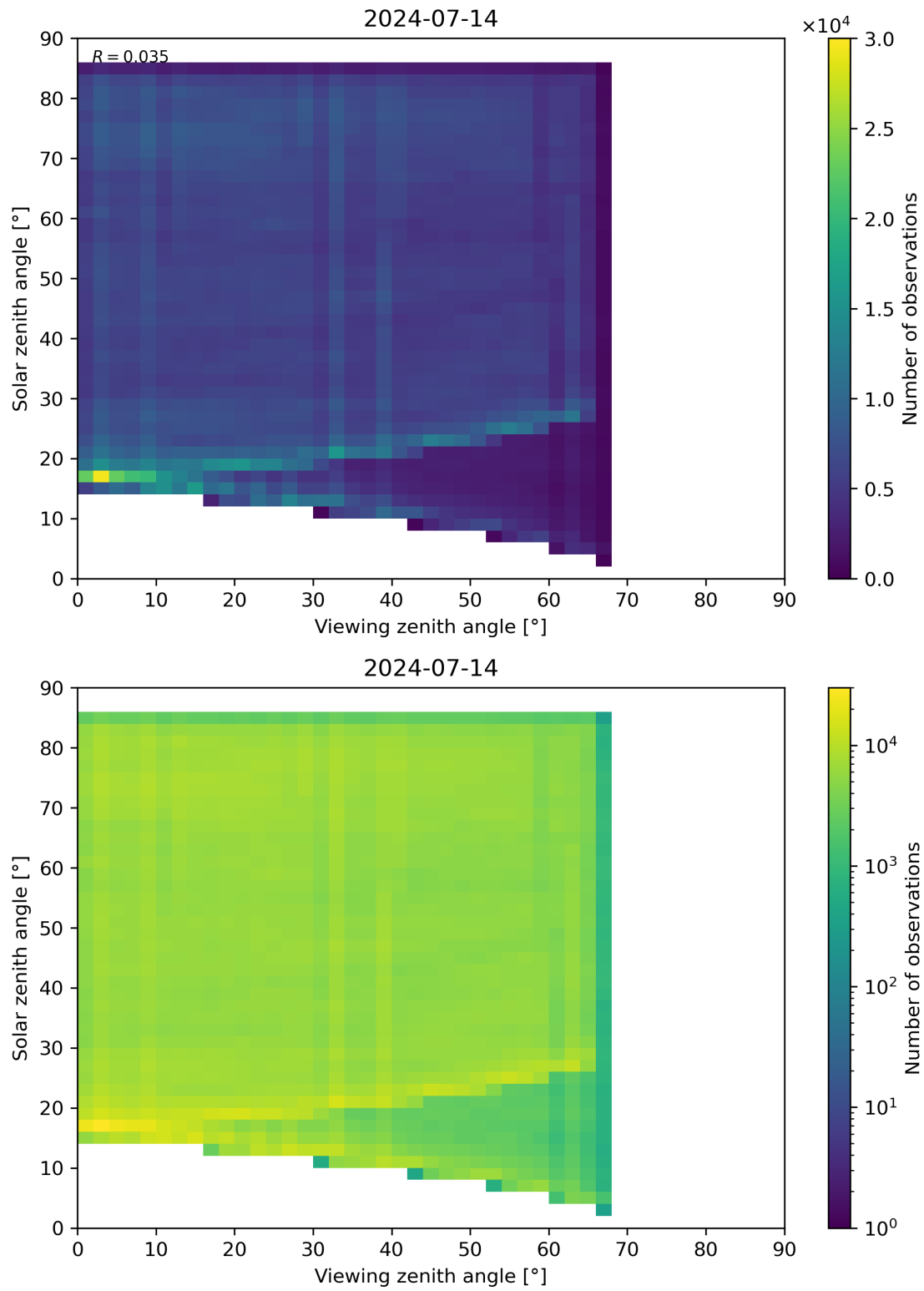
Figure 77: Scatter density plot of “Viewing zenith angle” against “Solar zenith angle” for 2024-07-13 to 2024-07-15.
