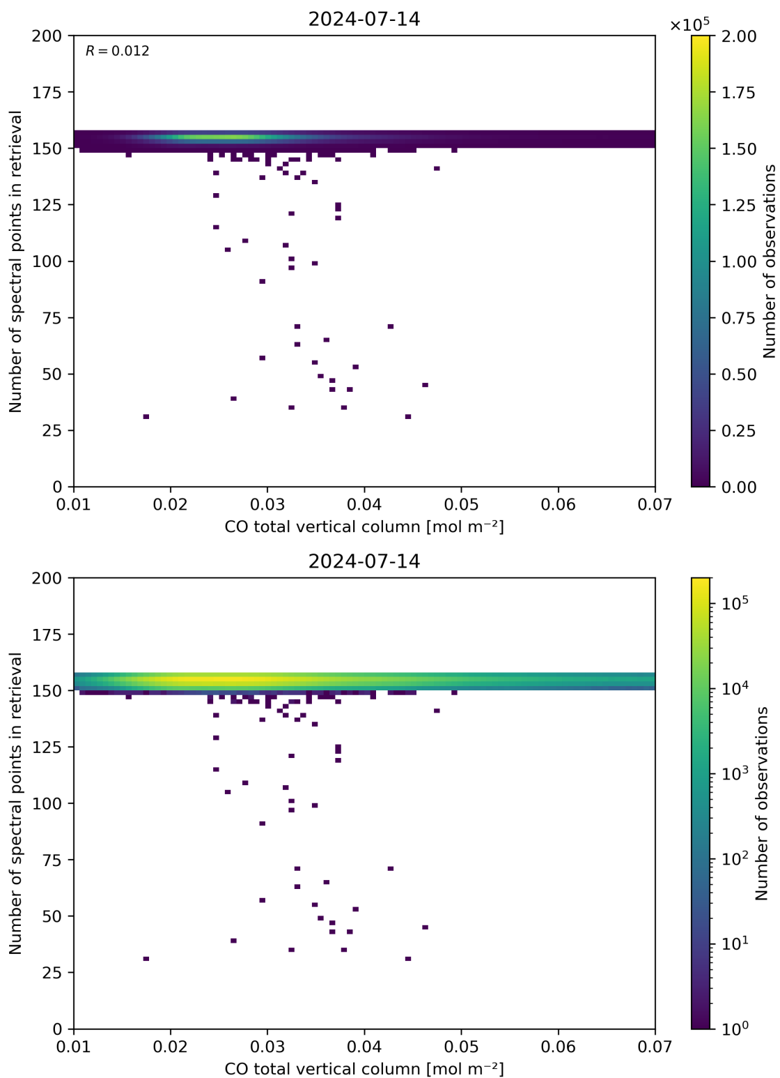
Figure 43: Scatter density plot of “CO total vertical column” against “Number of spectral points in retrieval” for 2024-07-13 to 2024-07-15.
