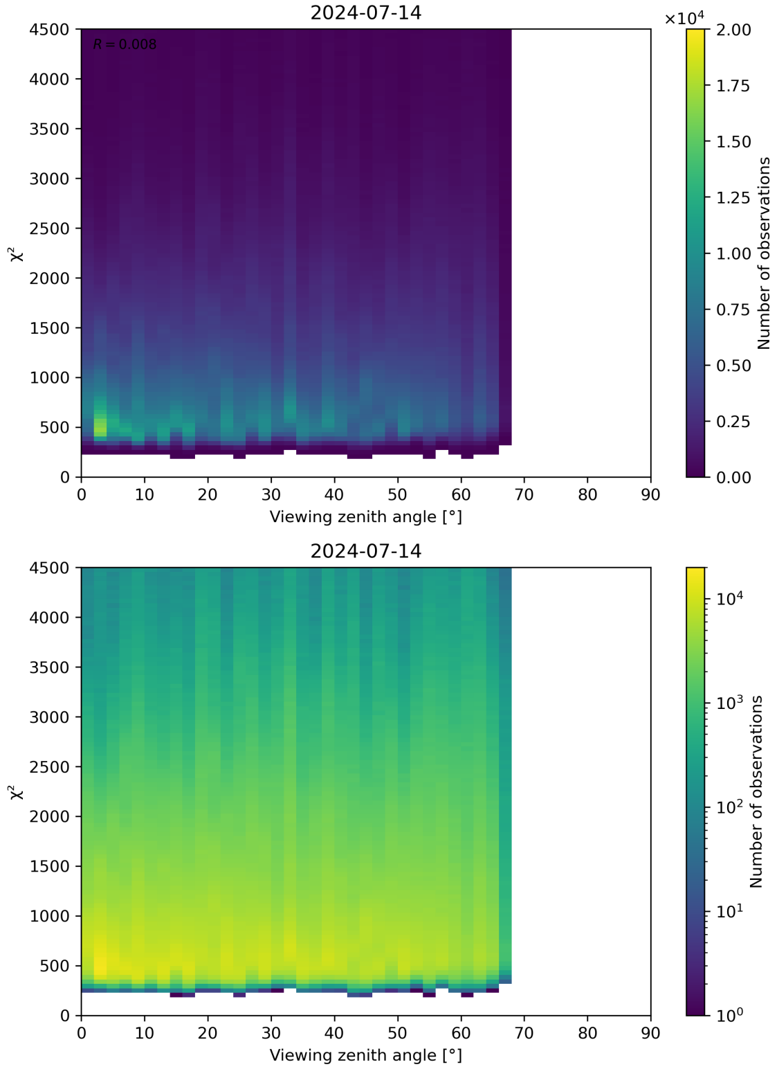
Figure 72: Scatter density plot of “Viewing zenith angle” against “ \chi^2 ” for 2024-07-13 to 2024-07-15.
