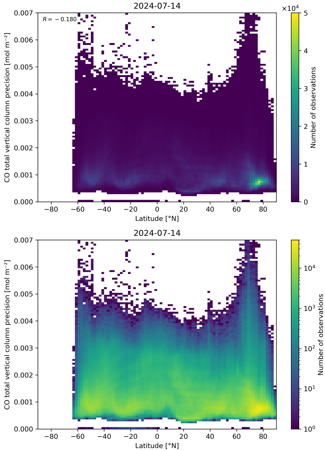
Figure 53: Scatter density plot of “Latitude” against “CO total vertical column precision” for 2024-07-13 to 2024-07-15.
