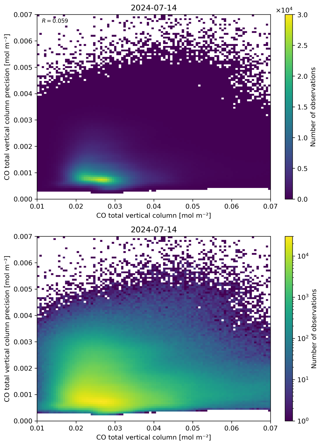
Figure 34: Scatter density plot of “CO total vertical column” against “CO total vertical column precision” for 2024-07-13 to 2024-07-15.
