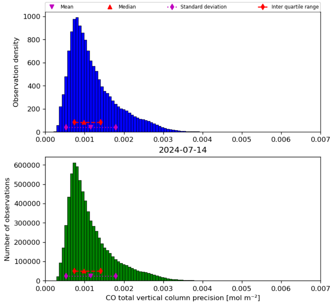
Figure 20: Histogram of “CO total vertical column precision” for 2024-07-13 to 2024-07-15
