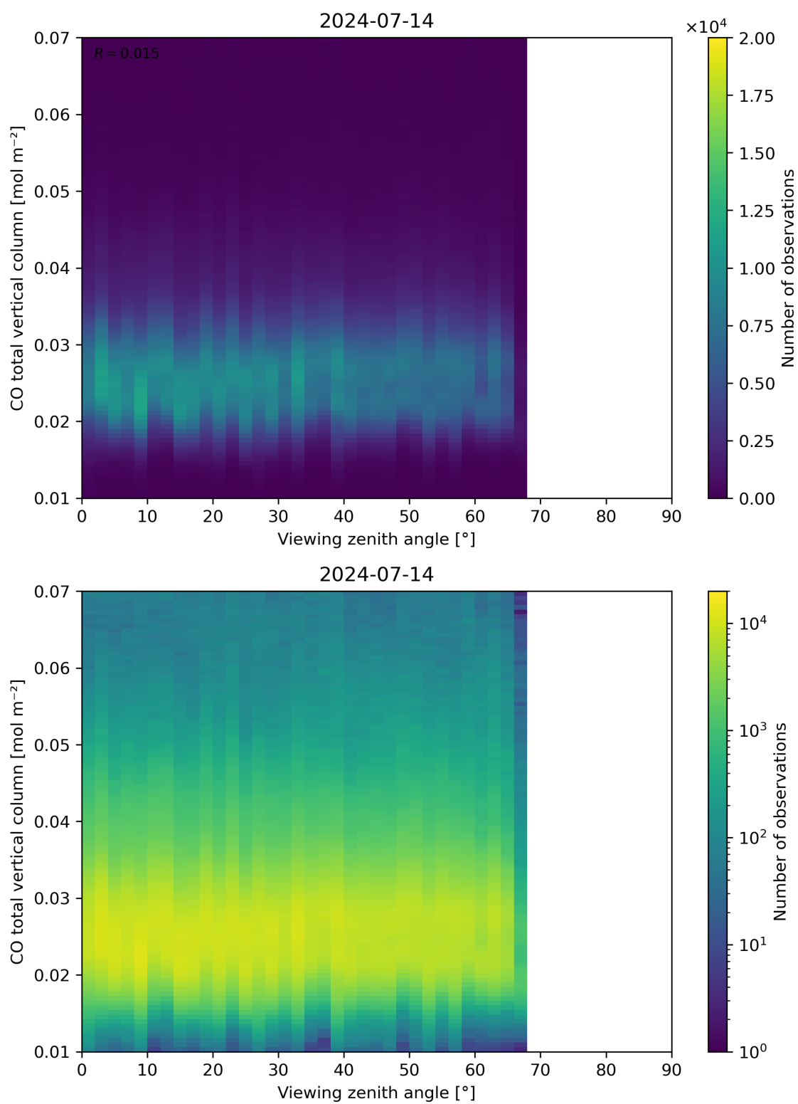
Figure 69: Scatter density plot of “Viewing zenith angle” against “CO total vertical column” for 2024-07-13 to 2024-07-15.
