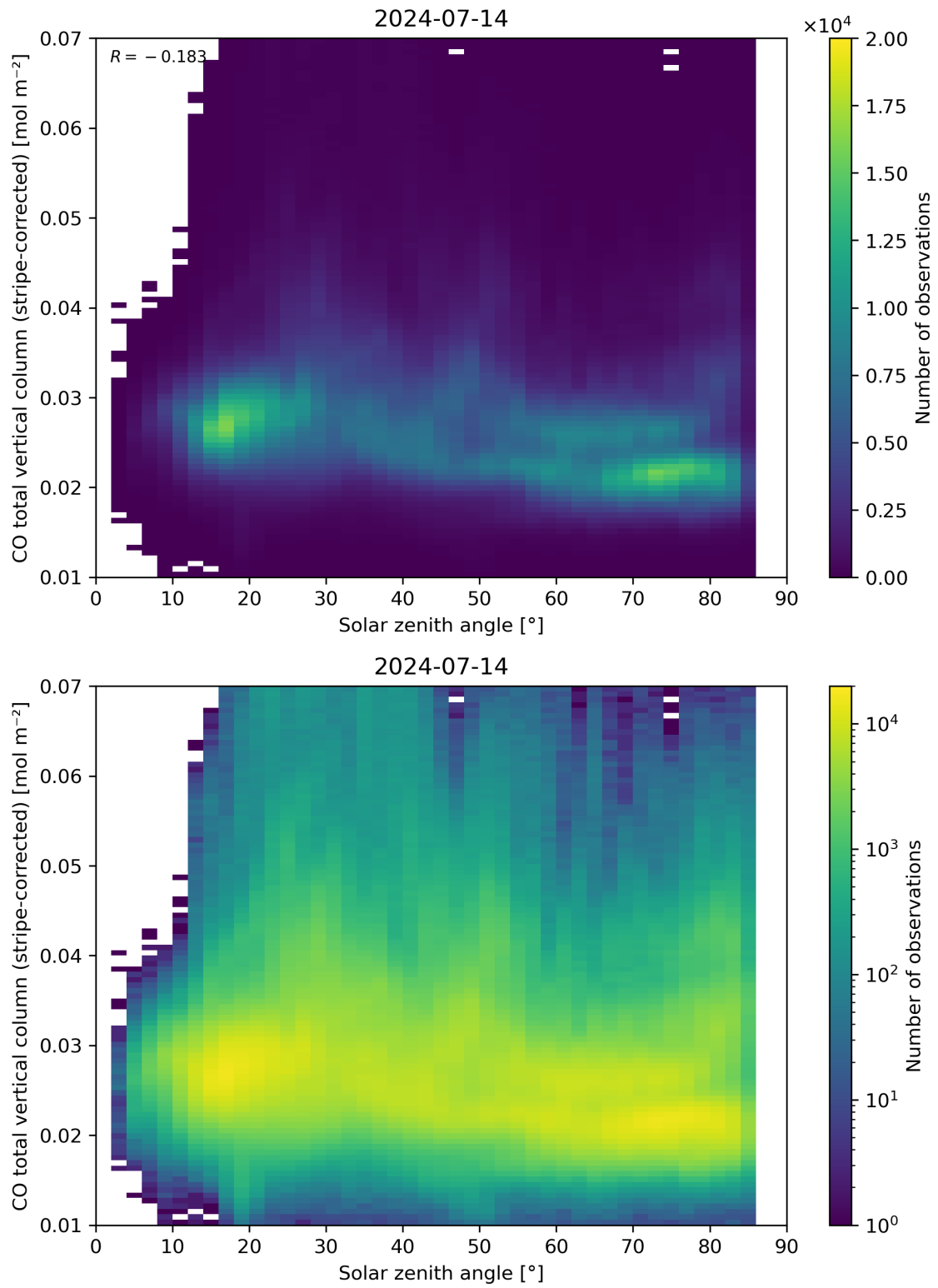
Figure 62: Scatter density plot of “Solar zenith angle” against “CO total vertical column (stripe-corrected)” for 2024-07-13 to 2024-07-15.
