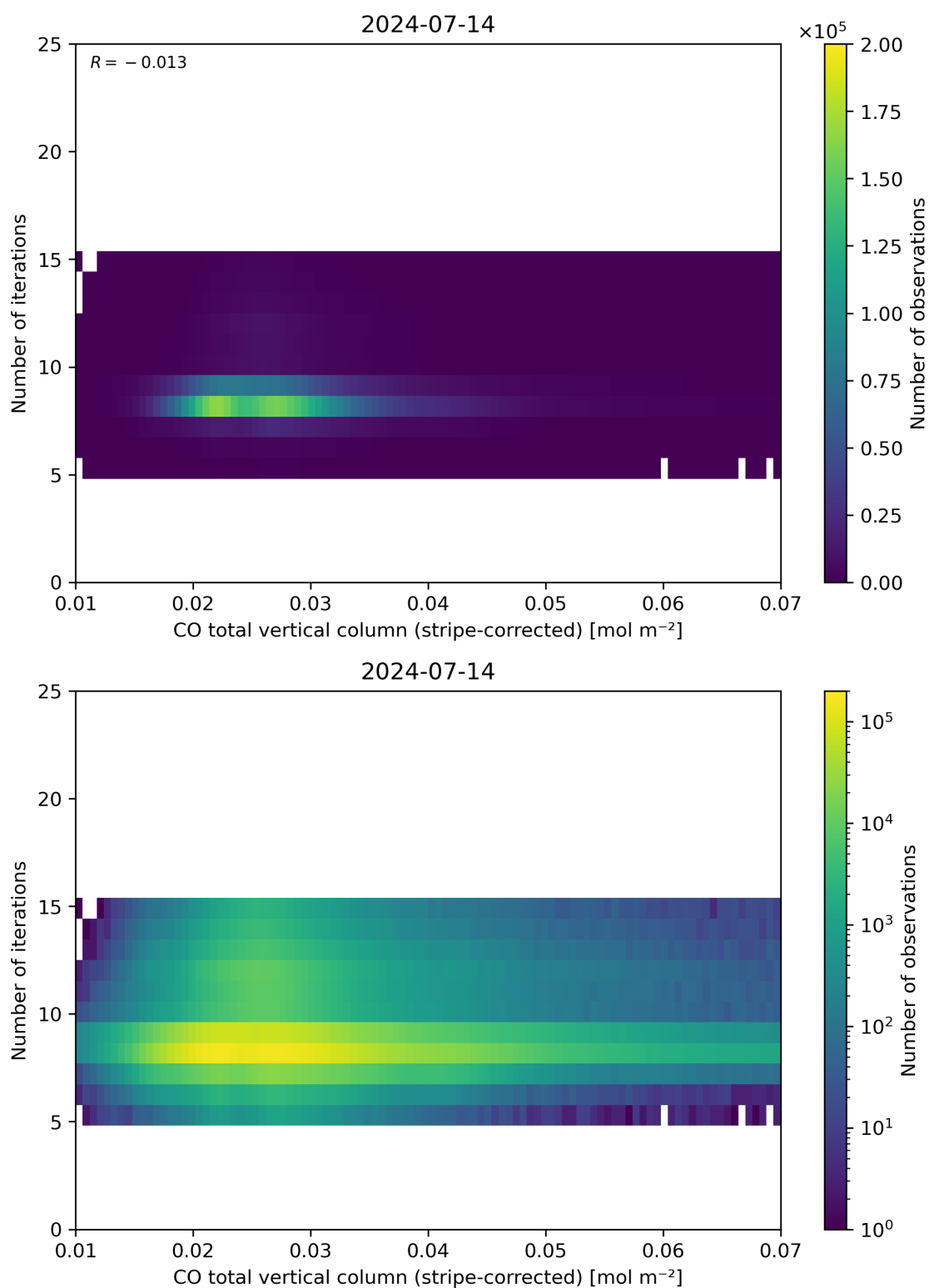
Figure 39: Scatter density plot of “CO total vertical column (stripe-corrected)” against “Number of iterations” for 2024-07-13 to 2024-07-15.
