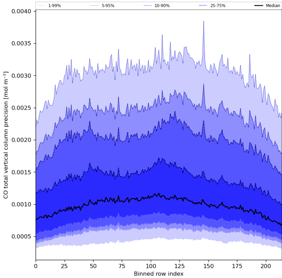
Figure 28: Along track statistics of “CO total vertical column precision” for 2024-07-13 to 2024-07-15
