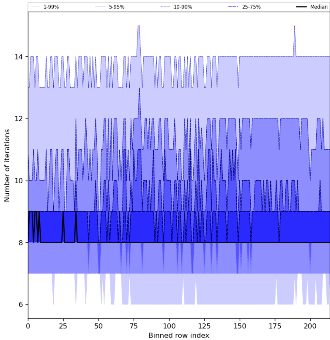
Figure 32: Along track statistics of “Number of iterations” for 2024-07-13 to 2024-07-15
