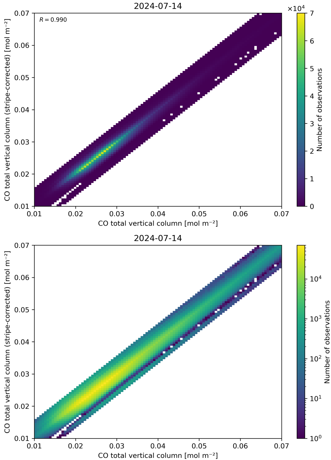
Figure 33: Scatter density plot of “CO total vertical column” against “CO total vertical column (stripe-corrected)” for 2024-07-13 to 2024-07-15.
