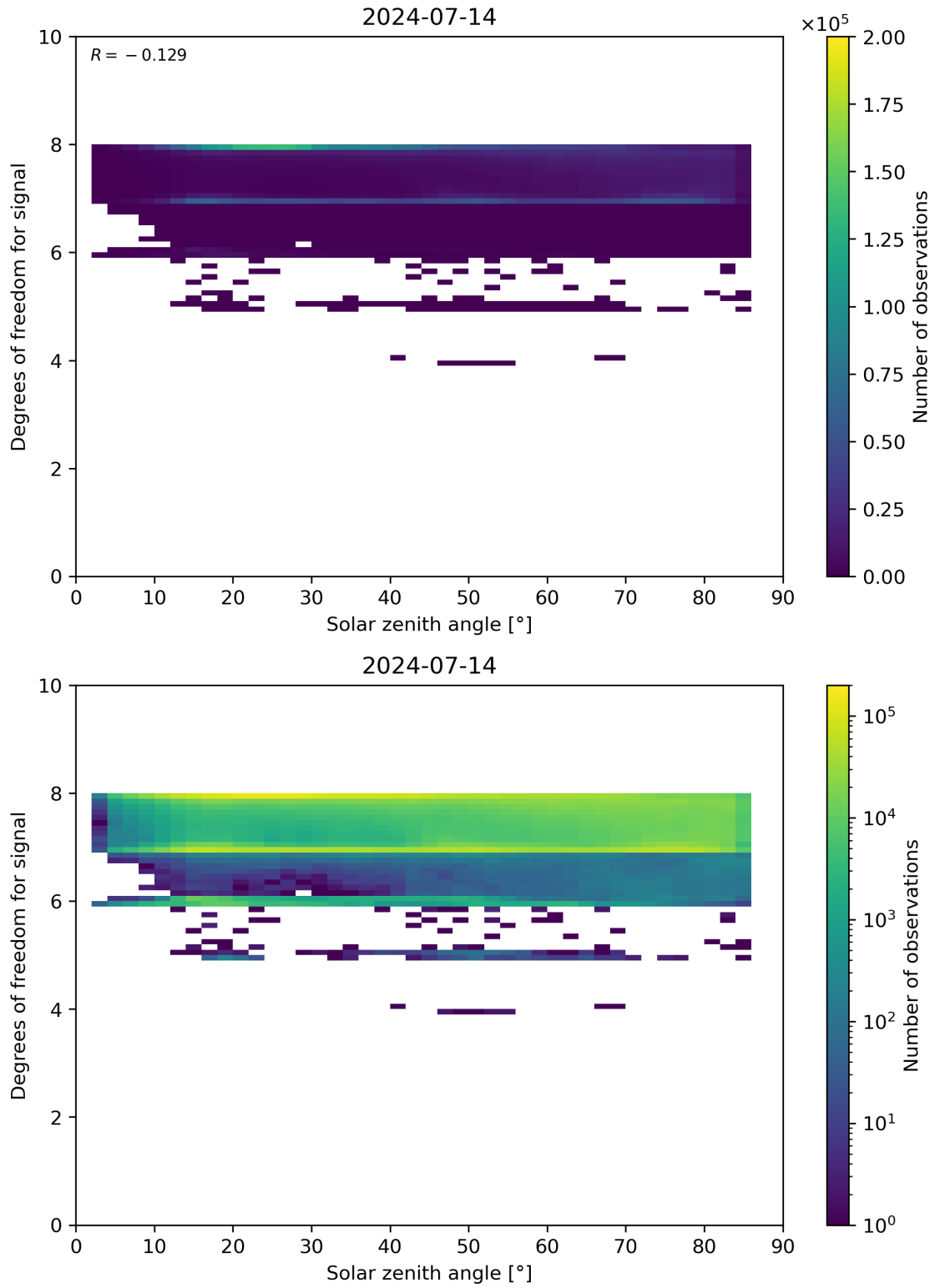
Figure 65: Scatter density plot of “Solar zenith angle” against “Degrees of freedom for signal” for 2024-07-13 to 2024-07-15.
