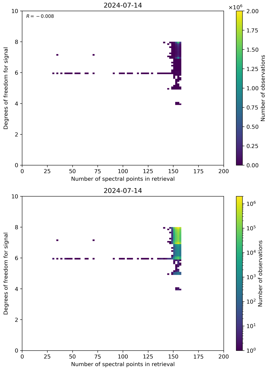
Figure 59: Scatter density plot of “Number of spectral points in retrieval” against “Degrees of freedom for signal” for 2024-07-13 to 2024-07-15.
