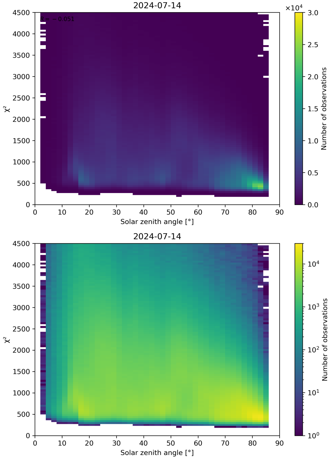
Figure 64: Scatter density plot of “Solar zenith angle” against “ \chi^2 ” for 2024-07-13 to 2024-07-15.
