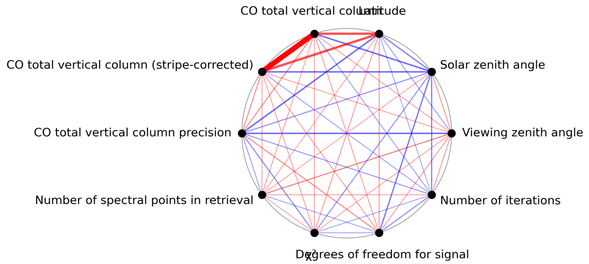
Figure 1: Map of correlation graph for 2024-07-13 to 2024-07-15.
