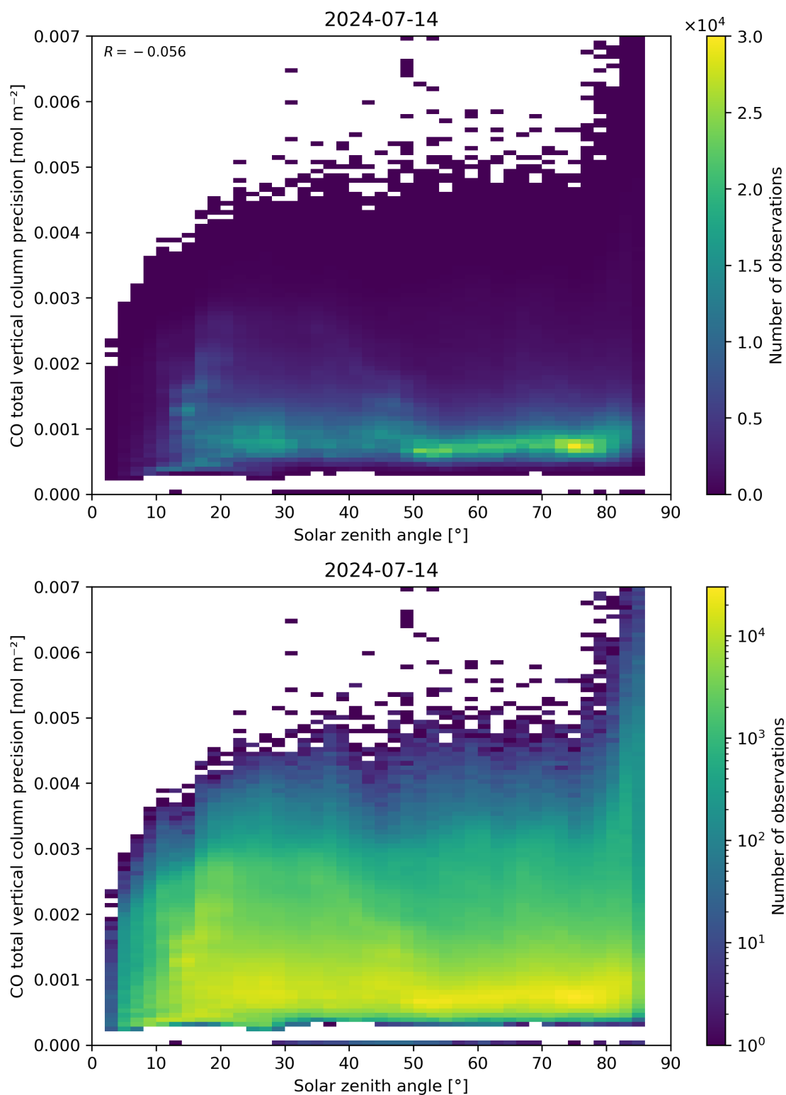
Figure 63: Scatter density plot of “Solar zenith angle” against “CO total vertical column precision” for 2024-07-13 to 2024-07-15.
