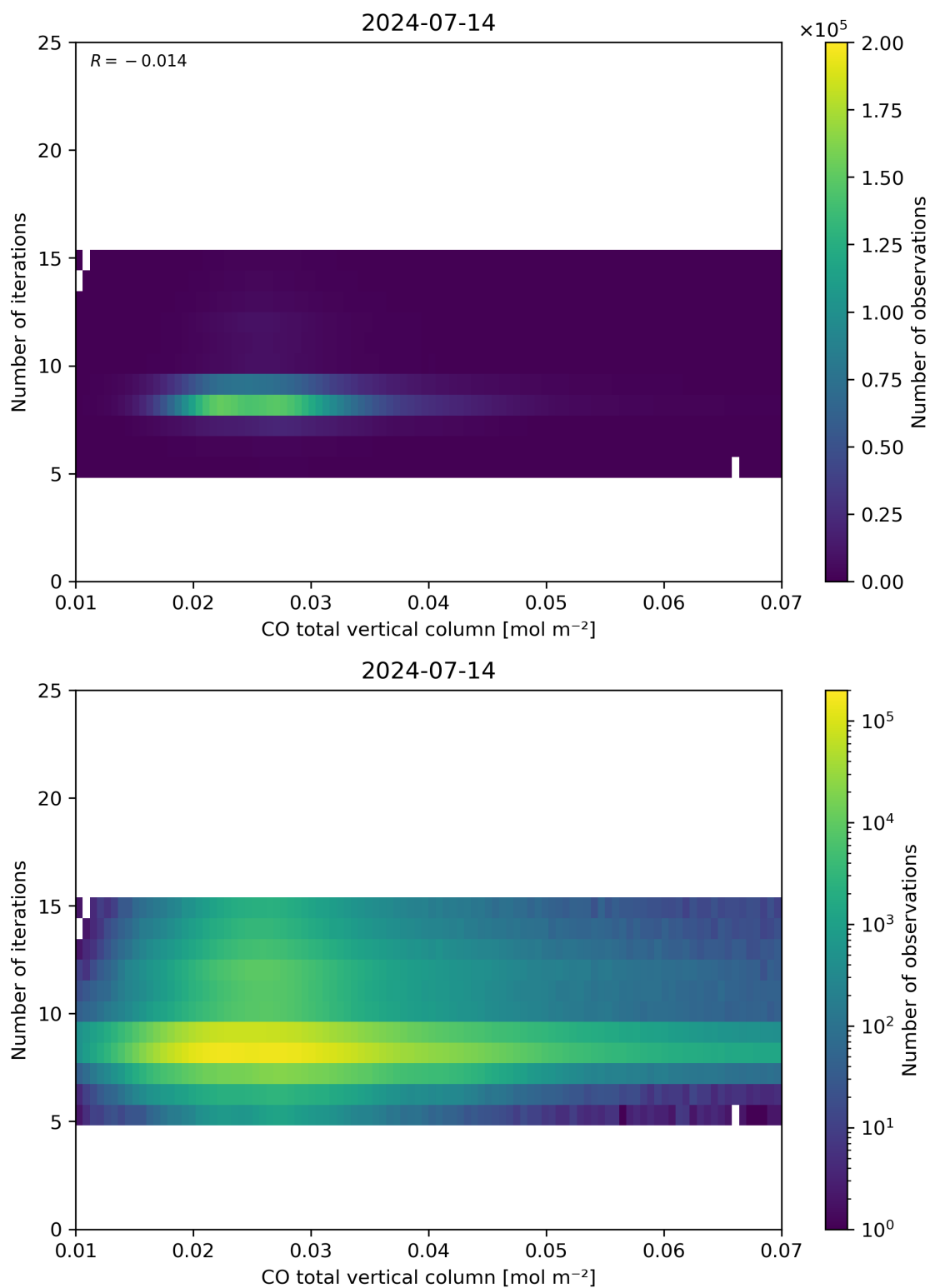
Figure 42: Scatter density plot of “CO total vertical column” against “Number of iterations” for 2024-07-13 to 2024-07-15.
