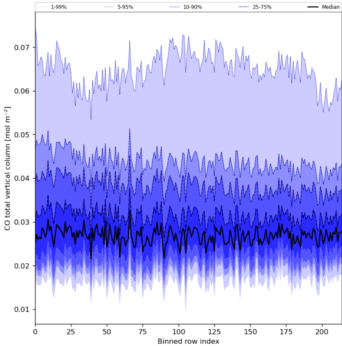
Figure 26: Along track statistics of “CO total vertical column” for 2024-07-13 to 2024-07-15
