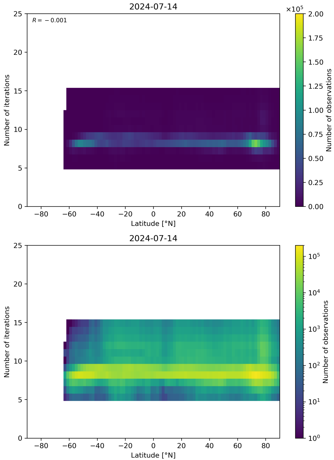
Figure 56: Scatter density plot of “Latitude” against “Number of iterations” for 2024-07-13 to 2024-07-15.
