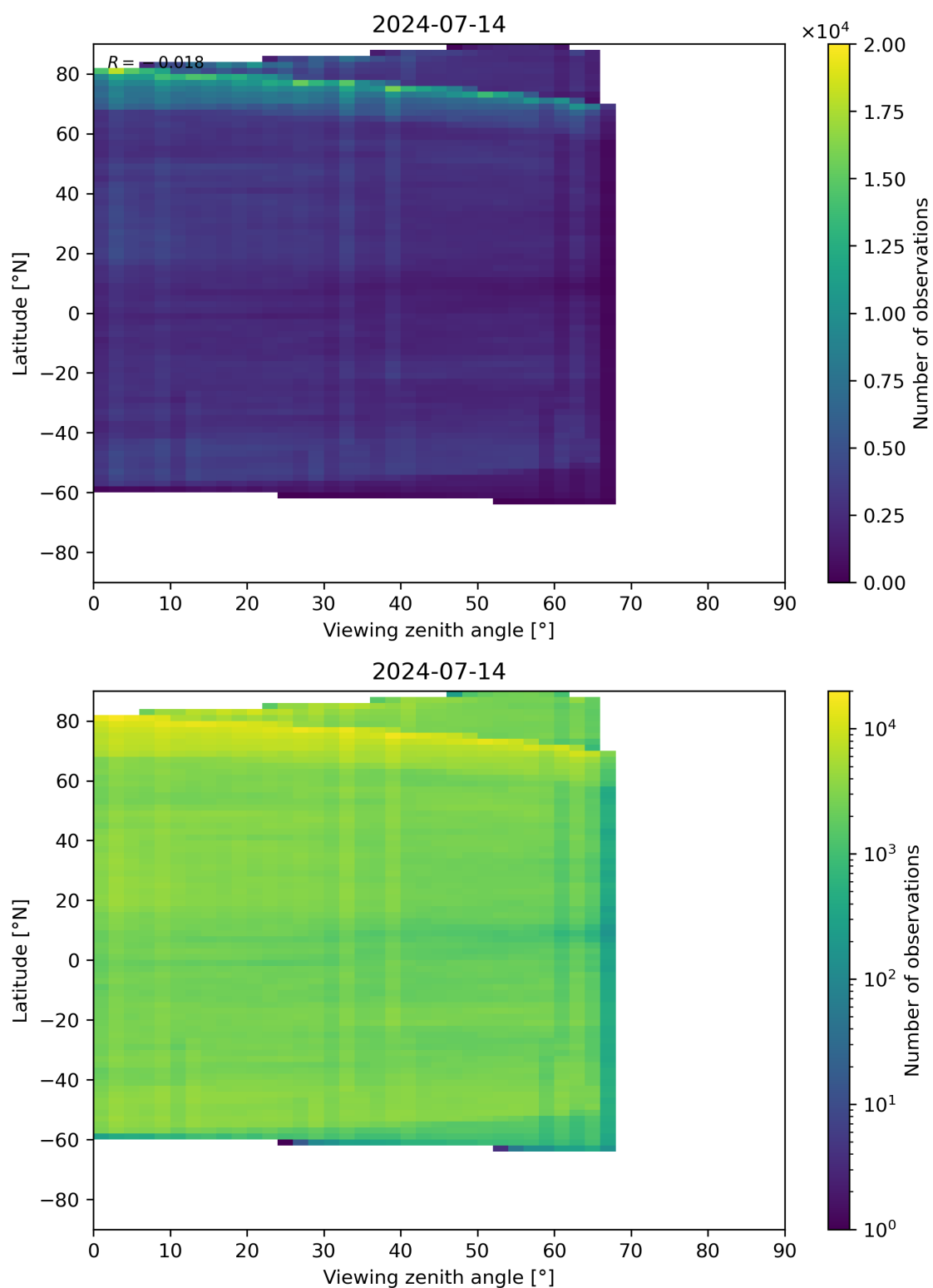
Figure 74: Scatter density plot of “Viewing zenith angle” against “Latitude” for 2024-07-13 to 2024-07-15.
