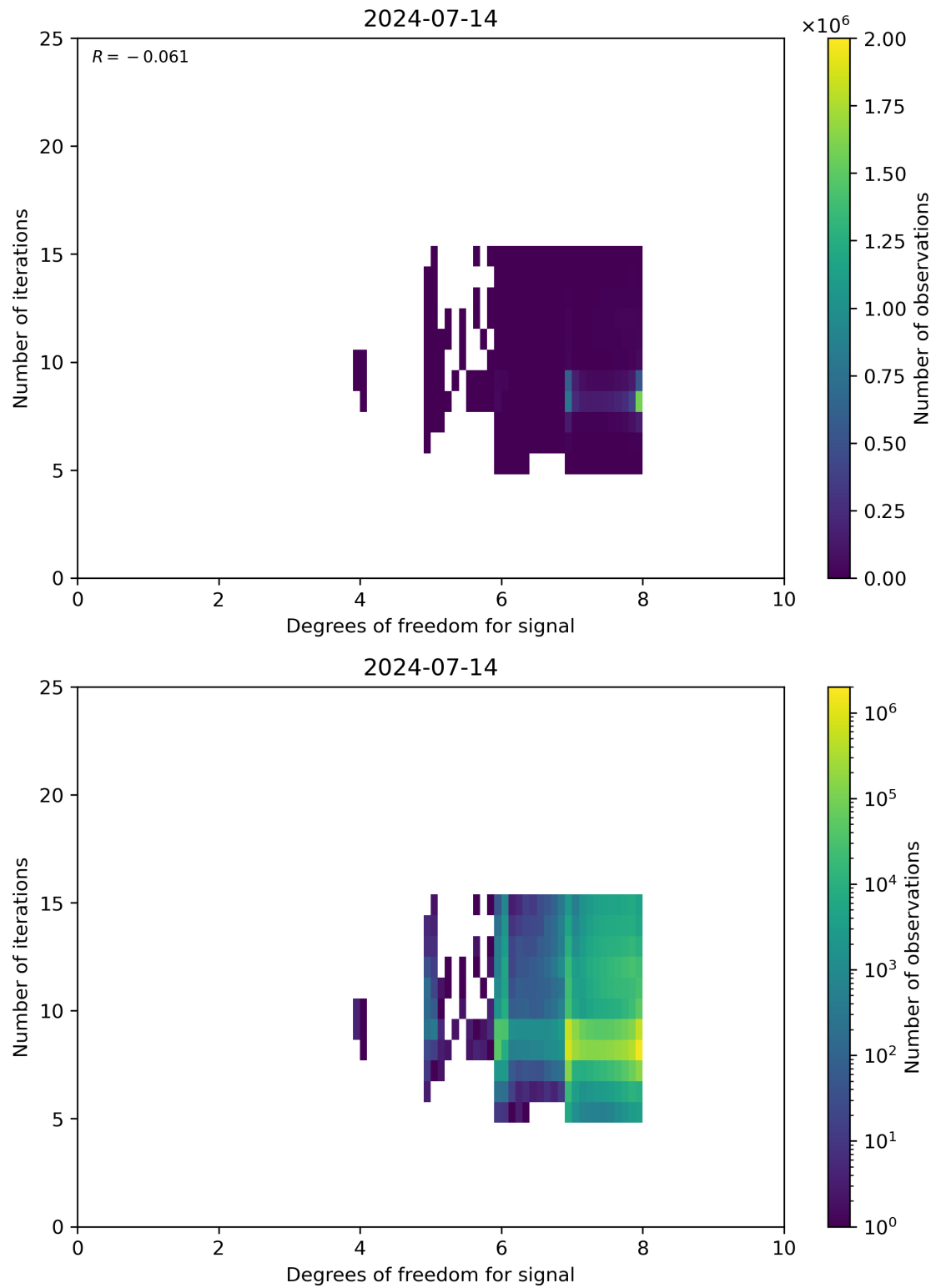
Figure 50: Scatter density plot of “Degrees of freedom for signal” against “Number of iterations” for 2024-07-13 to 2024-07-15.
