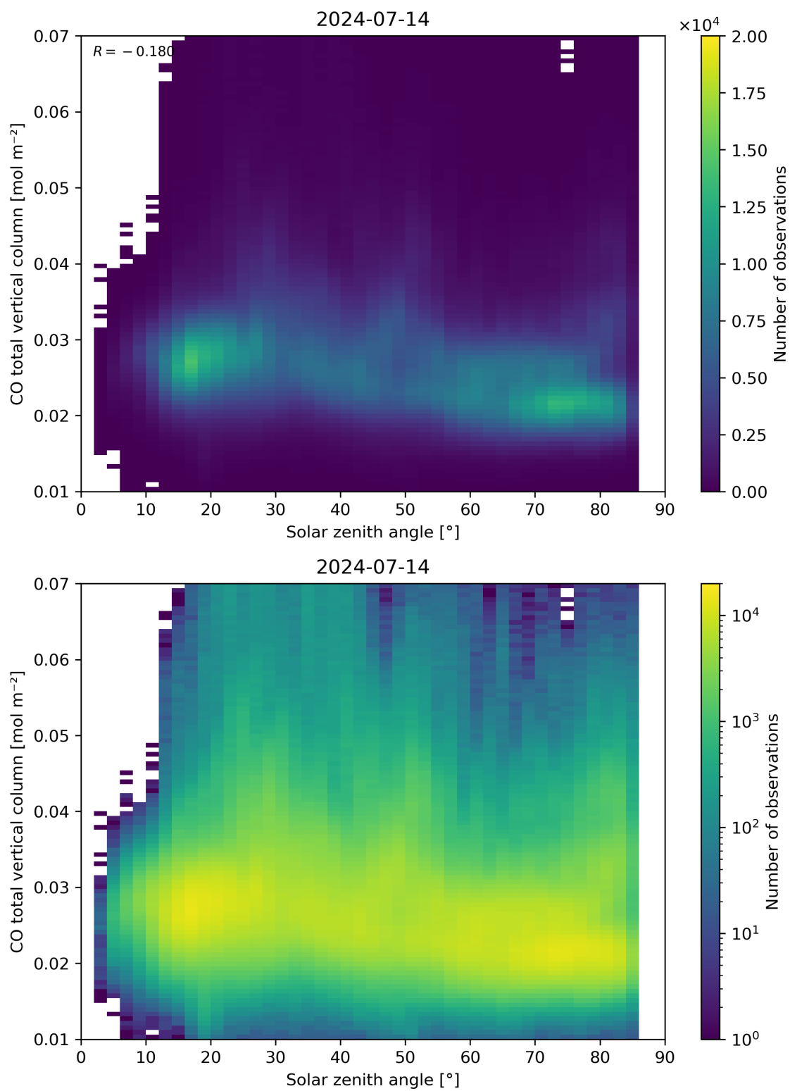
Figure 61: Scatter density plot of “Solar zenith angle” against “CO total vertical column” for 2024-07-13 to 2024-07-15.
