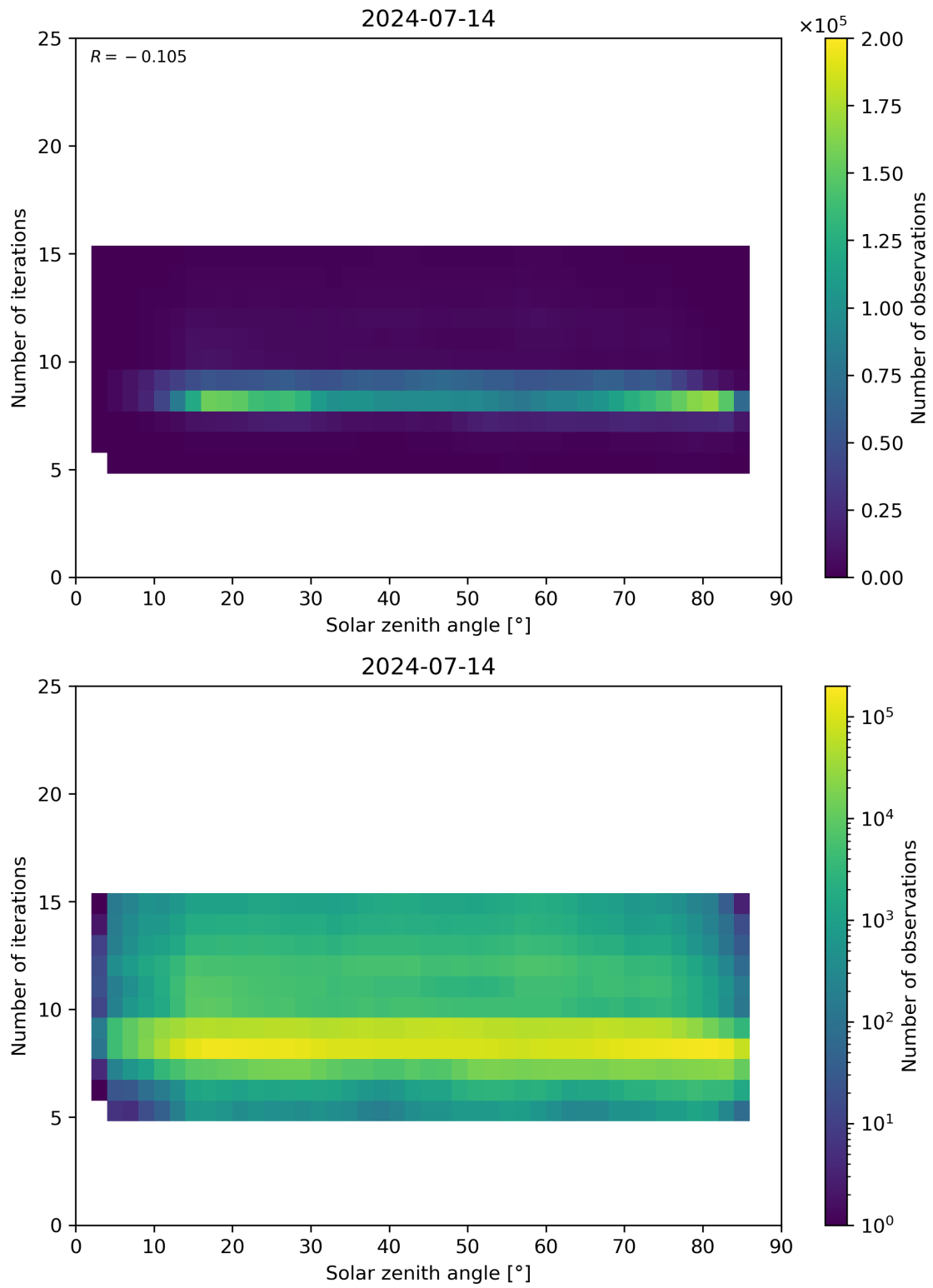
Figure 67: Scatter density plot of “Solar zenith angle” against “Number of iterations” for 2024-07-13 to 2024-07-15.
