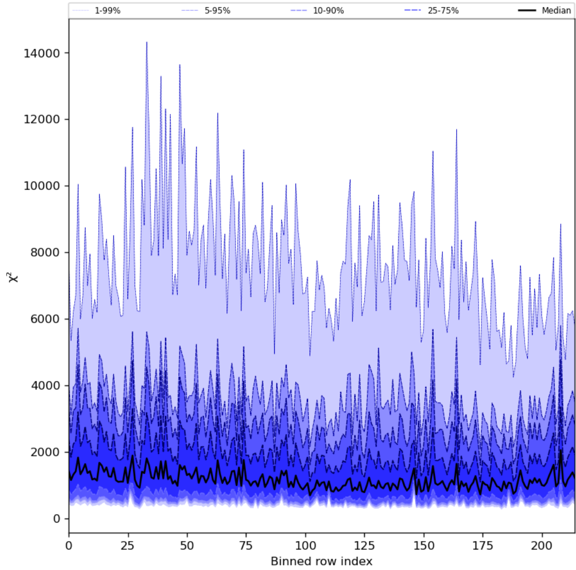
Figure 30: Along track statistics of “ \chi^2 ” for 2024-07-13 to 2024-07-15
