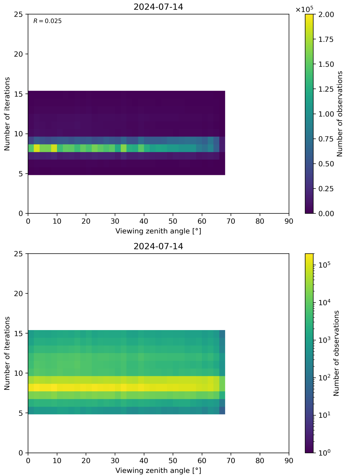
Figure 75: Scatter density plot of “Viewing zenith angle” against “Number of iterations” for 2024-07-13 to 2024-07-15.
