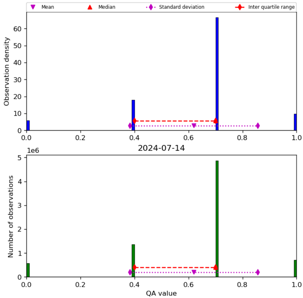
Figure 17: Histogram of “QA value” for 2024-07-13 to 2024-07-15
