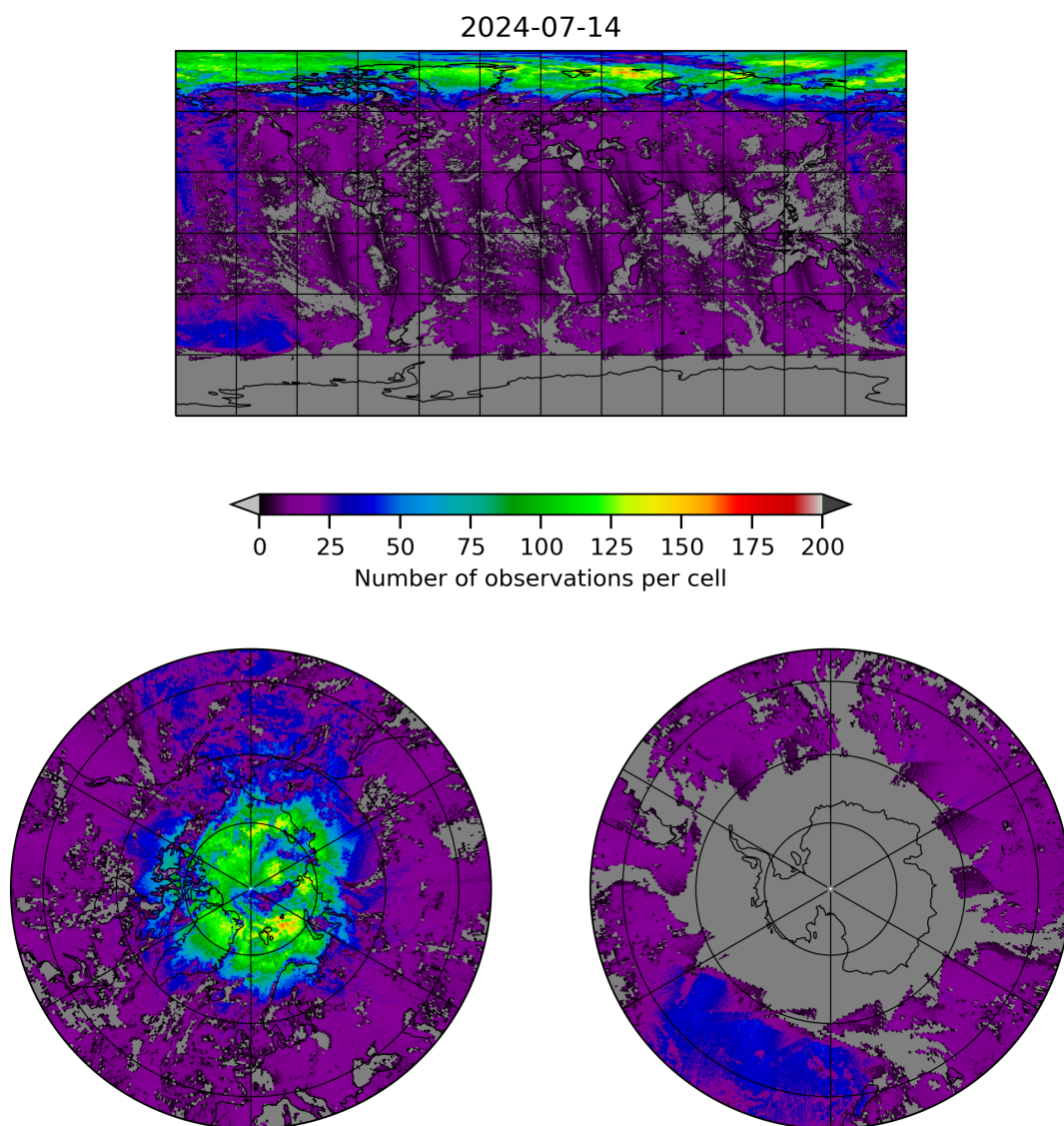
Figure 8: Map of the number of observations for 2024-07-13 to 2024-07-15
