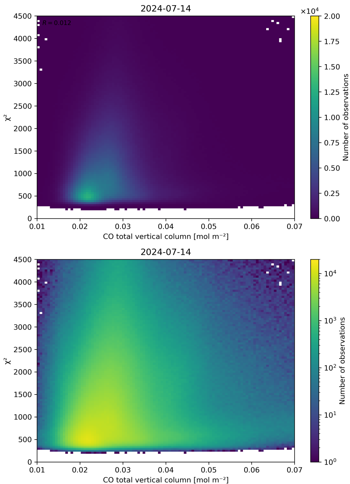
Figure 35: Scatter density plot of “CO total vertical column” against “ \chi^2 ” for 2024-07-13 to 2024-07-15.
