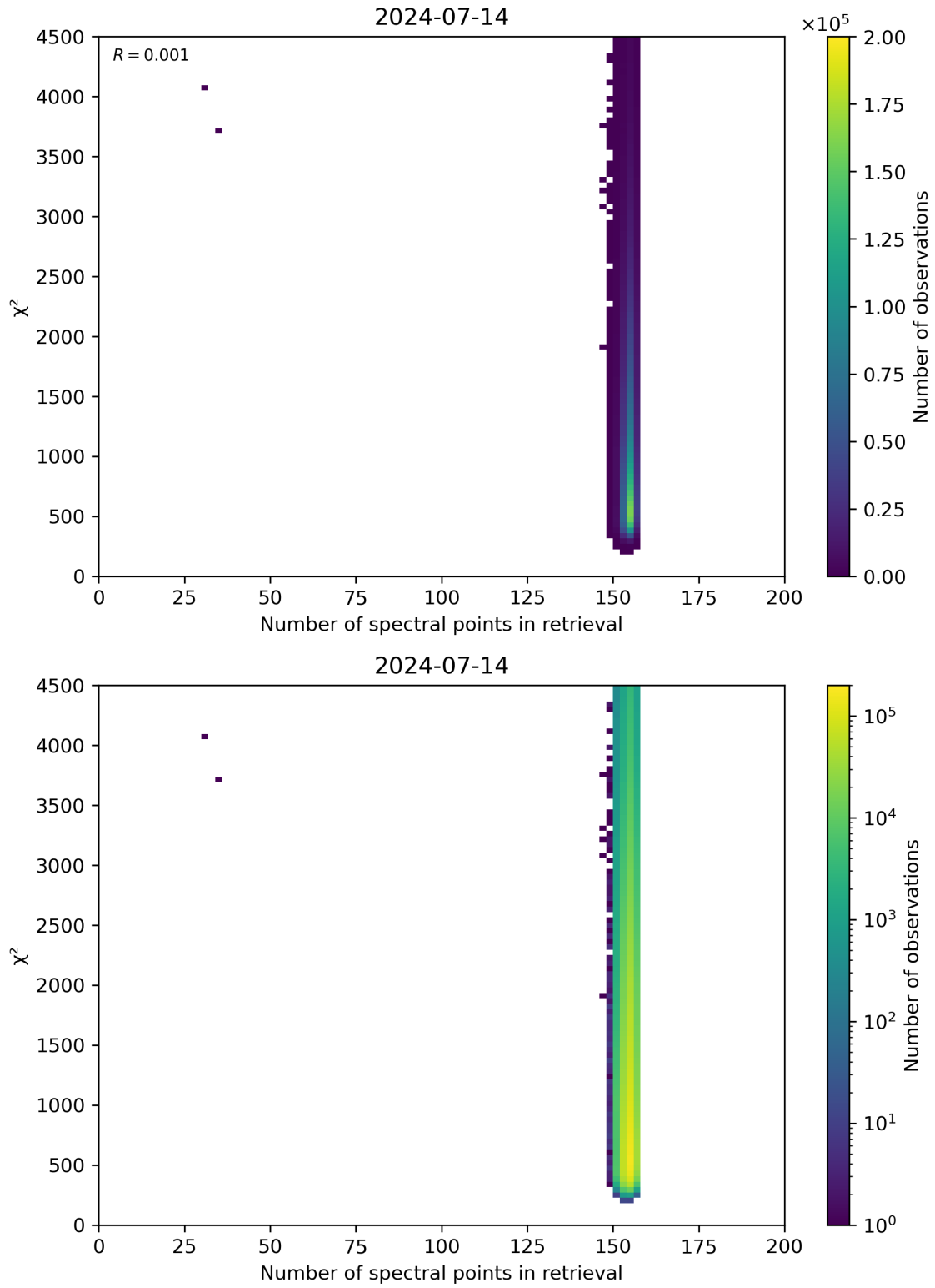
Figure 58: Scatter density plot of “Number of spectral points in retrieval” against “ \chi^2 ” for 2024-07-13 to 2024-07-15.
