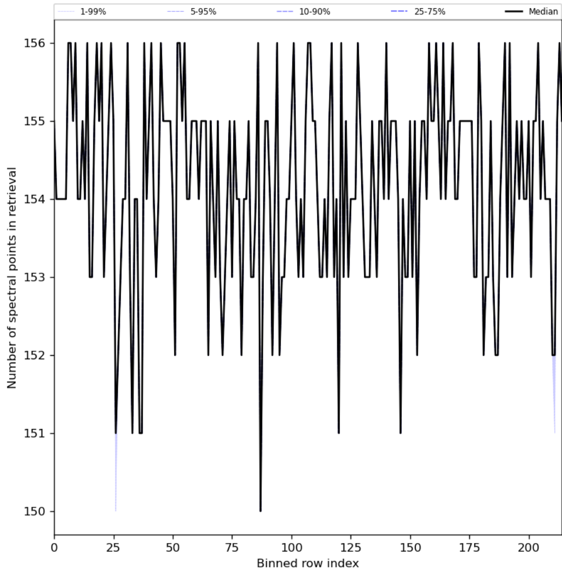
Figure 29: Along track statistics of “Number of spectral points in retrieval” for 2024-07-13 to 2024-07-15
