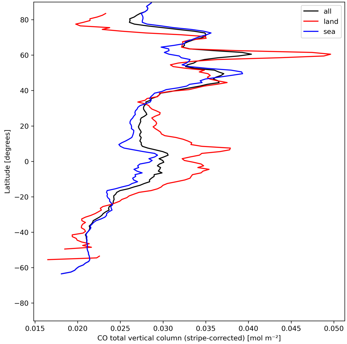
Figure 11: Zonal average of “CO total vertical column (stripe-corrected)” for 2024-07-13 to 2024-07-15.
