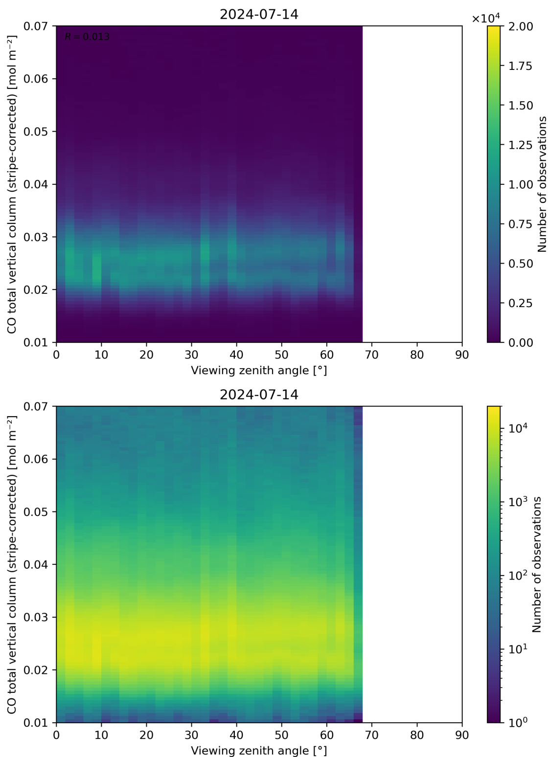
Figure 70: Scatter density plot of “Viewing zenith angle” against “CO total vertical column (stripe-corrected)” for 2024-07-13 to 2024-07-15.
