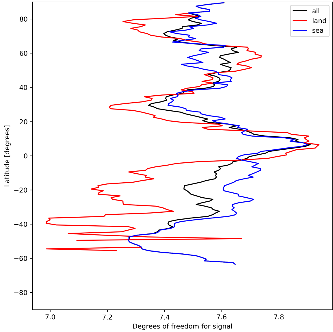
Figure 15: Zonal average of “Degrees of freedom for signal” for 2024-07-13 to 2024-07-15.
