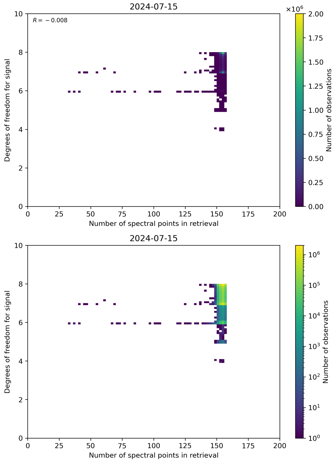
Figure 59: Scatter density plot of “Number of spectral points in retrieval” against “Degrees of freedom for signal” for 2024-07-15 to 2024-07-16.
