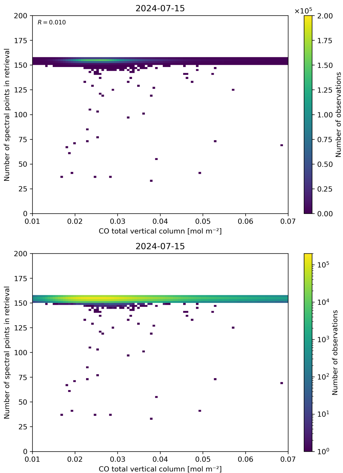
Figure 43: Scatter density plot of “CO total vertical column” against “Number of spectral points in retrieval” for 2024-07-15 to 2024-07-16.
