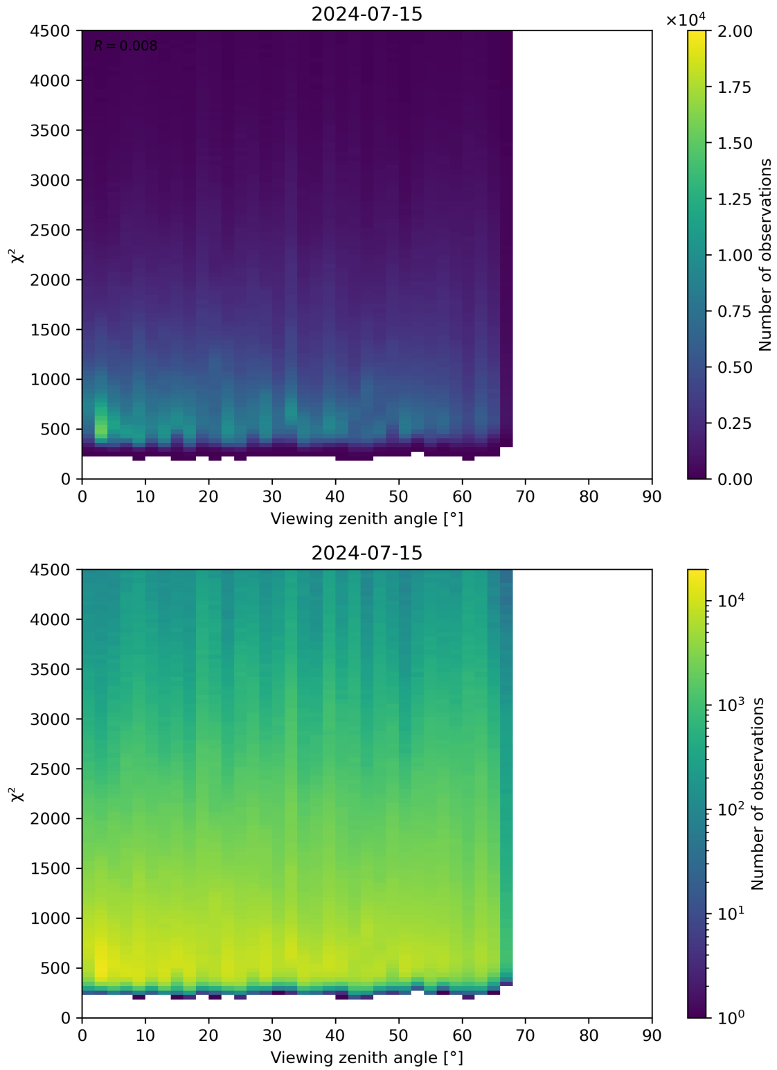
Figure 72: Scatter density plot of “Viewing zenith angle” against “ \chi^2 ” for 2024-07-15 to 2024-07-16.
