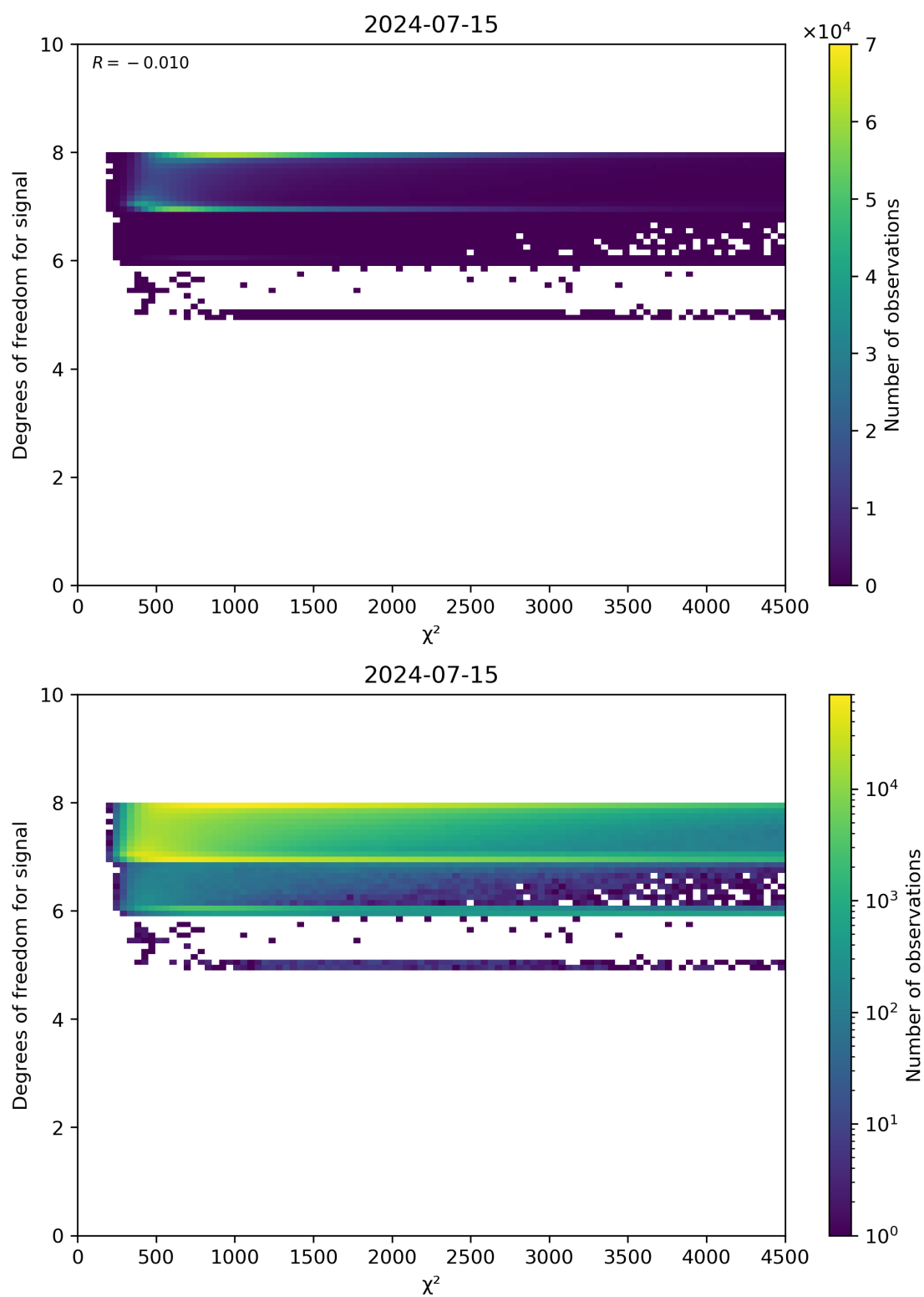
Figure 48: Scatter density plot of “ \chi^2 ” against “Degrees of freedom for signal” for 2024-07-15 to 2024-07-16.
