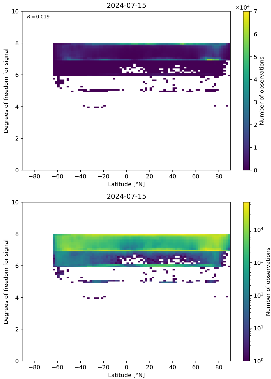
Figure 55: Scatter density plot of “Latitude” against “Degrees of freedom for signal” for 2024-07-15 to 2024-07-16.
