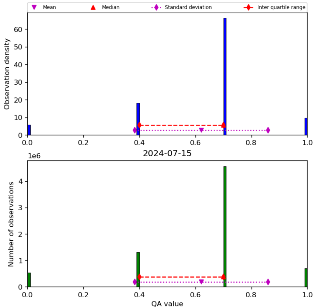
Figure 17: Histogram of “QA value” for 2024-07-15 to 2024-07-16
