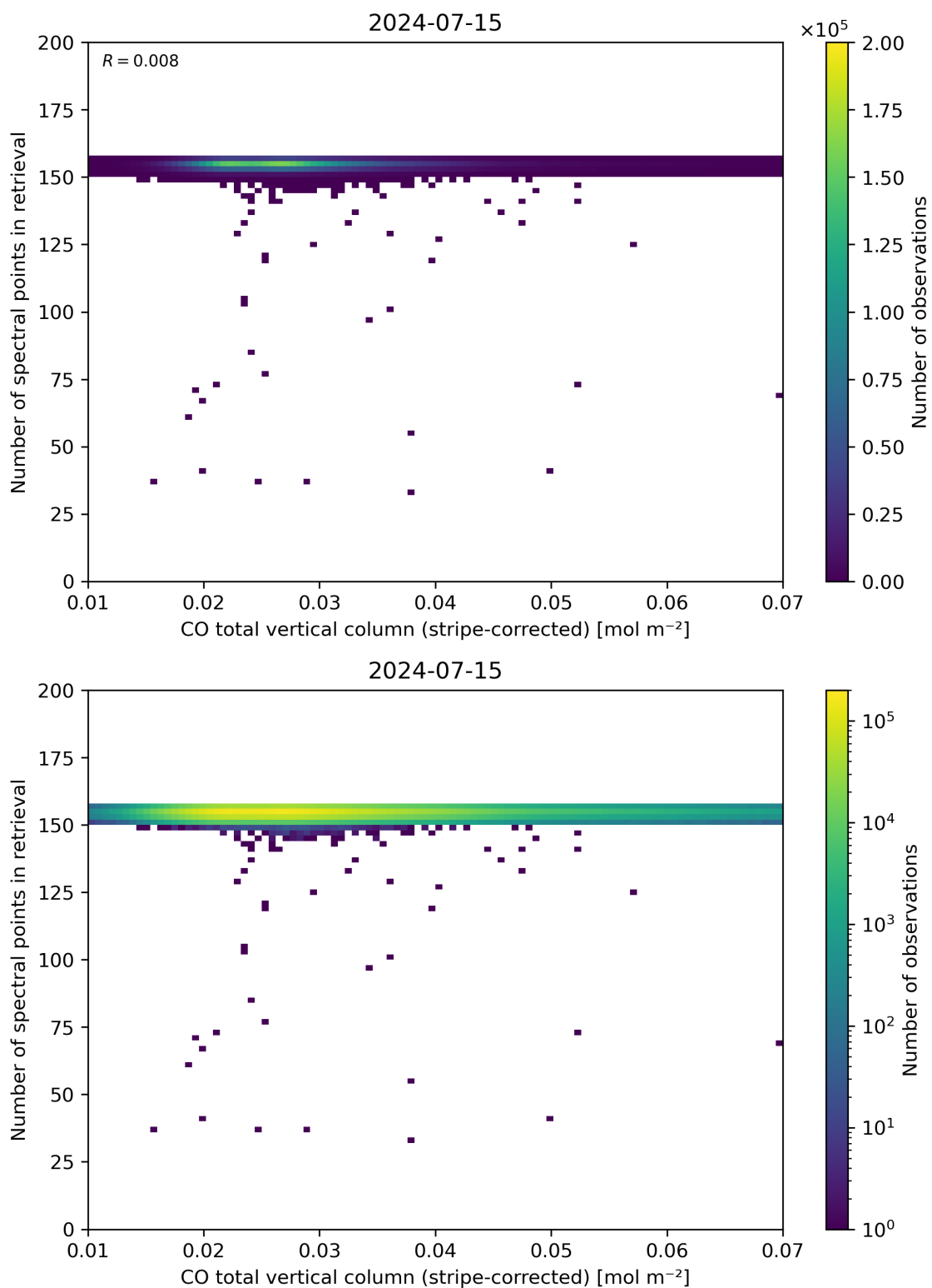
Figure 40: Scatter density plot of “CO total vertical column (stripe-corrected)” against “Number of spectral points in retrieval” for 2024-07-15 to 2024-07-16.
