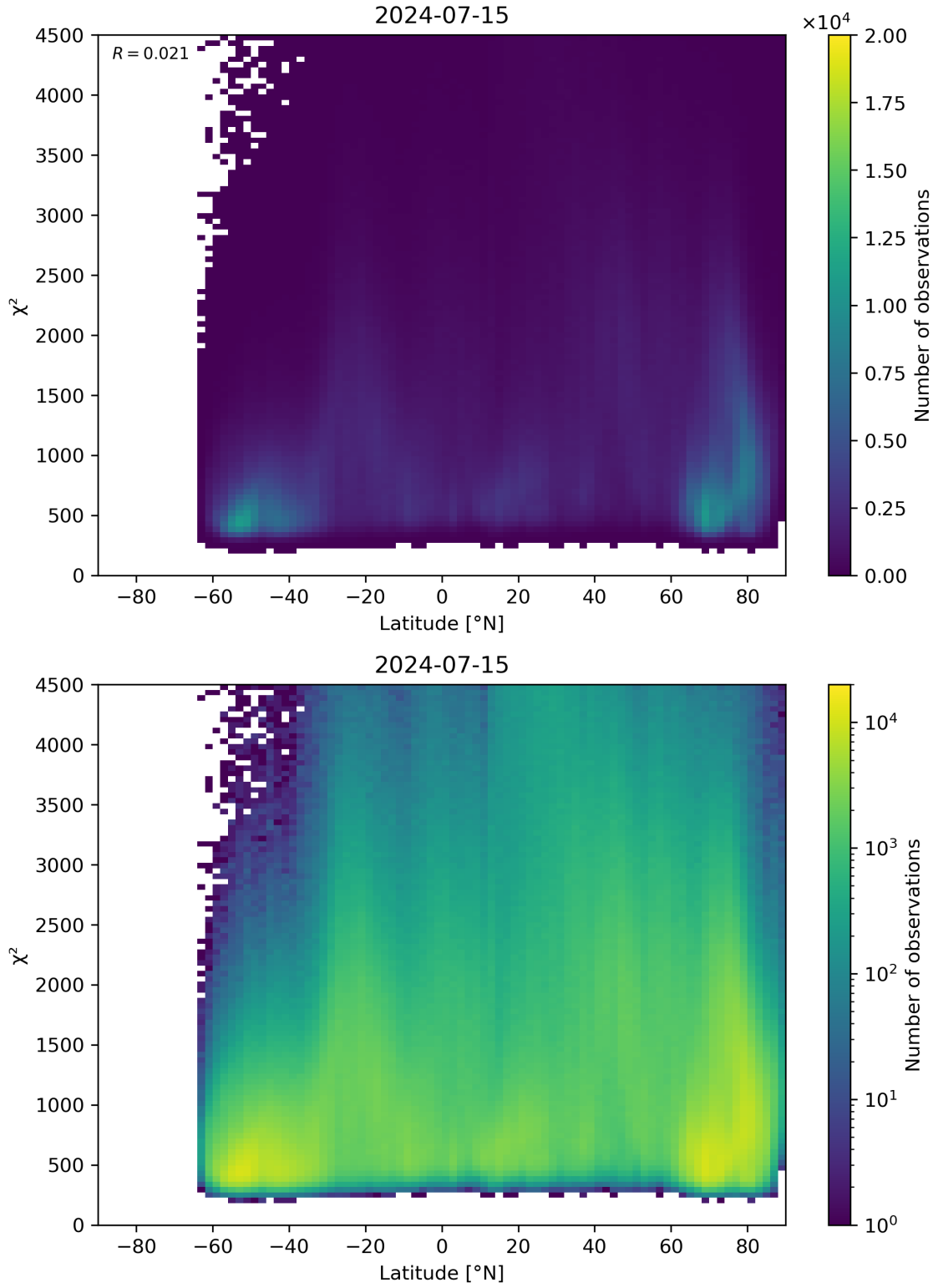
Figure 54: Scatter density plot of “Latitude” against “ \chi^2 ” for 2024-07-15 to 2024-07-16.
