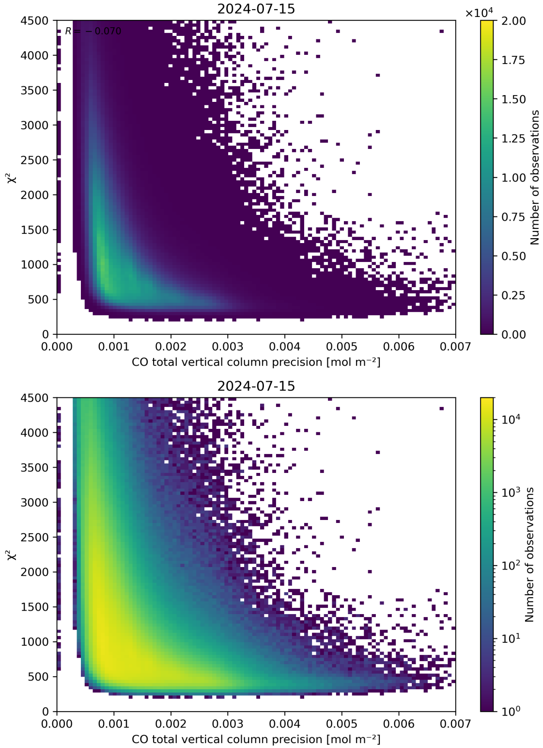
Figure 44: Scatter density plot of “CO total vertical column precision” against “ \chi^2 ” for 2024-07-15 to 2024-07-16.
