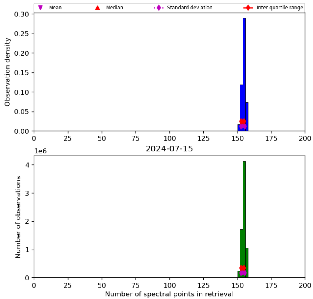
Figure 21: Histogram of “Number of spectral points in retrieval” for 2024-07-15 to 2024-07-16
