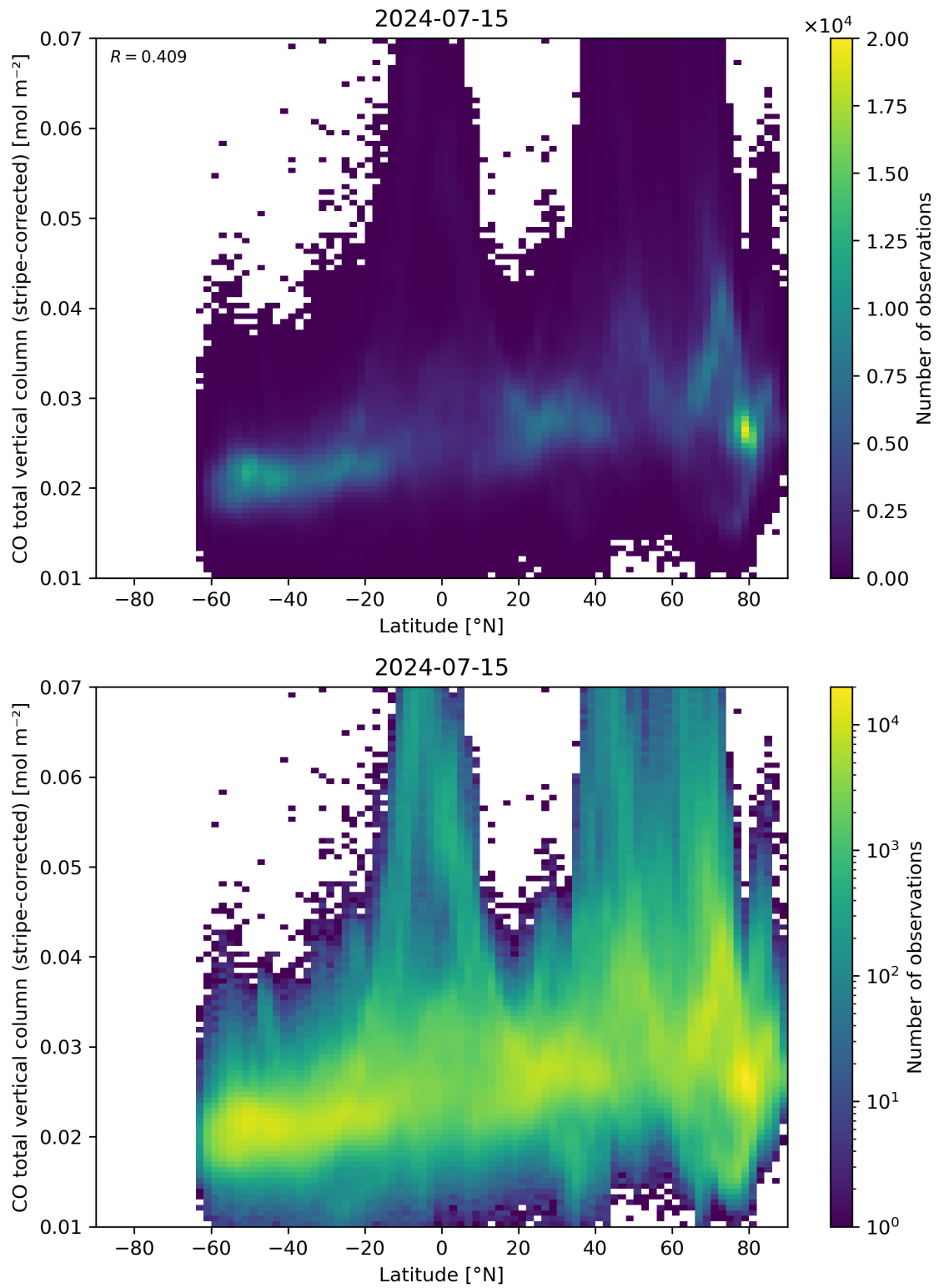
Figure 52: Scatter density plot of “Latitude” against “CO total vertical column (stripe-corrected)” for 2024-07-15 to 2024-07-16.
