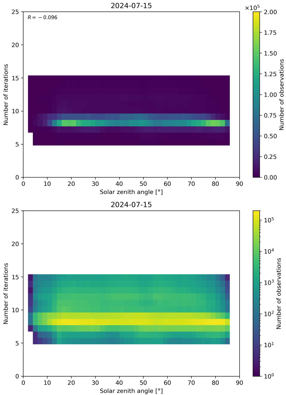
Figure 67: Scatter density plot of “Solar zenith angle” against “Number of iterations” for 2024-07-15 to 2024-07-16.
