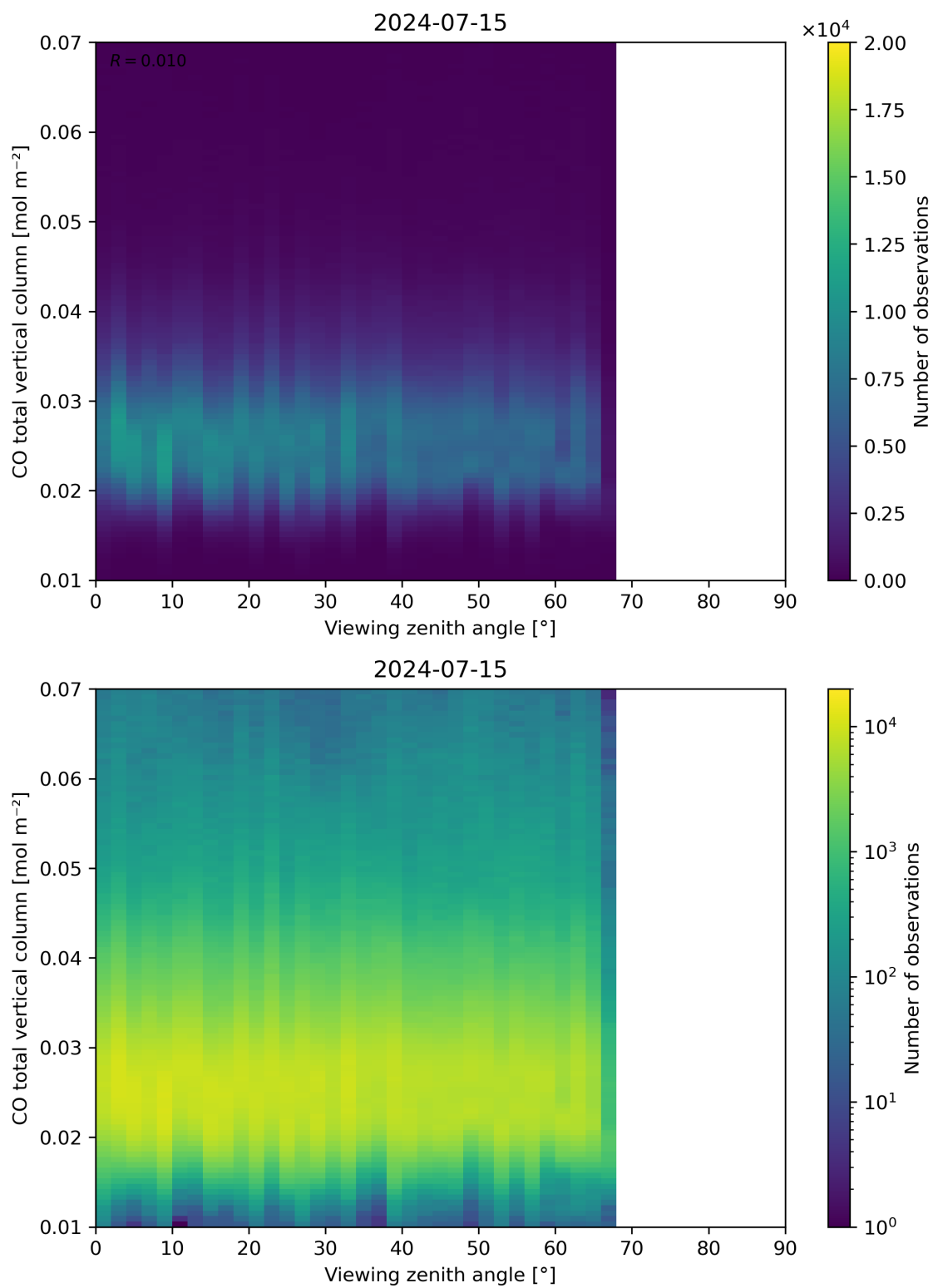
Figure 69: Scatter density plot of “Viewing zenith angle” against “CO total vertical column” for 2024-07-15 to 2024-07-16.
