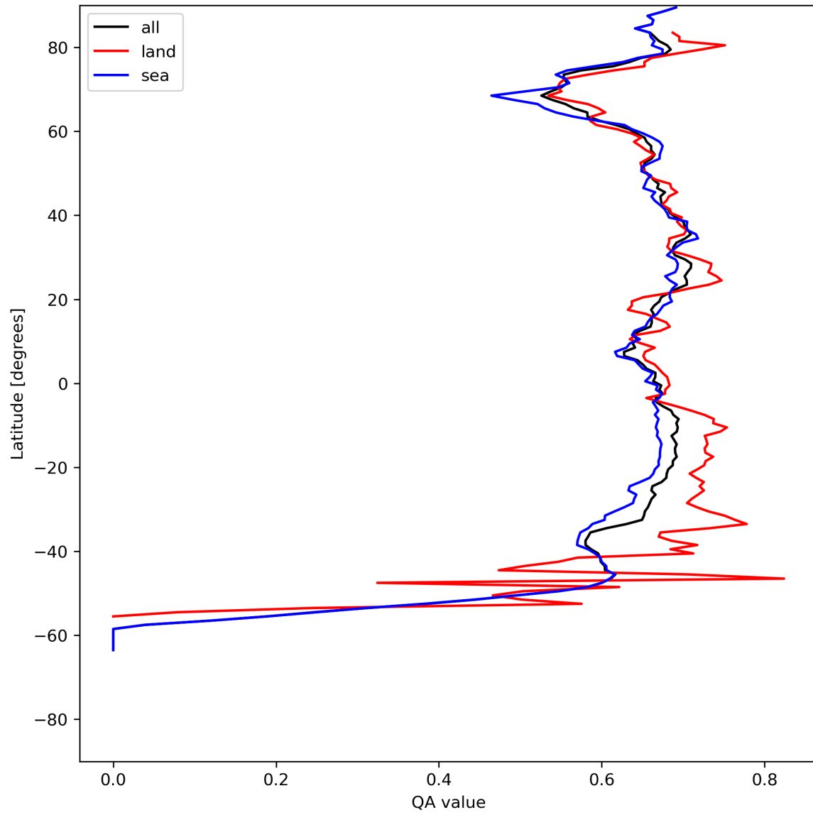
Figure 9: Zonal average of “QA value” for 2024-07-15 to 2024-07-16.
