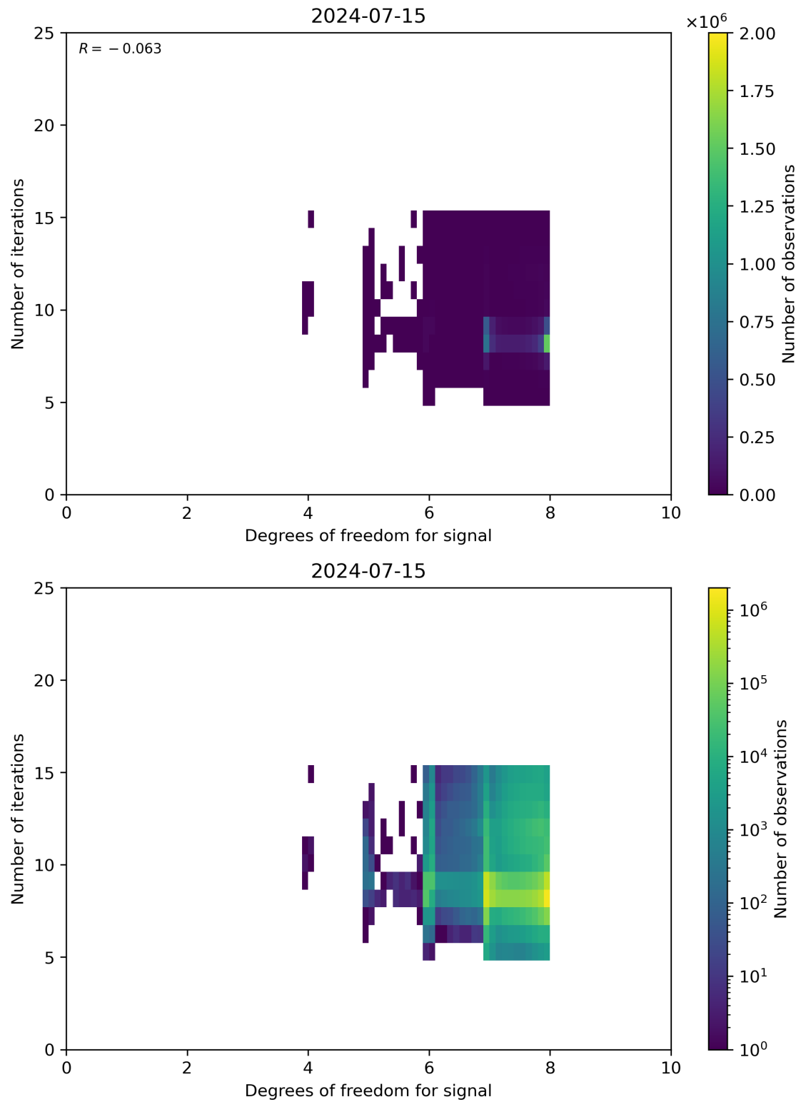
Figure 50: Scatter density plot of “Degrees of freedom for signal” against “Number of iterations” for 2024-07-15 to 2024-07-16.
