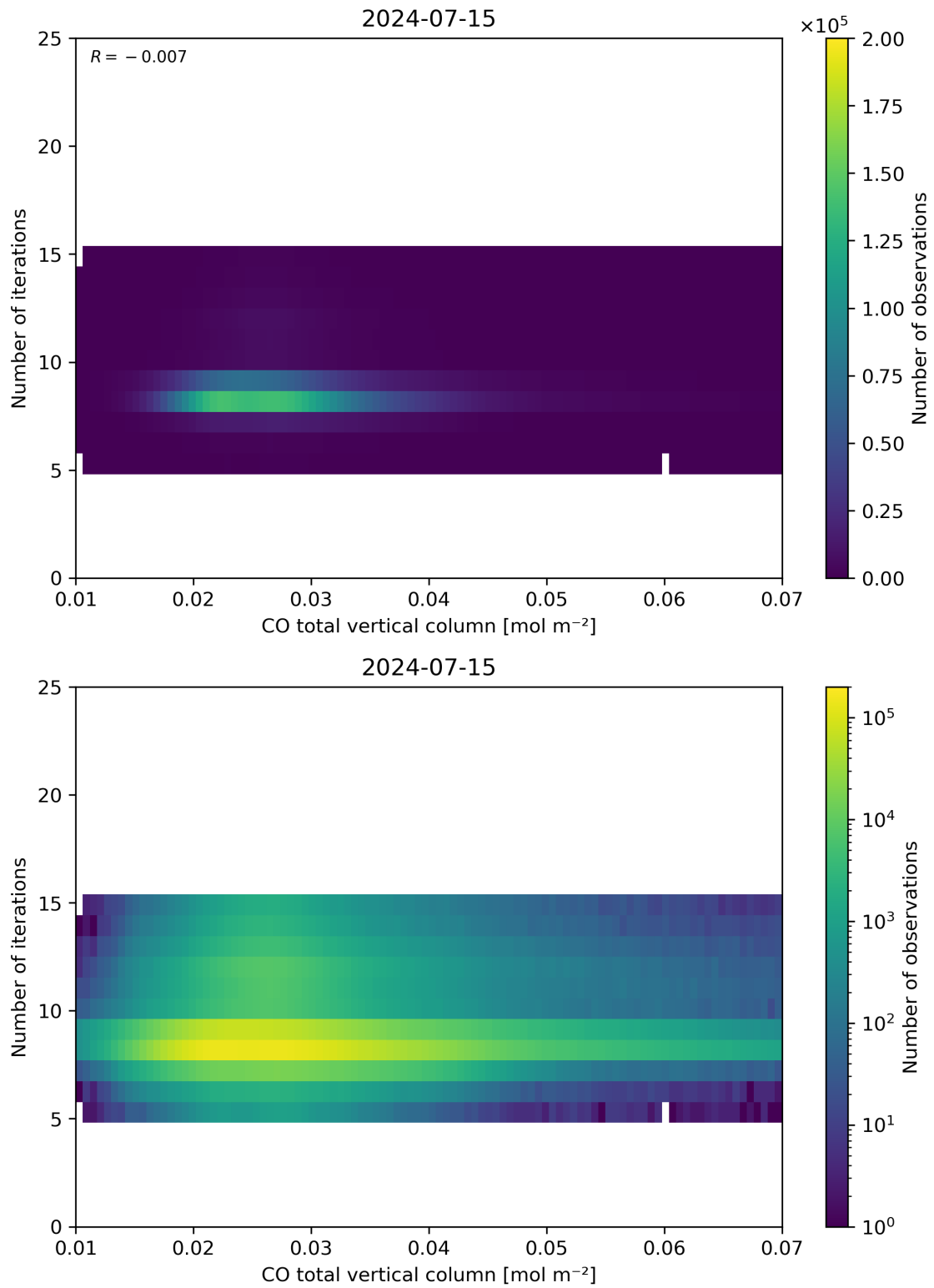
Figure 42: Scatter density plot of “CO total vertical column” against “Number of iterations” for 2024-07-15 to 2024-07-16.
