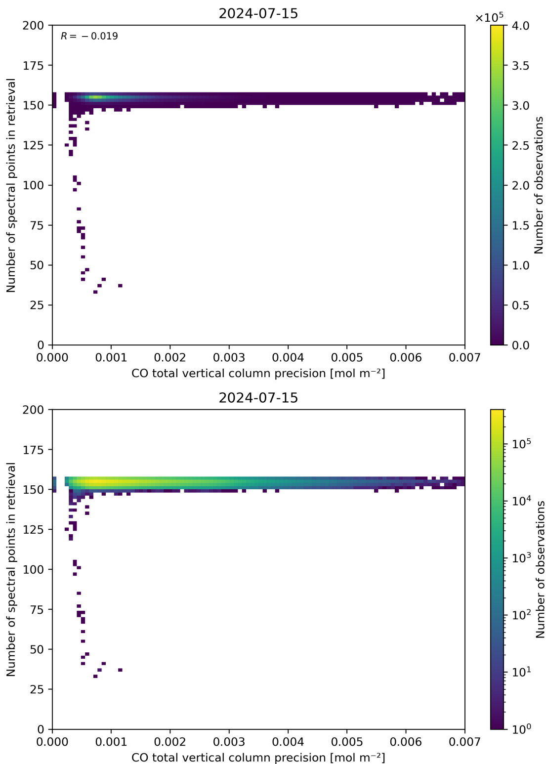
Figure 47: Scatter density plot of “CO total vertical column precision” against “Number of spectral points in retrieval” for 2024-07-15 to 2024-07-16.
