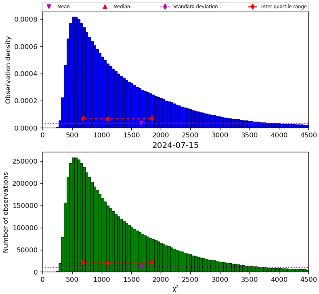
Figure 22: Histogram of “ \chi^2 ” for 2024-07-15 to 2024-07-16
