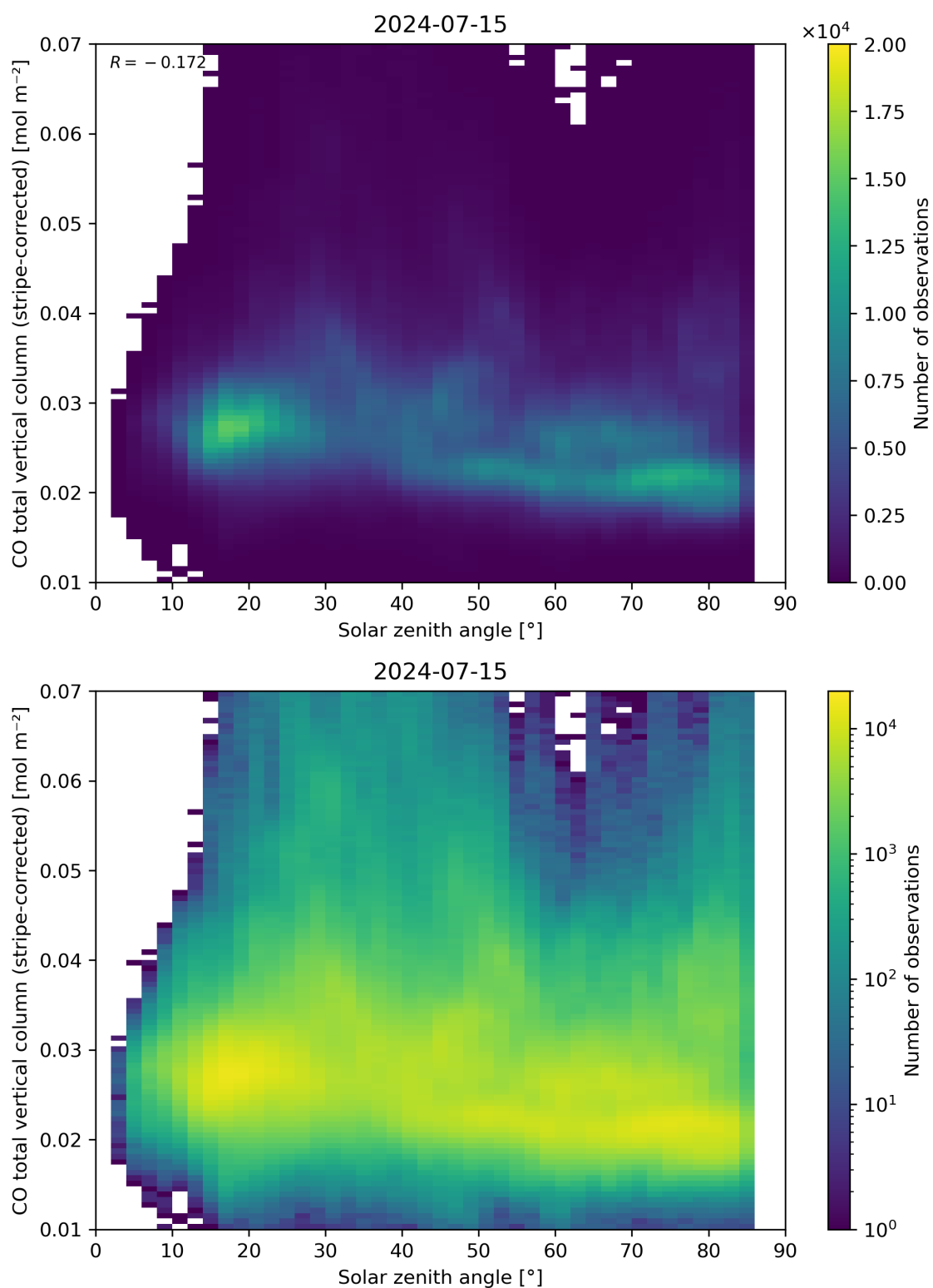
Figure 62: Scatter density plot of “Solar zenith angle” against “CO total vertical column (stripe-corrected)” for 2024-07-15 to 2024-07-16.
