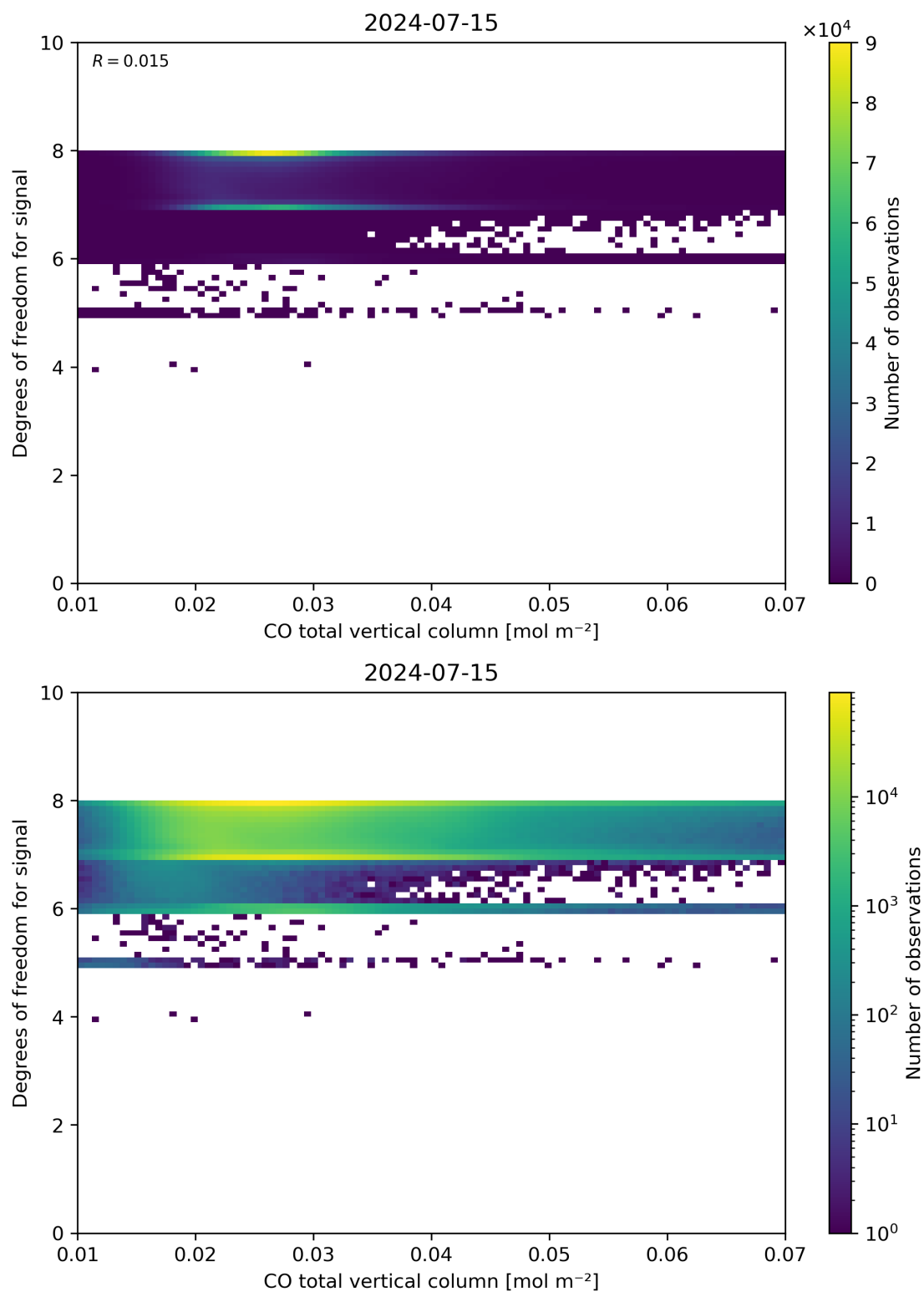
Figure 41: Scatter density plot of “CO total vertical column” against “Degrees of freedom for signal” for 2024-07-15 to 2024-07-16.
