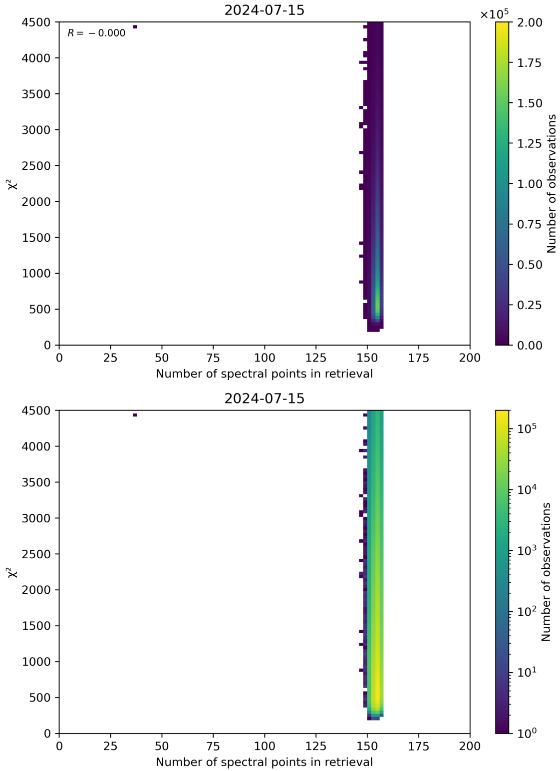
Figure 58: Scatter density plot of “Number of spectral points in retrieval” against “ \chi^2 ” for 2024-07-15 to 2024-07-16.
