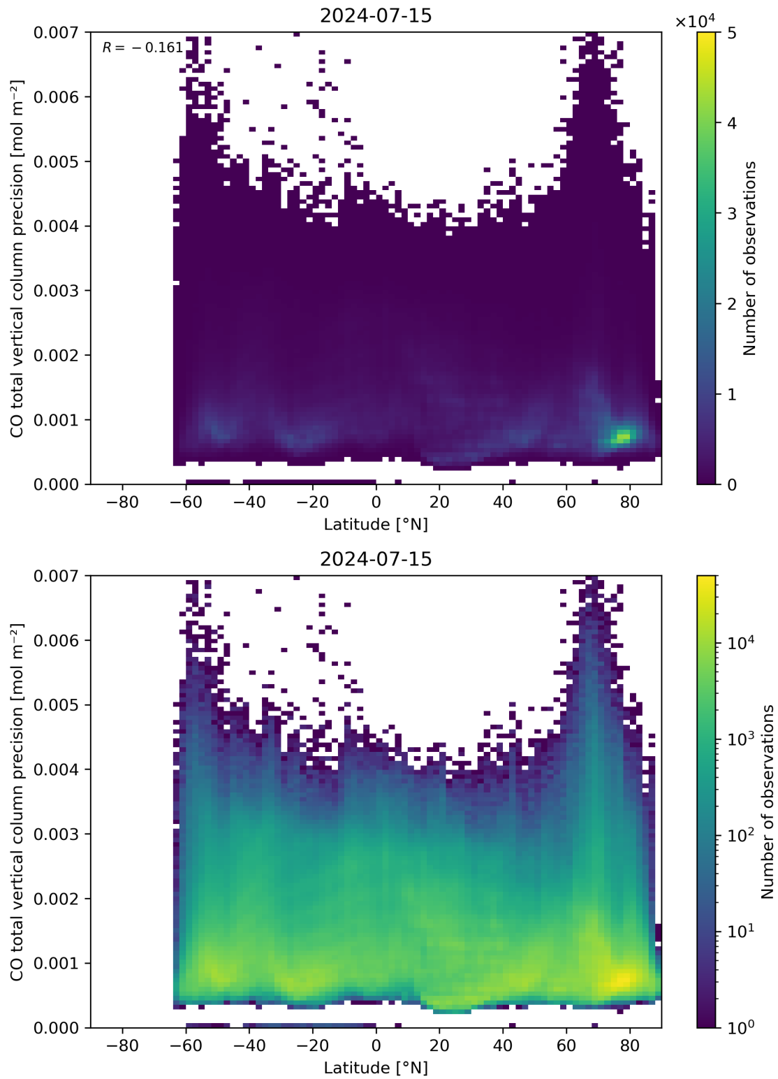
Figure 53: Scatter density plot of “Latitude” against “CO total vertical column precision” for 2024-07-15 to 2024-07-16.
