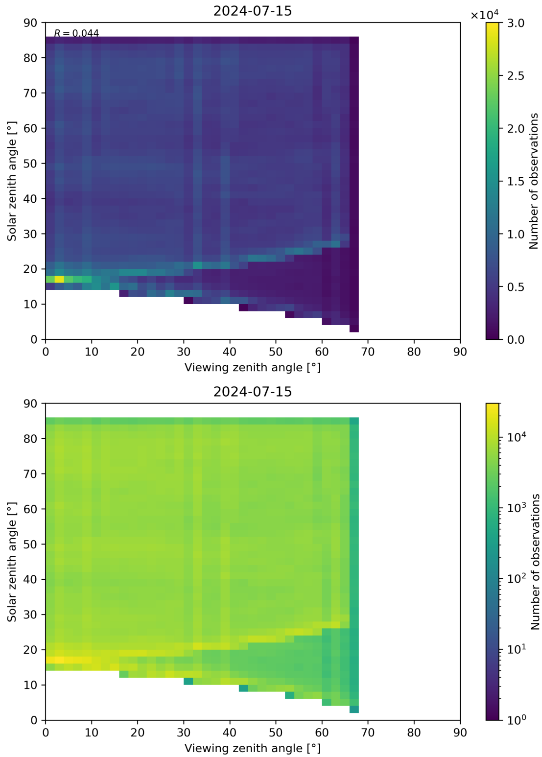
Figure 77: Scatter density plot of “Viewing zenith angle” against “Solar zenith angle” for 2024-07-15 to 2024-07-16.
