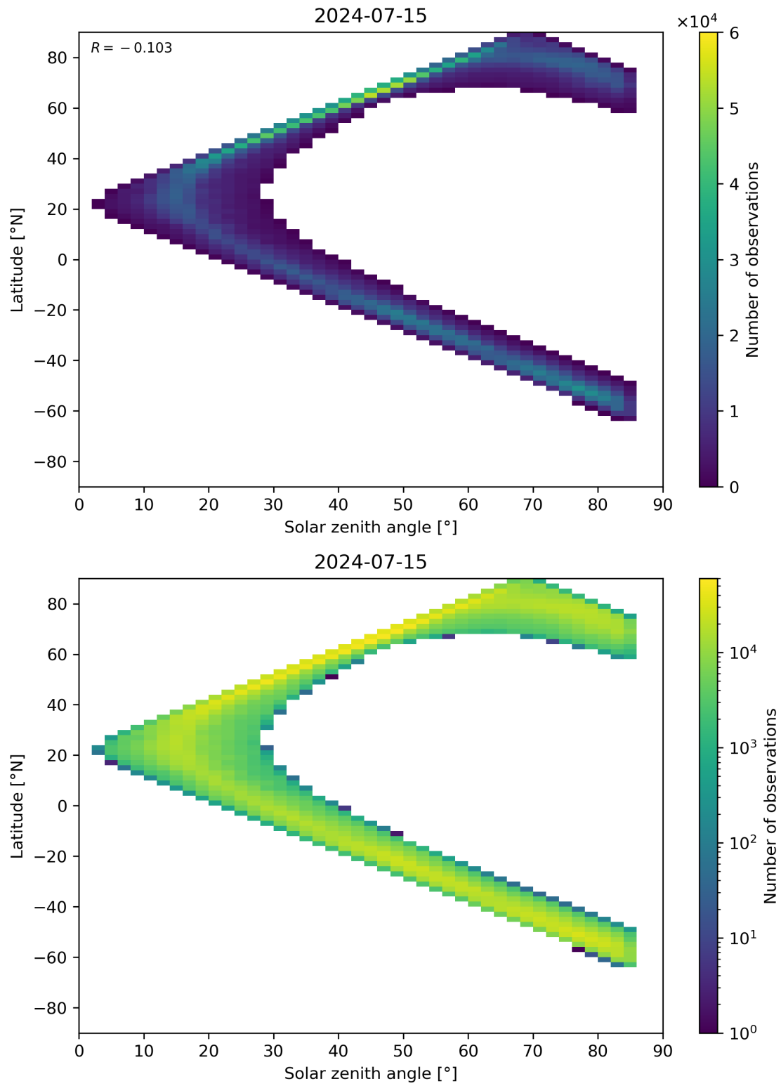
Figure 66: Scatter density plot of “Solar zenith angle” against “Latitude” for 2024-07-15 to 2024-07-16.
