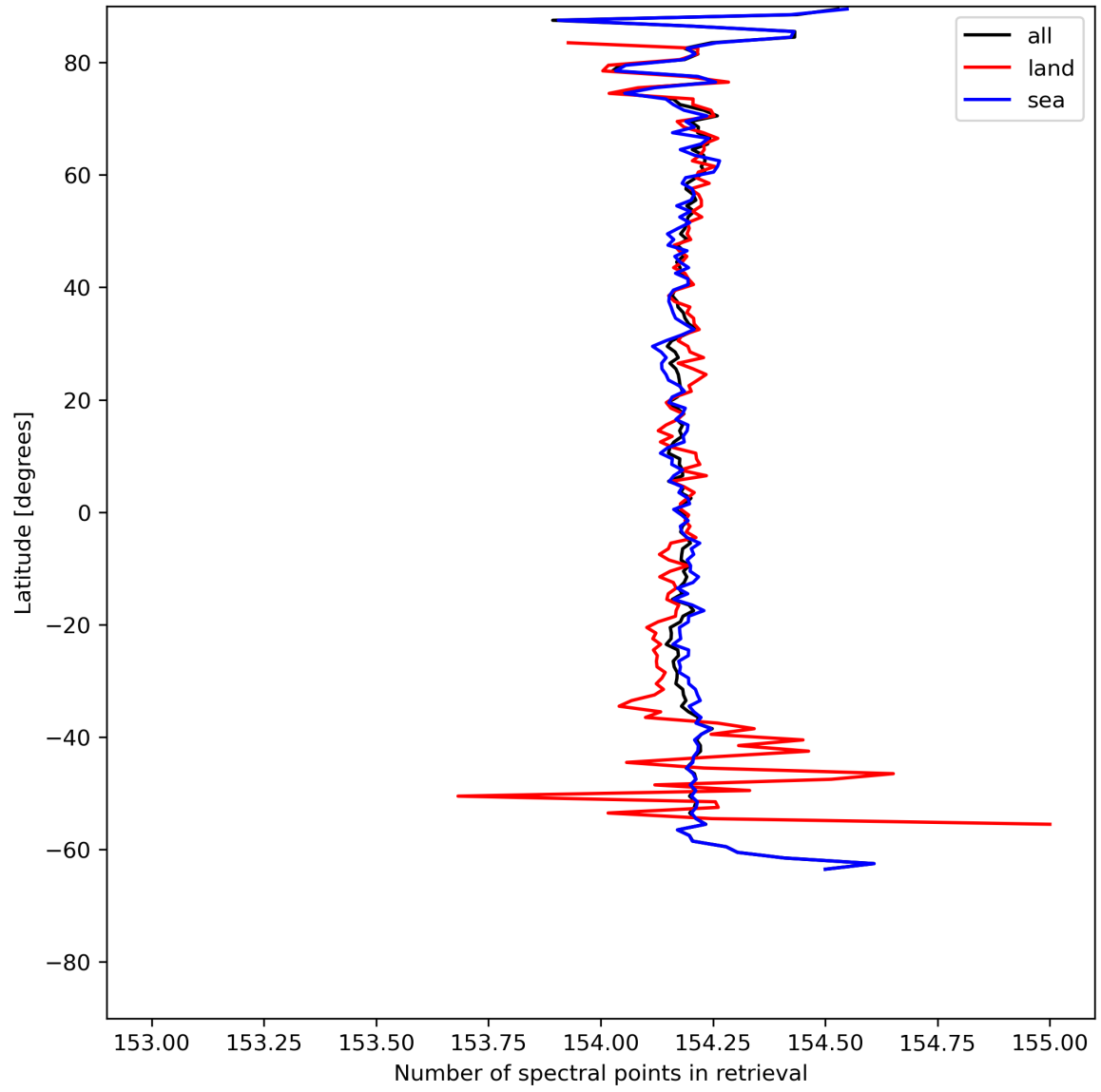
Figure 13: Zonal average of “Number of spectral points in retrieval” for 2024-07-15 to 2024-07-16.
