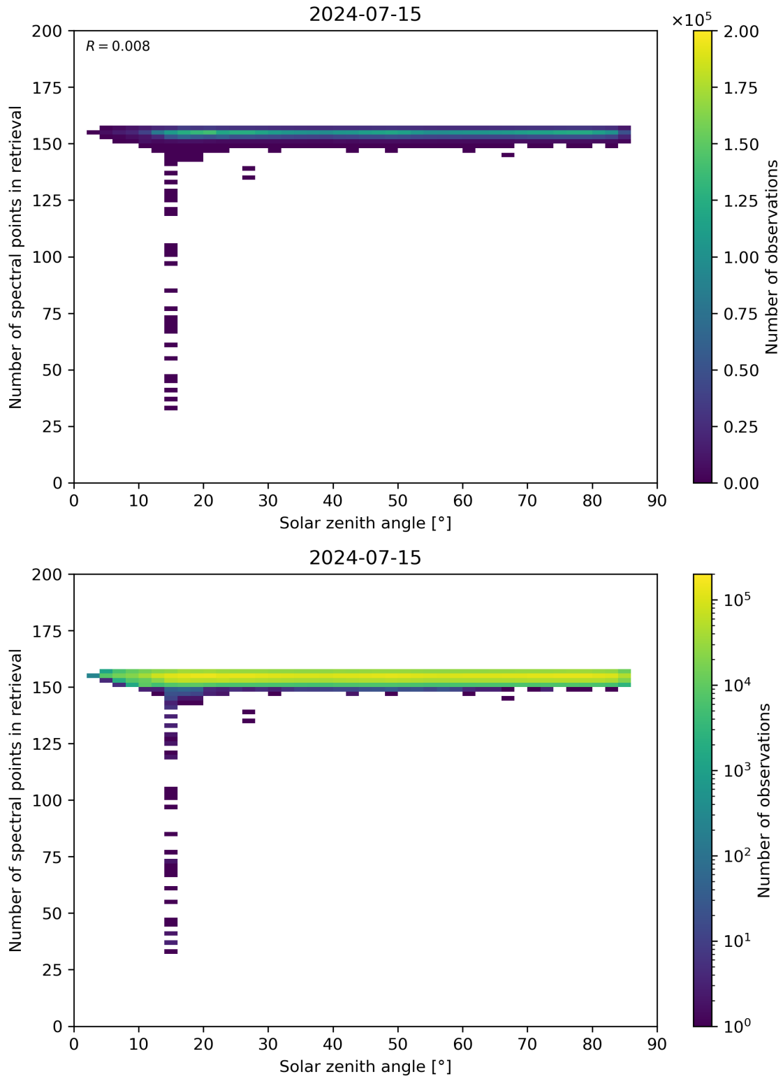
Figure 68: Scatter density plot of “Solar zenith angle” against “Number of spectral points in retrieval” for 2024-07-15 to 2024-07-16.
