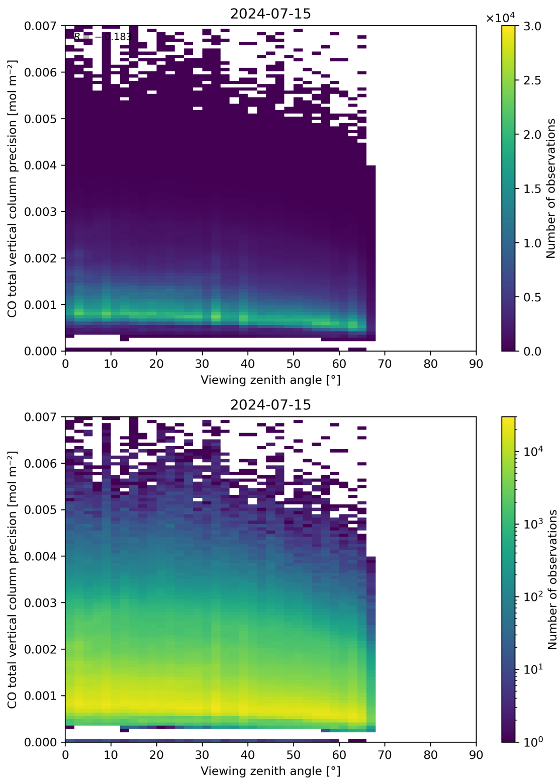
Figure 71: Scatter density plot of “Viewing zenith angle” against “CO total vertical column precision” for 2024-07-15 to 2024-07-16.
