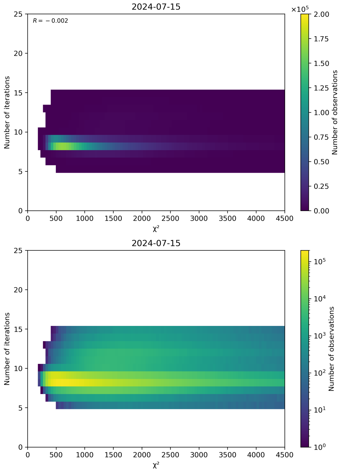
Figure 49: Scatter density plot of “ \chi^2 ” against “Number of iterations” for 2024-07-15 to 2024-07-16.
