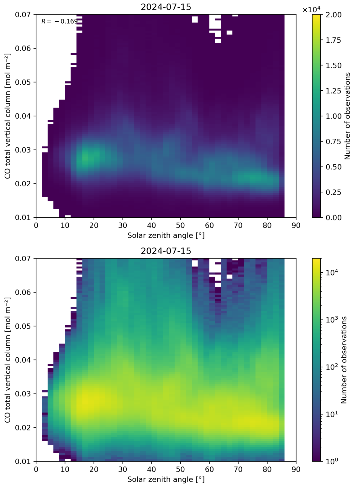
Figure 61: Scatter density plot of “Solar zenith angle” against “CO total vertical column” for 2024-07-15 to 2024-07-16.
