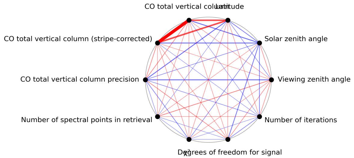
Figure 1: Map of correlation graph for 2024-07-15 to 2024-07-16.
