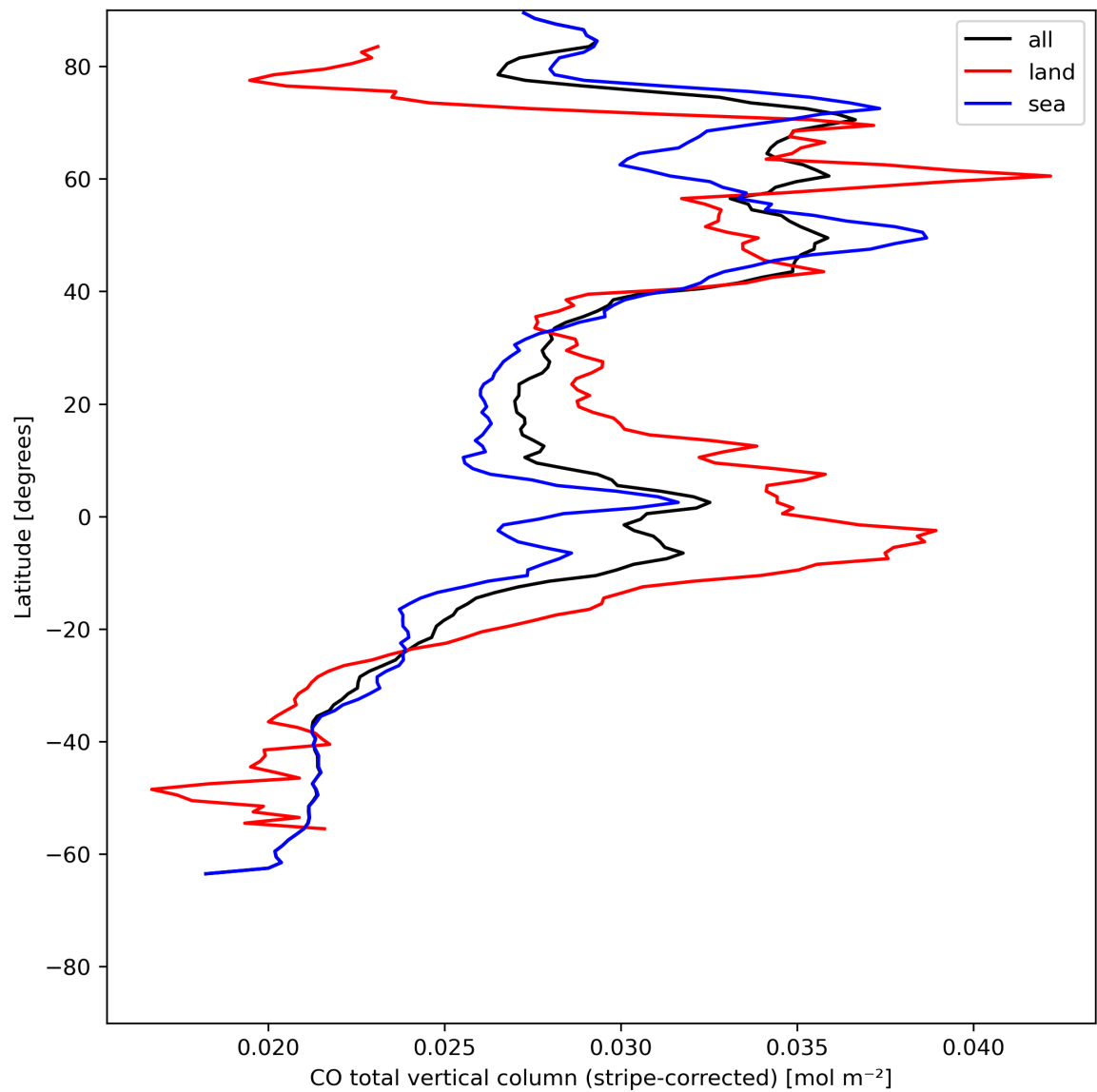
Figure 11: Zonal average of “CO total vertical column (stripe-corrected)” for 2024-07-15 to 2024-07-16.
