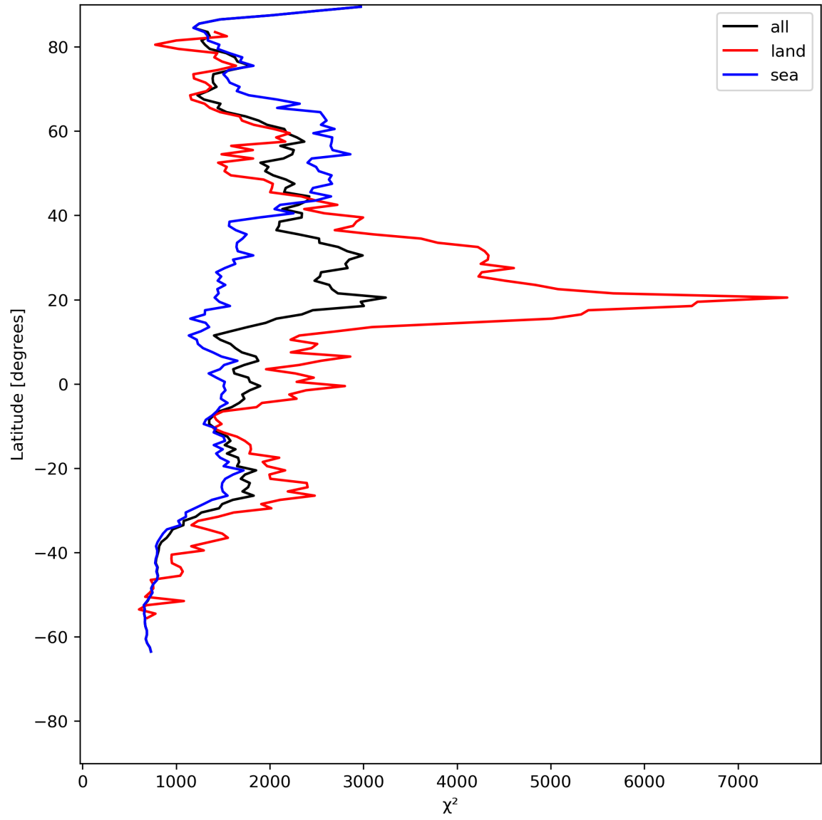
Figure 14: Zonal average of “ \chi^2 ” for 2024-07-15 to 2024-07-16.
