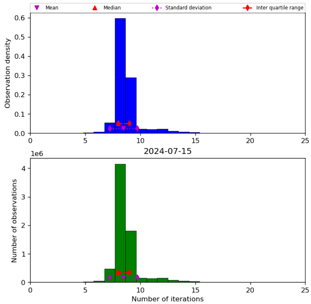
Figure 24: Histogram of “Number of iterations” for 2024-07-15 to 2024-07-16
