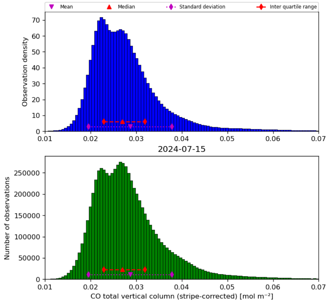
Figure 19: Histogram of “CO total vertical column (stripe-corrected)” for 2024-07-15 to 2024-07-16
