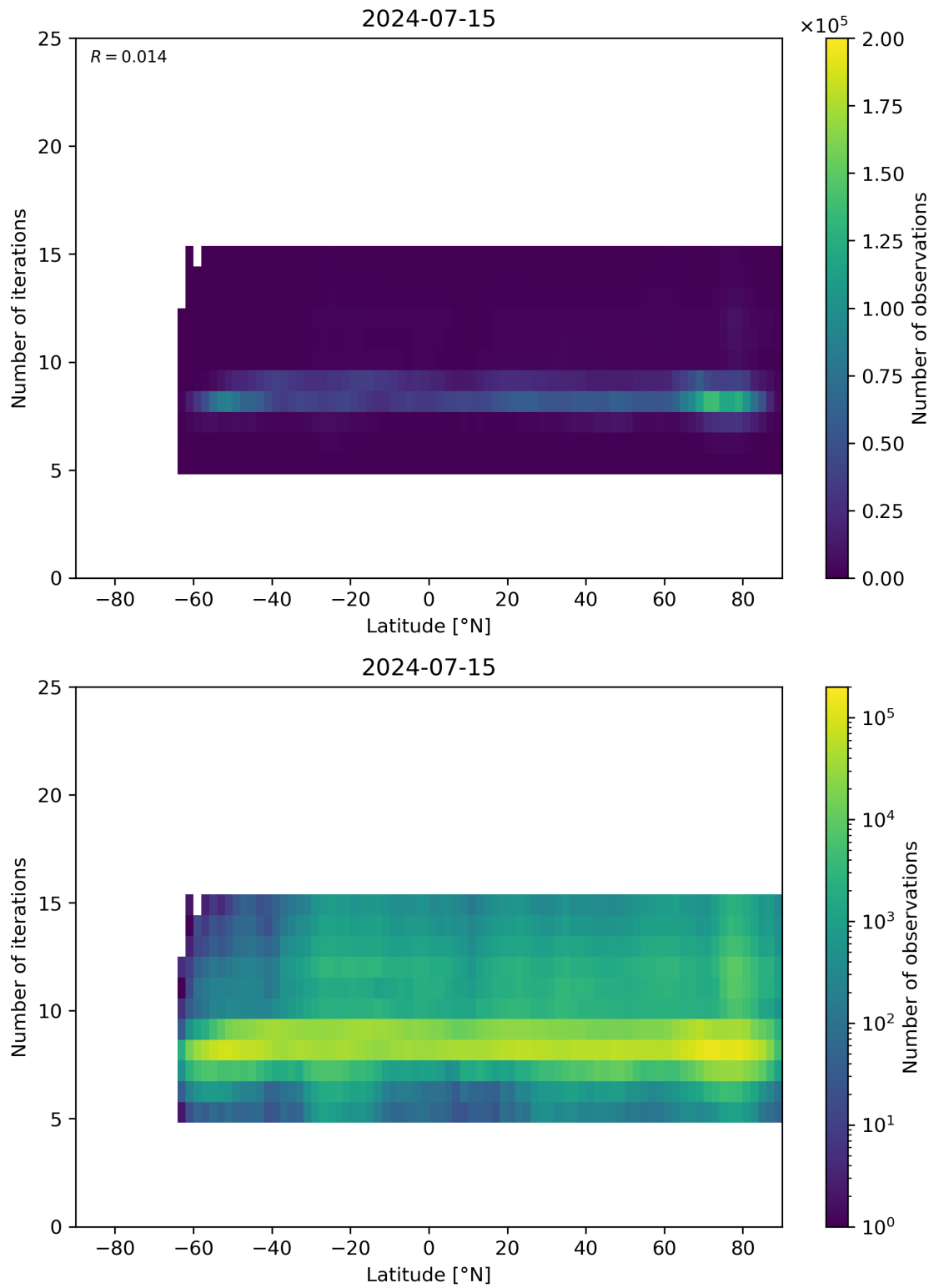
Figure 56: Scatter density plot of “Latitude” against “Number of iterations” for 2024-07-15 to 2024-07-16.
