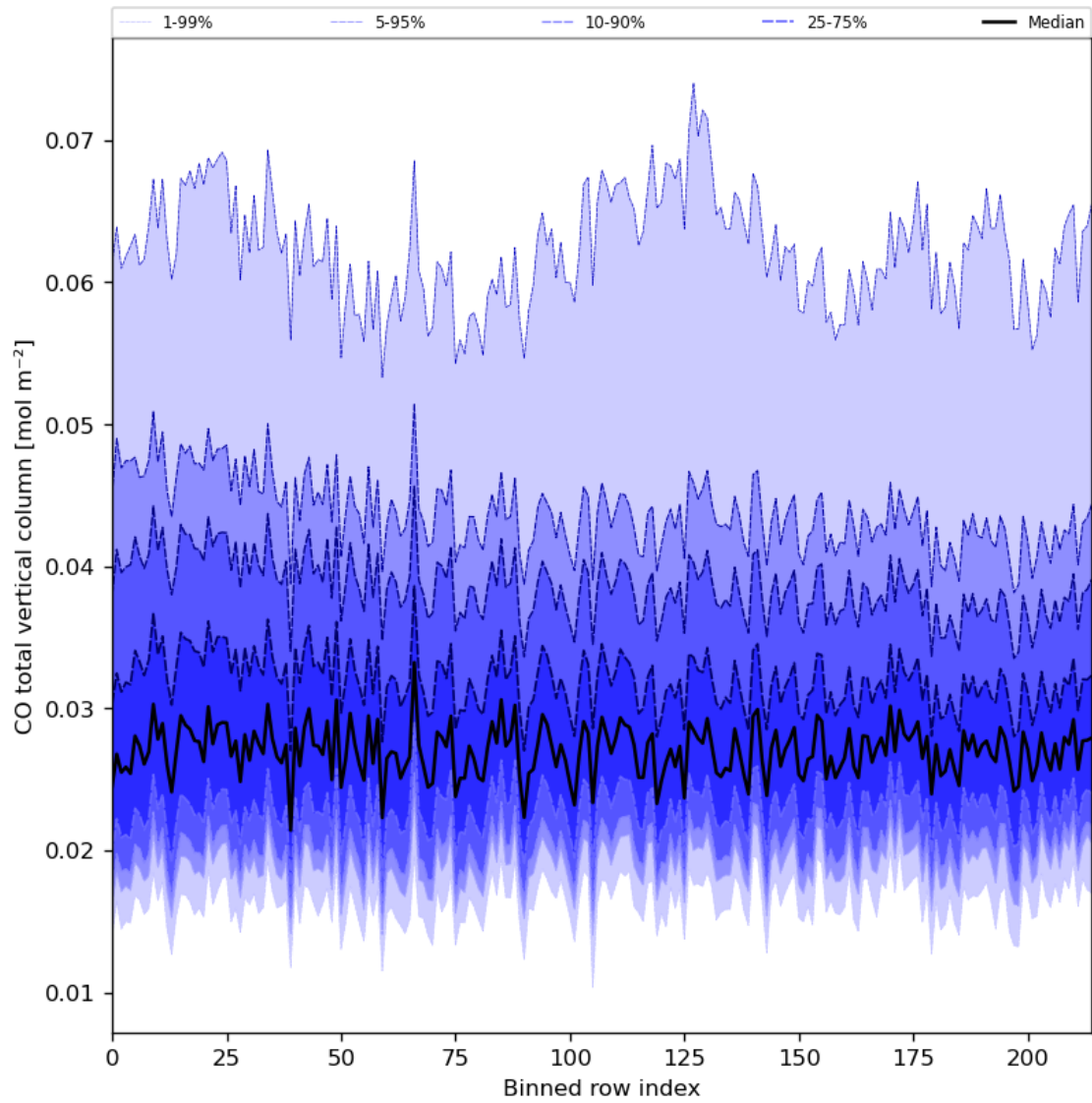
Figure 26: Along track statistics of “CO total vertical column” for 2024-07-15 to 2024-07-16
