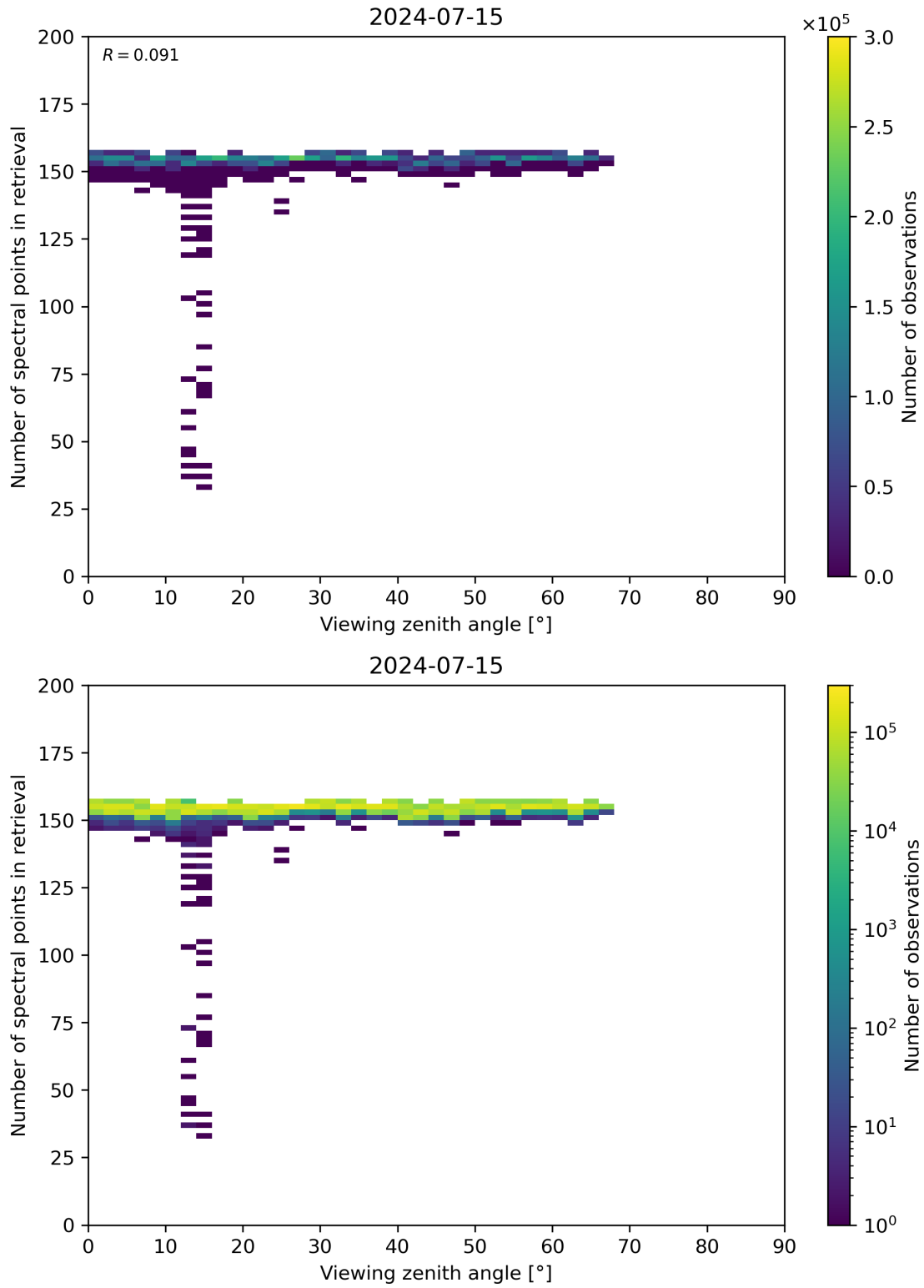
Figure 76: Scatter density plot of “Viewing zenith angle” against “Number of spectral points in retrieval” for 2024-07-15 to 2024-07-16.
