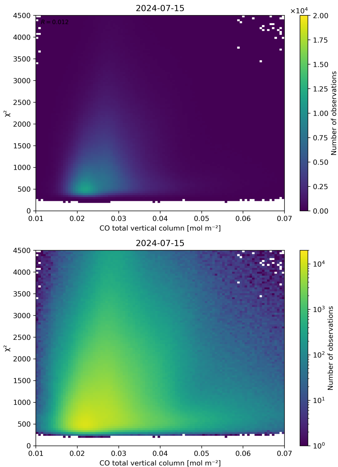
Figure 35: Scatter density plot of “CO total vertical column” against “ \chi^2 ” for 2024-07-15 to 2024-07-16.
