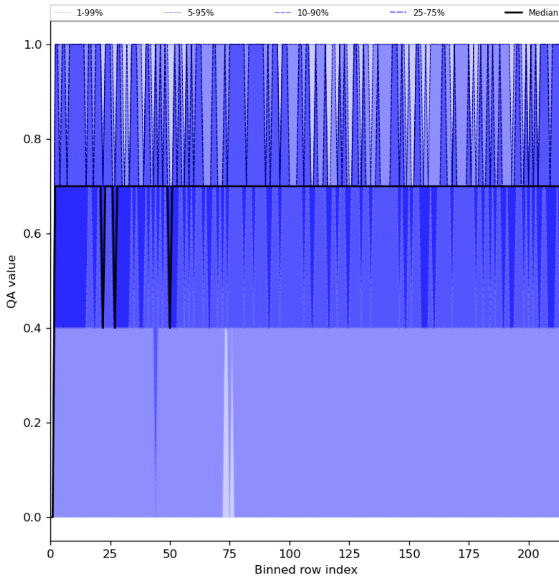
Figure 25: Along track statistics of “QA value” for 2024-07-15 to 2024-07-16
