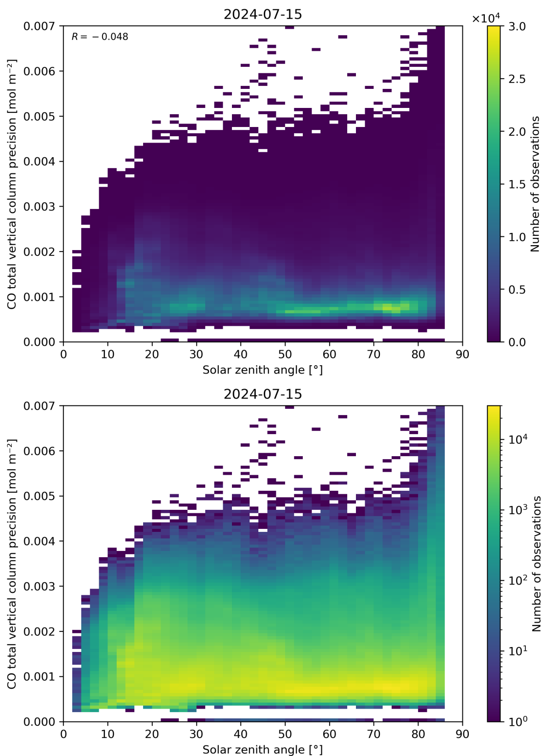
Figure 63: Scatter density plot of “Solar zenith angle” against “CO total vertical column precision” for 2024-07-15 to 2024-07-16.
