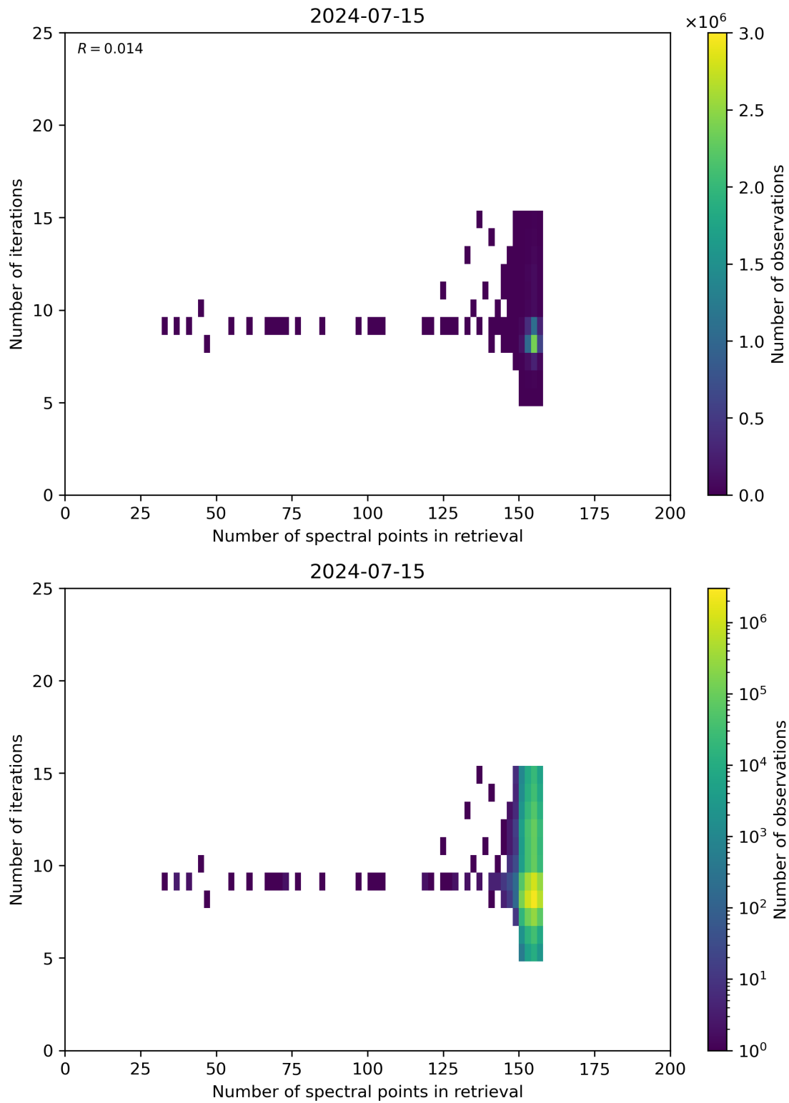
Figure 60: Scatter density plot of “Number of spectral points in retrieval” against “Number of iterations” for 2024-07-15 to 2024-07-16.
