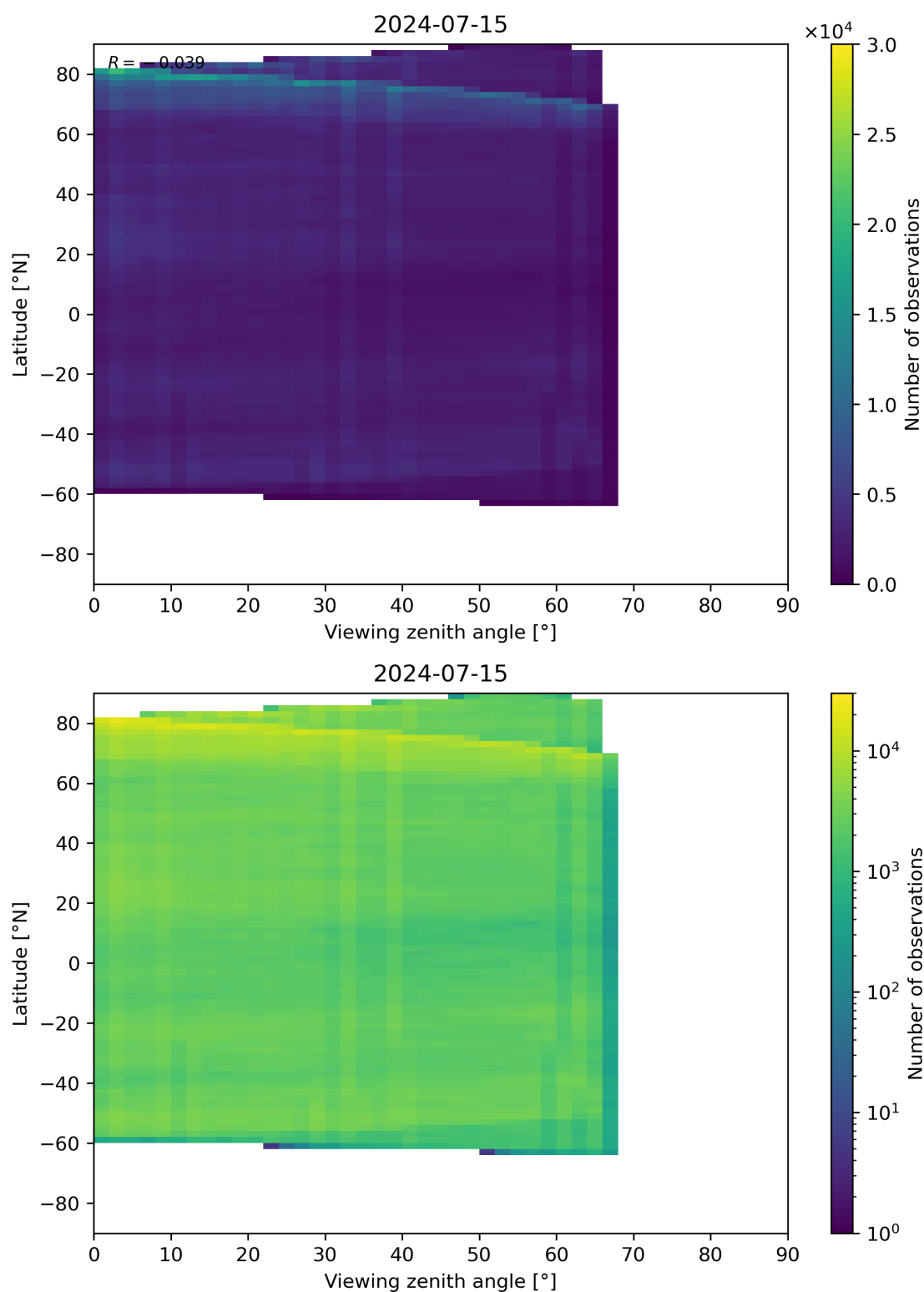
Figure 74: Scatter density plot of “Viewing zenith angle” against “Latitude” for 2024-07-15 to 2024-07-16.
