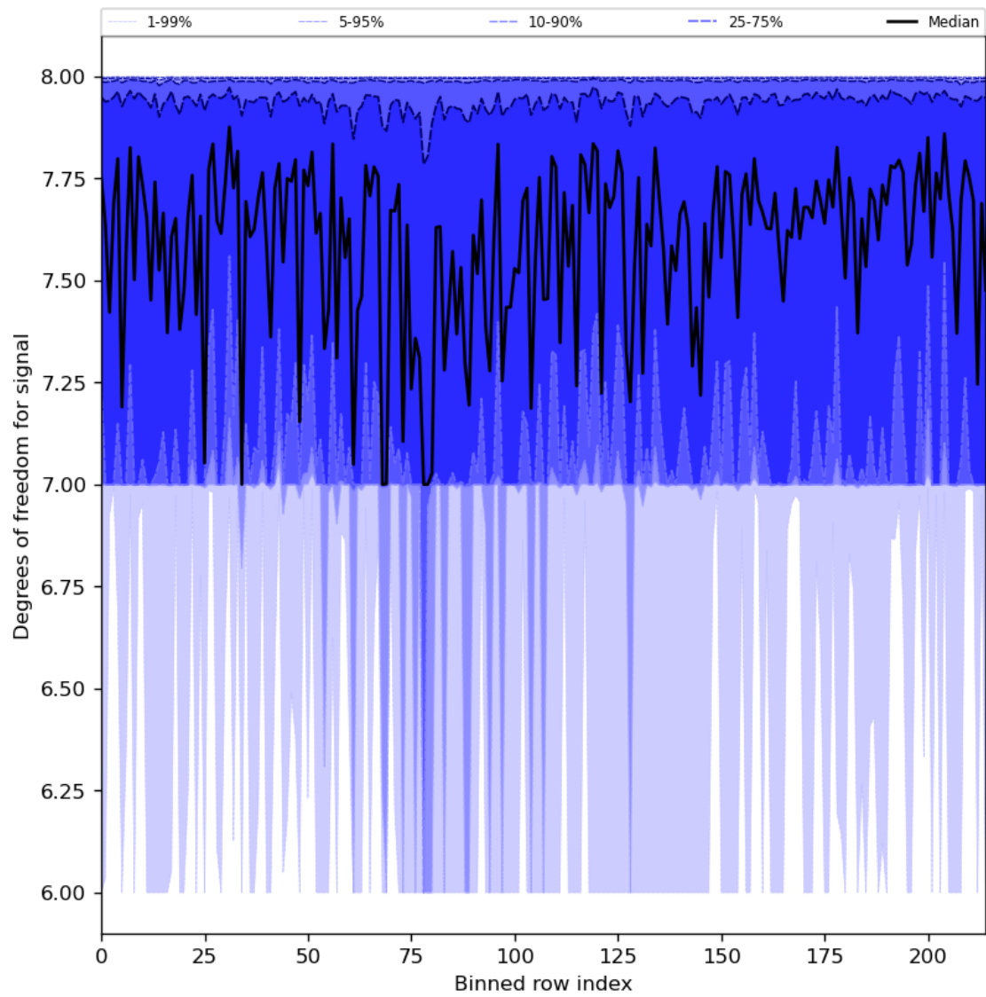
Figure 31: Along track statistics of “Degrees of freedom for signal” for 2024-07-15 to 2024-07-16
