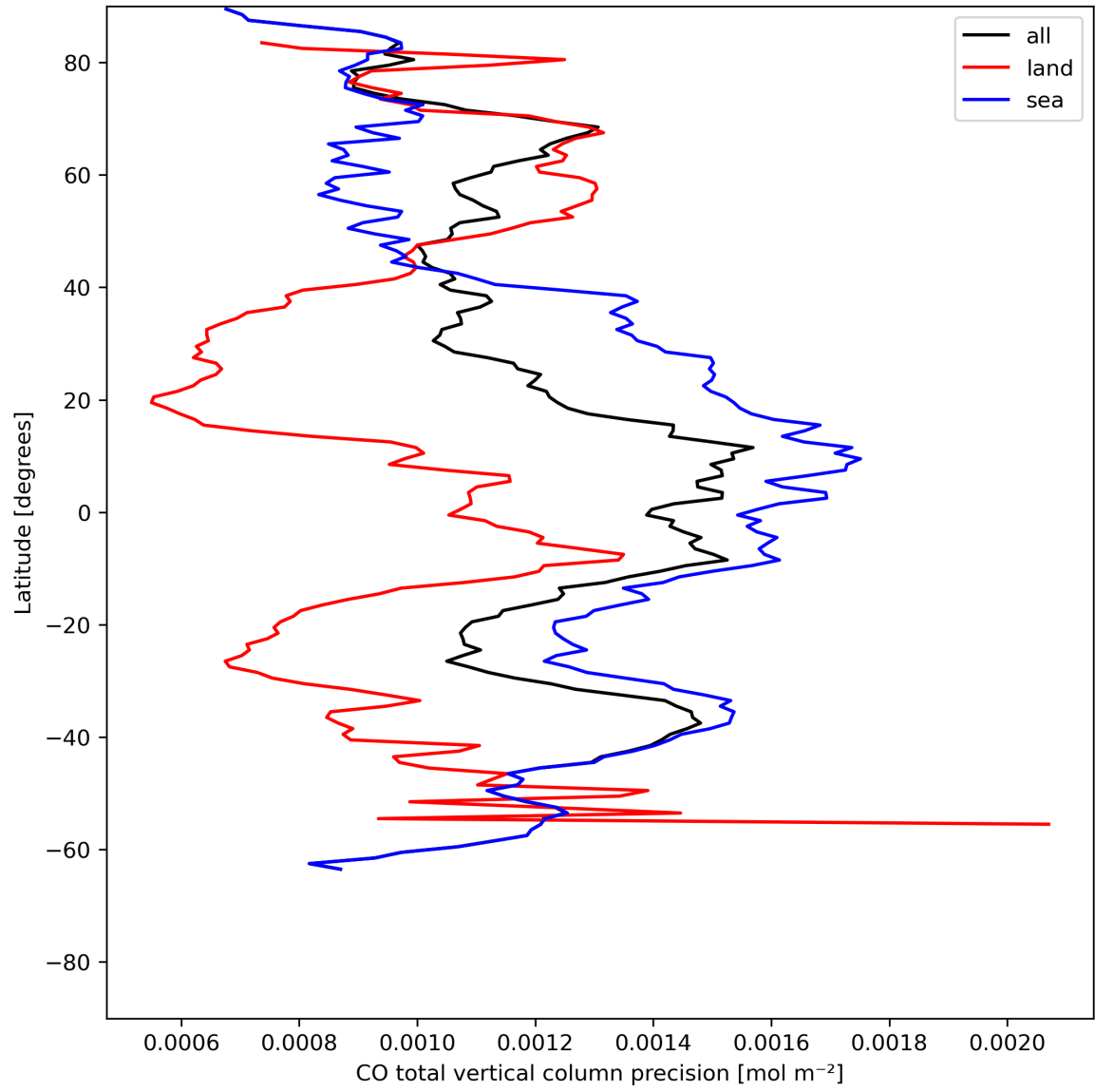
Figure 12: Zonal average of “CO total vertical column precision” for 2024-07-15 to 2024-07-16.
