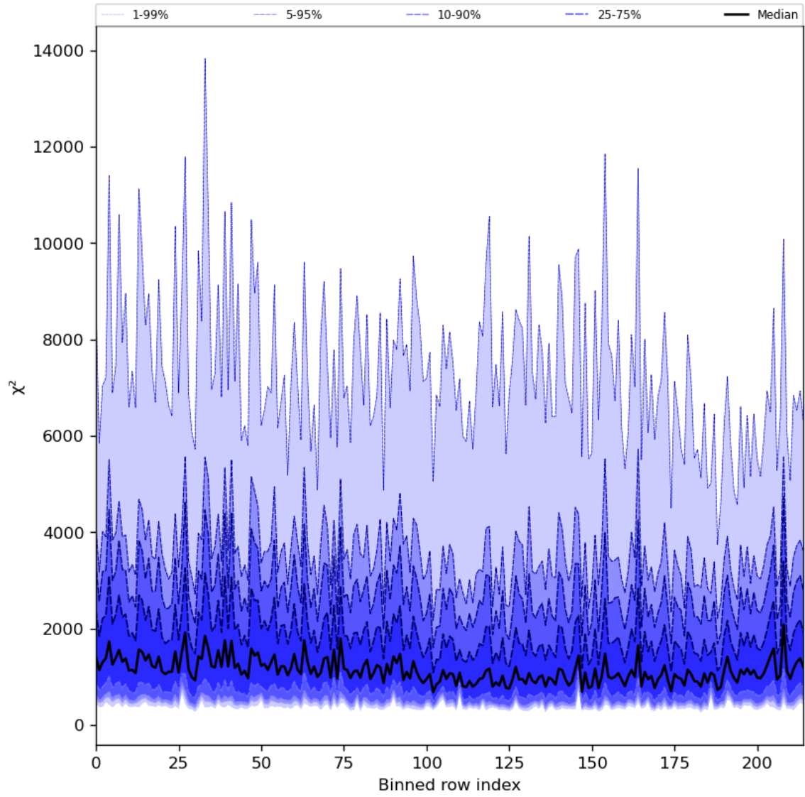
Figure 30: Along track statistics of “ \chi^2 ” for 2024-07-15 to 2024-07-16
