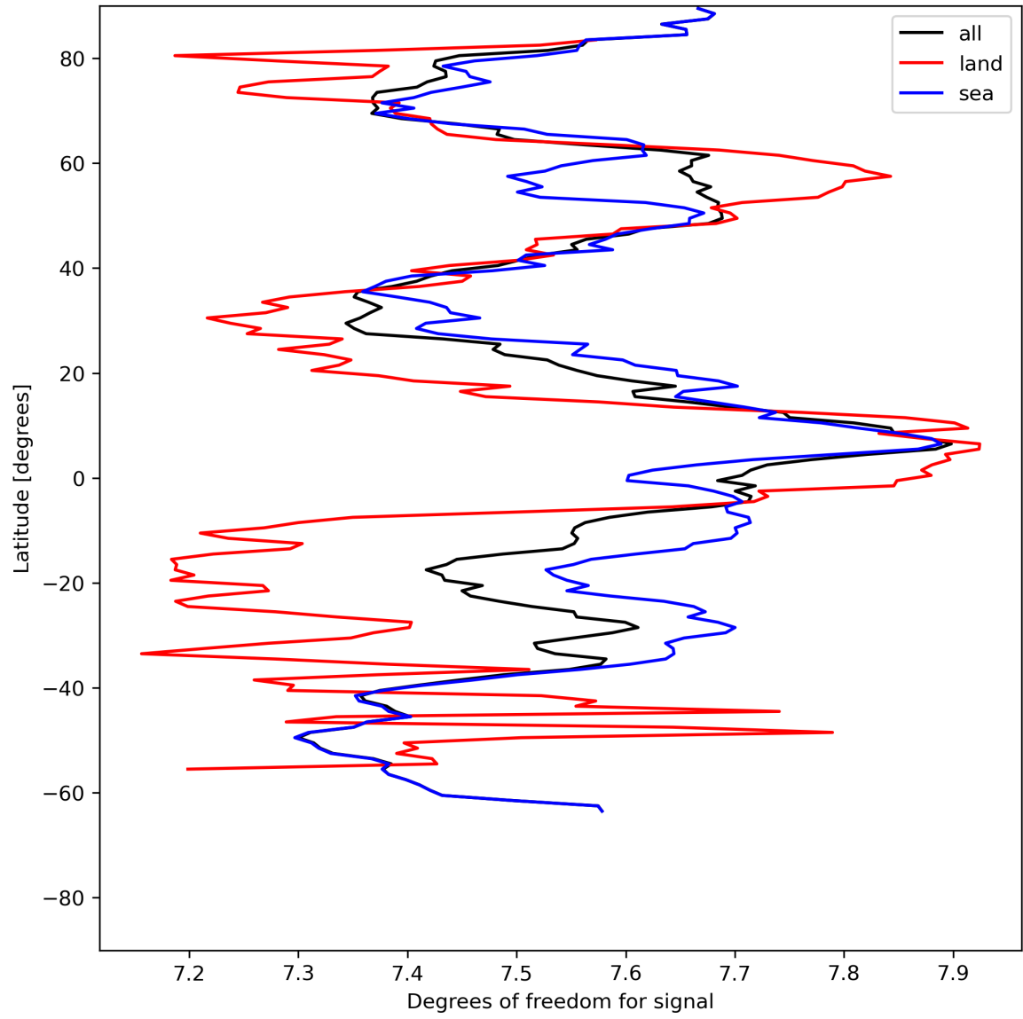
Figure 15: Zonal average of “Degrees of freedom for signal” for 2024-07-15 to 2024-07-16.
