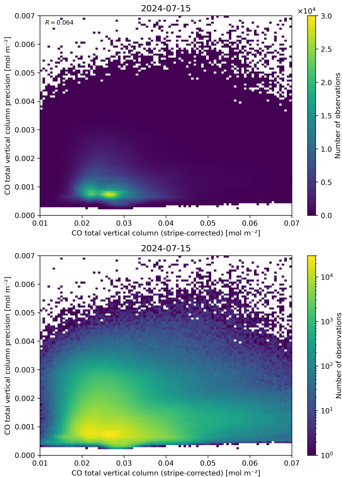
Figure 36: Scatter density plot of “CO total vertical column (stripe-corrected)” against “CO total vertical column precision” for 2024-07-15 to 2024-07-16.
