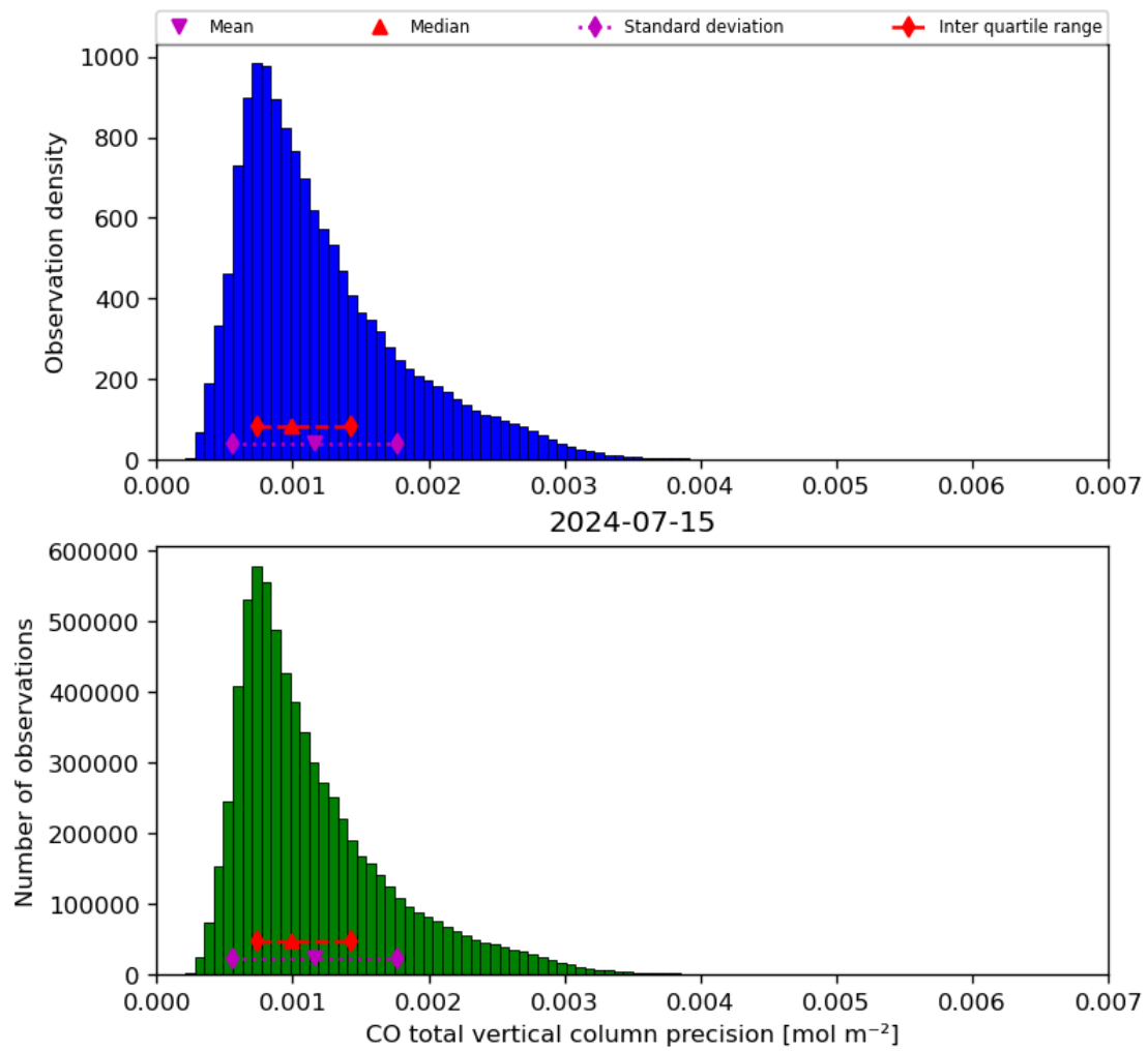
Figure 20: Histogram of “CO total vertical column precision” for 2024-07-15 to 2024-07-16
