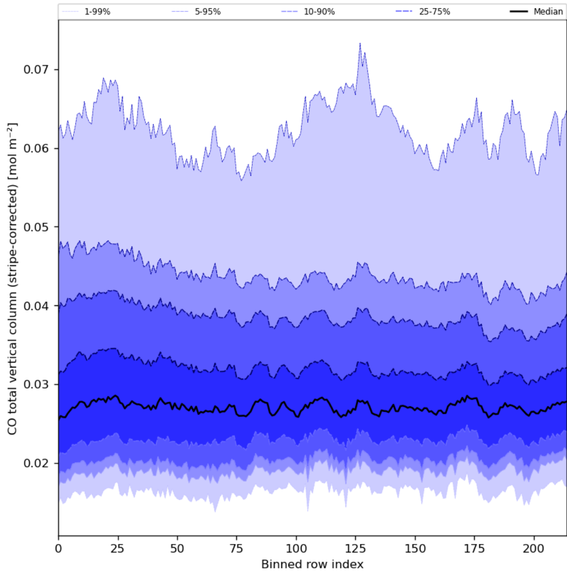
Figure 27: Along track statistics of “CO total vertical column (stripe-corrected)” for 2024-07-15 to 2024-07-16
