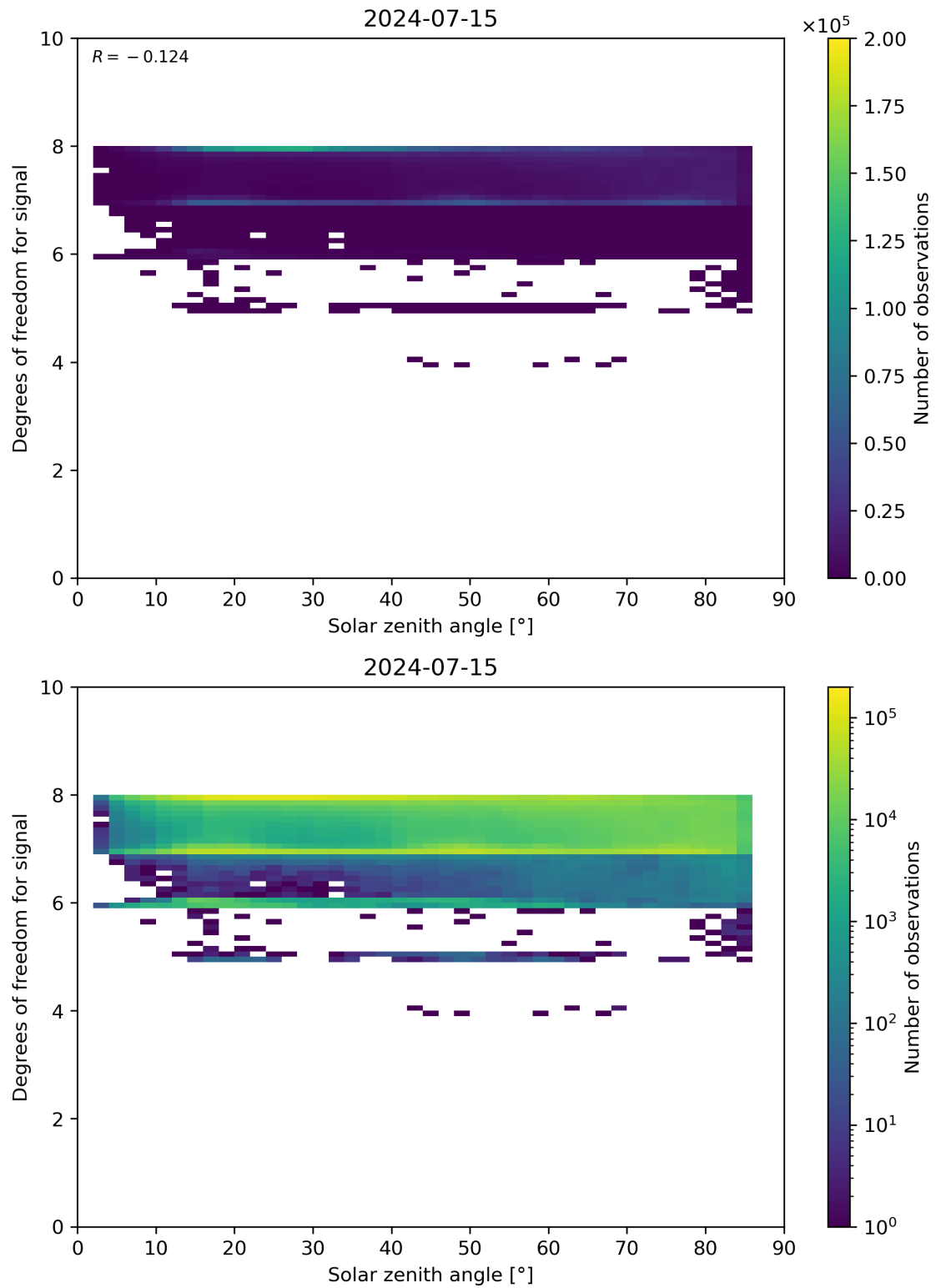
Figure 65: Scatter density plot of “Solar zenith angle” against “Degrees of freedom for signal” for 2024-07-15 to 2024-07-16.
