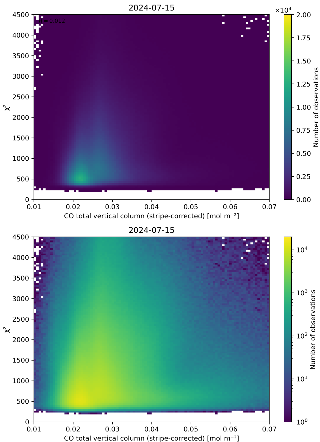
Figure 37: Scatter density plot of “CO total vertical column (stripe-corrected)” against “ \chi^2 ” for 2024-07-15 to 2024-07-16.
