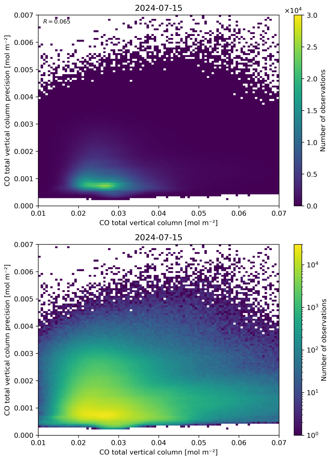
Figure 34: Scatter density plot of “CO total vertical column” against “CO total vertical column precision” for 2024-07-15 to 2024-07-16.
