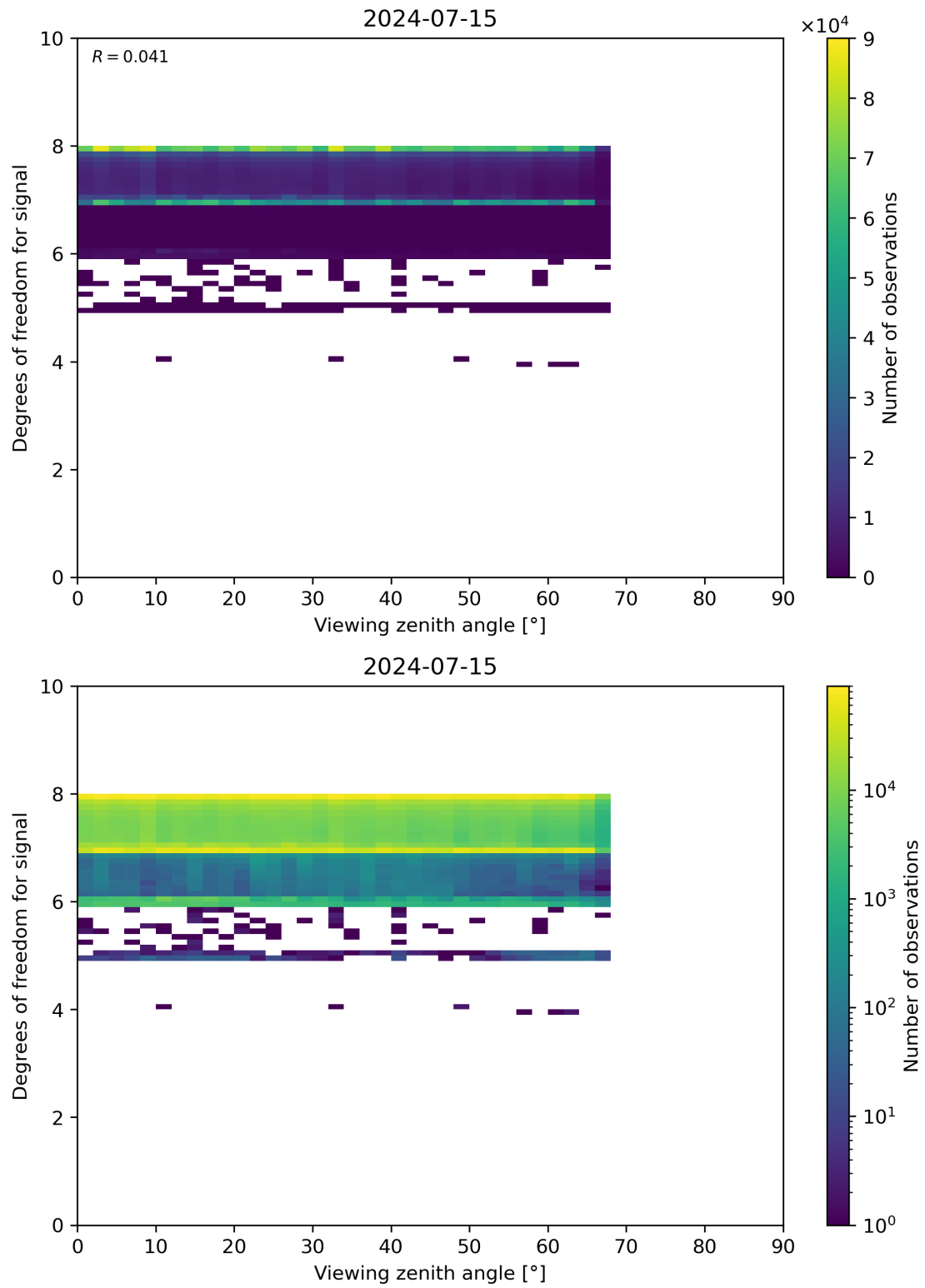
Figure 73: Scatter density plot of “Viewing zenith angle” against “Degrees of freedom for signal” for 2024-07-15 to 2024-07-16.
