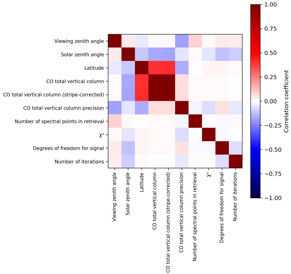
Figure 2: Map of correlation matrix for 2024-07-15 to 2024-07-16.
