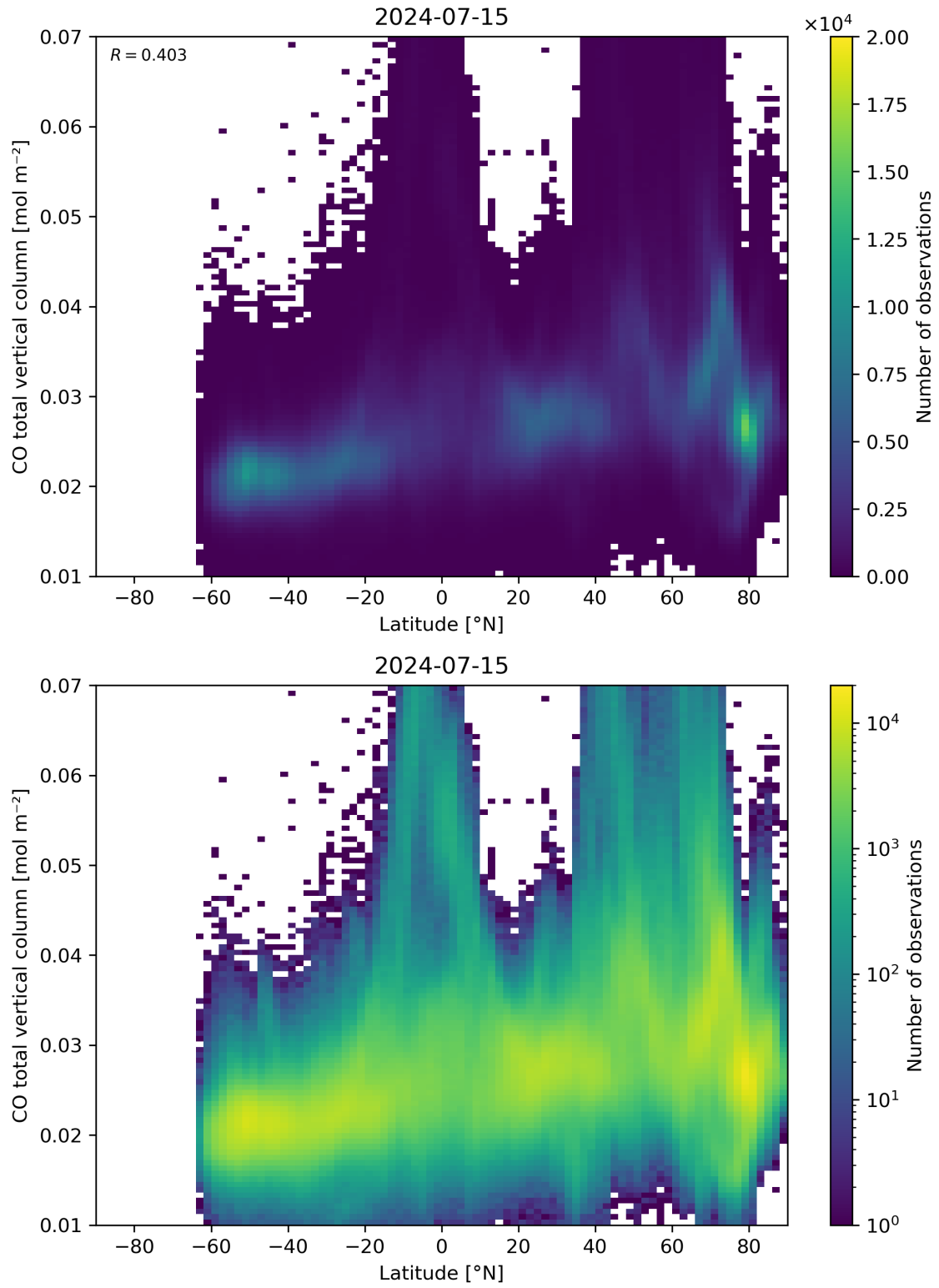
Figure 51: Scatter density plot of “Latitude” against “CO total vertical column” for 2024-07-15 to 2024-07-16.
