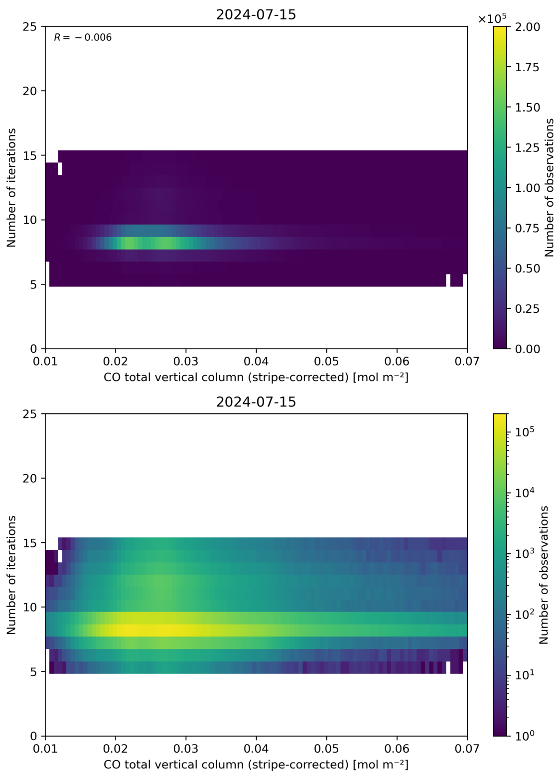
Figure 39: Scatter density plot of “CO total vertical column (stripe-corrected)” against “Number of iterations” for 2024-07-15 to 2024-07-16.
