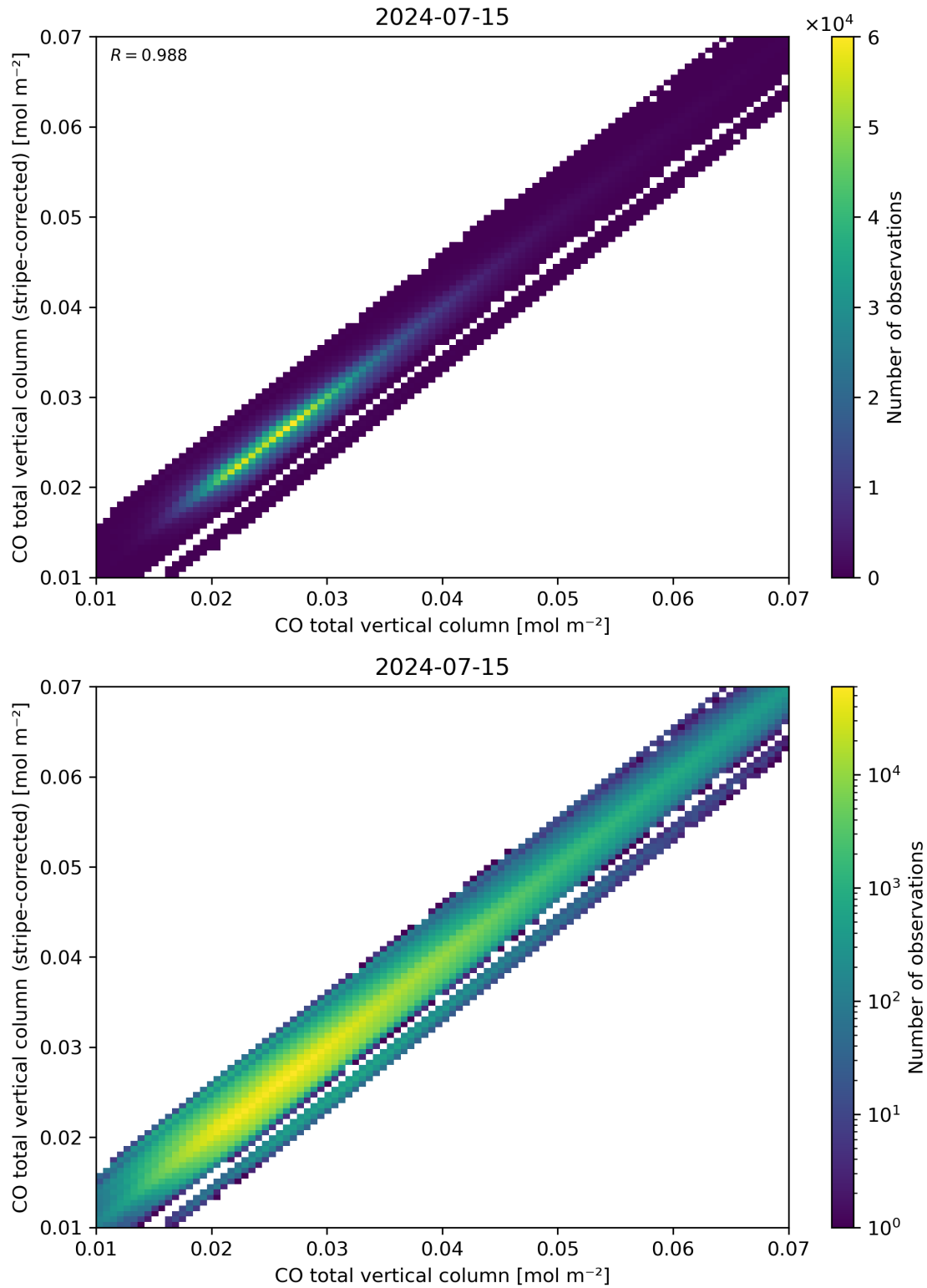
Figure 33: Scatter density plot of “CO total vertical column” against “CO total vertical column (stripe-corrected)” for 2024-07-15 to 2024-07-16.
