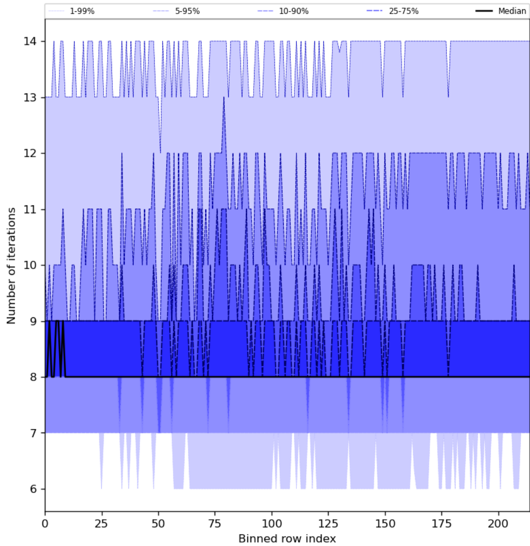
Figure 32: Along track statistics of “Number of iterations” for 2024-07-15 to 2024-07-16
