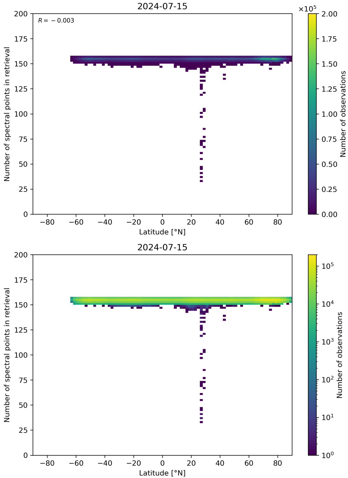
Figure 57: Scatter density plot of “Latitude” against “Number of spectral points in retrieval” for 2024-07-15 to 2024-07-16.
