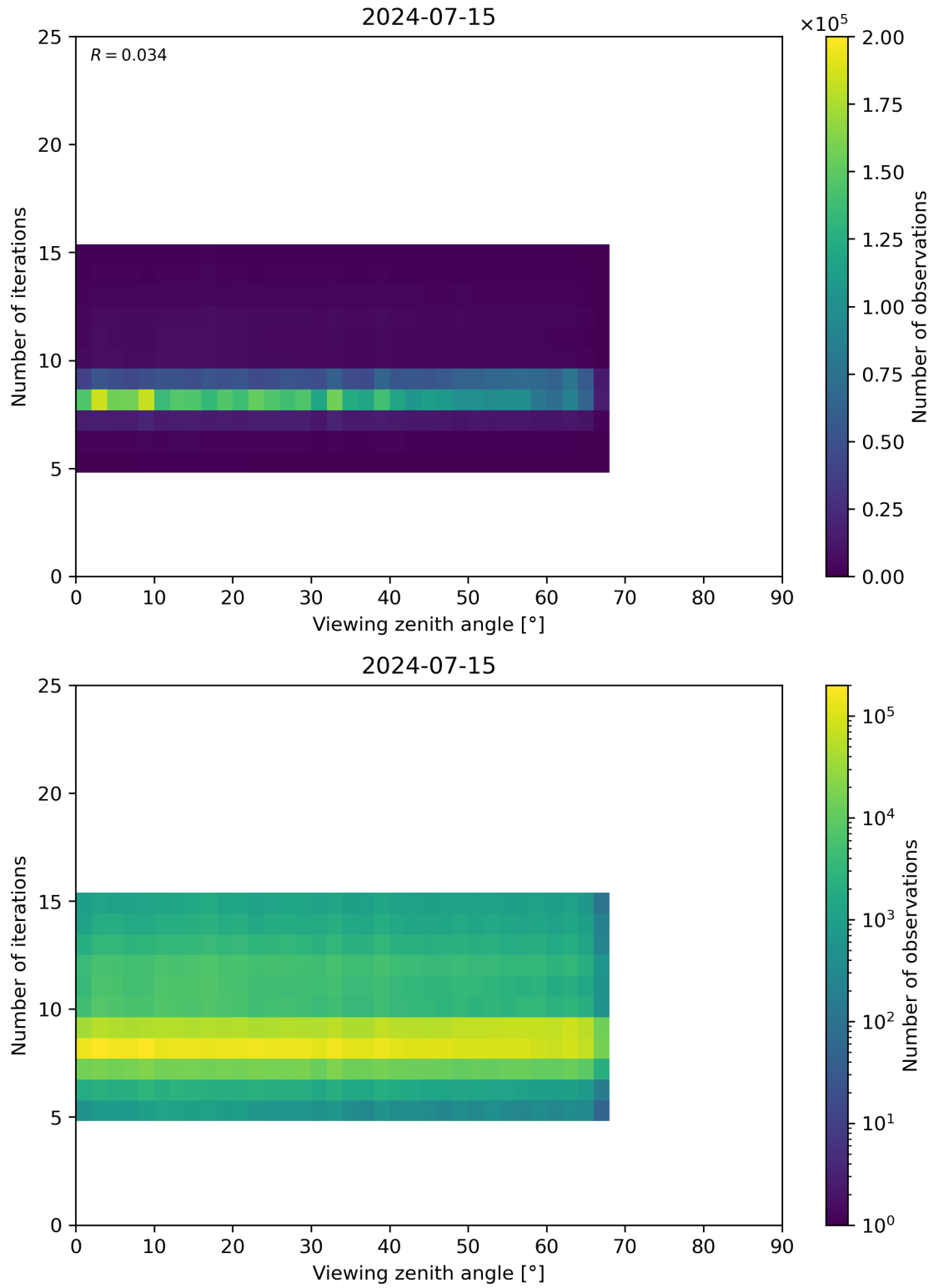
Figure 75: Scatter density plot of “Viewing zenith angle” against “Number of iterations” for 2024-07-15 to 2024-07-16.
