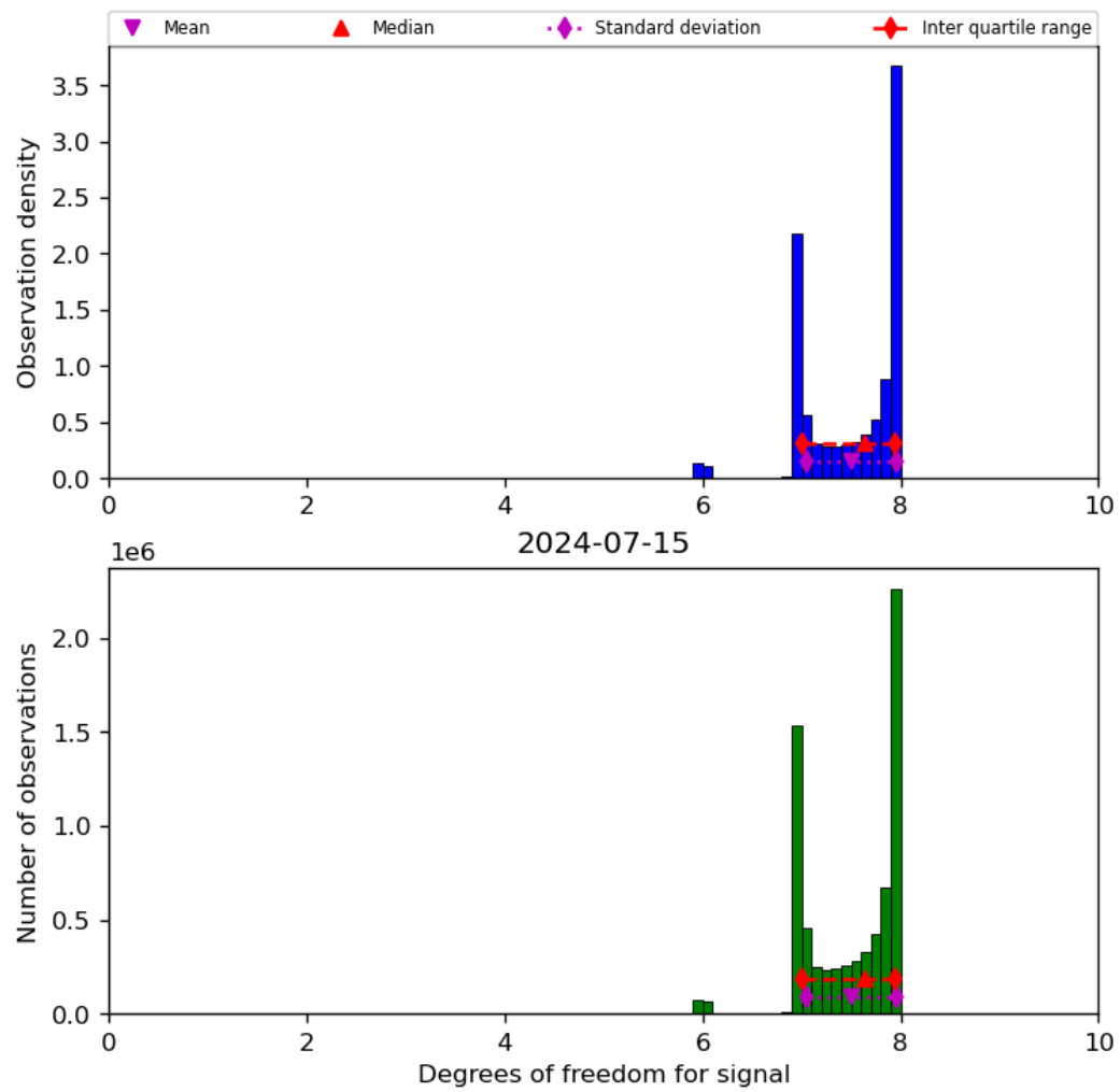
Figure 23: Histogram of “Degrees of freedom for signal” for 2024-07-15 to 2024-07-16
