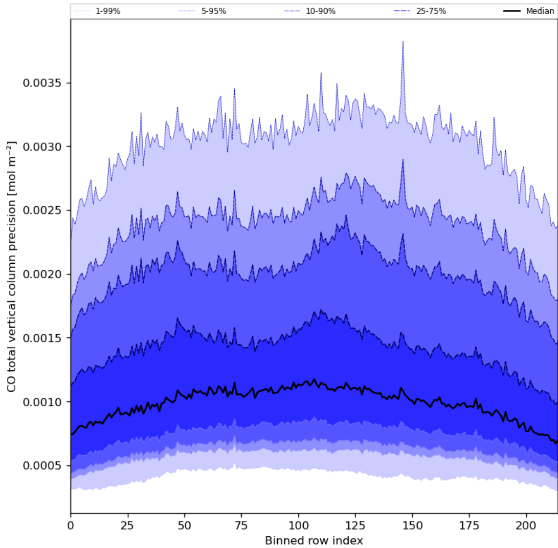
Figure 28: Along track statistics of “CO total vertical column precision” for 2024-07-15 to 2024-07-16
