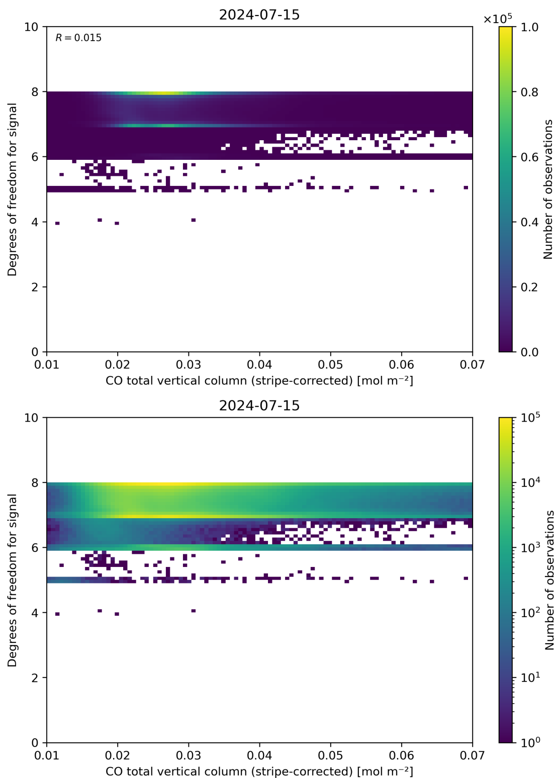
Figure 38: Scatter density plot of “CO total vertical column (stripe-corrected)” against “Degrees of freedom for signal” for 2024-07-15 to 2024-07-16.
