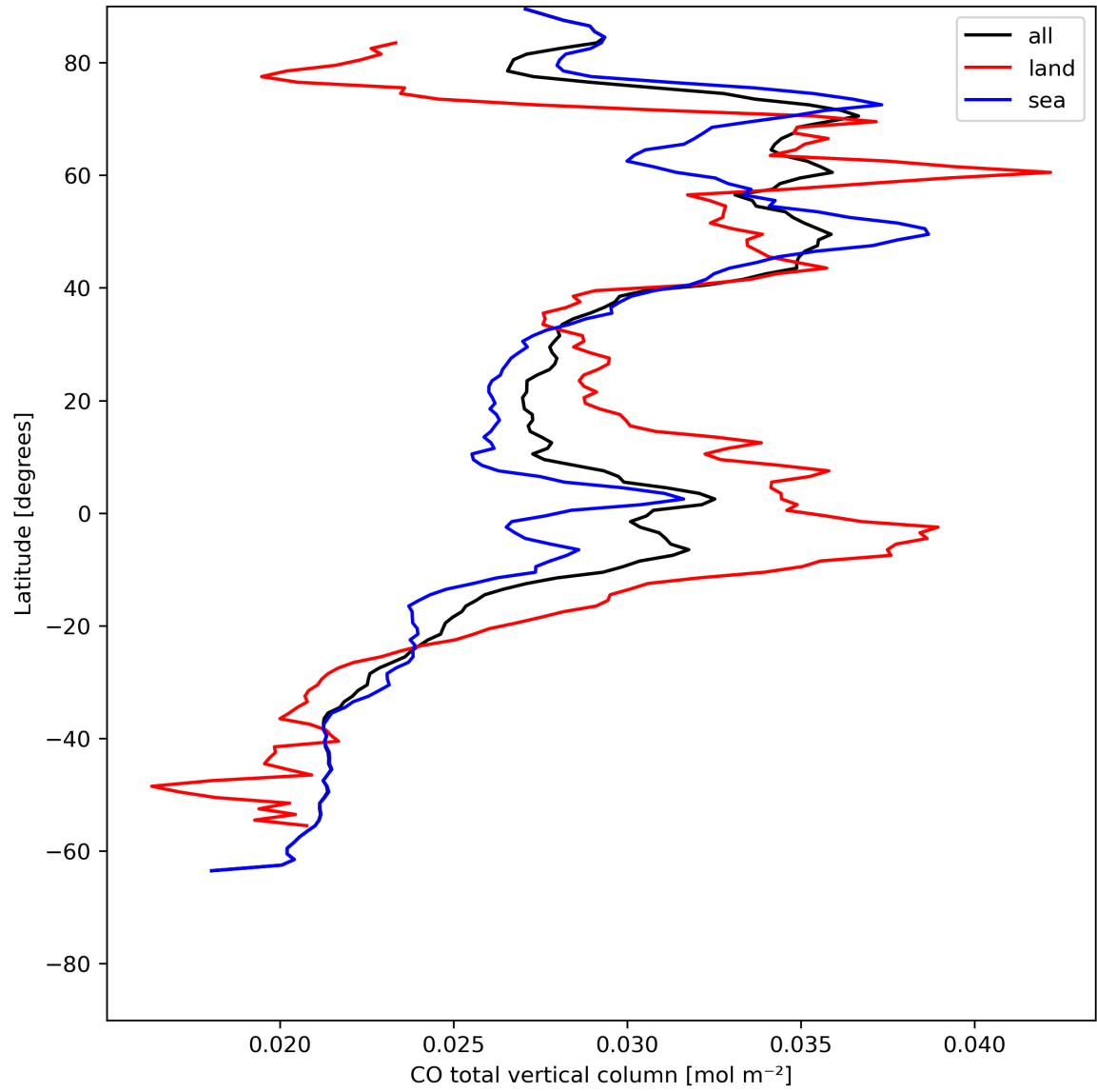
Figure 10: Zonal average of “CO total vertical column” for 2024-07-15 to 2024-07-16.
