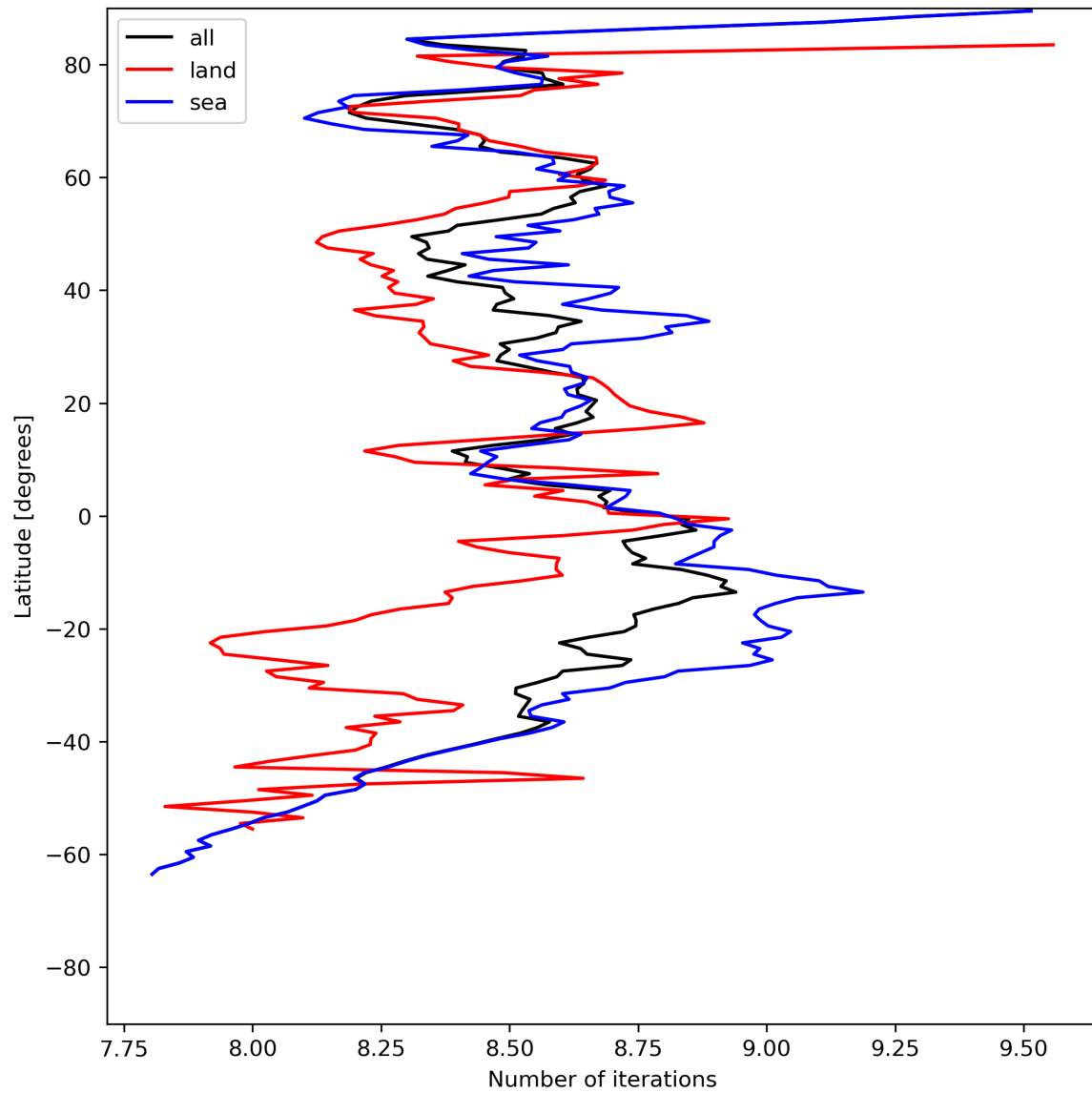
Figure 16: Zonal average of “Number of iterations” for 2024-07-15 to 2024-07-16.
