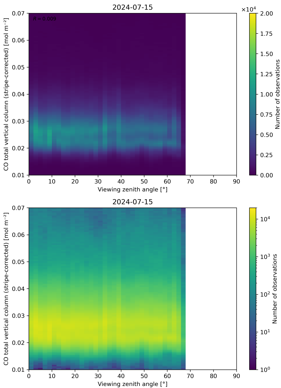
Figure 70: Scatter density plot of “Viewing zenith angle” against “CO total vertical column (stripe-corrected)” for 2024-07-15 to 2024-07-16.
