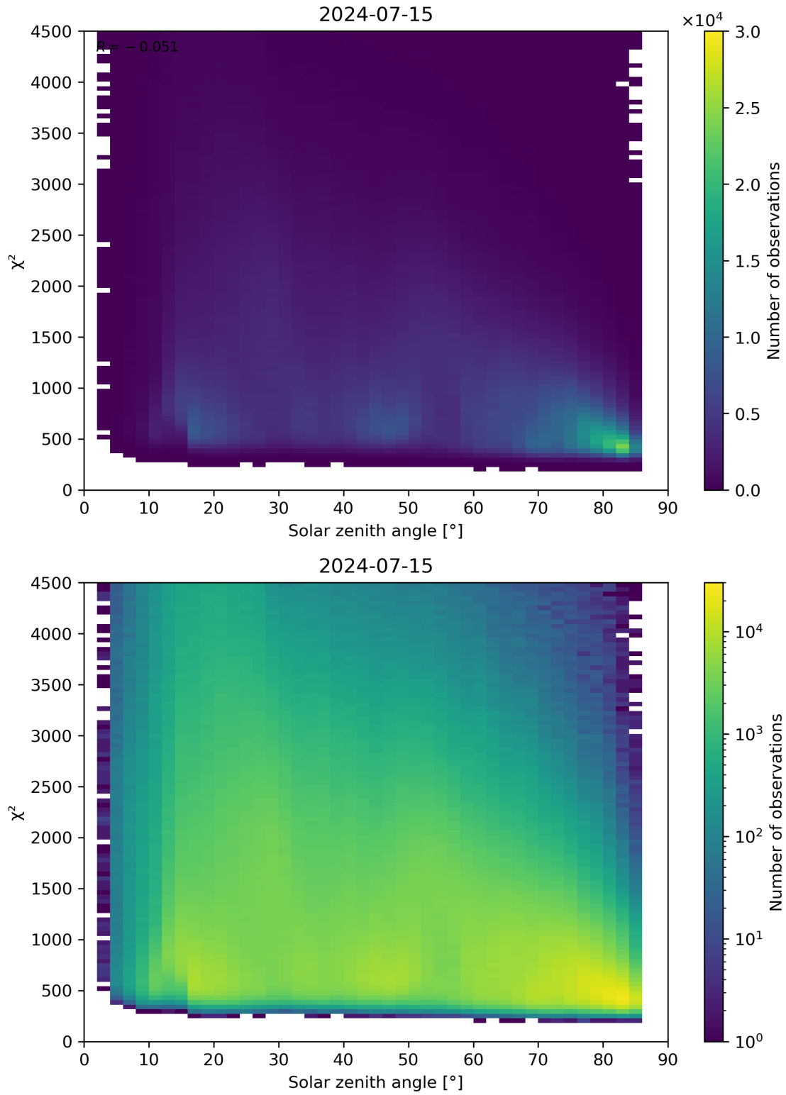
Figure 64: Scatter density plot of “Solar zenith angle” against “ \chi^2 ” for 2024-07-15 to 2024-07-16.
