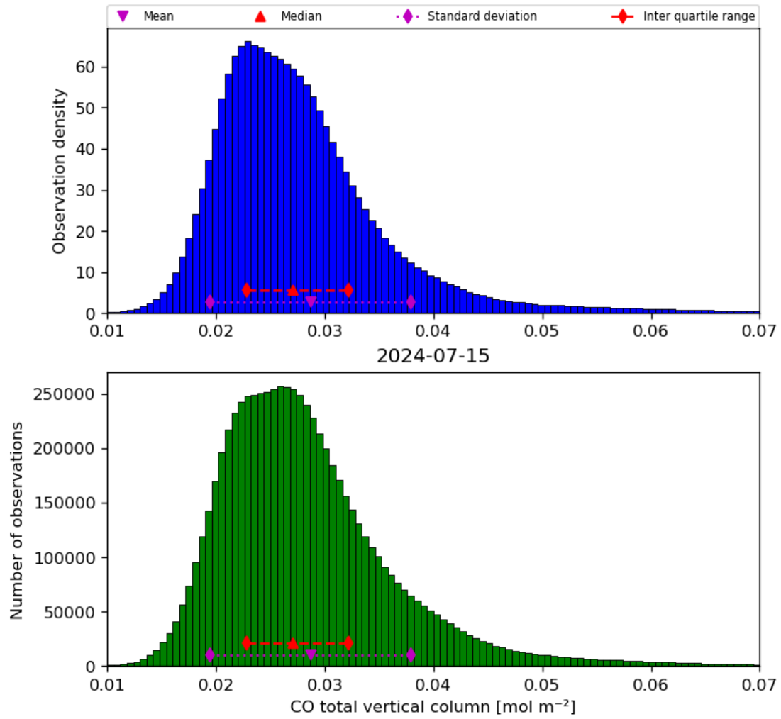
Figure 18: Histogram of “CO total vertical column” for 2024-07-15 to 2024-07-16
