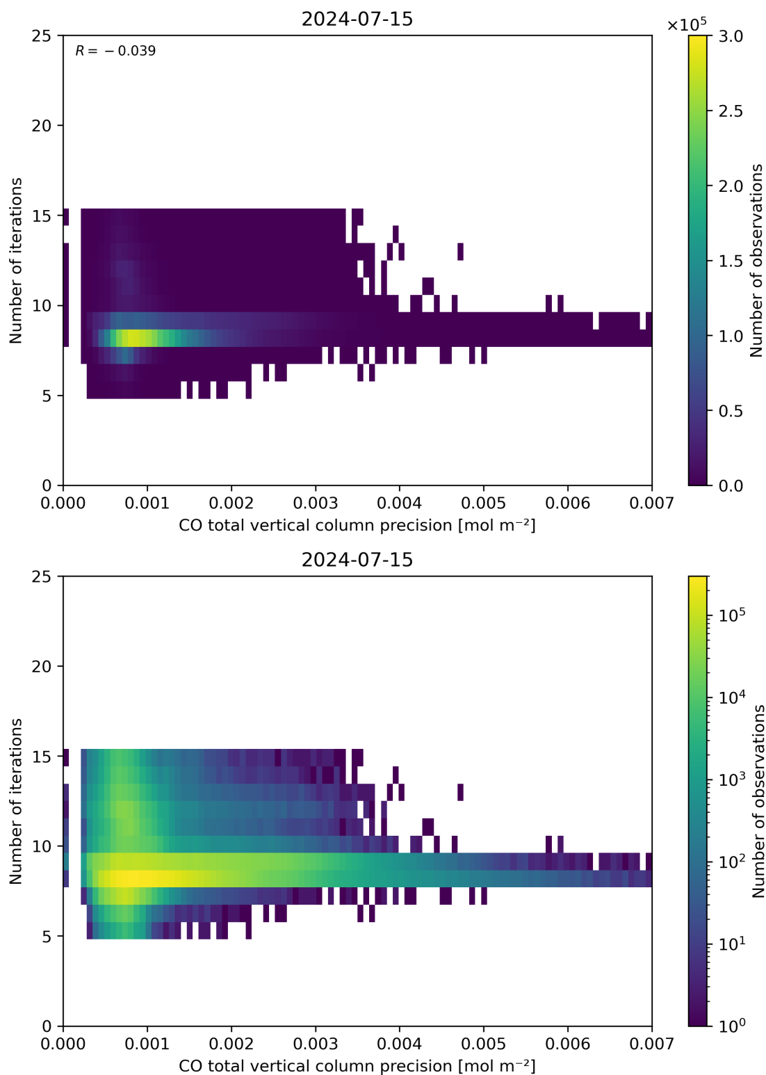
Figure 46: Scatter density plot of “CO total vertical column precision” against “Number of iterations” for 2024-07-15 to 2024-07-16.
