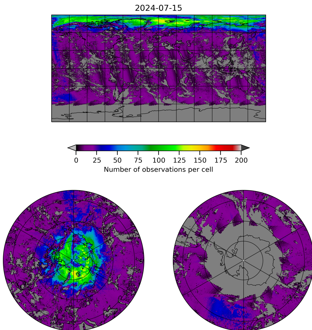
Figure 8: Map of the number of observations for 2024-07-15 to 2024-07-16
