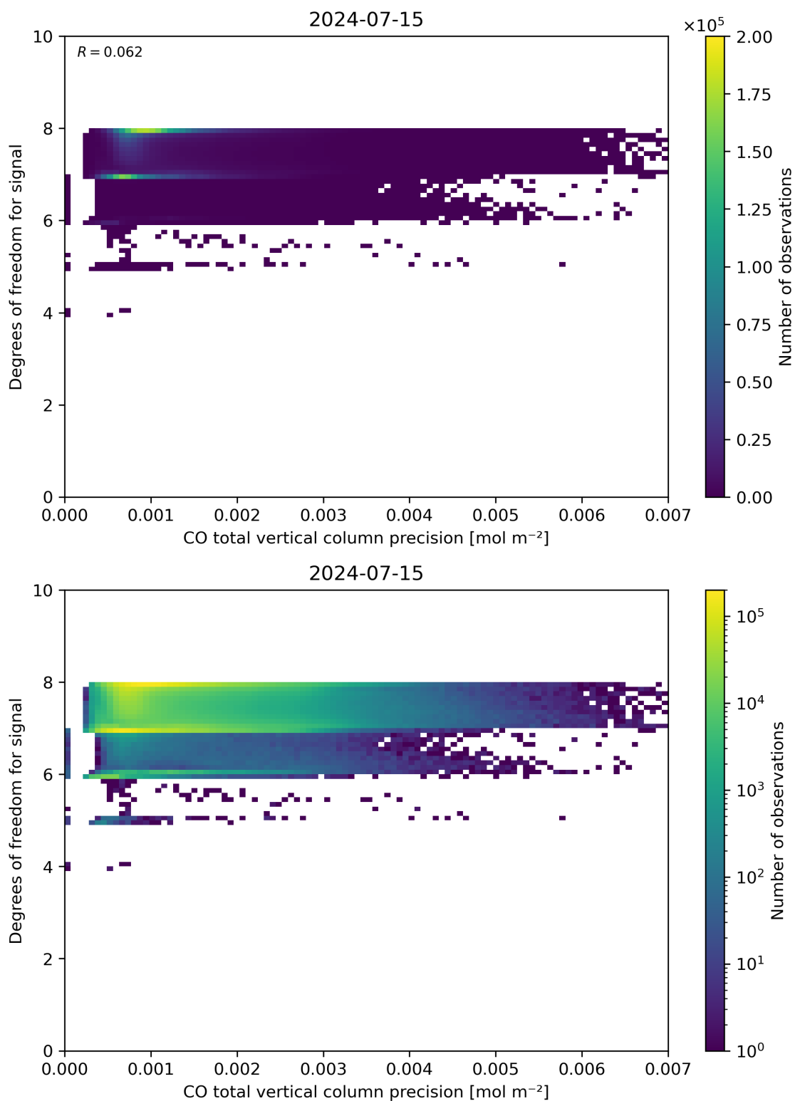
Figure 45: Scatter density plot of “CO total vertical column precision” against “Degrees of freedom for signal” for 2024-07-15 to 2024-07-16.
