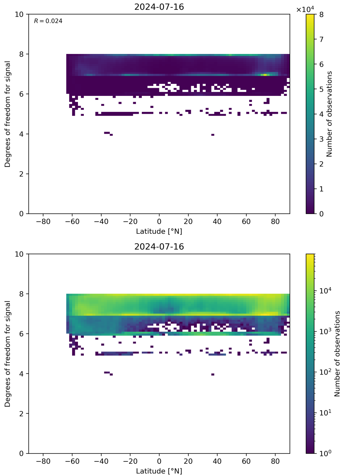
Figure 55: Scatter density plot of “Latitude” against “Degrees of freedom for signal” for 2024-07-15 to 2024-07-17.
