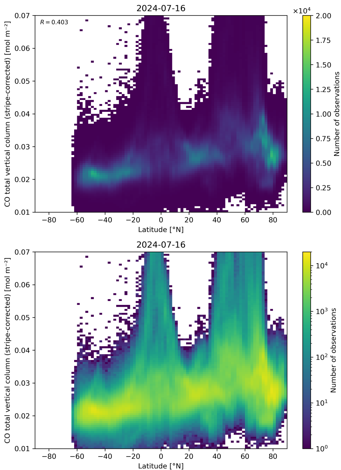
Figure 52: Scatter density plot of “Latitude” against “CO total vertical column (stripe-corrected)” for 2024-07-15 to 2024-07-17.
