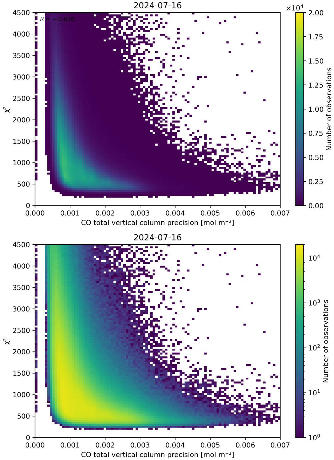
Figure 44: Scatter density plot of “CO total vertical column precision” against “ \chi^2 ” for 2024-07-15 to 2024-07-17.
