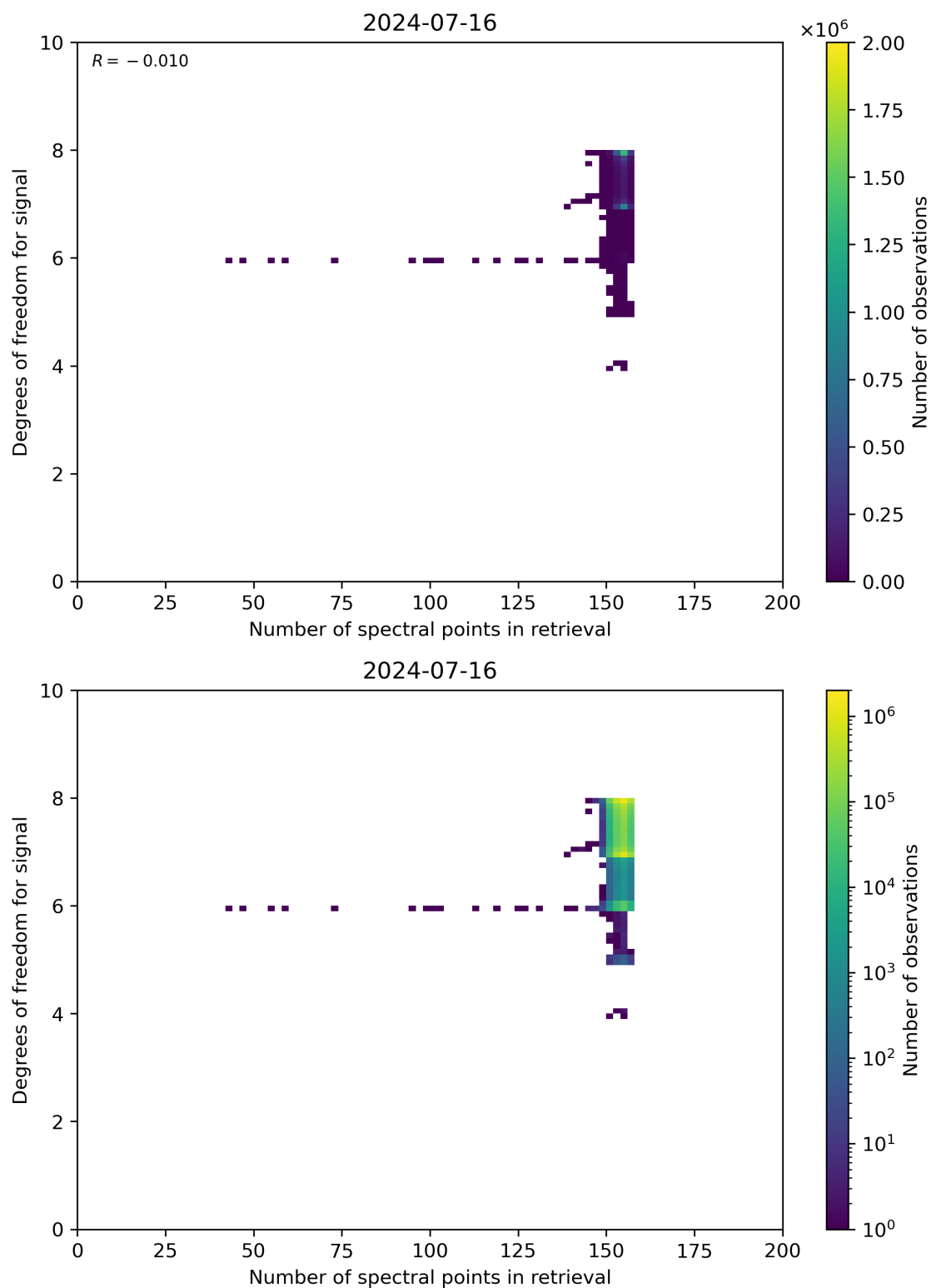
Figure 59: Scatter density plot of “Number of spectral points in retrieval” against “Degrees of freedom for signal” for 2024-07-15 to 2024-07-17.
