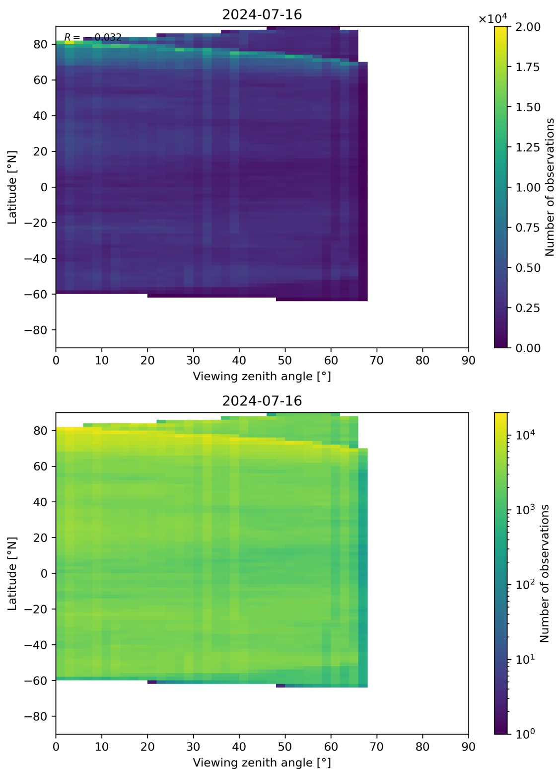
Figure 74: Scatter density plot of “Viewing zenith angle” against “Latitude” for 2024-07-15 to 2024-07-17.
