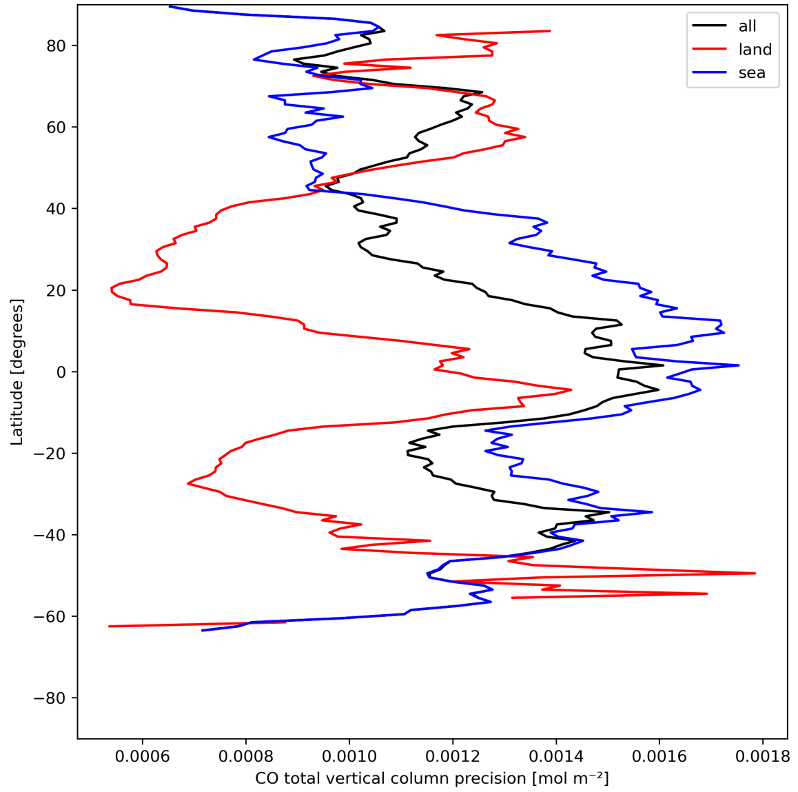
Figure 12: Zonal average of “CO total vertical column precision” for 2024-07-15 to 2024-07-17.
