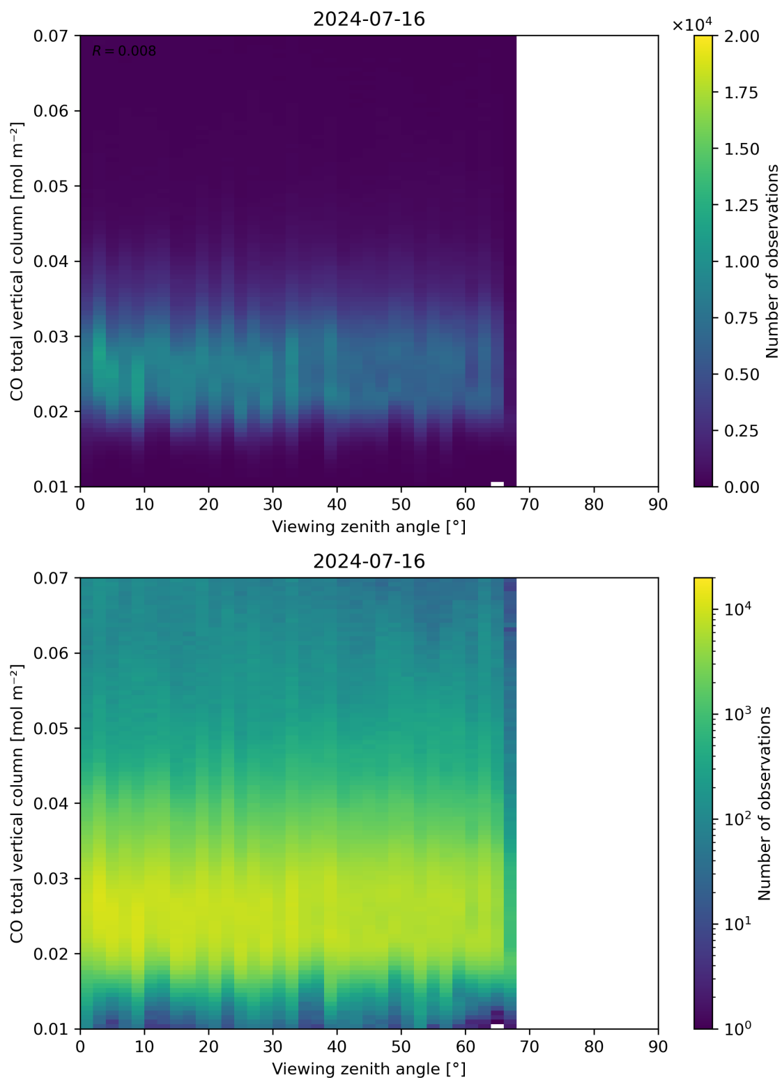
Figure 69: Scatter density plot of “Viewing zenith angle” against “CO total vertical column” for 2024-07-15 to 2024-07-17.
