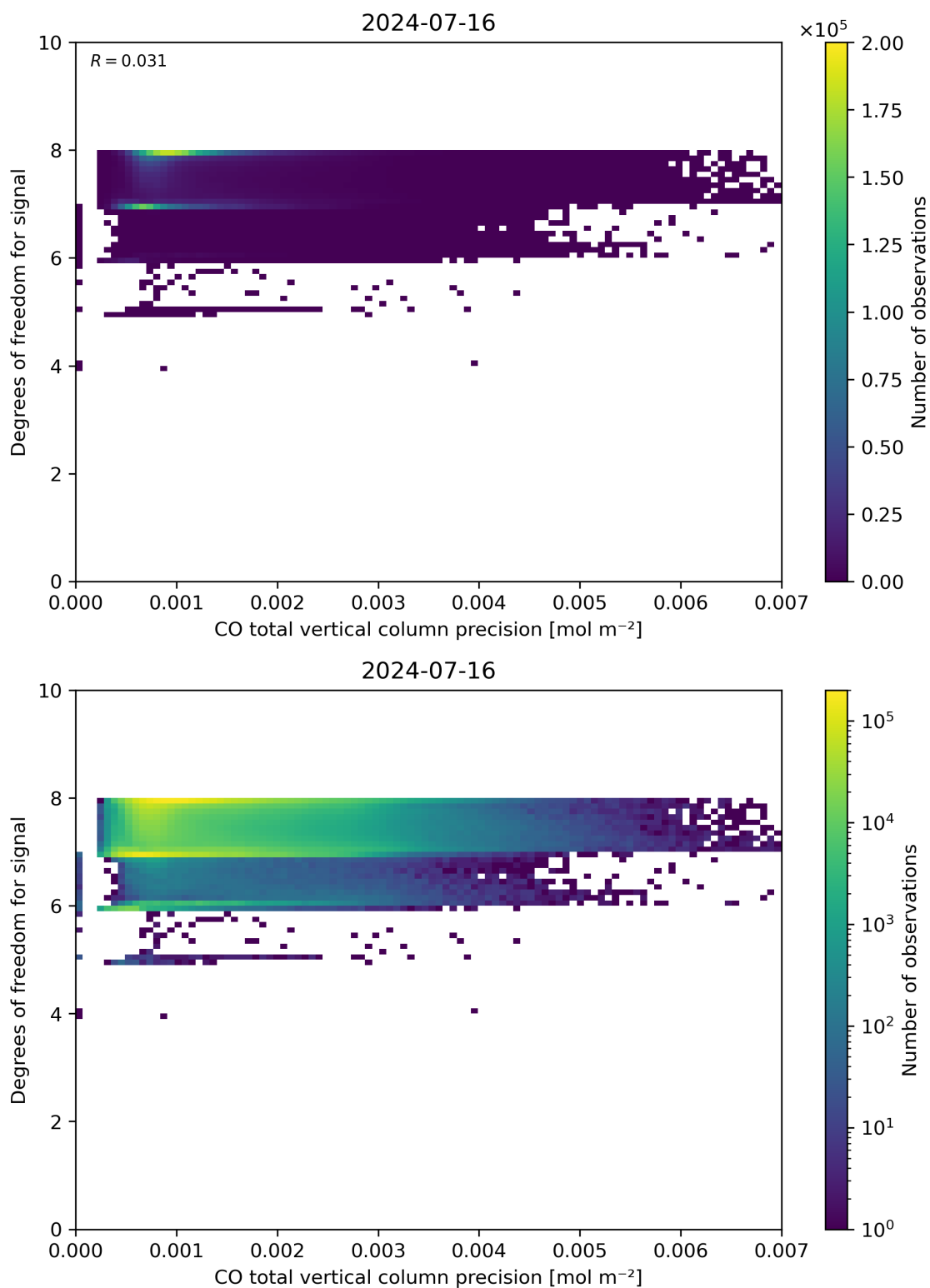
Figure 45: Scatter density plot of “CO total vertical column precision” against “Degrees of freedom for signal” for 2024-07-15 to 2024-07-17.
