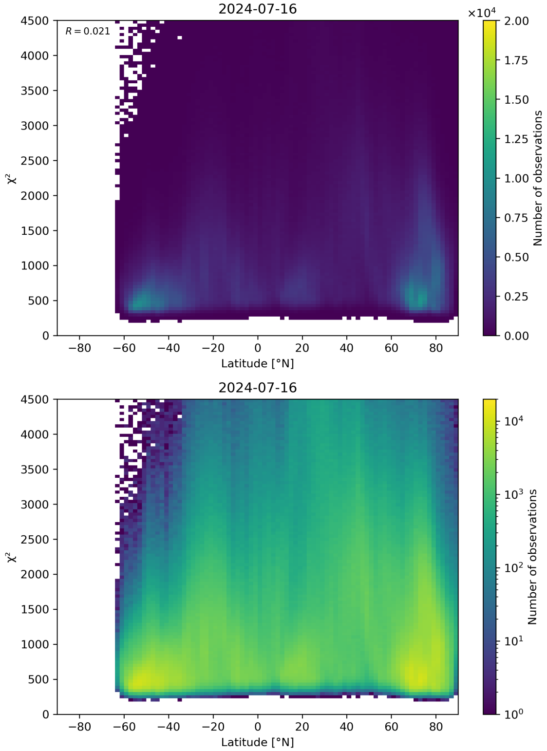
Figure 54: Scatter density plot of “Latitude” against “ \chi^2 ” for 2024-07-15 to 2024-07-17.
