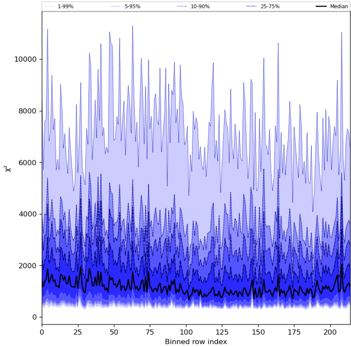
Figure 30: Along track statistics of “ \chi^2 ” for 2024-07-15 to 2024-07-17
