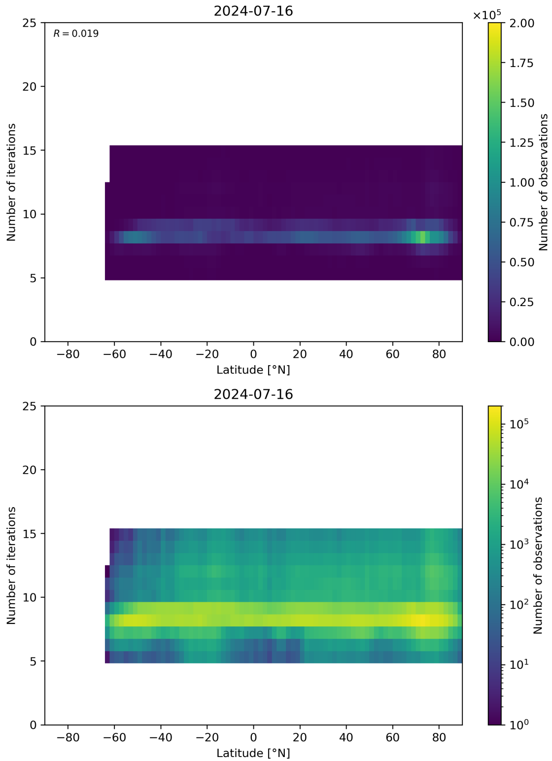
Figure 56: Scatter density plot of “Latitude” against “Number of iterations” for 2024-07-15 to 2024-07-17.
