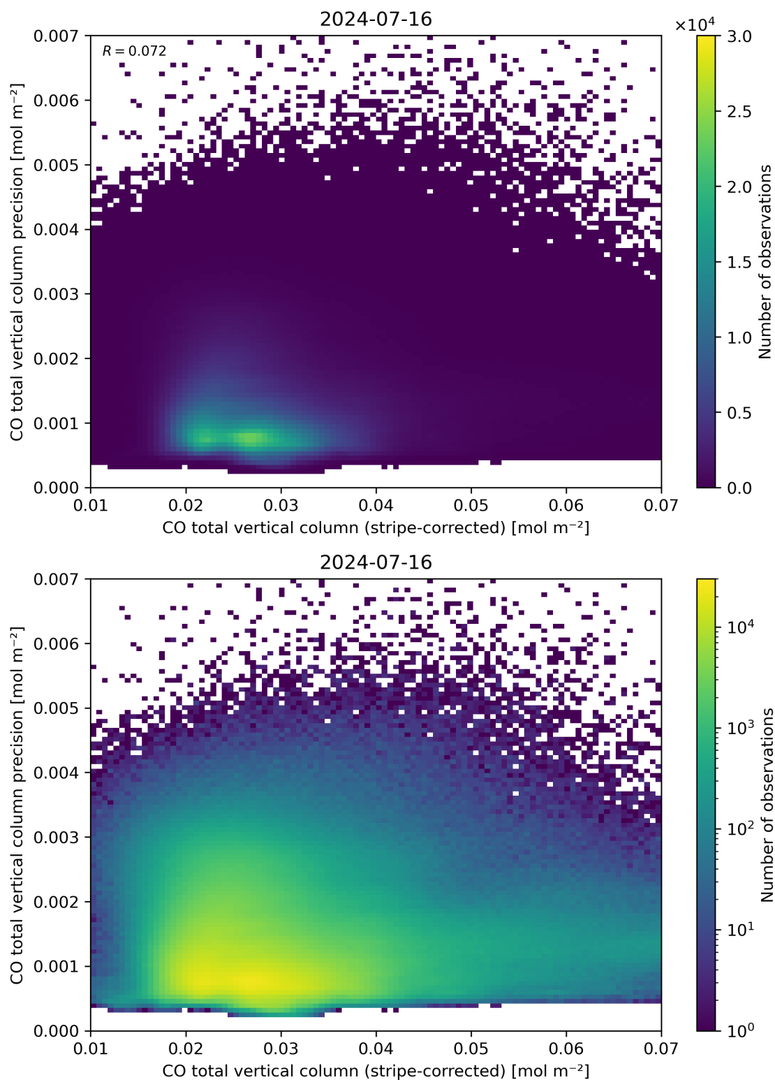
Figure 36: Scatter density plot of “CO total vertical column (stripe-corrected)” against “CO total vertical column precision” for 2024-07-15 to 2024-07-17.
