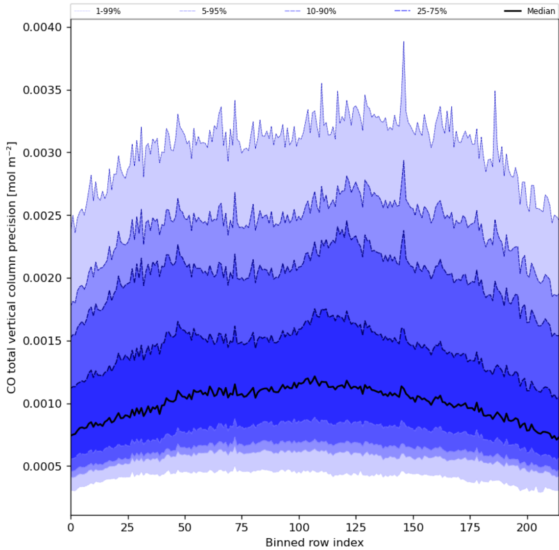
Figure 28: Along track statistics of “CO total vertical column precision” for 2024-07-15 to 2024-07-17
