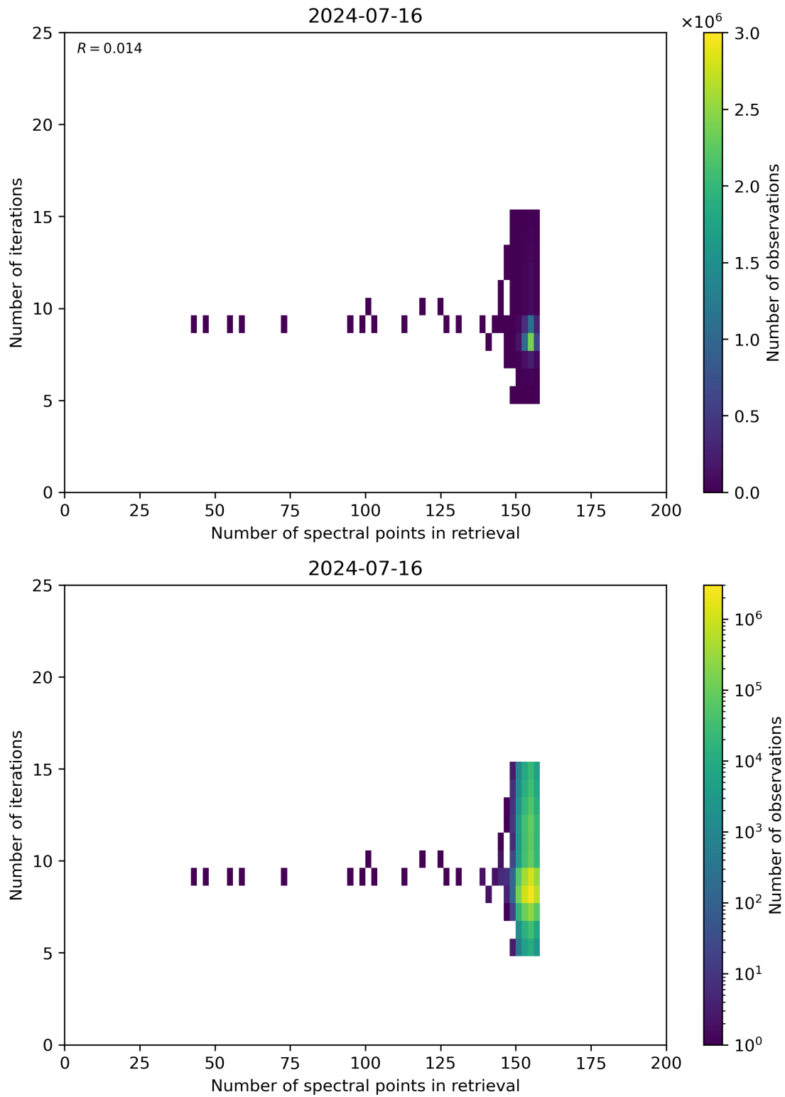
Figure 60: Scatter density plot of “Number of spectral points in retrieval” against “Number of iterations” for 2024-07-15 to 2024-07-17.
