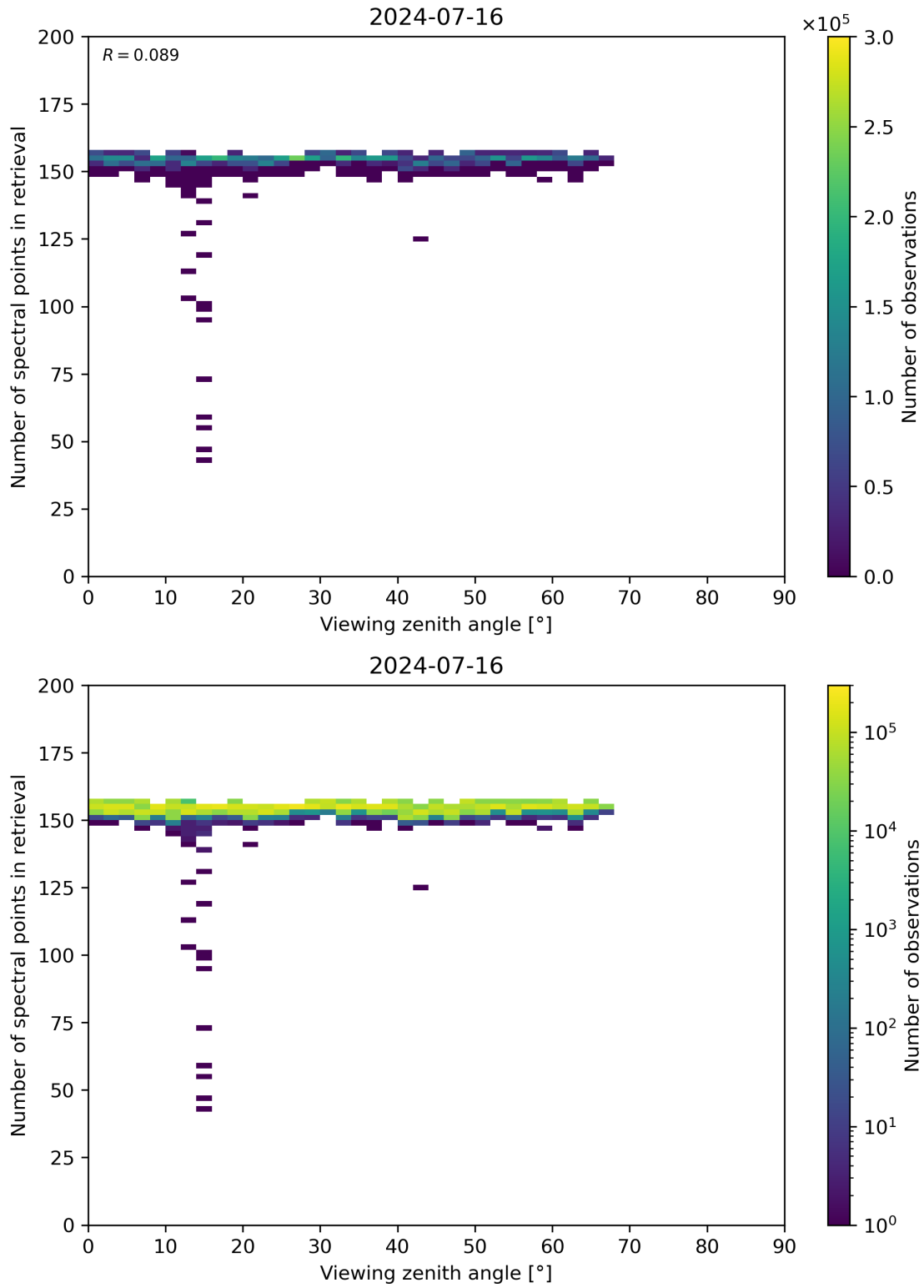
Figure 76: Scatter density plot of “Viewing zenith angle” against “Number of spectral points in retrieval” for 2024-07-15 to 2024-07-17.
