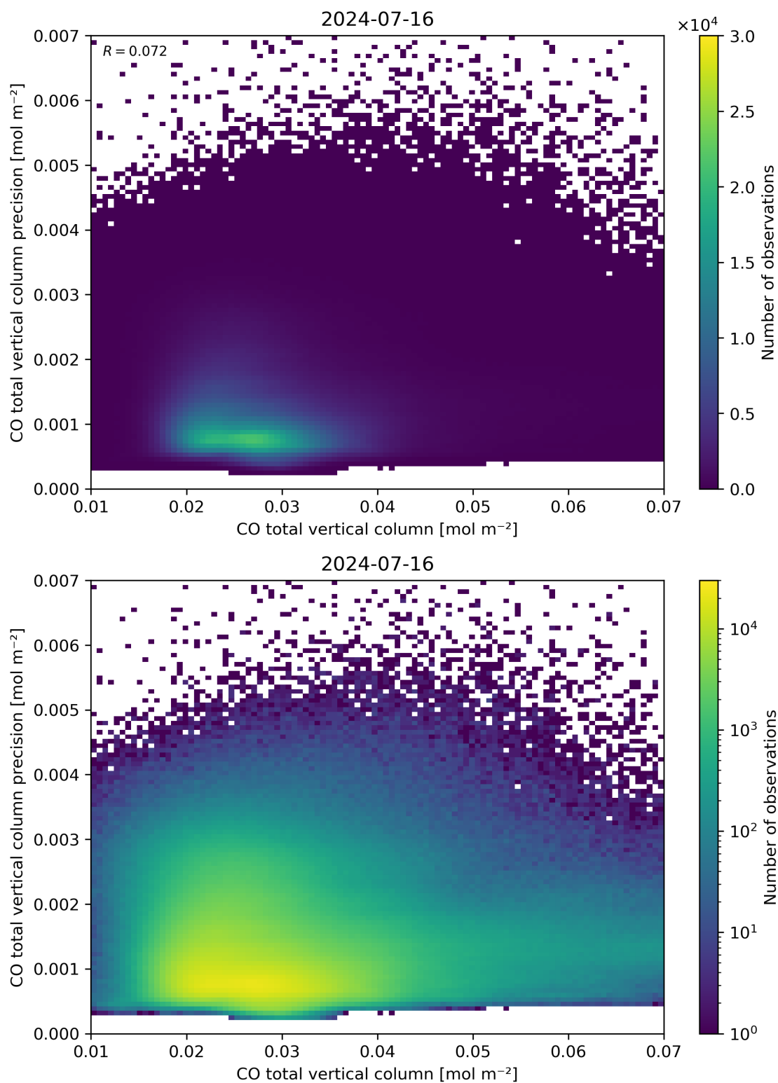
Figure 34: Scatter density plot of “CO total vertical column” against “CO total vertical column precision” for 2024-07-15 to 2024-07-17.
