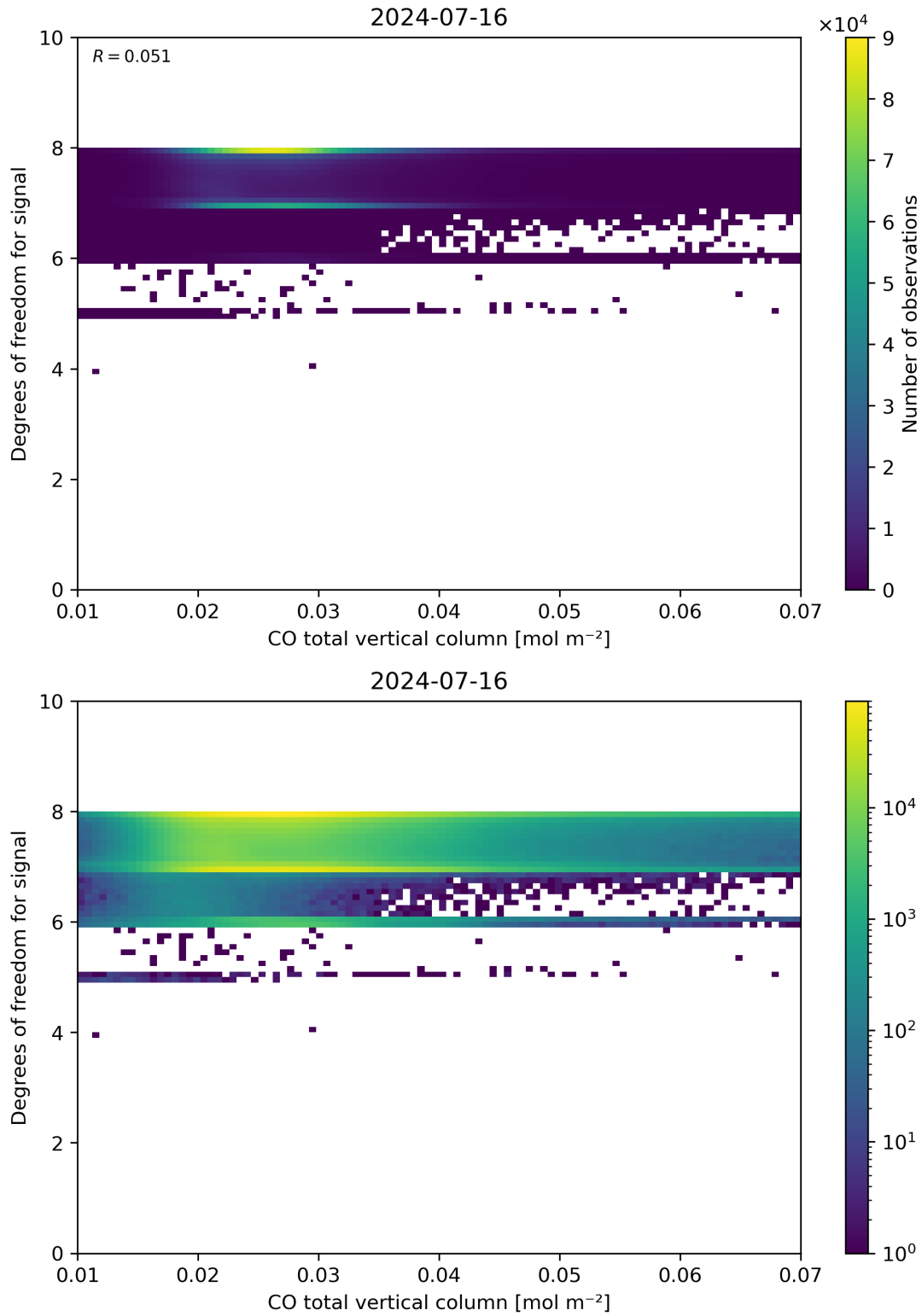
Figure 41: Scatter density plot of “CO total vertical column” against “Degrees of freedom for signal” for 2024-07-15 to 2024-07-17.
