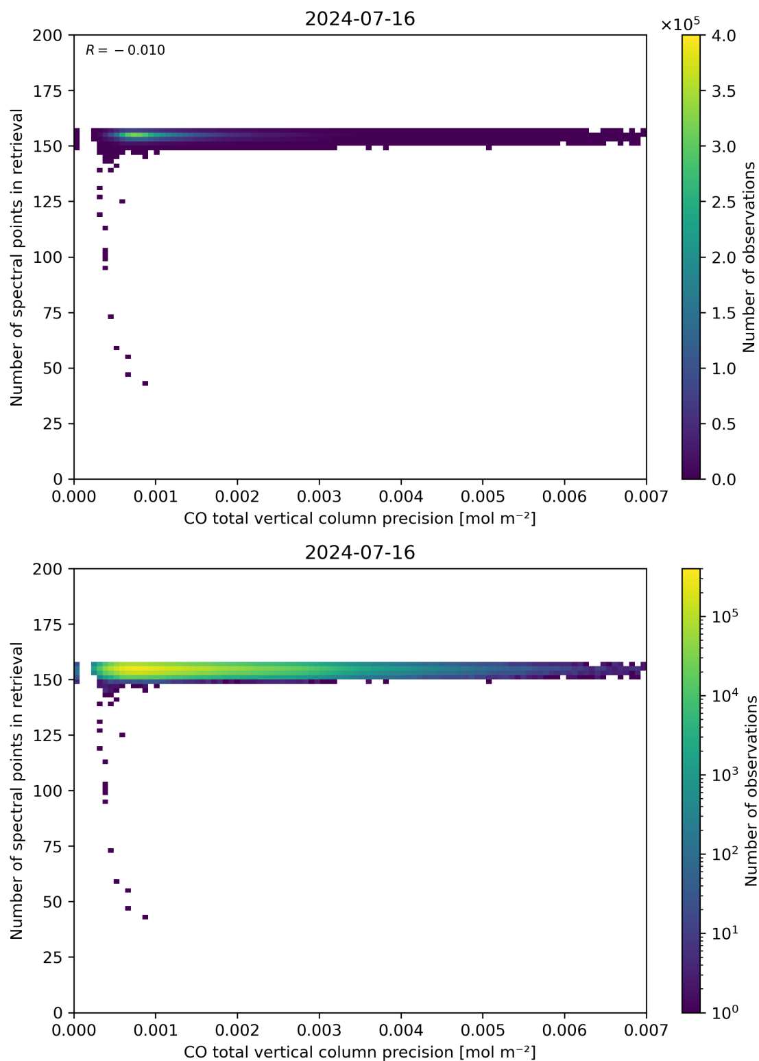
Figure 47: Scatter density plot of “CO total vertical column precision” against “Number of spectral points in retrieval” for 2024-07-15 to 2024-07-17.
