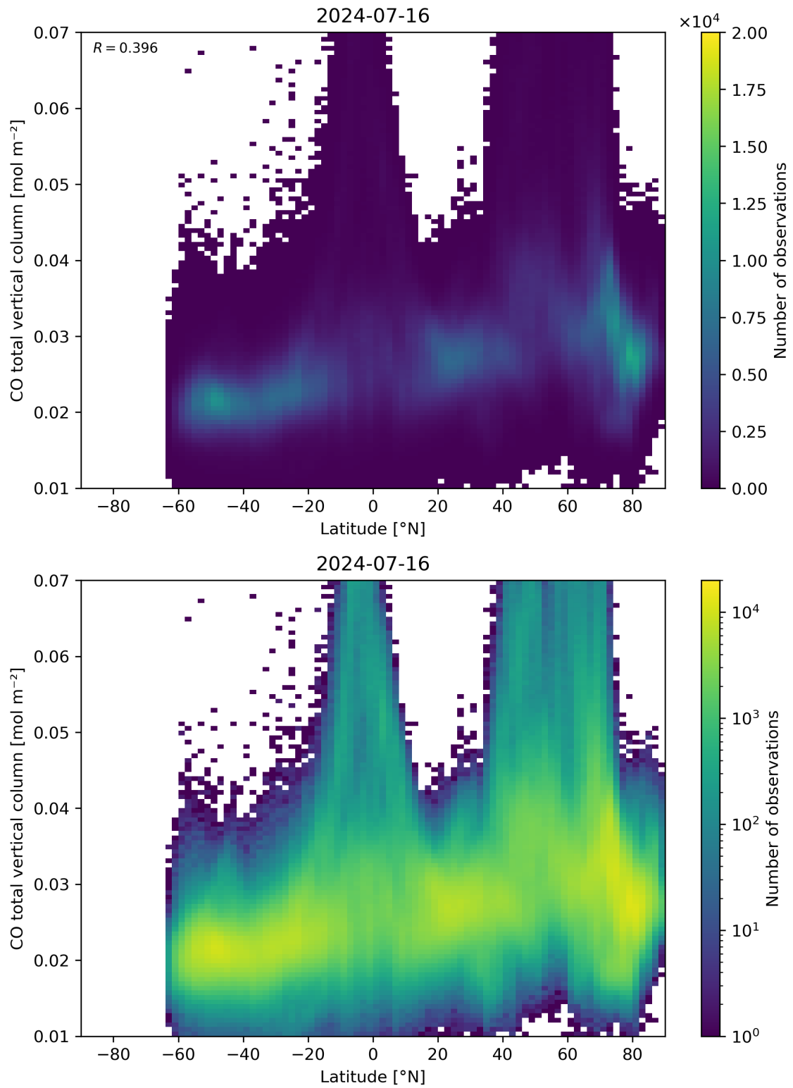
Figure 51: Scatter density plot of “Latitude” against “CO total vertical column” for 2024-07-15 to 2024-07-17.
