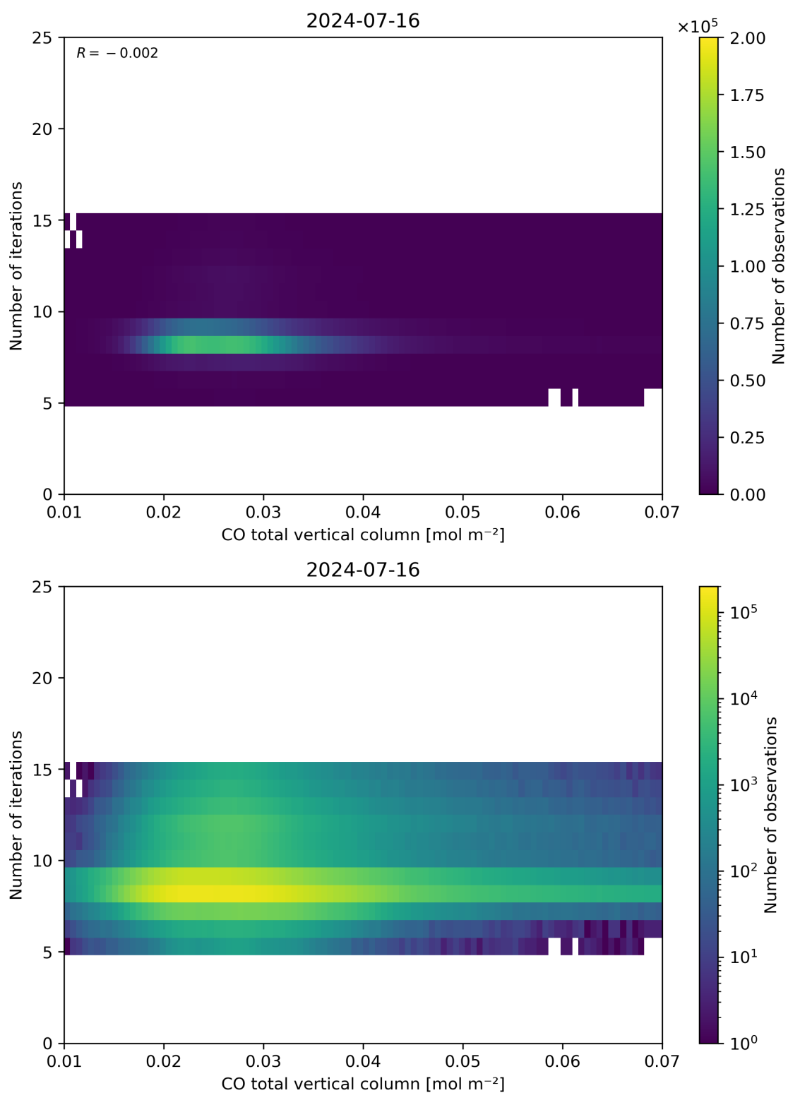
Figure 42: Scatter density plot of “CO total vertical column” against “Number of iterations” for 2024-07-15 to 2024-07-17.
