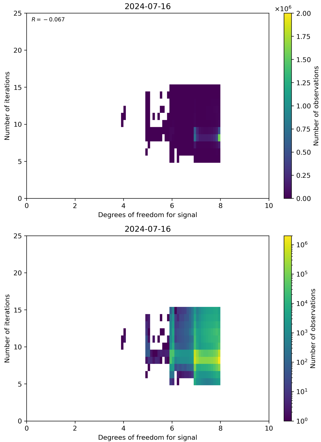
Figure 50: Scatter density plot of “Degrees of freedom for signal” against “Number of iterations” for 2024-07-15 to 2024-07-17.
