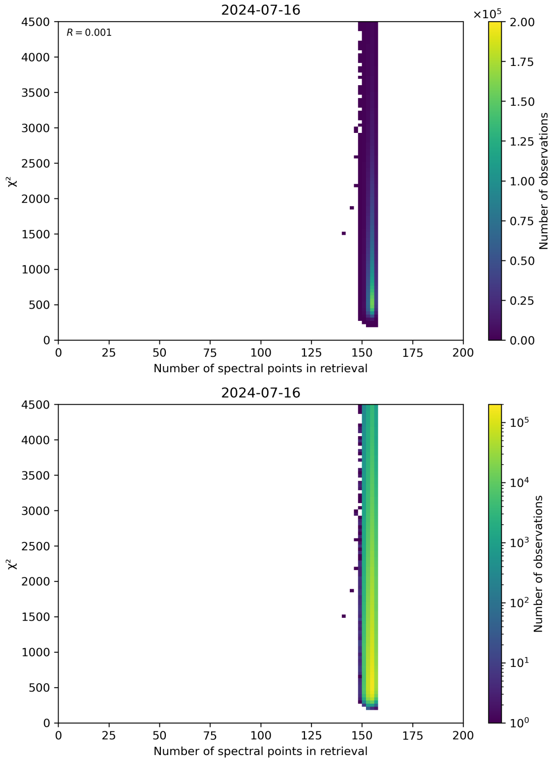
Figure 58: Scatter density plot of “Number of spectral points in retrieval” against “ \chi^2 ” for 2024-07-15 to 2024-07-17.
