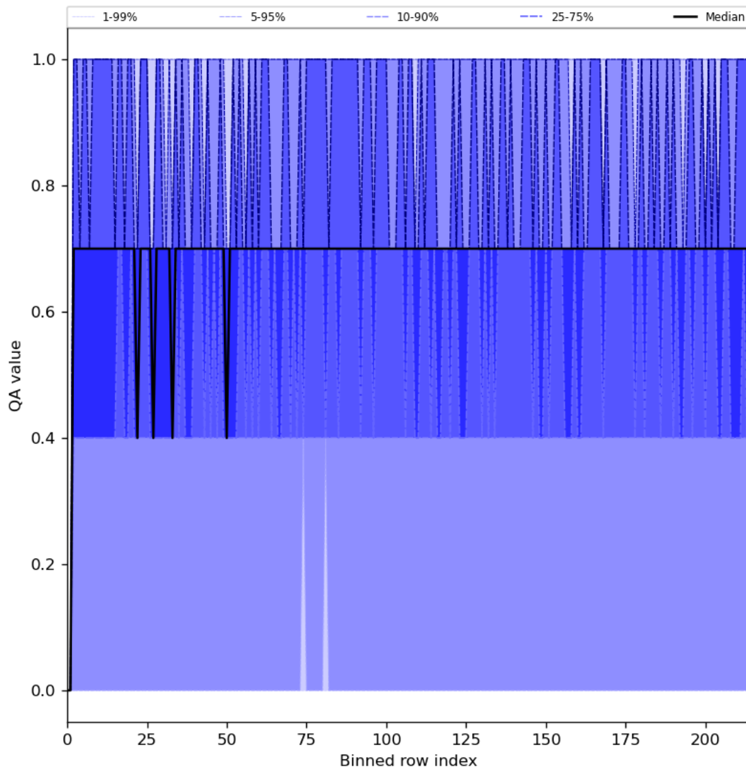
Figure 25: Along track statistics of “QA value” for 2024-07-15 to 2024-07-17
