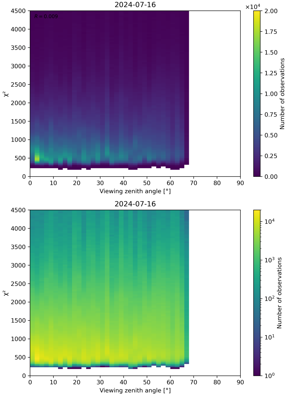
Figure 72: Scatter density plot of “Viewing zenith angle” against “ \chi^2 ” for 2024-07-15 to 2024-07-17.
