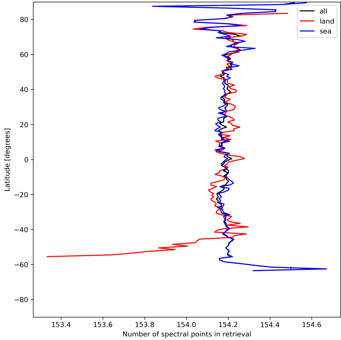
Figure 13: Zonal average of “Number of spectral points in retrieval” for 2024-07-15 to 2024-07-17.
