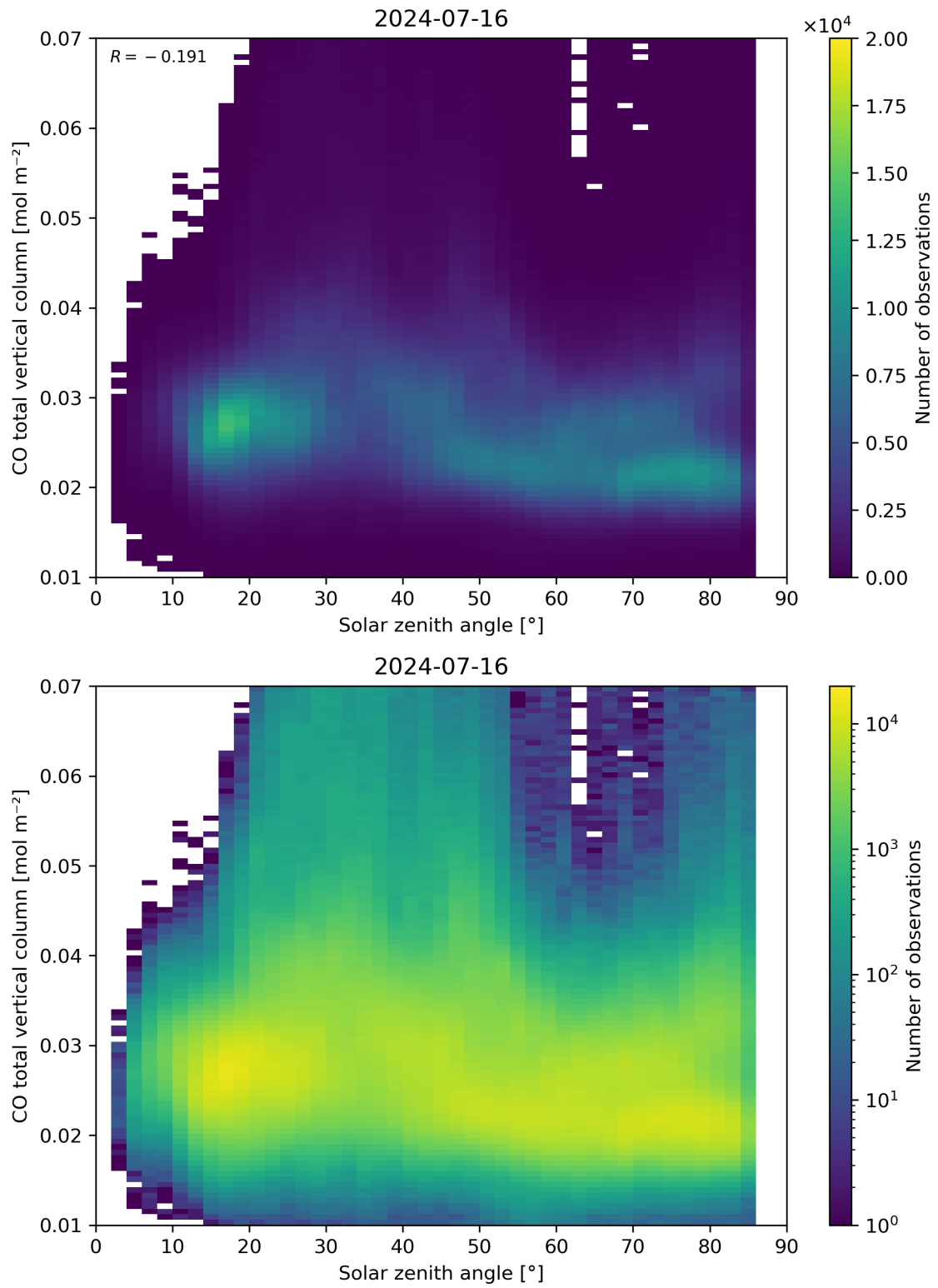
Figure 61: Scatter density plot of “Solar zenith angle” against “CO total vertical column” for 2024-07-15 to 2024-07-17.
