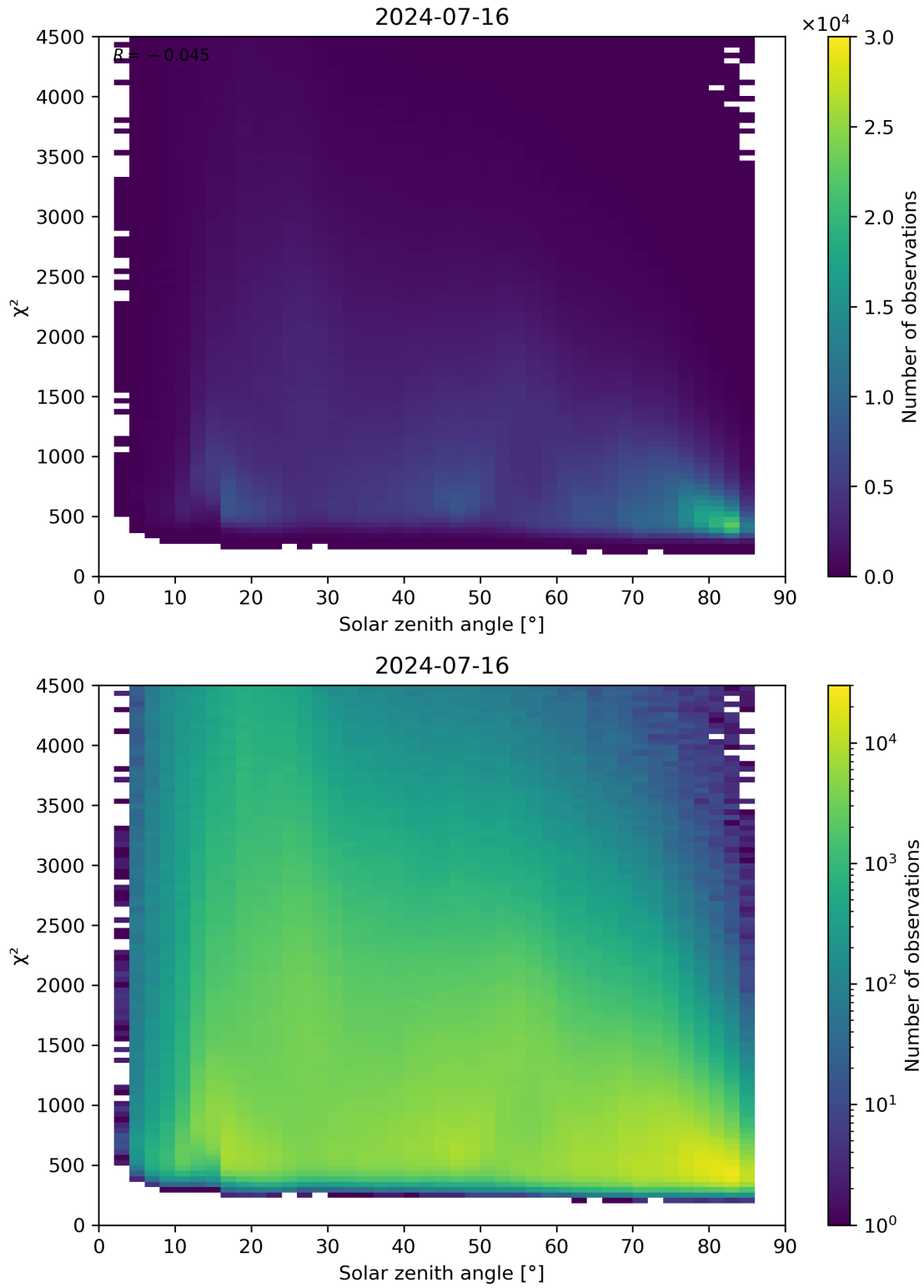
Figure 64: Scatter density plot of “Solar zenith angle” against “ \chi^2 ” for 2024-07-15 to 2024-07-17.
