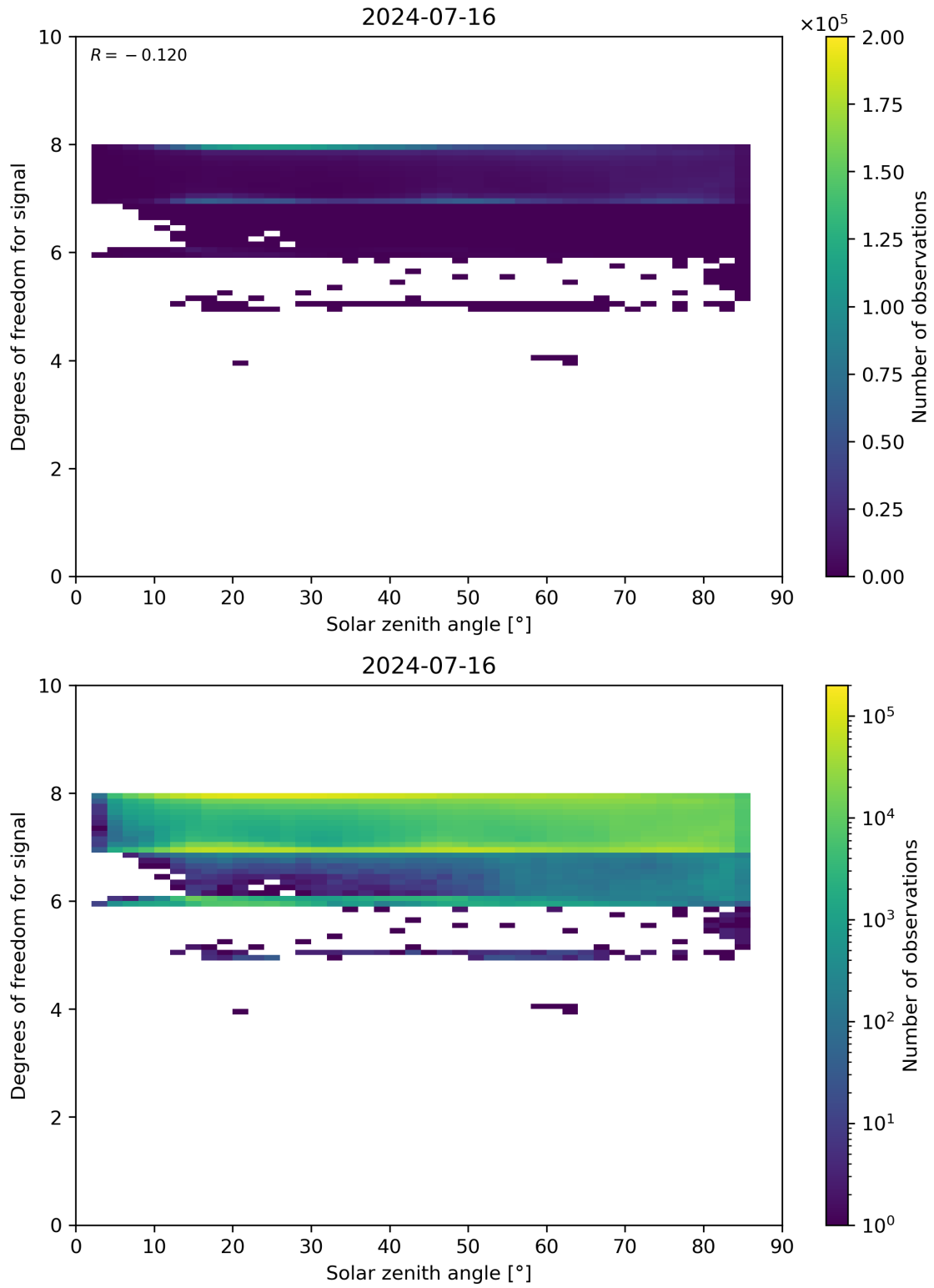
Figure 65: Scatter density plot of “Solar zenith angle” against “Degrees of freedom for signal” for 2024-07-15 to 2024-07-17.
