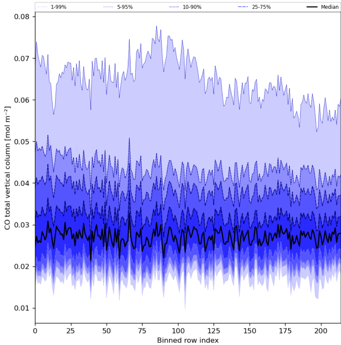
Figure 26: Along track statistics of “CO total vertical column” for 2024-07-15 to 2024-07-17
