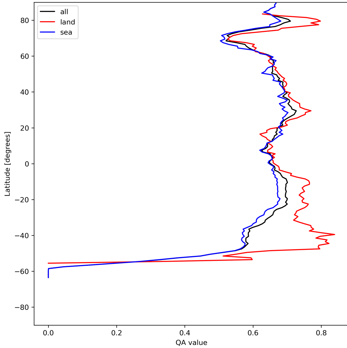
Figure 9: Zonal average of “QA value” for 2024-07-15 to 2024-07-17.
