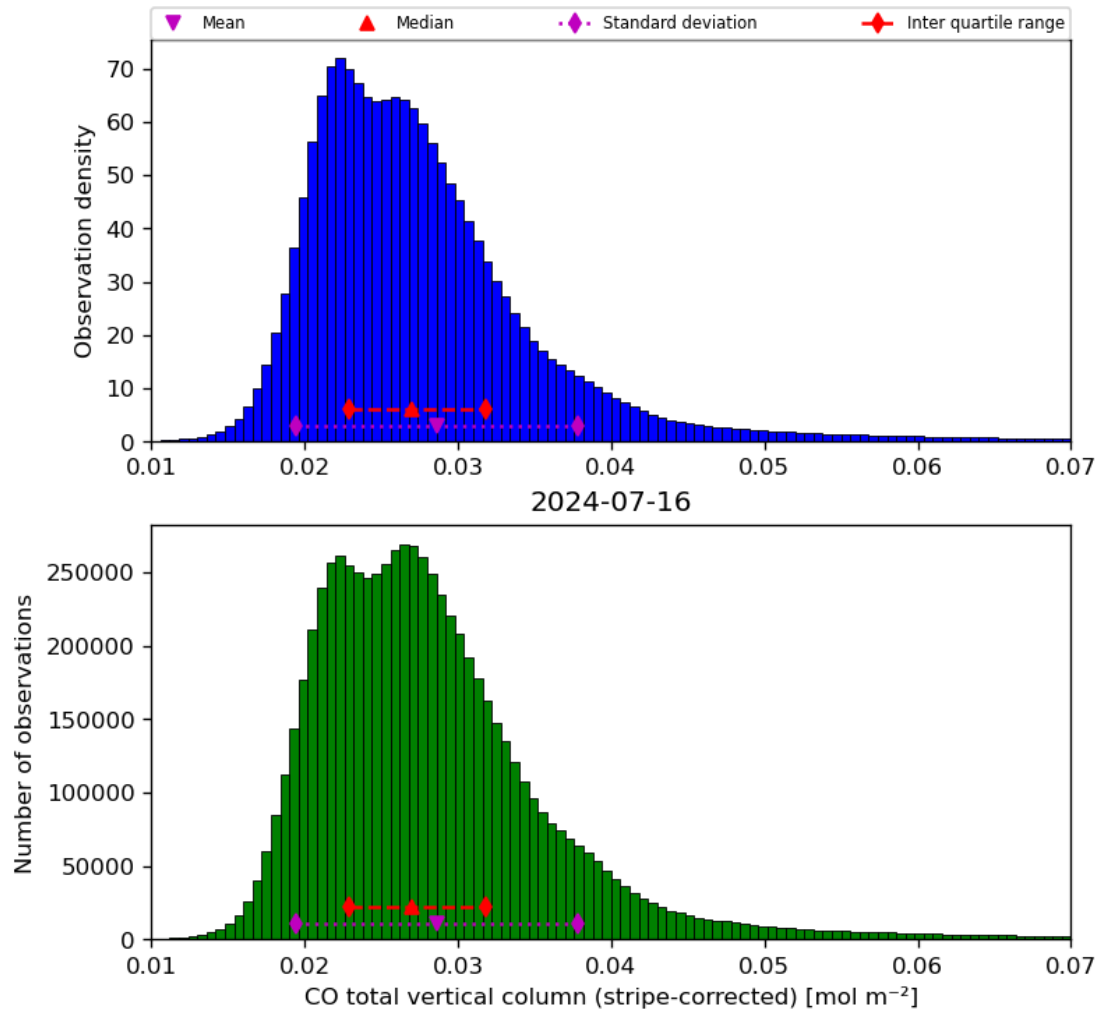
Figure 19: Histogram of “CO total vertical column (stripe-corrected)” for 2024-07-15 to 2024-07-17
