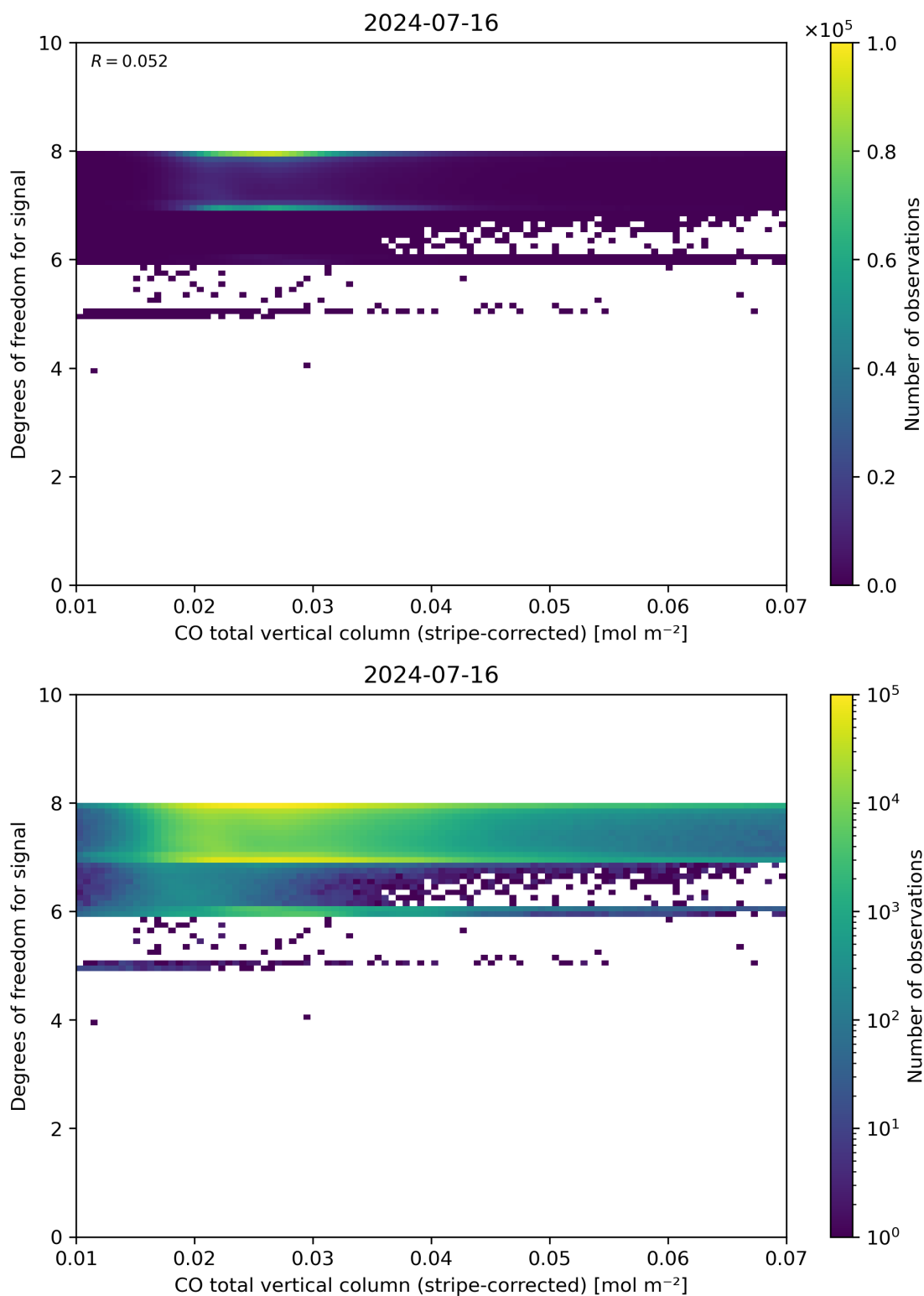
Figure 38: Scatter density plot of “CO total vertical column (stripe-corrected)” against “Degrees of freedom for signal” for 2024-07-15 to 2024-07-17.
