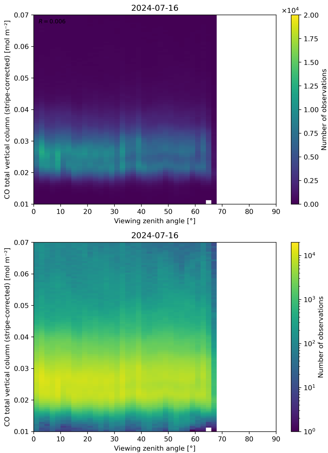
Figure 70: Scatter density plot of “Viewing zenith angle” against “CO total vertical column (stripe-corrected)” for 2024-07-15 to 2024-07-17.
