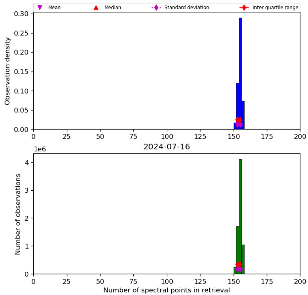
Figure 21: Histogram of “Number of spectral points in retrieval” for 2024-07-15 to 2024-07-17
