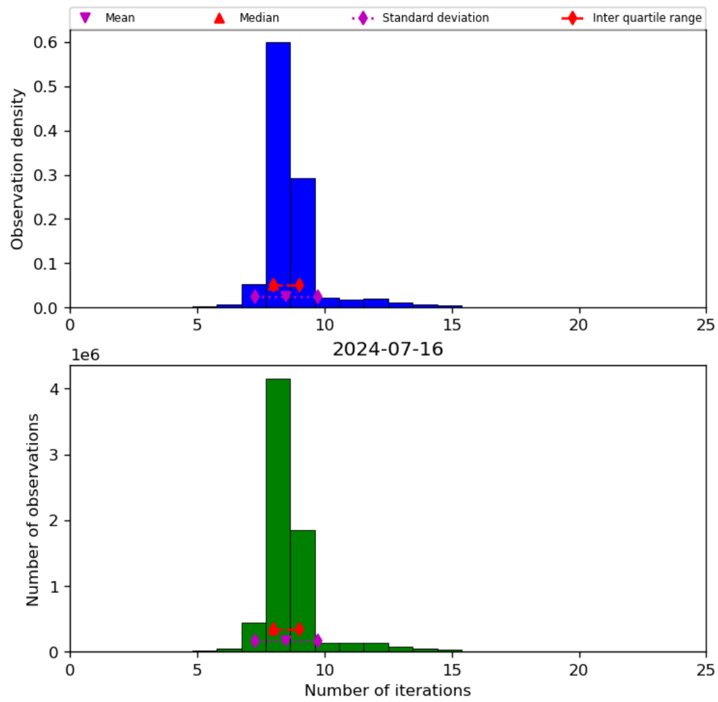
Figure 24: Histogram of “Number of iterations” for 2024-07-15 to 2024-07-17
