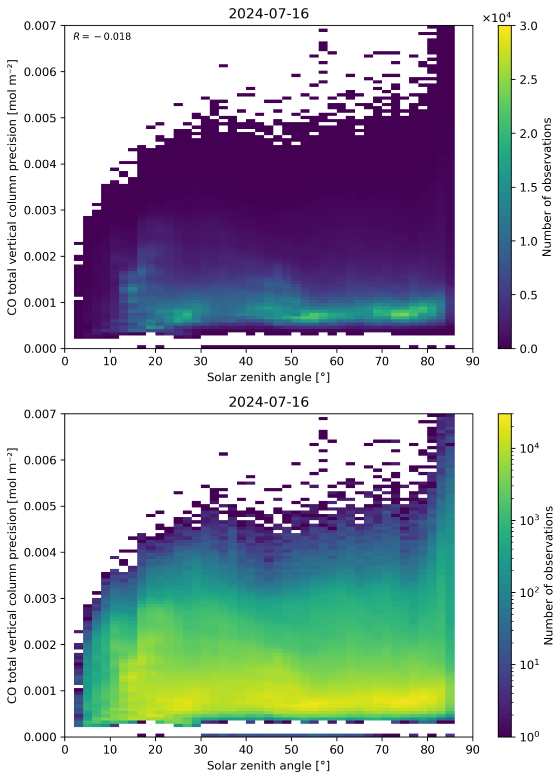
Figure 63: Scatter density plot of “Solar zenith angle” against “CO total vertical column precision” for 2024-07-15 to 2024-07-17.
