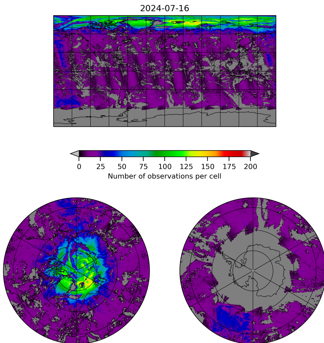
Figure 8: Map of the number of observations for 2024-07-15 to 2024-07-17
