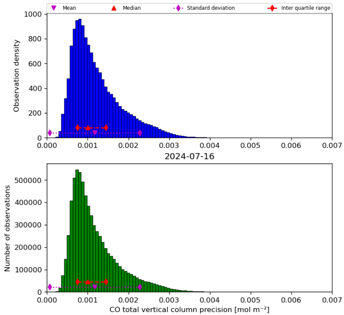
Figure 20: Histogram of “CO total vertical column precision” for 2024-07-15 to 2024-07-17
