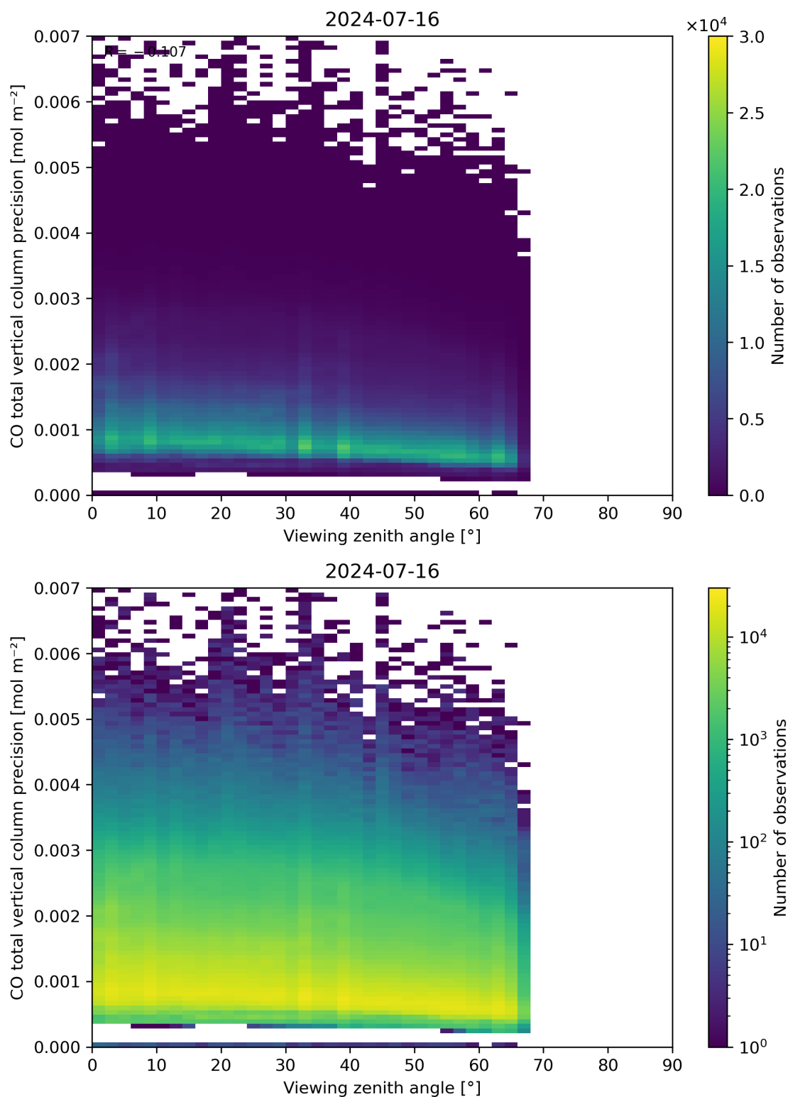
Figure 71: Scatter density plot of “Viewing zenith angle” against “CO total vertical column precision” for 2024-07-15 to 2024-07-17.
