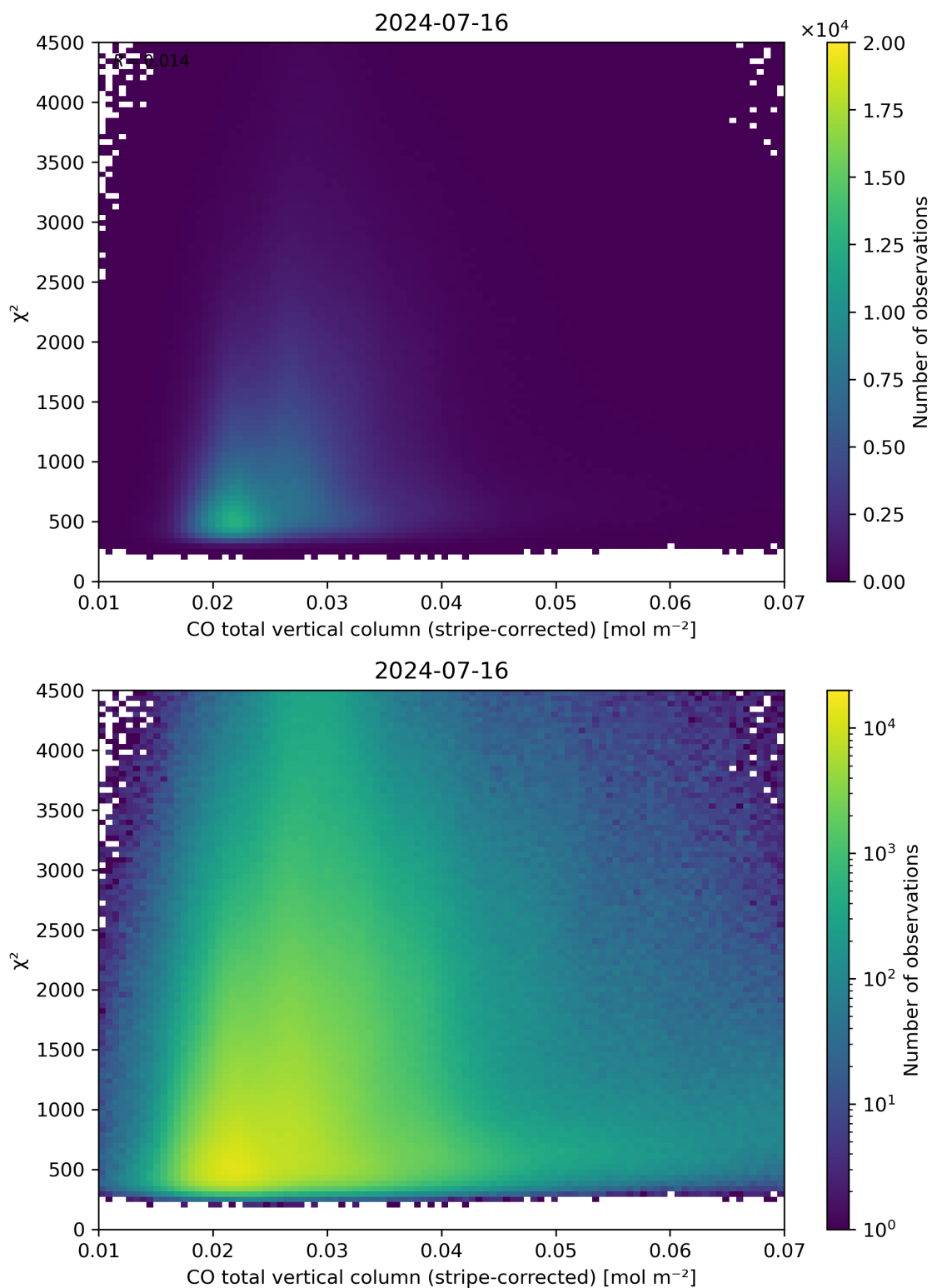
Figure 37: Scatter density plot of “CO total vertical column (stripe-corrected)” against “ \chi^2 ” for 2024-07-15 to 2024-07-17.
