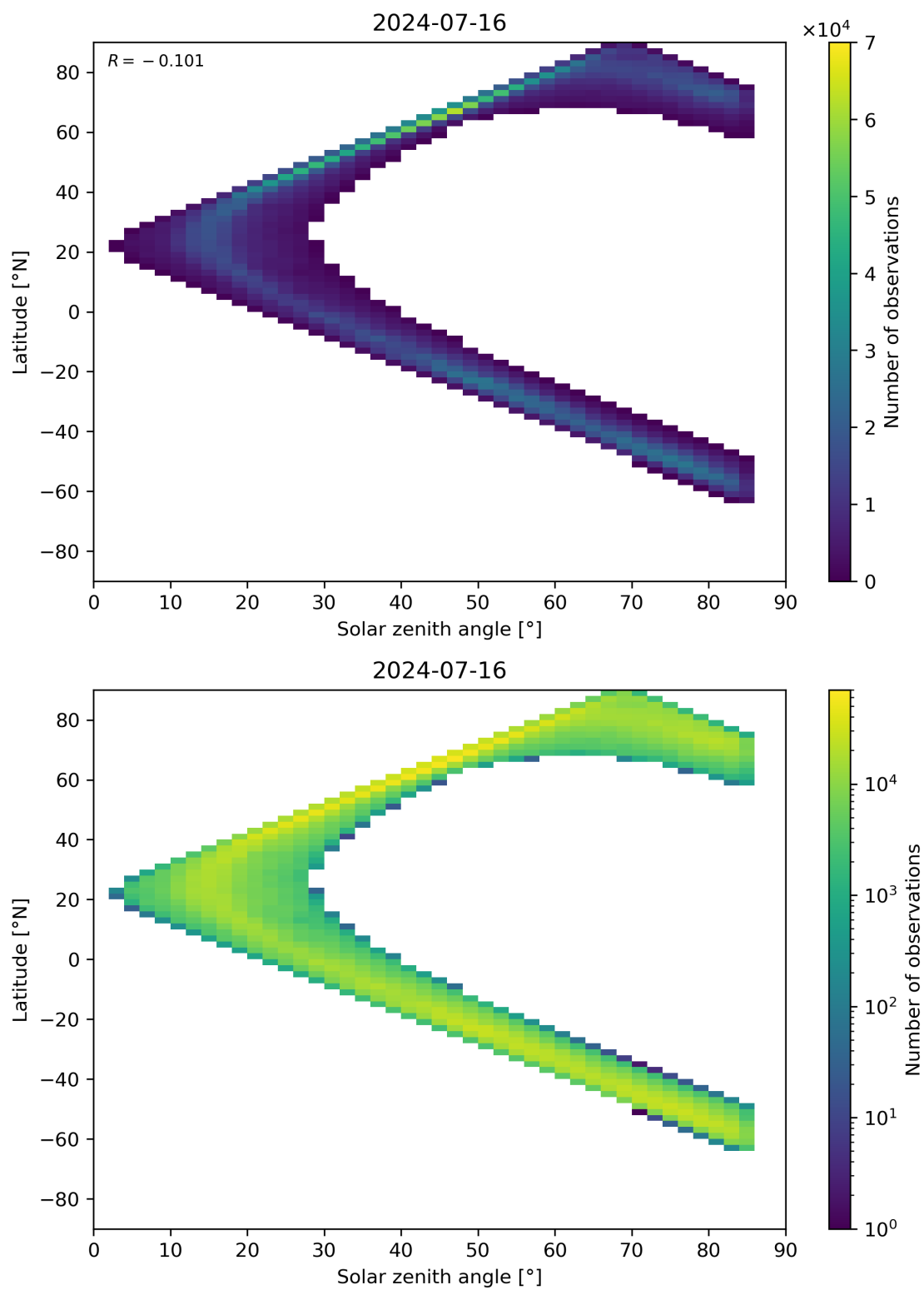
Figure 66: Scatter density plot of “Solar zenith angle” against “Latitude” for 2024-07-15 to 2024-07-17.
