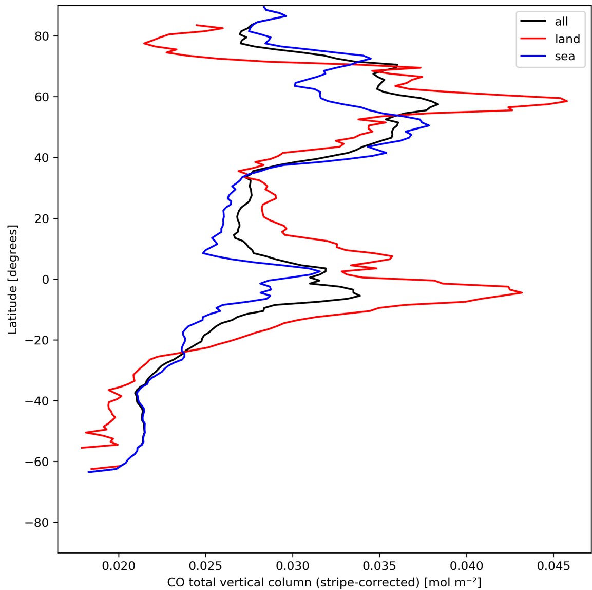
Figure 11: Zonal average of “CO total vertical column (stripe-corrected)” for 2024-07-15 to 2024-07-17.
