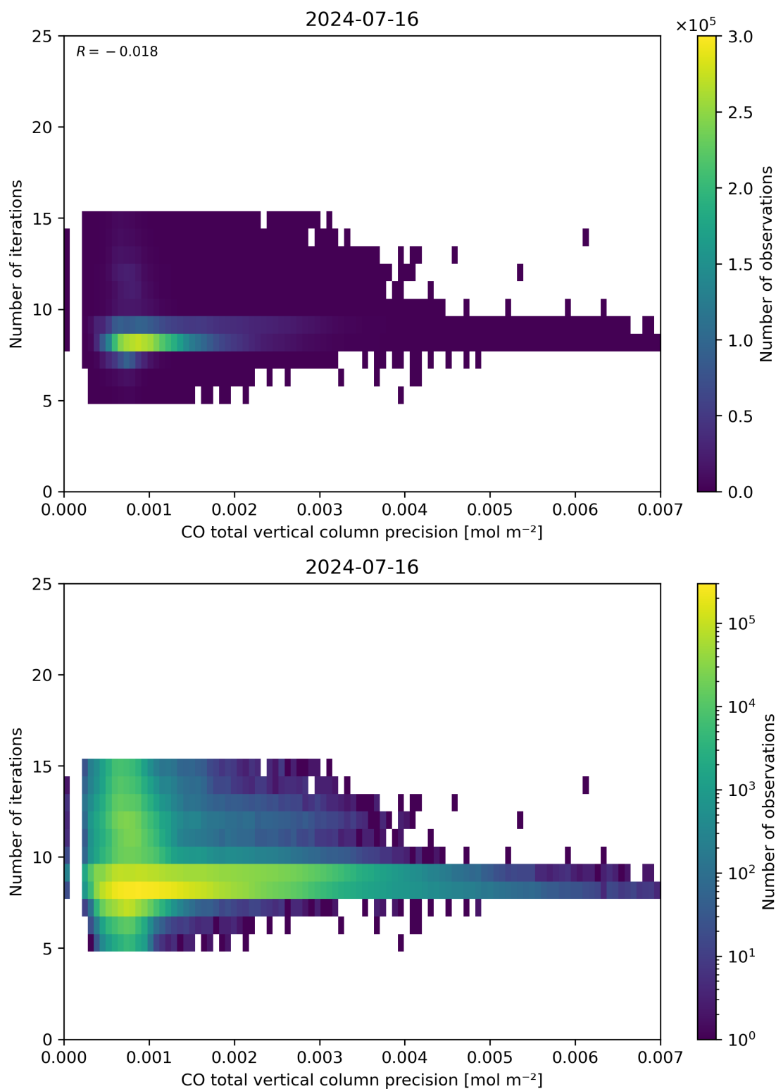
Figure 46: Scatter density plot of “CO total vertical column precision” against “Number of iterations” for 2024-07-15 to 2024-07-17.
