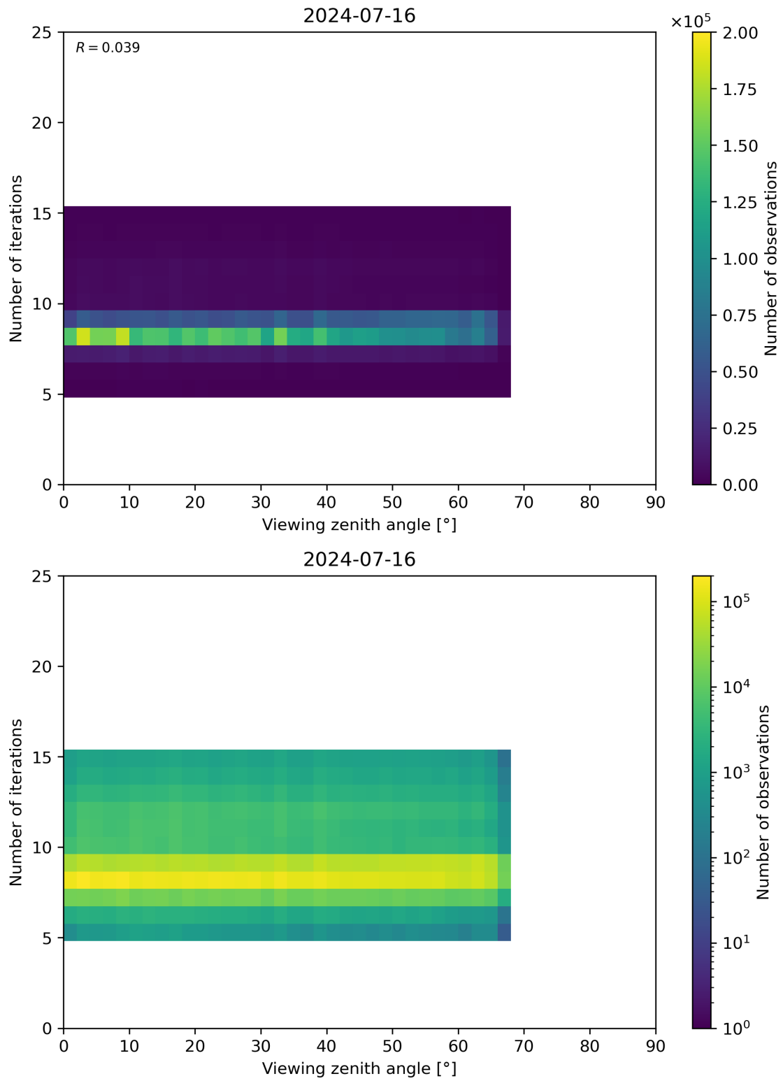
Figure 75: Scatter density plot of “Viewing zenith angle” against “Number of iterations” for 2024-07-15 to 2024-07-17.
