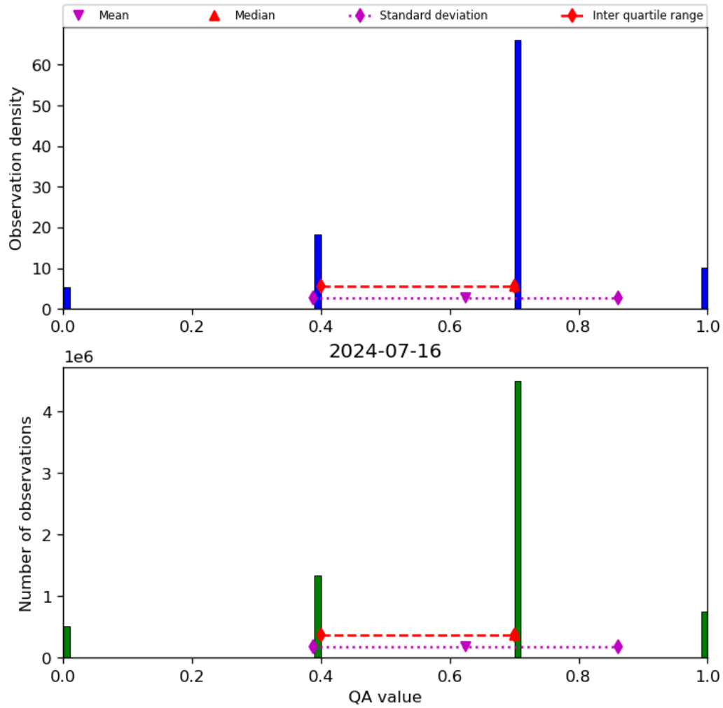
Figure 17: Histogram of “QA value” for 2024-07-15 to 2024-07-17
