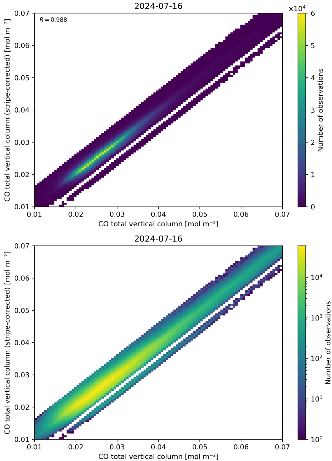
Figure 33: Scatter density plot of “CO total vertical column” against “CO total vertical column (stripe-corrected)” for 2024-07-15 to 2024-07-17.
