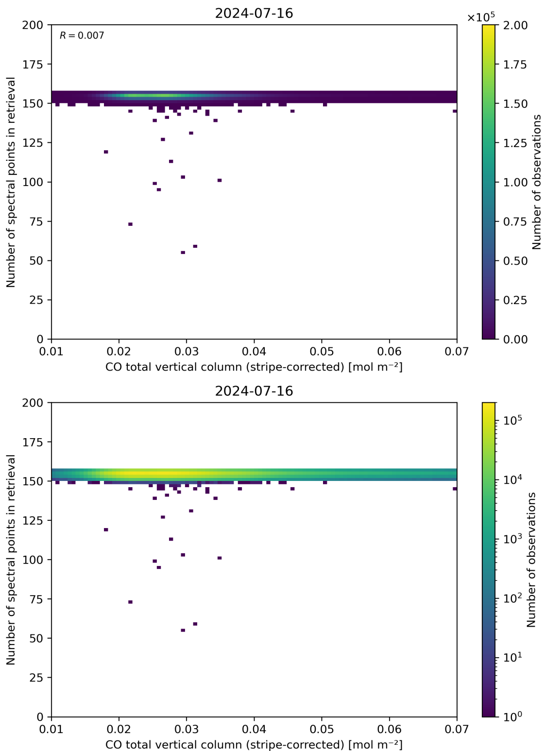
Figure 40: Scatter density plot of “CO total vertical column (stripe-corrected)” against “Number of spectral points in retrieval” for 2024-07-15 to 2024-07-17.
