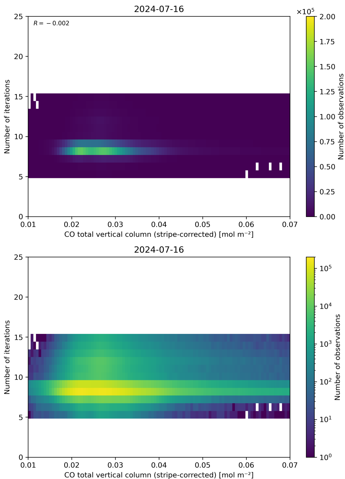
Figure 39: Scatter density plot of “CO total vertical column (stripe-corrected)” against “Number of iterations” for 2024-07-15 to 2024-07-17.
