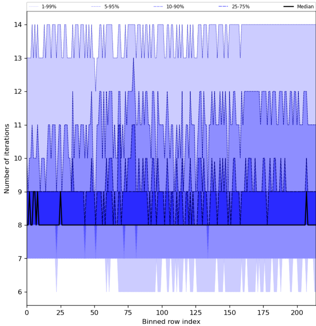
Figure 32: Along track statistics of “Number of iterations” for 2024-07-15 to 2024-07-17
