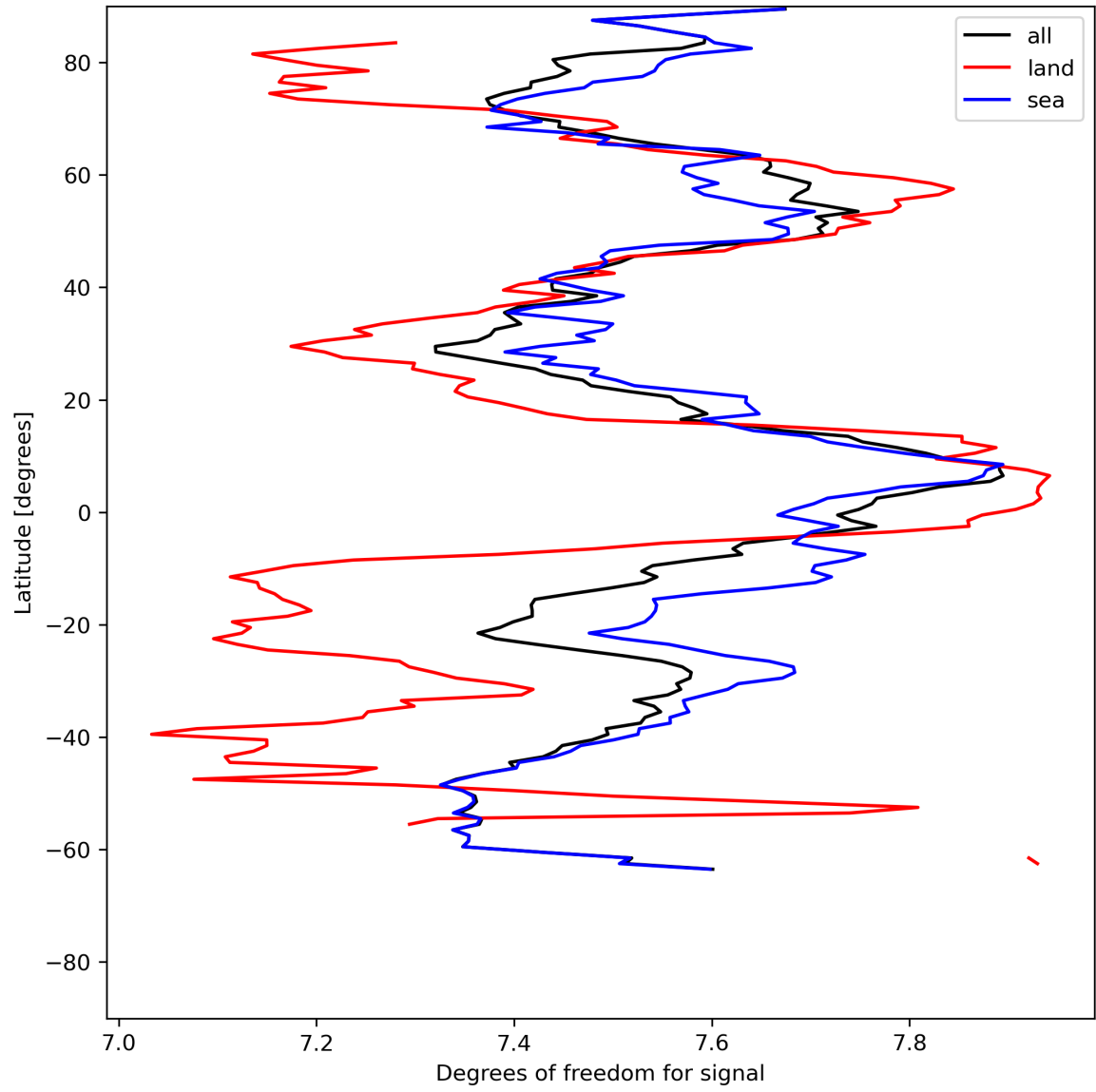
Figure 15: Zonal average of “Degrees of freedom for signal” for 2024-07-15 to 2024-07-17.
