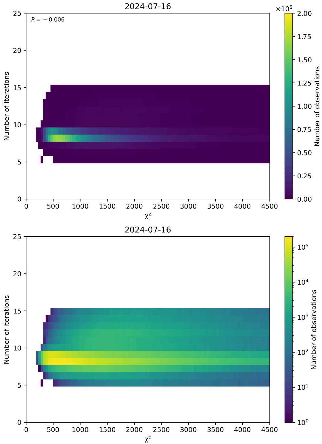
Figure 49: Scatter density plot of “ \chi^2 ” against “Number of iterations” for 2024-07-15 to 2024-07-17.
