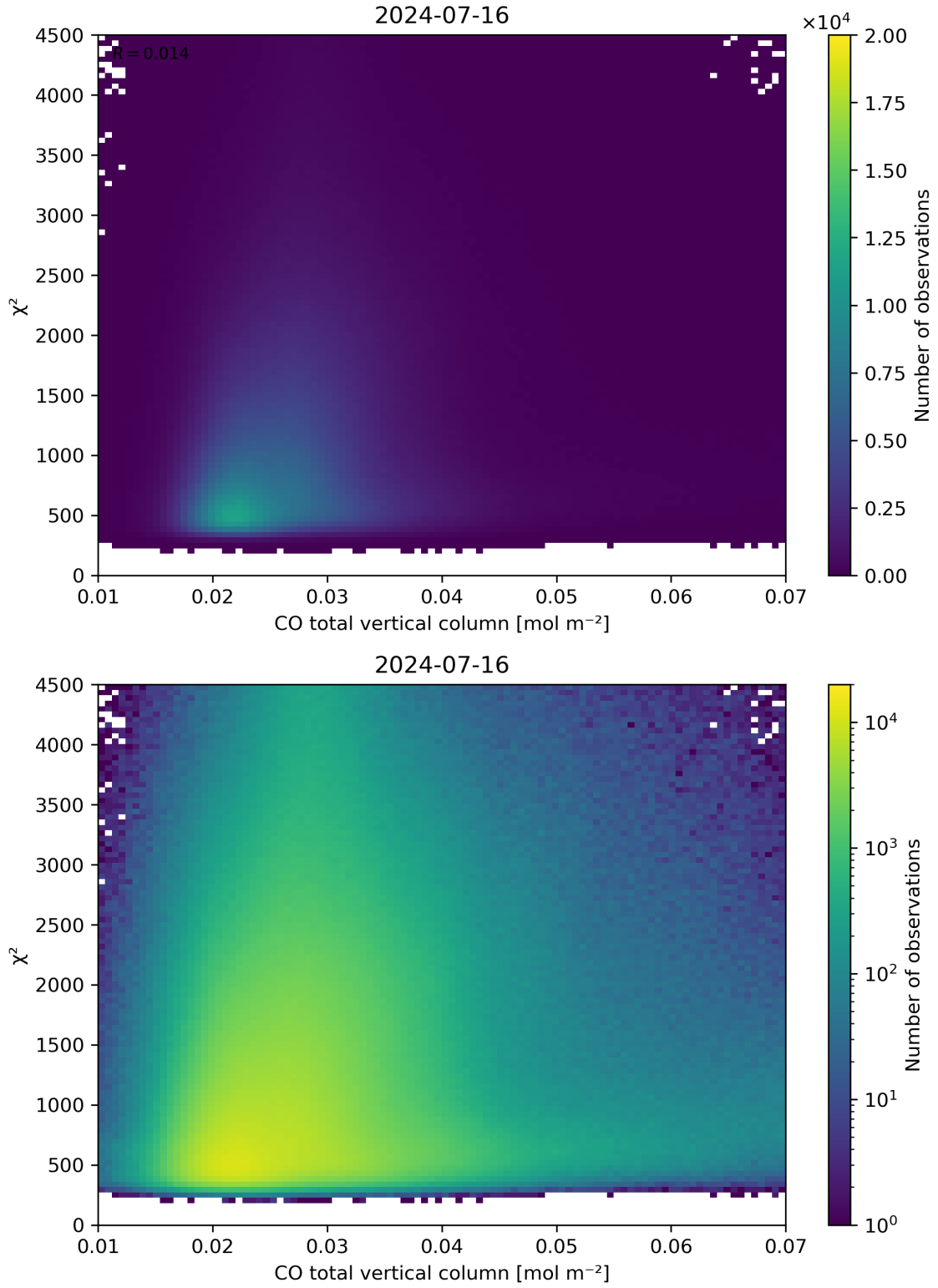
Figure 35: Scatter density plot of “CO total vertical column” against “ \chi^2 ” for 2024-07-15 to 2024-07-17.
