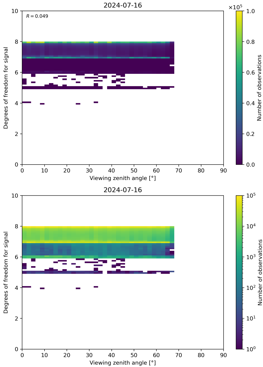
Figure 73: Scatter density plot of “Viewing zenith angle” against “Degrees of freedom for signal” for 2024-07-15 to 2024-07-17.
