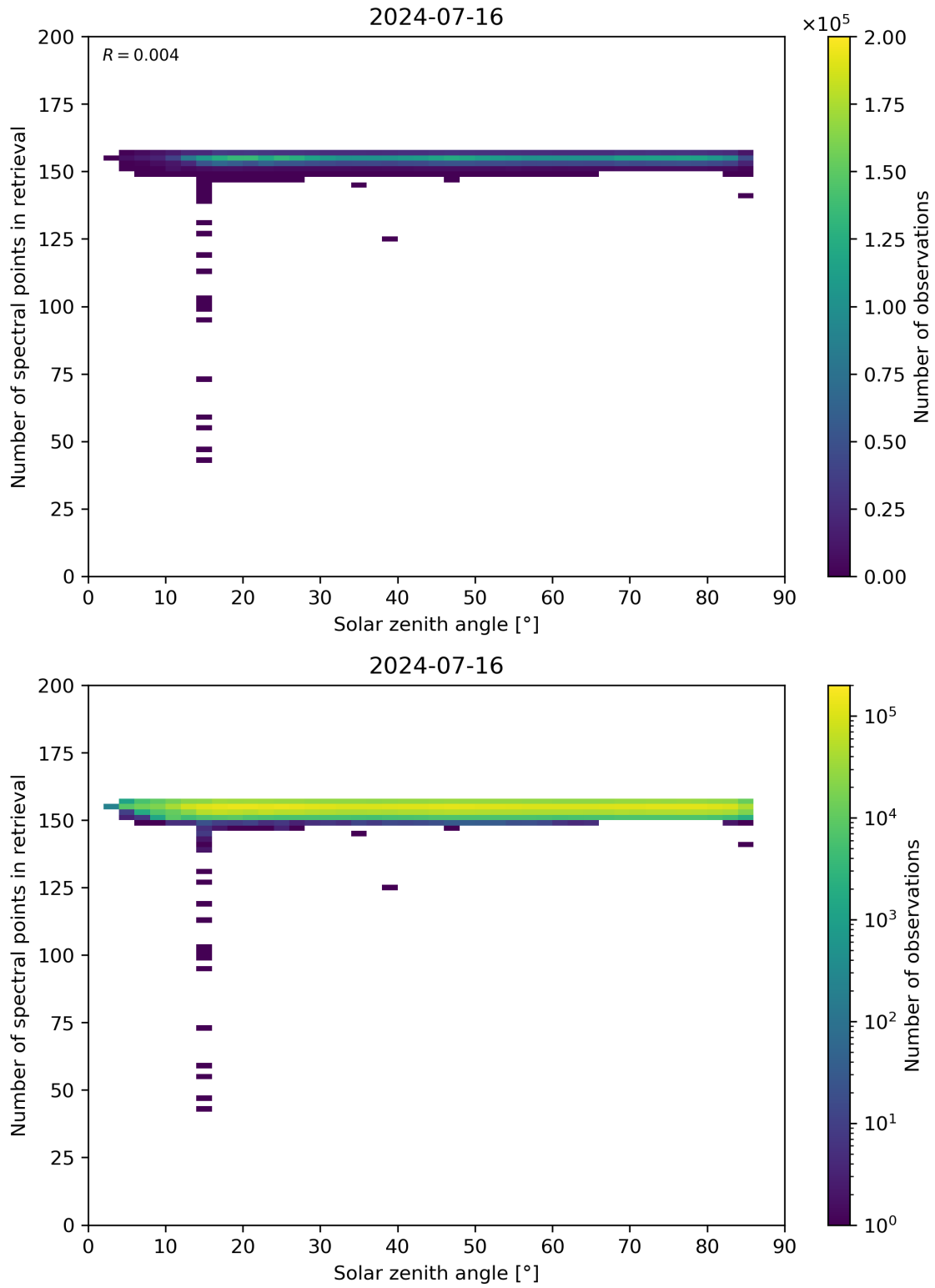
Figure 68: Scatter density plot of “Solar zenith angle” against “Number of spectral points in retrieval” for 2024-07-15 to 2024-07-17.
