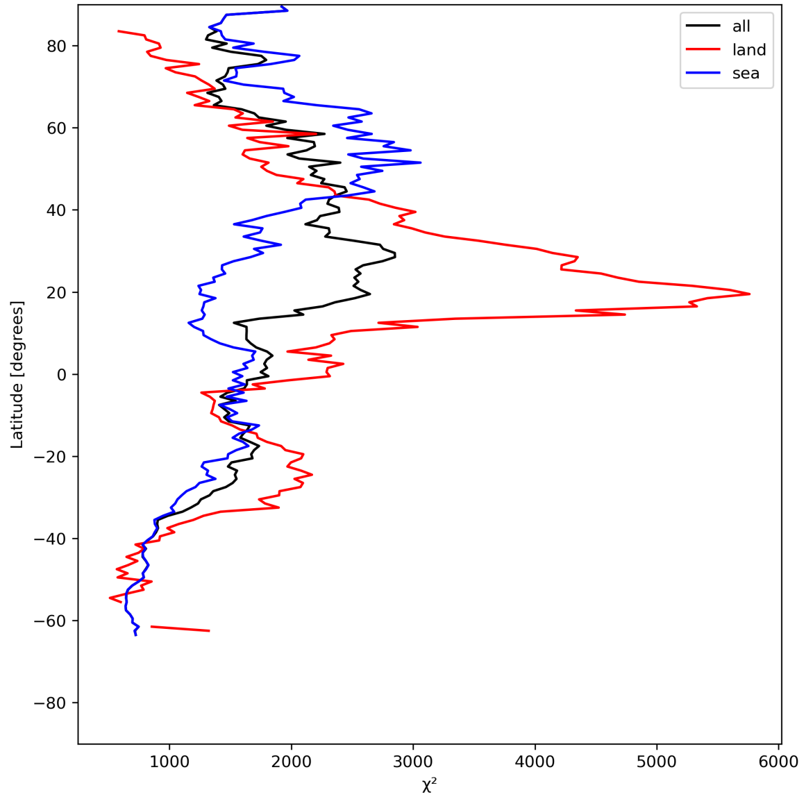
Figure 14: Zonal average of “ \chi^2 ” for 2024-07-15 to 2024-07-17.
