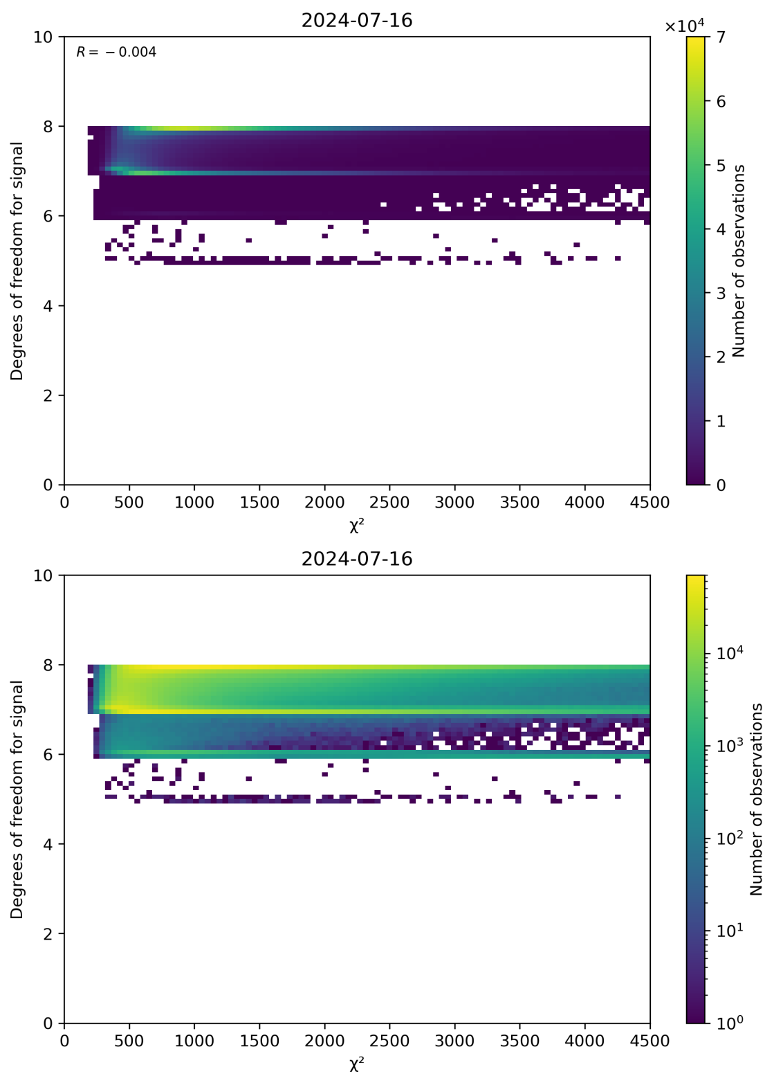
Figure 48: Scatter density plot of “ \chi^2 ” against “Degrees of freedom for signal” for 2024-07-15 to 2024-07-17.
