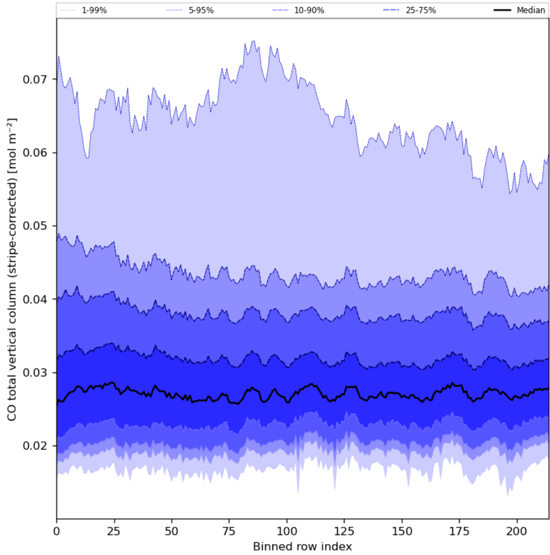
Figure 27: Along track statistics of “CO total vertical column (stripe-corrected)” for 2024-07-15 to 2024-07-17
