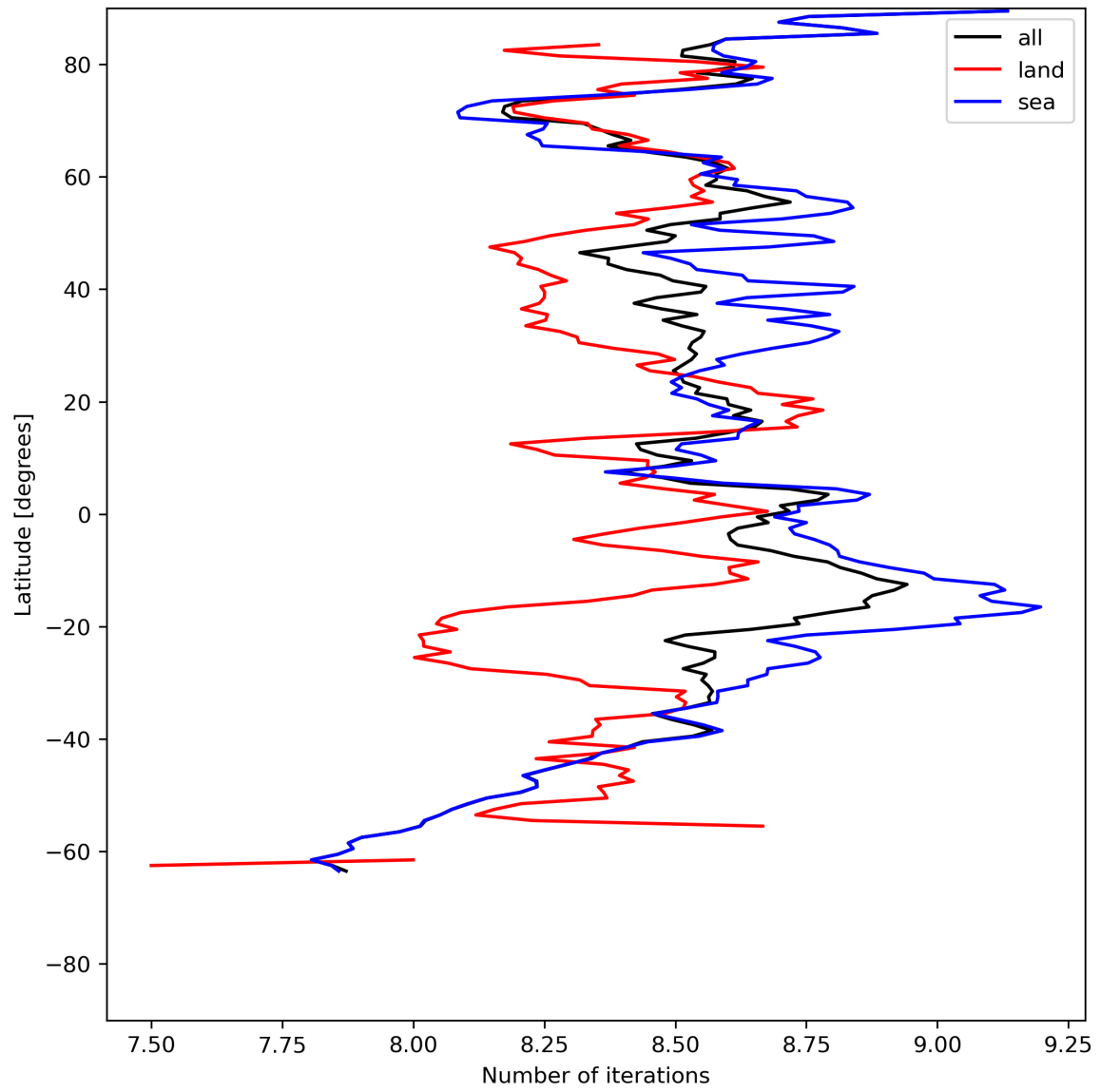
Figure 16: Zonal average of “Number of iterations” for 2024-07-15 to 2024-07-17.
