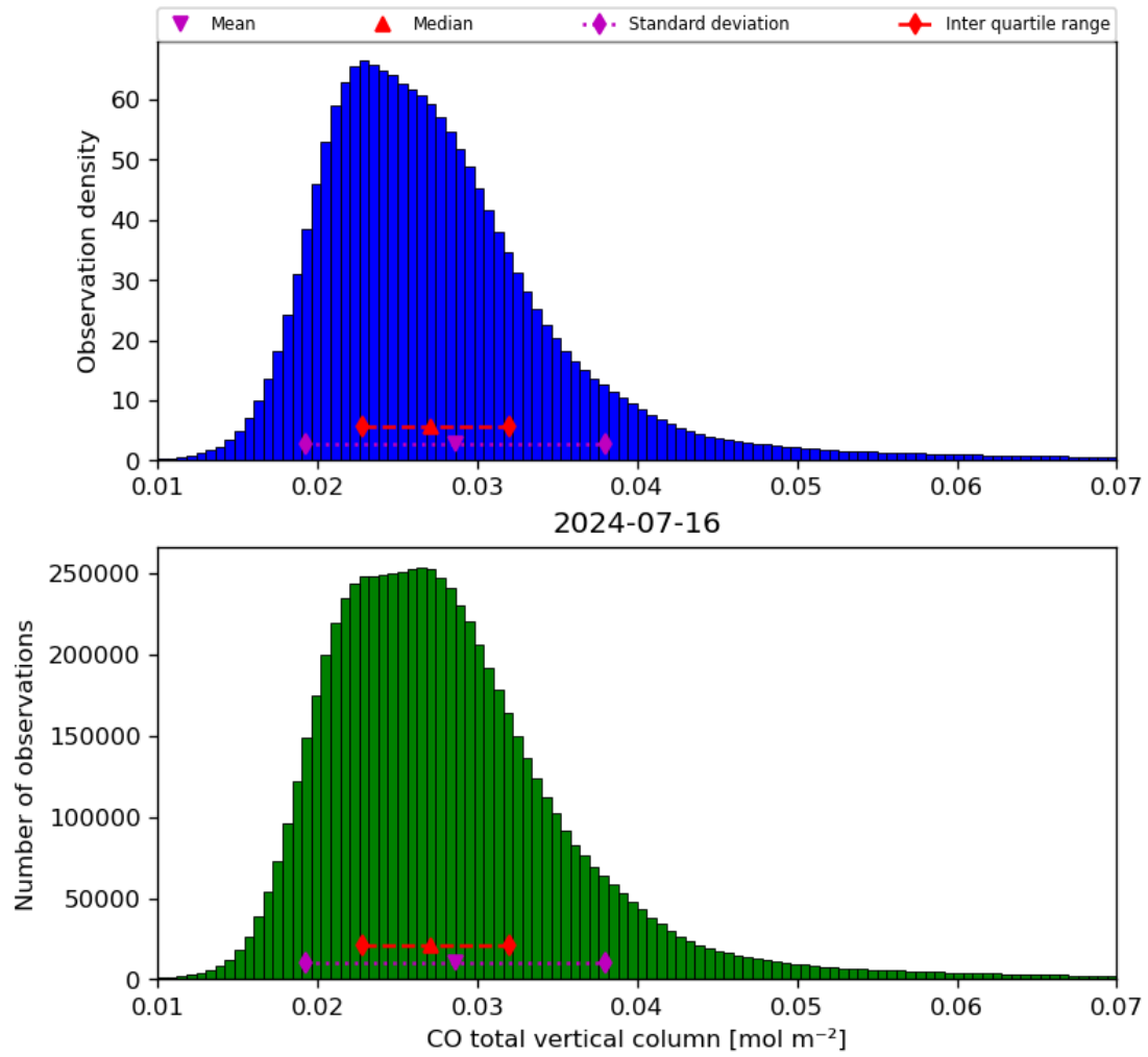
Figure 18: Histogram of “CO total vertical column” for 2024-07-15 to 2024-07-17
