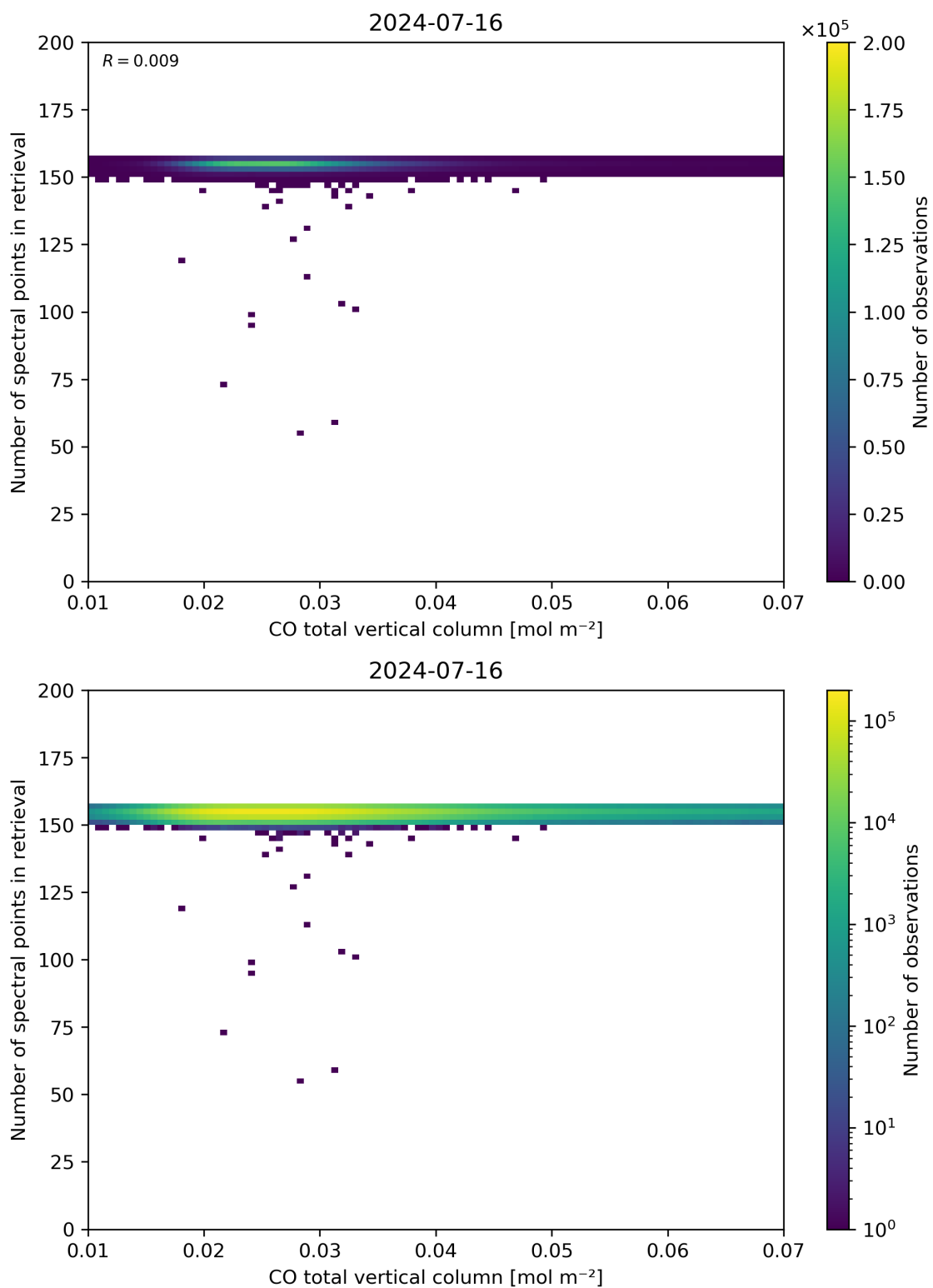
Figure 43: Scatter density plot of “CO total vertical column” against “Number of spectral points in retrieval” for 2024-07-15 to 2024-07-17.
