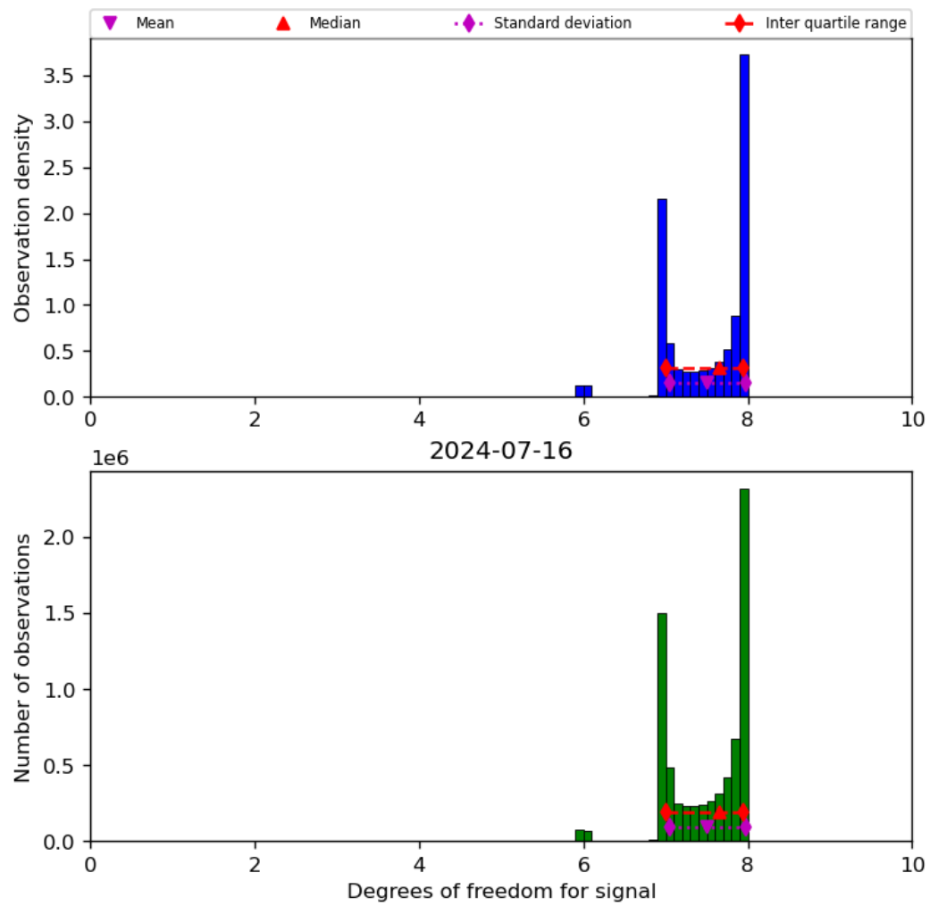
Figure 23: Histogram of “Degrees of freedom for signal” for 2024-07-15 to 2024-07-17
