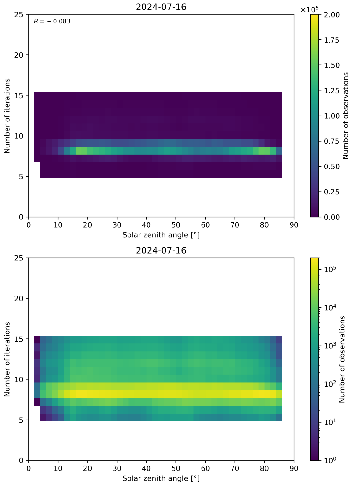
Figure 67: Scatter density plot of “Solar zenith angle” against “Number of iterations” for 2024-07-15 to 2024-07-17.
