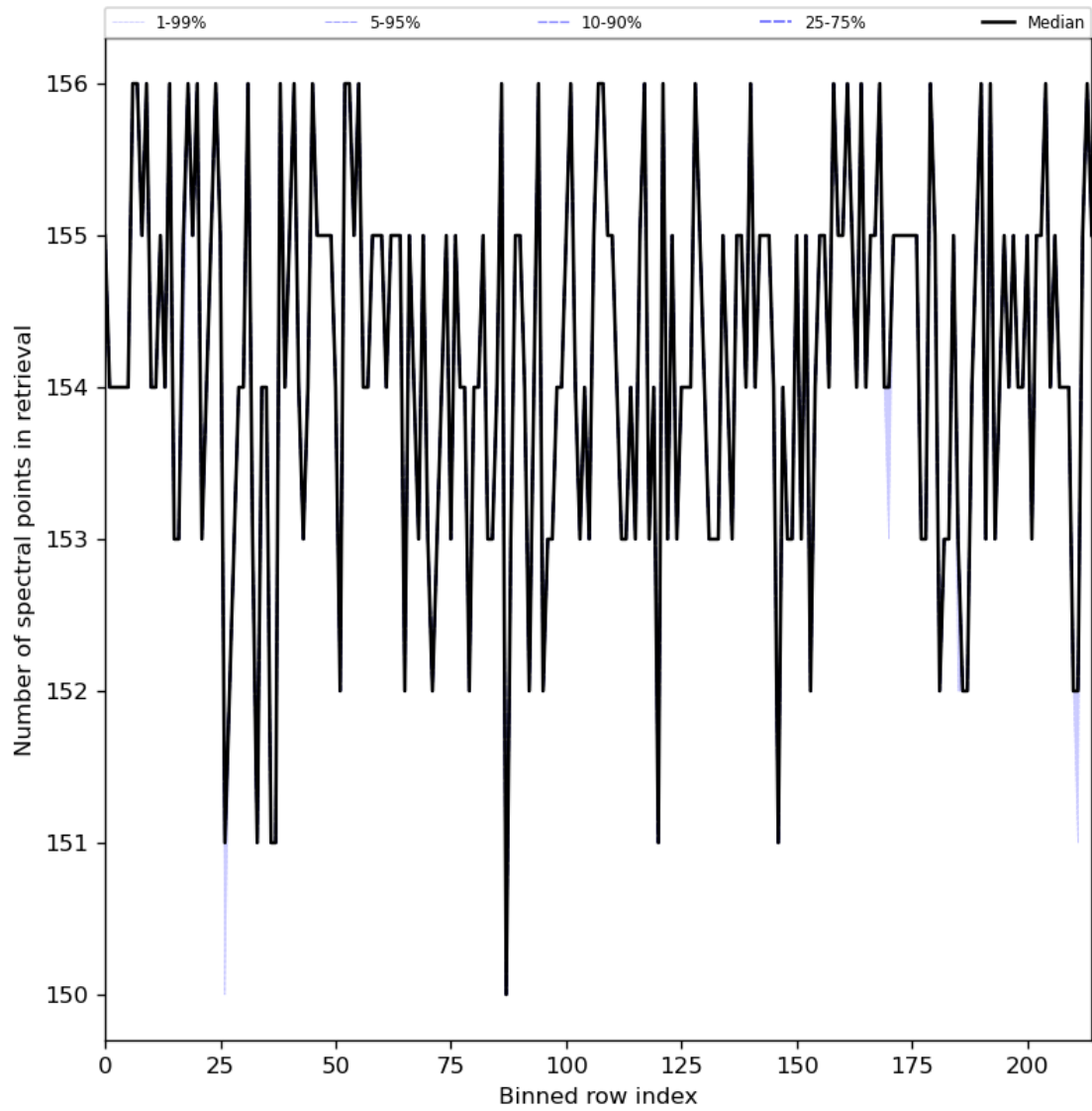
Figure 29: Along track statistics of “Number of spectral points in retrieval” for 2024-07-15 to 2024-07-17
