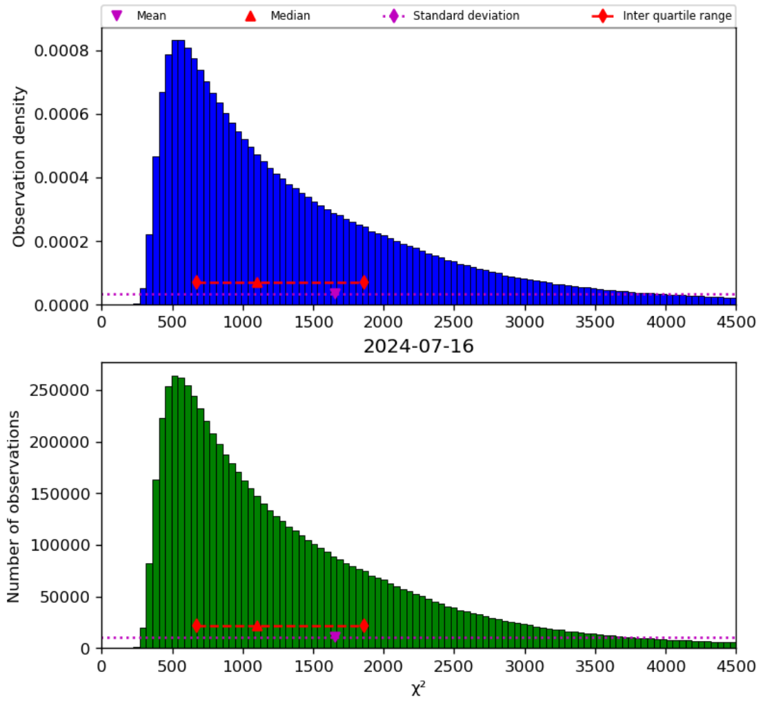
Figure 22: Histogram of “ \chi^2 ” for 2024-07-15 to 2024-07-17
