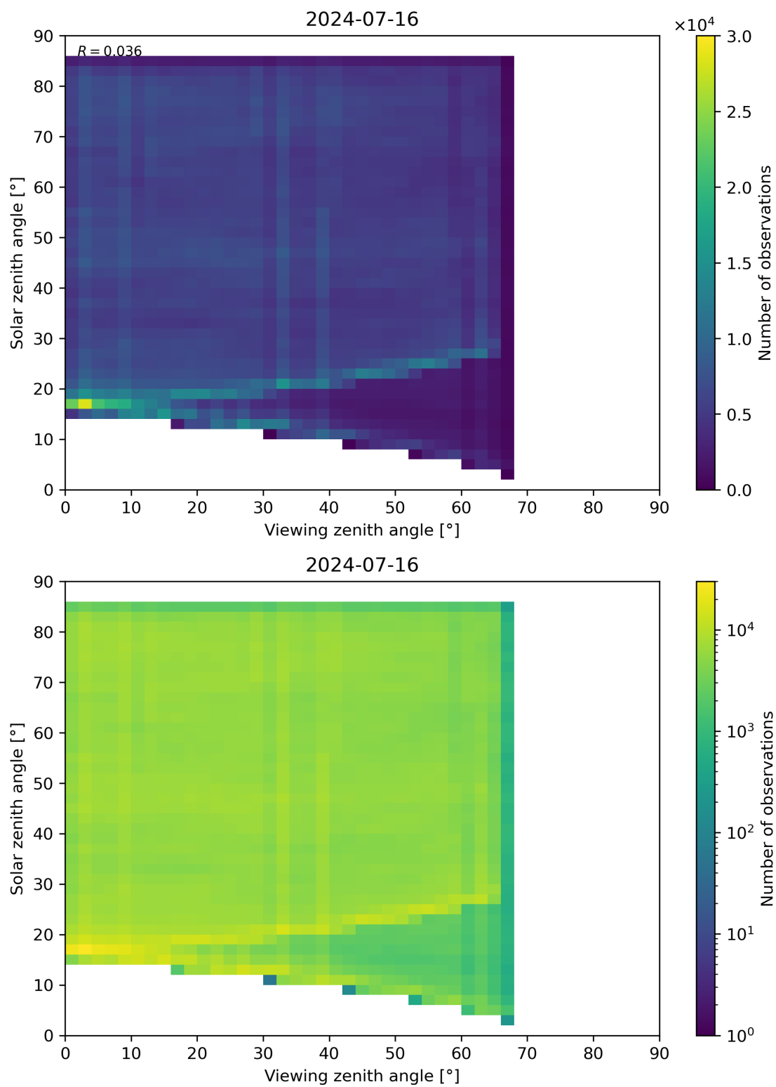
Figure 77: Scatter density plot of “Viewing zenith angle” against “Solar zenith angle” for 2024-07-15 to 2024-07-17.
