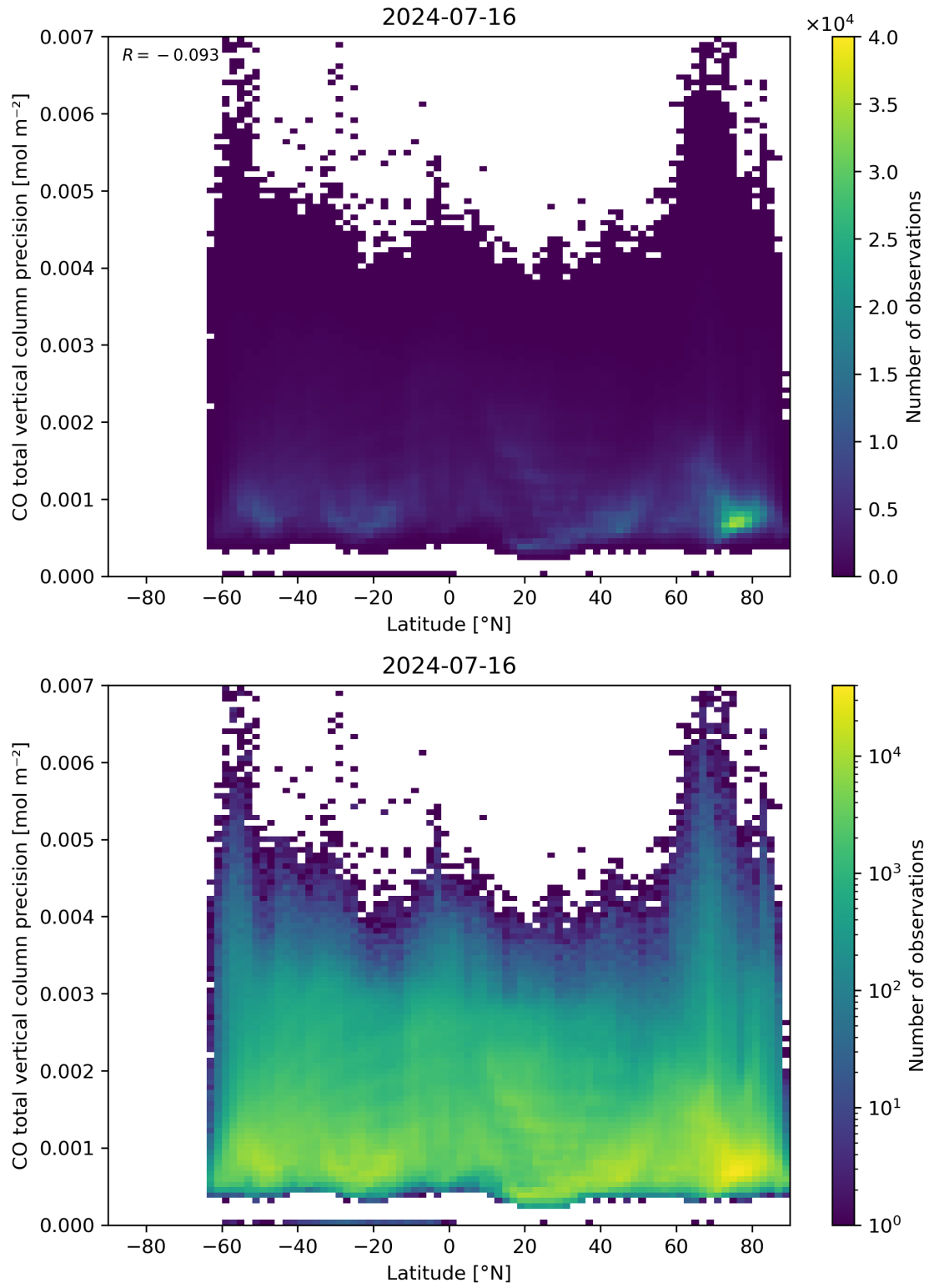
Figure 53: Scatter density plot of “Latitude” against “CO total vertical column precision” for 2024-07-15 to 2024-07-17.
