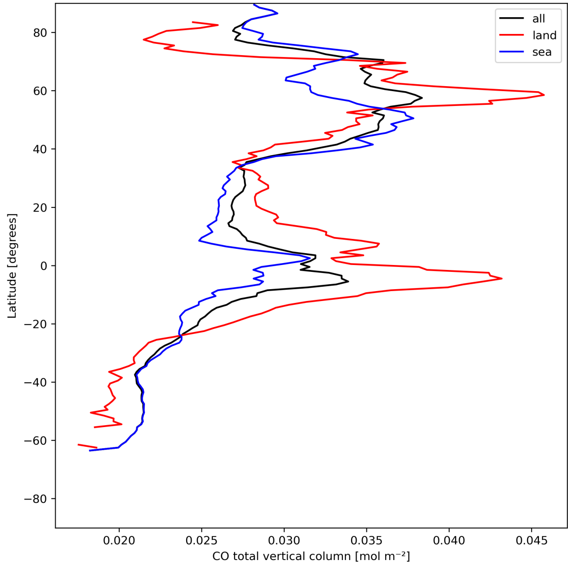
Figure 10: Zonal average of “CO total vertical column” for 2024-07-15 to 2024-07-17.
