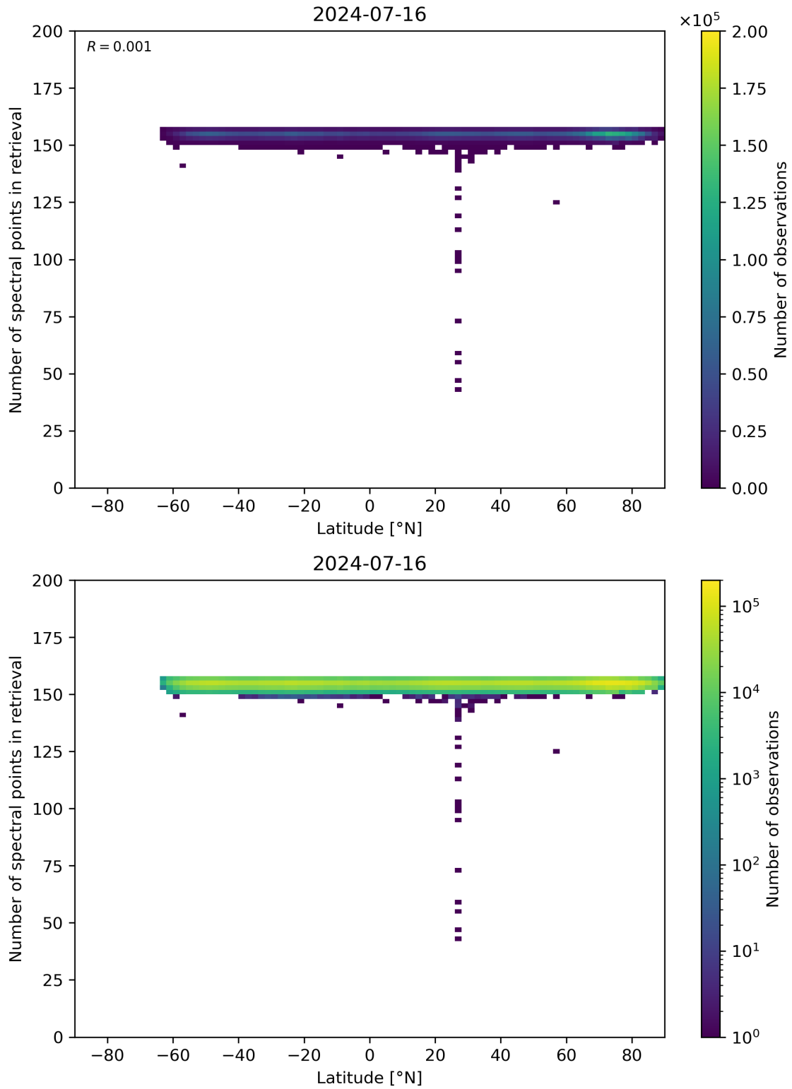
Figure 57: Scatter density plot of “Latitude” against “Number of spectral points in retrieval” for 2024-07-15 to 2024-07-17.
