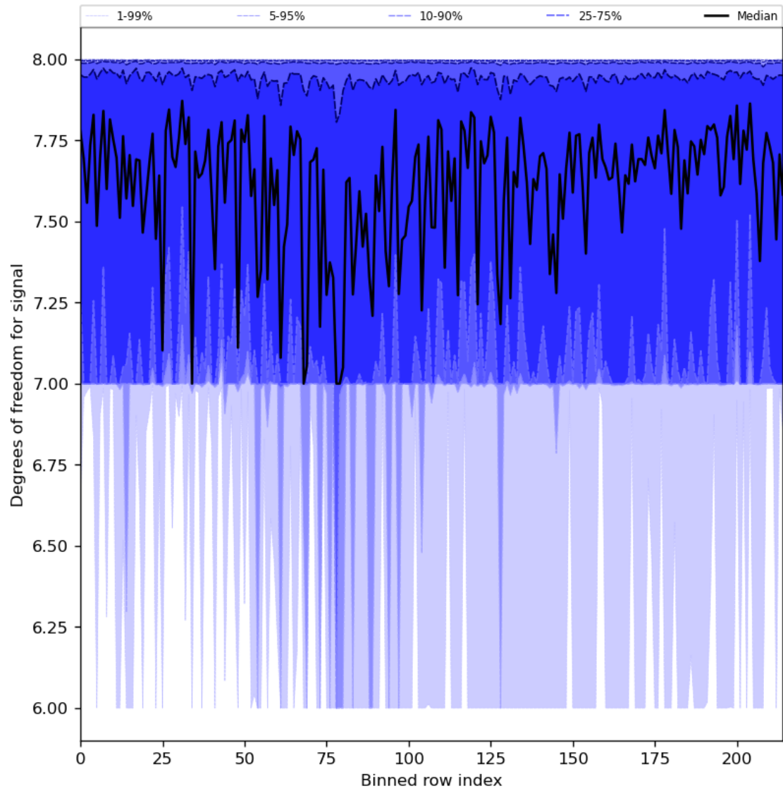
Figure 31: Along track statistics of “Degrees of freedom for signal” for 2024-07-15 to 2024-07-17
