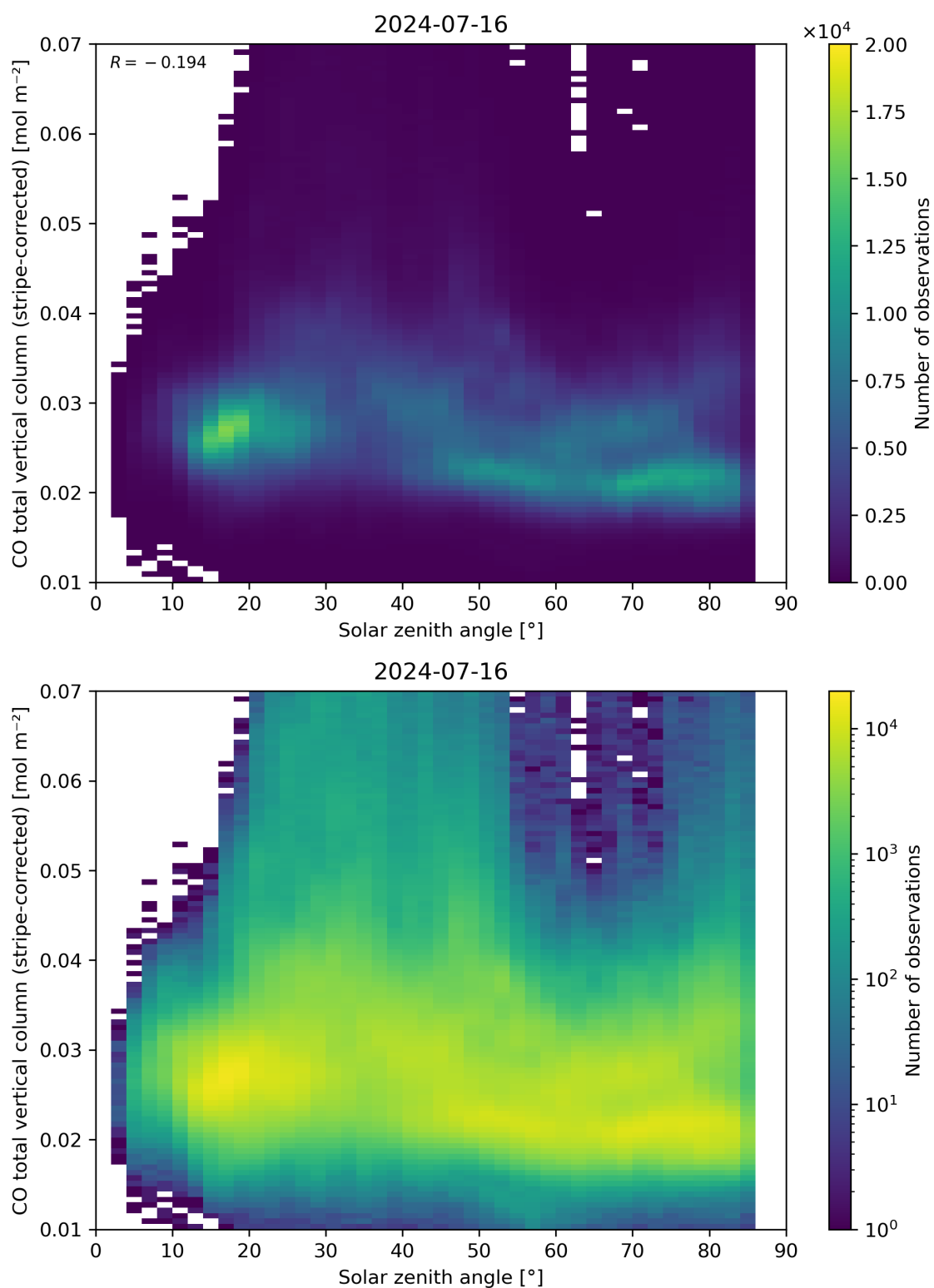
Figure 62: Scatter density plot of “Solar zenith angle” against “CO total vertical column (stripe-corrected)” for 2024-07-15 to 2024-07-17.
