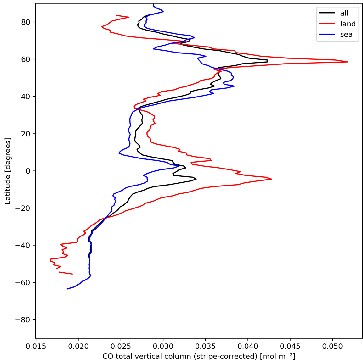
Figure 11: Zonal average of “CO total vertical column (stripe-corrected)” for 2024-07-16 to 2024-07-18.
