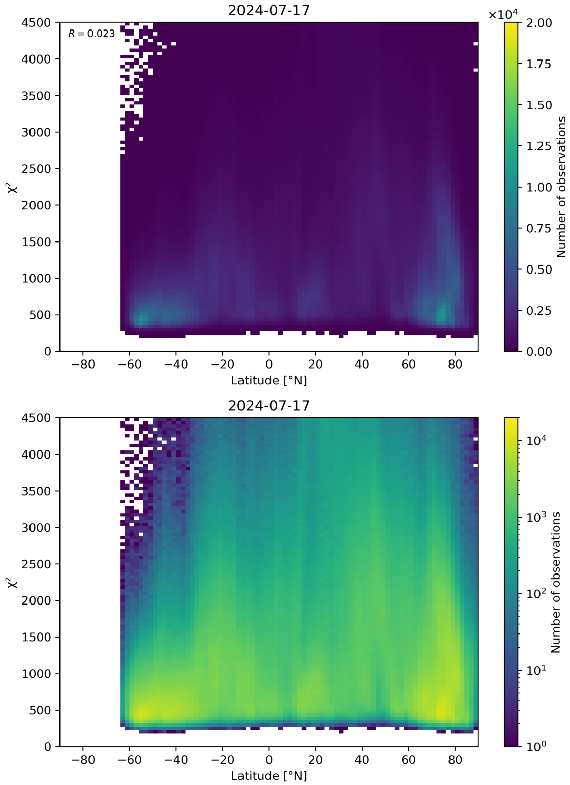
Figure 54: Scatter density plot of “Latitude” against “ \chi^2 ” for 2024-07-16 to 2024-07-18.
