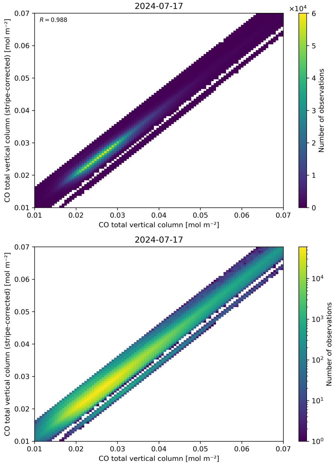
Figure 33: Scatter density plot of “CO total vertical column” against “CO total vertical column (stripe-corrected)” for 2024-07-16 to 2024-07-18.
