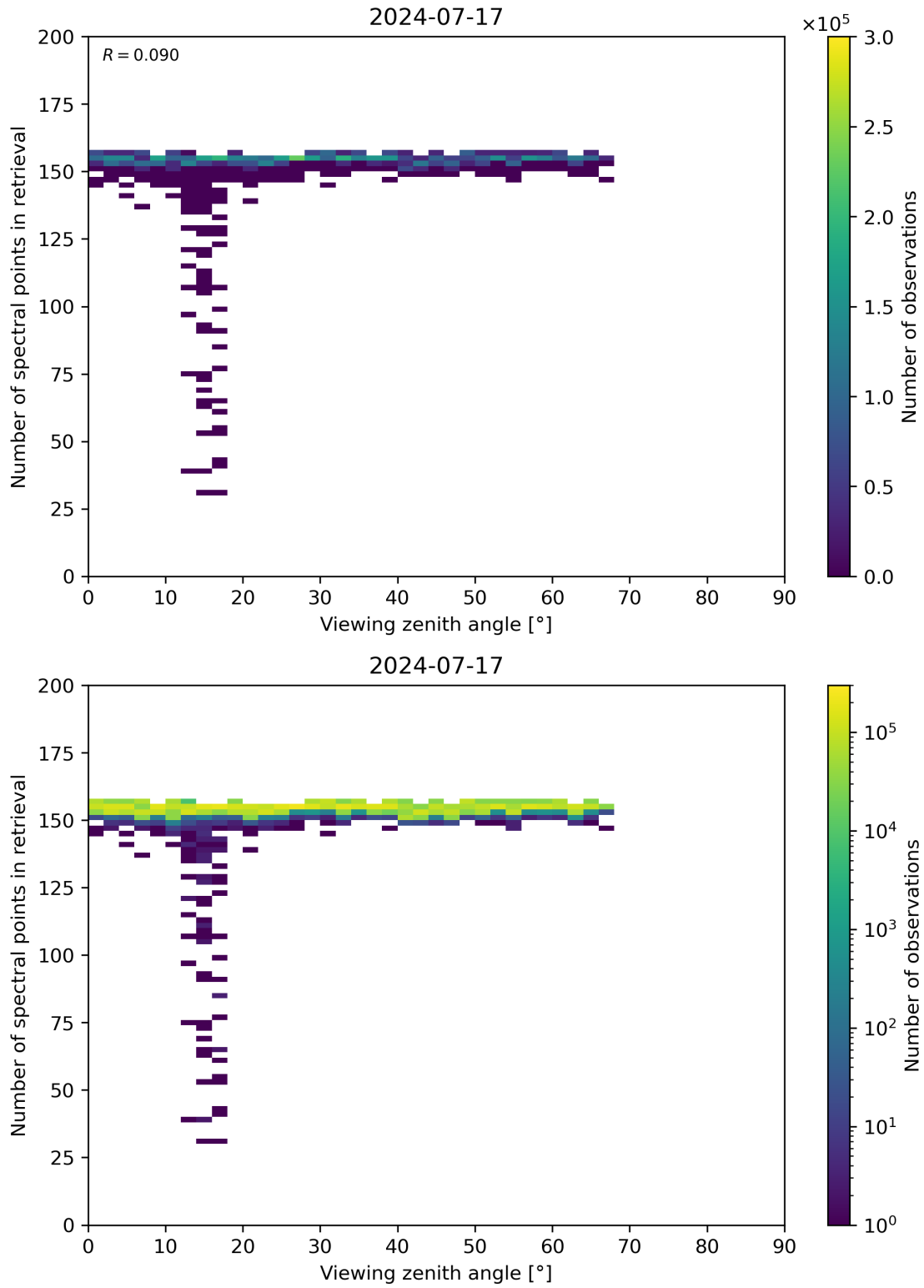
Figure 76: Scatter density plot of “Viewing zenith angle” against “Number of spectral points in retrieval” for 2024-07-16 to 2024-07-18.
