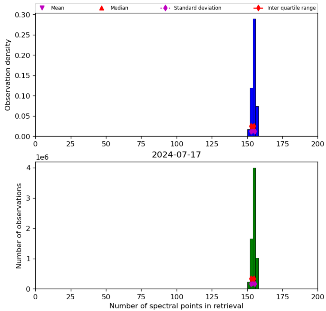
Figure 21: Histogram of “Number of spectral points in retrieval” for 2024-07-16 to 2024-07-18
