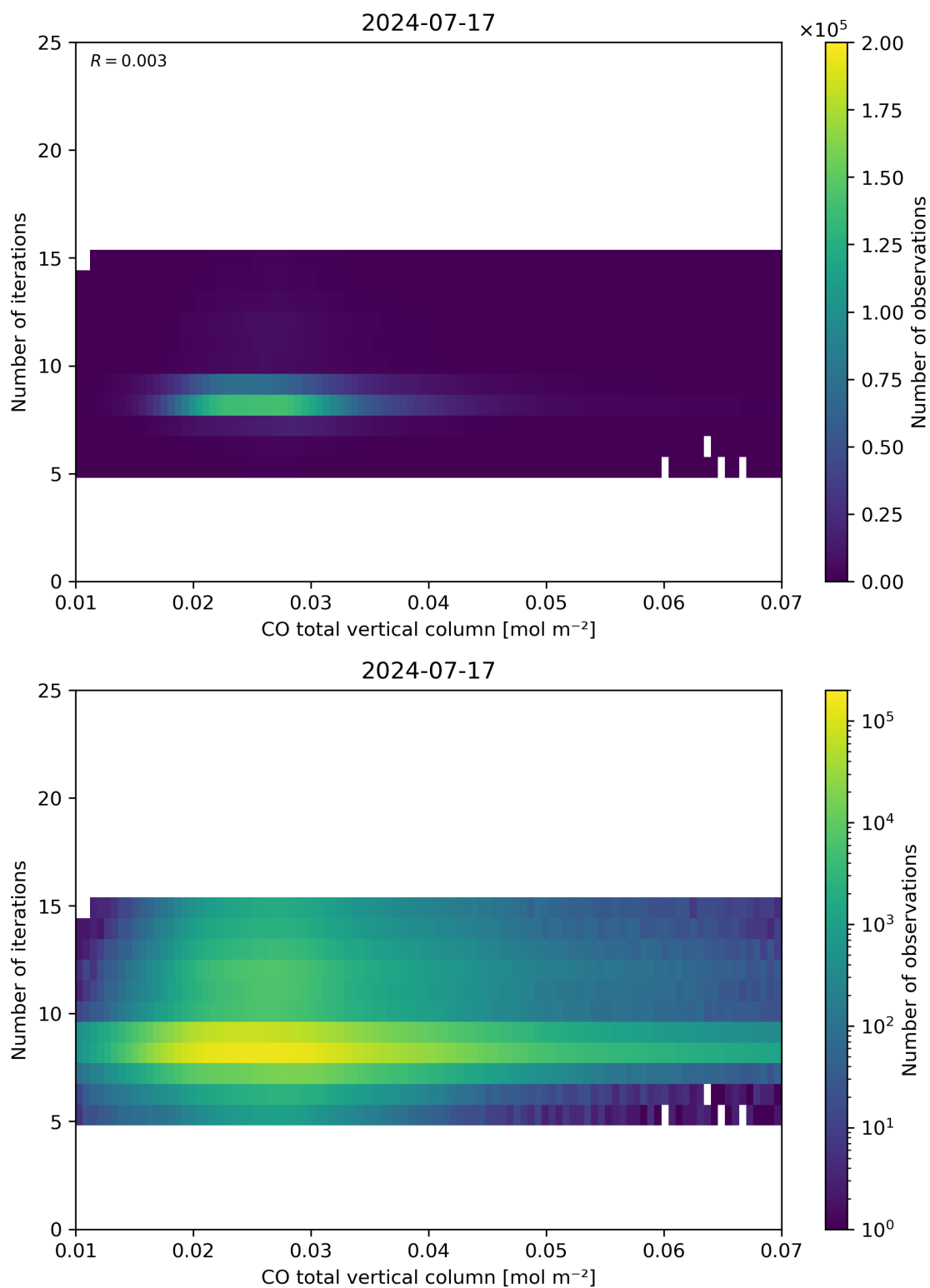
Figure 42: Scatter density plot of “CO total vertical column” against “Number of iterations” for 2024-07-16 to 2024-07-18.
