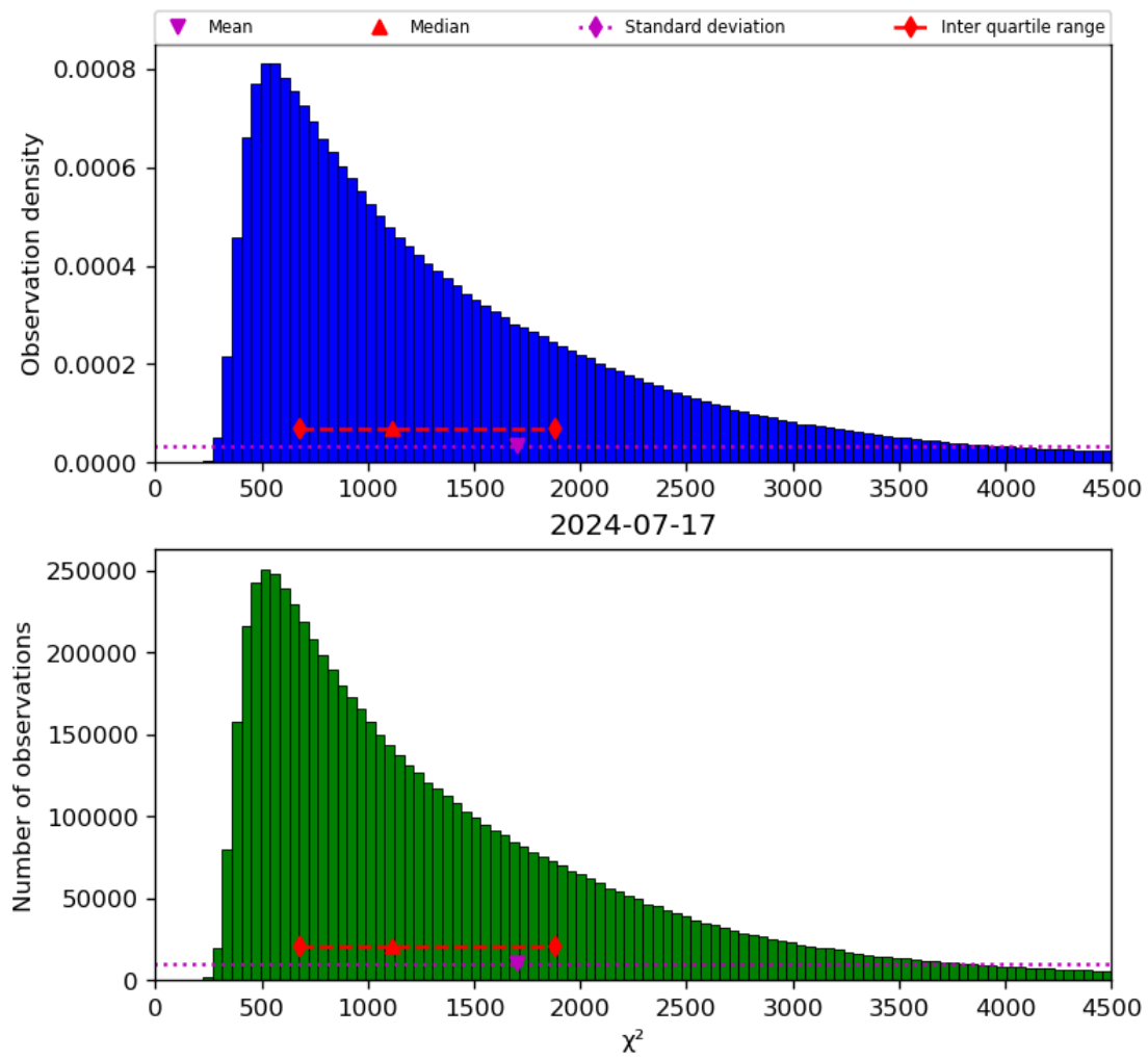
Figure 22: Histogram of “ \chi^2 ” for 2024-07-16 to 2024-07-18
