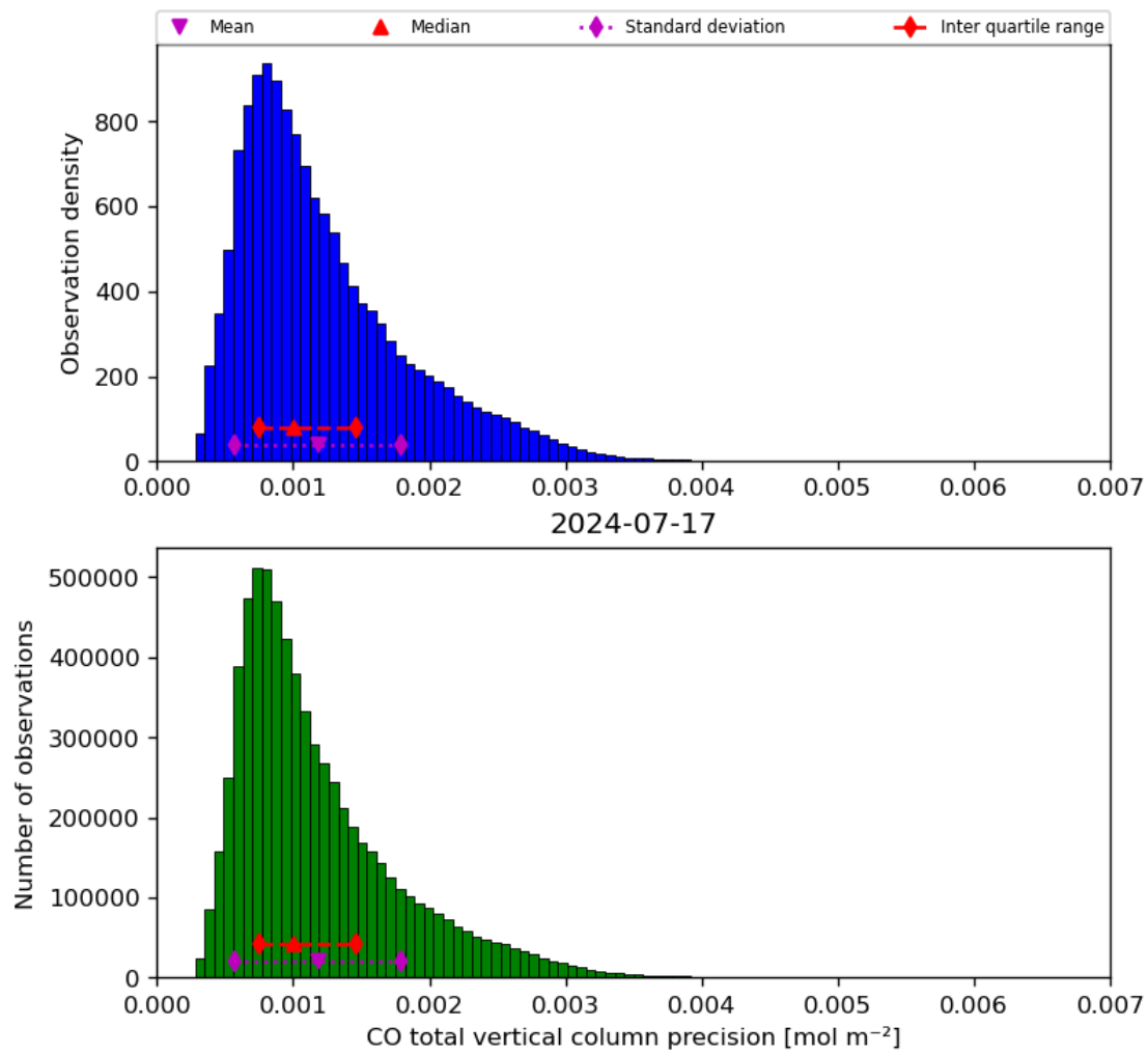
Figure 20: Histogram of “CO total vertical column precision” for 2024-07-16 to 2024-07-18
