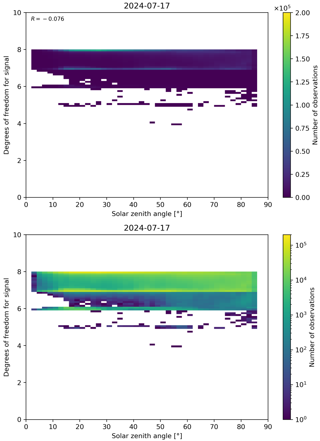
Figure 65: Scatter density plot of “Solar zenith angle” against “Degrees of freedom for signal” for 2024-07-16 to 2024-07-18.
