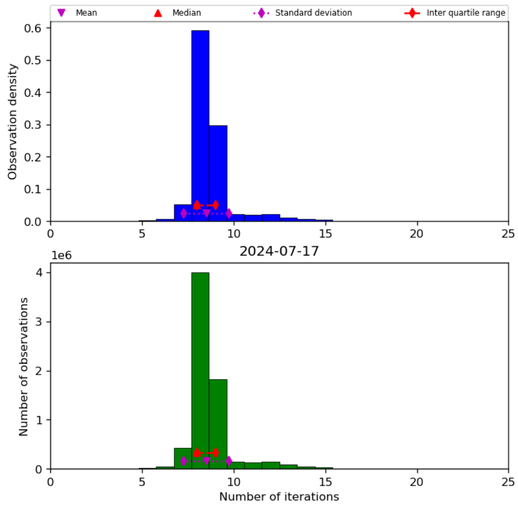
Figure 24: Histogram of “Number of iterations” for 2024-07-16 to 2024-07-18
