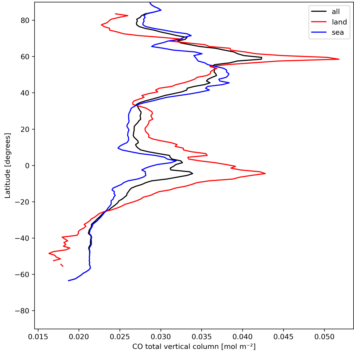
Figure 10: Zonal average of “CO total vertical column” for 2024-07-16 to 2024-07-18.
