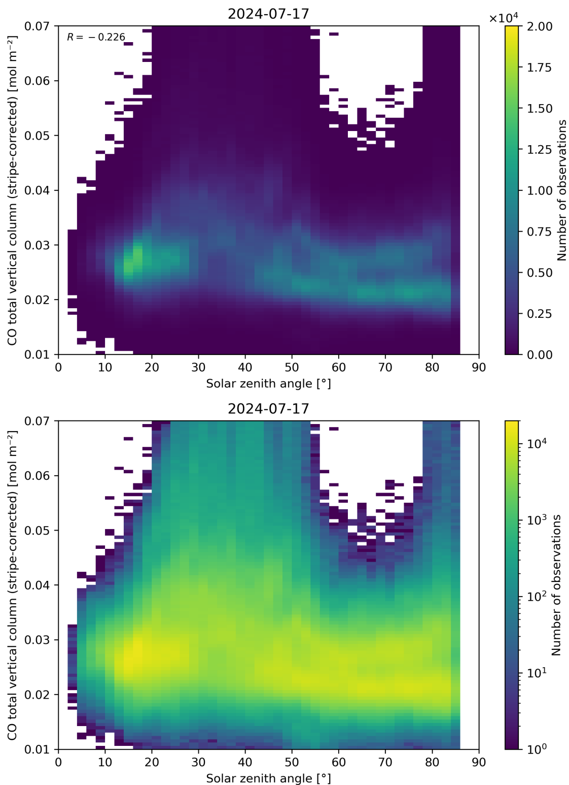
Figure 62: Scatter density plot of “Solar zenith angle” against “CO total vertical column (stripe-corrected)” for 2024-07-16 to 2024-07-18.
