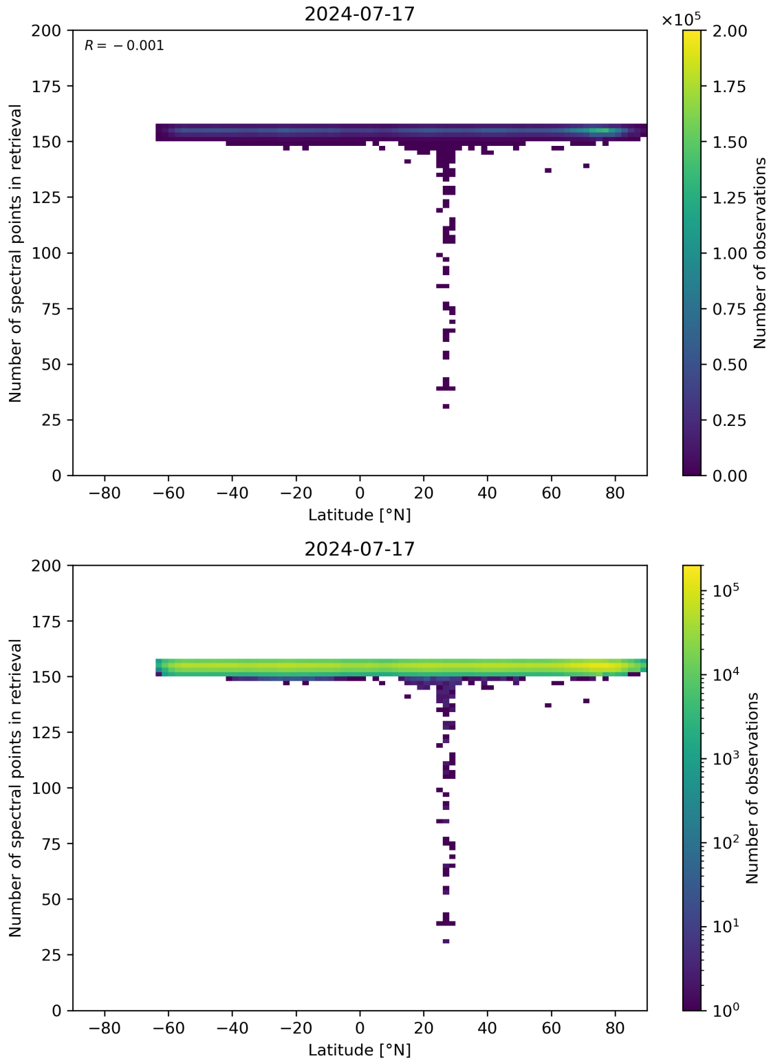
Figure 57: Scatter density plot of “Latitude” against “Number of spectral points in retrieval” for 2024-07-16 to 2024-07-18.
