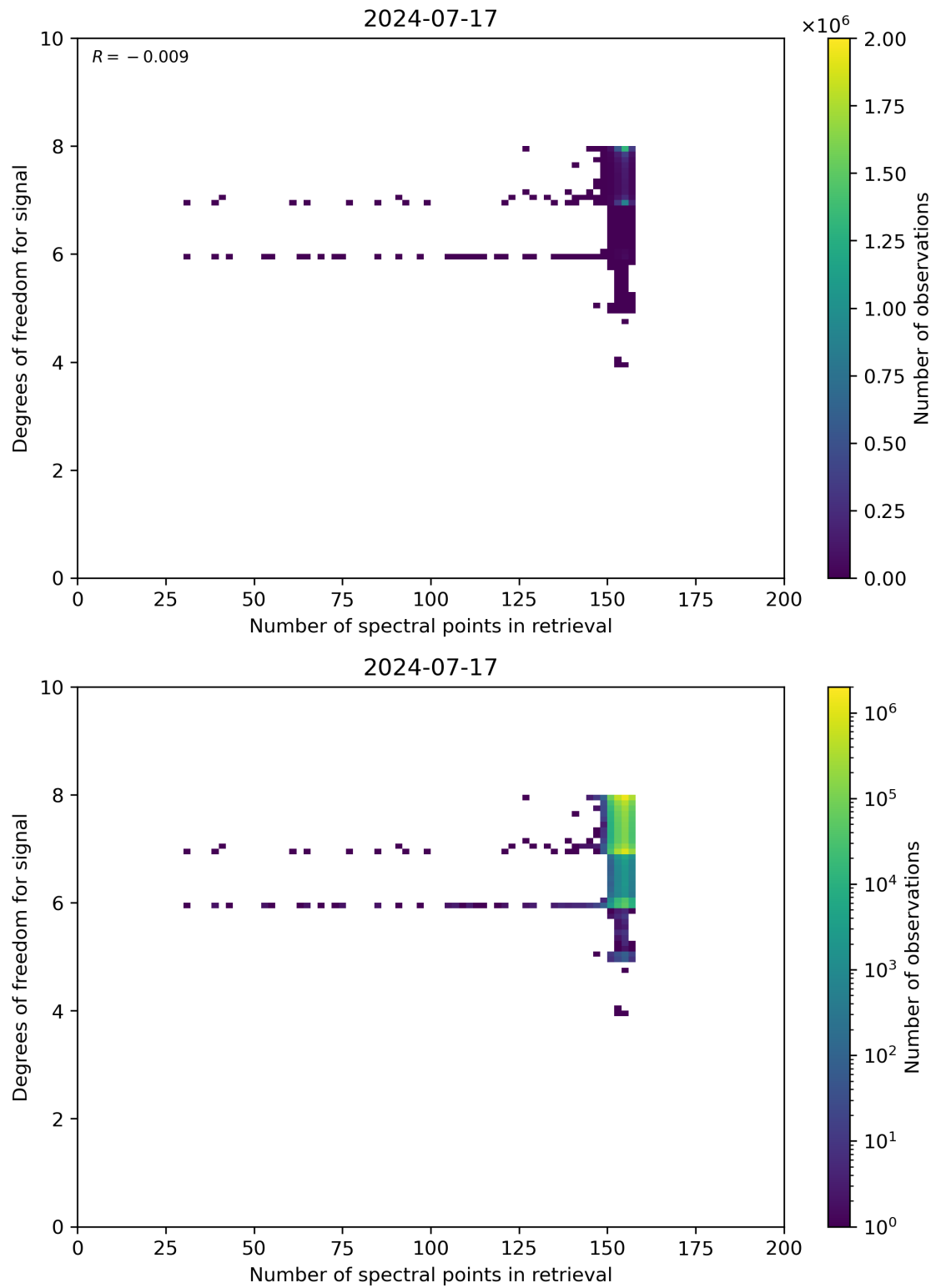
Figure 59: Scatter density plot of “Number of spectral points in retrieval” against “Degrees of freedom for signal” for 2024-07-16 to 2024-07-18.
