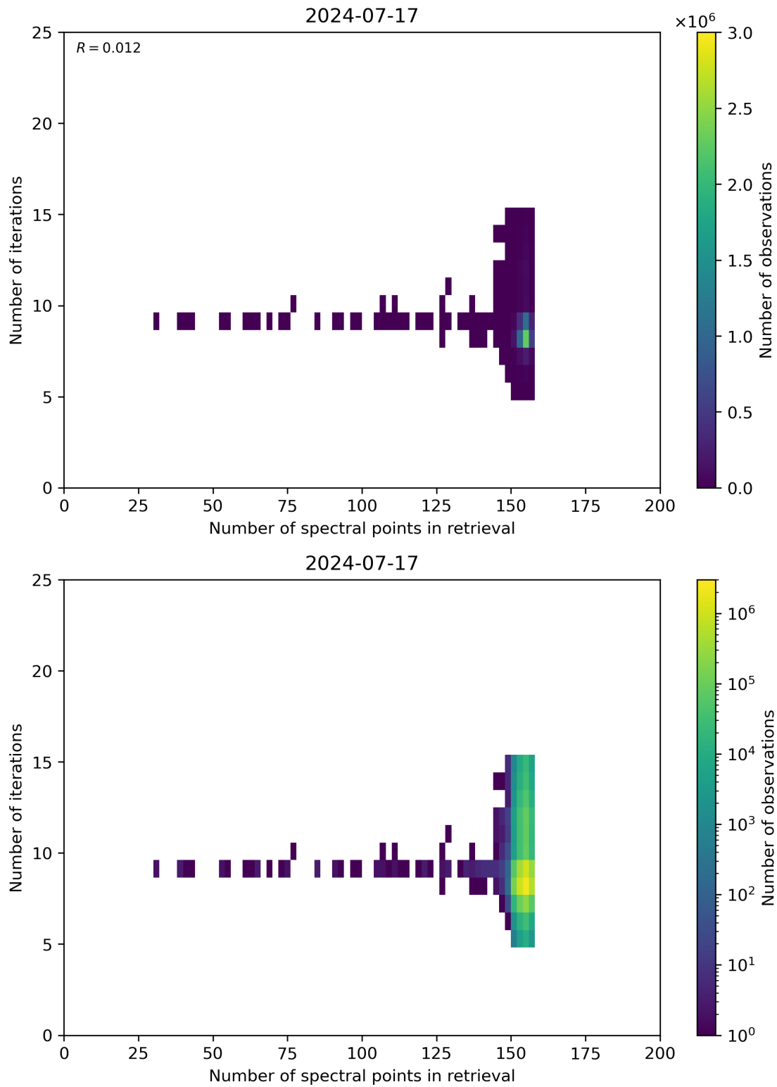
Figure 60: Scatter density plot of “Number of spectral points in retrieval” against “Number of iterations” for 2024-07-16 to 2024-07-18.
