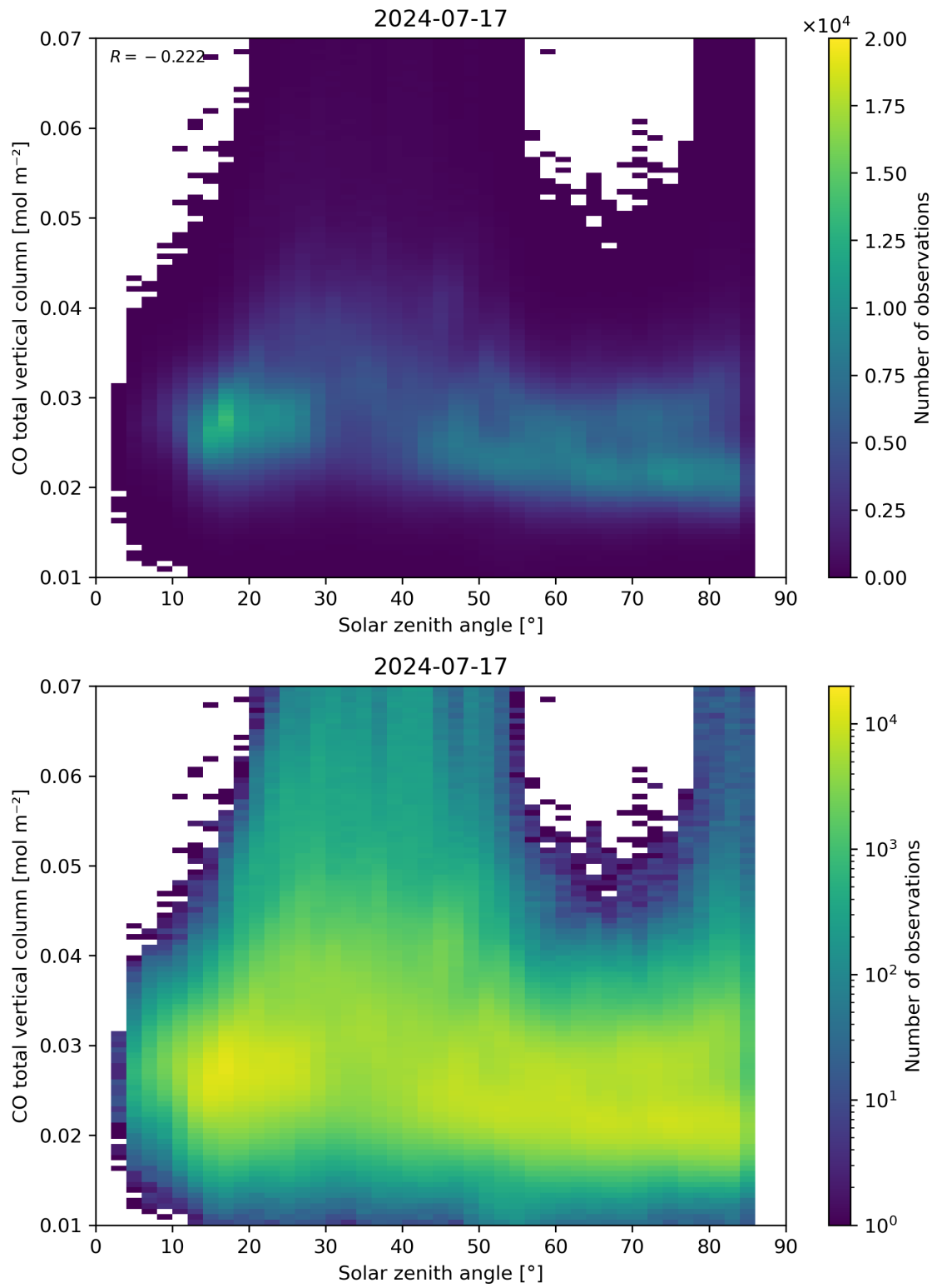
Figure 61: Scatter density plot of “Solar zenith angle” against “CO total vertical column” for 2024-07-16 to 2024-07-18.
