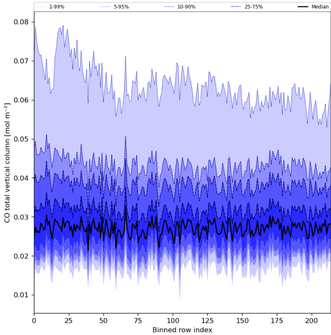
Figure 26: Along track statistics of “CO total vertical column” for 2024-07-16 to 2024-07-18
