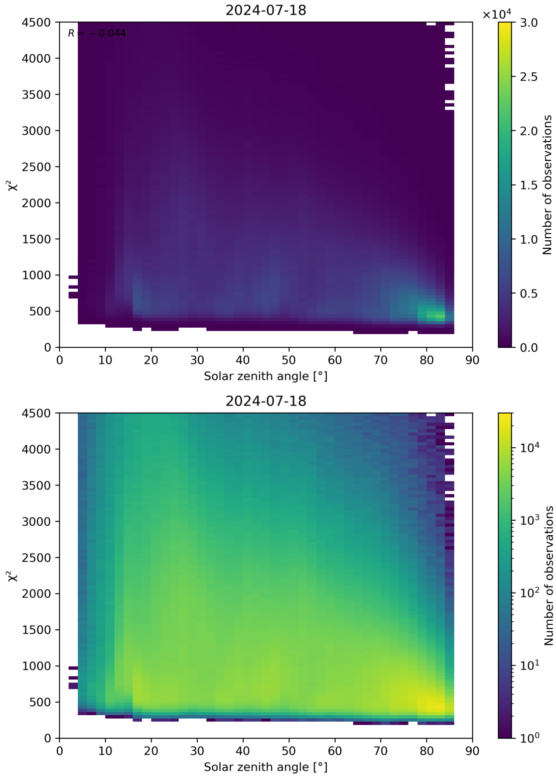
Figure 64: Scatter density plot of “Solar zenith angle” against “ \chi^2 ” for 2024-07-17 to 2024-07-19.
