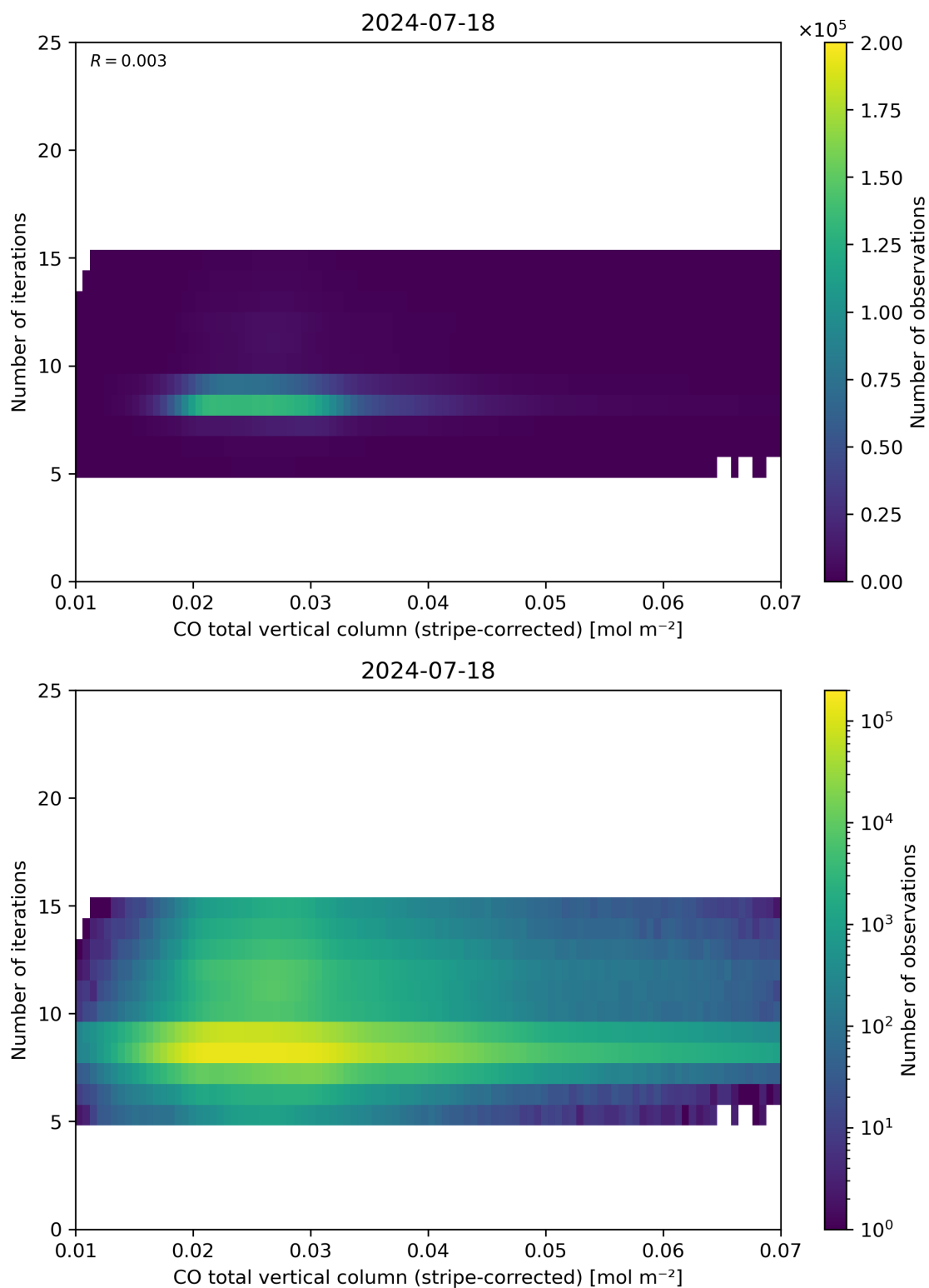
Figure 39: Scatter density plot of “CO total vertical column (stripe-corrected)” against “Number of iterations” for 2024-07-17 to 2024-07-19.
