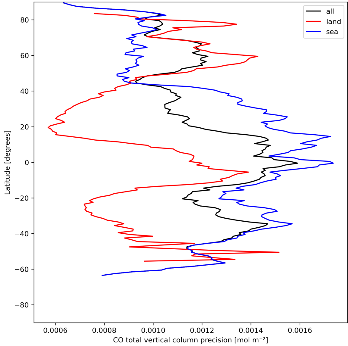
Figure 12: Zonal average of “CO total vertical column precision” for 2024-07-17 to 2024-07-19.
