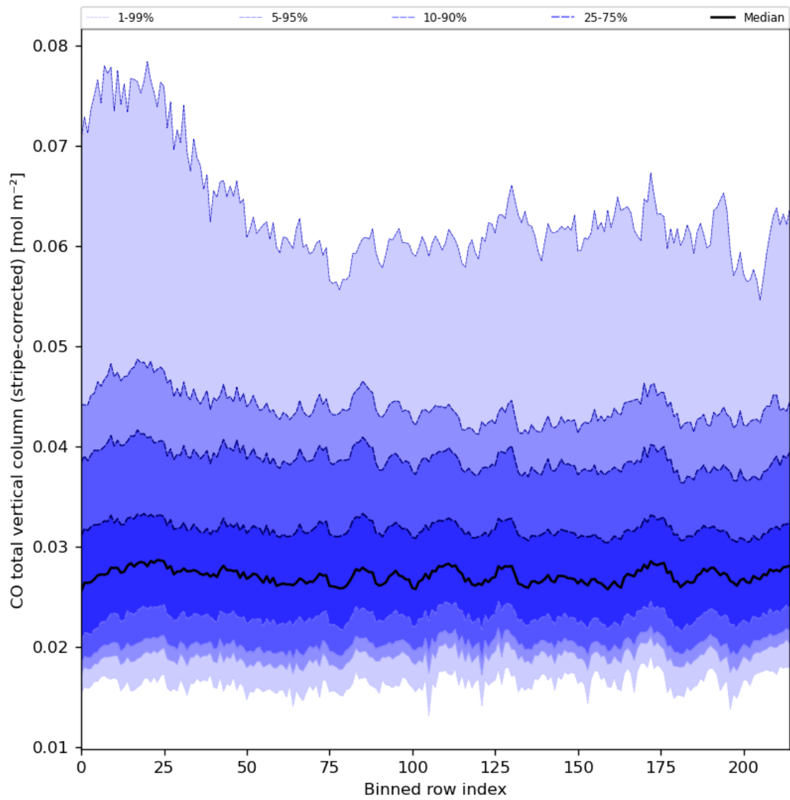
Figure 27: Along track statistics of “CO total vertical column (stripe-corrected)” for 2024-07-17 to 2024-07-19
