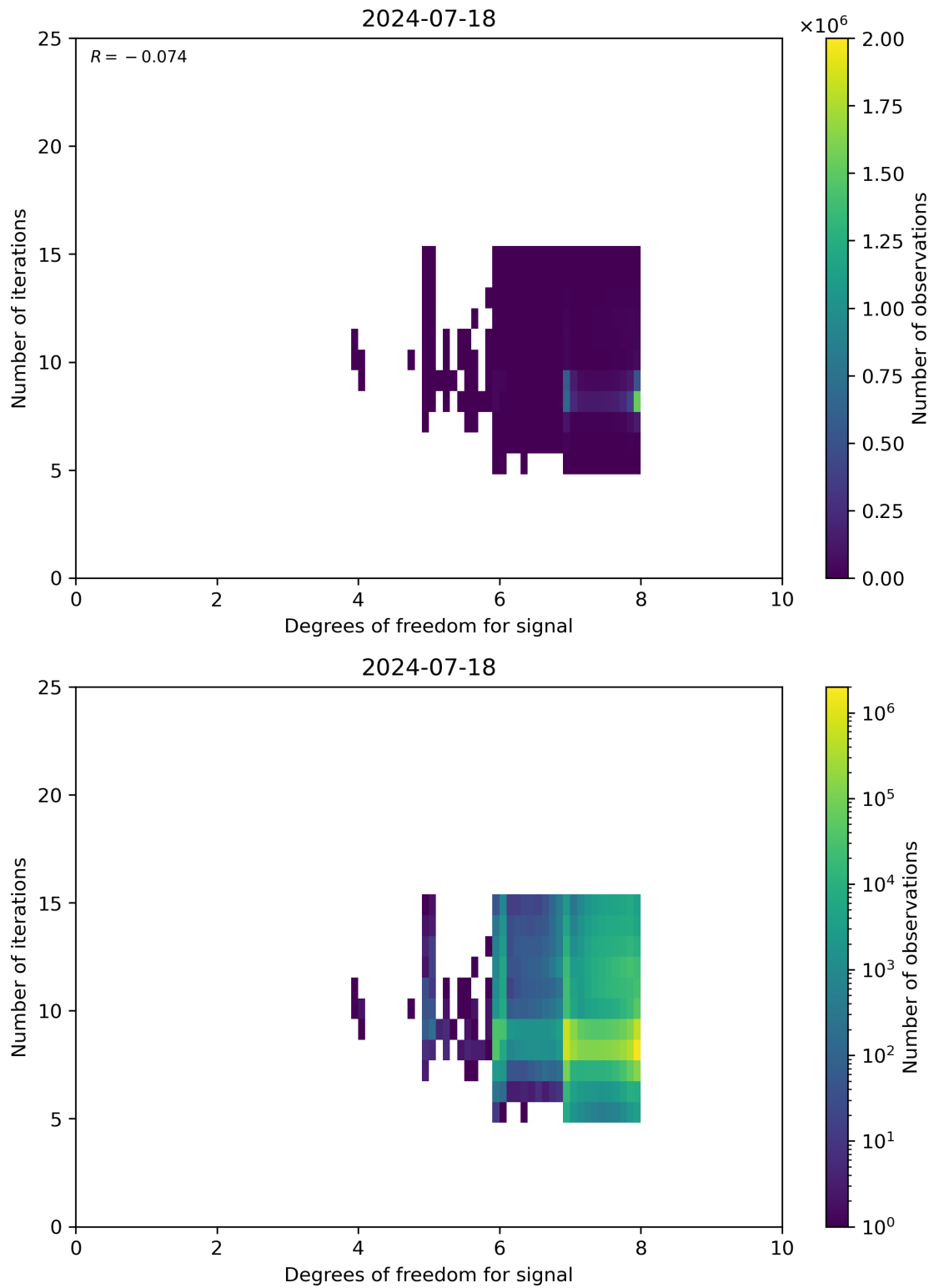
Figure 50: Scatter density plot of “Degrees of freedom for signal” against “Number of iterations” for 2024-07-17 to 2024-07-19.
