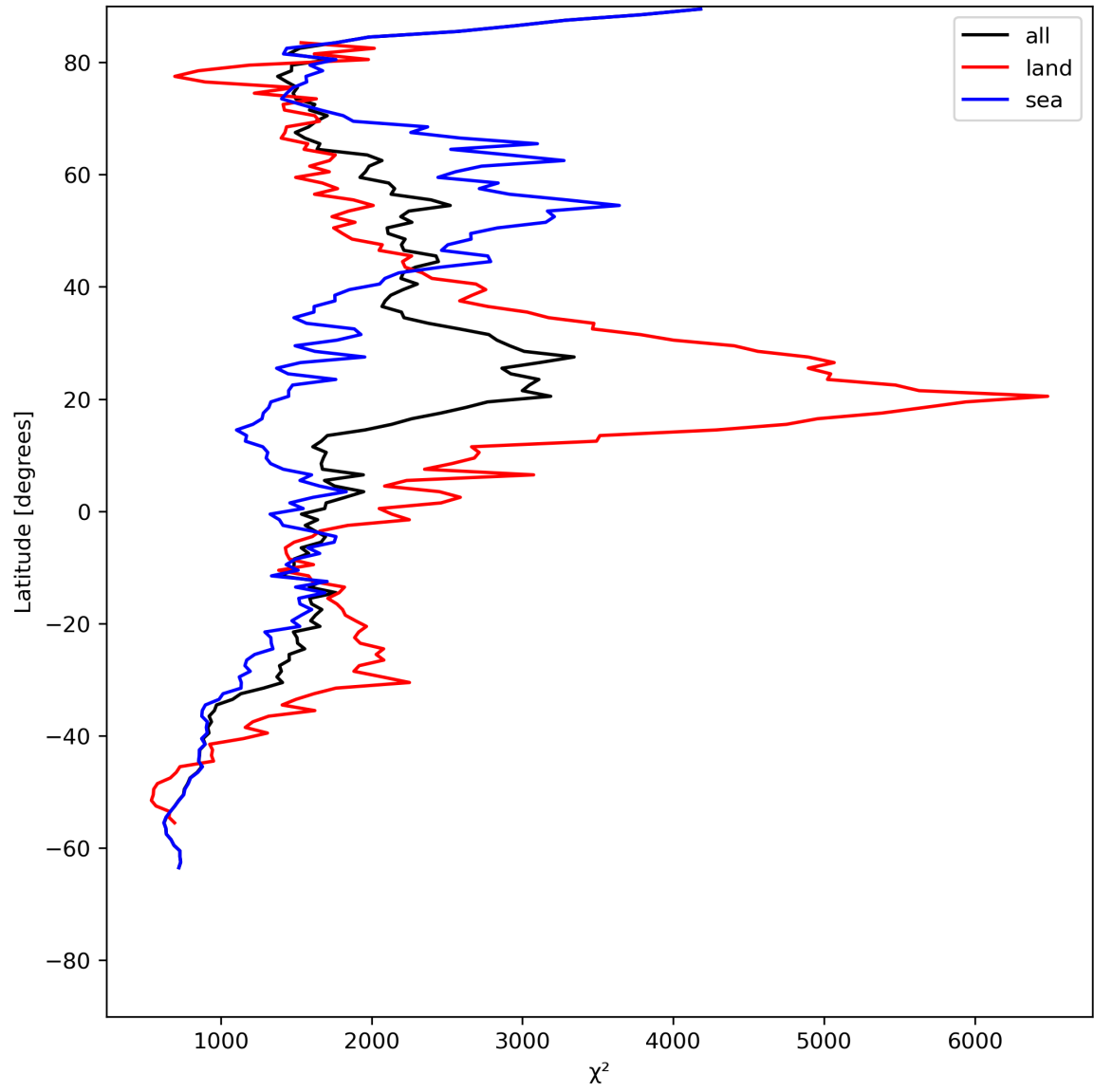
Figure 14: Zonal average of “ \chi^2 ” for 2024-07-17 to 2024-07-19.
