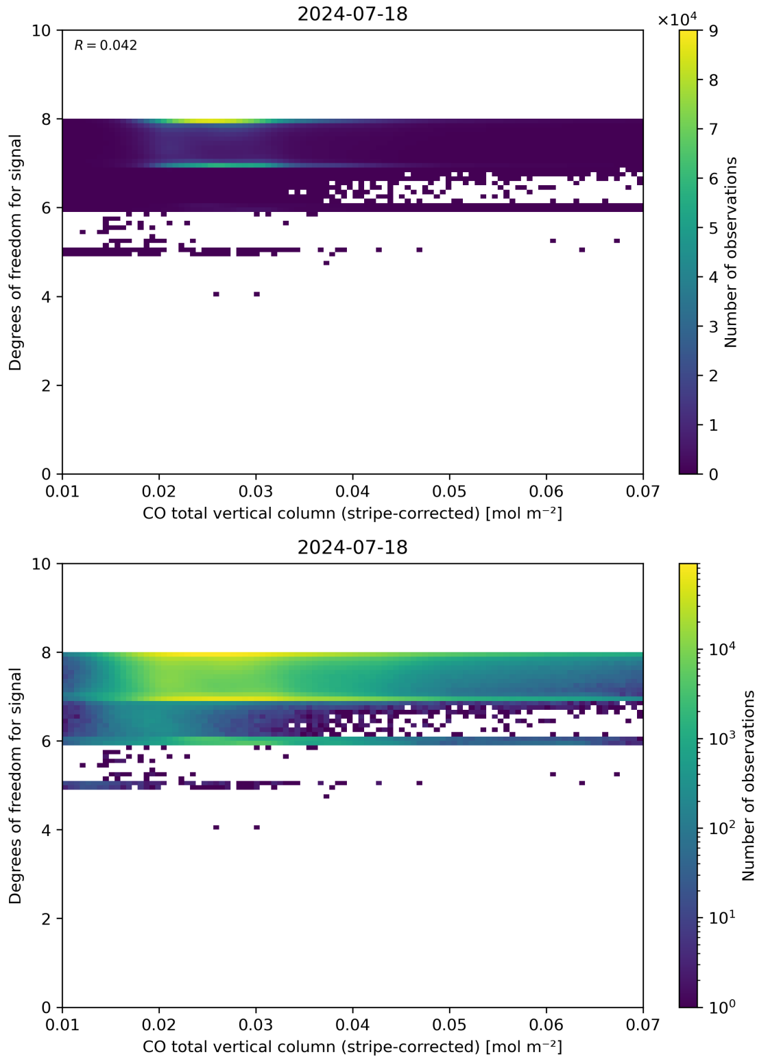
Figure 38: Scatter density plot of “CO total vertical column (stripe-corrected)” against “Degrees of freedom for signal” for 2024-07-17 to 2024-07-19.
