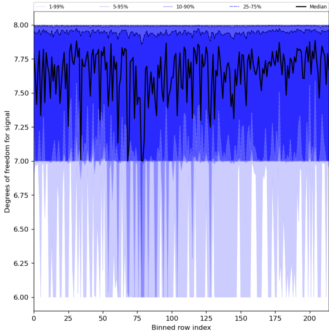
Figure 31: Along track statistics of “Degrees of freedom for signal” for 2024-07-17 to 2024-07-19
