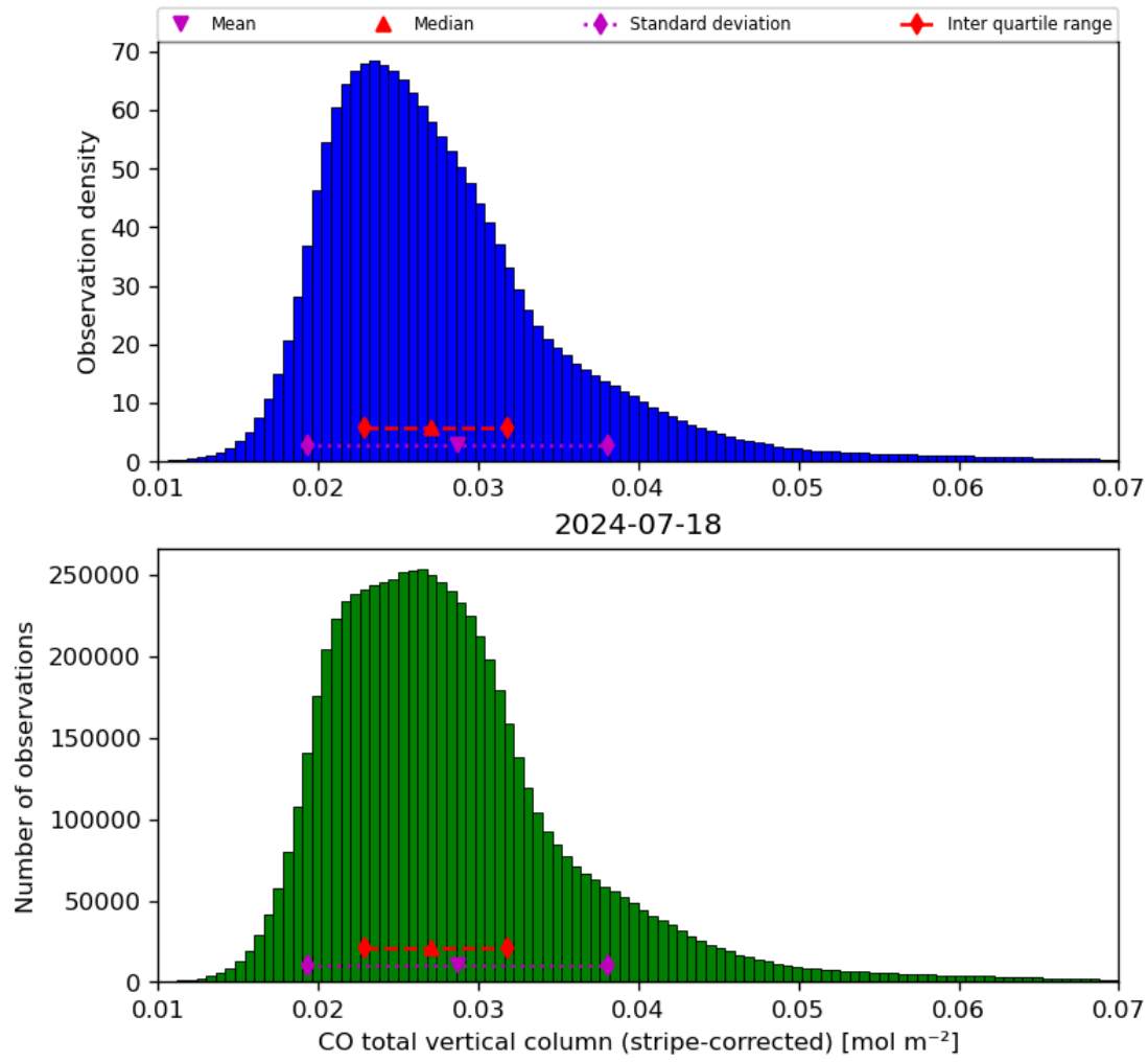
Figure 19: Histogram of “CO total vertical column (stripe-corrected)” for 2024-07-17 to 2024-07-19
