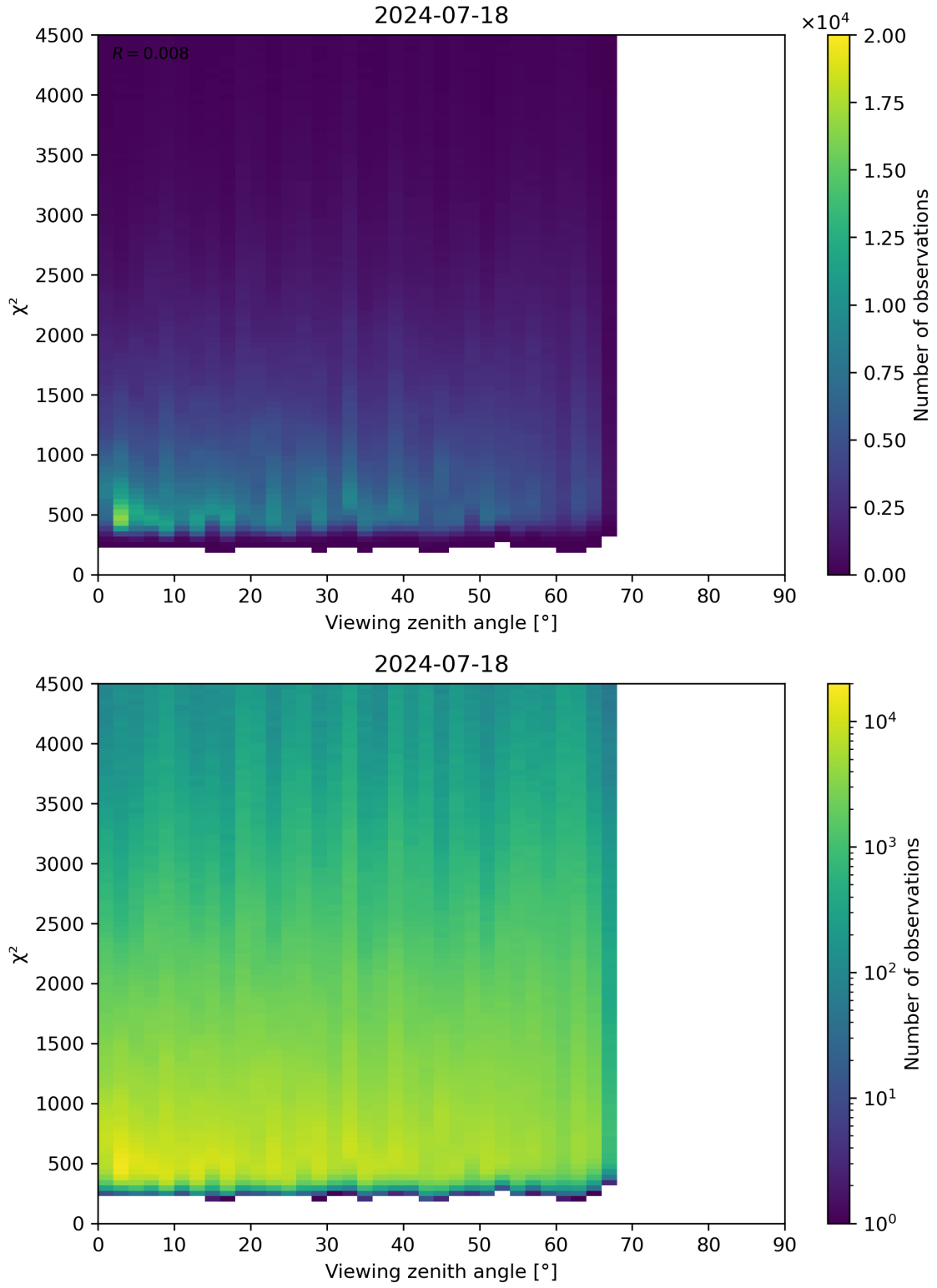
Figure 72: Scatter density plot of “Viewing zenith angle” against “ \chi^2 ” for 2024-07-17 to 2024-07-19.
