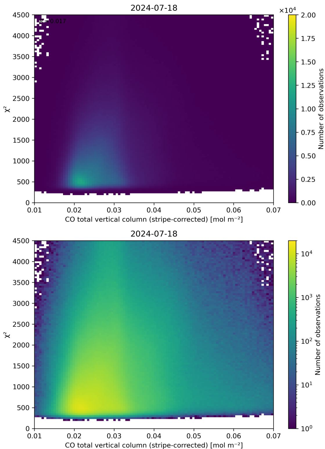
Figure 37: Scatter density plot of “CO total vertical column (stripe-corrected)” against “ \chi^2 ” for 2024-07-17 to 2024-07-19.
