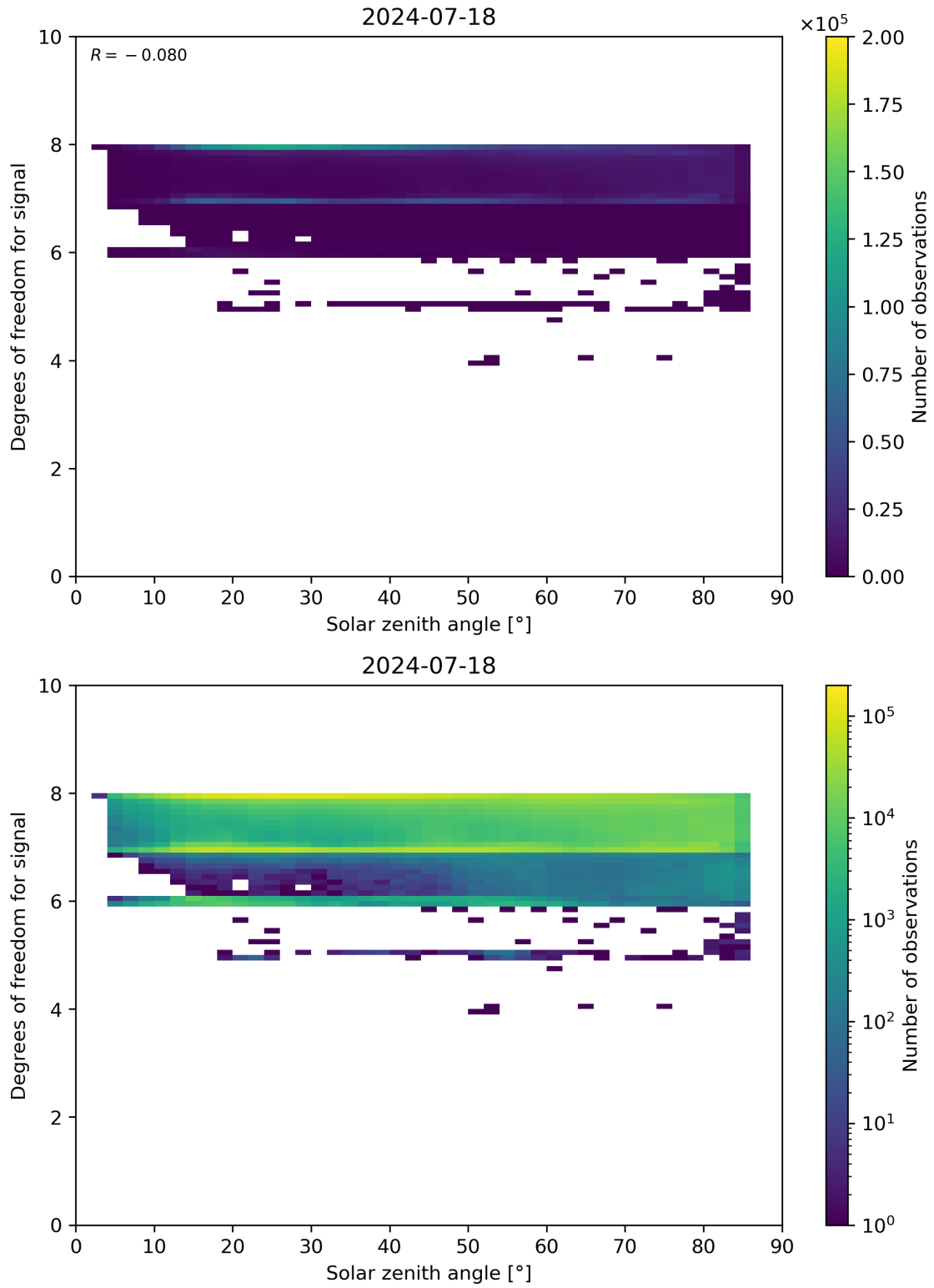
Figure 65: Scatter density plot of “Solar zenith angle” against “Degrees of freedom for signal” for 2024-07-17 to 2024-07-19.
