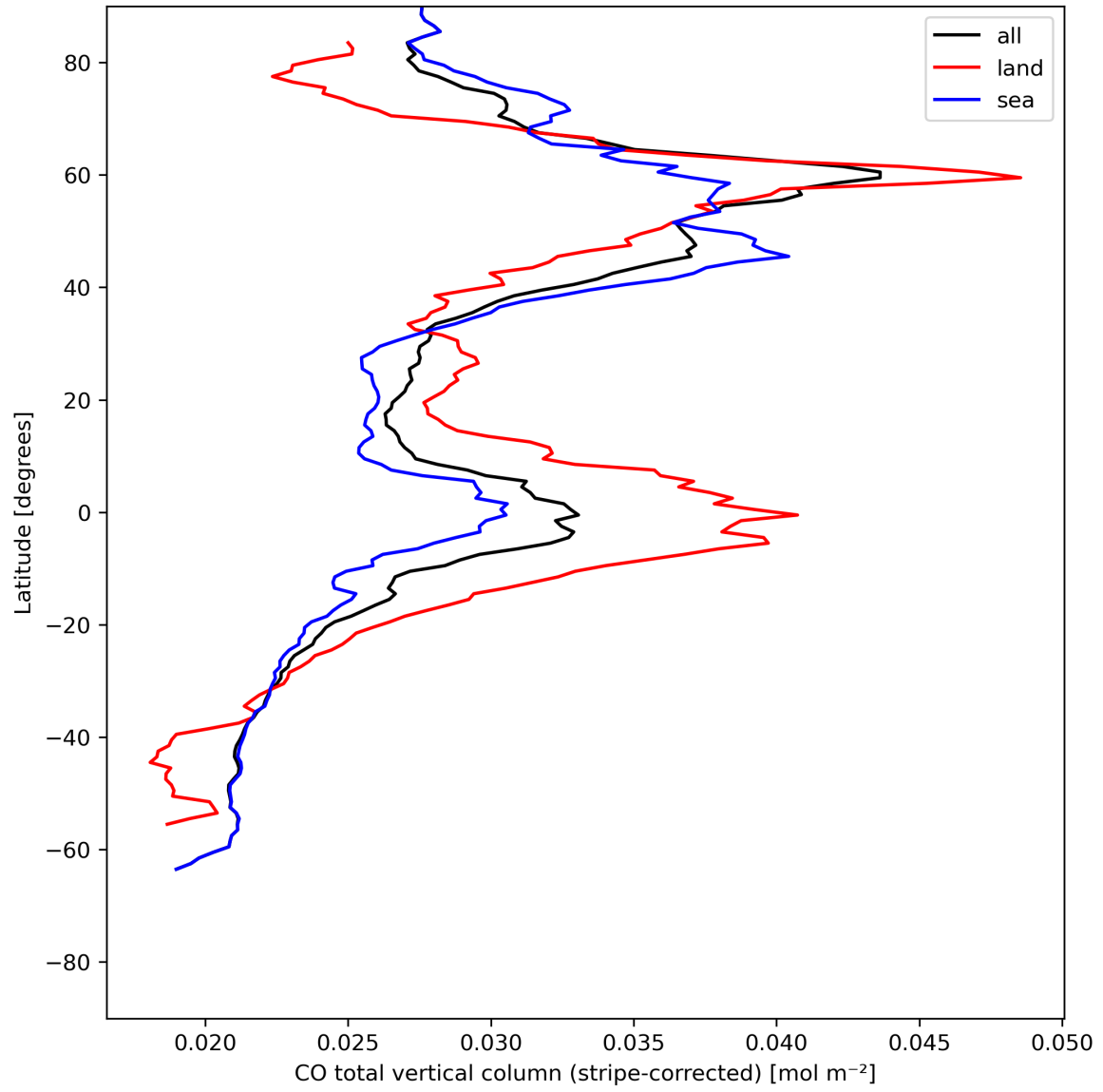
Figure 11: Zonal average of “CO total vertical column (stripe-corrected)” for 2024-07-17 to 2024-07-19.
