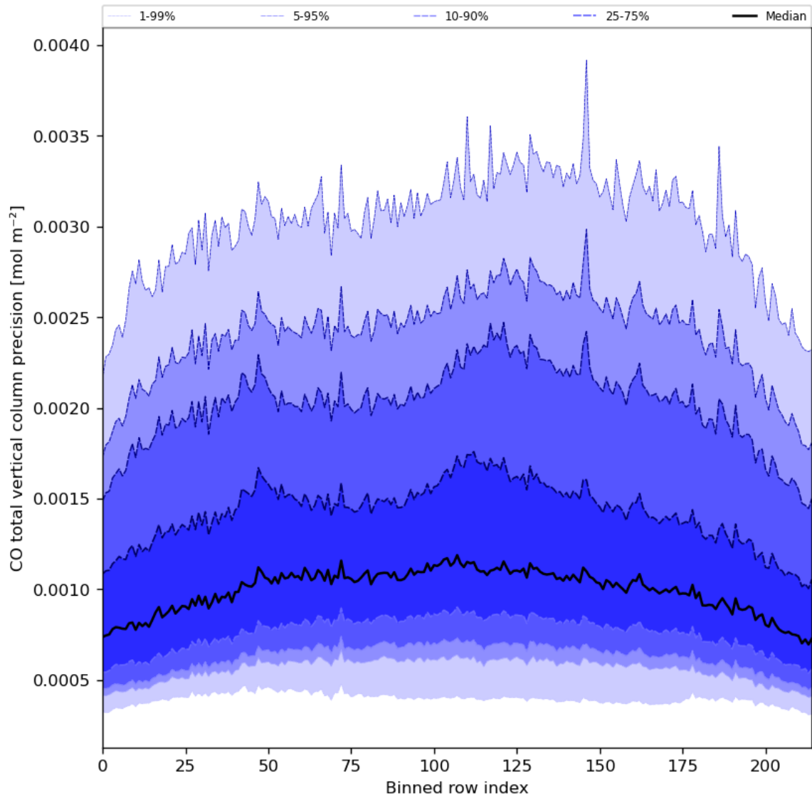
Figure 28: Along track statistics of “CO total vertical column precision” for 2024-07-17 to 2024-07-19
