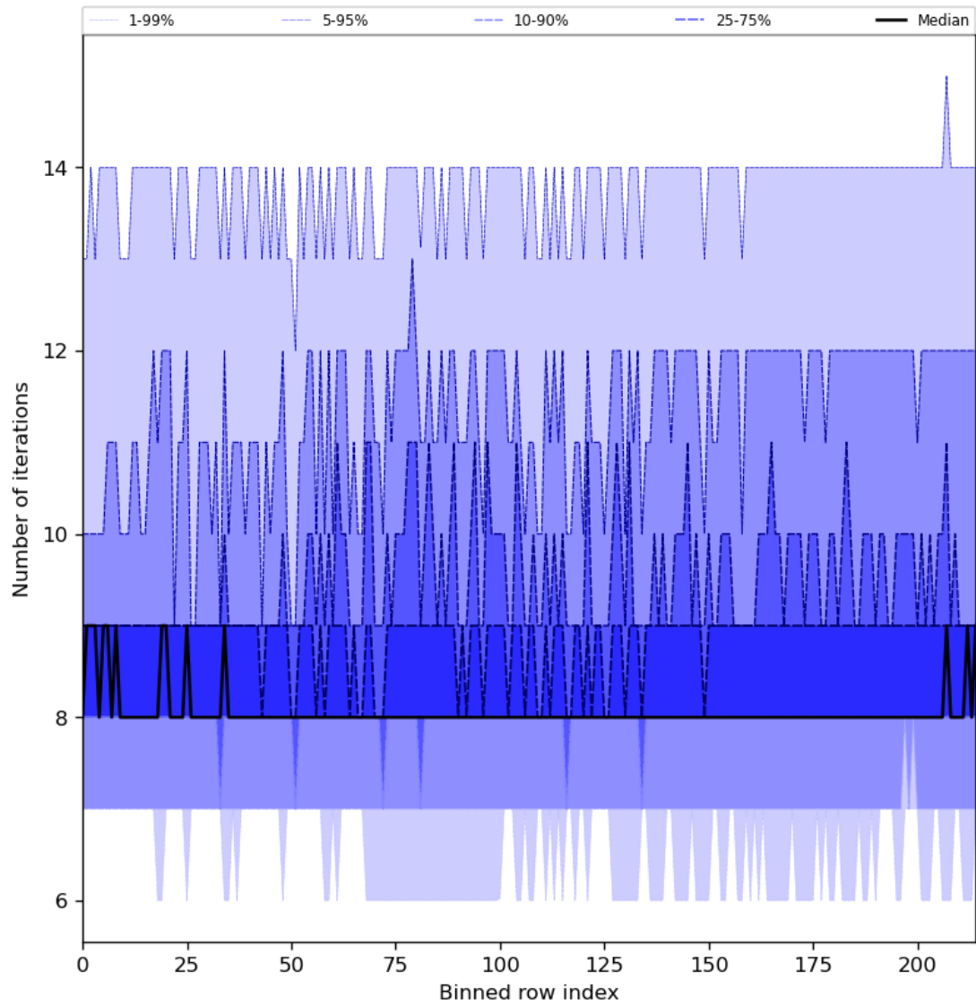
Figure 32: Along track statistics of “Number of iterations” for 2024-07-17 to 2024-07-19
