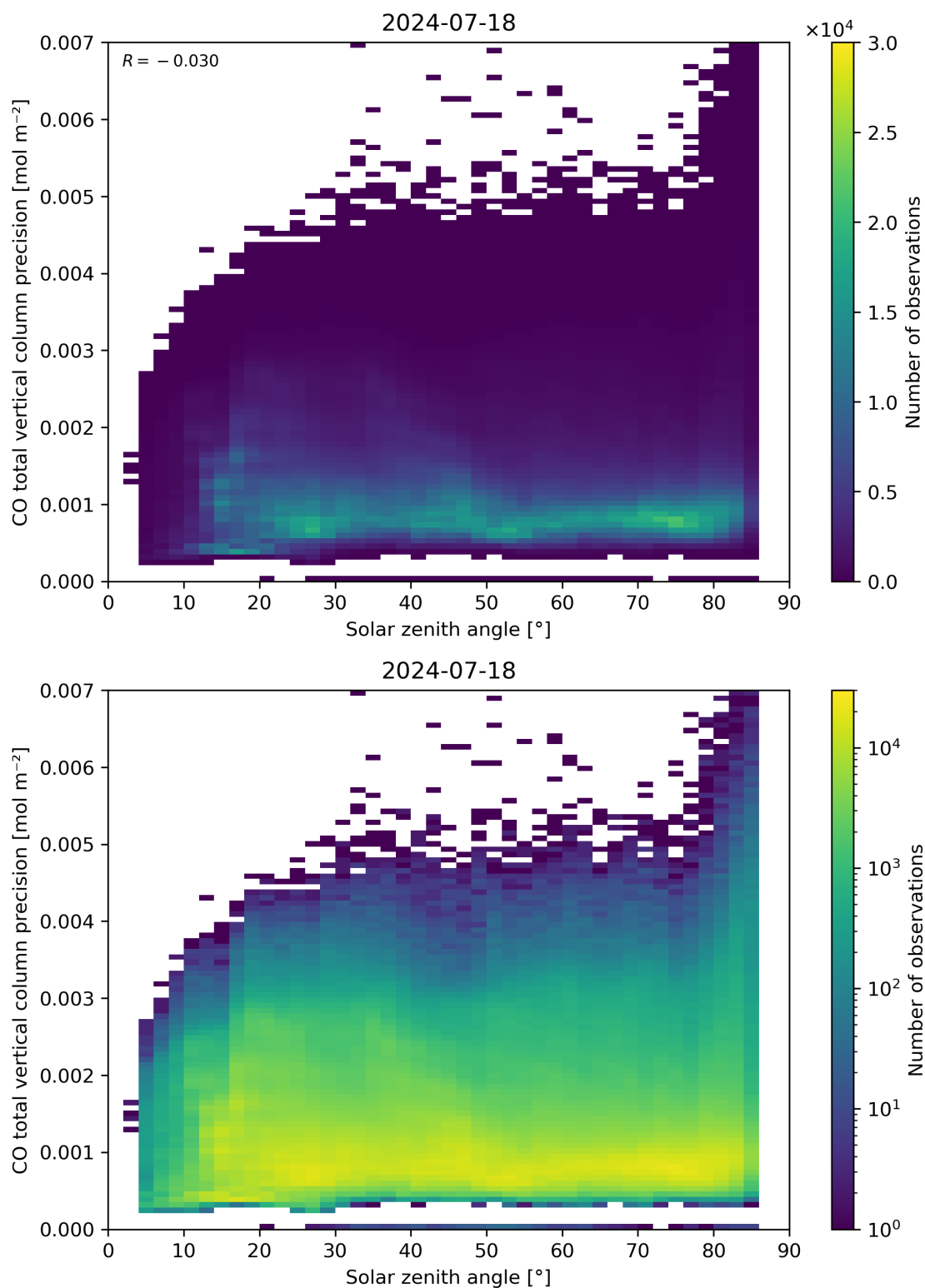
Figure 63: Scatter density plot of “Solar zenith angle” against “CO total vertical column precision” for 2024-07-17 to 2024-07-19.
