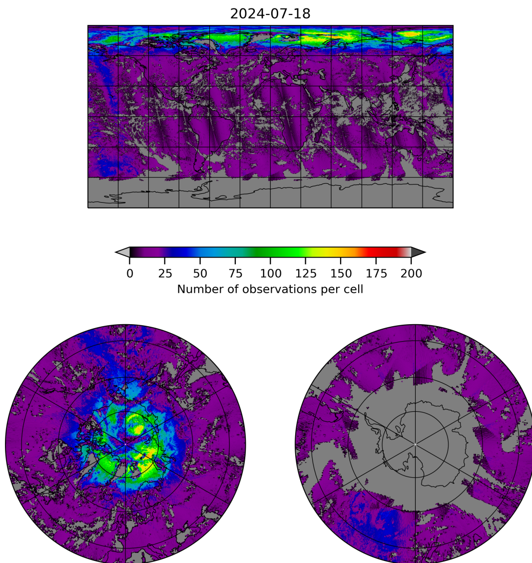
Figure 8: Map of the number of observations for 2024-07-17 to 2024-07-19
