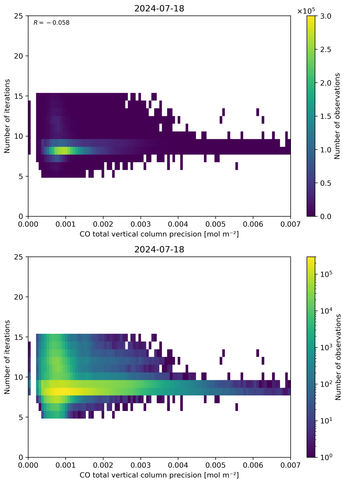
Figure 46: Scatter density plot of “CO total vertical column precision” against “Number of iterations” for 2024-07-17 to 2024-07-19.
