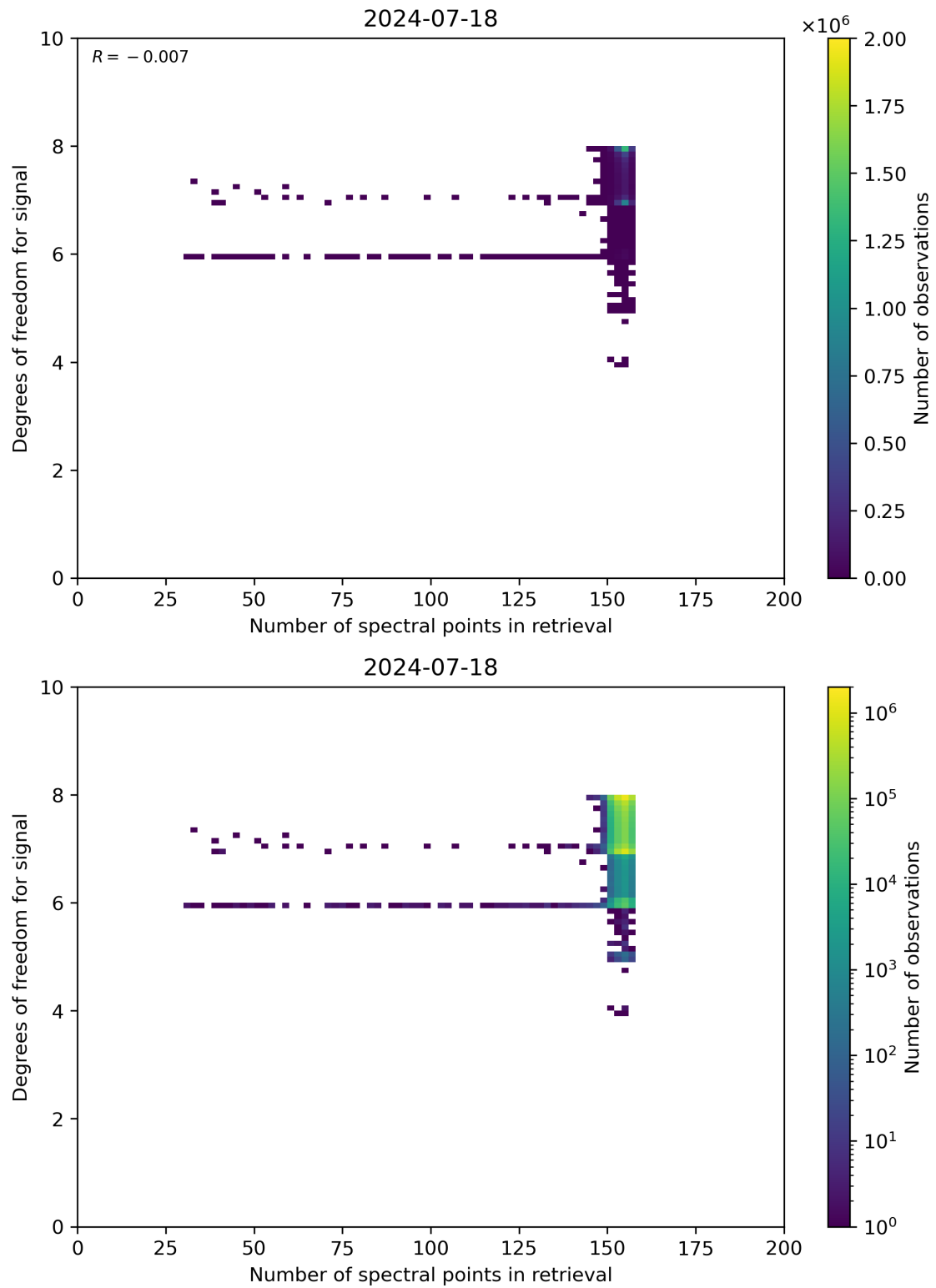
Figure 59: Scatter density plot of “Number of spectral points in retrieval” against “Degrees of freedom for signal” for 2024-07-17 to 2024-07-19.
