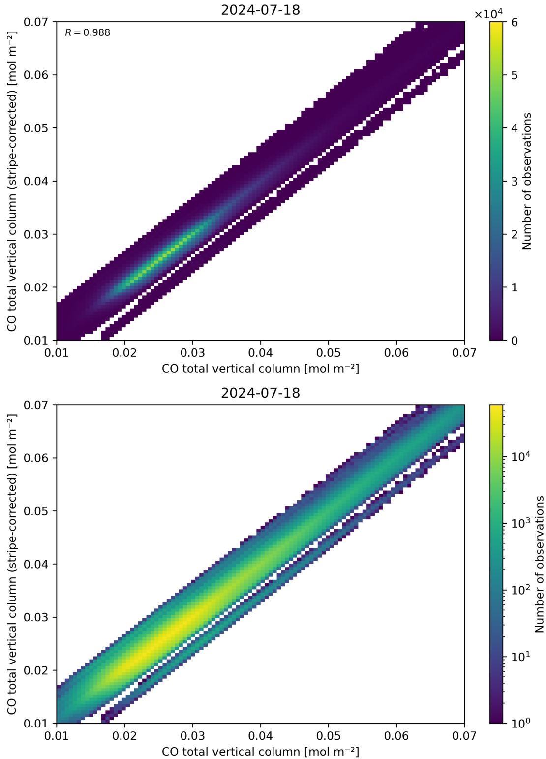
Figure 33: Scatter density plot of “CO total vertical column” against “CO total vertical column (stripe-corrected)” for 2024-07-17 to 2024-07-19.
