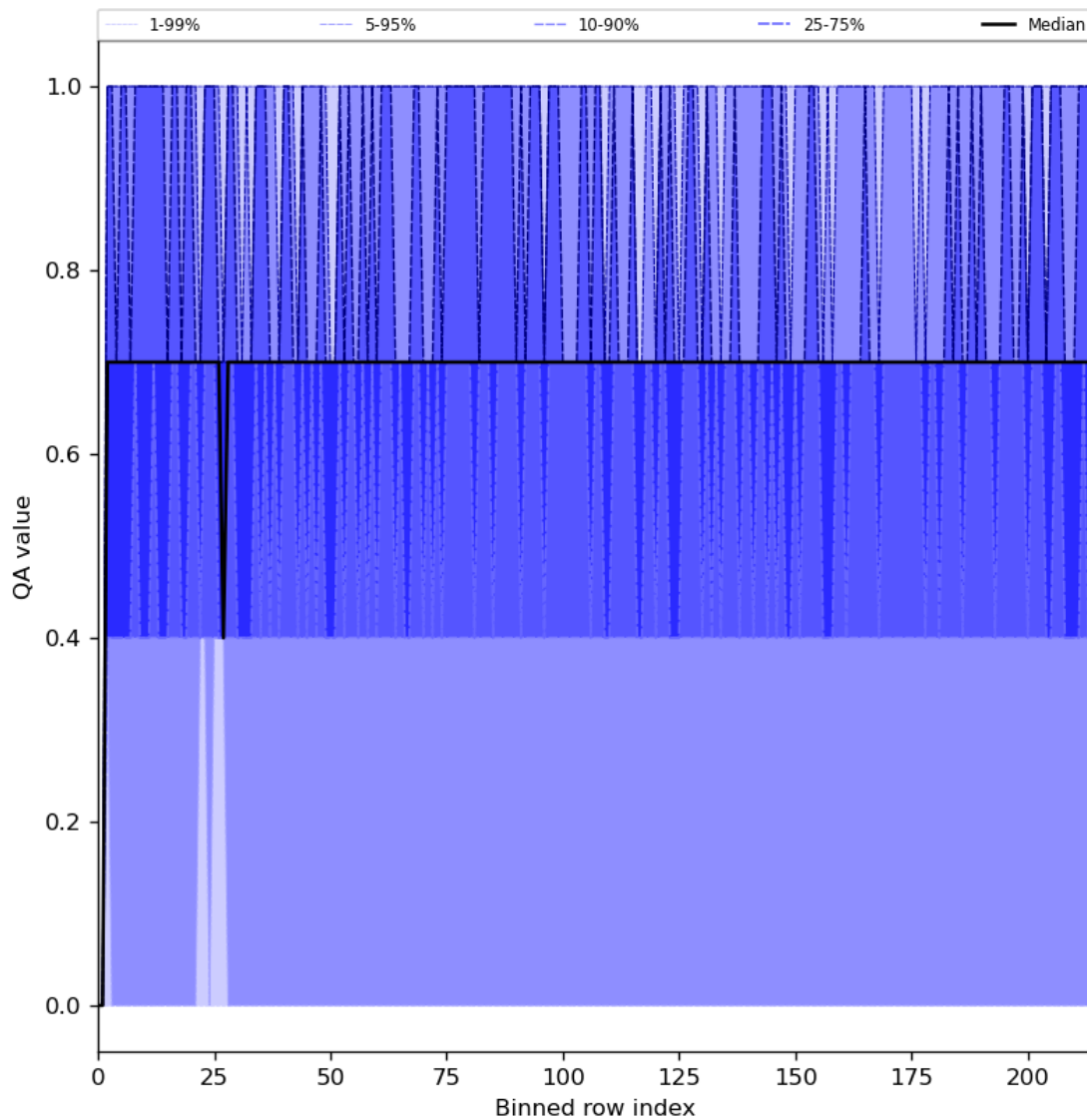
Figure 25: Along track statistics of “QA value” for 2024-07-17 to 2024-07-19
