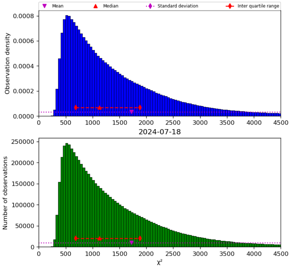
Figure 22: Histogram of “ \chi^2 ” for 2024-07-17 to 2024-07-19
