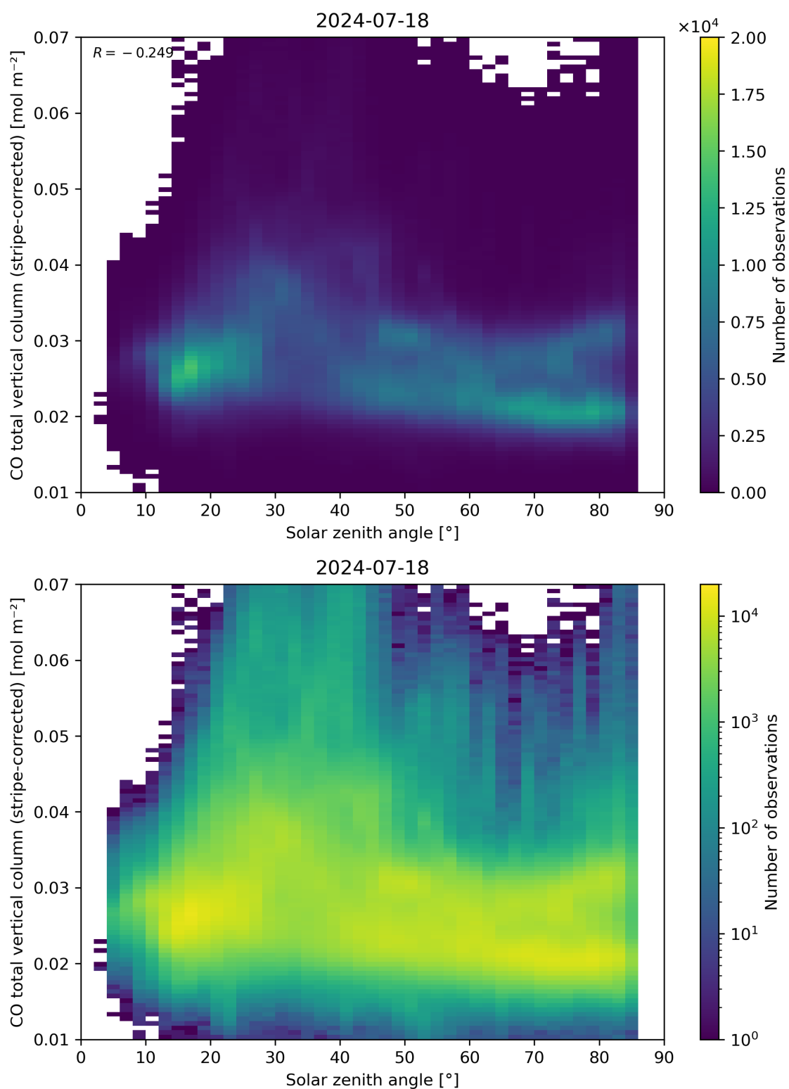
Figure 62: Scatter density plot of “Solar zenith angle” against “CO total vertical column (stripe-corrected)” for 2024-07-17 to 2024-07-19.
