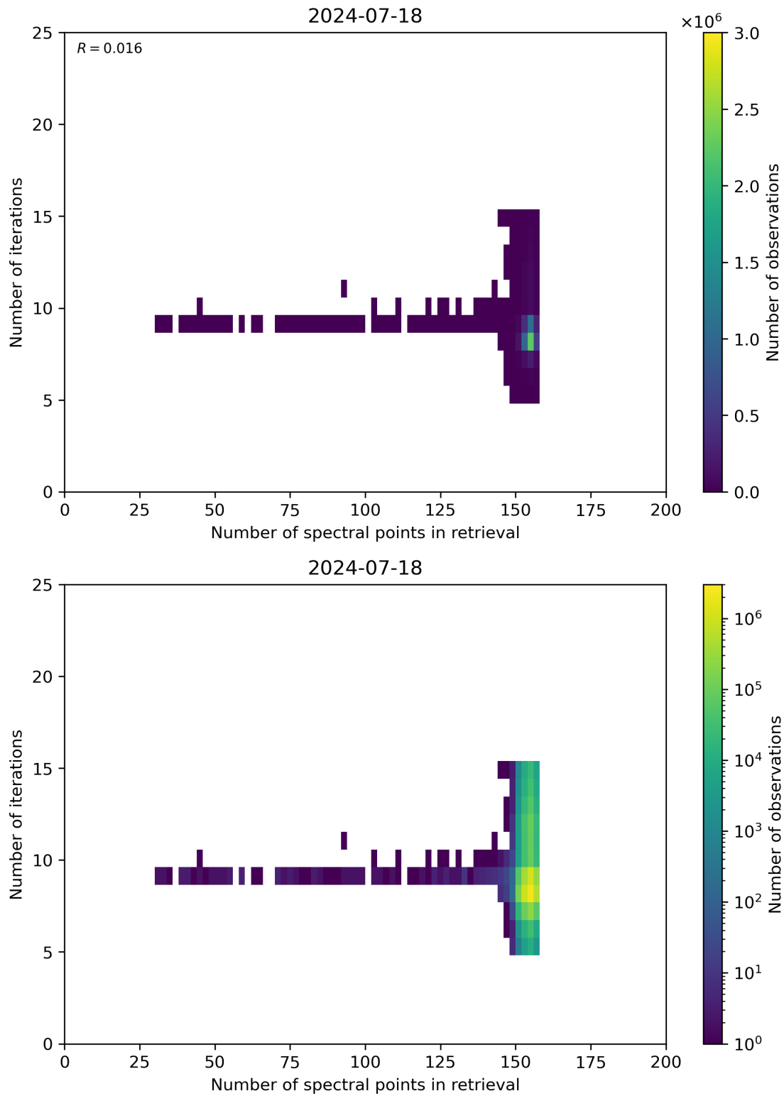
Figure 60: Scatter density plot of “Number of spectral points in retrieval” against “Number of iterations” for 2024-07-17 to 2024-07-19.
