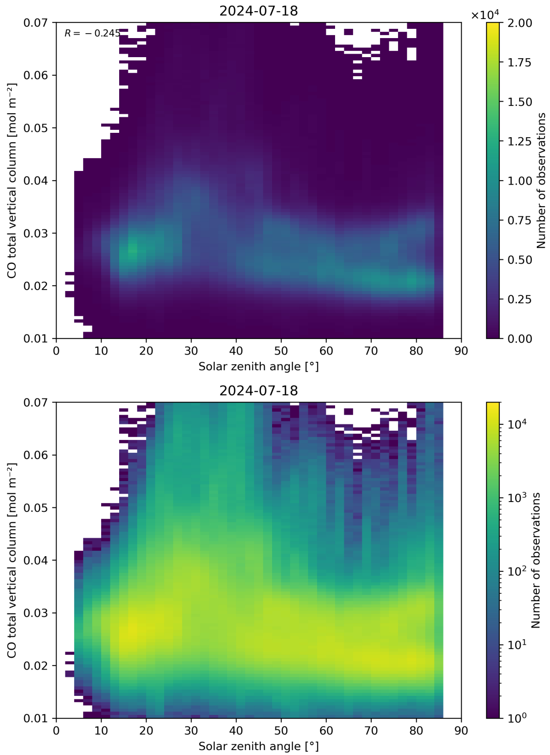
Figure 61: Scatter density plot of “Solar zenith angle” against “CO total vertical column” for 2024-07-17 to 2024-07-19.
