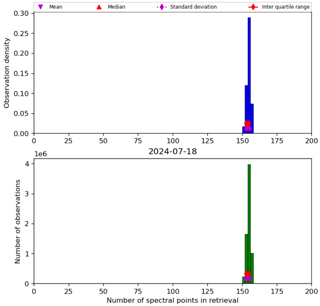
Figure 21: Histogram of “Number of spectral points in retrieval” for 2024-07-17 to 2024-07-19
