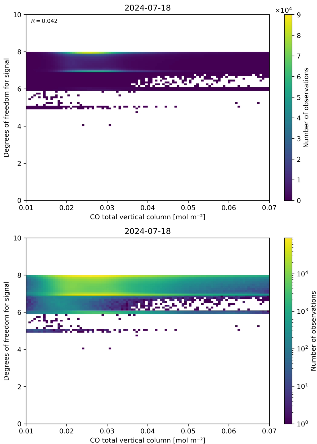
Figure 41: Scatter density plot of “CO total vertical column” against “Degrees of freedom for signal” for 2024-07-17 to 2024-07-19.
