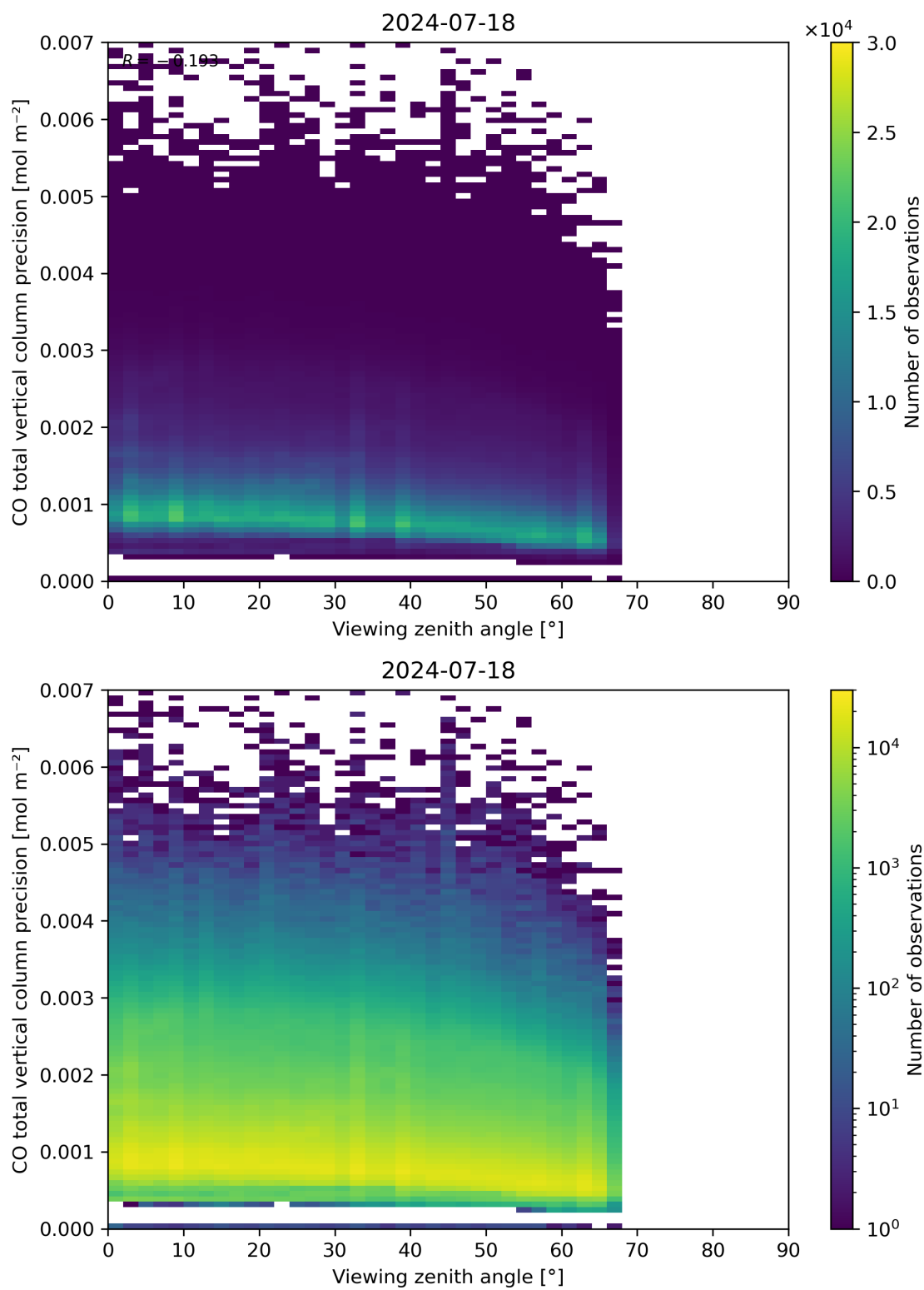
Figure 71: Scatter density plot of “Viewing zenith angle” against “CO total vertical column precision” for 2024-07-17 to 2024-07-19.
