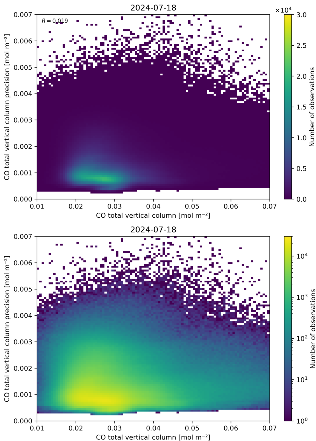
Figure 34: Scatter density plot of “CO total vertical column” against “CO total vertical column precision” for 2024-07-17 to 2024-07-19.
