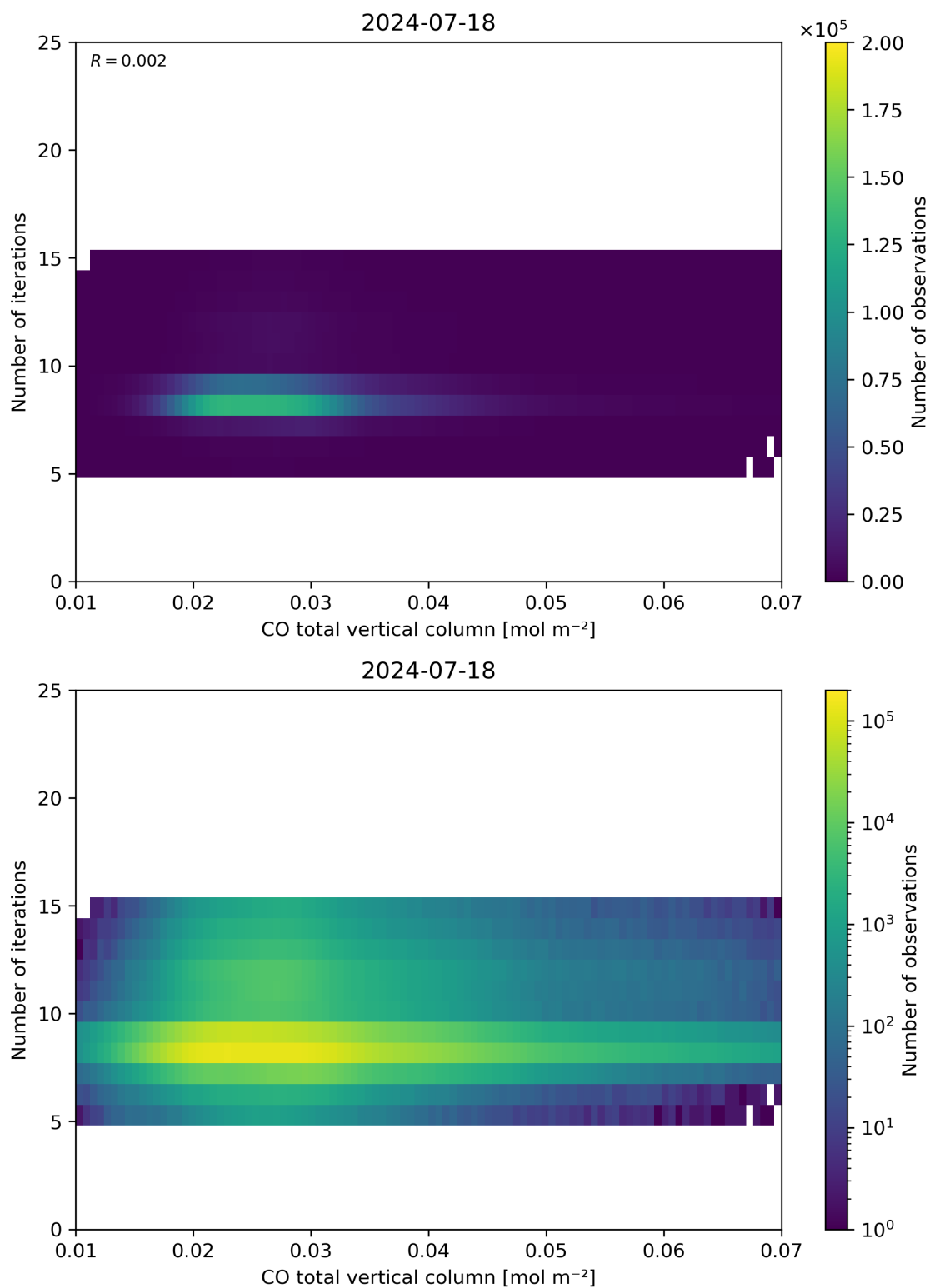
Figure 42: Scatter density plot of “CO total vertical column” against “Number of iterations” for 2024-07-17 to 2024-07-19.
