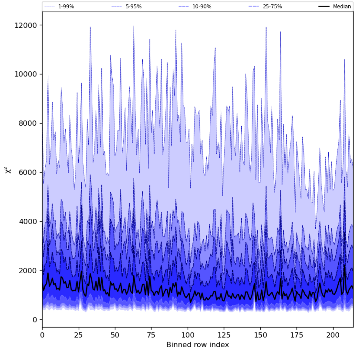
Figure 30: Along track statistics of “ \chi^2 ” for 2024-07-17 to 2024-07-19
