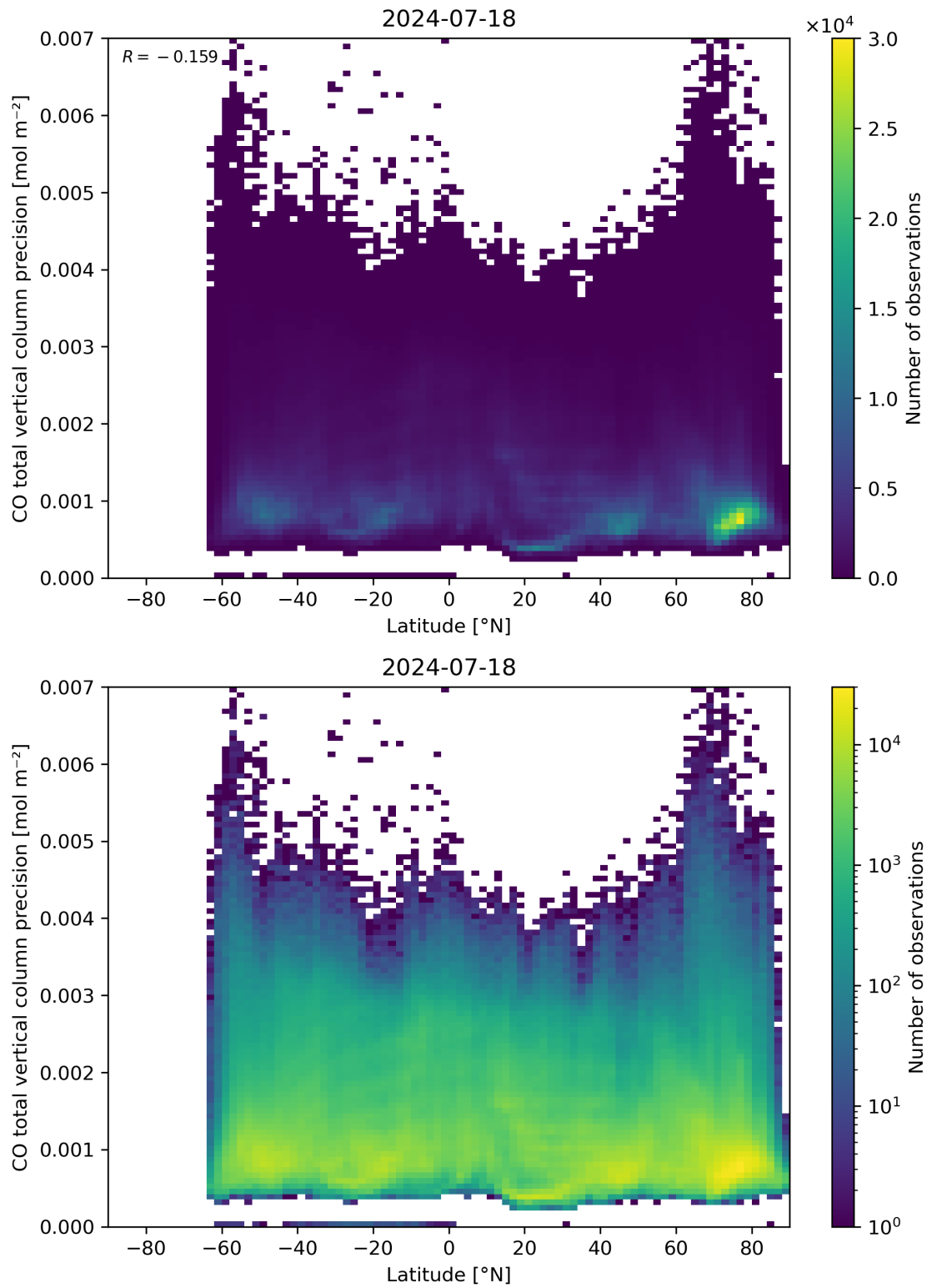
Figure 53: Scatter density plot of “Latitude” against “CO total vertical column precision” for 2024-07-17 to 2024-07-19.
