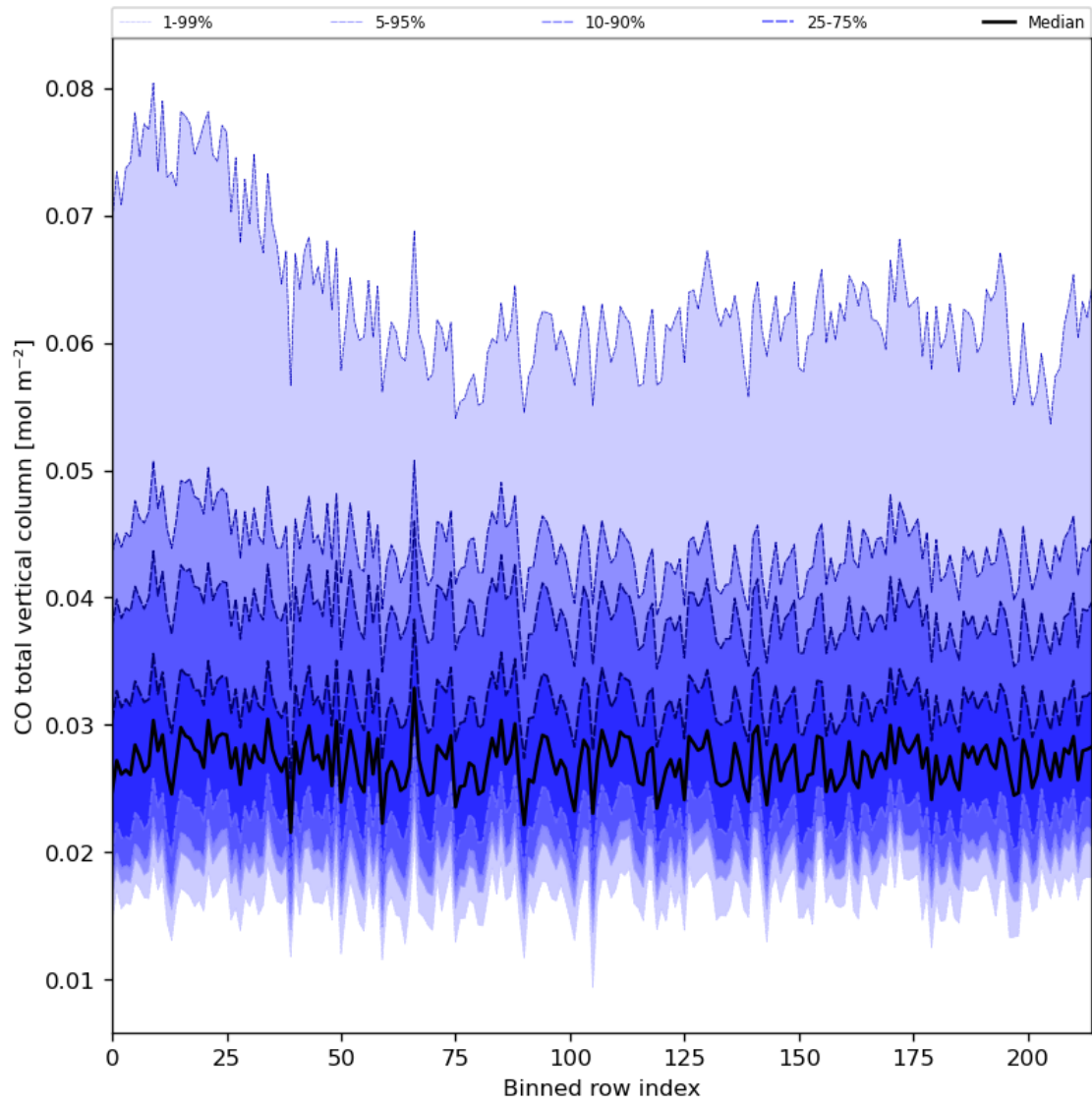
Figure 26: Along track statistics of “CO total vertical column” for 2024-07-17 to 2024-07-19
