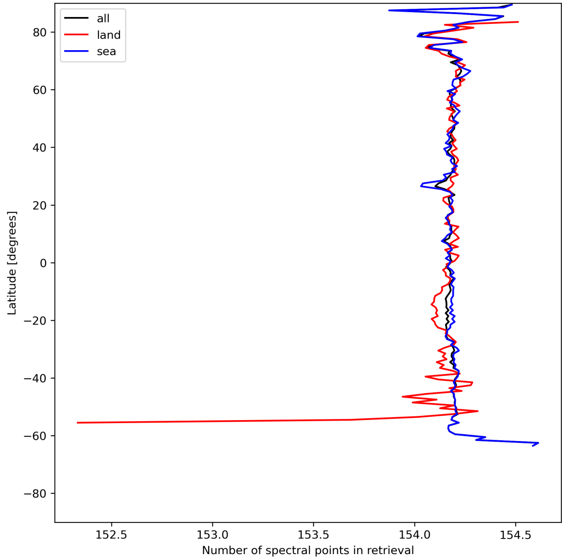
Figure 13: Zonal average of “Number of spectral points in retrieval” for 2024-07-17 to 2024-07-19.
