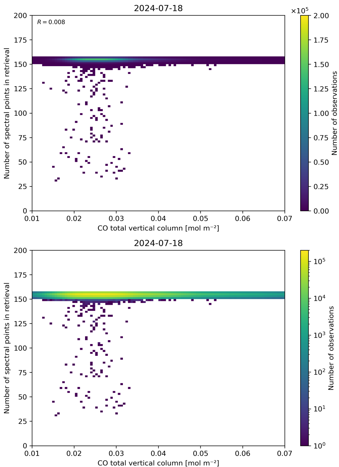
Figure 43: Scatter density plot of “CO total vertical column” against “Number of spectral points in retrieval” for 2024-07-17 to 2024-07-19.
