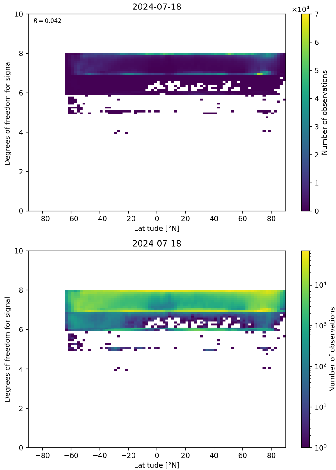
Figure 55: Scatter density plot of “Latitude” against “Degrees of freedom for signal” for 2024-07-17 to 2024-07-19.
