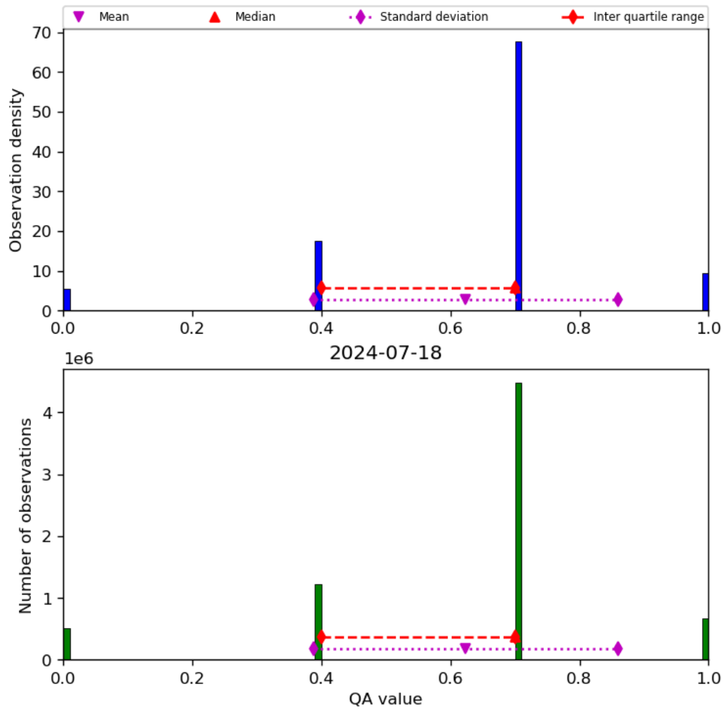
Figure 17: Histogram of “QA value” for 2024-07-17 to 2024-07-19
