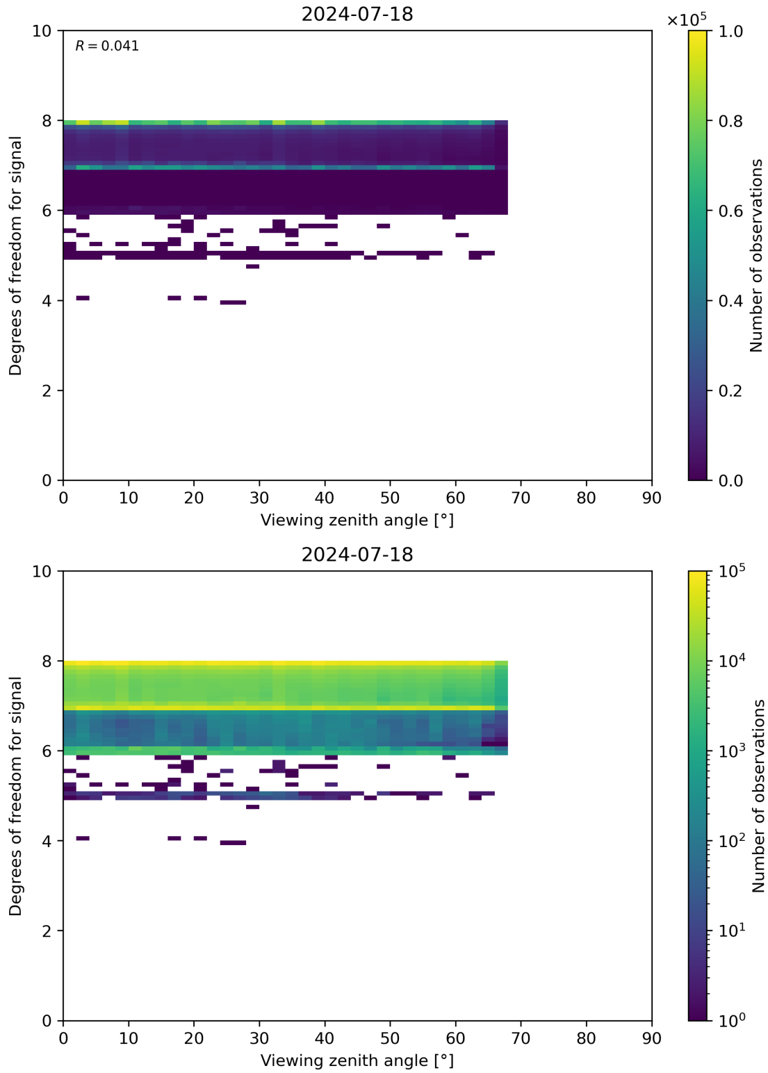
Figure 73: Scatter density plot of “Viewing zenith angle” against “Degrees of freedom for signal” for 2024-07-17 to 2024-07-19.
