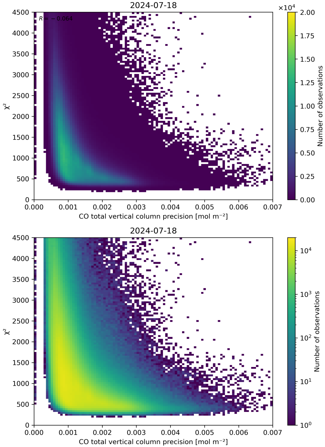
Figure 44: Scatter density plot of “CO total vertical column precision” against “ \chi^2 ” for 2024-07-17 to 2024-07-19.
