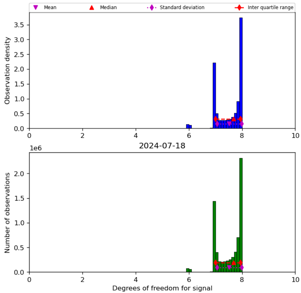
Figure 23: Histogram of “Degrees of freedom for signal” for 2024-07-17 to 2024-07-19
