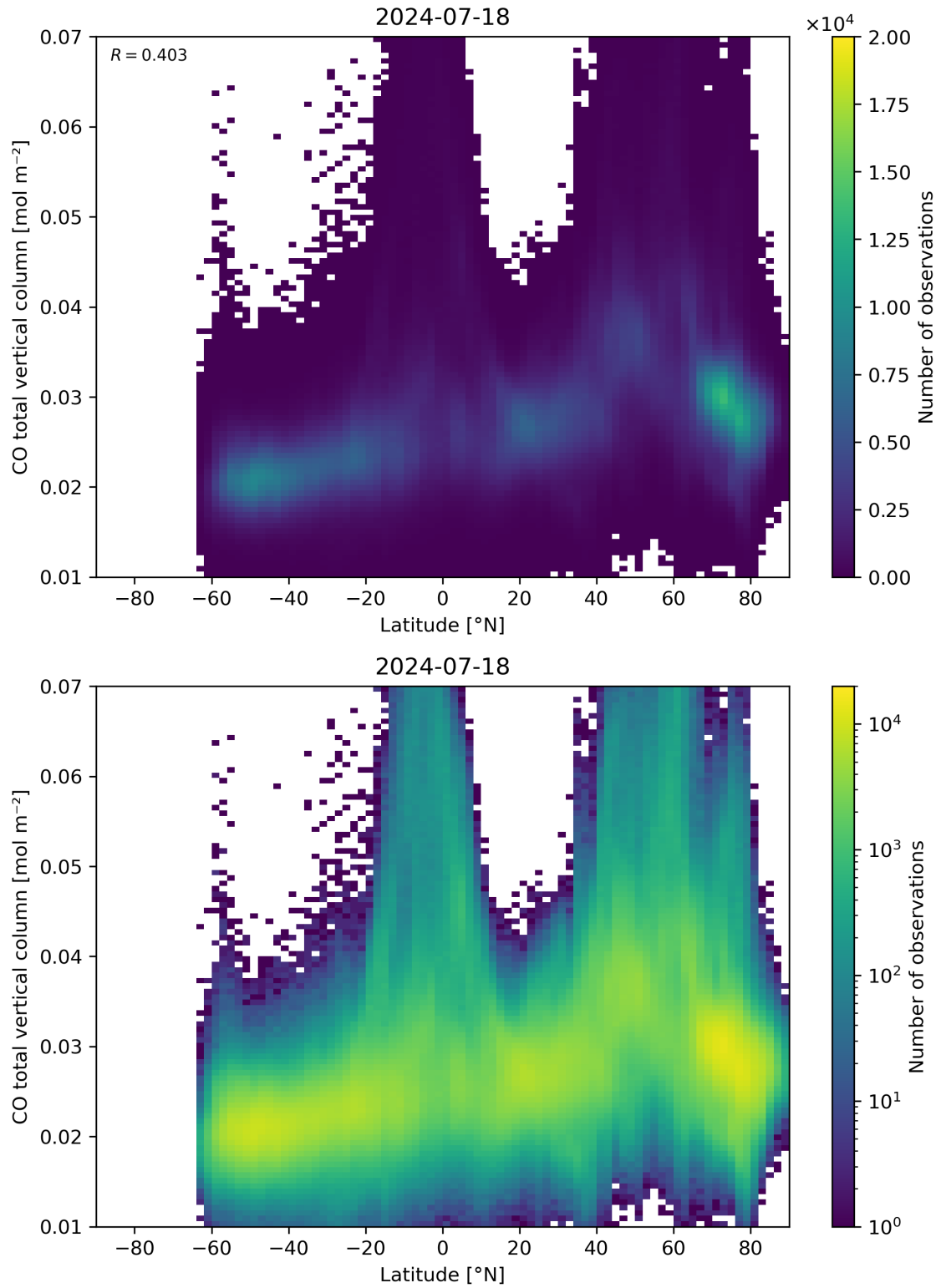
Figure 51: Scatter density plot of “Latitude” against “CO total vertical column” for 2024-07-17 to 2024-07-19.
