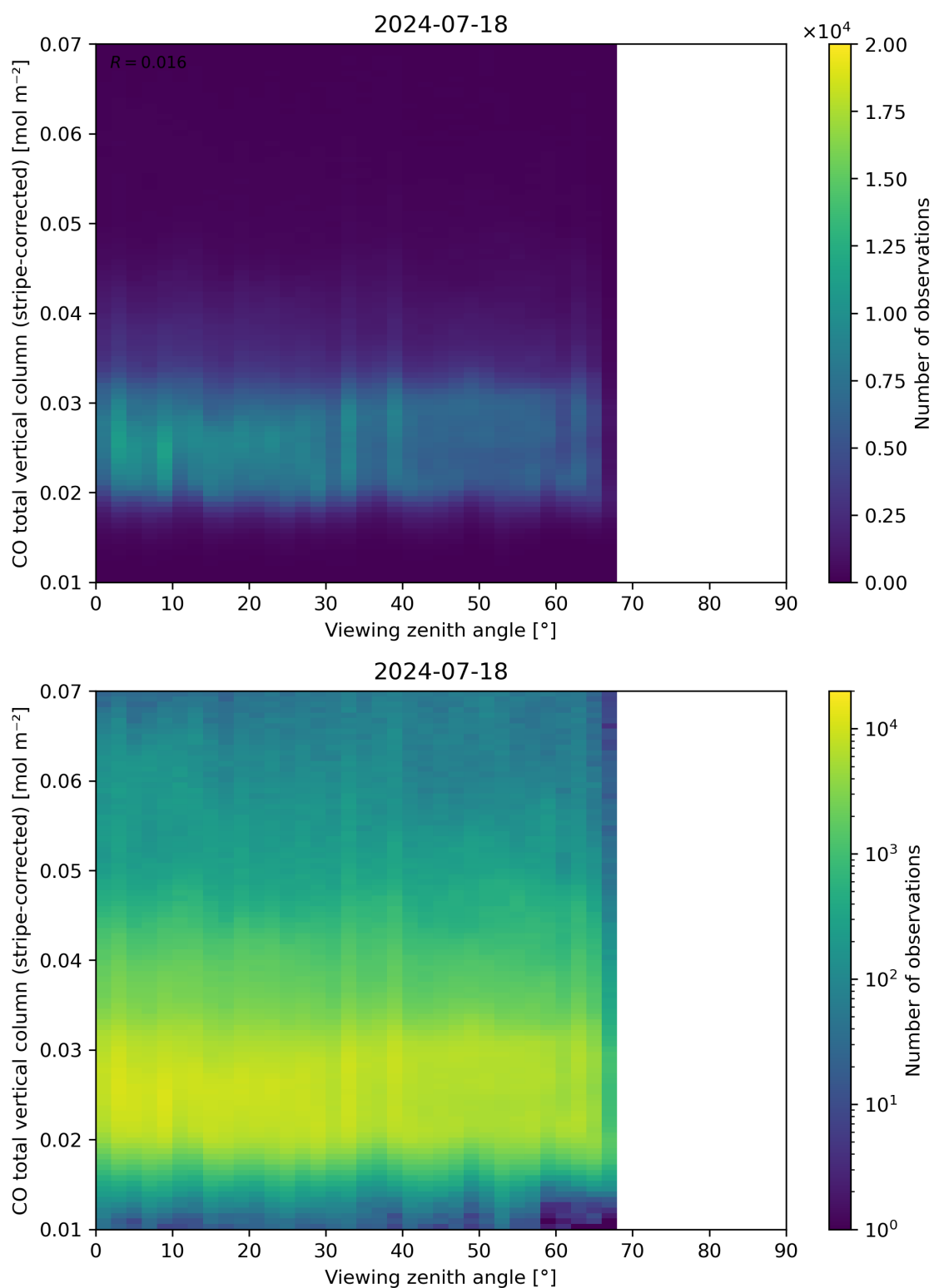
Figure 70: Scatter density plot of “Viewing zenith angle” against “CO total vertical column (stripe-corrected)” for 2024-07-17 to 2024-07-19.
