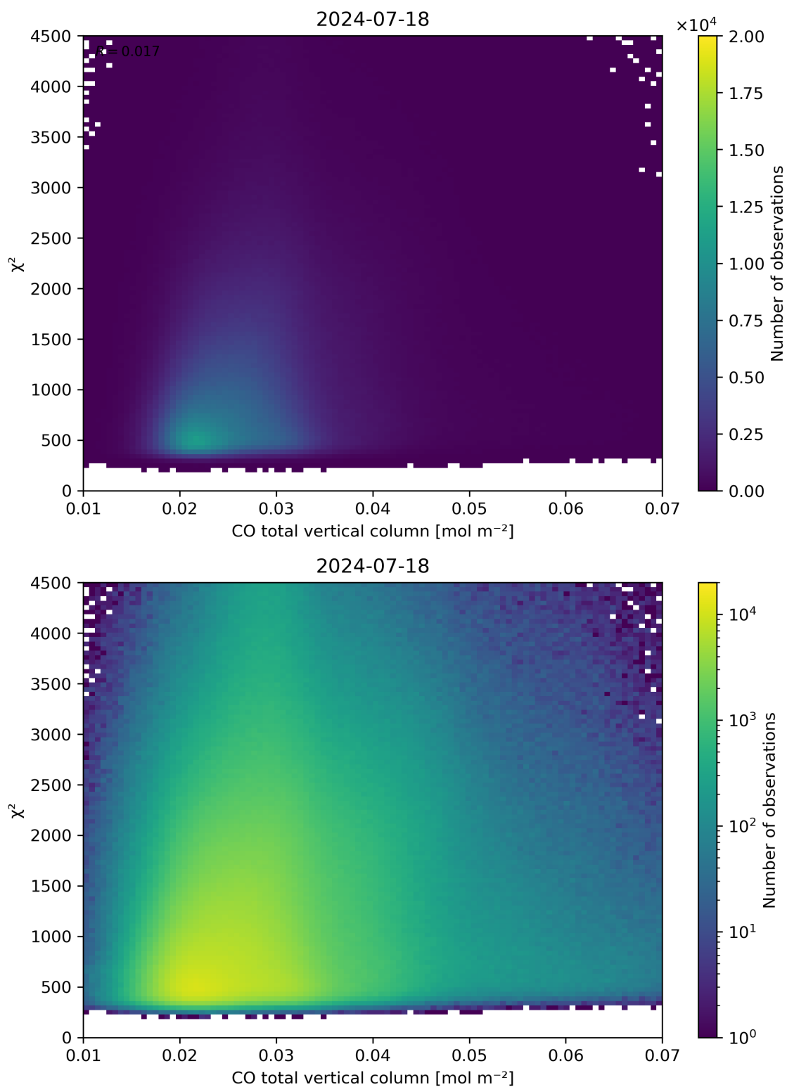
Figure 35: Scatter density plot of “CO total vertical column” against “ \chi^2 ” for 2024-07-17 to 2024-07-19.
