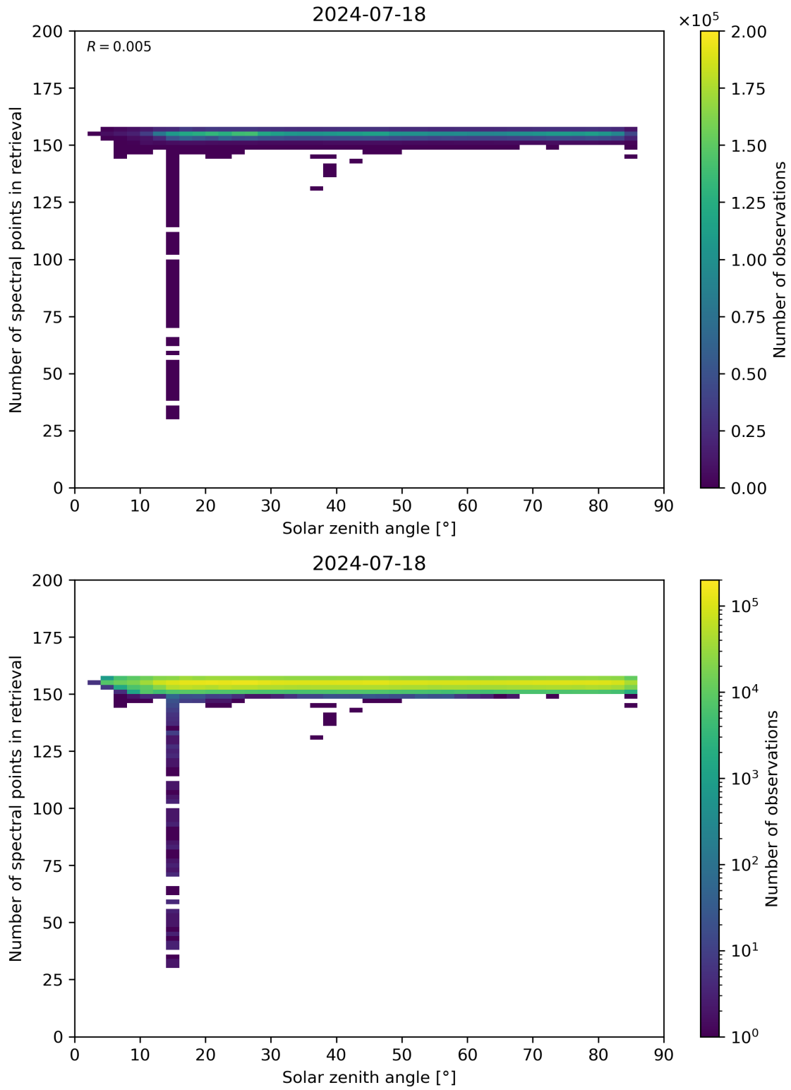
Figure 68: Scatter density plot of “Solar zenith angle” against “Number of spectral points in retrieval” for 2024-07-17 to 2024-07-19.
