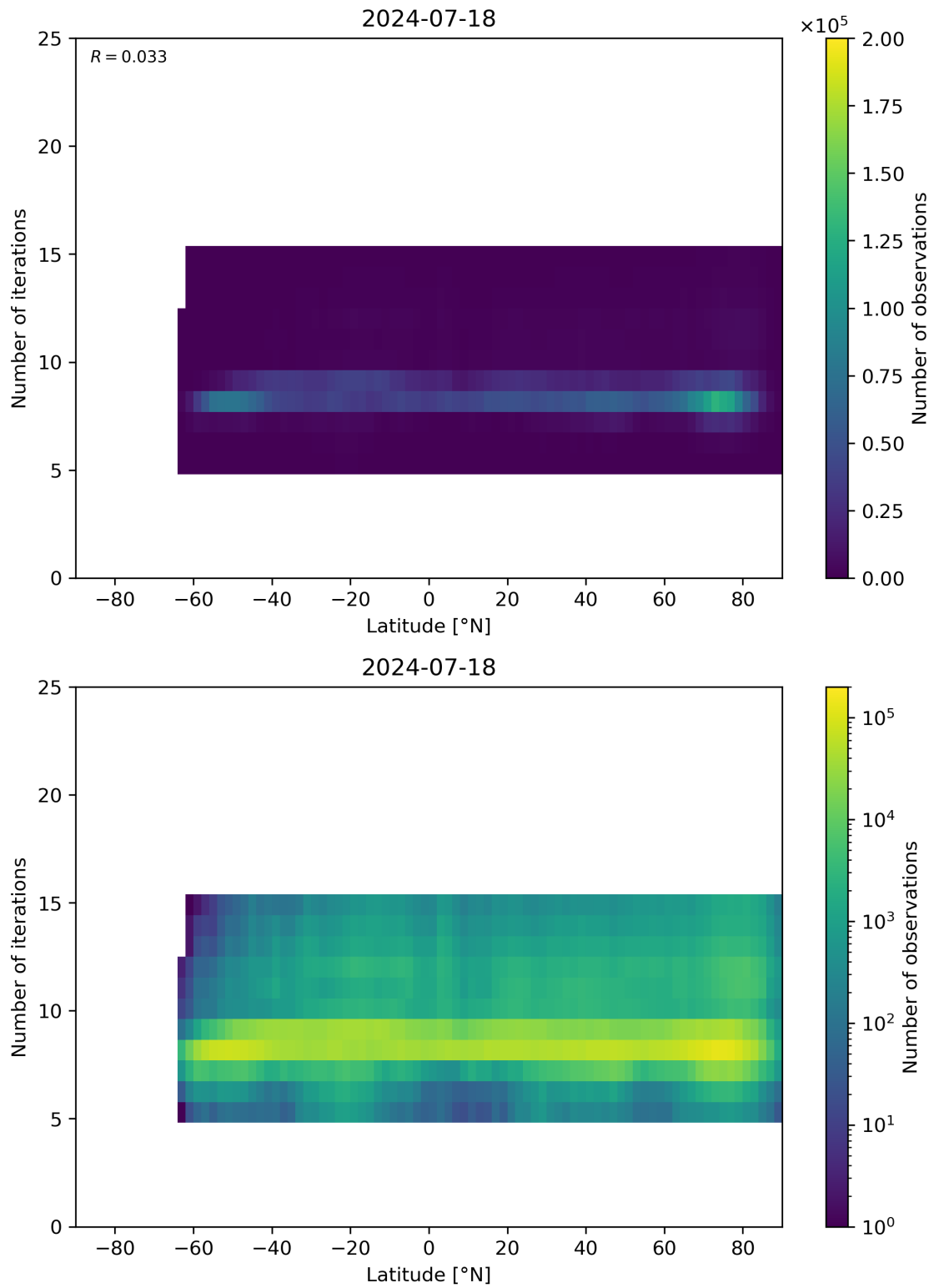
Figure 56: Scatter density plot of “Latitude” against “Number of iterations” for 2024-07-17 to 2024-07-19.
