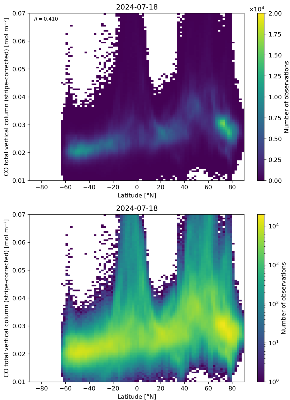
Figure 52: Scatter density plot of “Latitude” against “CO total vertical column (stripe-corrected)” for 2024-07-17 to 2024-07-19.
