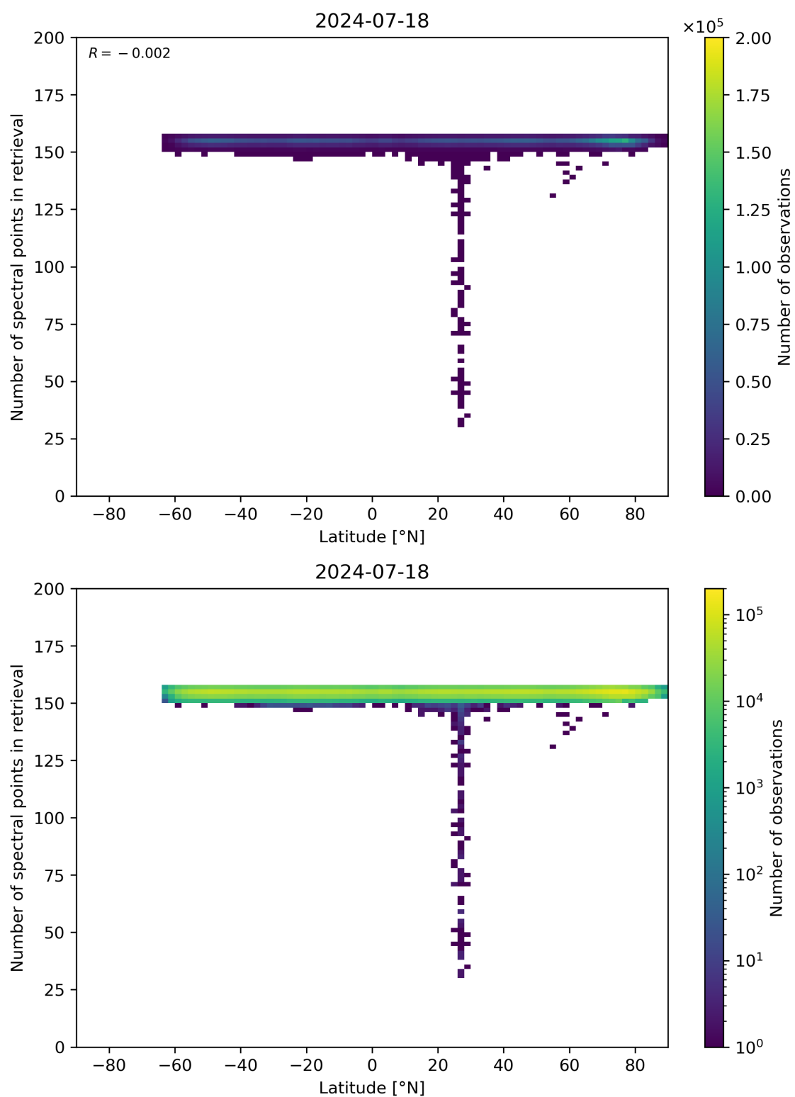
Figure 57: Scatter density plot of “Latitude” against “Number of spectral points in retrieval” for 2024-07-17 to 2024-07-19.
