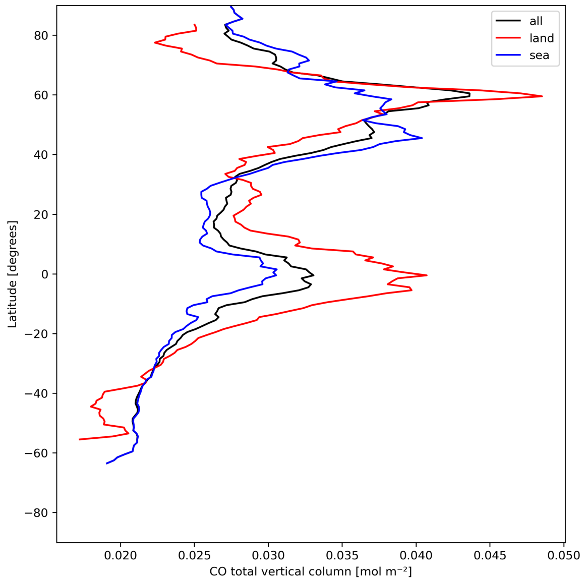
Figure 10: Zonal average of “CO total vertical column” for 2024-07-17 to 2024-07-19.
