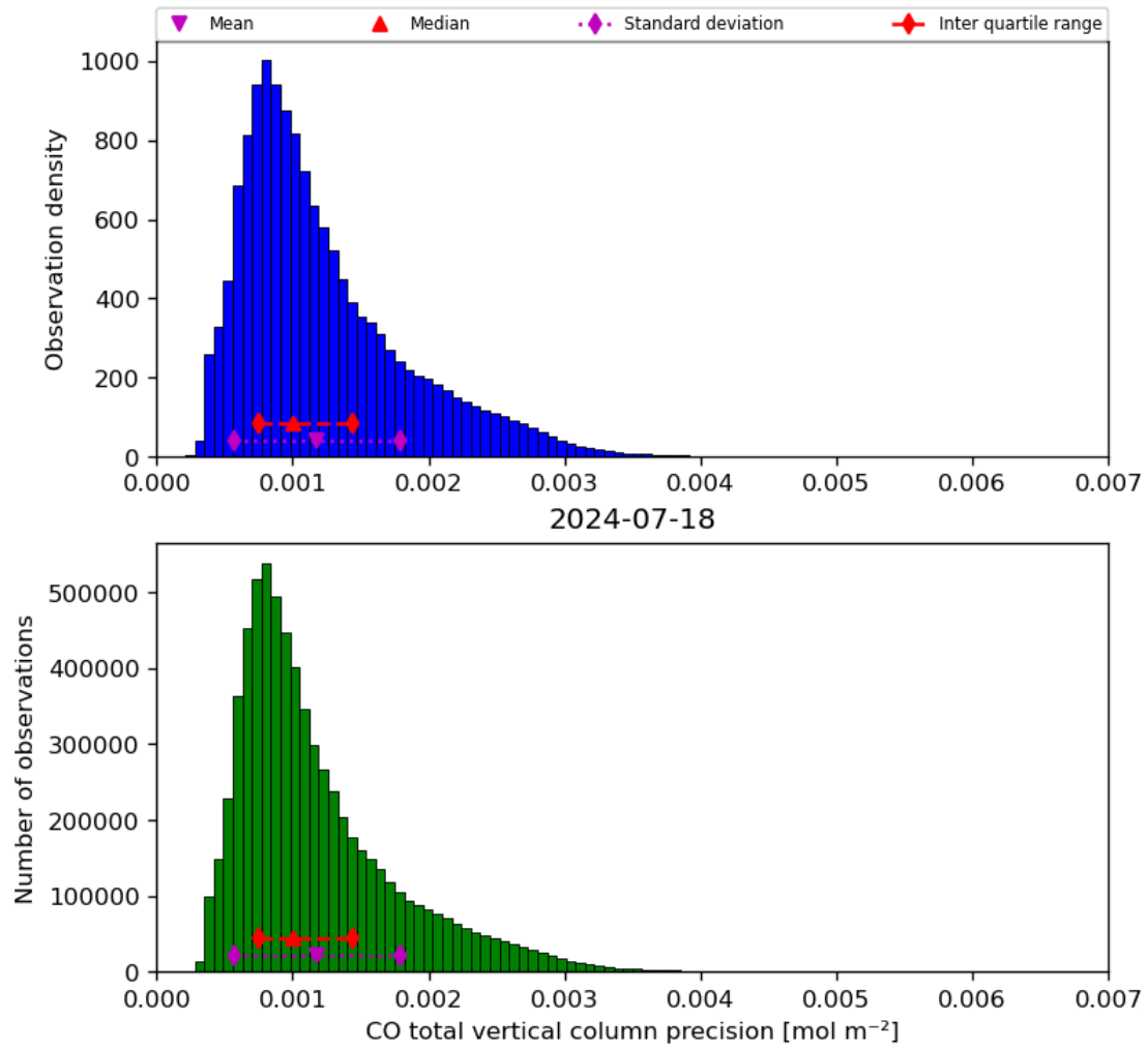
Figure 20: Histogram of “CO total vertical column precision” for 2024-07-17 to 2024-07-19
