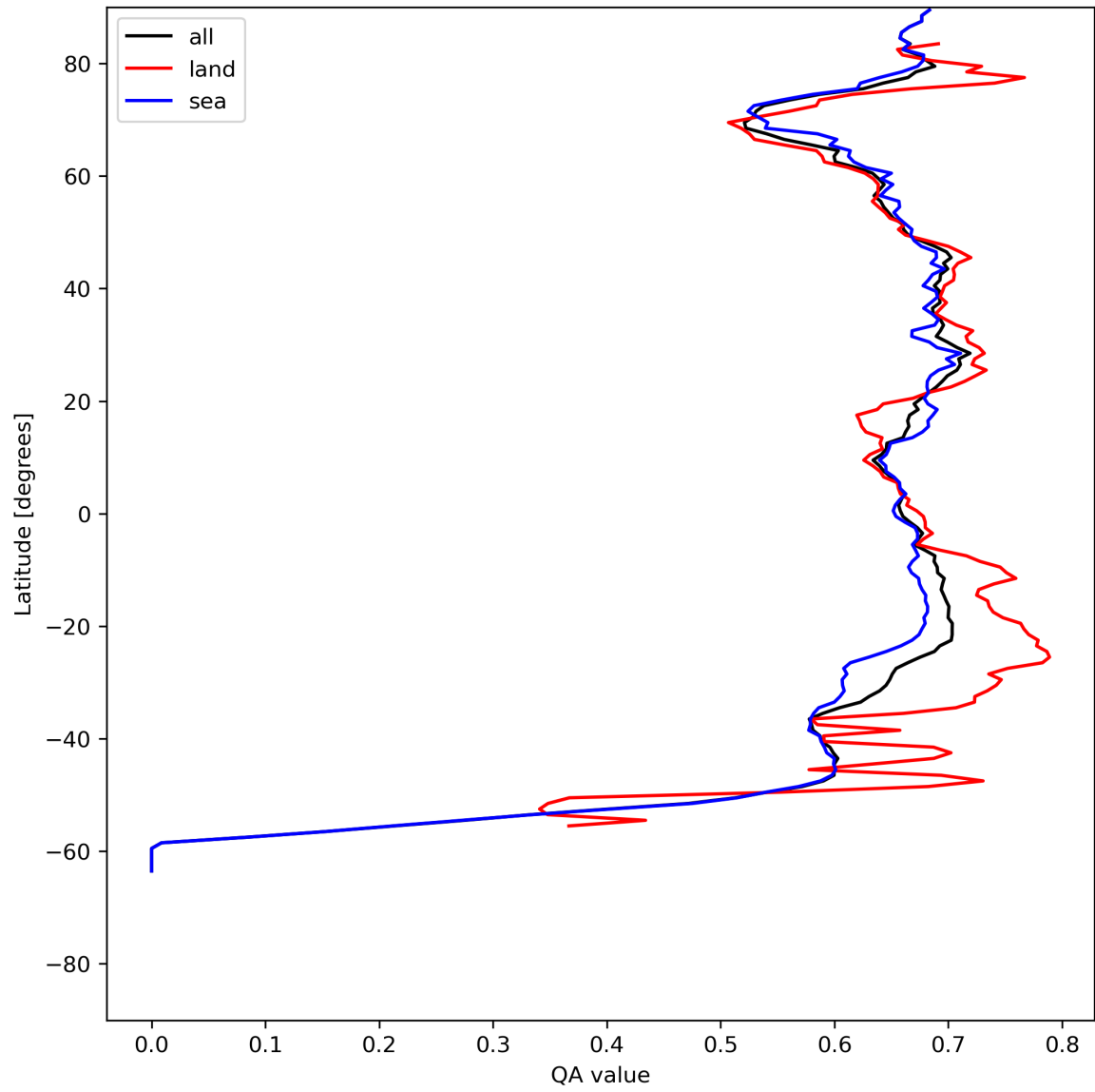
Figure 9: Zonal average of “QA value” for 2024-07-17 to 2024-07-19.
