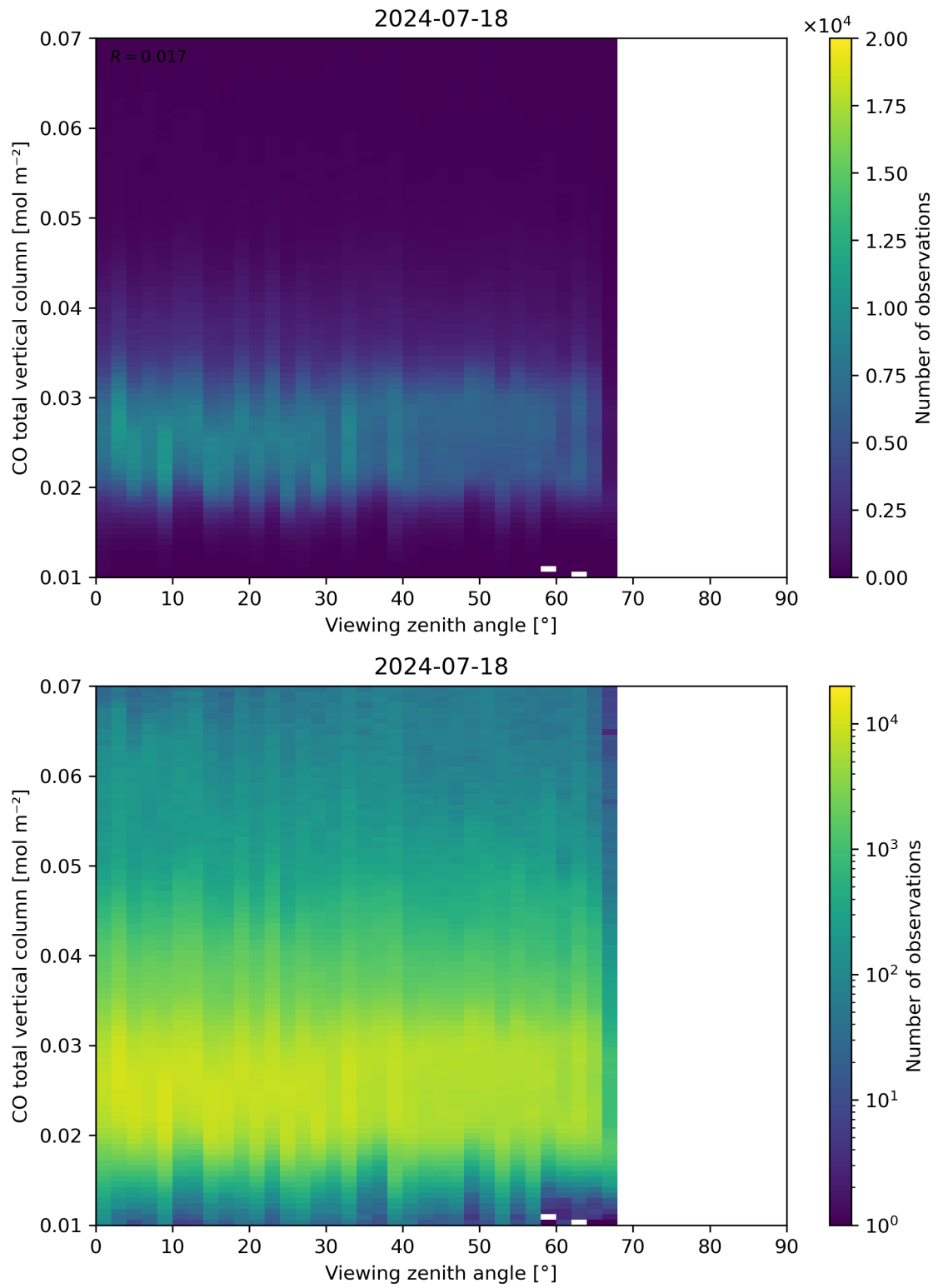
Figure 69: Scatter density plot of “Viewing zenith angle” against “CO total vertical column” for 2024-07-17 to 2024-07-19.
