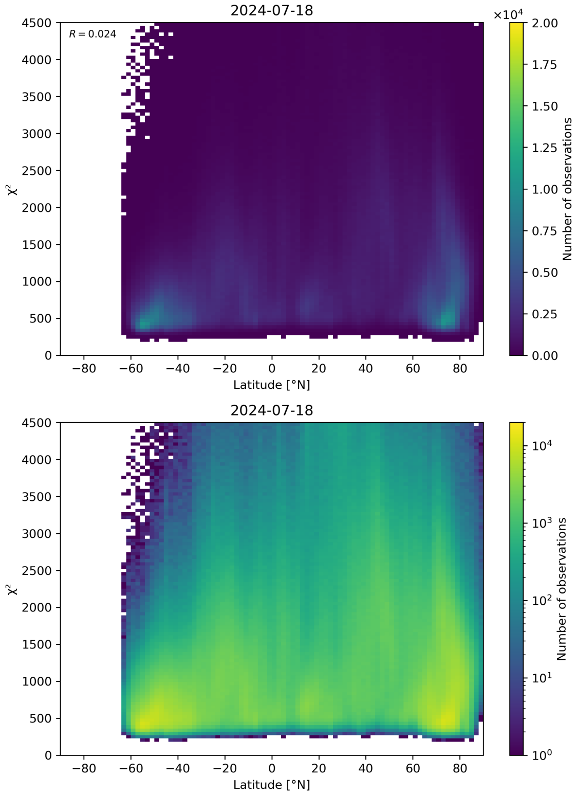
Figure 54: Scatter density plot of “Latitude” against “ \chi^2 ” for 2024-07-17 to 2024-07-19.
