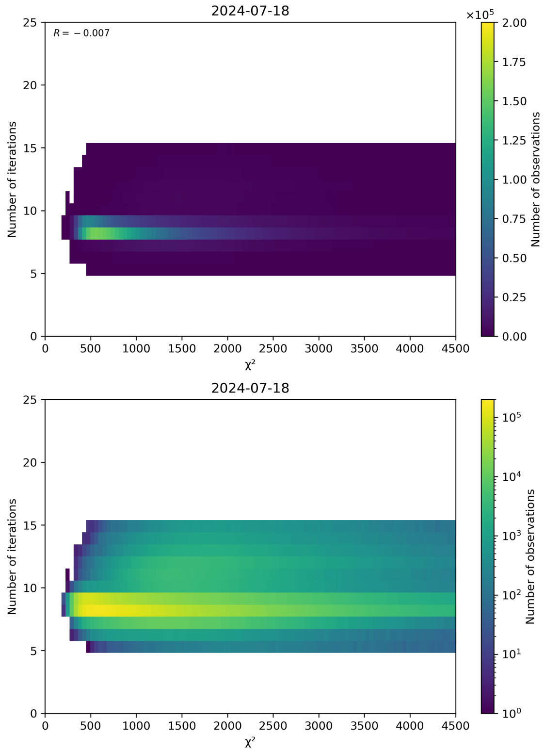
Figure 49: Scatter density plot of “ \chi^2 ” against “Number of iterations” for 2024-07-17 to 2024-07-19.
