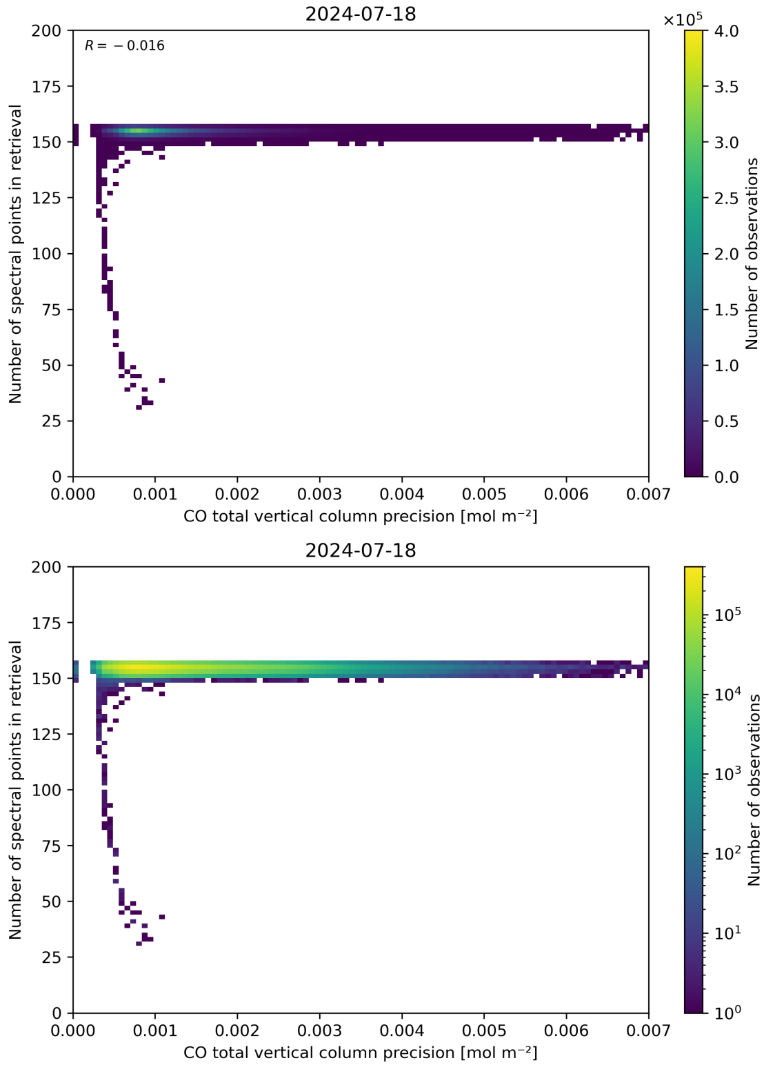
Figure 47: Scatter density plot of “CO total vertical column precision” against “Number of spectral points in retrieval” for 2024-07-17 to 2024-07-19.
