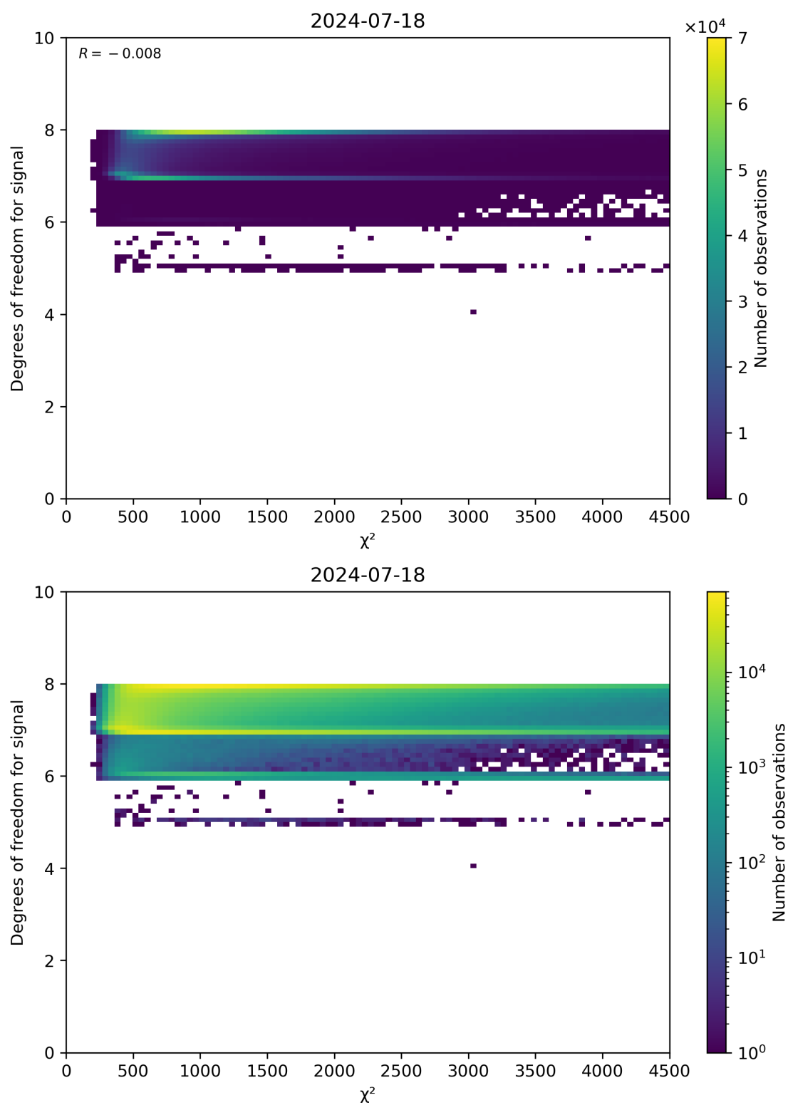
Figure 48: Scatter density plot of “ \chi^2 ” against “Degrees of freedom for signal” for 2024-07-17 to 2024-07-19.
