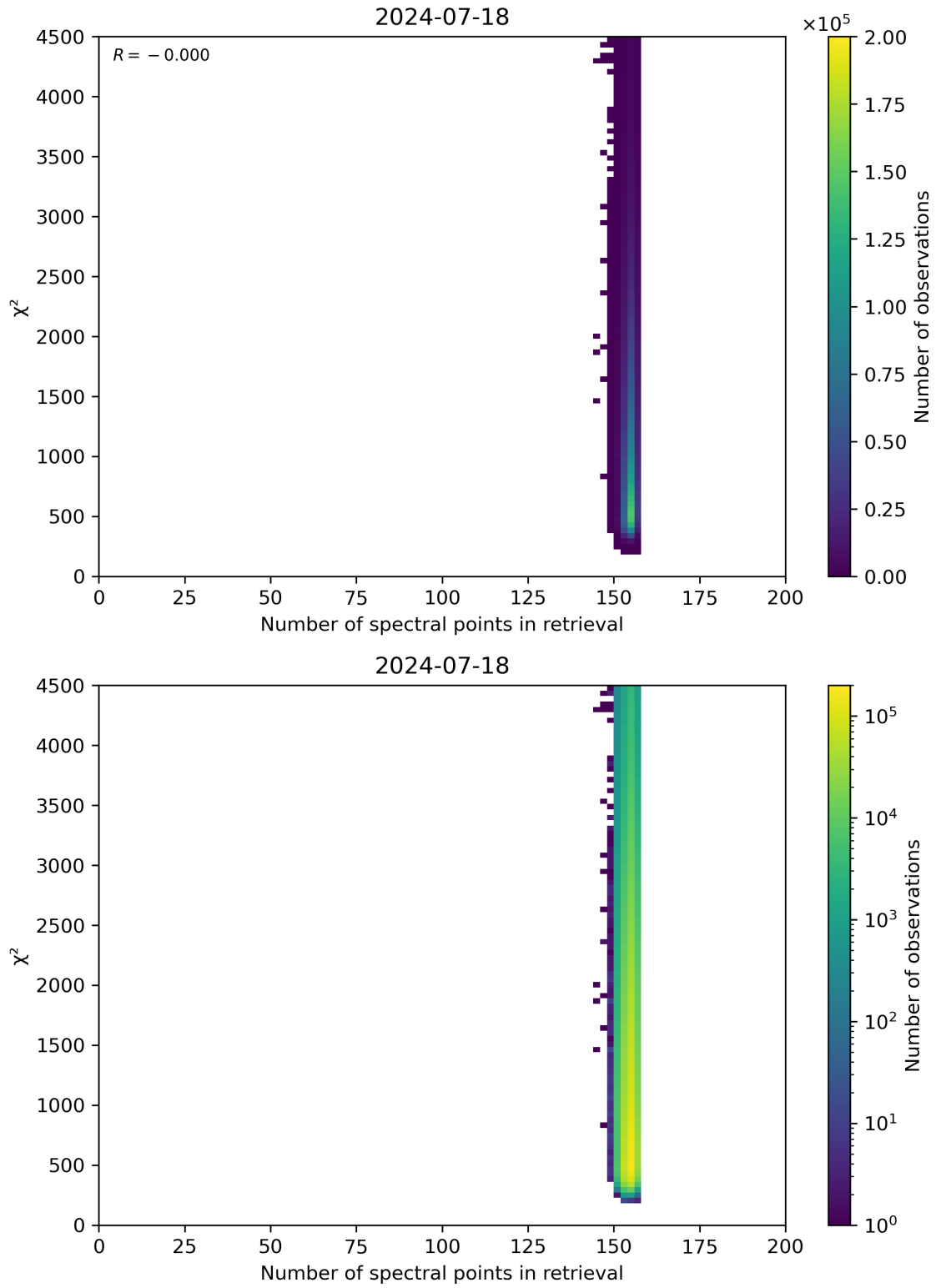
Figure 58: Scatter density plot of “Number of spectral points in retrieval” against “ \chi^2 ” for 2024-07-17 to 2024-07-19.
