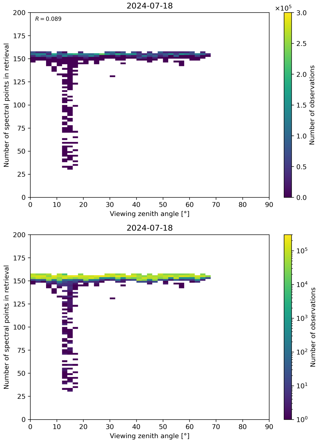
Figure 76: Scatter density plot of “Viewing zenith angle” against “Number of spectral points in retrieval” for 2024-07-17 to 2024-07-19.
