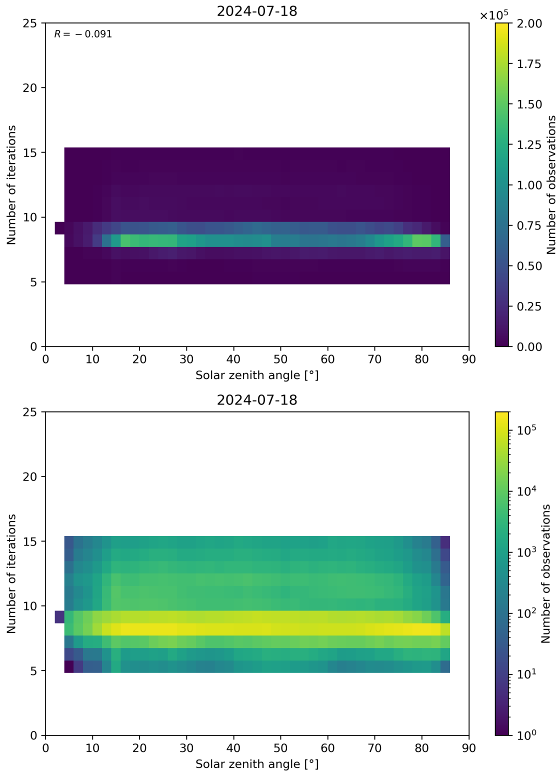
Figure 67: Scatter density plot of “Solar zenith angle” against “Number of iterations” for 2024-07-17 to 2024-07-19.
