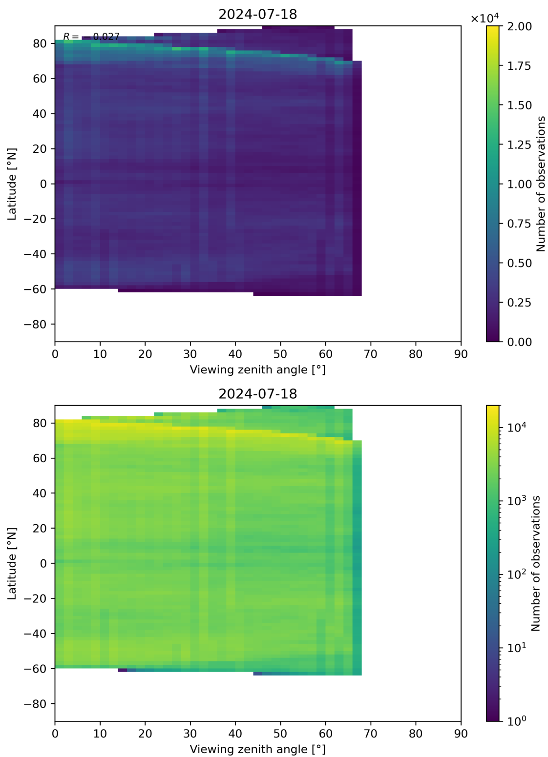
Figure 74: Scatter density plot of “Viewing zenith angle” against “Latitude” for 2024-07-17 to 2024-07-19.
