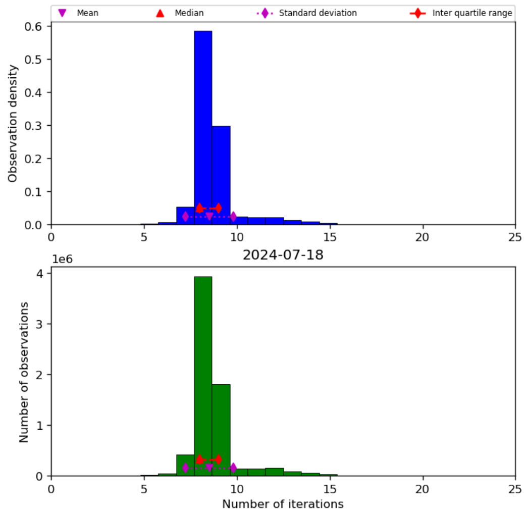
Figure 24: Histogram of “Number of iterations” for 2024-07-17 to 2024-07-19
