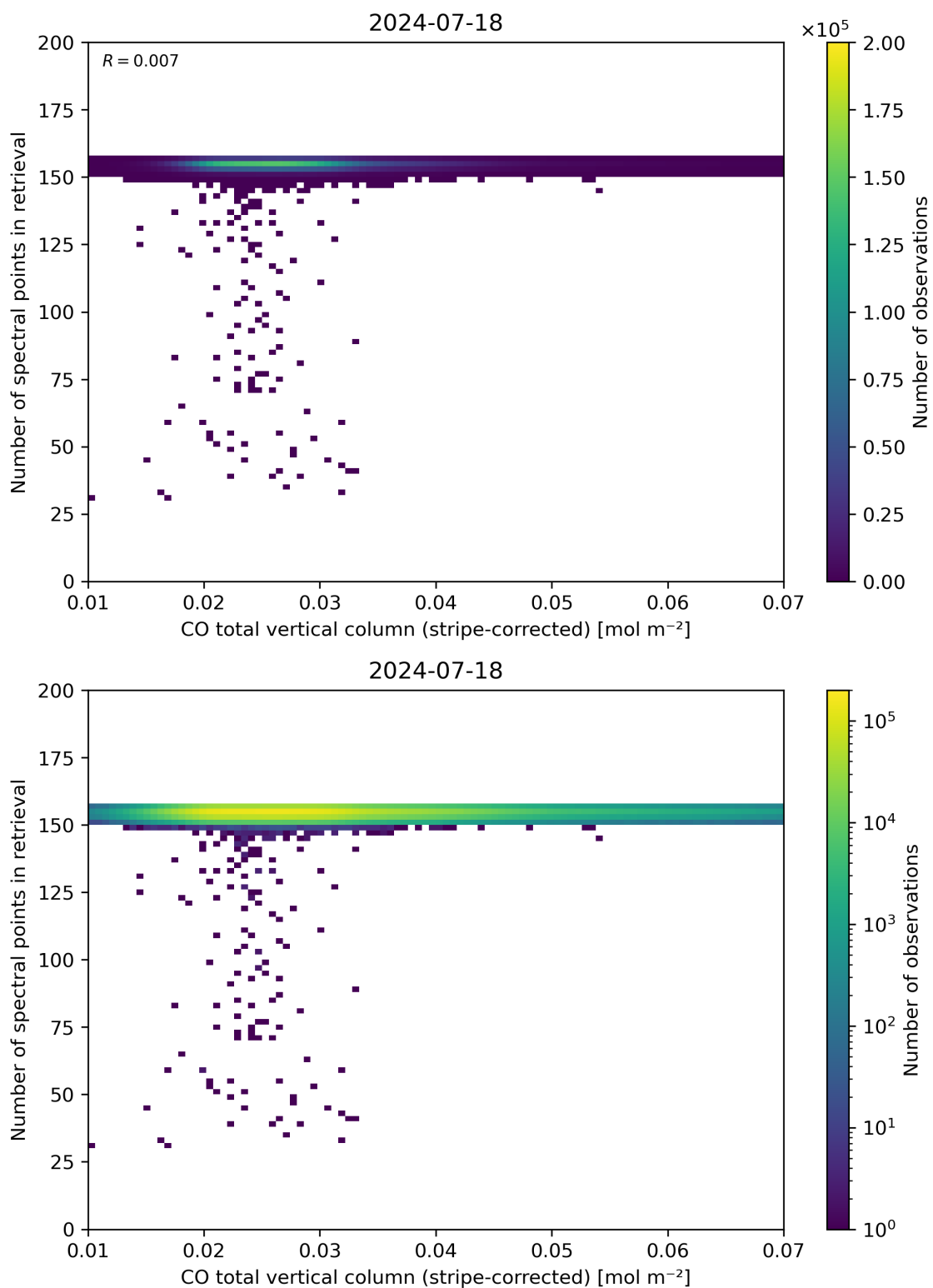
Figure 40: Scatter density plot of “CO total vertical column (stripe-corrected)” against “Number of spectral points in retrieval” for 2024-07-17 to 2024-07-19.
