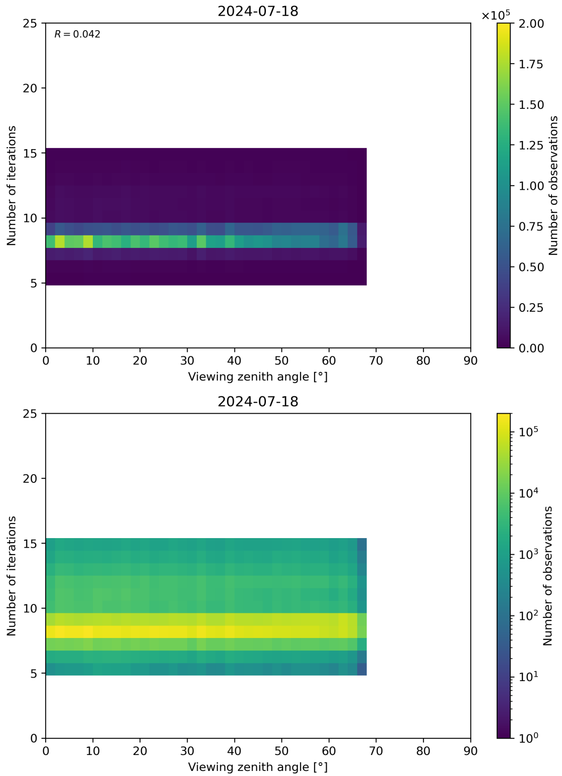
Figure 75: Scatter density plot of “Viewing zenith angle” against “Number of iterations” for 2024-07-17 to 2024-07-19.
