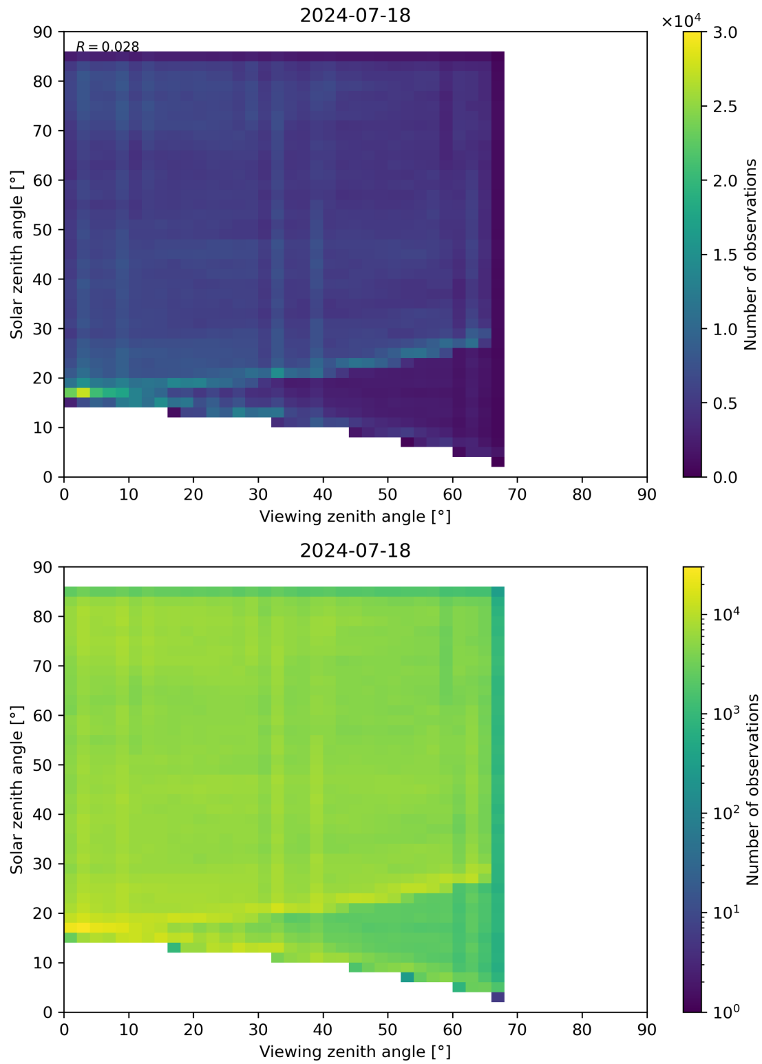
Figure 77: Scatter density plot of “Viewing zenith angle” against “Solar zenith angle” for 2024-07-17 to 2024-07-19.
