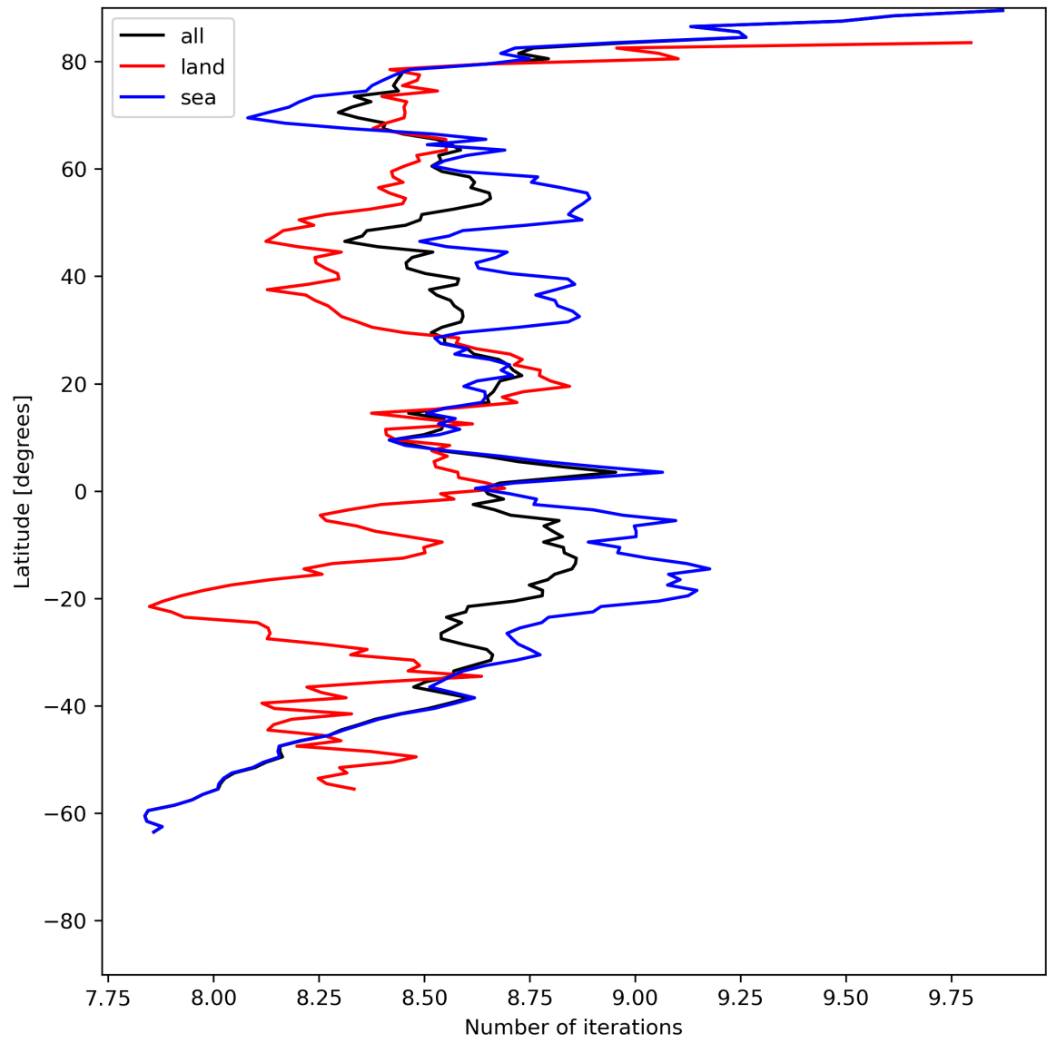
Figure 16: Zonal average of “Number of iterations” for 2024-07-17 to 2024-07-19.
