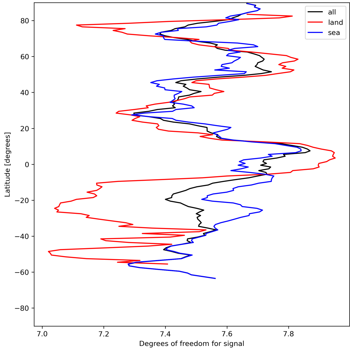
Figure 15: Zonal average of “Degrees of freedom for signal” for 2024-07-17 to 2024-07-19.
