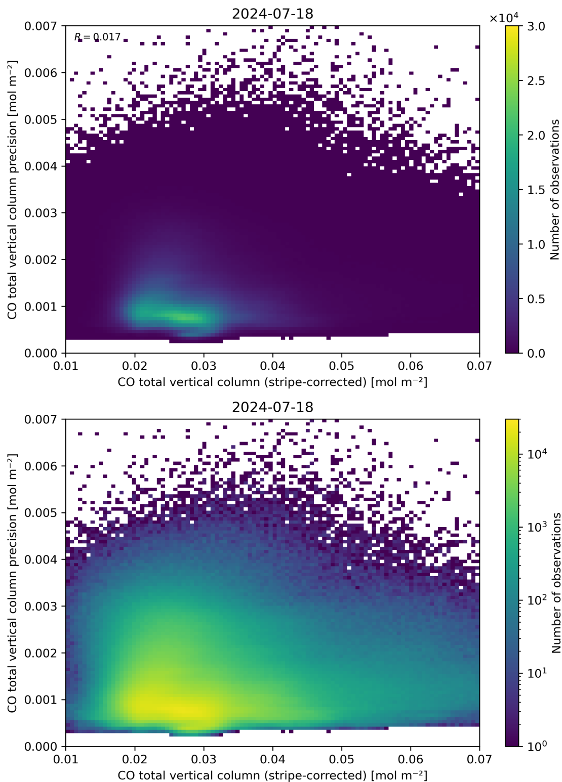
Figure 36: Scatter density plot of “CO total vertical column (stripe-corrected)” against “CO total vertical column precision” for 2024-07-17 to 2024-07-19.
