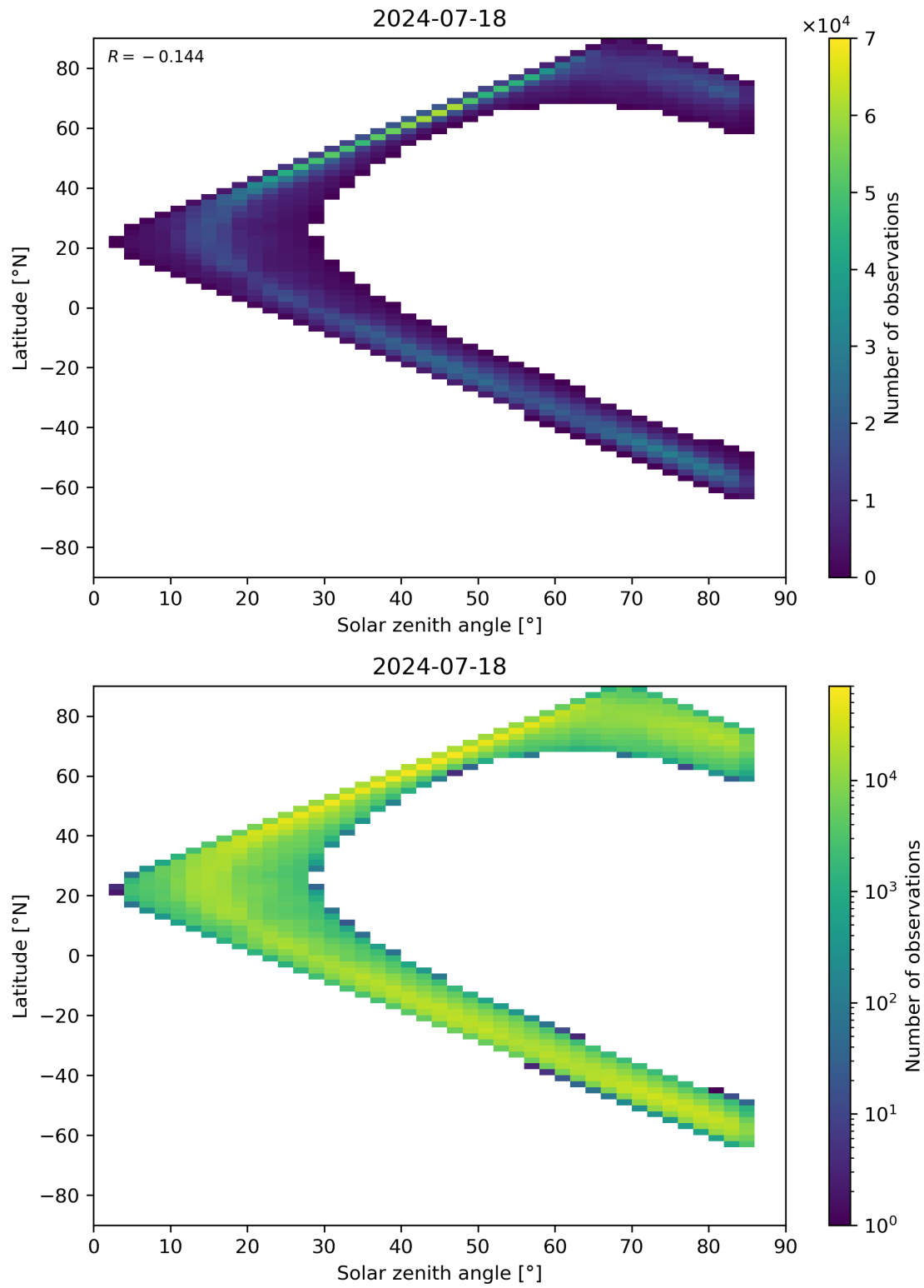
Figure 66: Scatter density plot of “Solar zenith angle” against “Latitude” for 2024-07-17 to 2024-07-19.
