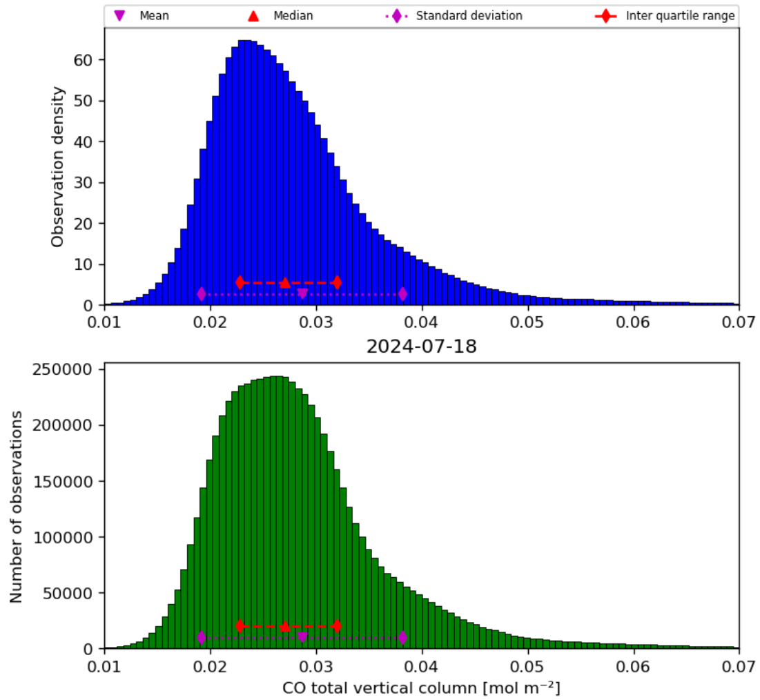
Figure 18: Histogram of “CO total vertical column” for 2024-07-17 to 2024-07-19
