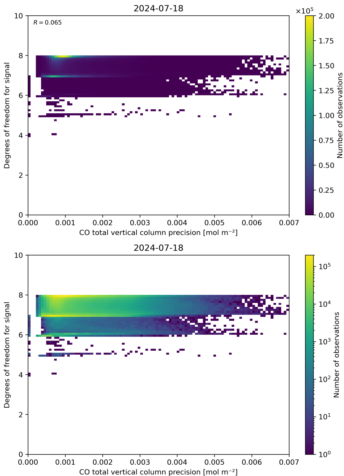
Figure 45: Scatter density plot of “CO total vertical column precision” against “Degrees of freedom for signal” for 2024-07-17 to 2024-07-19.
