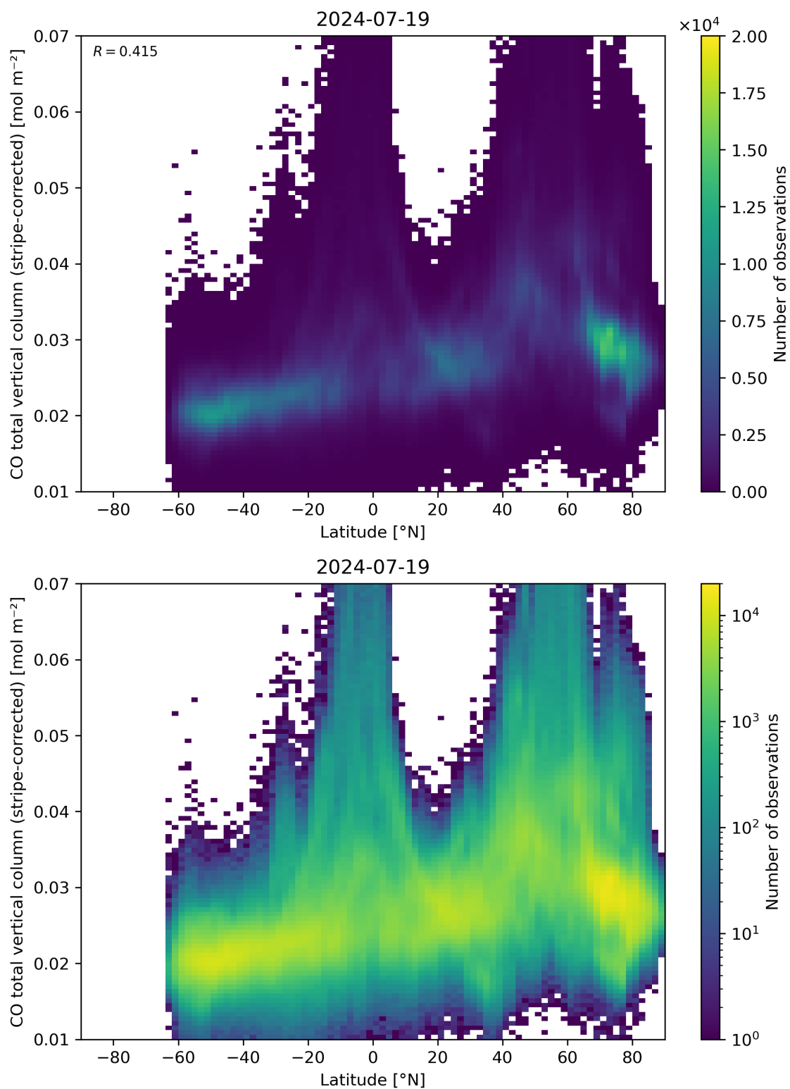
Figure 52: Scatter density plot of “Latitude” against “CO total vertical column (stripe-corrected)” for 2024-07-18 to 2024-07-20.
