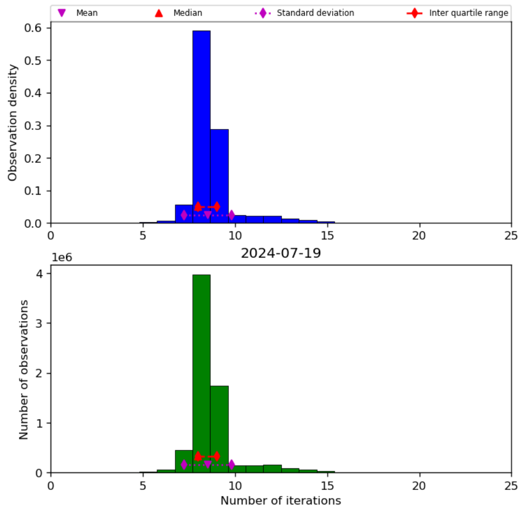
Figure 24: Histogram of “Number of iterations” for 2024-07-18 to 2024-07-20
