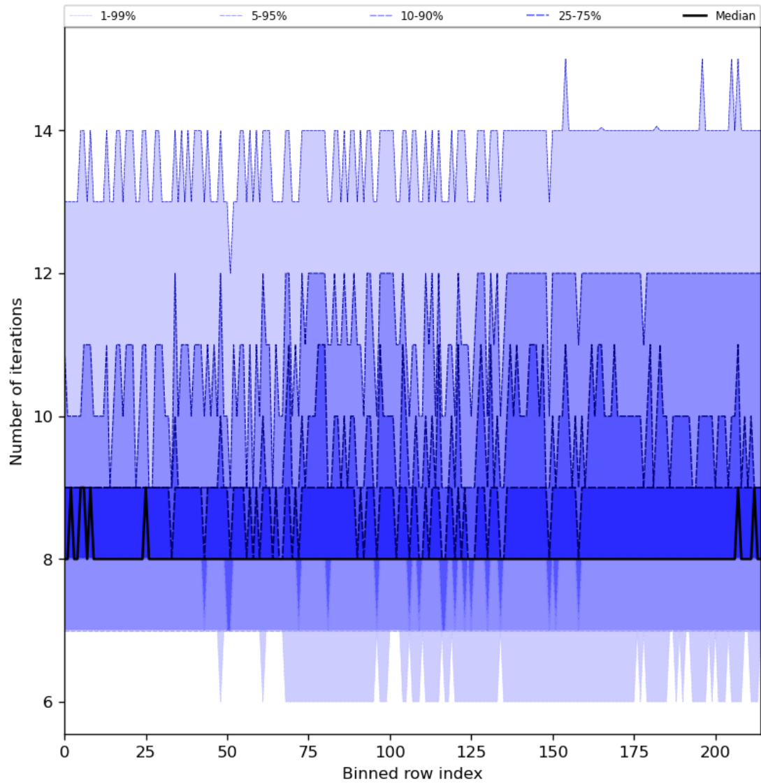
Figure 32: Along track statistics of “Number of iterations” for 2024-07-18 to 2024-07-20
