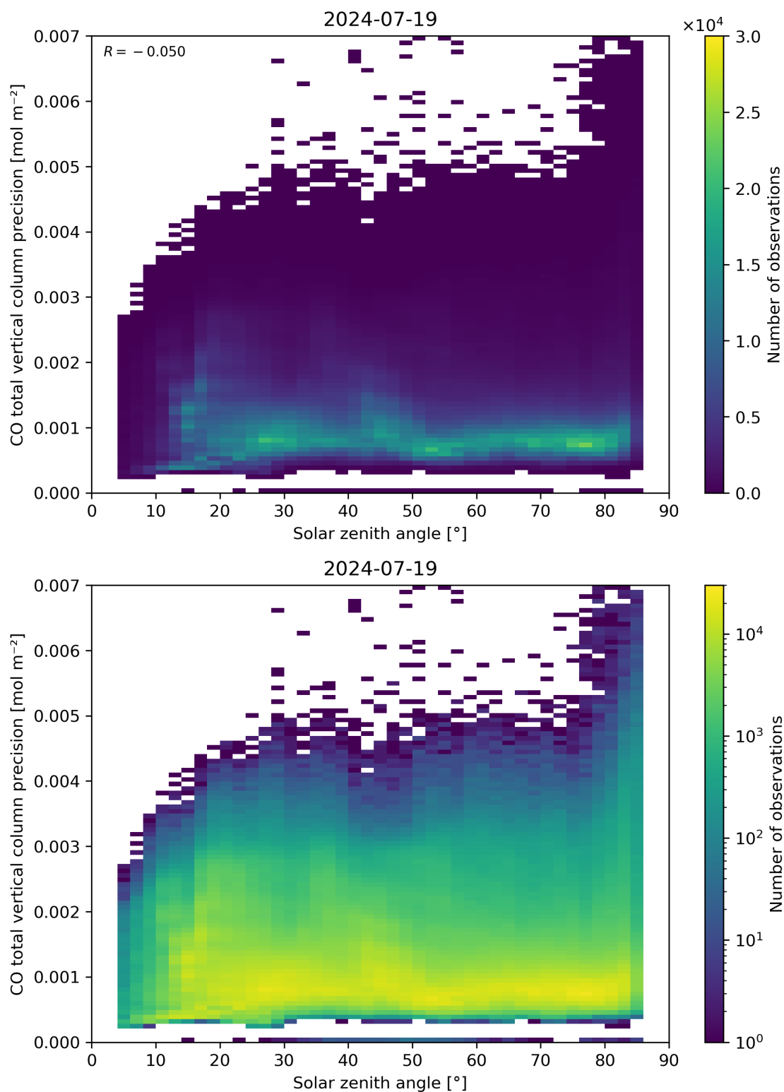
Figure 63: Scatter density plot of “Solar zenith angle” against “CO total vertical column precision” for 2024-07-18 to 2024-07-20.
