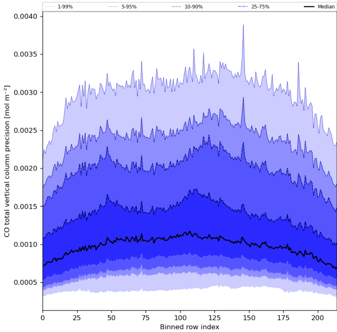
Figure 28: Along track statistics of “CO total vertical column precision” for 2024-07-18 to 2024-07-20
