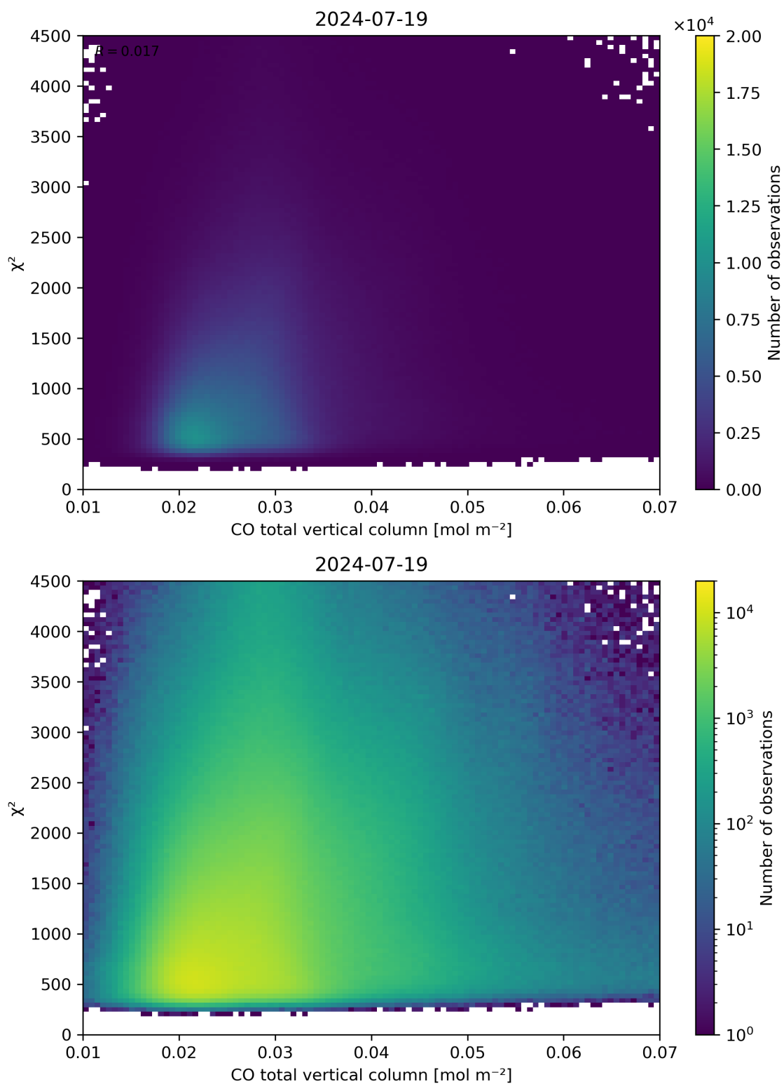
Figure 35: Scatter density plot of “CO total vertical column” against “ \chi^2 ” for 2024-07-18 to 2024-07-20.
