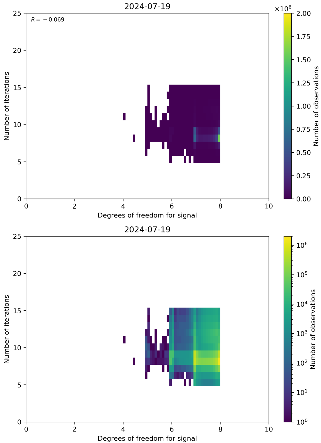
Figure 50: Scatter density plot of “Degrees of freedom for signal” against “Number of iterations” for 2024-07-18 to 2024-07-20.
