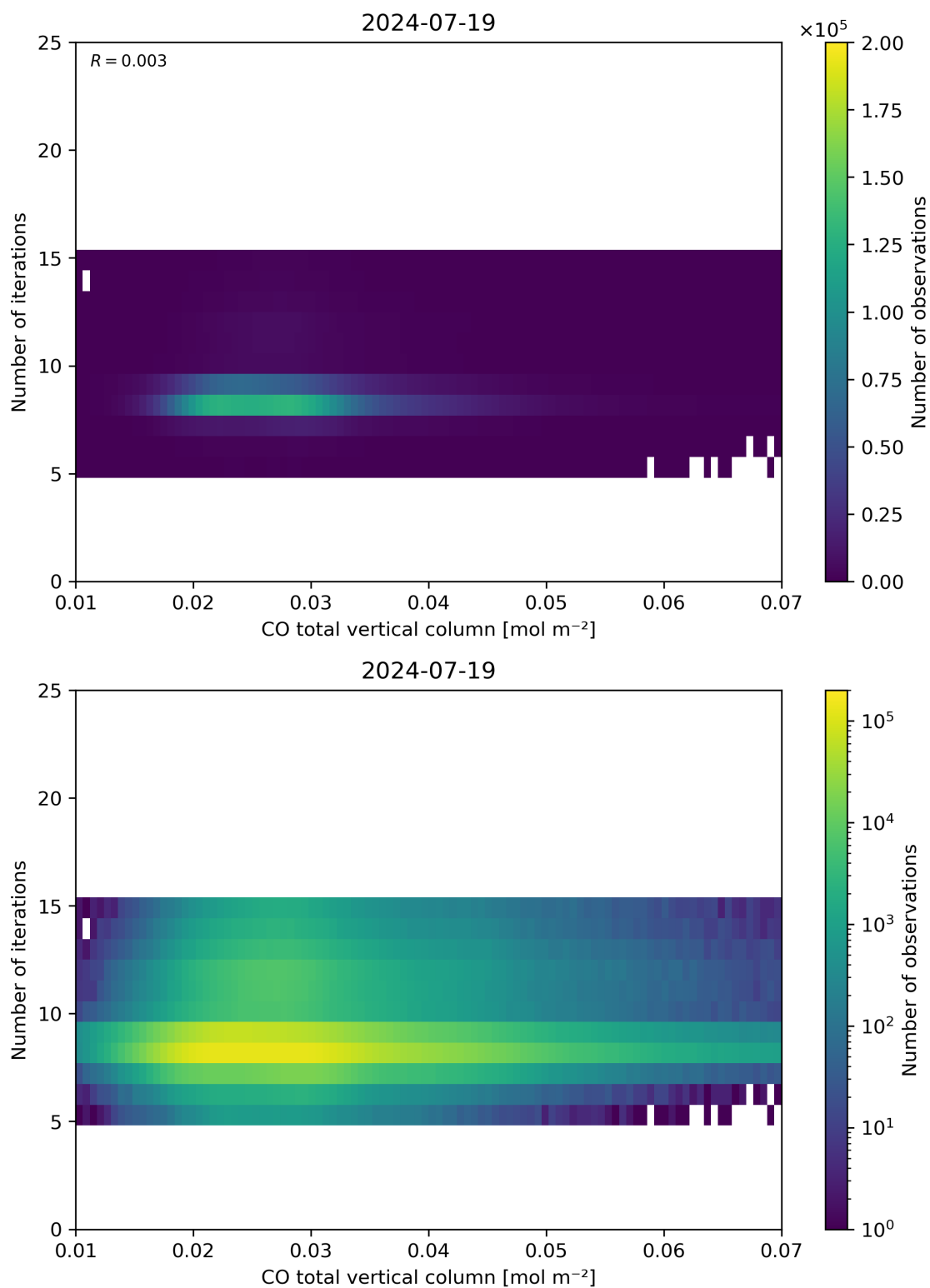
Figure 42: Scatter density plot of “CO total vertical column” against “Number of iterations” for 2024-07-18 to 2024-07-20.
