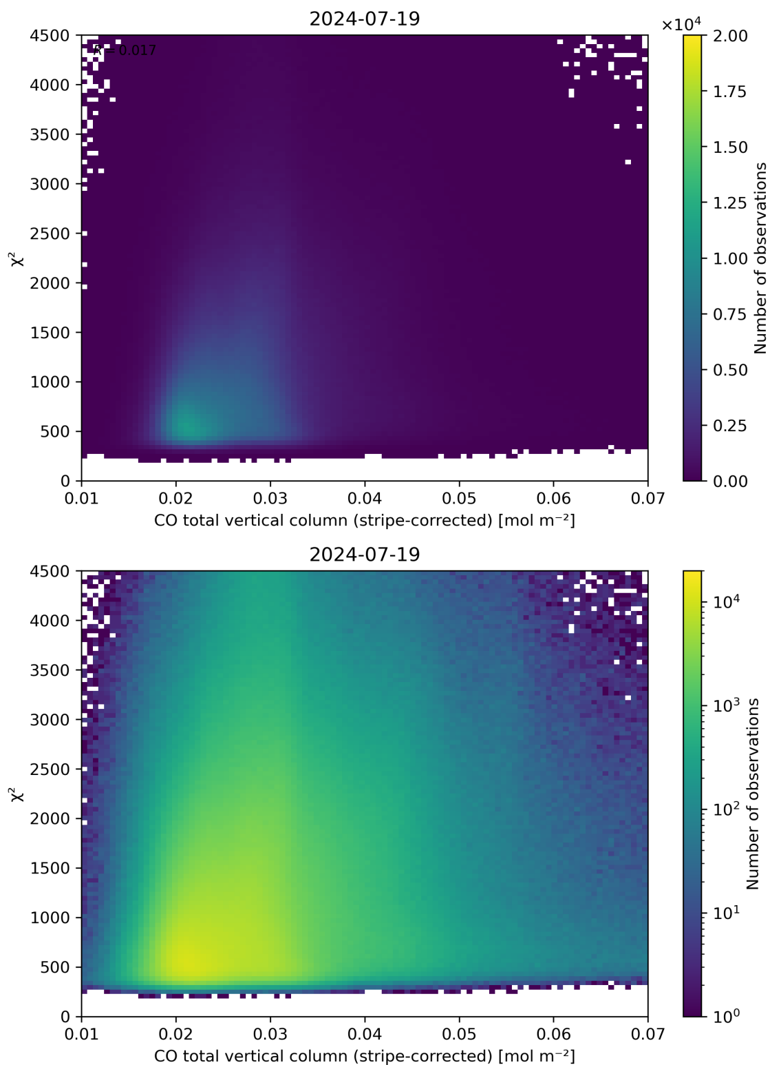
Figure 37: Scatter density plot of “CO total vertical column (stripe-corrected)” against “ \chi^2 ” for 2024-07-18 to 2024-07-20.
