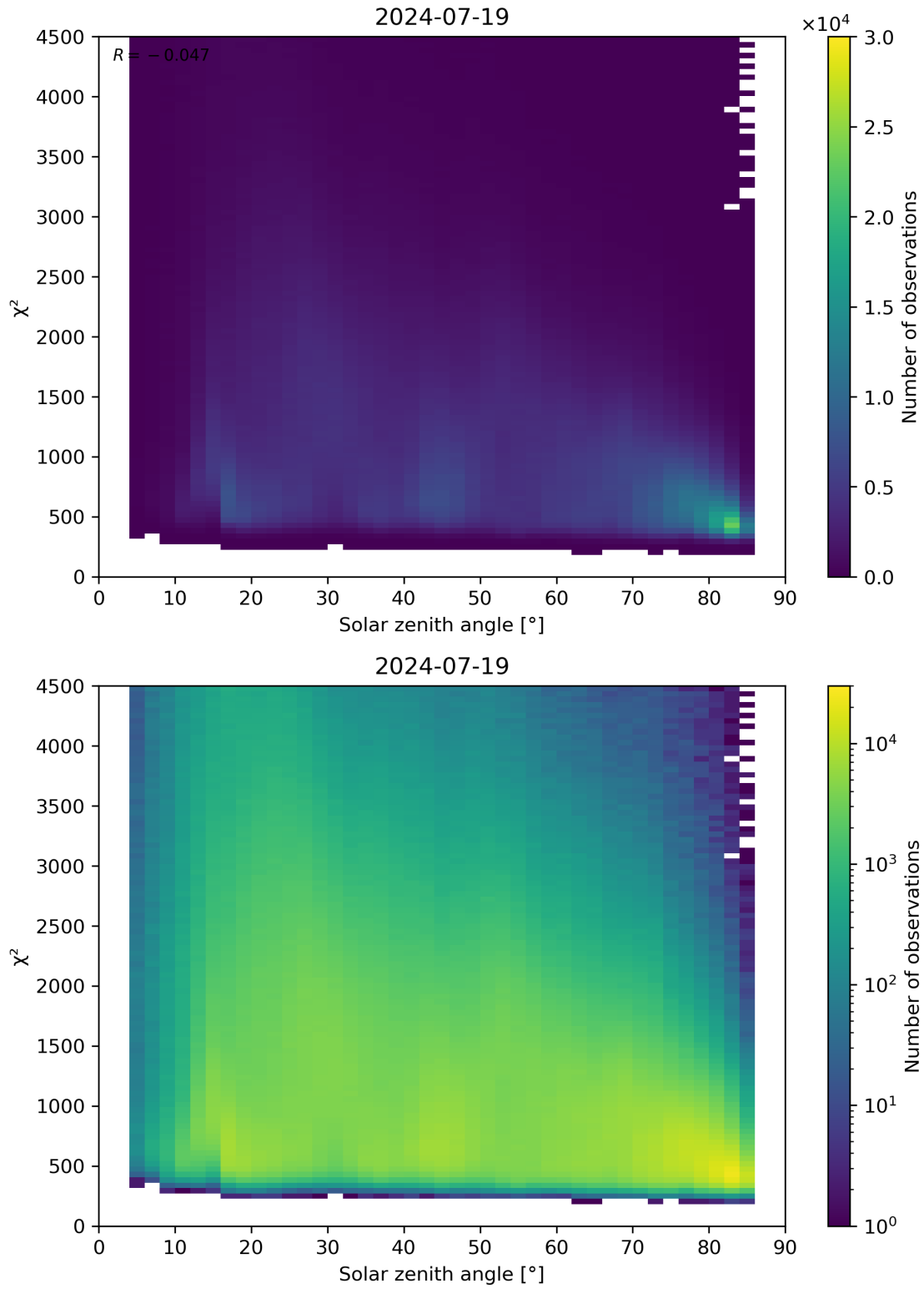
Figure 64: Scatter density plot of “Solar zenith angle” against “ \chi^2 ” for 2024-07-18 to 2024-07-20.
