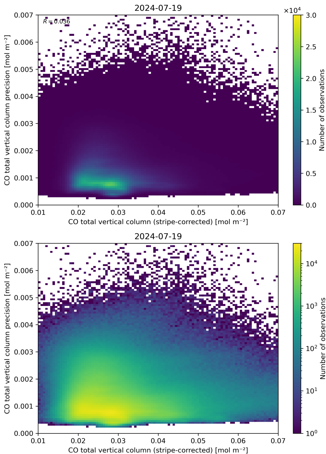
Figure 36: Scatter density plot of “CO total vertical column (stripe-corrected)” against “CO total vertical column precision” for 2024-07-18 to 2024-07-20.
