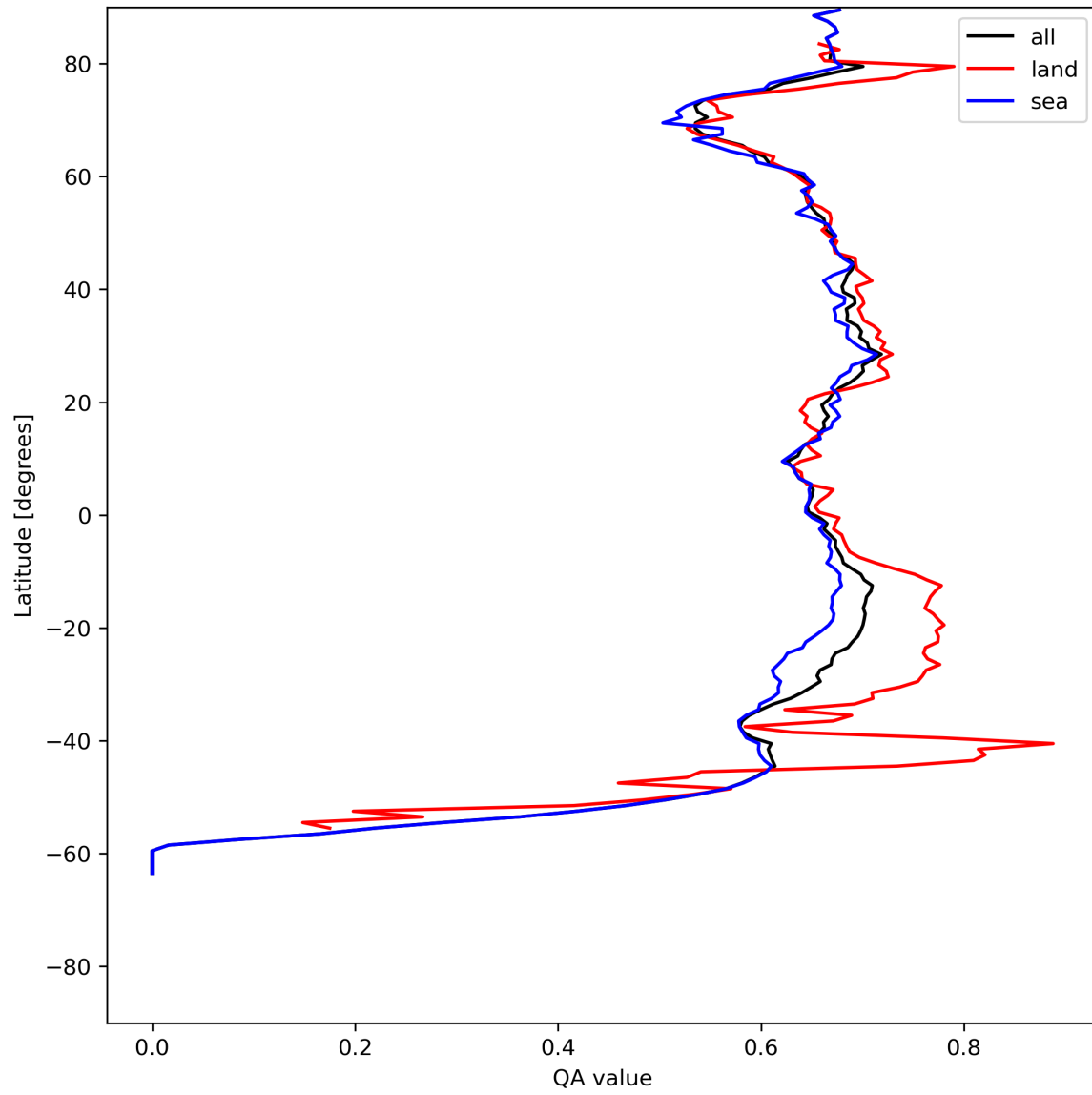
Figure 9: Zonal average of “QA value” for 2024-07-18 to 2024-07-20.
