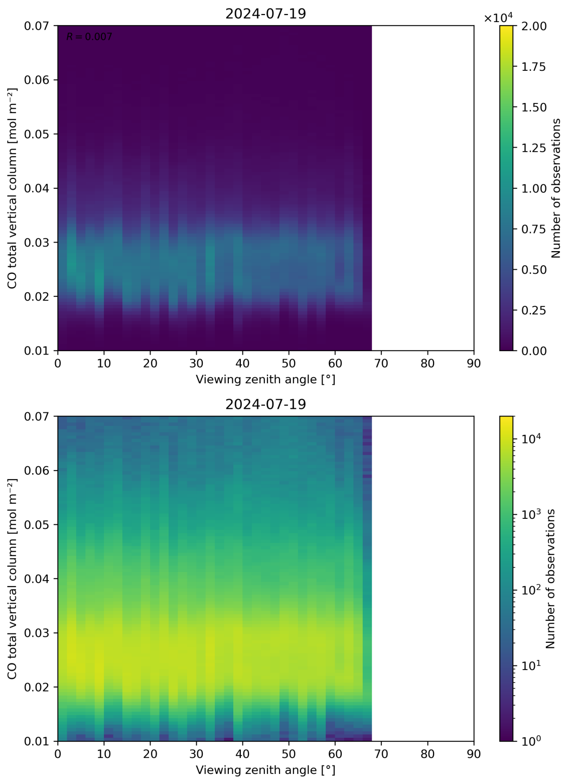
Figure 69: Scatter density plot of “Viewing zenith angle” against “CO total vertical column” for 2024-07-18 to 2024-07-20.
