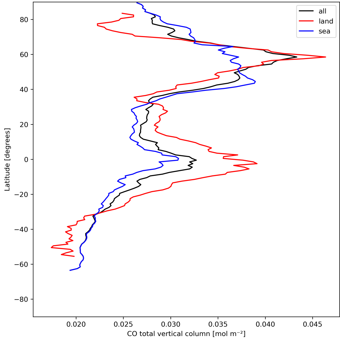
Figure 10: Zonal average of “CO total vertical column” for 2024-07-18 to 2024-07-20.
