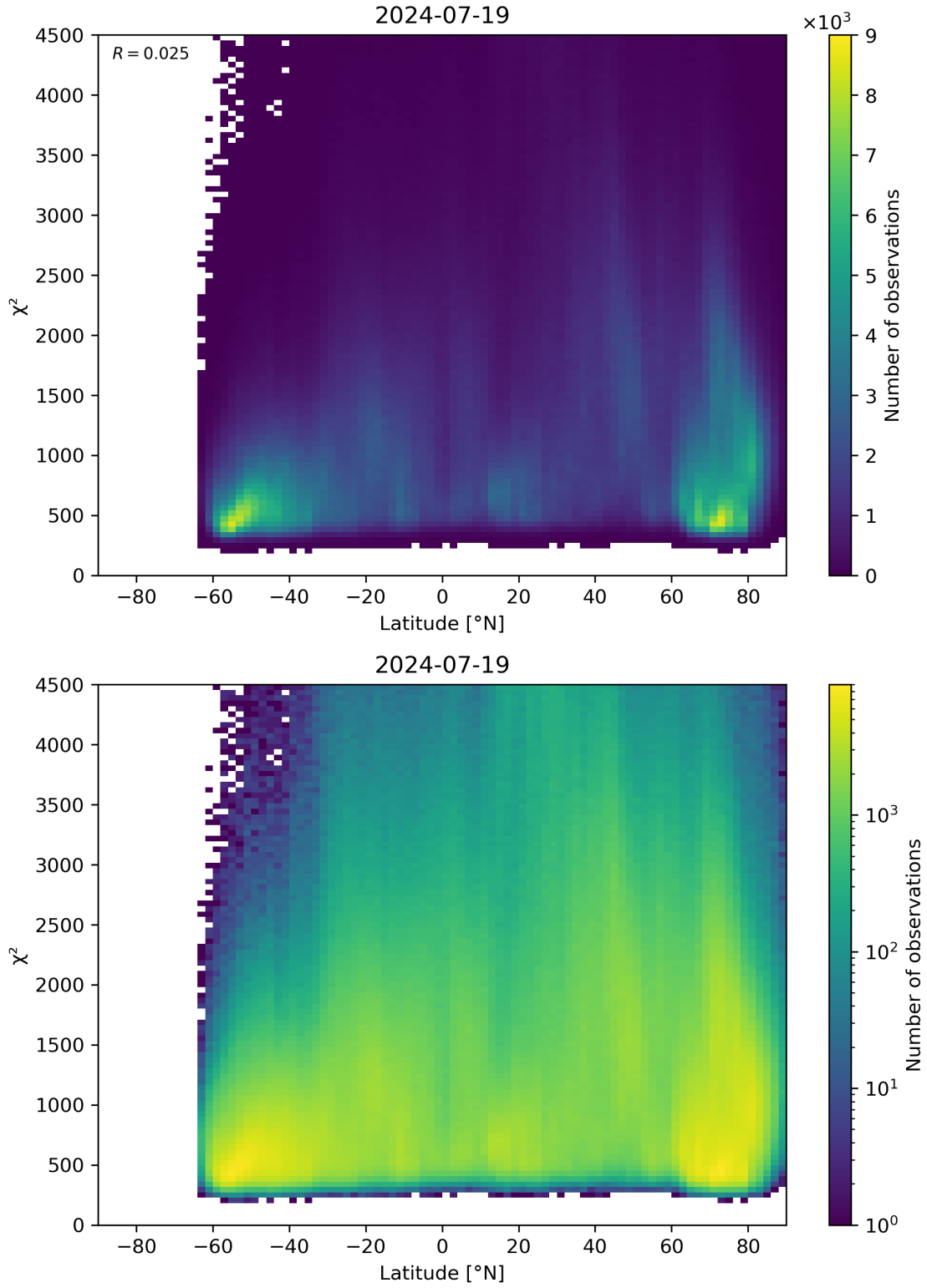
Figure 54: Scatter density plot of “Latitude” against “ \chi^2 ” for 2024-07-18 to 2024-07-20.
