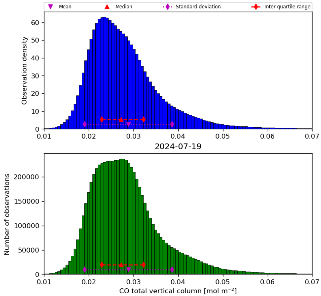
Figure 18: Histogram of “CO total vertical column” for 2024-07-18 to 2024-07-20
