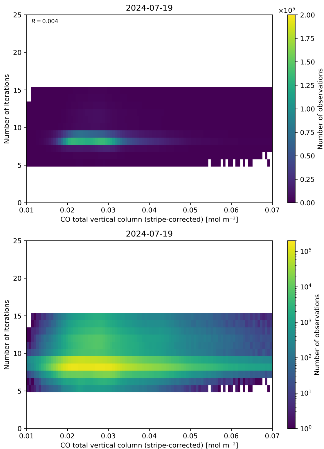
Figure 39: Scatter density plot of “CO total vertical column (stripe-corrected)” against “Number of iterations” for 2024-07-18 to 2024-07-20.
