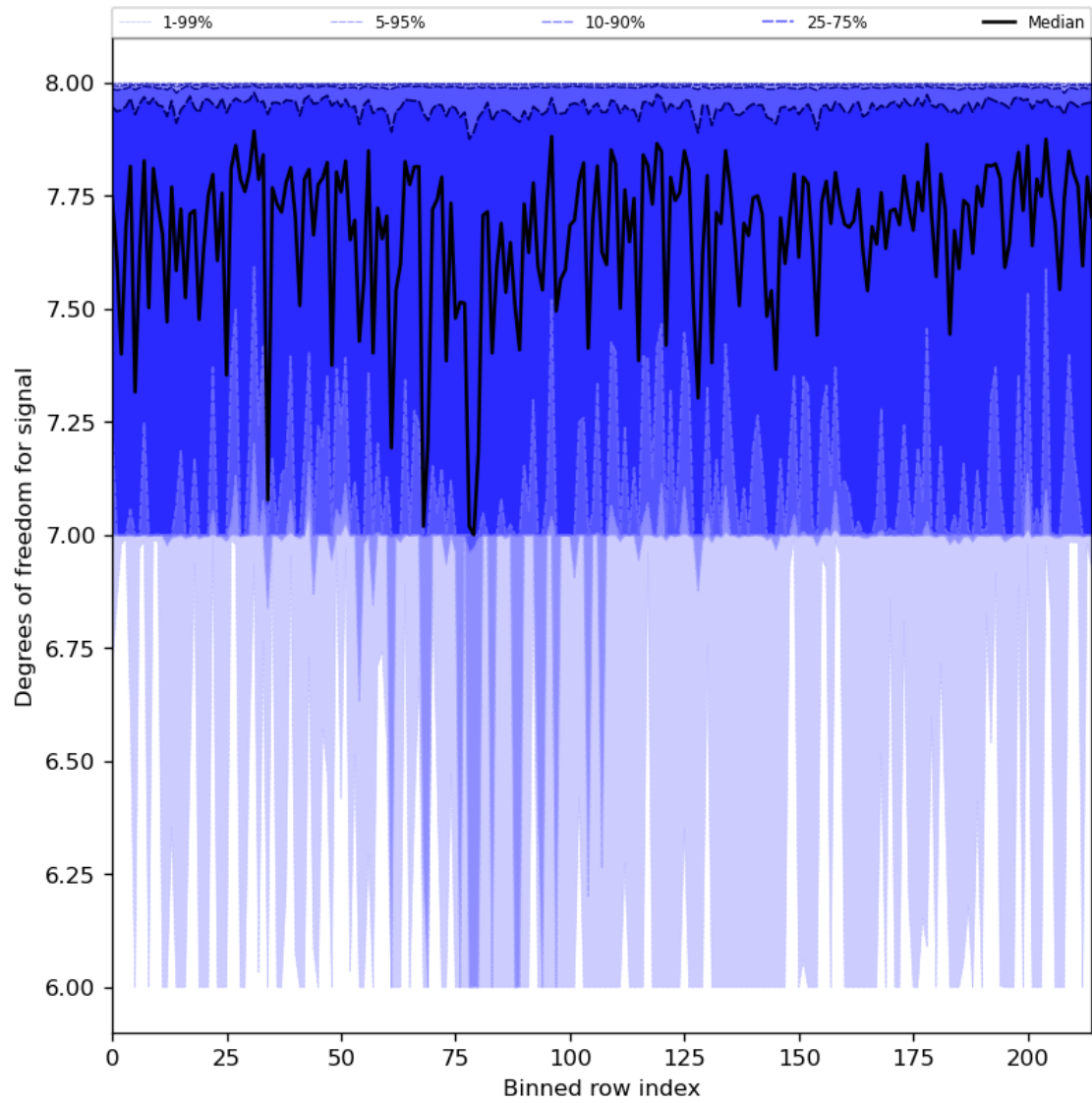
Figure 31: Along track statistics of “Degrees of freedom for signal” for 2024-07-18 to 2024-07-20
