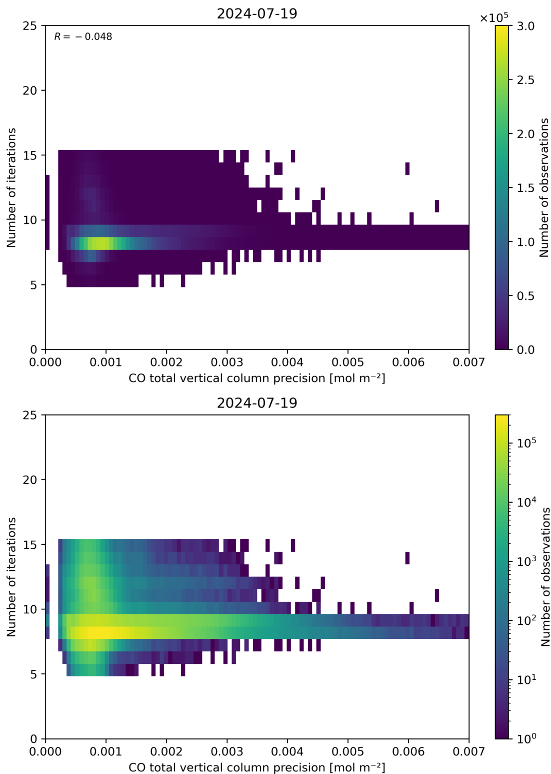
Figure 46: Scatter density plot of “CO total vertical column precision” against “Number of iterations” for 2024-07-18 to 2024-07-20.
