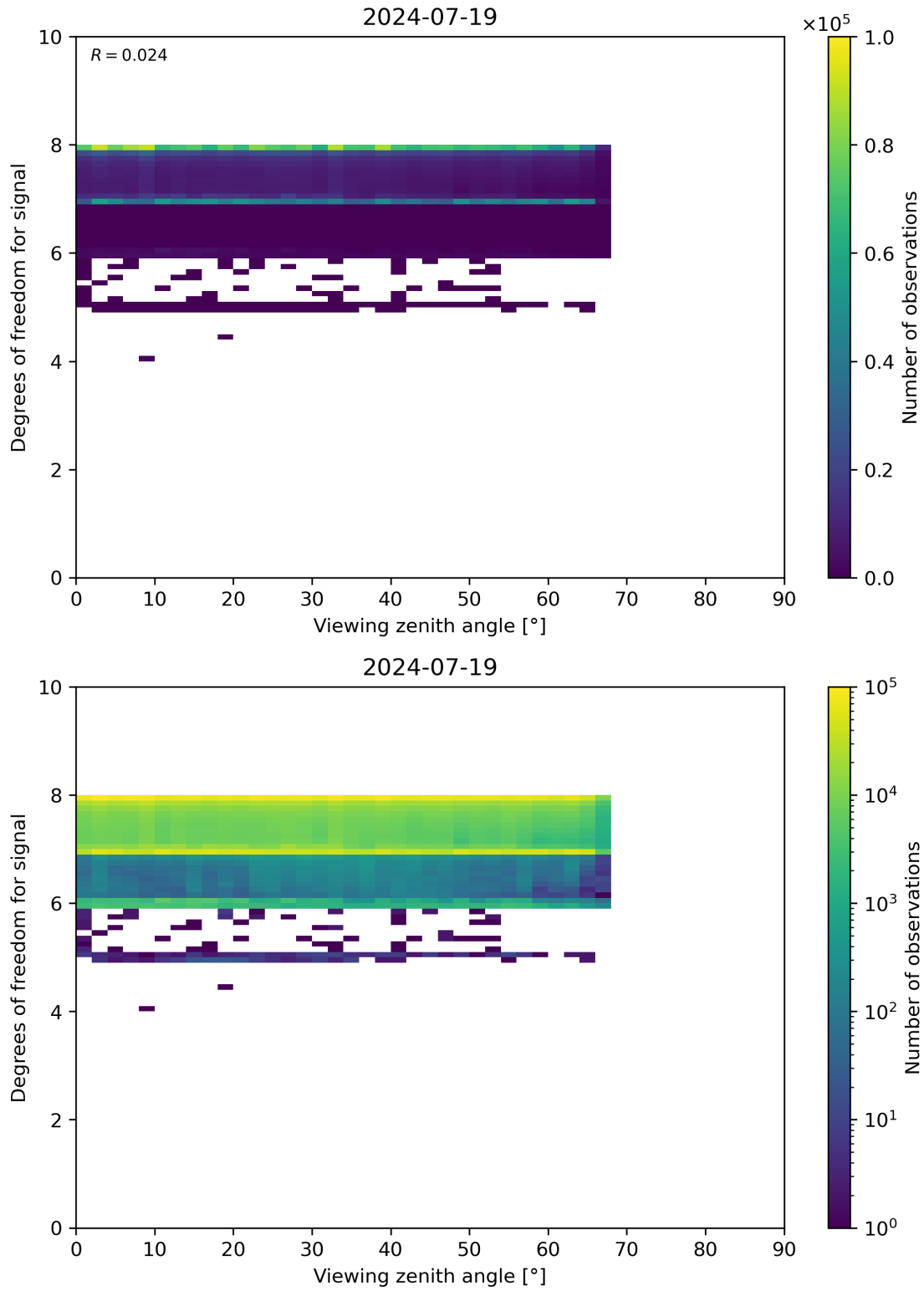
Figure 73: Scatter density plot of “Viewing zenith angle” against “Degrees of freedom for signal” for 2024-07-18 to 2024-07-20.
