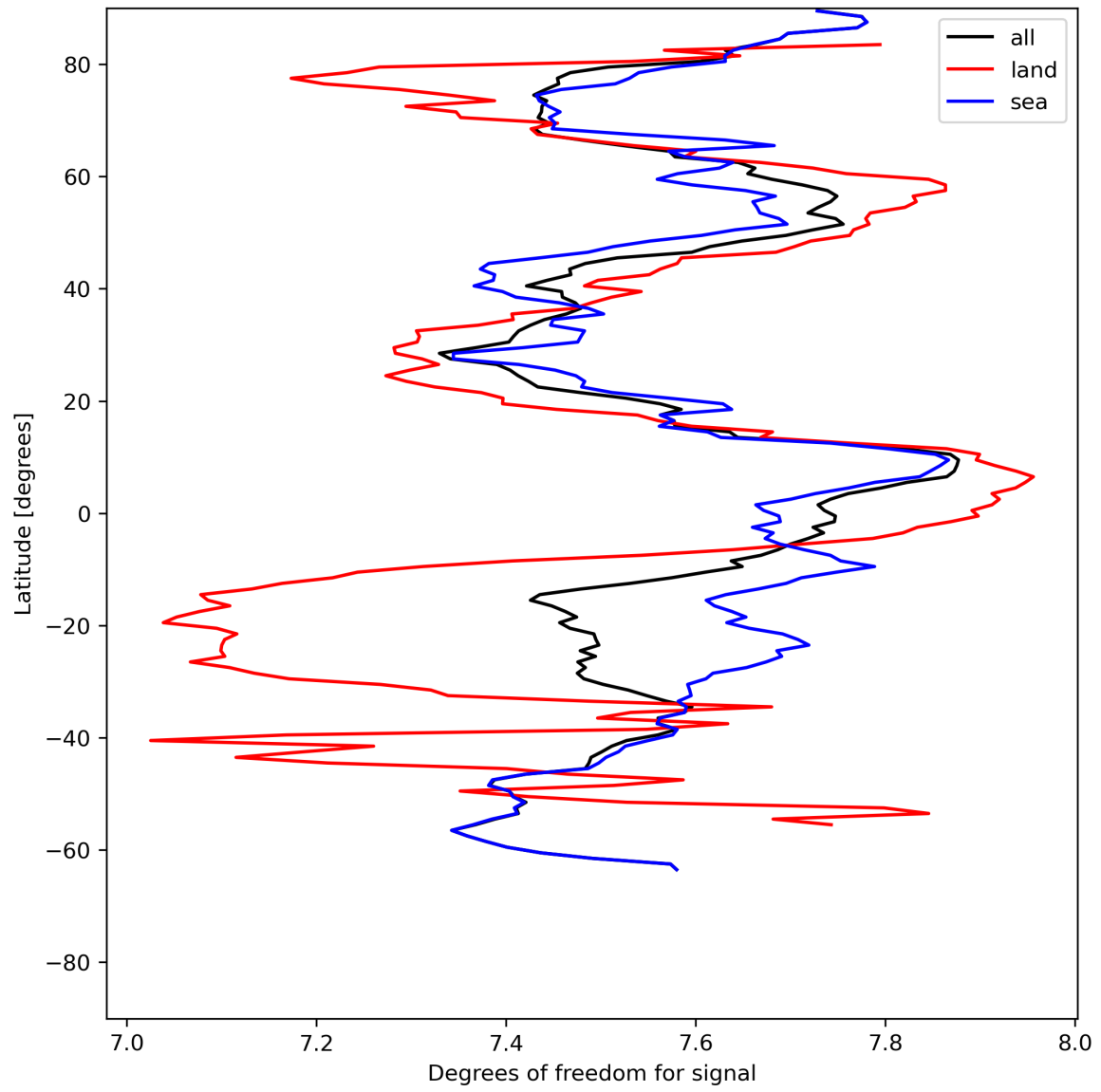
Figure 15: Zonal average of “Degrees of freedom for signal” for 2024-07-18 to 2024-07-20.
