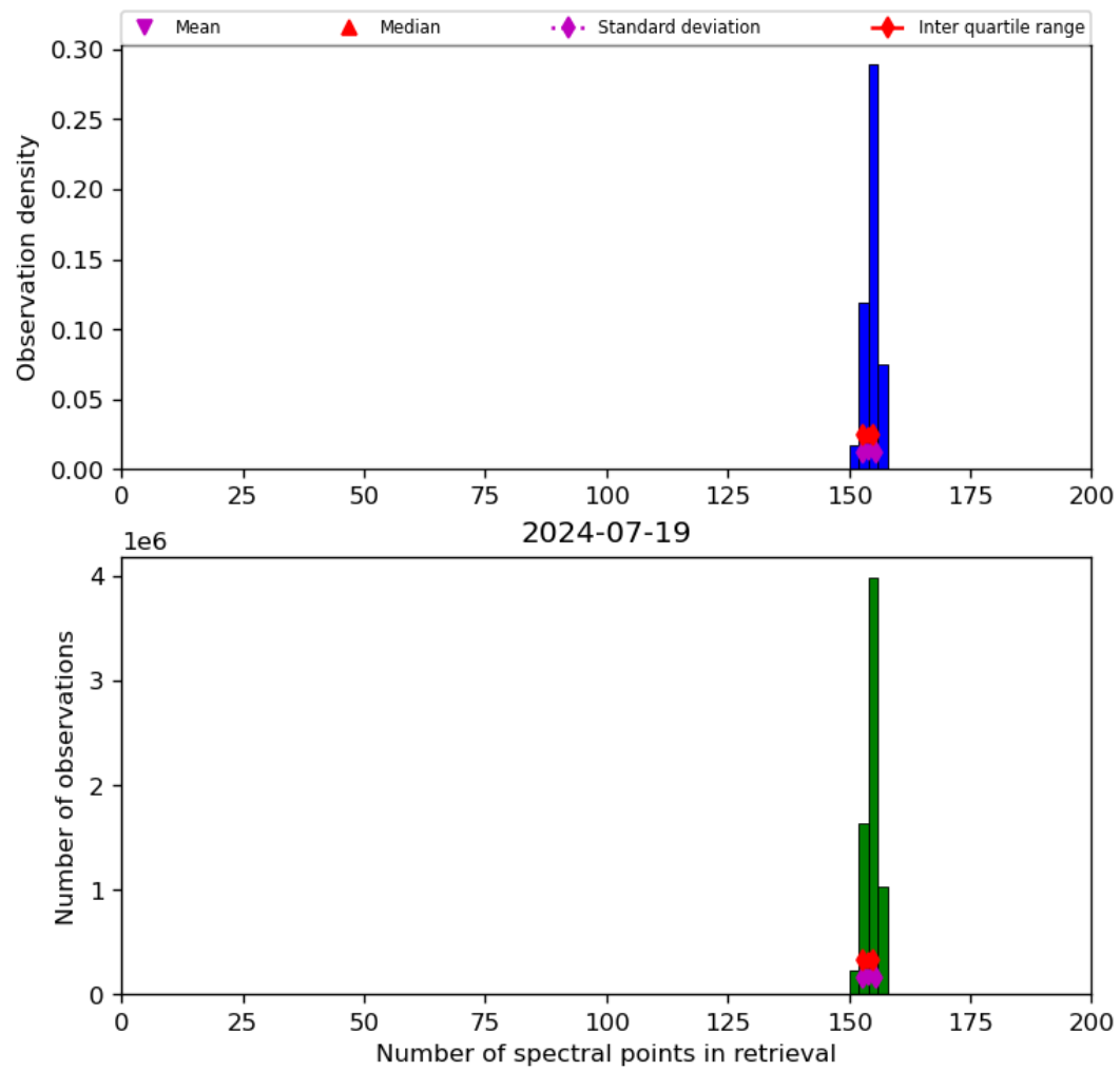
Figure 21: Histogram of “Number of spectral points in retrieval” for 2024-07-18 to 2024-07-20
