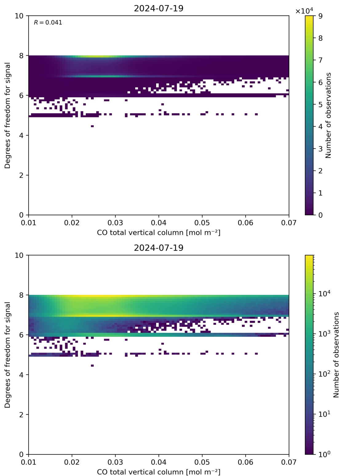
Figure 41: Scatter density plot of “CO total vertical column” against “Degrees of freedom for signal” for 2024-07-18 to 2024-07-20.
