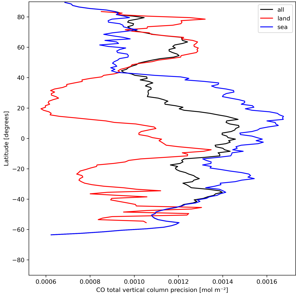
Figure 12: Zonal average of “CO total vertical column precision” for 2024-07-18 to 2024-07-20.
