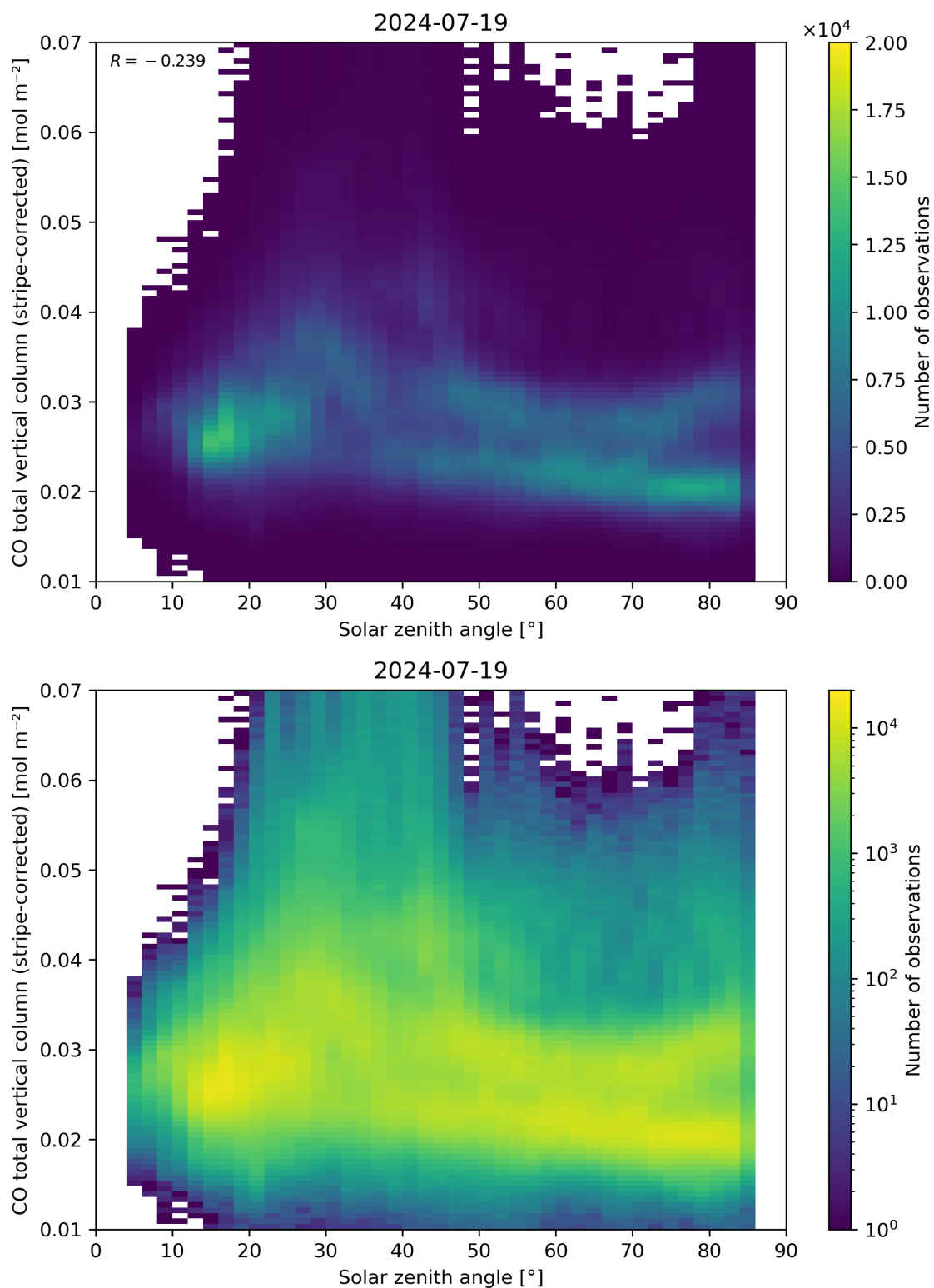
Figure 62: Scatter density plot of “Solar zenith angle” against “CO total vertical column (stripe-corrected)” for 2024-07-18 to 2024-07-20.
