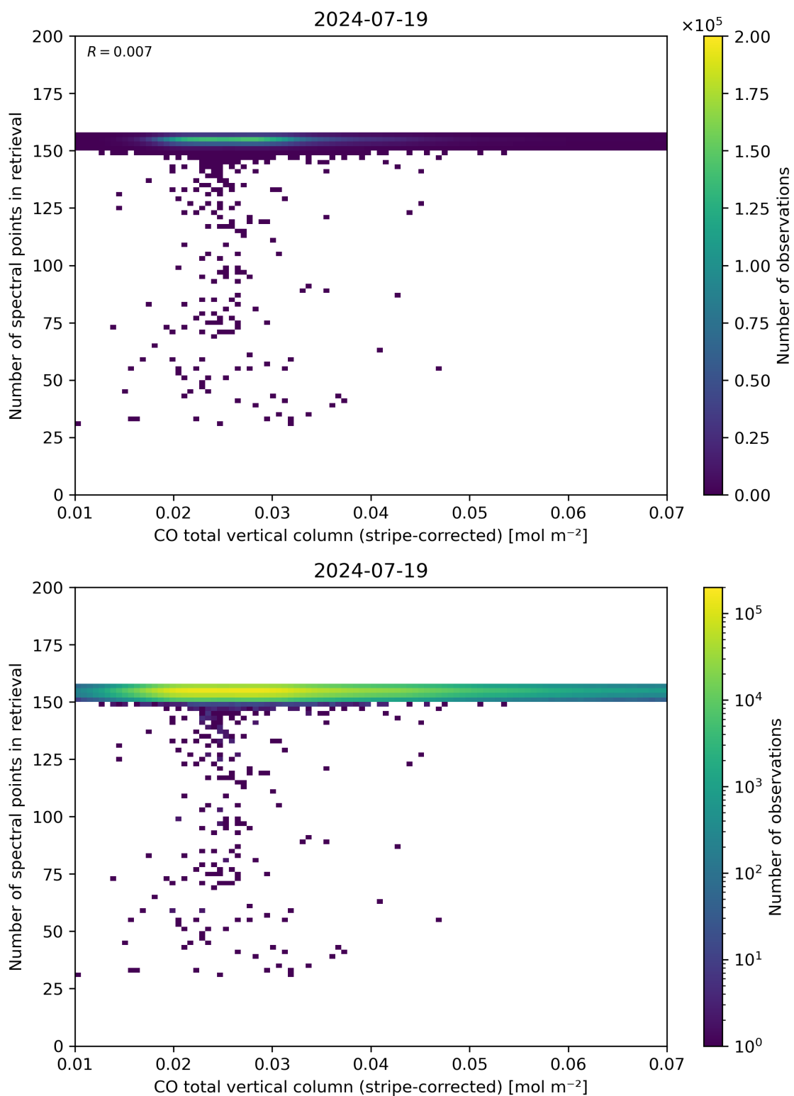
Figure 40: Scatter density plot of “CO total vertical column (stripe-corrected)” against “Number of spectral points in retrieval” for 2024-07-18 to 2024-07-20.
