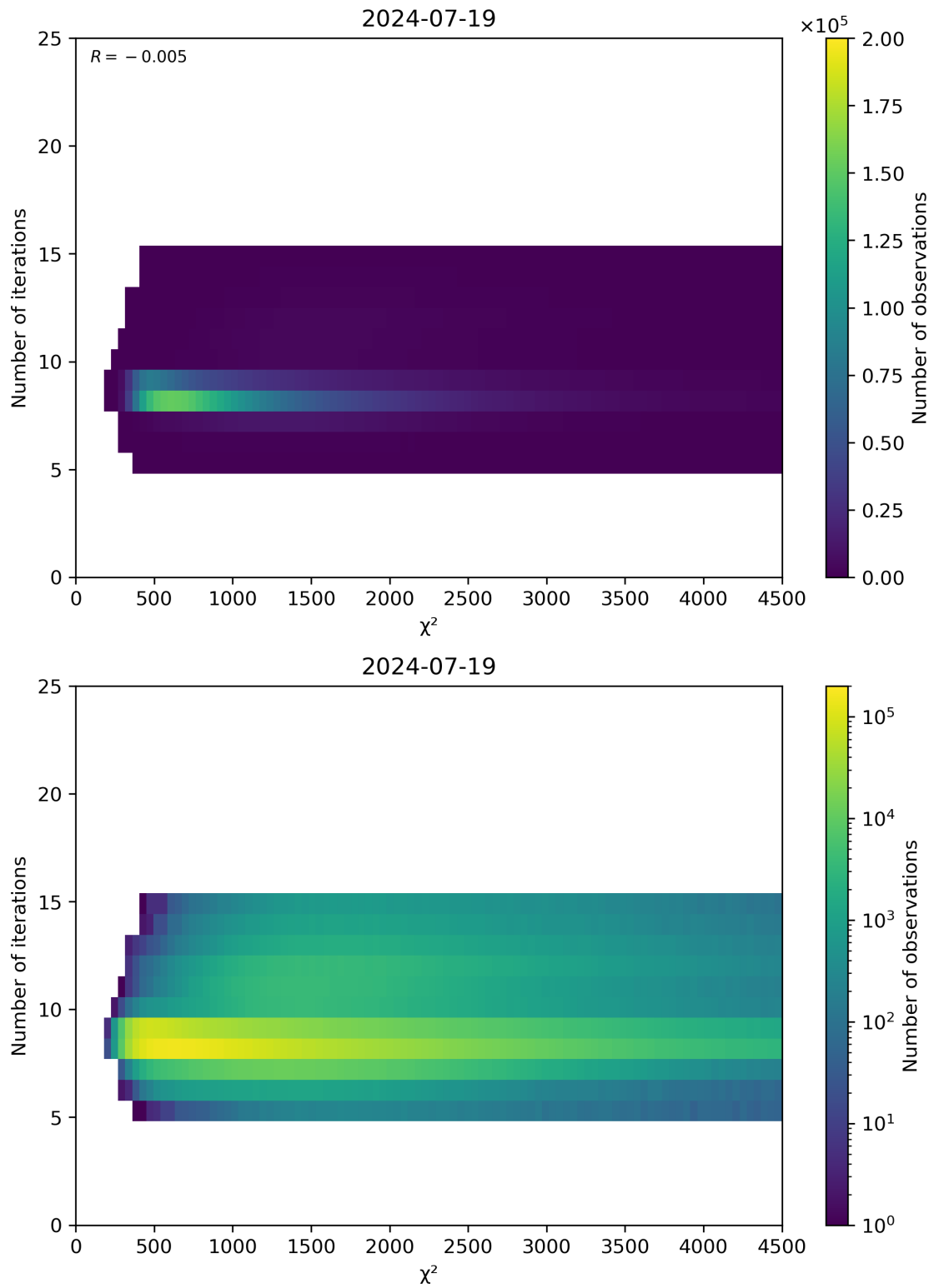
Figure 49: Scatter density plot of “ \chi^2 ” against “Number of iterations” for 2024-07-18 to 2024-07-20.
