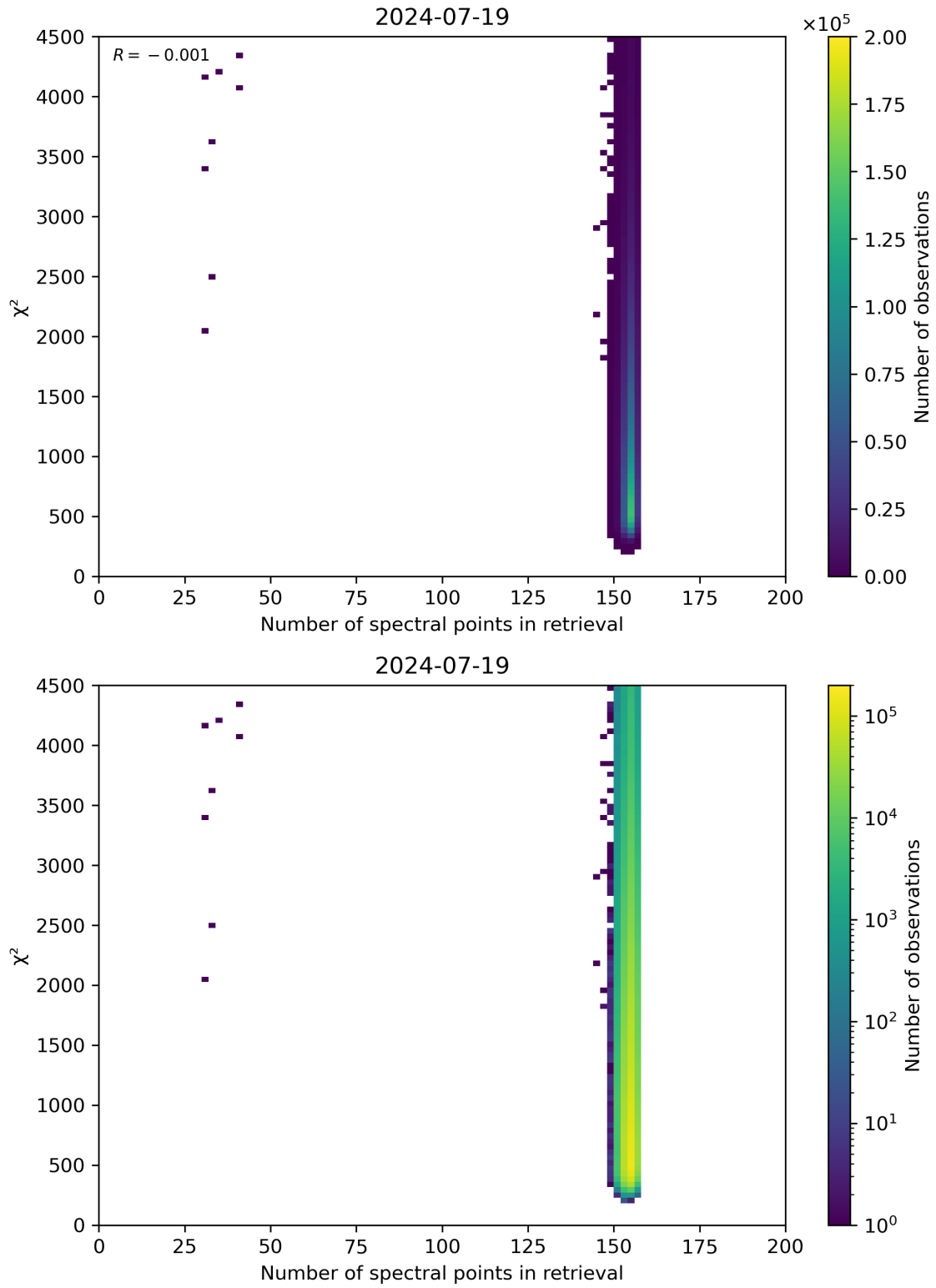
Figure 58: Scatter density plot of “Number of spectral points in retrieval” against “ \chi^2 ” for 2024-07-18 to 2024-07-20.
