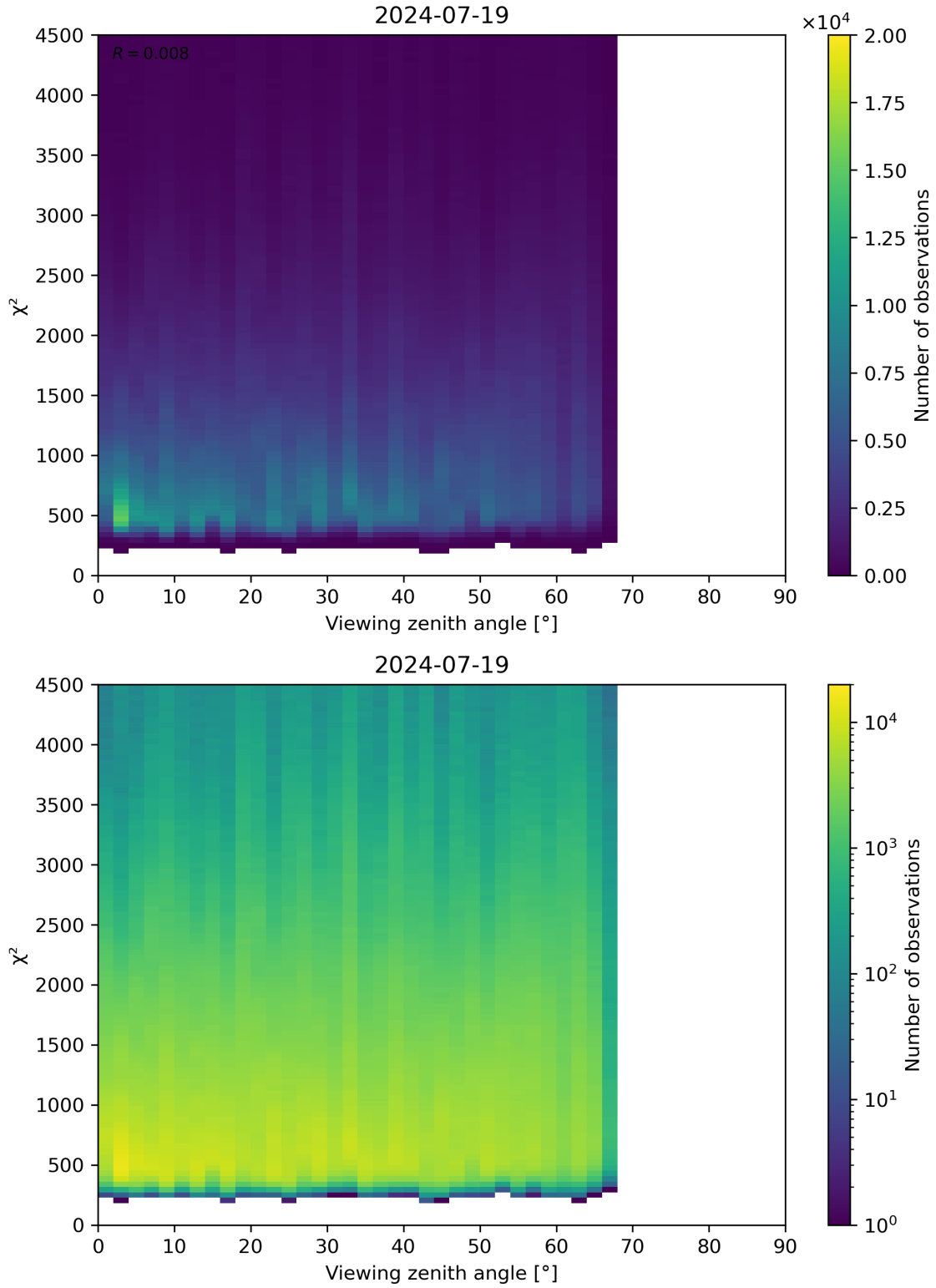
Figure 72: Scatter density plot of “Viewing zenith angle” against “ \chi^2 ” for 2024-07-18 to 2024-07-20.
