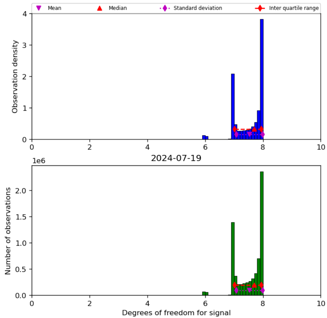
Figure 23: Histogram of “Degrees of freedom for signal” for 2024-07-18 to 2024-07-20
