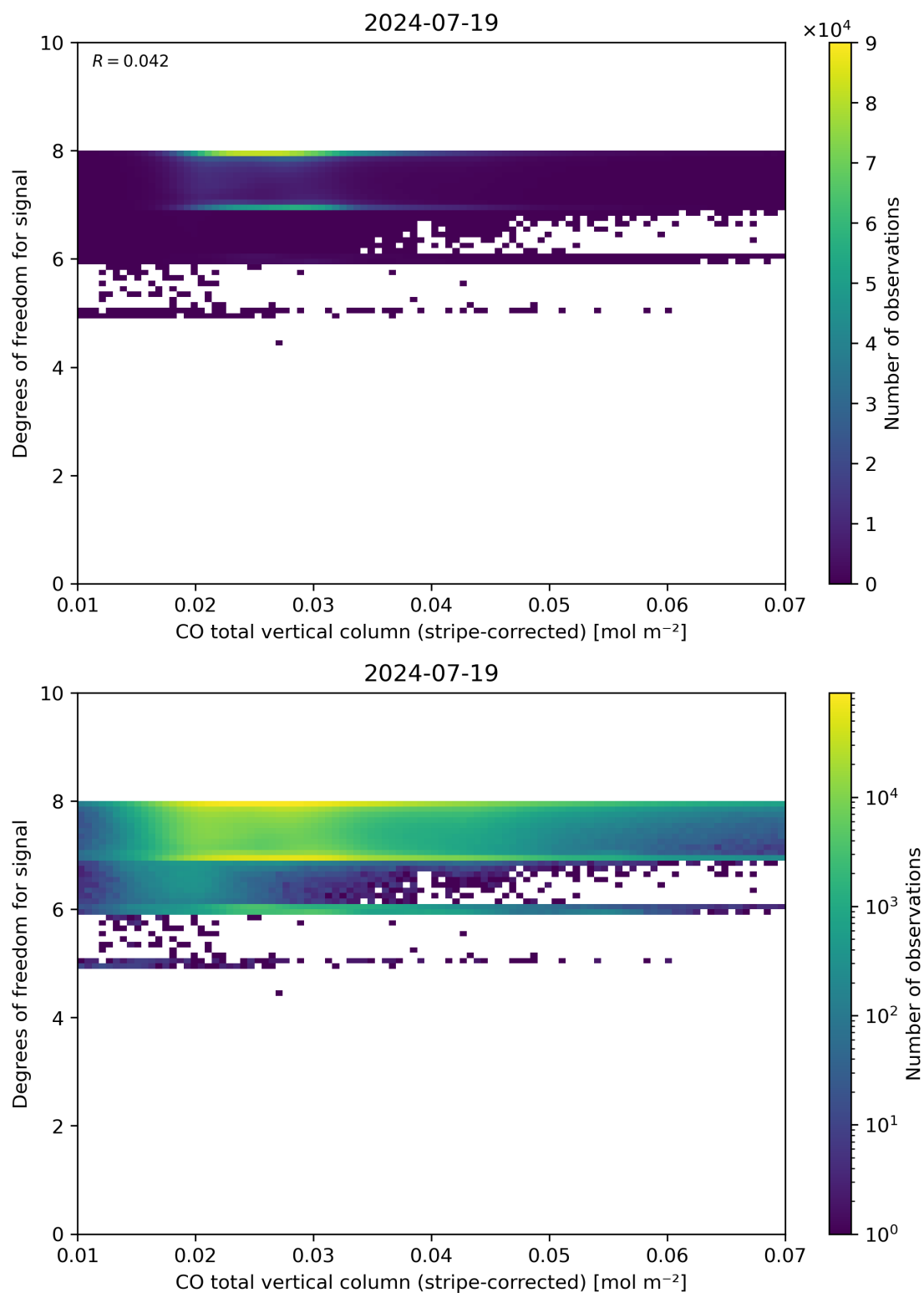
Figure 38: Scatter density plot of “CO total vertical column (stripe-corrected)” against “Degrees of freedom for signal” for 2024-07-18 to 2024-07-20.
