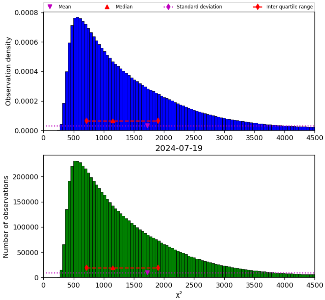
Figure 22: Histogram of “ \chi^2 ” for 2024-07-18 to 2024-07-20
