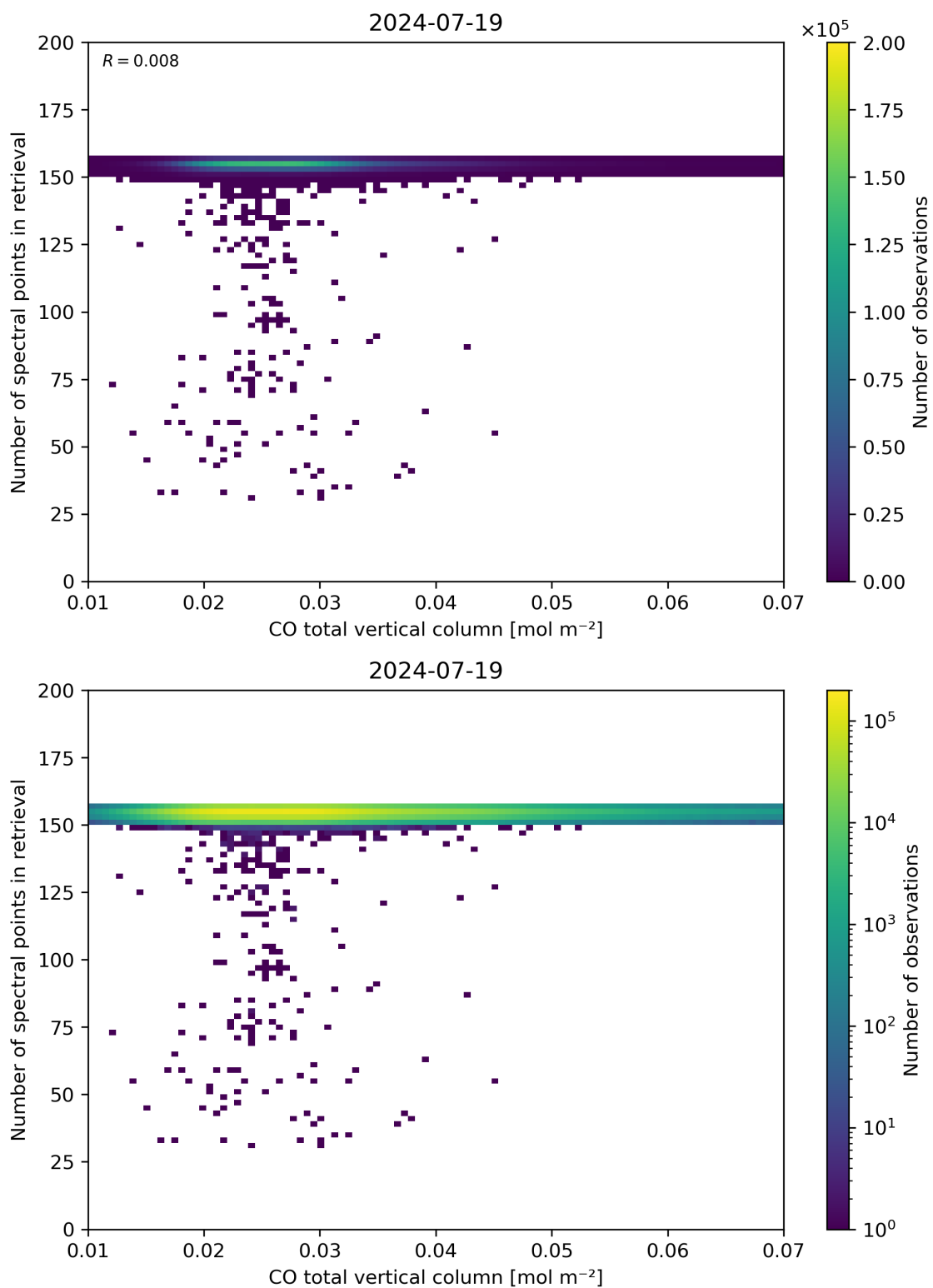
Figure 43: Scatter density plot of “CO total vertical column” against “Number of spectral points in retrieval” for 2024-07-18 to 2024-07-20.
