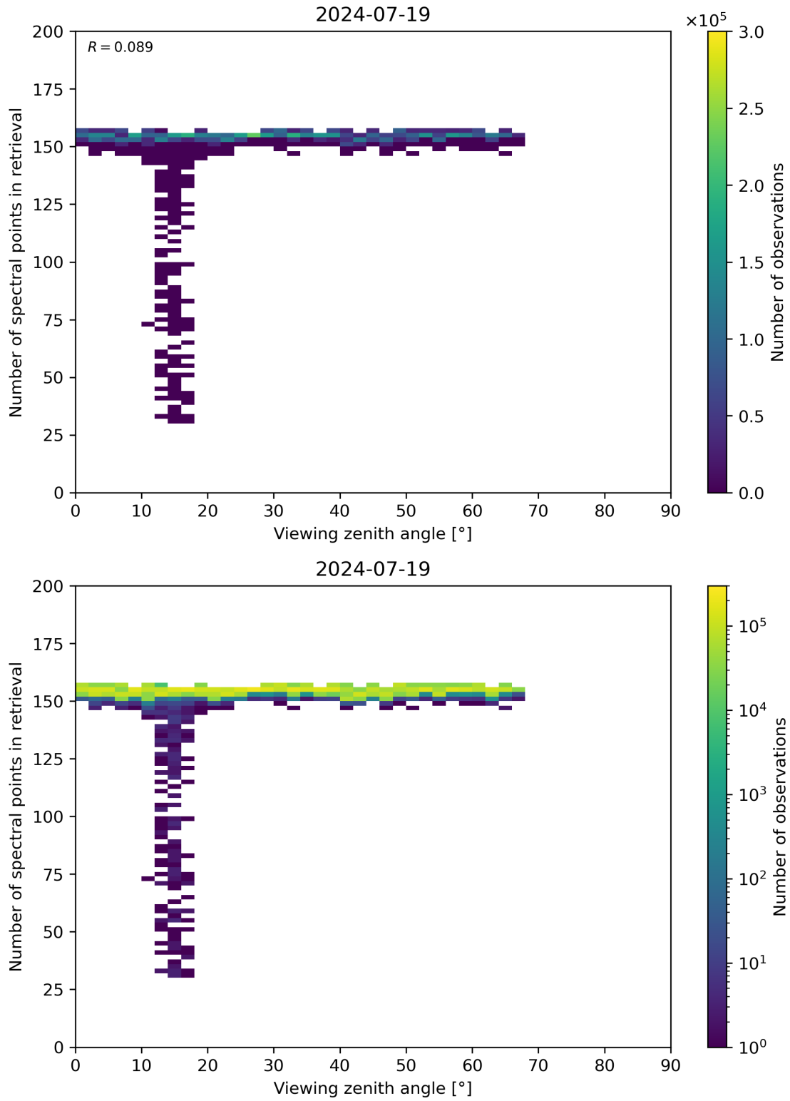
Figure 76: Scatter density plot of “Viewing zenith angle” against “Number of spectral points in retrieval” for 2024-07-18 to 2024-07-20.
