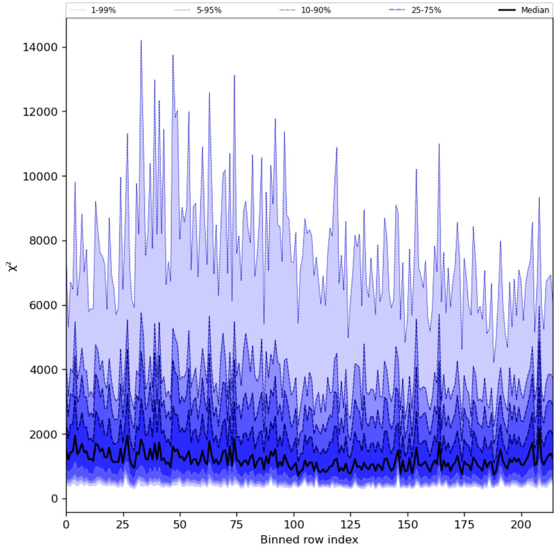
Figure 30: Along track statistics of “ \chi^2 ” for 2024-07-18 to 2024-07-20
