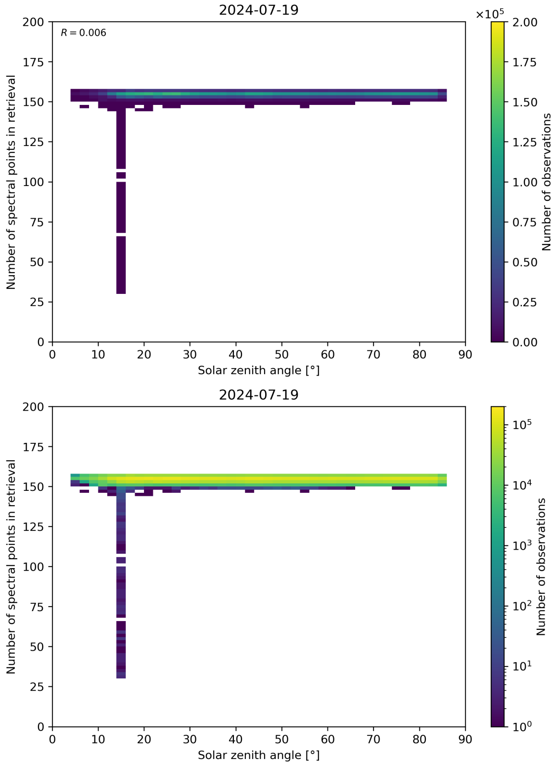
Figure 68: Scatter density plot of “Solar zenith angle” against “Number of spectral points in retrieval” for 2024-07-18 to 2024-07-20.
