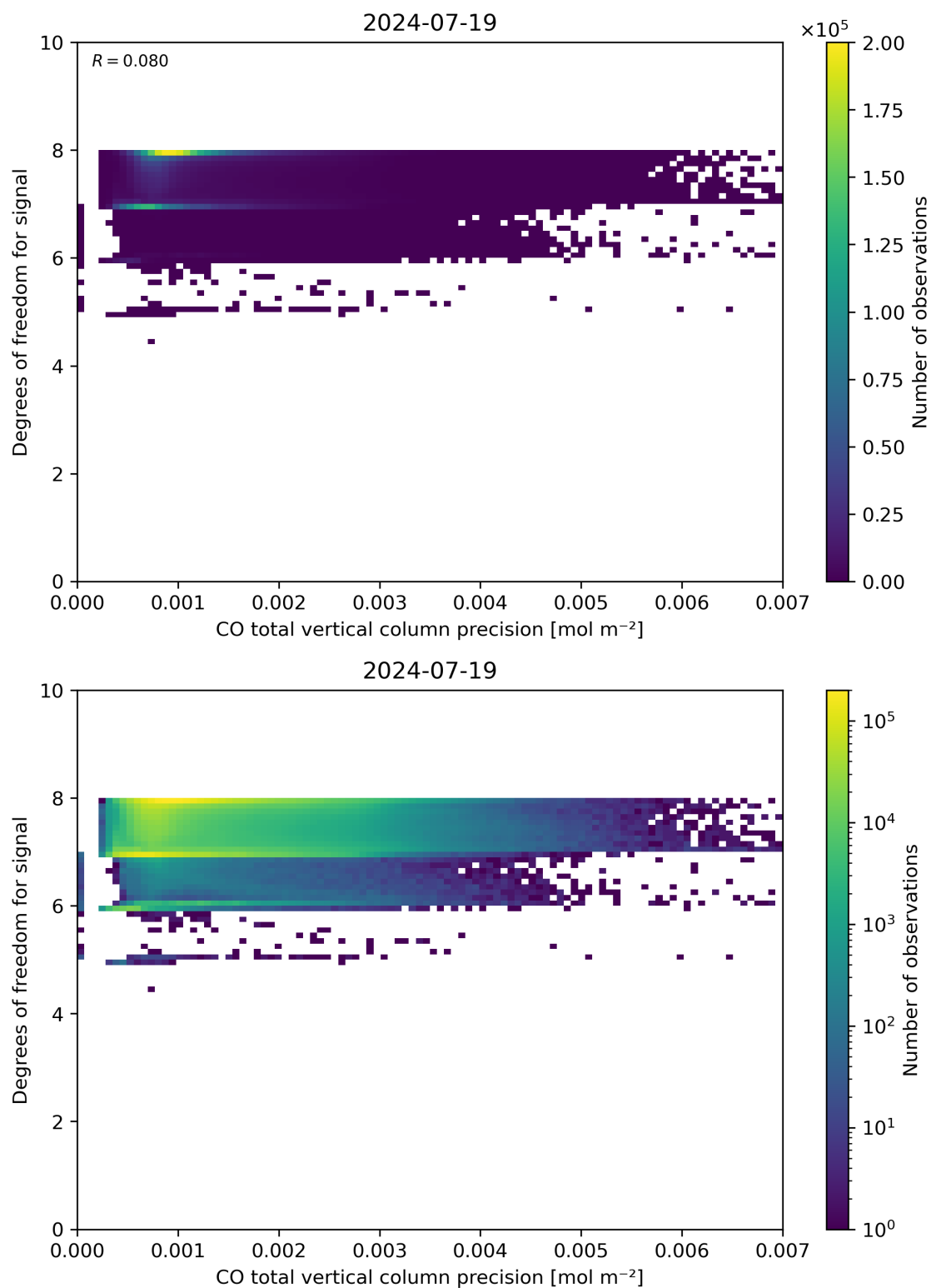
Figure 45: Scatter density plot of “CO total vertical column precision” against “Degrees of freedom for signal” for 2024-07-18 to 2024-07-20.
