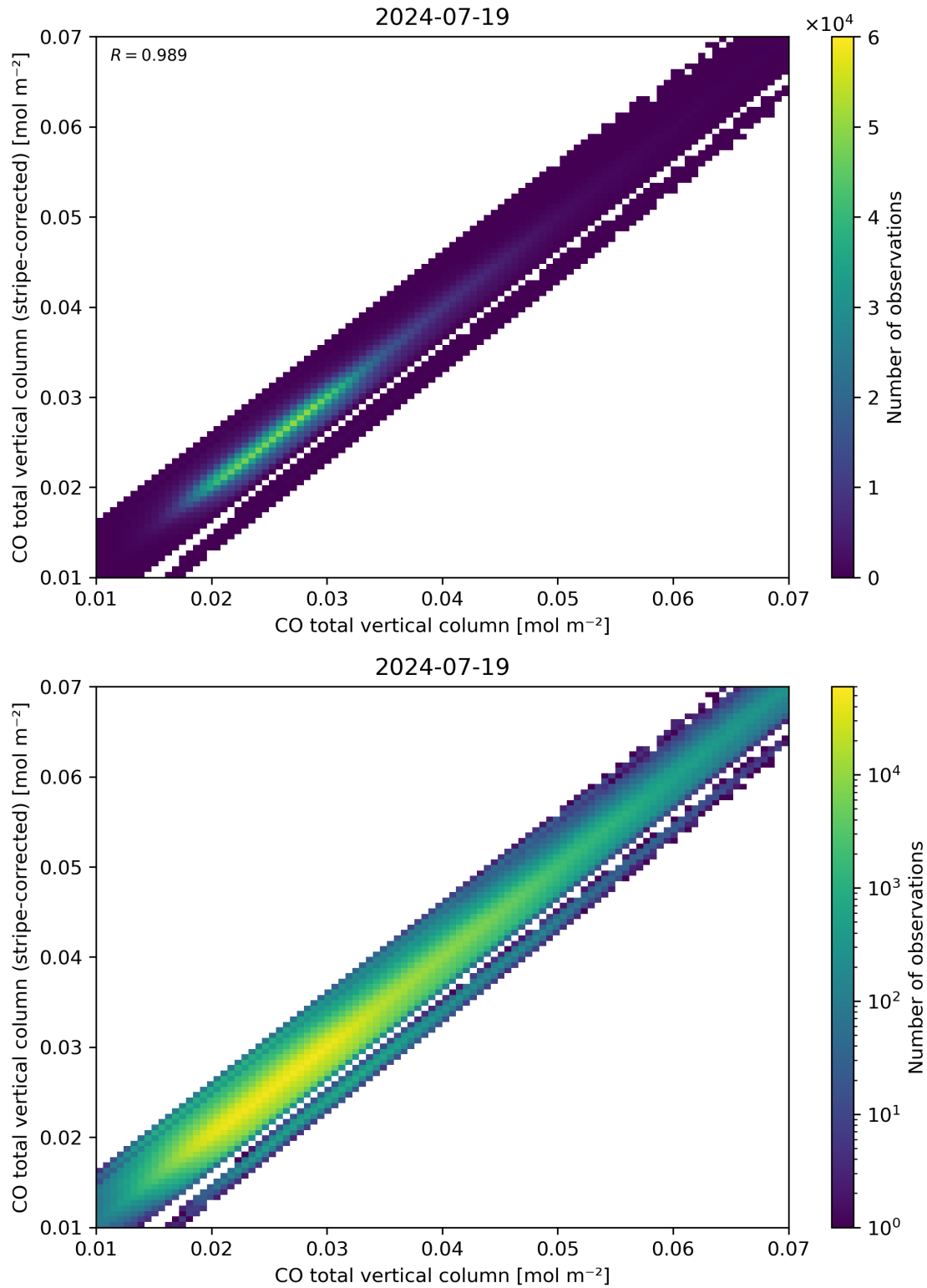
Figure 33: Scatter density plot of “CO total vertical column” against “CO total vertical column (stripe-corrected)” for 2024-07-18 to 2024-07-20.
