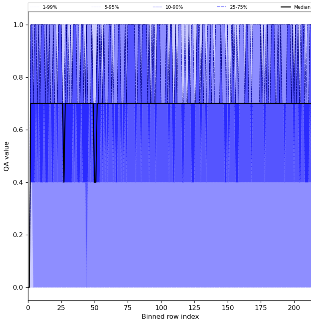
Figure 25: Along track statistics of “QA value” for 2024-07-18 to 2024-07-20
