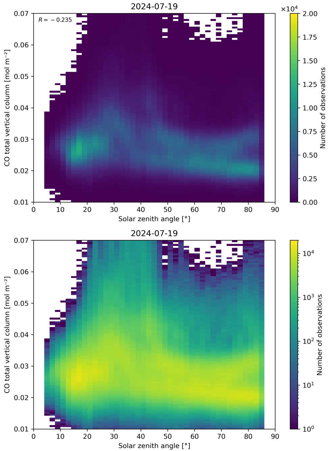
Figure 61: Scatter density plot of “Solar zenith angle” against “CO total vertical column” for 2024-07-18 to 2024-07-20.
