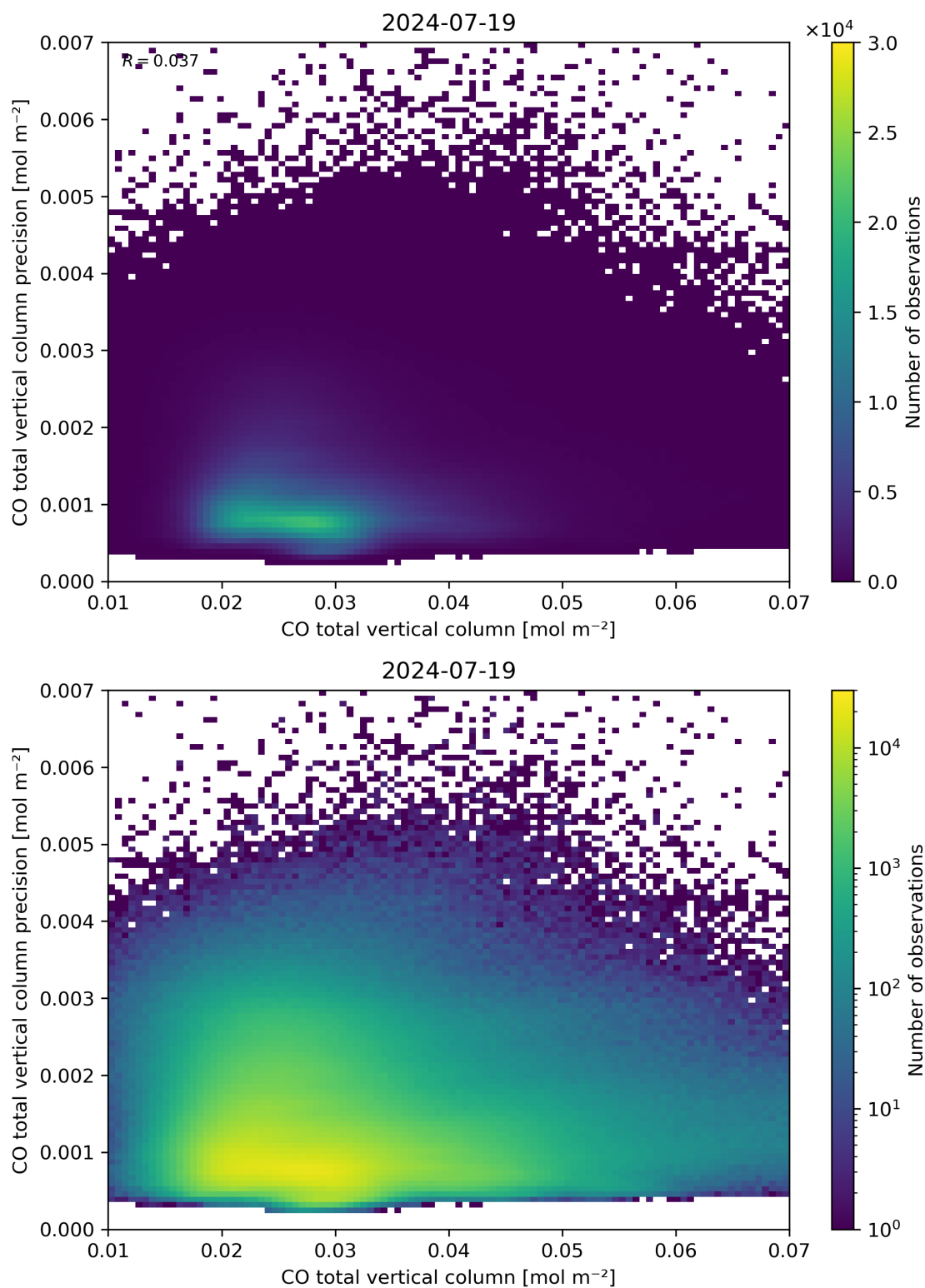
Figure 34: Scatter density plot of “CO total vertical column” against “CO total vertical column precision” for 2024-07-18 to 2024-07-20.
