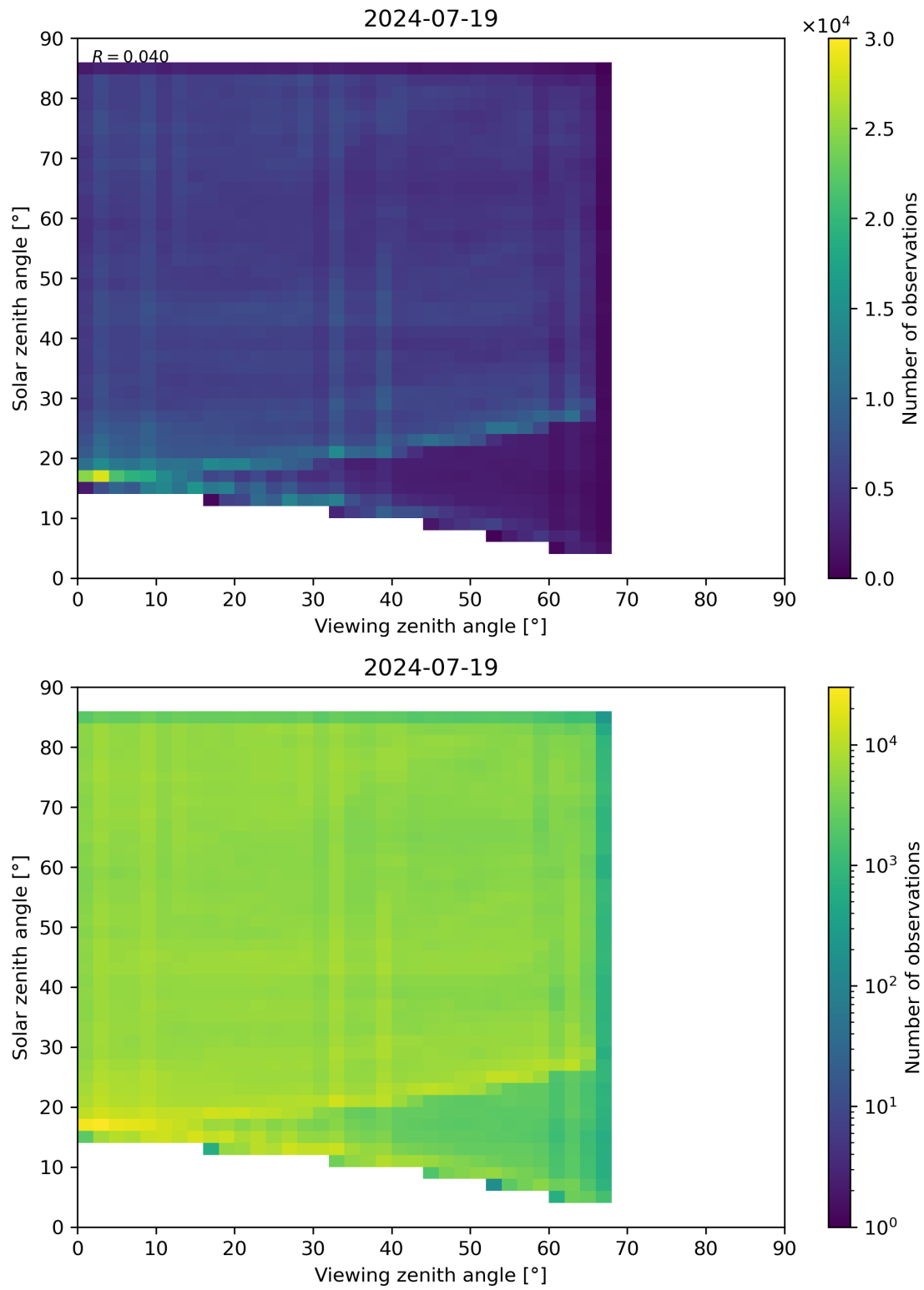
Figure 77: Scatter density plot of “Viewing zenith angle” against “Solar zenith angle” for 2024-07-18 to 2024-07-20.
