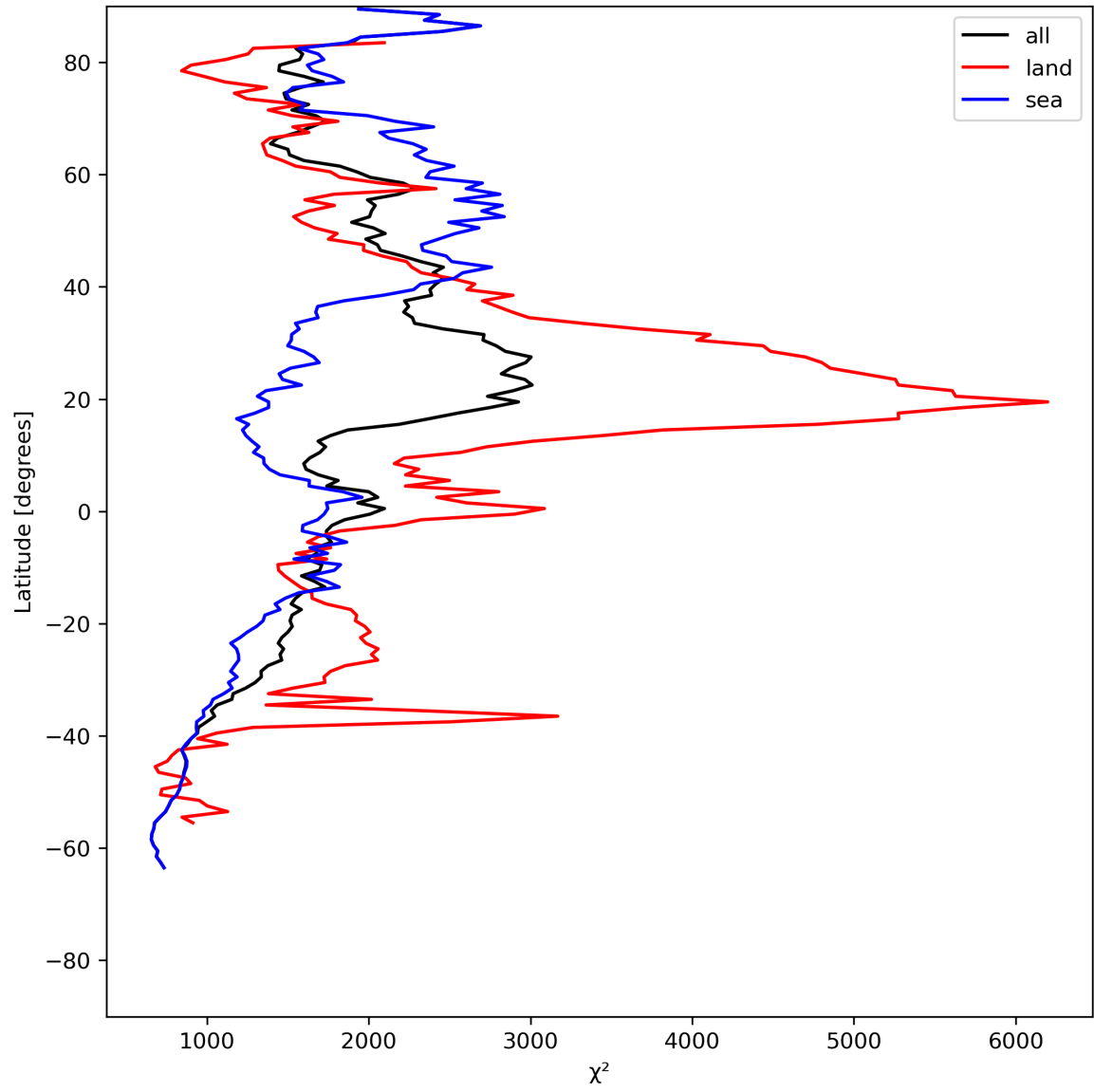
Figure 14: Zonal average of “ \chi^2 ” for 2024-07-18 to 2024-07-20.
