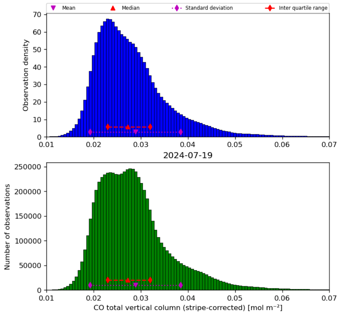
Figure 19: Histogram of “CO total vertical column (stripe-corrected)” for 2024-07-18 to 2024-07-20
