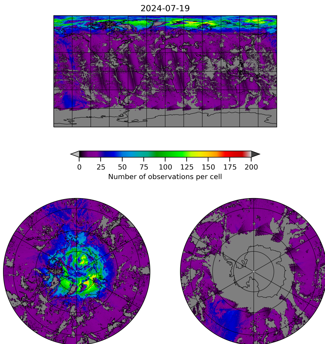
Figure 8: Map of the number of observations for 2024-07-18 to 2024-07-20
