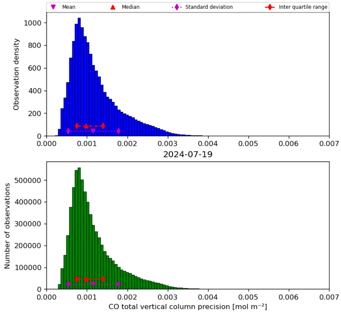
Figure 20: Histogram of “CO total vertical column precision” for 2024-07-18 to 2024-07-20
