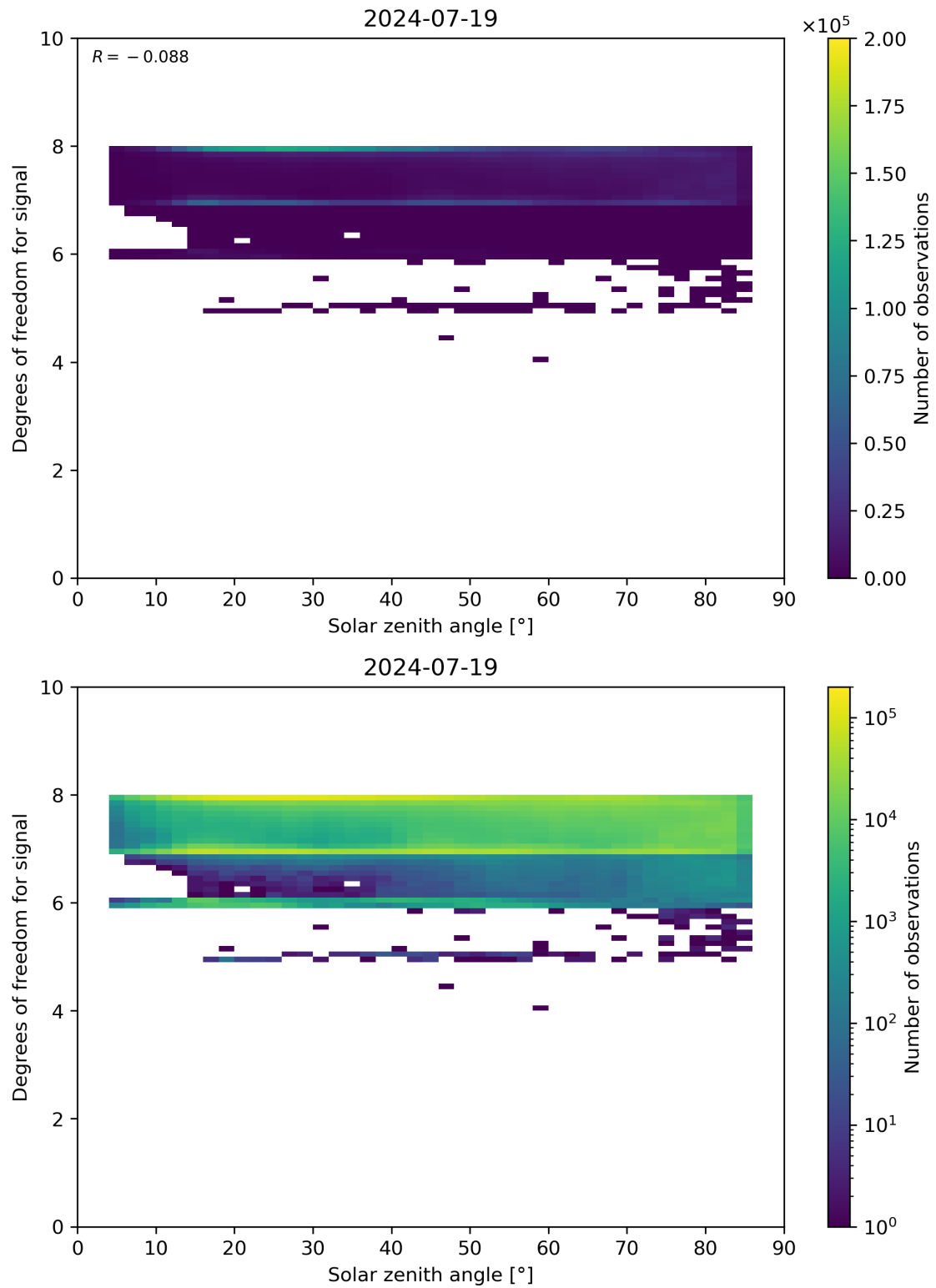
Figure 65: Scatter density plot of “Solar zenith angle” against “Degrees of freedom for signal” for 2024-07-18 to 2024-07-20.
