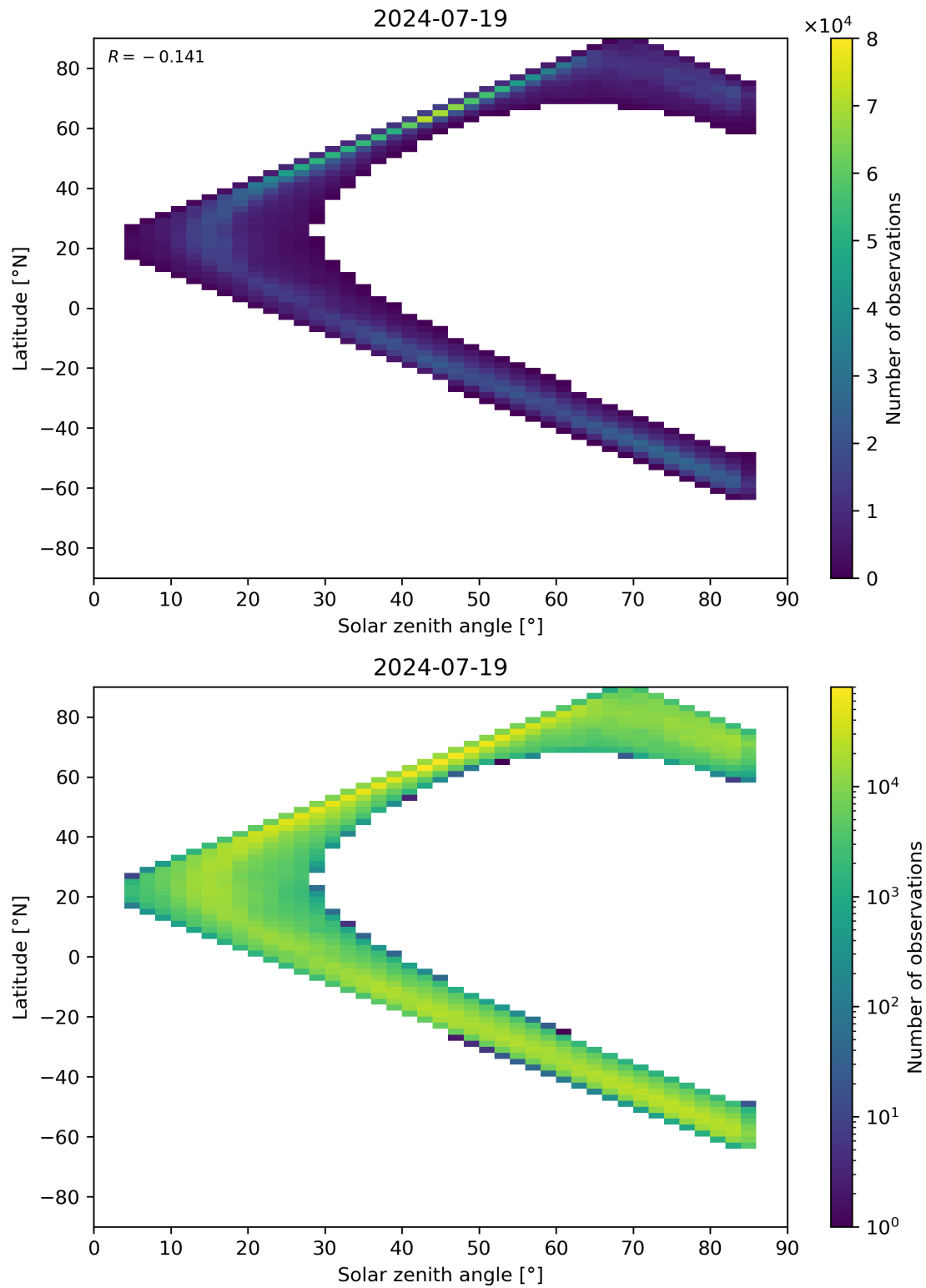
Figure 66: Scatter density plot of “Solar zenith angle” against “Latitude” for 2024-07-18 to 2024-07-20.
