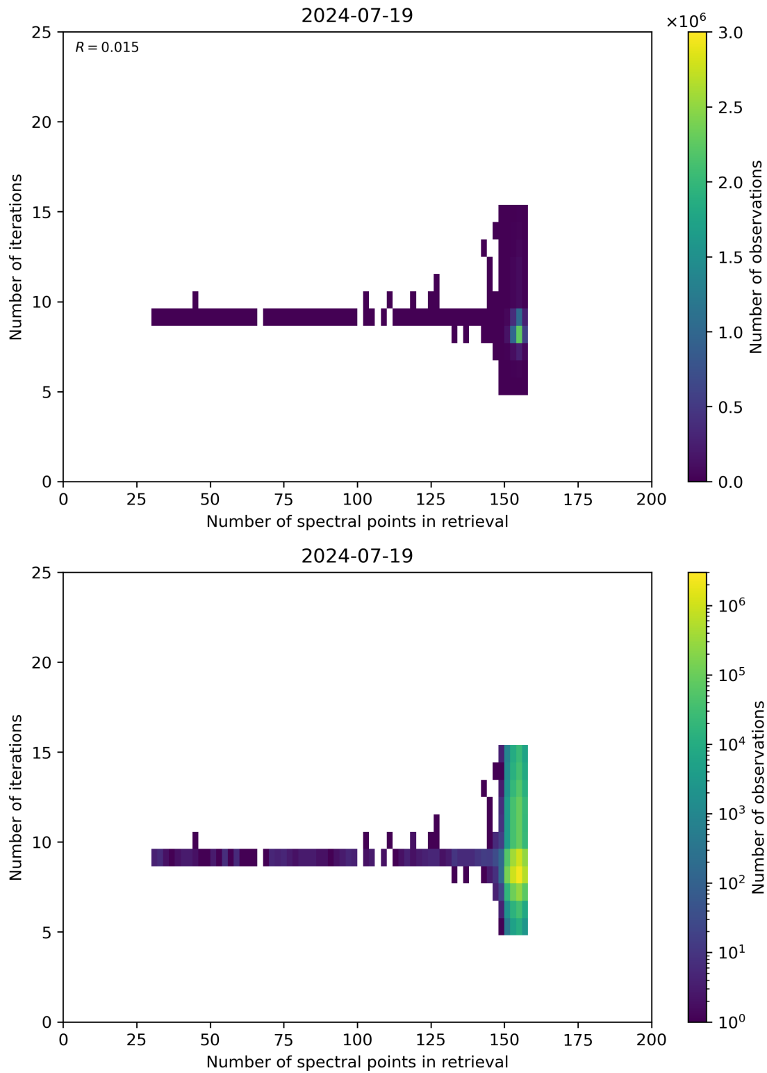
Figure 60: Scatter density plot of “Number of spectral points in retrieval” against “Number of iterations” for 2024-07-18 to 2024-07-20.
