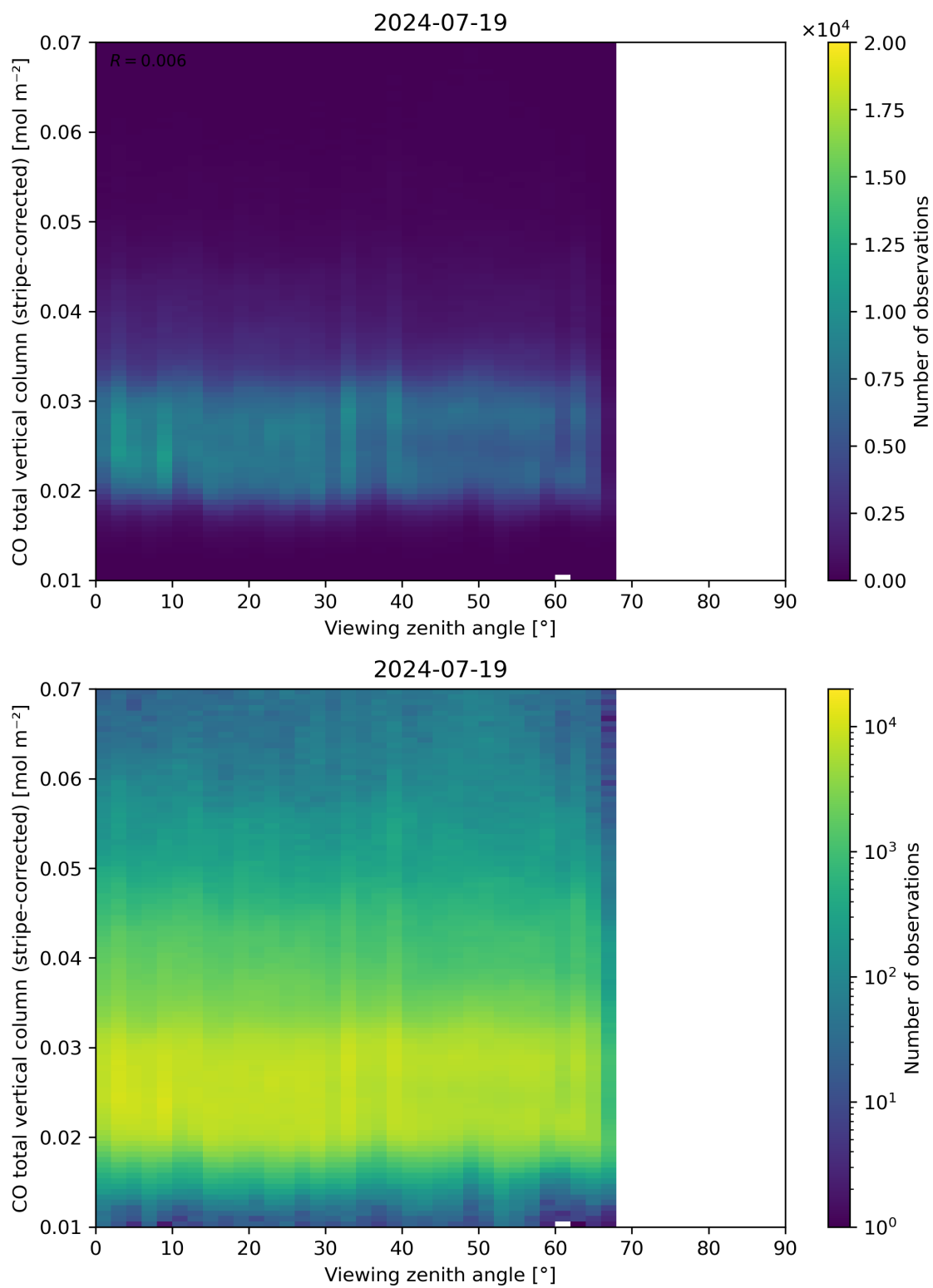
Figure 70: Scatter density plot of “Viewing zenith angle” against “CO total vertical column (stripe-corrected)” for 2024-07-18 to 2024-07-20.
