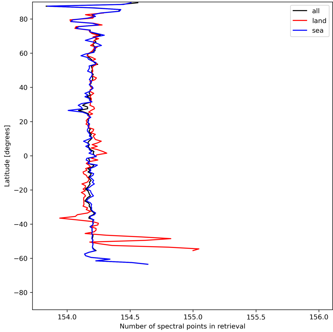
Figure 13: Zonal average of “Number of spectral points in retrieval” for 2024-07-18 to 2024-07-20.
