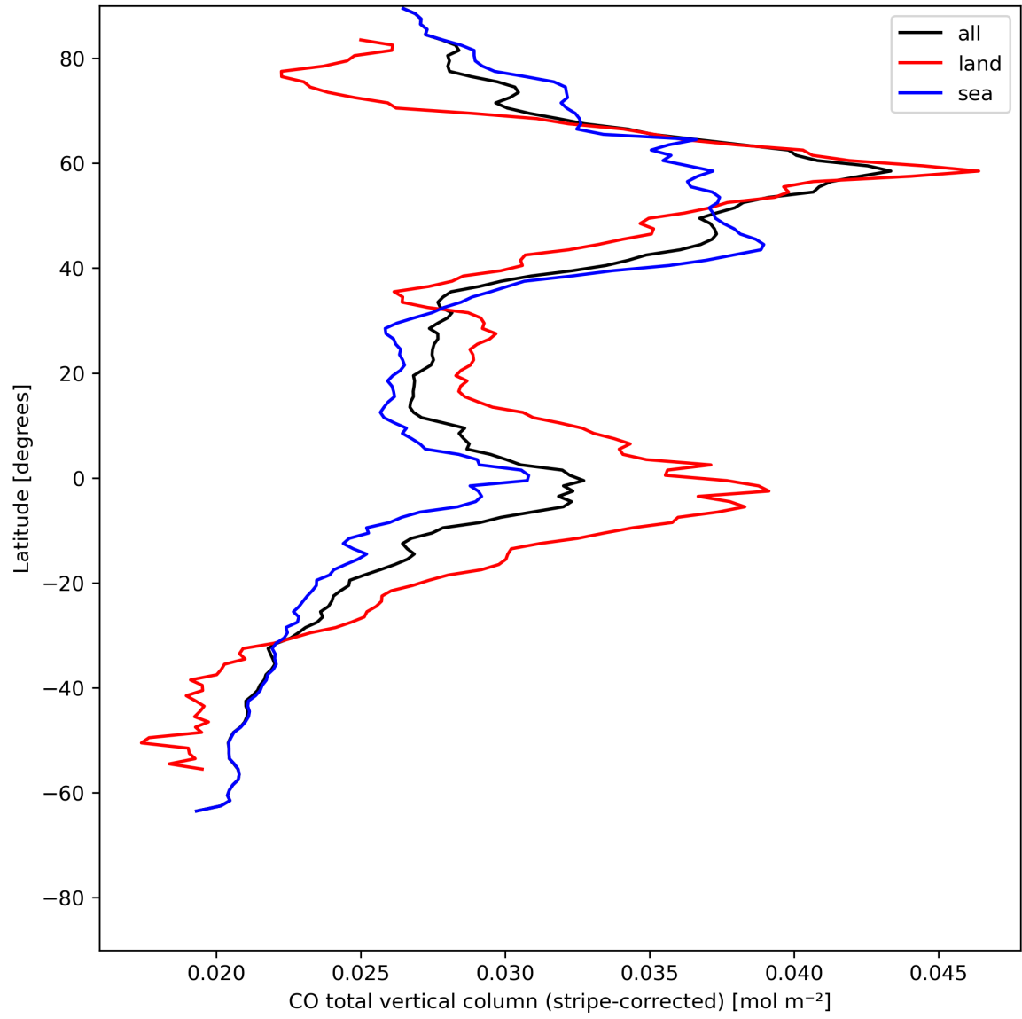
Figure 11: Zonal average of “CO total vertical column (stripe-corrected)” for 2024-07-18 to 2024-07-20.
