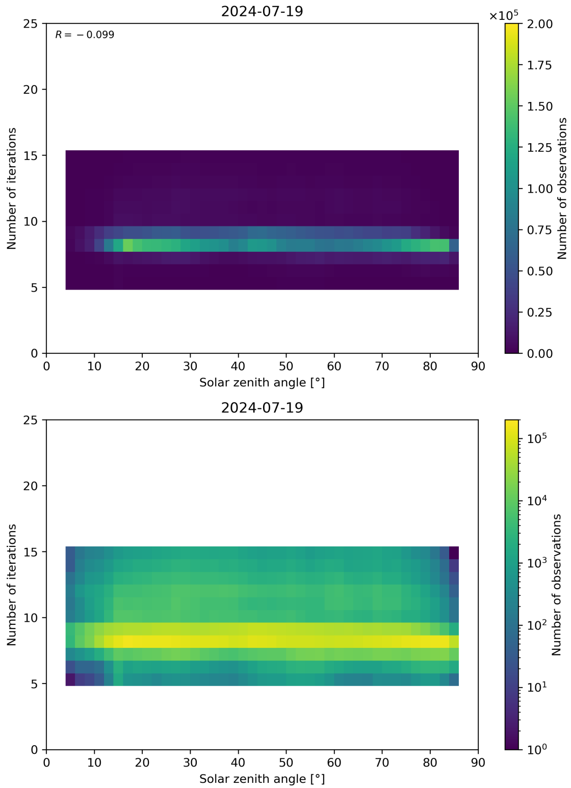
Figure 67: Scatter density plot of “Solar zenith angle” against “Number of iterations” for 2024-07-18 to 2024-07-20.
