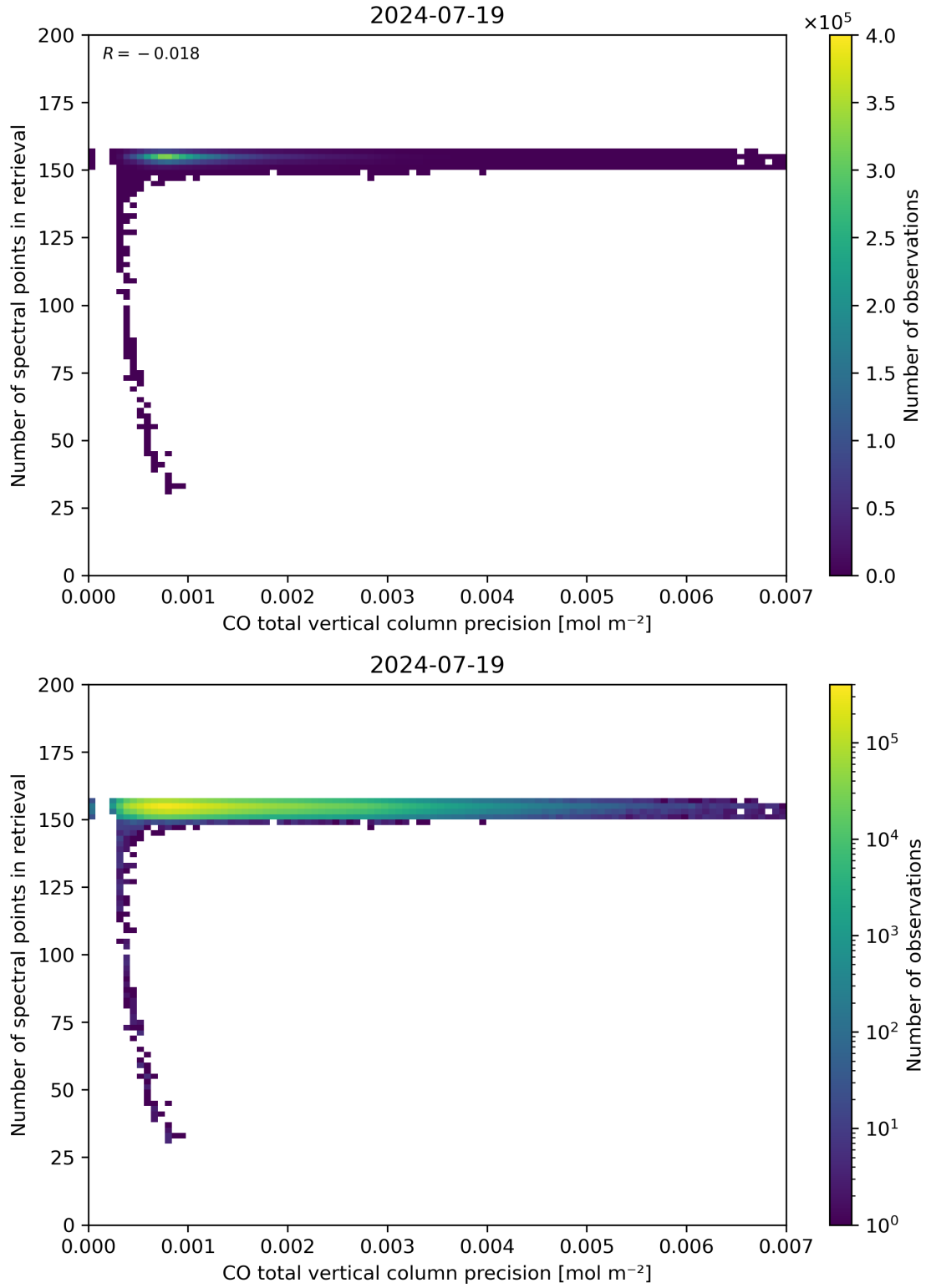
Figure 47: Scatter density plot of “CO total vertical column precision” against “Number of spectral points in retrieval” for 2024-07-18 to 2024-07-20.
