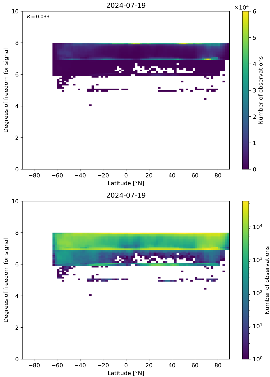
Figure 55: Scatter density plot of “Latitude” against “Degrees of freedom for signal” for 2024-07-18 to 2024-07-20.
