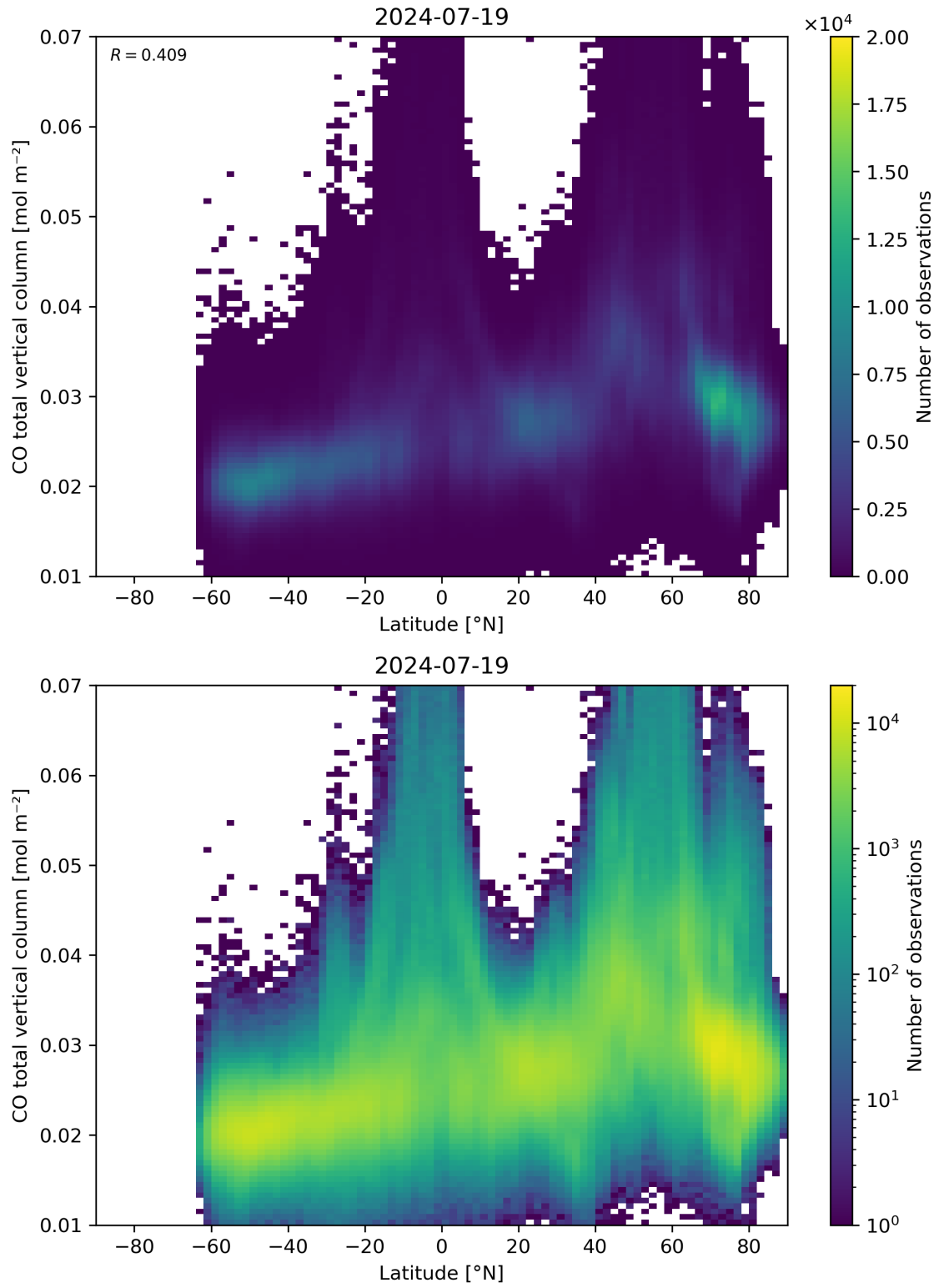
Figure 51: Scatter density plot of “Latitude” against “CO total vertical column” for 2024-07-18 to 2024-07-20.
