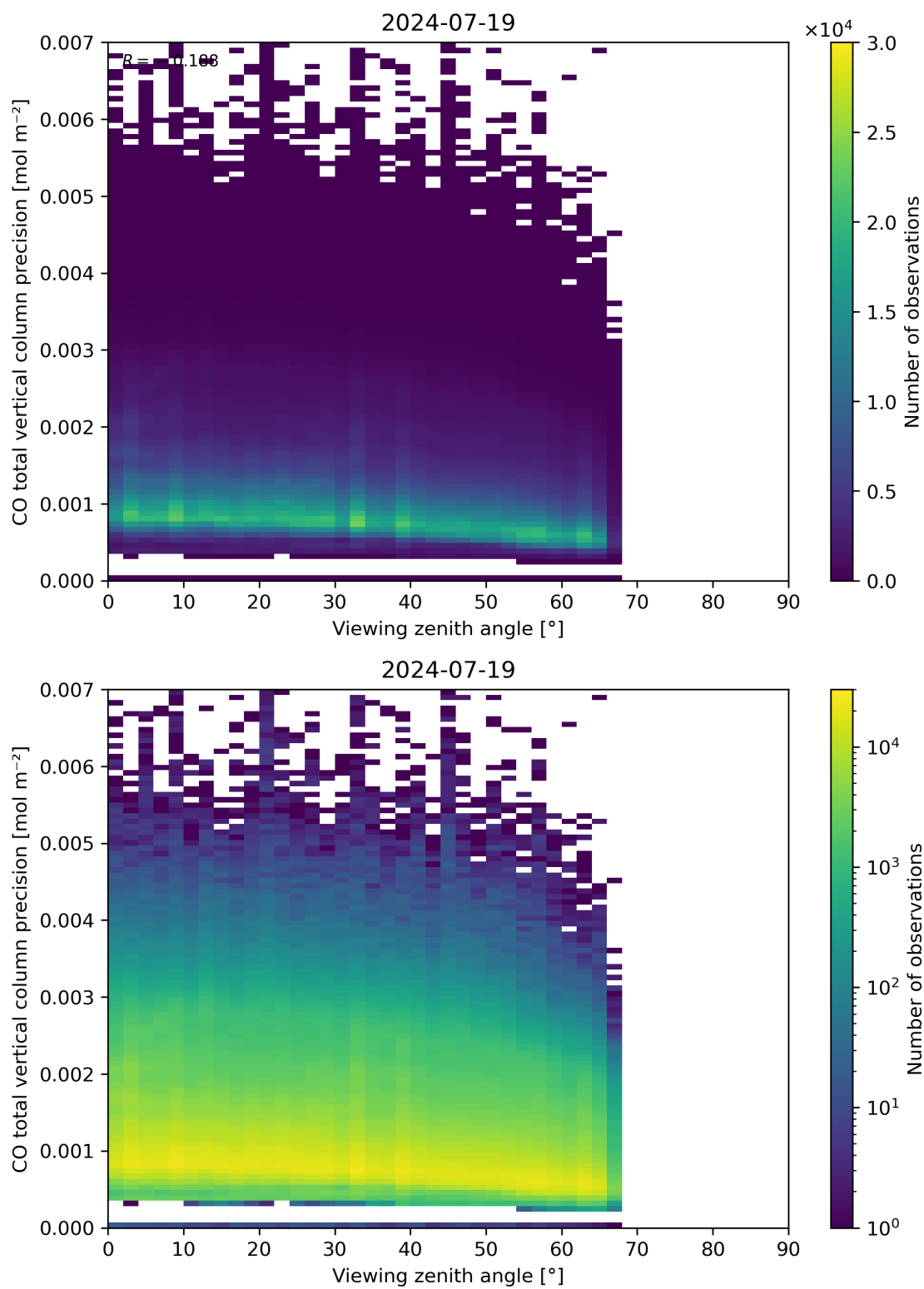
Figure 71: Scatter density plot of “Viewing zenith angle” against “CO total vertical column precision” for 2024-07-18 to 2024-07-20.
