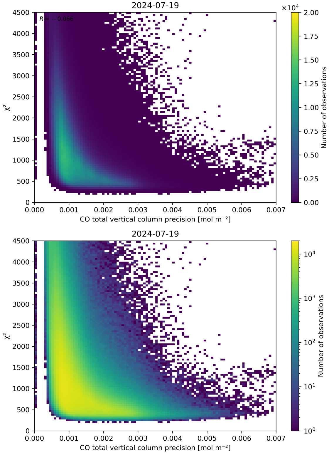
Figure 44: Scatter density plot of “CO total vertical column precision” against “ \chi^2 ” for 2024-07-18 to 2024-07-20.
