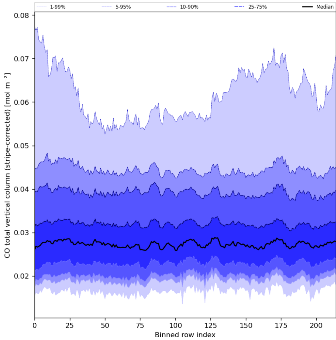
Figure 27: Along track statistics of “CO total vertical column (stripe-corrected)” for 2024-07-18 to 2024-07-20
