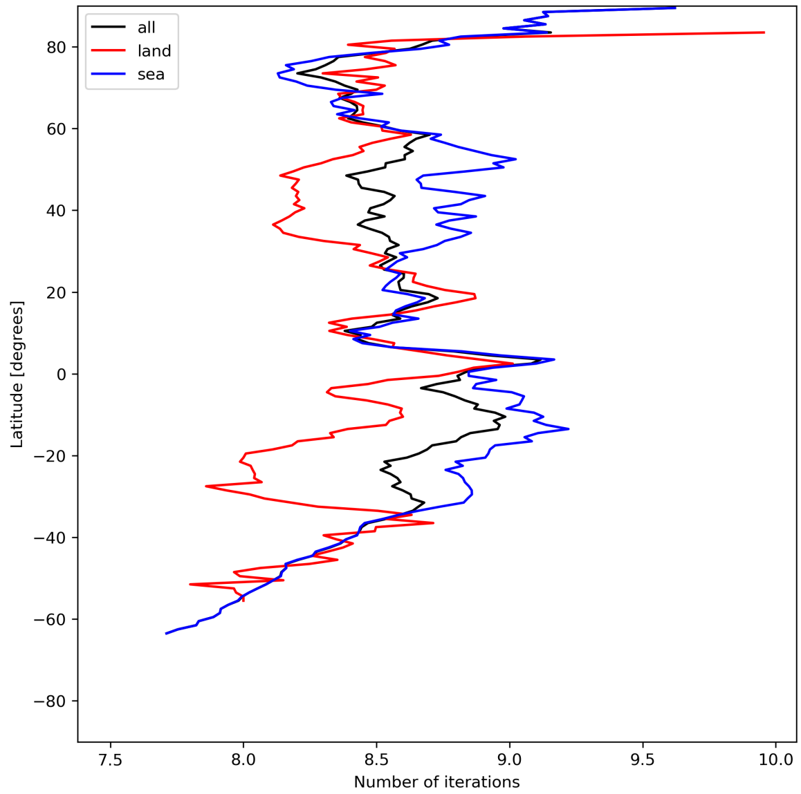
Figure 16: Zonal average of “Number of iterations” for 2024-07-18 to 2024-07-20.
