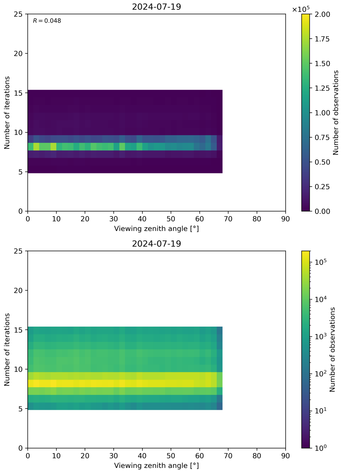
Figure 75: Scatter density plot of “Viewing zenith angle” against “Number of iterations” for 2024-07-18 to 2024-07-20.
