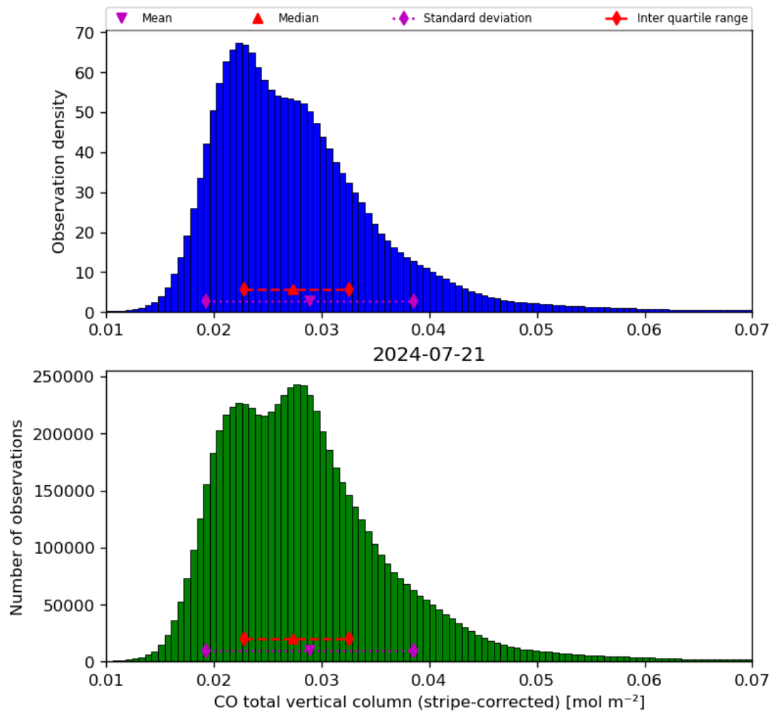
Figure 19: Histogram of “CO total vertical column (stripe-corrected)” for 2024-07-21 to 2024-07-22
