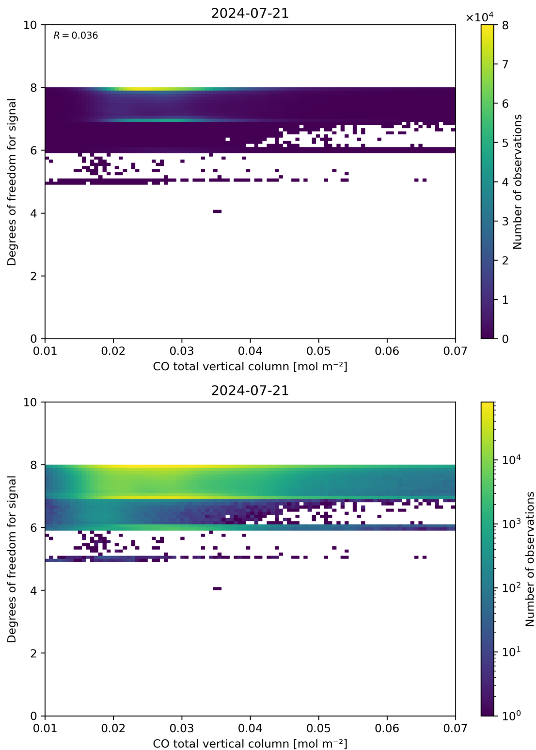
Figure 41: Scatter density plot of “CO total vertical column” against “Degrees of freedom for signal” for 2024-07-21 to 2024-07-22.
