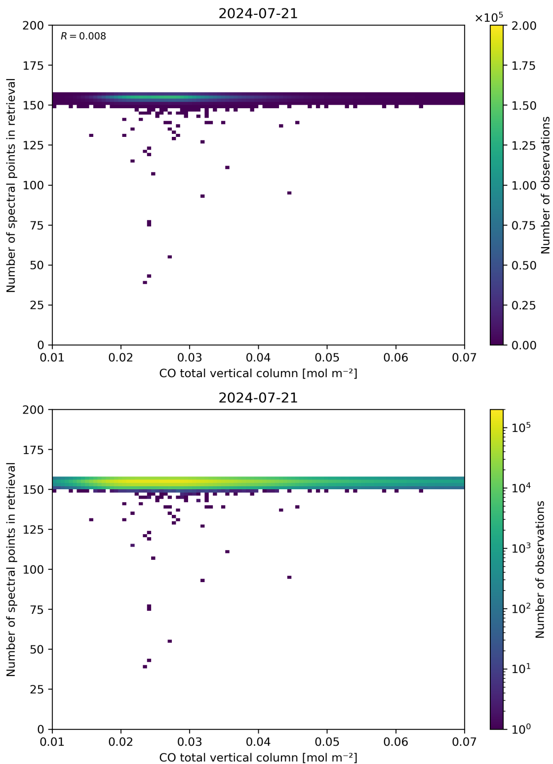
Figure 43: Scatter density plot of “CO total vertical column” against “Number of spectral points in retrieval” for 2024-07-21 to 2024-07-22.
