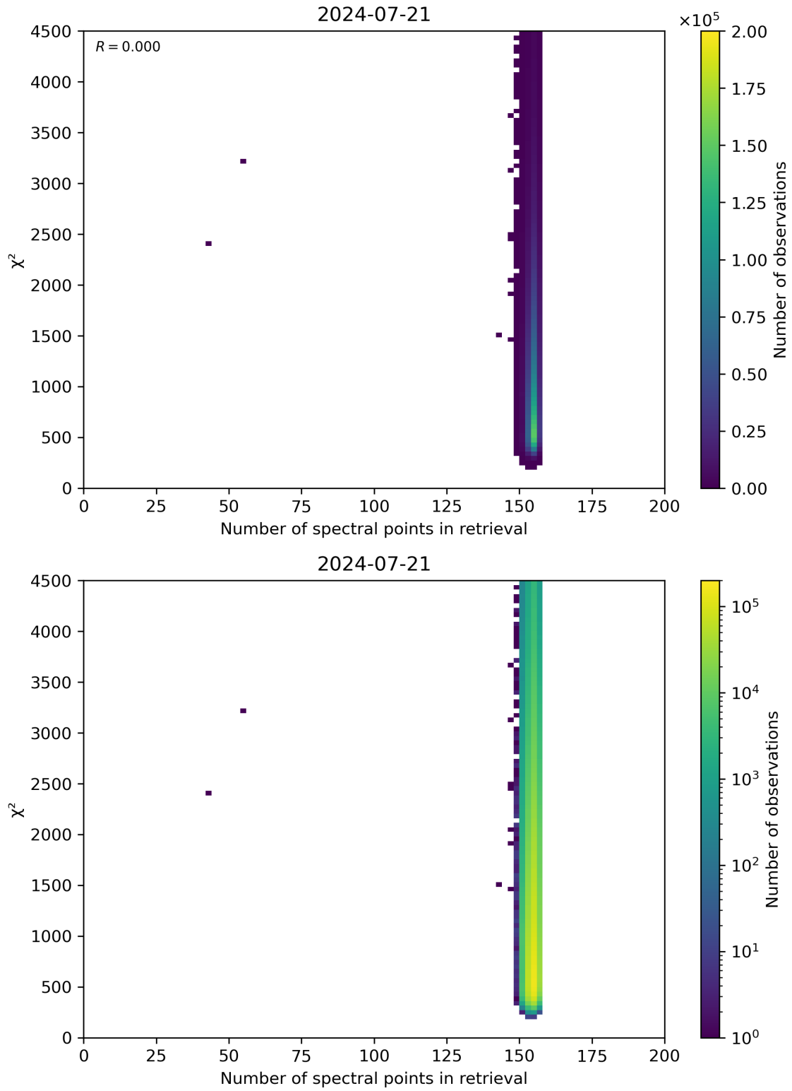
Figure 58: Scatter density plot of “Number of spectral points in retrieval” against “ \chi^2 ” for 2024-07-21 to 2024-07-22.
