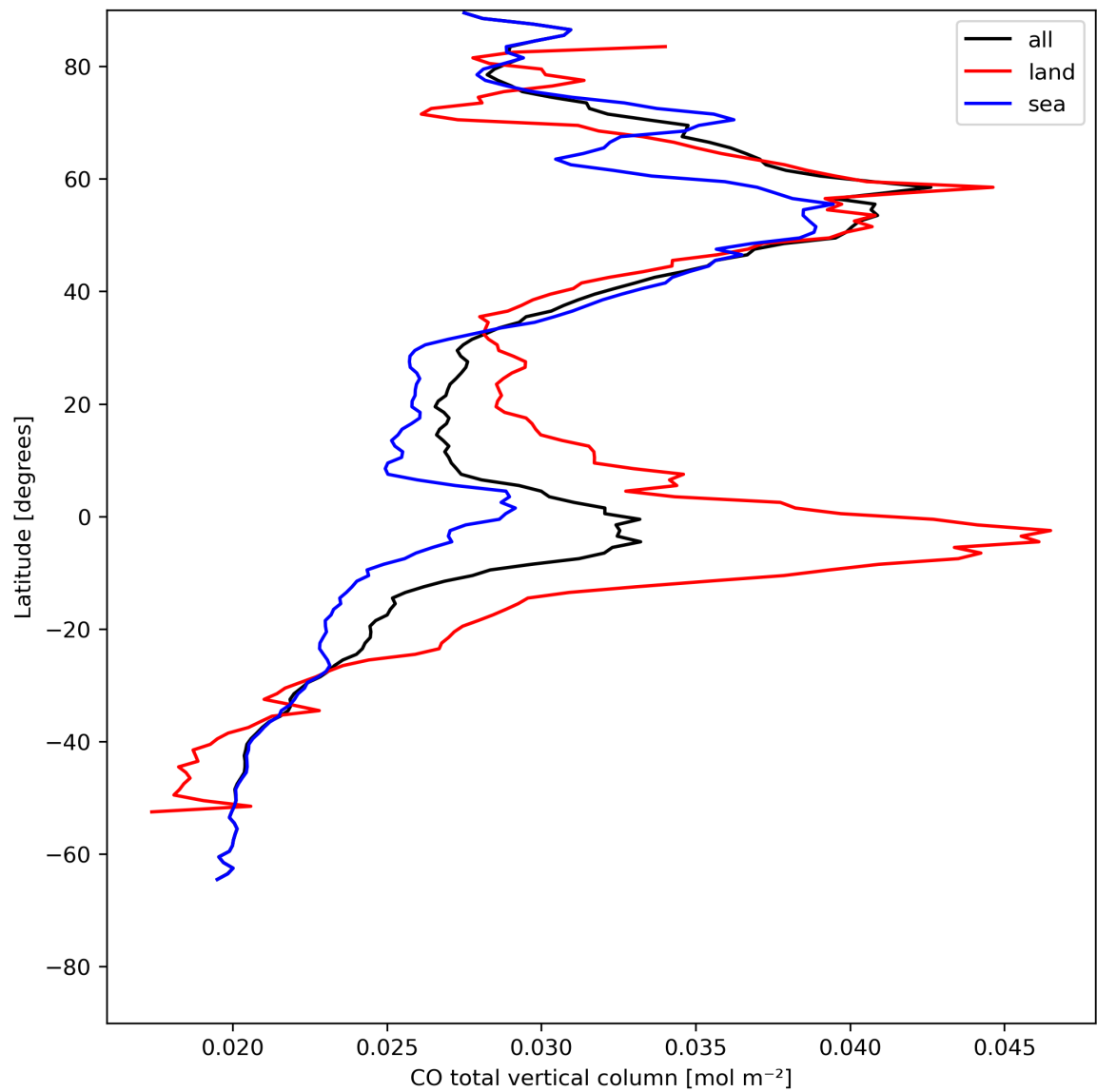
Figure 10: Zonal average of “CO total vertical column” for 2024-07-21 to 2024-07-22.
