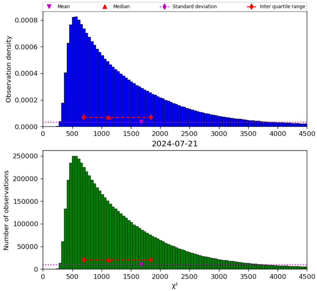
Figure 22: Histogram of “ \chi^2 ” for 2024-07-21 to 2024-07-22
