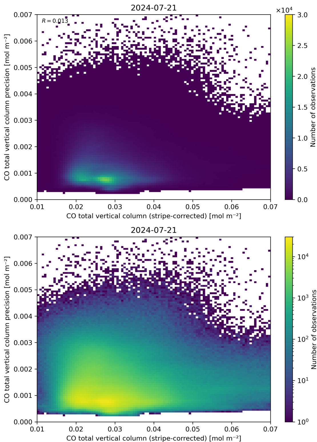
Figure 36: Scatter density plot of “CO total vertical column (stripe-corrected)” against “CO total vertical column precision” for 2024-07-21 to 2024-07-22.
