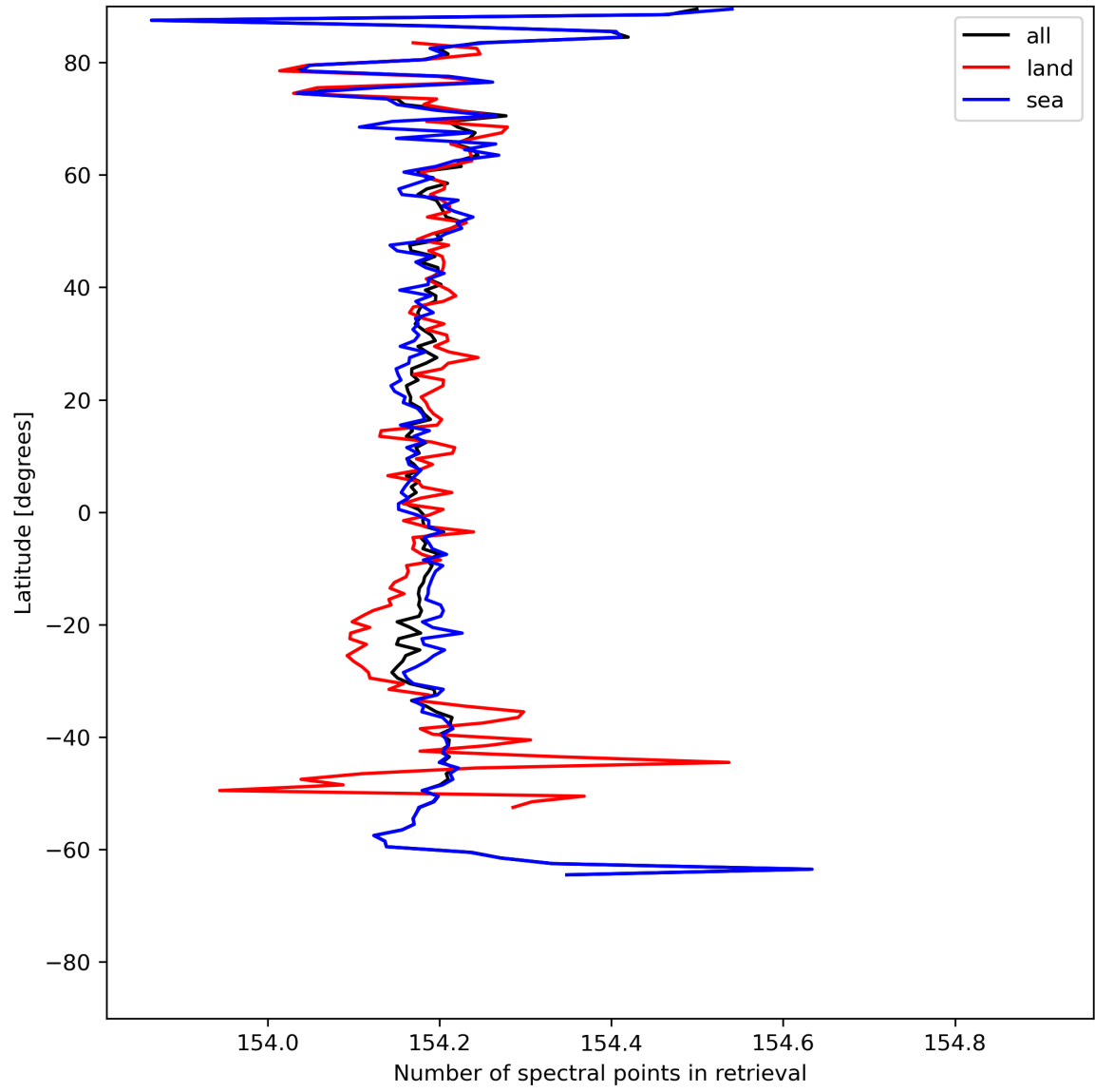
Figure 13: Zonal average of “Number of spectral points in retrieval” for 2024-07-21 to 2024-07-22.
