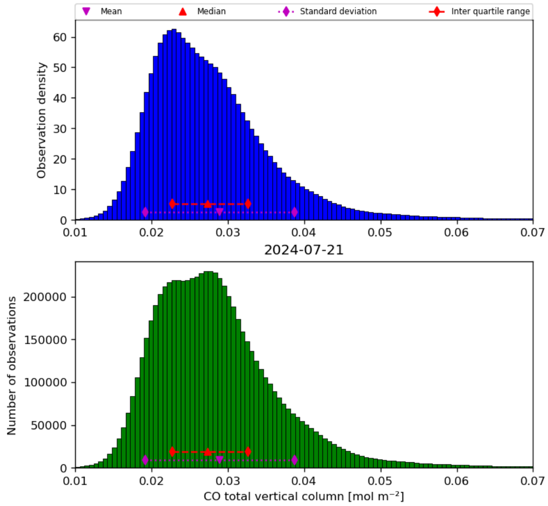
Figure 18: Histogram of “CO total vertical column” for 2024-07-21 to 2024-07-22
