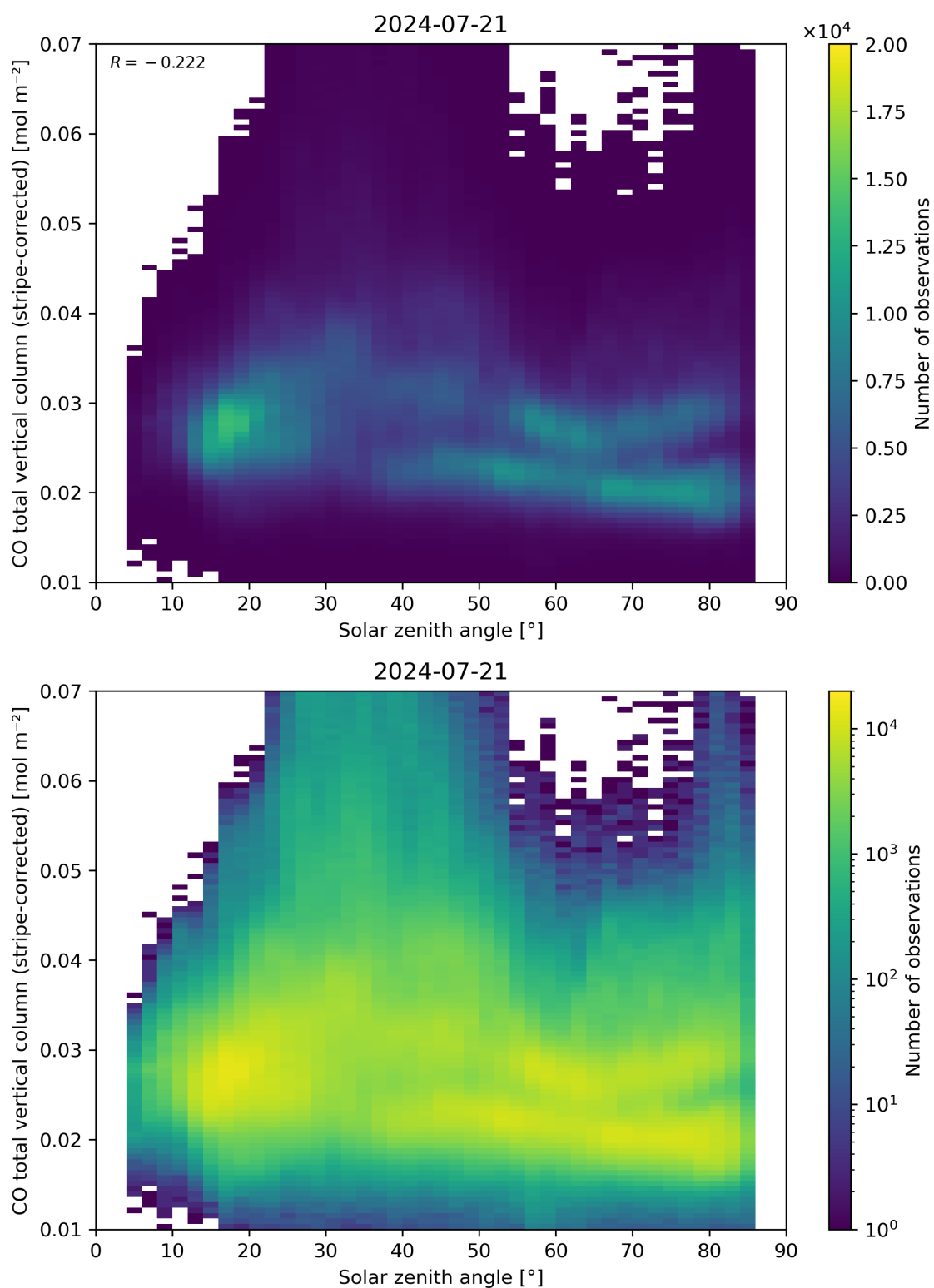
Figure 62: Scatter density plot of “Solar zenith angle” against “CO total vertical column (stripe-corrected)” for 2024-07-21 to 2024-07-22.
