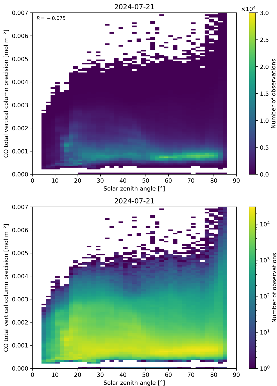
Figure 63: Scatter density plot of “Solar zenith angle” against “CO total vertical column precision” for 2024-07-21 to 2024-07-22.
