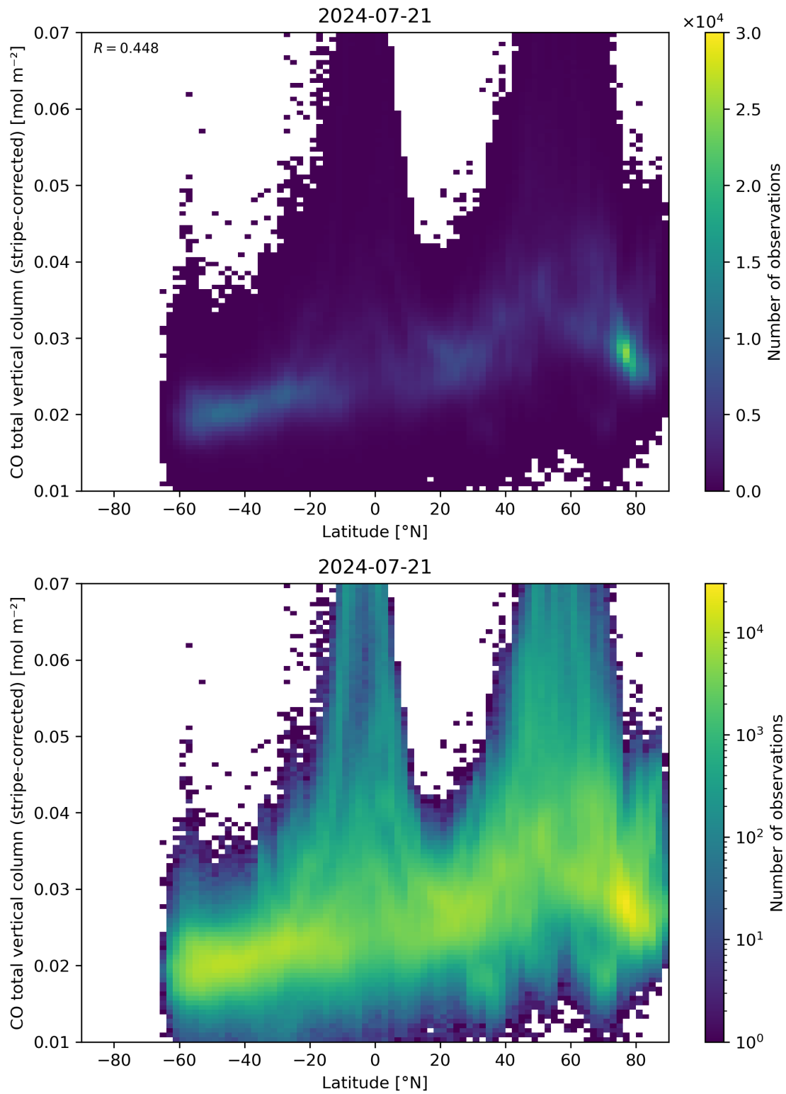
Figure 52: Scatter density plot of “Latitude” against “CO total vertical column (stripe-corrected)” for 2024-07-21 to 2024-07-22.
