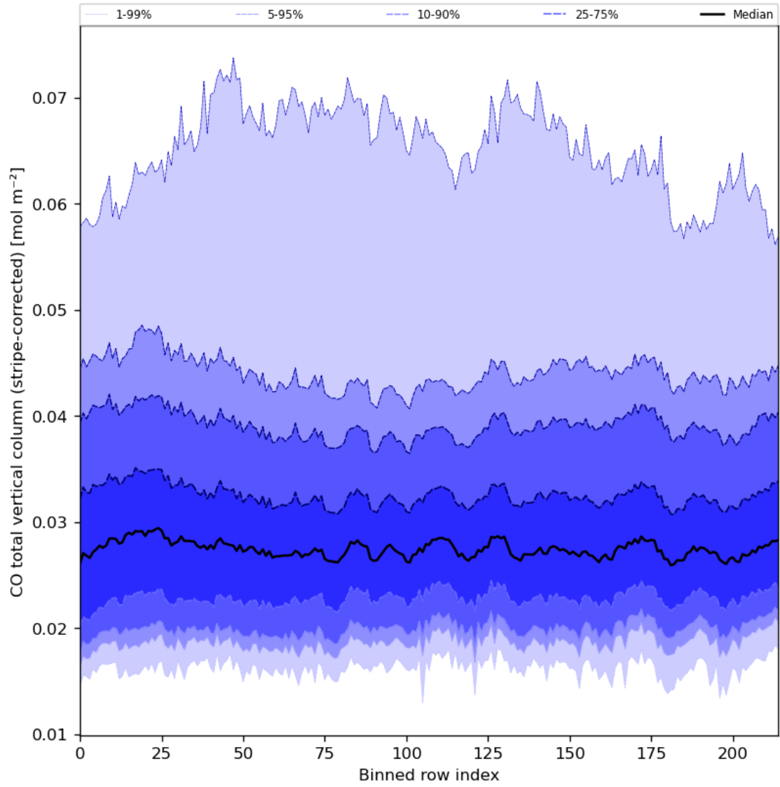
Figure 27: Along track statistics of “CO total vertical column (stripe-corrected)” for 2024-07-21 to 2024-07-22
