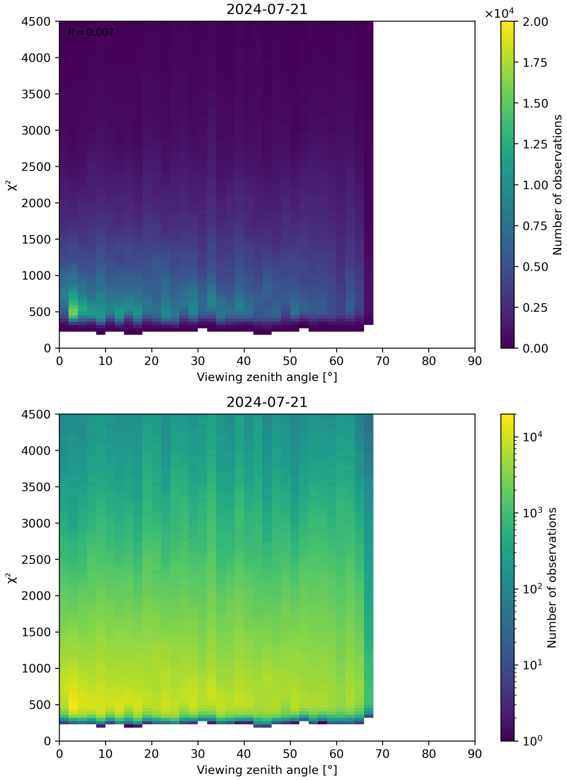
Figure 72: Scatter density plot of “Viewing zenith angle” against “ \chi^2 ” for 2024-07-21 to 2024-07-22.
