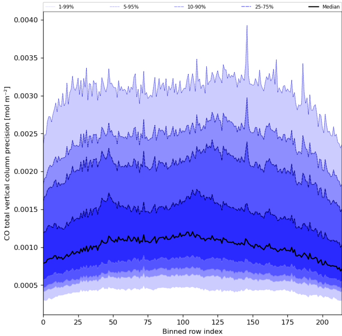
Figure 28: Along track statistics of “CO total vertical column precision” for 2024-07-21 to 2024-07-22
