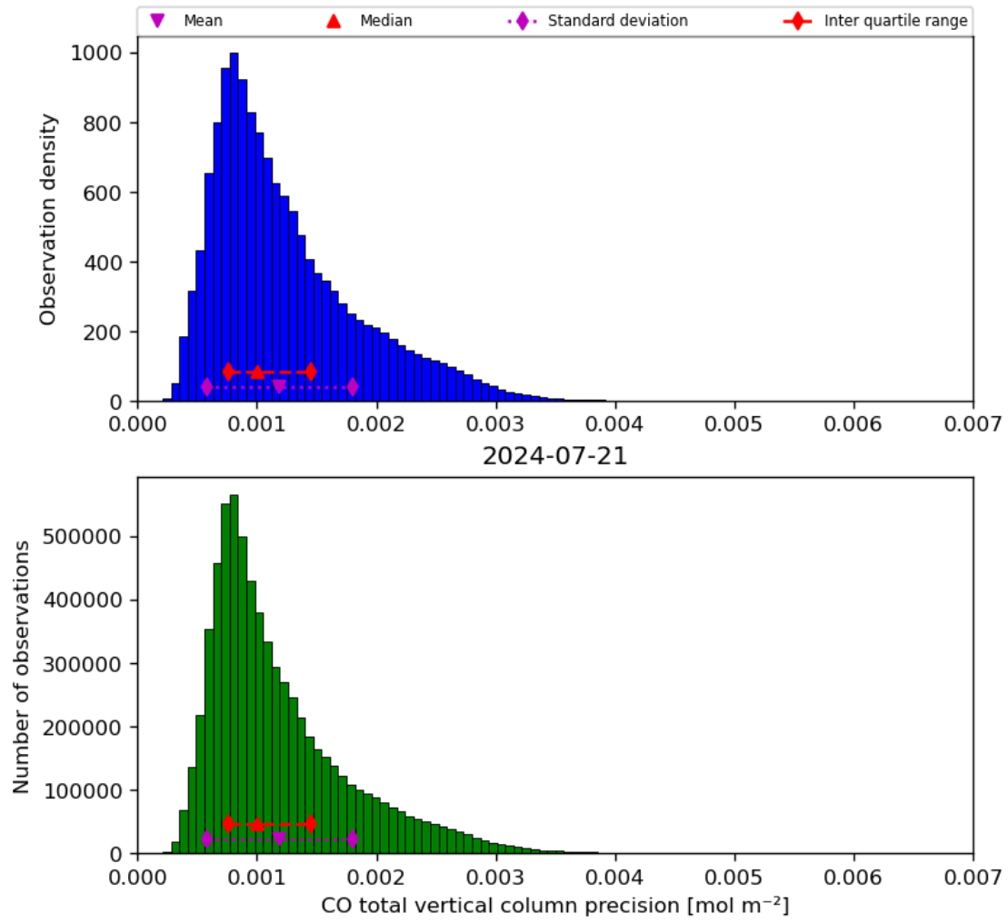
Figure 20: Histogram of “CO total vertical column precision” for 2024-07-21 to 2024-07-22
