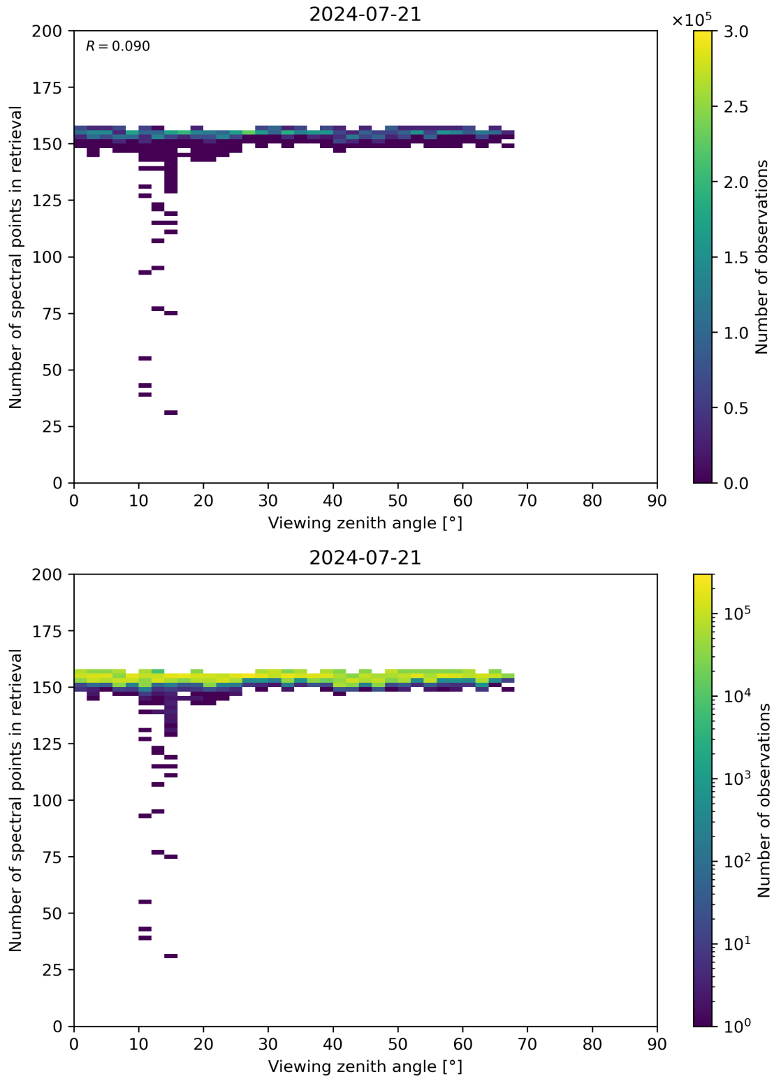
Figure 76: Scatter density plot of “Viewing zenith angle” against “Number of spectral points in retrieval” for 2024-07-21 to 2024-07-22.
