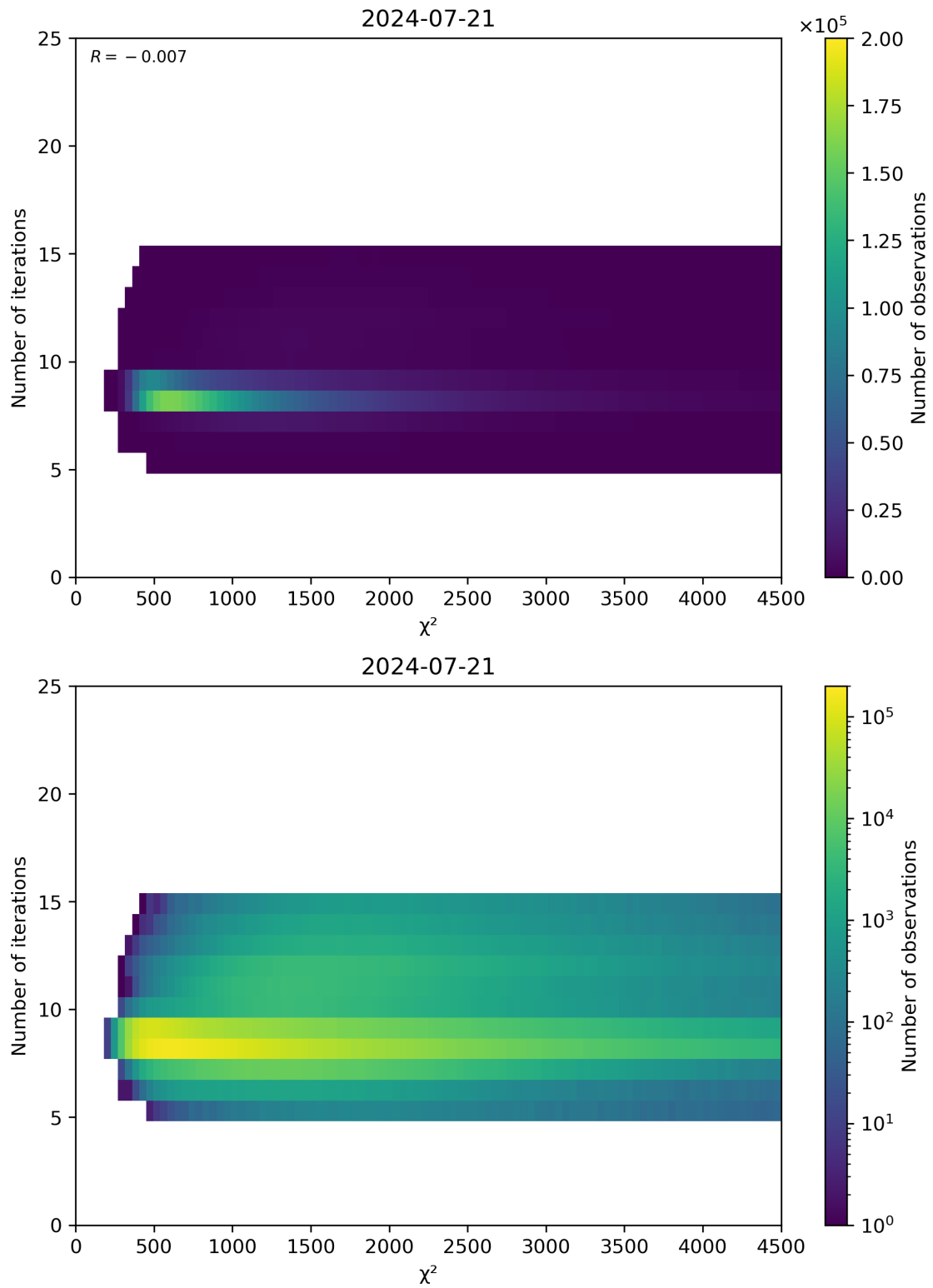
Figure 49: Scatter density plot of “ \chi^2 ” against “Number of iterations” for 2024-07-21 to 2024-07-22.
