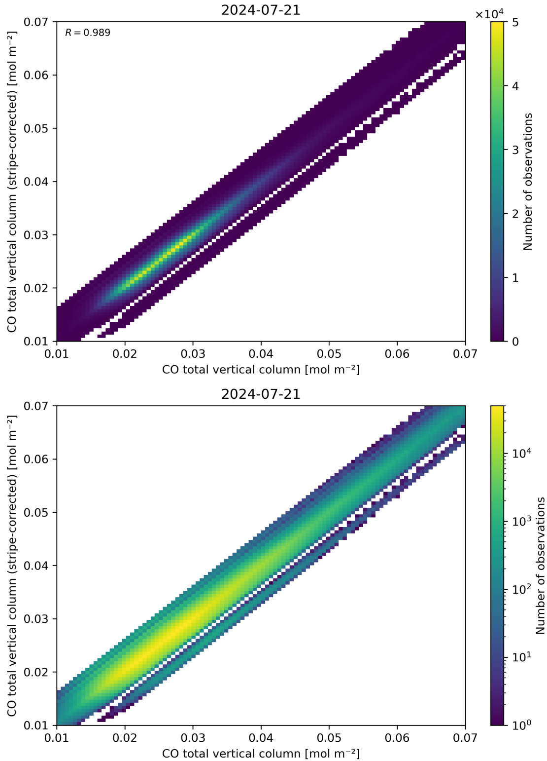
Figure 33: Scatter density plot of “CO total vertical column” against “CO total vertical column (stripe-corrected)” for 2024-07-21 to 2024-07-22.
