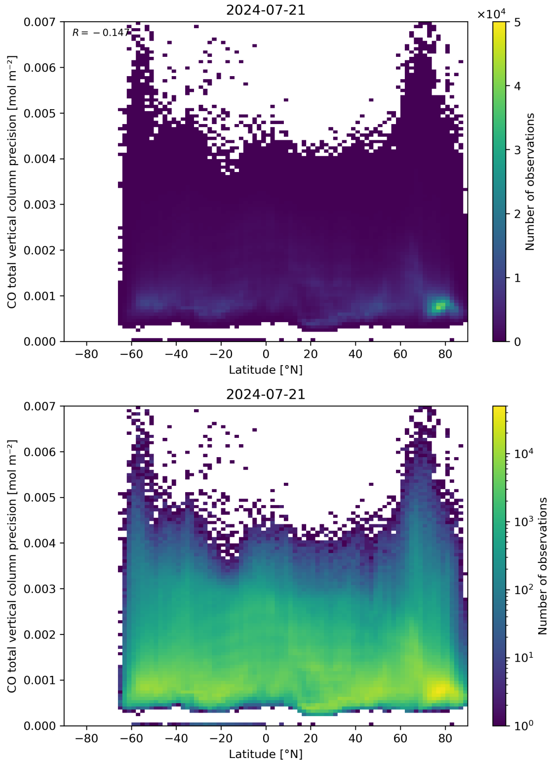
Figure 53: Scatter density plot of “Latitude” against “CO total vertical column precision” for 2024-07-21 to 2024-07-22.
