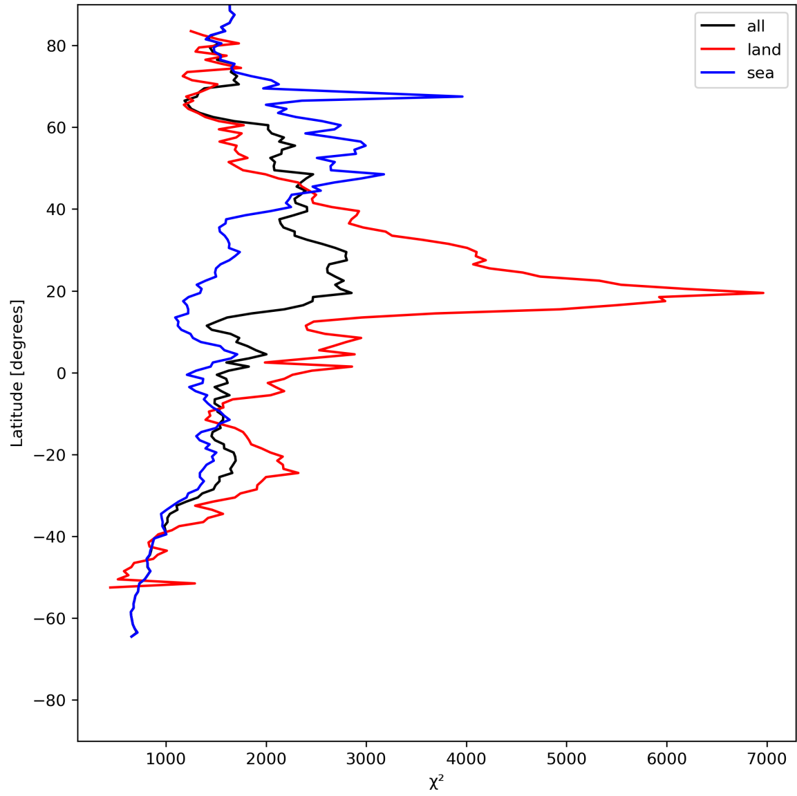
Figure 14: Zonal average of “ \chi^2 ” for 2024-07-21 to 2024-07-22.
