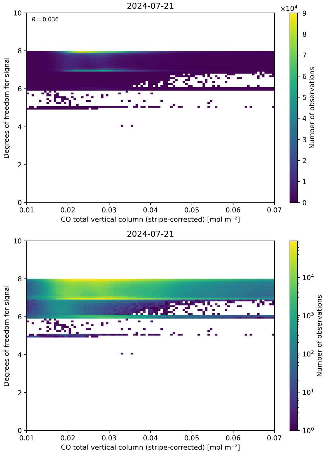
Figure 38: Scatter density plot of “CO total vertical column (stripe-corrected)” against “Degrees of freedom for signal” for 2024-07-21 to 2024-07-22.
