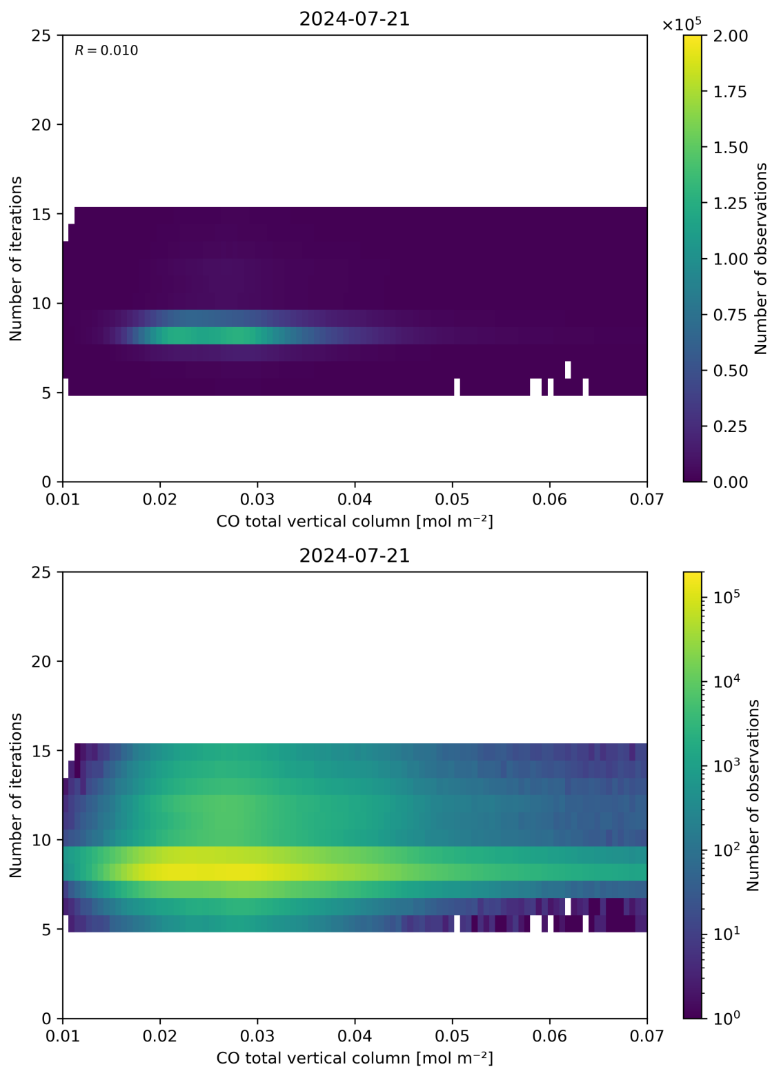
Figure 42: Scatter density plot of “CO total vertical column” against “Number of iterations” for 2024-07-21 to 2024-07-22.
