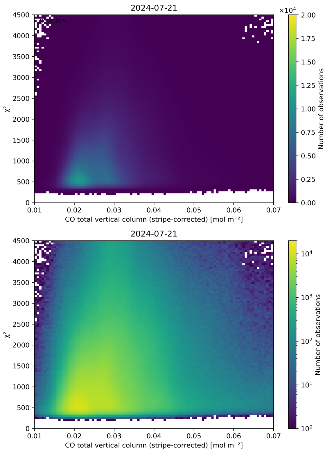
Figure 37: Scatter density plot of “CO total vertical column (stripe-corrected)” against “ \chi^2 ” for 2024-07-21 to 2024-07-22.
