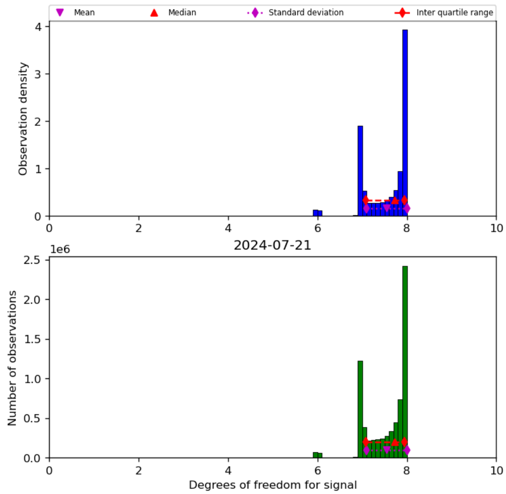
Figure 23: Histogram of “Degrees of freedom for signal” for 2024-07-21 to 2024-07-22
