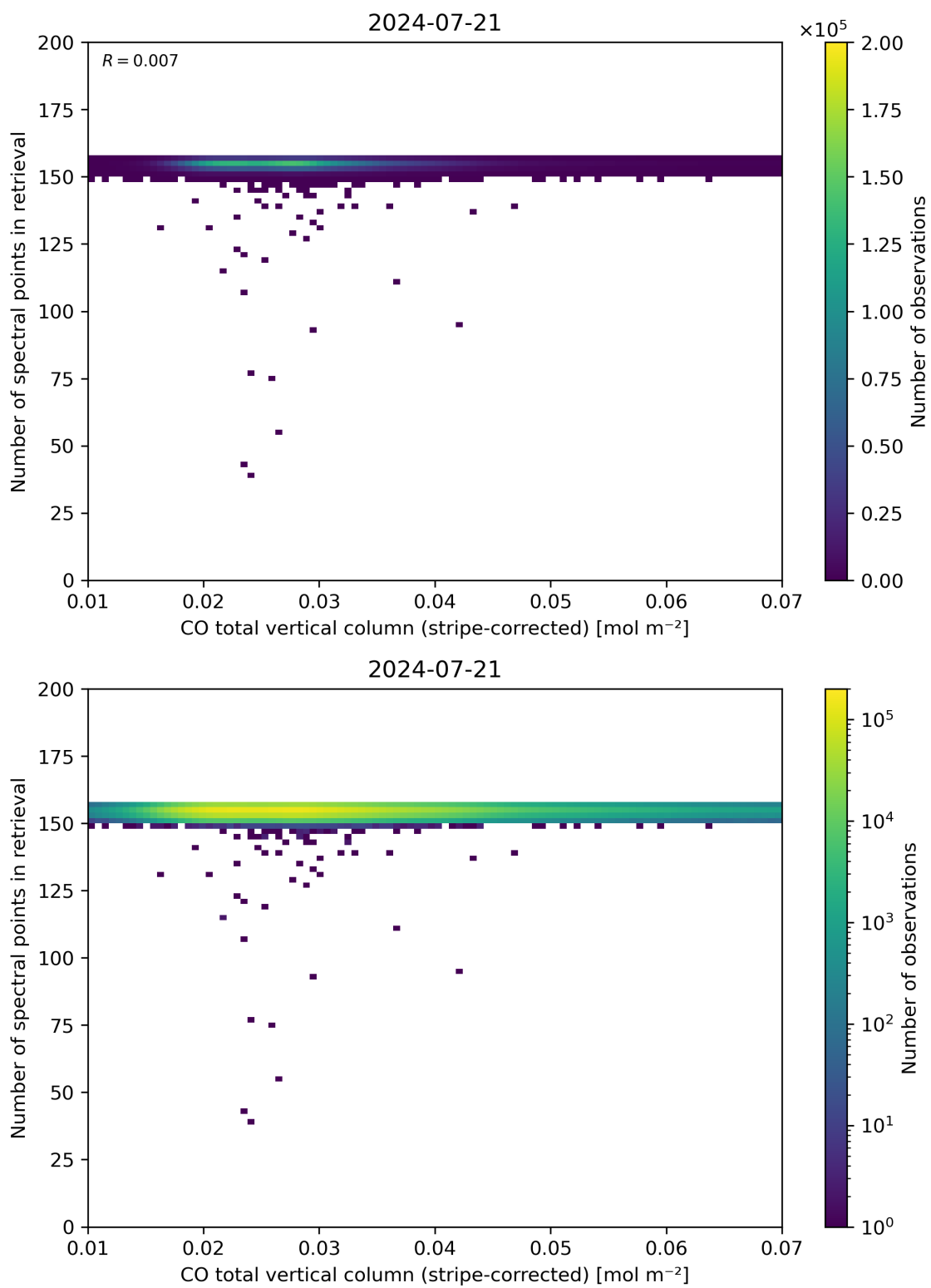
Figure 40: Scatter density plot of “CO total vertical column (stripe-corrected)” against “Number of spectral points in retrieval” for 2024-07-21 to 2024-07-22.
