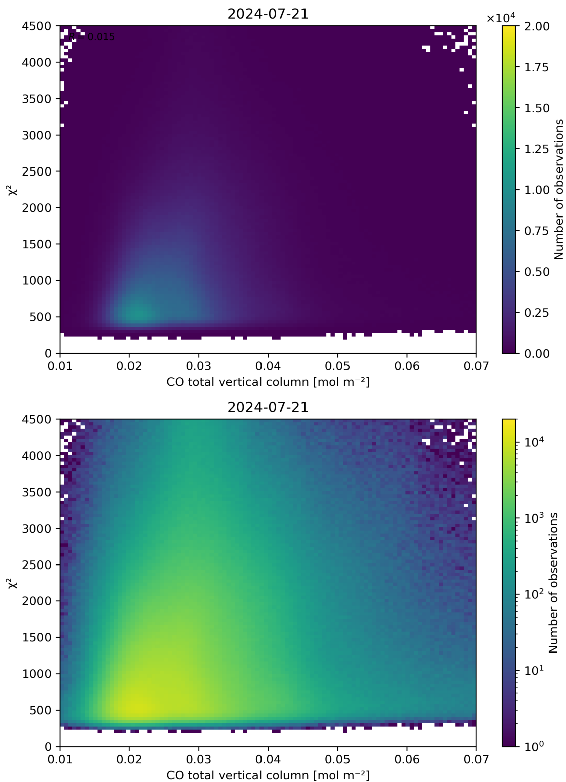
Figure 35: Scatter density plot of “CO total vertical column” against “ \chi^2 ” for 2024-07-21 to 2024-07-22.
