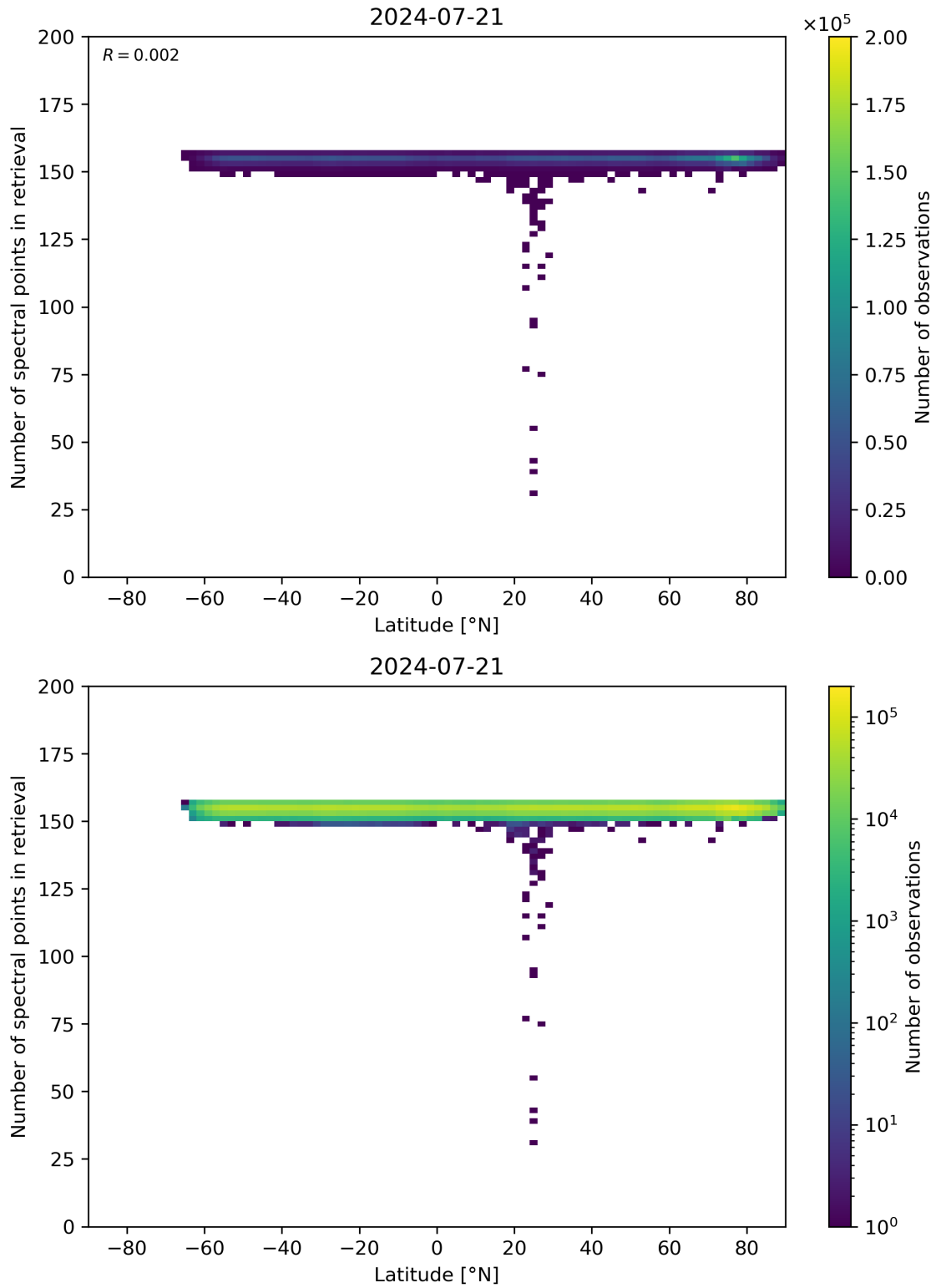
Figure 57: Scatter density plot of “Latitude” against “Number of spectral points in retrieval” for 2024-07-21 to 2024-07-22.
