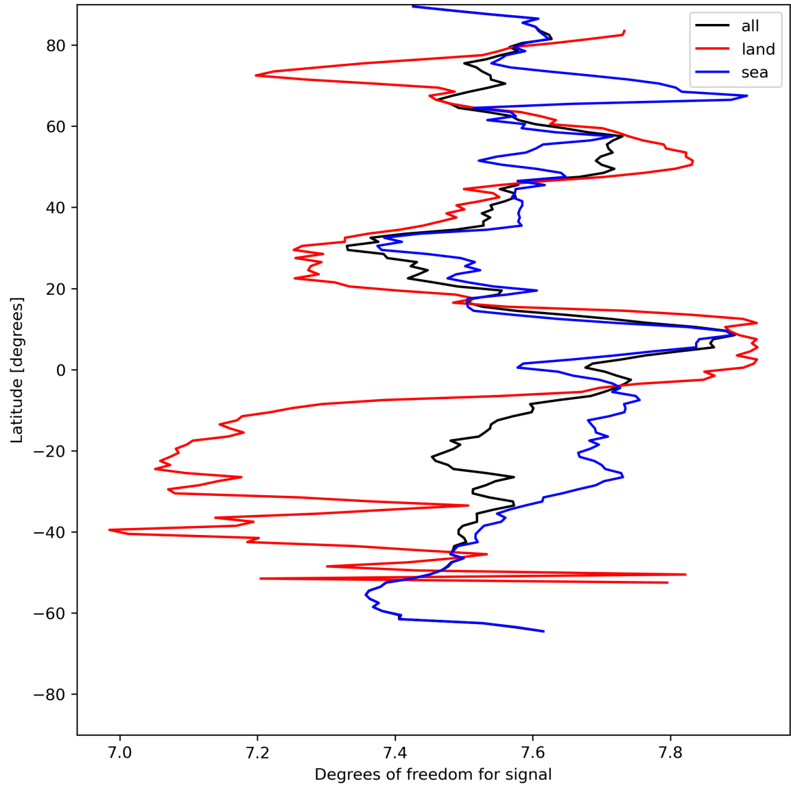
Figure 15: Zonal average of “Degrees of freedom for signal” for 2024-07-21 to 2024-07-22.
