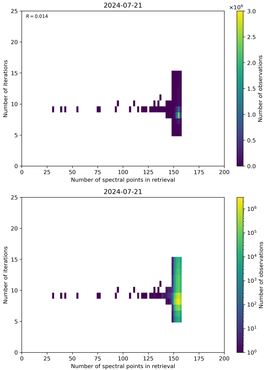
Figure 60: Scatter density plot of “Number of spectral points in retrieval” against “Number of iterations” for 2024-07-21 to 2024-07-22.
