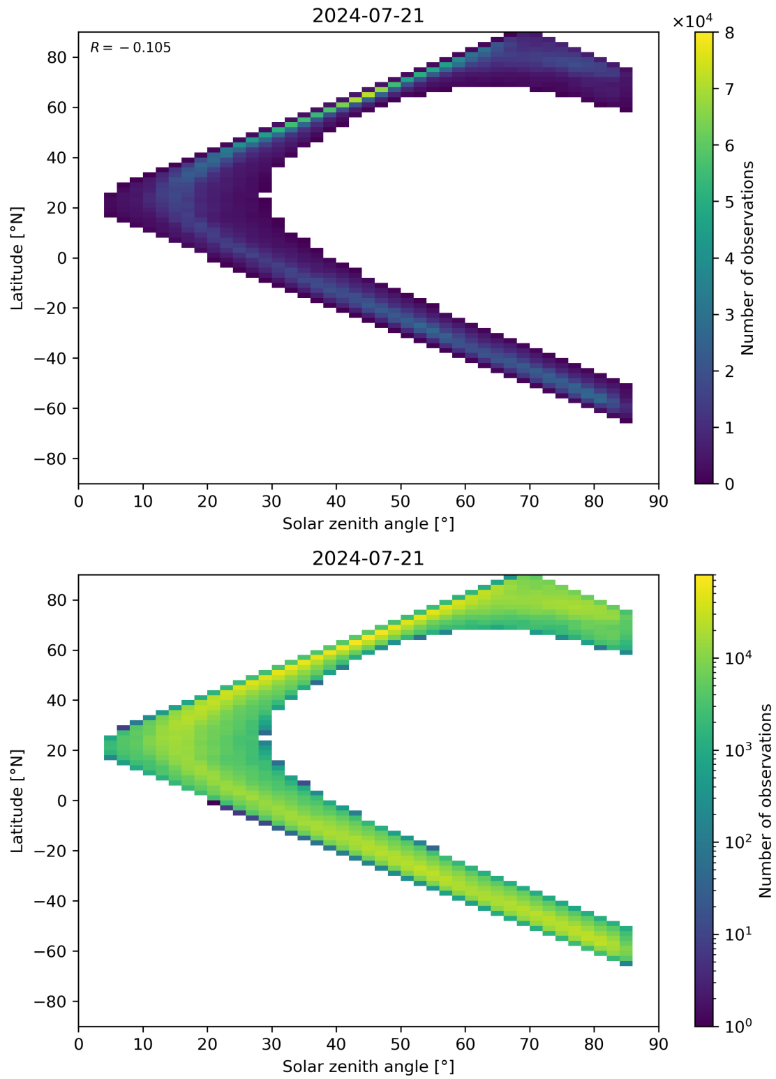
Figure 66: Scatter density plot of “Solar zenith angle” against “Latitude” for 2024-07-21 to 2024-07-22.
