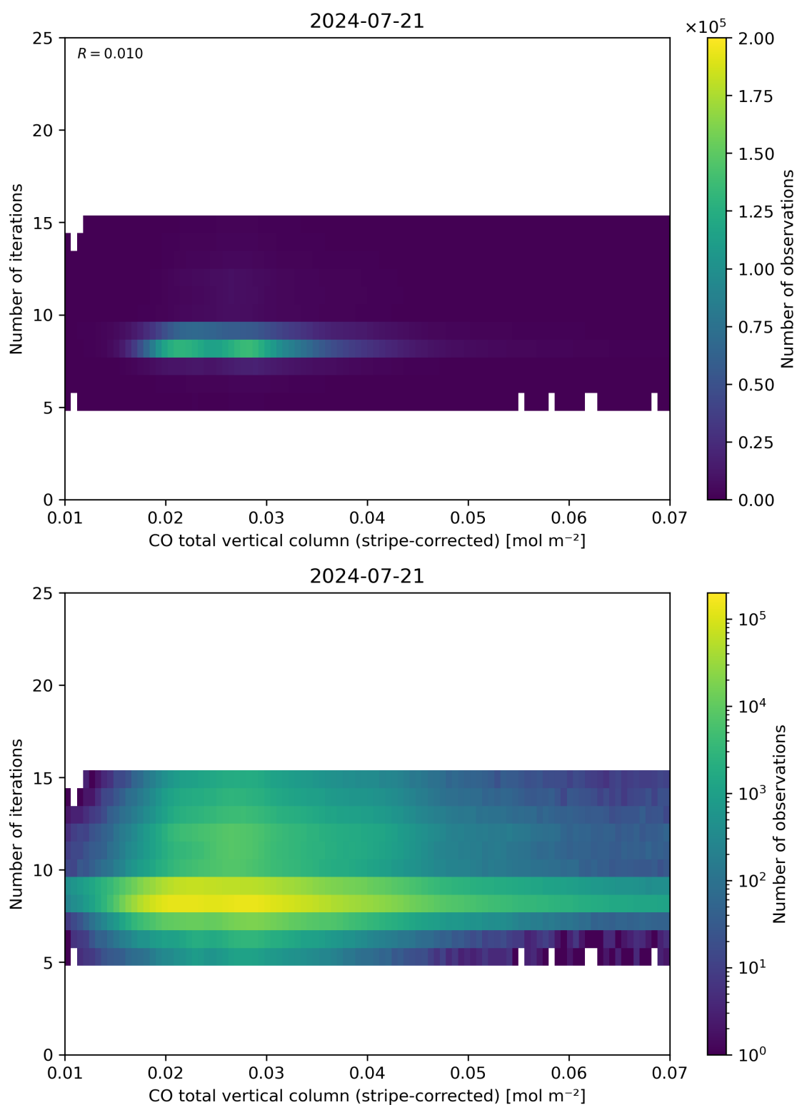
Figure 39: Scatter density plot of “CO total vertical column (stripe-corrected)” against “Number of iterations” for 2024-07-21 to 2024-07-22.
