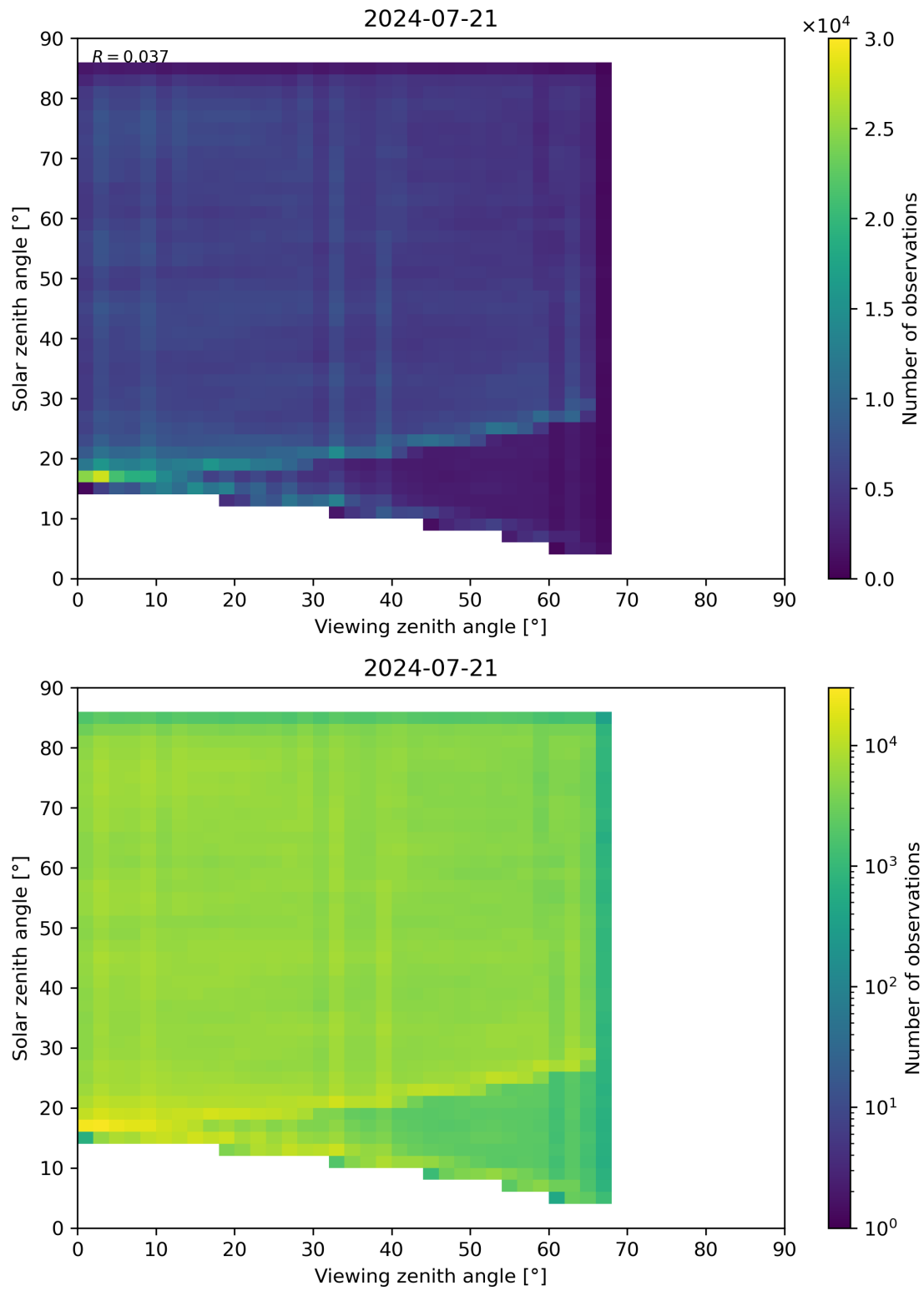
Figure 77: Scatter density plot of “Viewing zenith angle” against “Solar zenith angle” for 2024-07-21 to 2024-07-22.
