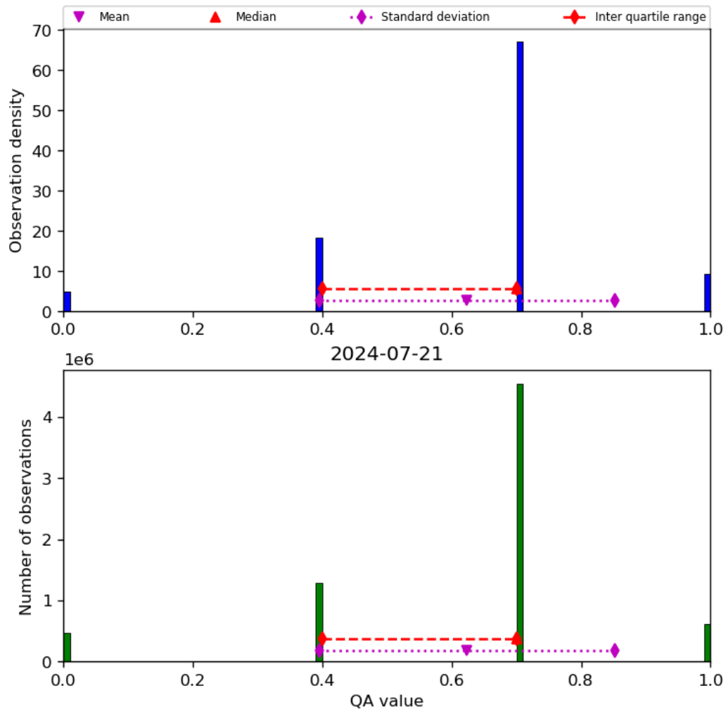
Figure 17: Histogram of “QA value” for 2024-07-21 to 2024-07-22
