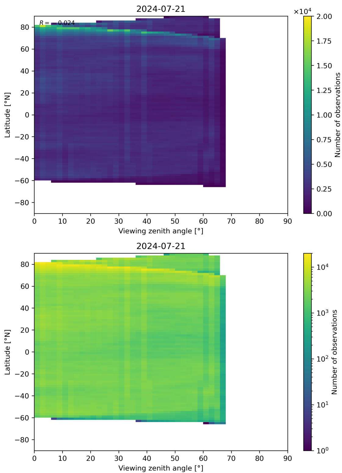
Figure 74: Scatter density plot of “Viewing zenith angle” against “Latitude” for 2024-07-21 to 2024-07-22.
