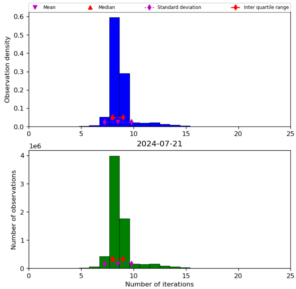
Figure 24: Histogram of “Number of iterations” for 2024-07-21 to 2024-07-22
