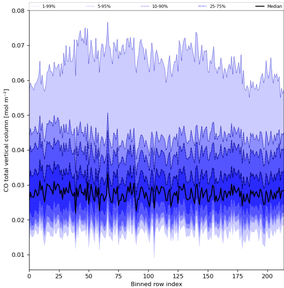
Figure 26: Along track statistics of “CO total vertical column” for 2024-07-21 to 2024-07-22
