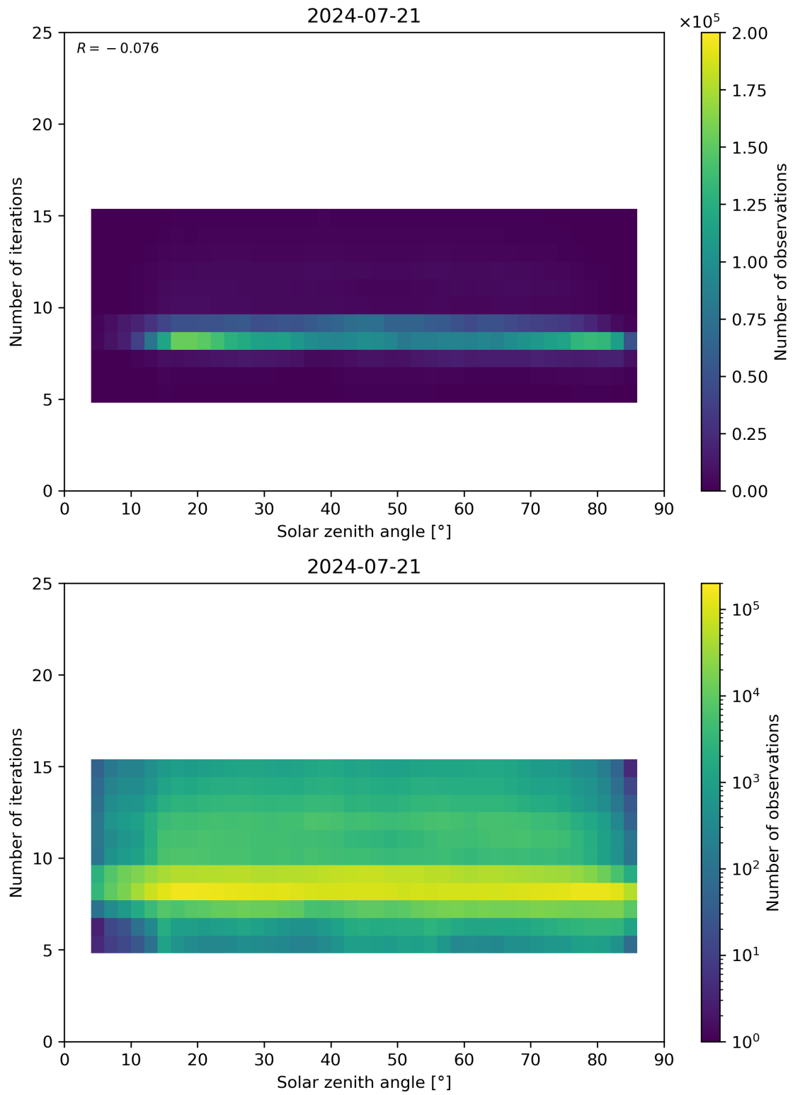
Figure 67: Scatter density plot of “Solar zenith angle” against “Number of iterations” for 2024-07-21 to 2024-07-22.
