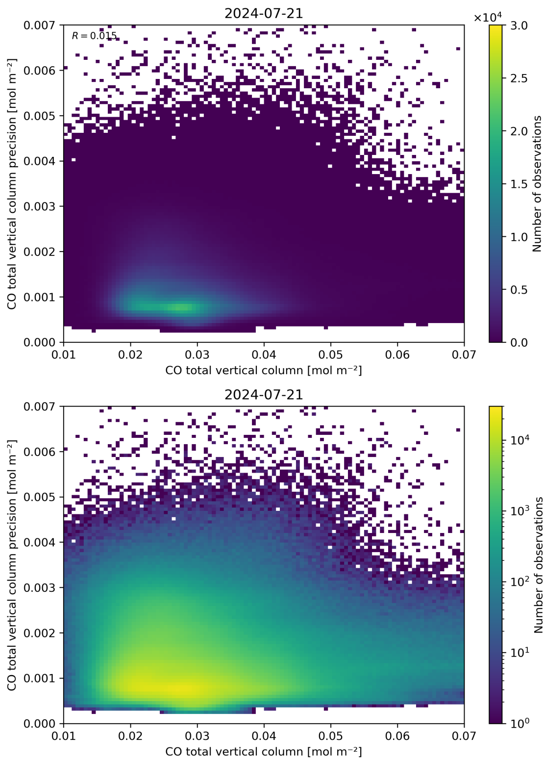
Figure 34: Scatter density plot of “CO total vertical column” against “CO total vertical column precision” for 2024-07-21 to 2024-07-22.
