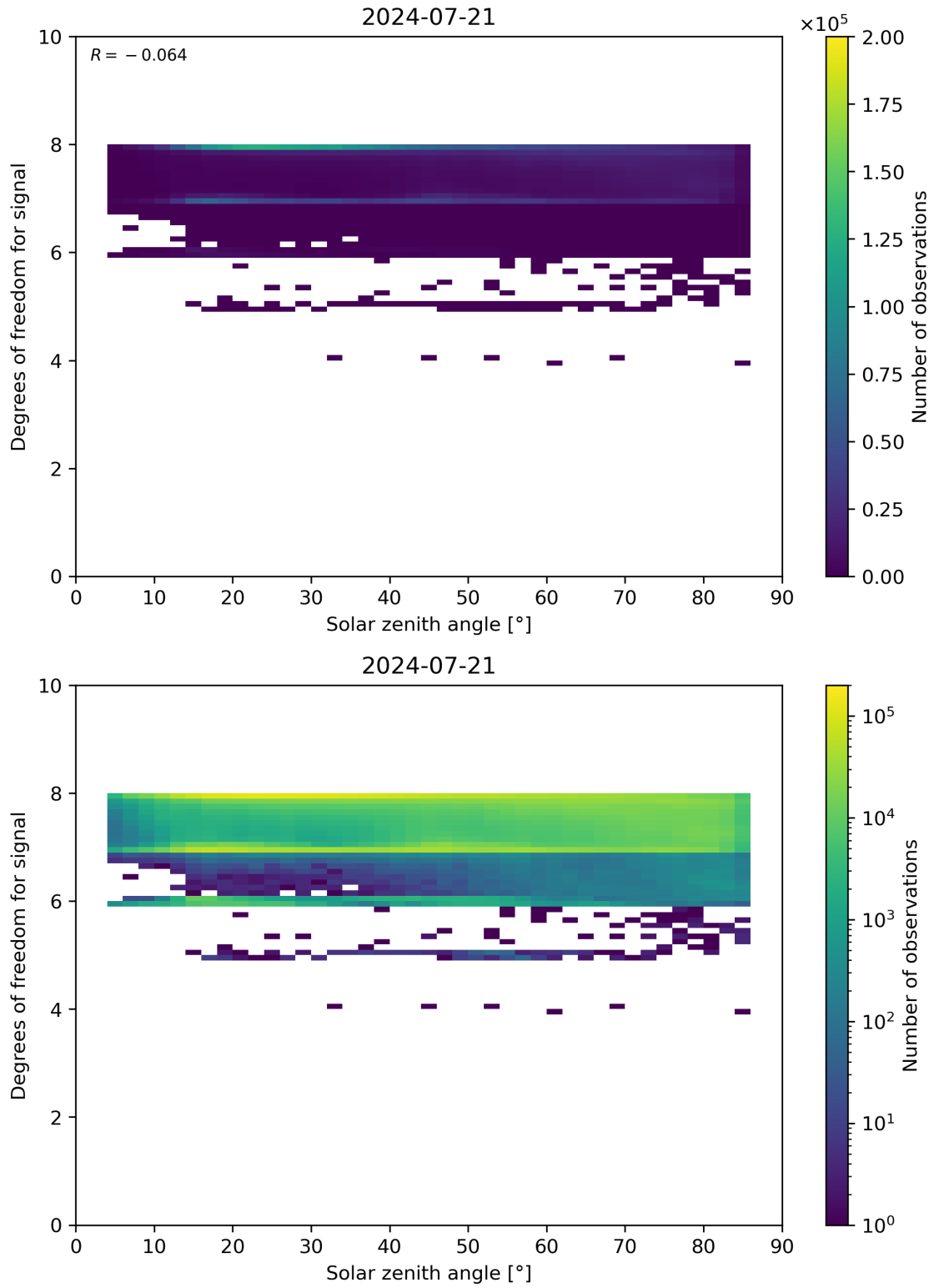
Figure 65: Scatter density plot of “Solar zenith angle” against “Degrees of freedom for signal” for 2024-07-21 to 2024-07-22.
