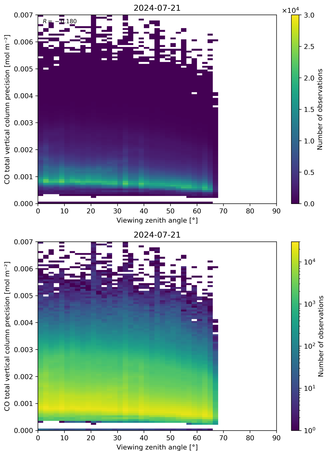
Figure 71: Scatter density plot of “Viewing zenith angle” against “CO total vertical column precision” for 2024-07-21 to 2024-07-22.
