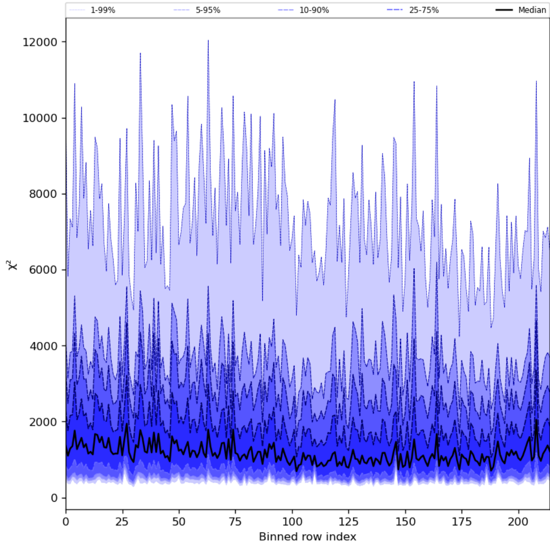
Figure 30: Along track statistics of “ \chi^2 ” for 2024-07-21 to 2024-07-22
