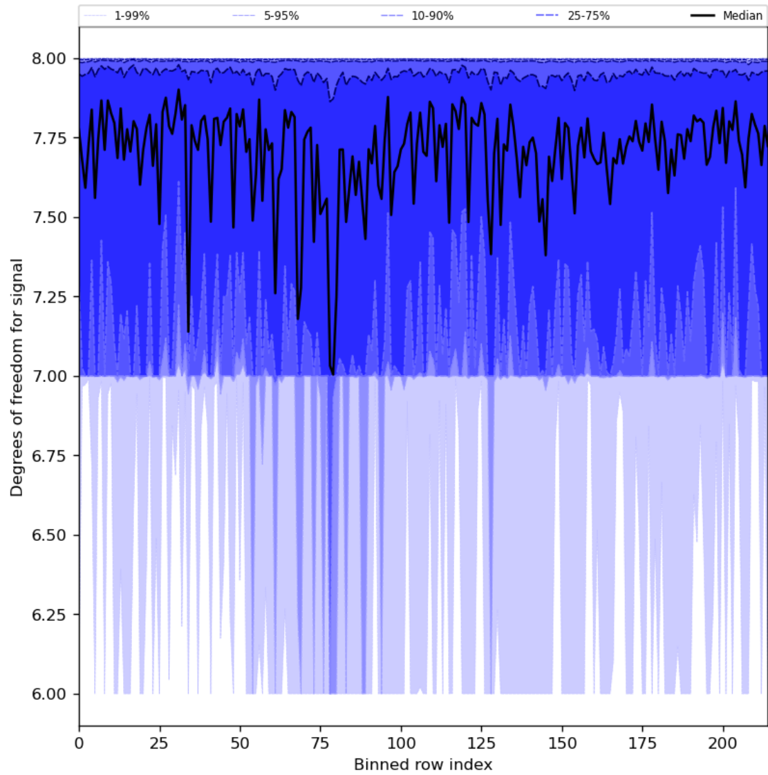
Figure 31: Along track statistics of “Degrees of freedom for signal” for 2024-07-21 to 2024-07-22
