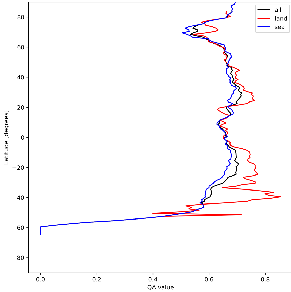
Figure 9: Zonal average of “QA value” for 2024-07-21 to 2024-07-22.
