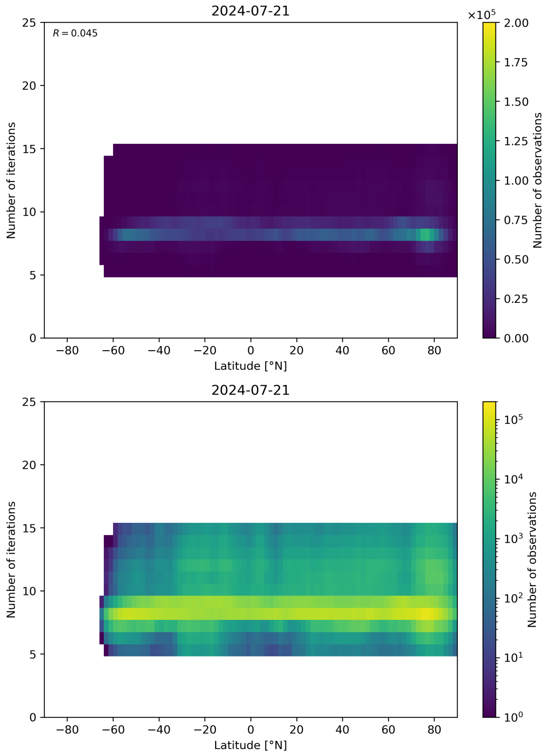
Figure 56: Scatter density plot of “Latitude” against “Number of iterations” for 2024-07-21 to 2024-07-22.
