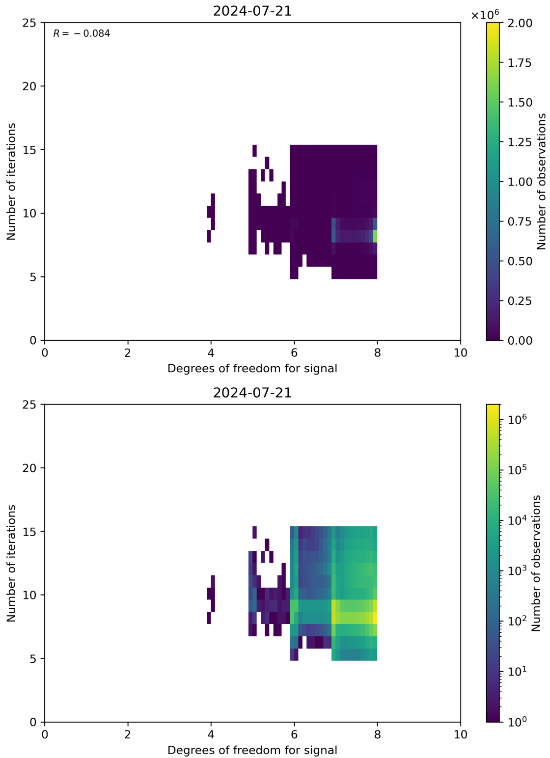
Figure 50: Scatter density plot of “Degrees of freedom for signal” against “Number of iterations” for 2024-07-21 to 2024-07-22.
