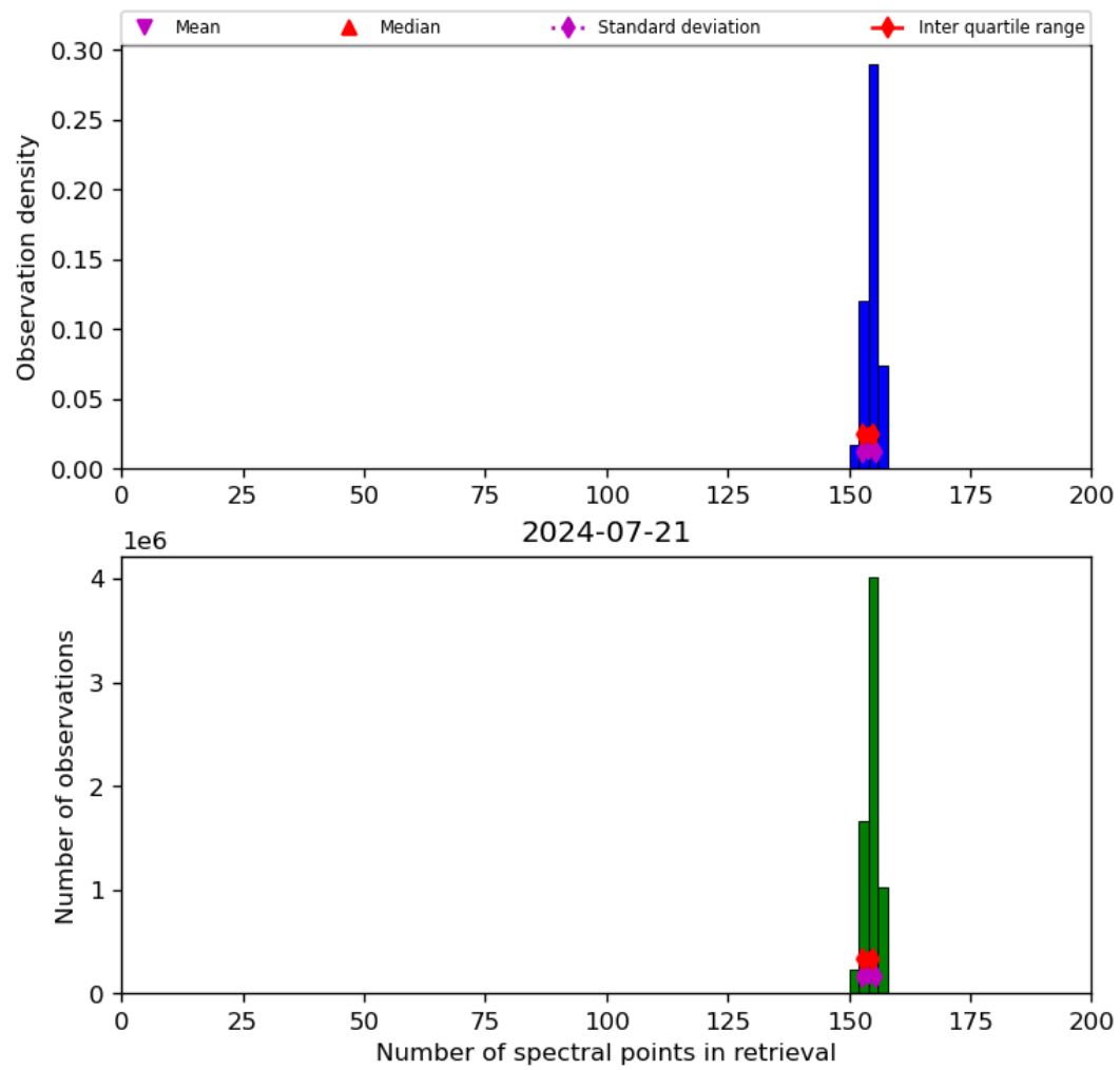
Figure 21: Histogram of “Number of spectral points in retrieval” for 2024-07-21 to 2024-07-22
