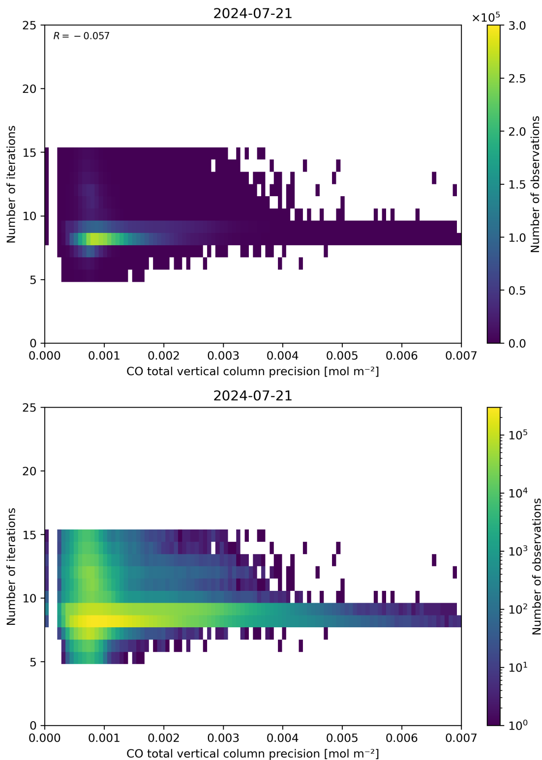
Figure 46: Scatter density plot of “CO total vertical column precision” against “Number of iterations” for 2024-07-21 to 2024-07-22.
