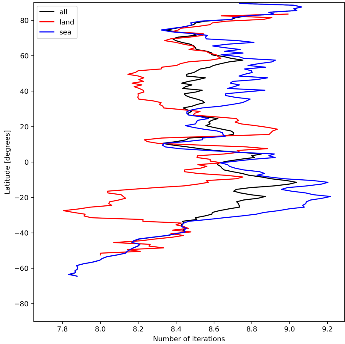
Figure 16: Zonal average of “Number of iterations” for 2024-07-21 to 2024-07-22.
