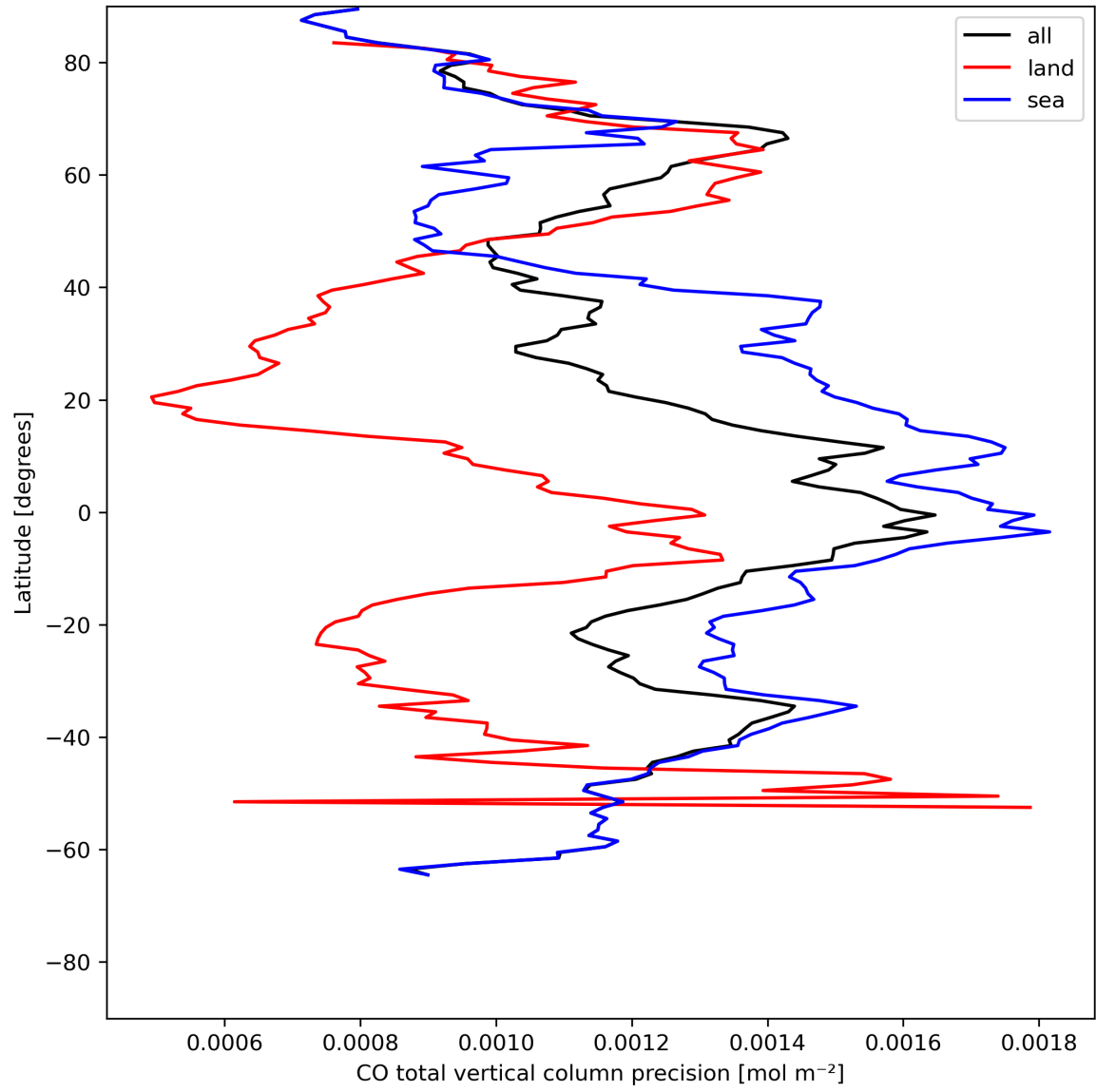
Figure 12: Zonal average of "CO total vertical column precision" for 2024-07-21 to 2024-07-22.
