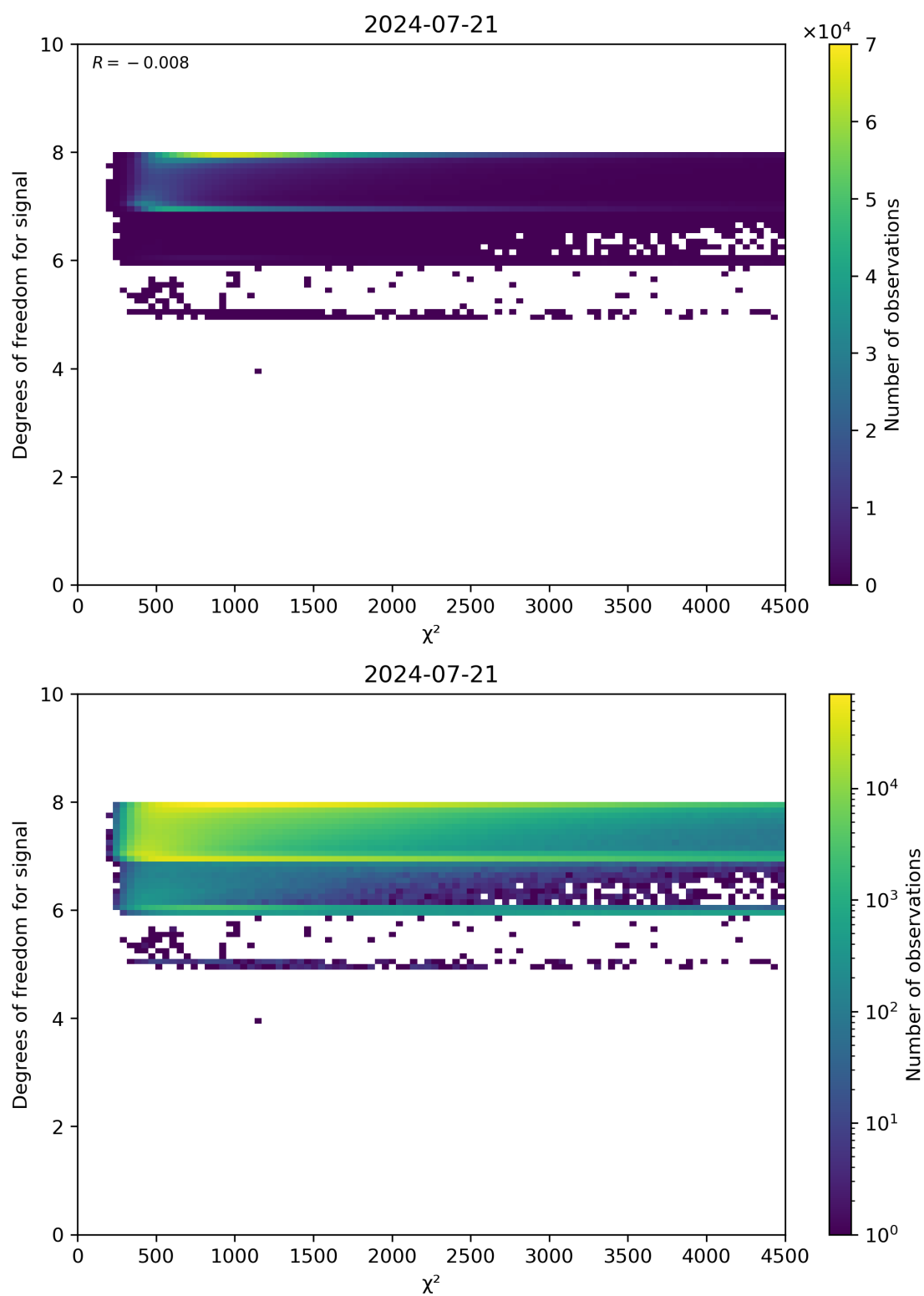
Figure 48: Scatter density plot of “ \chi^2 ” against “Degrees of freedom for signal” for 2024-07-21 to 2024-07-22.
