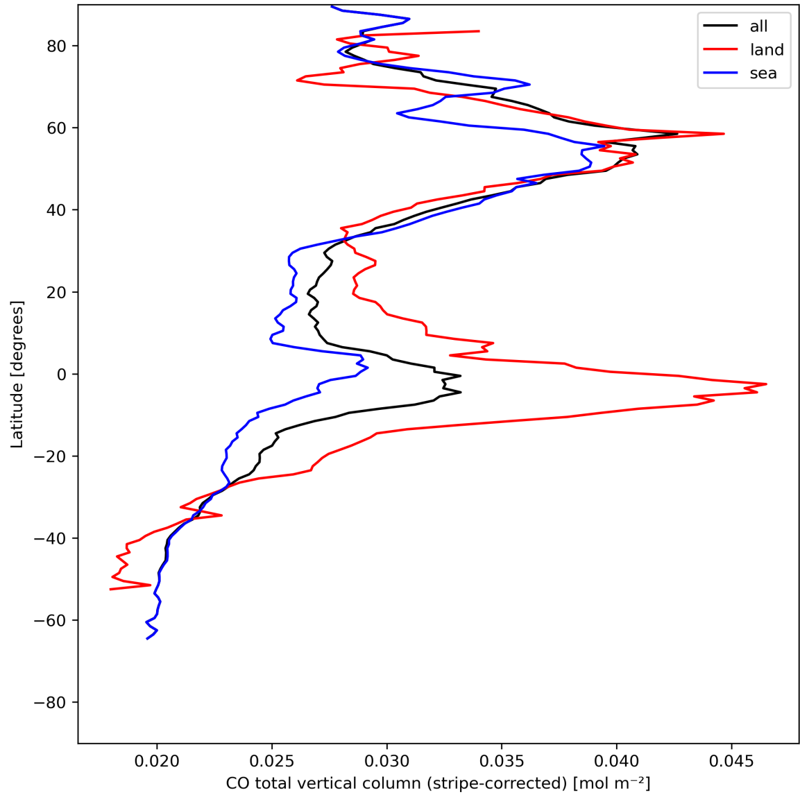
Figure 11: Zonal average of “CO total vertical column (stripe-corrected)” for 2024-07-21 to 2024-07-22.
