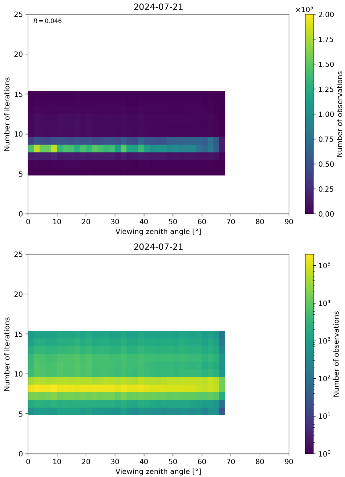
Figure 75: Scatter density plot of “Viewing zenith angle” against “Number of iterations” for 2024-07-21 to 2024-07-22.
