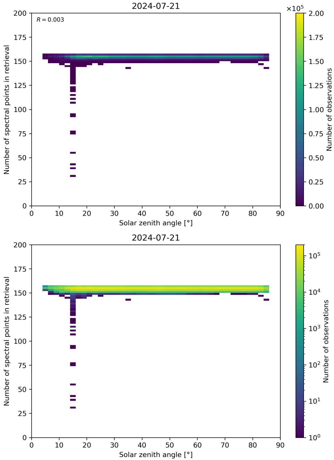
Figure 68: Scatter density plot of “Solar zenith angle” against “Number of spectral points in retrieval” for 2024-07-21 to 2024-07-22.
