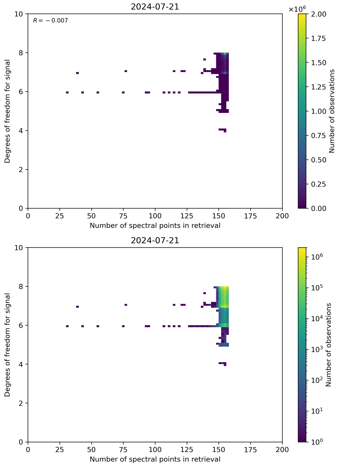
Figure 59: Scatter density plot of “Number of spectral points in retrieval” against “Degrees of freedom for signal” for 2024-07-21 to 2024-07-22.
