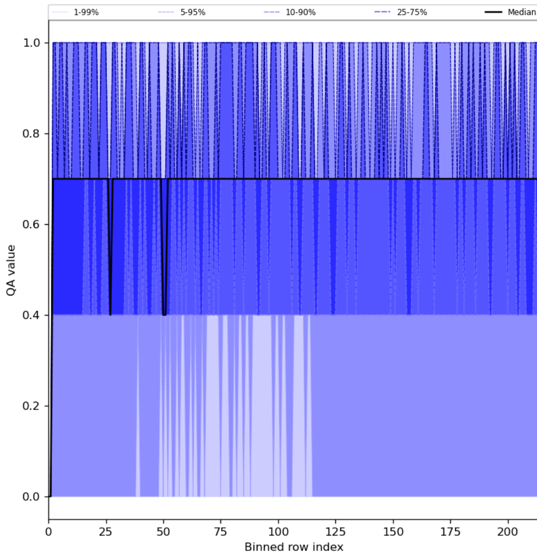
Figure 25: Along track statistics of “QA value” for 2024-07-21 to 2024-07-22
