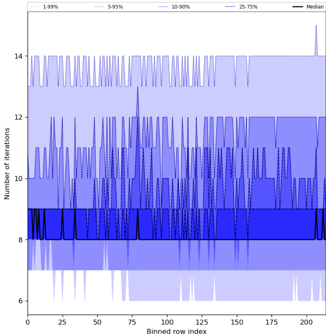
Figure 32: Along track statistics of “Number of iterations” for 2024-07-21 to 2024-07-22
