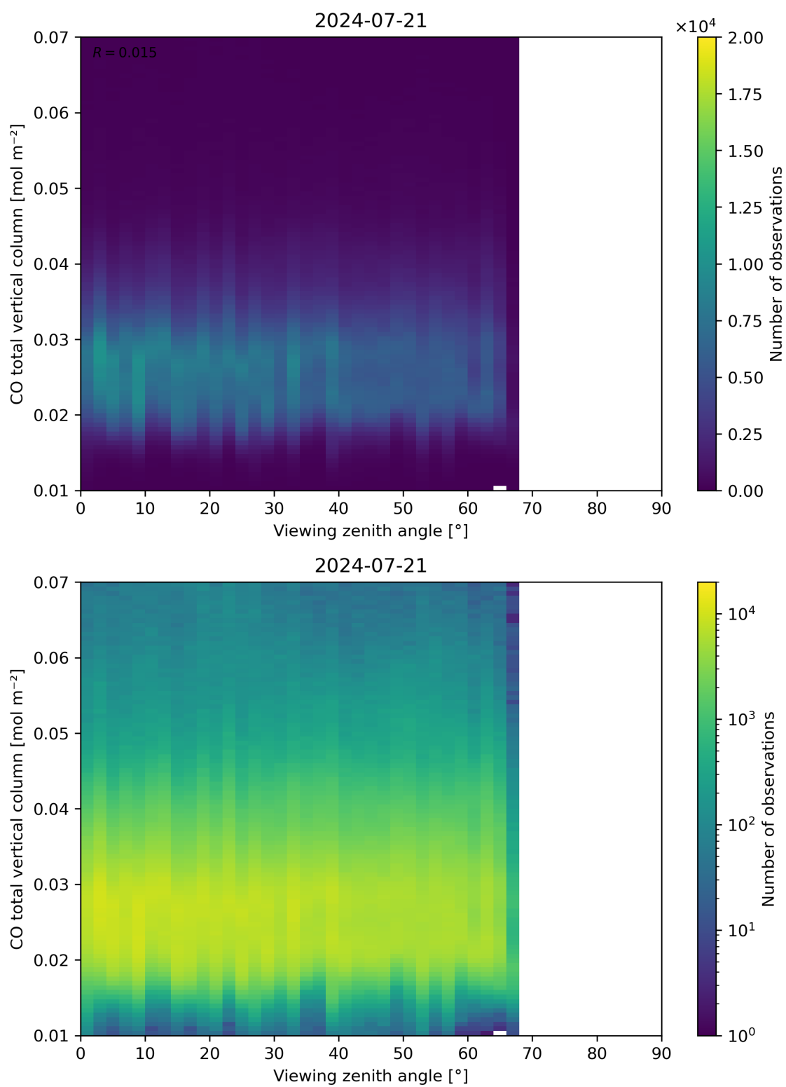
Figure 69: Scatter density plot of “Viewing zenith angle” against “CO total vertical column” for 2024-07-21 to 2024-07-22.
