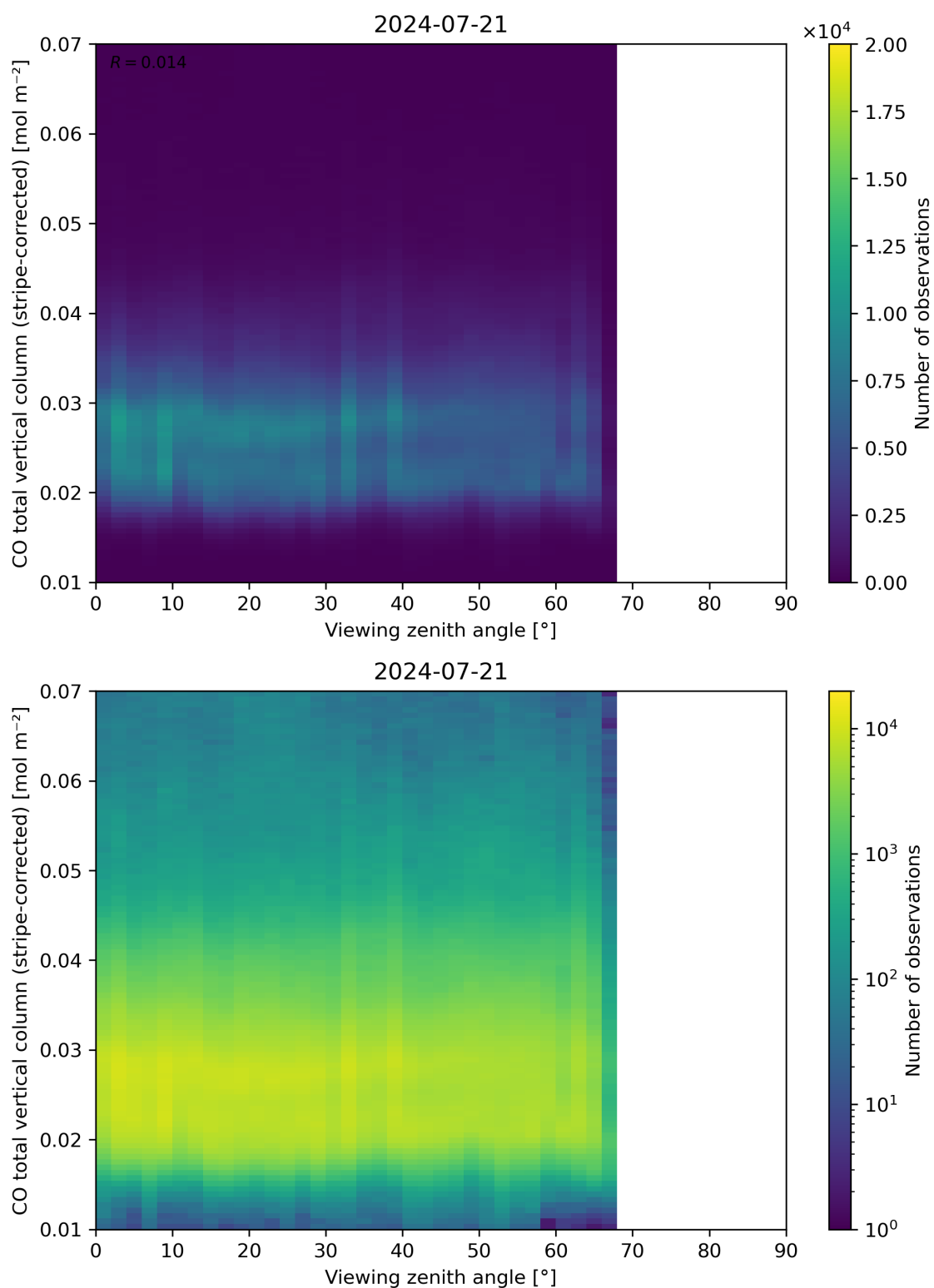
Figure 70: Scatter density plot of “Viewing zenith angle” against “CO total vertical column (stripe-corrected)” for 2024-07-21 to 2024-07-22.
