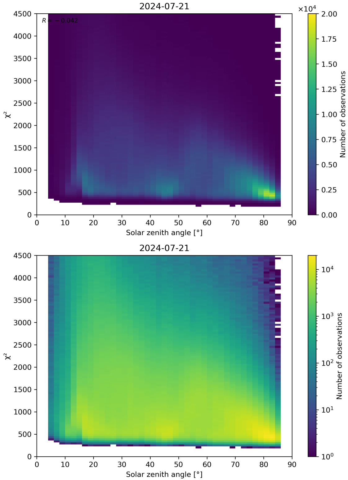
Figure 64: Scatter density plot of “Solar zenith angle” against “ \chi^2 ” for 2024-07-21 to 2024-07-22.
