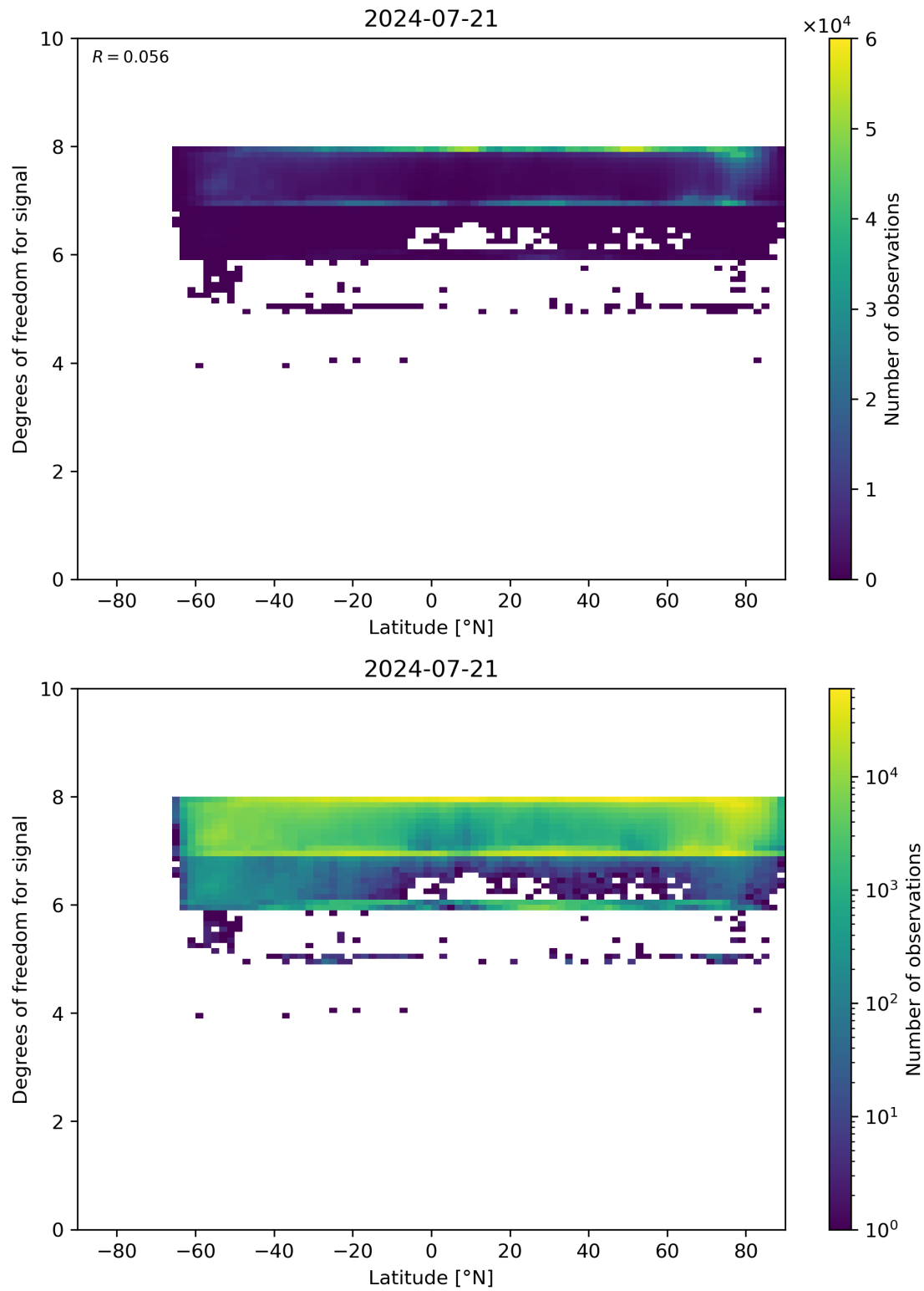
Figure 55: Scatter density plot of “Latitude” against “Degrees of freedom for signal” for 2024-07-21 to 2024-07-22.
