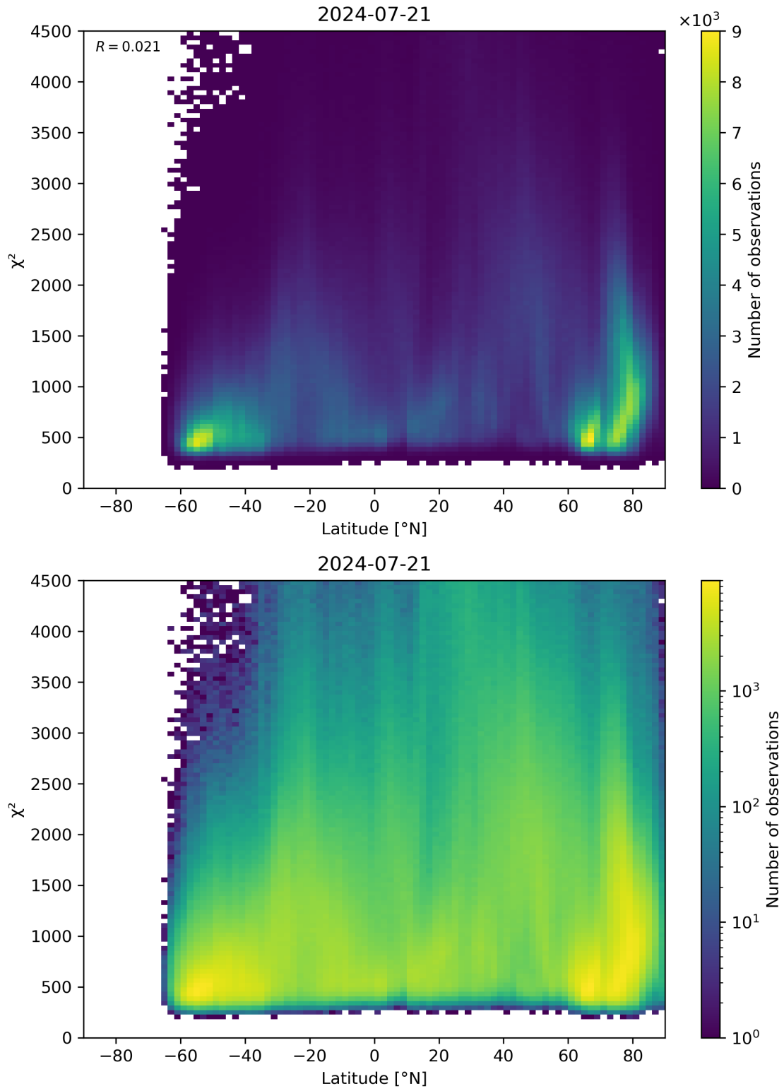
Figure 54: Scatter density plot of “Latitude” against “ \chi^2 ” for 2024-07-21 to 2024-07-22.
