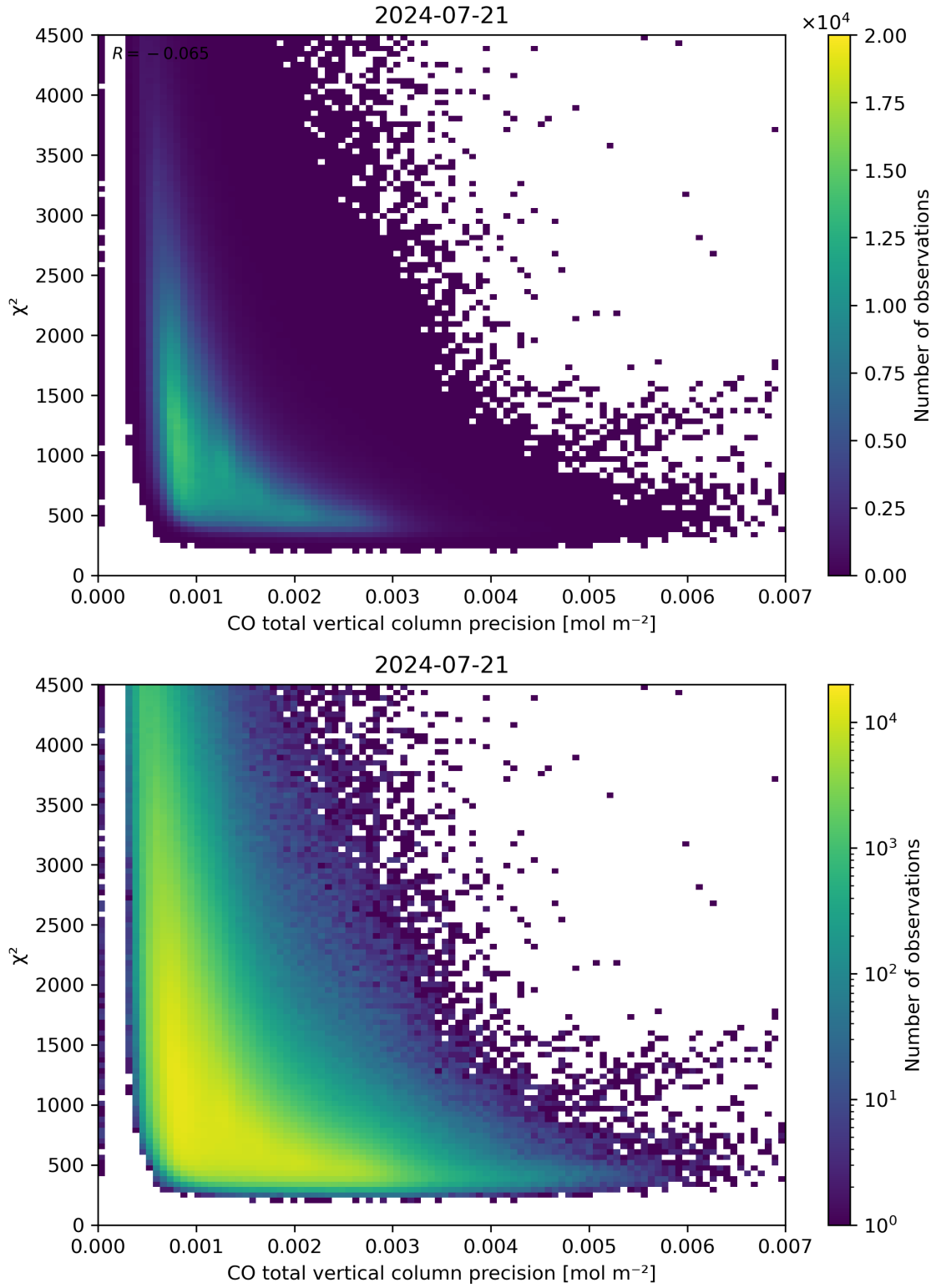
Figure 44: Scatter density plot of “CO total vertical column precision” against “ \chi^2 ” for 2024-07-21 to 2024-07-22.
