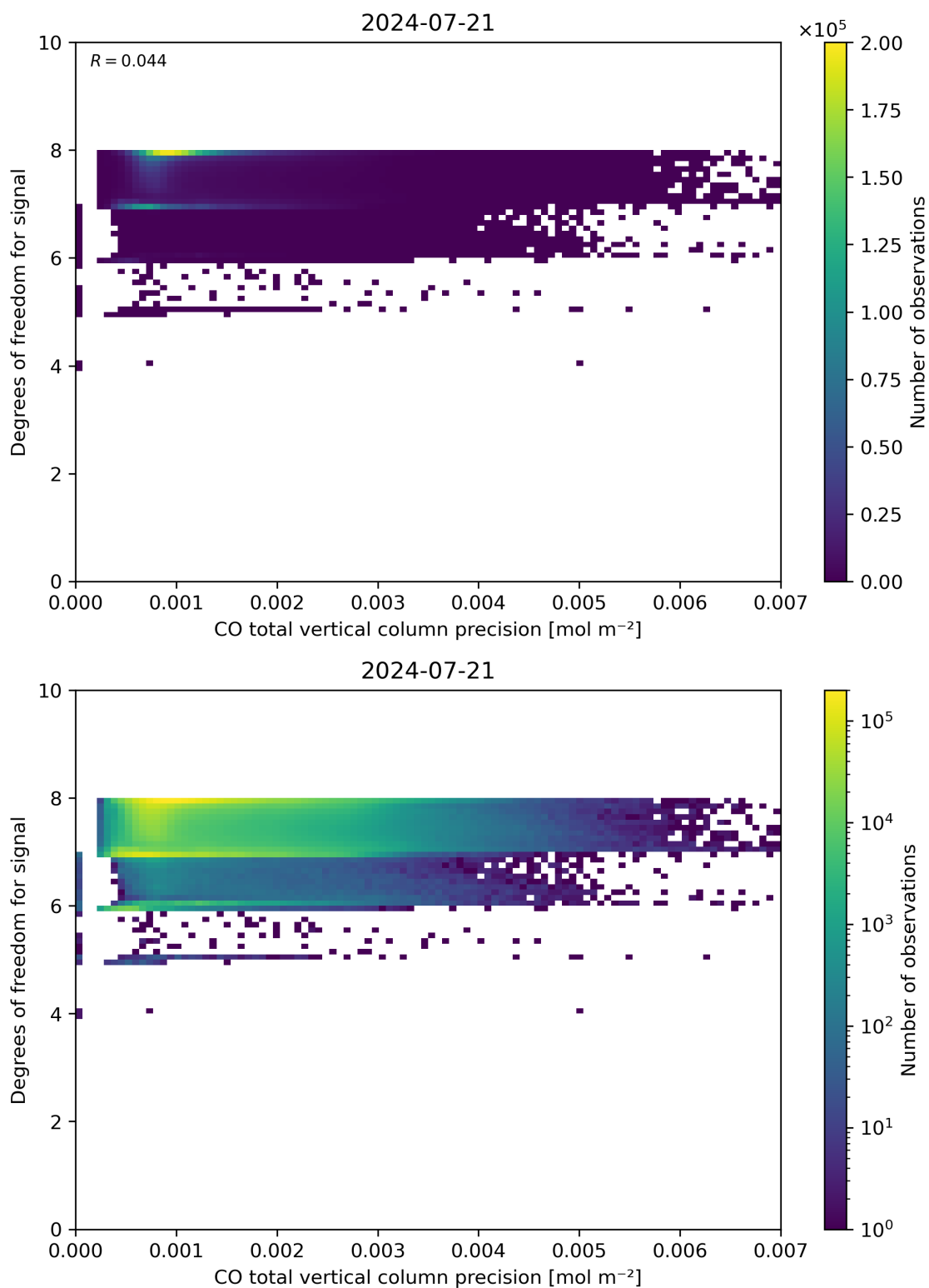
Figure 45: Scatter density plot of “CO total vertical column precision” against “Degrees of freedom for signal” for 2024-07-21 to 2024-07-22.
