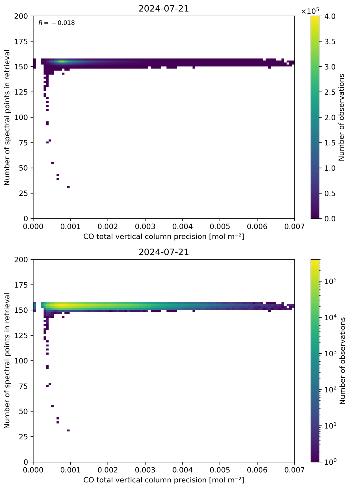
Figure 47: Scatter density plot of “CO total vertical column precision” against “Number of spectral points in retrieval” for 2024-07-21 to 2024-07-22.
