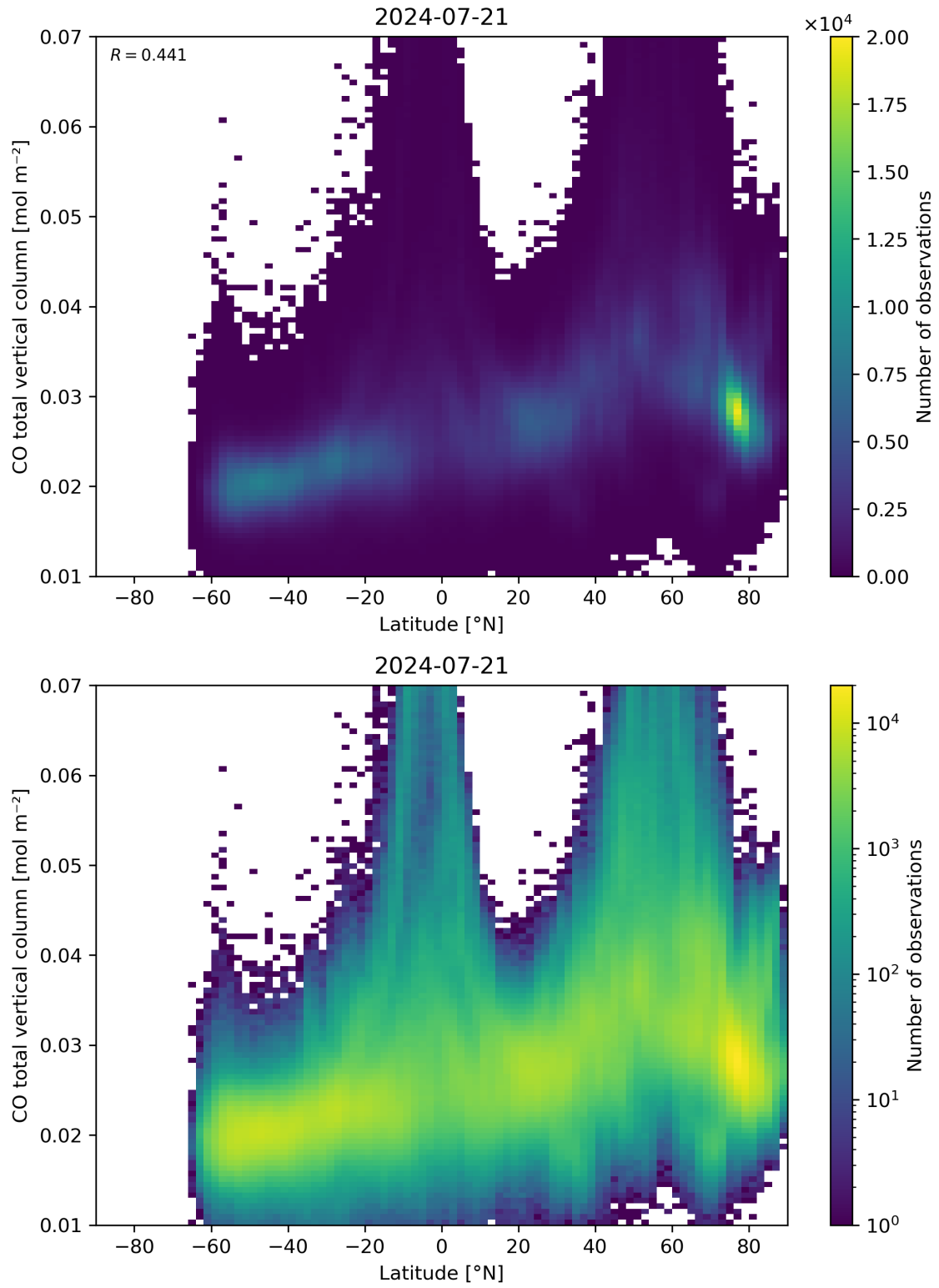
Figure 51: Scatter density plot of “Latitude” against “CO total vertical column” for 2024-07-21 to 2024-07-22.
