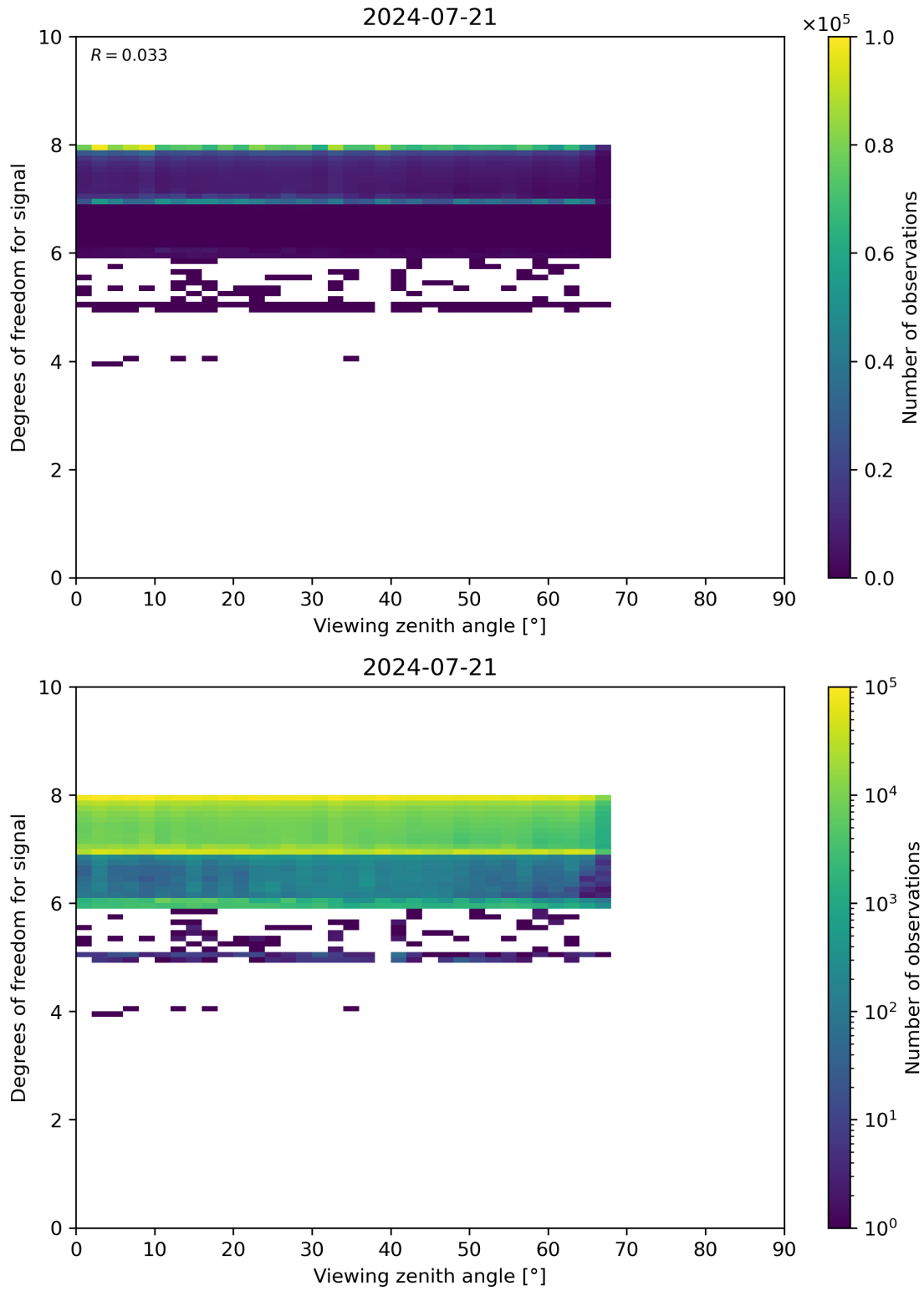
Figure 73: Scatter density plot of “Viewing zenith angle” against “Degrees of freedom for signal” for 2024-07-21 to 2024-07-22.
