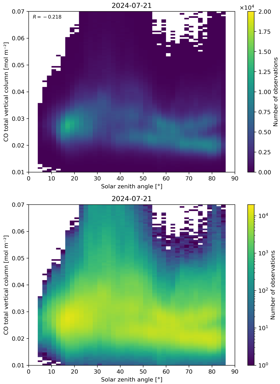
Figure 61: Scatter density plot of “Solar zenith angle” against “CO total vertical column” for 2024-07-21 to 2024-07-22.
