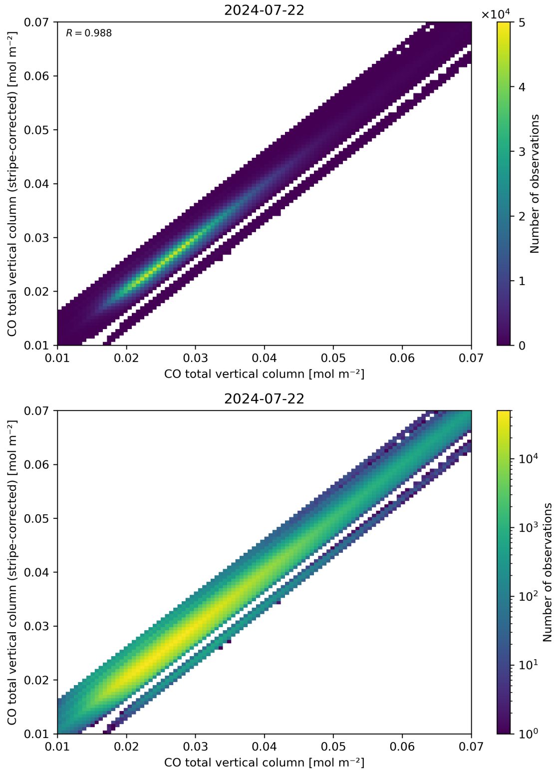
Figure 33: Scatter density plot of “CO total vertical column” against “CO total vertical column (stripe-corrected)” for 2024-07-21 to 2024-07-23.
