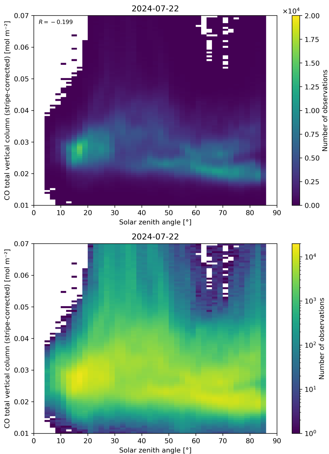
Figure 62: Scatter density plot of “Solar zenith angle” against “CO total vertical column (stripe-corrected)” for 2024-07-21 to 2024-07-23.
