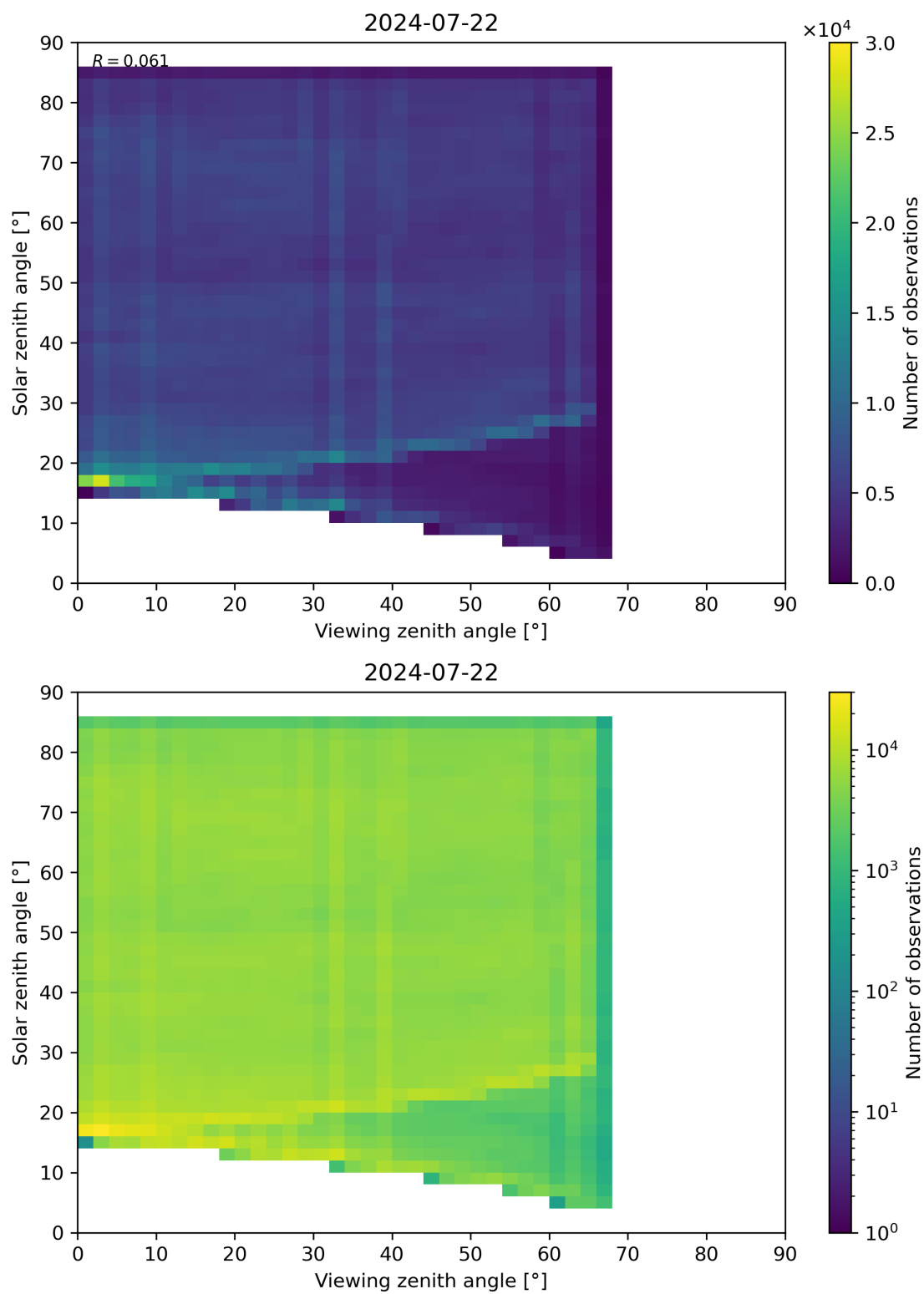
Figure 77: Scatter density plot of “Viewing zenith angle” against “Solar zenith angle” for 2024-07-21 to 2024-07-23.
