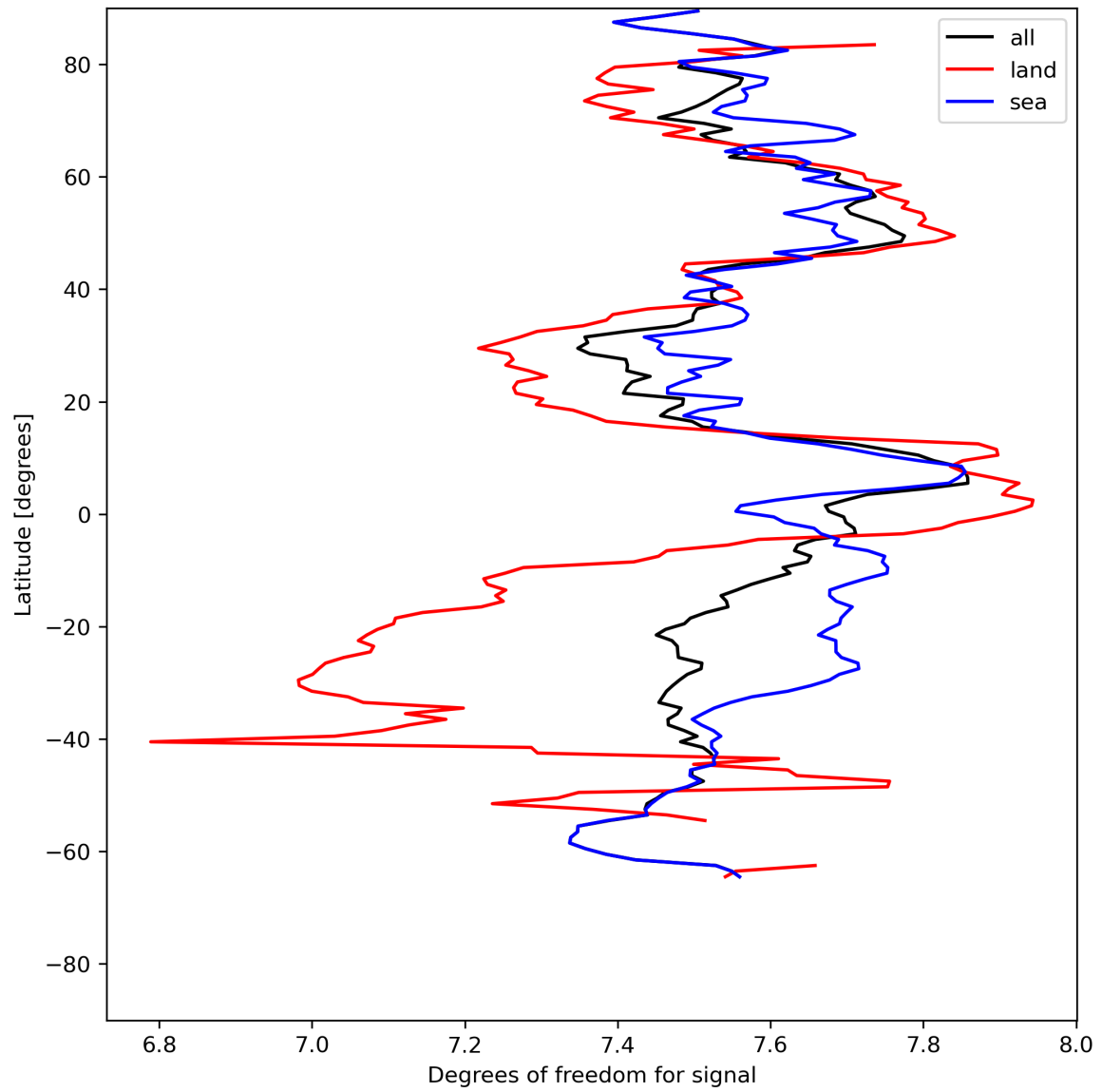
Figure 15: Zonal average of “Degrees of freedom for signal” for 2024-07-21 to 2024-07-23.
