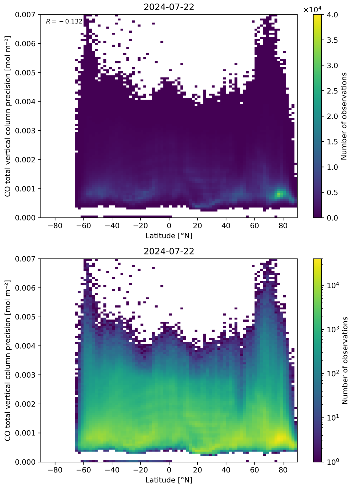
Figure 53: Scatter density plot of “Latitude” against “CO total vertical column precision” for 2024-07-21 to 2024-07-23.
