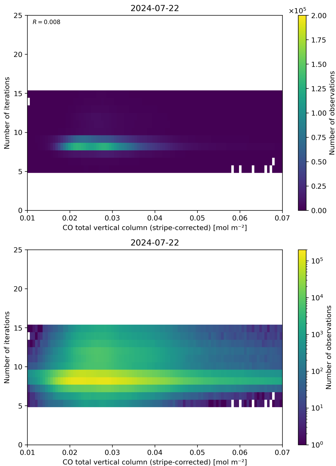
Figure 39: Scatter density plot of “CO total vertical column (stripe-corrected)” against “Number of iterations” for 2024-07-21 to 2024-07-23.
