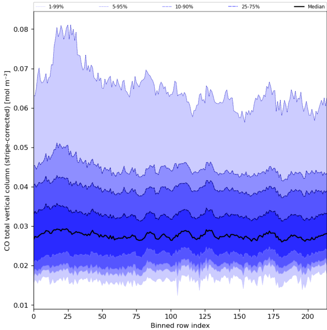
Figure 27: Along track statistics of “CO total vertical column (stripe-corrected)” for 2024-07-21 to 2024-07-23
