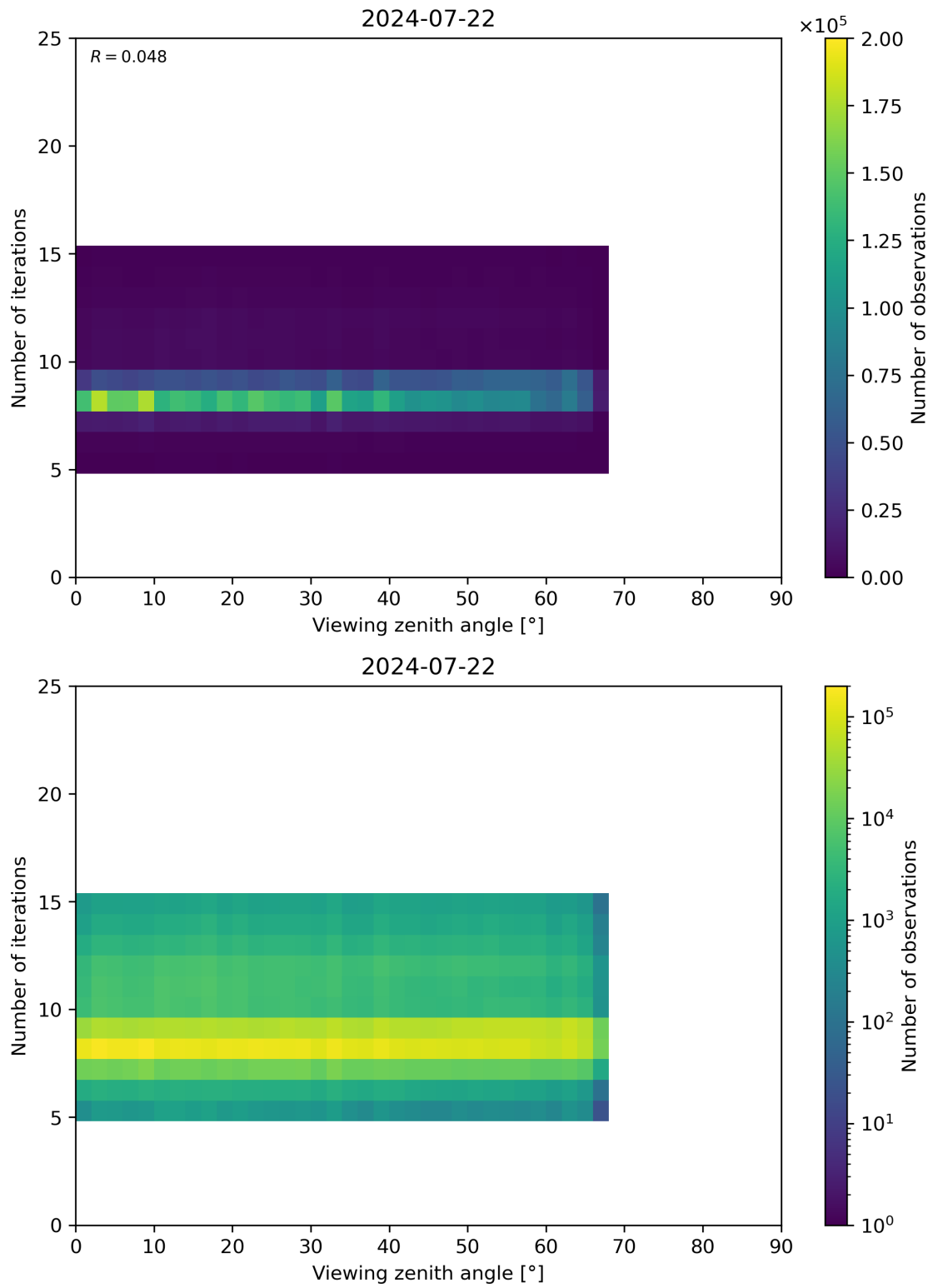
Figure 75: Scatter density plot of “Viewing zenith angle” against “Number of iterations” for 2024-07-21 to 2024-07-23.
