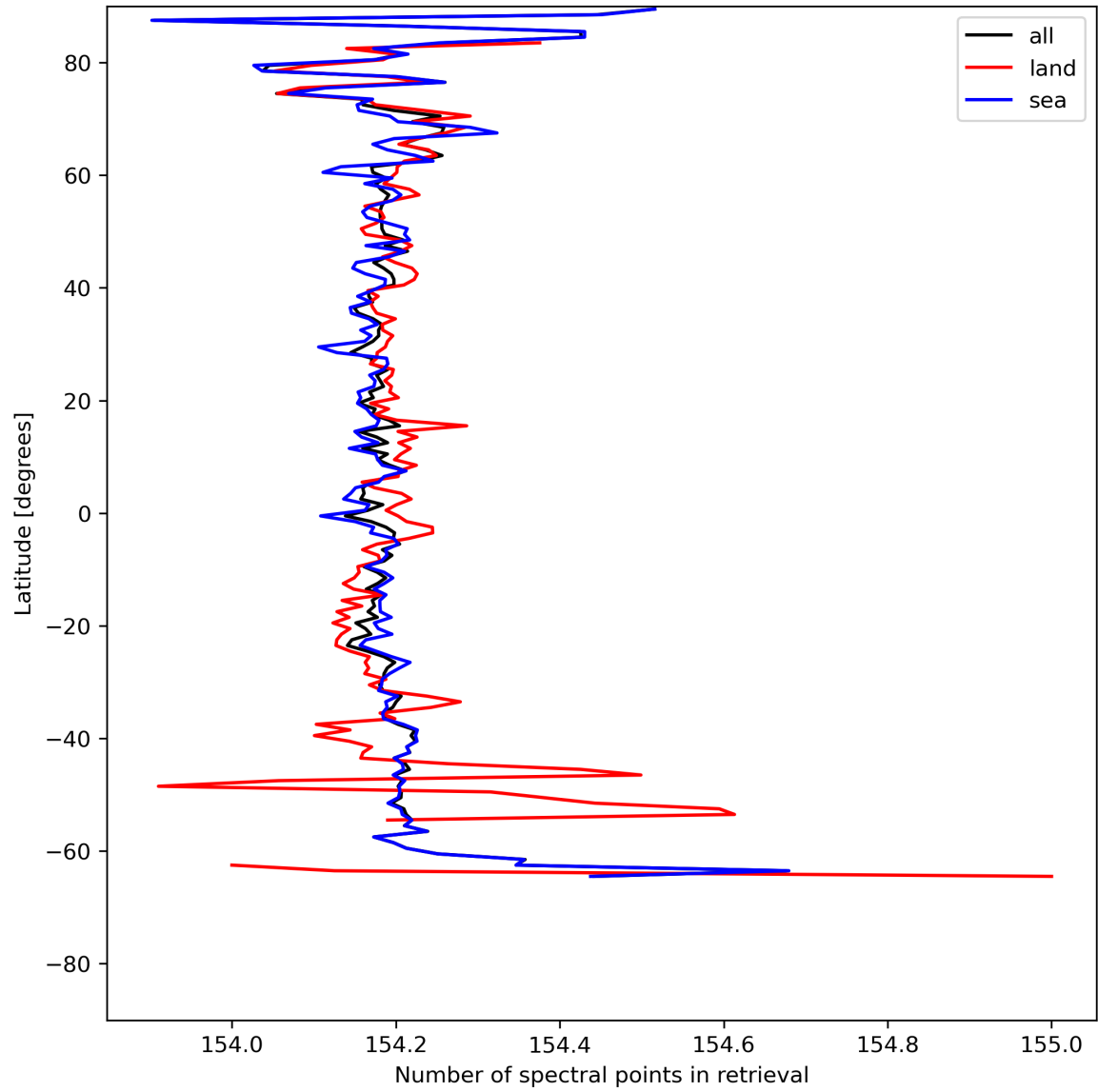
Figure 13: Zonal average of “Number of spectral points in retrieval” for 2024-07-21 to 2024-07-23.
