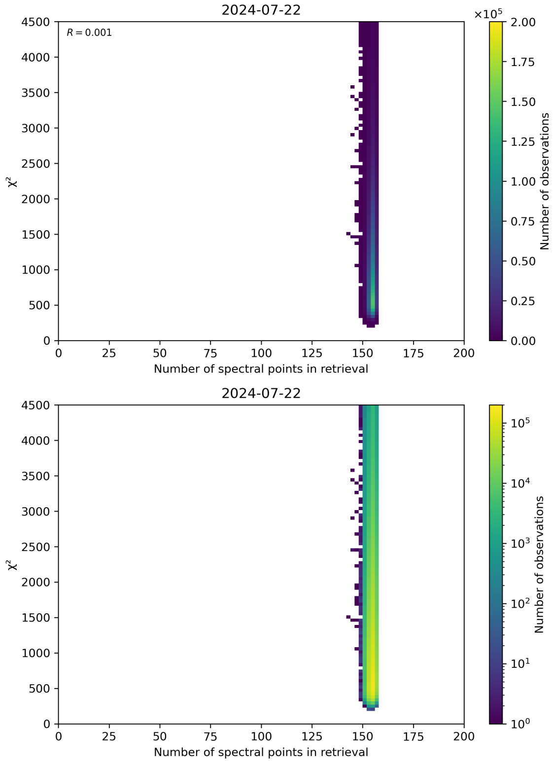
Figure 58: Scatter density plot of “Number of spectral points in retrieval” against “ \chi^2 ” for 2024-07-21 to 2024-07-23.
