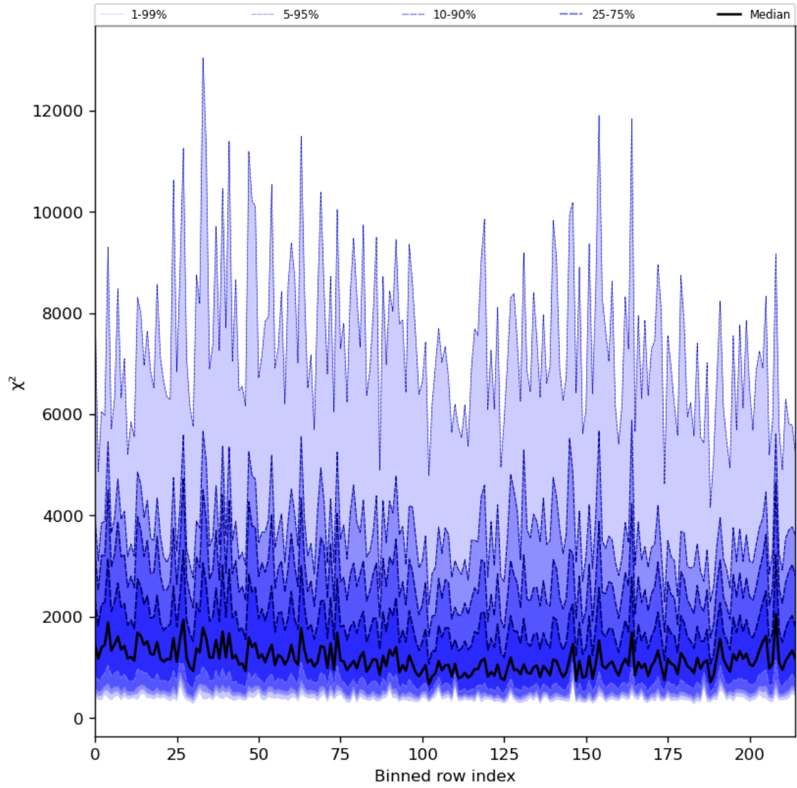
Figure 30: Along track statistics of “ \chi^2 ” for 2024-07-21 to 2024-07-23
