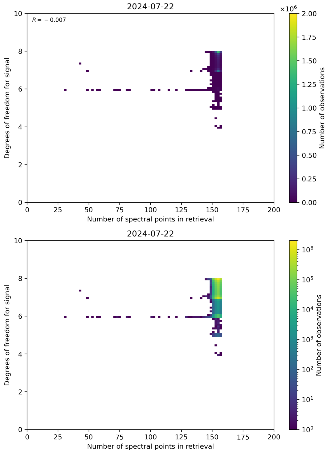
Figure 59: Scatter density plot of “Number of spectral points in retrieval” against “Degrees of freedom for signal” for 2024-07-21 to 2024-07-23.
