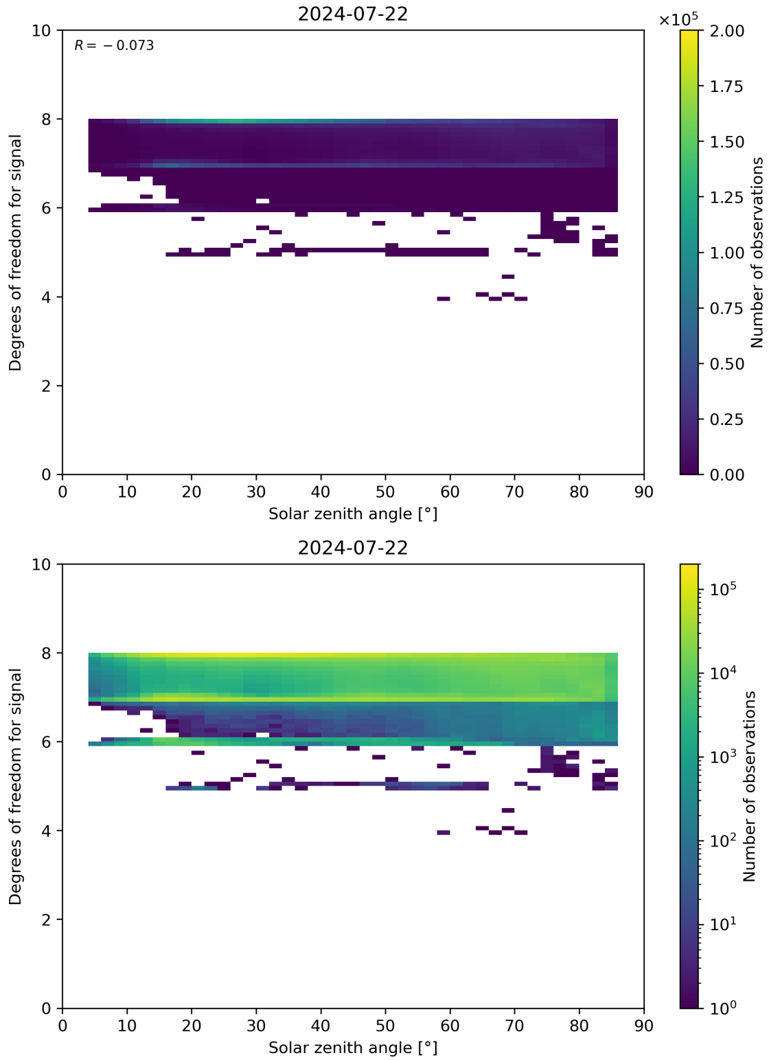
Figure 65: Scatter density plot of “Solar zenith angle” against “Degrees of freedom for signal” for 2024-07-21 to 2024-07-23.
