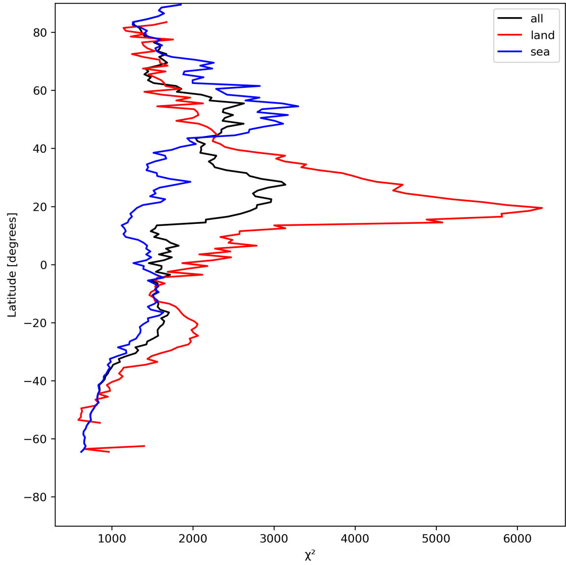
Figure 14: Zonal average of “ \chi^2 ” for 2024-07-21 to 2024-07-23.
