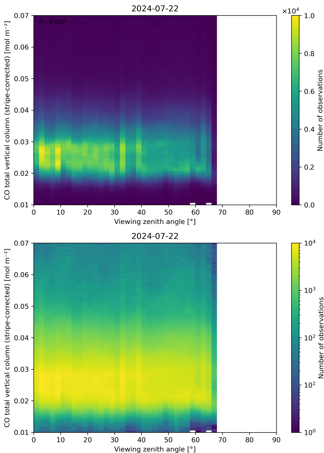
Figure 70: Scatter density plot of “Viewing zenith angle” against “CO total vertical column (stripe-corrected)” for 2024-07-21 to 2024-07-23.
