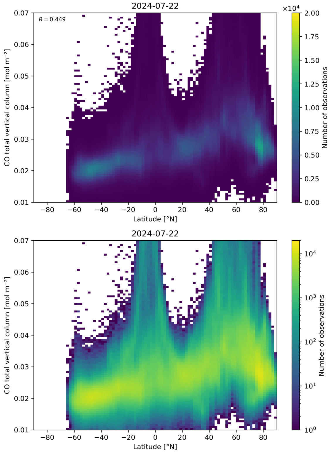
Figure 51: Scatter density plot of “Latitude” against “CO total vertical column” for 2024-07-21 to 2024-07-23.
