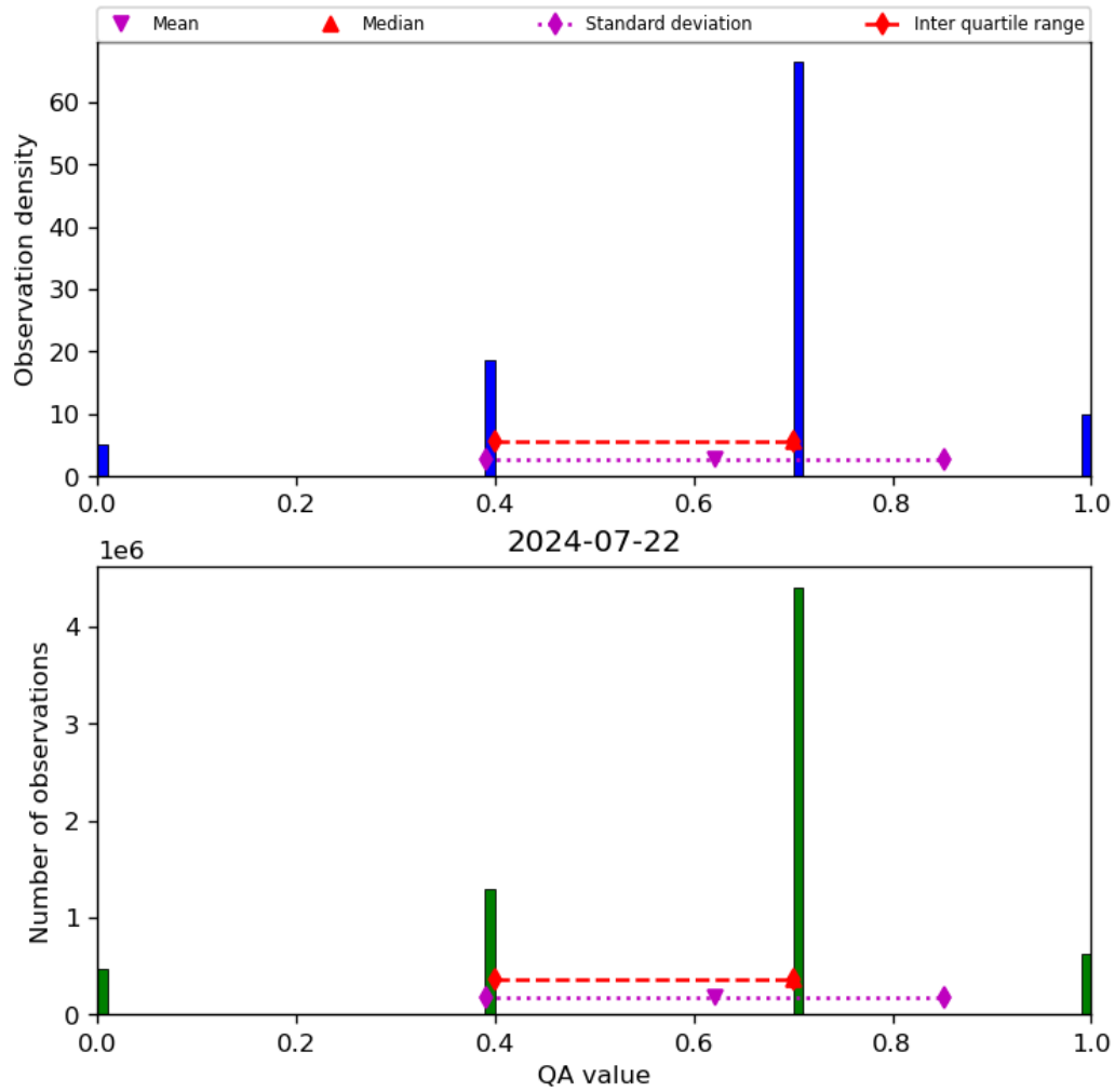
Figure 17: Histogram of “QA value” for 2024-07-21 to 2024-07-23
