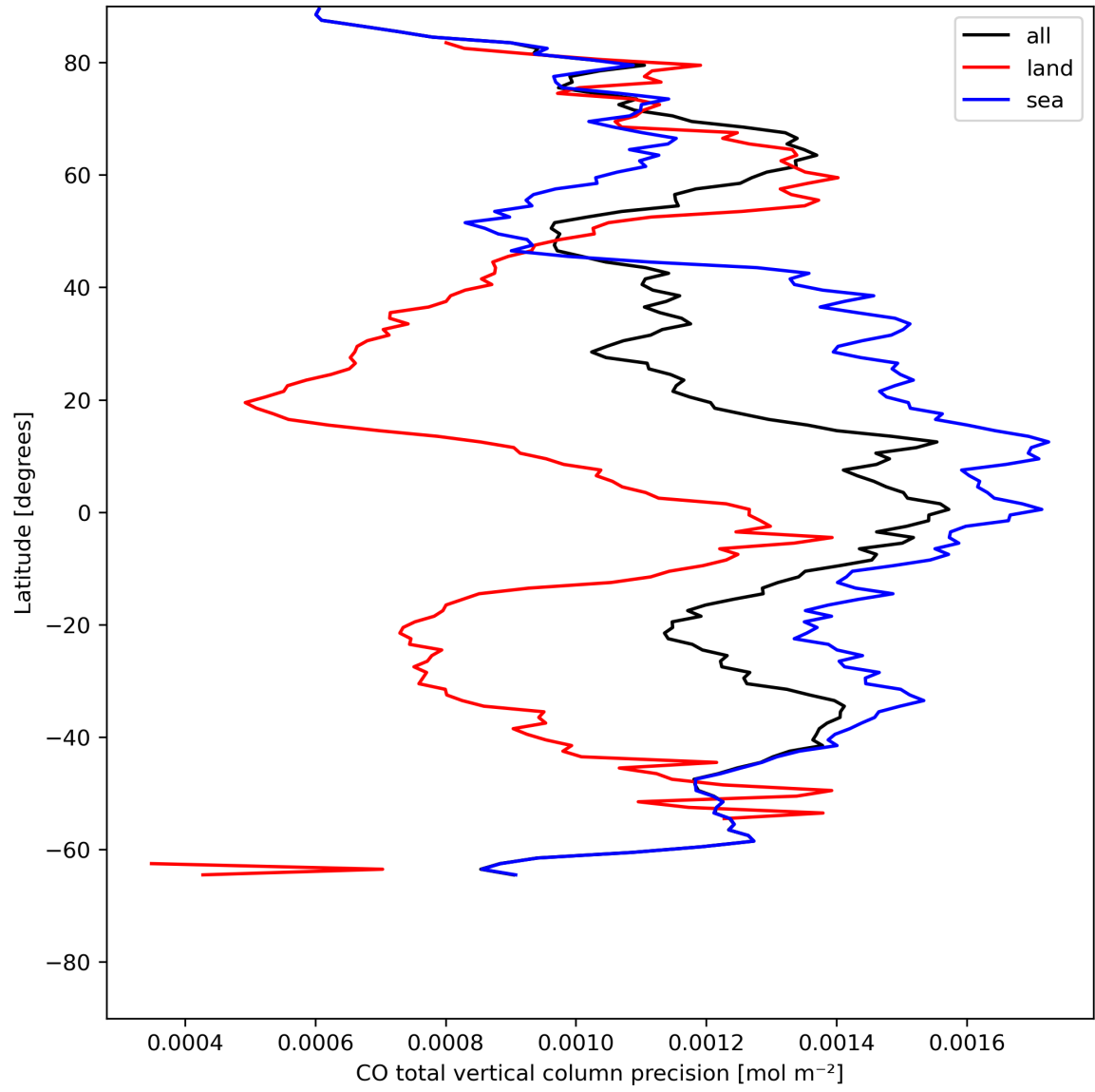
Figure 12: Zonal average of “CO total vertical column precision” for 2024-07-21 to 2024-07-23.
