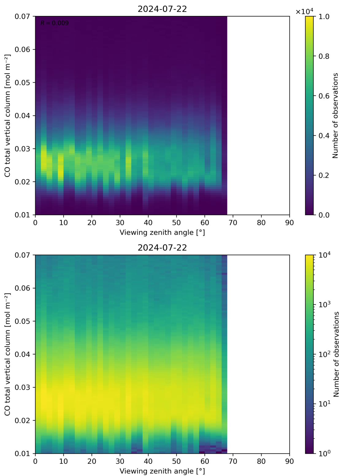
Figure 69: Scatter density plot of “Viewing zenith angle” against “CO total vertical column” for 2024-07-21 to 2024-07-23.
