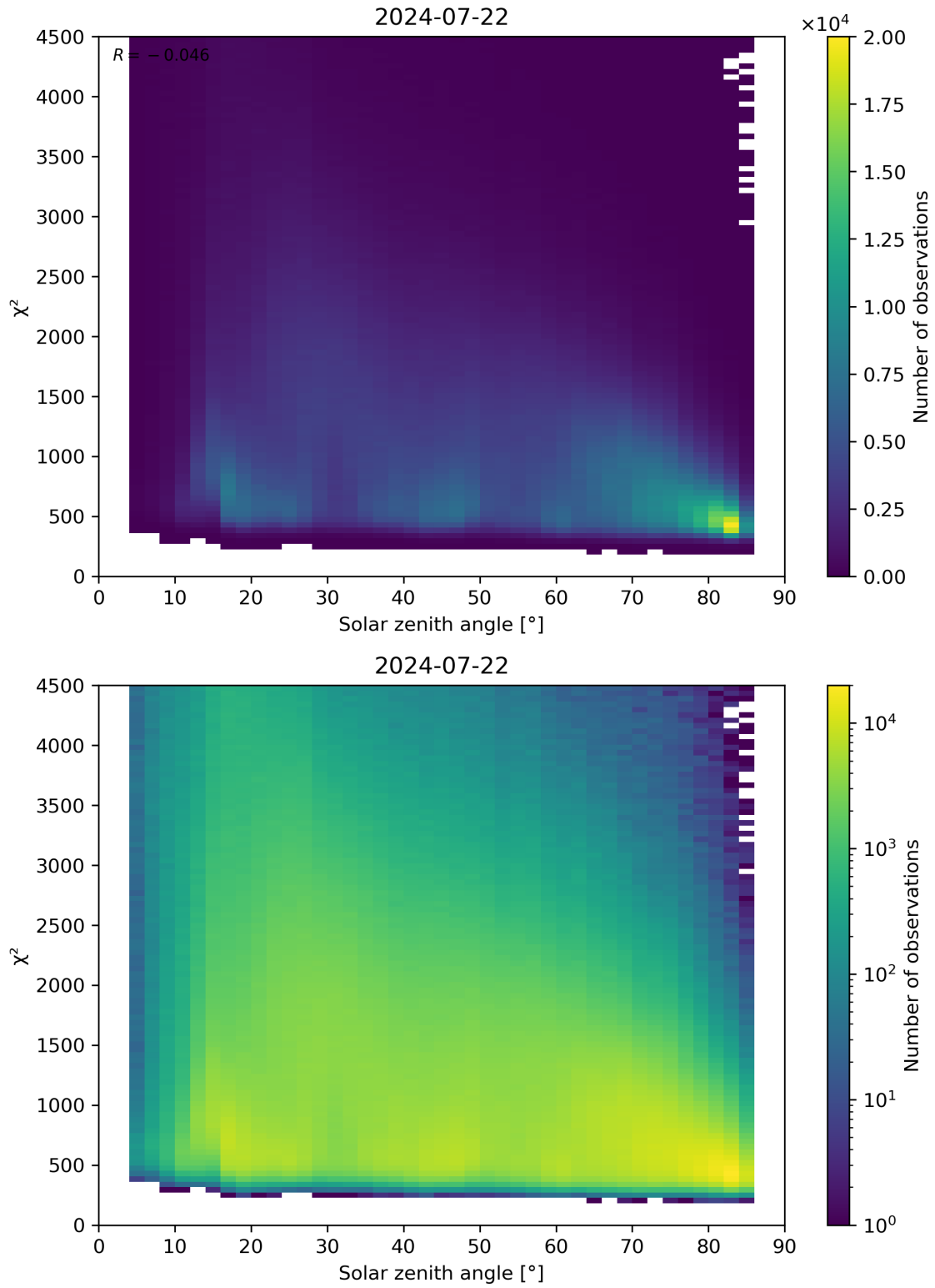
Figure 64: Scatter density plot of “Solar zenith angle” against “ \chi^2 ” for 2024-07-21 to 2024-07-23.
