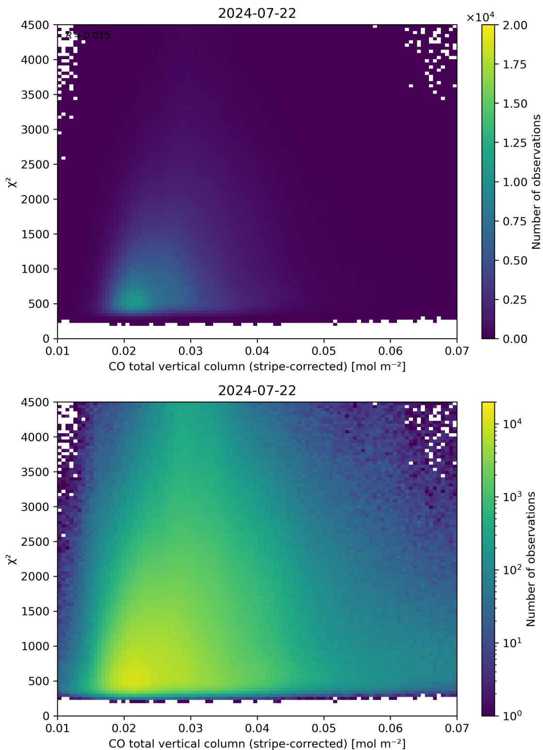
Figure 37: Scatter density plot of “CO total vertical column (stripe-corrected)” against “ \chi^2 ” for 2024-07-21 to 2024-07-23.
