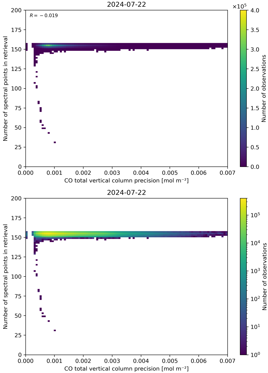
Figure 47: Scatter density plot of “CO total vertical column precision” against “Number of spectral points in retrieval” for 2024-07-21 to 2024-07-23.
