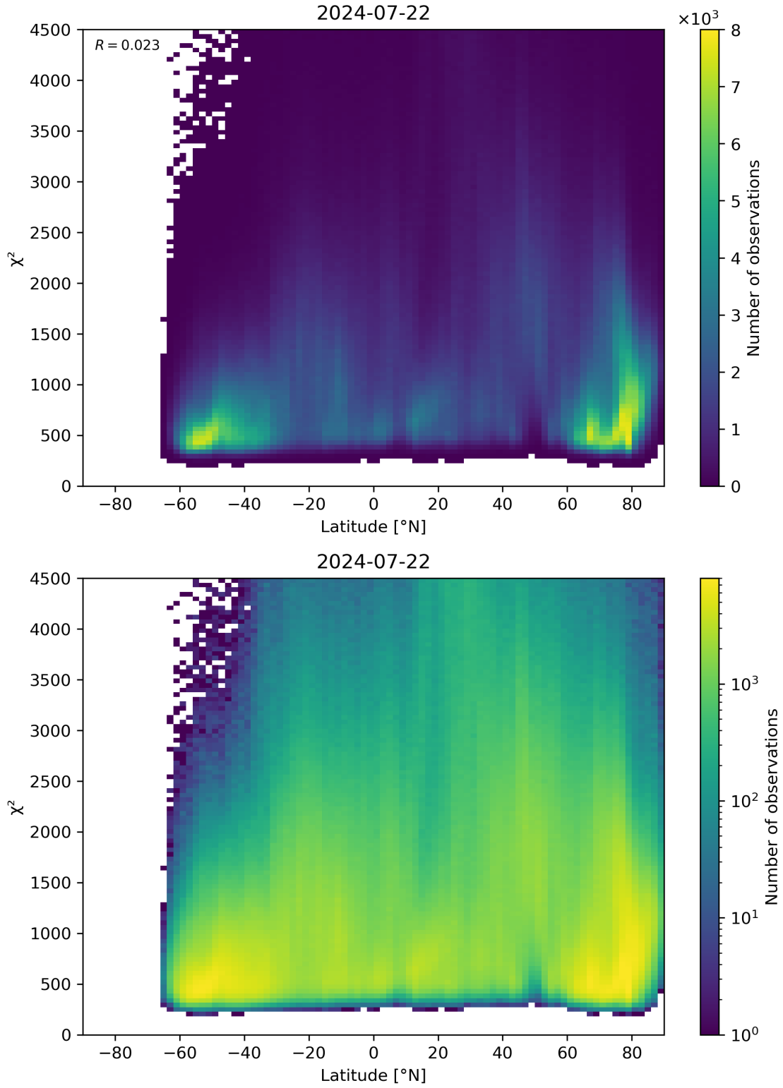
Figure 54: Scatter density plot of “Latitude” against “ \chi^2 ” for 2024-07-21 to 2024-07-23.
