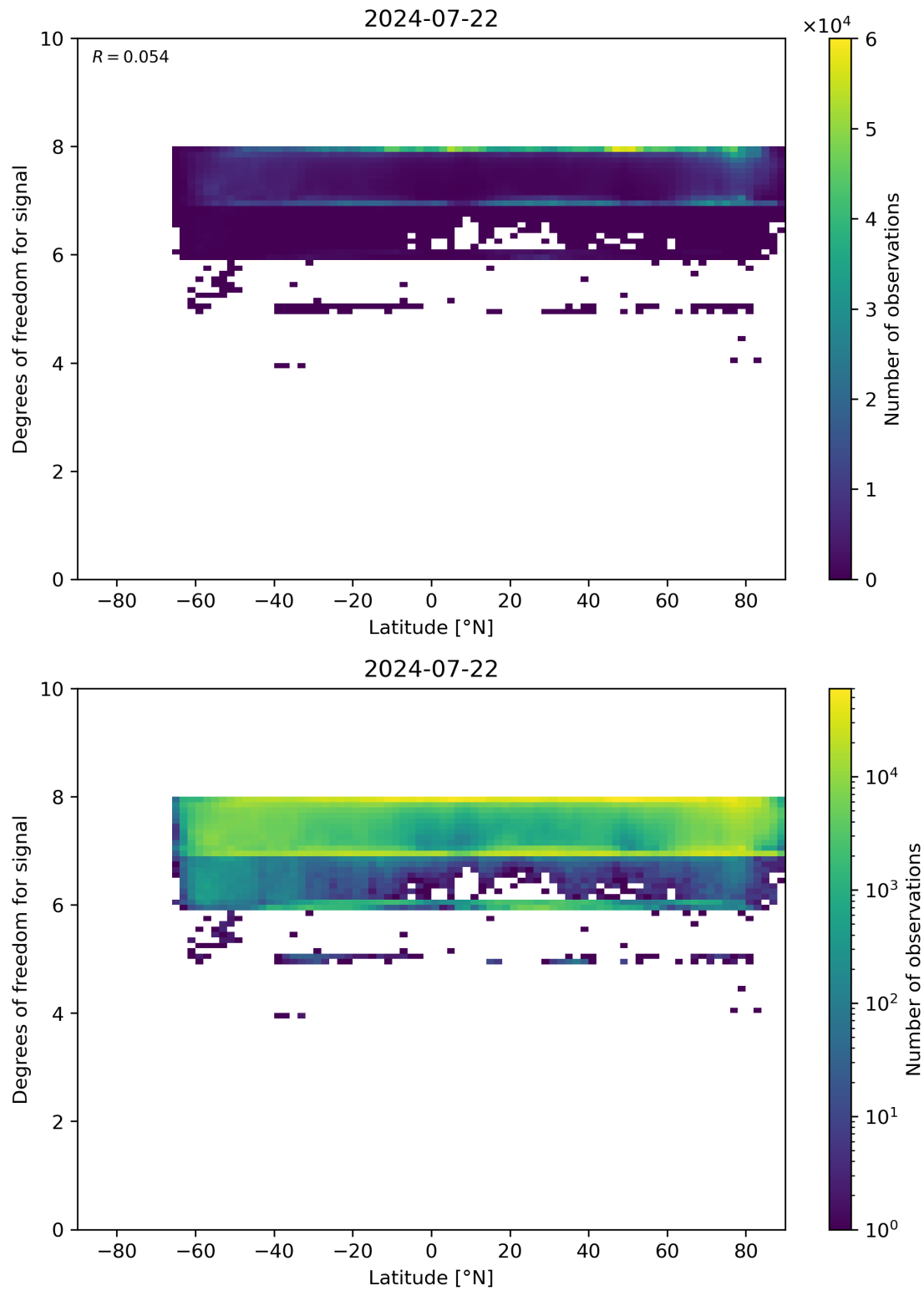
Figure 55: Scatter density plot of “Latitude” against “Degrees of freedom for signal” for 2024-07-21 to 2024-07-23.
