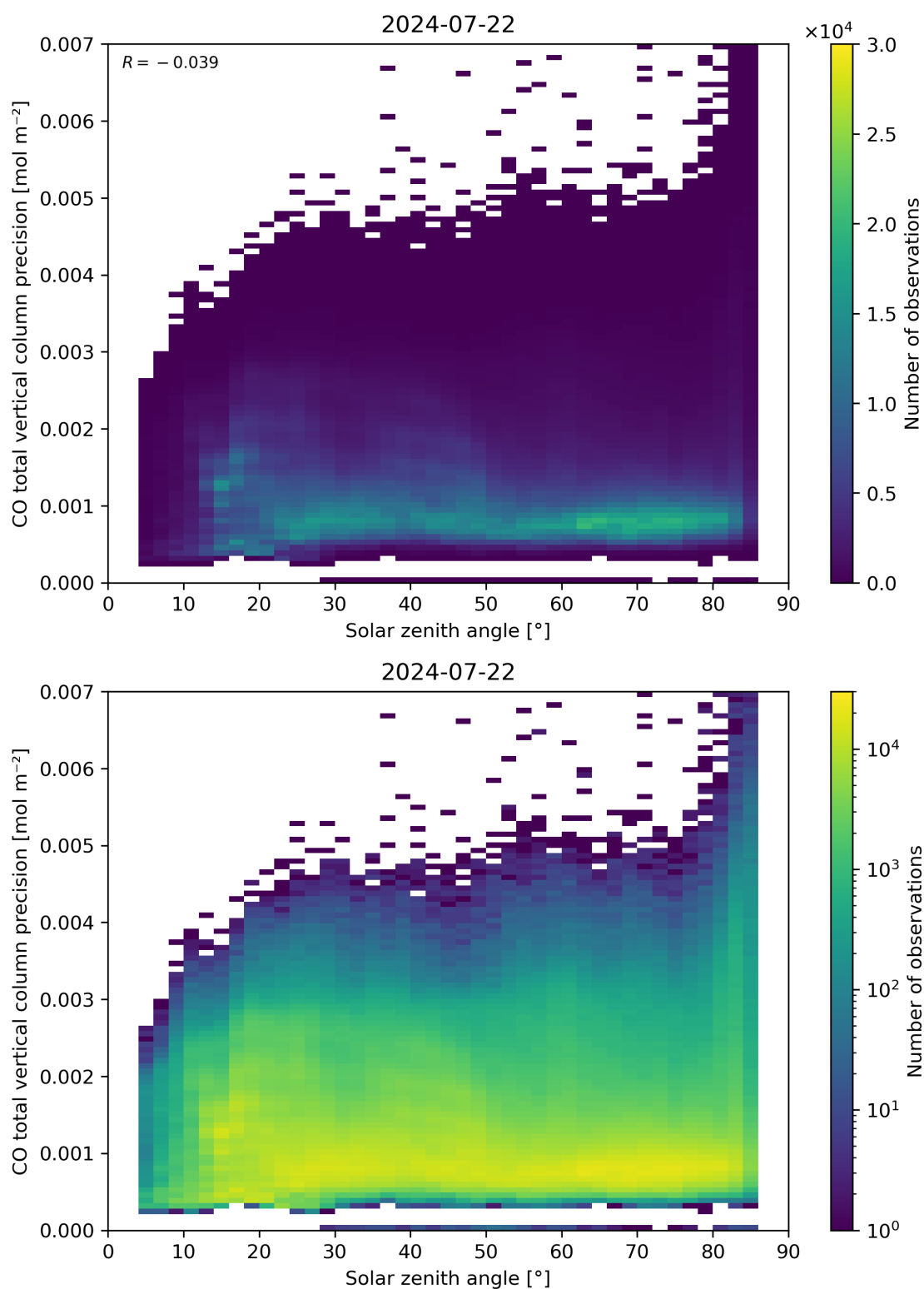
Figure 63: Scatter density plot of “Solar zenith angle” against “CO total vertical column precision” for 2024-07-21 to 2024-07-23.
