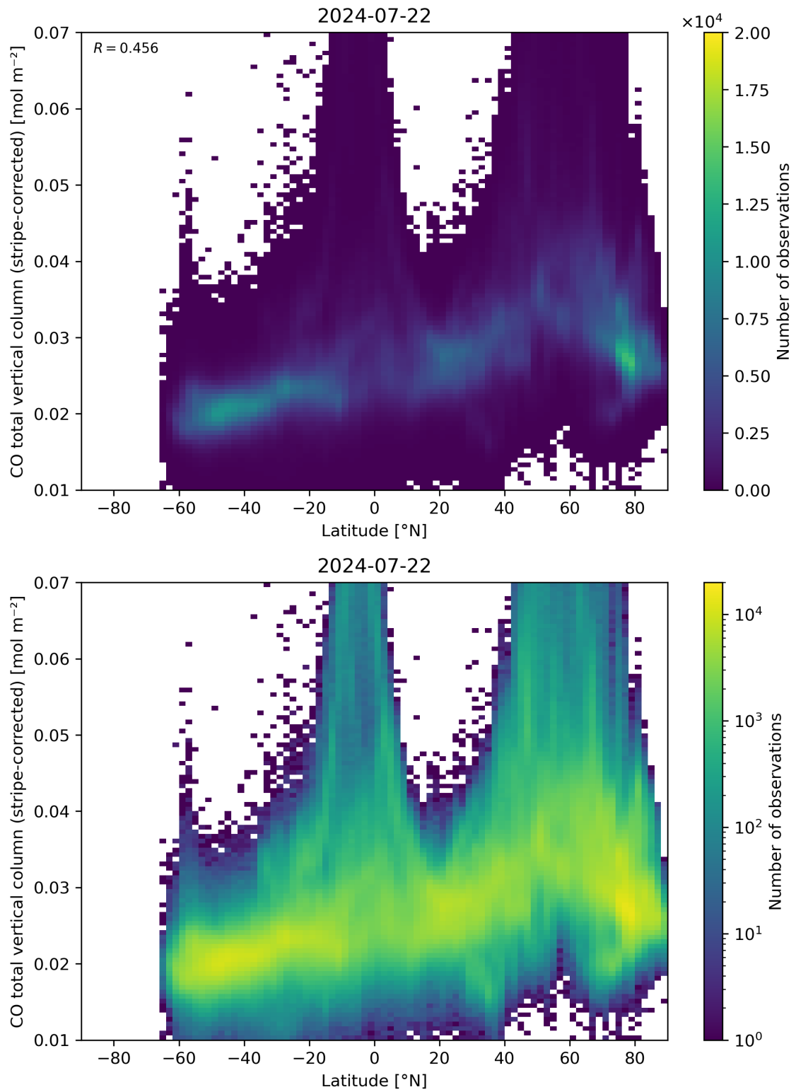
Figure 52: Scatter density plot of “Latitude” against “CO total vertical column (stripe-corrected)” for 2024-07-21 to 2024-07-23.
