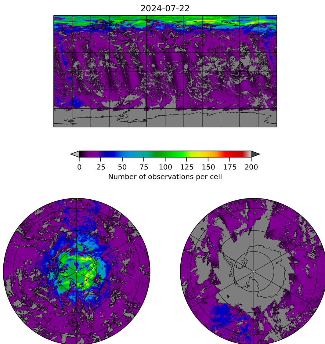
Figure 8: Map of the number of observations for 2024-07-21 to 2024-07-23
