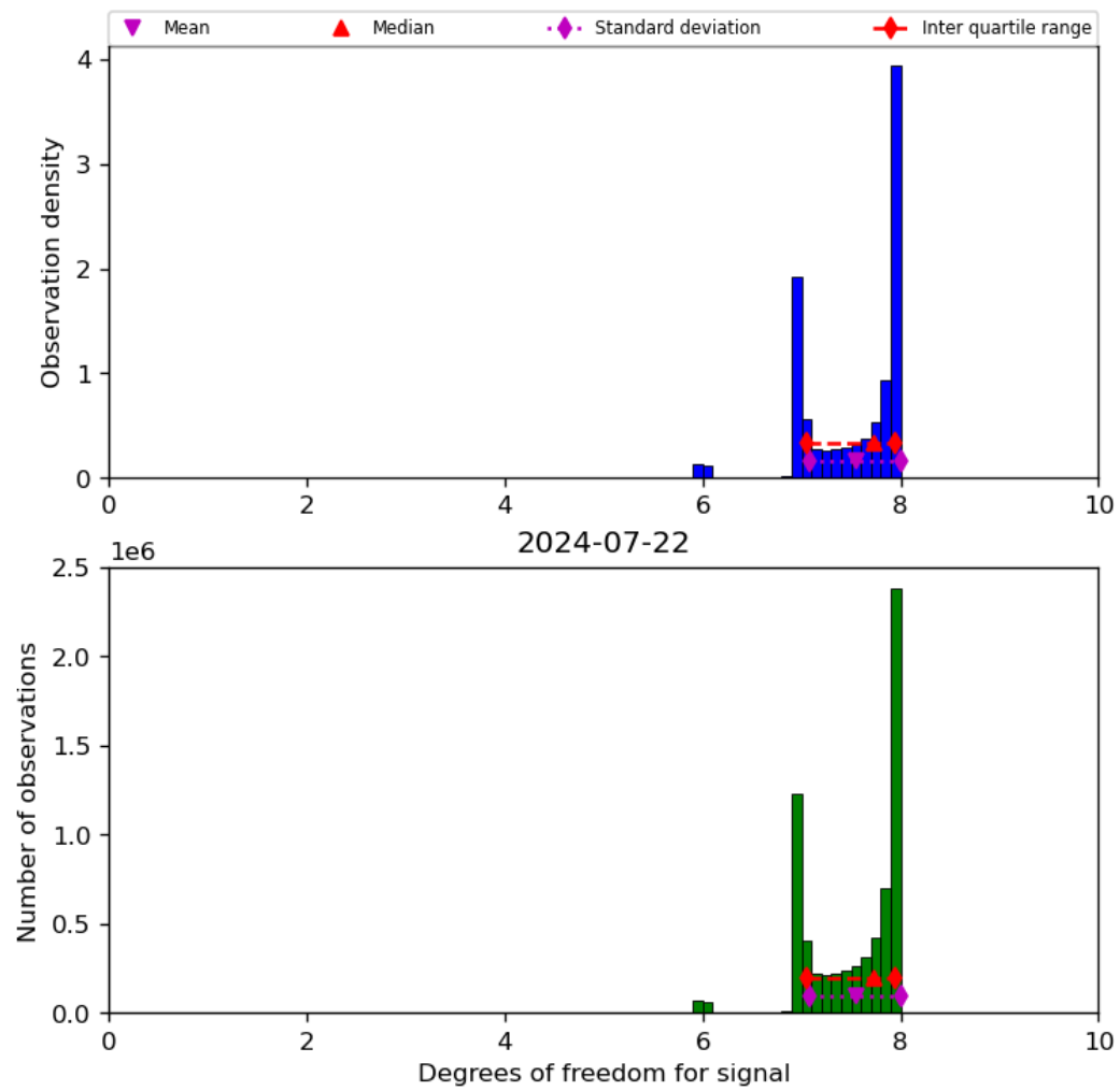
Figure 23: Histogram of “Degrees of freedom for signal” for 2024-07-21 to 2024-07-23
