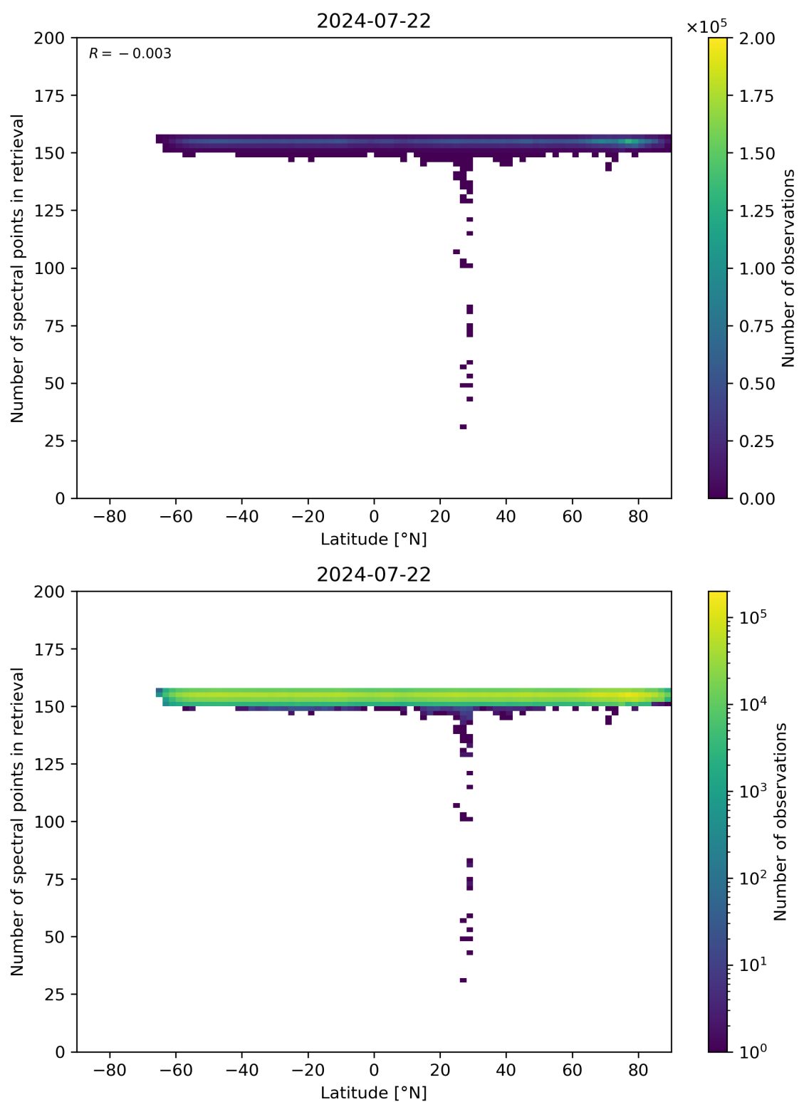
Figure 57: Scatter density plot of “Latitude” against “Number of spectral points in retrieval” for 2024-07-21 to 2024-07-23.
