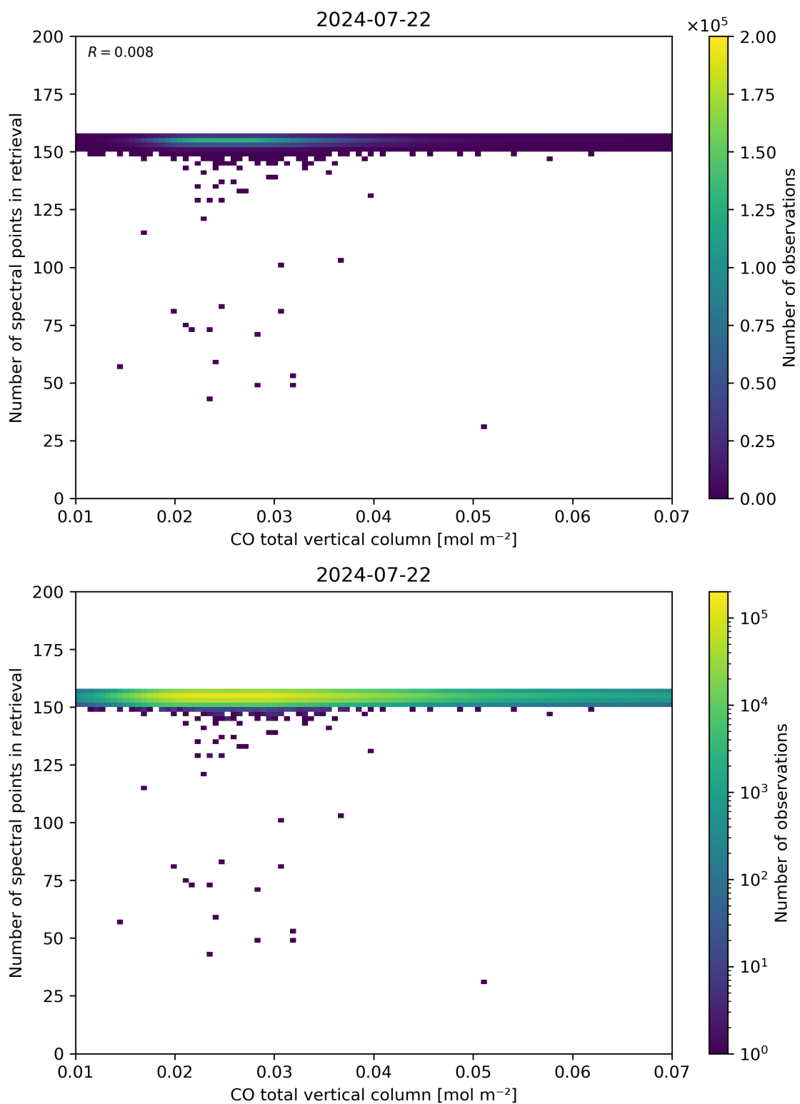
Figure 43: Scatter density plot of “CO total vertical column” against “Number of spectral points in retrieval” for 2024-07-21 to 2024-07-23.
