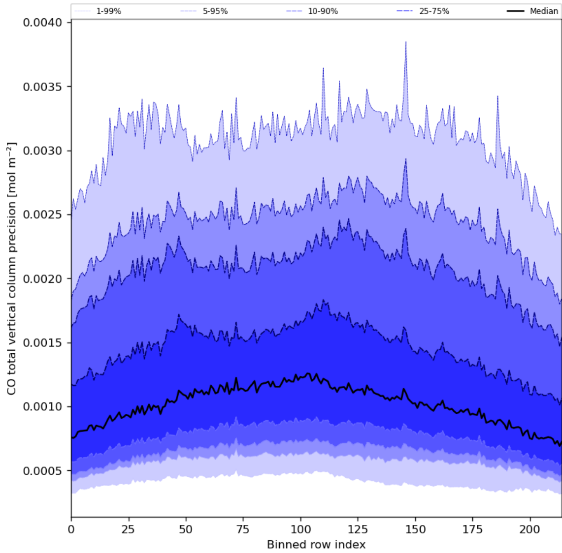
Figure 28: Along track statistics of “CO total vertical column precision” for 2024-07-21 to 2024-07-23
