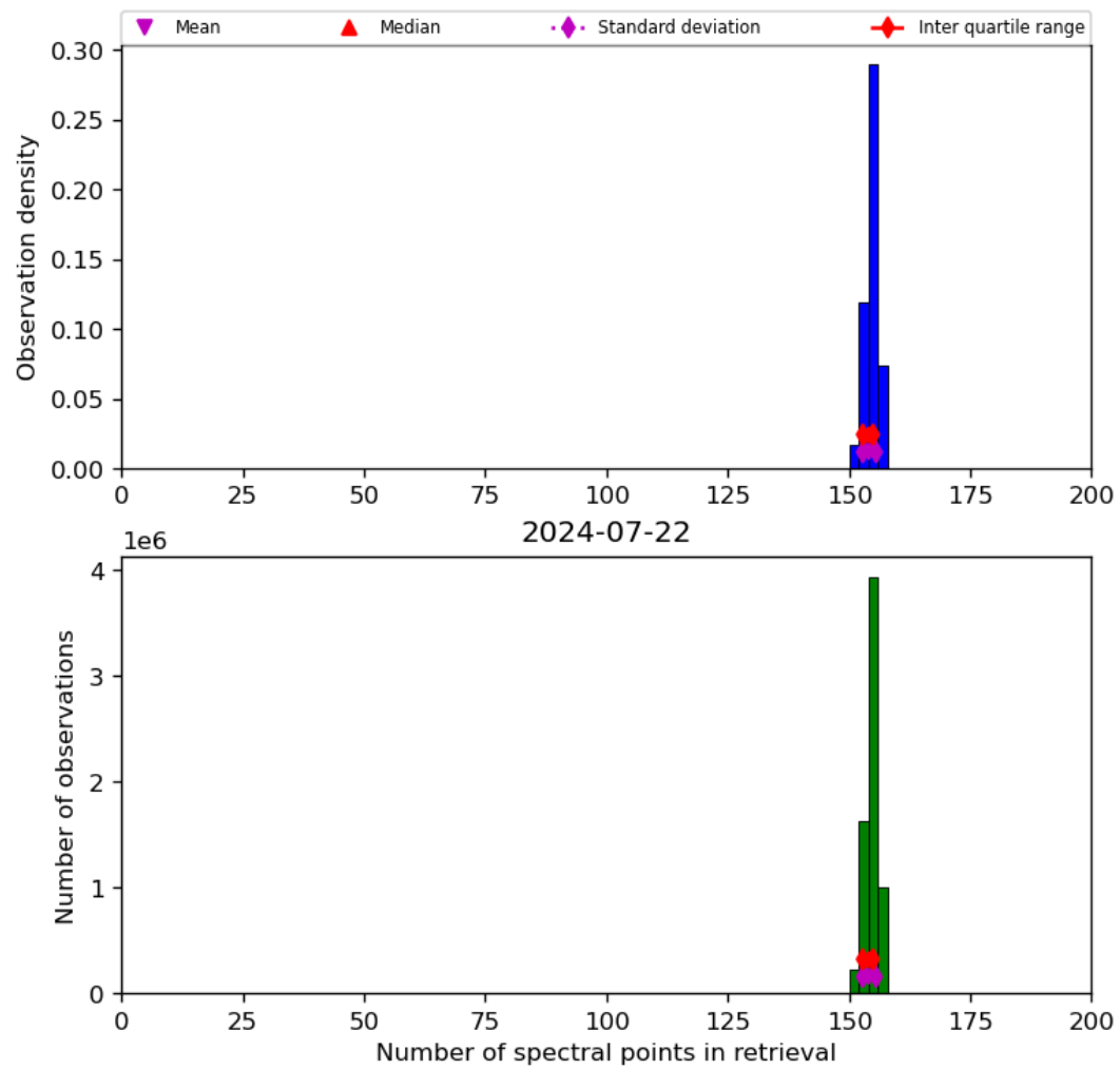
Figure 21: Histogram of “Number of spectral points in retrieval” for 2024-07-21 to 2024-07-23
