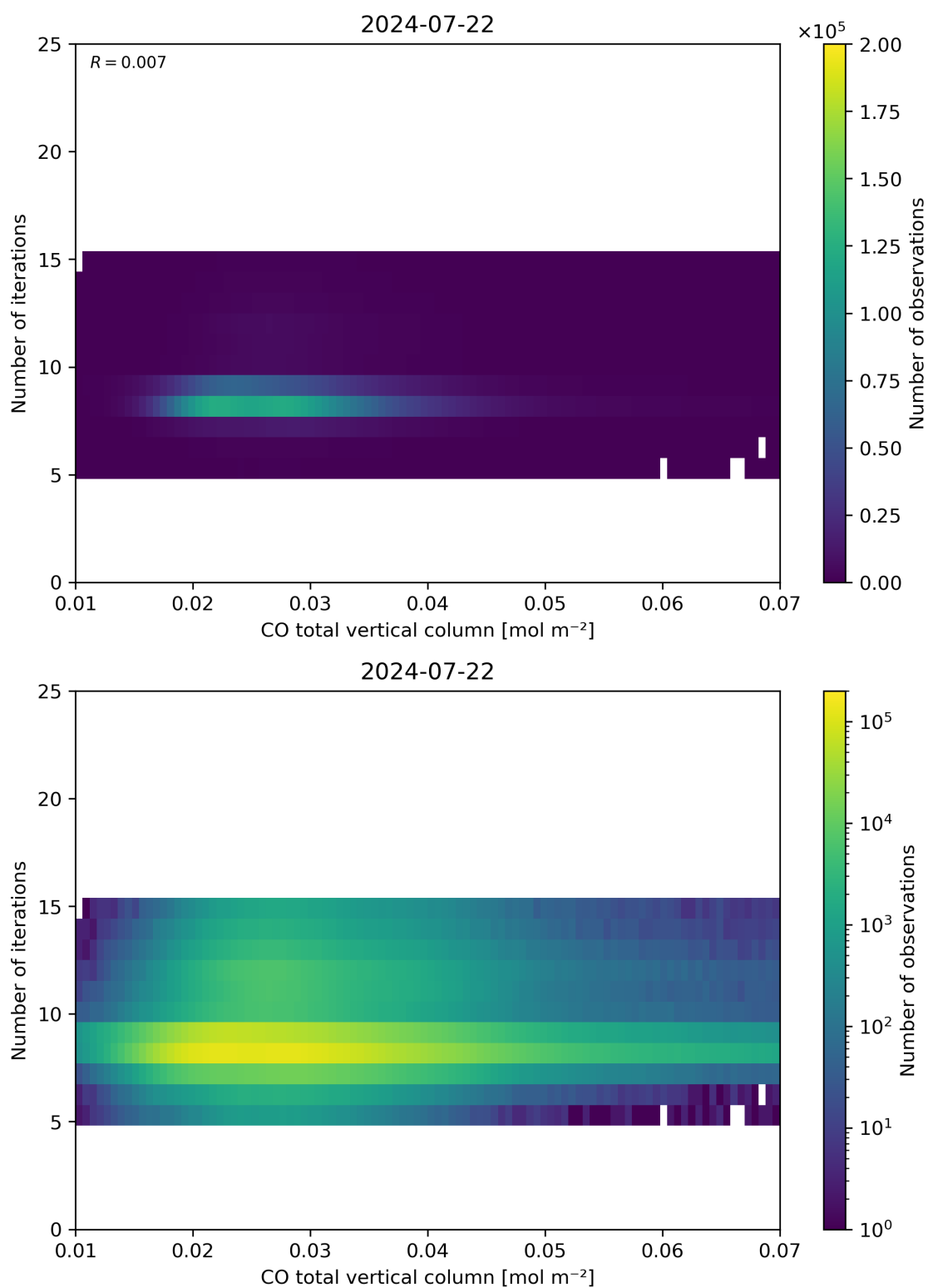
Figure 42: Scatter density plot of “CO total vertical column” against “Number of iterations” for 2024-07-21 to 2024-07-23.
