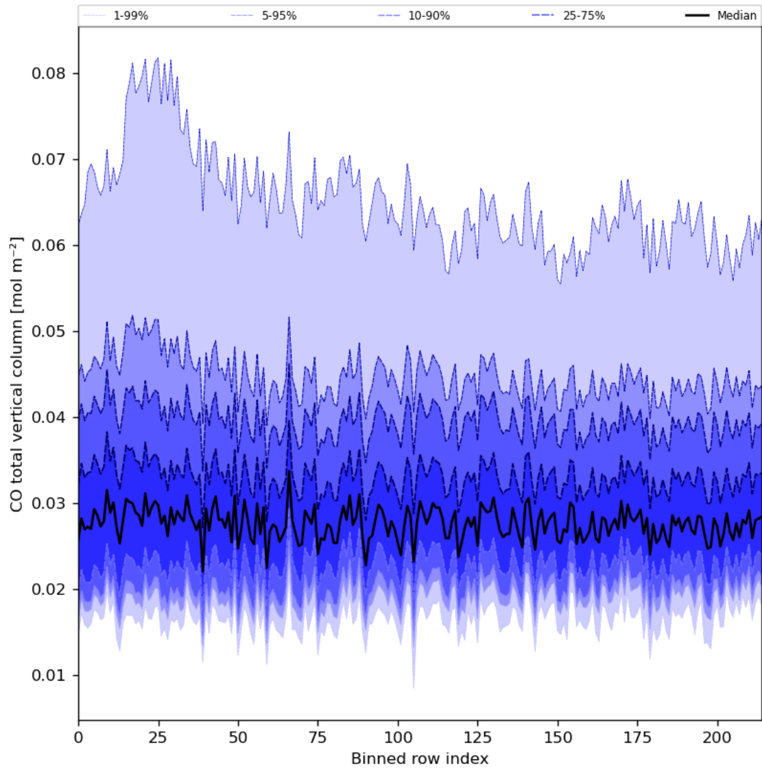
Figure 26: Along track statistics of “CO total vertical column” for 2024-07-21 to 2024-07-23
