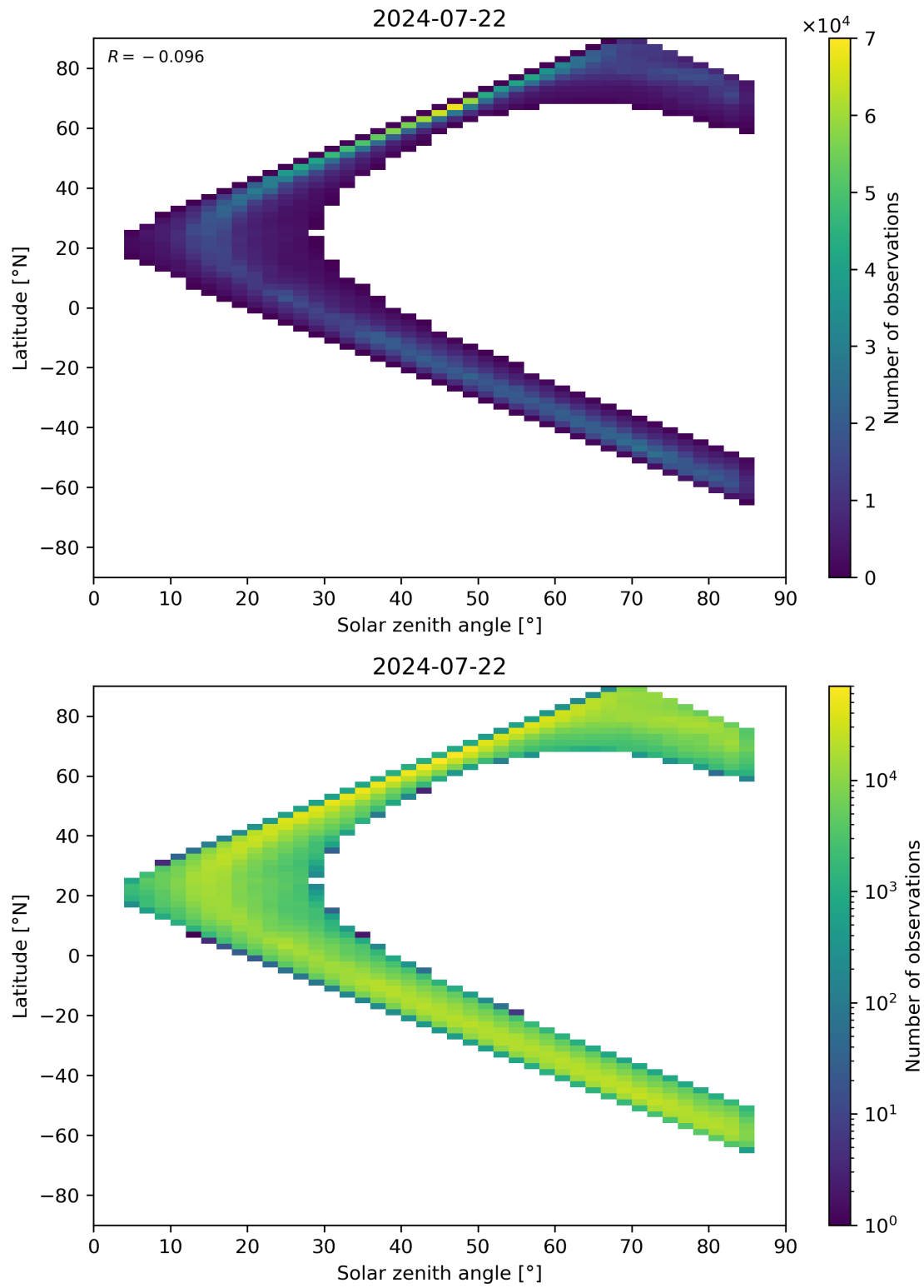
Figure 66: Scatter density plot of “Solar zenith angle” against “Latitude” for 2024-07-21 to 2024-07-23.
