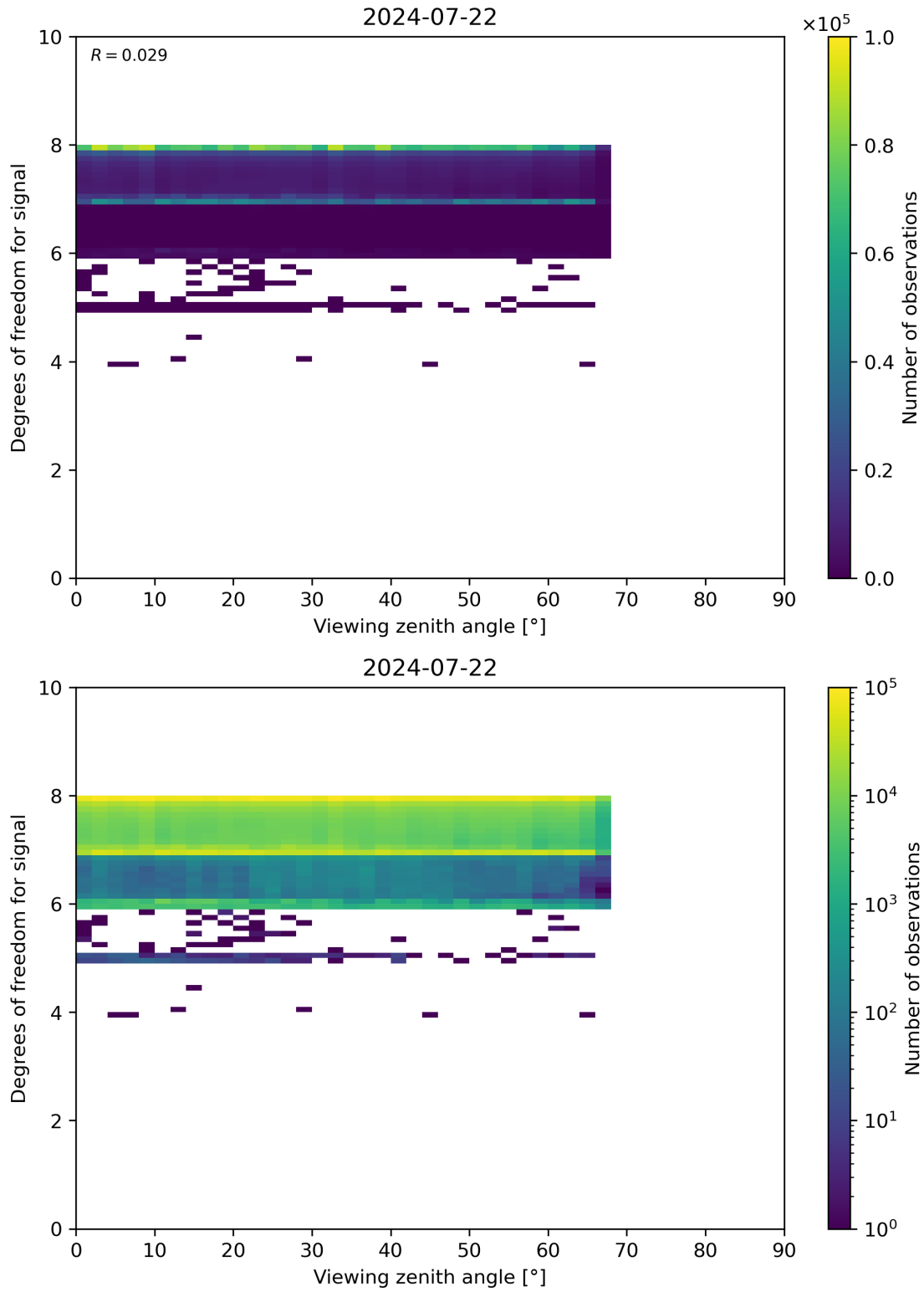
Figure 73: Scatter density plot of “Viewing zenith angle” against “Degrees of freedom for signal” for 2024-07-21 to 2024-07-23.
