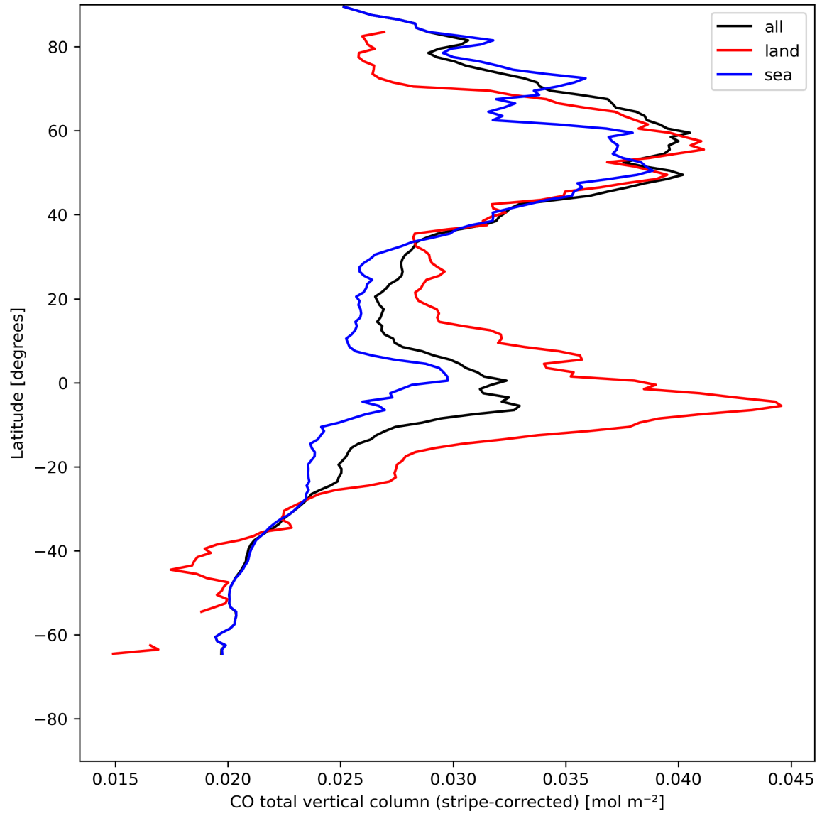
Figure 11: Zonal average of “CO total vertical column (stripe-corrected)” for 2024-07-21 to 2024-07-23.
