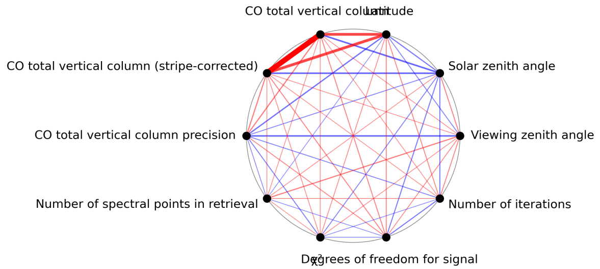
Figure 1: Map of correlation graph for 2024-07-21 to 2024-07-23.
