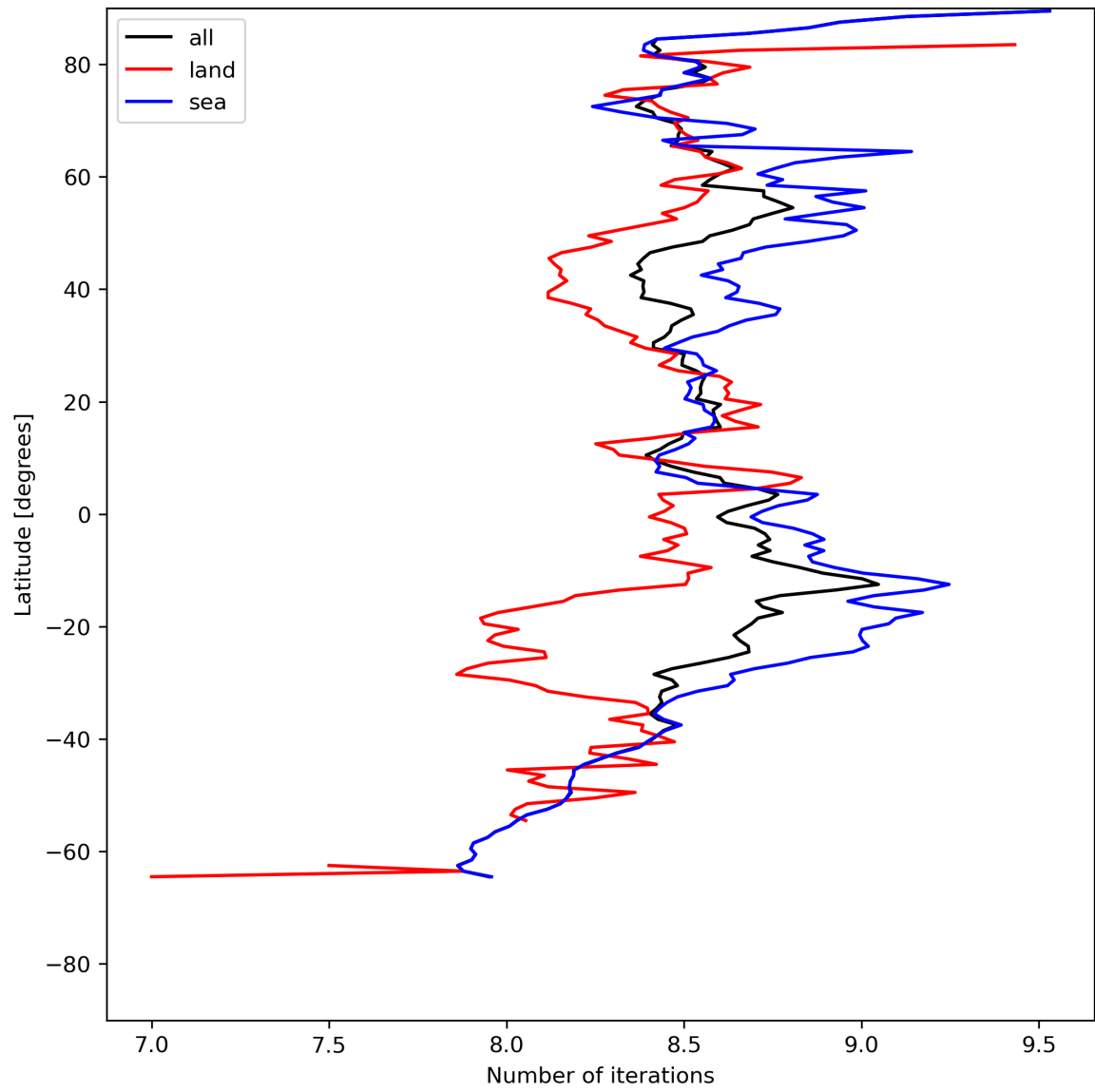
Figure 16: Zonal average of “Number of iterations” for 2024-07-21 to 2024-07-23.
