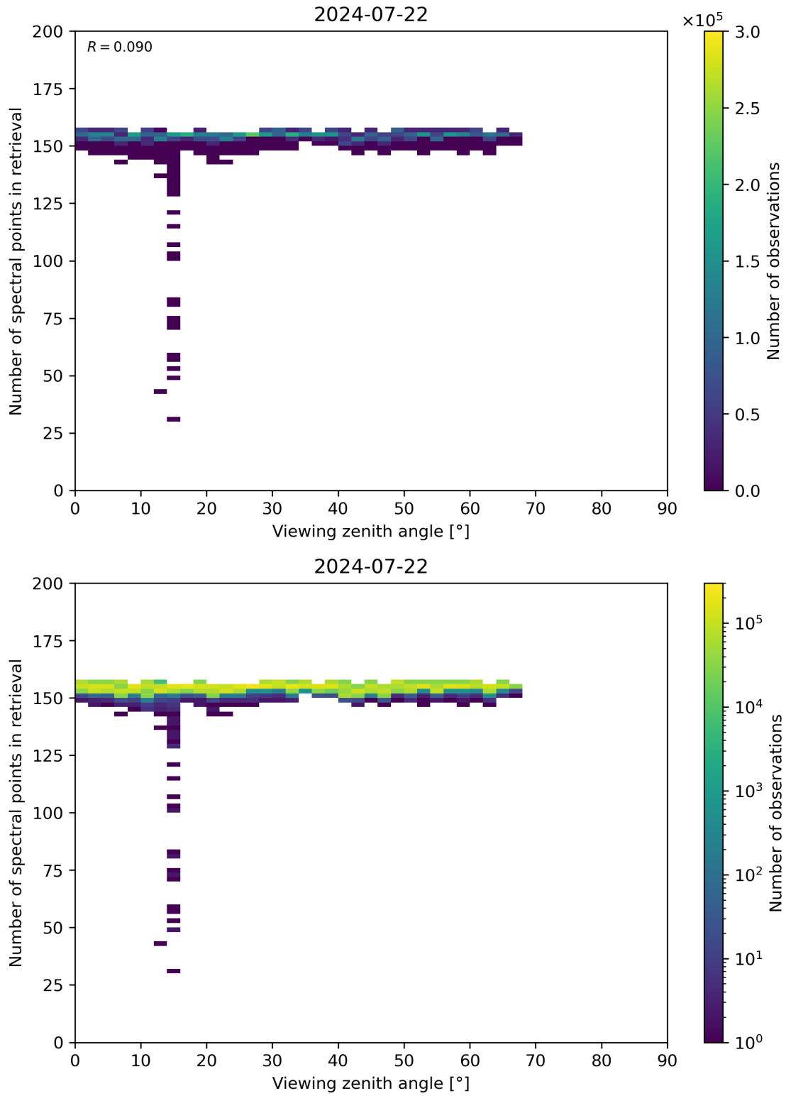
Figure 76: Scatter density plot of “Viewing zenith angle” against “Number of spectral points in retrieval” for 2024-07-21 to 2024-07-23.
