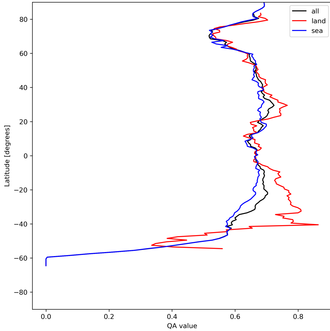
Figure 9: Zonal average of “QA value” for 2024-07-21 to 2024-07-23.
