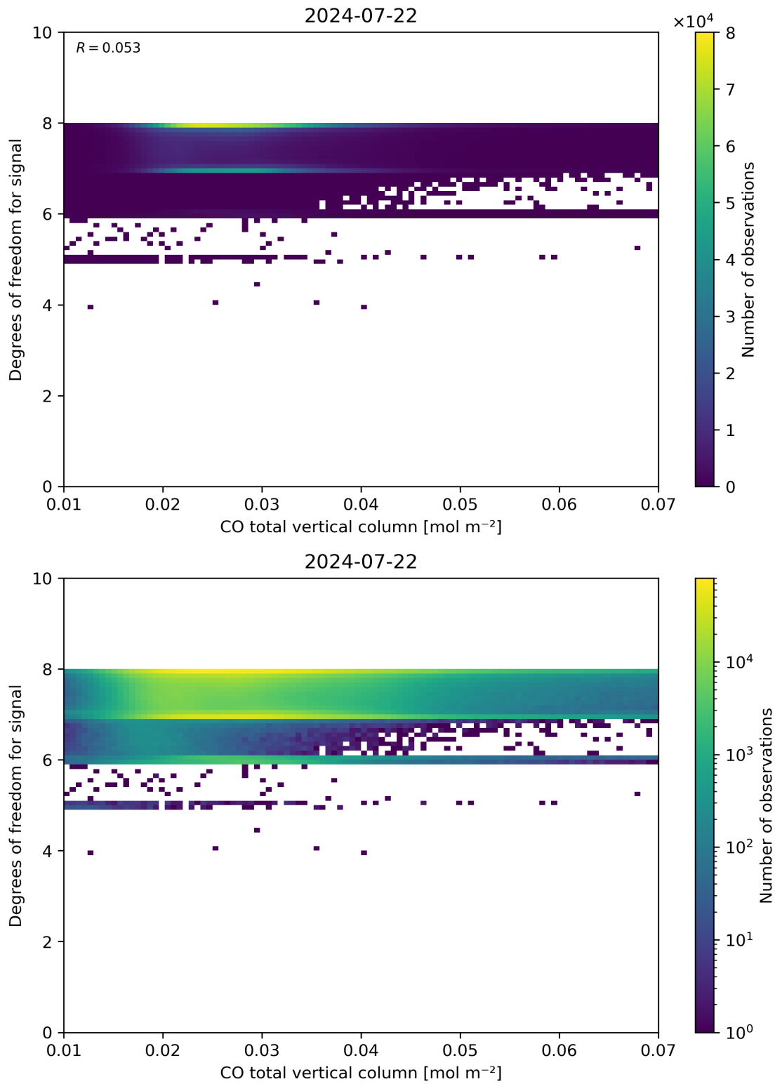
Figure 41: Scatter density plot of “CO total vertical column” against “Degrees of freedom for signal” for 2024-07-21 to 2024-07-23.
