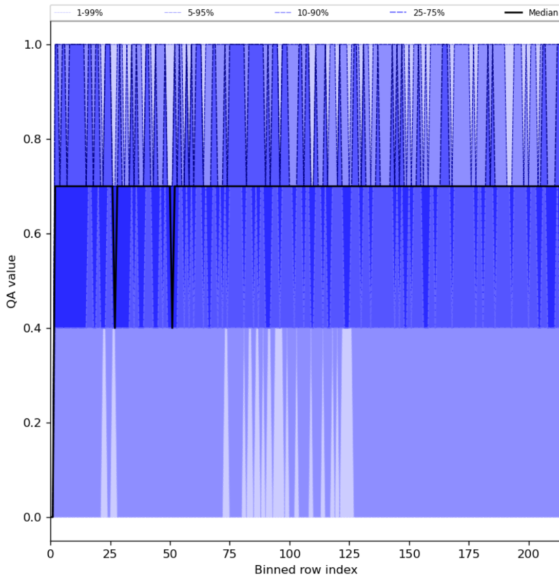
Figure 25: Along track statistics of “QA value” for 2024-07-21 to 2024-07-23
