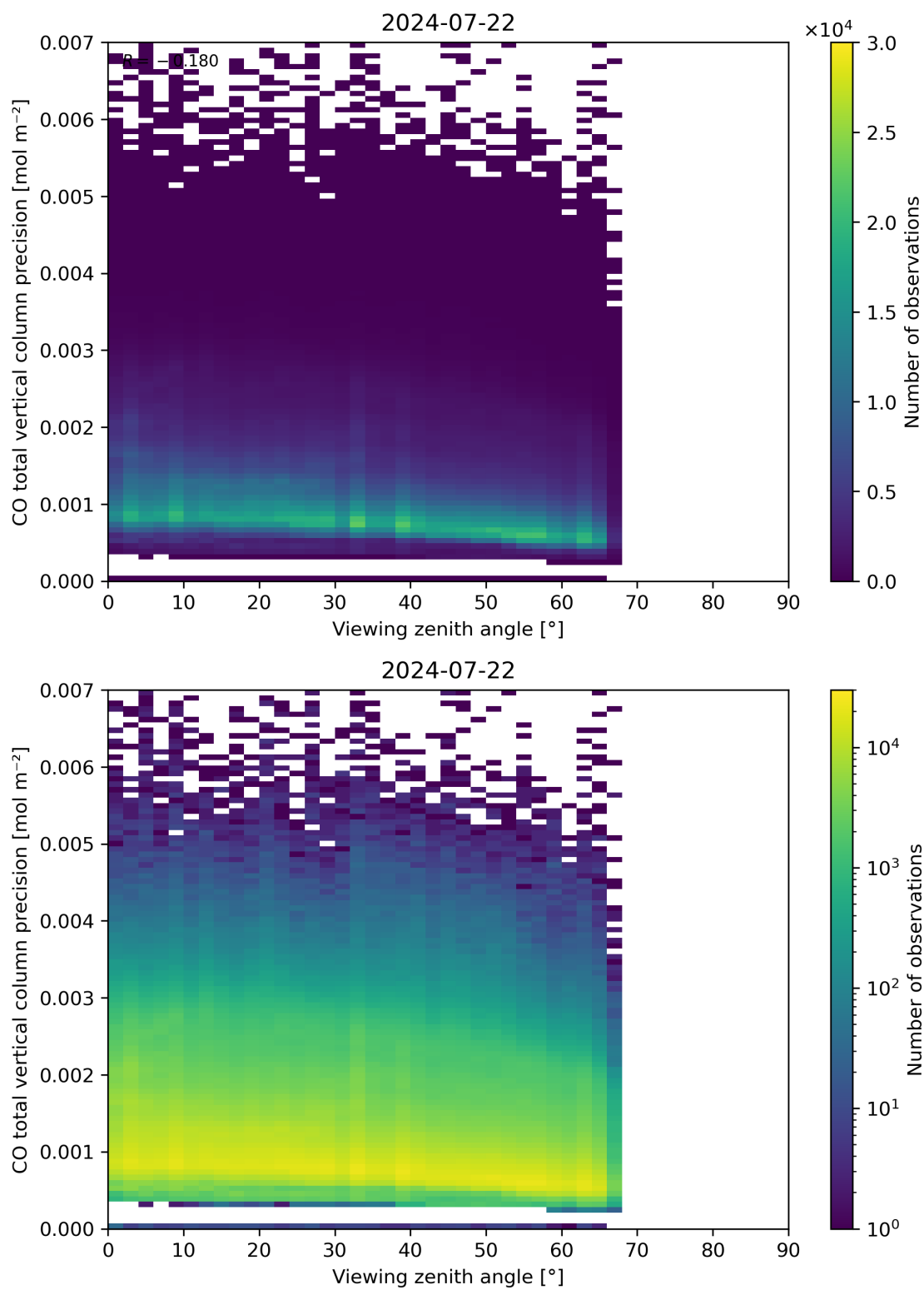
Figure 71: Scatter density plot of “Viewing zenith angle” against “CO total vertical column precision” for 2024-07-21 to 2024-07-23.
