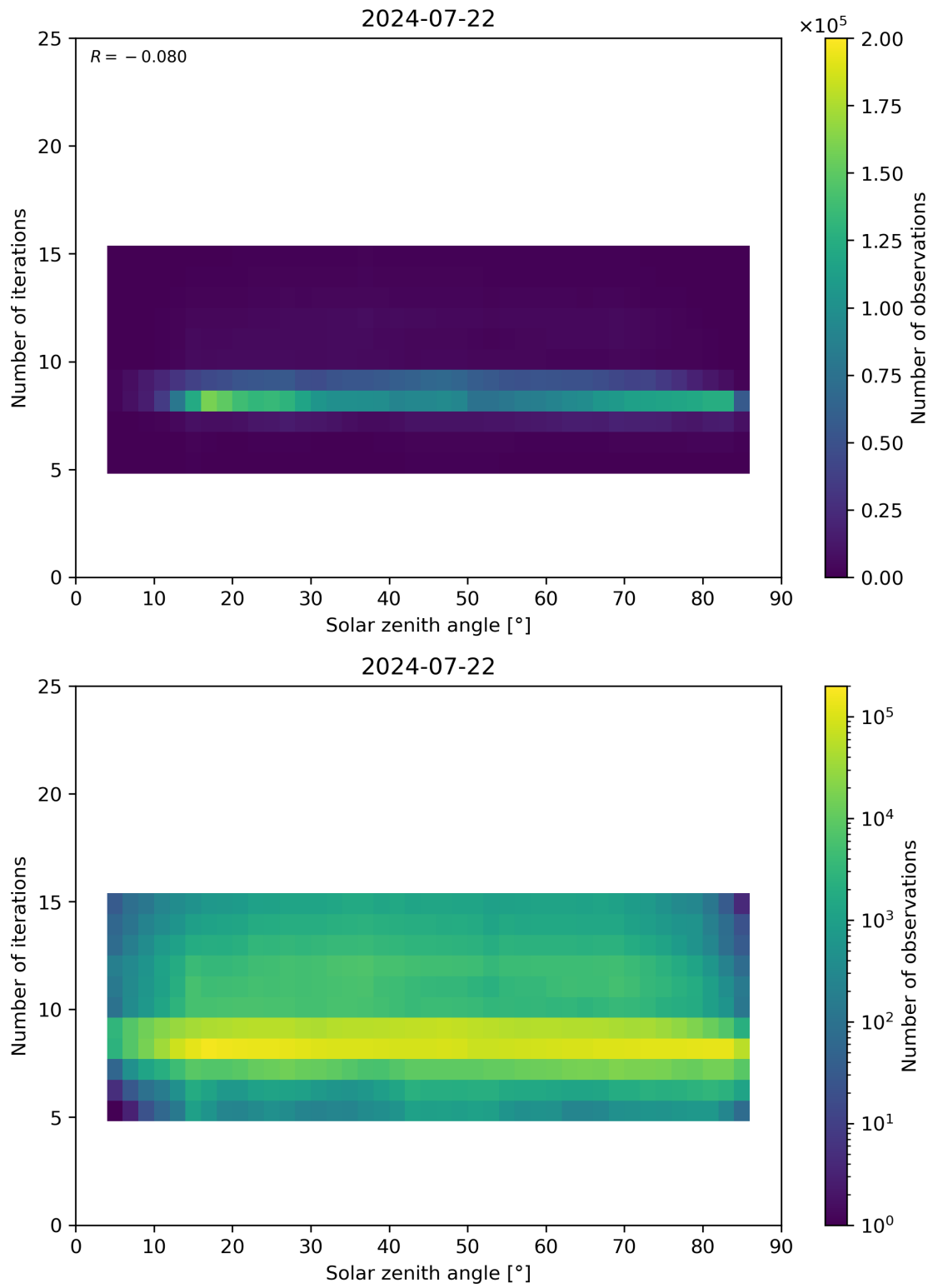
Figure 67: Scatter density plot of “Solar zenith angle” against “Number of iterations” for 2024-07-21 to 2024-07-23.
