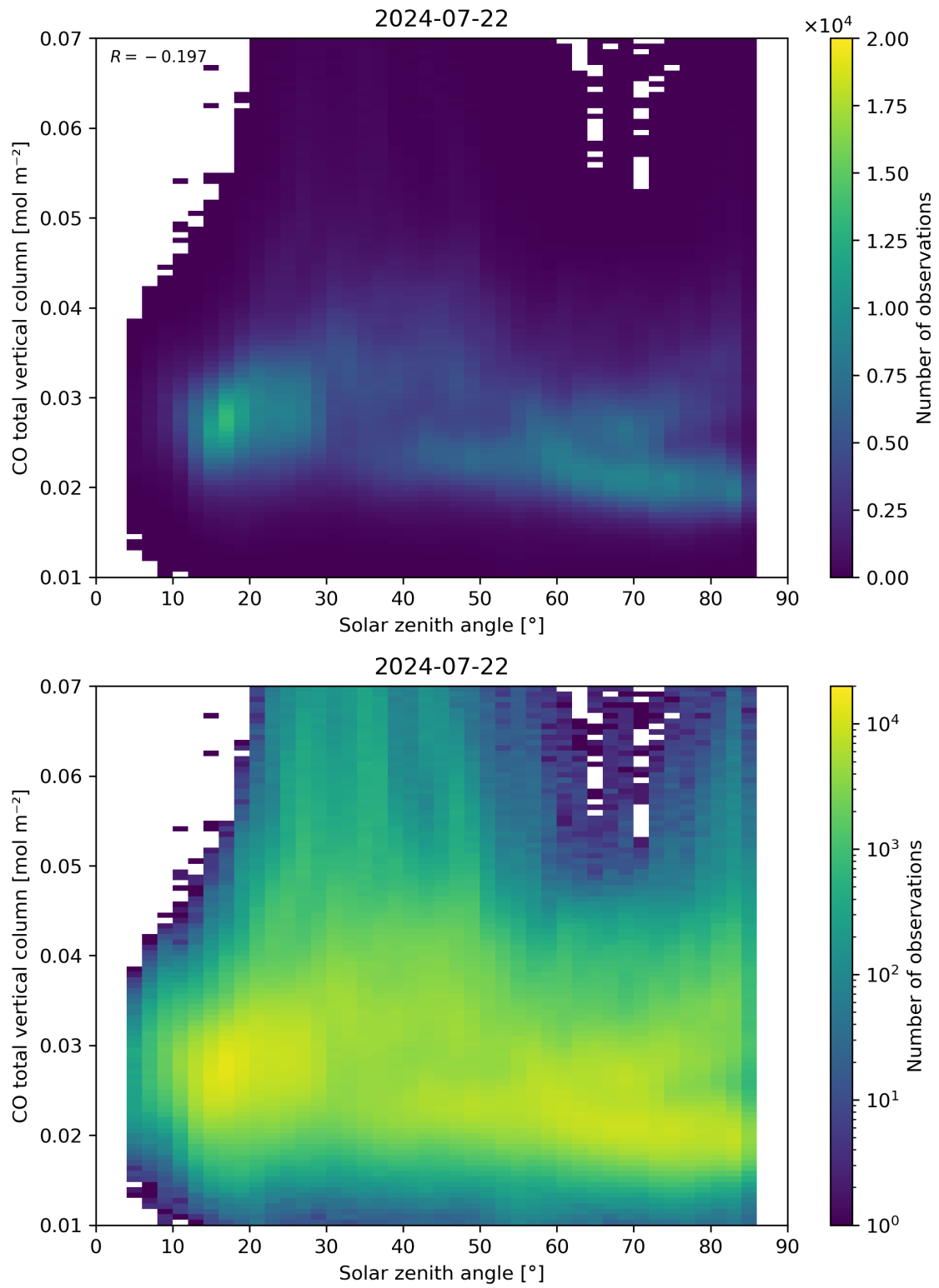
Figure 61: Scatter density plot of “Solar zenith angle” against “CO total vertical column” for 2024-07-21 to 2024-07-23.
