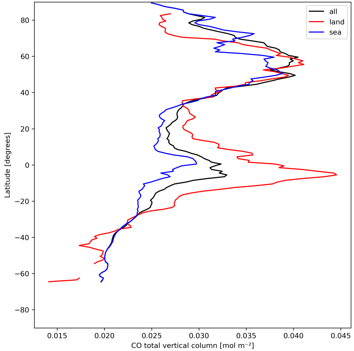
Figure 10: Zonal average of “CO total vertical column” for 2024-07-21 to 2024-07-23.
