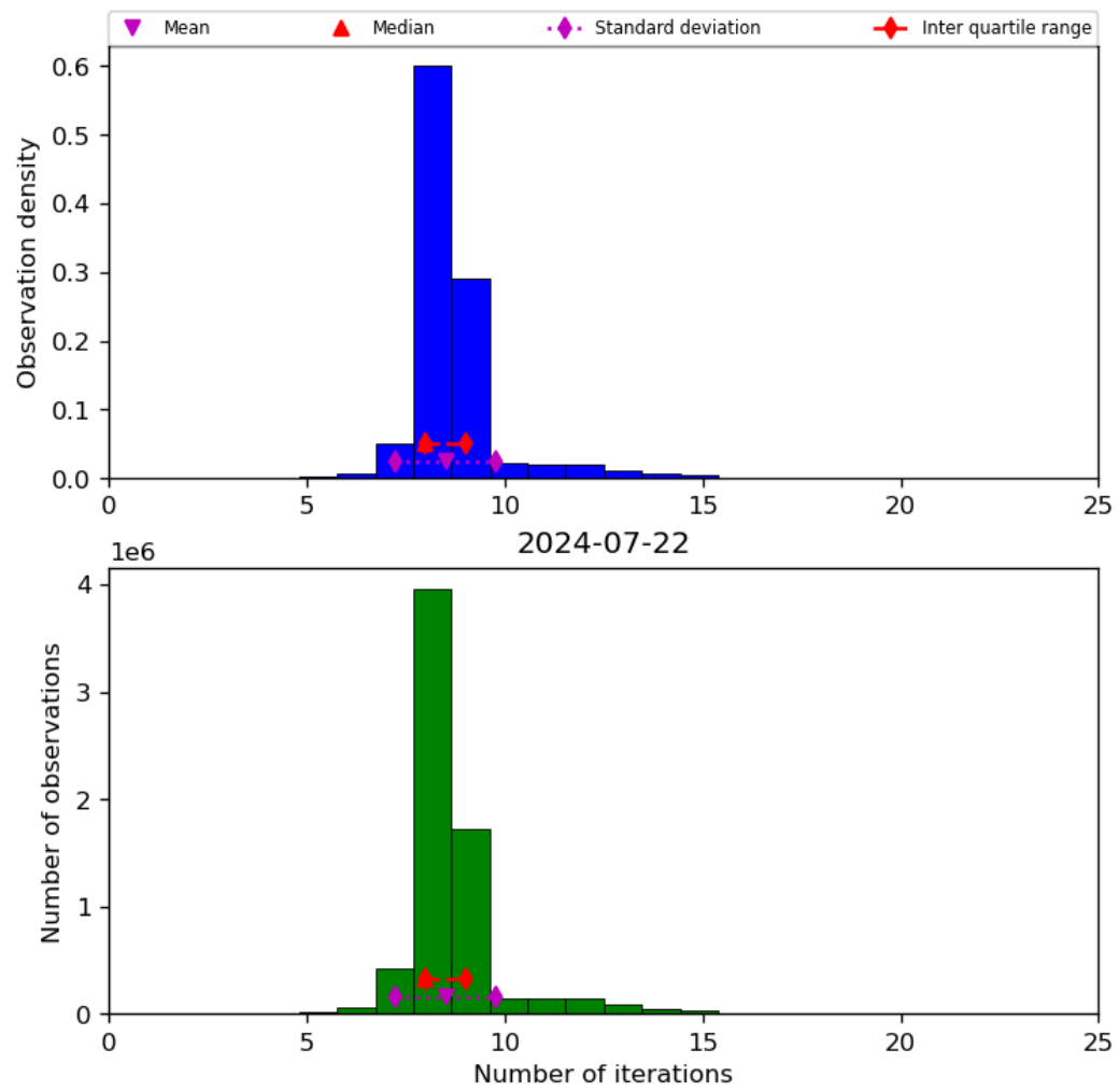
Figure 24: Histogram of “Number of iterations” for 2024-07-21 to 2024-07-23
