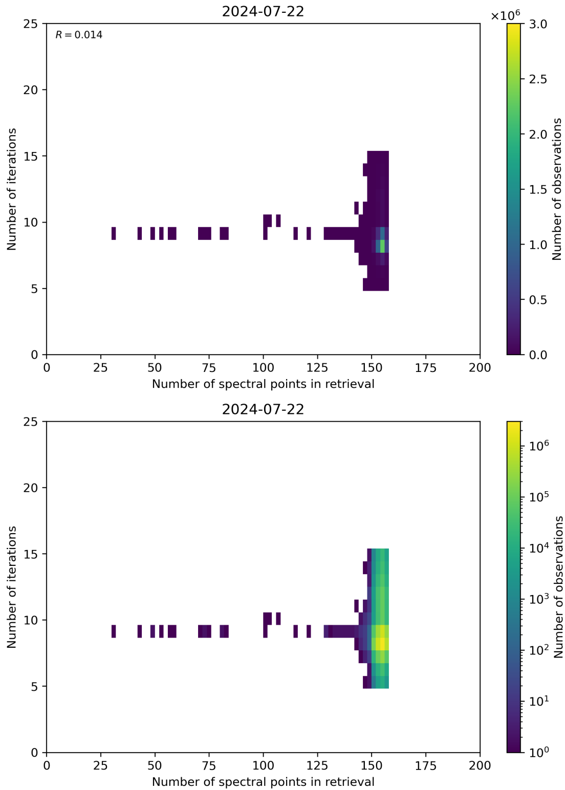
Figure 60: Scatter density plot of “Number of spectral points in retrieval” against “Number of iterations” for 2024-07-21 to 2024-07-23.
