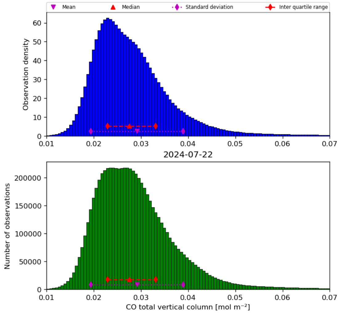
Figure 18: Histogram of “CO total vertical column” for 2024-07-21 to 2024-07-23
