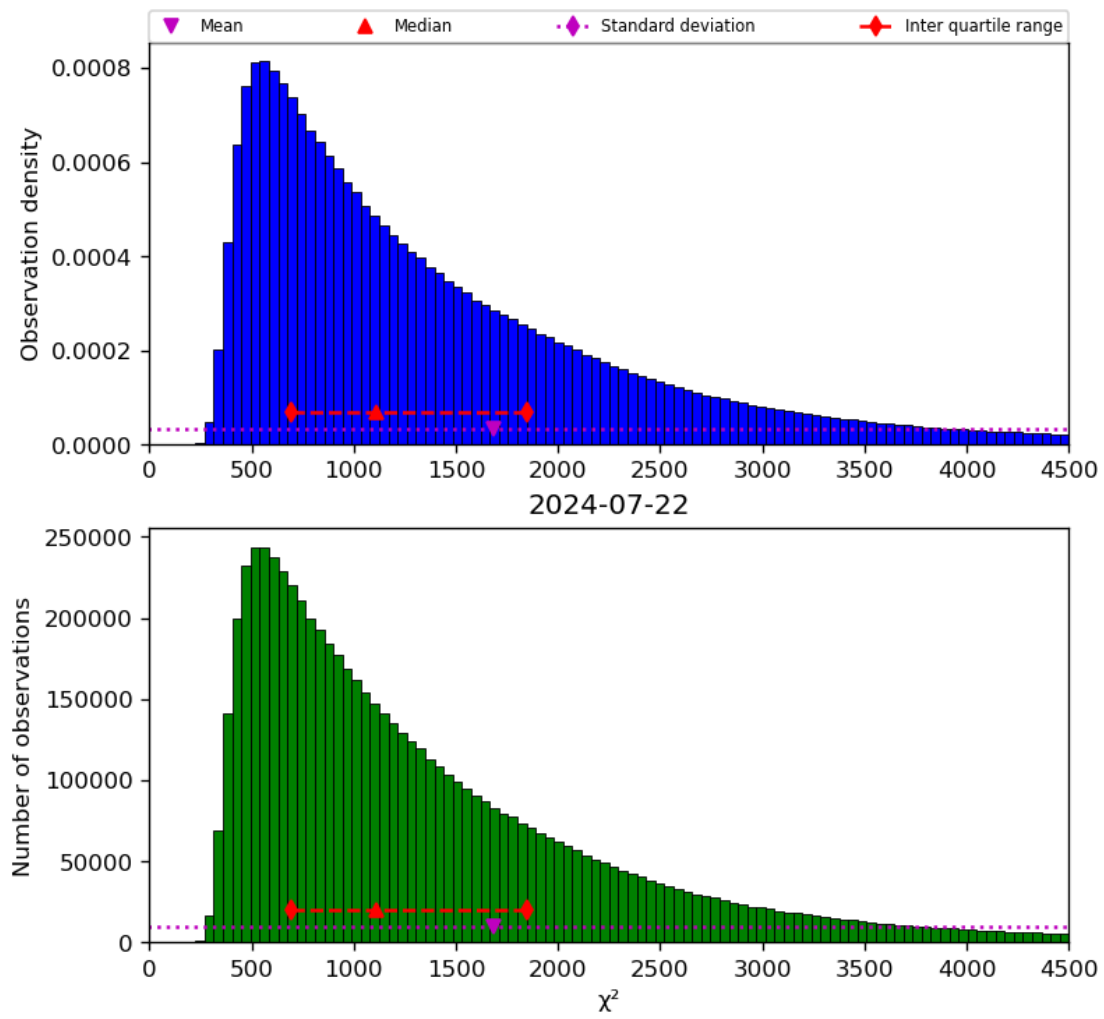
Figure 22: Histogram of “ \chi^2 ” for 2024-07-21 to 2024-07-23
