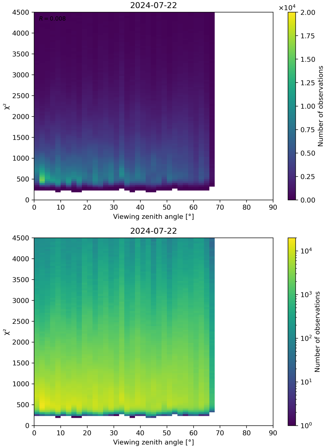
Figure 72: Scatter density plot of “Viewing zenith angle” against “ \chi^2 ” for 2024-07-21 to 2024-07-23.
