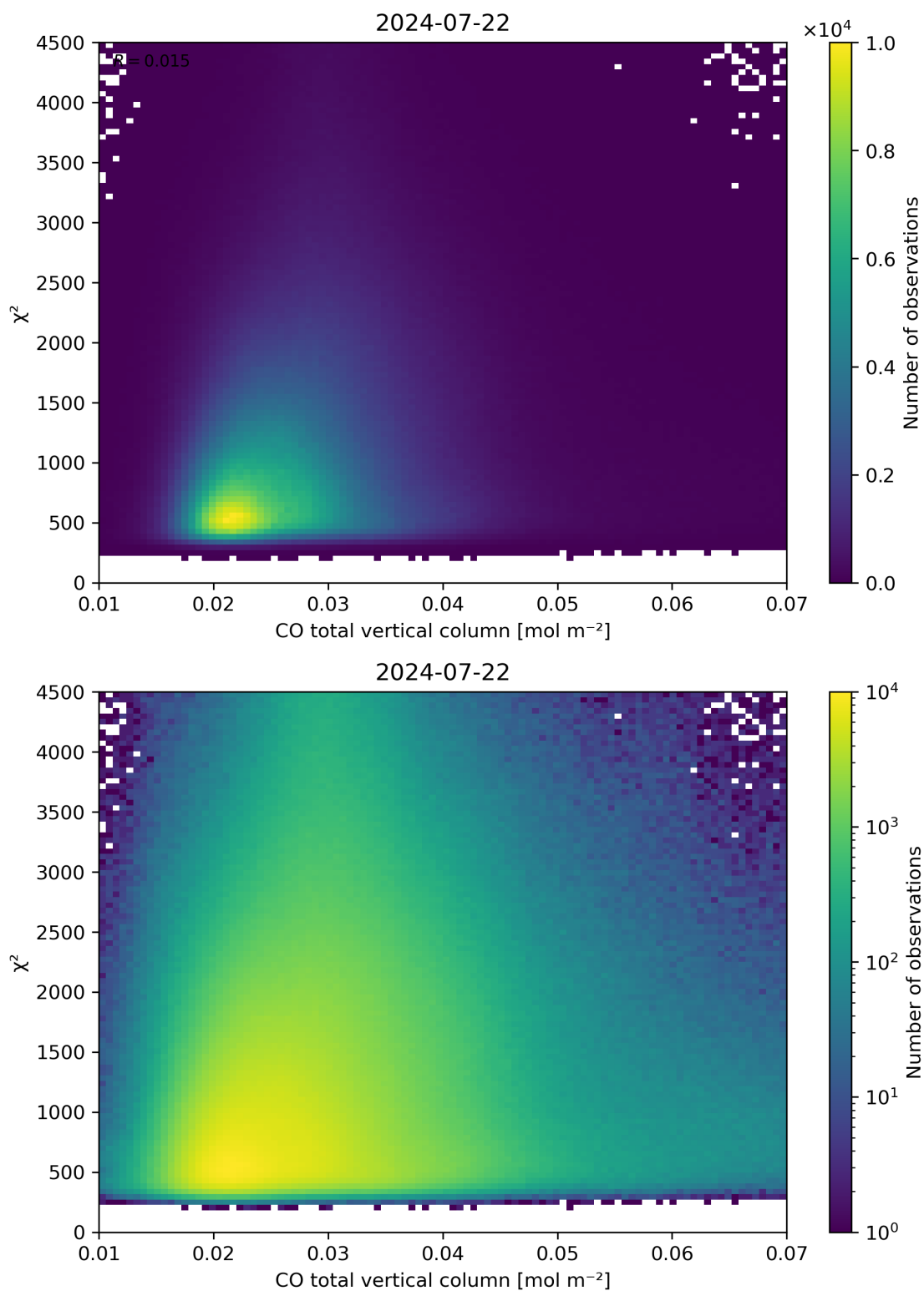
Figure 35: Scatter density plot of “CO total vertical column” against “ \chi^2 ” for 2024-07-21 to 2024-07-23.
