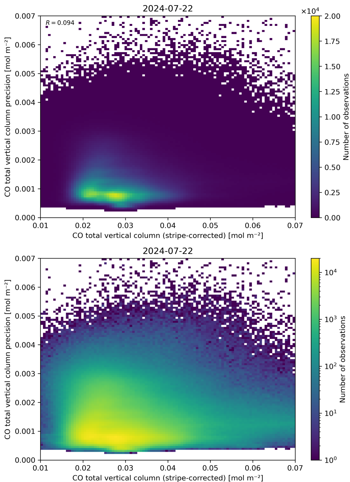
Figure 36: Scatter density plot of “CO total vertical column (stripe-corrected)” against “CO total vertical column precision” for 2024-07-21 to 2024-07-23.
