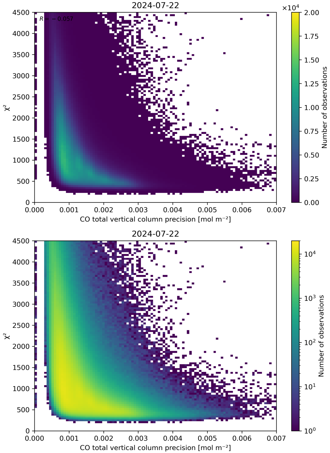
Figure 44: Scatter density plot of “CO total vertical column precision” against “ \chi^2 ” for 2024-07-21 to 2024-07-23.
