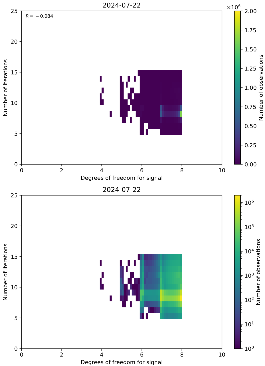
Figure 50: Scatter density plot of “Degrees of freedom for signal” against “Number of iterations” for 2024-07-21 to 2024-07-23.
