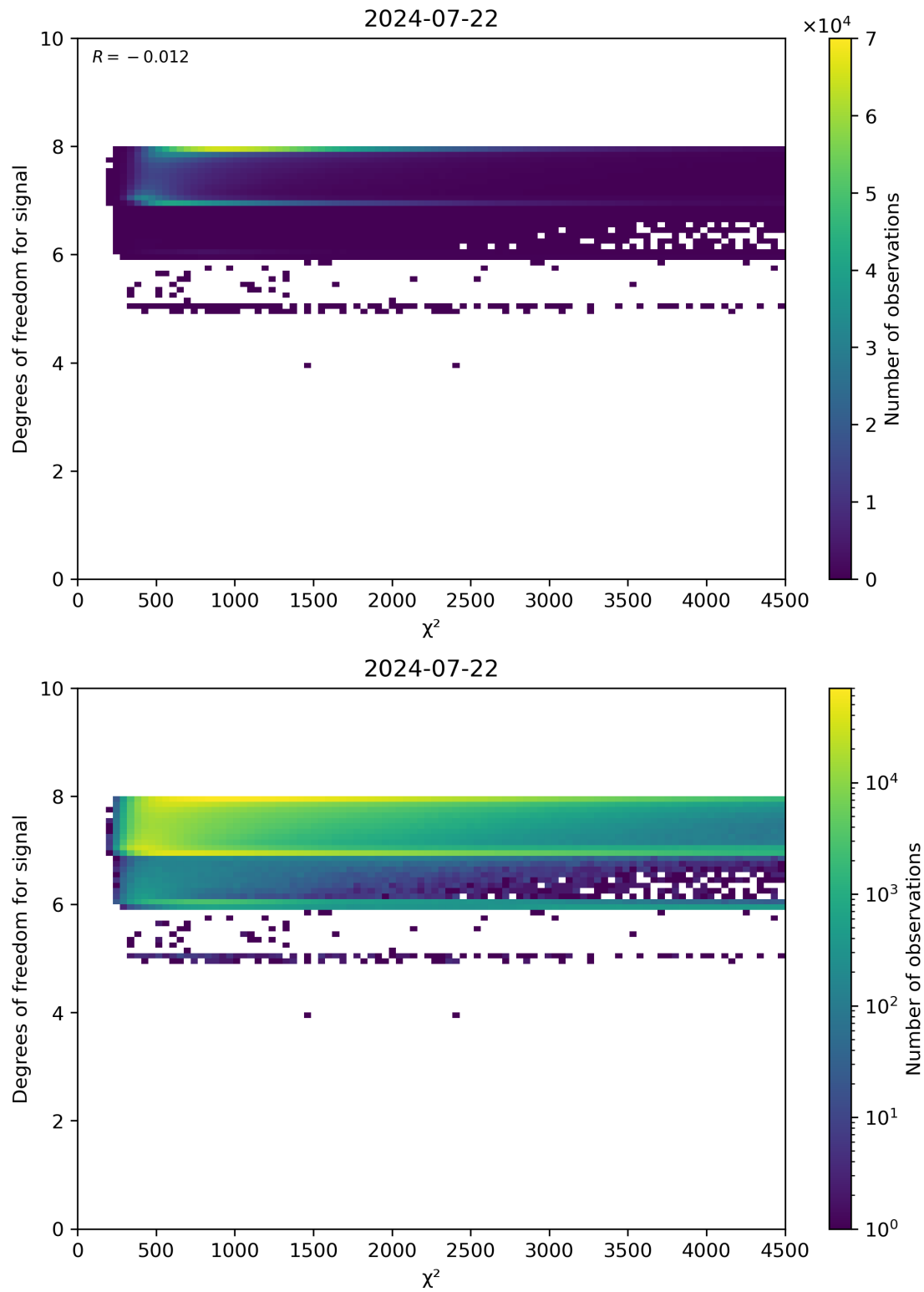
Figure 48: Scatter density plot of “ \chi^2 ” against “Degrees of freedom for signal” for 2024-07-21 to 2024-07-23.
