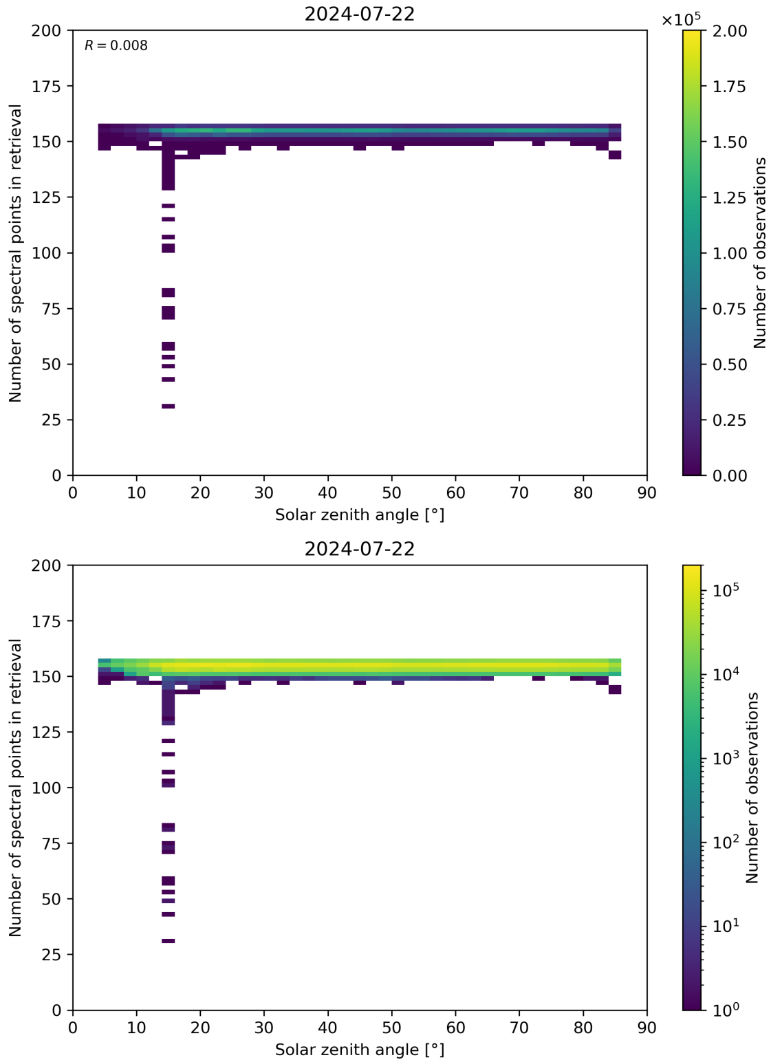
Figure 68: Scatter density plot of “Solar zenith angle” against “Number of spectral points in retrieval” for 2024-07-21 to 2024-07-23.
