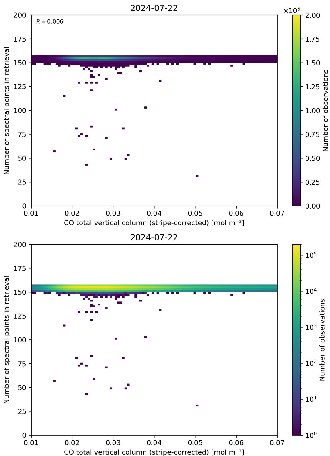
Figure 40: Scatter density plot of “CO total vertical column (stripe-corrected)” against “Number of spectral points in retrieval” for 2024-07-21 to 2024-07-23.
