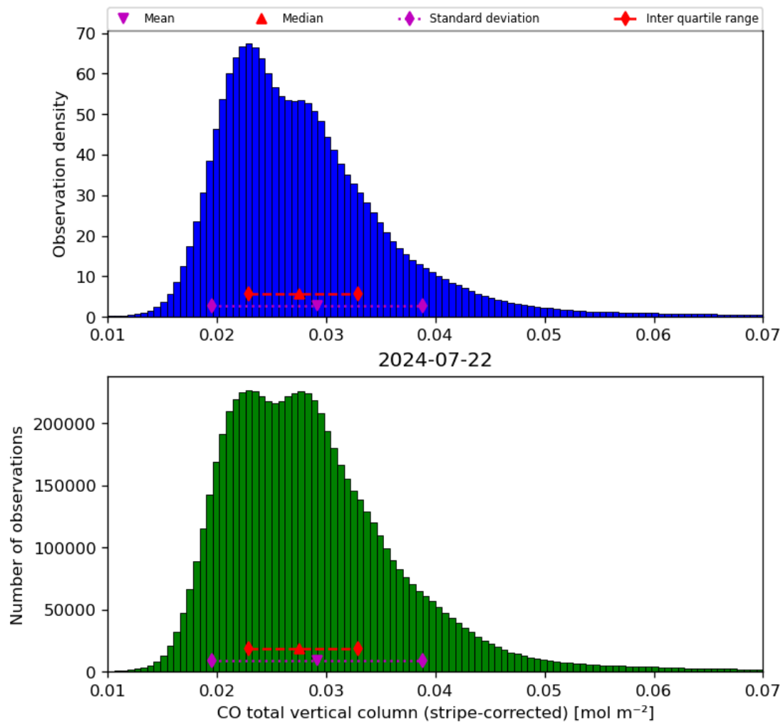
Figure 19: Histogram of “CO total vertical column (stripe-corrected)” for 2024-07-21 to 2024-07-23
