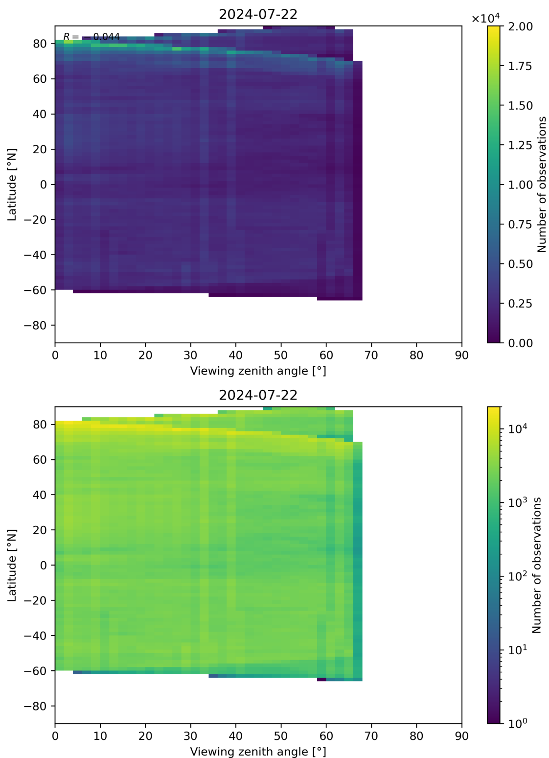
Figure 74: Scatter density plot of “Viewing zenith angle” against “Latitude” for 2024-07-21 to 2024-07-23.
