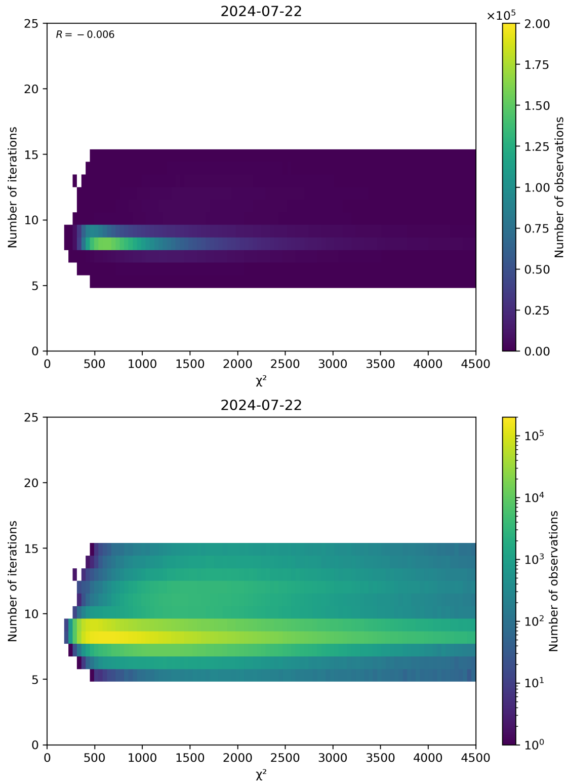
Figure 49: Scatter density plot of “ \chi^2 ” against “Number of iterations” for 2024-07-21 to 2024-07-23.
