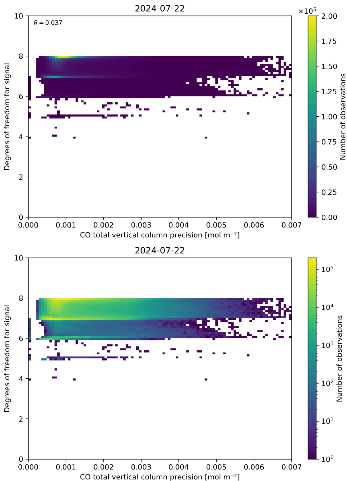
Figure 45: Scatter density plot of “CO total vertical column precision” against “Degrees of freedom for signal” for 2024-07-21 to 2024-07-23.
