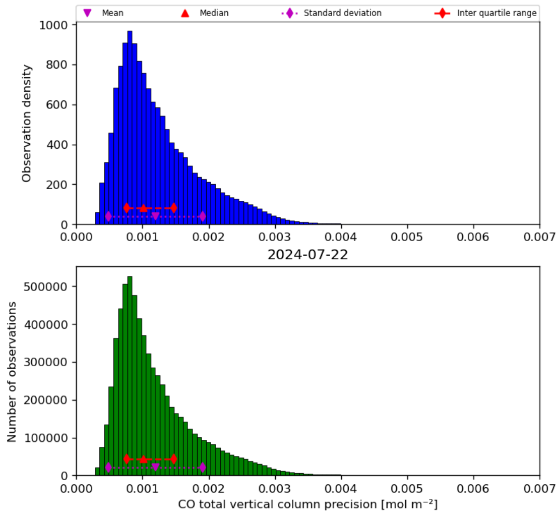
Figure 20: Histogram of “CO total vertical column precision” for 2024-07-21 to 2024-07-23
