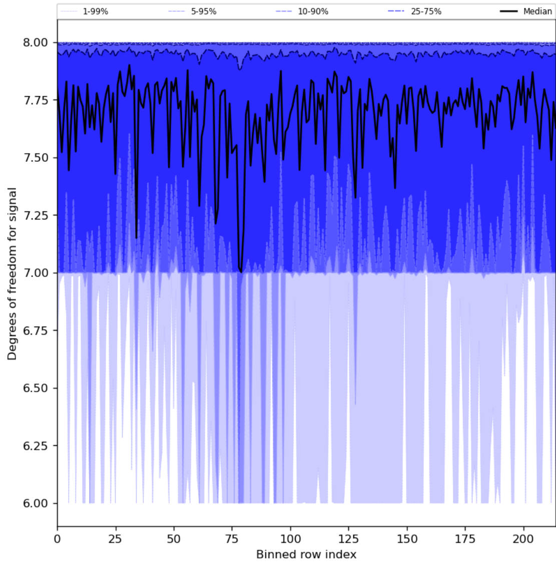
Figure 31: Along track statistics of “Degrees of freedom for signal” for 2024-07-21 to 2024-07-23
