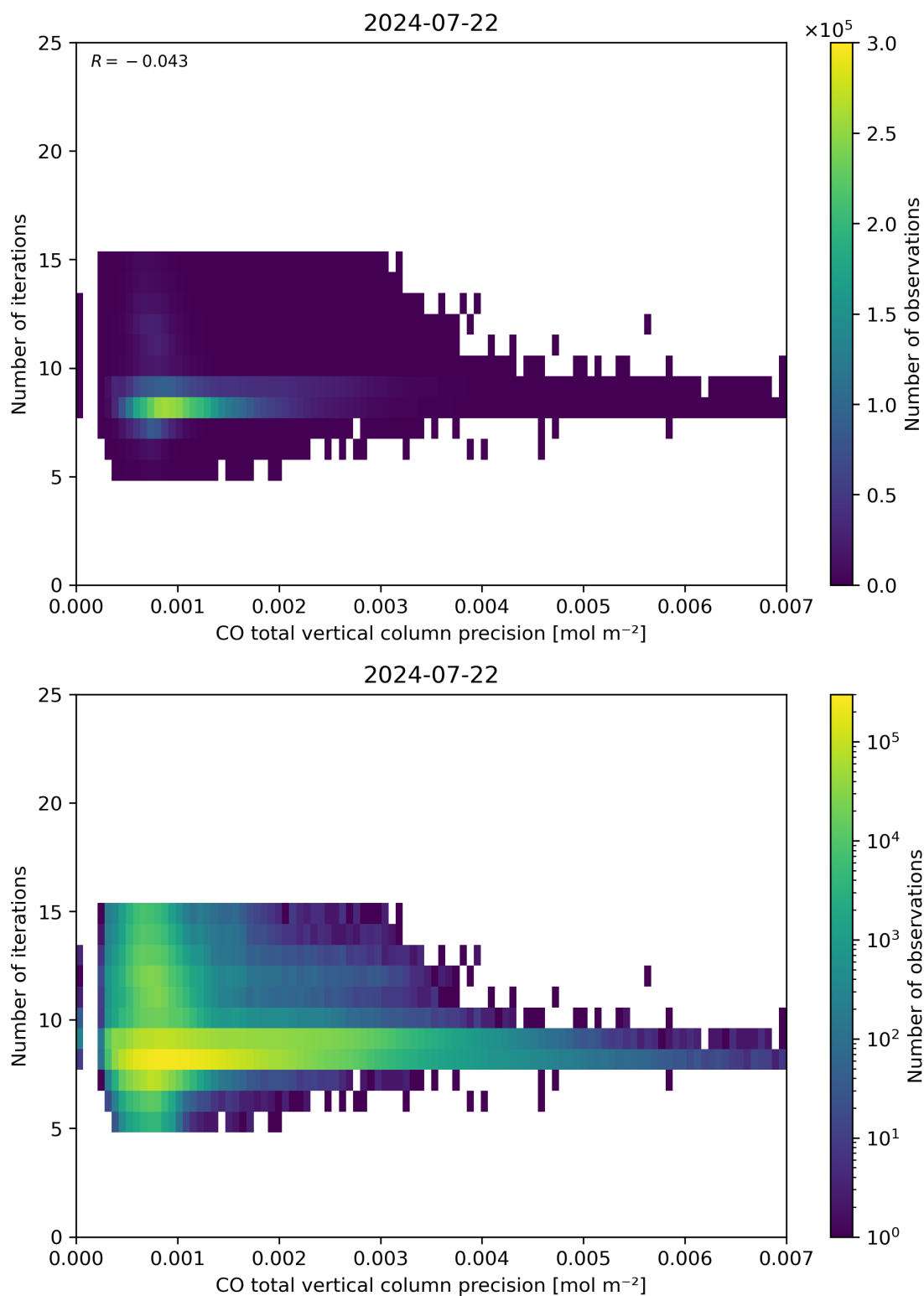
Figure 46: Scatter density plot of “CO total vertical column precision” against “Number of iterations” for 2024-07-21 to 2024-07-23.
