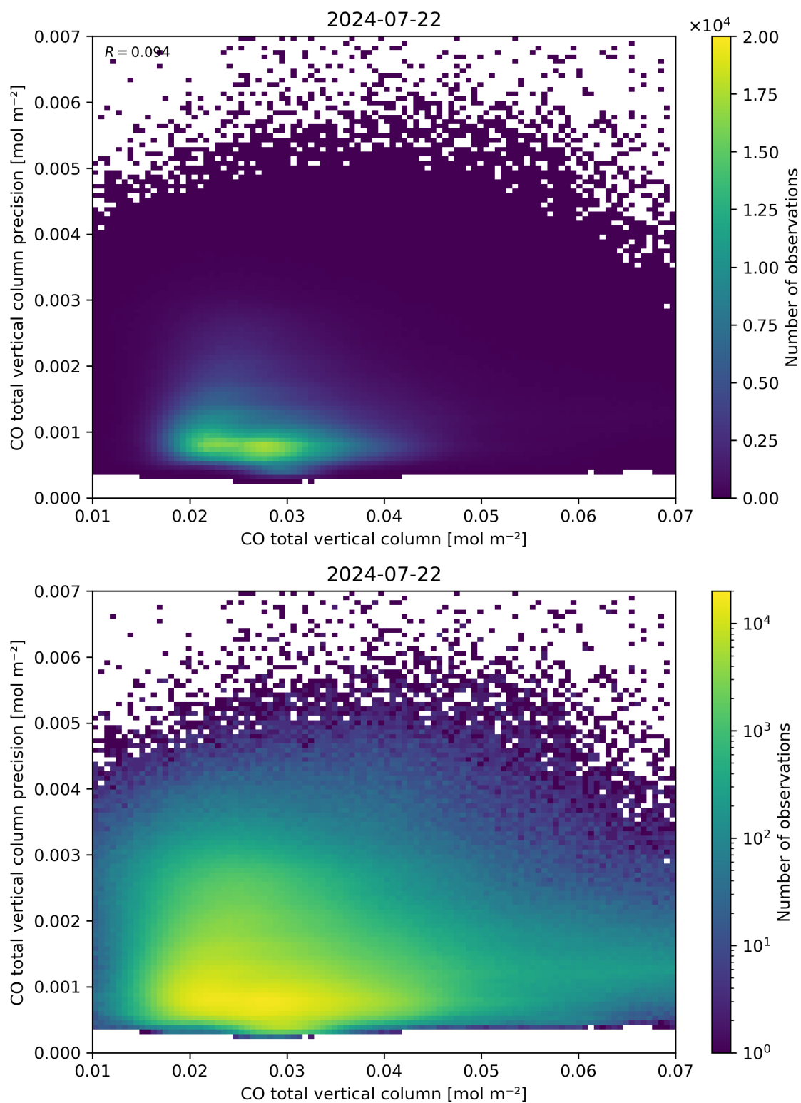
Figure 34: Scatter density plot of “CO total vertical column” against “CO total vertical column precision” for 2024-07-21 to 2024-07-23.
