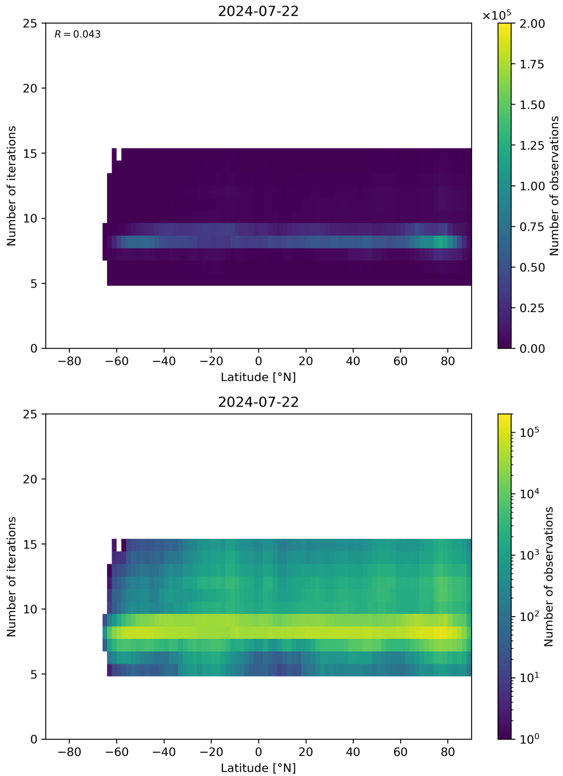
Figure 56: Scatter density plot of “Latitude” against “Number of iterations” for 2024-07-21 to 2024-07-23.
