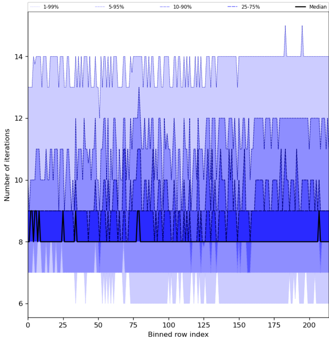
Figure 32: Along track statistics of “Number of iterations” for 2024-07-21 to 2024-07-23
