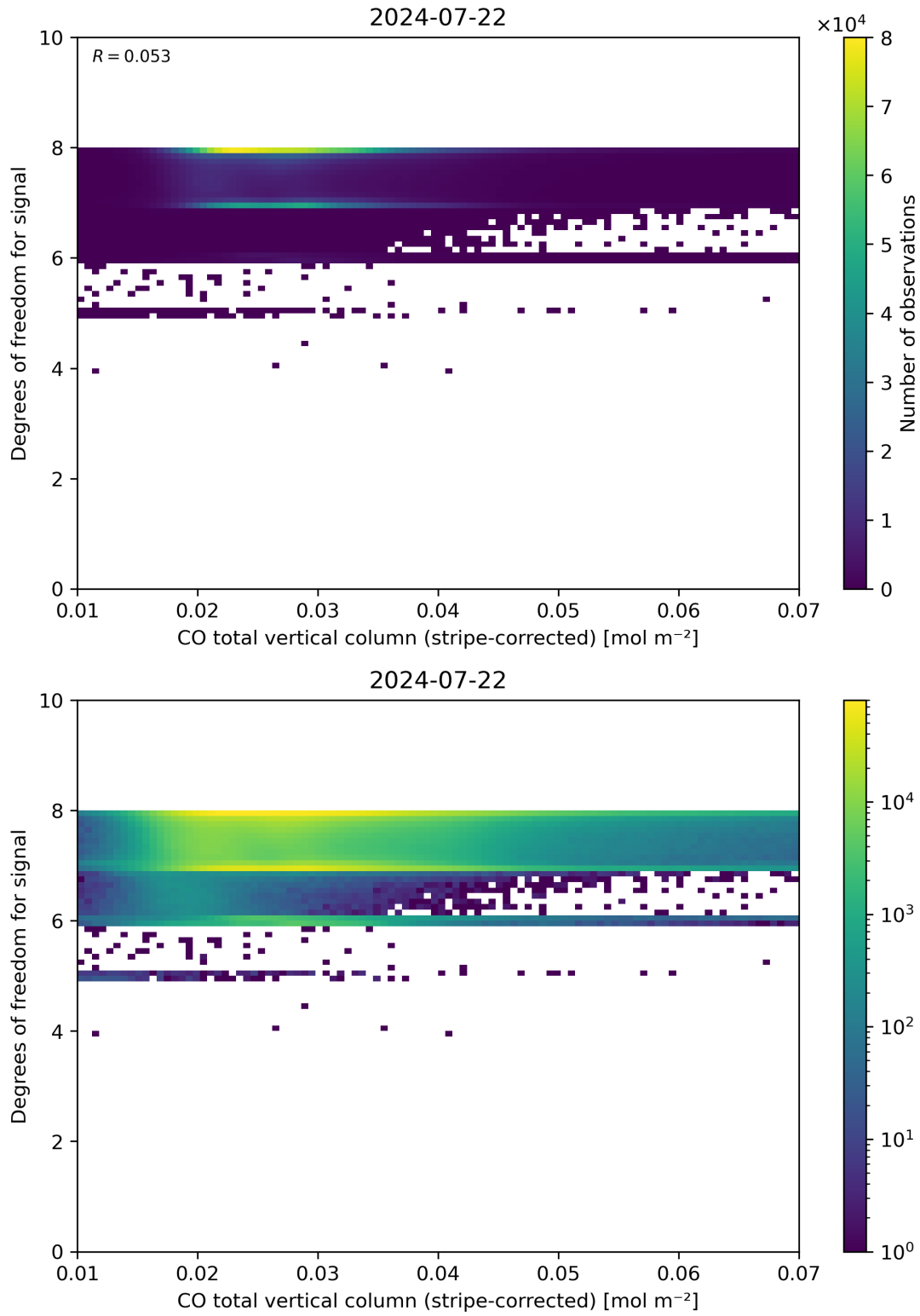
Figure 38: Scatter density plot of “CO total vertical column (stripe-corrected)” against “Degrees of freedom for signal” for 2024-07-21 to 2024-07-23.
