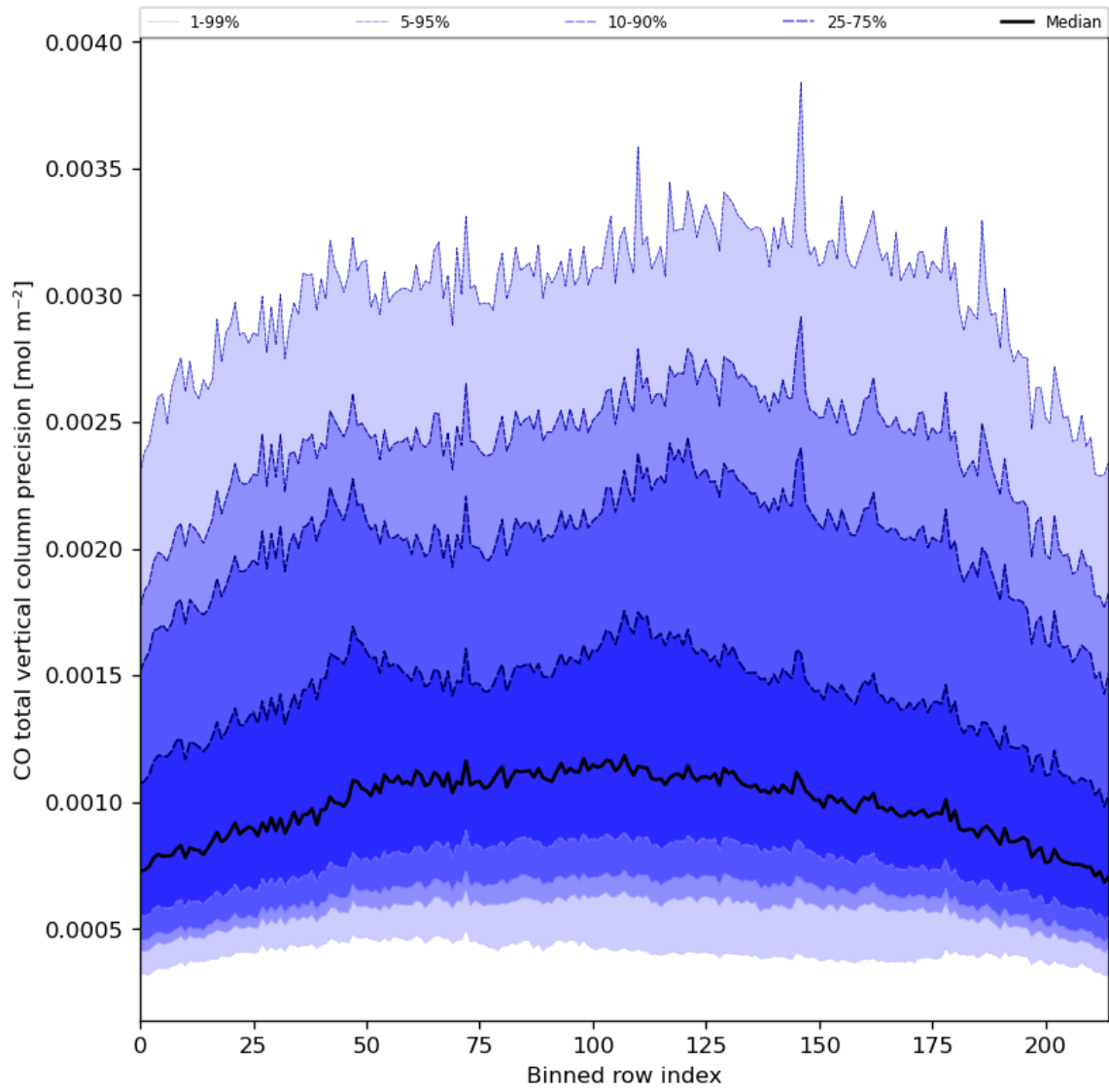
Figure 28: Along track statistics of “CO total vertical column precision” for 2024-07-22 to 2024-07-24
