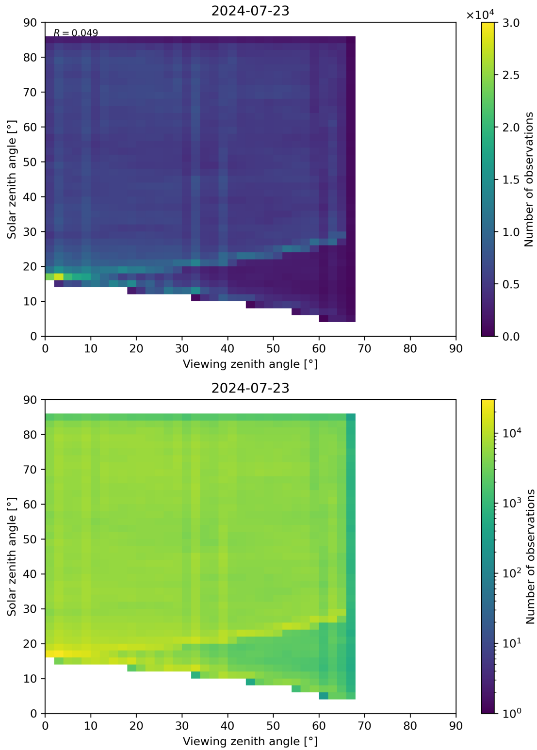
Figure 77: Scatter density plot of “Viewing zenith angle” against “Solar zenith angle” for 2024-07-22 to 2024-07-24.
