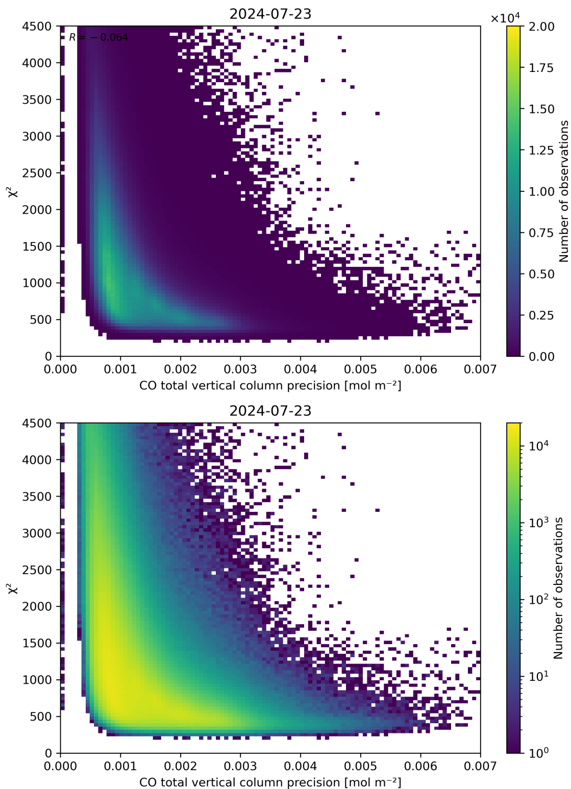
Figure 44: Scatter density plot of “CO total vertical column precision” against “ \chi^2 ” for 2024-07-22 to 2024-07-24.
