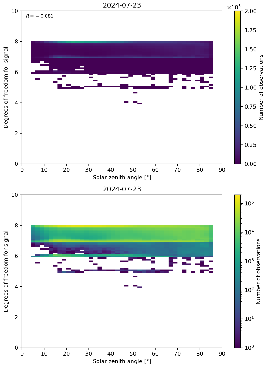
Figure 65: Scatter density plot of “Solar zenith angle” against “Degrees of freedom for signal” for 2024-07-22 to 2024-07-24.
