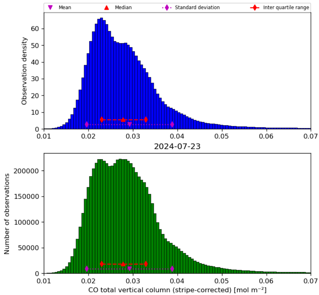
Figure 19: Histogram of “CO total vertical column (stripe-corrected)” for 2024-07-22 to 2024-07-24
