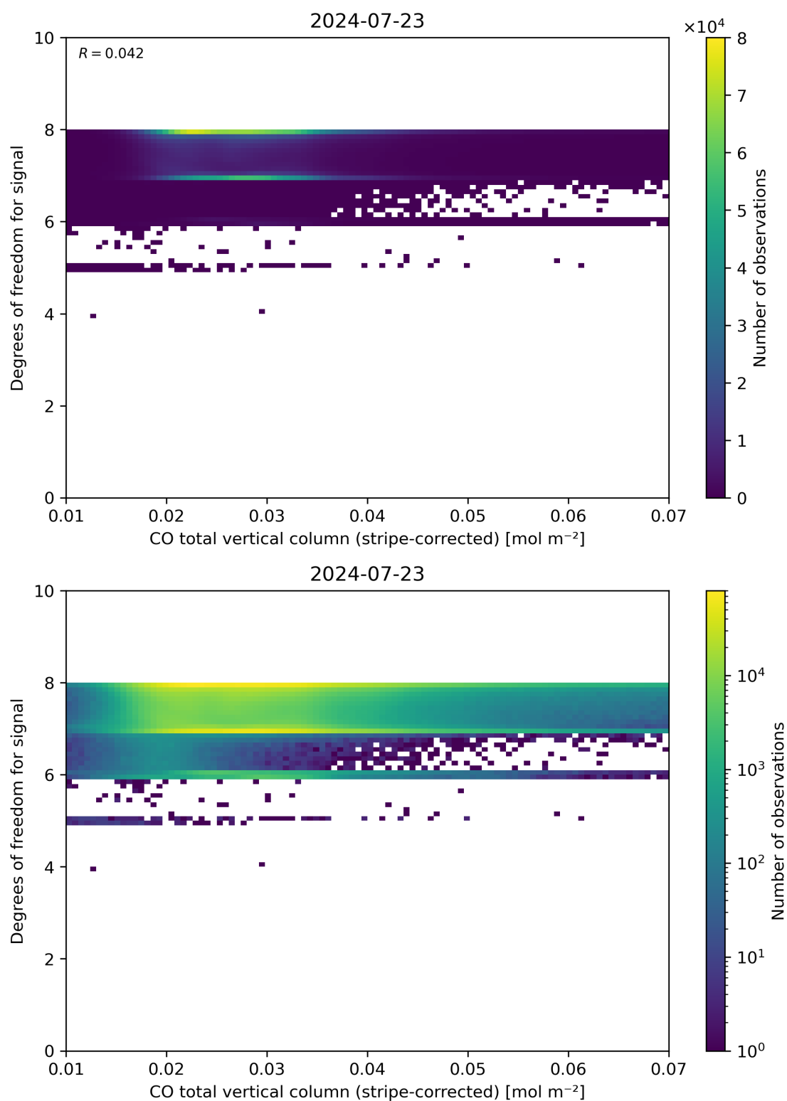
Figure 38: Scatter density plot of “CO total vertical column (stripe-corrected)” against “Degrees of freedom for signal” for 2024-07-22 to 2024-07-24.
