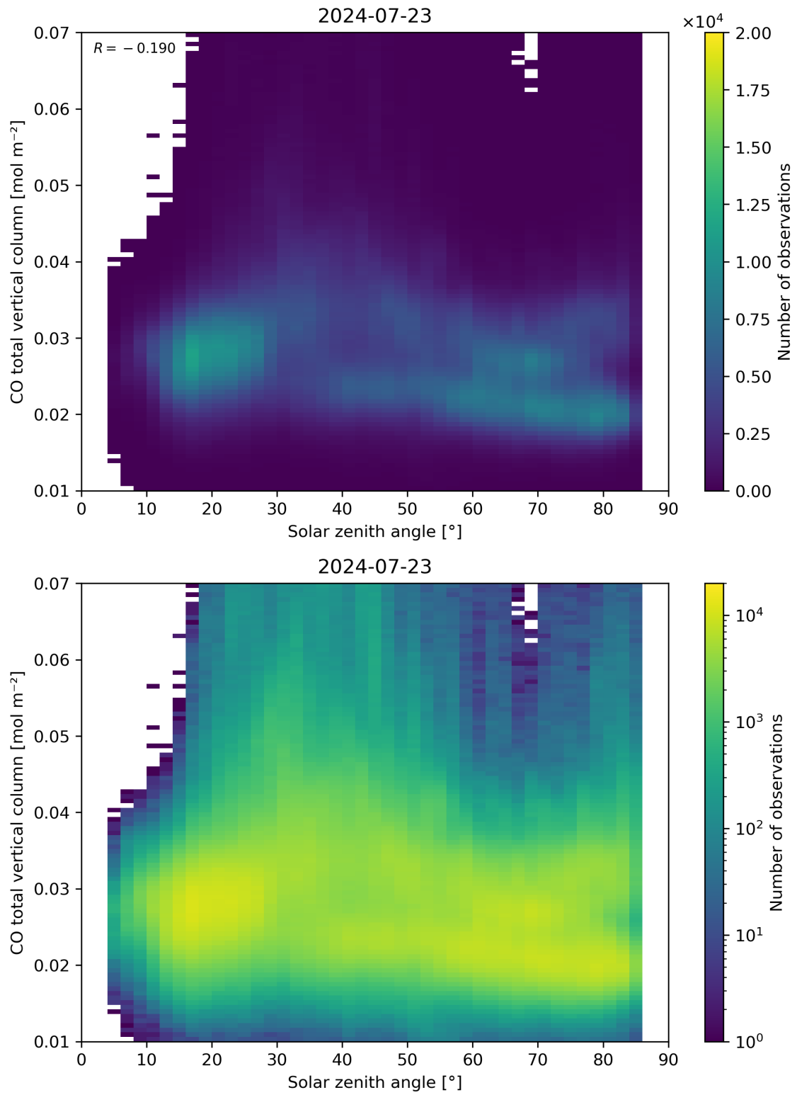
Figure 61: Scatter density plot of “Solar zenith angle” against “CO total vertical column” for 2024-07-22 to 2024-07-24.
