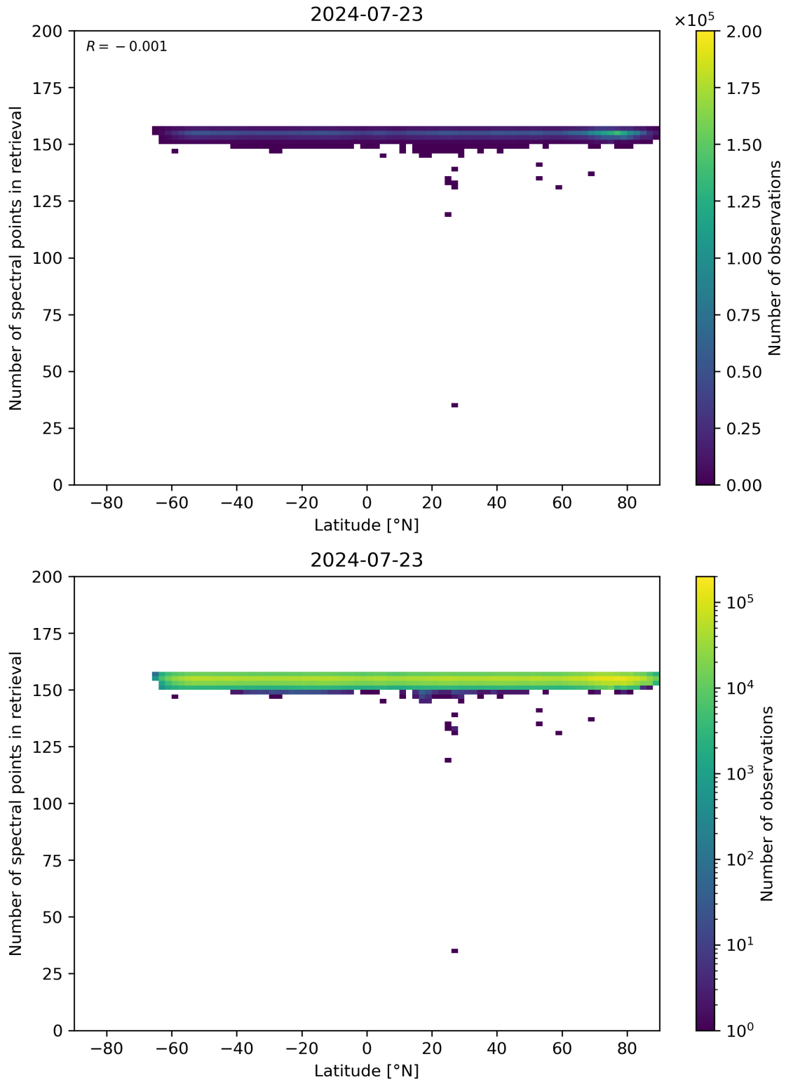
Figure 57: Scatter density plot of “Latitude” against “Number of spectral points in retrieval” for 2024-07-22 to 2024-07-24.
