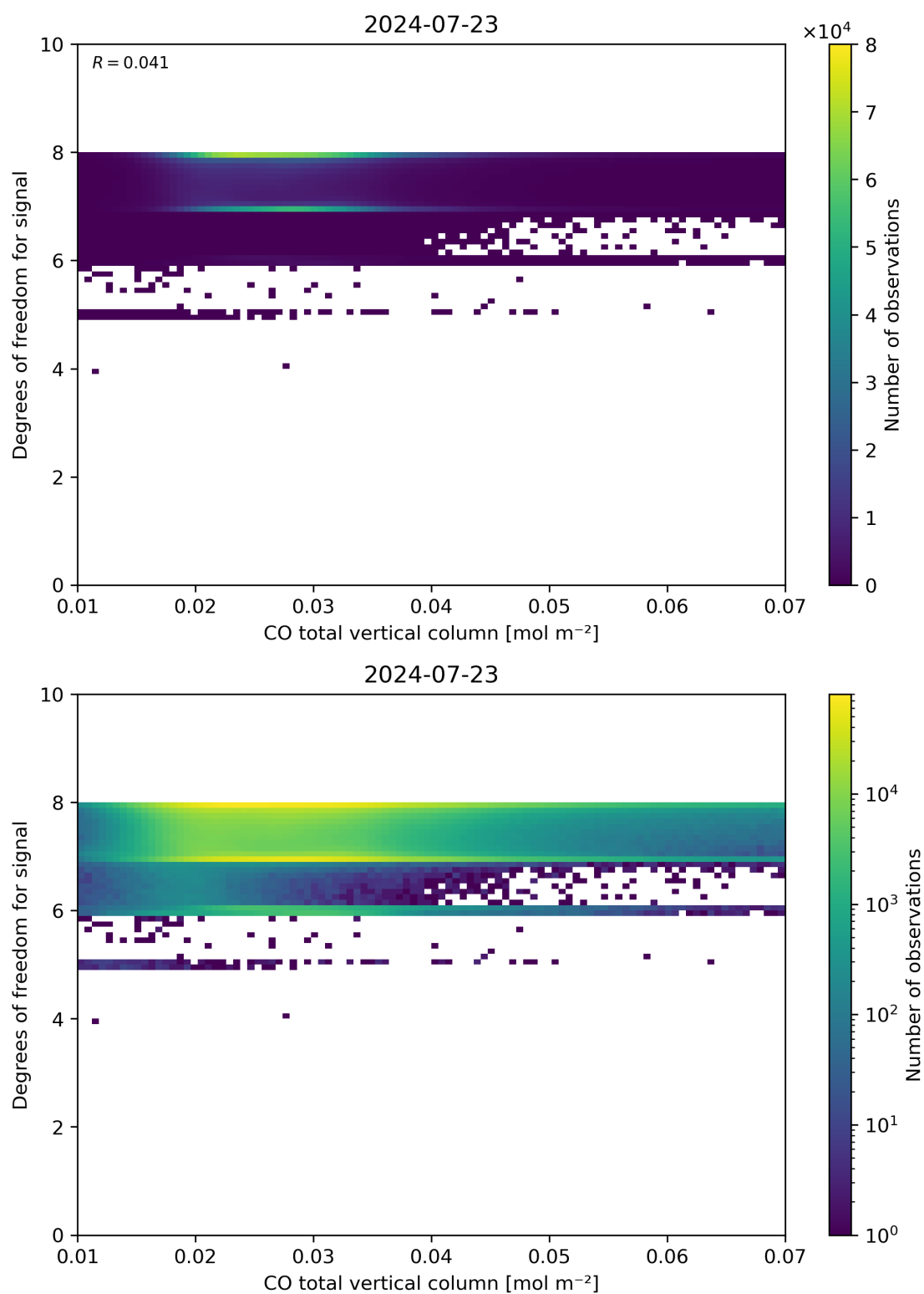
Figure 41: Scatter density plot of “CO total vertical column” against “Degrees of freedom for signal” for 2024-07-22 to 2024-07-24.
