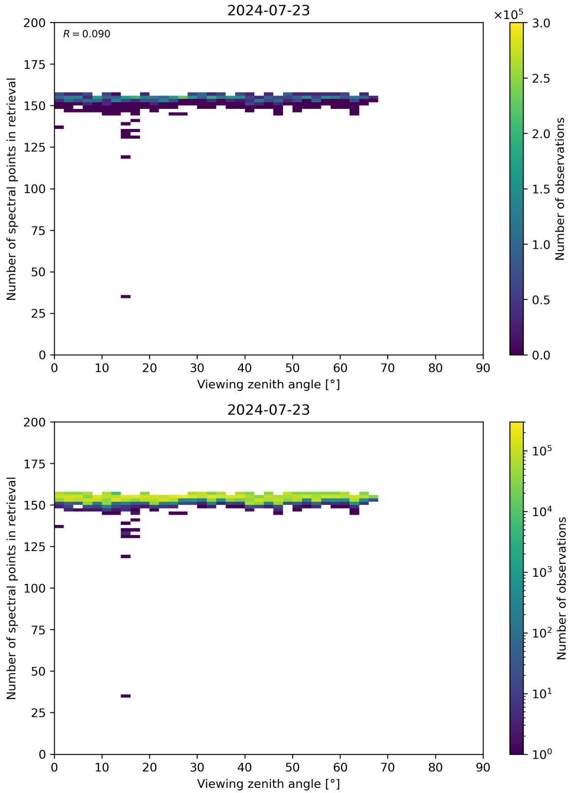
Figure 76: Scatter density plot of “Viewing zenith angle” against “Number of spectral points in retrieval” for 2024-07-22 to 2024-07-24.
