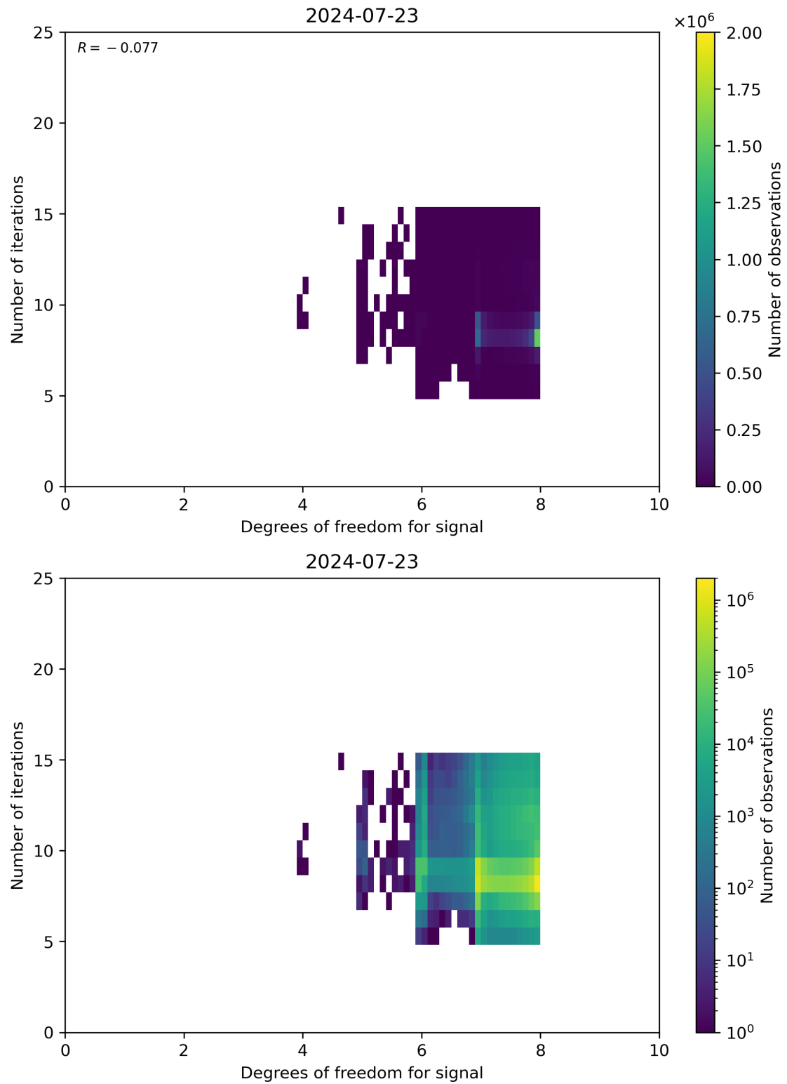
Figure 50: Scatter density plot of “Degrees of freedom for signal” against “Number of iterations” for 2024-07-22 to 2024-07-24.
