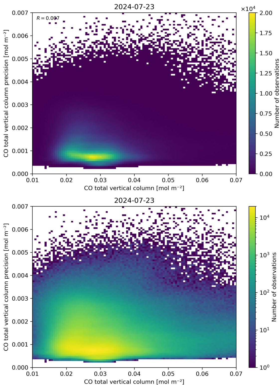
Figure 34: Scatter density plot of “CO total vertical column” against “CO total vertical column precision” for 2024-07-22 to 2024-07-24.
