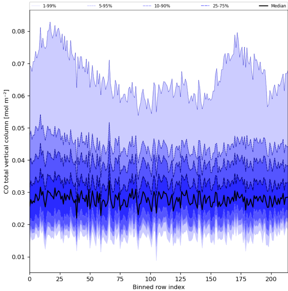
Figure 26: Along track statistics of “CO total vertical column” for 2024-07-22 to 2024-07-24
