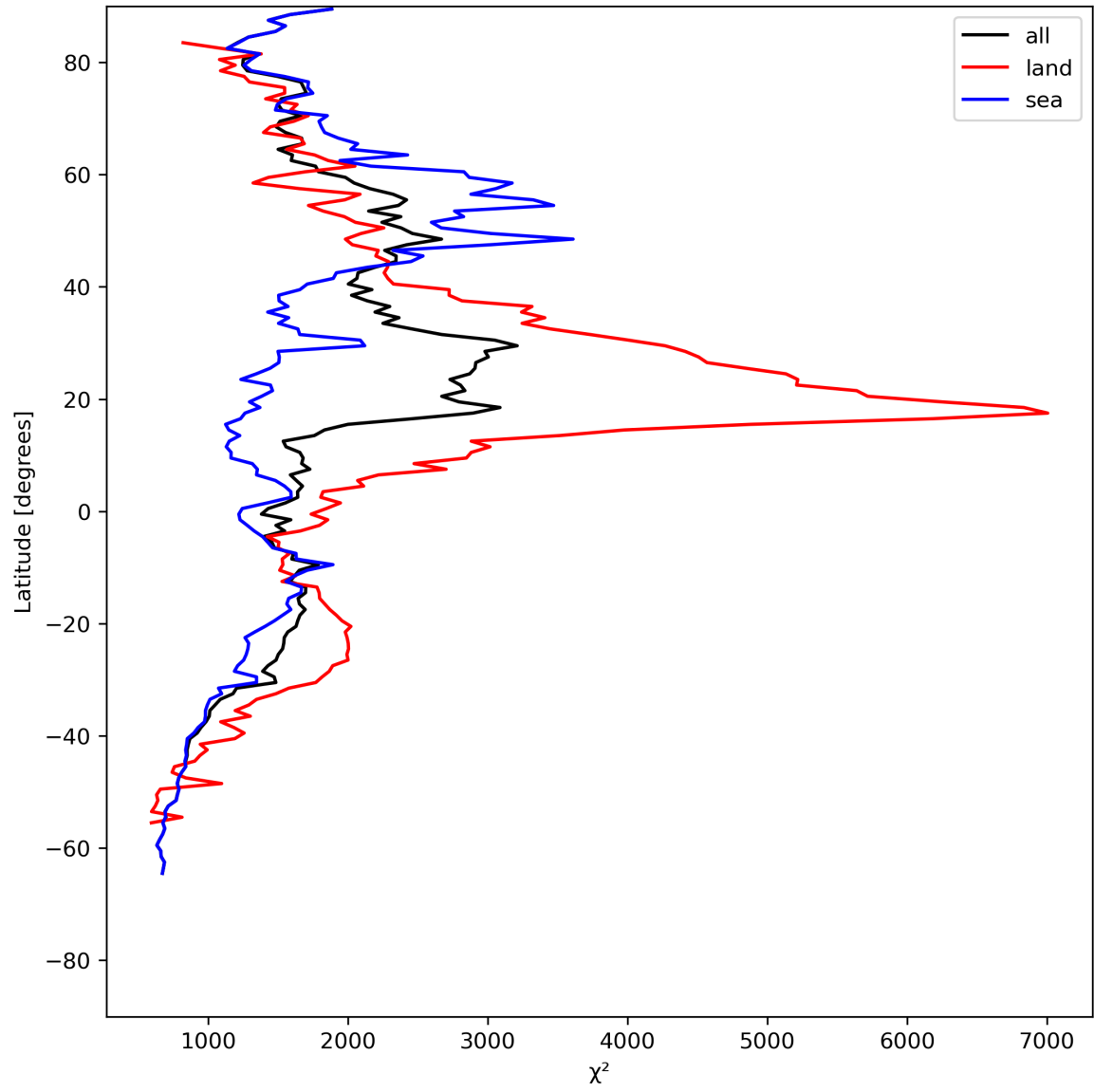
Figure 14: Zonal average of “ \chi^2 ” for 2024-07-22 to 2024-07-24.
