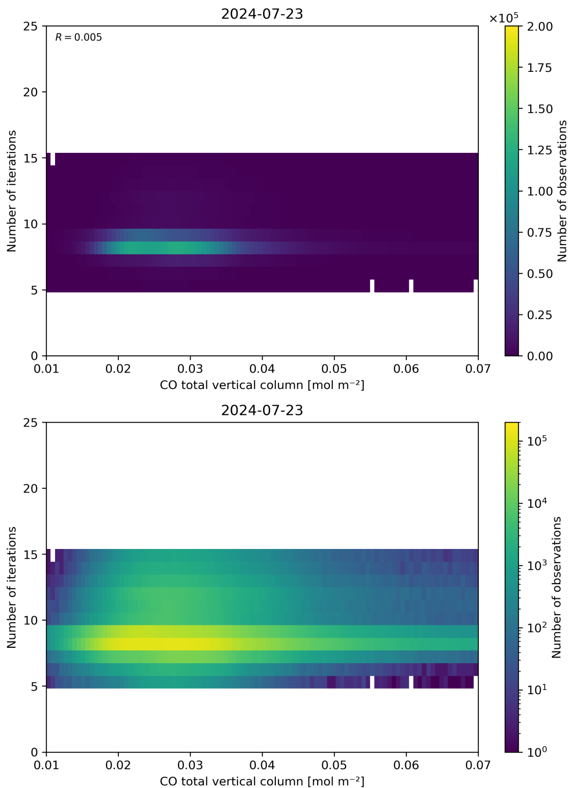
Figure 42: Scatter density plot of “CO total vertical column” against “Number of iterations” for 2024-07-22 to 2024-07-24.
