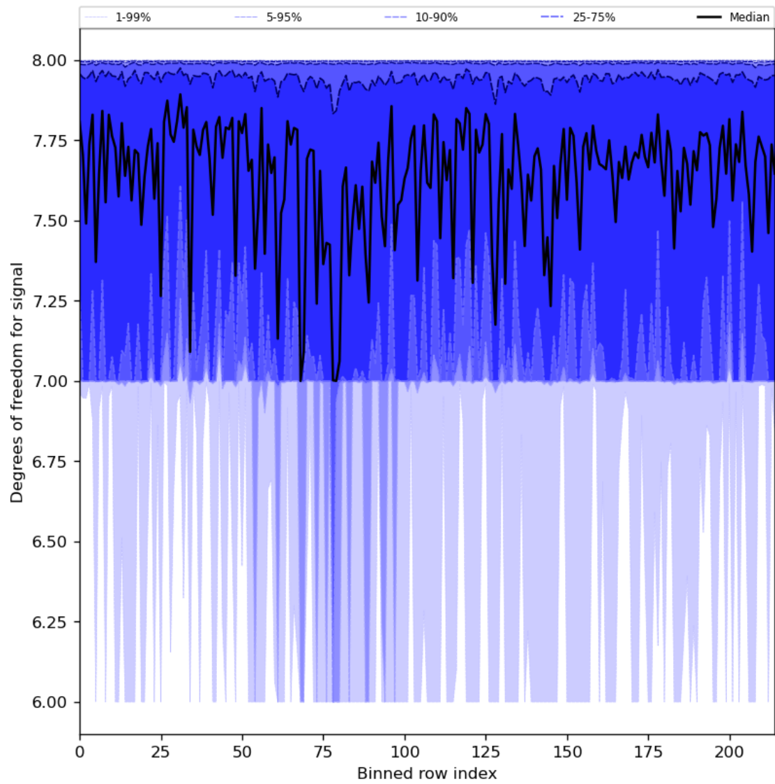
Figure 31: Along track statistics of “Degrees of freedom for signal” for 2024-07-22 to 2024-07-24
