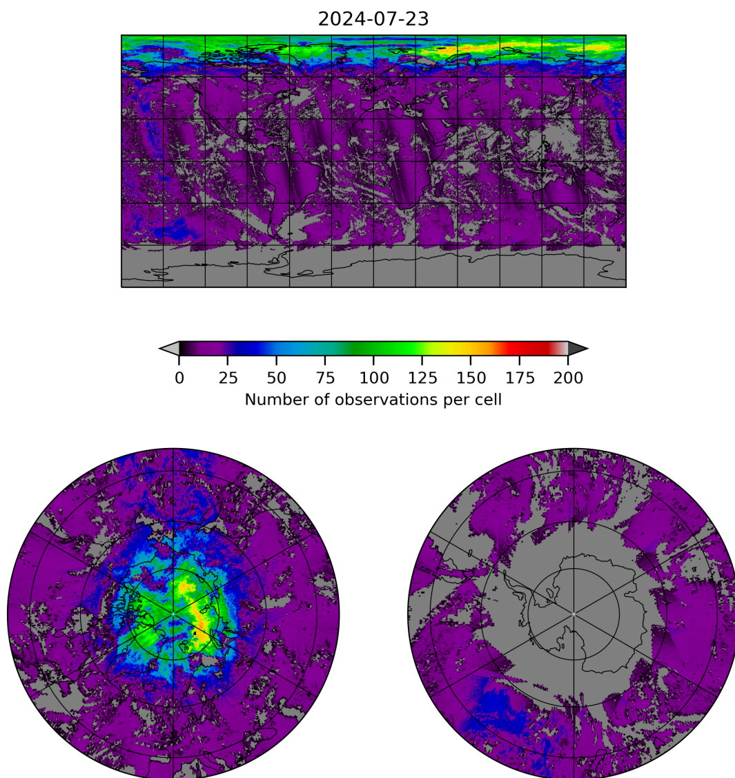
Figure 8: Map of the number of observations for 2024-07-22 to 2024-07-24
