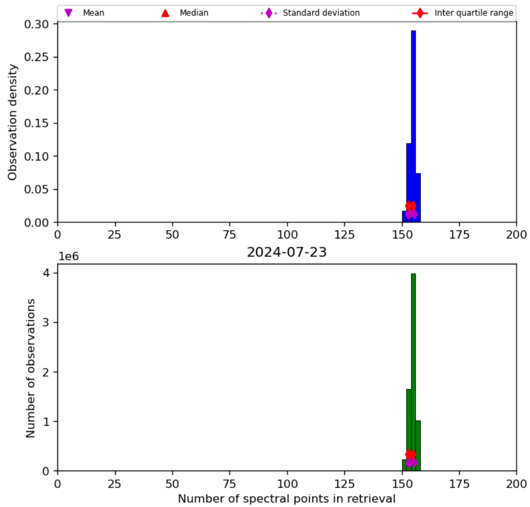
Figure 21: Histogram of “Number of spectral points in retrieval” for 2024-07-22 to 2024-07-24
