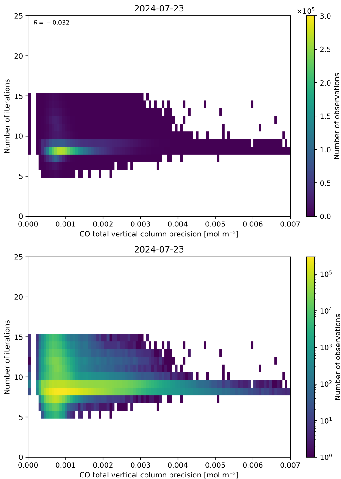
Figure 46: Scatter density plot of “CO total vertical column precision” against “Number of iterations” for 2024-07-22 to 2024-07-24.
