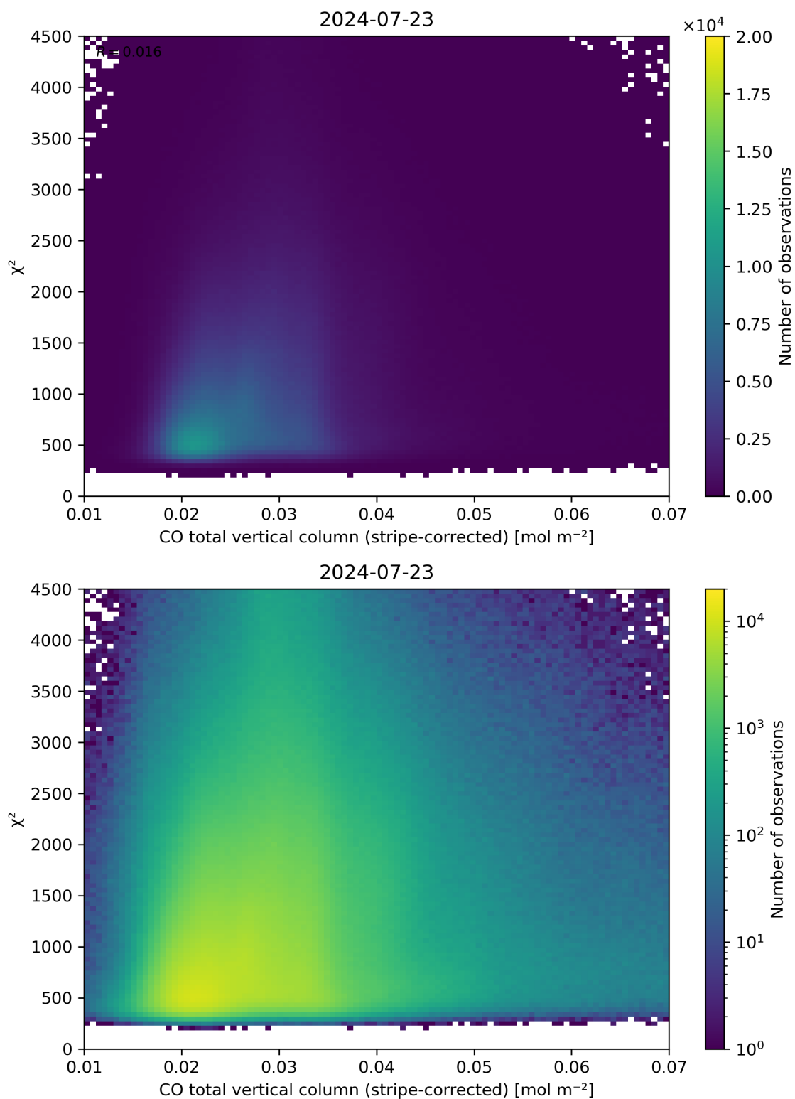
Figure 37: Scatter density plot of “CO total vertical column (stripe-corrected)” against “ \chi^2 ” for 2024-07-22 to 2024-07-24.
