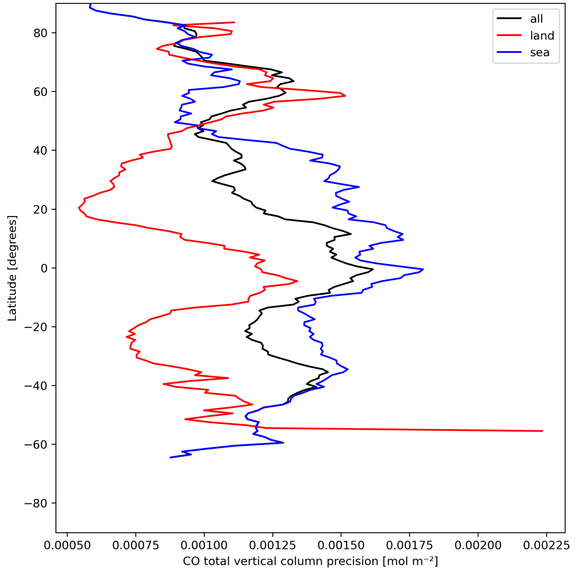
Figure 12: Zonal average of “CO total vertical column precision” for 2024-07-22 to 2024-07-24.
