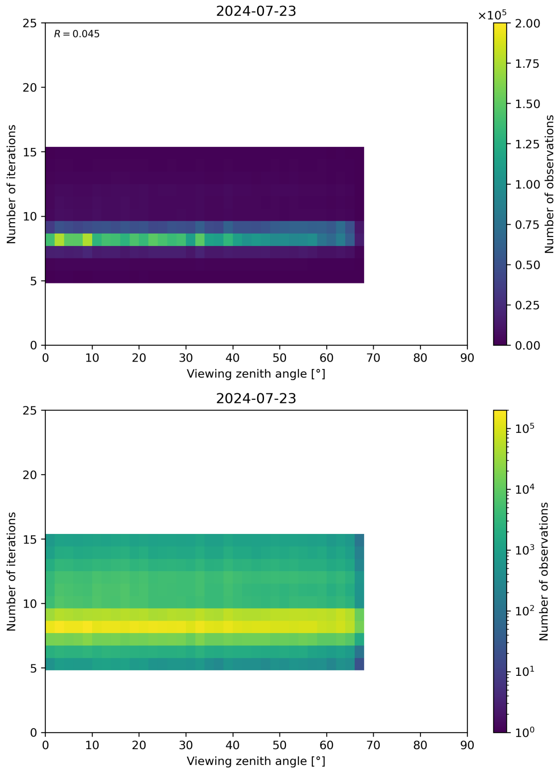
Figure 75: Scatter density plot of “Viewing zenith angle” against “Number of iterations” for 2024-07-22 to 2024-07-24.
