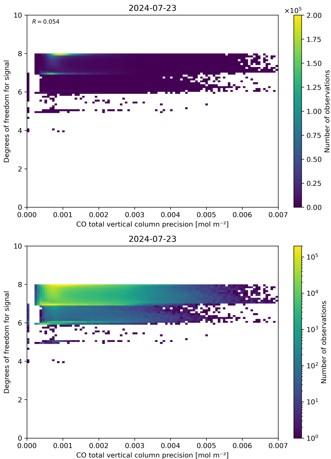
Figure 45: Scatter density plot of “CO total vertical column precision” against “Degrees of freedom for signal” for 2024-07-22 to 2024-07-24.
