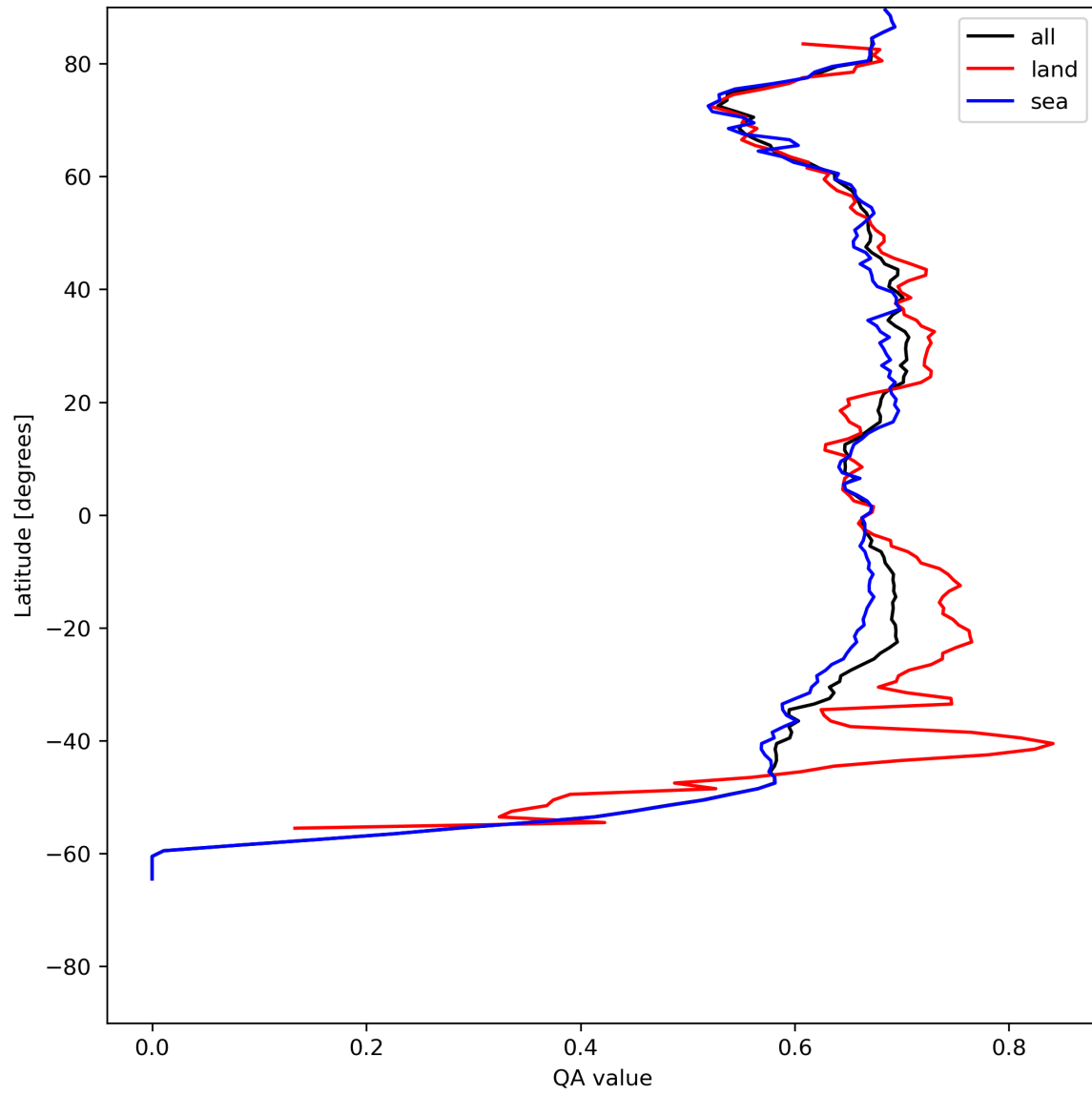
Figure 9: Zonal average of “QA value” for 2024-07-22 to 2024-07-24.
