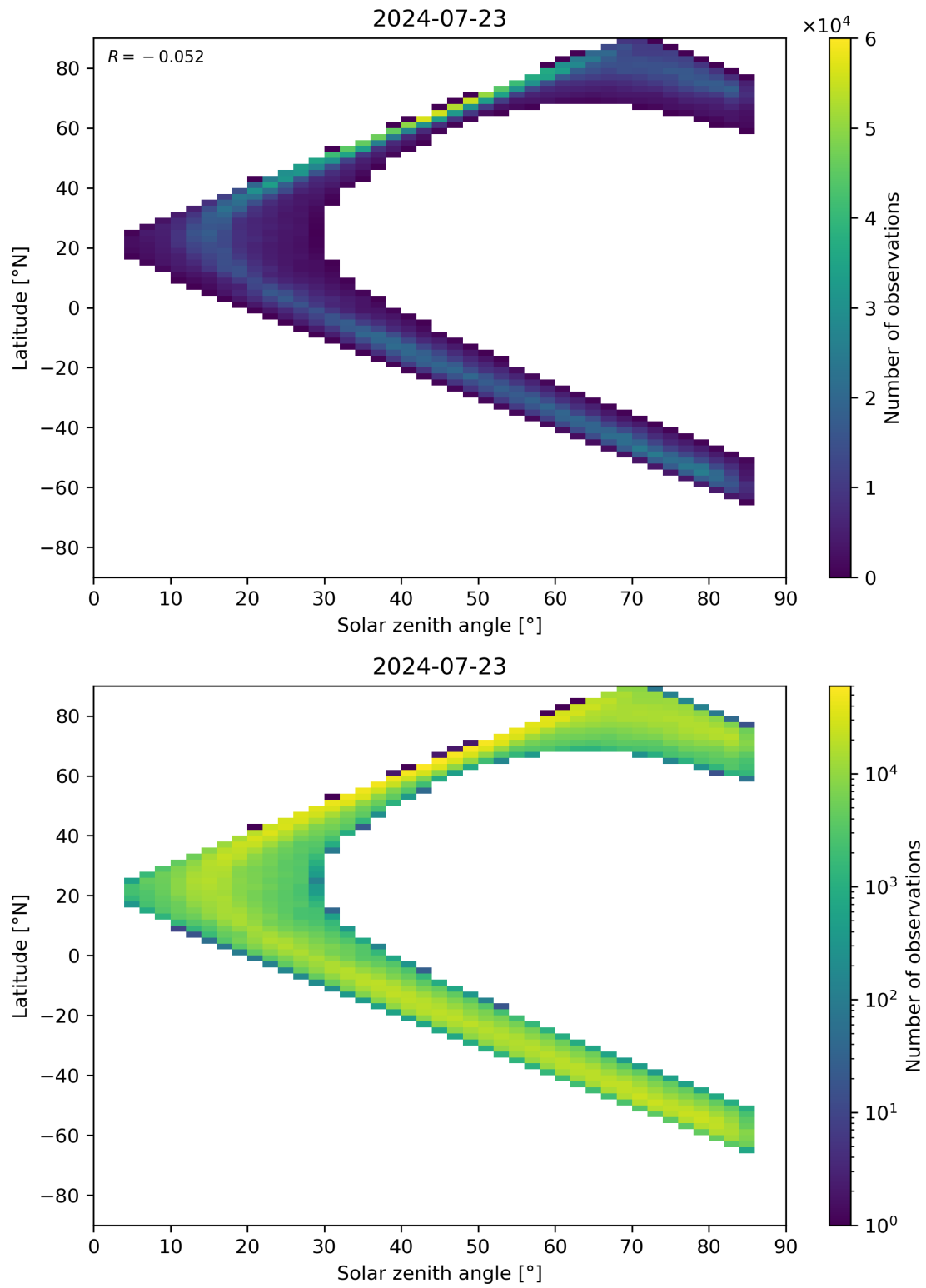
Figure 66: Scatter density plot of “Solar zenith angle” against “Latitude” for 2024-07-22 to 2024-07-24.
