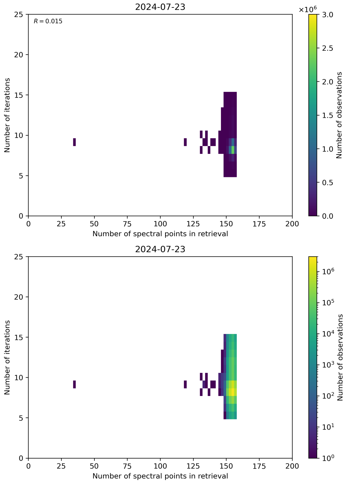
Figure 60: Scatter density plot of “Number of spectral points in retrieval” against “Number of iterations” for 2024-07-22 to 2024-07-24.
