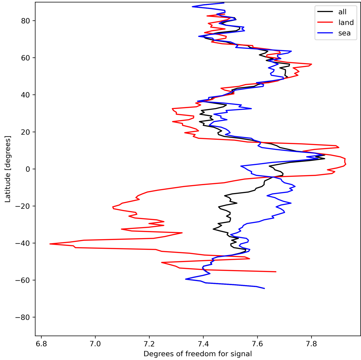
Figure 15: Zonal average of “Degrees of freedom for signal” for 2024-07-22 to 2024-07-24.
