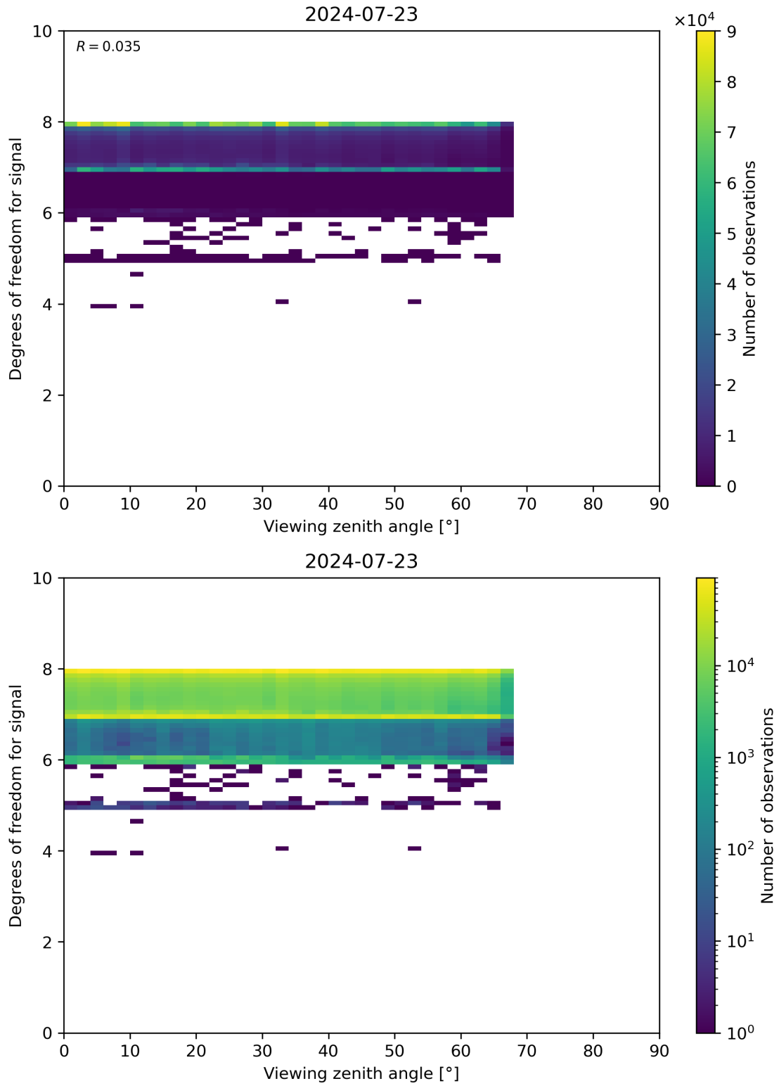
Figure 73: Scatter density plot of “Viewing zenith angle” against “Degrees of freedom for signal” for 2024-07-22 to 2024-07-24.
