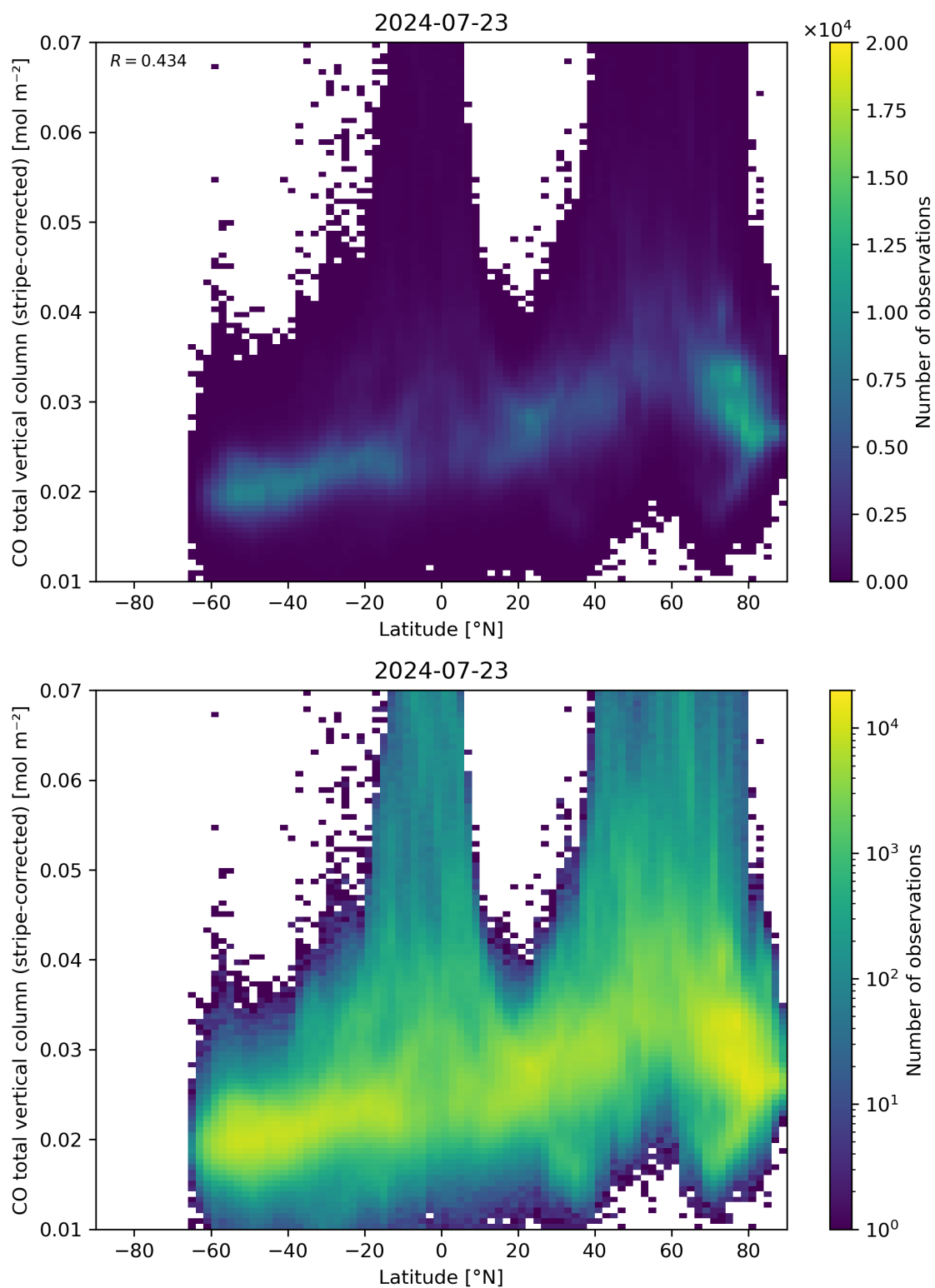
Figure 52: Scatter density plot of “Latitude” against “CO total vertical column (stripe-corrected)” for 2024-07-22 to 2024-07-24.
