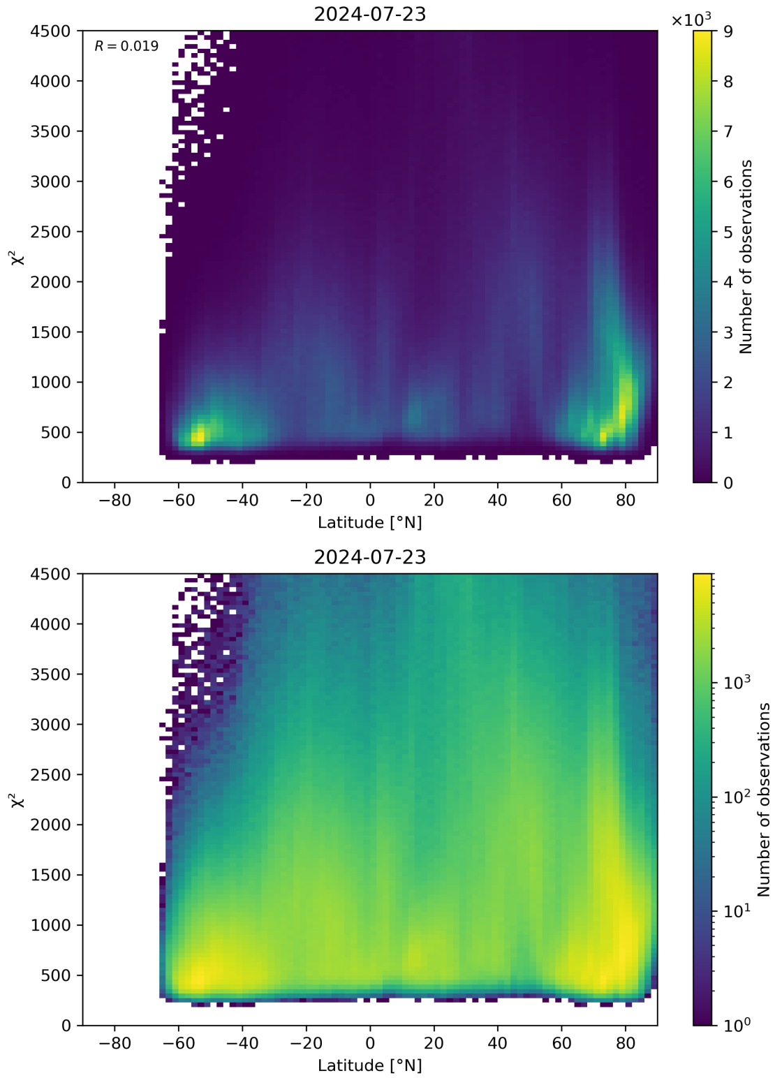
Figure 54: Scatter density plot of “Latitude” against “ \chi^2 ” for 2024-07-22 to 2024-07-24.
