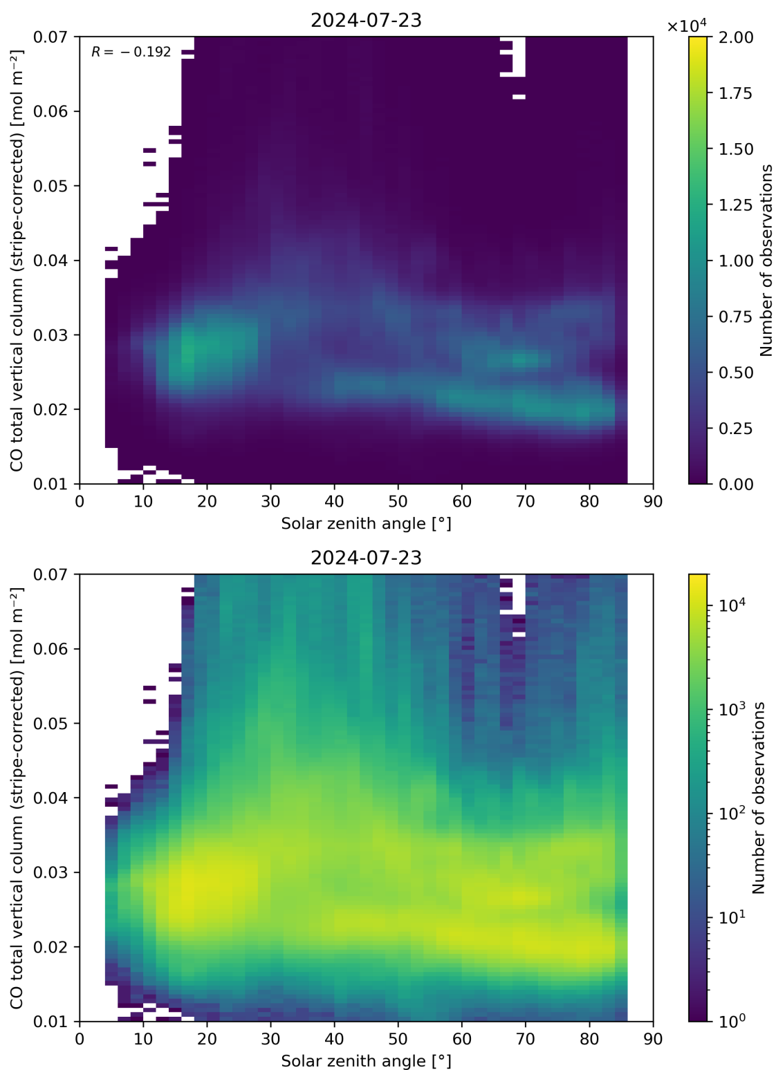
Figure 62: Scatter density plot of “Solar zenith angle” against “CO total vertical column (stripe-corrected)” for 2024-07-22 to 2024-07-24.
