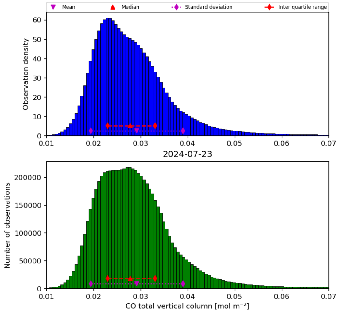
Figure 18: Histogram of “CO total vertical column” for 2024-07-22 to 2024-07-24
