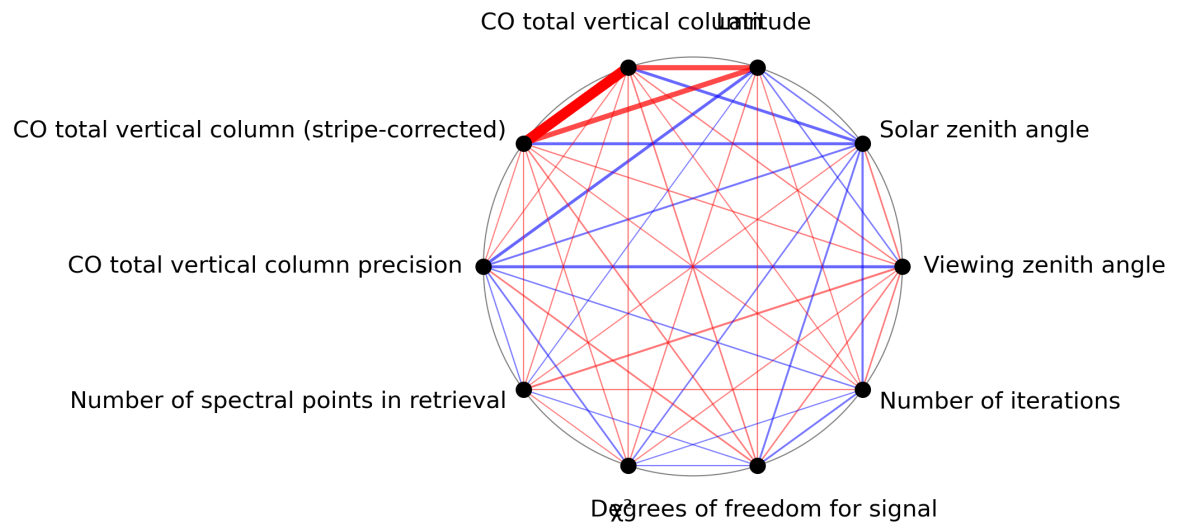
Figure 1: Map of correlation graph for 2024-07-22 to 2024-07-24.
