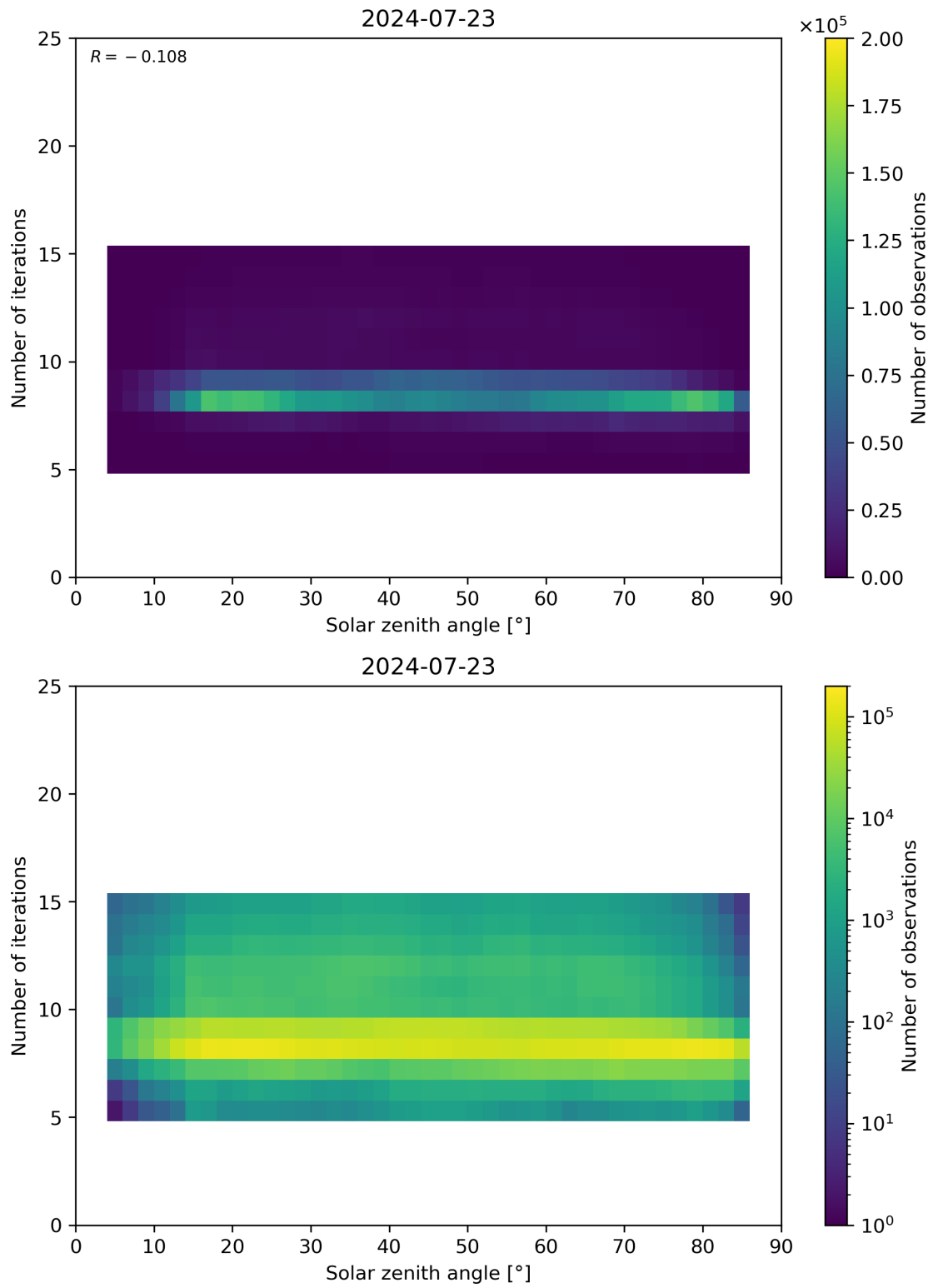
Figure 67: Scatter density plot of “Solar zenith angle” against “Number of iterations” for 2024-07-22 to 2024-07-24.
