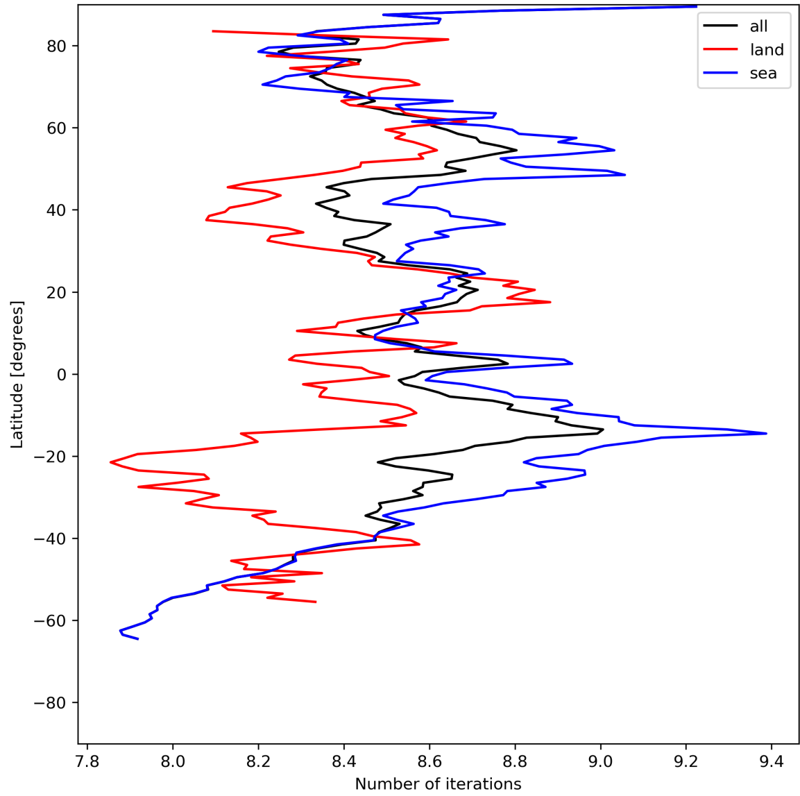
Figure 16: Zonal average of “Number of iterations” for 2024-07-22 to 2024-07-24.
