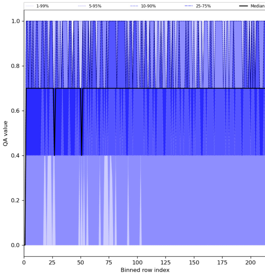
Figure 25: Along track statistics of “QA value” for 2024-07-22 to 2024-07-24
