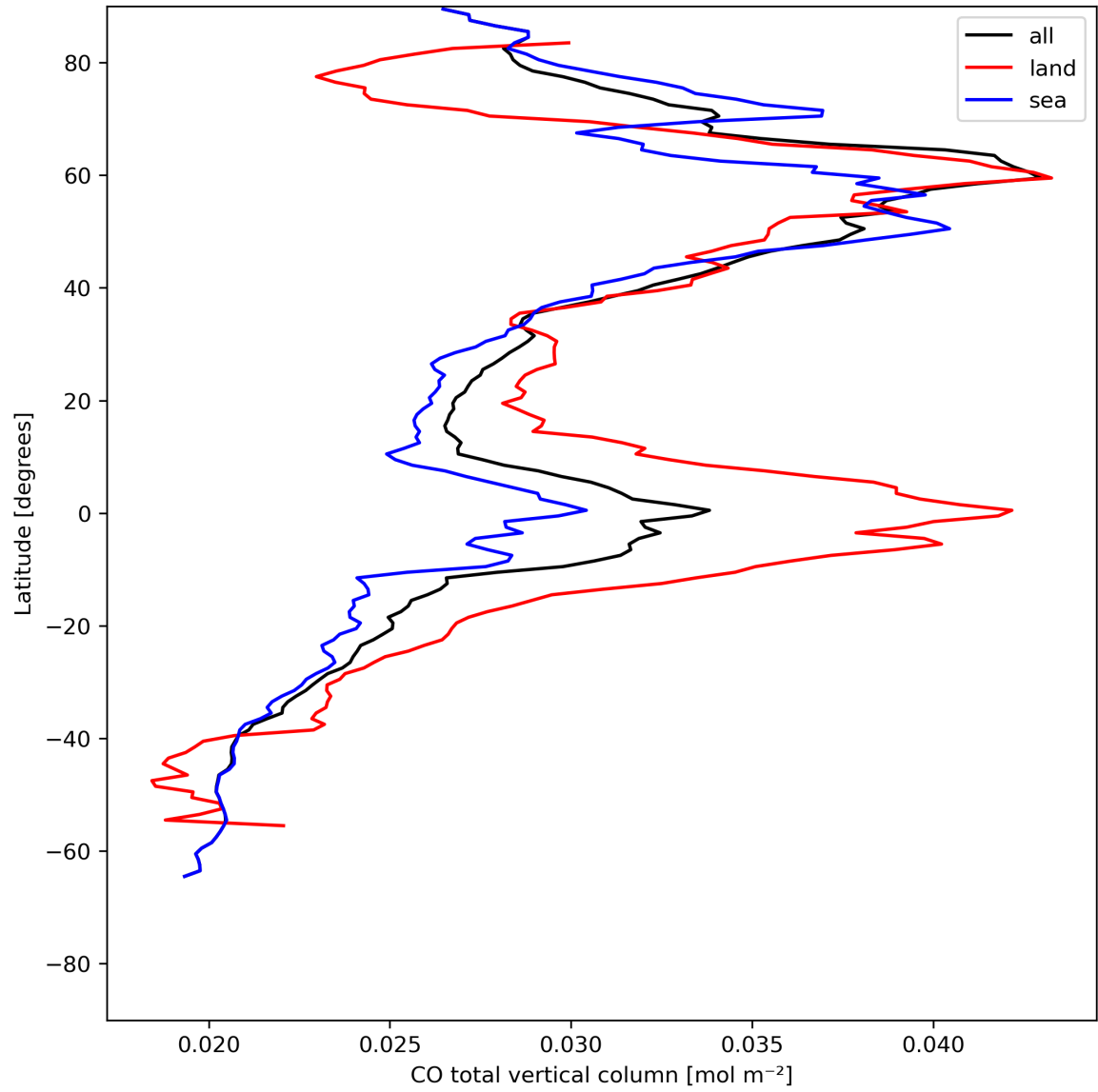
Figure 10: Zonal average of “CO total vertical column” for 2024-07-22 to 2024-07-24.
