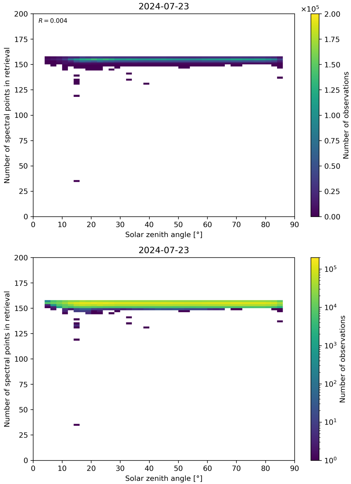
Figure 68: Scatter density plot of “Solar zenith angle” against “Number of spectral points in retrieval” for 2024-07-22 to 2024-07-24.
