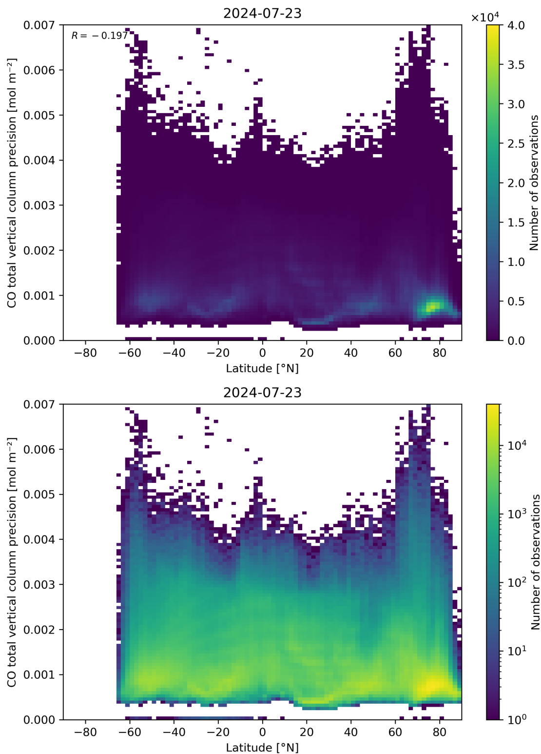
Figure 53: Scatter density plot of “Latitude” against “CO total vertical column precision” for 2024-07-22 to 2024-07-24.
