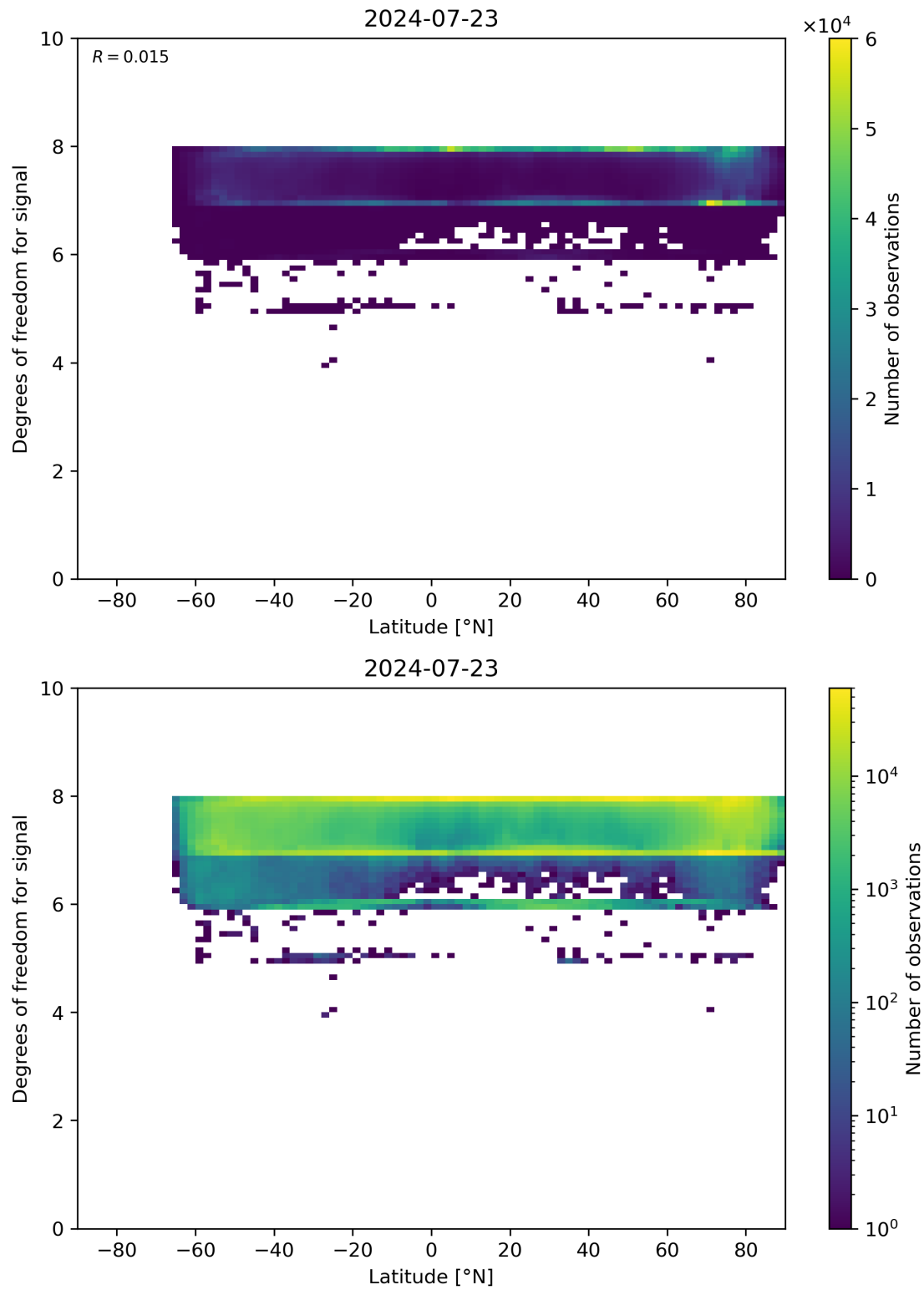
Figure 55: Scatter density plot of “Latitude” against “Degrees of freedom for signal” for 2024-07-22 to 2024-07-24.
