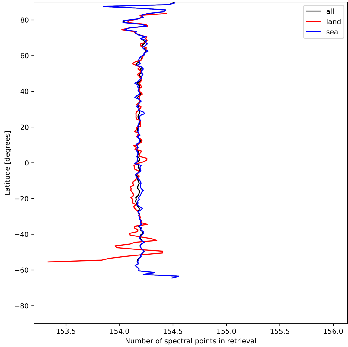
Figure 13: Zonal average of “Number of spectral points in retrieval” for 2024-07-22 to 2024-07-24.
