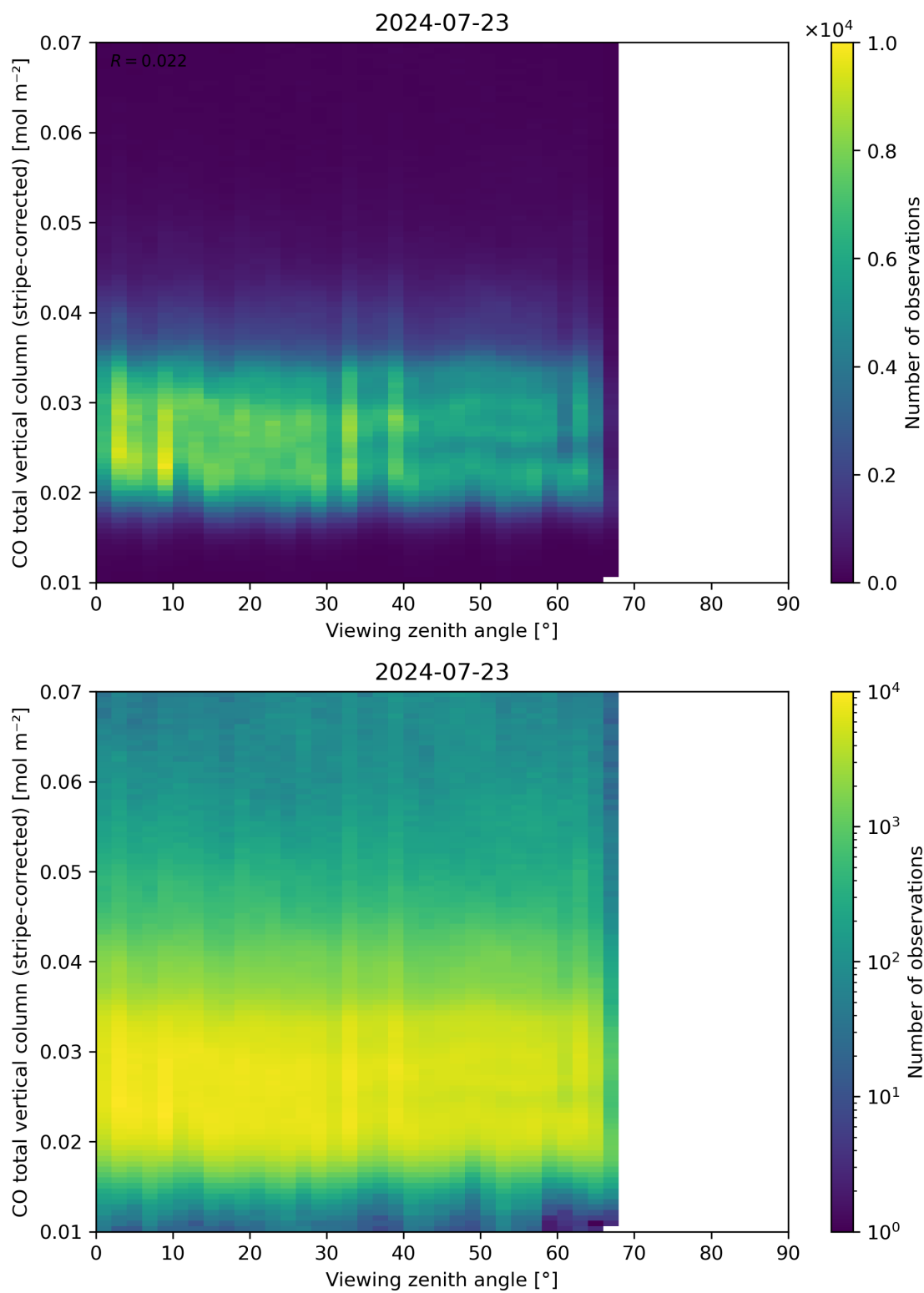
Figure 70: Scatter density plot of “Viewing zenith angle” against “CO total vertical column (stripe-corrected)” for 2024-07-22 to 2024-07-24.
