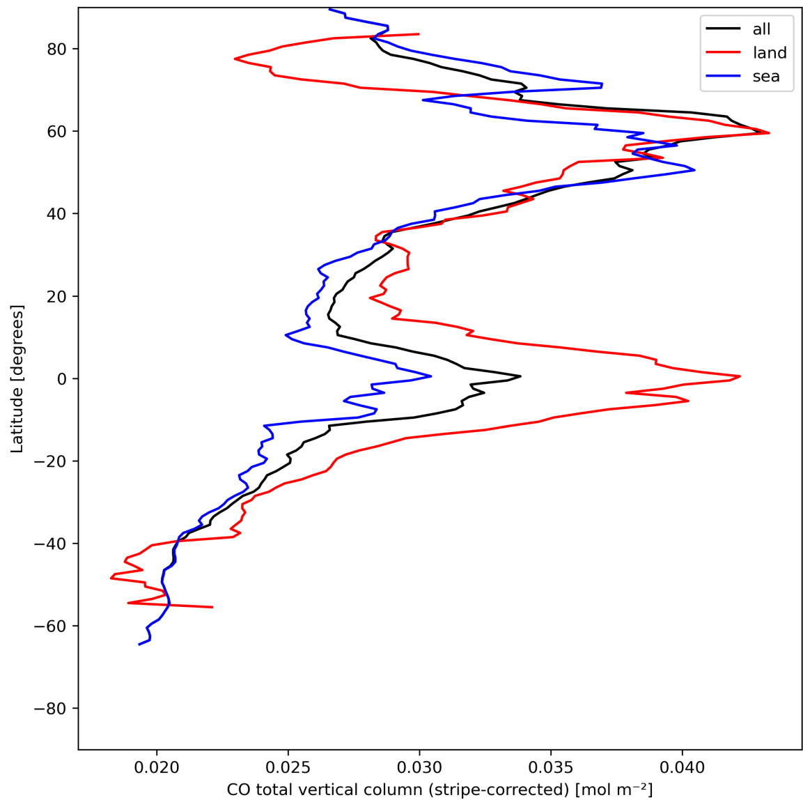
Figure 11: Zonal average of “CO total vertical column (stripe-corrected)” for 2024-07-22 to 2024-07-24.
