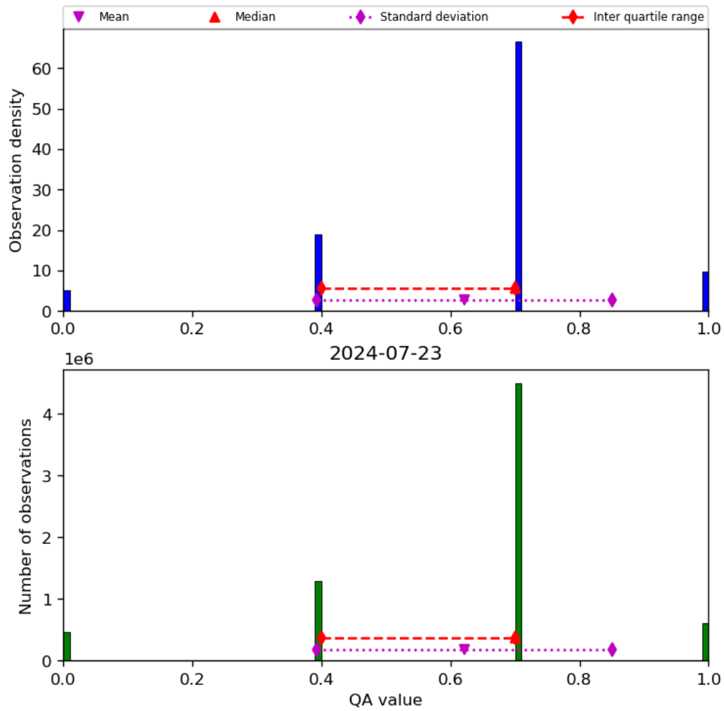
Figure 17: Histogram of “QA value” for 2024-07-22 to 2024-07-24
