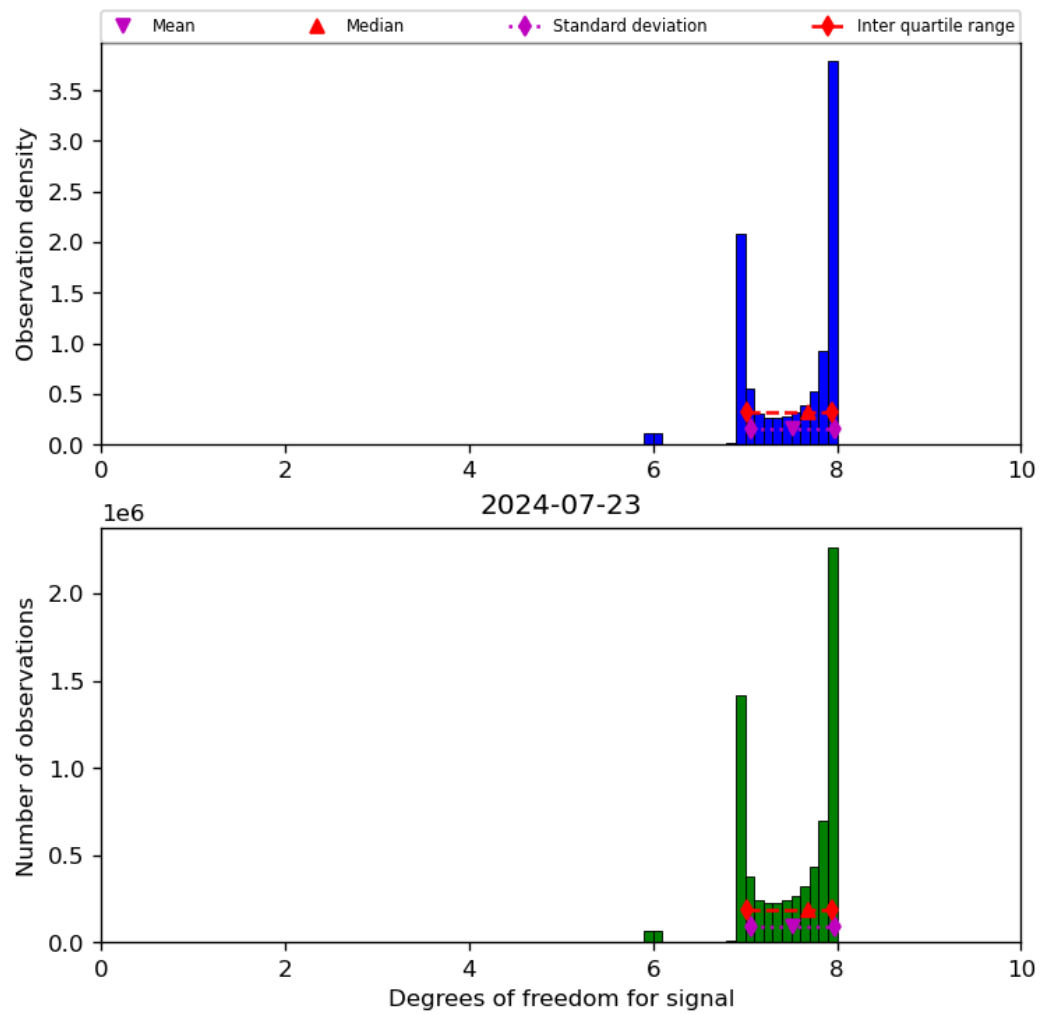
Figure 23: Histogram of “Degrees of freedom for signal” for 2024-07-22 to 2024-07-24
