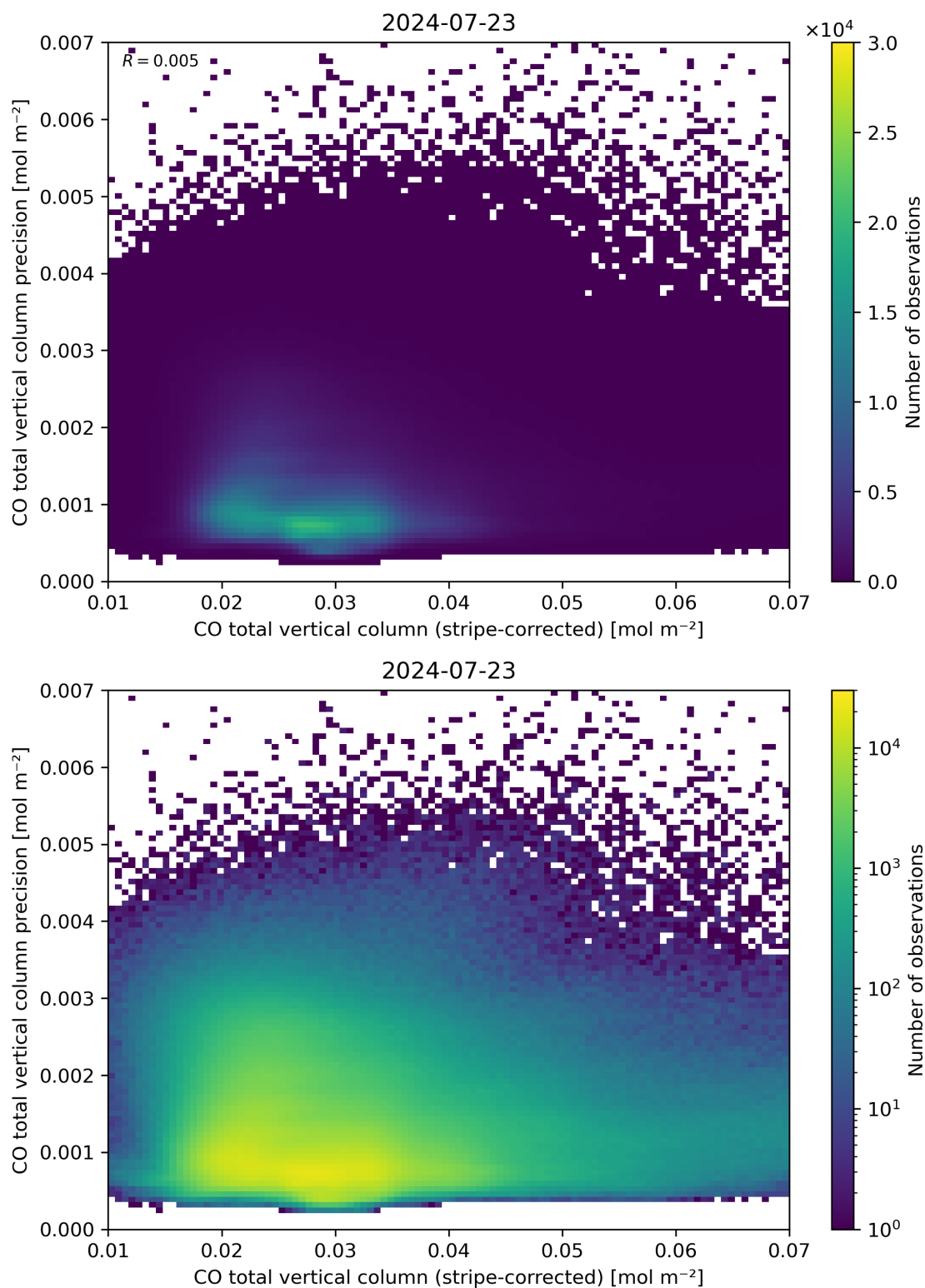
Figure 36: Scatter density plot of “CO total vertical column (stripe-corrected)” against “CO total vertical column precision” for 2024-07-22 to 2024-07-24.
