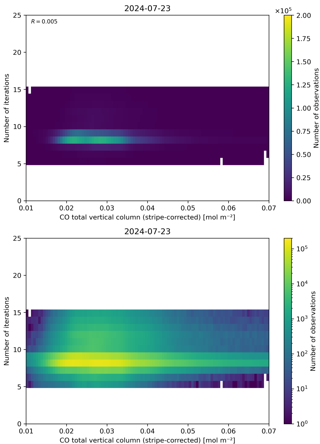
Figure 39: Scatter density plot of “CO total vertical column (stripe-corrected)” against “Number of iterations” for 2024-07-22 to 2024-07-24.
