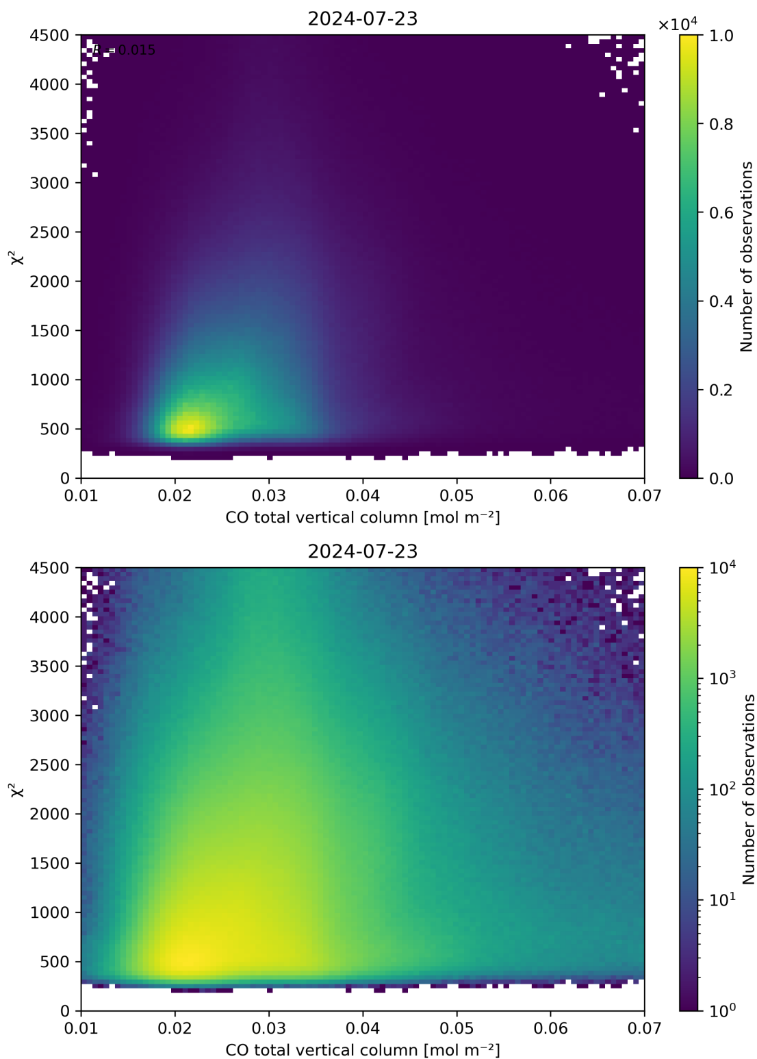
Figure 35: Scatter density plot of “CO total vertical column” against “ \chi^2 ” for 2024-07-22 to 2024-07-24.
