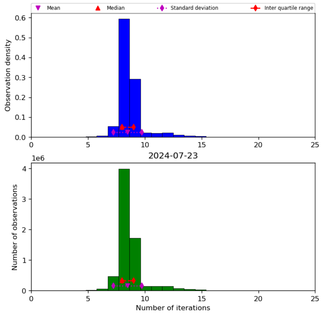
Figure 24: Histogram of “Number of iterations” for 2024-07-22 to 2024-07-24
