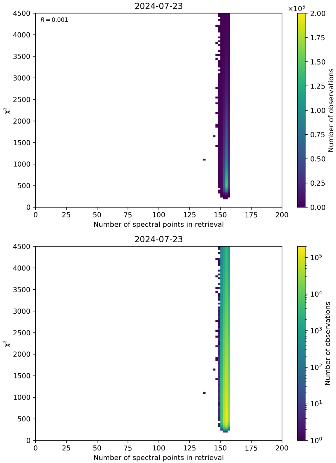
Figure 58: Scatter density plot of “Number of spectral points in retrieval” against “ \chi^2 ” for 2024-07-22 to 2024-07-24.
