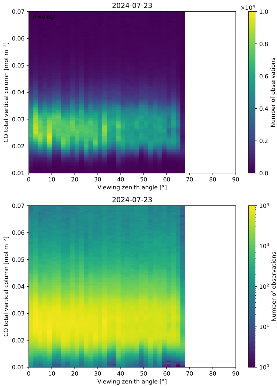
Figure 69: Scatter density plot of “Viewing zenith angle” against “CO total vertical column” for 2024-07-22 to 2024-07-24.
