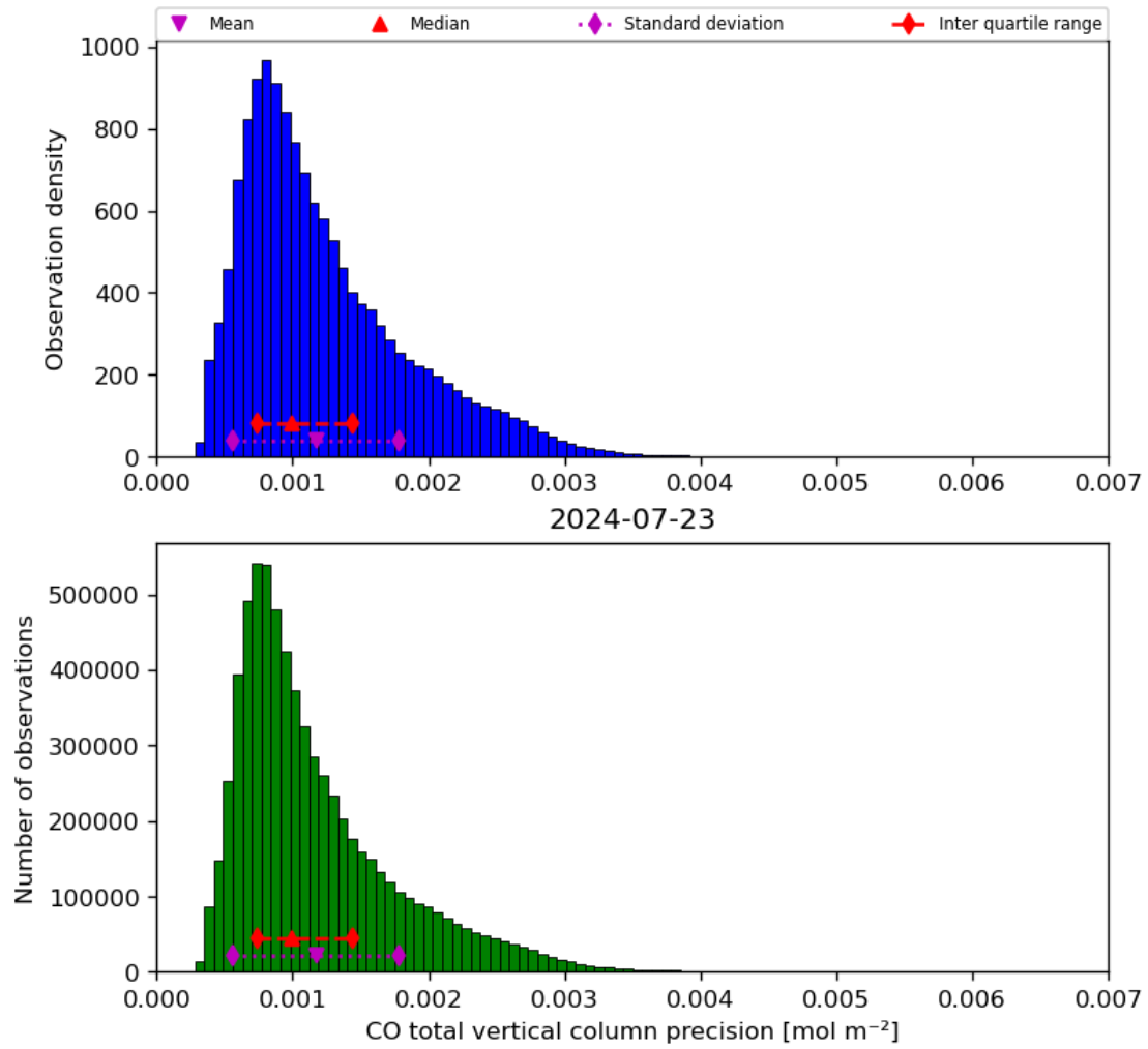
Figure 20: Histogram of “CO total vertical column precision” for 2024-07-22 to 2024-07-24
