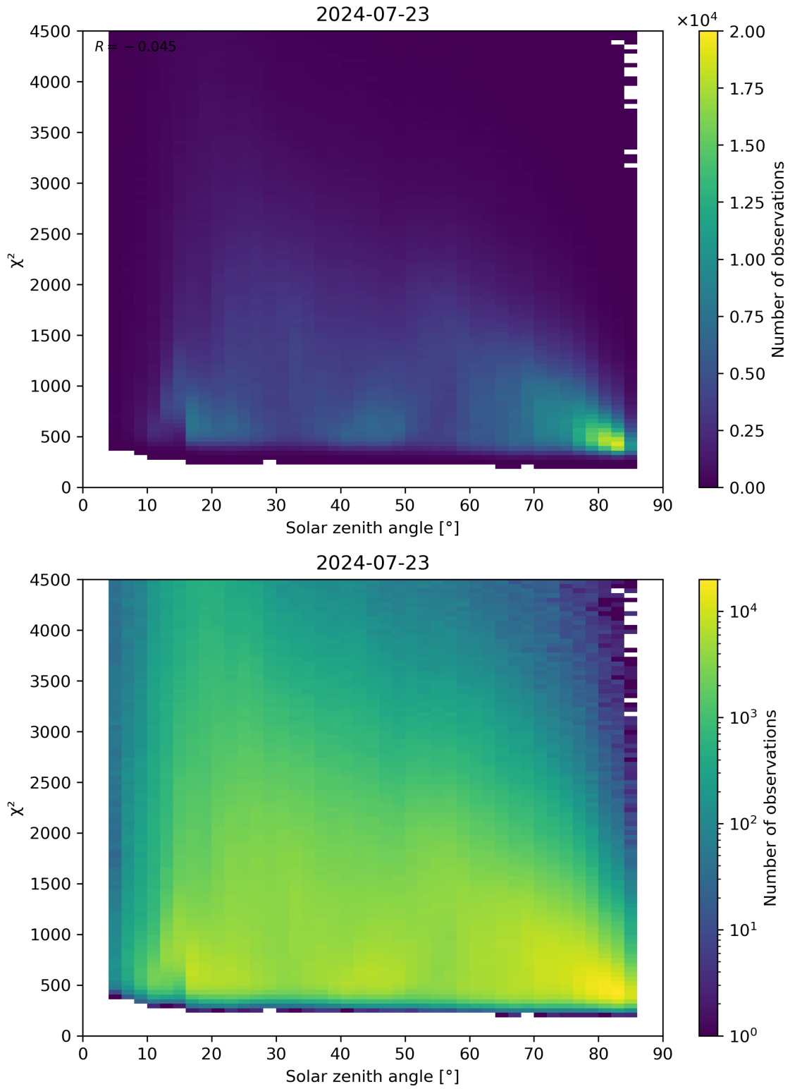
Figure 64: Scatter density plot of “Solar zenith angle” against “ \chi^2 ” for 2024-07-22 to 2024-07-24.
