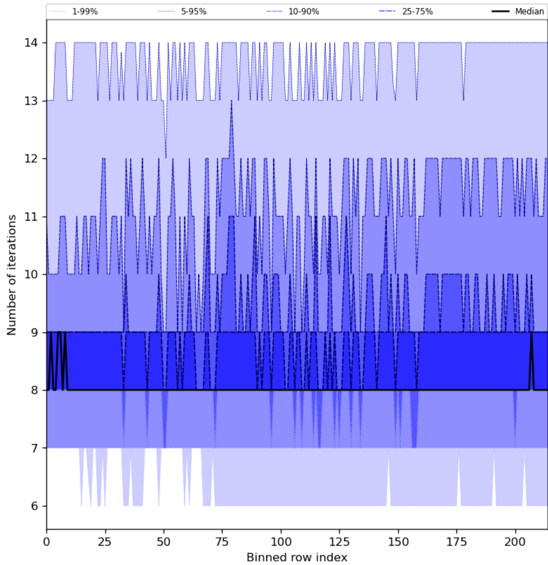
Figure 32: Along track statistics of “Number of iterations” for 2024-07-22 to 2024-07-24
