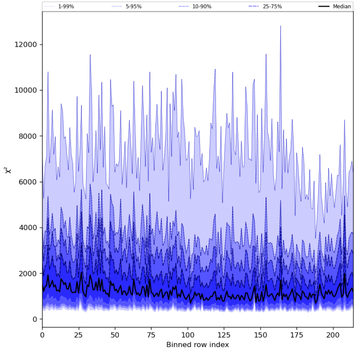
Figure 30: Along track statistics of “ \chi^2 ” for 2024-07-22 to 2024-07-24
