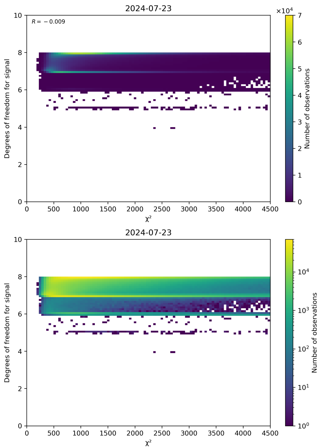
Figure 48: Scatter density plot of “ \chi^2 ” against “Degrees of freedom for signal” for 2024-07-22 to 2024-07-24.
