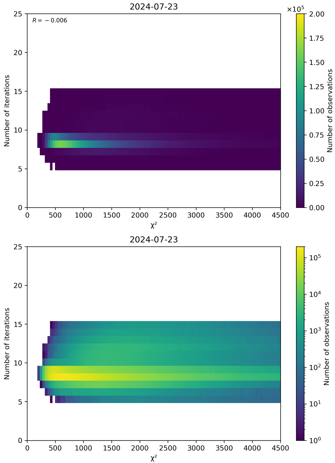
Figure 49: Scatter density plot of “ \chi^2 ” against “Number of iterations” for 2024-07-22 to 2024-07-24.
