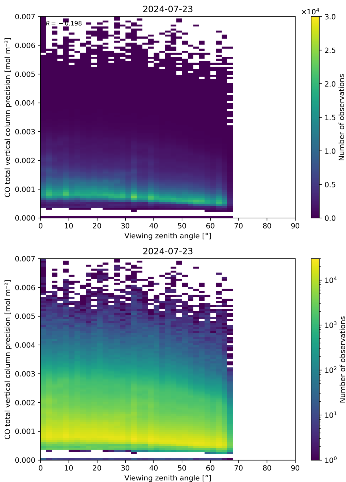
Figure 71: Scatter density plot of “Viewing zenith angle” against “CO total vertical column precision” for 2024-07-22 to 2024-07-24.
