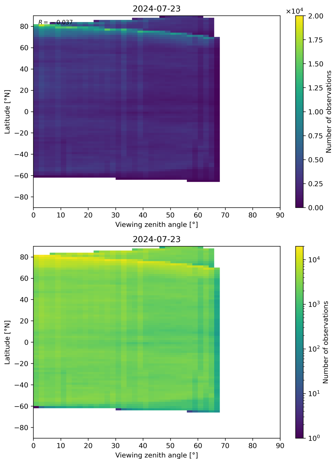
Figure 74: Scatter density plot of “Viewing zenith angle” against “Latitude” for 2024-07-22 to 2024-07-24.
