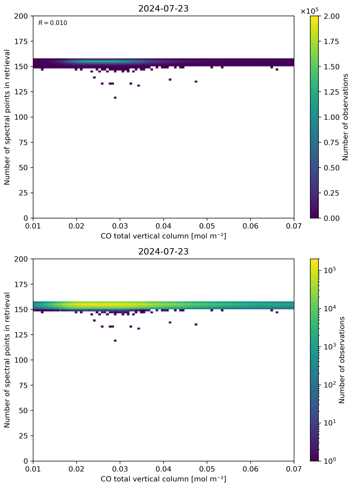
Figure 43: Scatter density plot of “CO total vertical column” against “Number of spectral points in retrieval” for 2024-07-22 to 2024-07-24.
