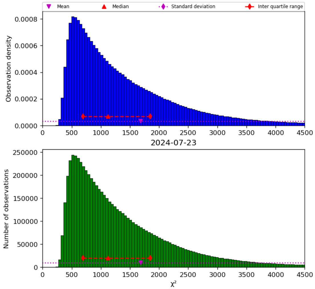
Figure 22: Histogram of “ \chi^2 ” for 2024-07-22 to 2024-07-24
