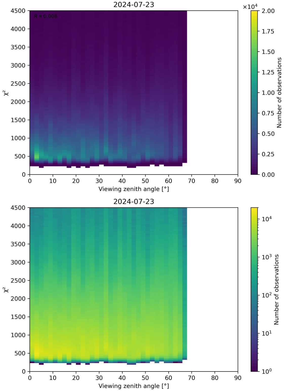
Figure 72: Scatter density plot of “Viewing zenith angle” against “ \chi^2 ” for 2024-07-22 to 2024-07-24.
