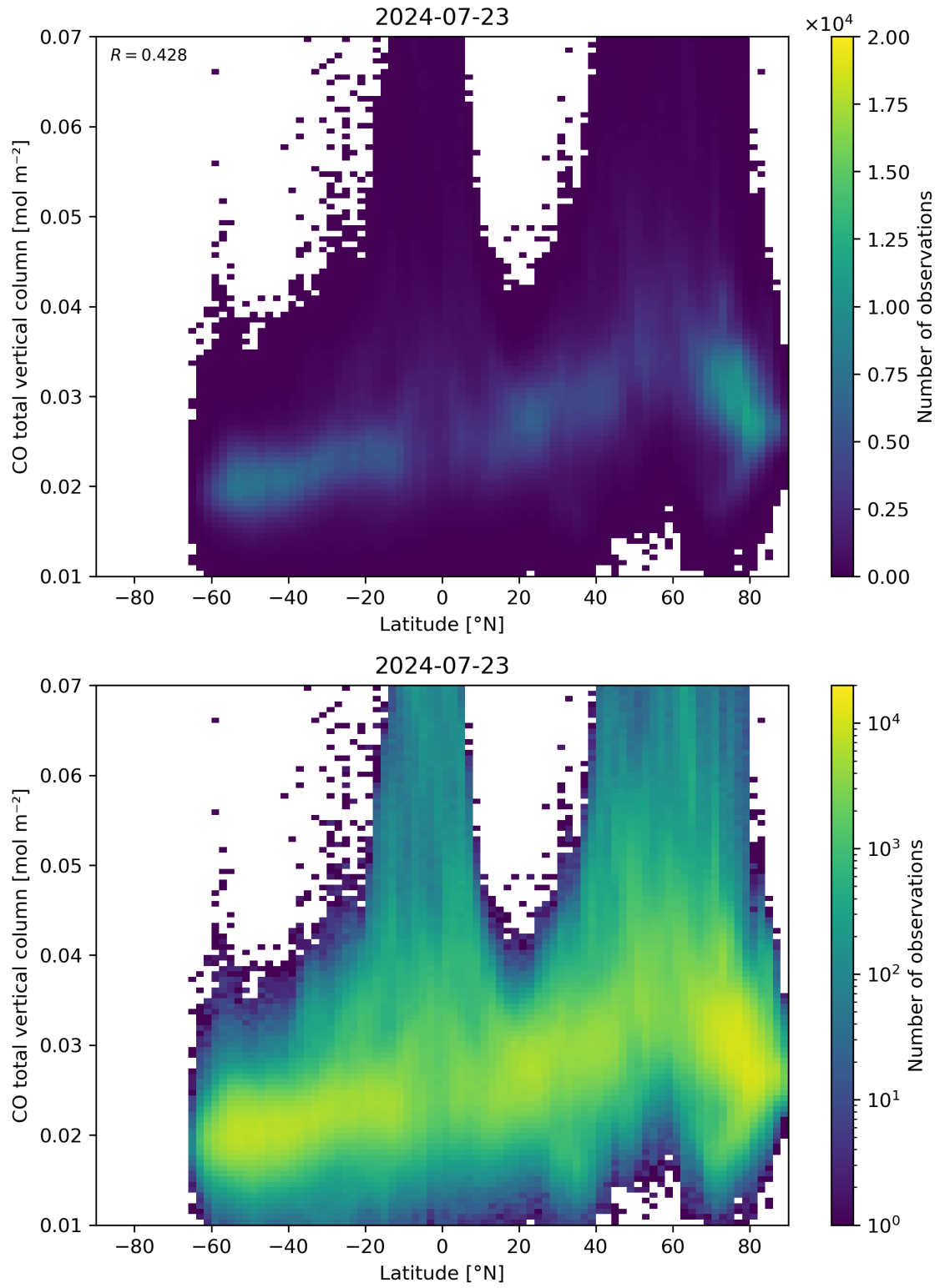
Figure 51: Scatter density plot of “Latitude” against “CO total vertical column” for 2024-07-22 to 2024-07-24.
