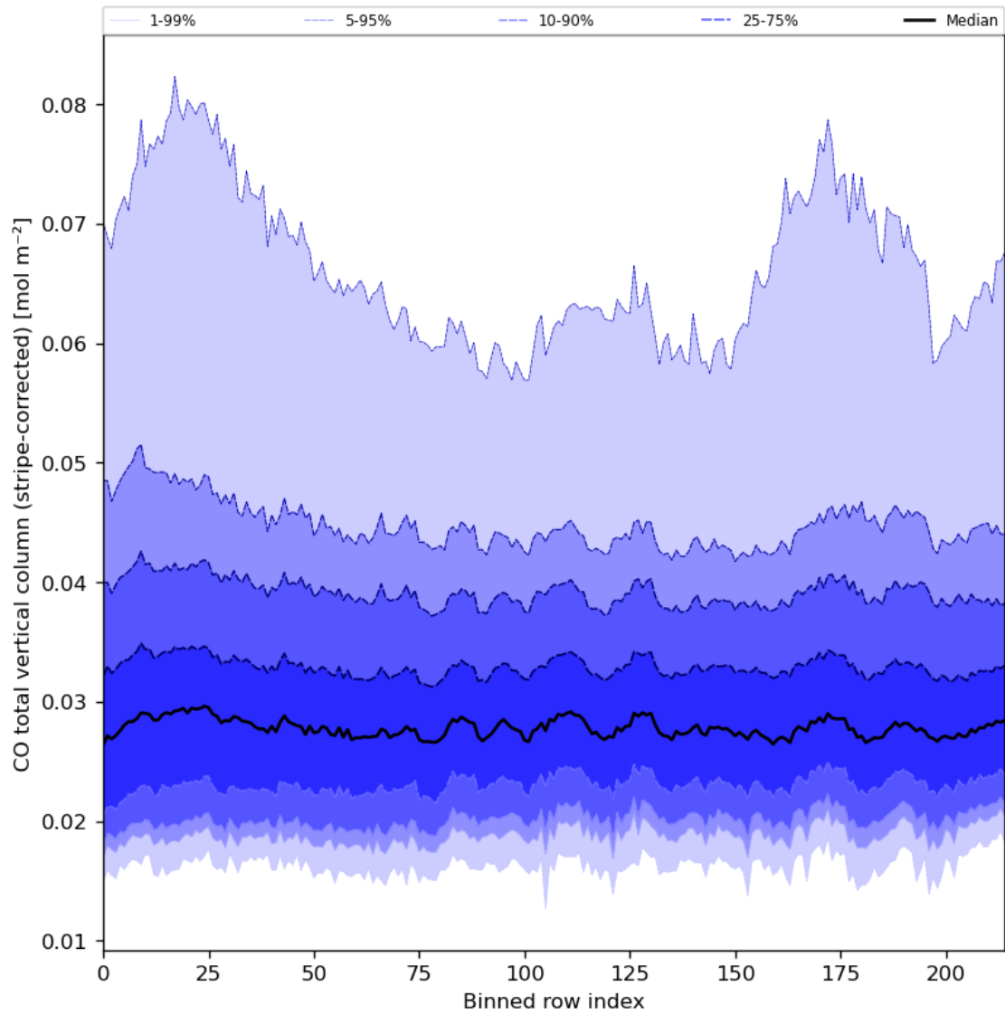
Figure 27: Along track statistics of “CO total vertical column (stripe-corrected)” for 2024-07-22 to 2024-07-24
