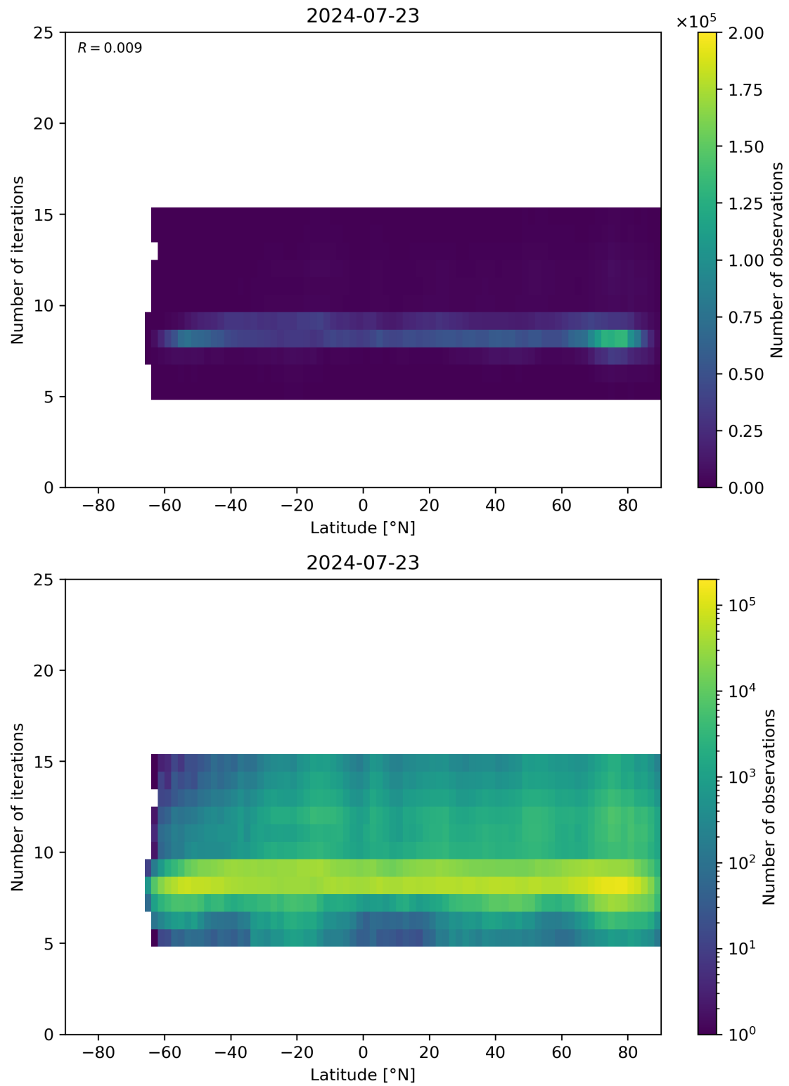
Figure 56: Scatter density plot of “Latitude” against “Number of iterations” for 2024-07-22 to 2024-07-24.
