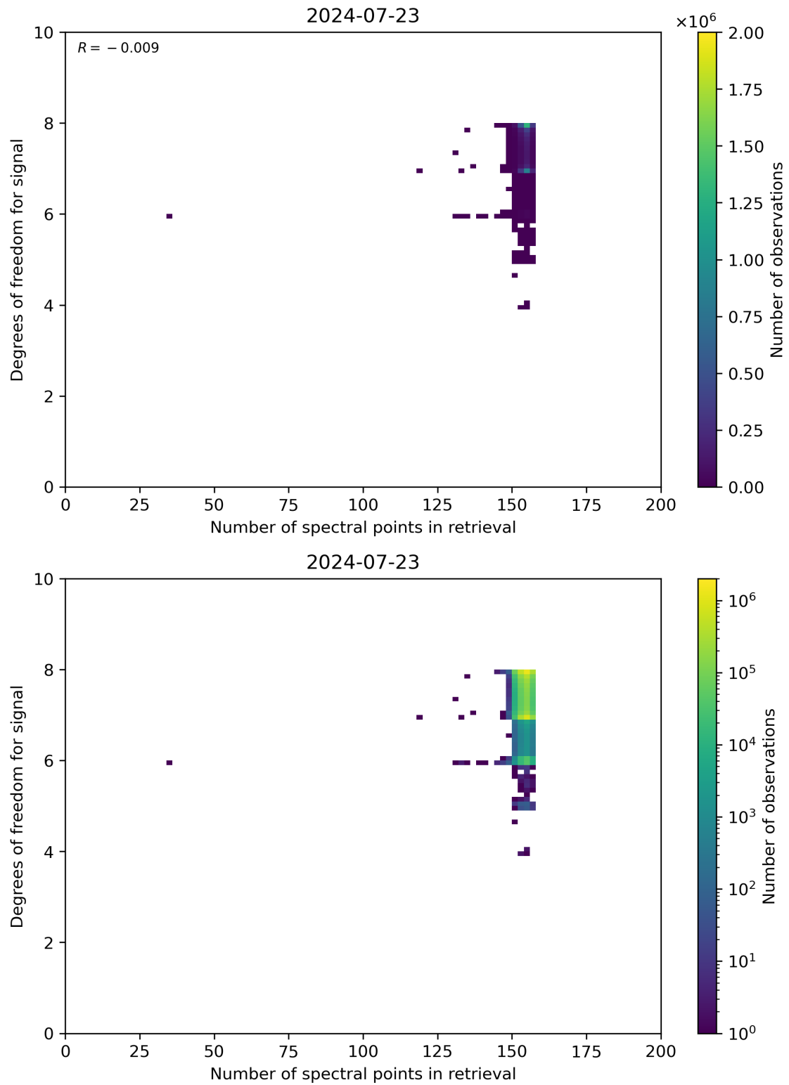
Figure 59: Scatter density plot of “Number of spectral points in retrieval” against “Degrees of freedom for signal” for 2024-07-22 to 2024-07-24.
