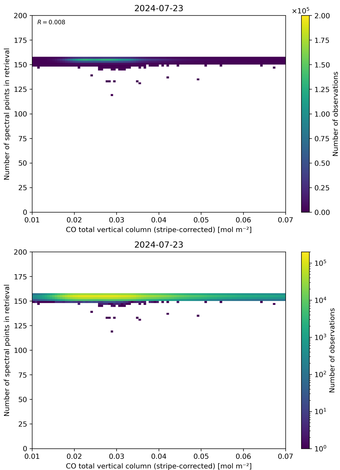
Figure 40: Scatter density plot of “CO total vertical column (stripe-corrected)” against “Number of spectral points in retrieval” for 2024-07-22 to 2024-07-24.
