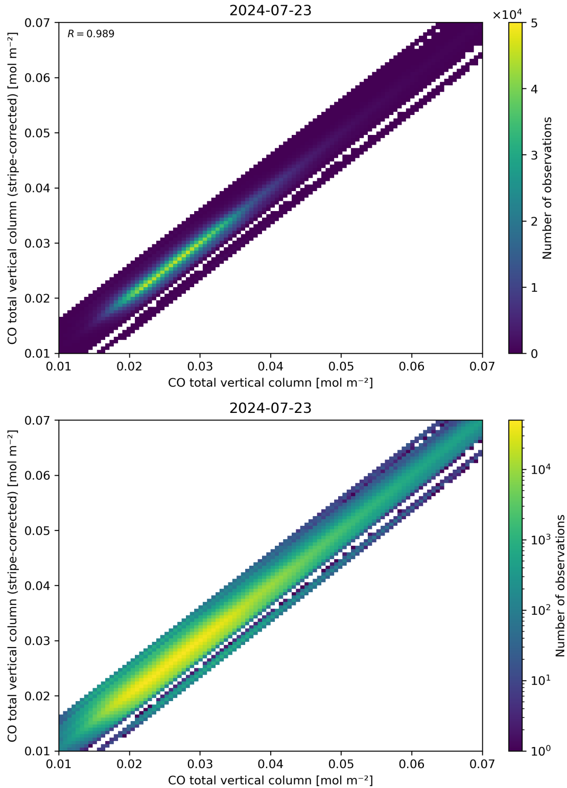
Figure 33: Scatter density plot of “CO total vertical column” against “CO total vertical column (stripe-corrected)” for 2024-07-22 to 2024-07-24.
