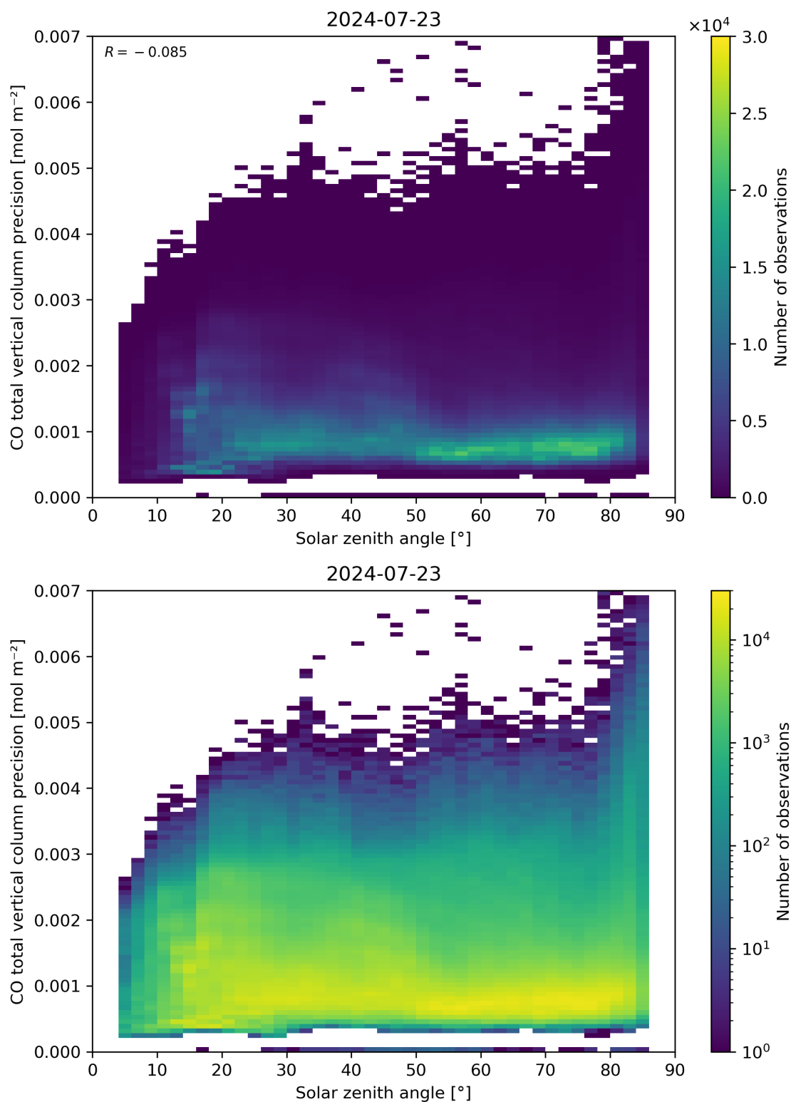
Figure 63: Scatter density plot of “Solar zenith angle” against “CO total vertical column precision” for 2024-07-22 to 2024-07-24.
