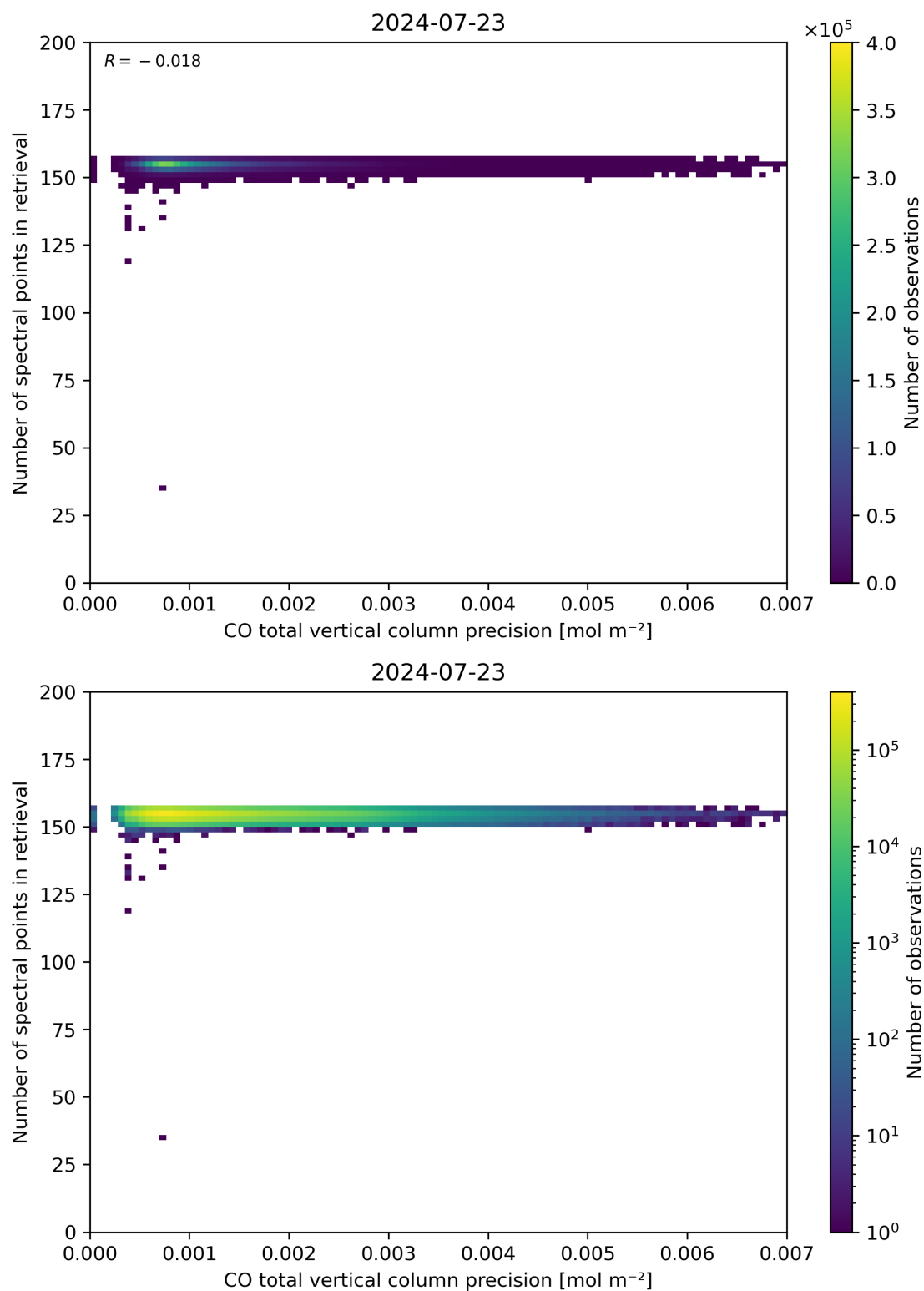
Figure 47: Scatter density plot of “CO total vertical column precision” against “Number of spectral points in retrieval” for 2024-07-22 to 2024-07-24.
