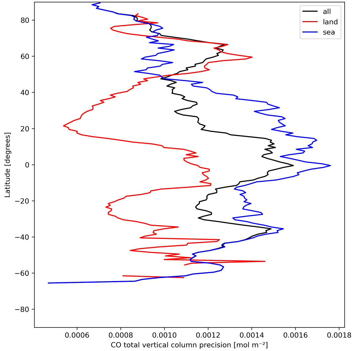
Figure 12: Zonal average of “CO total vertical column precision” for 2024-07-23 to 2024-07-25.
