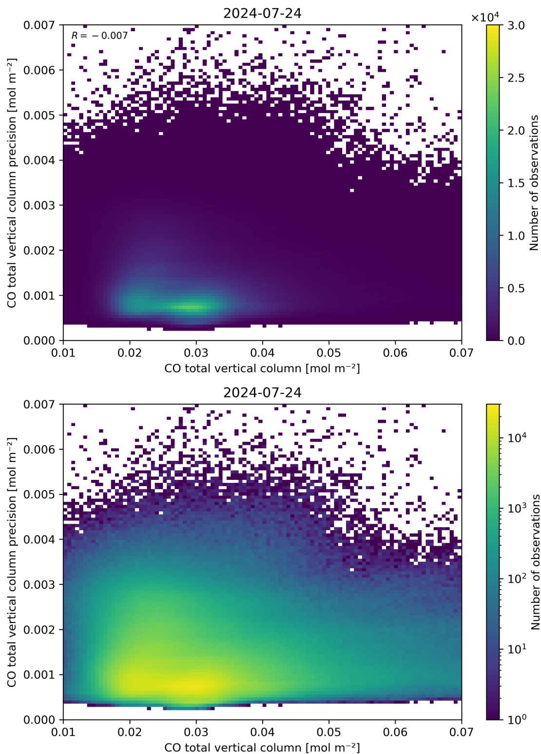
Figure 34: Scatter density plot of “CO total vertical column” against “CO total vertical column precision” for 2024-07-23 to 2024-07-25.
