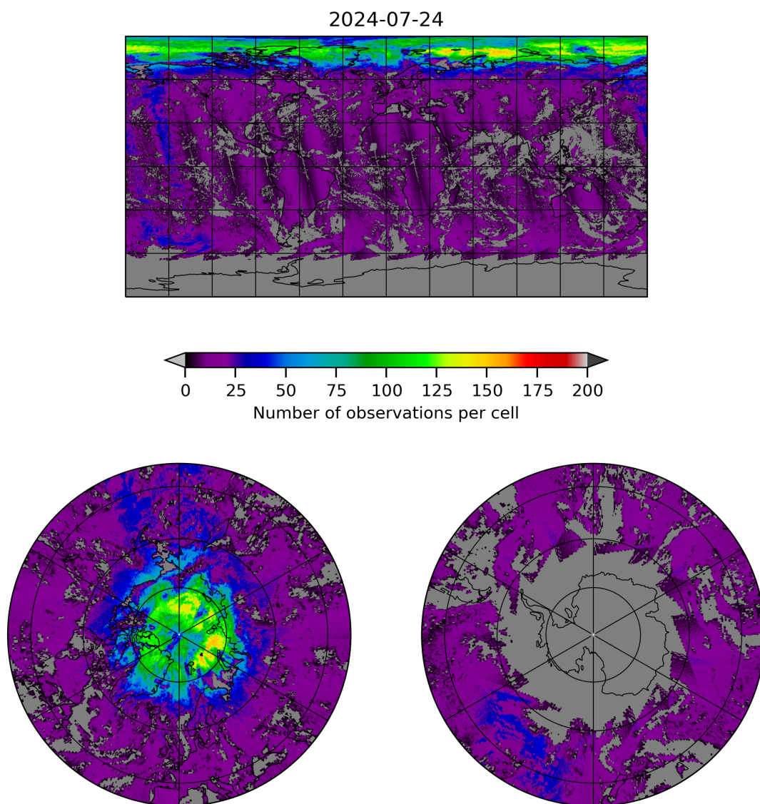
Figure 8: Map of the number of observations for 2024-07-23 to 2024-07-25
