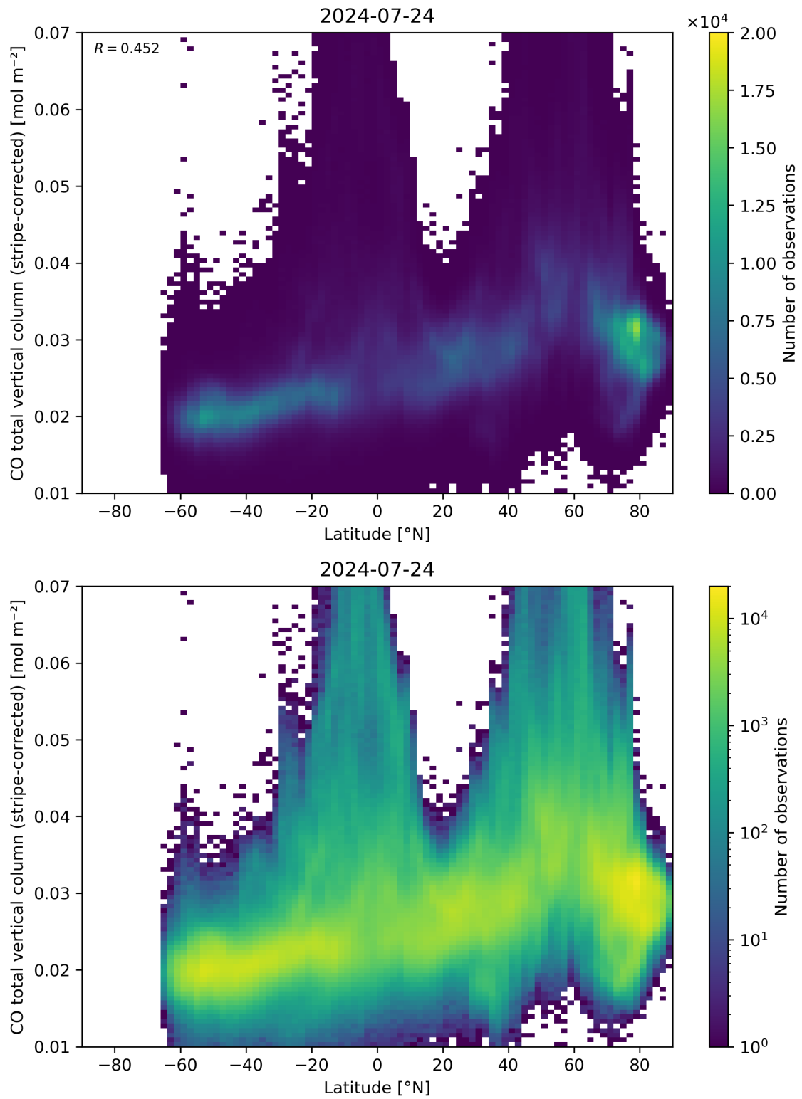
Figure 52: Scatter density plot of “Latitude” against “CO total vertical column (stripe-corrected)” for 2024-07-23 to 2024-07-25.
