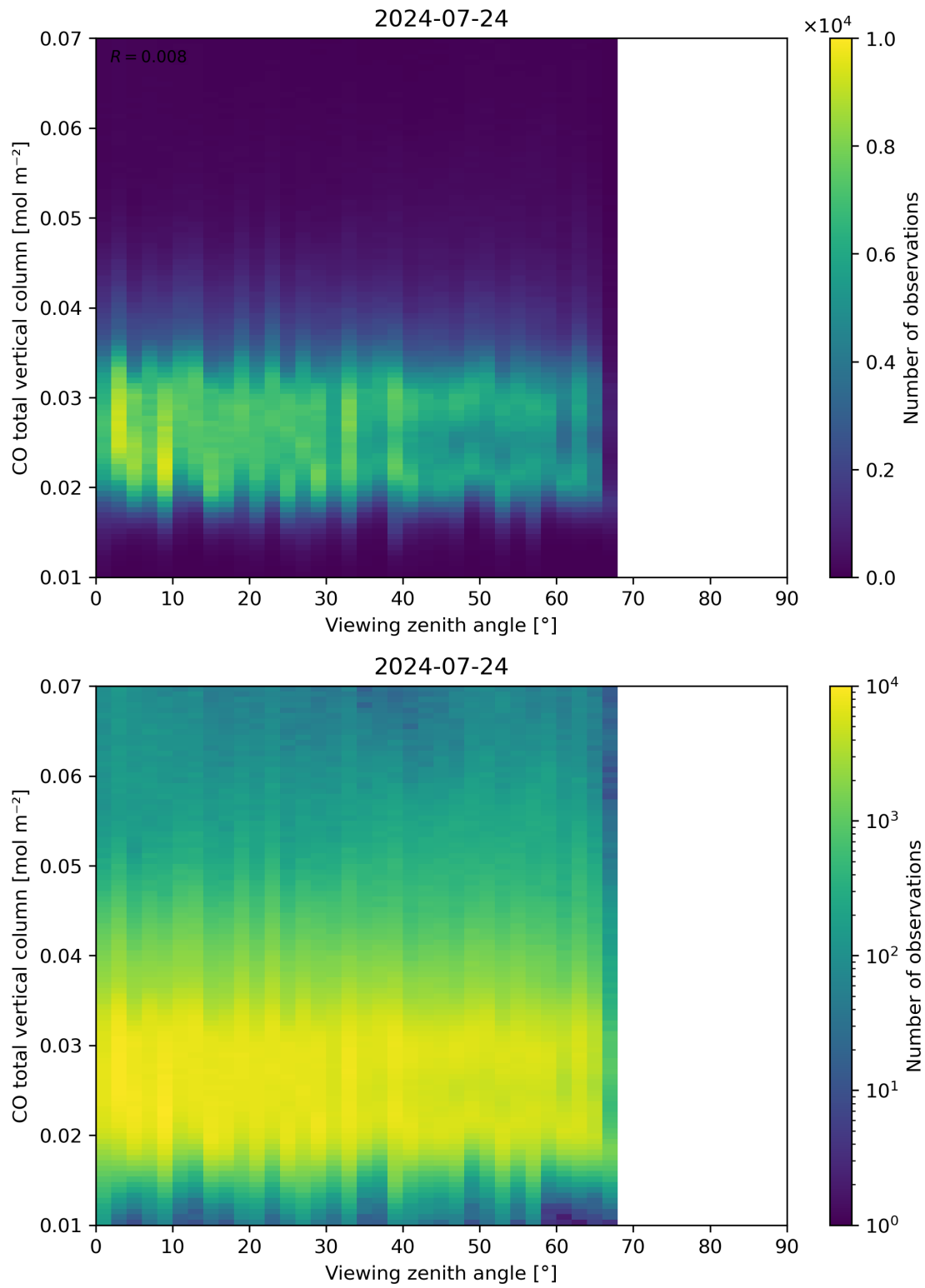
Figure 69: Scatter density plot of “Viewing zenith angle” against “CO total vertical column” for 2024-07-23 to 2024-07-25.
