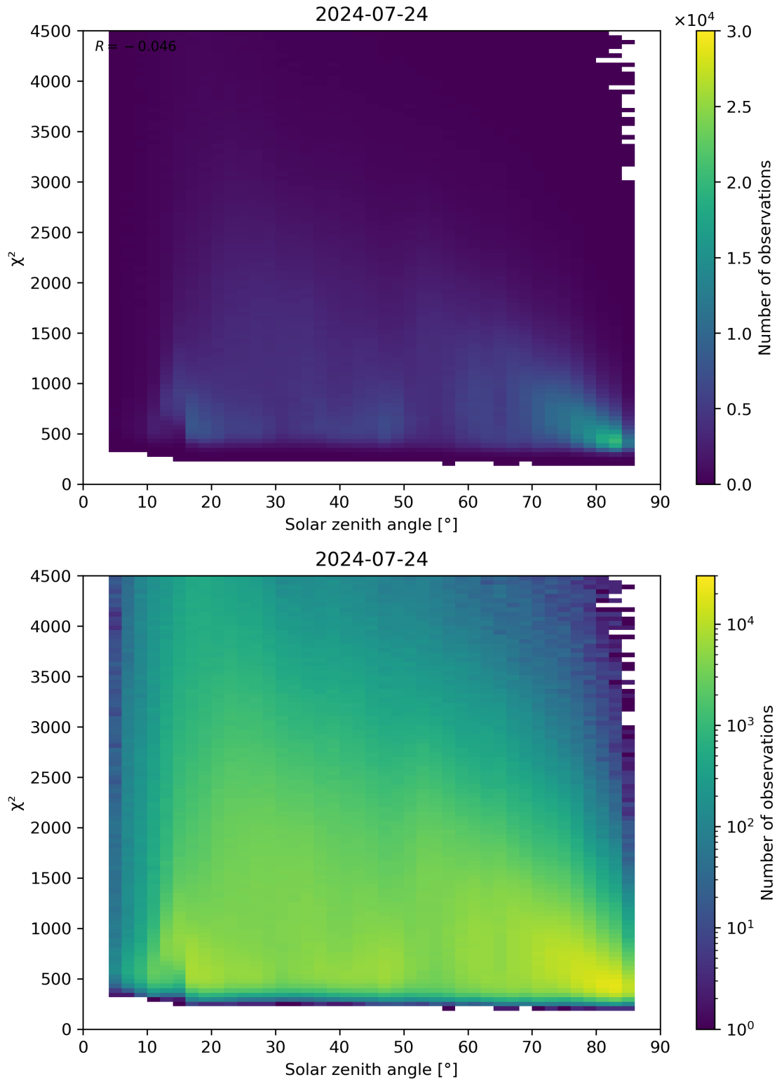
Figure 64: Scatter density plot of “Solar zenith angle” against “ \chi^2 ” for 2024-07-23 to 2024-07-25.
