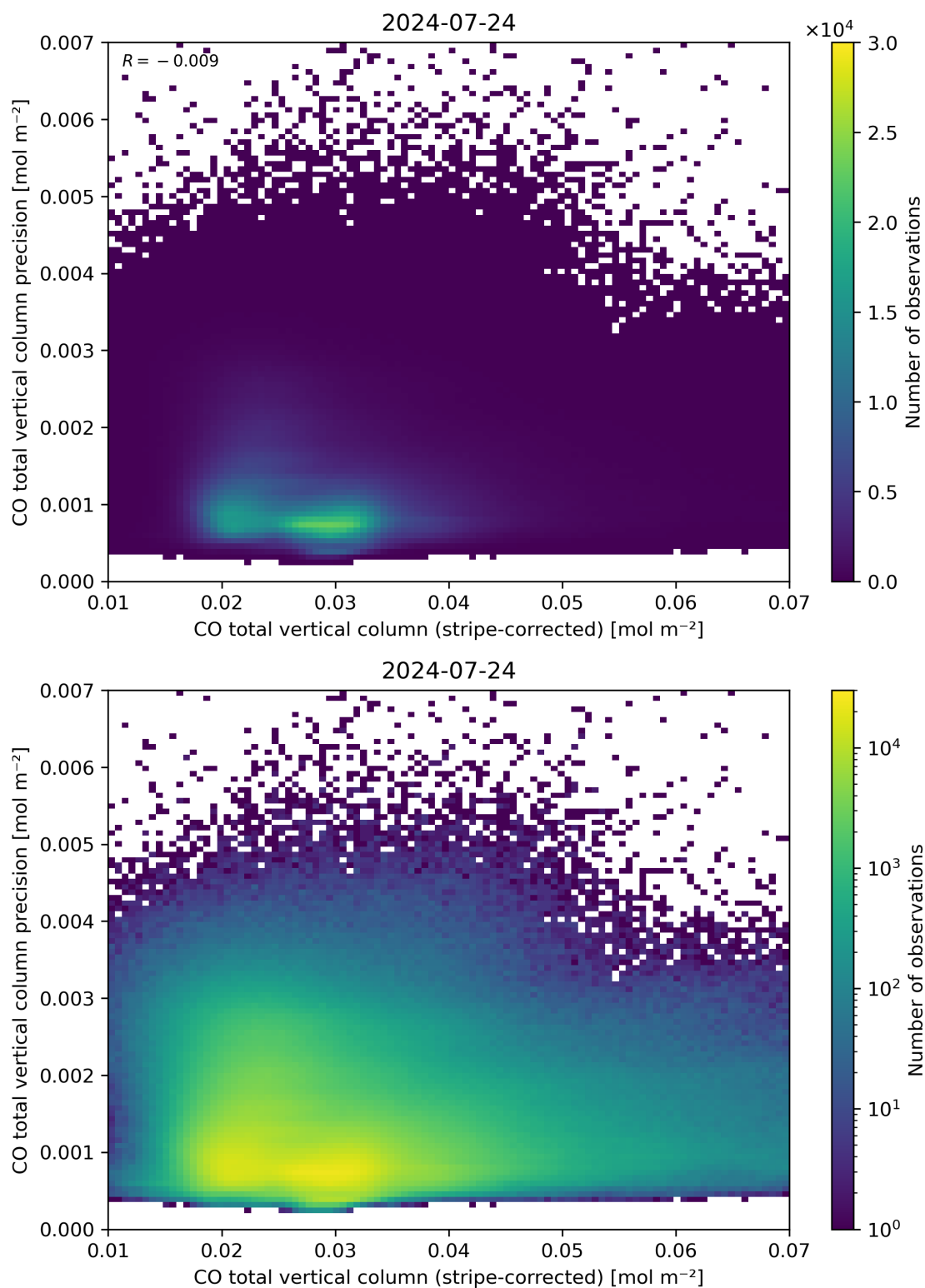
Figure 36: Scatter density plot of “CO total vertical column (stripe-corrected)” against “CO total vertical column precision” for 2024-07-23 to 2024-07-25.
