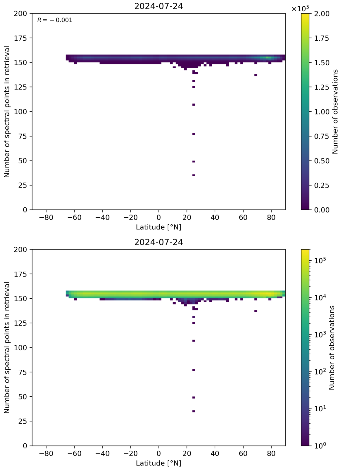
Figure 57: Scatter density plot of “Latitude” against “Number of spectral points in retrieval” for 2024-07-23 to 2024-07-25.
