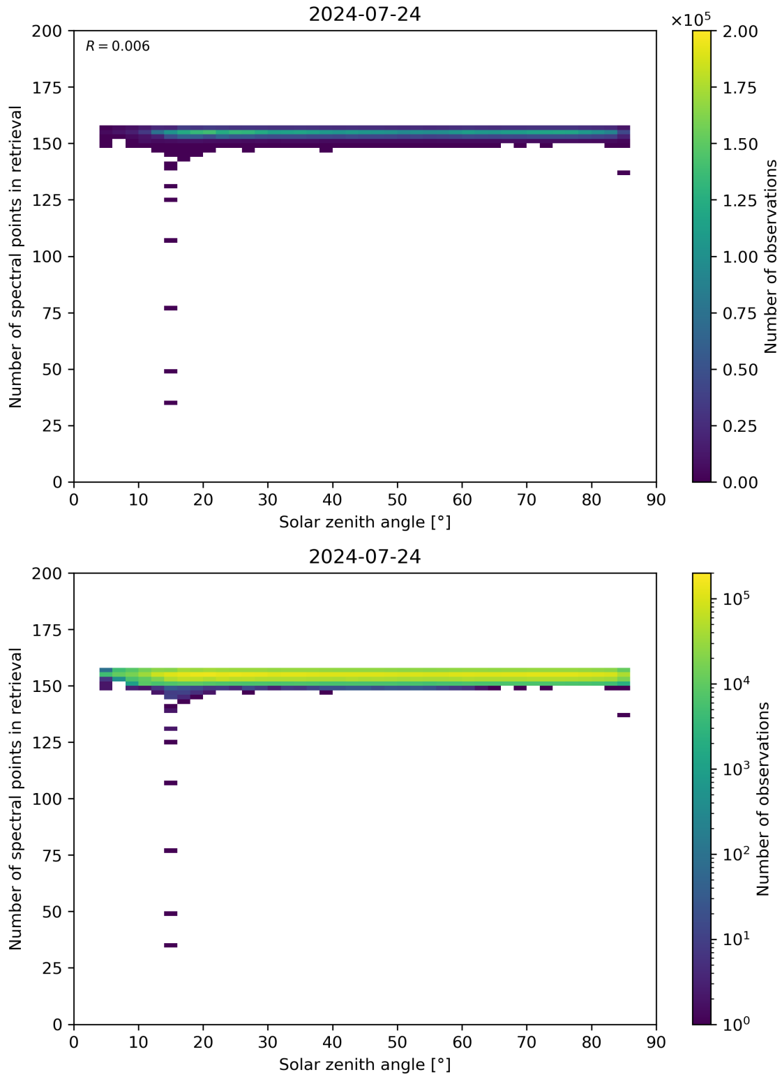
Figure 68: Scatter density plot of “Solar zenith angle” against “Number of spectral points in retrieval” for 2024-07-23 to 2024-07-25.
