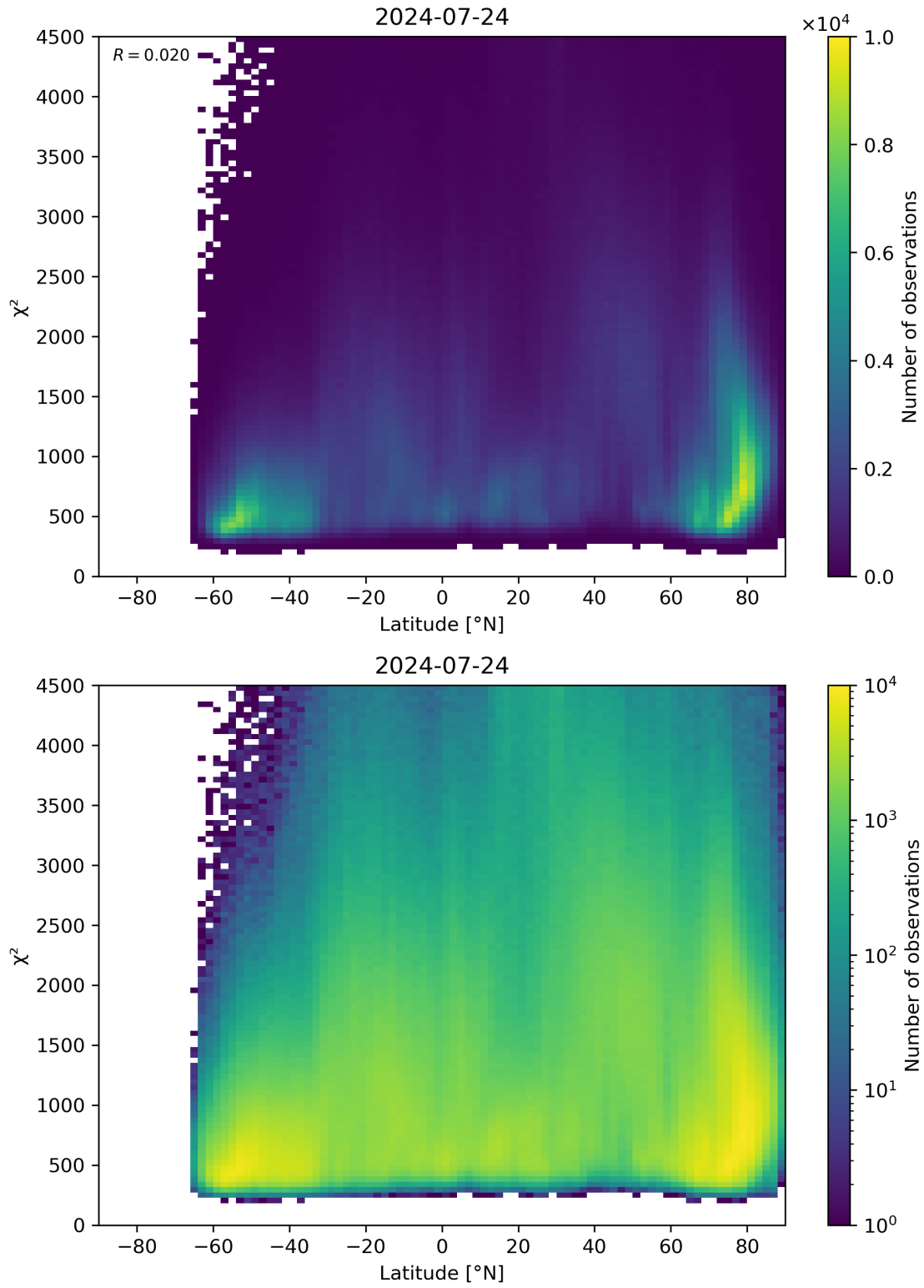
Figure 54: Scatter density plot of “Latitude” against “ \chi^2 ” for 2024-07-23 to 2024-07-25.
