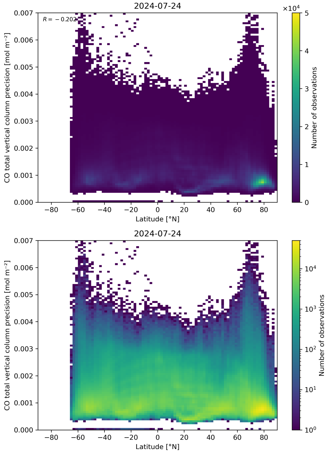
Figure 53: Scatter density plot of “Latitude” against “CO total vertical column precision” for 2024-07-23 to 2024-07-25.
