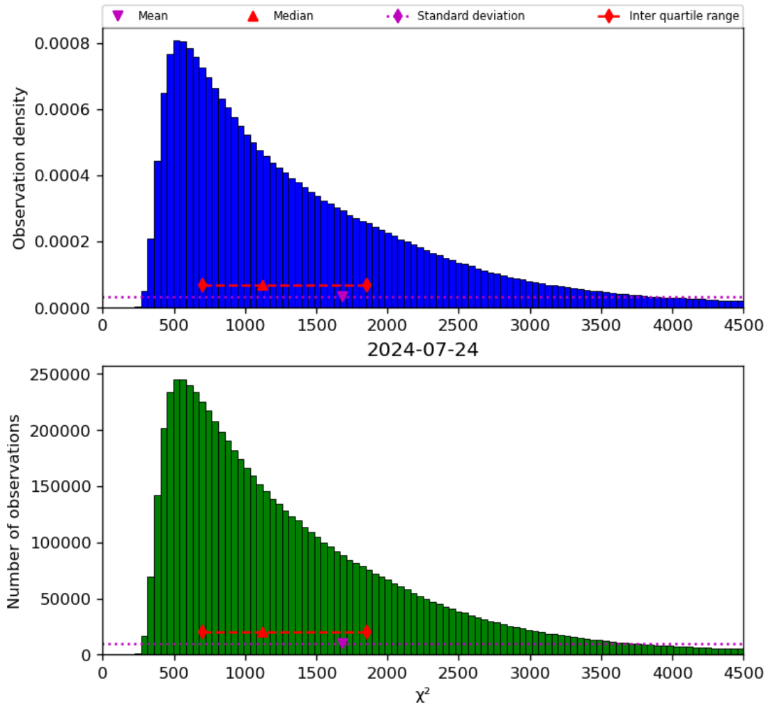
Figure 22: Histogram of “ \chi^2 ” for 2024-07-23 to 2024-07-25
