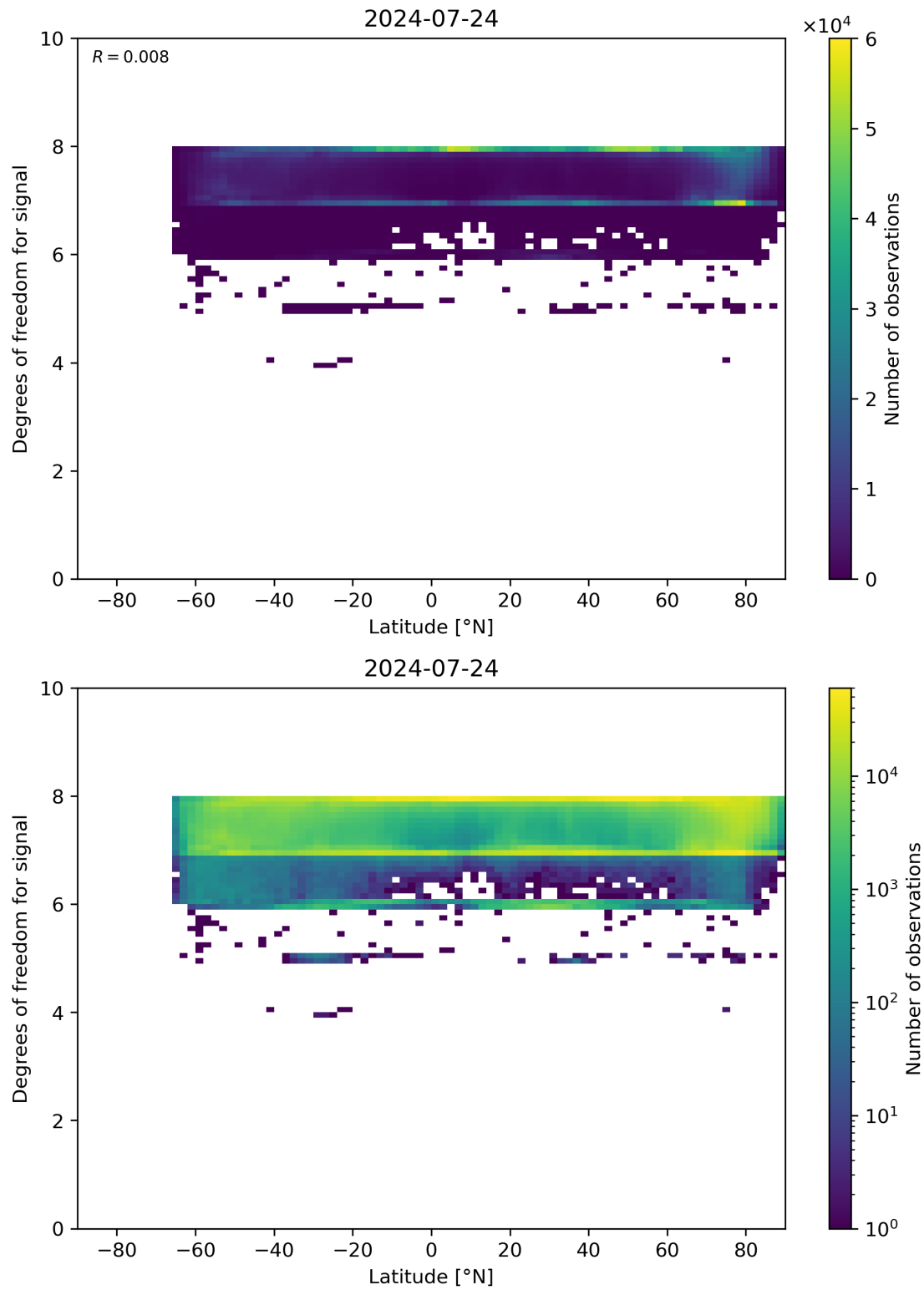
Figure 55: Scatter density plot of “Latitude” against “Degrees of freedom for signal” for 2024-07-23 to 2024-07-25.
