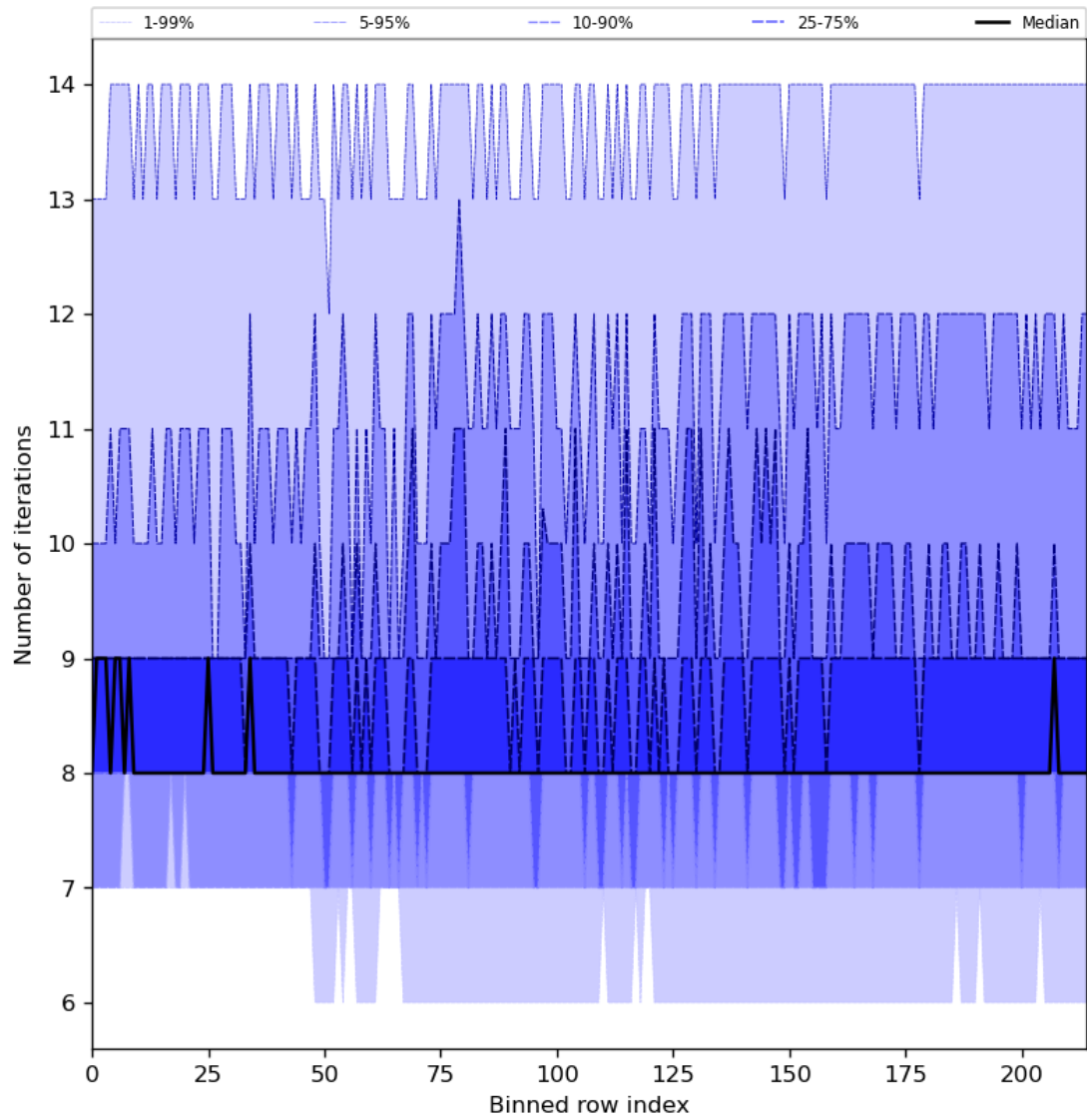
Figure 32: Along track statistics of “Number of iterations” for 2024-07-23 to 2024-07-25
