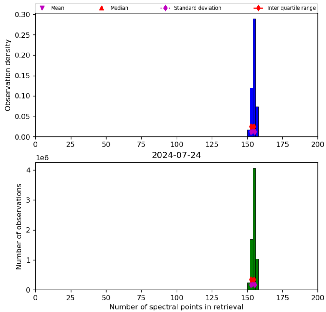
Figure 21: Histogram of “Number of spectral points in retrieval” for 2024-07-23 to 2024-07-25
