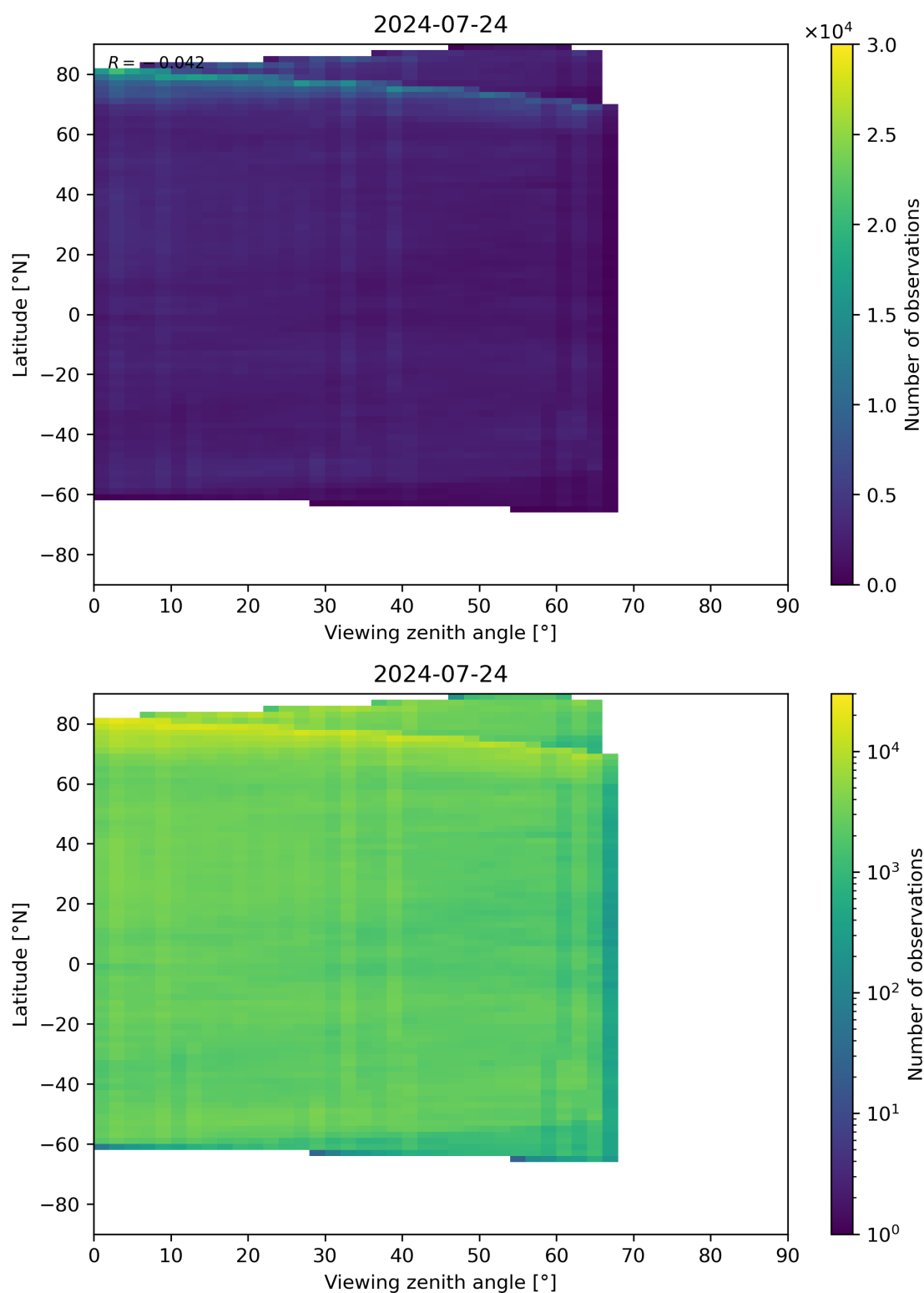
Figure 74: Scatter density plot of “Viewing zenith angle” against “Latitude” for 2024-07-23 to 2024-07-25.
