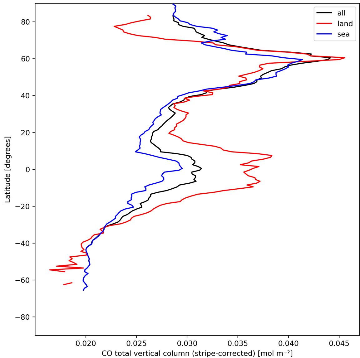
Figure 11: Zonal average of “CO total vertical column (stripe-corrected)” for 2024-07-23 to 2024-07-25.
