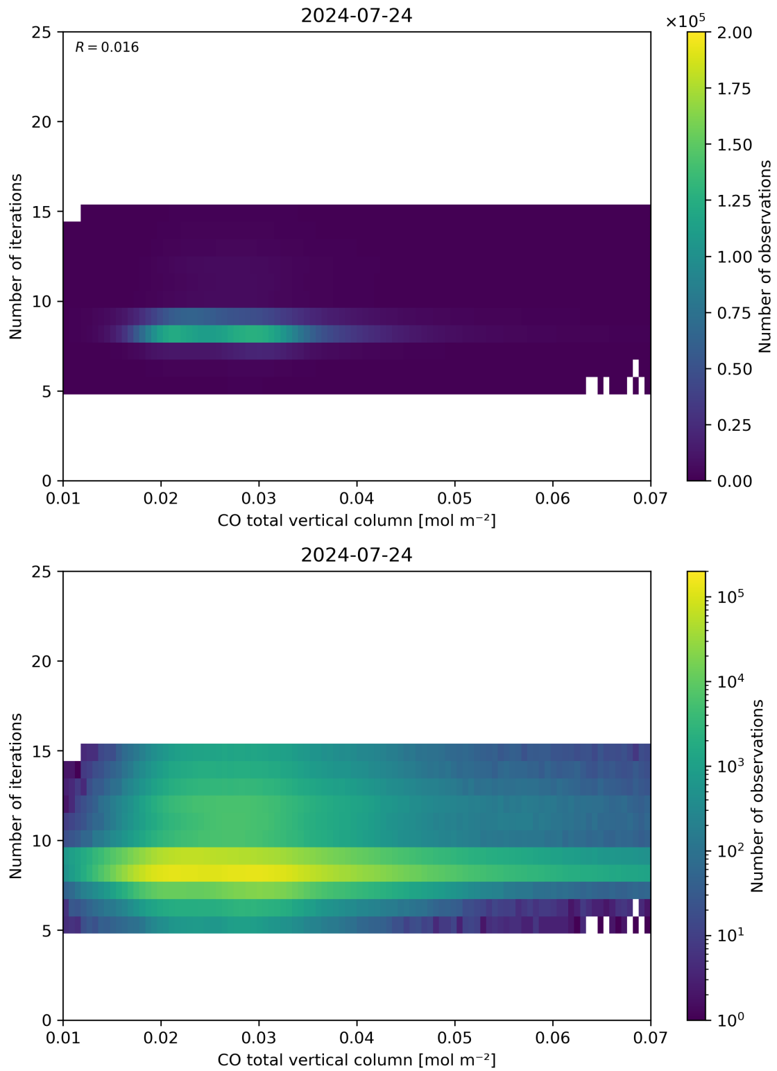
Figure 42: Scatter density plot of “CO total vertical column” against “Number of iterations” for 2024-07-23 to 2024-07-25.
