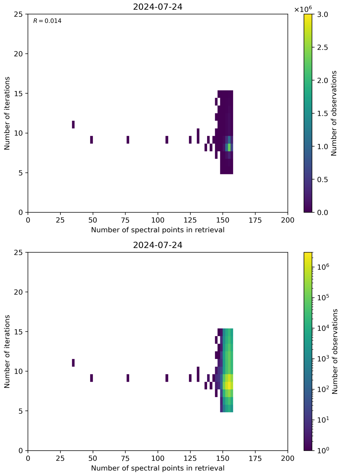
Figure 60: Scatter density plot of “Number of spectral points in retrieval” against “Number of iterations” for 2024-07-23 to 2024-07-25.
