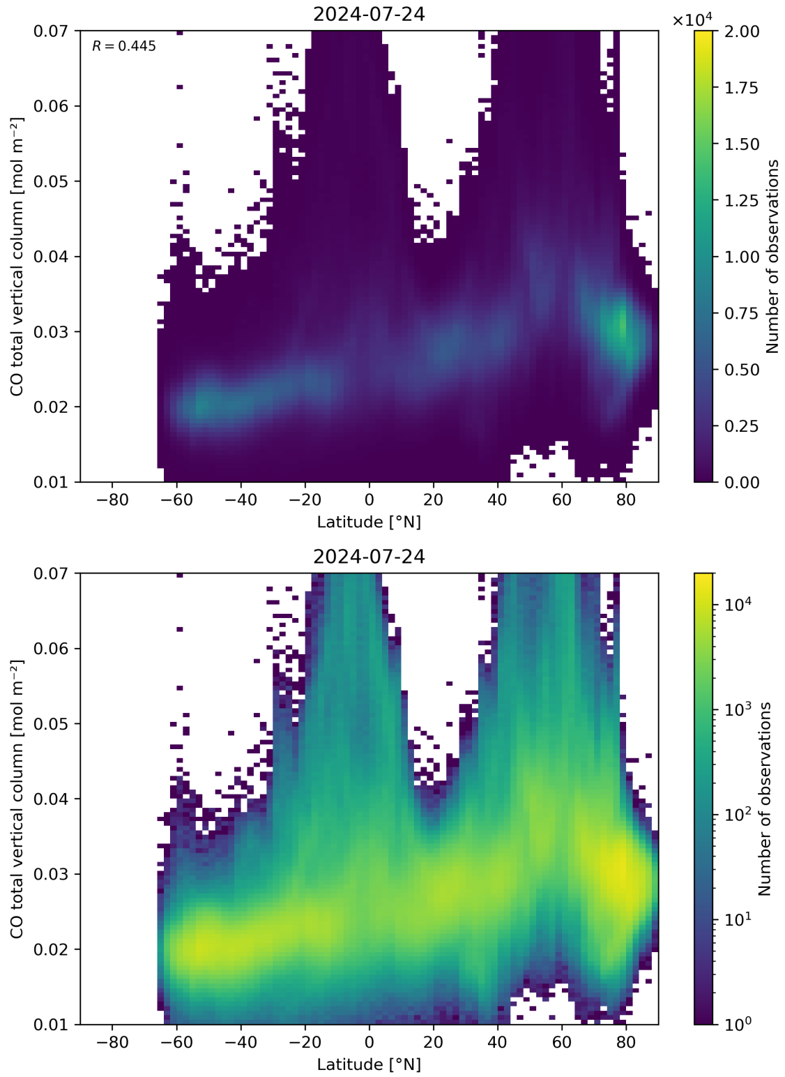
Figure 51: Scatter density plot of “Latitude” against “CO total vertical column” for 2024-07-23 to 2024-07-25.
