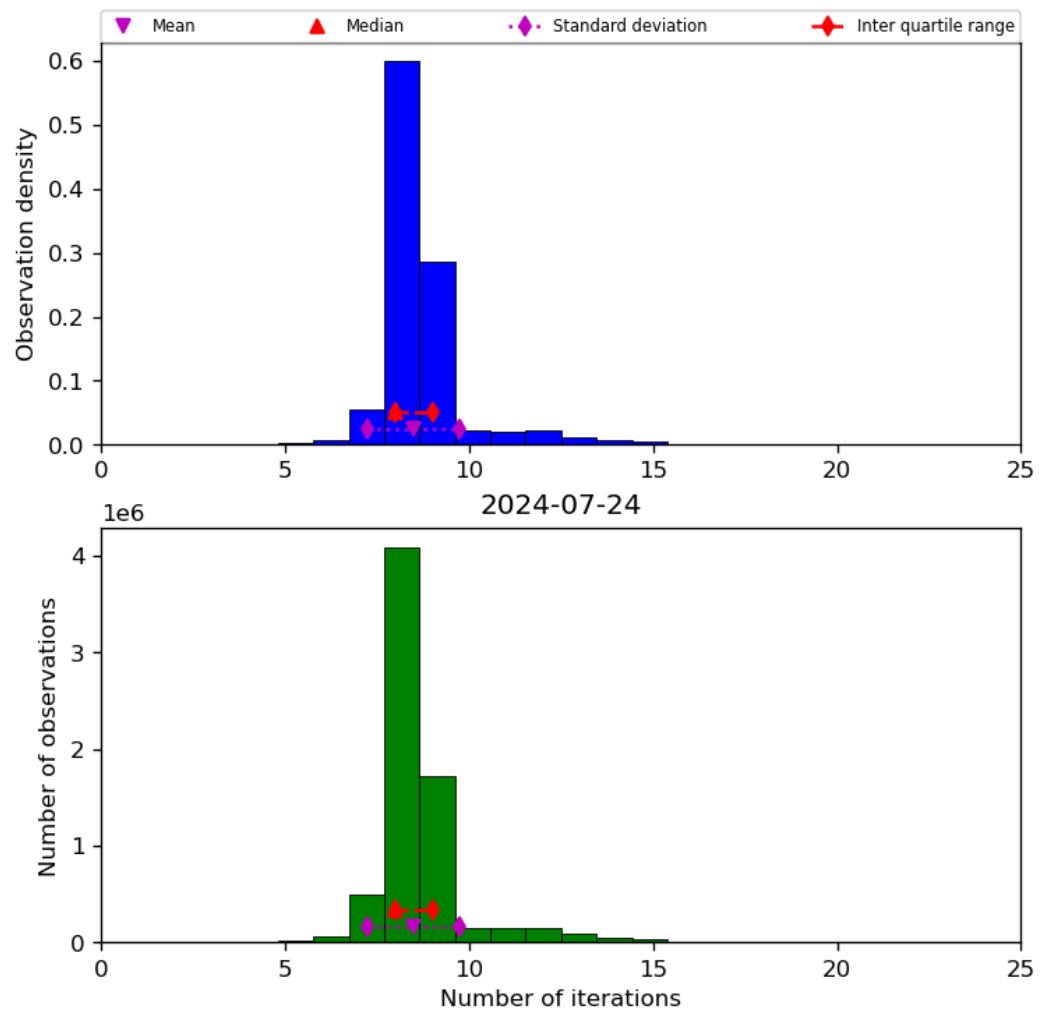
Figure 24: Histogram of “Number of iterations” for 2024-07-23 to 2024-07-25
