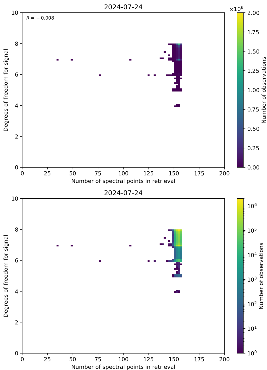
Figure 59: Scatter density plot of “Number of spectral points in retrieval” against “Degrees of freedom for signal” for 2024-07-23 to 2024-07-25.
