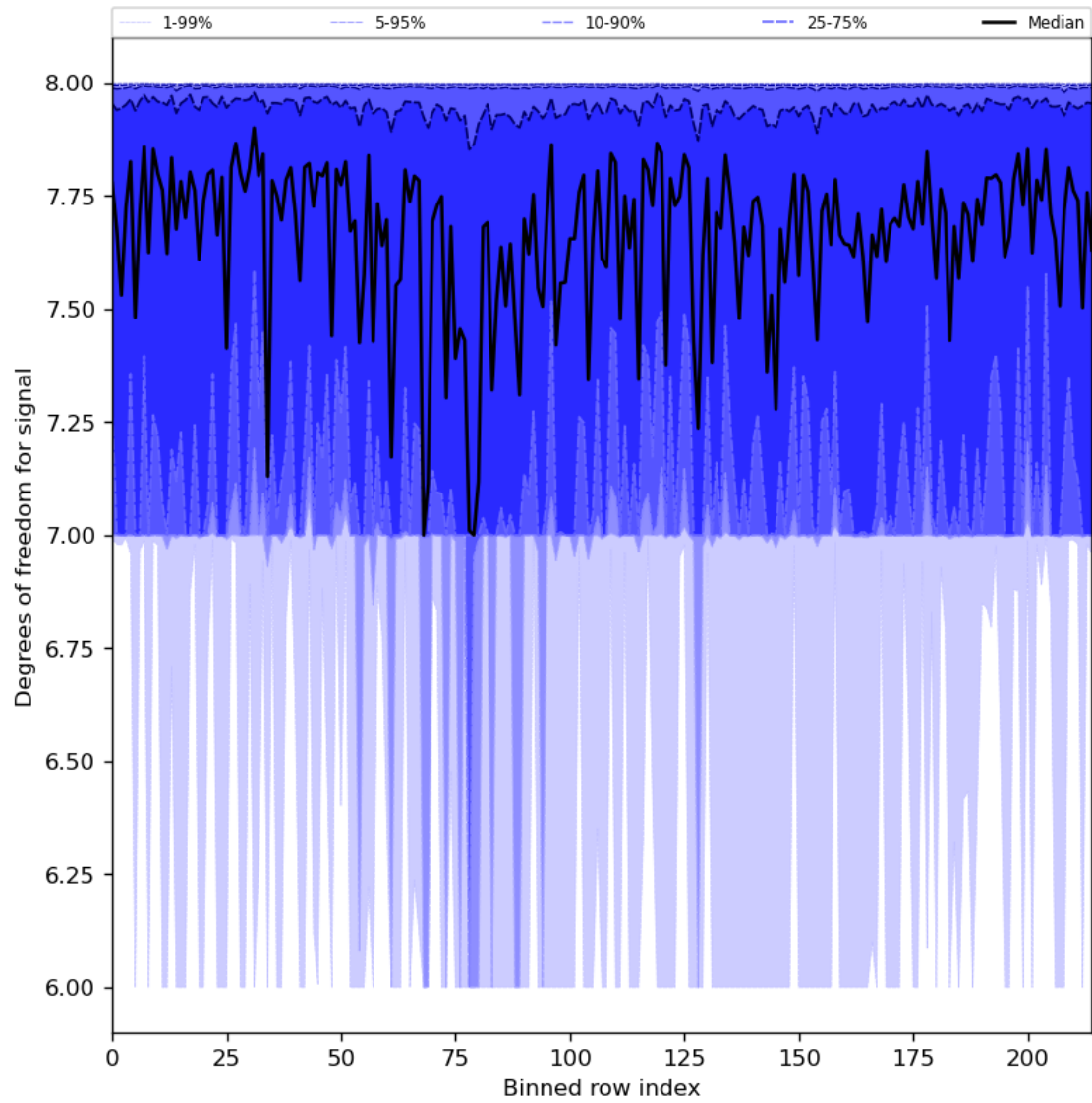
Figure 31: Along track statistics of “Degrees of freedom for signal” for 2024-07-23 to 2024-07-25
