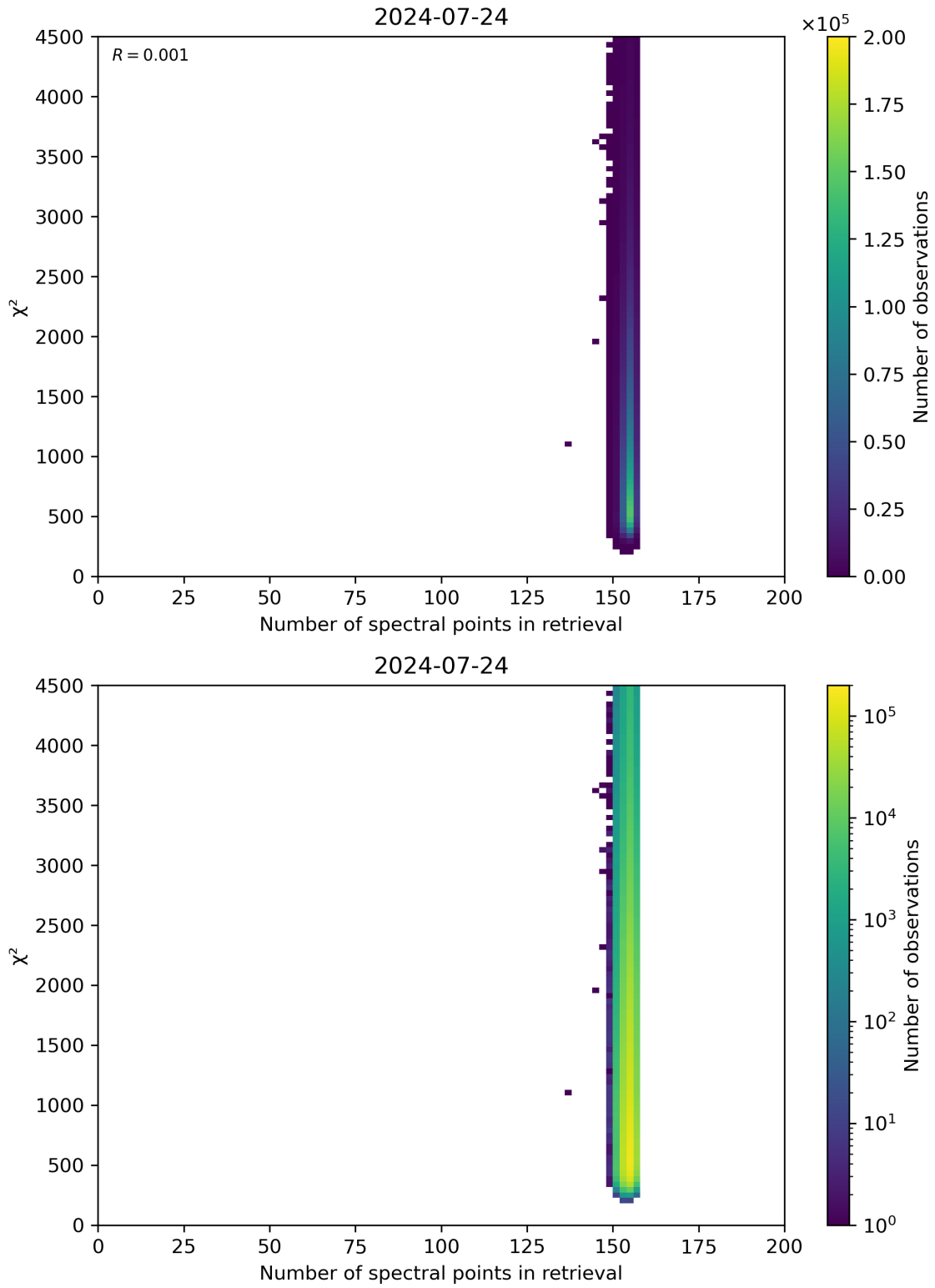
Figure 58: Scatter density plot of “Number of spectral points in retrieval” against “ \chi^2 ” for 2024-07-23 to 2024-07-25.
