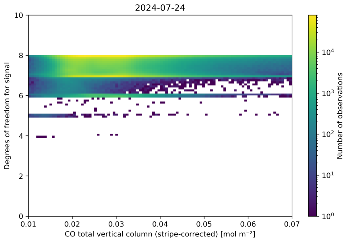
Figure 38: Scatter density plot of “CO total vertical column (stripe-corrected)” against “Degrees of freedom for signal” for 2024-07-23 to 2024-07-25.
