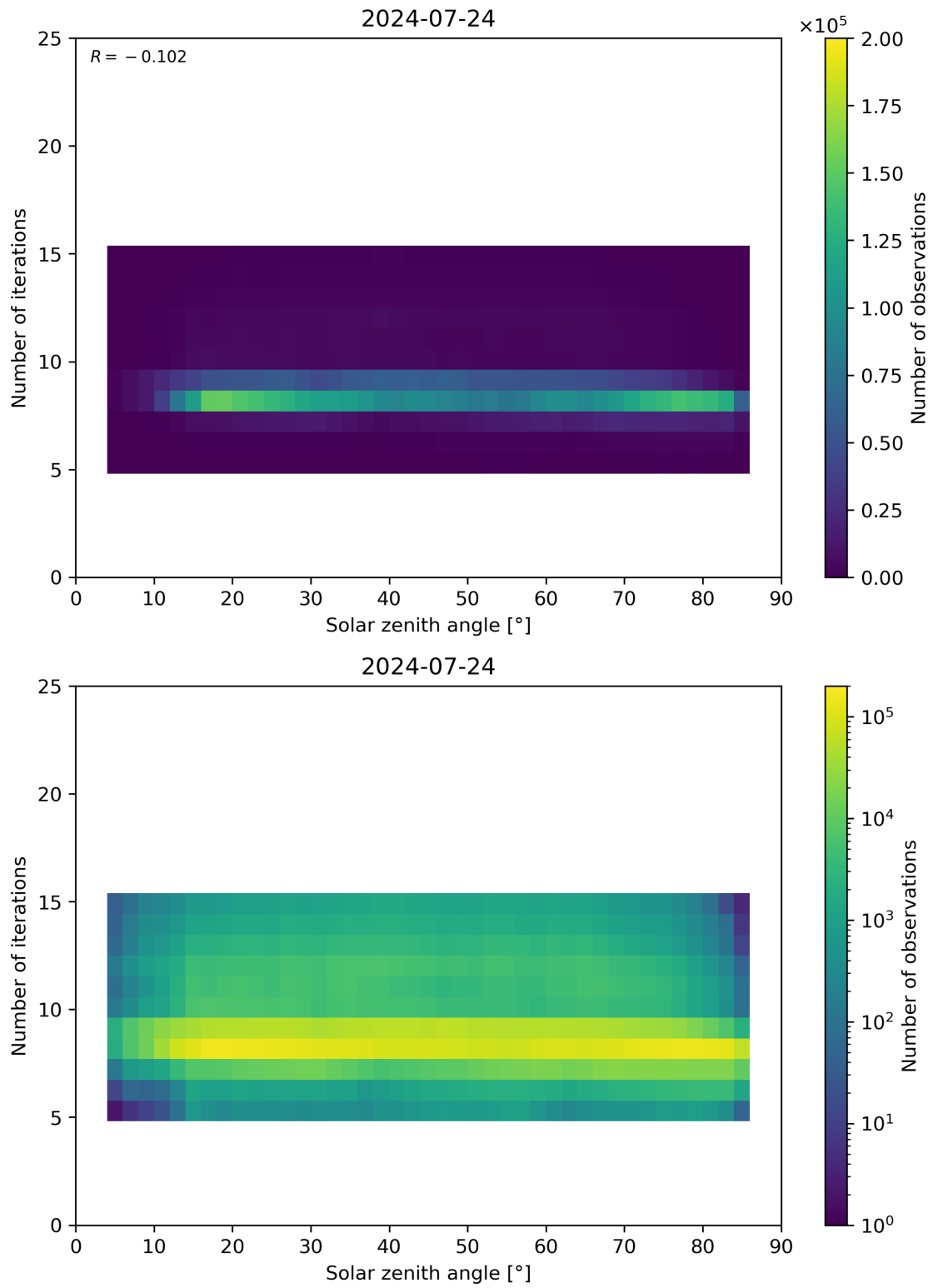
Figure 67: Scatter density plot of “Solar zenith angle” against “Number of iterations” for 2024-07-23 to 2024-07-25.
