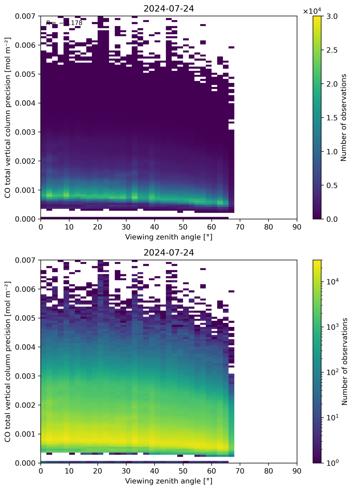
Figure 71: Scatter density plot of “Viewing zenith angle” against “CO total vertical column precision” for 2024-07-23 to 2024-07-25.
