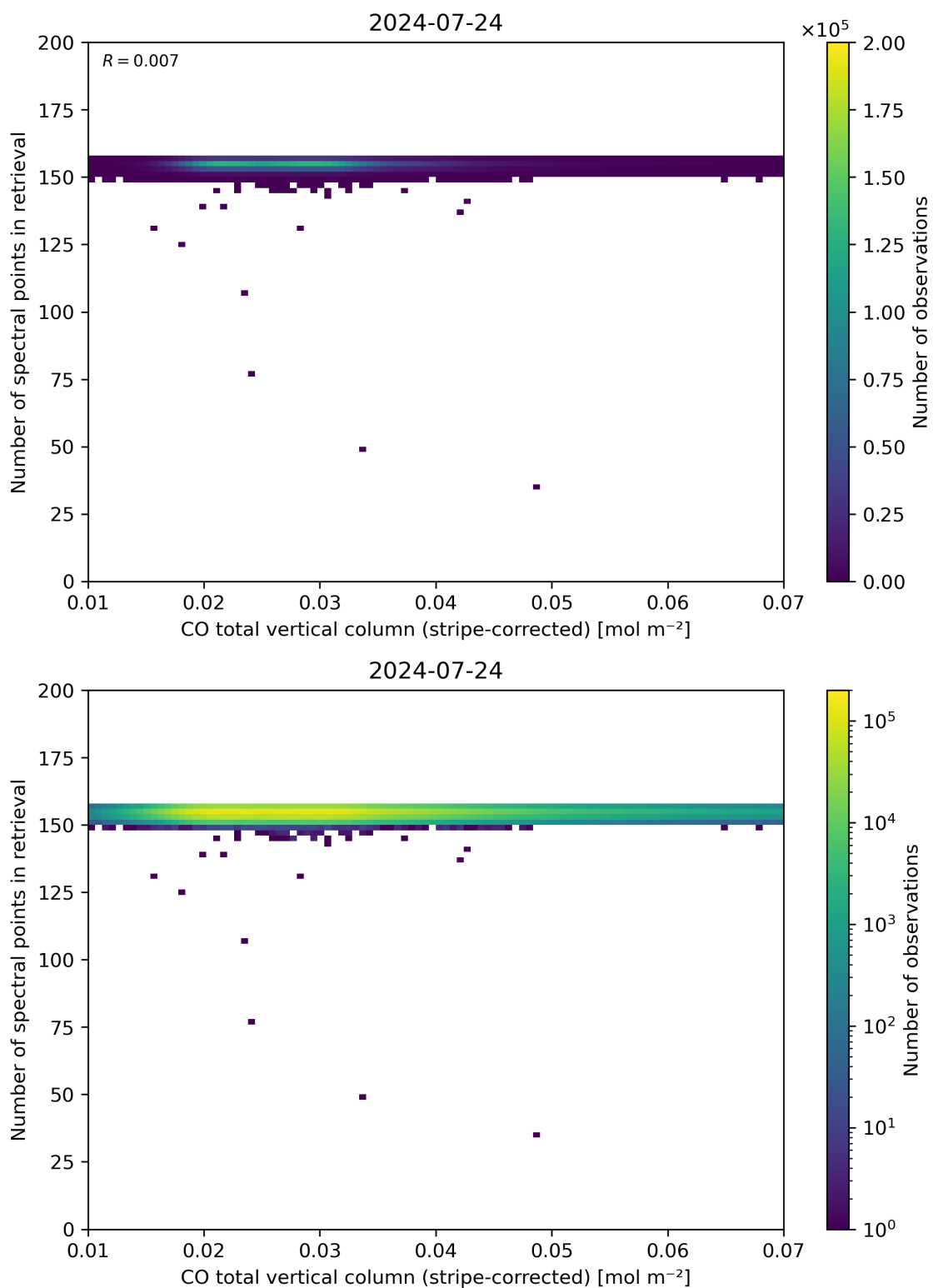
Figure 40: Scatter density plot of “CO total vertical column (stripe-corrected)” against “Number of spectral points in retrieval” for 2024-07-23 to 2024-07-25.
