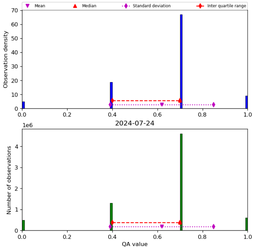
Figure 17: Histogram of “QA value” for 2024-07-23 to 2024-07-25
