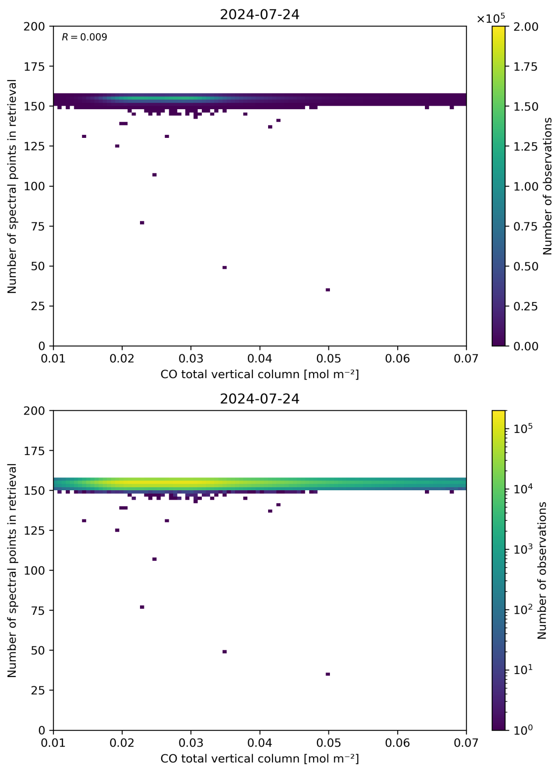
Figure 43: Scatter density plot of “CO total vertical column” against “Number of spectral points in retrieval” for 2024-07-23 to 2024-07-25.
