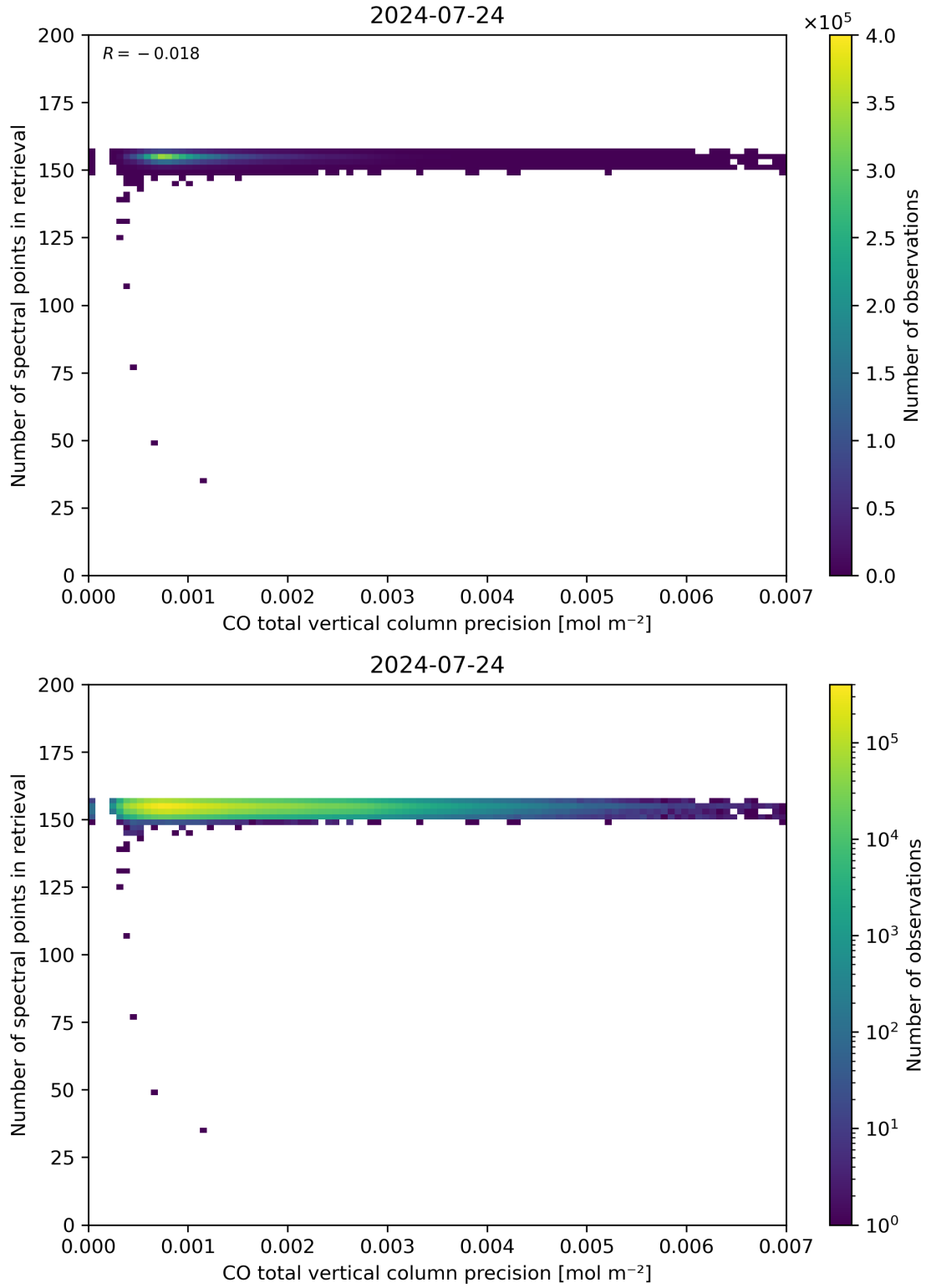
Figure 47: Scatter density plot of “CO total vertical column precision” against “Number of spectral points in retrieval” for 2024-07-23 to 2024-07-25.
