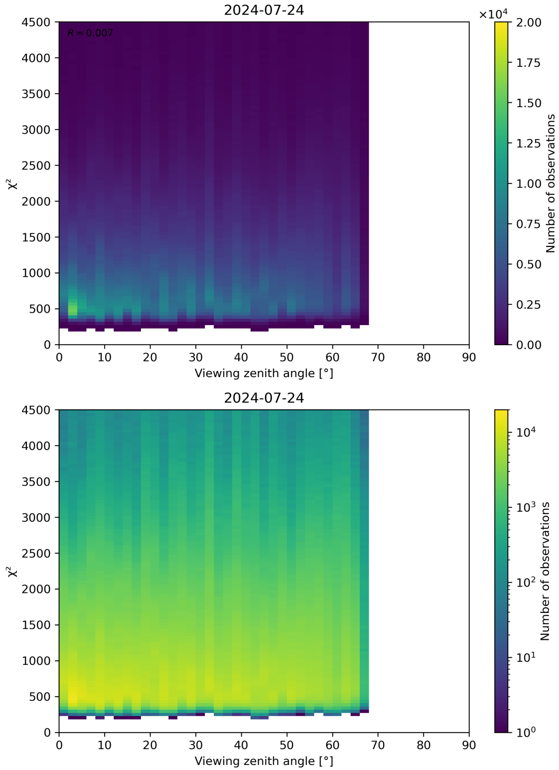
Figure 72: Scatter density plot of “Viewing zenith angle” against “ \chi^2 ” for 2024-07-23 to 2024-07-25.
