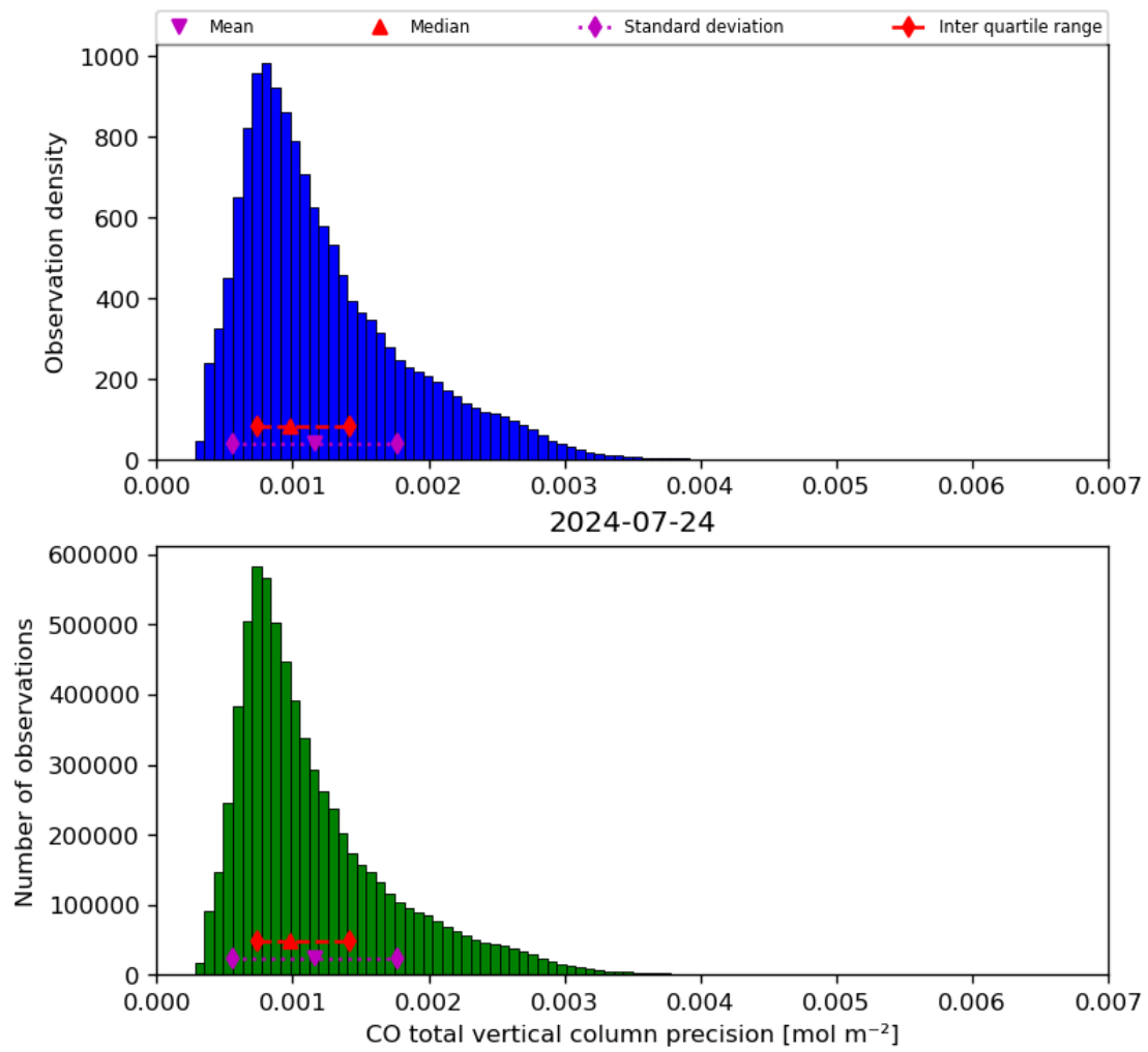
Figure 20: Histogram of “CO total vertical column precision” for 2024-07-23 to 2024-07-25
