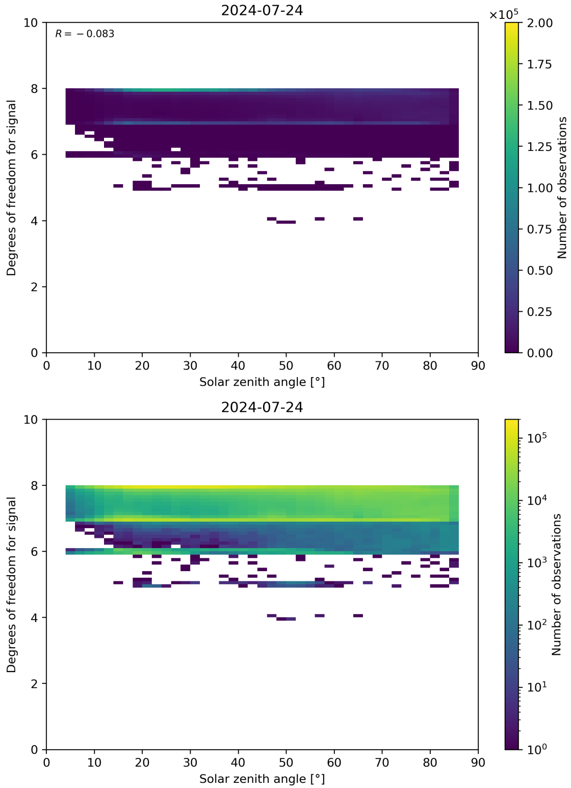
Figure 65: Scatter density plot of “Solar zenith angle” against “Degrees of freedom for signal” for 2024-07-23 to 2024-07-25.
