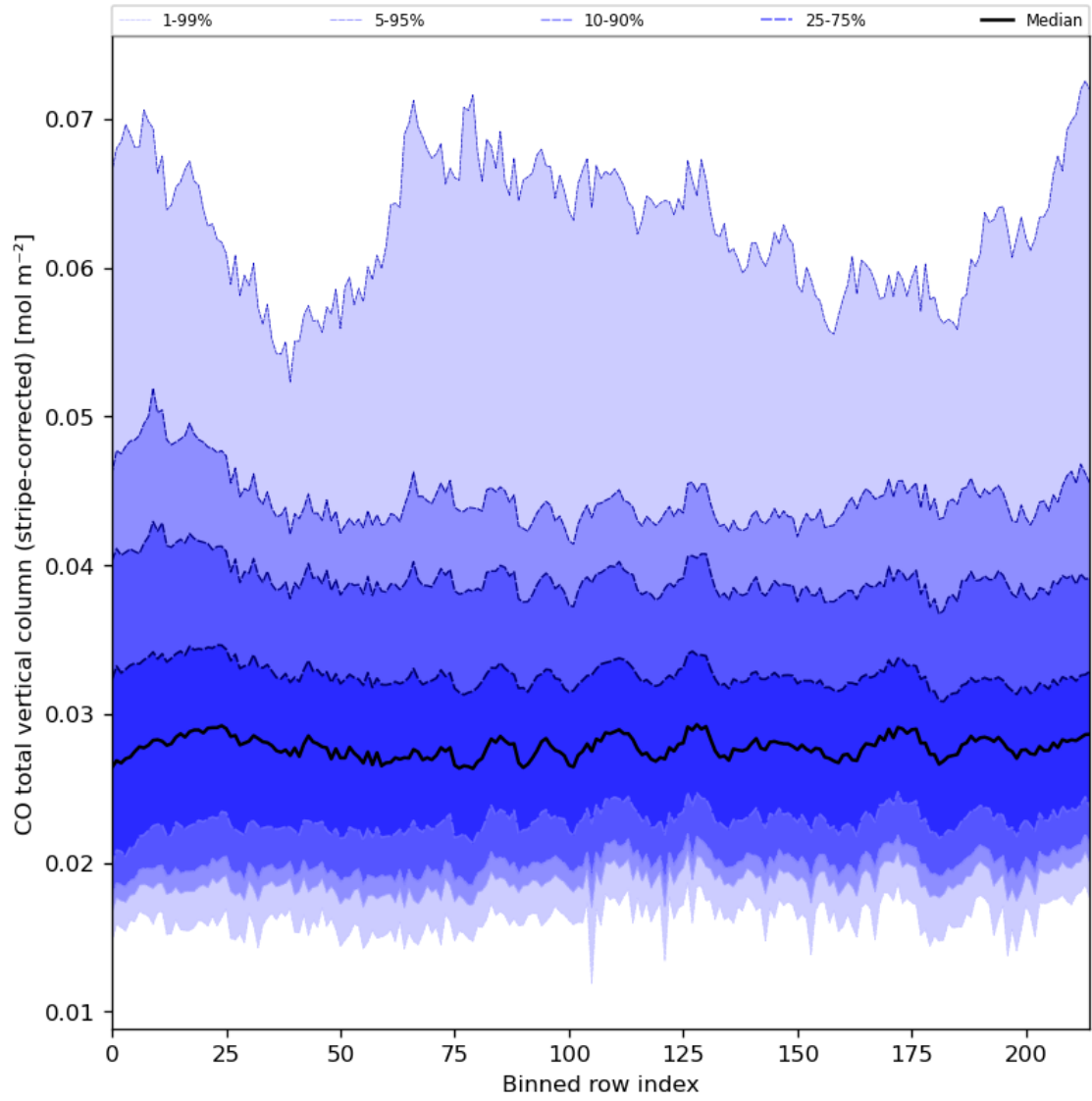
Figure 27: Along track statistics of “CO total vertical column (stripe-corrected)” for 2024-07-23 to 2024-07-25
