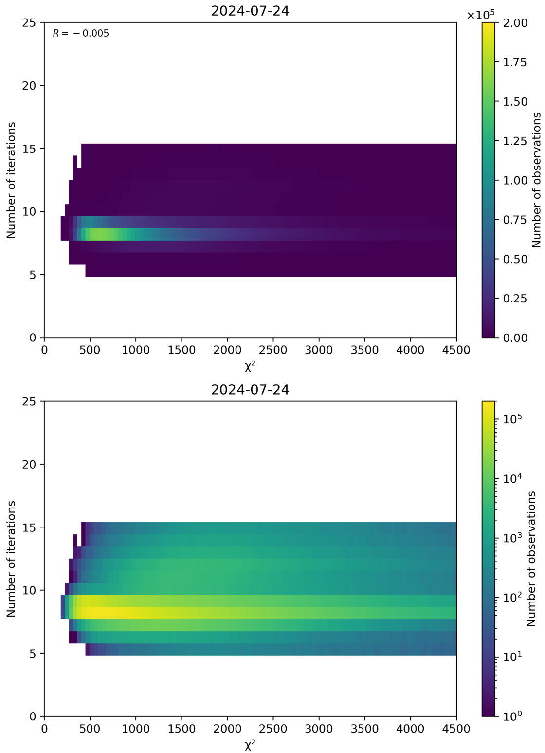
Figure 49: Scatter density plot of “ \chi^2 ” against “Number of iterations” for 2024-07-23 to 2024-07-25.
