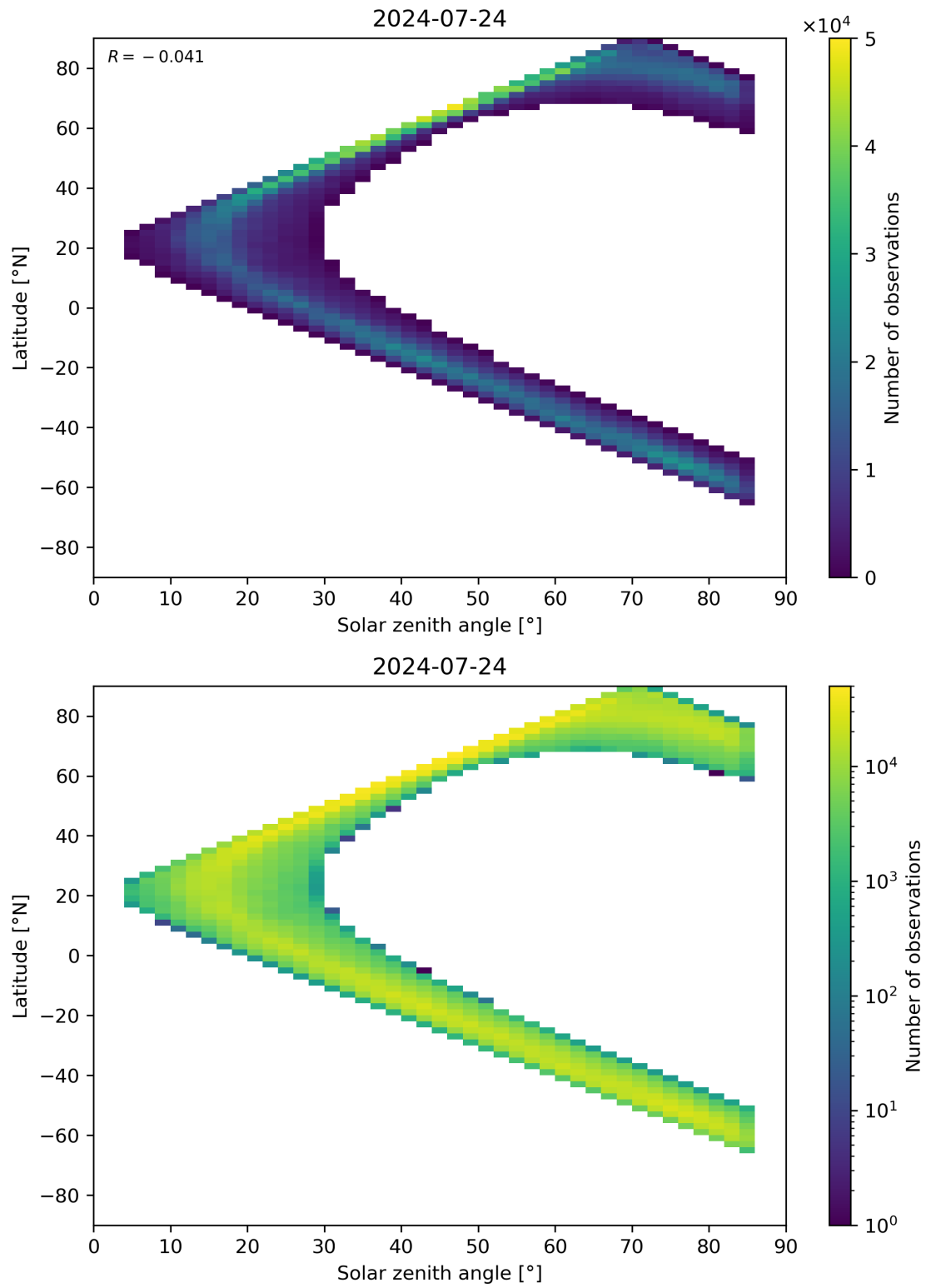
Figure 66: Scatter density plot of “Solar zenith angle” against “Latitude” for 2024-07-23 to 2024-07-25.
