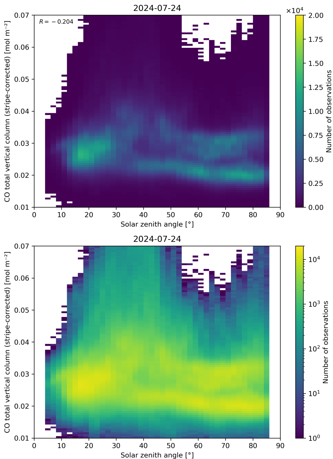
Figure 62: Scatter density plot of “Solar zenith angle” against “CO total vertical column (stripe-corrected)” for 2024-07-23 to 2024-07-25.
