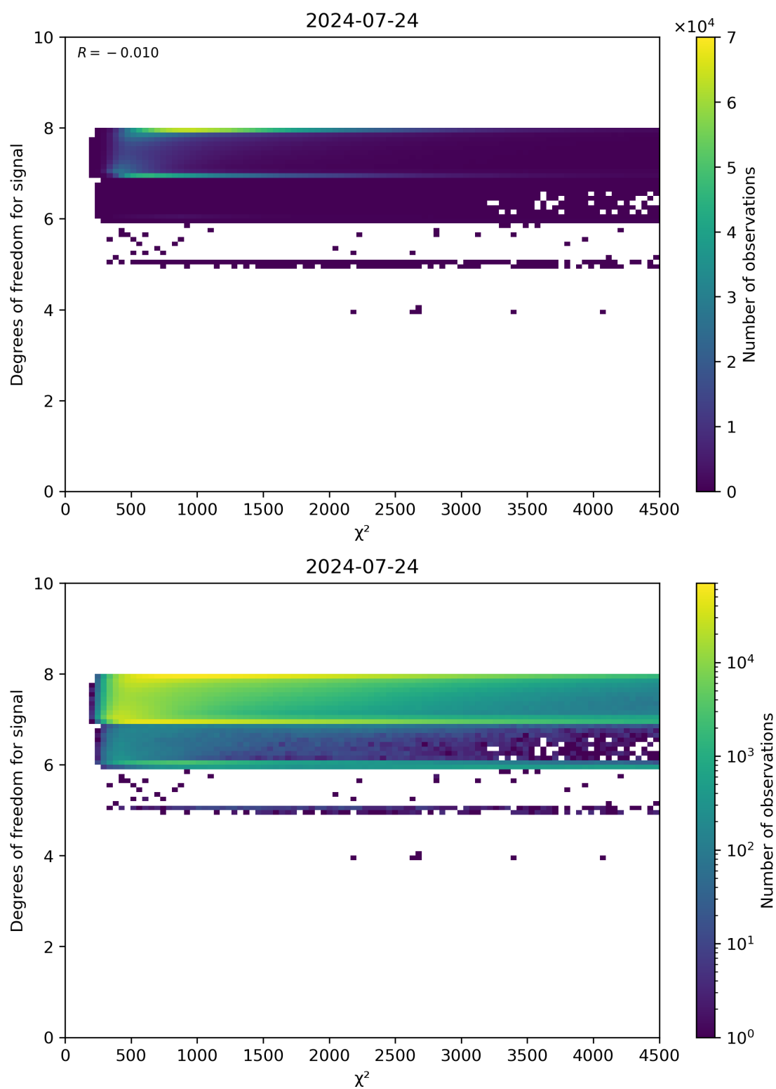
Figure 48: Scatter density plot of " \chi^2 " against "Degrees of freedom for signal" for 2024-07-23 to 2024-07-25.
