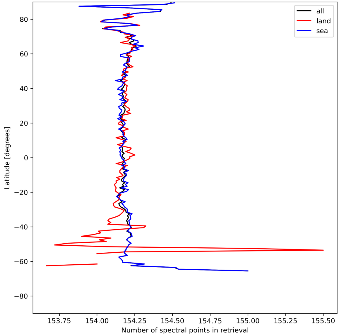
Figure 13: Zonal average of “Number of spectral points in retrieval” for 2024-07-23 to 2024-07-25.
