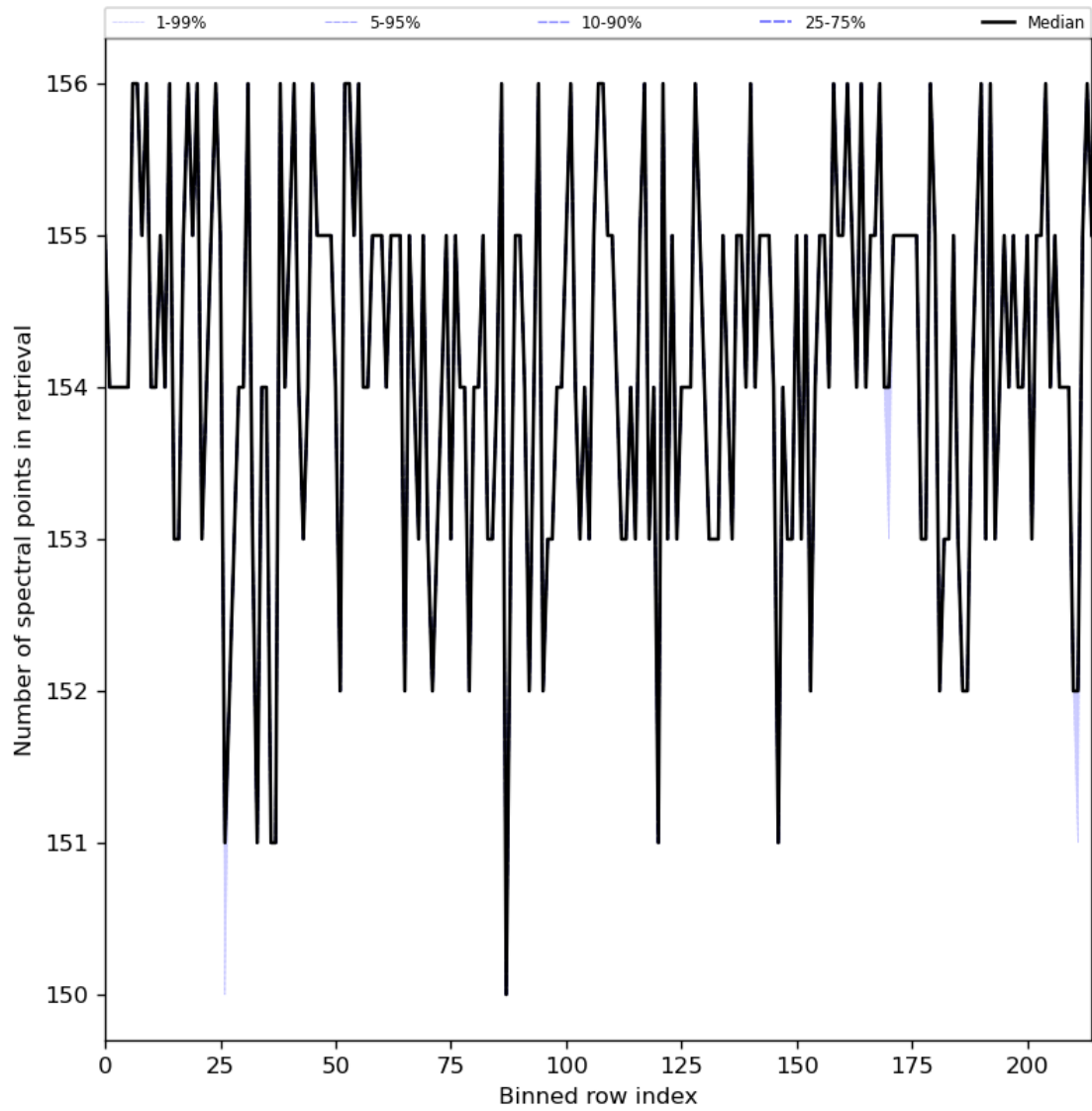
Figure 29: Along track statistics of “Number of spectral points in retrieval” for 2024-07-23 to 2024-07-25
