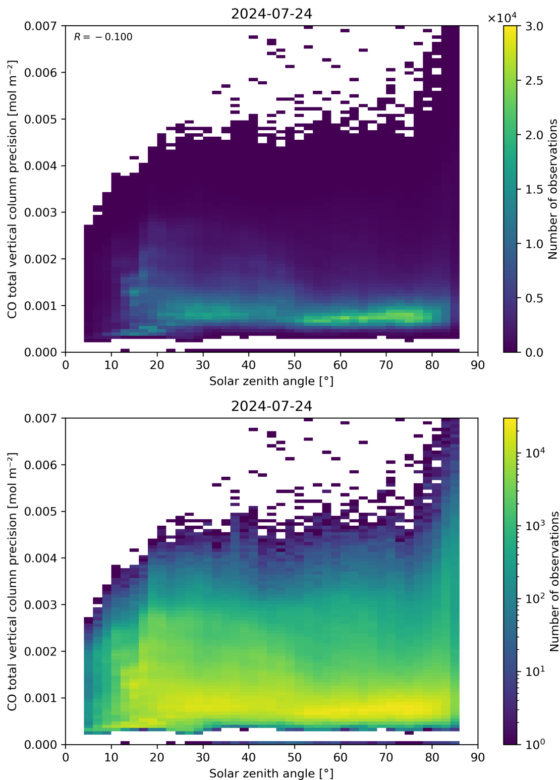
Figure 63: Scatter density plot of “Solar zenith angle” against “CO total vertical column precision” for 2024-07-23 to 2024-07-25.
