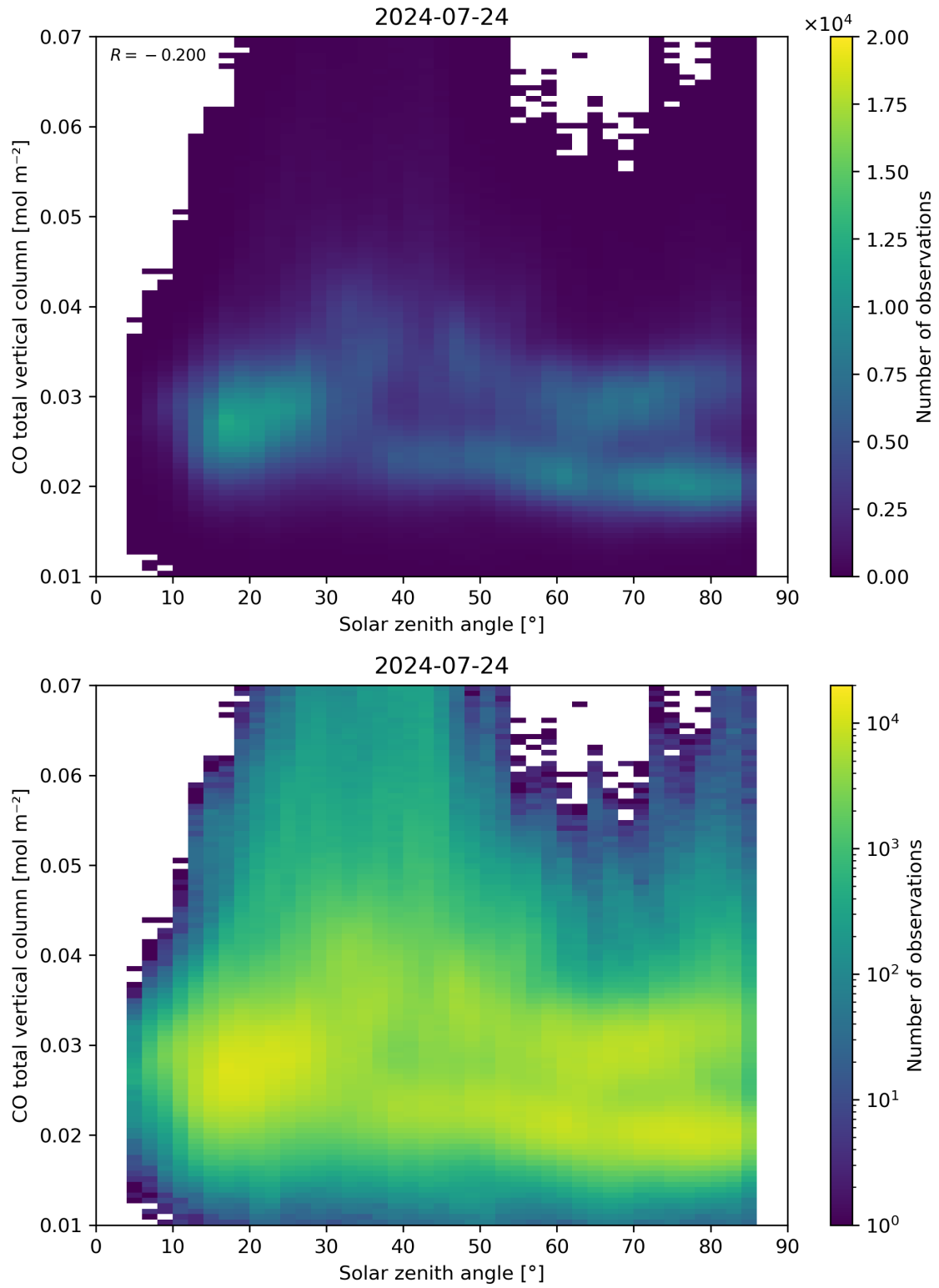
Figure 61: Scatter density plot of “Solar zenith angle” against “CO total vertical column” for 2024-07-23 to 2024-07-25.
