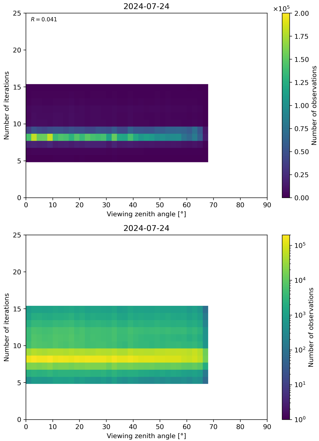
Figure 75: Scatter density plot of “Viewing zenith angle” against “Number of iterations” for 2024-07-23 to 2024-07-25.
