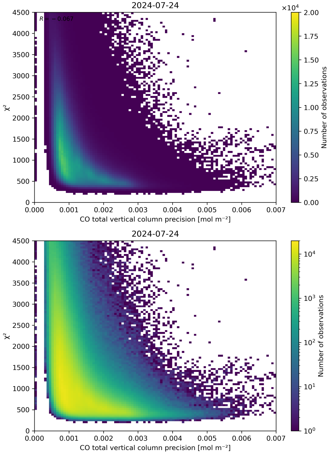
Figure 44: Scatter density plot of “CO total vertical column precision” against “ \chi^2 ” for 2024-07-23 to 2024-07-25.
