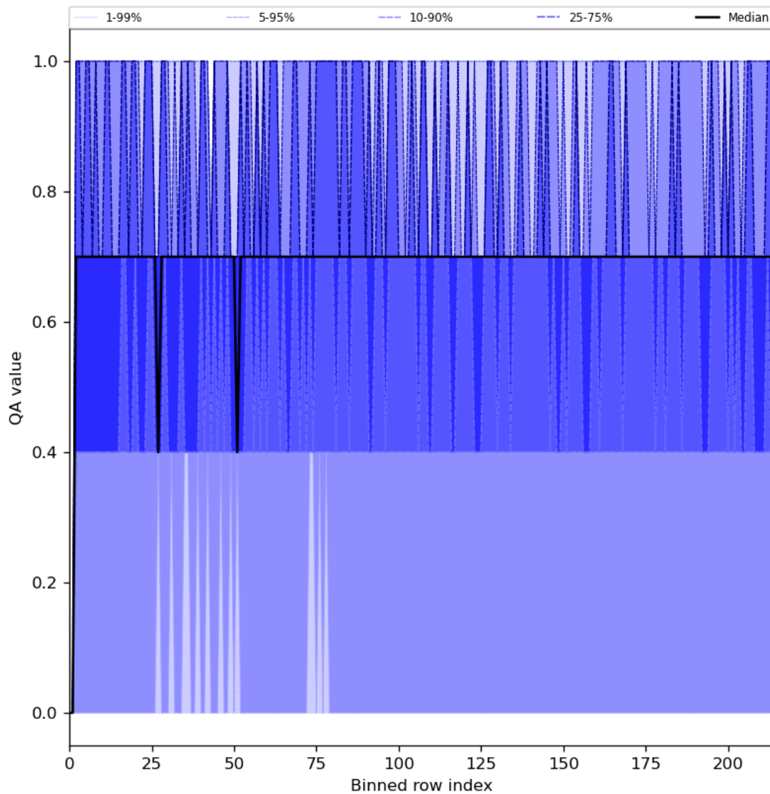
Figure 25: Along track statistics of “QA value” for 2024-07-23 to 2024-07-25
