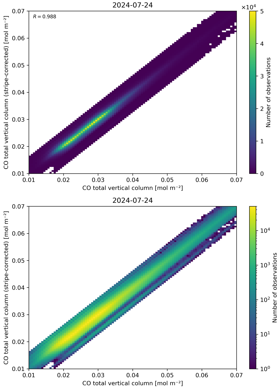
Figure 33: Scatter density plot of “CO total vertical column” against “CO total vertical column (stripe-corrected)” for 2024-07-23 to 2024-07-25.
