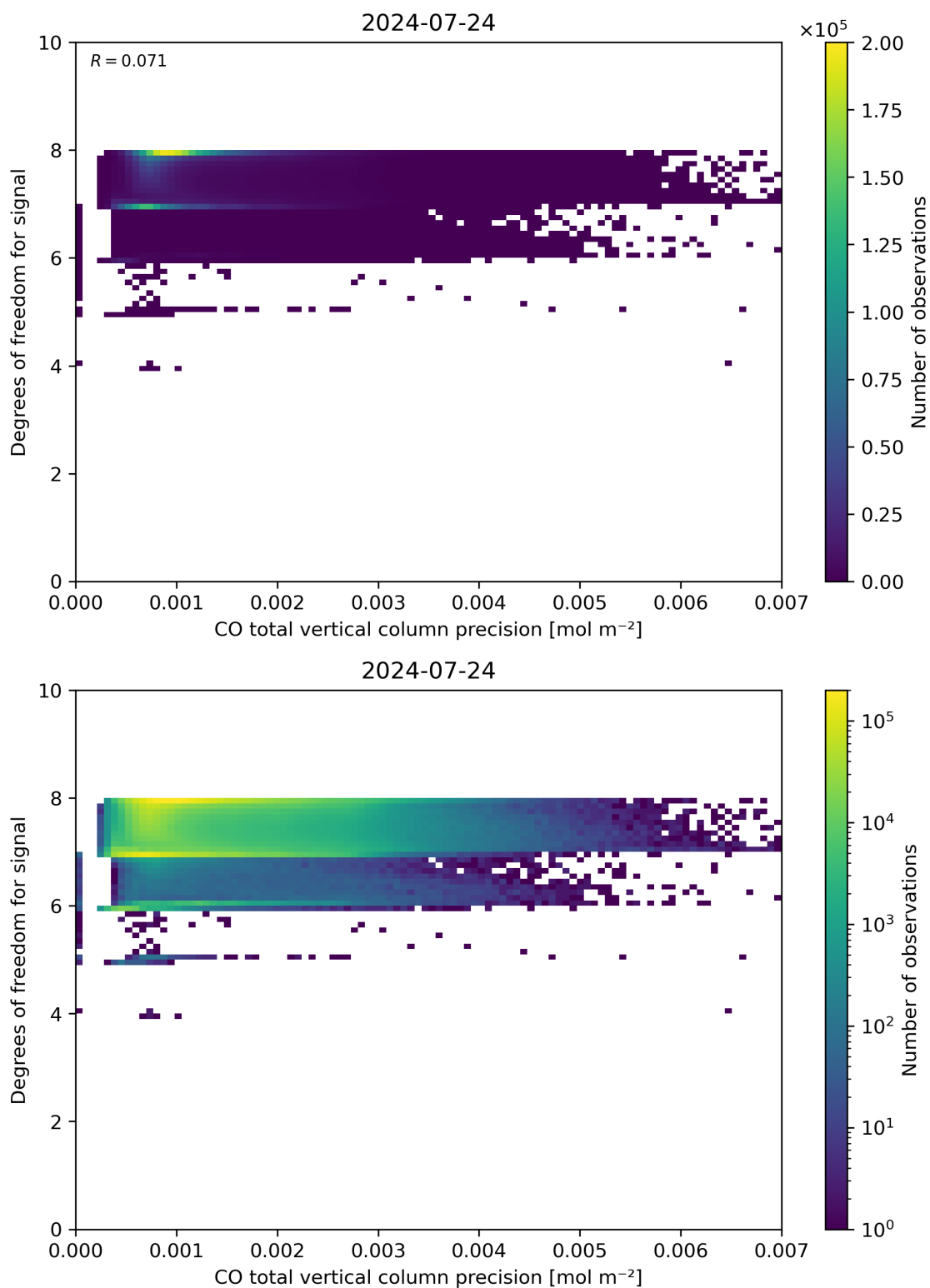
Figure 45: Scatter density plot of “CO total vertical column precision” against “Degrees of freedom for signal” for 2024-07-23 to 2024-07-25.
