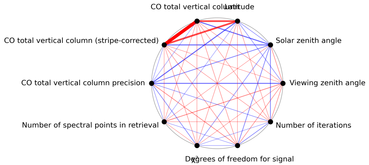
Figure 1: Map of correlation graph for 2024-07-23 to 2024-07-25.
