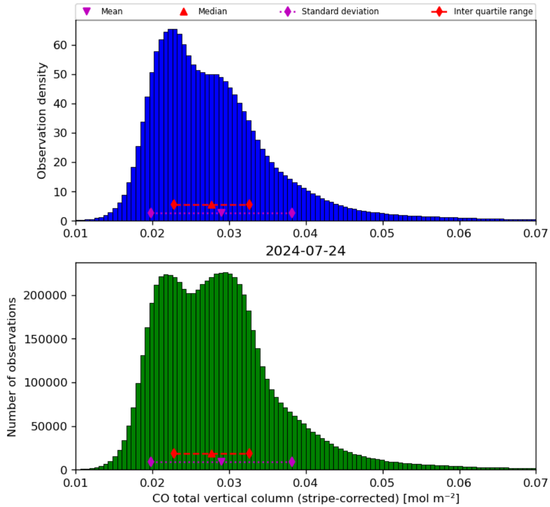
Figure 19: Histogram of “CO total vertical column (stripe-corrected)” for 2024-07-23 to 2024-07-25
