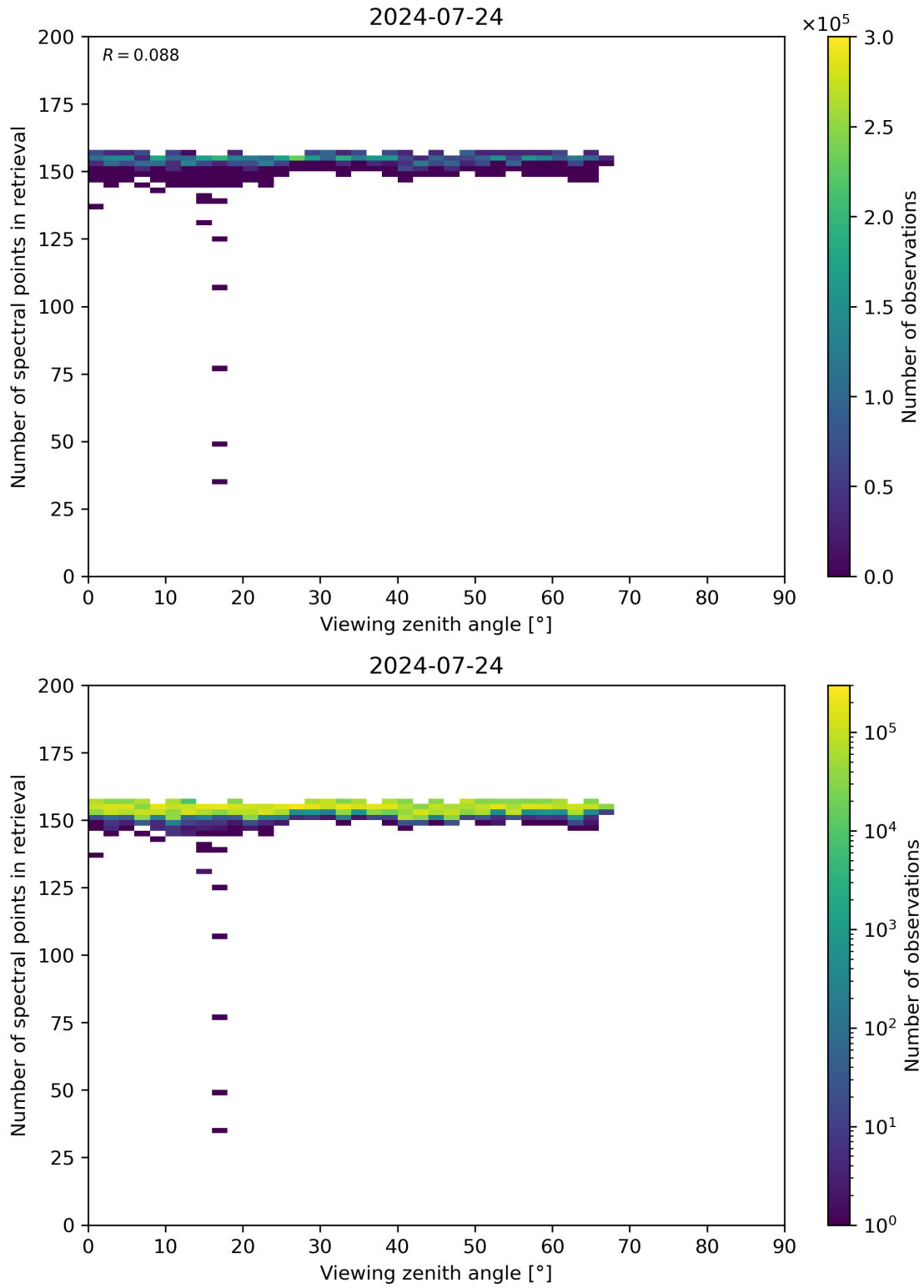
Figure 76: Scatter density plot of “Viewing zenith angle” against “Number of spectral points in retrieval” for 2024-07-23 to 2024-07-25.
