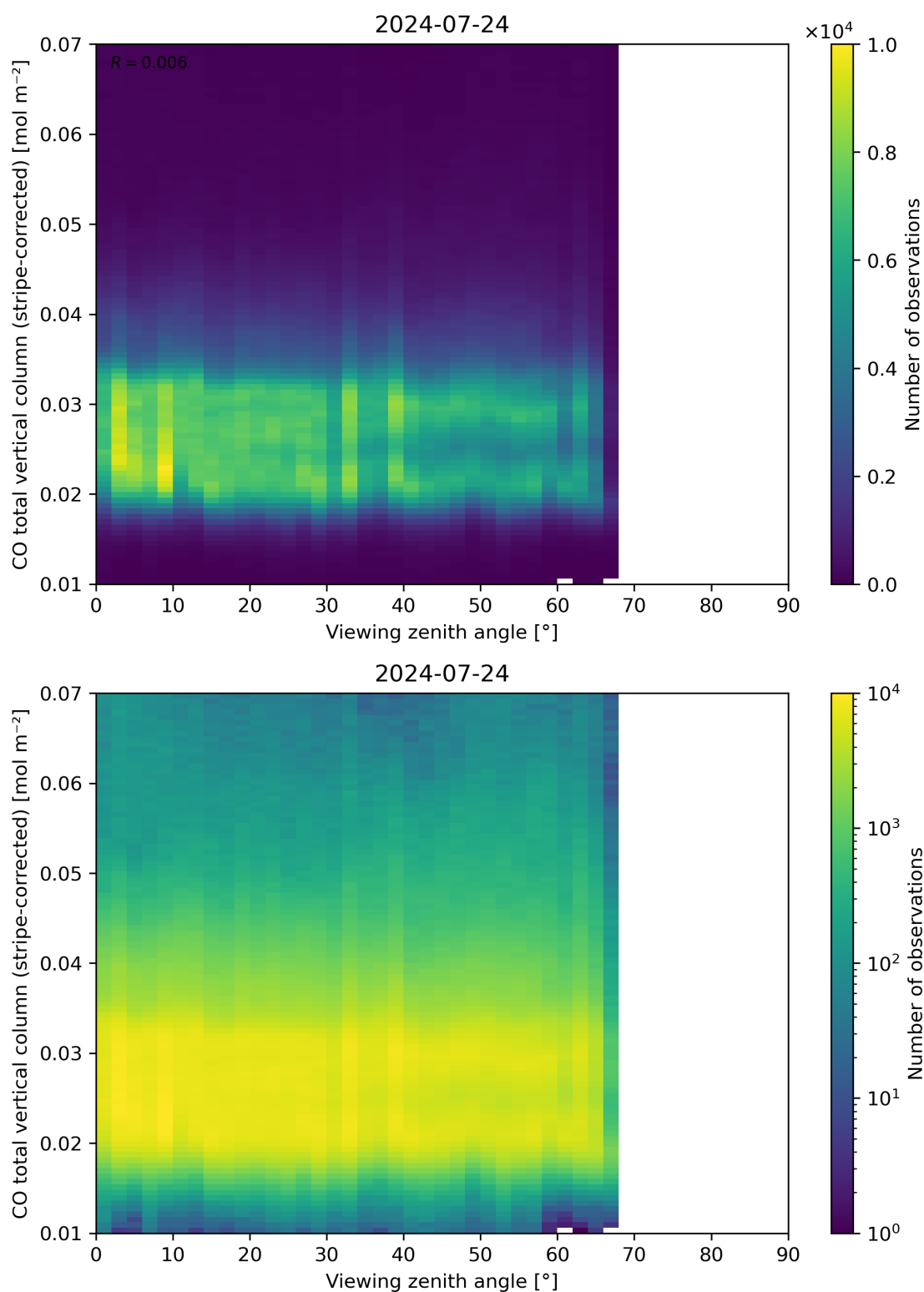
Figure 70: Scatter density plot of “Viewing zenith angle” against “CO total vertical column (stripe-corrected)” for 2024-07-23 to 2024-07-25.
