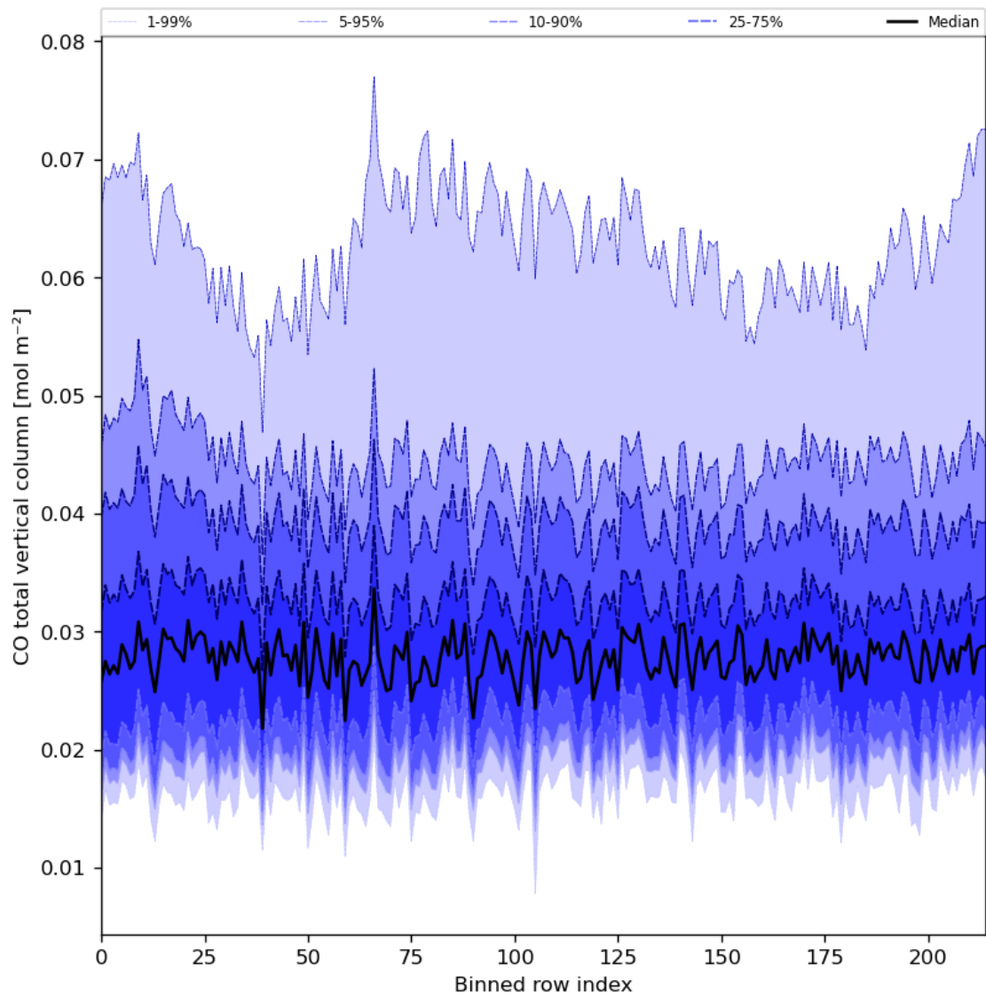
Figure 26: Along track statistics of “CO total vertical column” for 2024-07-23 to 2024-07-25
