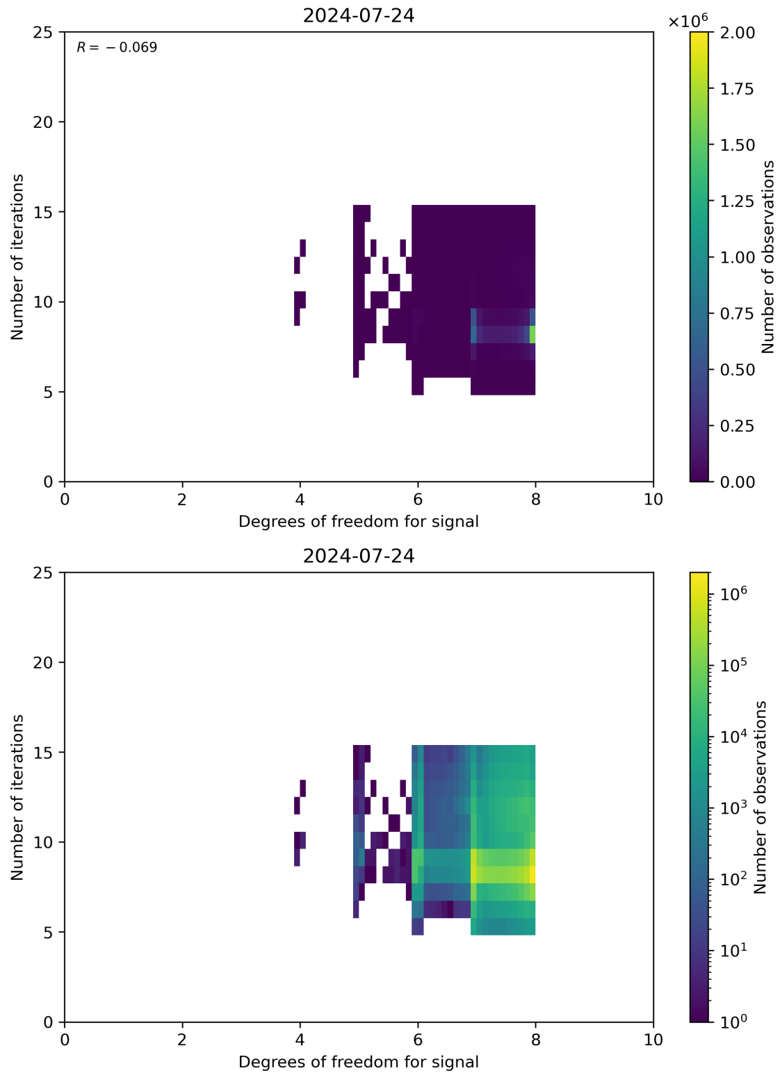
Figure 50: Scatter density plot of “Degrees of freedom for signal” against “Number of iterations” for 2024-07-23 to 2024-07-25.
