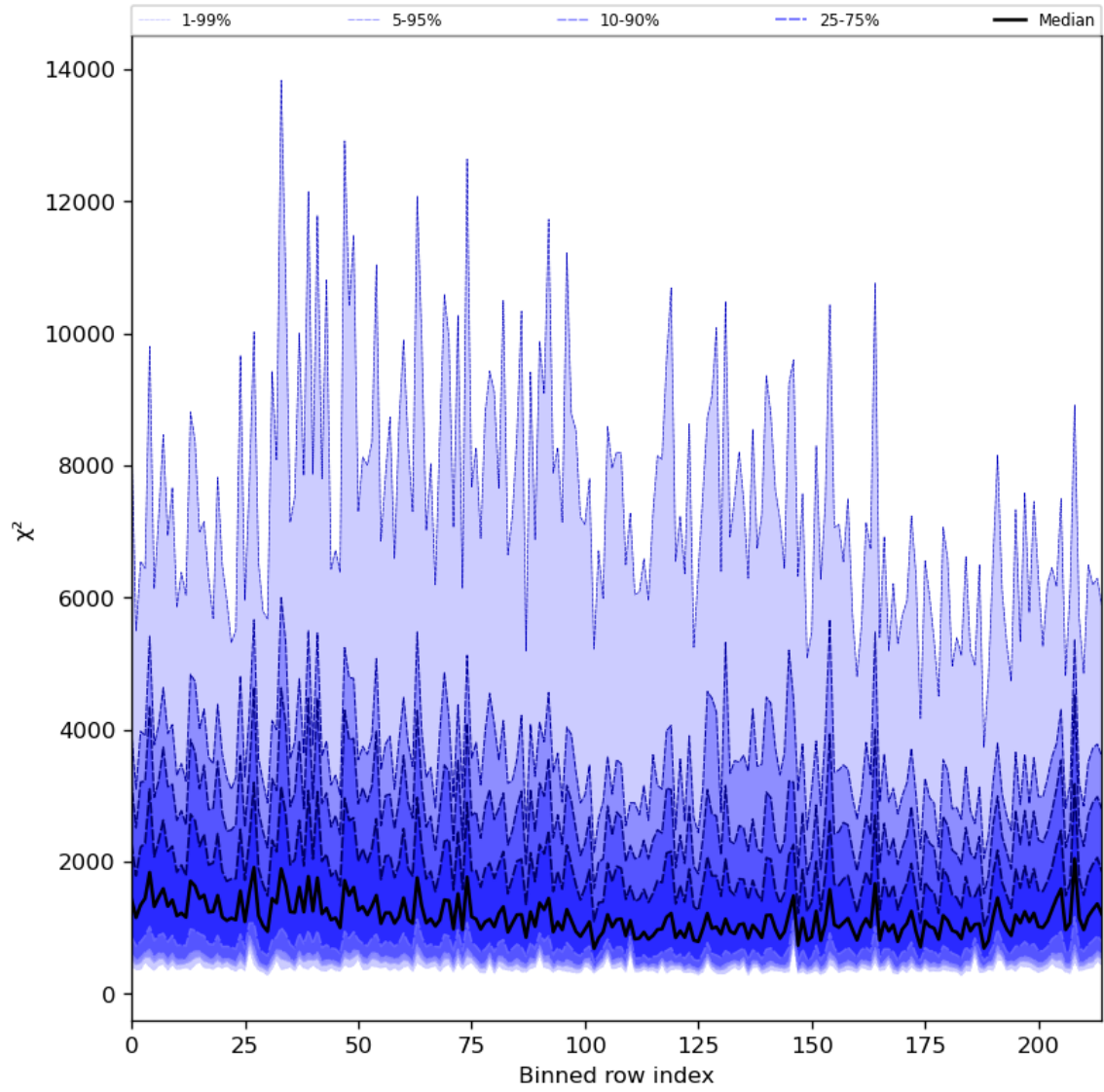
Figure 30: Along track statistics of “ \chi^2 ” for 2024-07-23 to 2024-07-25
