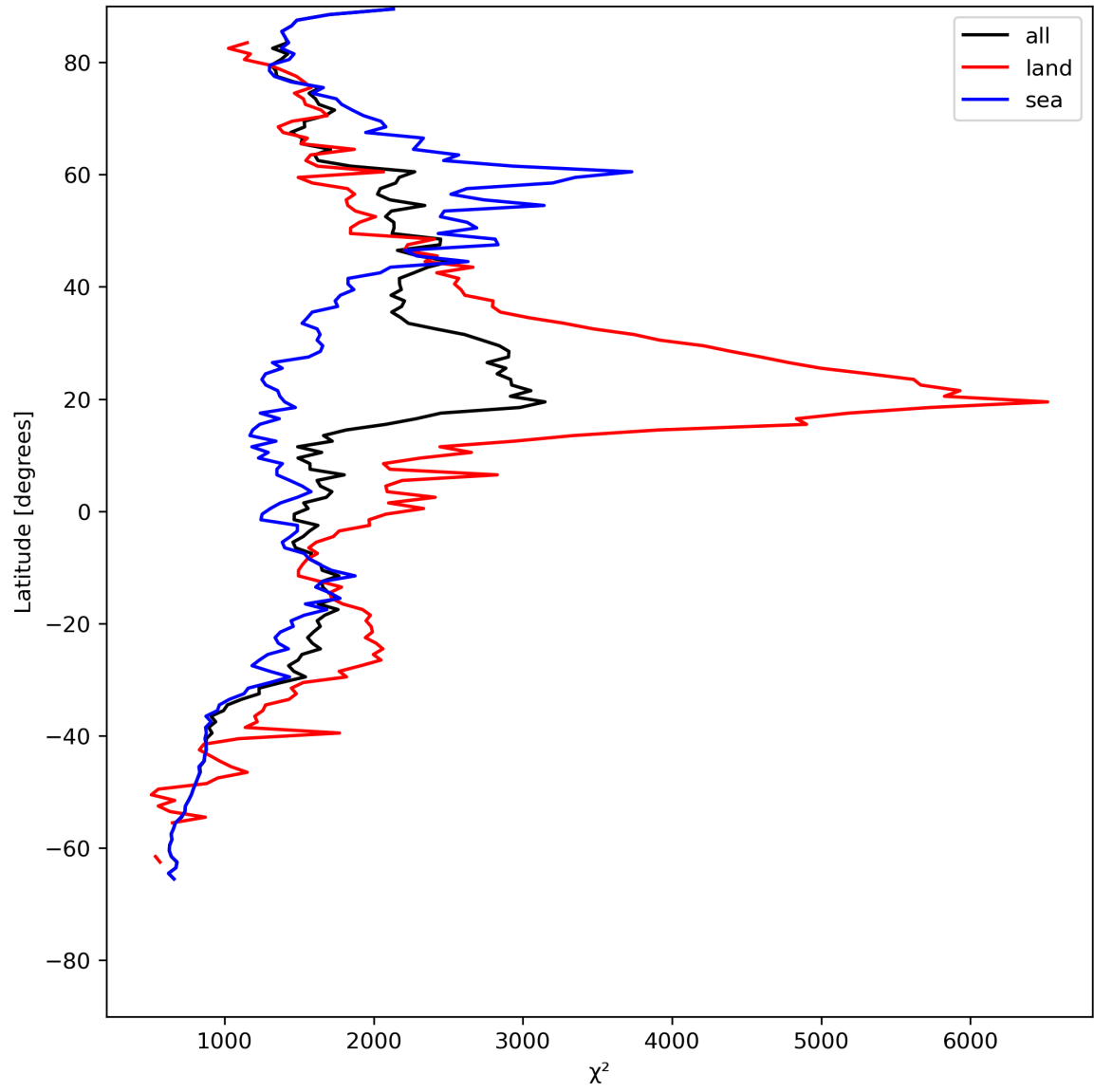
Figure 14: Zonal average of “ \chi^2 ” for 2024-07-23 to 2024-07-25.
