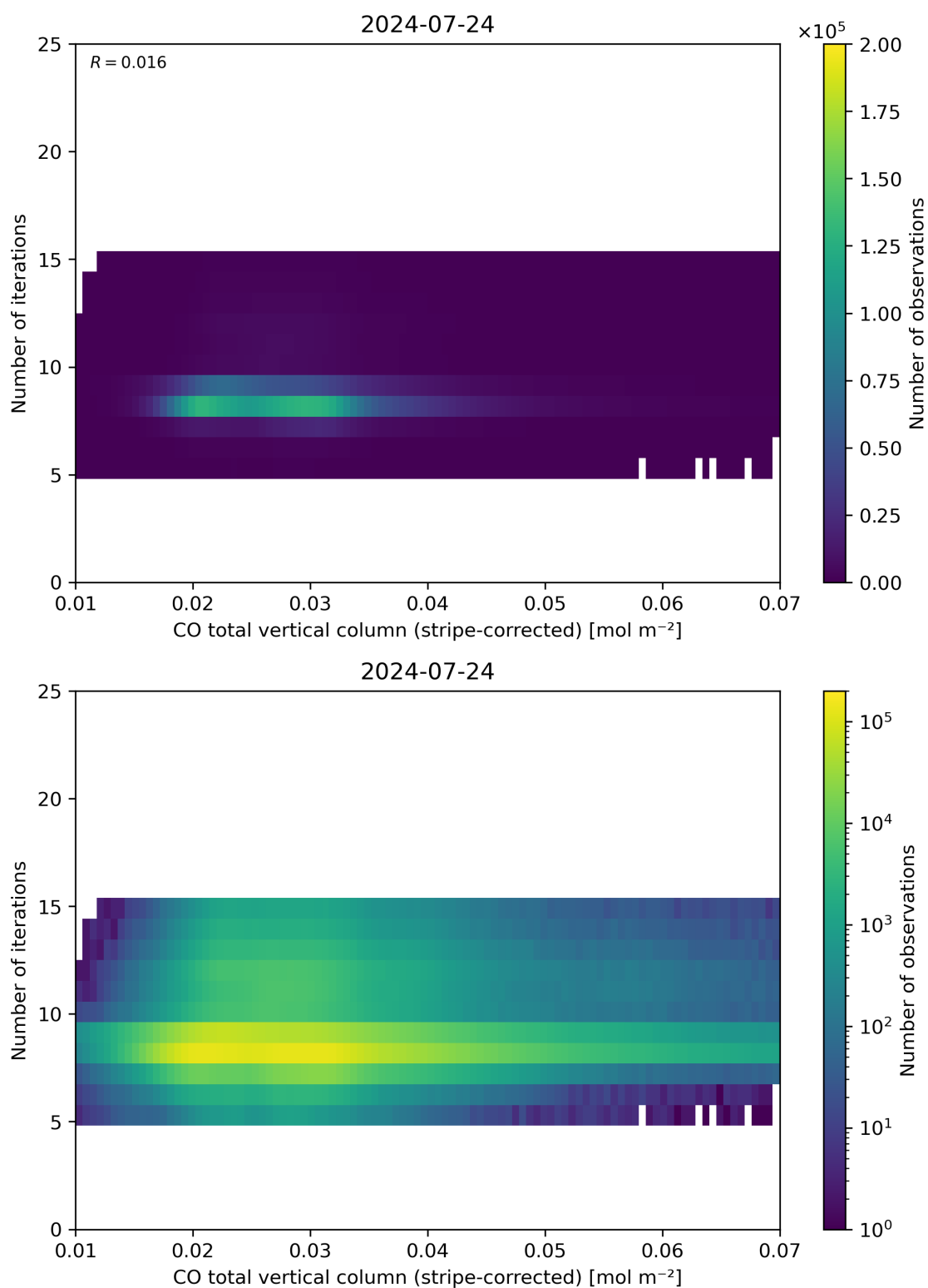
Figure 39: Scatter density plot of “CO total vertical column (stripe-corrected)” against “Number of iterations” for 2024-07-23 to 2024-07-25.
