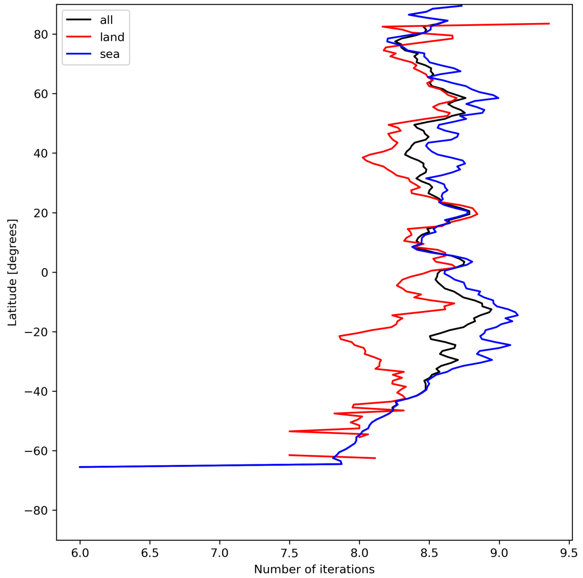
Figure 16: Zonal average of “Number of iterations” for 2024-07-23 to 2024-07-25.
