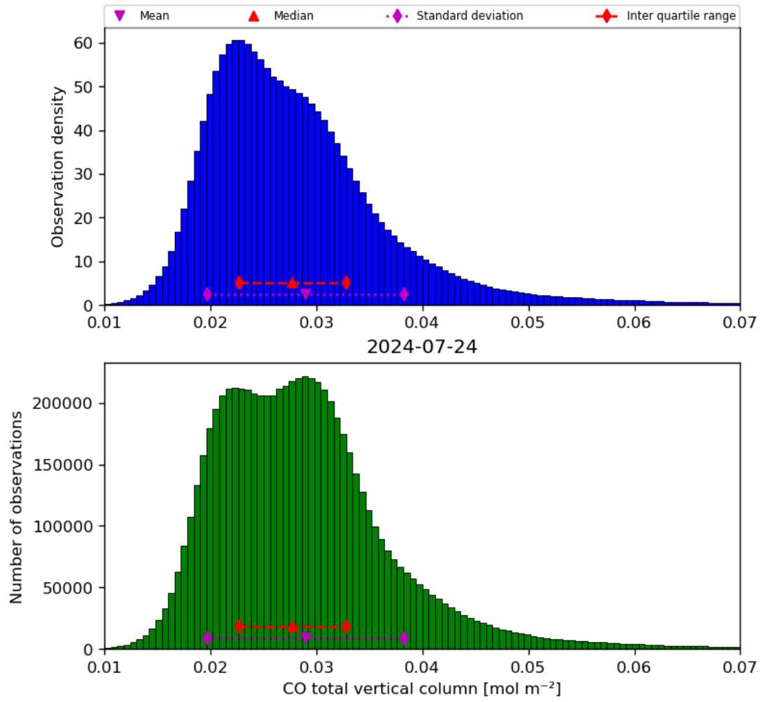
Figure 18: Histogram of “CO total vertical column” for 2024-07-23 to 2024-07-25
