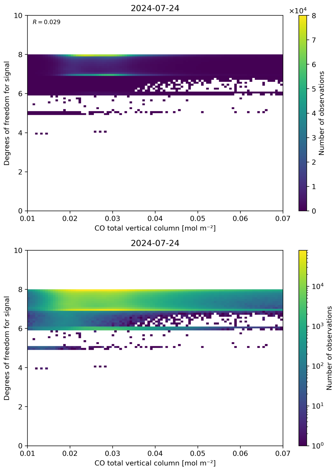
Figure 41: Scatter density plot of “CO total vertical column” against “Degrees of freedom for signal” for 2024-07-23 to 2024-07-25.
