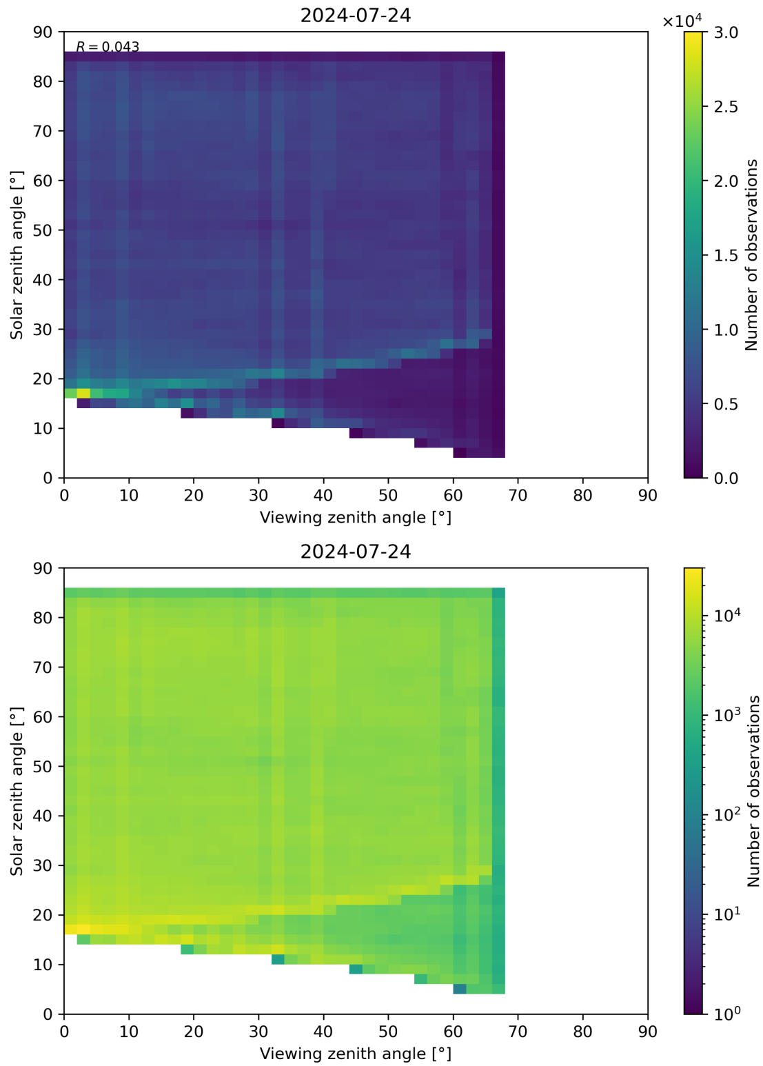
Figure 77: Scatter density plot of “Viewing zenith angle” against “Solar zenith angle” for 2024-07-23 to 2024-07-25.
