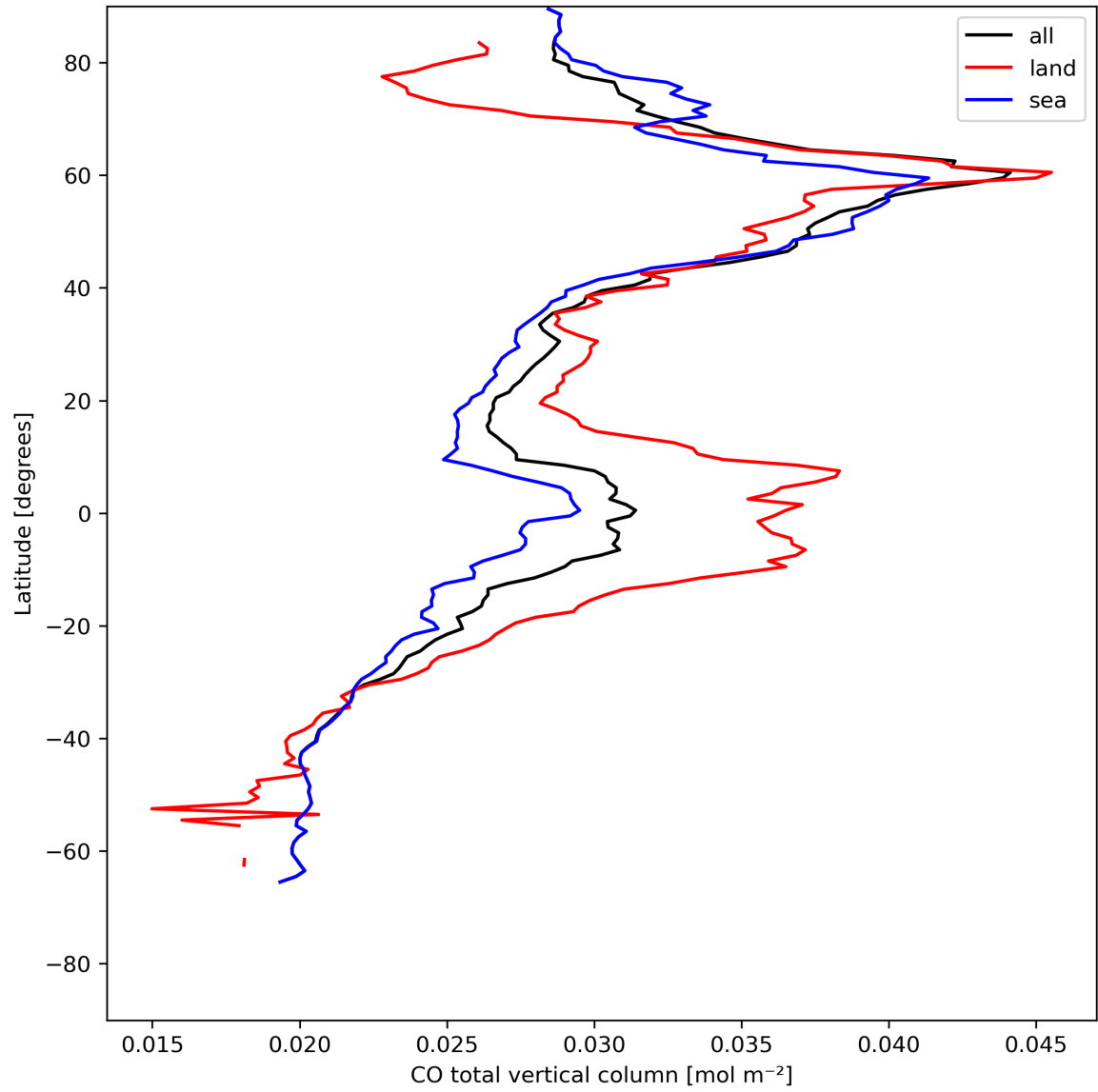
Figure 10: Zonal average of “CO total vertical column” for 2024-07-23 to 2024-07-25.
