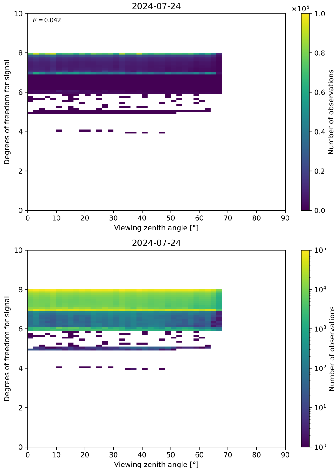
Figure 73: Scatter density plot of “Viewing zenith angle” against “Degrees of freedom for signal” for 2024-07-23 to 2024-07-25.
