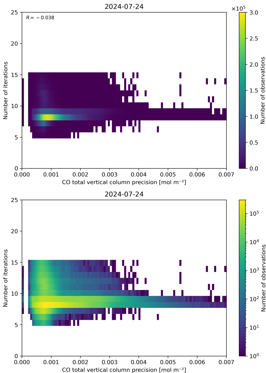
Figure 46: Scatter density plot of “CO total vertical column precision” against “Number of iterations” for 2024-07-23 to 2024-07-25.
