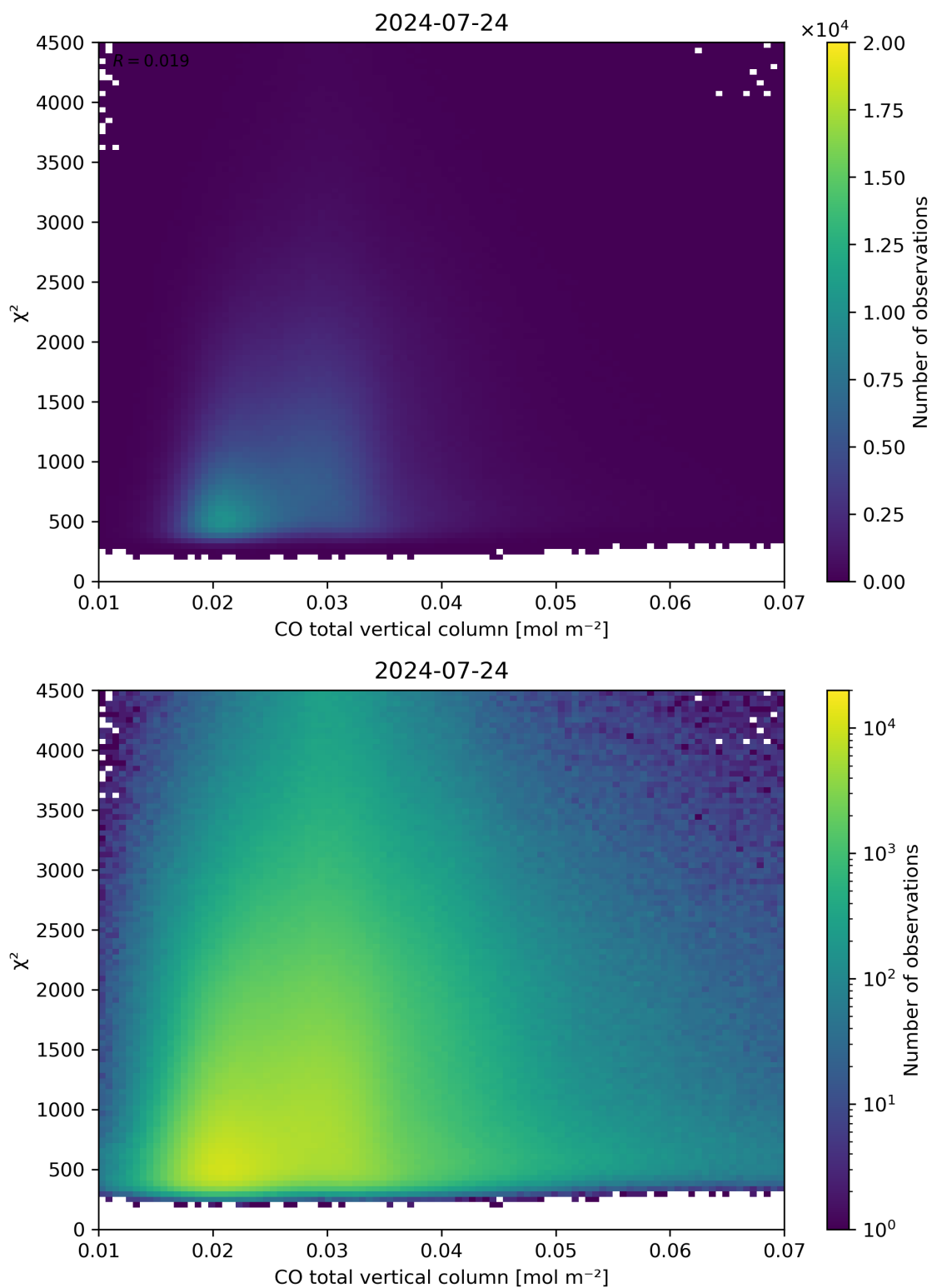
Figure 35: Scatter density plot of “CO total vertical column” against “ \chi^2 ” for 2024-07-23 to 2024-07-25.
