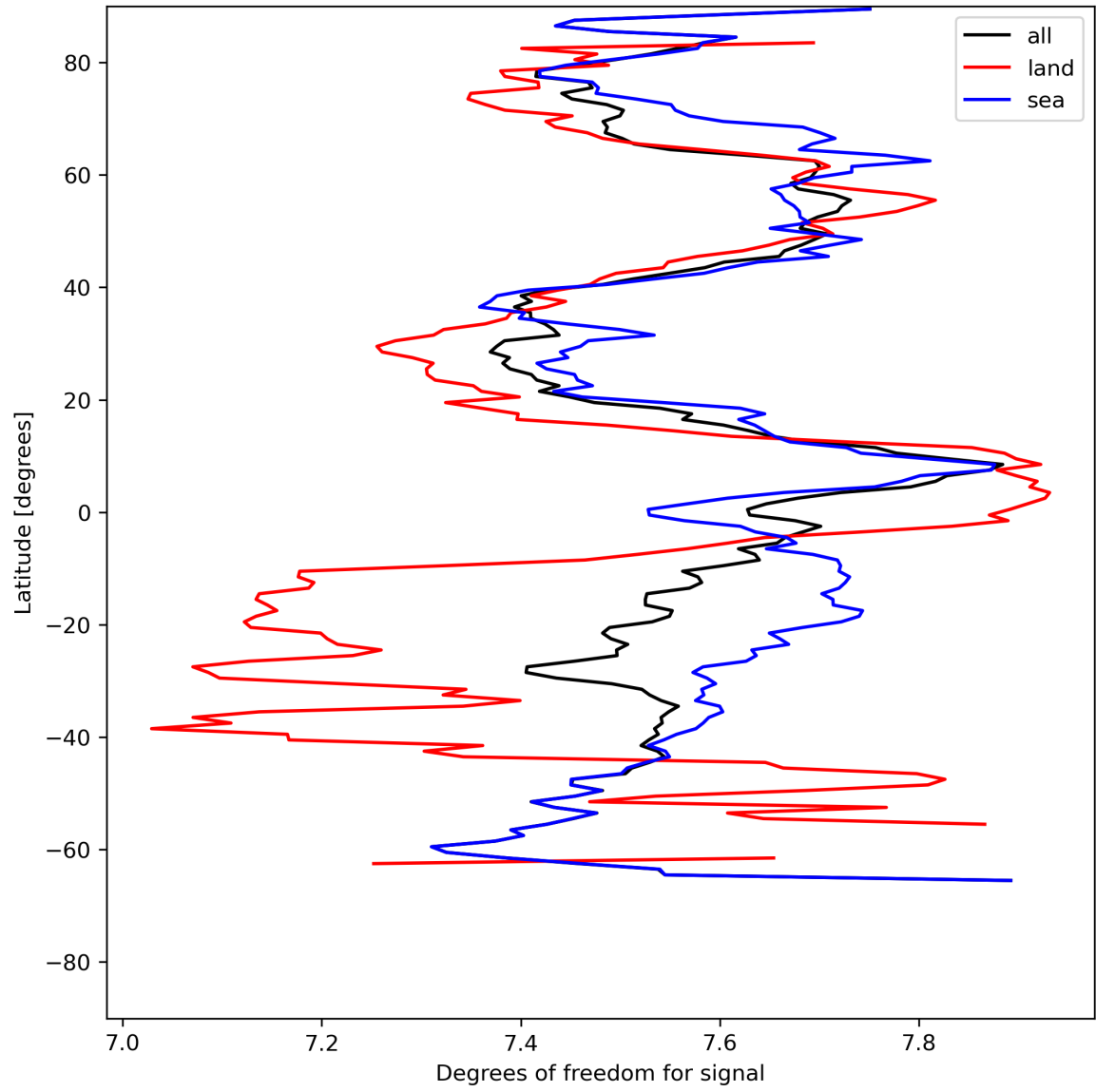
Figure 15: Zonal average of “Degrees of freedom for signal” for 2024-07-23 to 2024-07-25.
