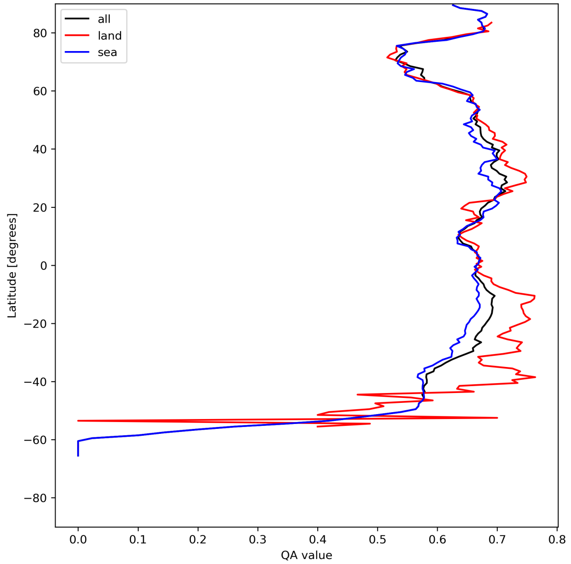
Figure 9: Zonal average of “QA value” for 2024-07-23 to 2024-07-25.
