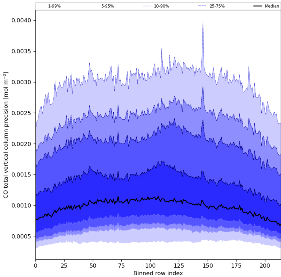
Figure 28: Along track statistics of “CO total vertical column precision” for 2024-07-23 to 2024-07-25
