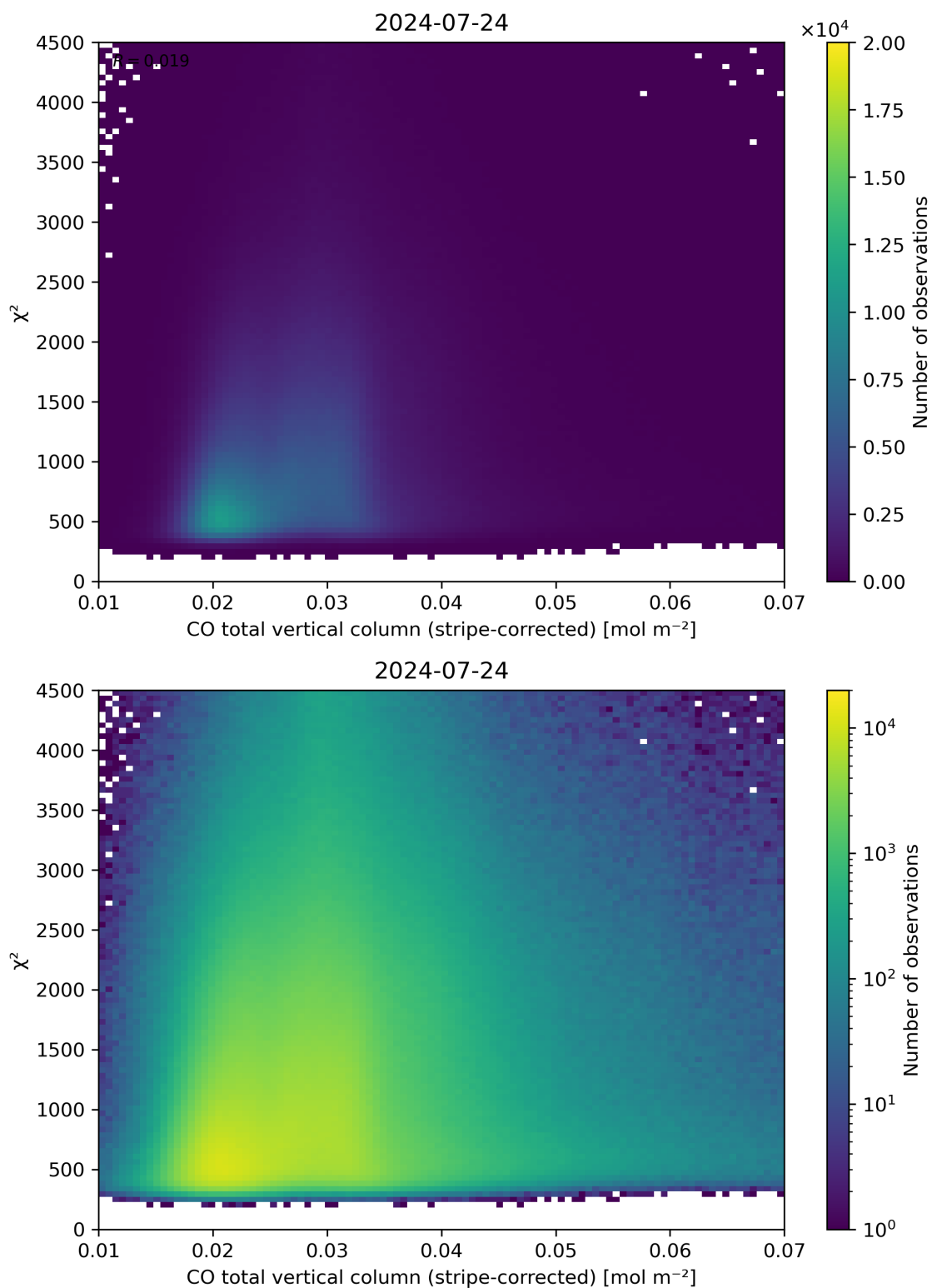
Figure 37: Scatter density plot of “CO total vertical column (stripe-corrected)” against “ \chi^2 ” for 2024-07-23 to 2024-07-25.
