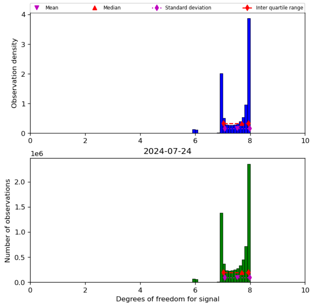
Figure 23: Histogram of “Degrees of freedom for signal” for 2024-07-23 to 2024-07-25
