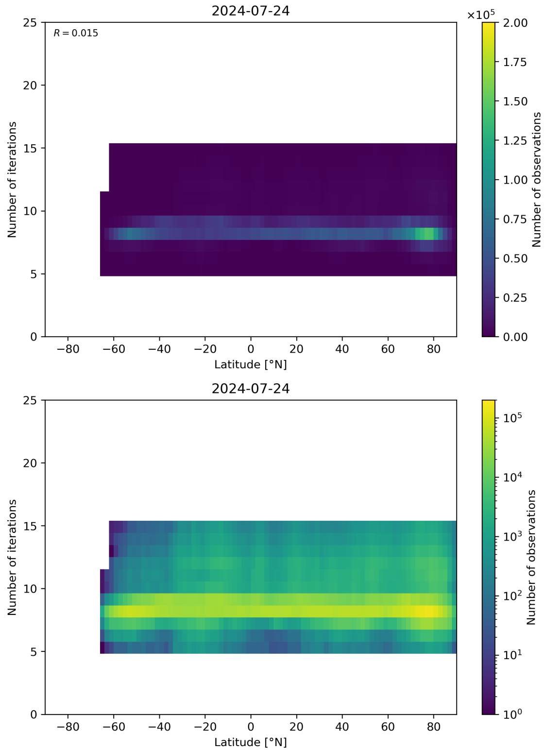
Figure 56: Scatter density plot of “Latitude” against “Number of iterations” for 2024-07-23 to 2024-07-25.
