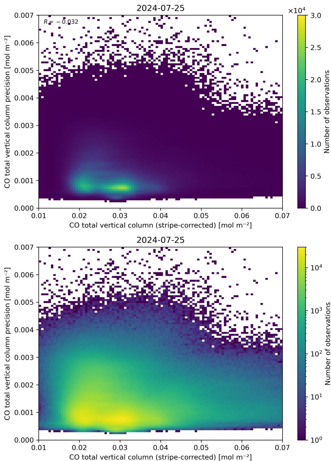
Figure 36: Scatter density plot of “CO total vertical column (stripe-corrected)” against “CO total vertical column precision” for 2024-07-24 to 2024-07-26.
