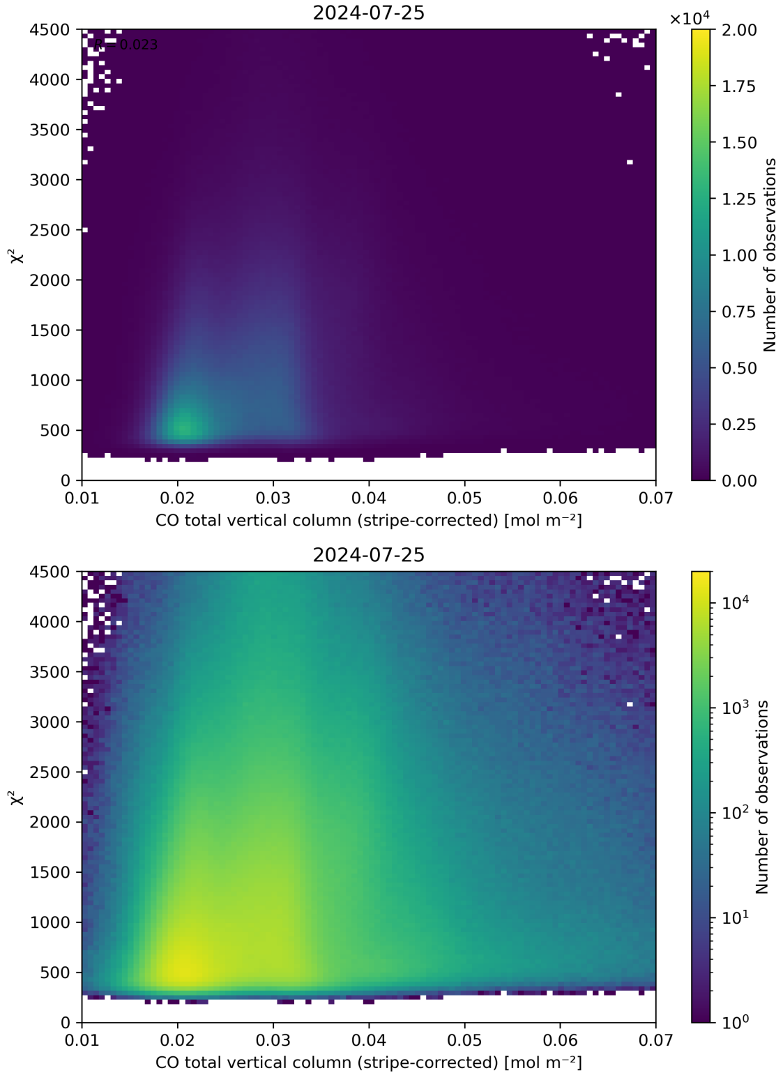
Figure 37: Scatter density plot of “CO total vertical column (stripe-corrected)” against “ \chi^2 ” for 2024-07-24 to 2024-07-26.
