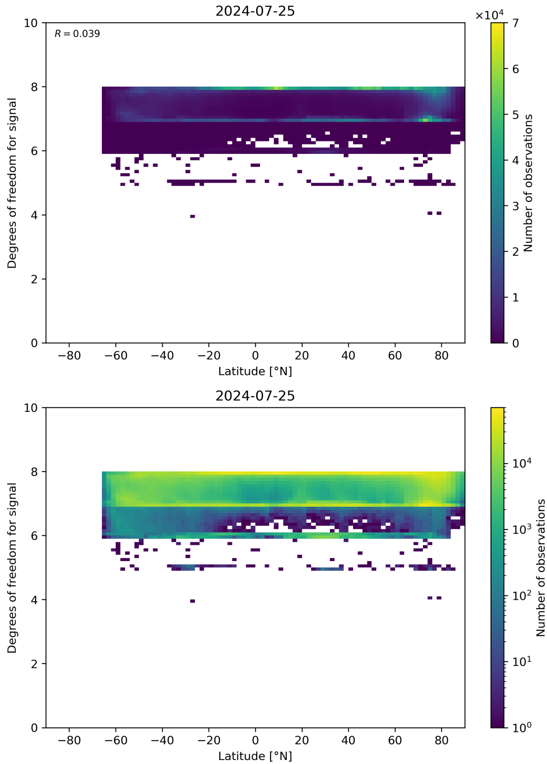
Figure 55: Scatter density plot of “Latitude” against “Degrees of freedom for signal” for 2024-07-24 to 2024-07-26.
