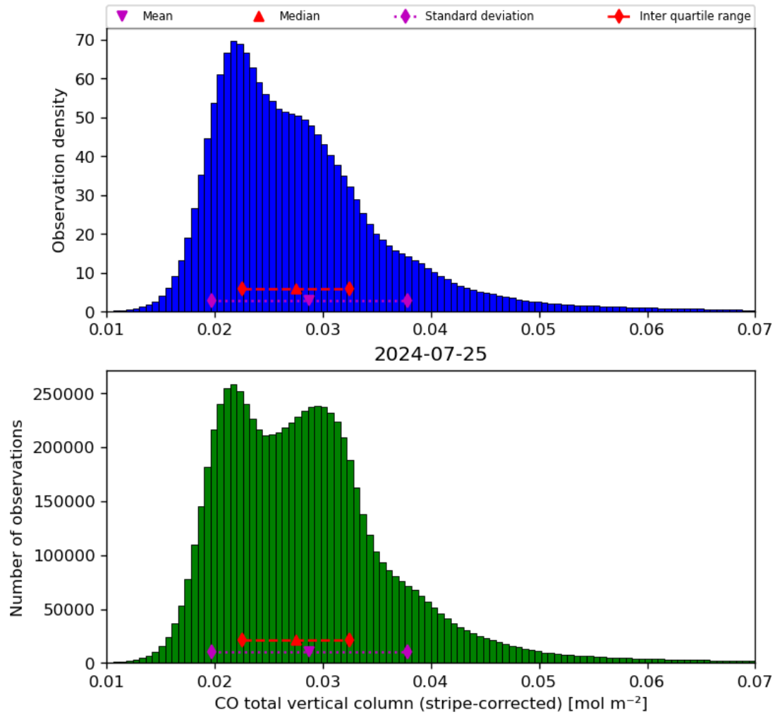
Figure 19: Histogram of “CO total vertical column (stripe-corrected)” for 2024-07-24 to 2024-07-26
