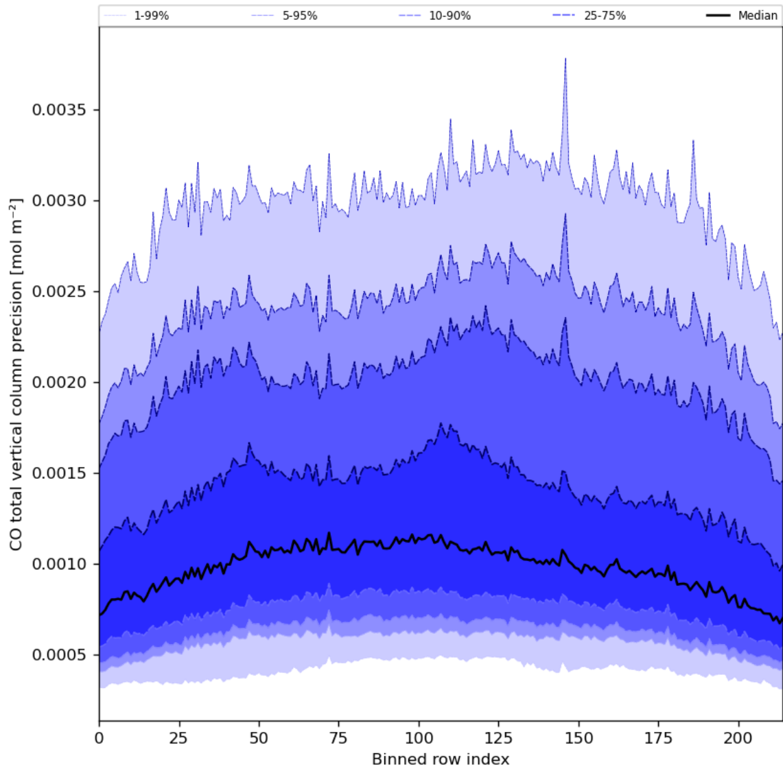
Figure 28: Along track statistics of “CO total vertical column precision” for 2024-07-24 to 2024-07-26
