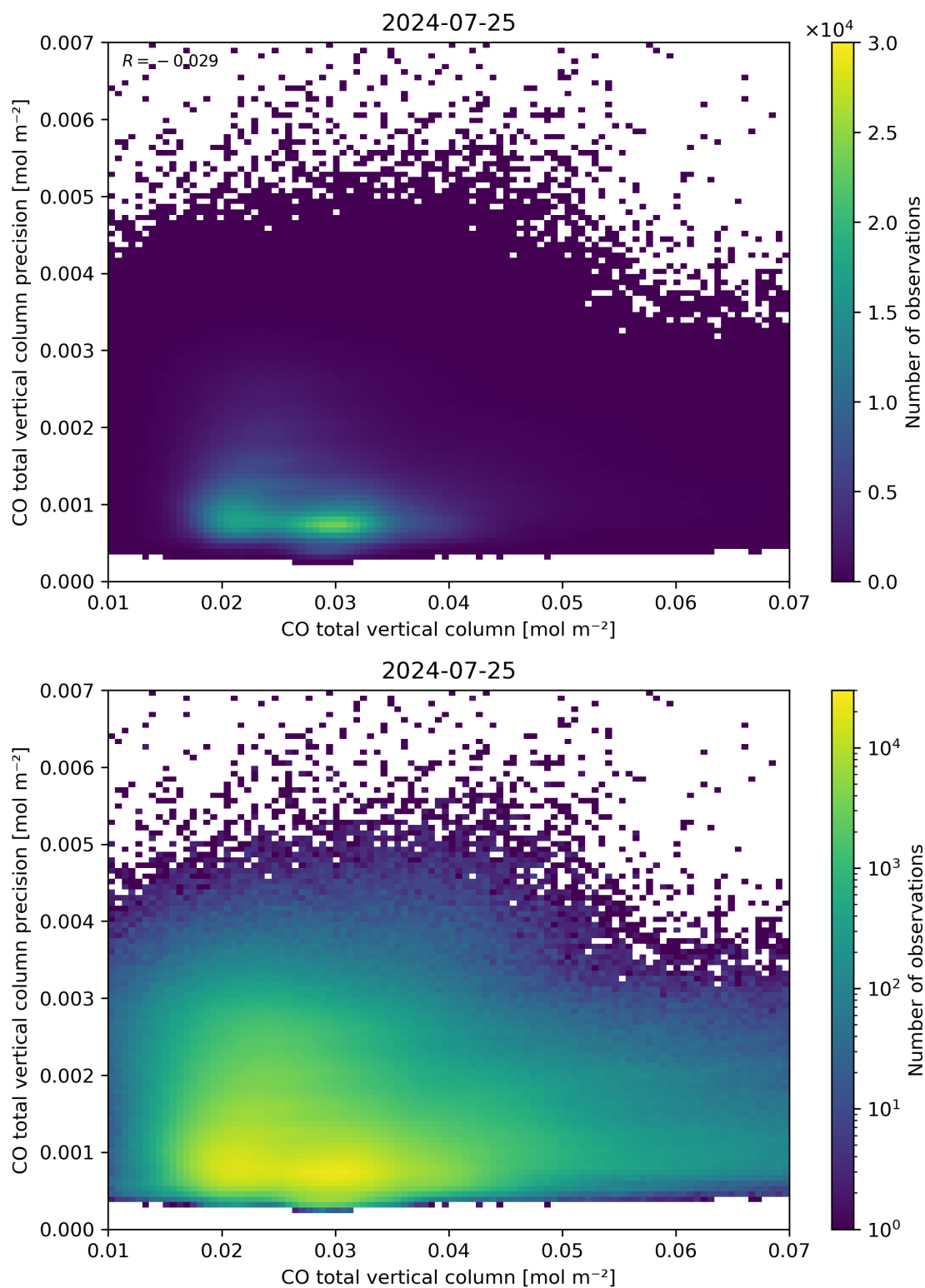
Figure 34: Scatter density plot of “CO total vertical column” against “CO total vertical column precision” for 2024-07-24 to 2024-07-26.
