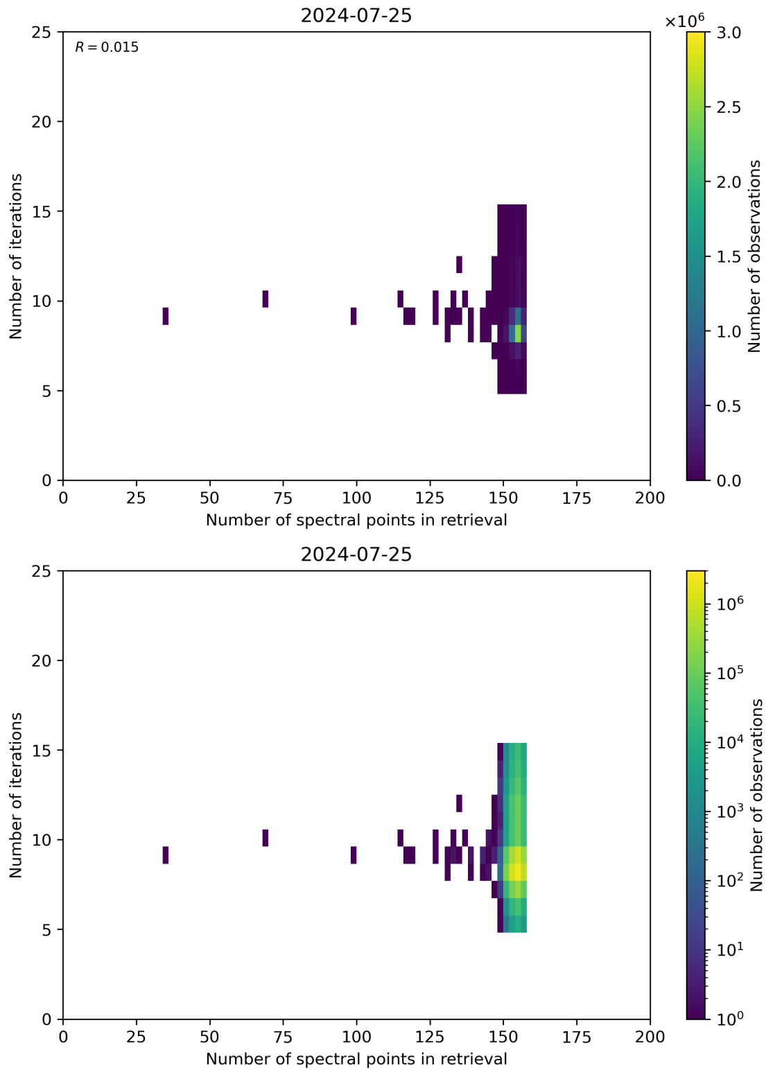
Figure 60: Scatter density plot of “Number of spectral points in retrieval” against “Number of iterations” for 2024-07-24 to 2024-07-26.
