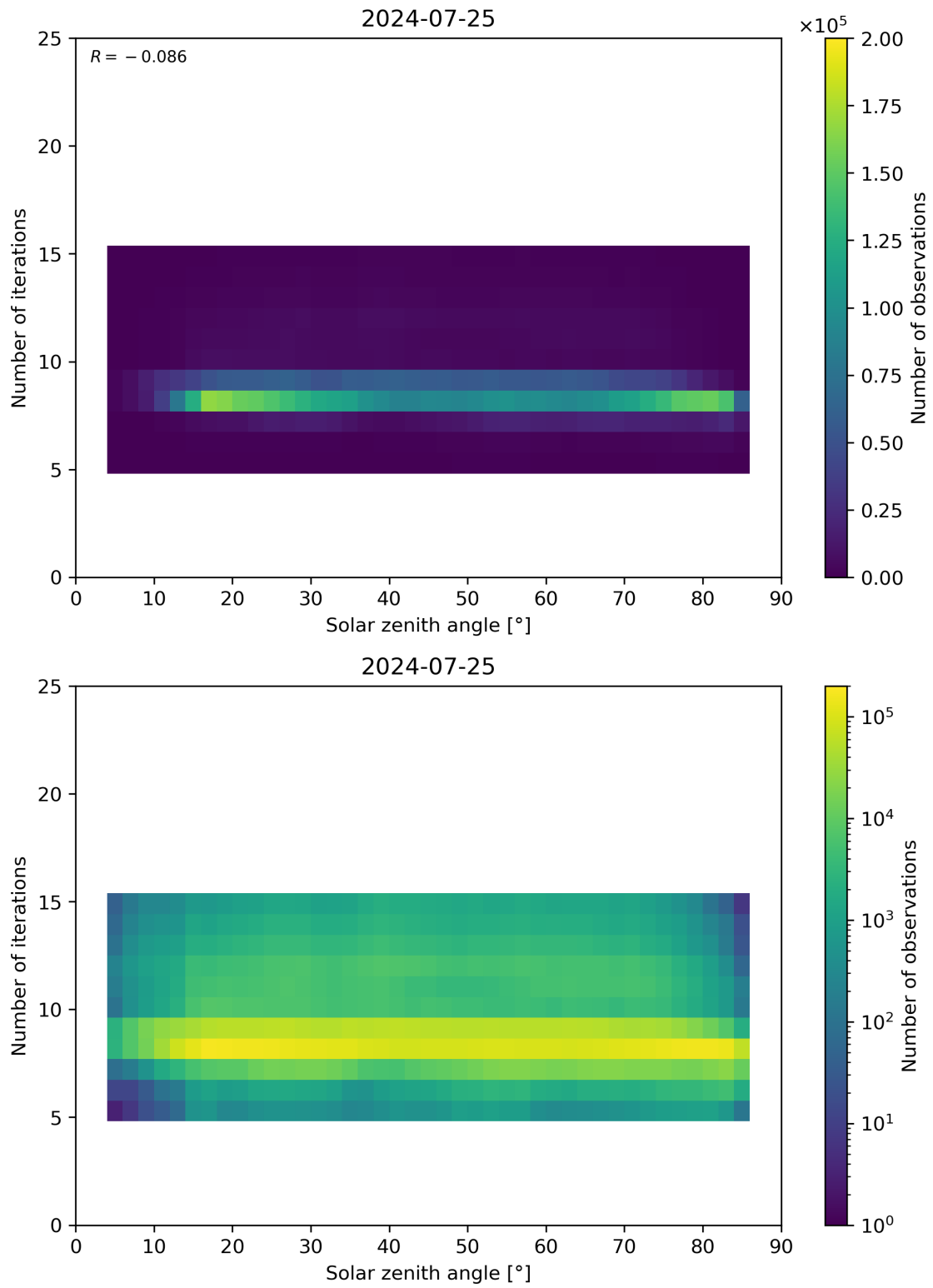
Figure 67: Scatter density plot of “Solar zenith angle” against “Number of iterations” for 2024-07-24 to 2024-07-26.
