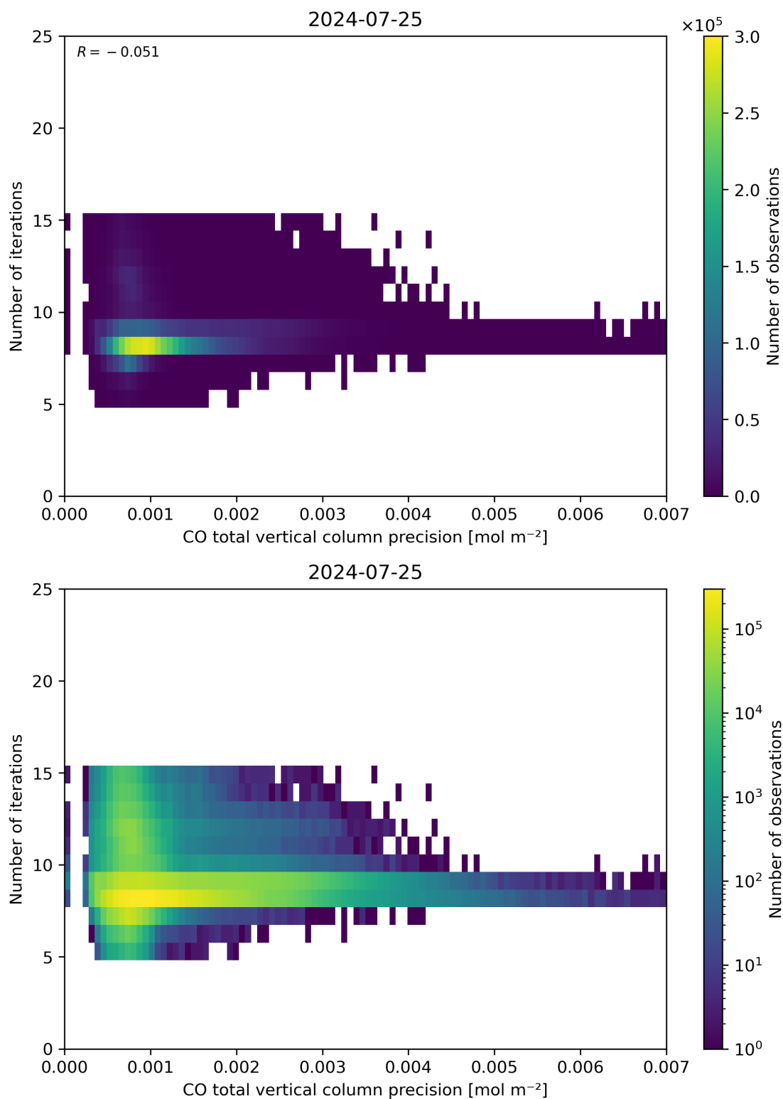
Figure 46: Scatter density plot of “CO total vertical column precision” against “Number of iterations” for 2024-07-24 to 2024-07-26.
