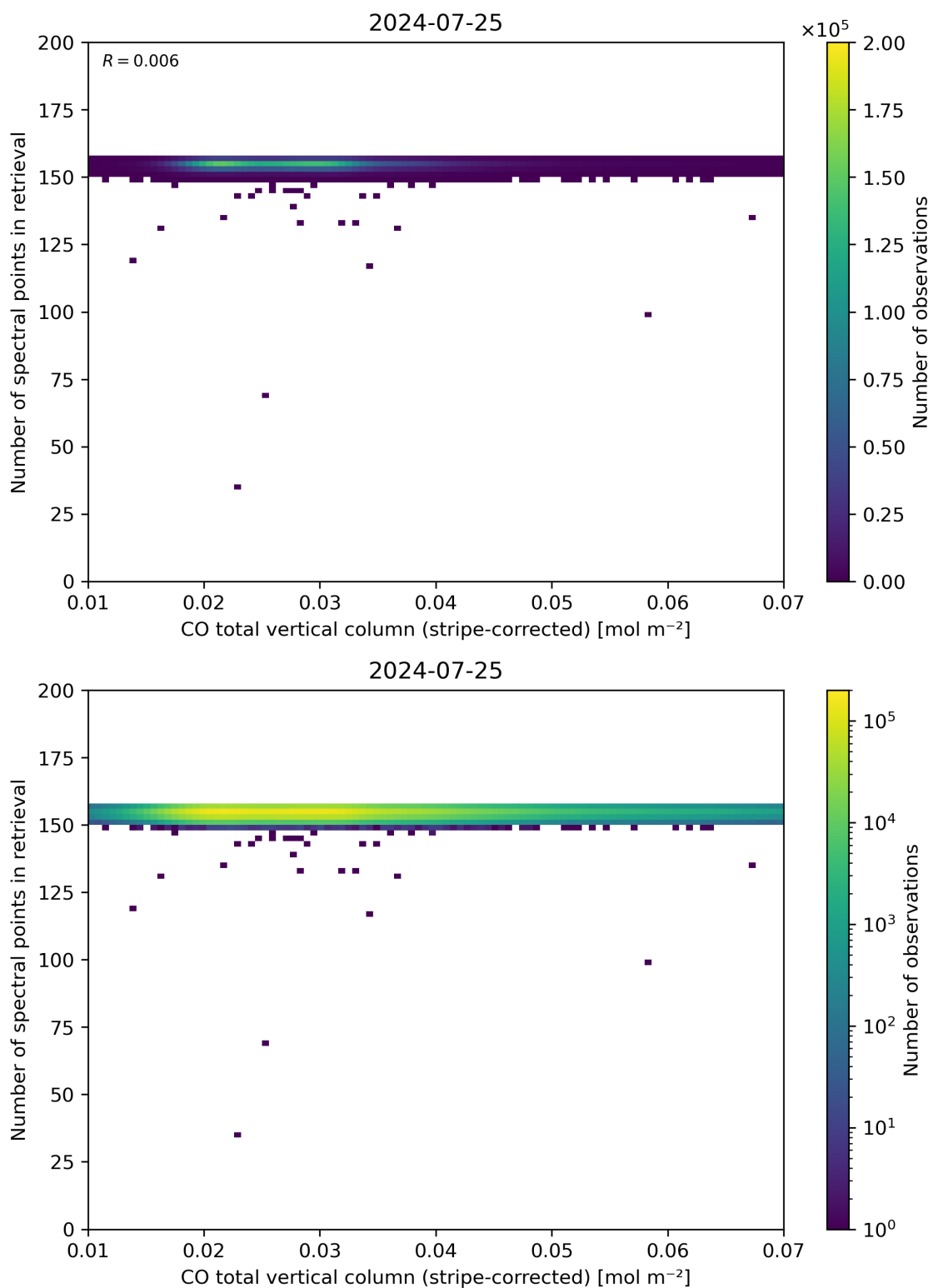
Figure 40: Scatter density plot of “CO total vertical column (stripe-corrected)” against “Number of spectral points in retrieval” for 2024-07-24 to 2024-07-26.
