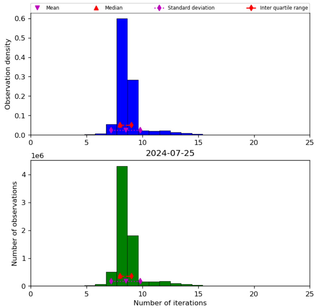
Figure 24: Histogram of “Number of iterations” for 2024-07-24 to 2024-07-26
