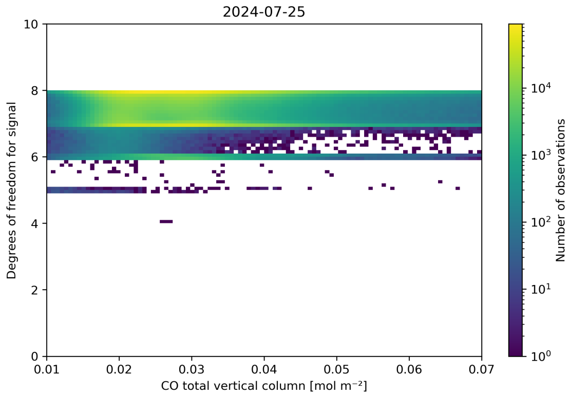
Figure 41: Scatter density plot of “CO total vertical column” against “Degrees of freedom for signal” for 2024-07-24 to 2024-07-26.
