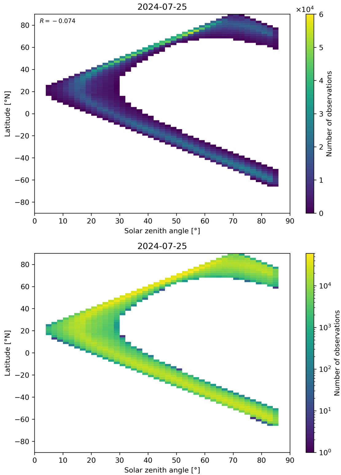
Figure 66: Scatter density plot of “Solar zenith angle” against “Latitude” for 2024-07-24 to 2024-07-26.
