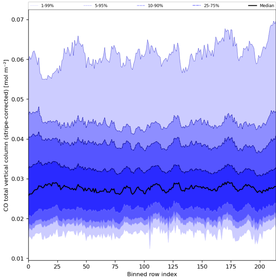
Figure 27: Along track statistics of “CO total vertical column (stripe-corrected)” for 2024-07-24 to 2024-07-26
