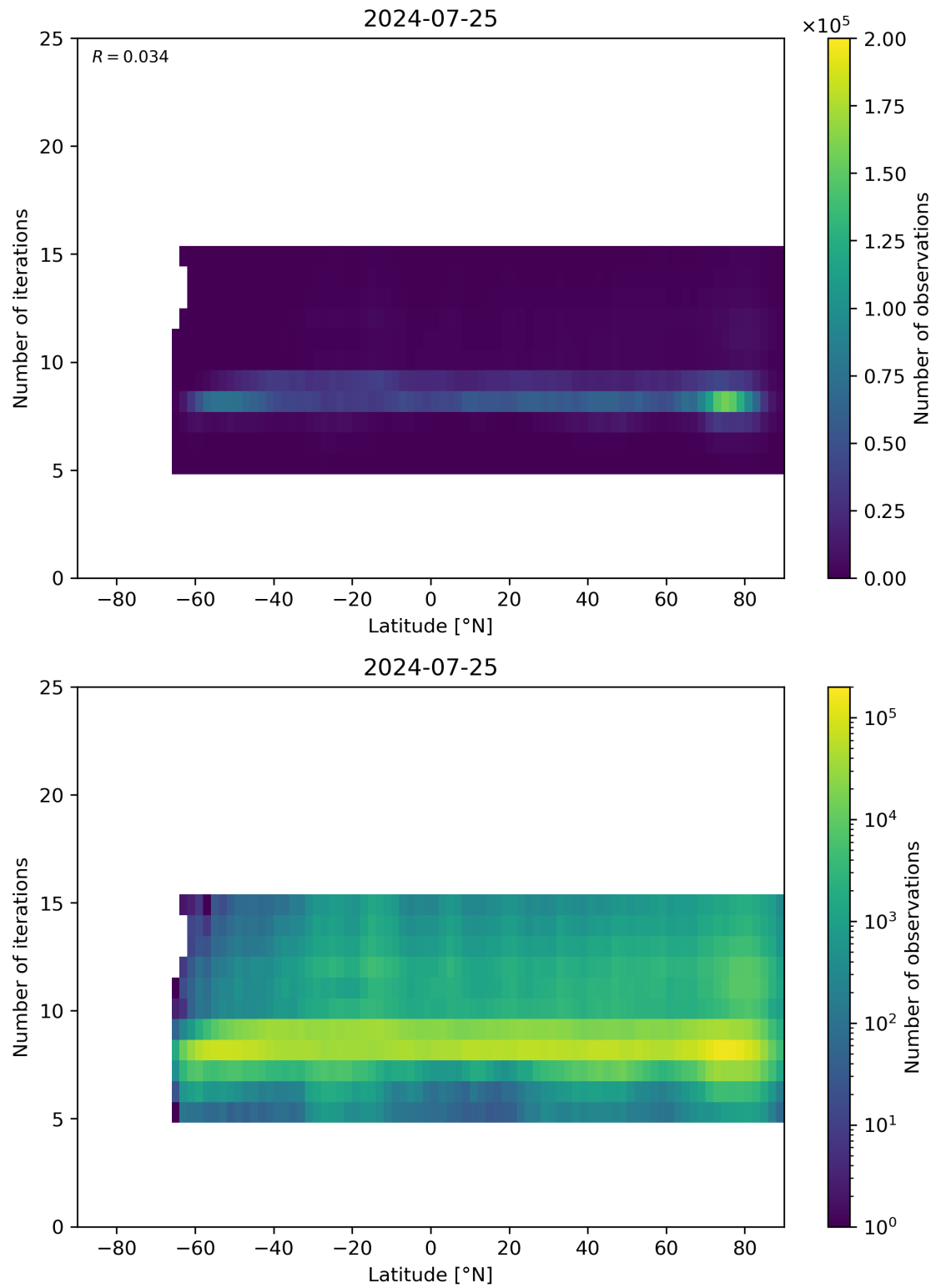
Figure 56: Scatter density plot of “Latitude” against “Number of iterations” for 2024-07-24 to 2024-07-26.
