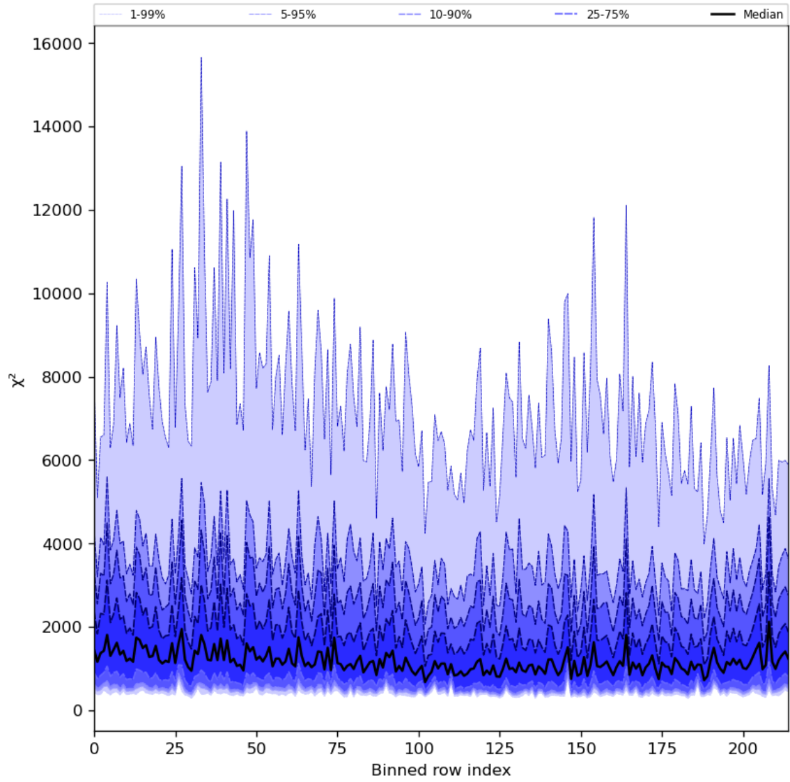
Figure 30: Along track statistics of “ \chi^2 ” for 2024-07-24 to 2024-07-26
