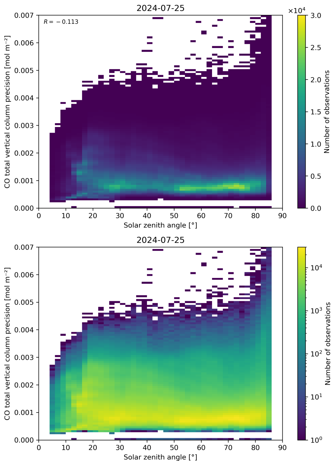
Figure 63: Scatter density plot of “Solar zenith angle” against “CO total vertical column precision” for 2024-07-24 to 2024-07-26.
