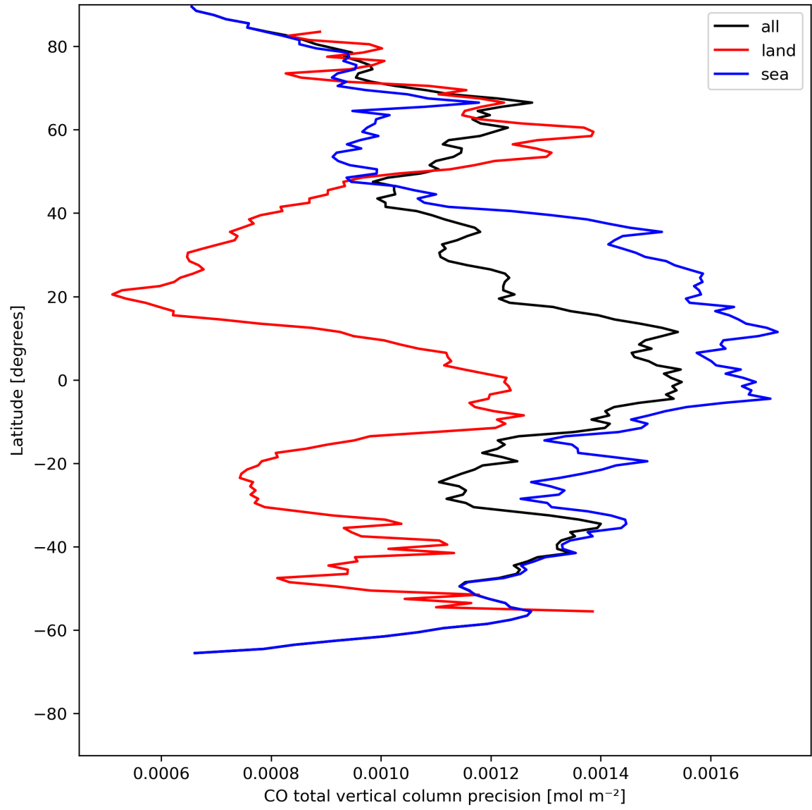
Figure 12: Zonal average of “CO total vertical column precision” for 2024-07-24 to 2024-07-26.
