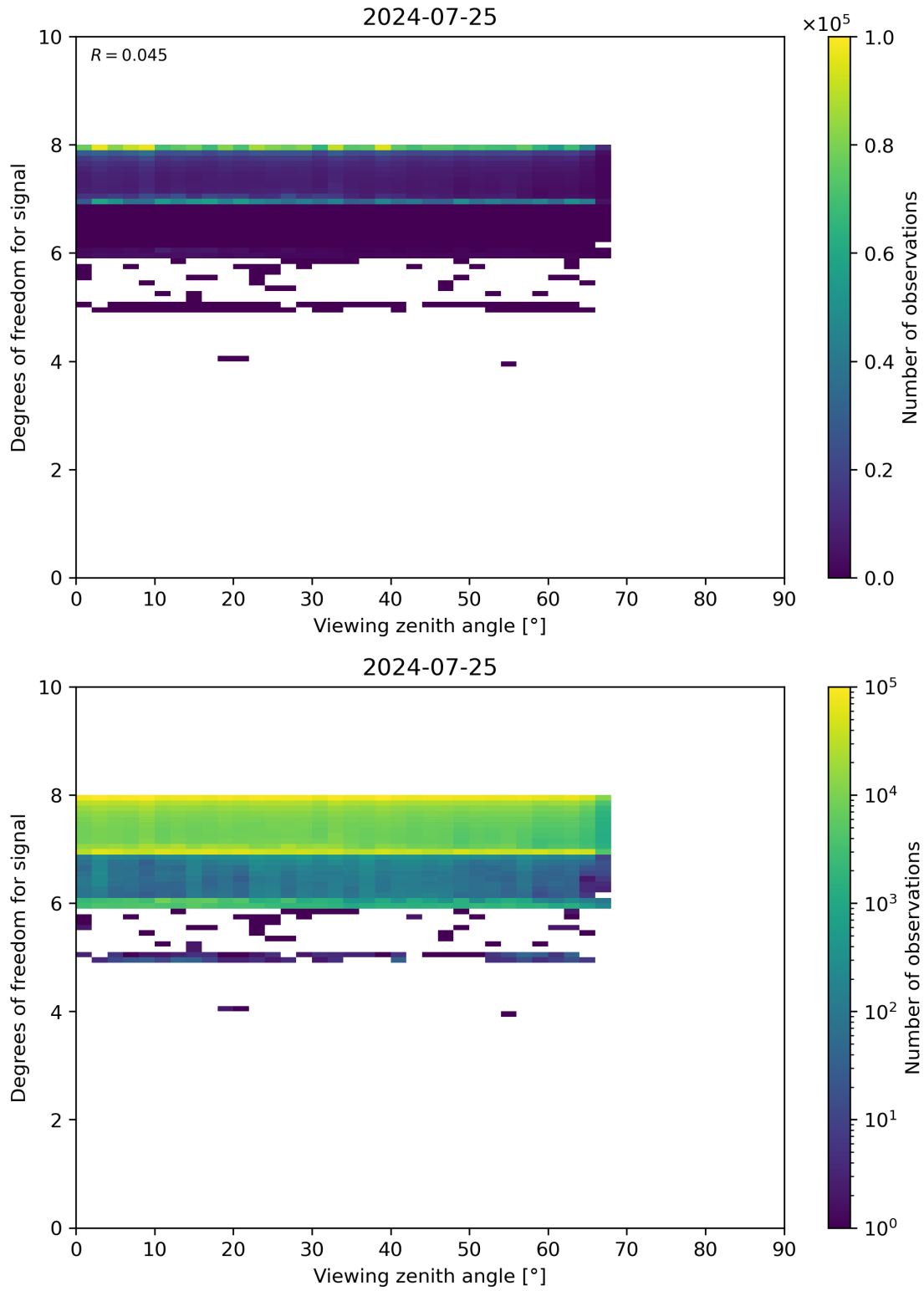
Figure 73: Scatter density plot of “Viewing zenith angle” against “Degrees of freedom for signal” for 2024-07-24 to 2024-07-26.
