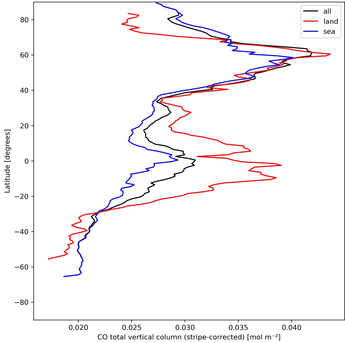
Figure 11: Zonal average of “CO total vertical column (stripe-corrected)” for 2024-07-24 to 2024-07-26.
