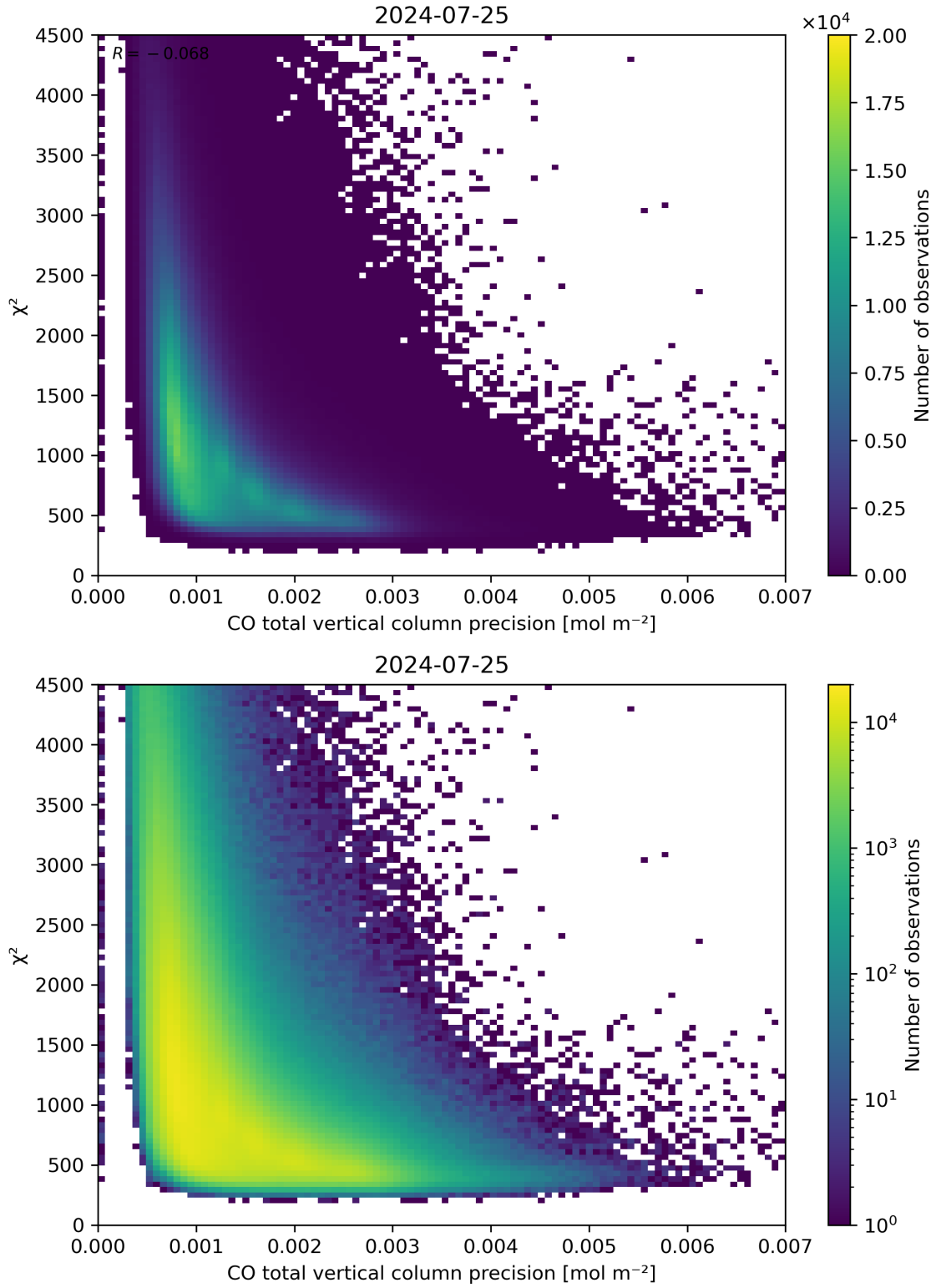
Figure 44: Scatter density plot of “CO total vertical column precision” against “ \chi^2 ” for 2024-07-24 to 2024-07-26.
