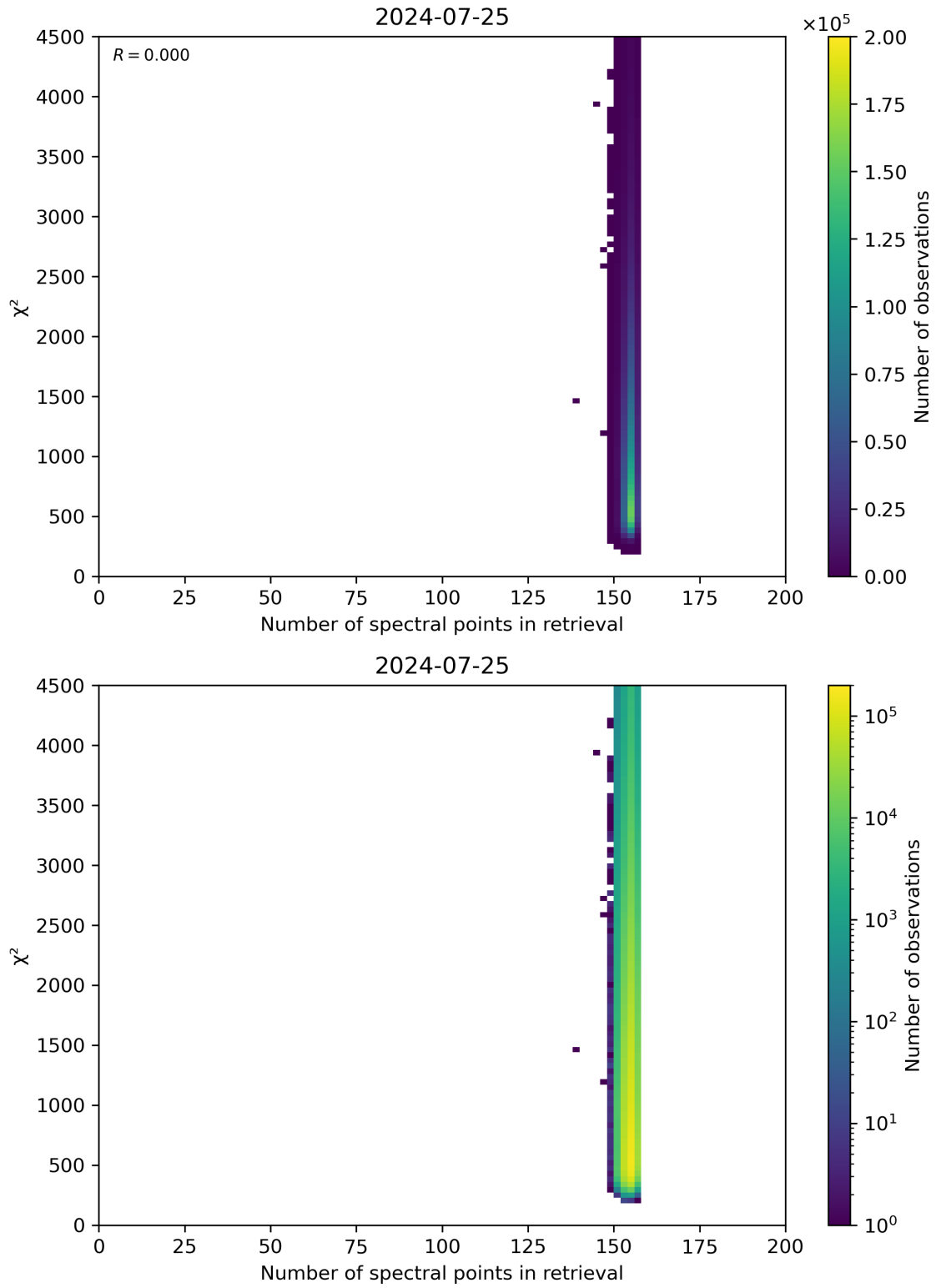
Figure 58: Scatter density plot of “Number of spectral points in retrieval” against “ \chi^2 ” for 2024-07-24 to 2024-07-26.
