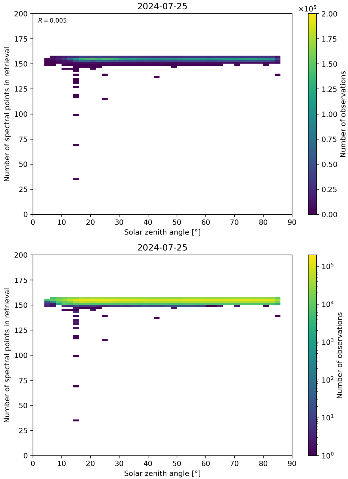
Figure 68: Scatter density plot of “Solar zenith angle” against “Number of spectral points in retrieval” for 2024-07-24 to 2024-07-26.
