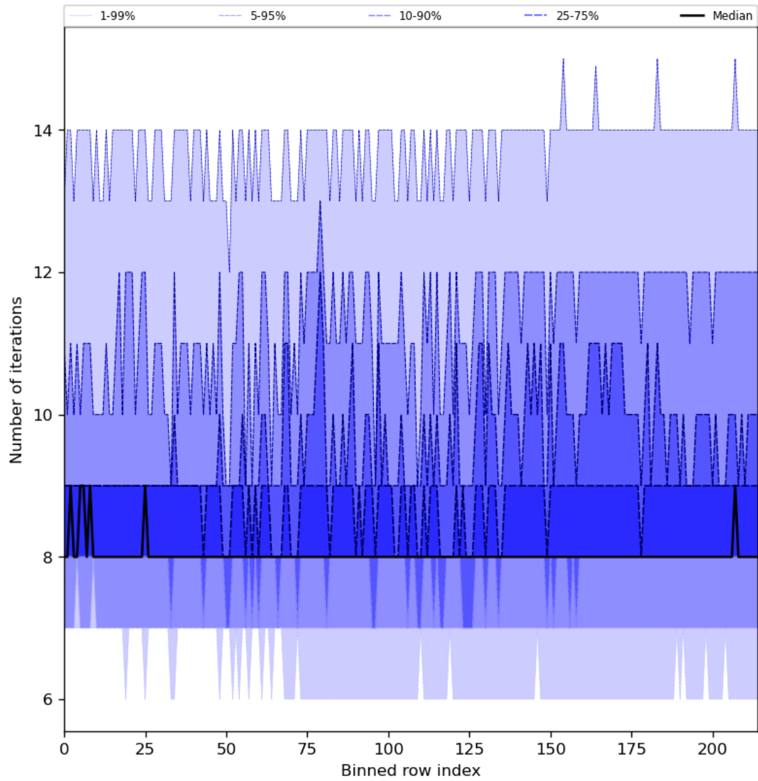
Figure 32: Along track statistics of “Number of iterations” for 2024-07-24 to 2024-07-26
