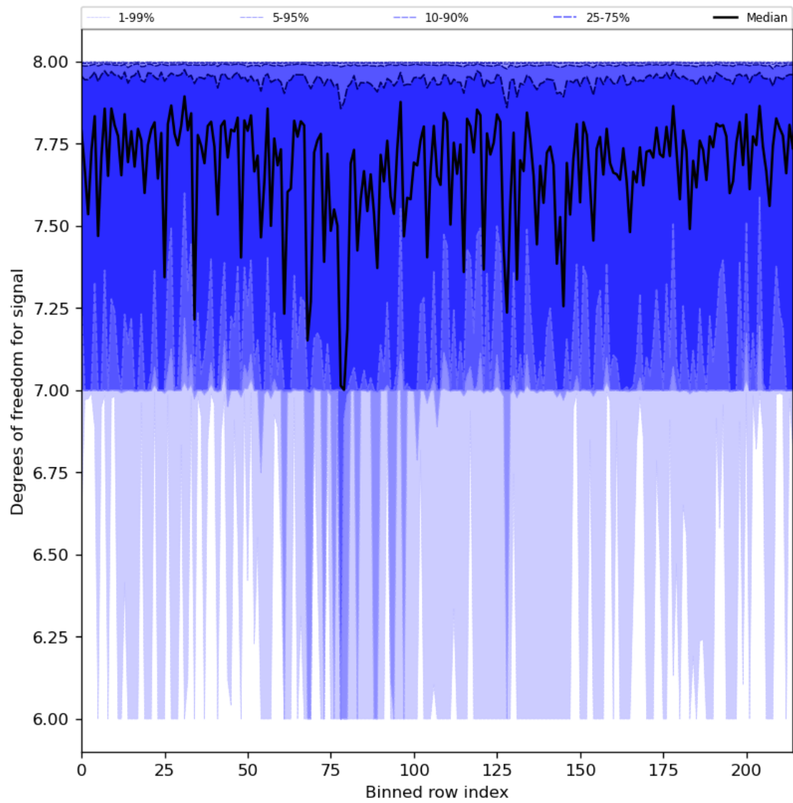
Figure 31: Along track statistics of “Degrees of freedom for signal” for 2024-07-24 to 2024-07-26
