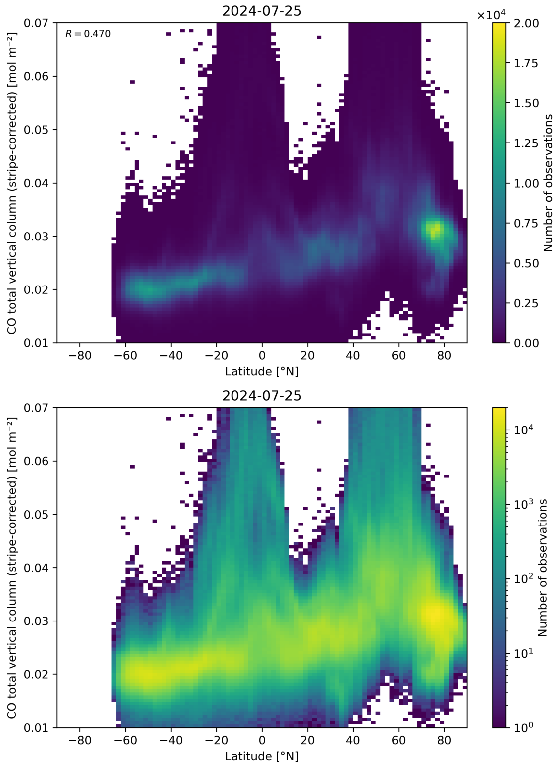
Figure 52: Scatter density plot of “Latitude” against “CO total vertical column (stripe-corrected)” for 2024-07-24 to 2024-07-26.
