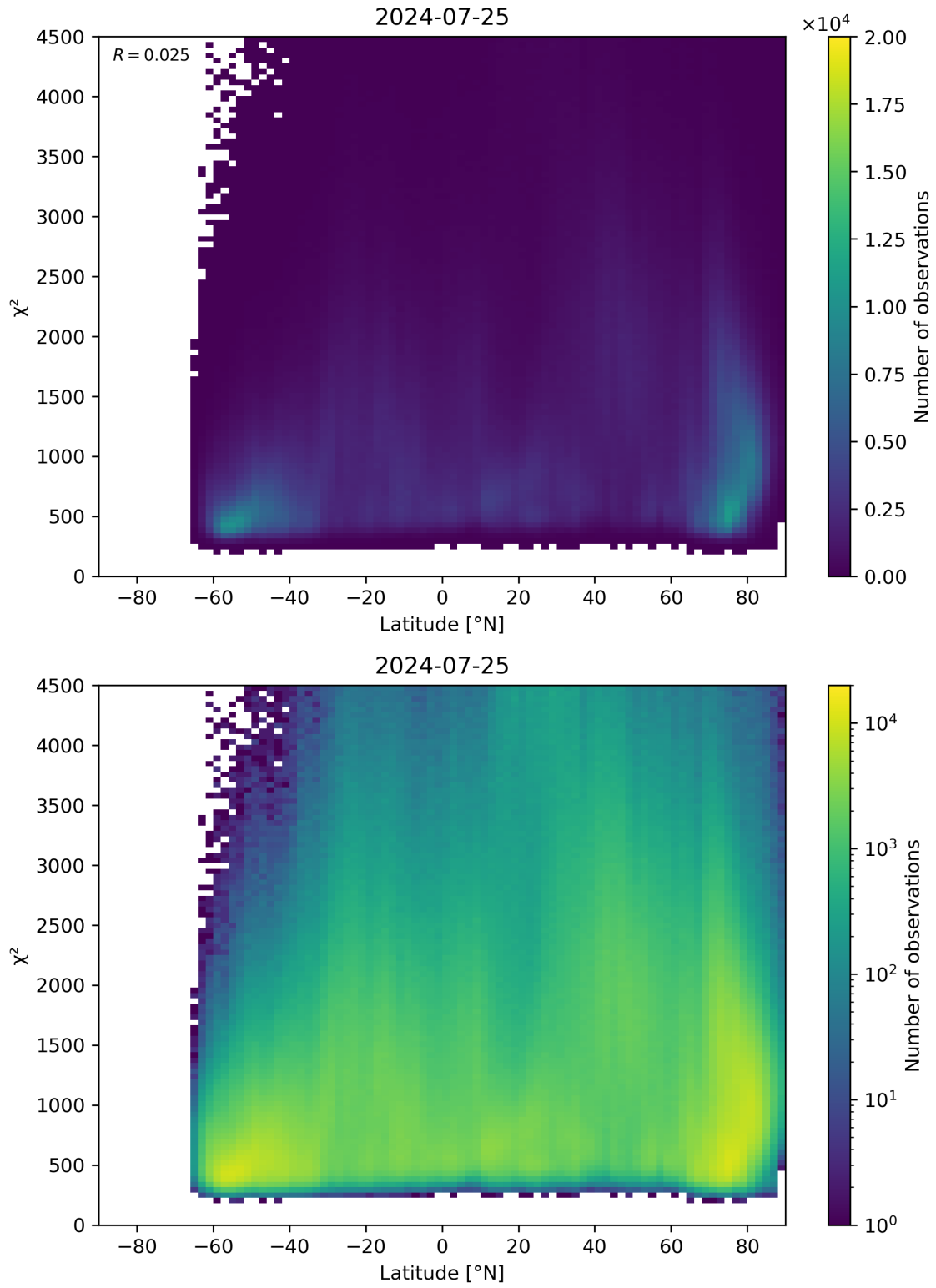
Figure 54: Scatter density plot of “Latitude” against “ \chi^2 ” for 2024-07-24 to 2024-07-26.
