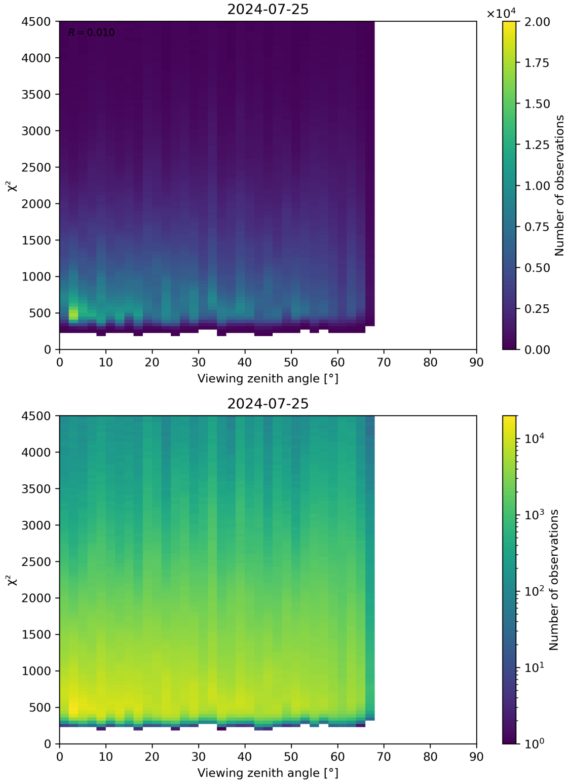
Figure 72: Scatter density plot of “Viewing zenith angle” against “ \chi^2 ” for 2024-07-24 to 2024-07-26.
