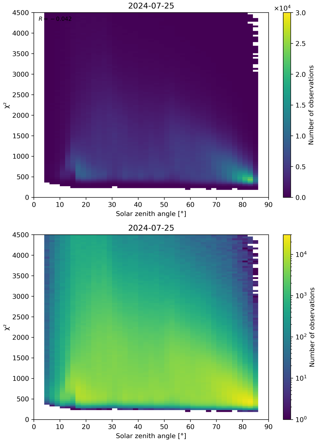
Figure 64: Scatter density plot of “Solar zenith angle” against “ \chi^2 ” for 2024-07-24 to 2024-07-26.
