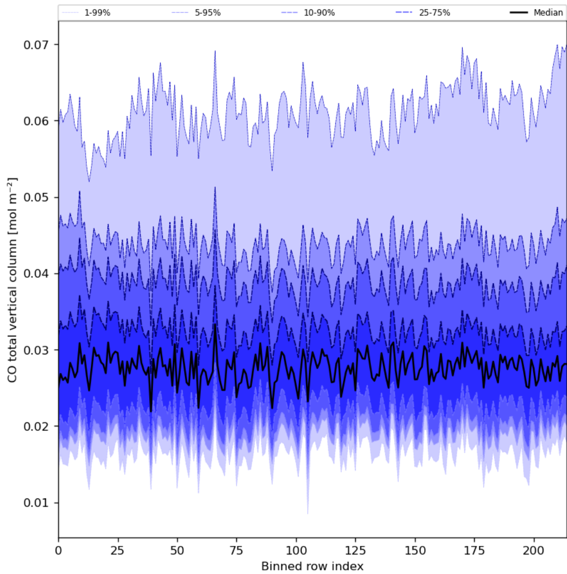
Figure 26: Along track statistics of “CO total vertical column” for 2024-07-24 to 2024-07-26
