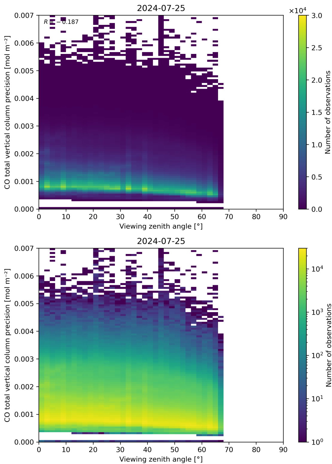
Figure 71: Scatter density plot of “Viewing zenith angle” against “CO total vertical column precision” for 2024-07-24 to 2024-07-26.
