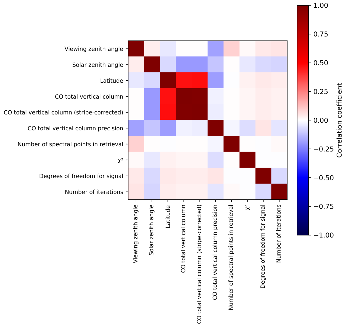
Figure 2: Map of correlation matrix for 2024-07-24 to 2024-07-26.
