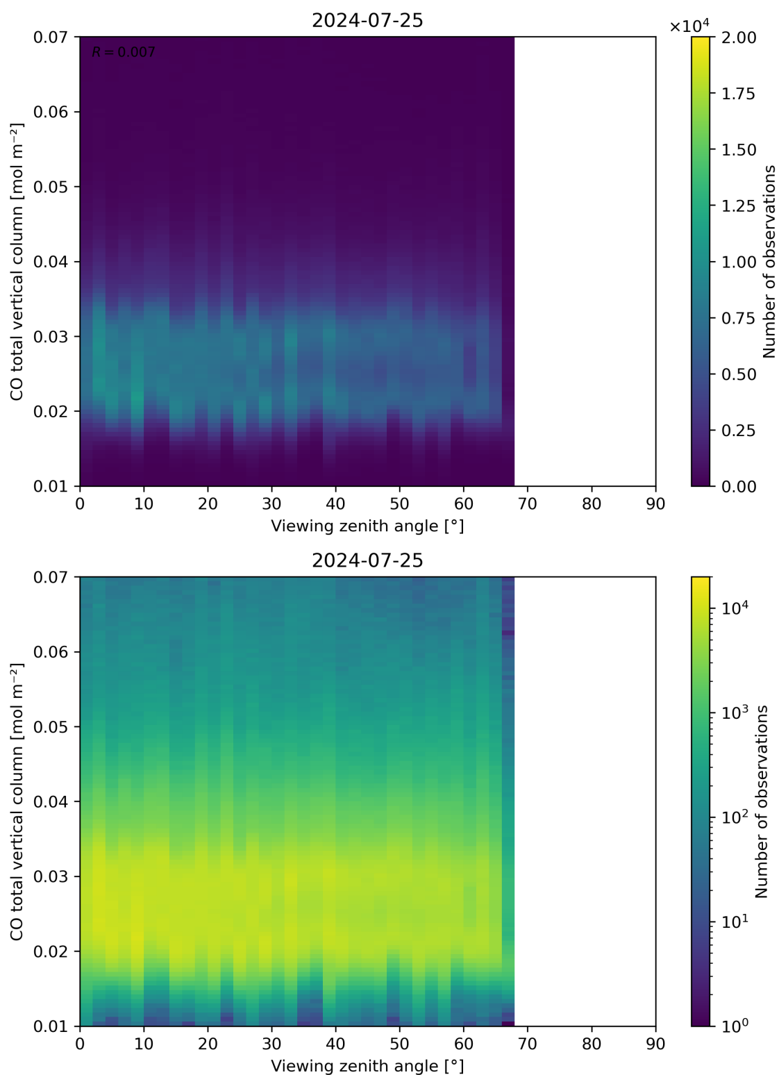
Figure 69: Scatter density plot of “Viewing zenith angle” against “CO total vertical column” for 2024-07-24 to 2024-07-26.
