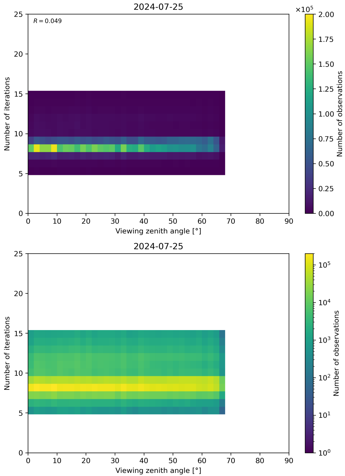
Figure 75: Scatter density plot of “Viewing zenith angle” against “Number of iterations” for 2024-07-24 to 2024-07-26.
