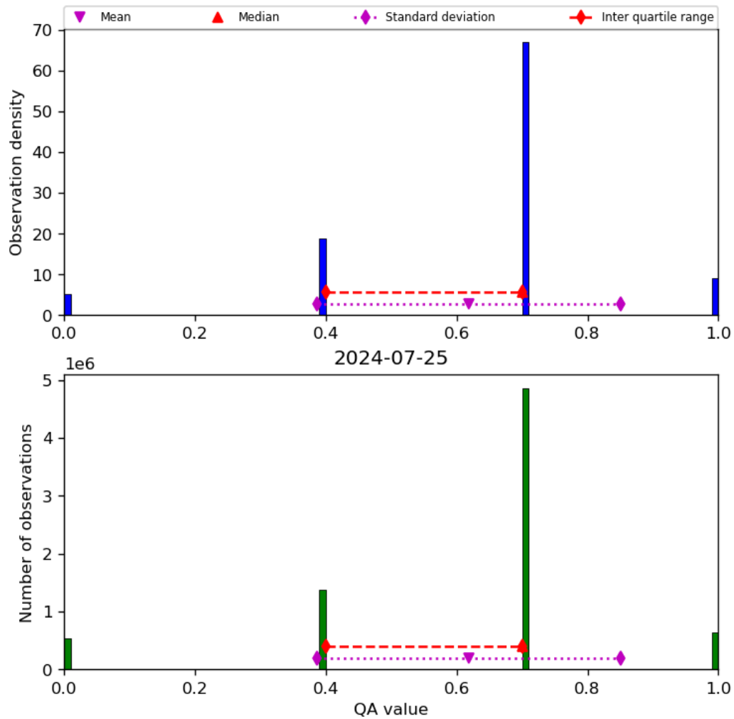
Figure 17: Histogram of “QA value” for 2024-07-24 to 2024-07-26
