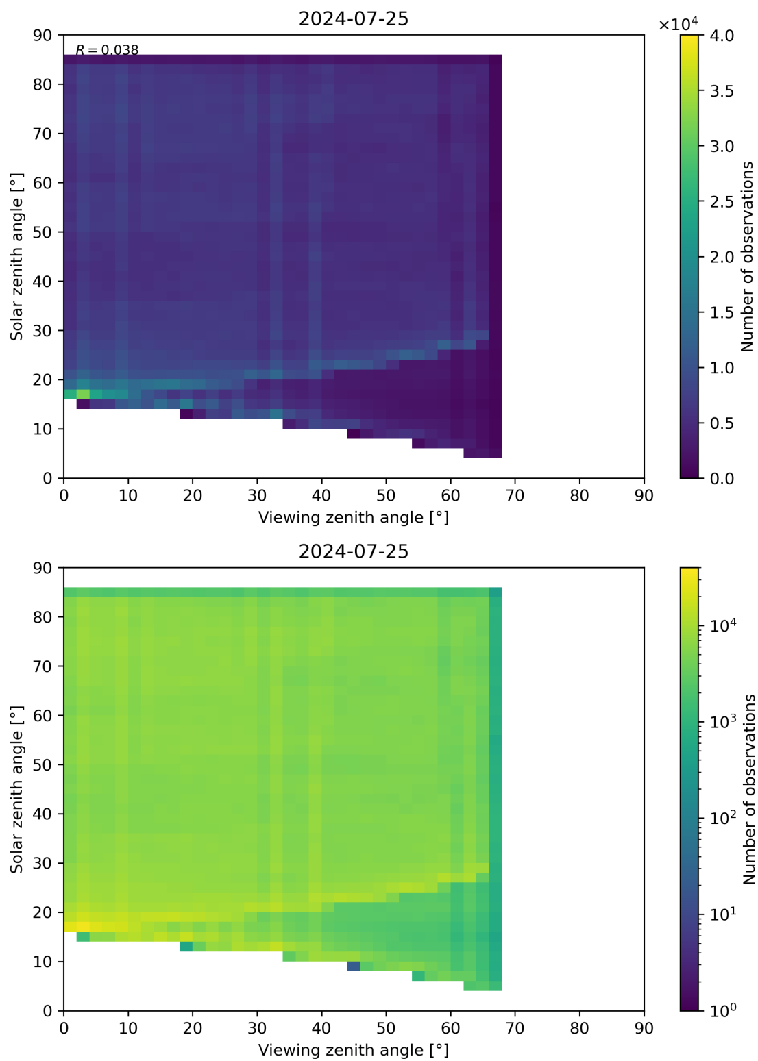
Figure 77: Scatter density plot of “Viewing zenith angle” against “Solar zenith angle” for 2024-07-24 to 2024-07-26.
