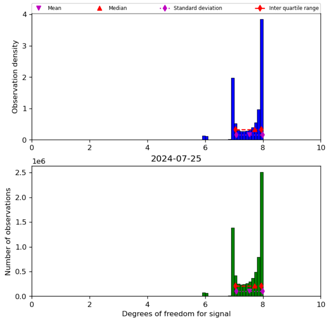
Figure 23: Histogram of “Degrees of freedom for signal” for 2024-07-24 to 2024-07-26
