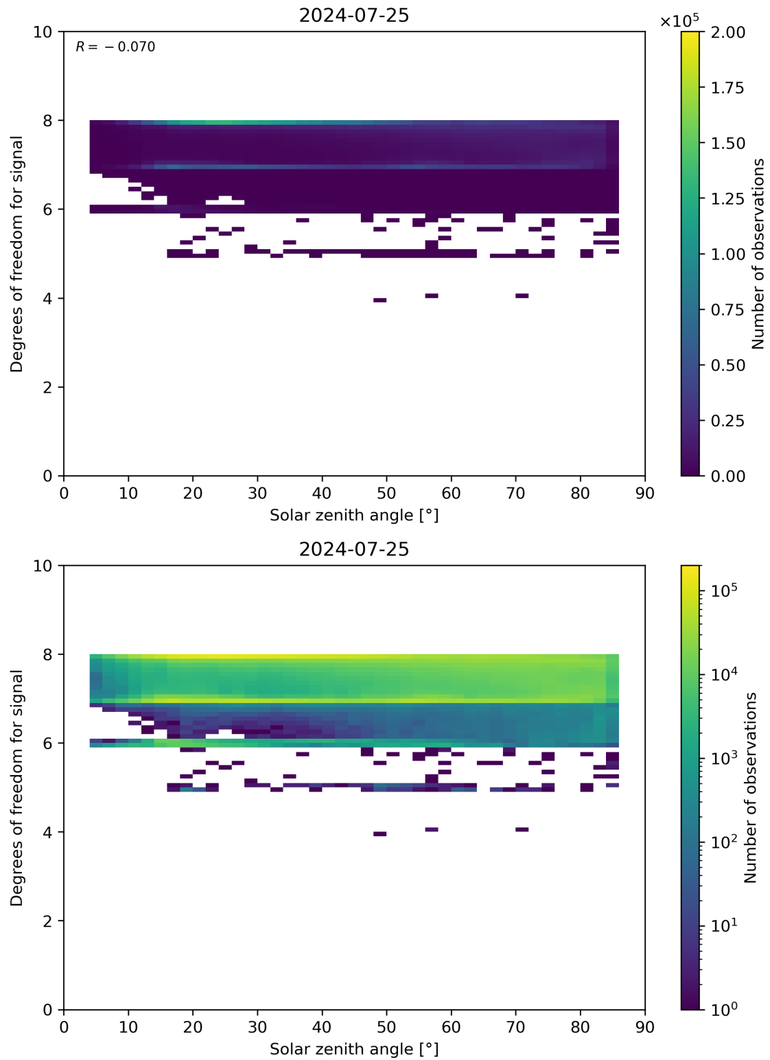
Figure 65: Scatter density plot of “Solar zenith angle” against “Degrees of freedom for signal” for 2024-07-24 to 2024-07-26.
