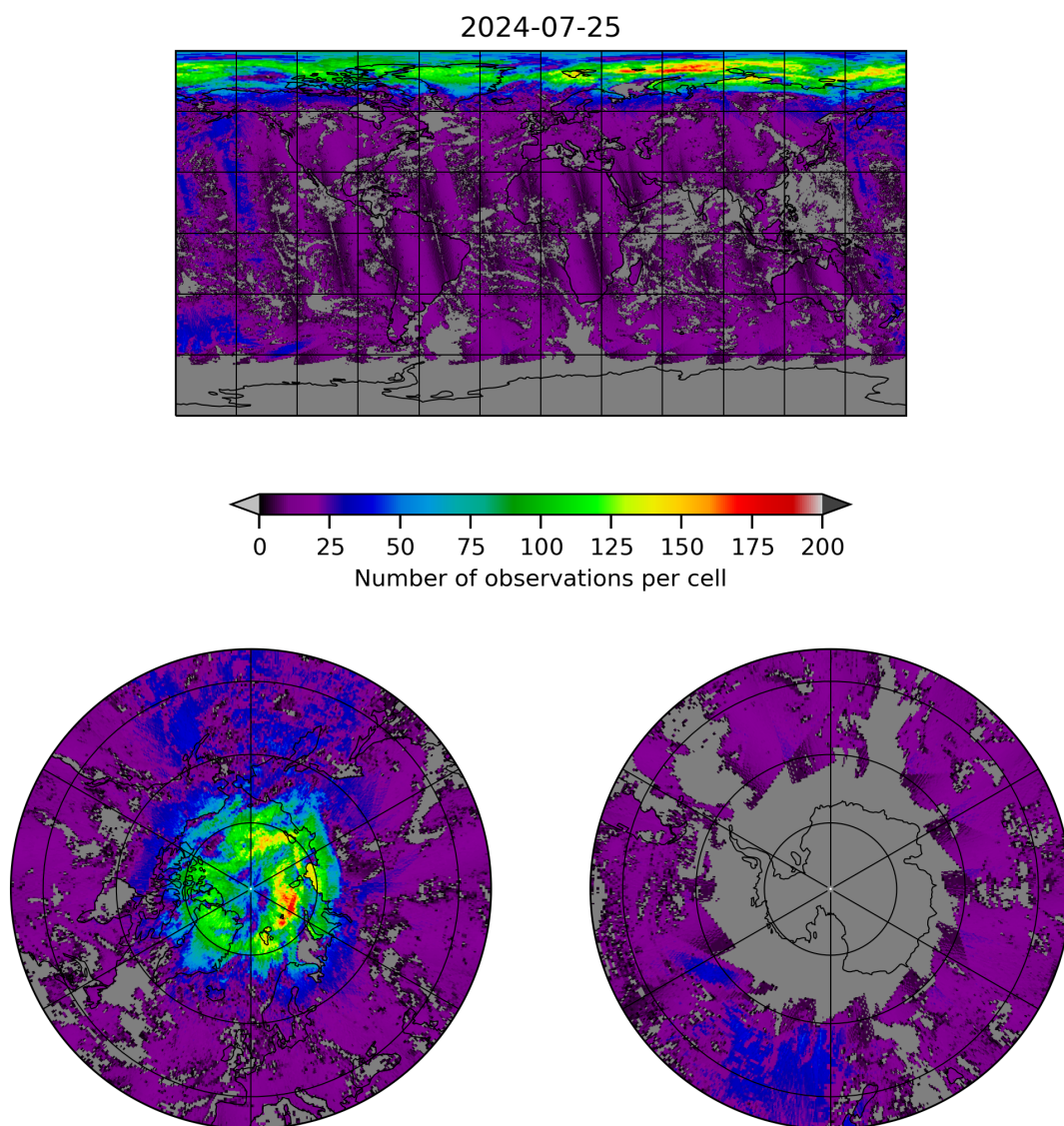
Figure 8: Map of the number of observations for 2024-07-24 to 2024-07-26
