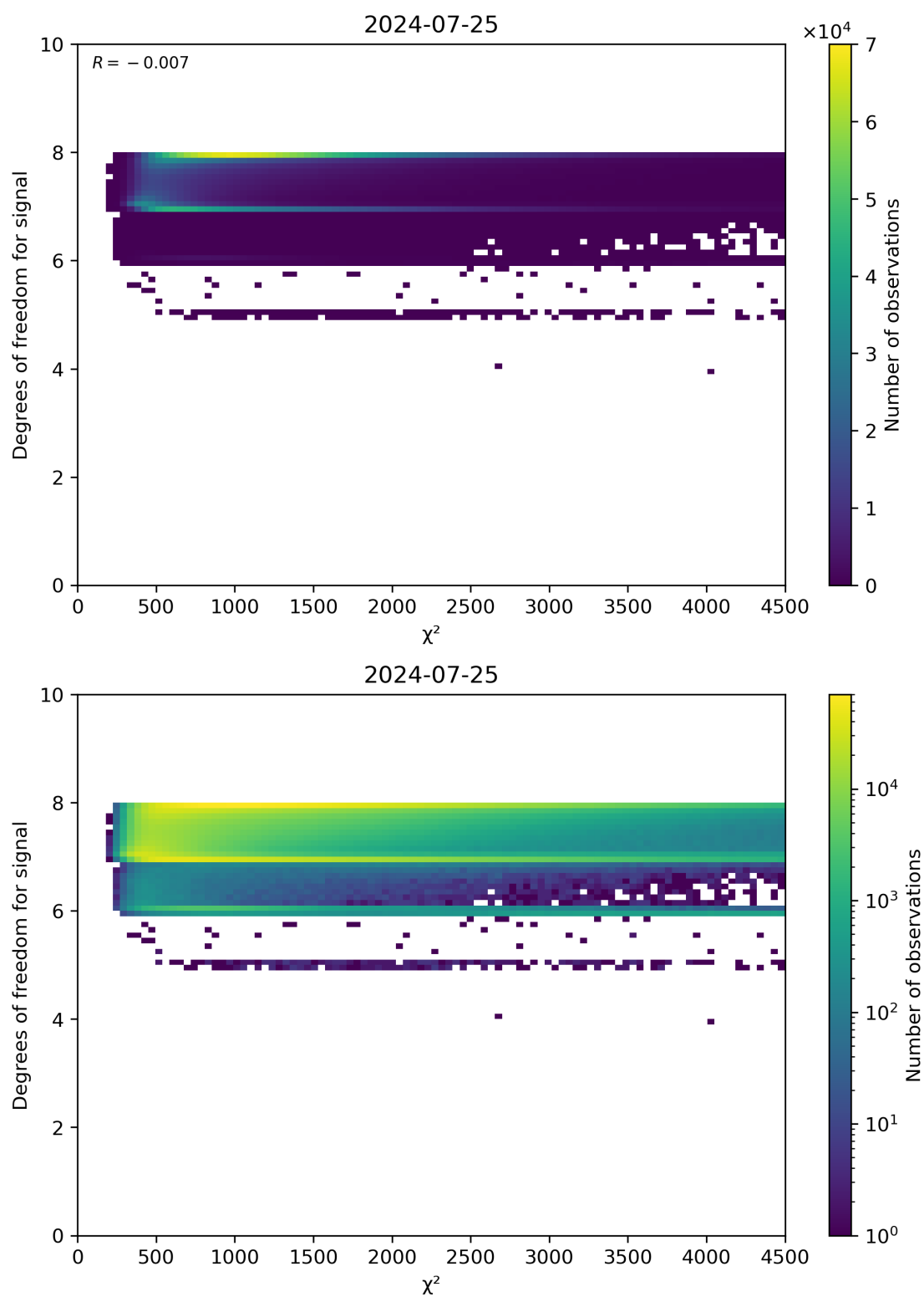
Figure 48: Scatter density plot of " \chi^2 " against "Degrees of freedom for signal" for 2024-07-24 to 2024-07-26.
