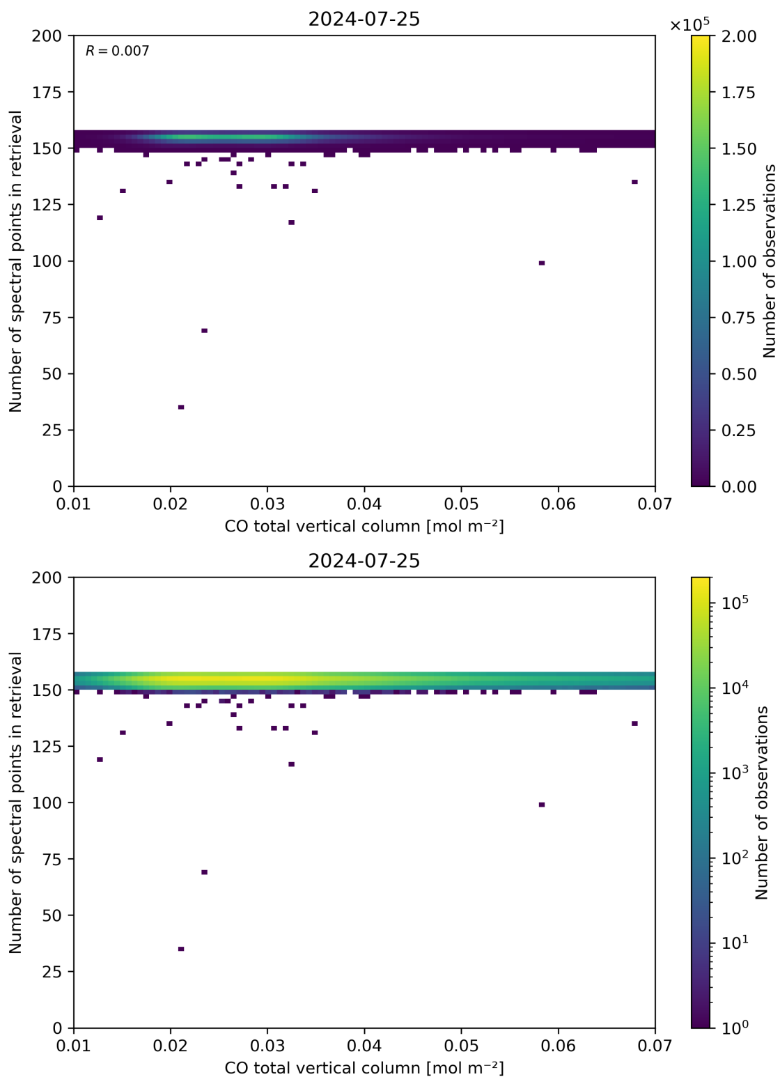
Figure 43: Scatter density plot of “CO total vertical column” against “Number of spectral points in retrieval” for 2024-07-24 to 2024-07-26.
