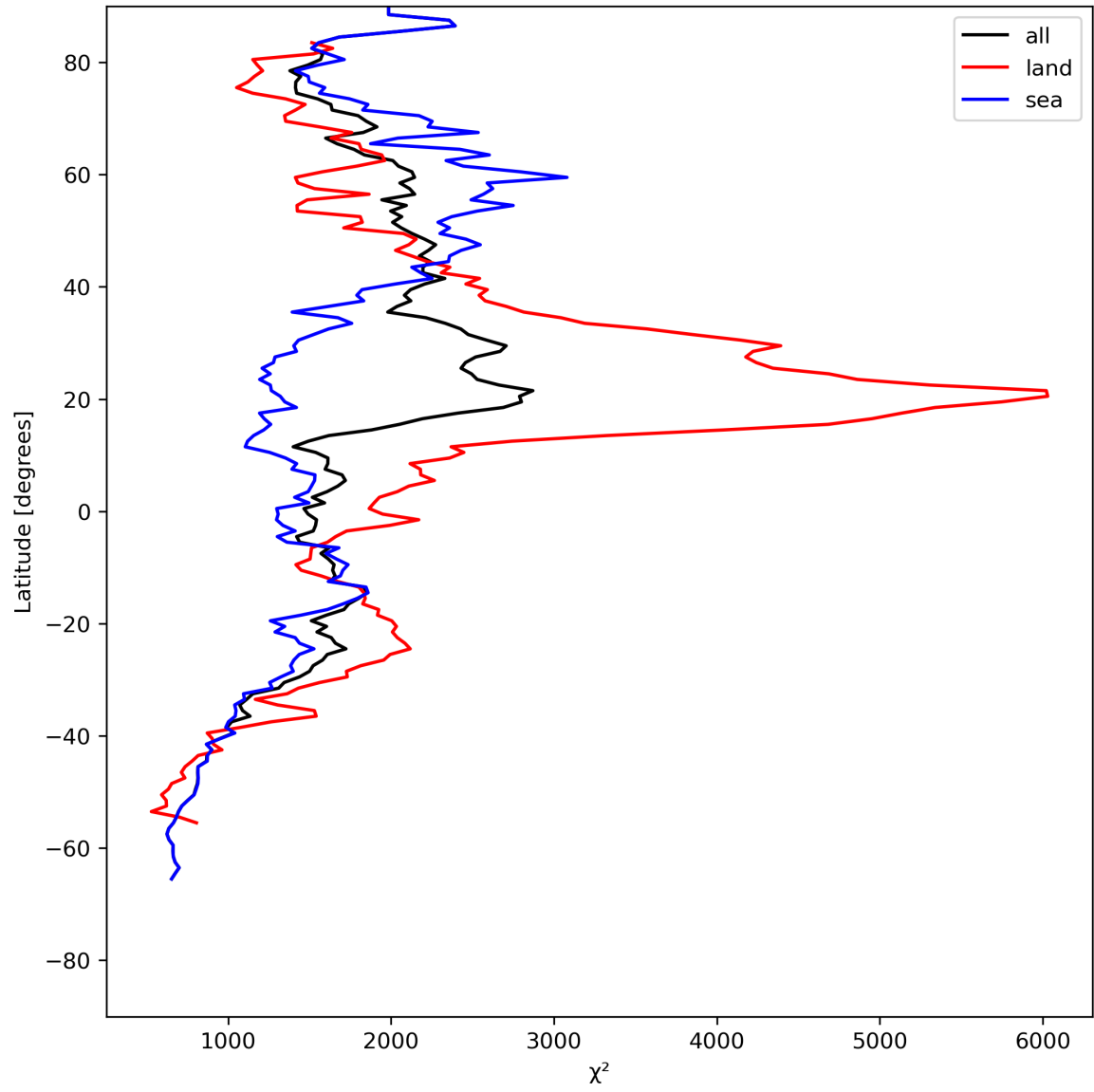
Figure 14: Zonal average of “ \chi^2 ” for 2024-07-24 to 2024-07-26.
