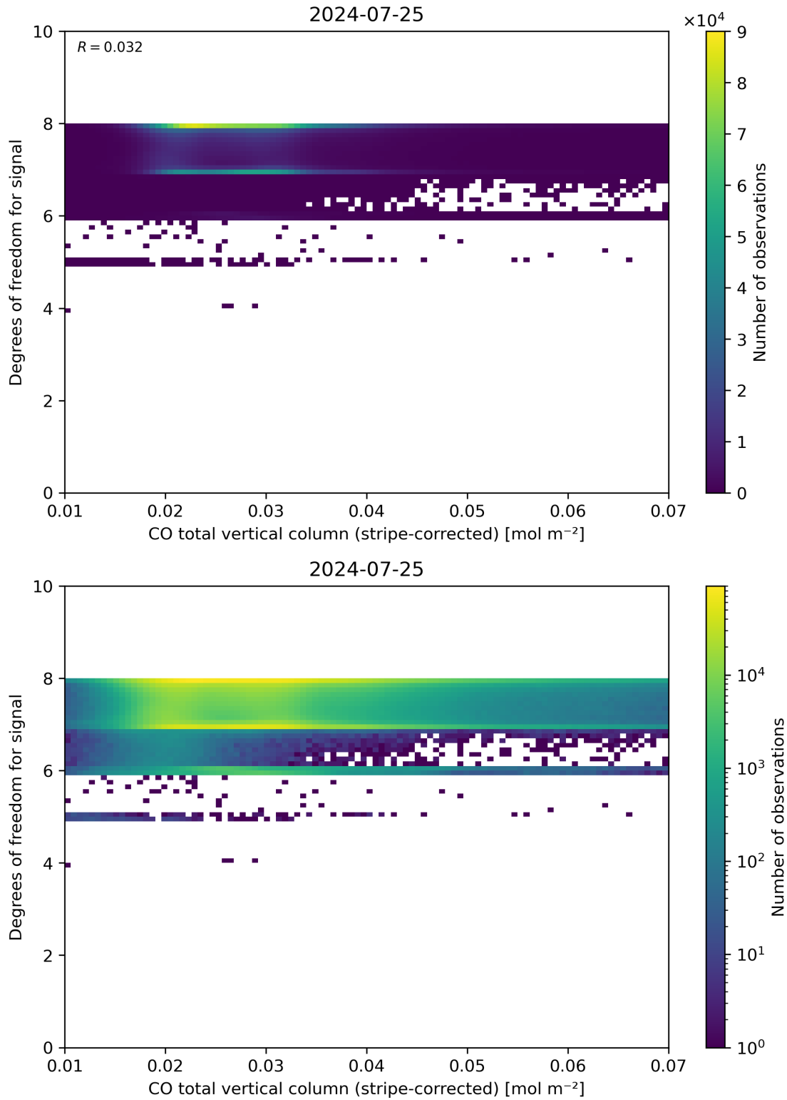
Figure 38: Scatter density plot of “CO total vertical column (stripe-corrected)” against “Degrees of freedom for signal” for 2024-07-24 to 2024-07-26.
