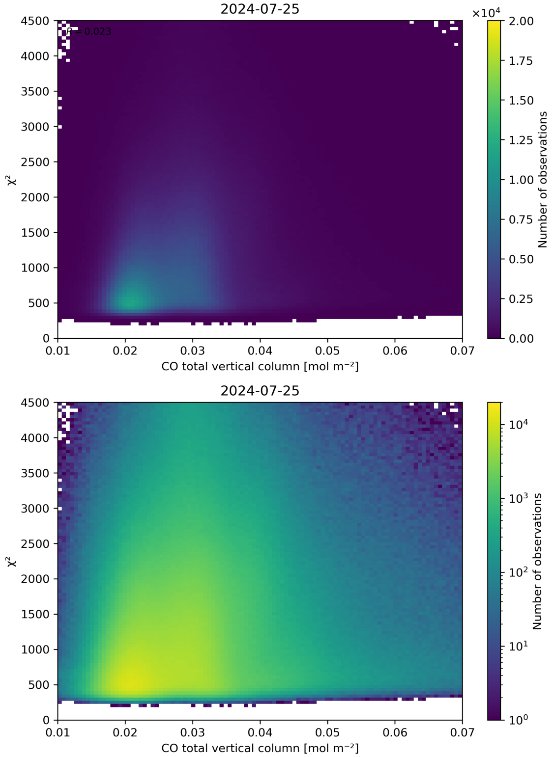
Figure 35: Scatter density plot of “CO total vertical column” against “ \chi^2 ” for 2024-07-24 to 2024-07-26.
