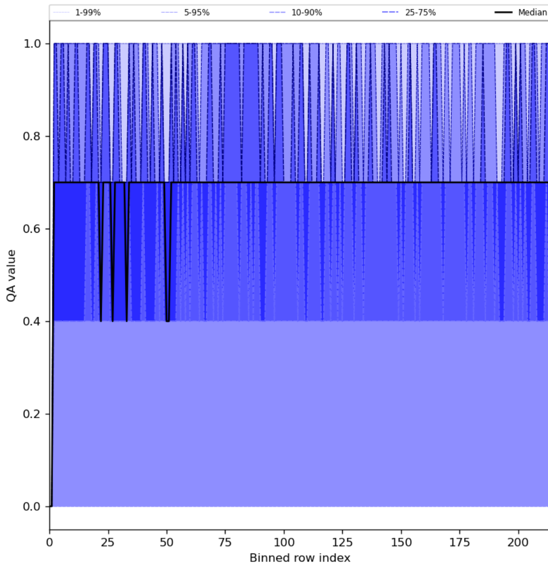
Figure 25: Along track statistics of “QA value” for 2024-07-24 to 2024-07-26
