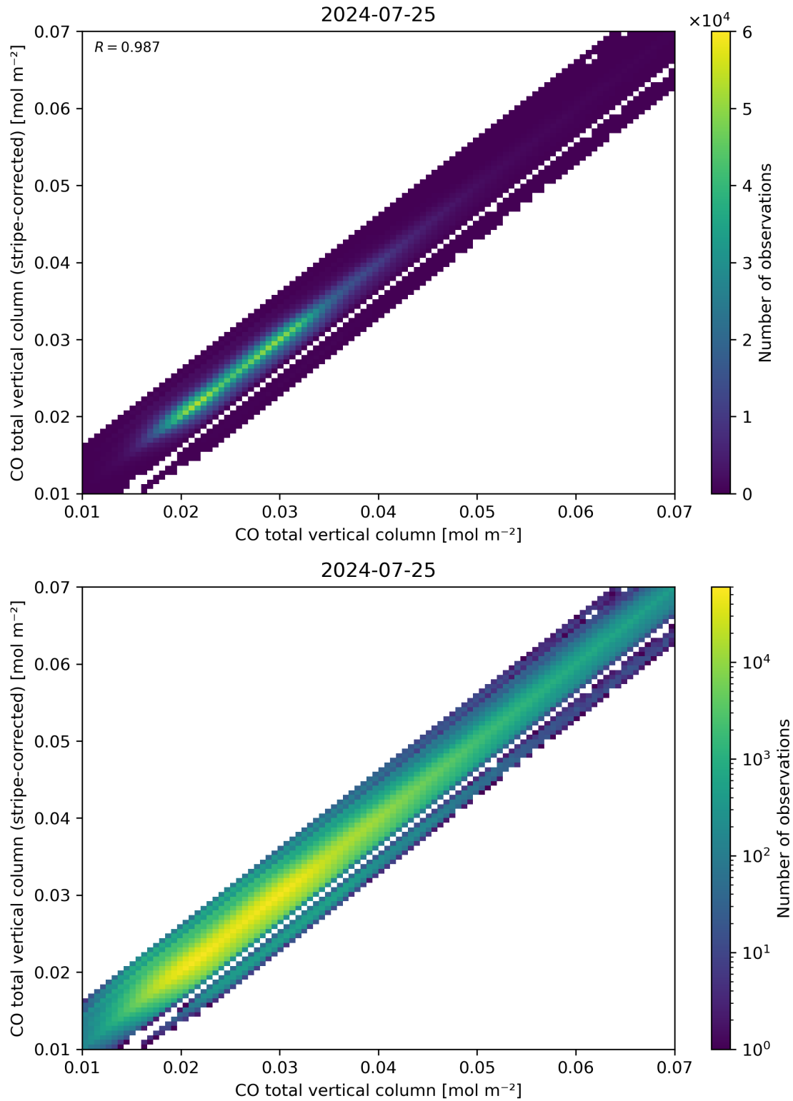
Figure 33: Scatter density plot of “CO total vertical column” against “CO total vertical column (stripe-corrected)” for 2024-07-24 to 2024-07-26.
