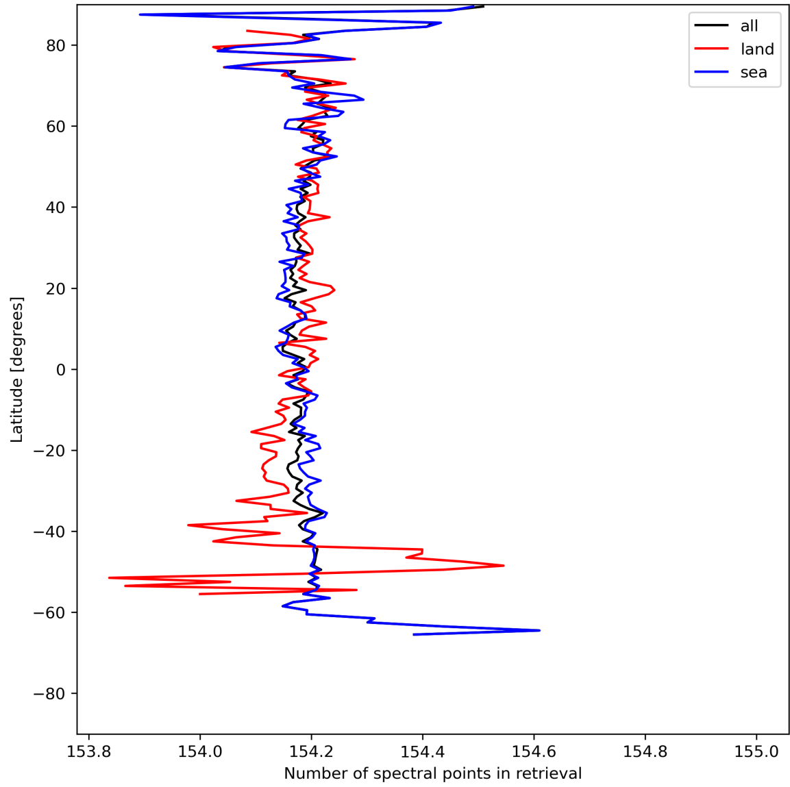
Figure 13: Zonal average of “Number of spectral points in retrieval” for 2024-07-24 to 2024-07-26.
