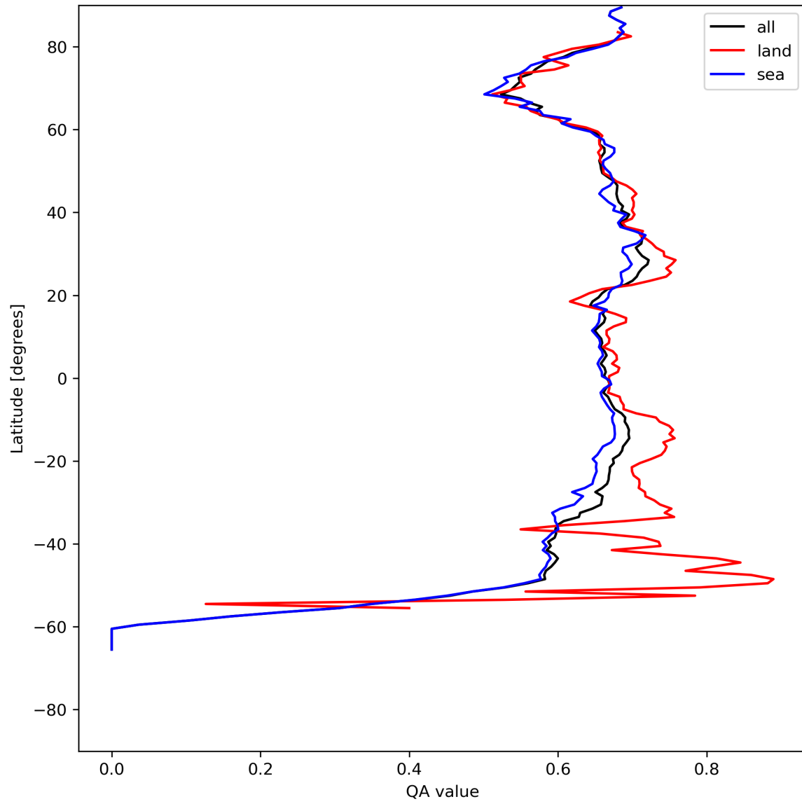
Figure 9: Zonal average of “QA value” for 2024-07-24 to 2024-07-26.
