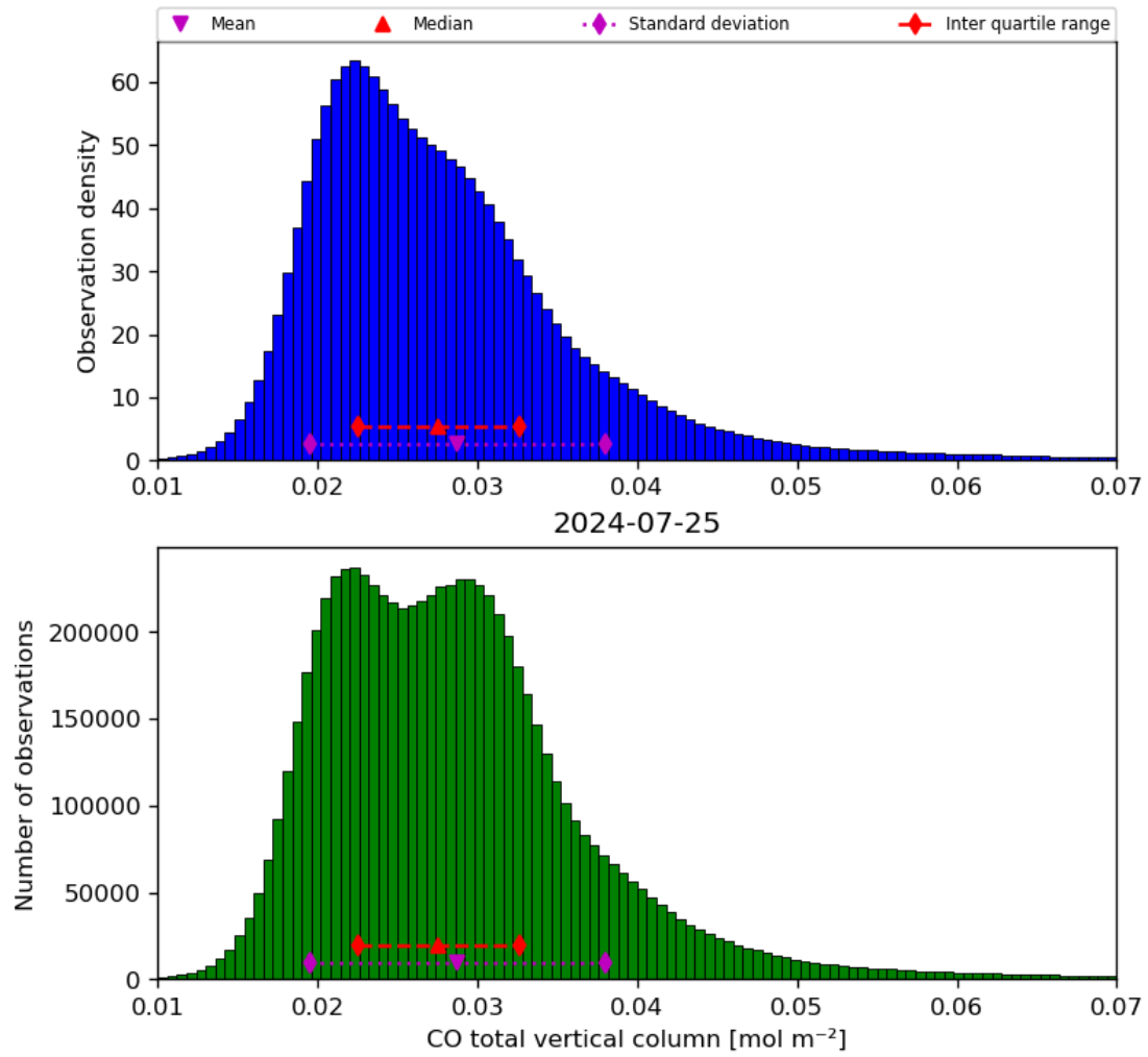
Figure 18: Histogram of “CO total vertical column” for 2024-07-24 to 2024-07-26
