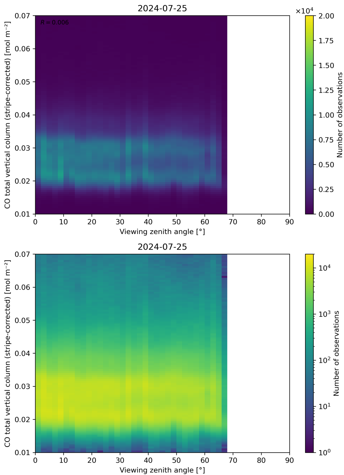
Figure 70: Scatter density plot of “Viewing zenith angle” against “CO total vertical column (stripe-corrected)” for 2024-07-24 to 2024-07-26.
