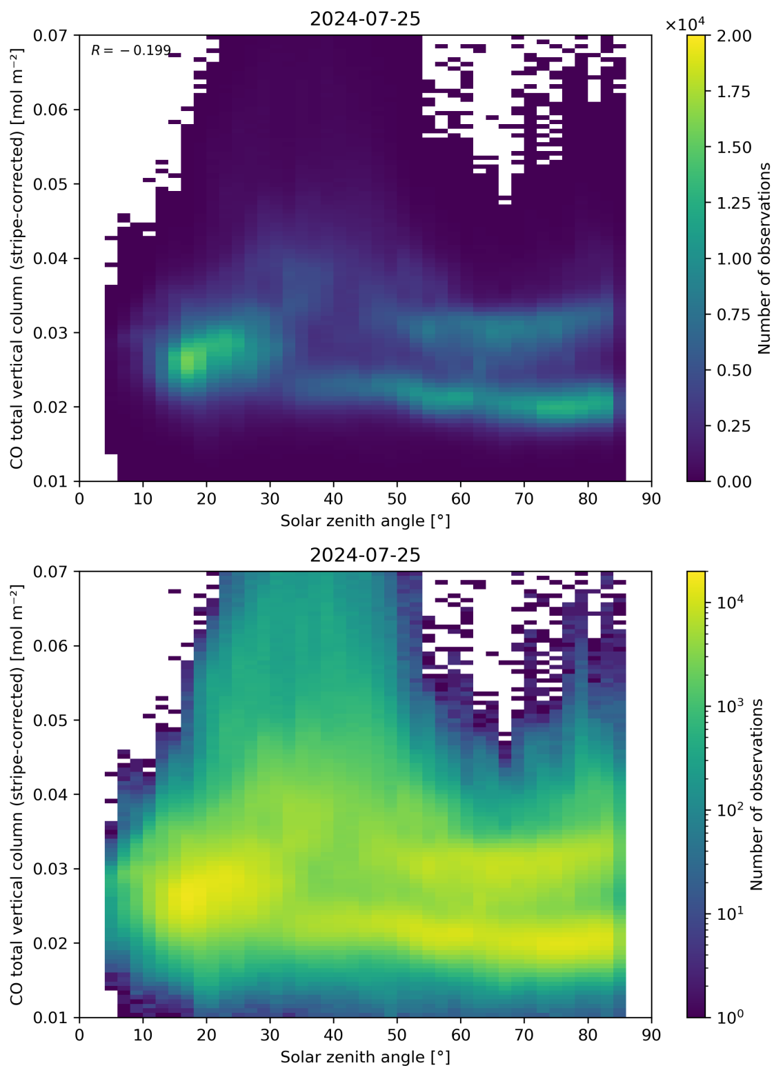
Figure 62: Scatter density plot of “Solar zenith angle” against “CO total vertical column (stripe-corrected)” for 2024-07-24 to 2024-07-26.
