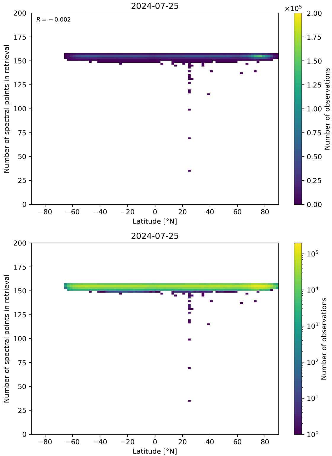
Figure 57: Scatter density plot of “Latitude” against “Number of spectral points in retrieval” for 2024-07-24 to 2024-07-26.
