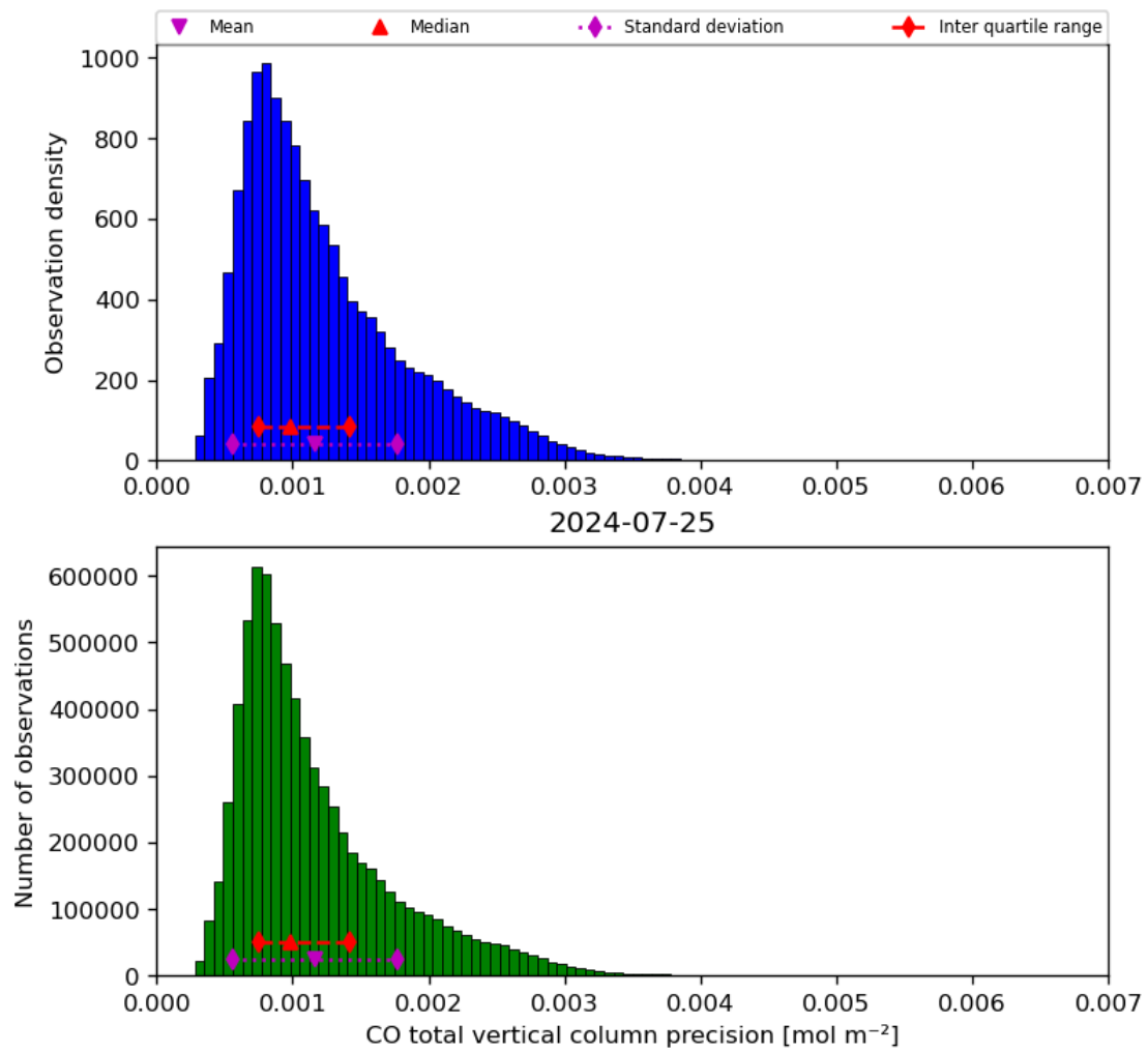
Figure 20: Histogram of “CO total vertical column precision” for 2024-07-24 to 2024-07-26
