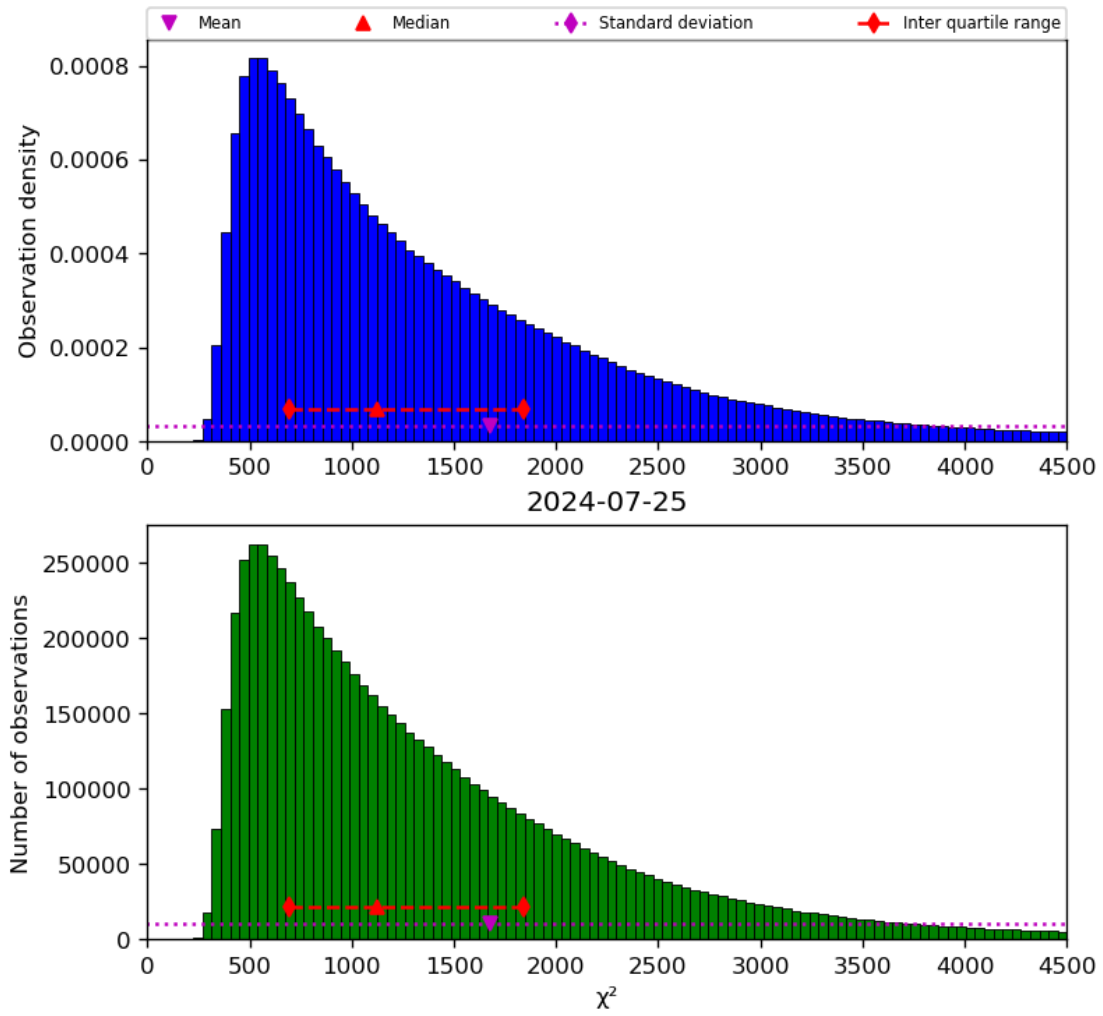
Figure 22: Histogram of “ \chi^2 ” for 2024-07-24 to 2024-07-26
