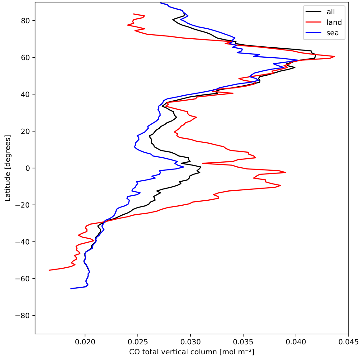
Figure 10: Zonal average of “CO total vertical column” for 2024-07-24 to 2024-07-26.
