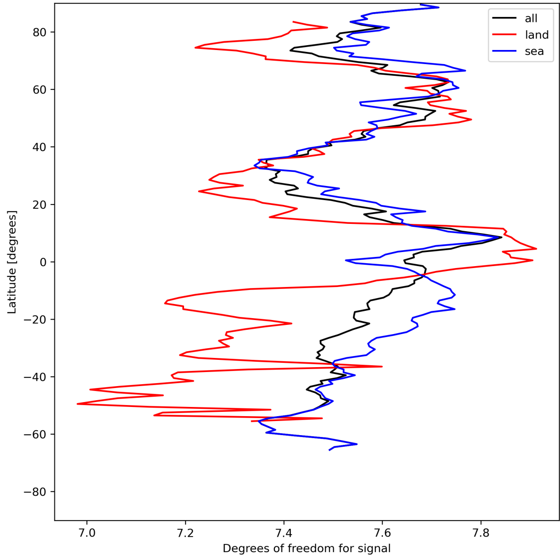
Figure 15: Zonal average of “Degrees of freedom for signal” for 2024-07-24 to 2024-07-26.
