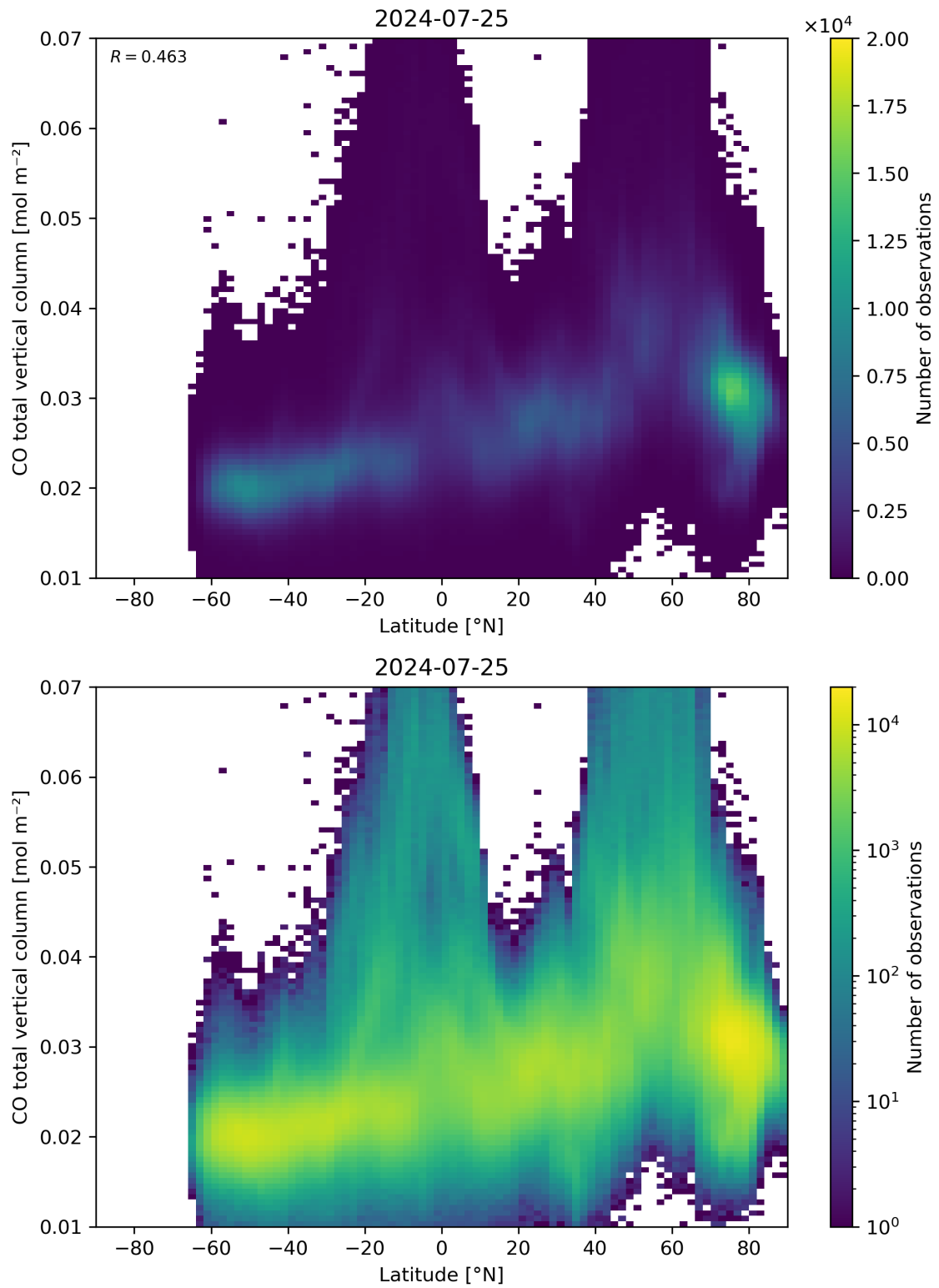
Figure 51: Scatter density plot of “Latitude” against “CO total vertical column” for 2024-07-24 to 2024-07-26.
