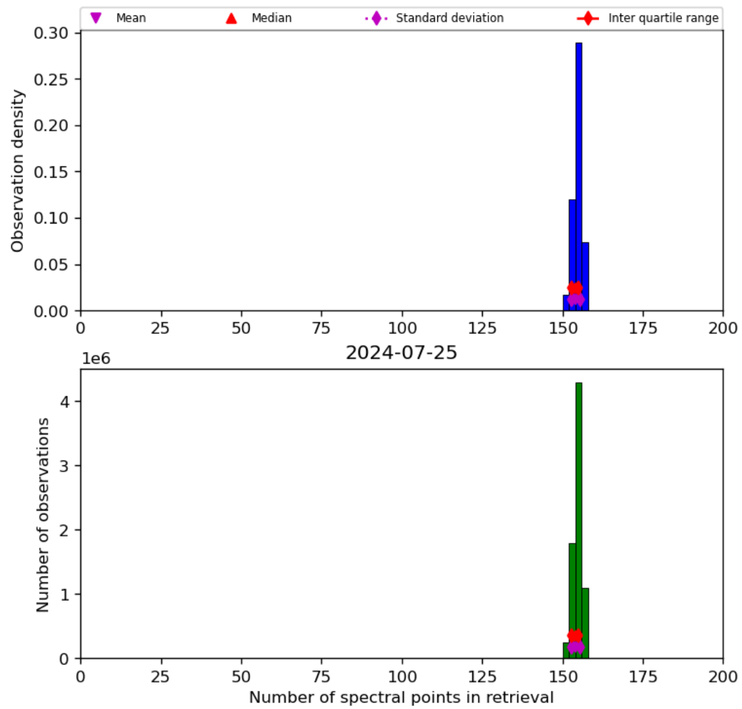
Figure 21: Histogram of “Number of spectral points in retrieval” for 2024-07-24 to 2024-07-26
