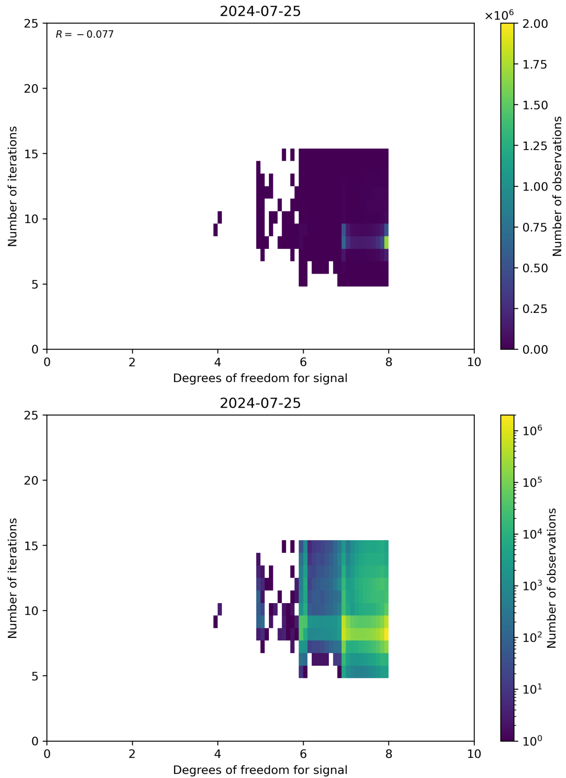
Figure 50: Scatter density plot of “Degrees of freedom for signal” against “Number of iterations” for 2024-07-24 to 2024-07-26.
