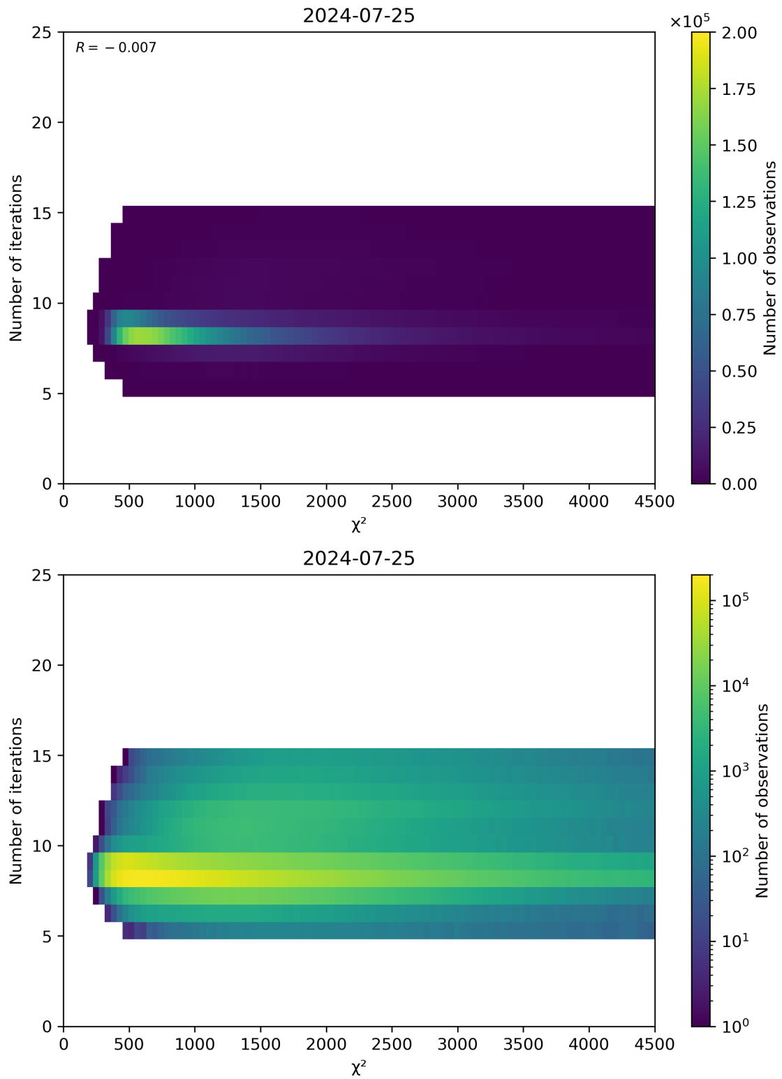
Figure 49: Scatter density plot of “ \chi^2 ” against “Number of iterations” for 2024-07-24 to 2024-07-26.
