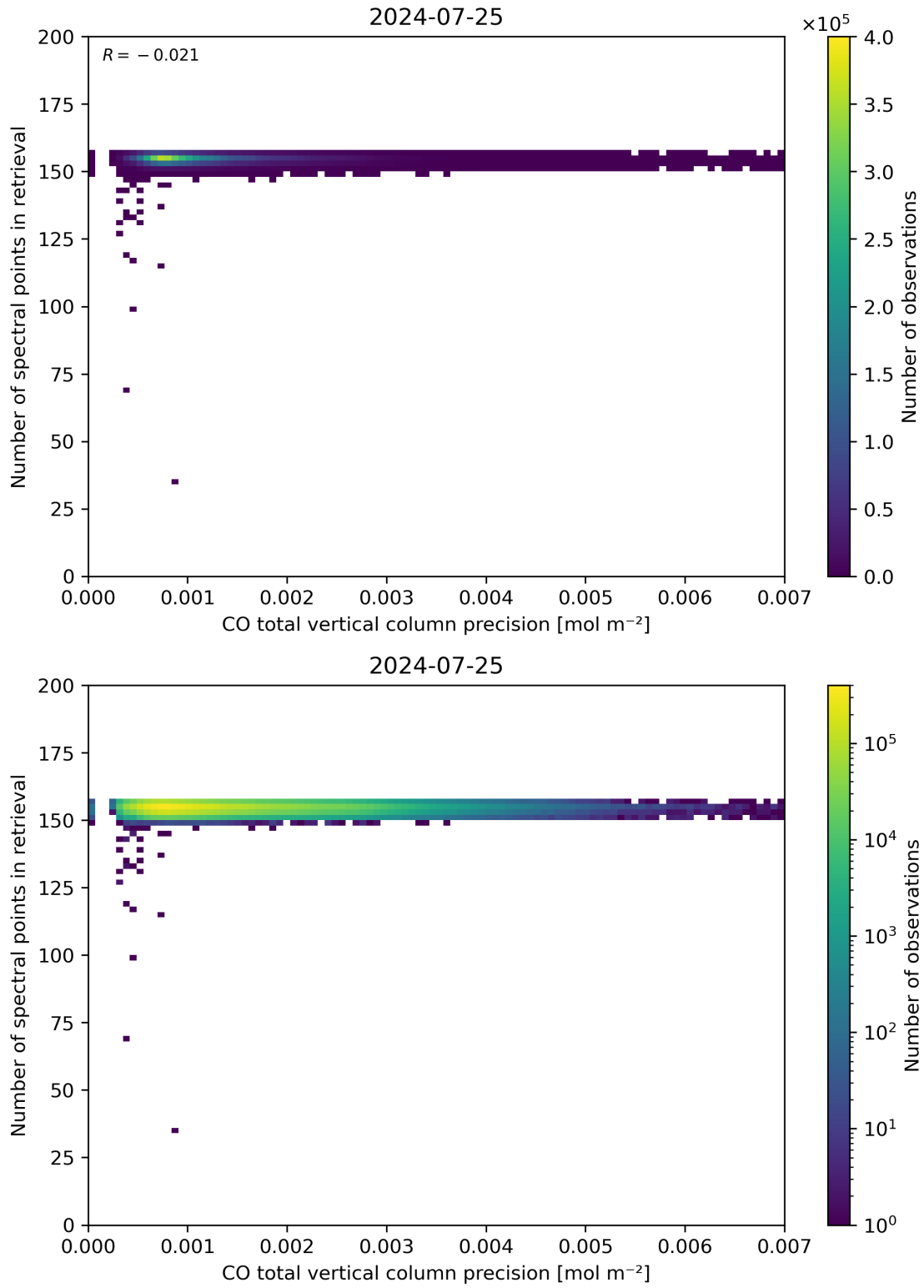
Figure 47: Scatter density plot of “CO total vertical column precision” against “Number of spectral points in retrieval” for 2024-07-24 to 2024-07-26.
