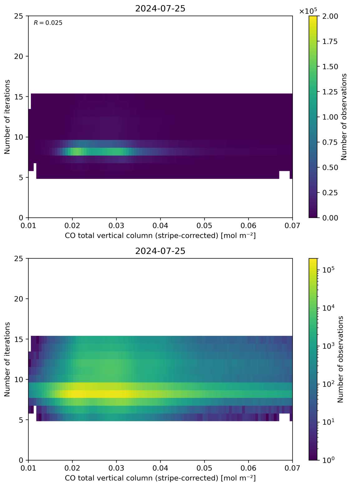
Figure 39: Scatter density plot of “CO total vertical column (stripe-corrected)” against “Number of iterations” for 2024-07-24 to 2024-07-26.
