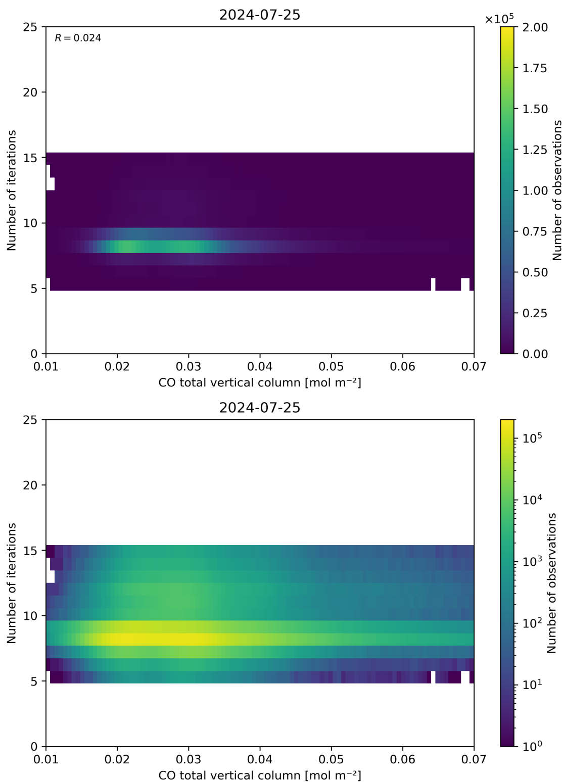
Figure 42: Scatter density plot of “CO total vertical column” against “Number of iterations” for 2024-07-24 to 2024-07-26.
