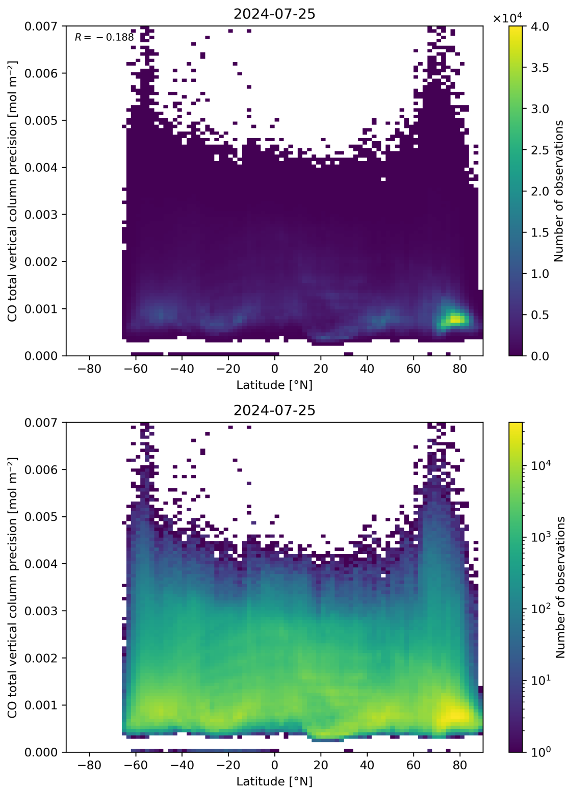
Figure 53: Scatter density plot of “Latitude” against “CO total vertical column precision” for 2024-07-24 to 2024-07-26.
