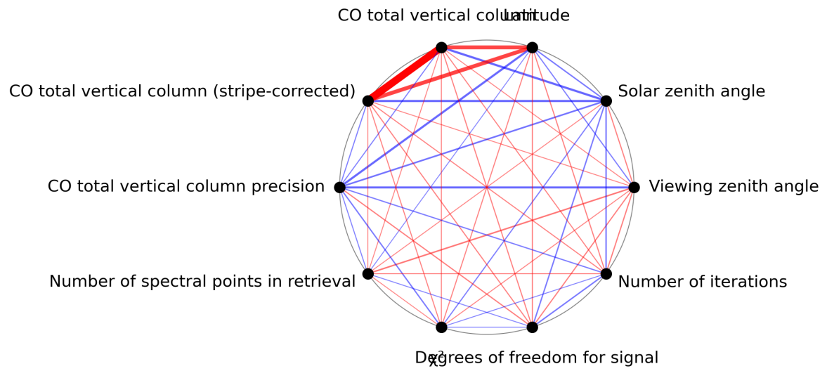
Figure 1: Map of correlation graph for 2024-07-24 to 2024-07-26.
