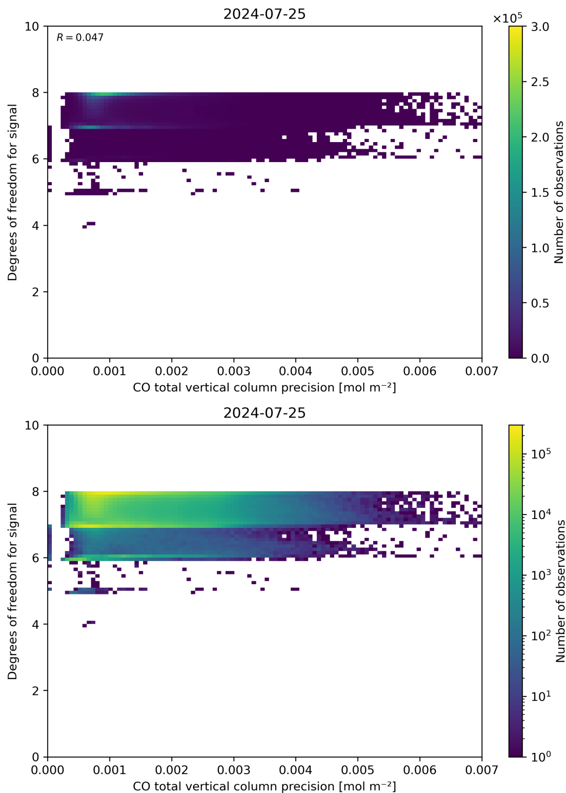
Figure 45: Scatter density plot of “CO total vertical column precision” against “Degrees of freedom for signal” for 2024-07-24 to 2024-07-26.
