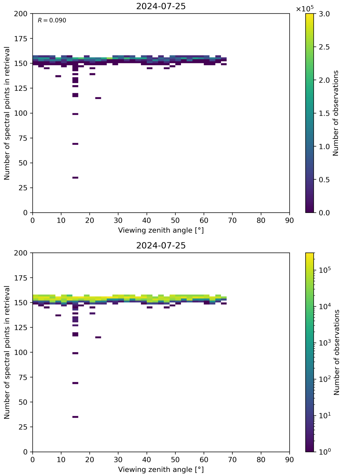
Figure 76: Scatter density plot of “Viewing zenith angle” against “Number of spectral points in retrieval” for 2024-07-24 to 2024-07-26.
