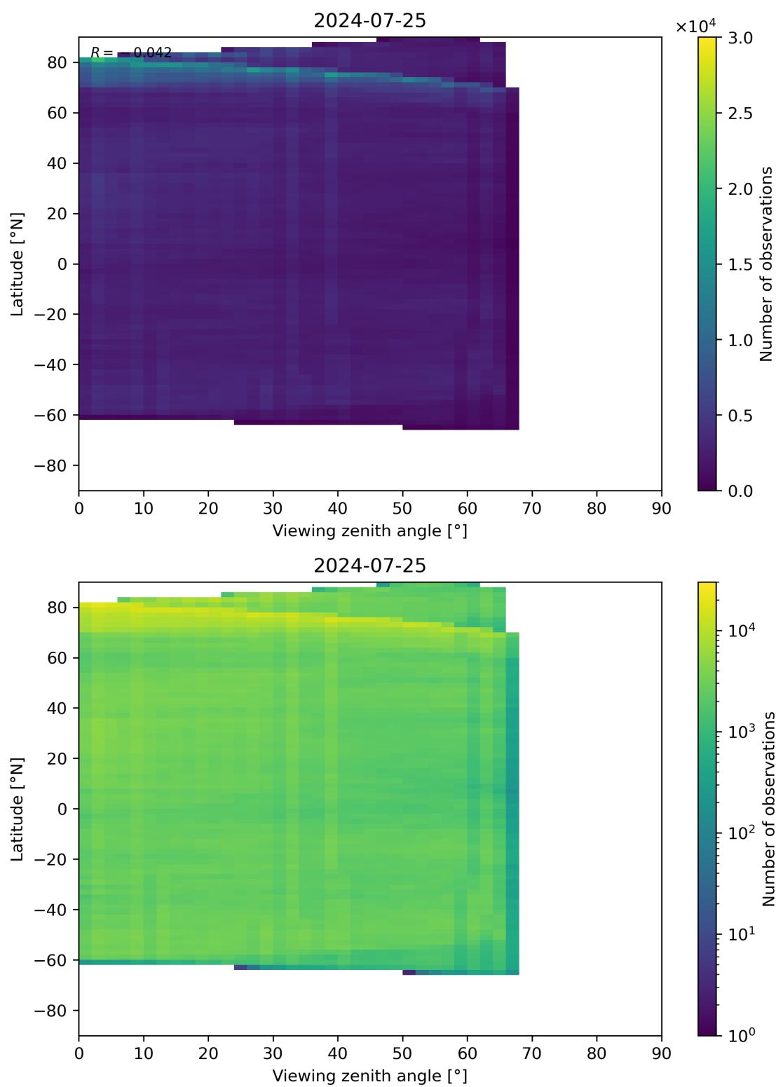
Figure 74: Scatter density plot of “Viewing zenith angle” against “Latitude” for 2024-07-24 to 2024-07-26.
