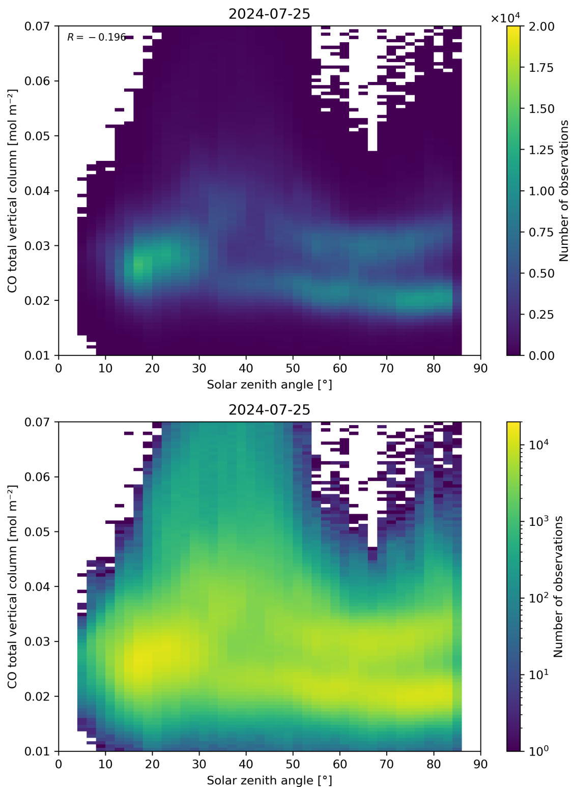
Figure 61: Scatter density plot of “Solar zenith angle” against “CO total vertical column” for 2024-07-24 to 2024-07-26.
