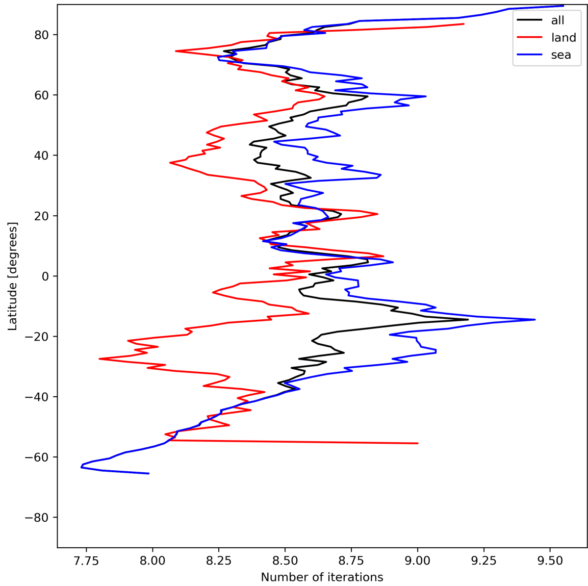
Figure 16: Zonal average of “Number of iterations” for 2024-07-24 to 2024-07-26.
