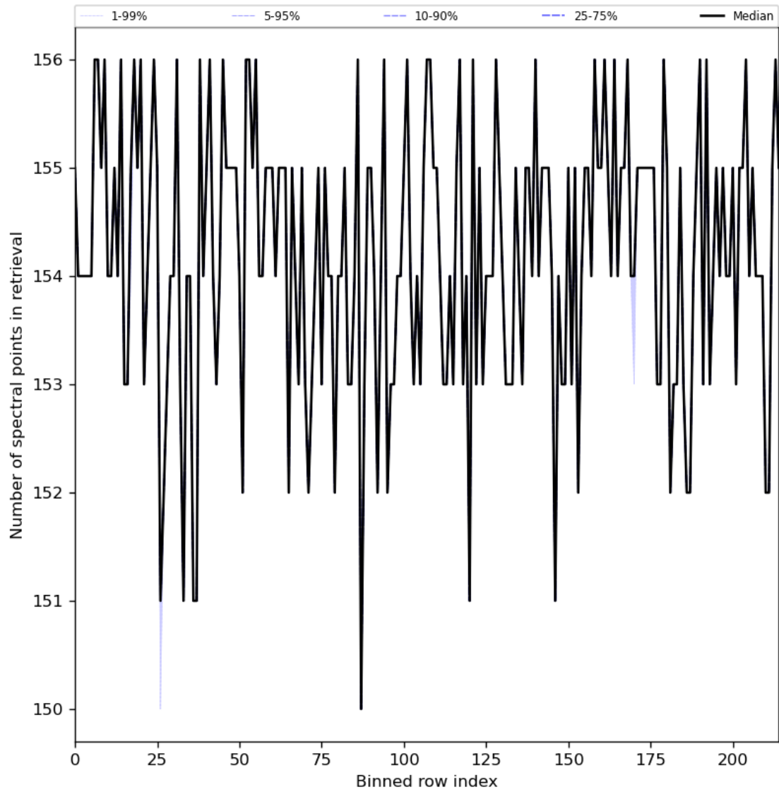
Figure 29: Along track statistics of “Number of spectral points in retrieval” for 2024-07-26 to 2024-07-27
