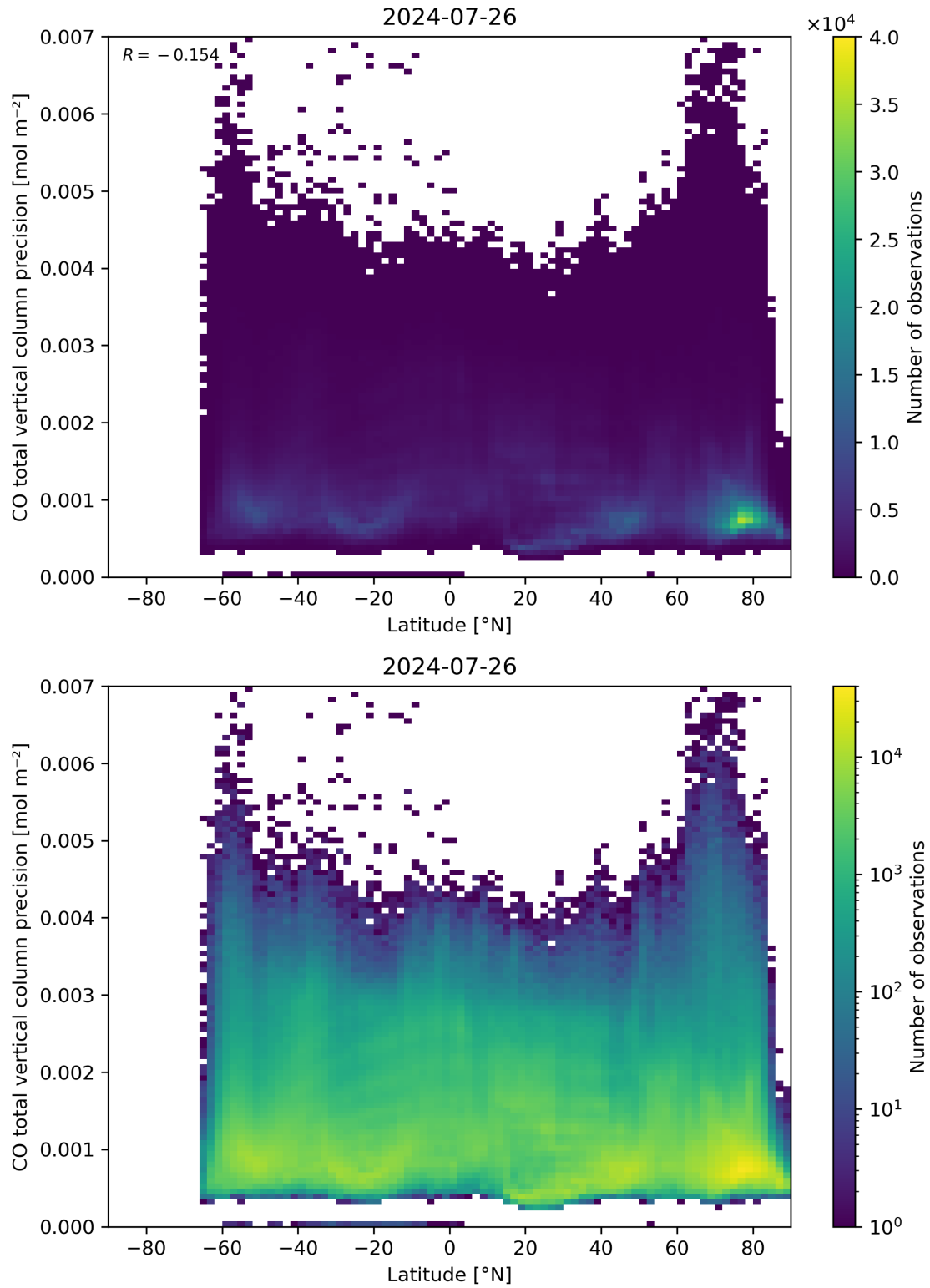
Figure 53: Scatter density plot of “Latitude” against “CO total vertical column precision” for 2024-07-26 to 2024-07-27.
