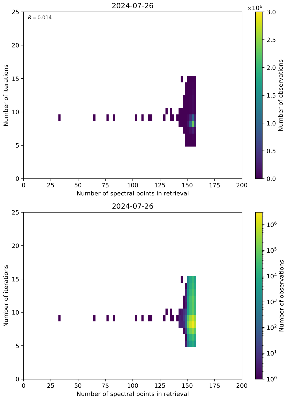
Figure 60: Scatter density plot of “Number of spectral points in retrieval” against “Number of iterations” for 2024-07-26 to 2024-07-27.
