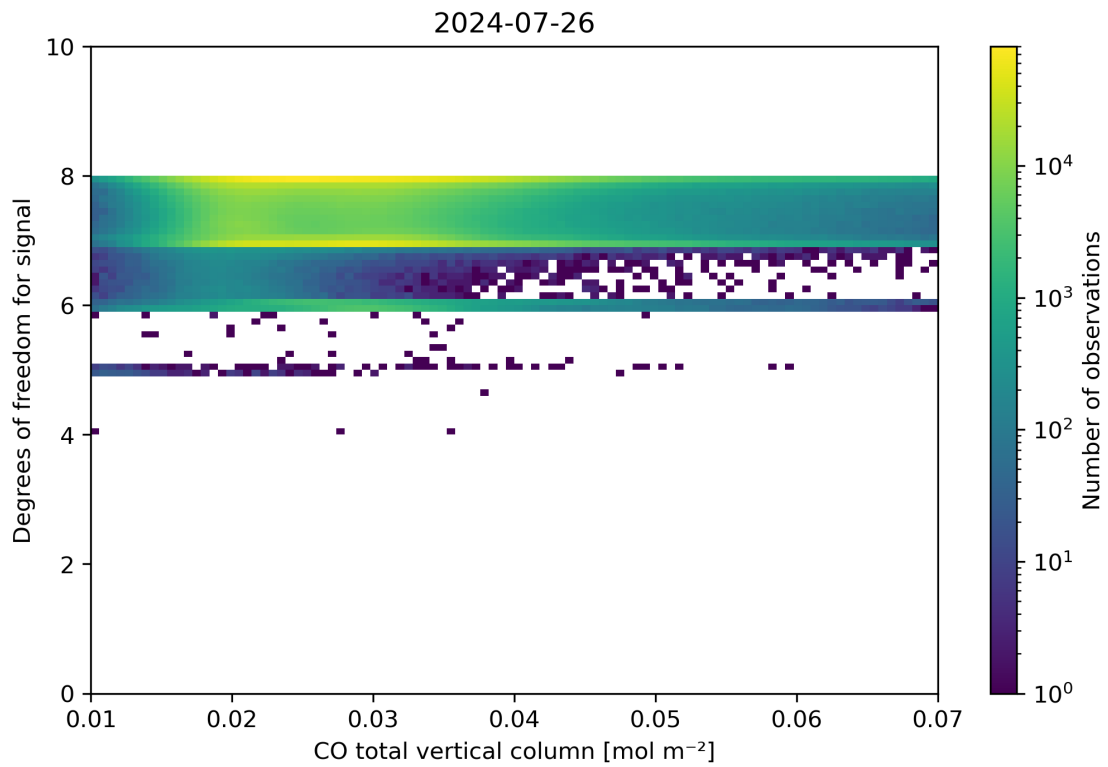
Figure 41: Scatter density plot of “CO total vertical column” against “Degrees of freedom for signal” for 2024-07-26 to 2024-07-27.
