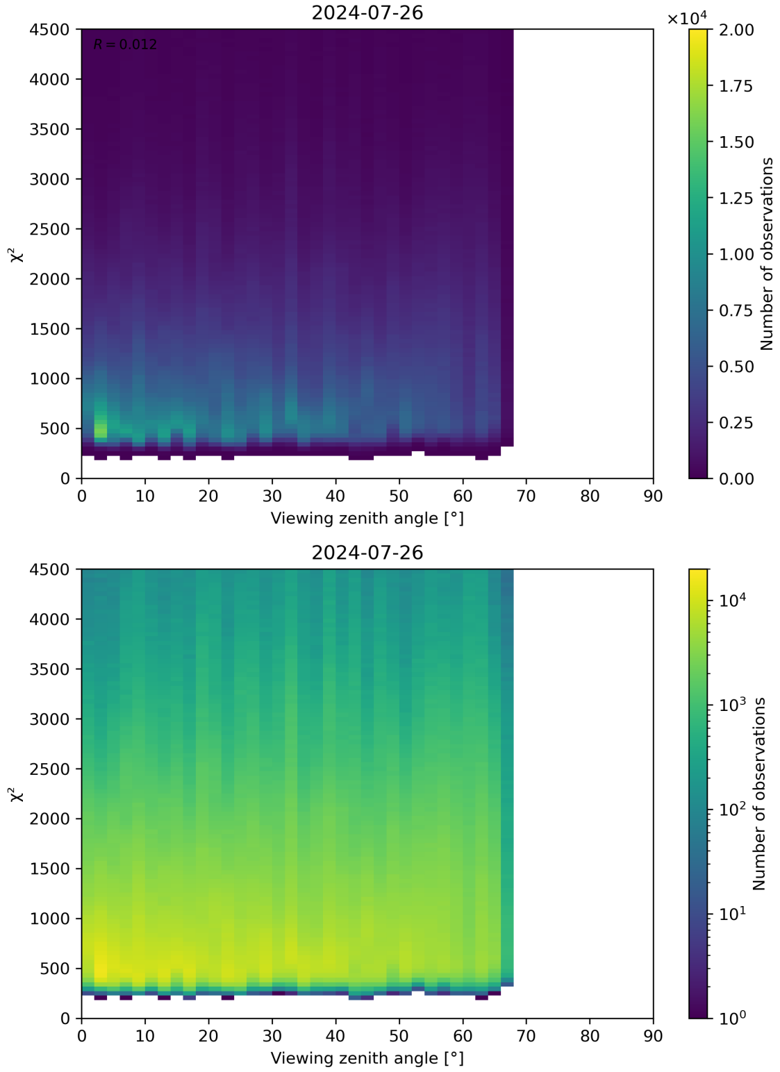
Figure 72: Scatter density plot of “Viewing zenith angle” against “ \chi^2 ” for 2024-07-26 to 2024-07-27.
