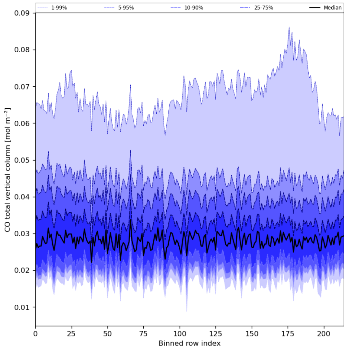
Figure 26: Along track statistics of “CO total vertical column” for 2024-07-26 to 2024-07-27
