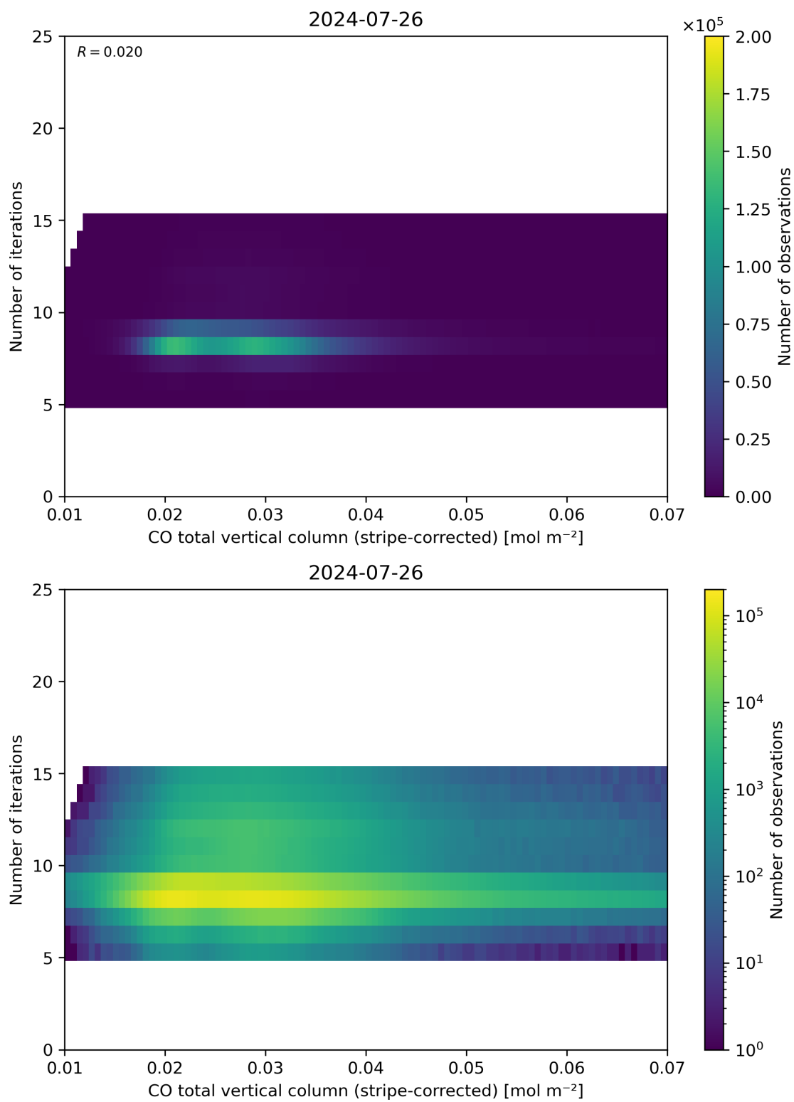
Figure 39: Scatter density plot of “CO total vertical column (stripe-corrected)” against “Number of iterations” for 2024-07-26 to 2024-07-27.
