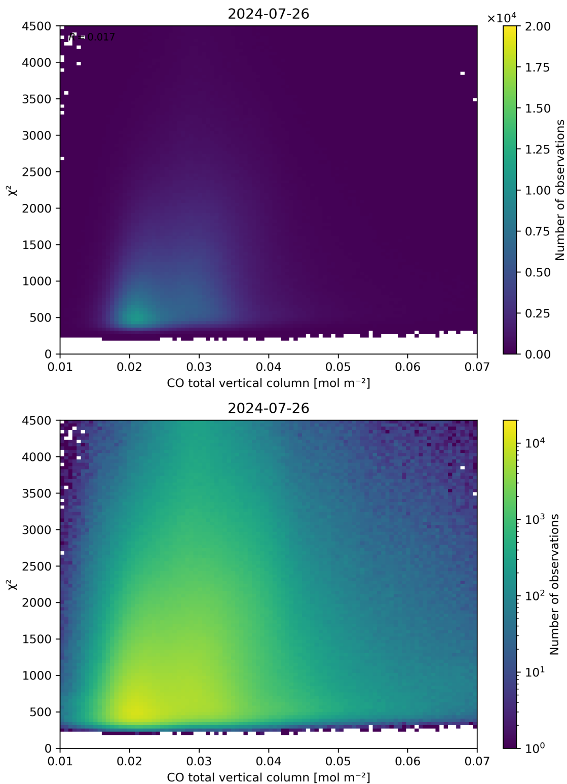
Figure 35: Scatter density plot of “CO total vertical column” against “ \chi^2 ” for 2024-07-26 to 2024-07-27.
