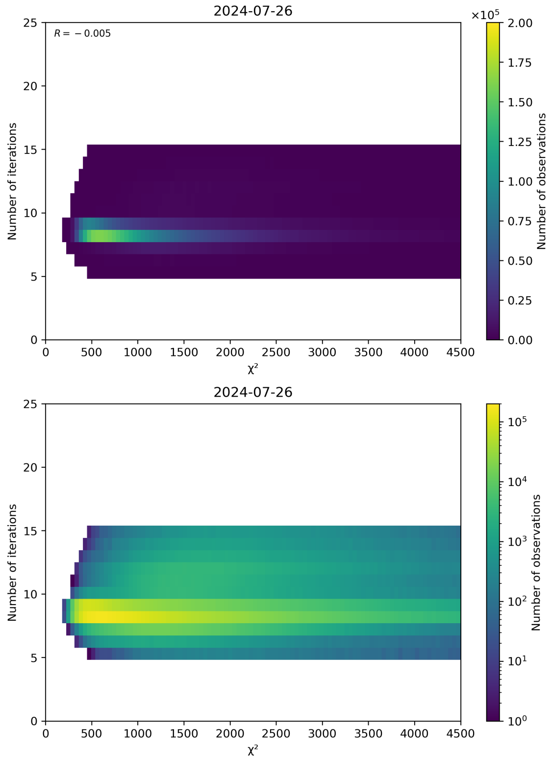
Figure 49: Scatter density plot of “ \chi^2 ” against “Number of iterations” for 2024-07-26 to 2024-07-27.
