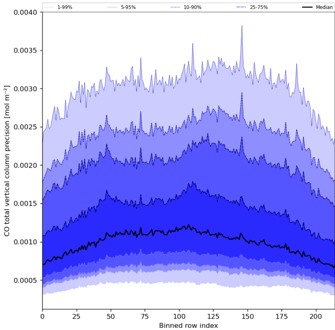
Figure 28: Along track statistics of “CO total vertical column precision” for 2024-07-26 to 2024-07-27
