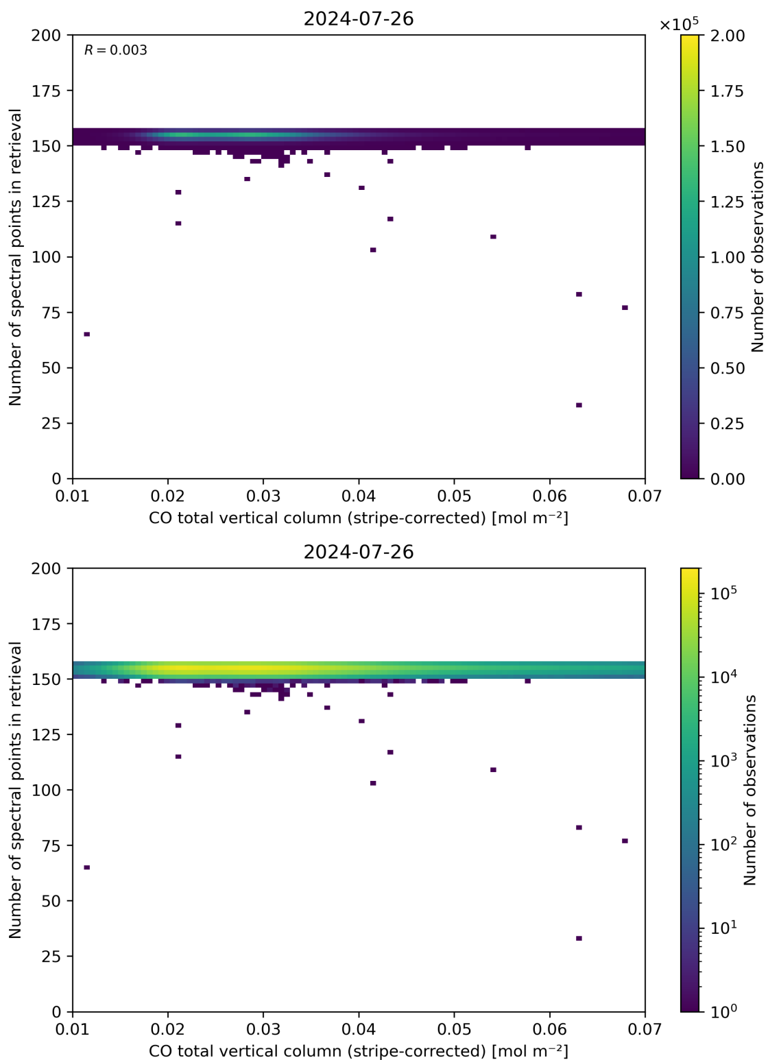
Figure 40: Scatter density plot of “CO total vertical column (stripe-corrected)” against “Number of spectral points in retrieval” for 2024-07-26 to 2024-07-27.
