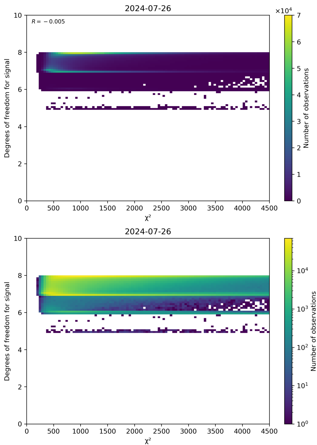
Figure 48: Scatter density plot of " \chi^2 " against "Degrees of freedom for signal" for 2024-07-26 to 2024-07-27.
