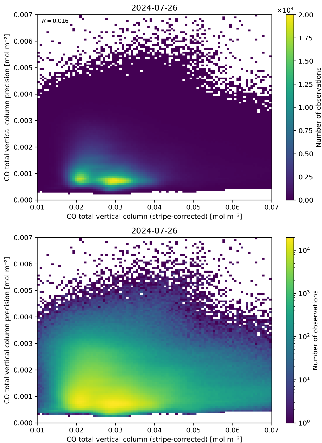
Figure 36: Scatter density plot of “CO total vertical column (stripe-corrected)” against “CO total vertical column precision” for 2024-07-26 to 2024-07-27.
