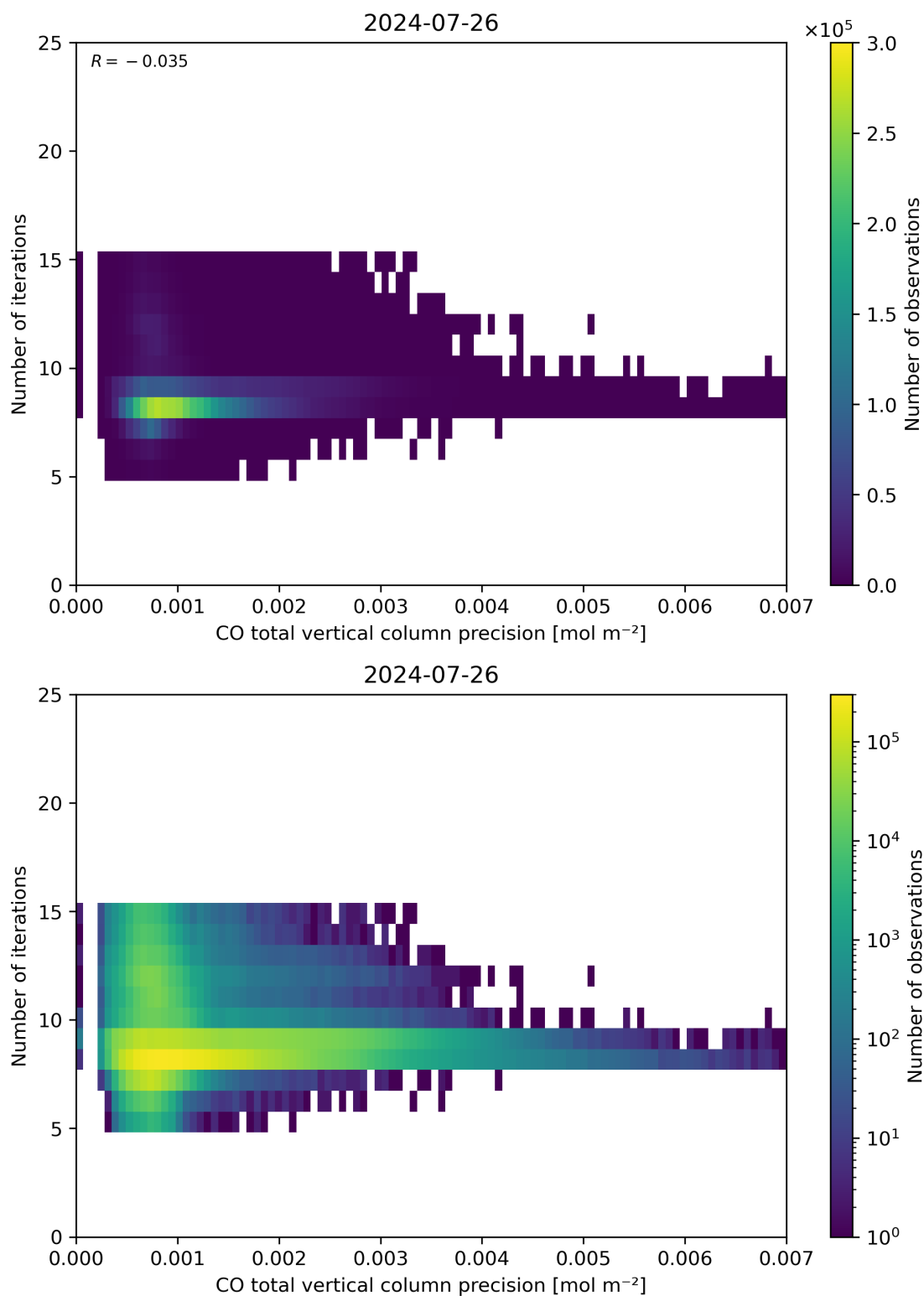
Figure 46: Scatter density plot of “CO total vertical column precision” against “Number of iterations” for 2024-07-26 to 2024-07-27.
