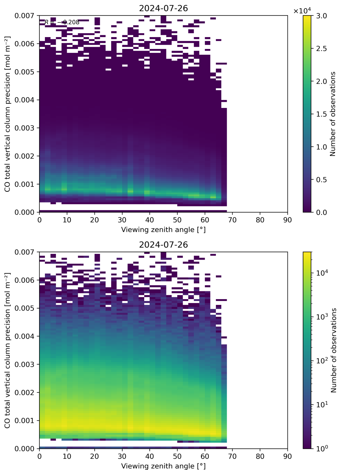
Figure 71: Scatter density plot of “Viewing zenith angle” against “CO total vertical column precision” for 2024-07-26 to 2024-07-27.
