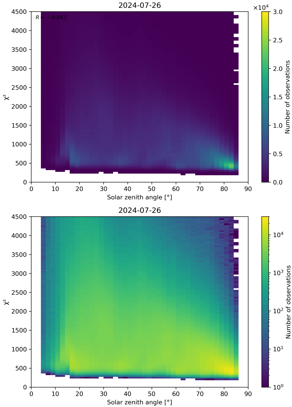
Figure 64: Scatter density plot of “Solar zenith angle” against “ \chi^2 ” for 2024-07-26 to 2024-07-27.
