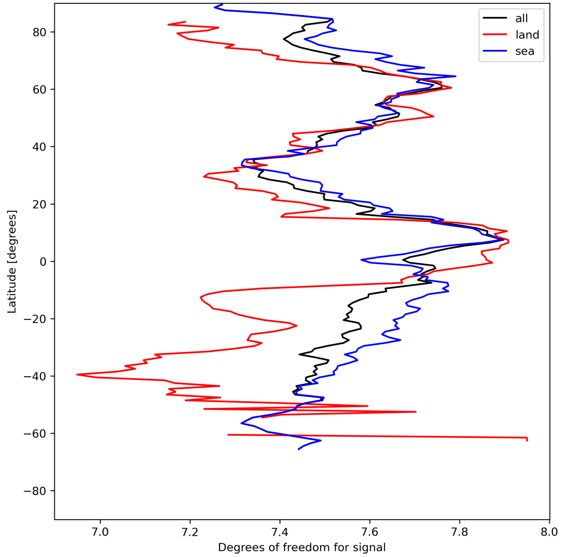
Figure 15: Zonal average of “Degrees of freedom for signal” for 2024-07-26 to 2024-07-27.
