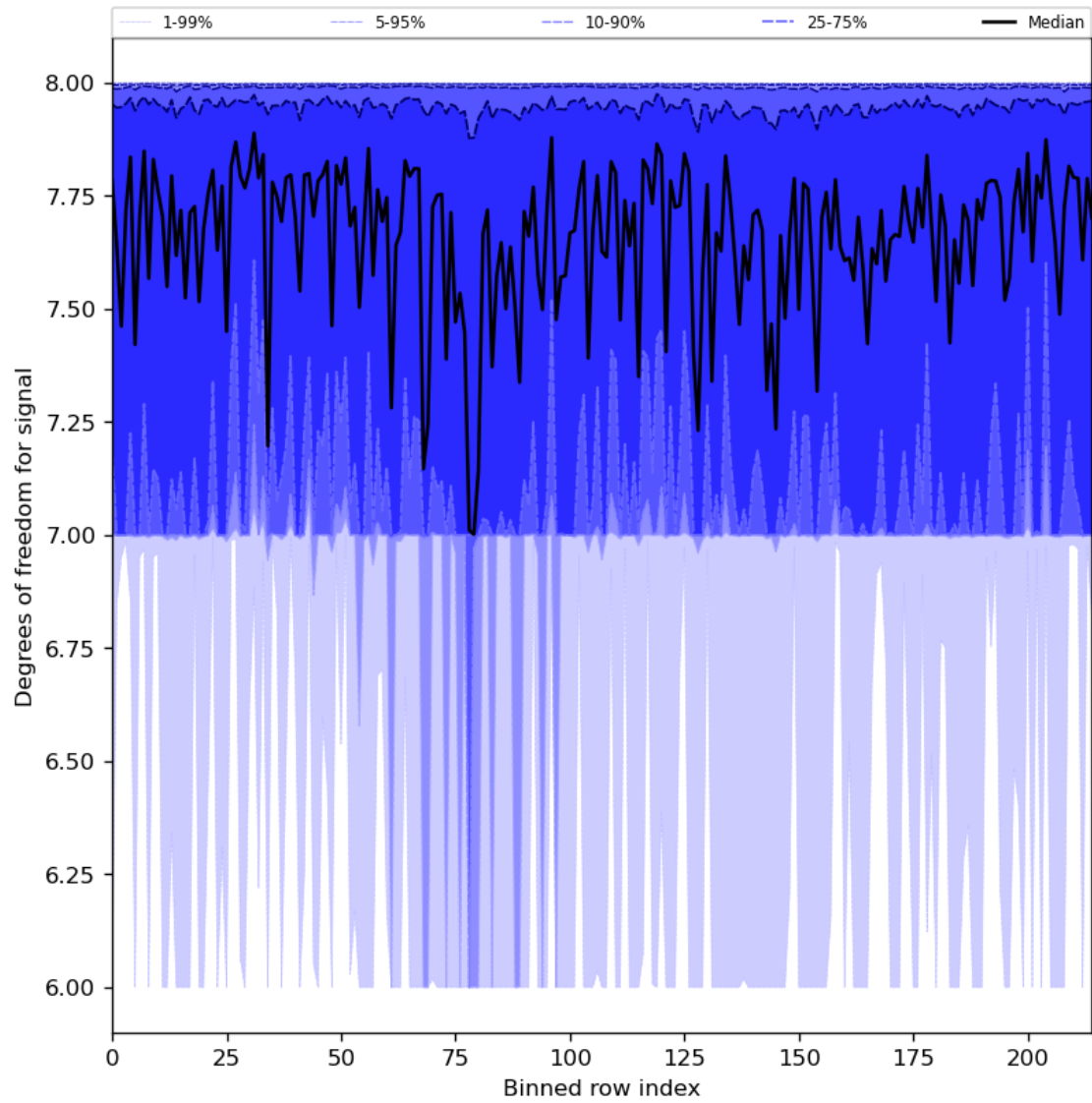
Figure 31: Along track statistics of “Degrees of freedom for signal” for 2024-07-26 to 2024-07-27
