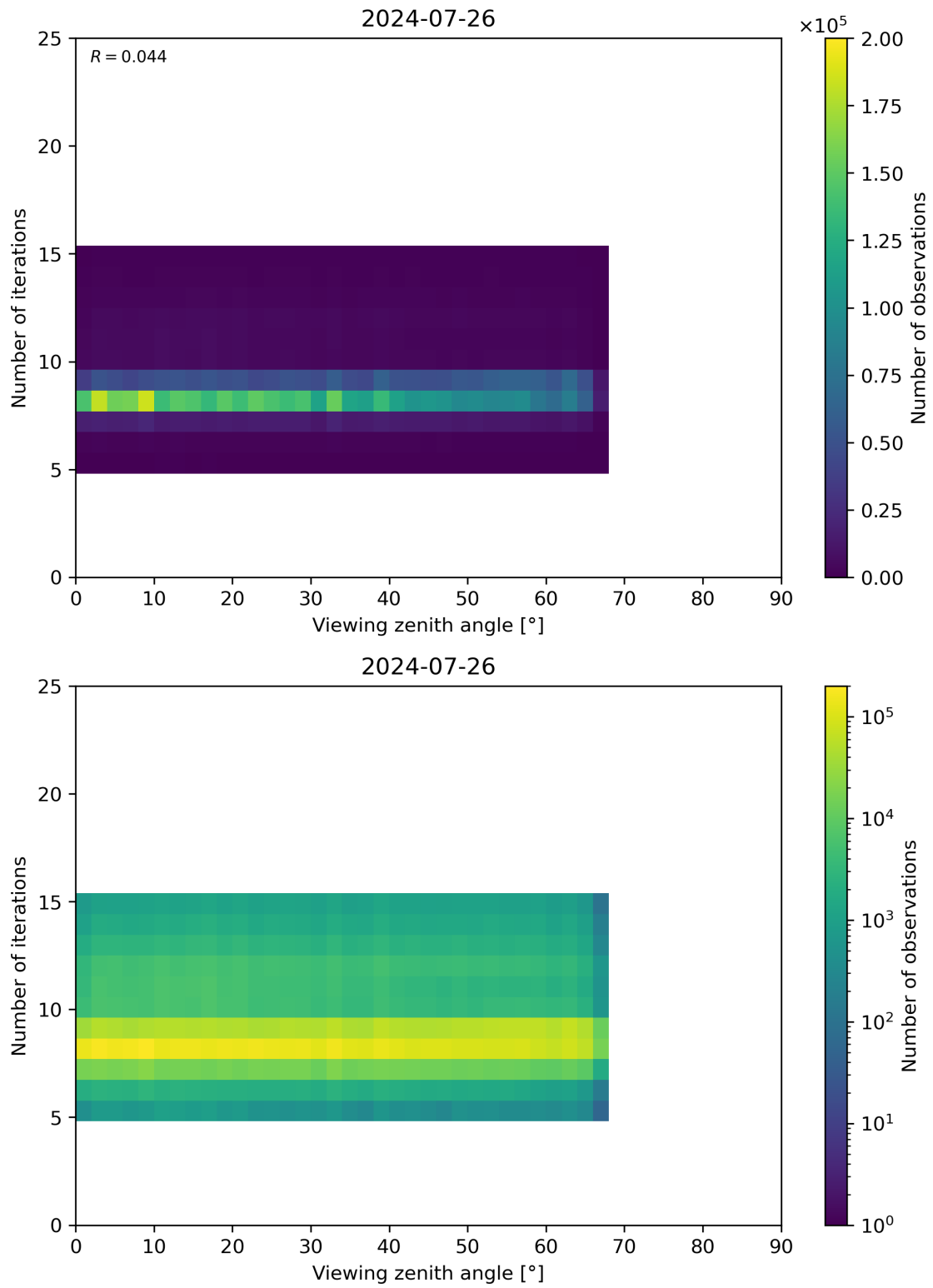
Figure 75: Scatter density plot of “Viewing zenith angle” against “Number of iterations” for 2024-07-26 to 2024-07-27.
