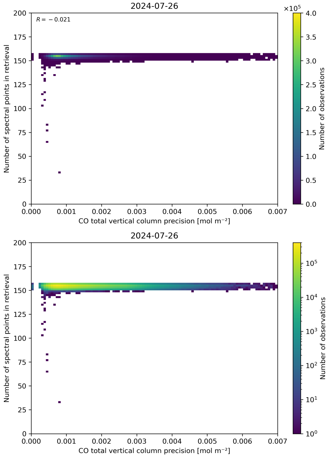
Figure 47: Scatter density plot of “CO total vertical column precision” against “Number of spectral points in retrieval” for 2024-07-26 to 2024-07-27.
