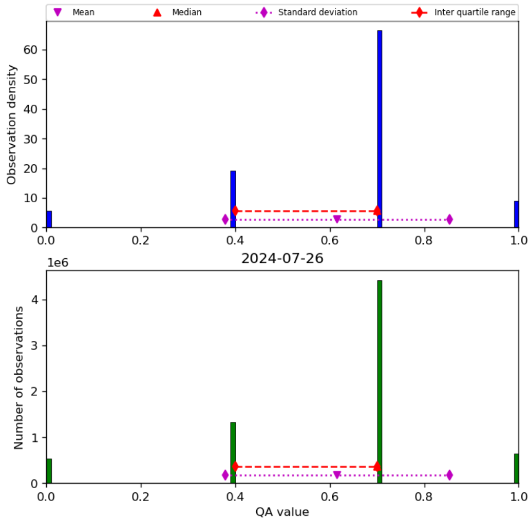
Figure 17: Histogram of “QA value” for 2024-07-26 to 2024-07-27
