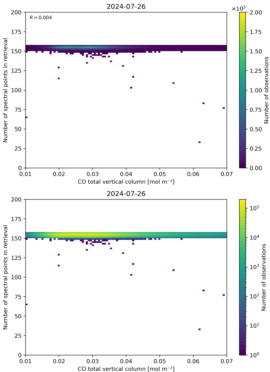
Figure 43: Scatter density plot of “CO total vertical column” against “Number of spectral points in retrieval” for 2024-07-26 to 2024-07-27.
