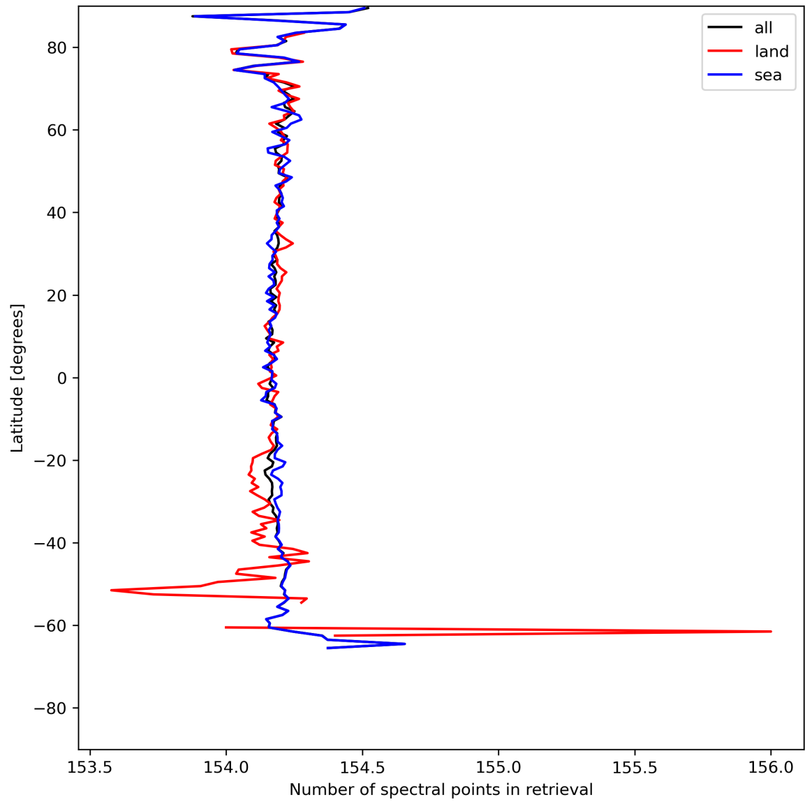
Figure 13: Zonal average of “Number of spectral points in retrieval” for 2024-07-26 to 2024-07-27.
