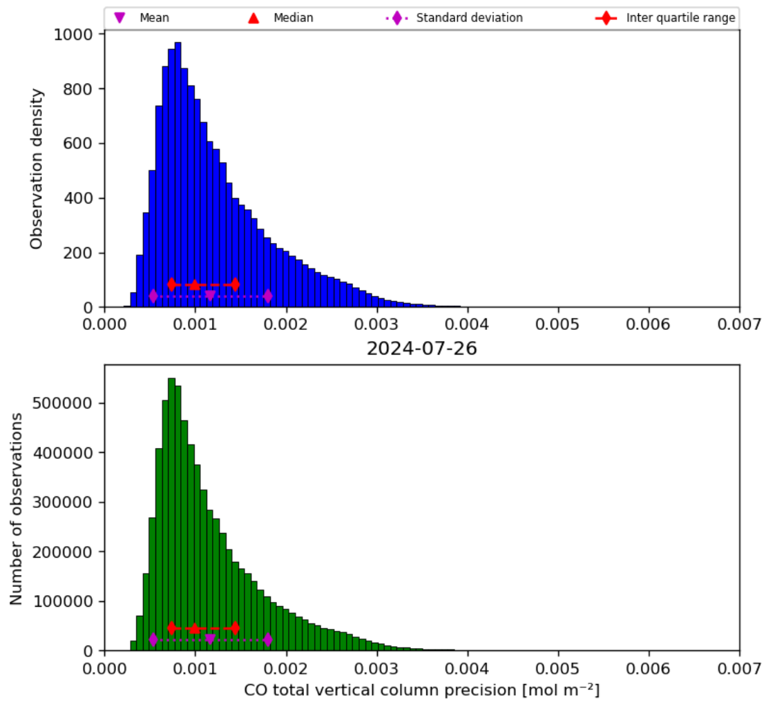
Figure 20: Histogram of “CO total vertical column precision” for 2024-07-26 to 2024-07-27
