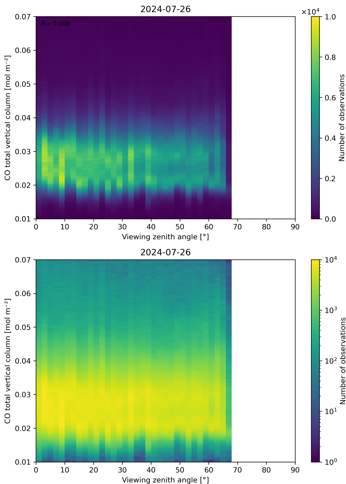
Figure 69: Scatter density plot of “Viewing zenith angle” against “CO total vertical column” for 2024-07-26 to 2024-07-27.
