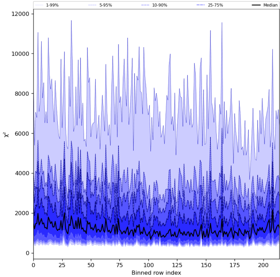
Figure 30: Along track statistics of “ \chi^2 ” for 2024-07-26 to 2024-07-27
