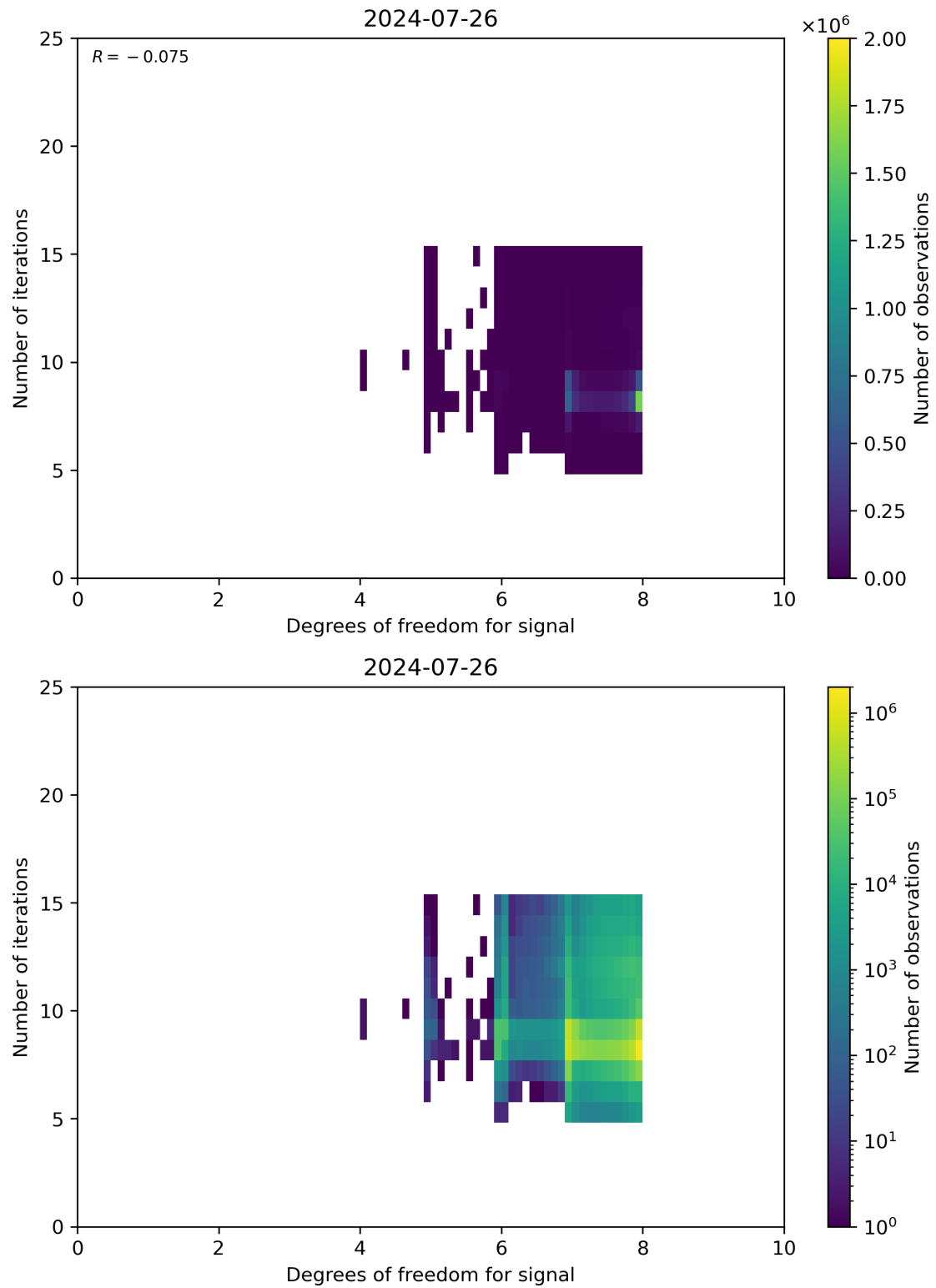
Figure 50: Scatter density plot of “Degrees of freedom for signal” against “Number of iterations” for 2024-07-26 to 2024-07-27.
