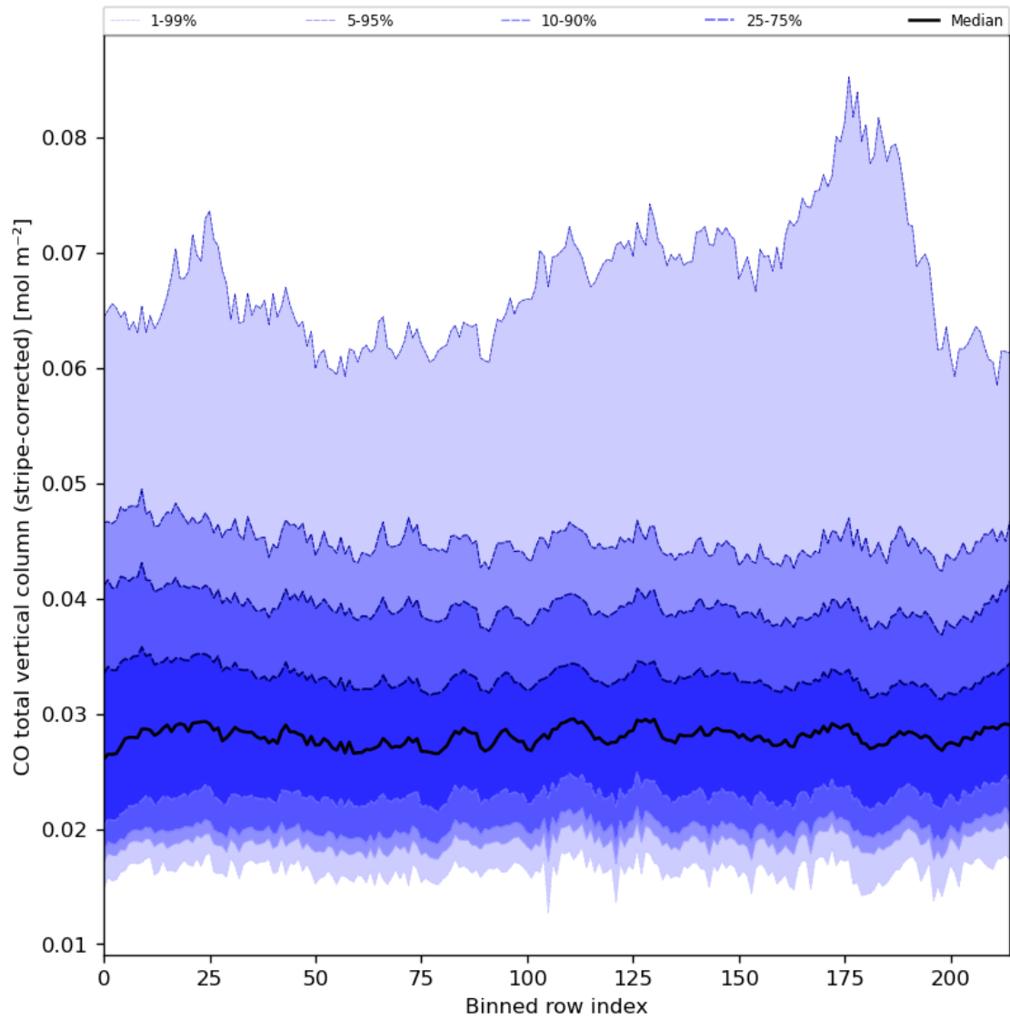
Figure 27: Along track statistics of “CO total vertical column (stripe-corrected)” for 2024-07-26 to 2024-07-27
