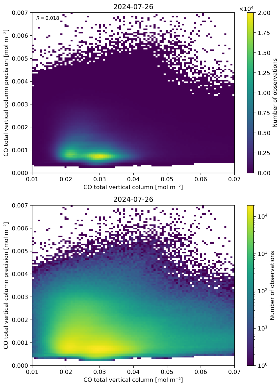
Figure 34: Scatter density plot of “CO total vertical column” against “CO total vertical column precision” for 2024-07-26 to 2024-07-27.
