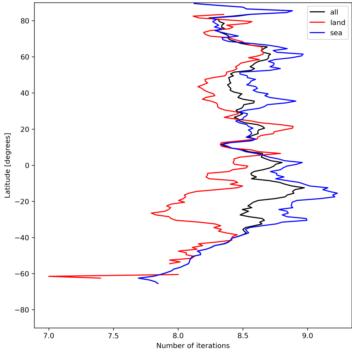
Figure 16: Zonal average of “Number of iterations” for 2024-07-26 to 2024-07-27.
