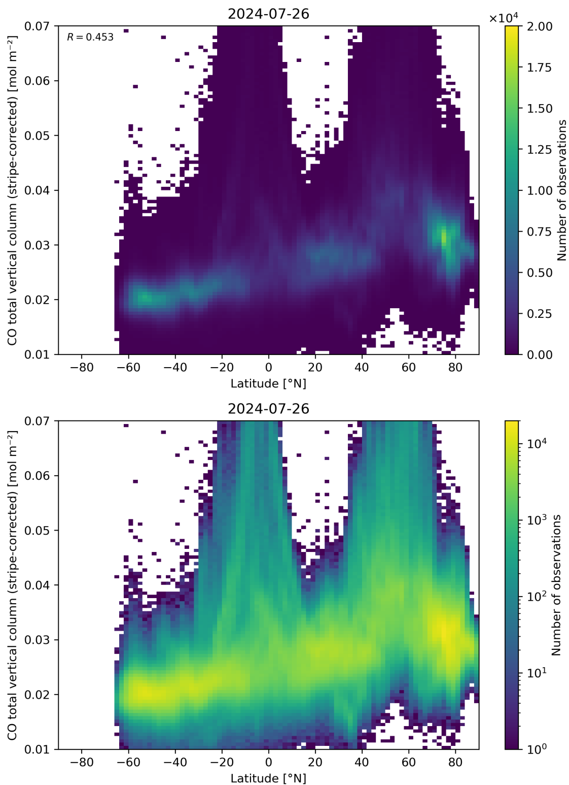
Figure 52: Scatter density plot of “Latitude” against “CO total vertical column (stripe-corrected)” for 2024-07-26 to 2024-07-27.
