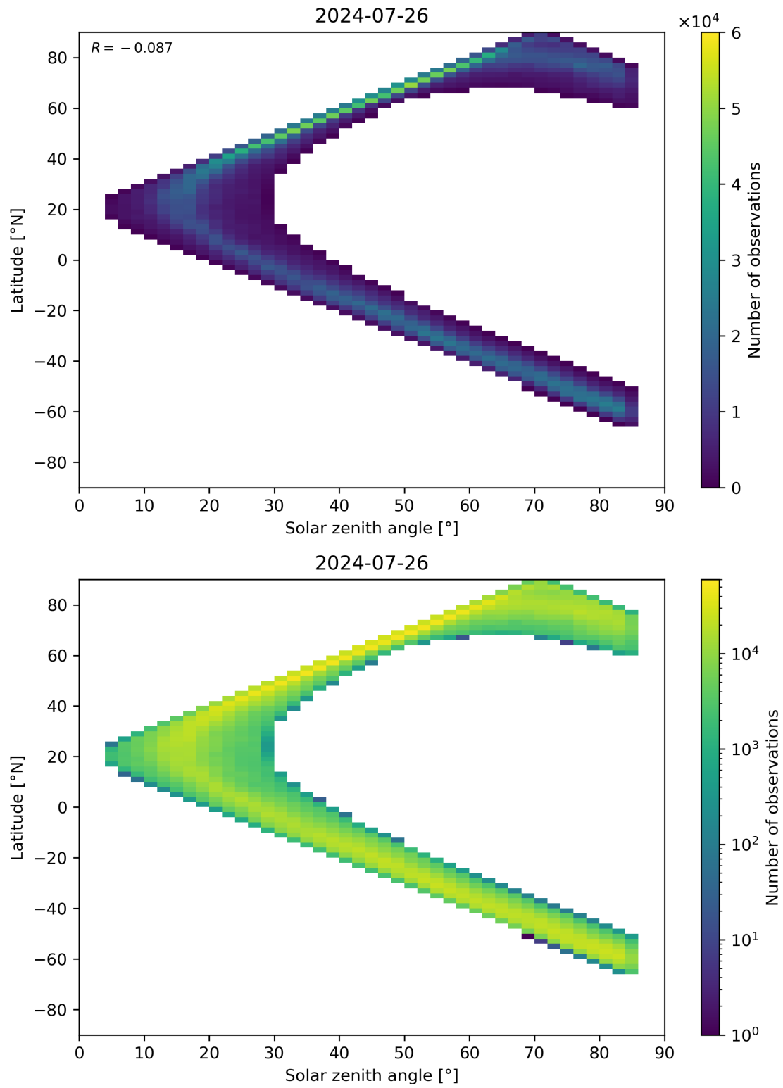
Figure 66: Scatter density plot of “Solar zenith angle” against “Latitude” for 2024-07-26 to 2024-07-27.
