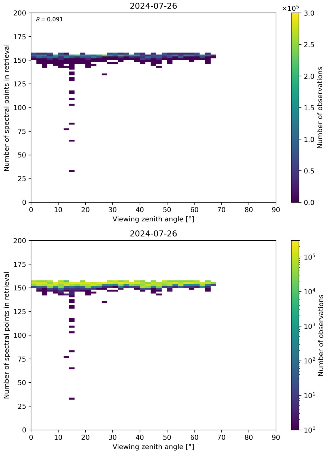
Figure 76: Scatter density plot of “Viewing zenith angle” against “Number of spectral points in retrieval” for 2024-07-26 to 2024-07-27.
