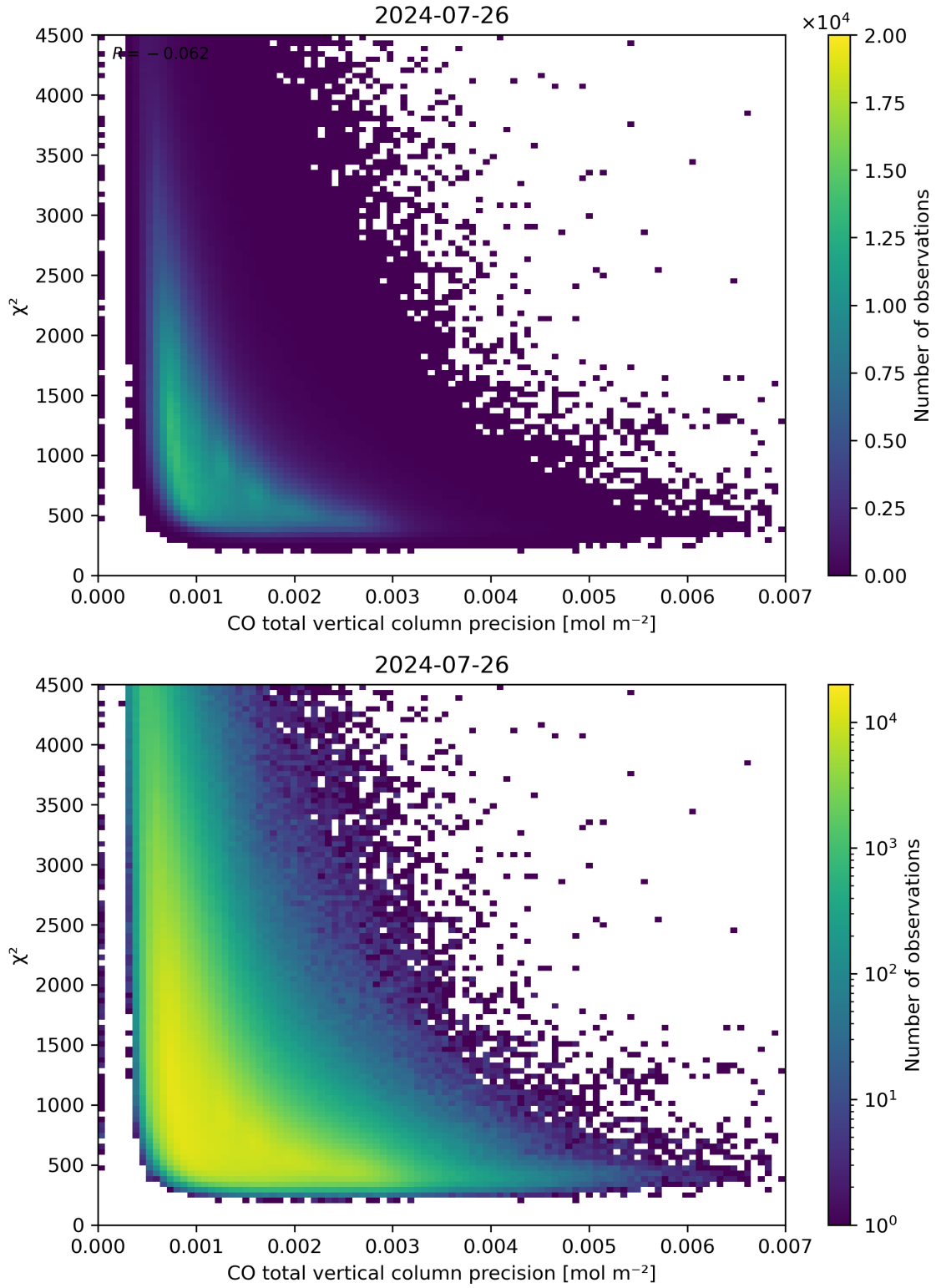
Figure 44: Scatter density plot of “CO total vertical column precision” against “ \chi^2 ” for 2024-07-26 to 2024-07-27.
