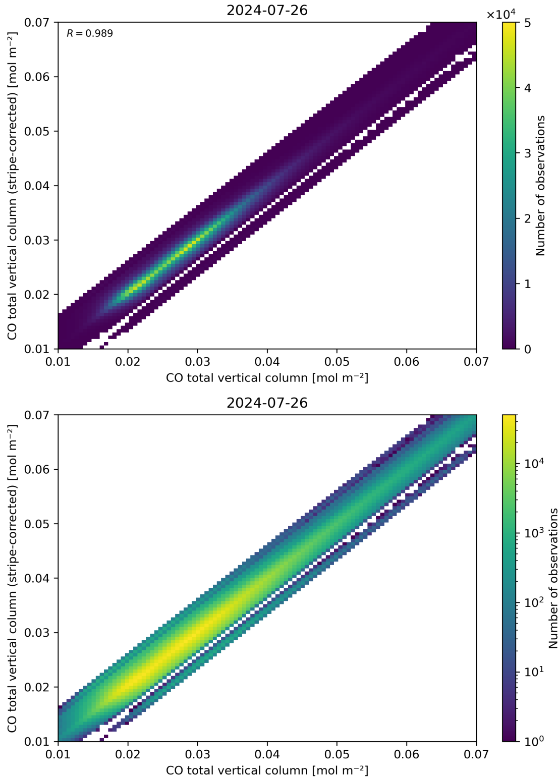
Figure 33: Scatter density plot of “CO total vertical column” against “CO total vertical column (stripe-corrected)” for 2024-07-26 to 2024-07-27.
