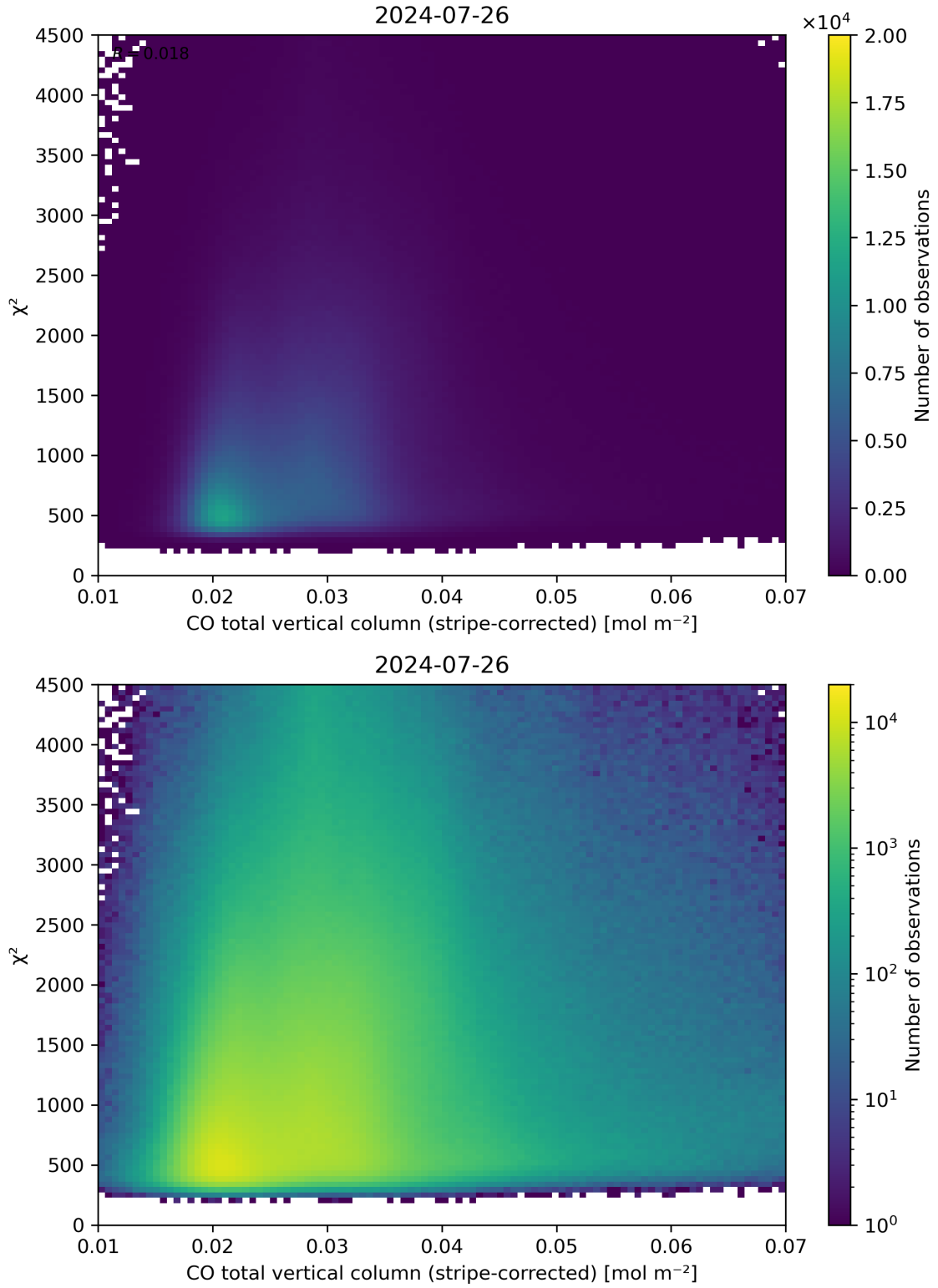
Figure 37: Scatter density plot of “CO total vertical column (stripe-corrected)” against “ \chi^2 ” for 2024-07-26 to 2024-07-27.
