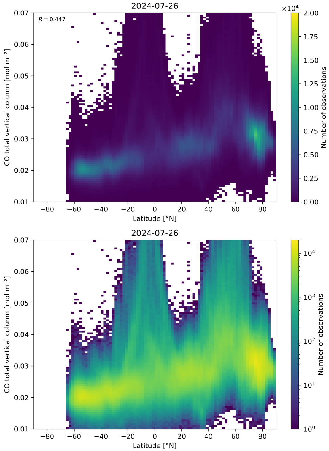
Figure 51: Scatter density plot of “Latitude” against “CO total vertical column” for 2024-07-26 to 2024-07-27.
