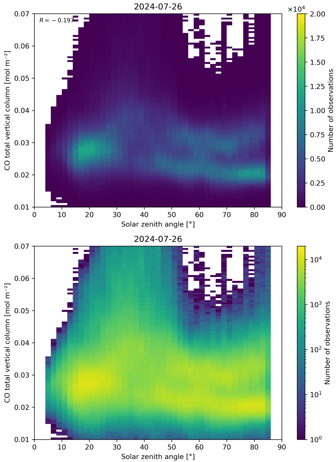
Figure 61: Scatter density plot of “Solar zenith angle” against “CO total vertical column” for 2024-07-26 to 2024-07-27.
