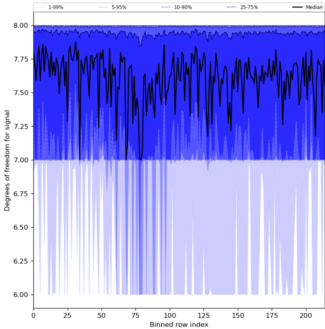
Figure 31: Along track statistics of “Degrees of freedom for signal” for 2024-07-26 to 2024-07-28
