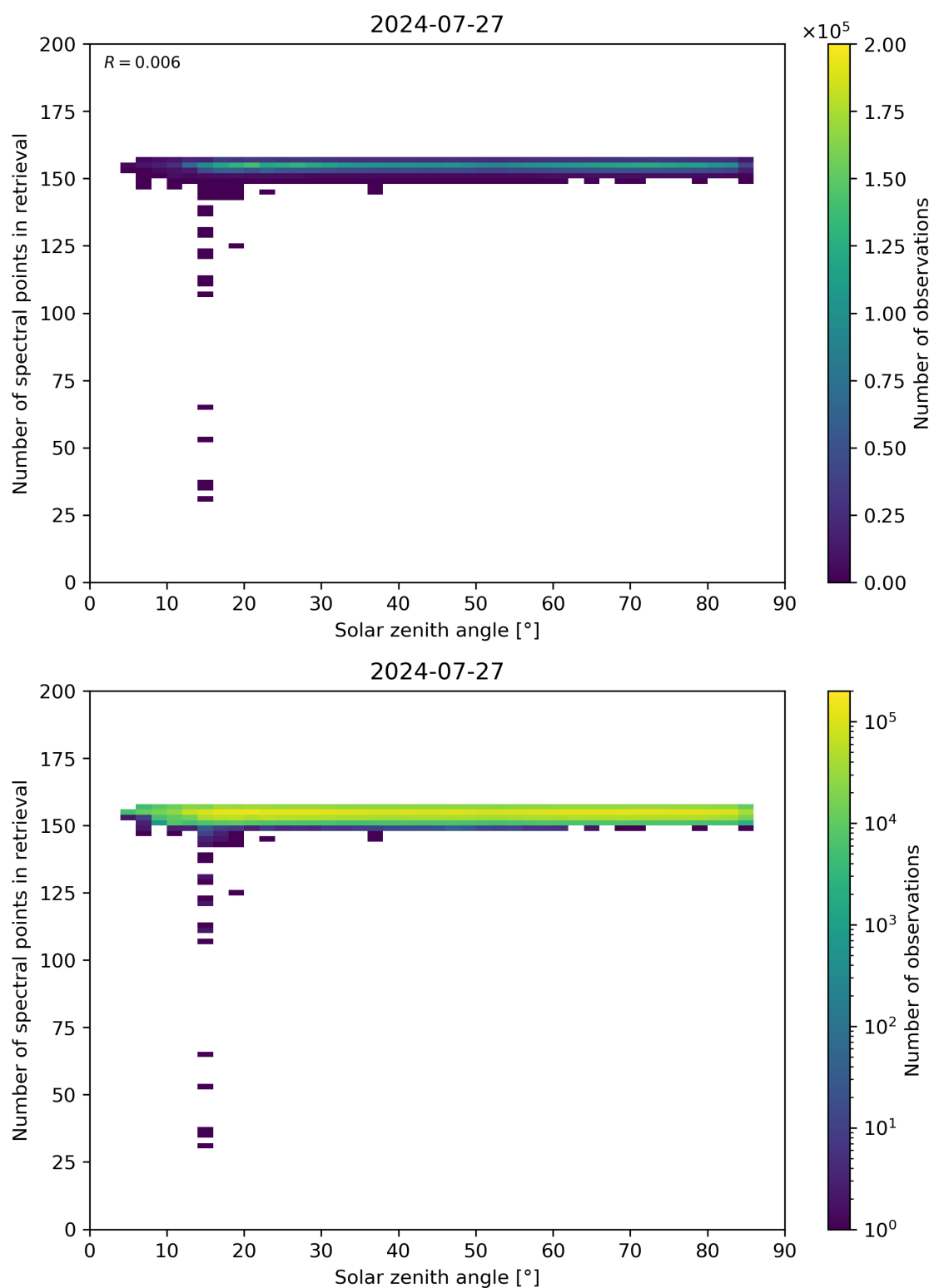
Figure 68: Scatter density plot of “Solar zenith angle” against “Number of spectral points in retrieval” for 2024-07-26 to 2024-07-28.
