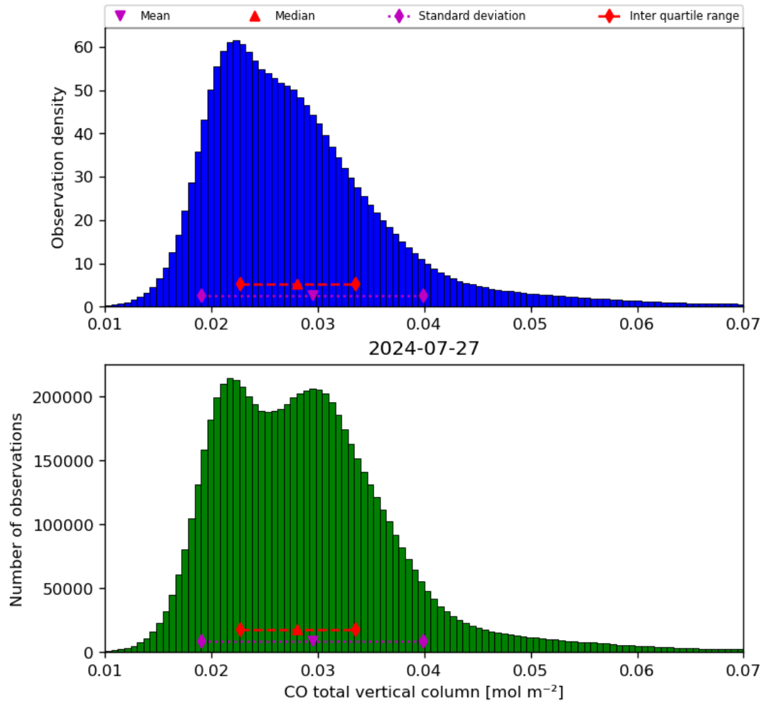
Figure 18: Histogram of “CO total vertical column” for 2024-07-26 to 2024-07-28
