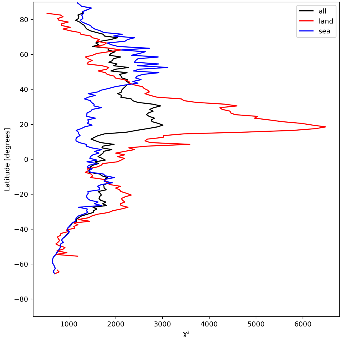
Figure 14: Zonal average of “ \chi^2 ” for 2024-07-26 to 2024-07-28.
