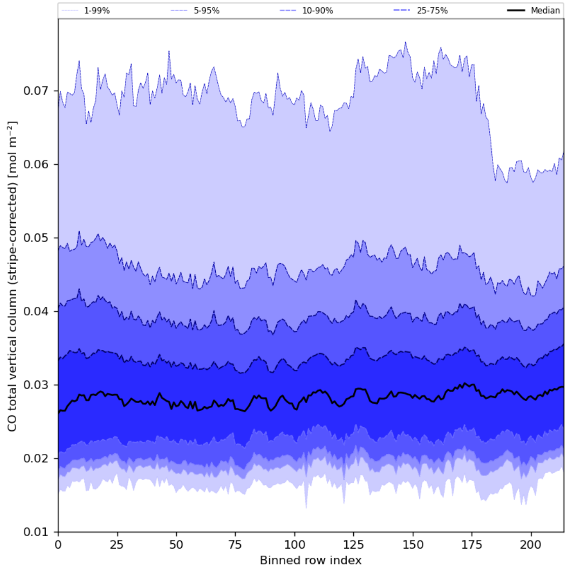
Figure 27: Along track statistics of “CO total vertical column (stripe-corrected)” for 2024-07-26 to 2024-07-28
