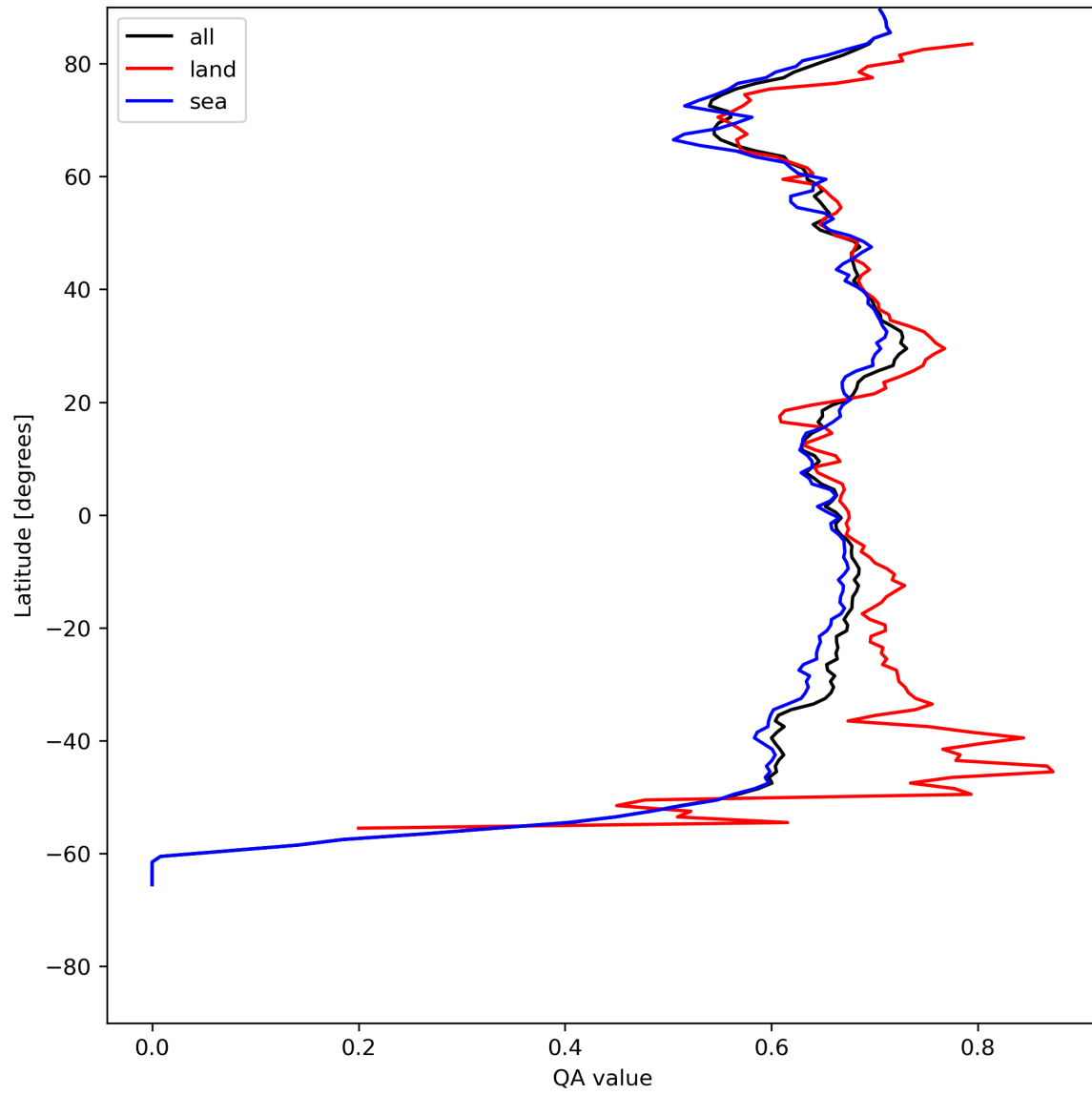
Figure 9: Zonal average of “QA value” for 2024-07-26 to 2024-07-28.
