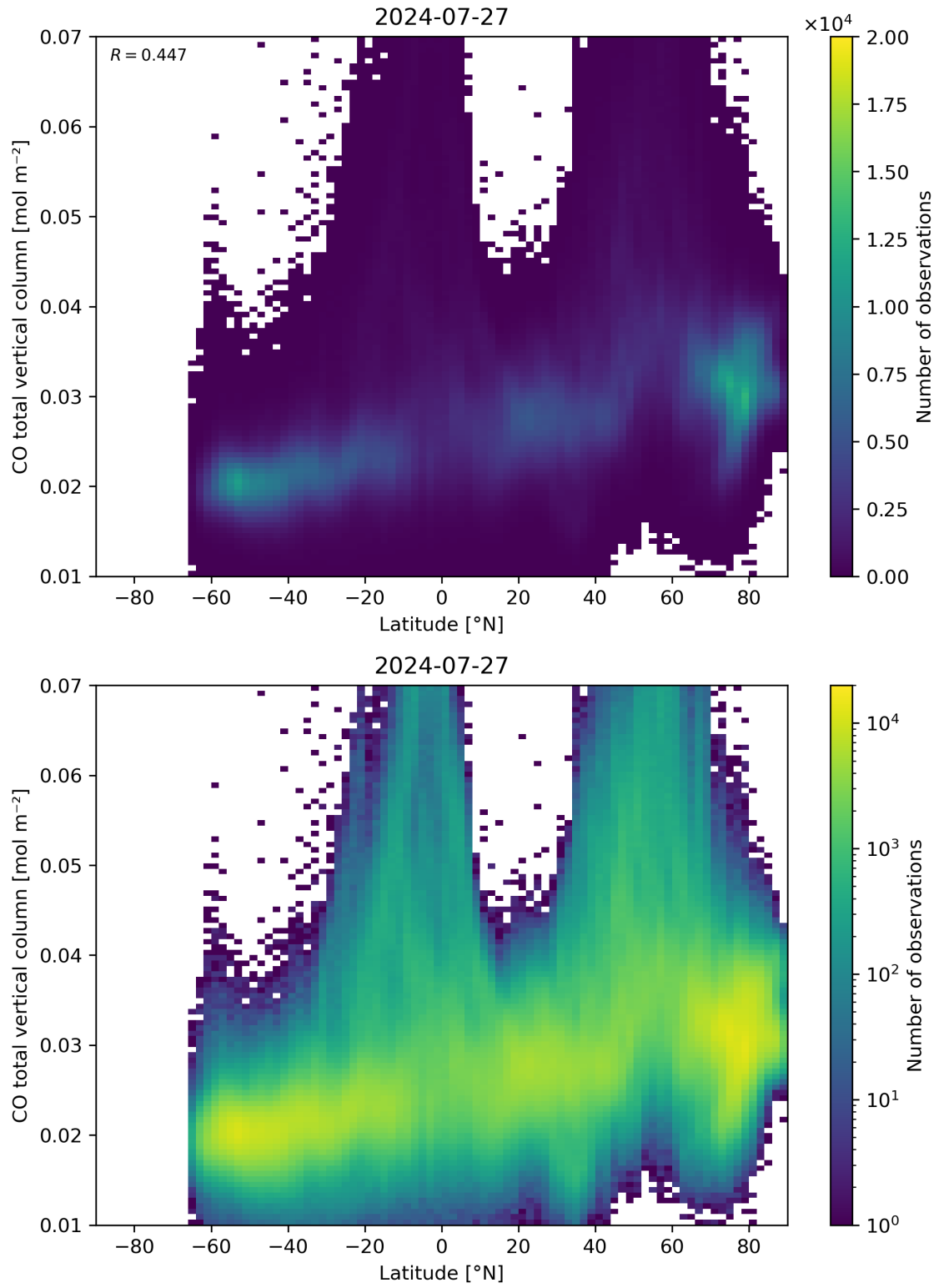
Figure 51: Scatter density plot of “Latitude” against “CO total vertical column” for 2024-07-26 to 2024-07-28.
