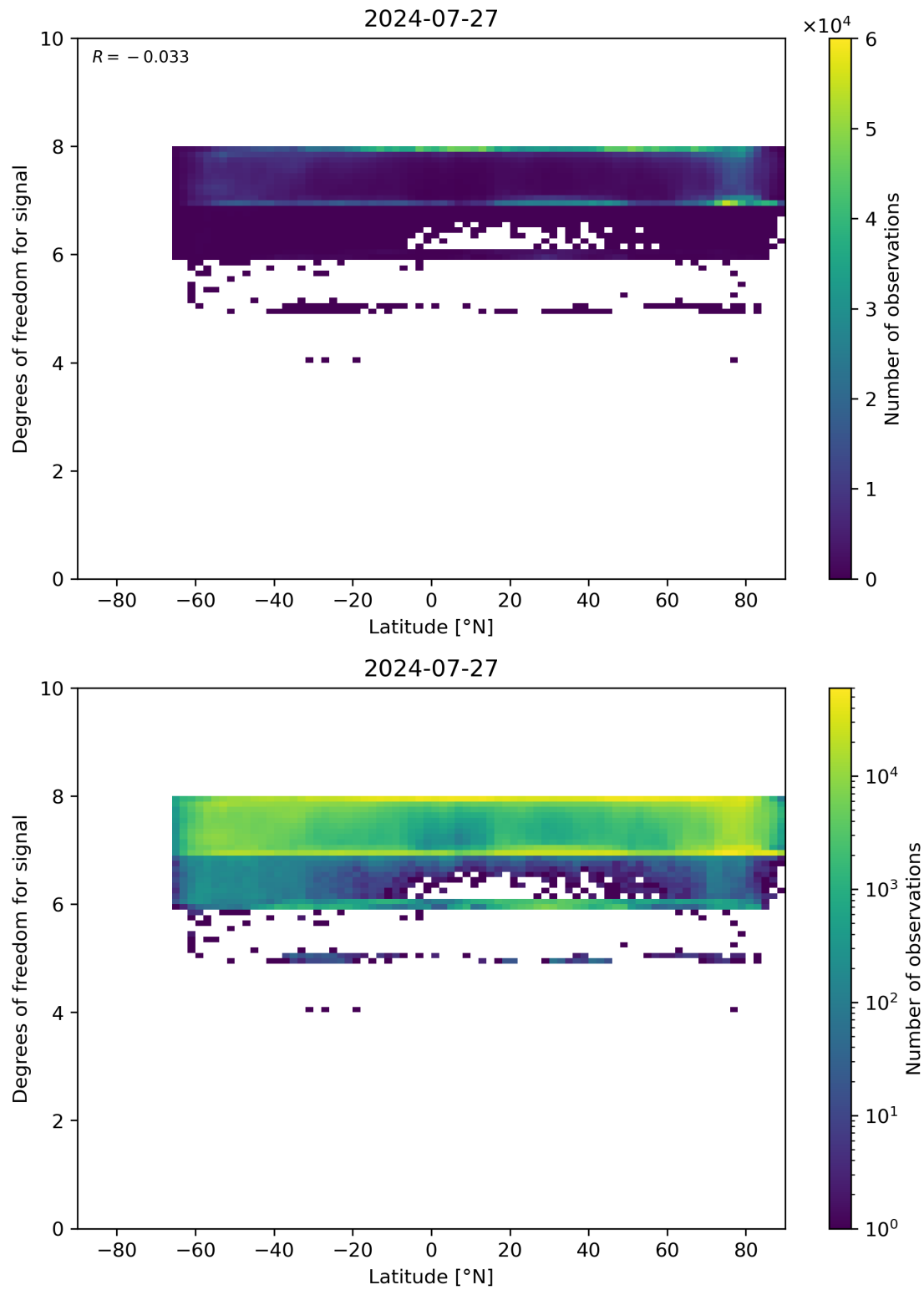
Figure 55: Scatter density plot of “Latitude” against “Degrees of freedom for signal” for 2024-07-26 to 2024-07-28.
