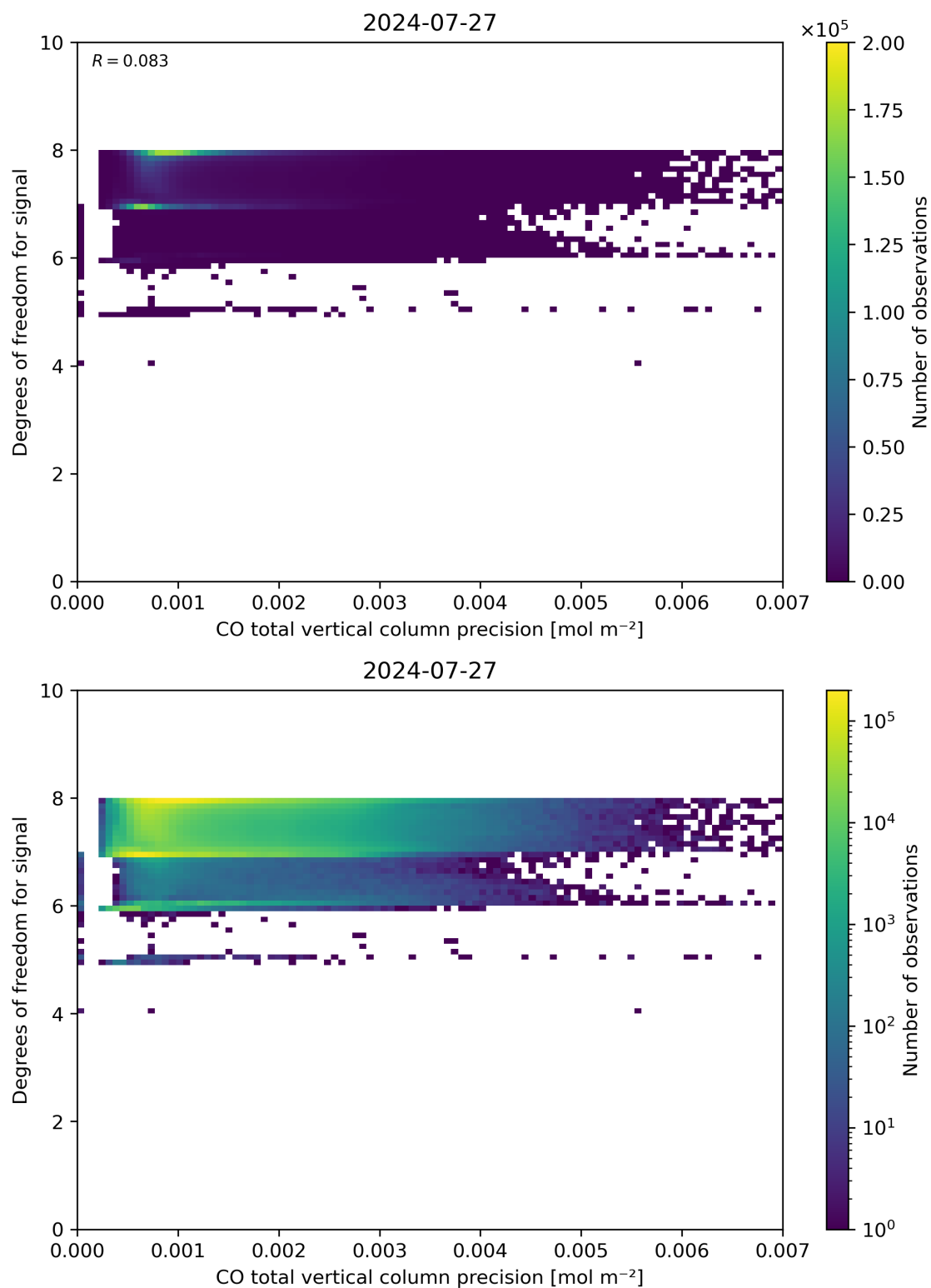
Figure 45: Scatter density plot of “CO total vertical column precision” against “Degrees of freedom for signal” for 2024-07-26 to 2024-07-28.
