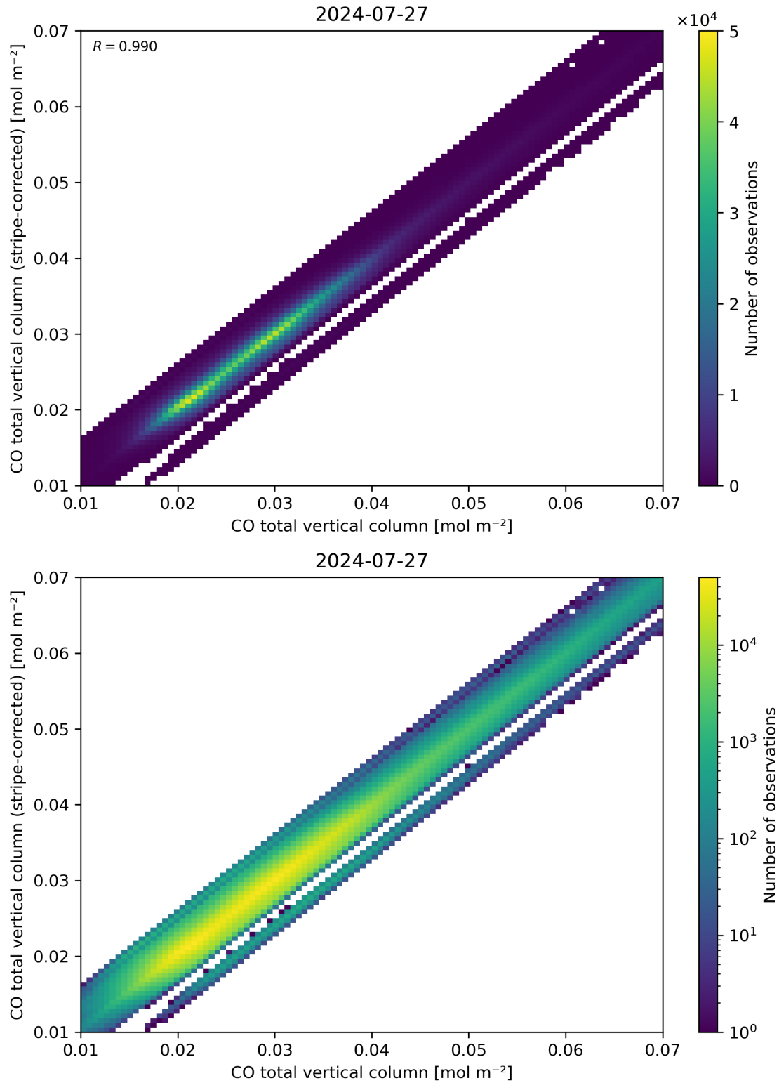
Figure 33: Scatter density plot of “CO total vertical column” against “CO total vertical column (stripe-corrected)” for 2024-07-26 to 2024-07-28.
