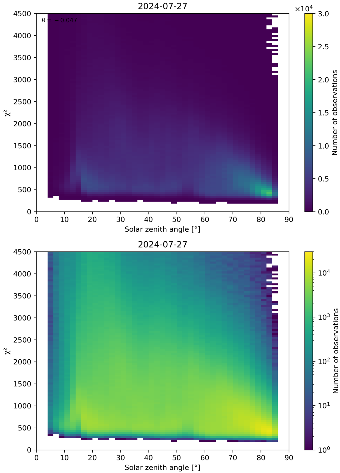
Figure 64: Scatter density plot of “Solar zenith angle” against “ \chi^2 ” for 2024-07-26 to 2024-07-28.
