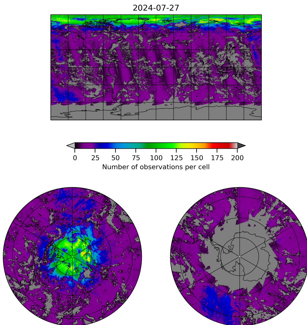
Figure 8: Map of the number of observations for 2024-07-26 to 2024-07-28
