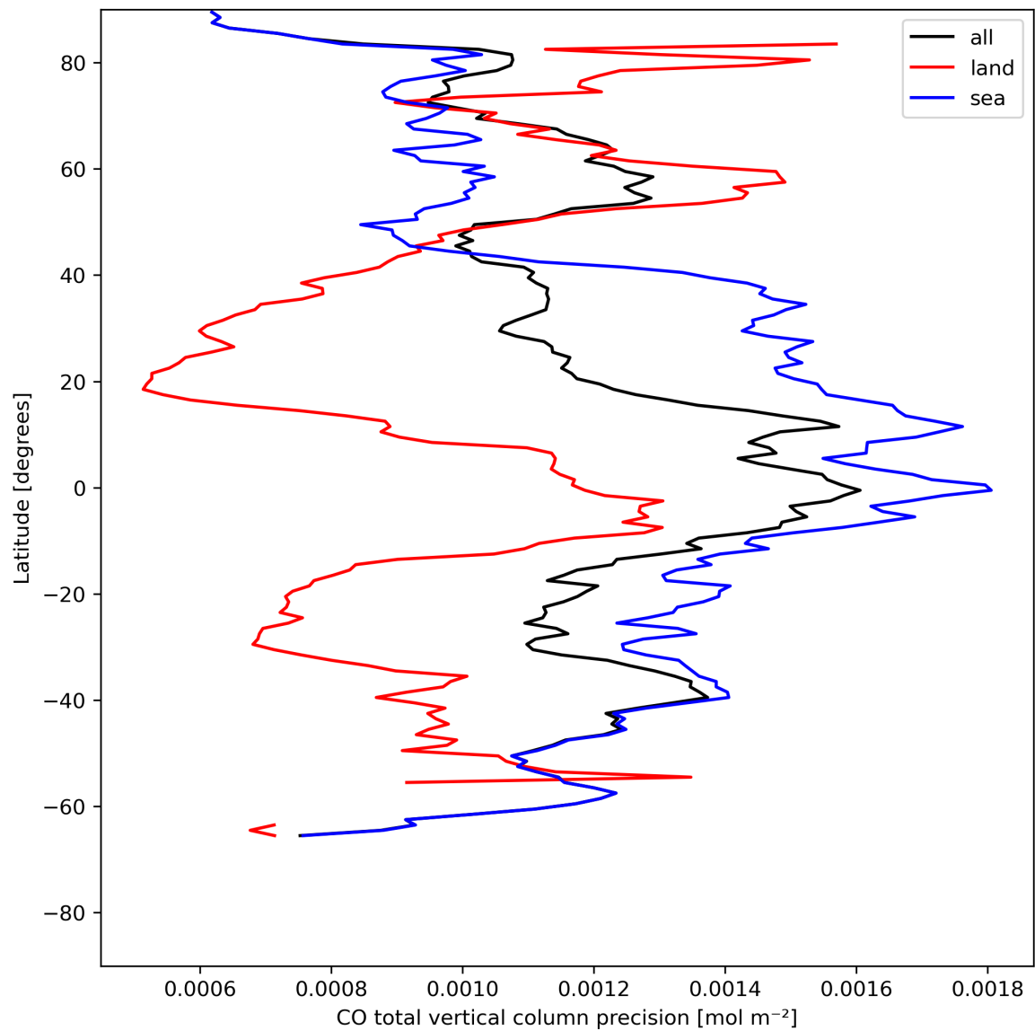
Figure 12: Zonal average of “CO total vertical column precision” for 2024-07-26 to 2024-07-28.
