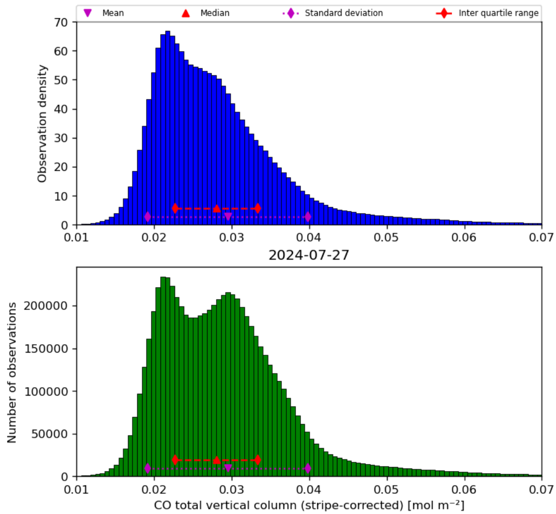
Figure 19: Histogram of “CO total vertical column (stripe-corrected)” for 2024-07-26 to 2024-07-28
