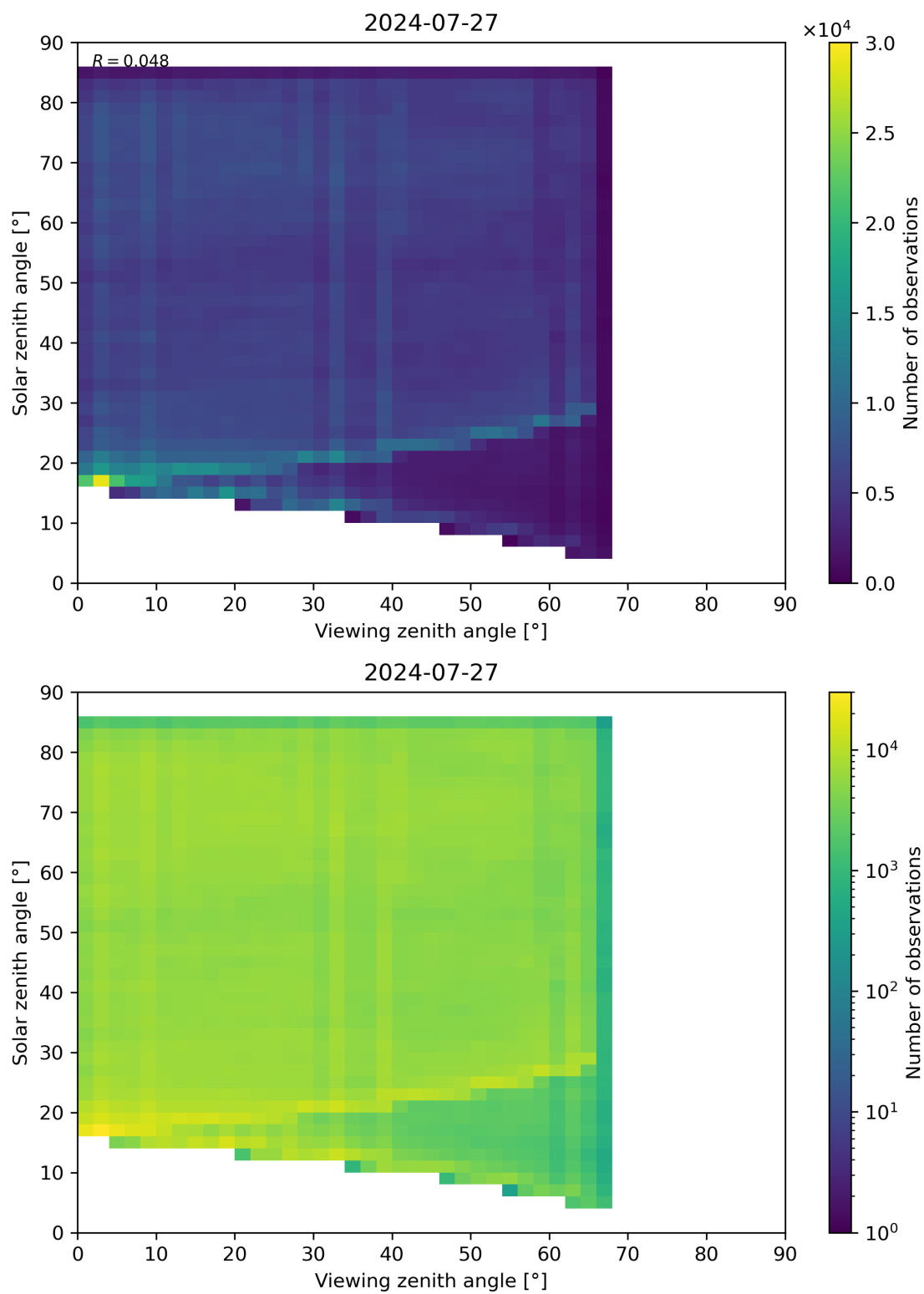
Figure 77: Scatter density plot of “Viewing zenith angle” against “Solar zenith angle” for 2024-07-26 to 2024-07-28.
