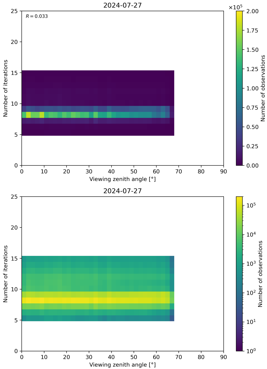
Figure 75: Scatter density plot of “Viewing zenith angle” against “Number of iterations” for 2024-07-26 to 2024-07-28.
