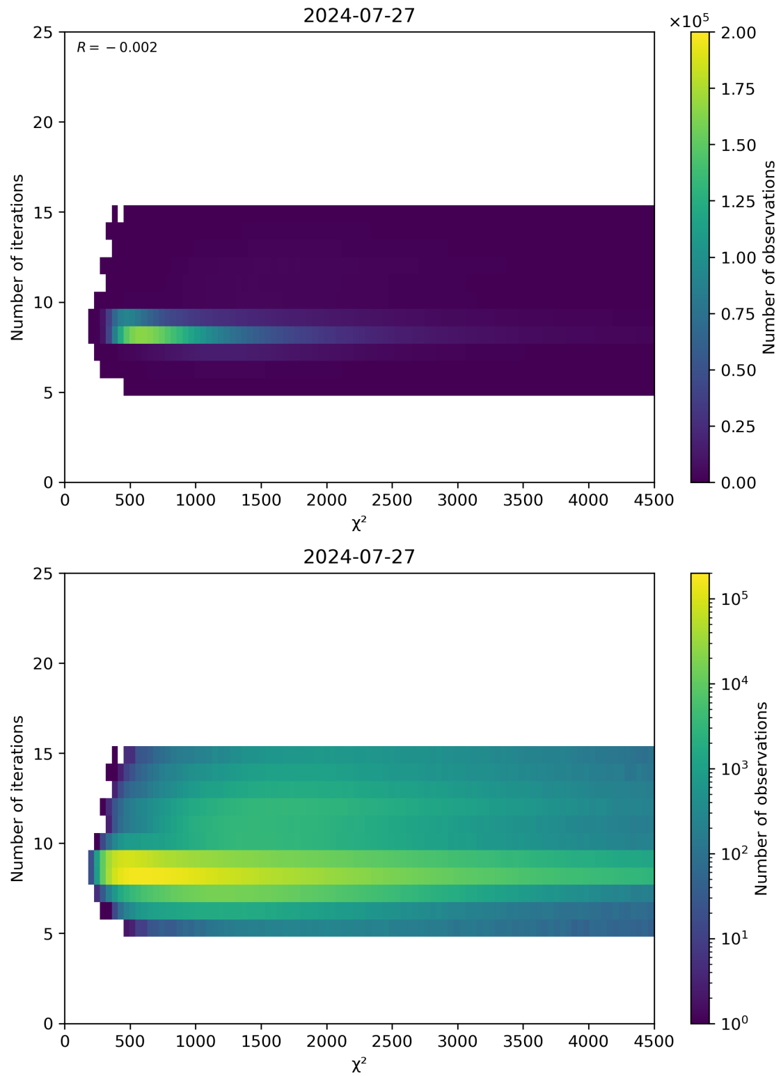
Figure 49: Scatter density plot of “ \chi^2 ” against “Number of iterations” for 2024-07-26 to 2024-07-28.
