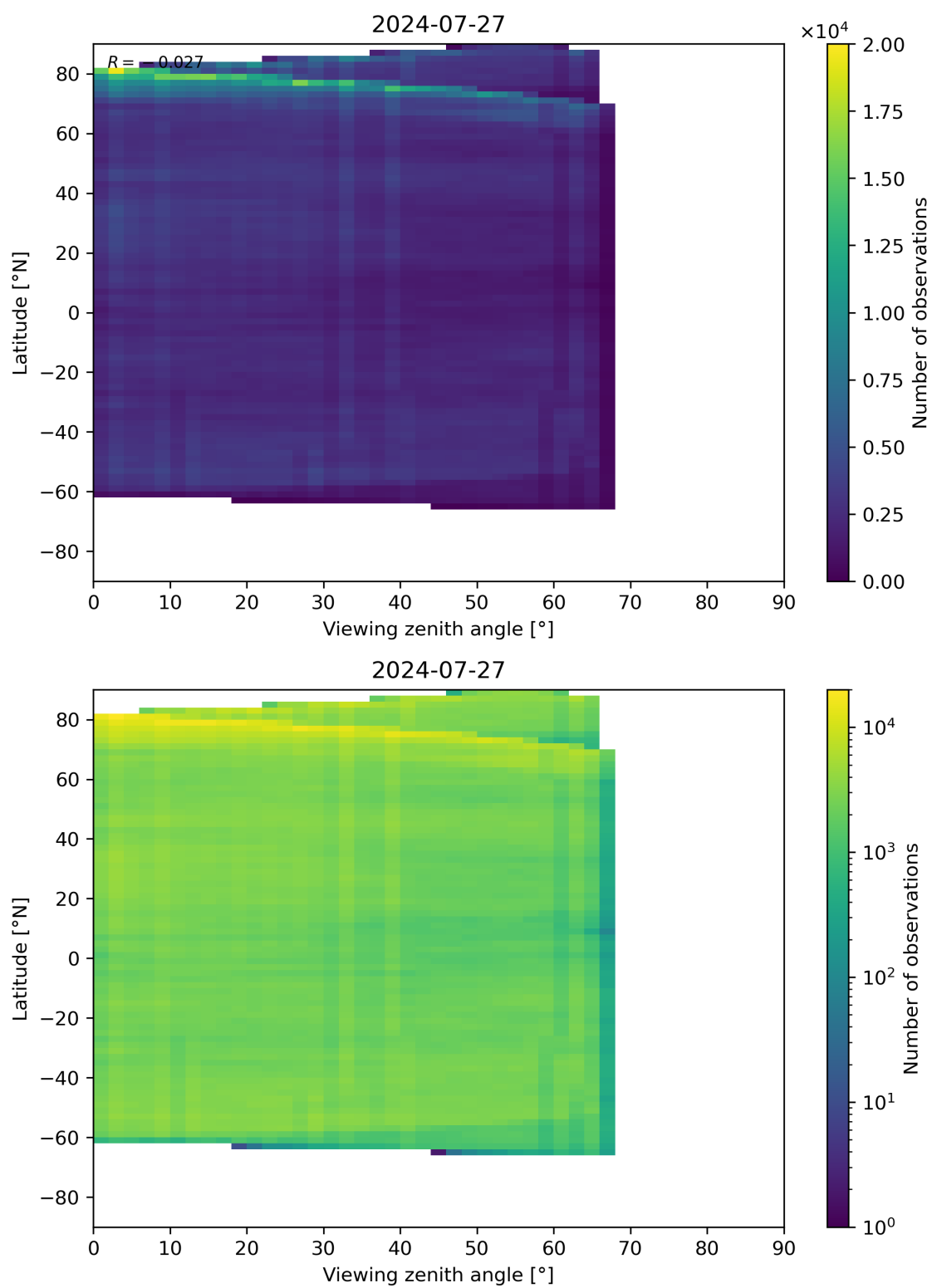
Figure 74: Scatter density plot of “Viewing zenith angle” against “Latitude” for 2024-07-26 to 2024-07-28.
