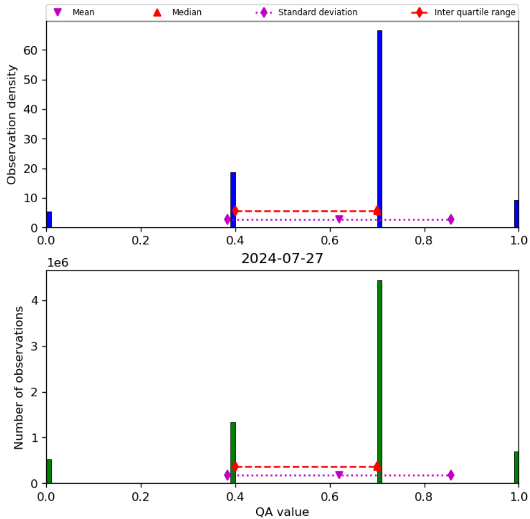
Figure 17: Histogram of “QA value” for 2024-07-26 to 2024-07-28
