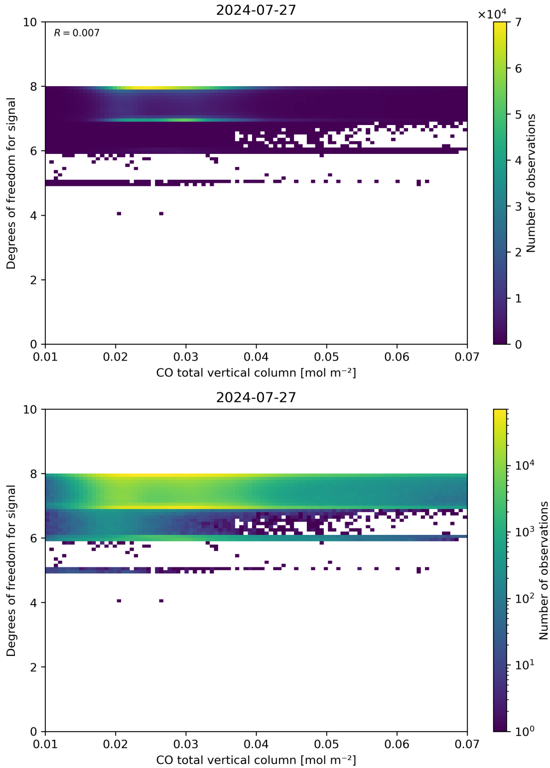
Figure 41: Scatter density plot of “CO total vertical column” against “Degrees of freedom for signal” for 2024-07-26 to 2024-07-28.
