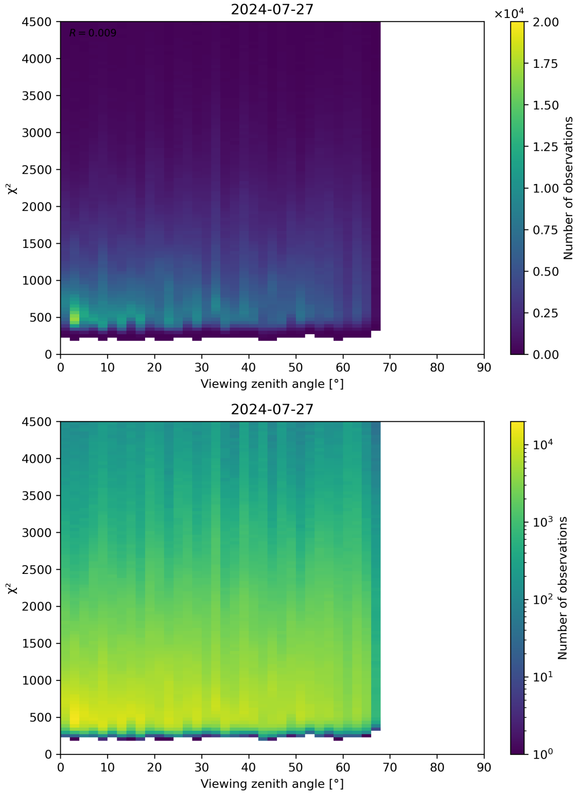
Figure 72: Scatter density plot of “Viewing zenith angle” against “ \chi^2 ” for 2024-07-26 to 2024-07-28.
