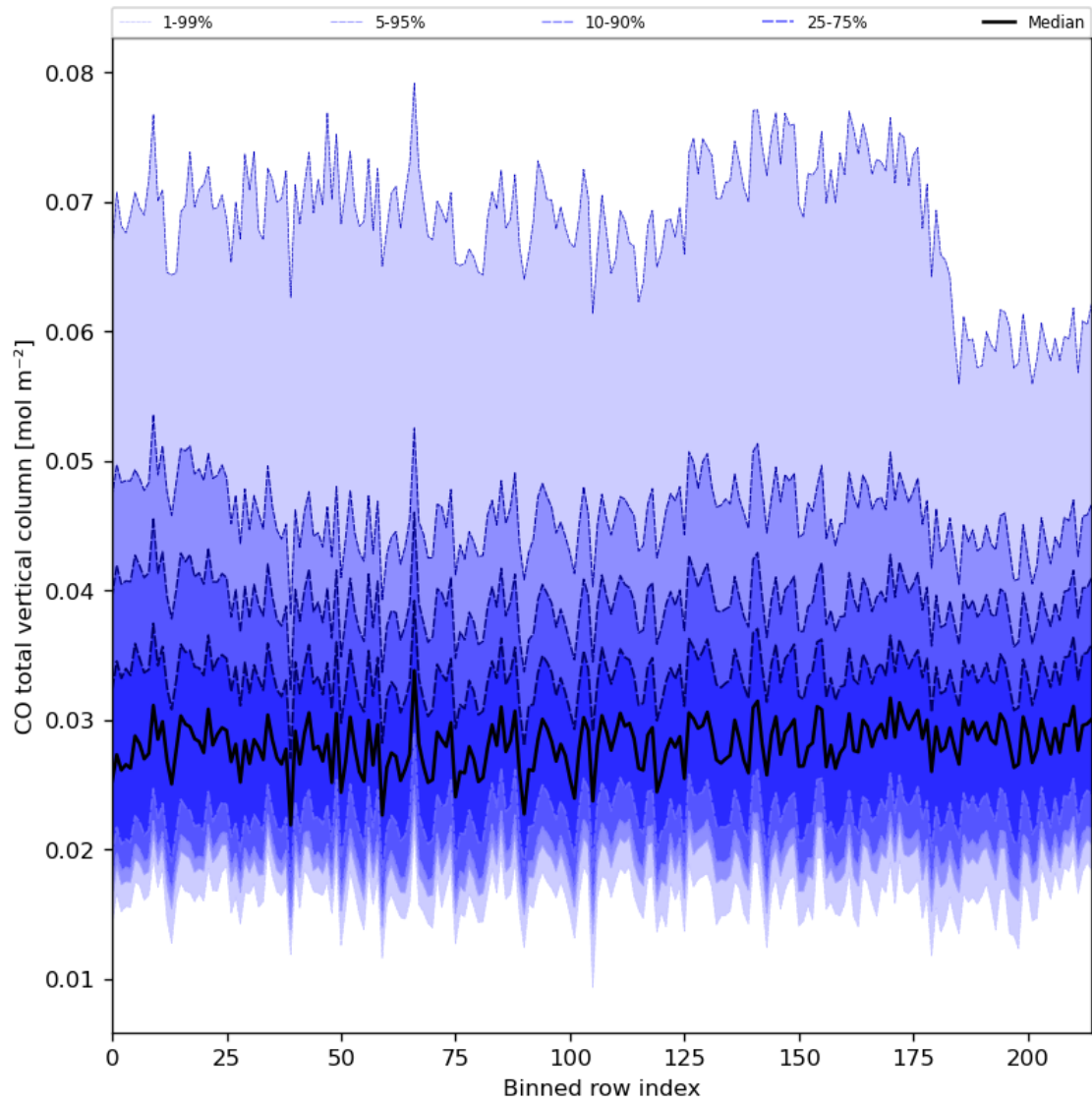
Figure 26: Along track statistics of “CO total vertical column” for 2024-07-26 to 2024-07-28
