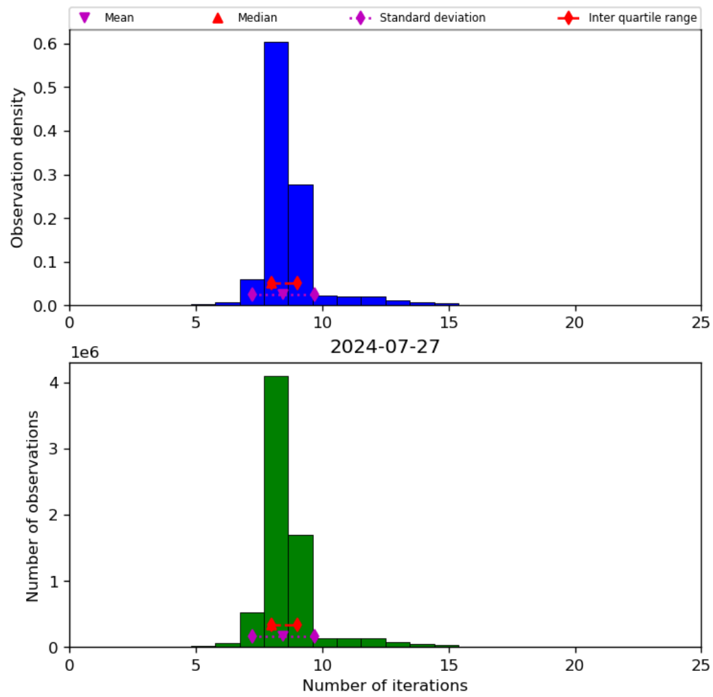
Figure 24: Histogram of “Number of iterations” for 2024-07-26 to 2024-07-28
