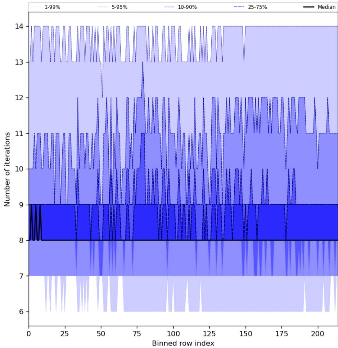
Figure 32: Along track statistics of “Number of iterations” for 2024-07-26 to 2024-07-28
