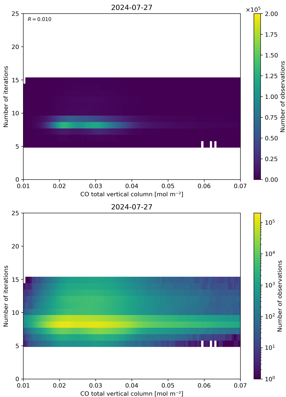
Figure 42: Scatter density plot of “CO total vertical column” against “Number of iterations” for 2024-07-26 to 2024-07-28.
