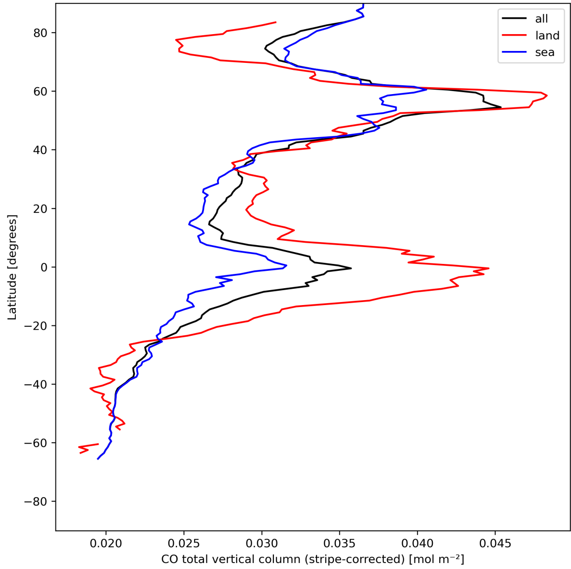
Figure 11: Zonal average of “CO total vertical column (stripe-corrected)” for 2024-07-27 to 2024-07-29.
