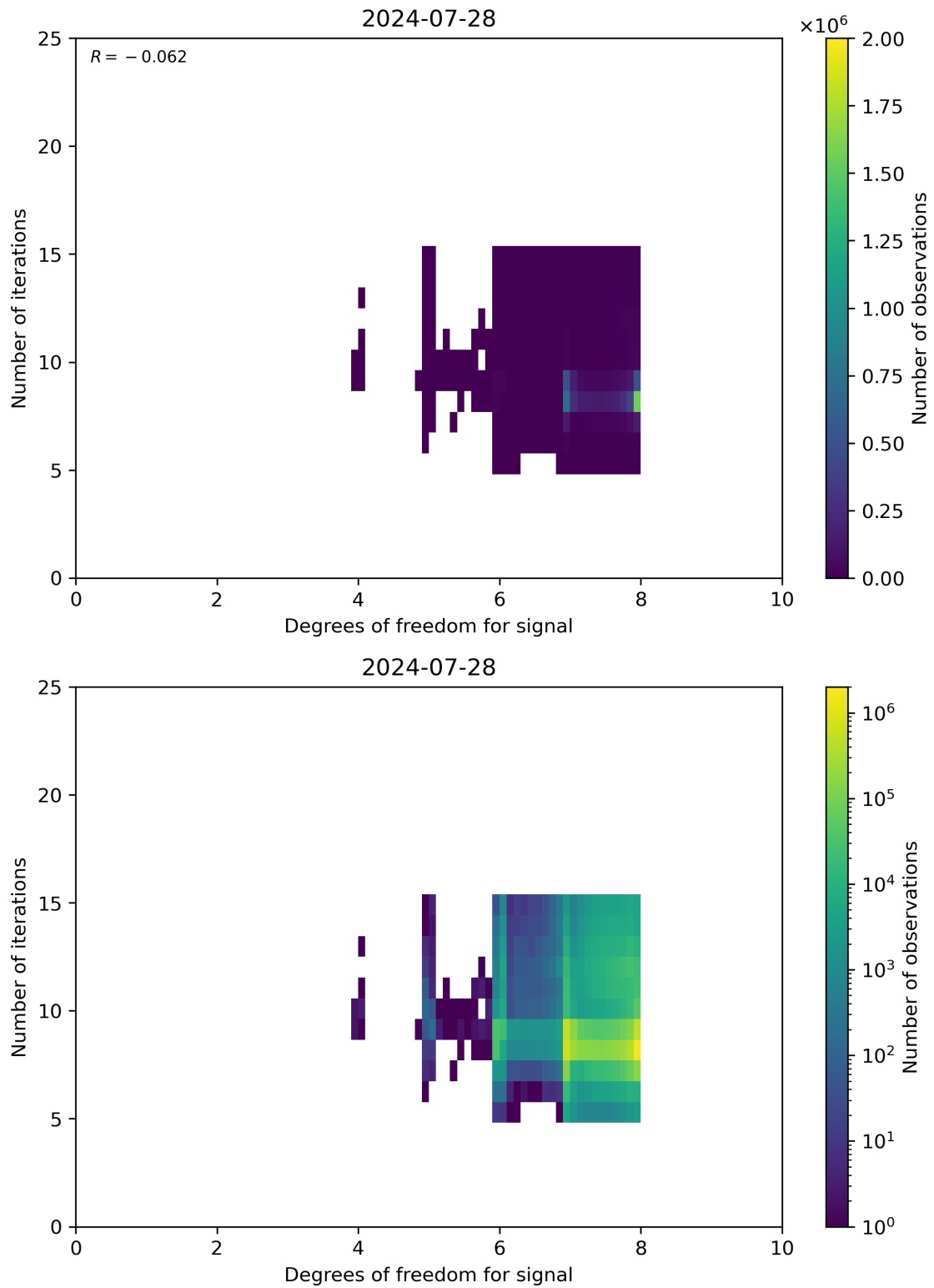
Figure 50: Scatter density plot of “Degrees of freedom for signal” against “Number of iterations” for 2024-07-27 to 2024-07-29.
