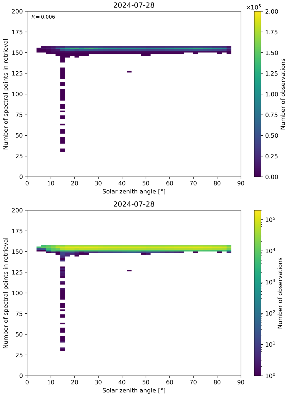
Figure 68: Scatter density plot of “Solar zenith angle” against “Number of spectral points in retrieval” for 2024-07-27 to 2024-07-29.
