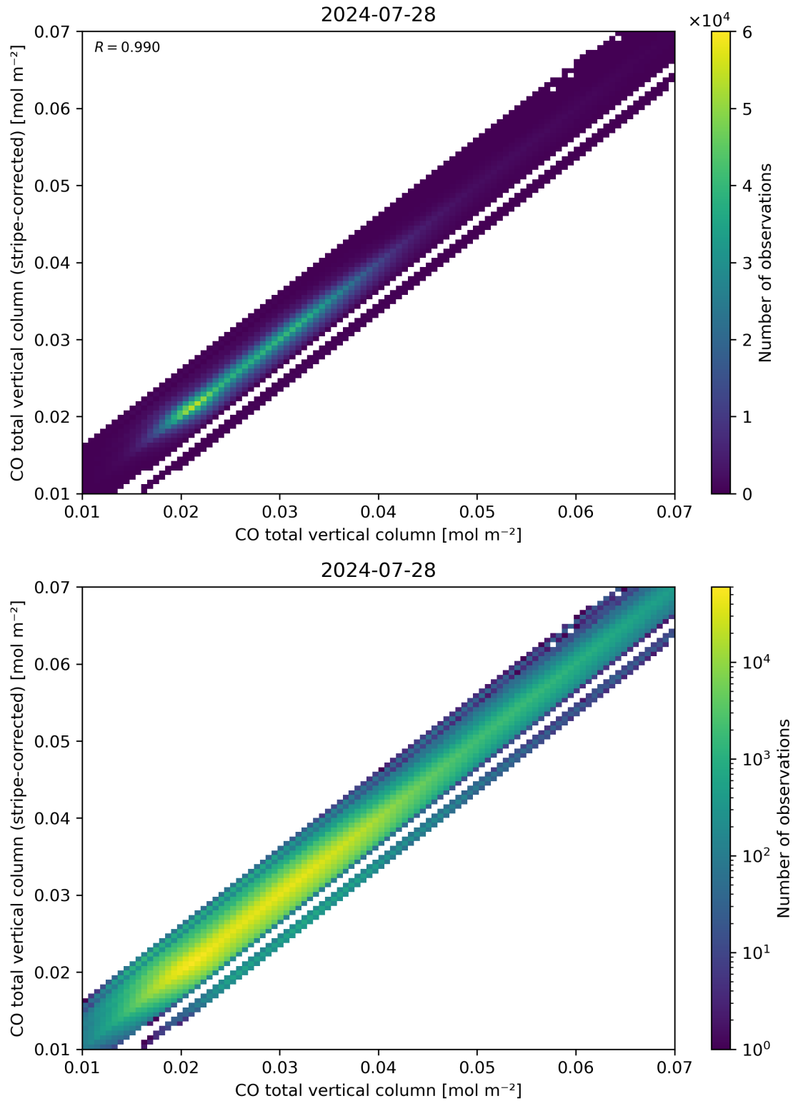
Figure 33: Scatter density plot of “CO total vertical column” against “CO total vertical column (stripe-corrected)” for 2024-07-27 to 2024-07-29.
