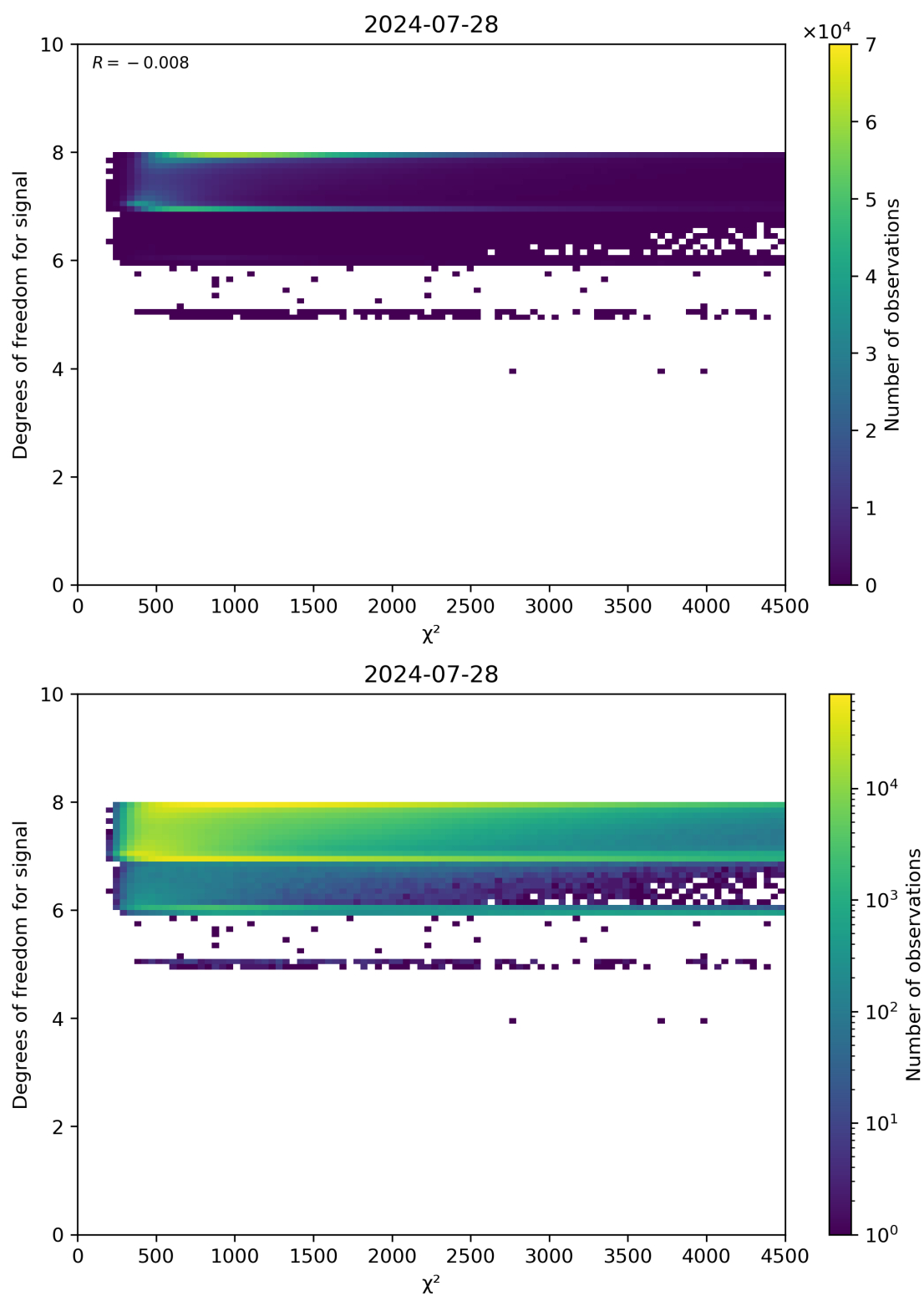
Figure 48: Scatter density plot of “ \chi^2 ” against “Degrees of freedom for signal” for 2024-07-27 to 2024-07-29.
