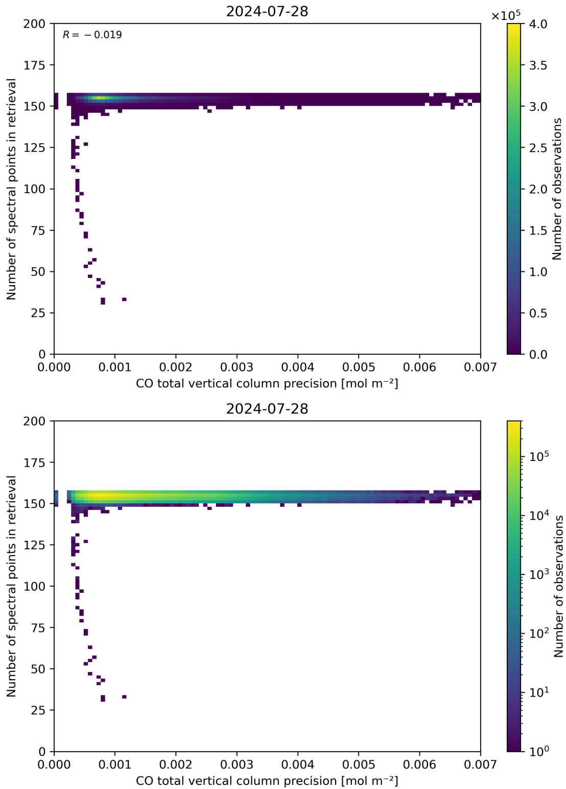
Figure 47: Scatter density plot of “CO total vertical column precision” against “Number of spectral points in retrieval” for 2024-07-27 to 2024-07-29.
