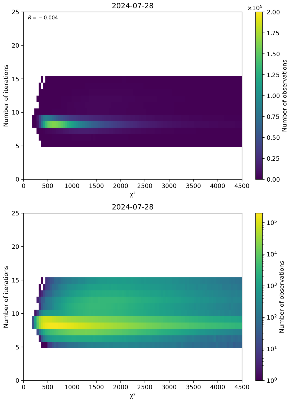
Figure 49: Scatter density plot of “ \chi^2 ” against “Number of iterations” for 2024-07-27 to 2024-07-29.
