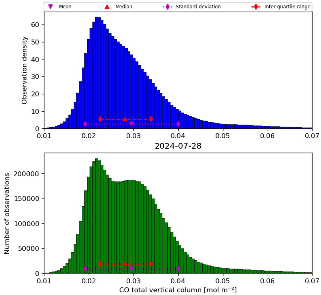
Figure 18: Histogram of “CO total vertical column” for 2024-07-27 to 2024-07-29
