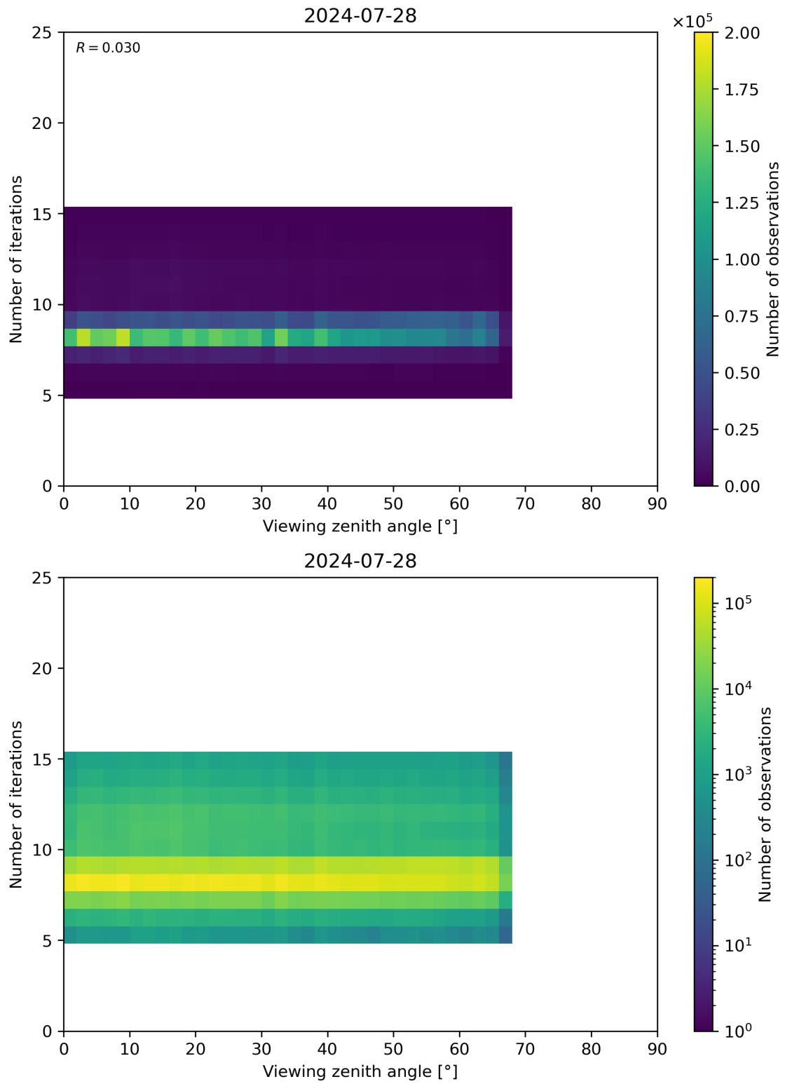
Figure 75: Scatter density plot of “Viewing zenith angle” against “Number of iterations” for 2024-07-27 to 2024-07-29.
