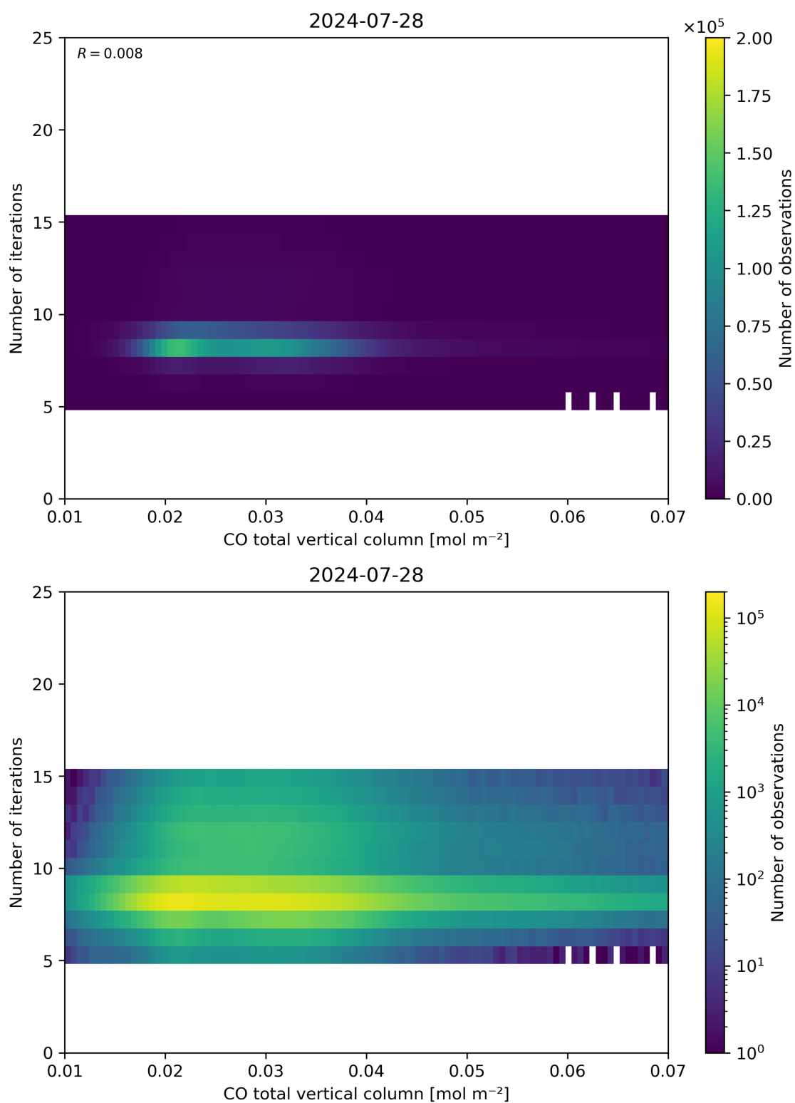
Figure 42: Scatter density plot of “CO total vertical column” against “Number of iterations” for 2024-07-27 to 2024-07-29.
