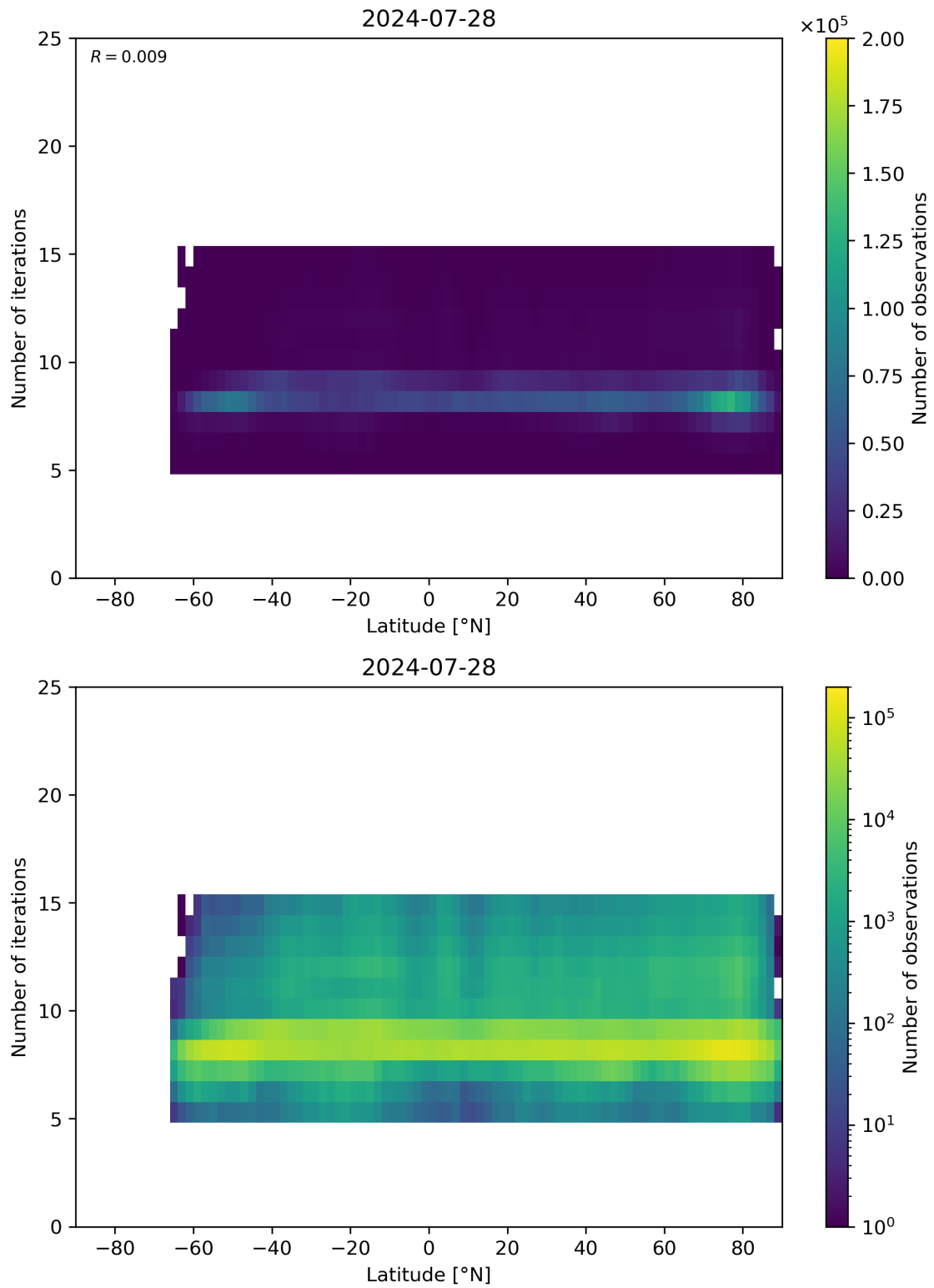
Figure 56: Scatter density plot of “Latitude” against “Number of iterations” for 2024-07-27 to 2024-07-29.
