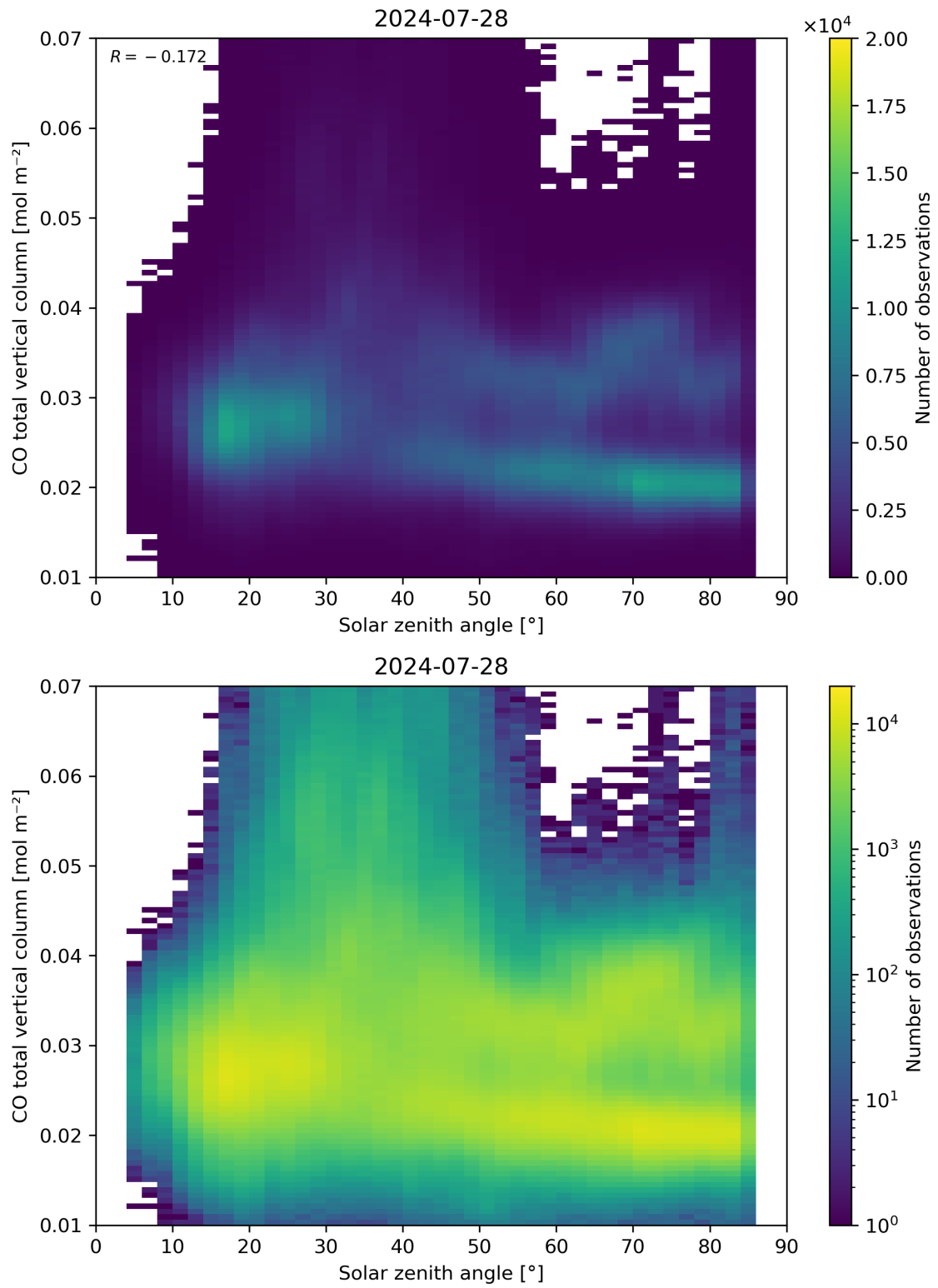
Figure 61: Scatter density plot of “Solar zenith angle” against “CO total vertical column” for 2024-07-27 to 2024-07-29.
