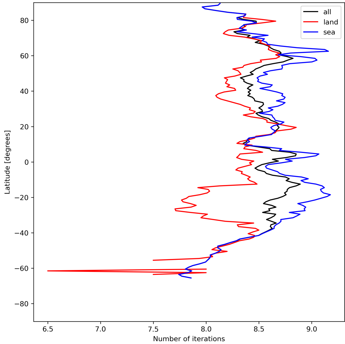
Figure 16: Zonal average of “Number of iterations” for 2024-07-27 to 2024-07-29.
