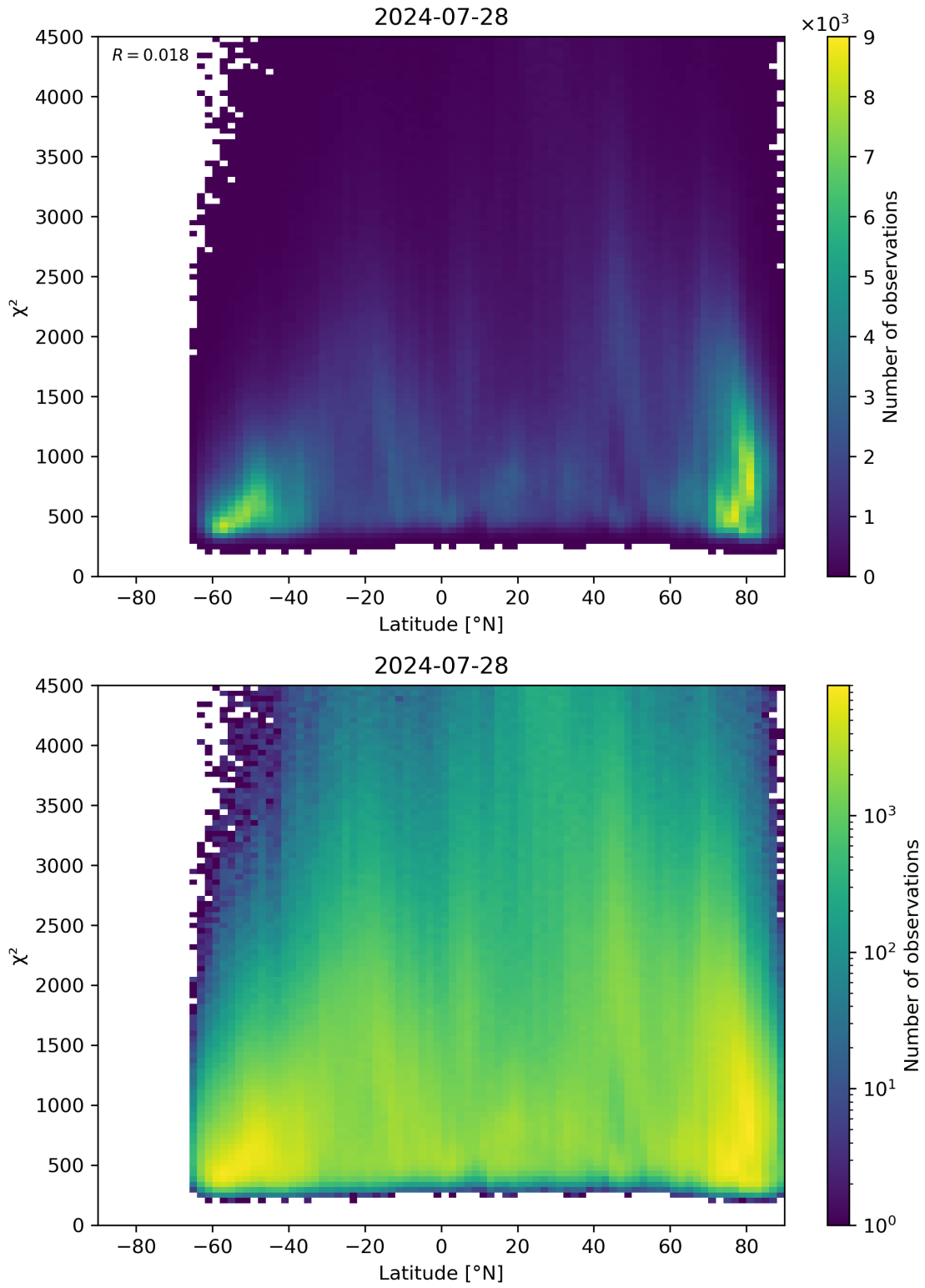
Figure 54: Scatter density plot of “Latitude” against “ \chi^2 ” for 2024-07-27 to 2024-07-29.
