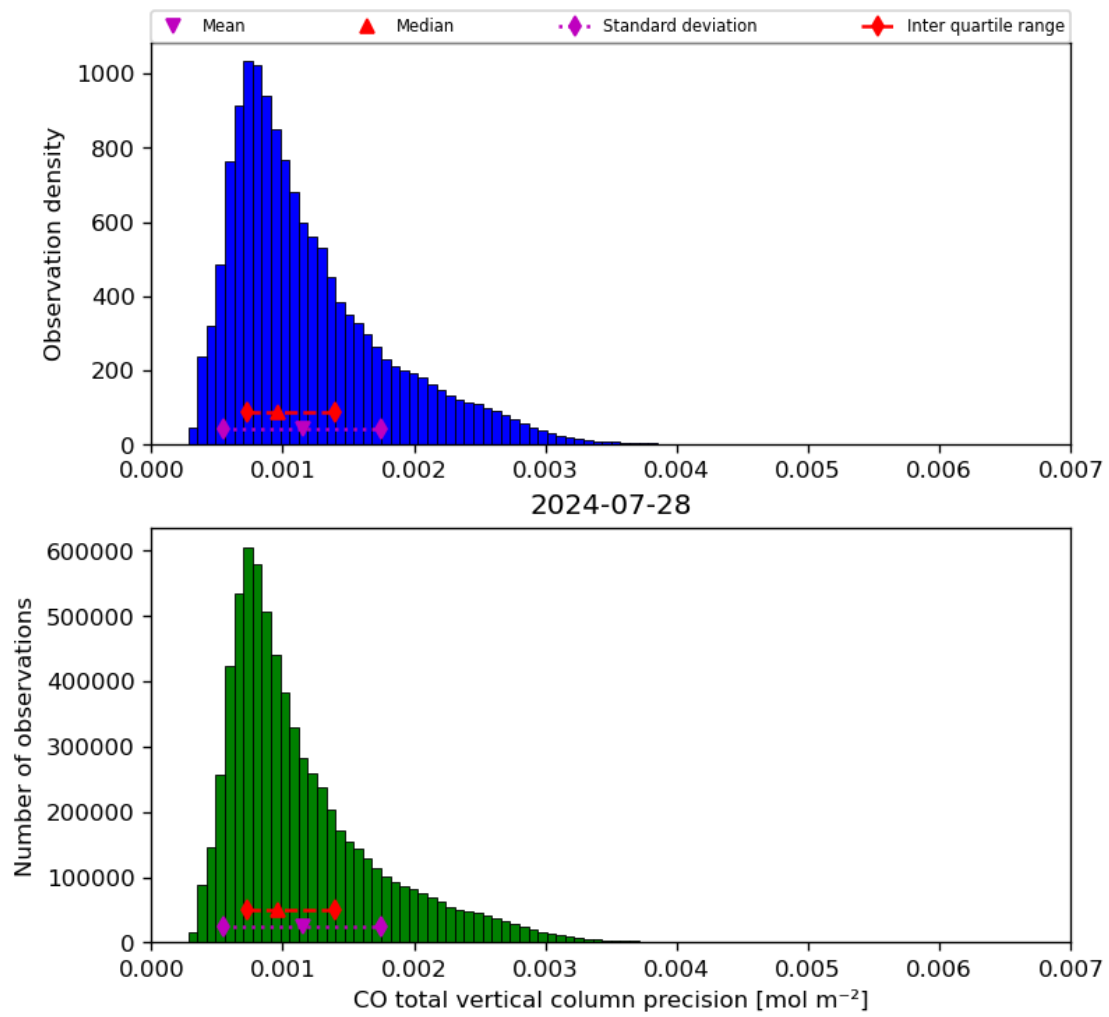
Figure 20: Histogram of “CO total vertical column precision” for 2024-07-27 to 2024-07-29
