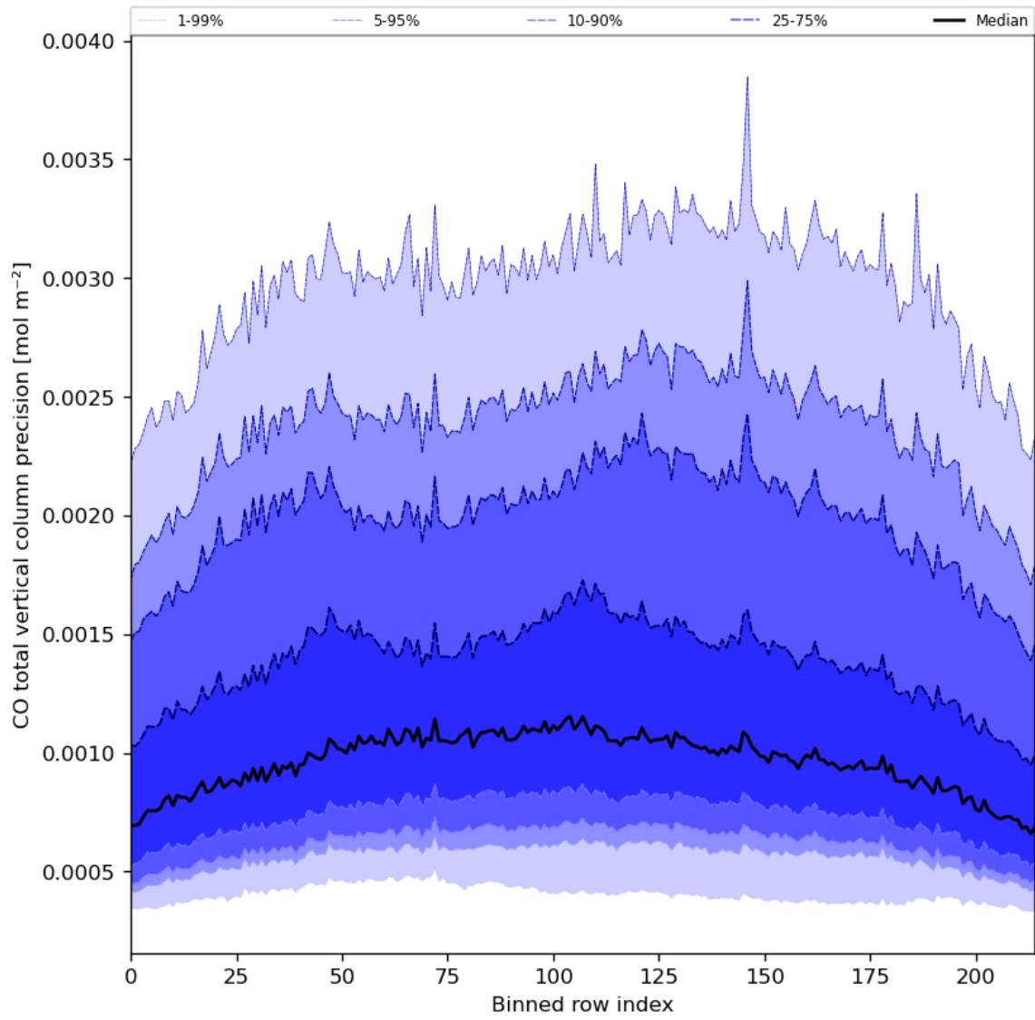
Figure 28: Along track statistics of “CO total vertical column precision” for 2024-07-27 to 2024-07-29
