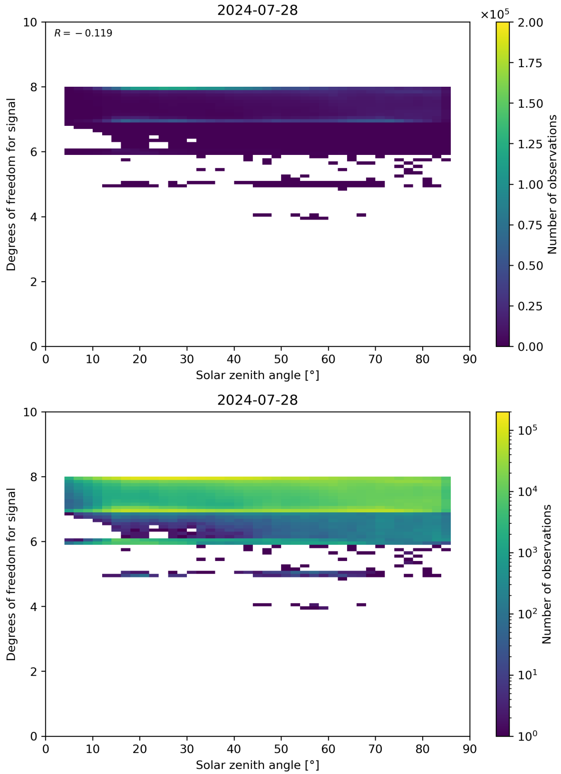
Figure 65: Scatter density plot of “Solar zenith angle” against “Degrees of freedom for signal” for 2024-07-27 to 2024-07-29.
