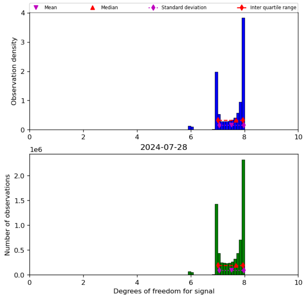
Figure 23: Histogram of “Degrees of freedom for signal” for 2024-07-27 to 2024-07-29
