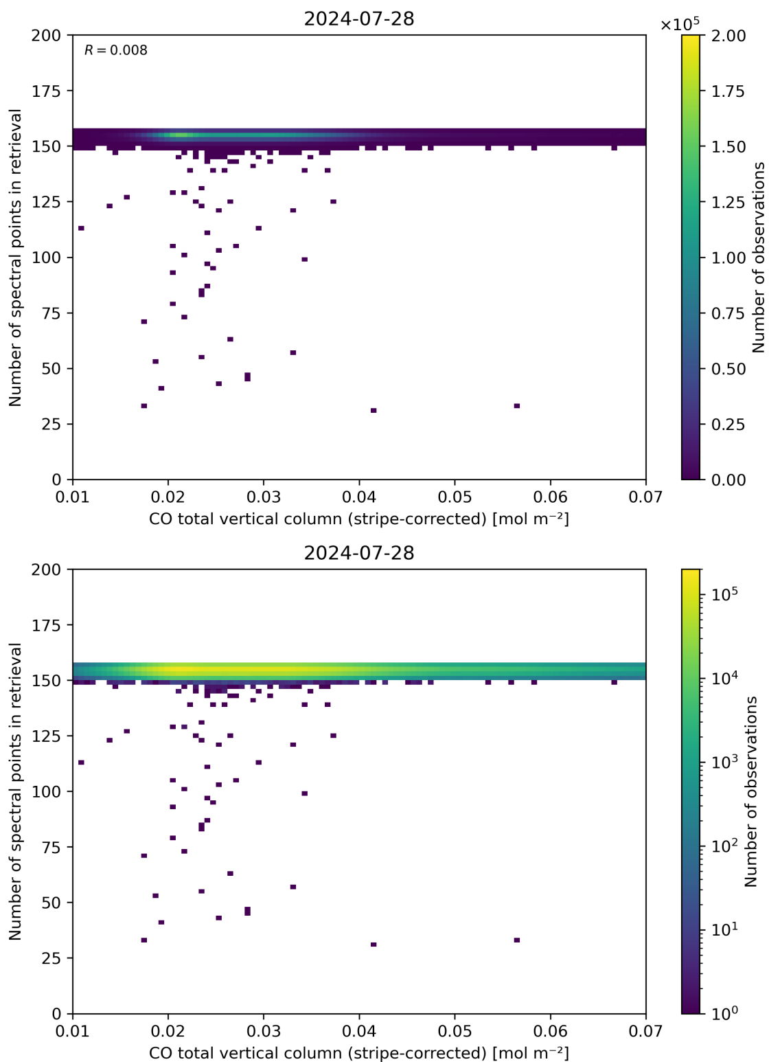
Figure 40: Scatter density plot of “CO total vertical column (stripe-corrected)” against “Number of spectral points in retrieval” for 2024-07-27 to 2024-07-29.
