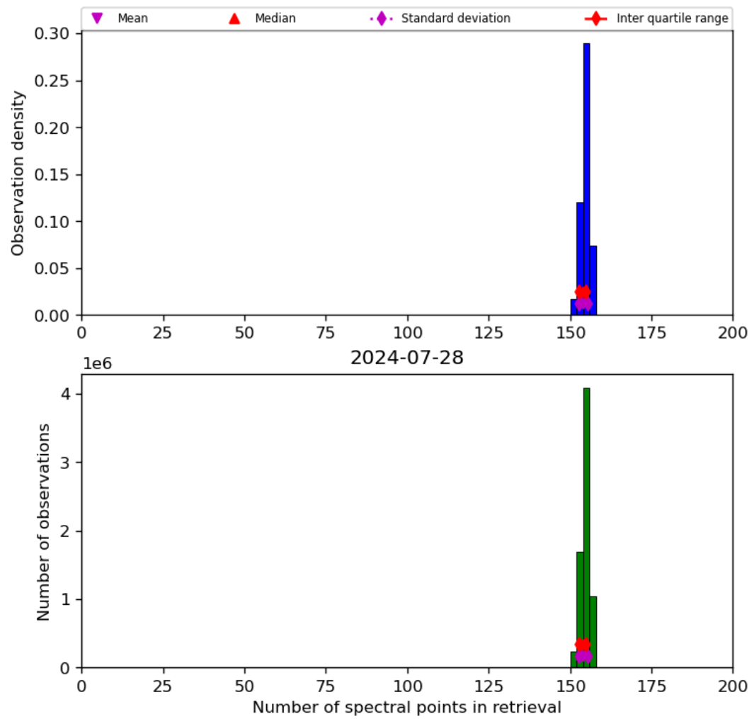
Figure 21: Histogram of “Number of spectral points in retrieval” for 2024-07-27 to 2024-07-29
