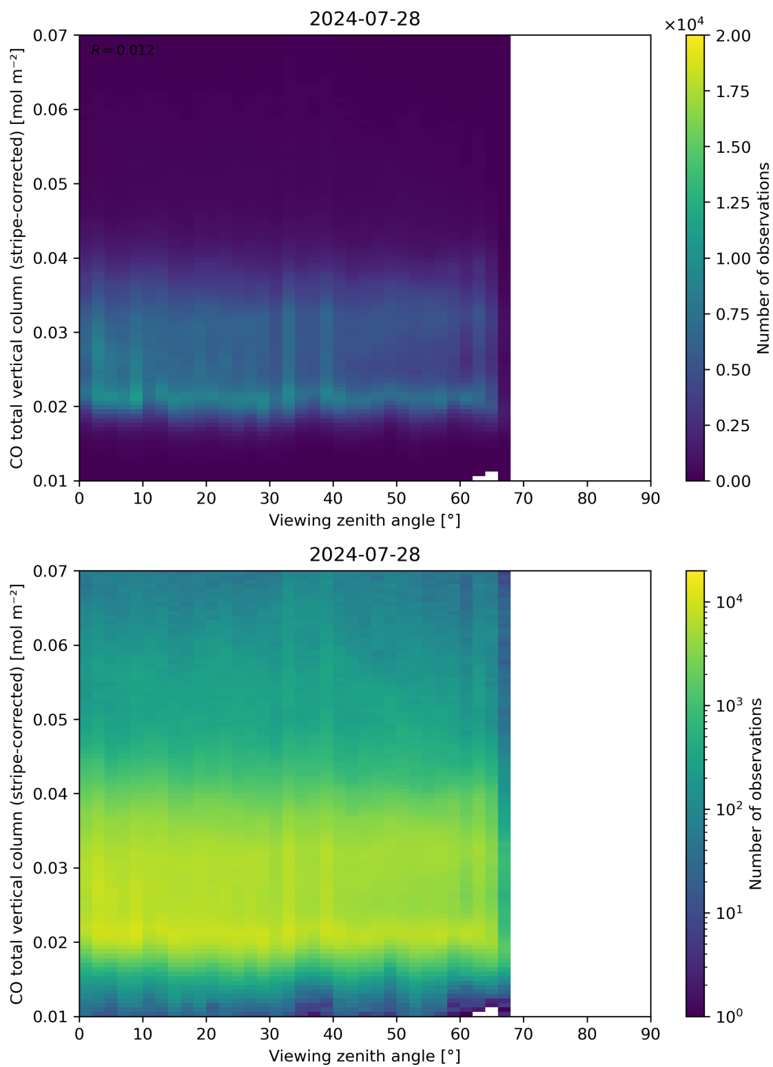
Figure 70: Scatter density plot of “Viewing zenith angle” against “CO total vertical column (stripe-corrected)” for 2024-07-27 to 2024-07-29.
