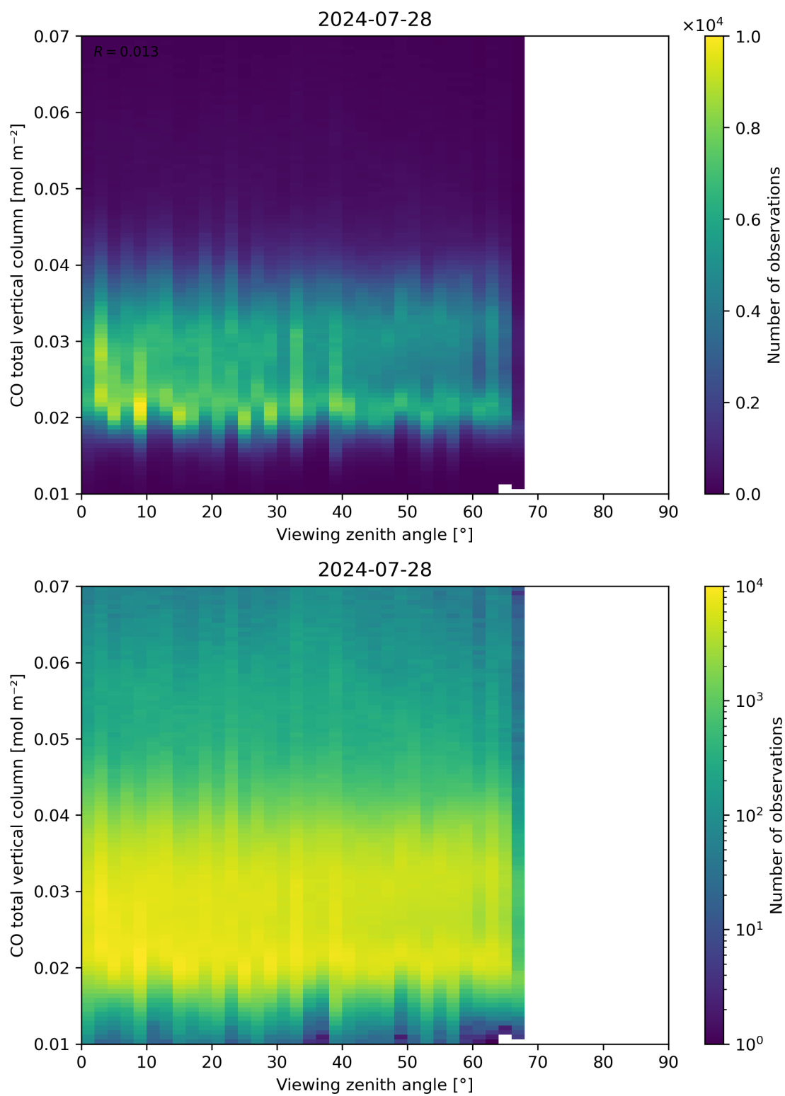
Figure 69: Scatter density plot of “Viewing zenith angle” against “CO total vertical column” for 2024-07-27 to 2024-07-29.
