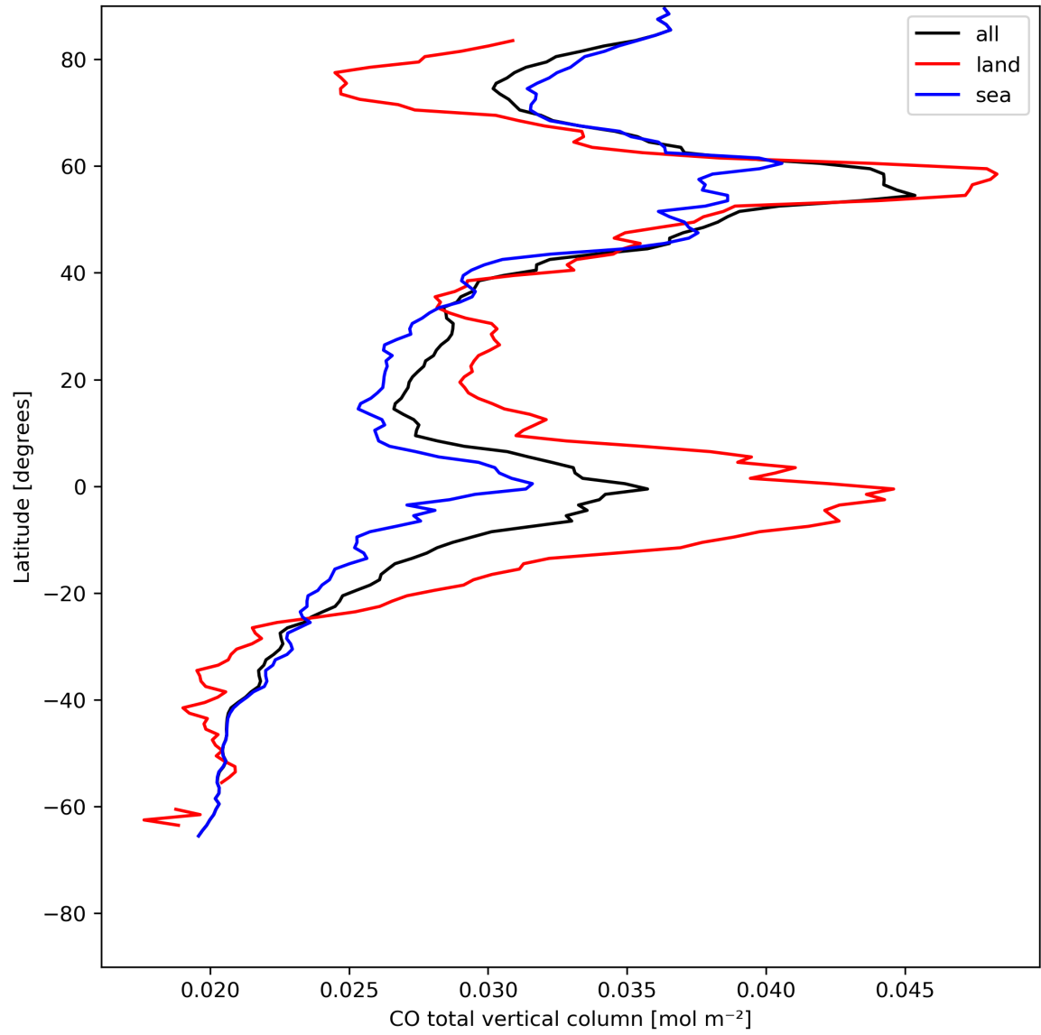
Figure 10: Zonal average of “CO total vertical column” for 2024-07-27 to 2024-07-29.
