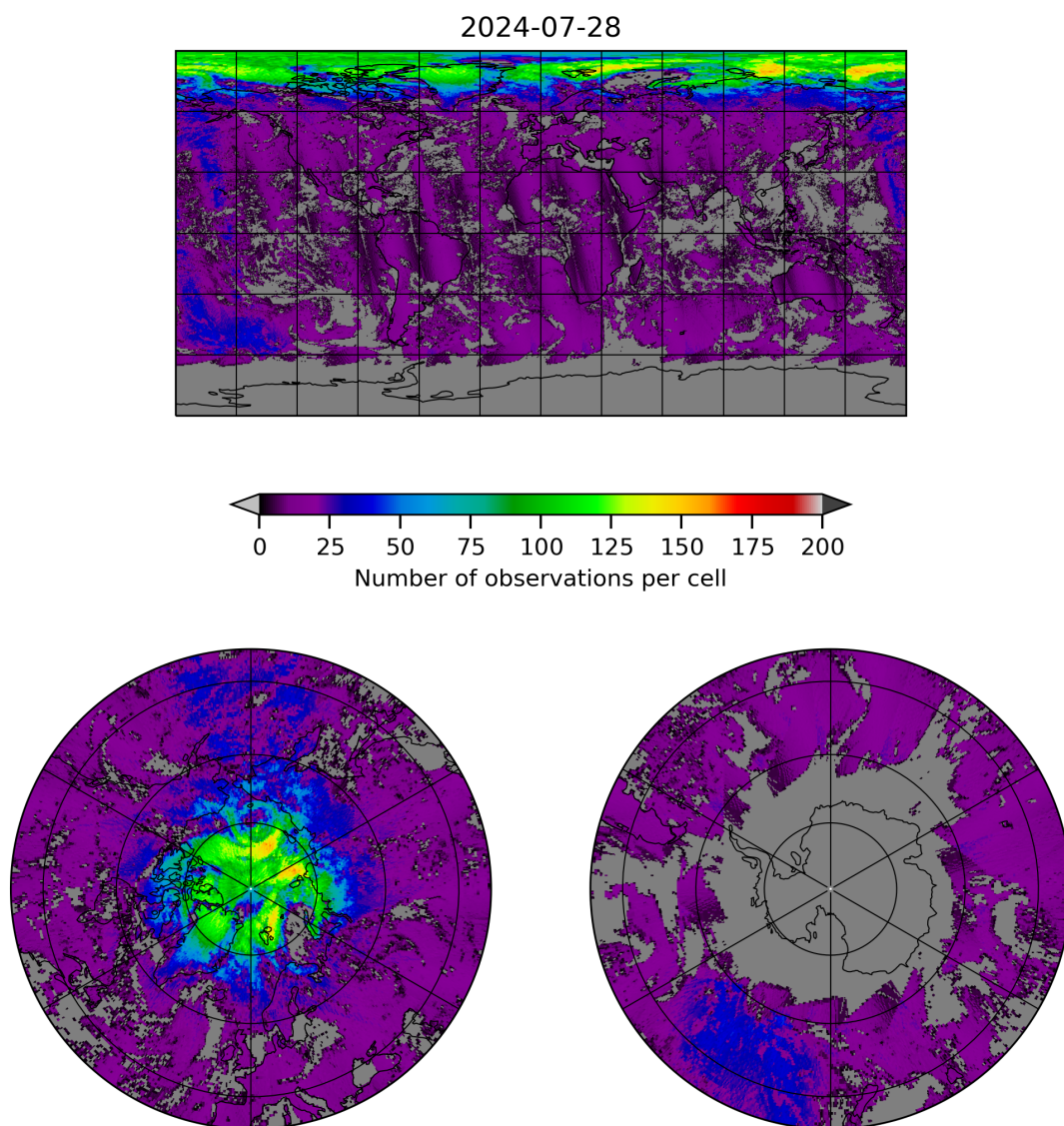
Figure 8: Map of the number of observations for 2024-07-27 to 2024-07-29
