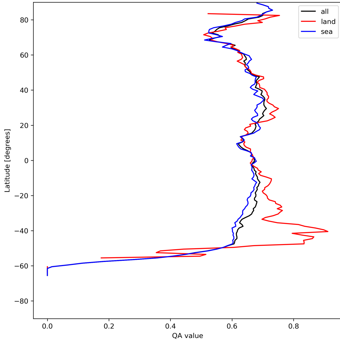
Figure 9: Zonal average of “QA value” for 2024-07-27 to 2024-07-29.
