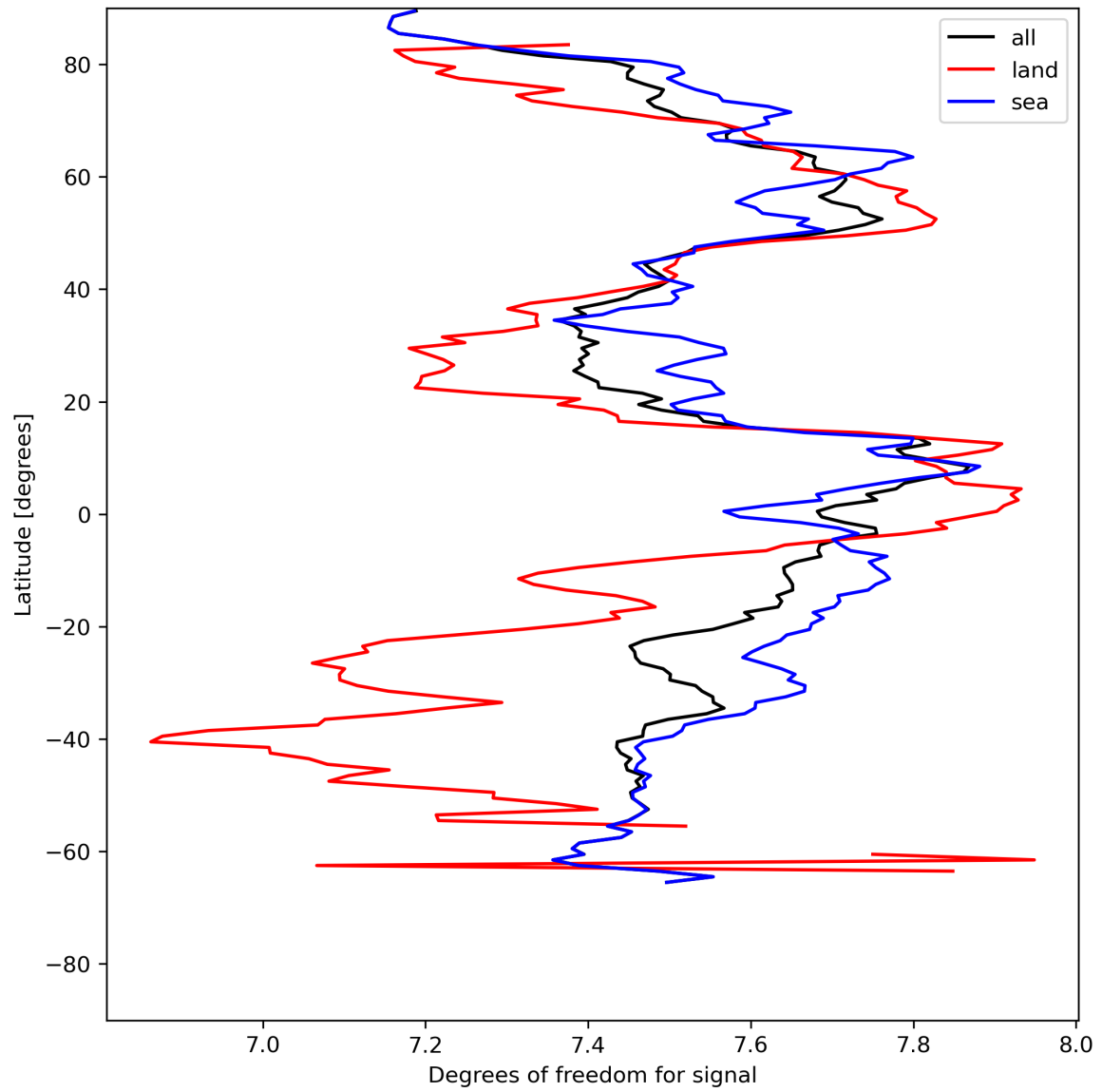
Figure 15: Zonal average of “Degrees of freedom for signal” for 2024-07-27 to 2024-07-29.
