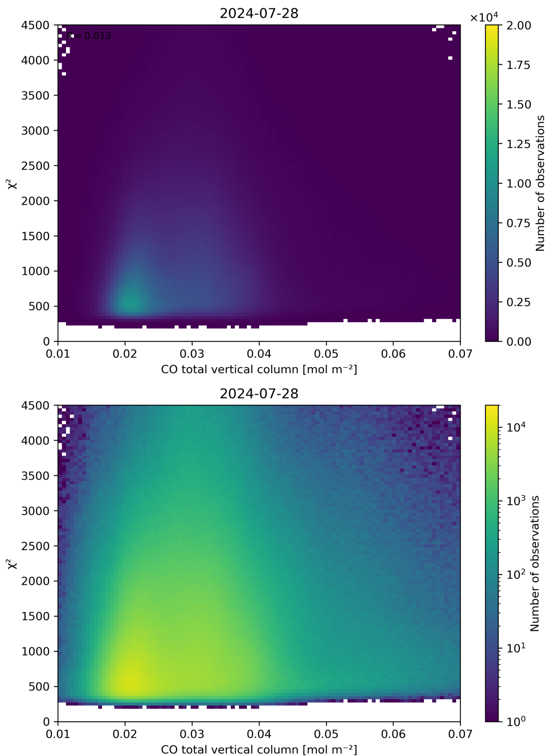
Figure 35: Scatter density plot of “CO total vertical column” against “ \chi^2 ” for 2024-07-27 to 2024-07-29.
