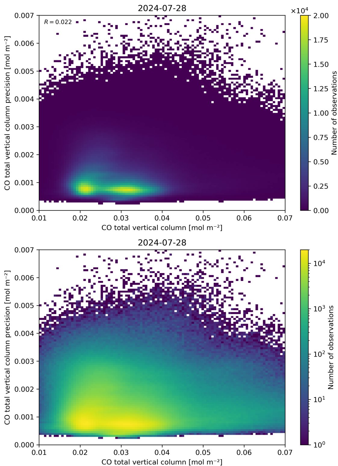
Figure 34: Scatter density plot of “CO total vertical column” against “CO total vertical column precision” for 2024-07-27 to 2024-07-29.
