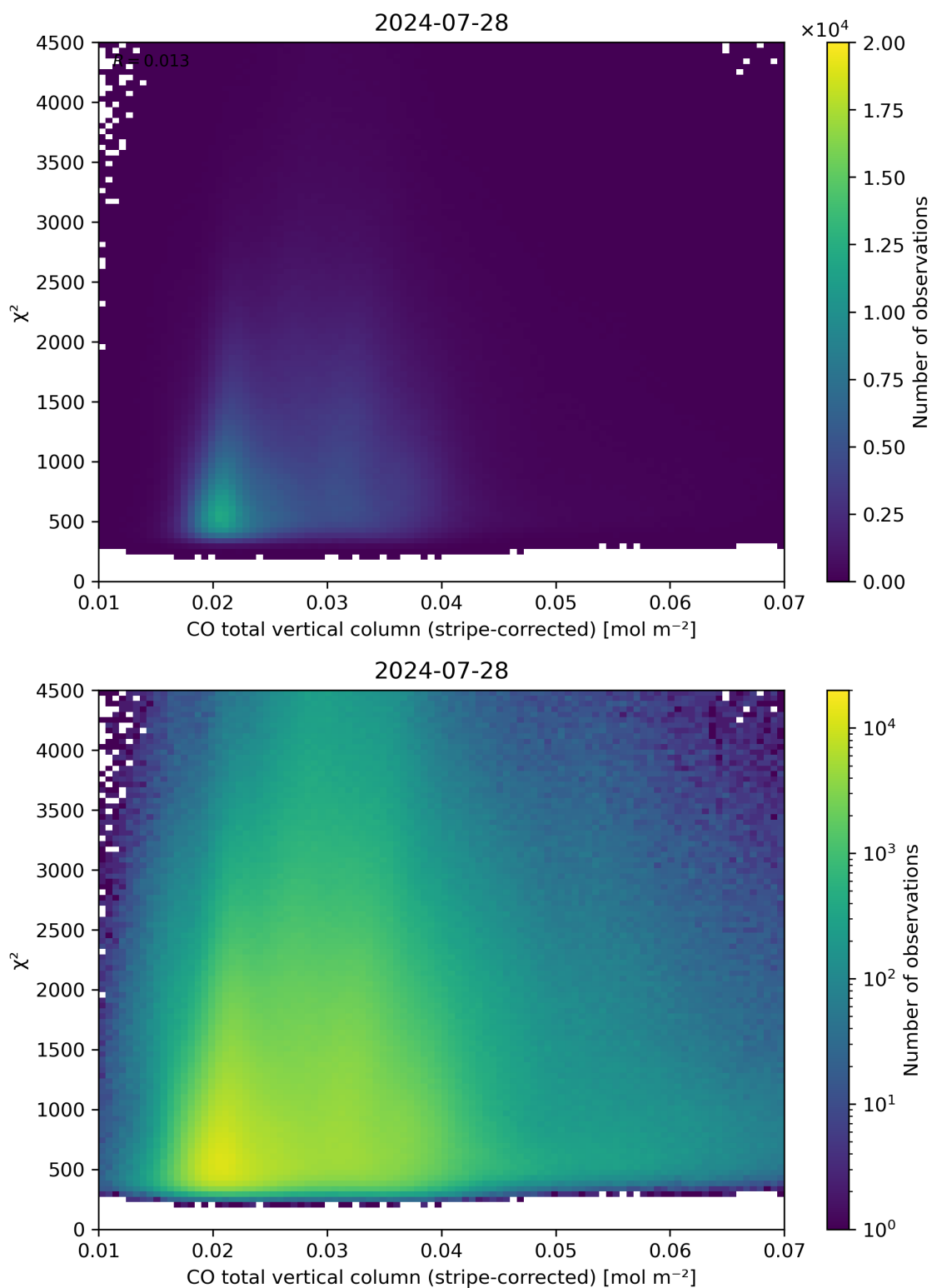
Figure 37: Scatter density plot of “CO total vertical column (stripe-corrected)” against “ \chi^2 ” for 2024-07-27 to 2024-07-29.
