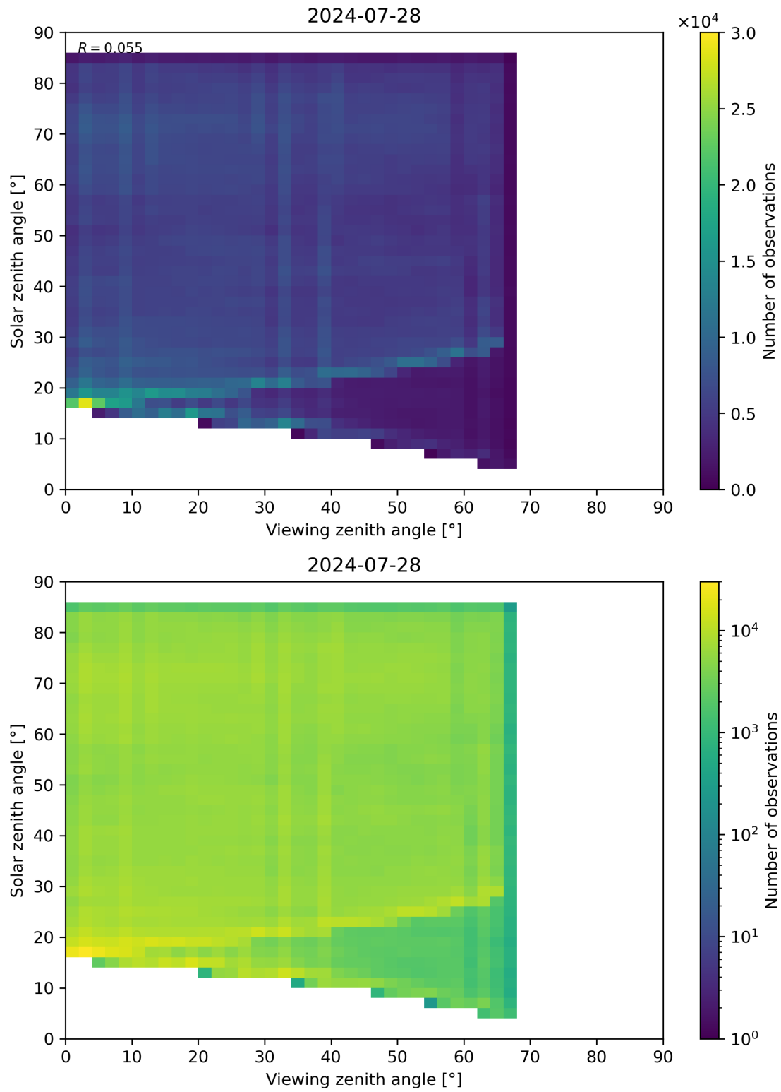
Figure 77: Scatter density plot of “Viewing zenith angle” against “Solar zenith angle” for 2024-07-27 to 2024-07-29.
