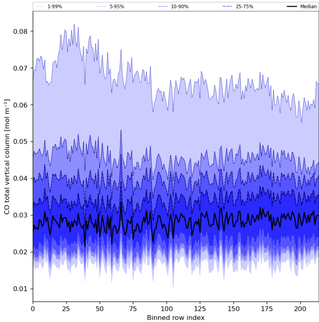
Figure 26: Along track statistics of “CO total vertical column” for 2024-07-27 to 2024-07-29
