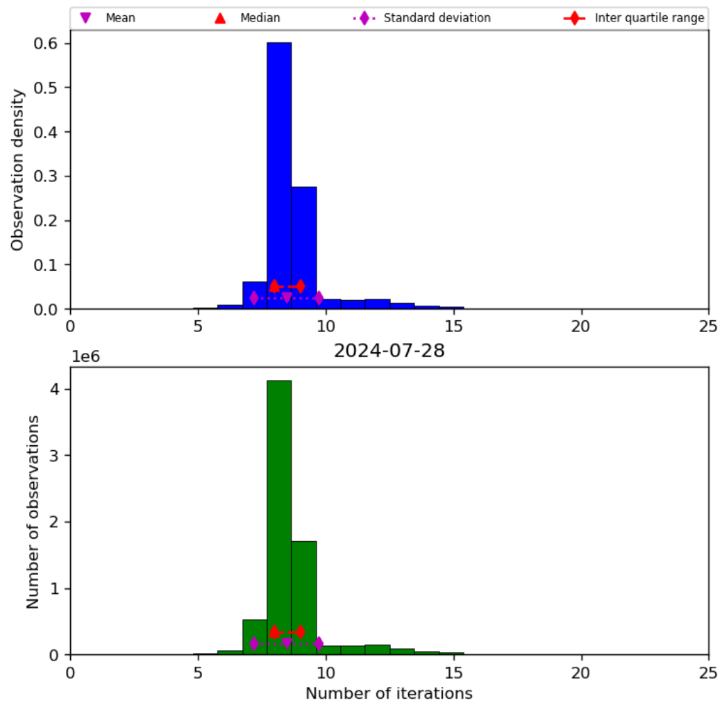
Figure 24: Histogram of “Number of iterations” for 2024-07-27 to 2024-07-29
