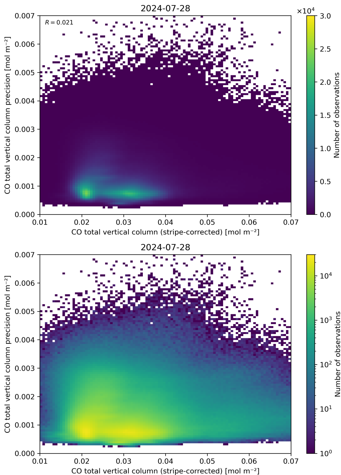
Figure 36: Scatter density plot of “CO total vertical column (stripe-corrected)” against “CO total vertical column precision” for 2024-07-27 to 2024-07-29.
