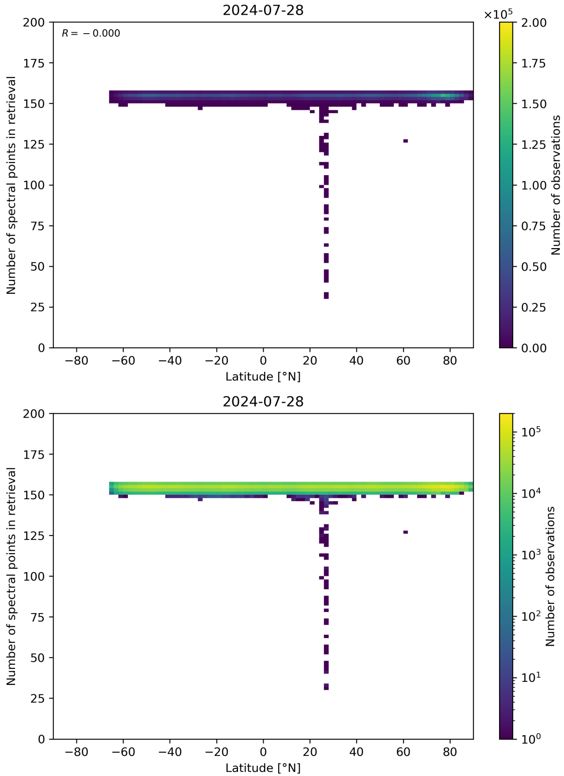
Figure 57: Scatter density plot of “Latitude” against “Number of spectral points in retrieval” for 2024-07-27 to 2024-07-29.
