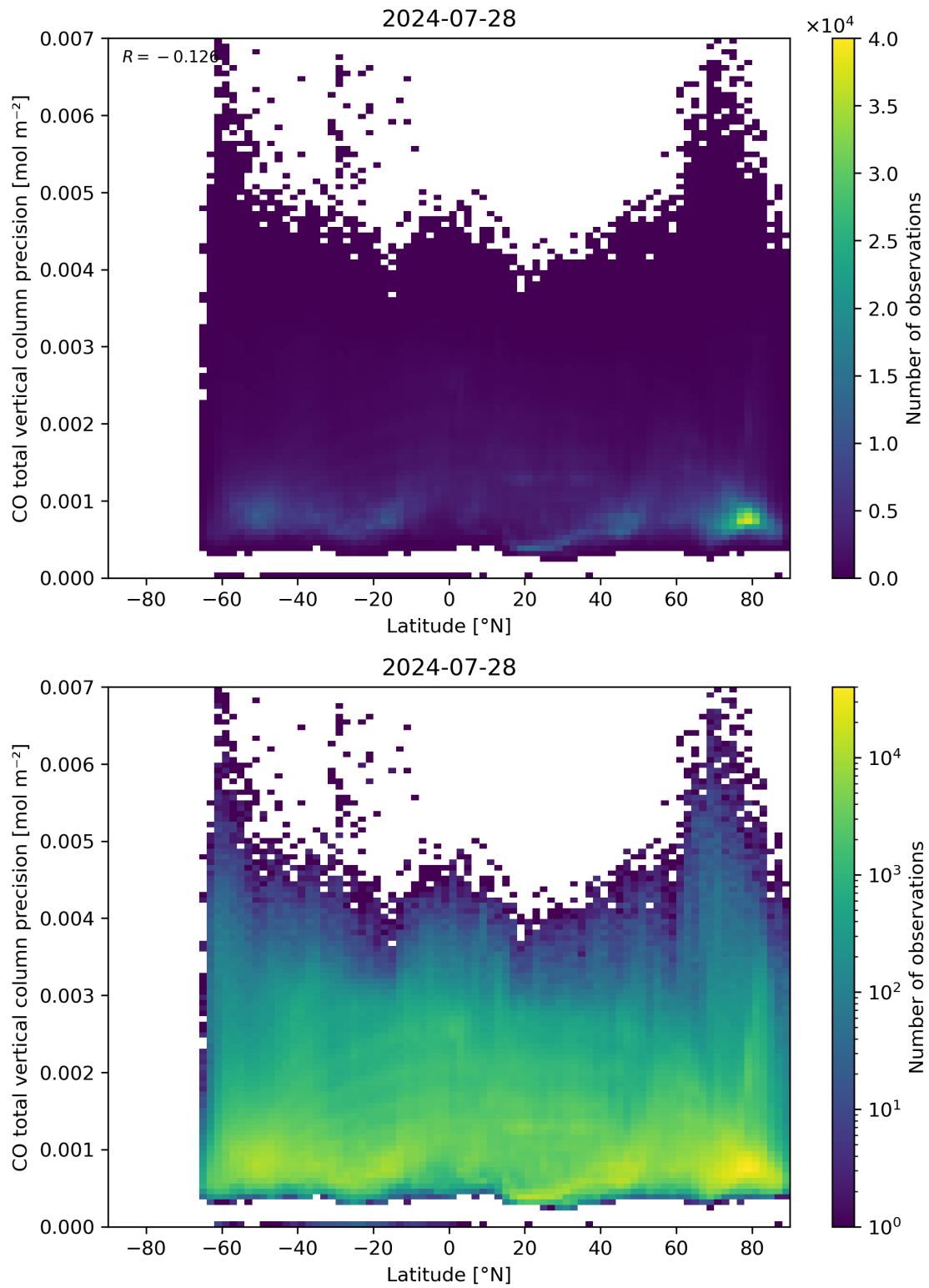
Figure 53: Scatter density plot of “Latitude” against “CO total vertical column precision” for 2024-07-27 to 2024-07-29.
