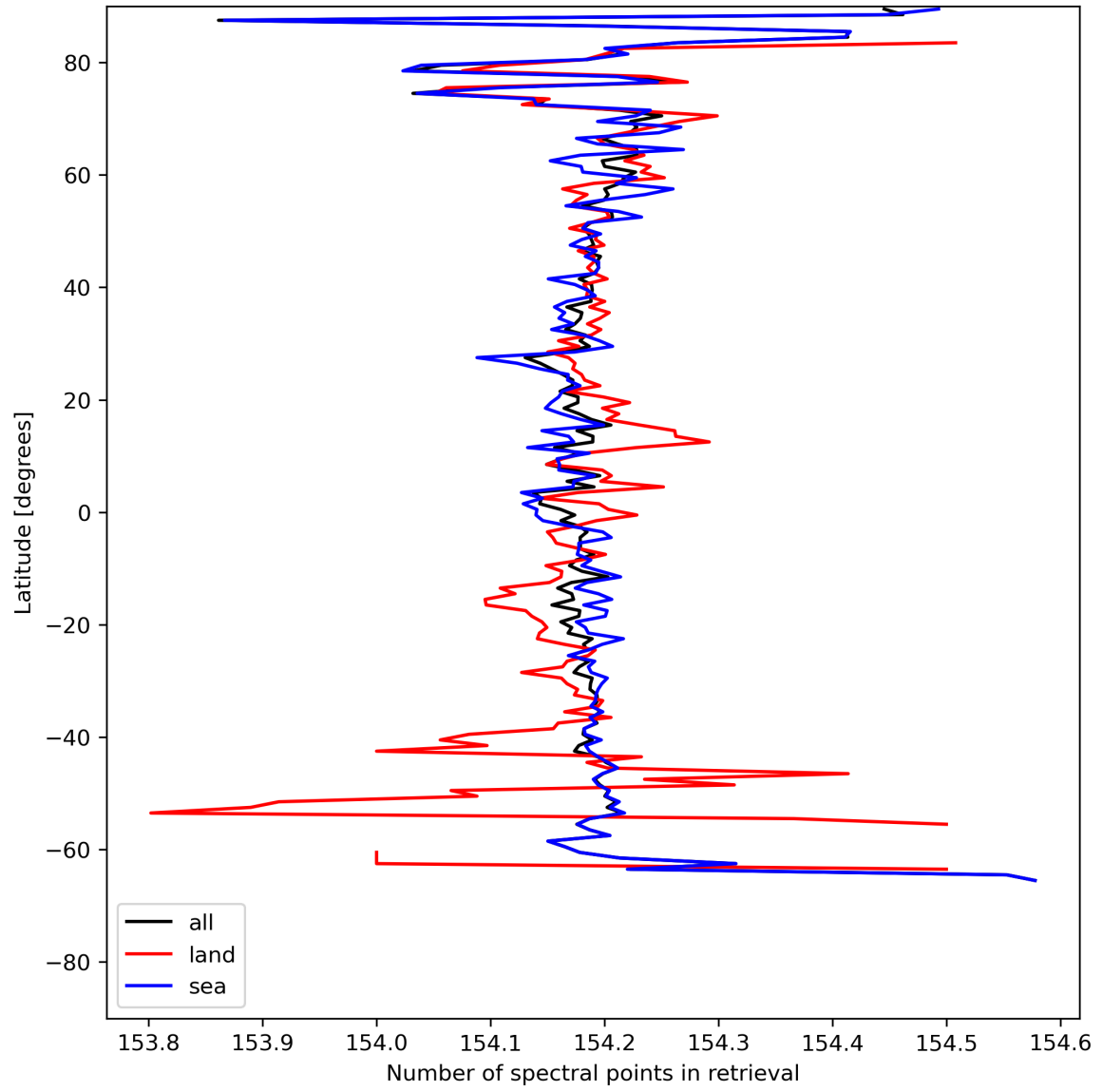
Figure 13: Zonal average of “Number of spectral points in retrieval” for 2024-07-27 to 2024-07-29.
