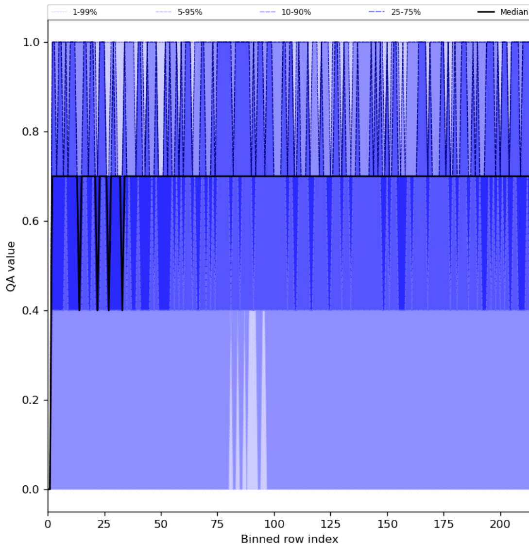
Figure 25: Along track statistics of “QA value” for 2024-07-27 to 2024-07-29
