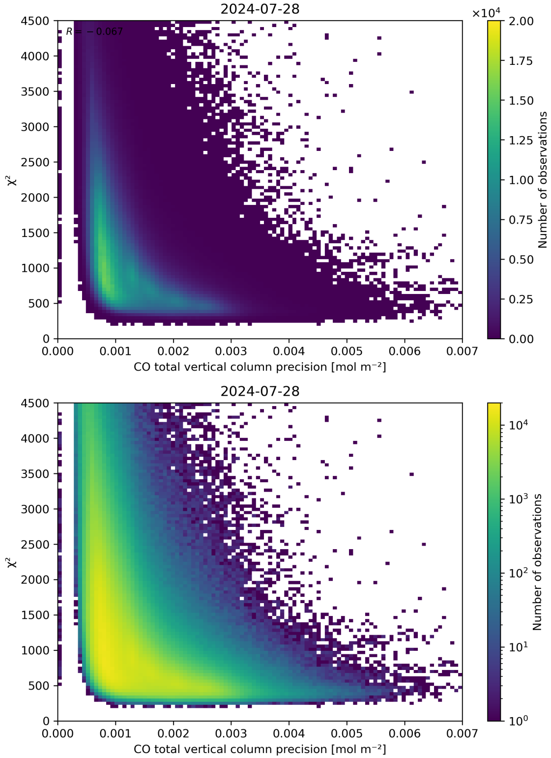
Figure 44: Scatter density plot of “CO total vertical column precision” against “ \chi^2 ” for 2024-07-27 to 2024-07-29.
