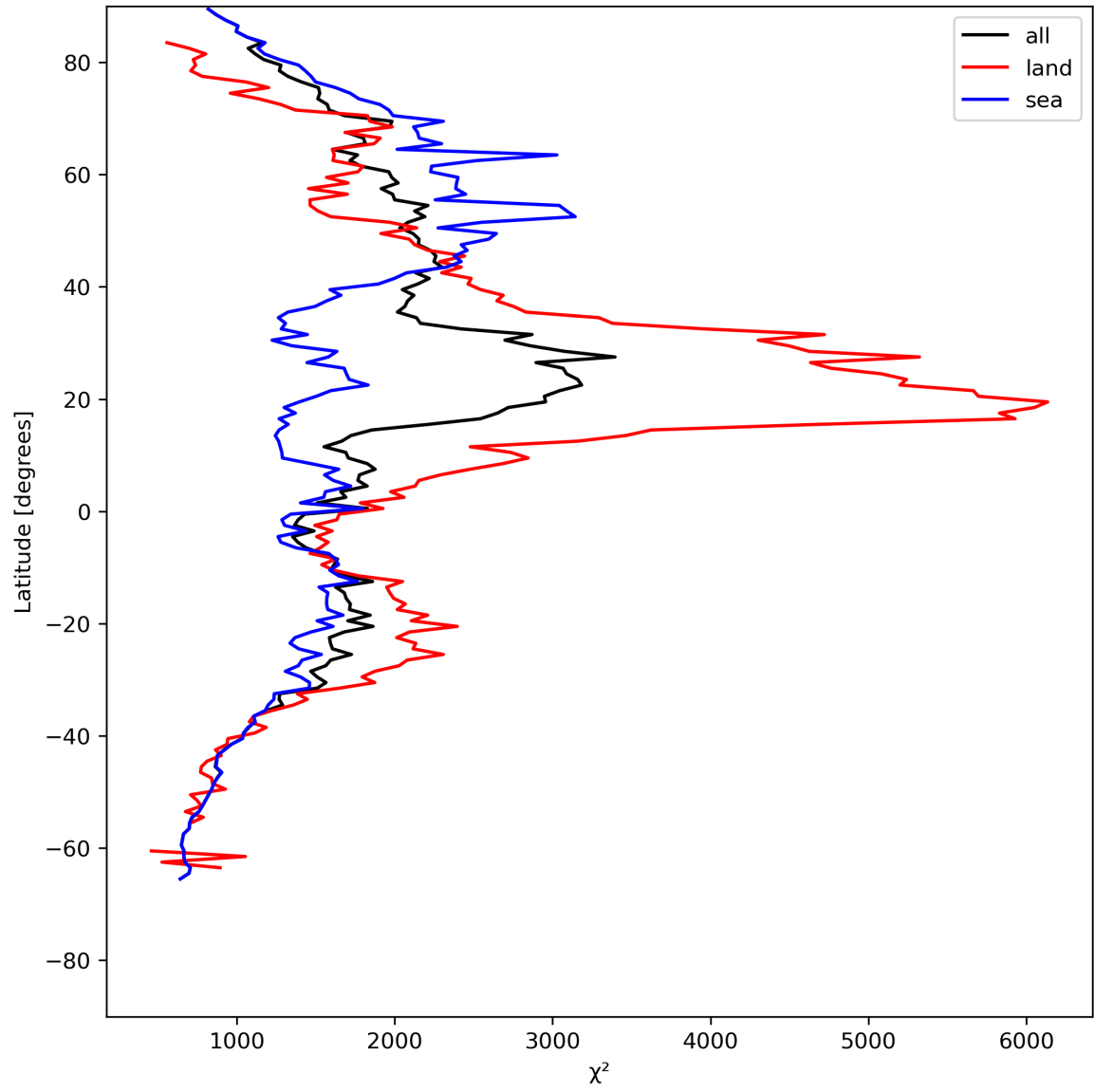
Figure 14: Zonal average of “ \chi^2 ” for 2024-07-27 to 2024-07-29.
