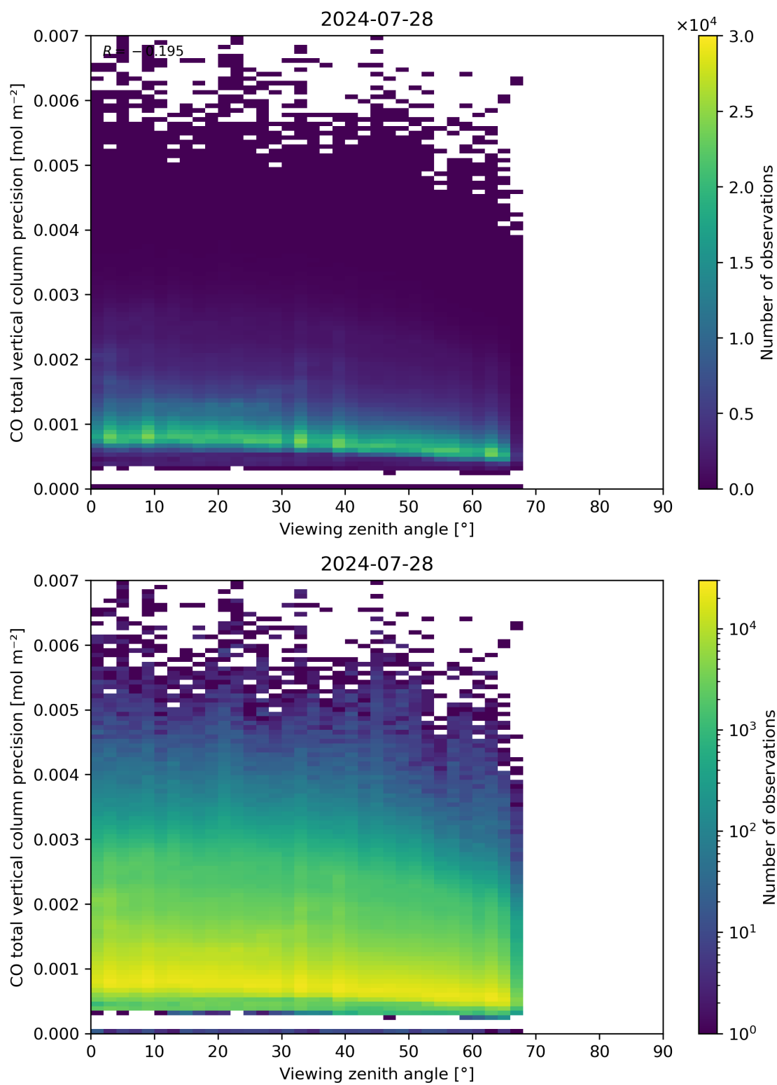
Figure 71: Scatter density plot of “Viewing zenith angle” against “CO total vertical column precision” for 2024-07-27 to 2024-07-29.
