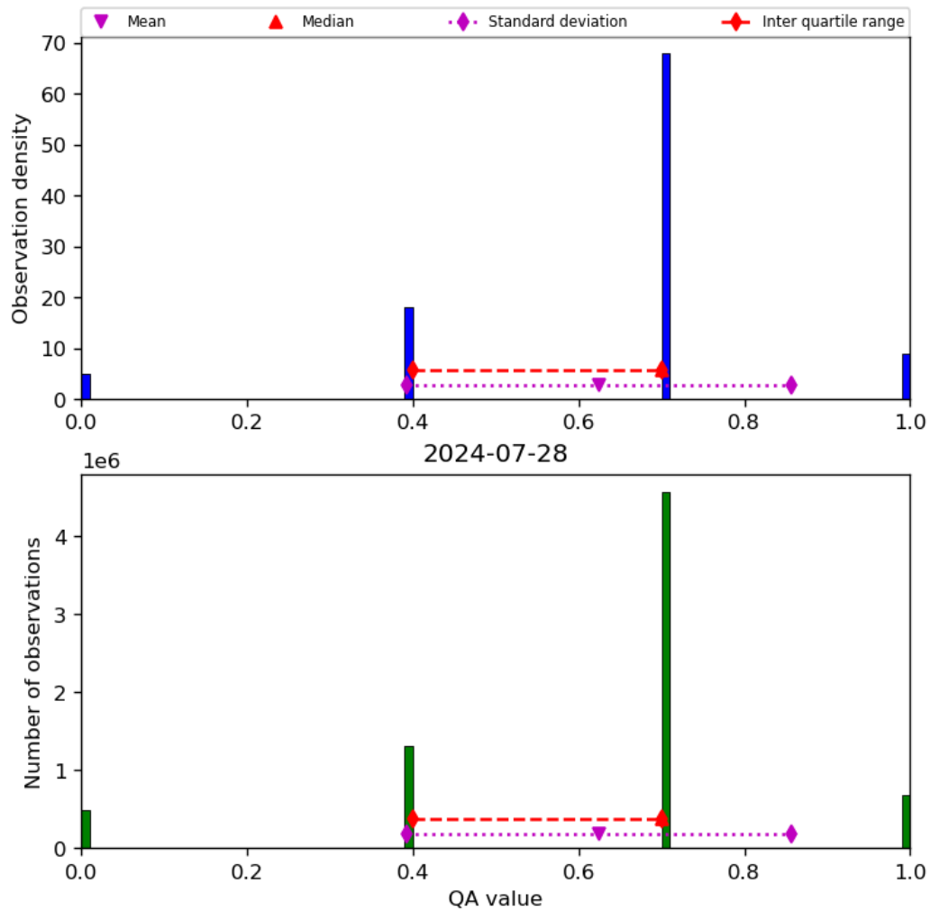
Figure 17: Histogram of “QA value” for 2024-07-27 to 2024-07-29
