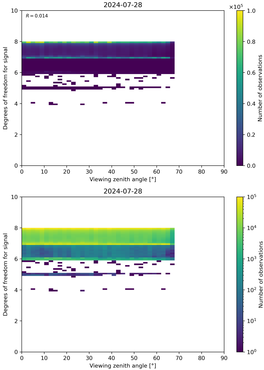
Figure 73: Scatter density plot of “Viewing zenith angle” against “Degrees of freedom for signal” for 2024-07-27 to 2024-07-29.
