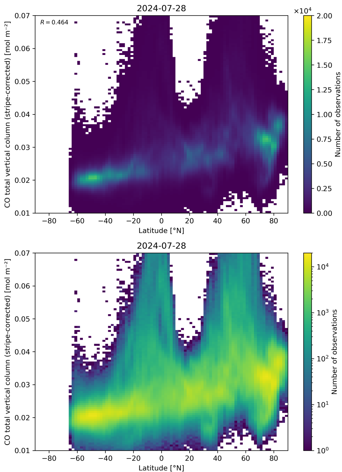
Figure 52: Scatter density plot of “Latitude” against “CO total vertical column (stripe-corrected)” for 2024-07-27 to 2024-07-29.
