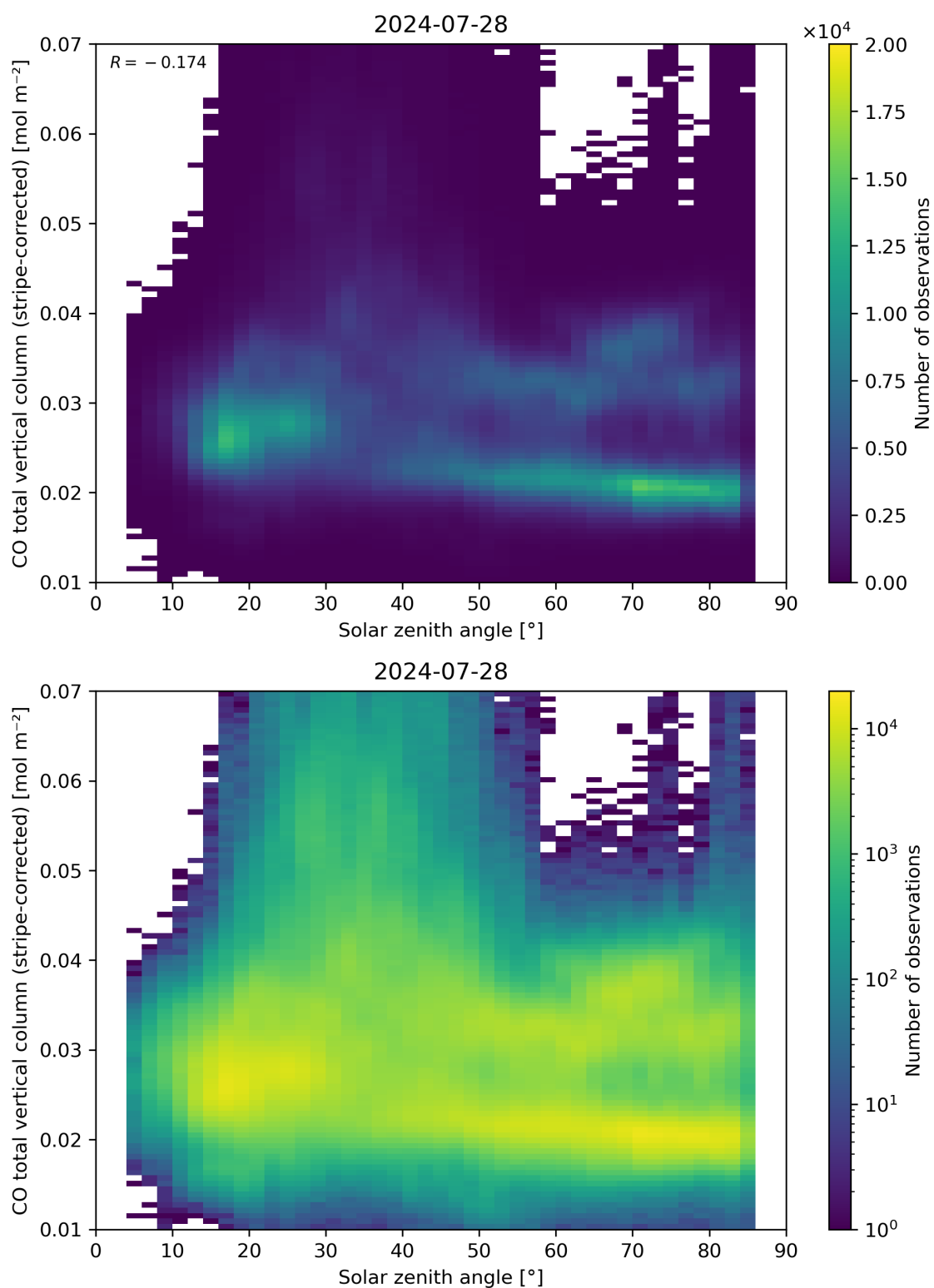
Figure 62: Scatter density plot of “Solar zenith angle” against “CO total vertical column (stripe-corrected)” for 2024-07-27 to 2024-07-29.
