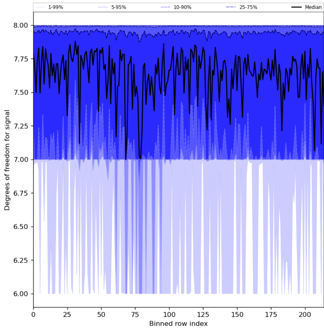
Figure 31: Along track statistics of “Degrees of freedom for signal” for 2024-07-27 to 2024-07-29
