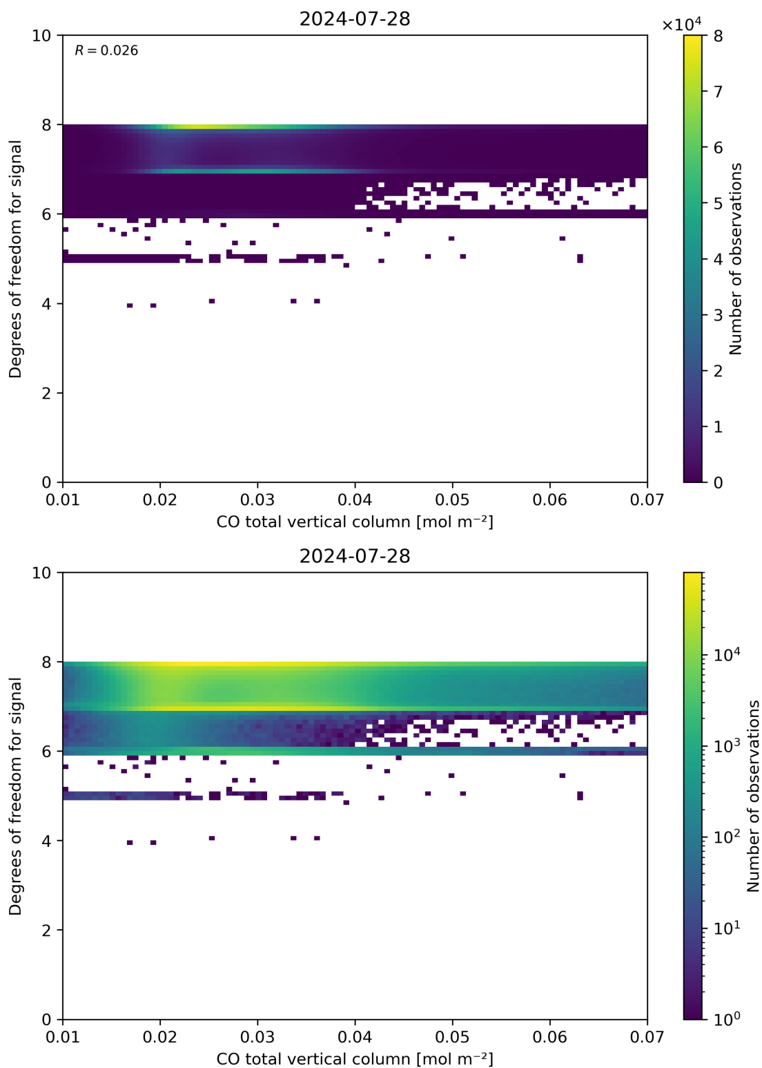
Figure 41: Scatter density plot of “CO total vertical column” against “Degrees of freedom for signal” for 2024-07-27 to 2024-07-29.
