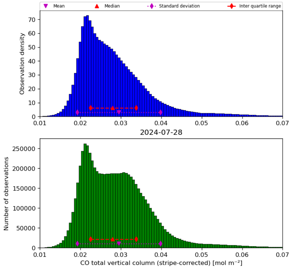
Figure 19: Histogram of “CO total vertical column (stripe-corrected)” for 2024-07-27 to 2024-07-29
