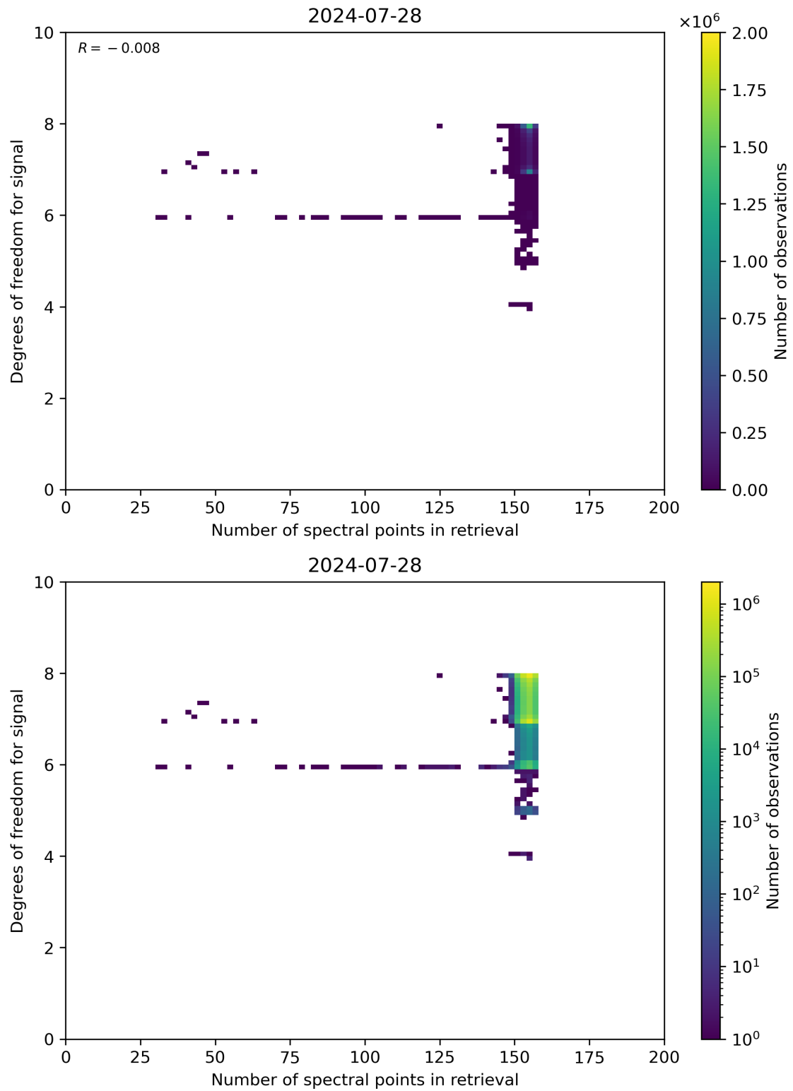
Figure 59: Scatter density plot of “Number of spectral points in retrieval” against “Degrees of freedom for signal” for 2024-07-27 to 2024-07-29.
