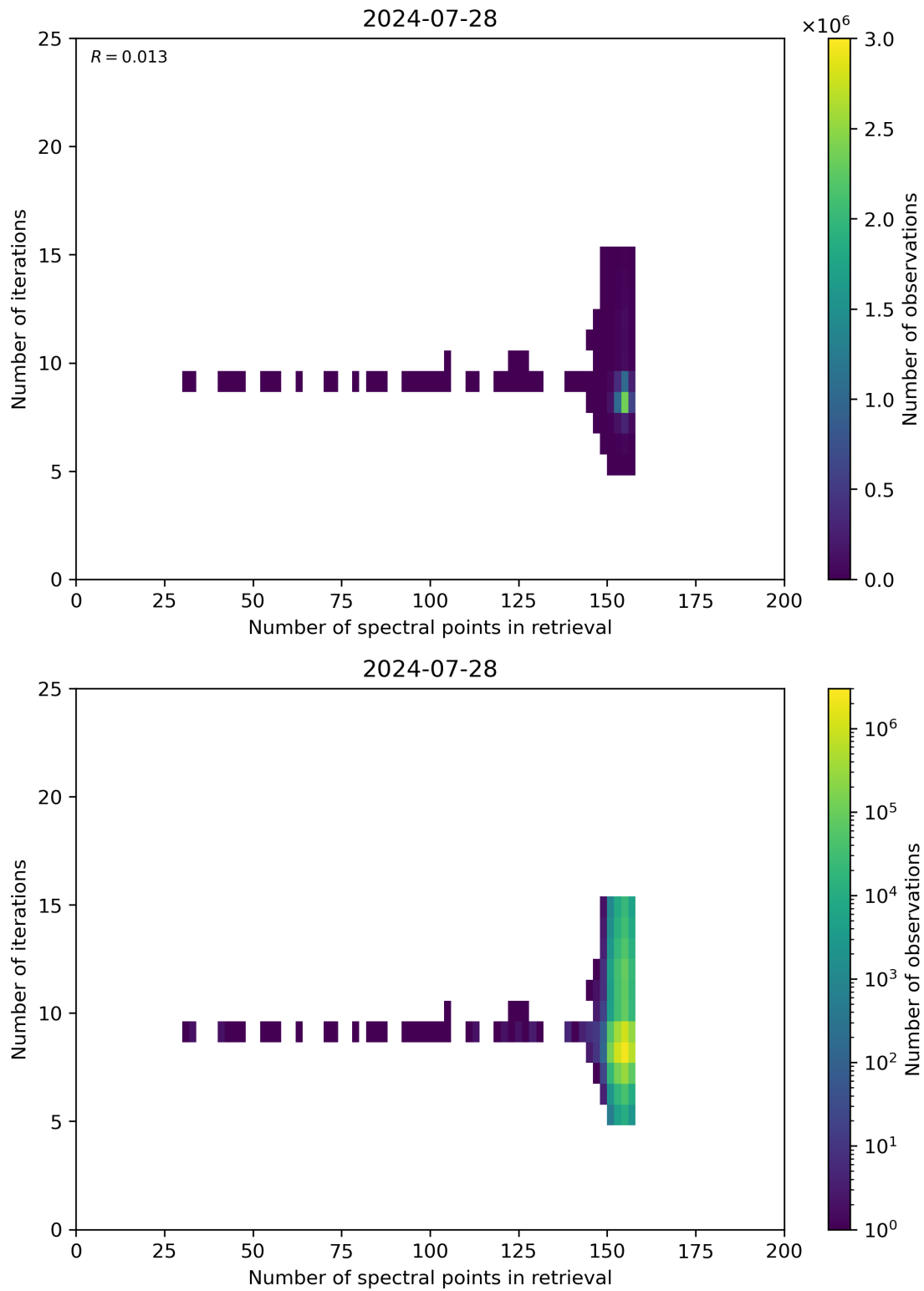
Figure 60: Scatter density plot of “Number of spectral points in retrieval” against “Number of iterations” for 2024-07-27 to 2024-07-29.
