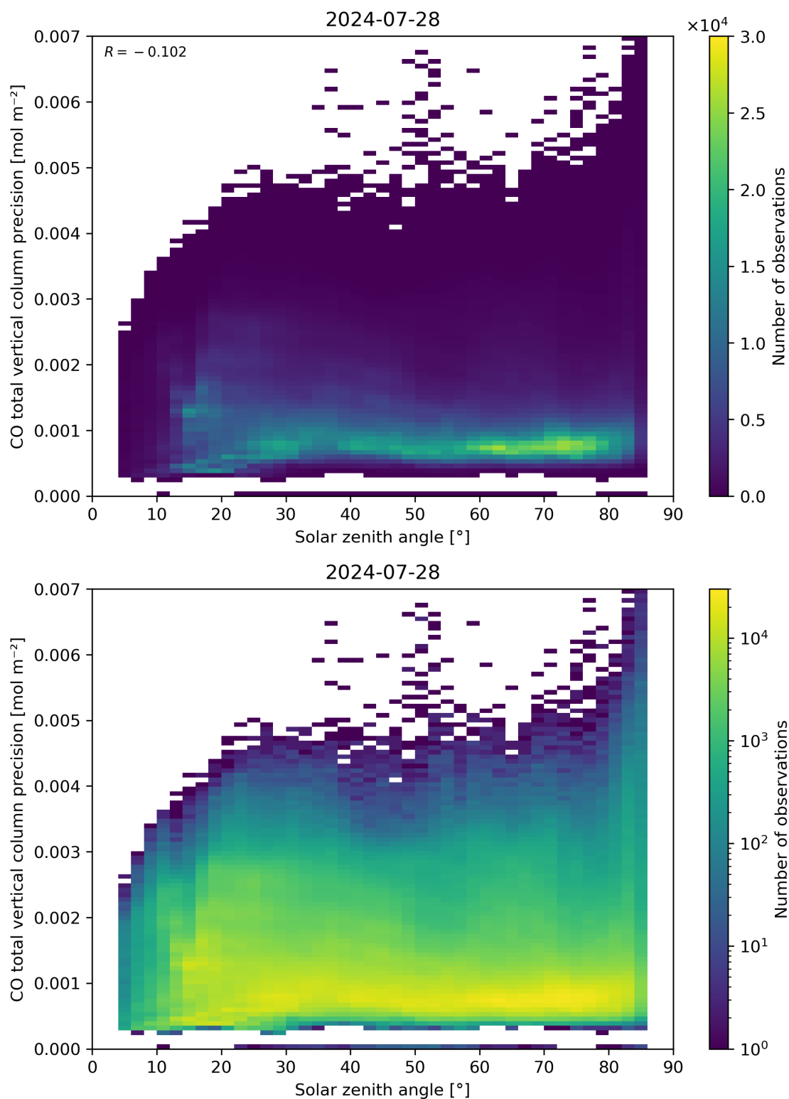
Figure 63: Scatter density plot of “Solar zenith angle” against “CO total vertical column precision” for 2024-07-27 to 2024-07-29.
