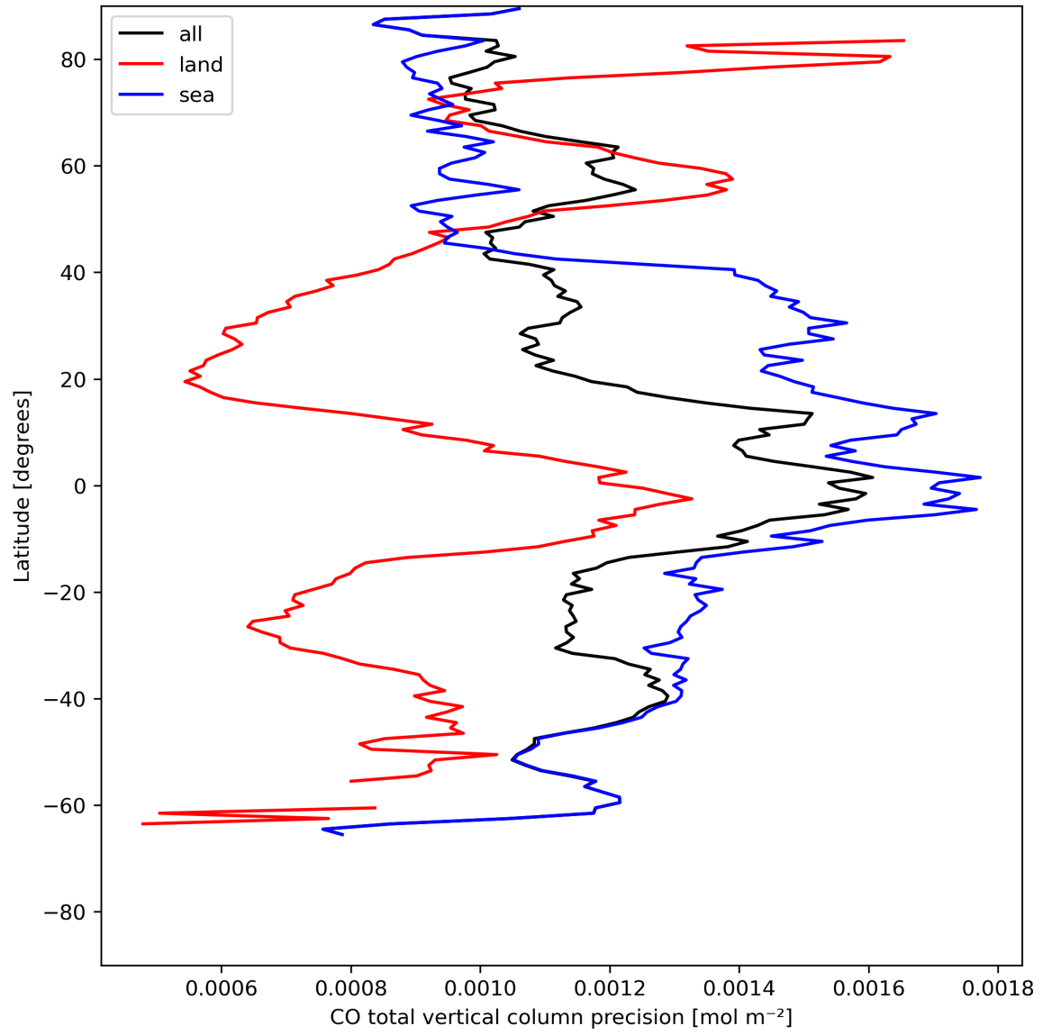
Figure 12: Zonal average of "CO total vertical column precision" for 2024-07-27 to 2024-07-29.
