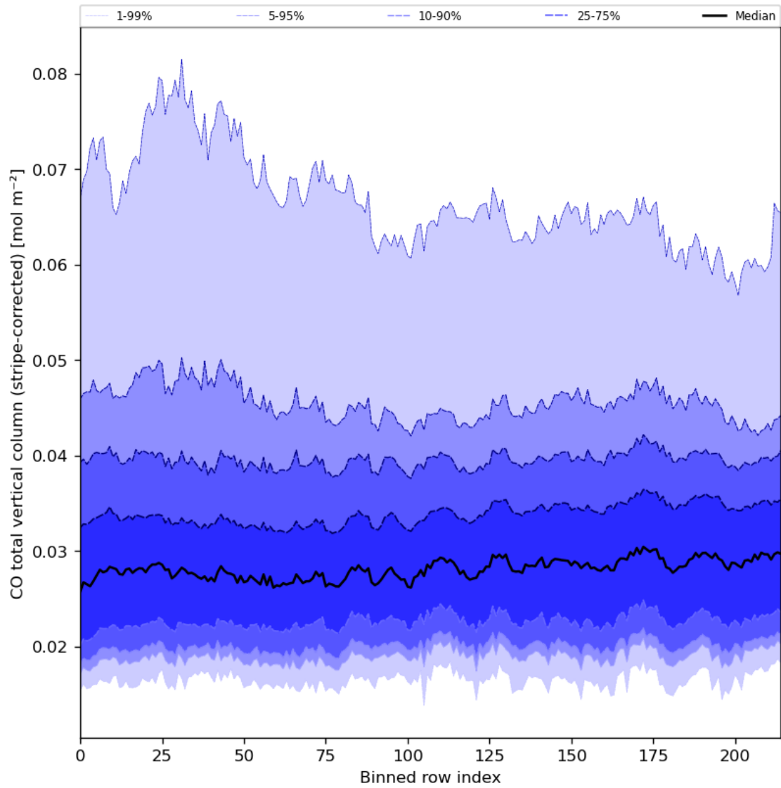
Figure 27: Along track statistics of “CO total vertical column (stripe-corrected)” for 2024-07-27 to 2024-07-29
