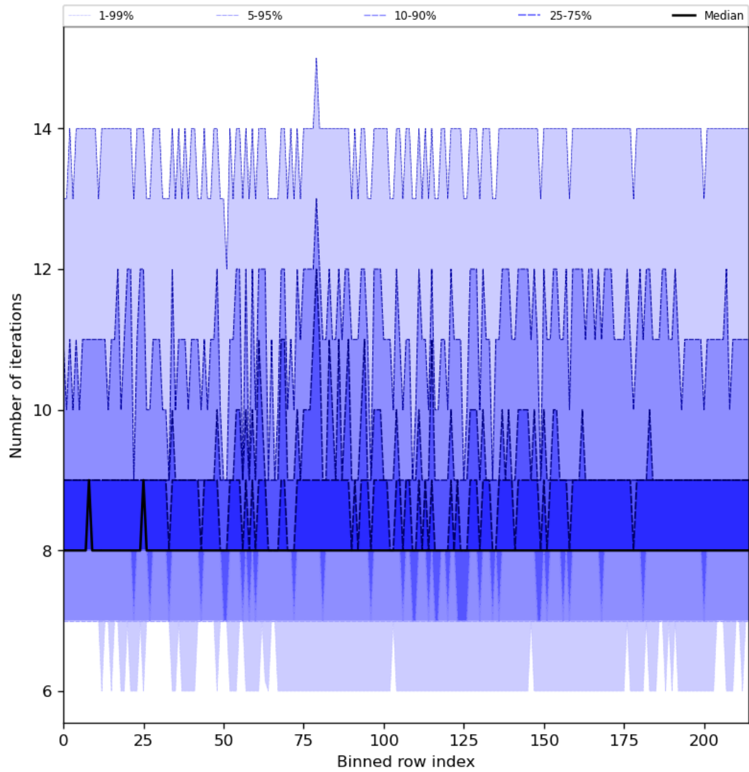
Figure 32: Along track statistics of “Number of iterations” for 2024-07-27 to 2024-07-29
