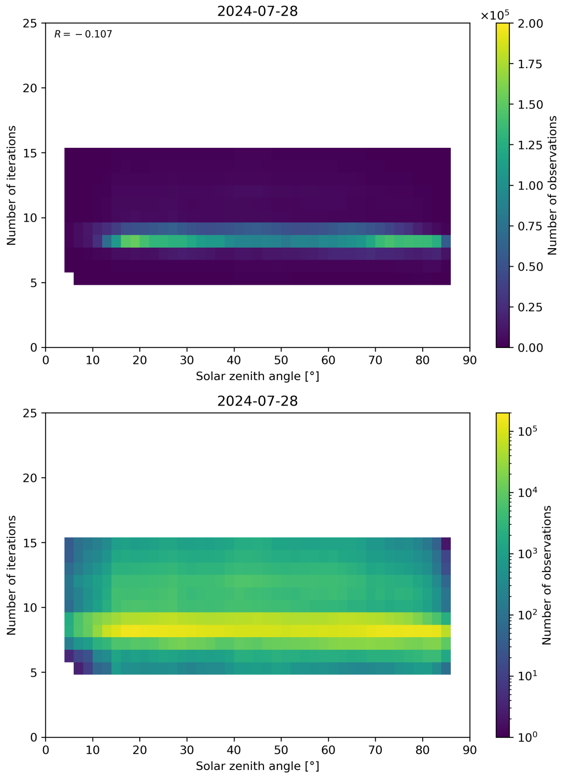
Figure 67: Scatter density plot of “Solar zenith angle” against “Number of iterations” for 2024-07-27 to 2024-07-29.
