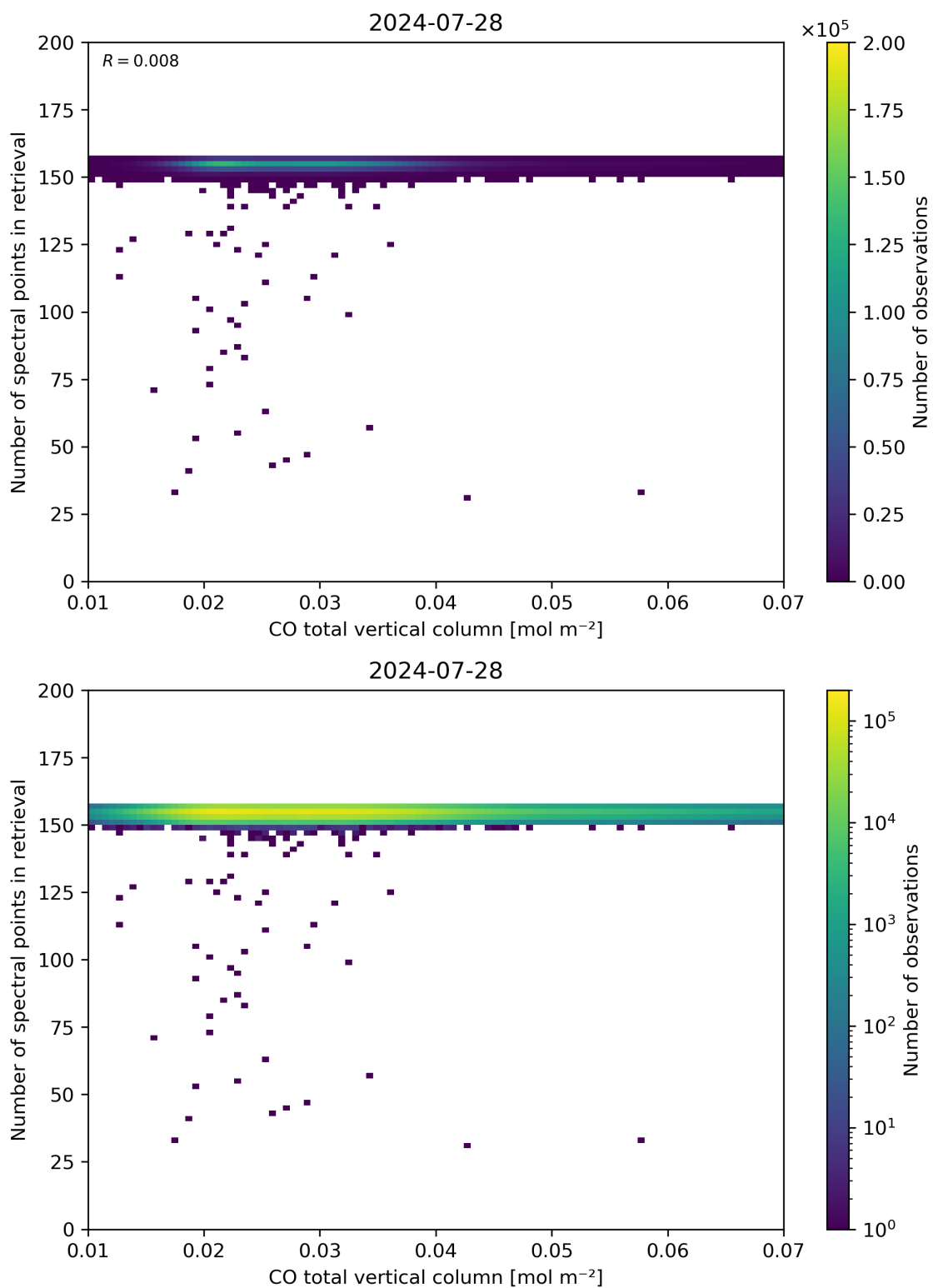
Figure 43: Scatter density plot of “CO total vertical column” against “Number of spectral points in retrieval” for 2024-07-27 to 2024-07-29.
