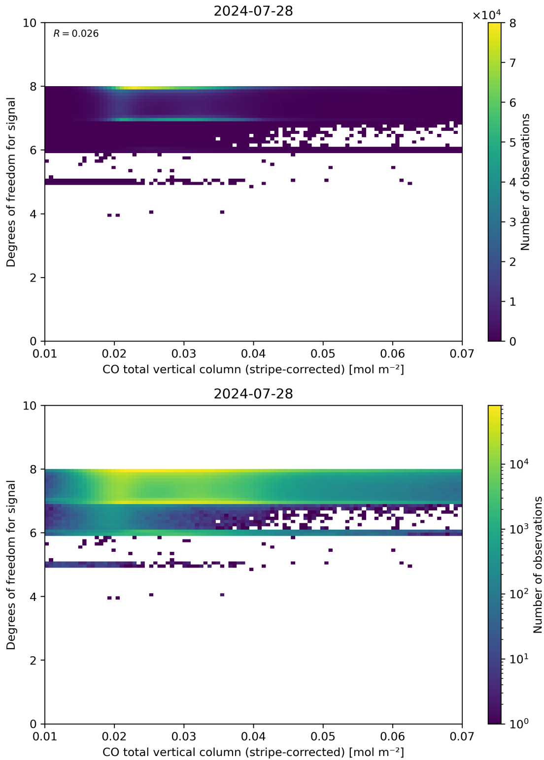
Figure 38: Scatter density plot of “CO total vertical column (stripe-corrected)” against “Degrees of freedom for signal” for 2024-07-27 to 2024-07-29.
