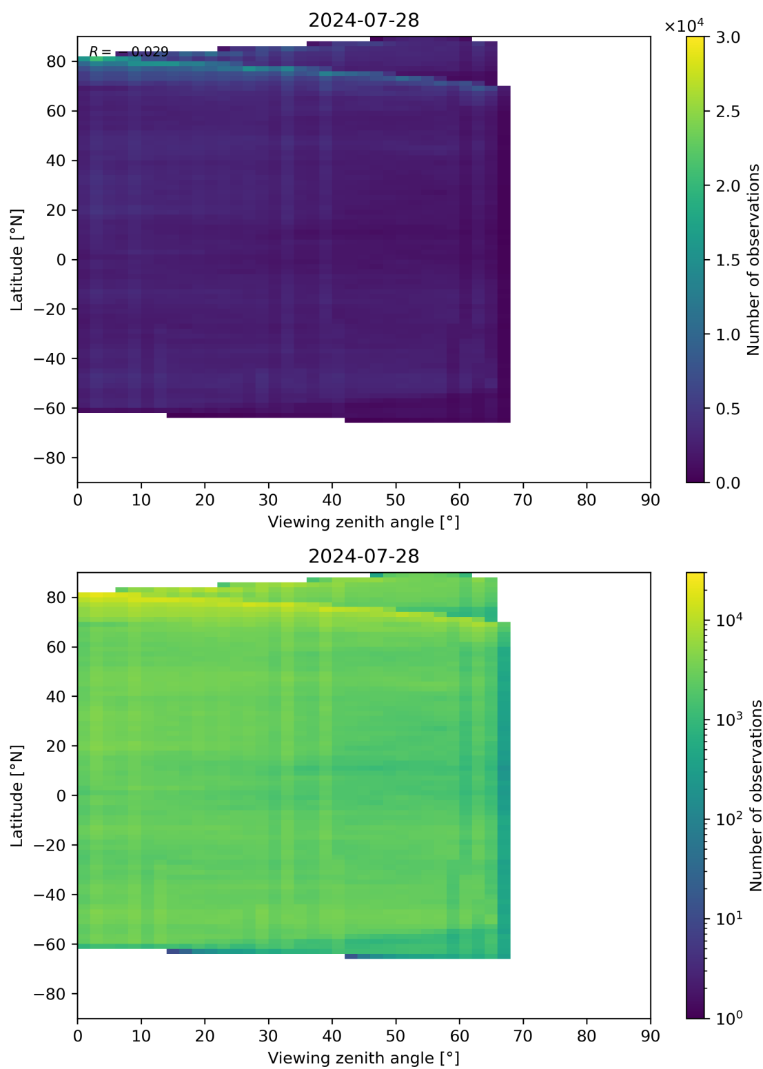
Figure 74: Scatter density plot of “Viewing zenith angle” against “Latitude” for 2024-07-27 to 2024-07-29.
