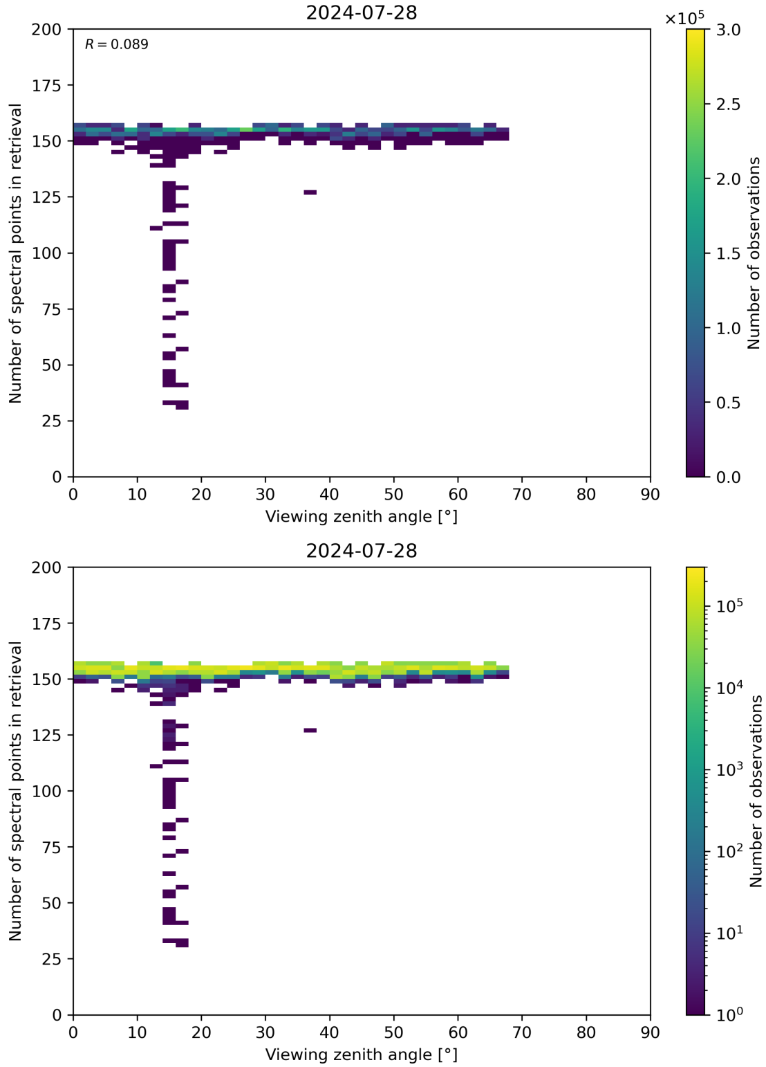
Figure 76: Scatter density plot of “Viewing zenith angle” against “Number of spectral points in retrieval” for 2024-07-27 to 2024-07-29.
