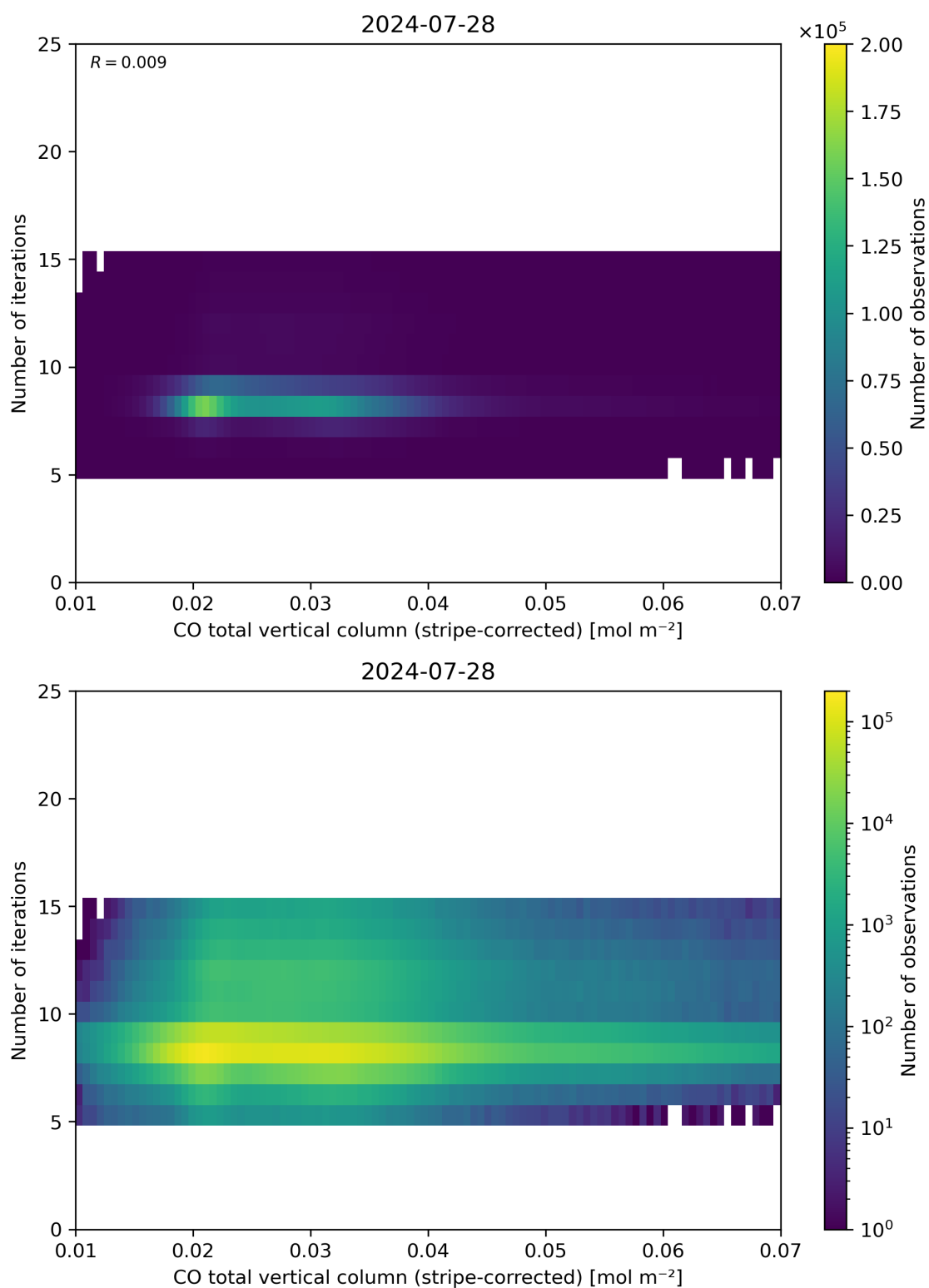
Figure 39: Scatter density plot of “CO total vertical column (stripe-corrected)” against “Number of iterations” for 2024-07-27 to 2024-07-29.
