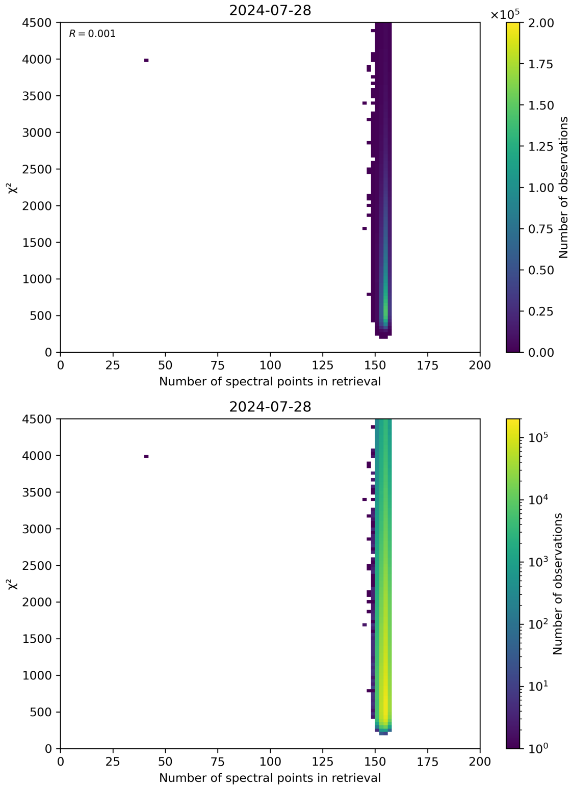
Figure 58: Scatter density plot of “Number of spectral points in retrieval” against “ \chi^2 ” for 2024-07-27 to 2024-07-29.
