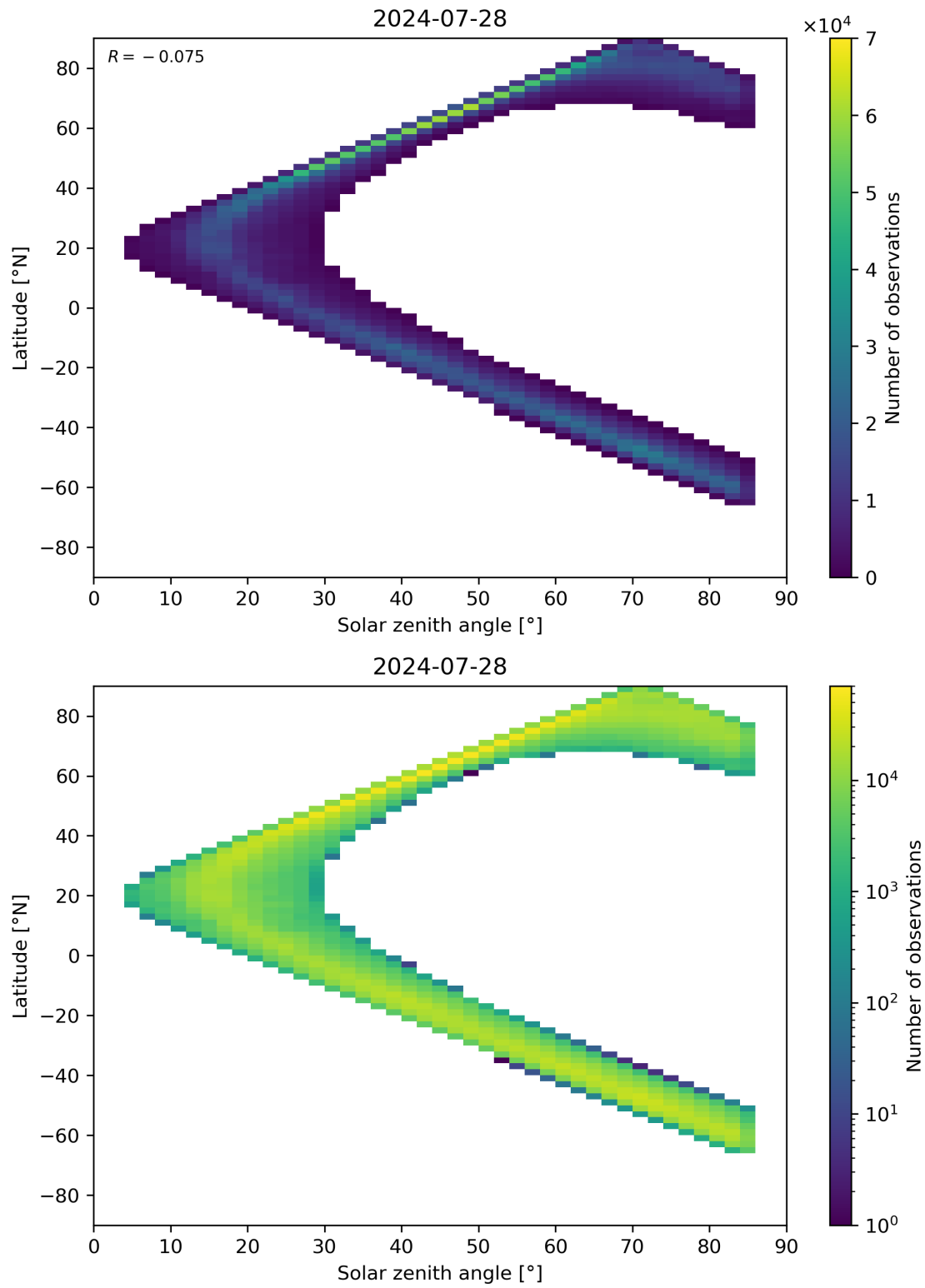
Figure 66: Scatter density plot of “Solar zenith angle” against “Latitude” for 2024-07-27 to 2024-07-29.
