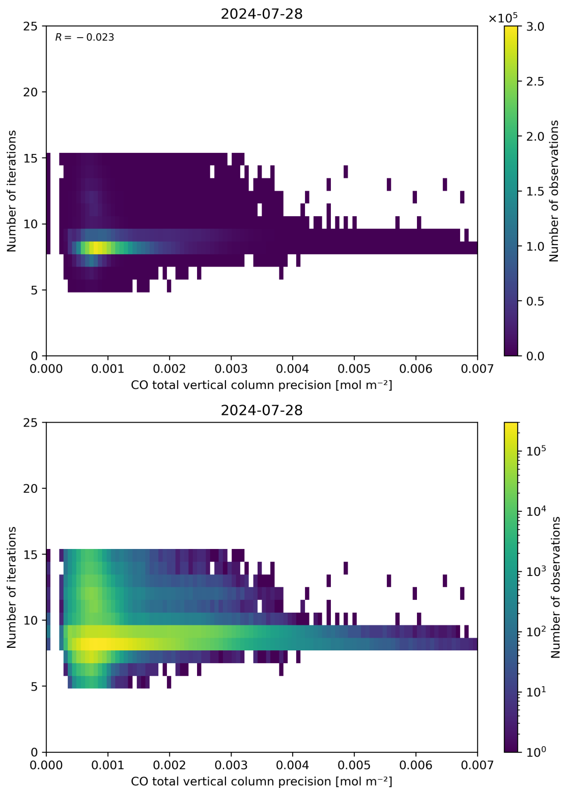
Figure 46: Scatter density plot of “CO total vertical column precision” against “Number of iterations” for 2024-07-27 to 2024-07-29.
