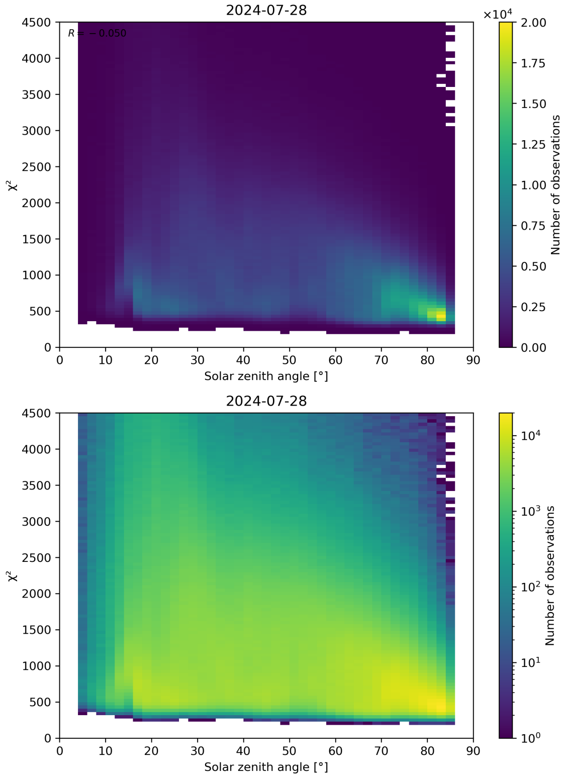
Figure 64: Scatter density plot of “Solar zenith angle” against “ \chi^2 ” for 2024-07-27 to 2024-07-29.
