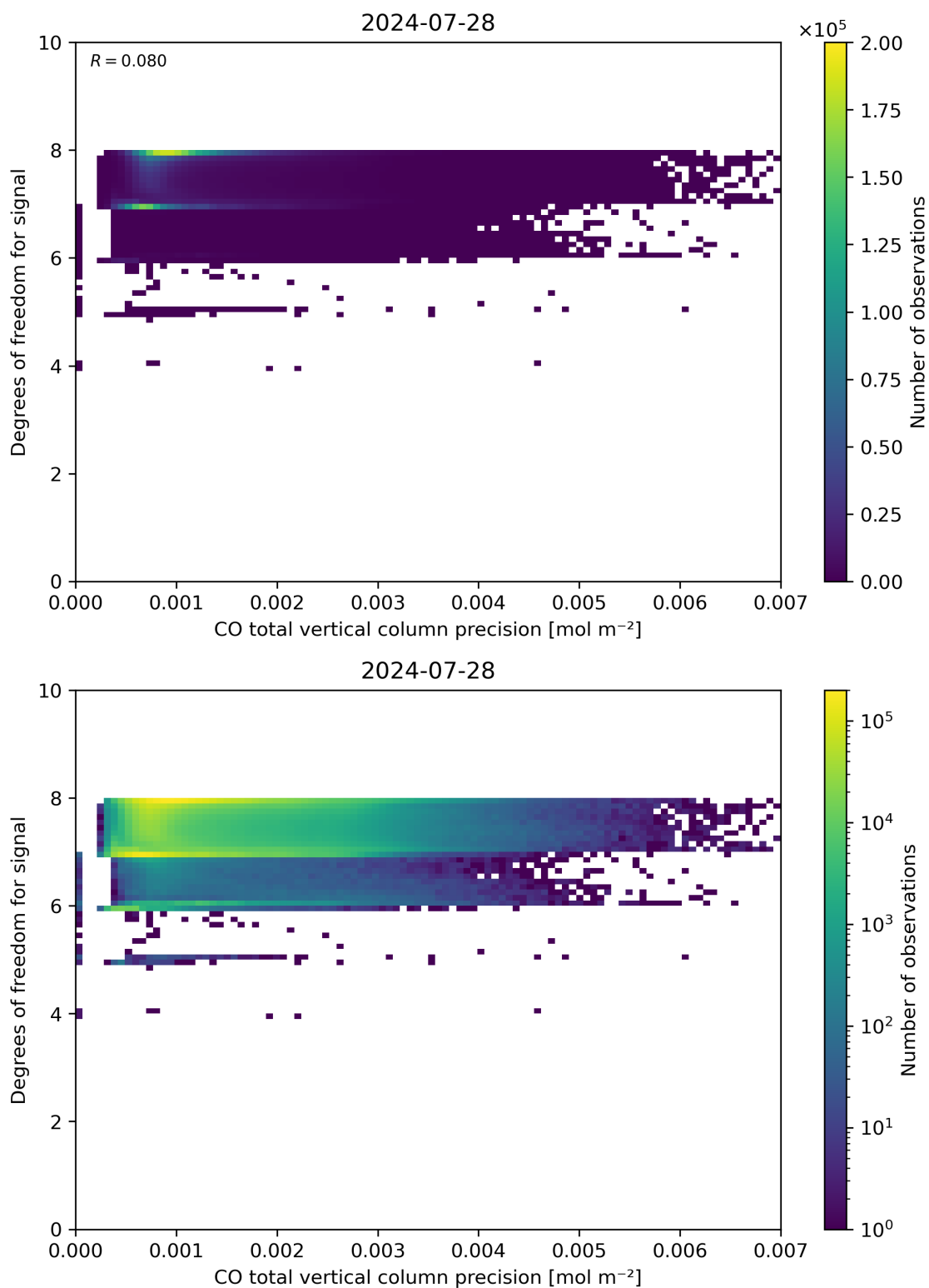
Figure 45: Scatter density plot of “CO total vertical column precision” against “Degrees of freedom for signal” for 2024-07-27 to 2024-07-29.
