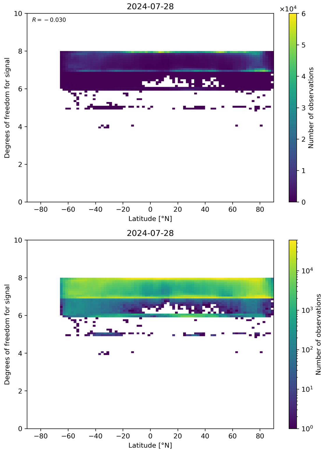
Figure 55: Scatter density plot of “Latitude” against “Degrees of freedom for signal” for 2024-07-27 to 2024-07-29.
