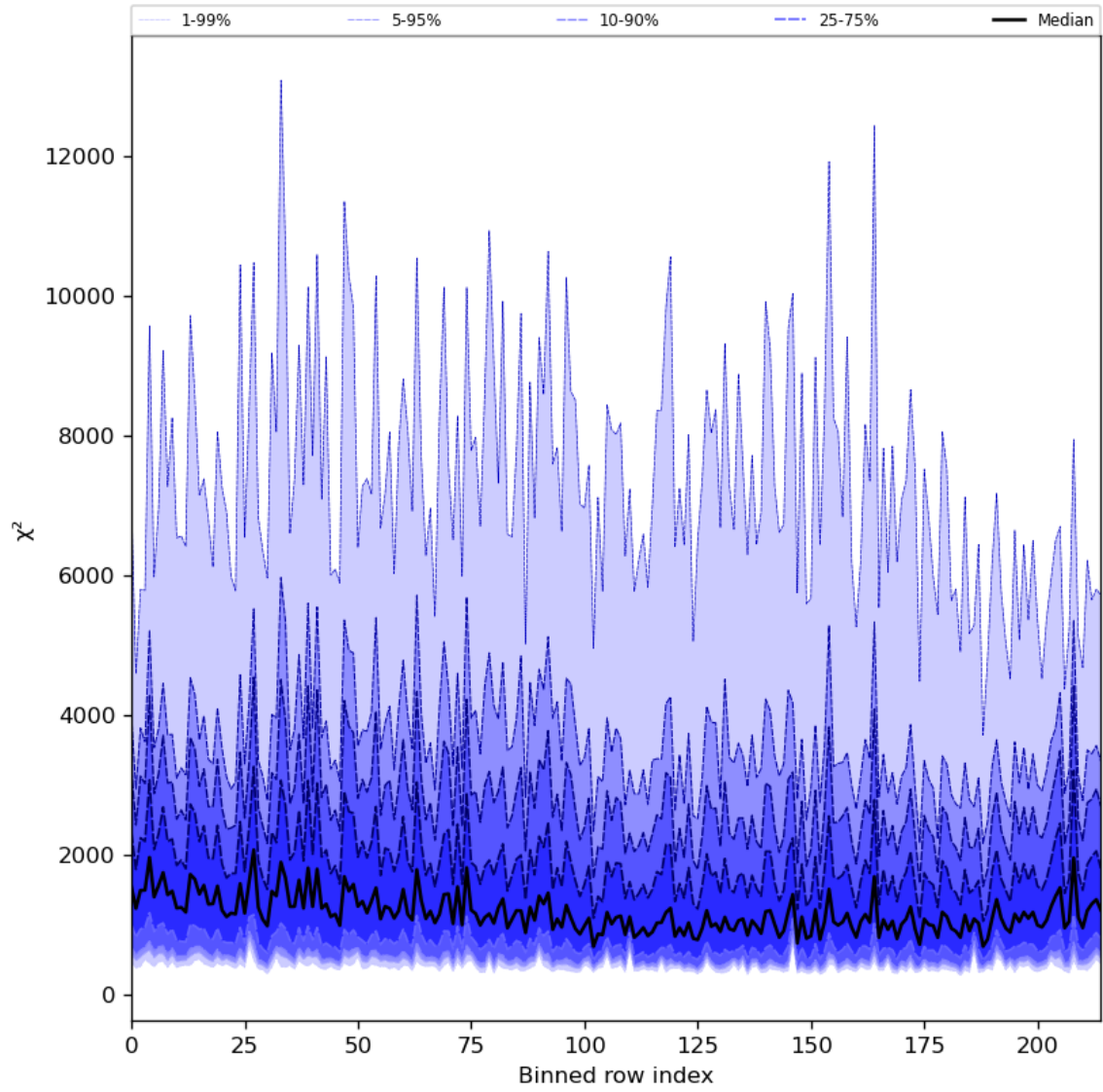
Figure 30: Along track statistics of “ \chi^2 ” for 2024-07-27 to 2024-07-29
