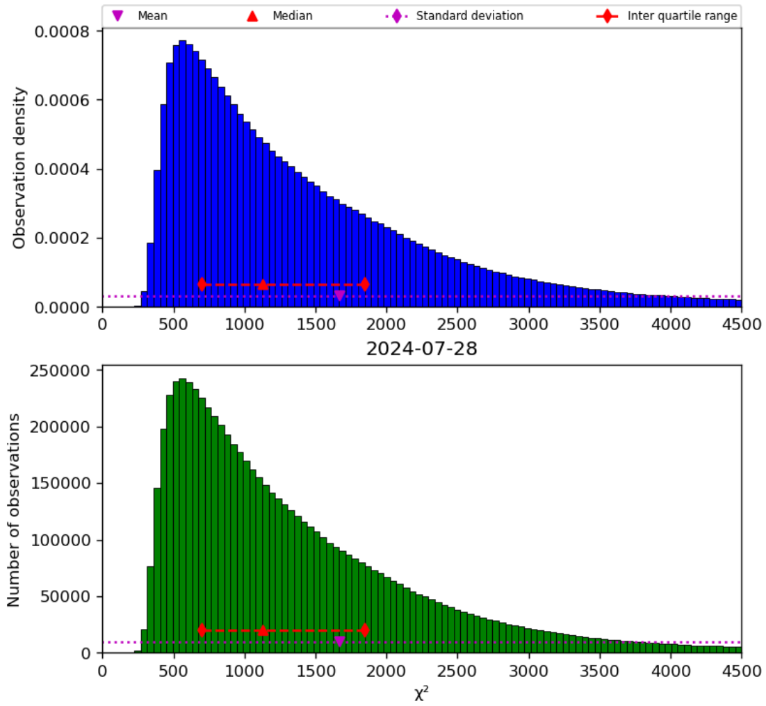
Figure 22: Histogram of “ \chi^2 ” for 2024-07-27 to 2024-07-29
