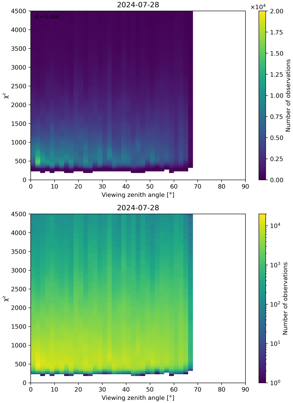
Figure 72: Scatter density plot of “Viewing zenith angle” against “ \chi^2 ” for 2024-07-27 to 2024-07-29.
