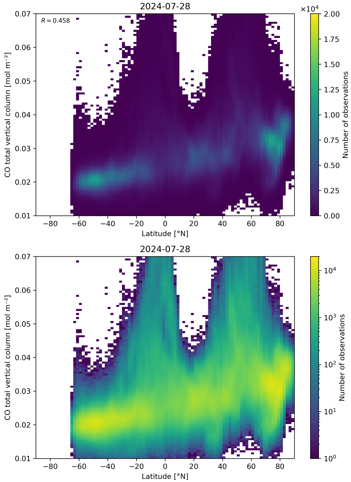
Figure 51: Scatter density plot of “Latitude” against “CO total vertical column” for 2024-07-27 to 2024-07-29.
