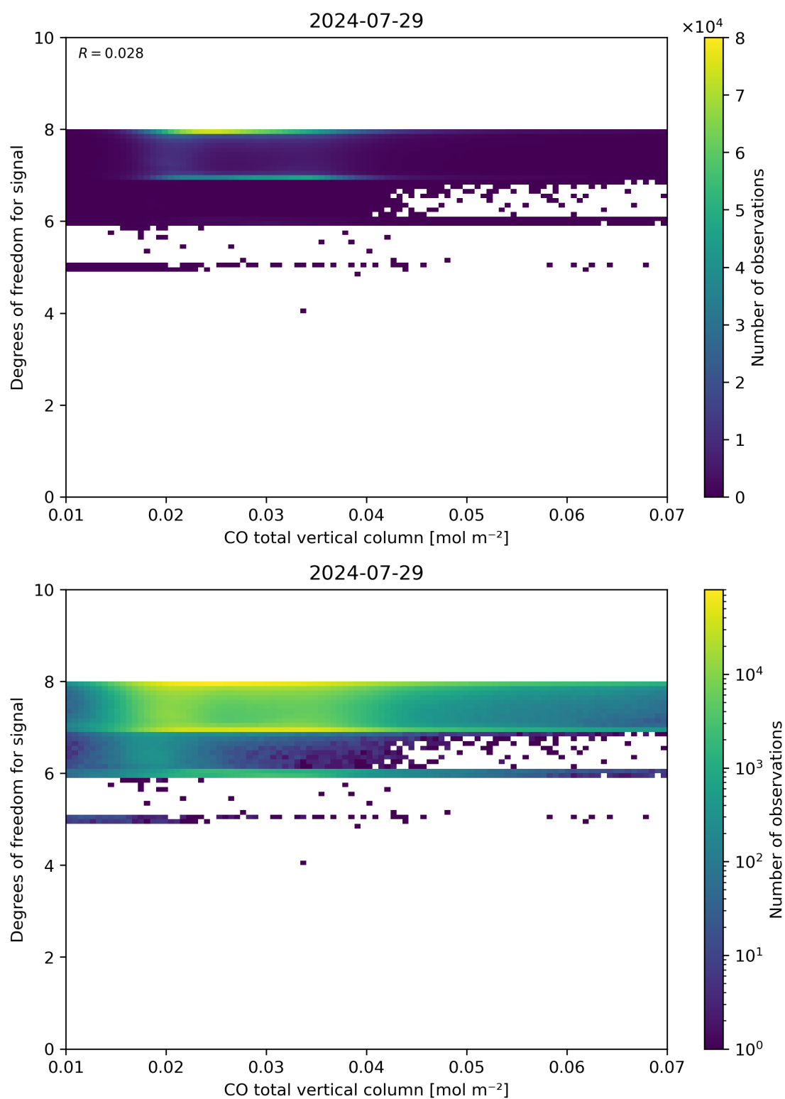
Figure 41: Scatter density plot of “CO total vertical column” against “Degrees of freedom for signal” for 2024-07-28 to 2024-07-30.
