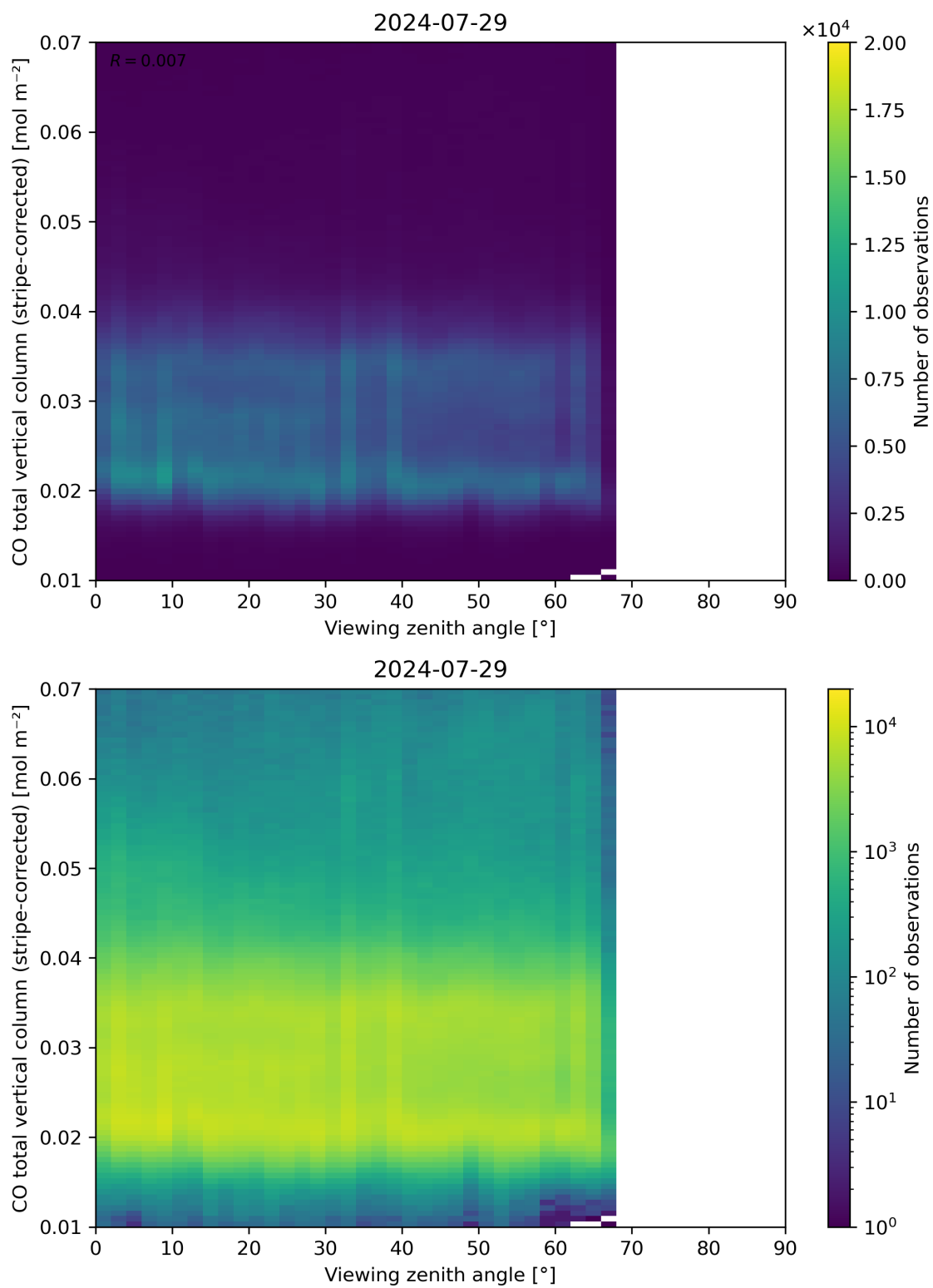
Figure 70: Scatter density plot of “Viewing zenith angle” against “CO total vertical column (stripe-corrected)” for 2024-07-28 to 2024-07-30.
