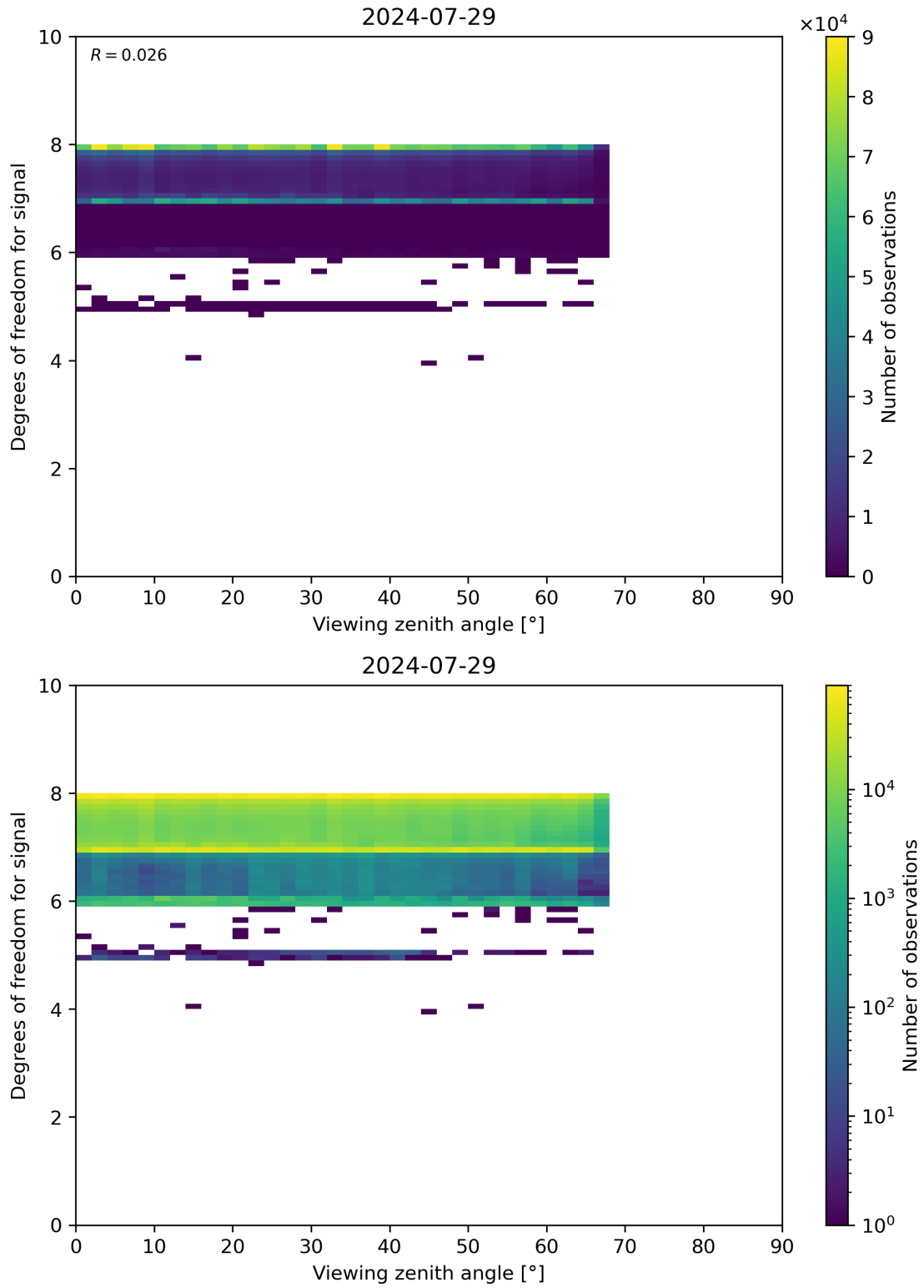
Figure 73: Scatter density plot of “Viewing zenith angle” against “Degrees of freedom for signal” for 2024-07-28 to 2024-07-30.
