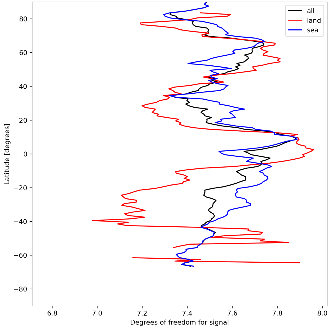
Figure 15: Zonal average of “Degrees of freedom for signal” for 2024-07-28 to 2024-07-30.
