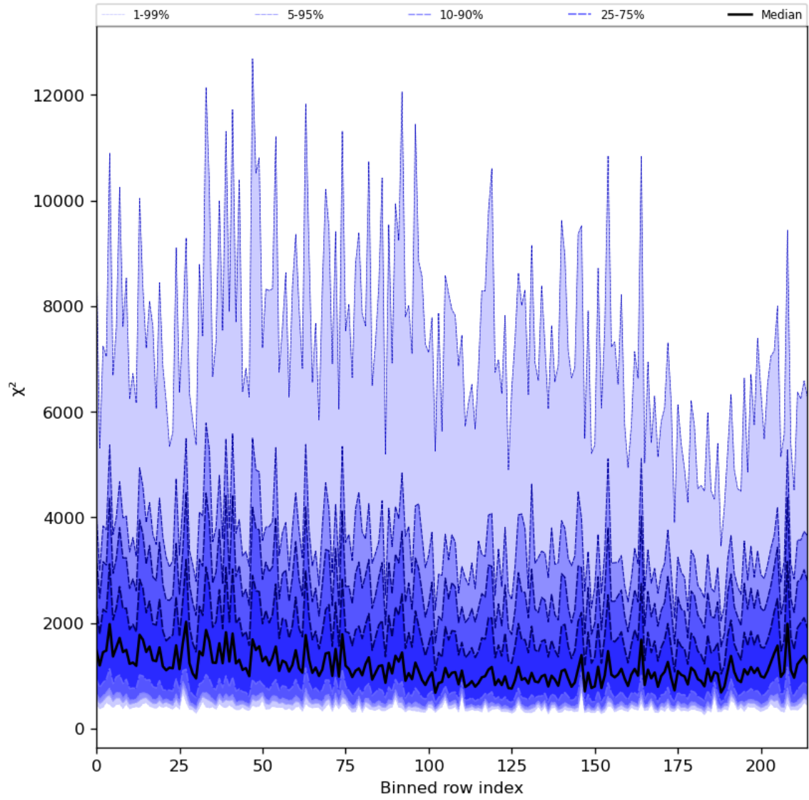
Figure 30: Along track statistics of “ \chi^2 ” for 2024-07-28 to 2024-07-30
