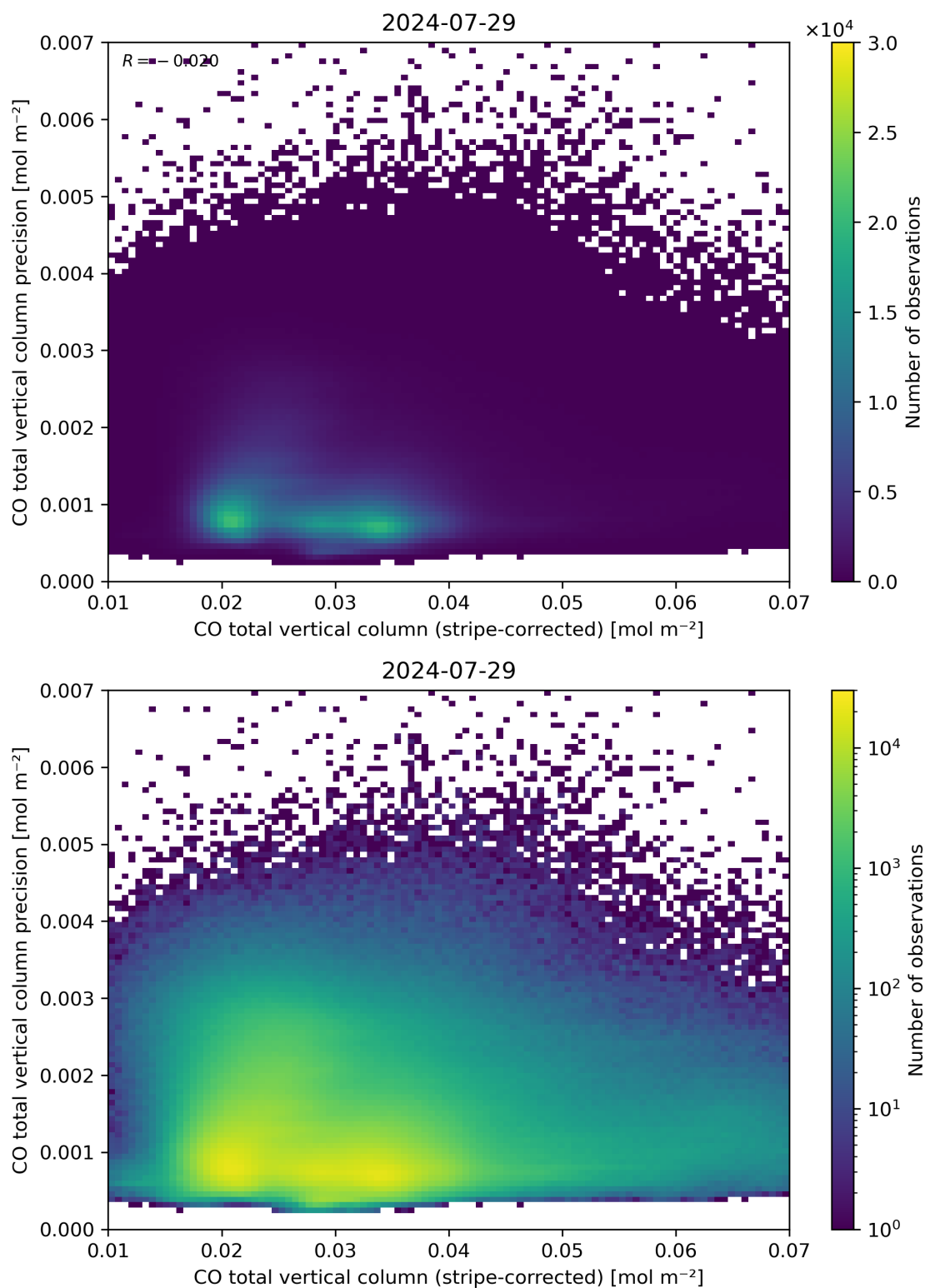
Figure 36: Scatter density plot of “CO total vertical column (stripe-corrected)” against “CO total vertical column precision” for 2024-07-28 to 2024-07-30.
