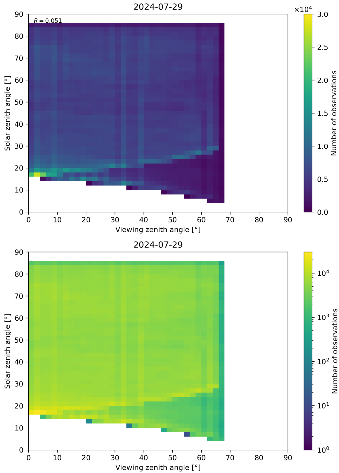
Figure 77: Scatter density plot of “Viewing zenith angle” against “Solar zenith angle” for 2024-07-28 to 2024-07-30.
