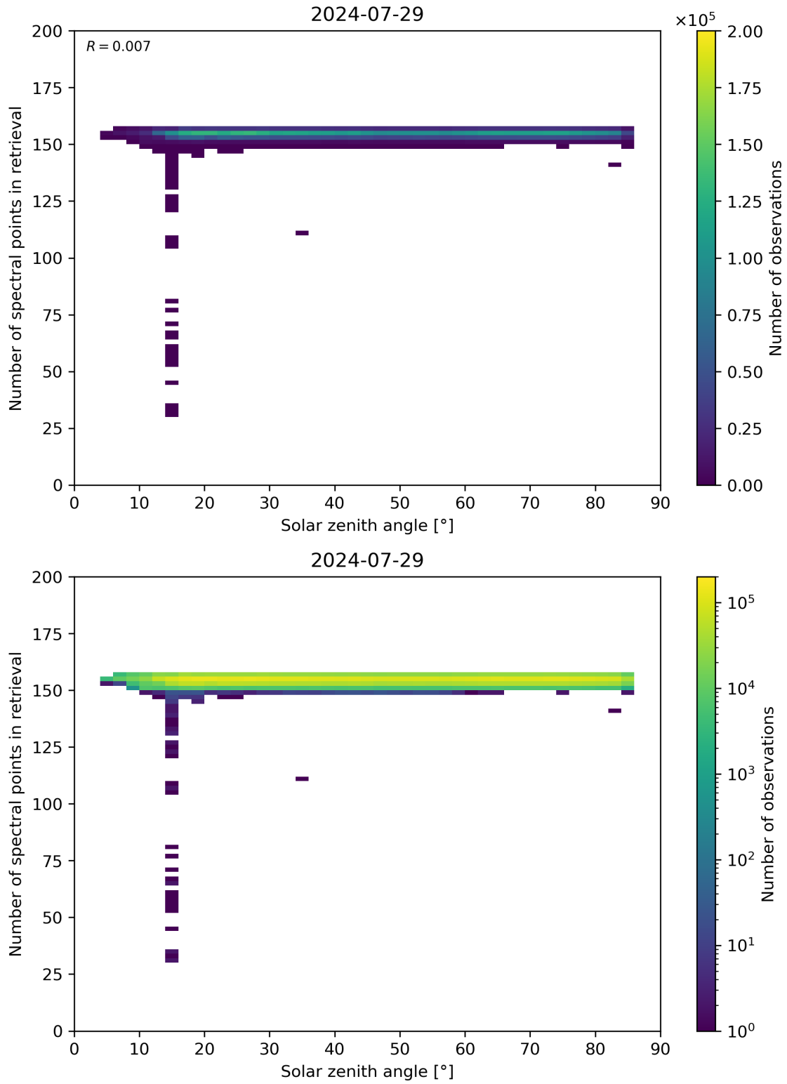
Figure 68: Scatter density plot of “Solar zenith angle” against “Number of spectral points in retrieval” for 2024-07-28 to 2024-07-30.
