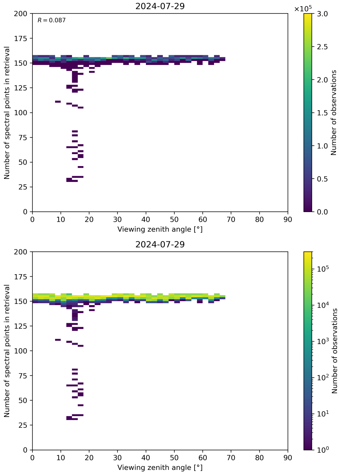
Figure 76: Scatter density plot of “Viewing zenith angle” against “Number of spectral points in retrieval” for 2024-07-28 to 2024-07-30.
