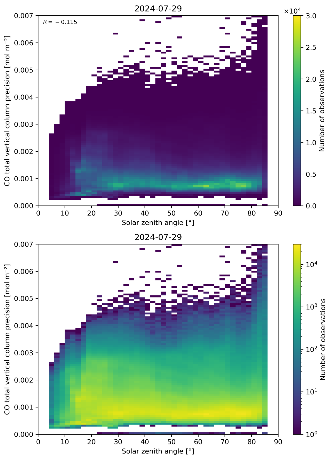
Figure 63: Scatter density plot of “Solar zenith angle” against “CO total vertical column precision” for 2024-07-28 to 2024-07-30.
