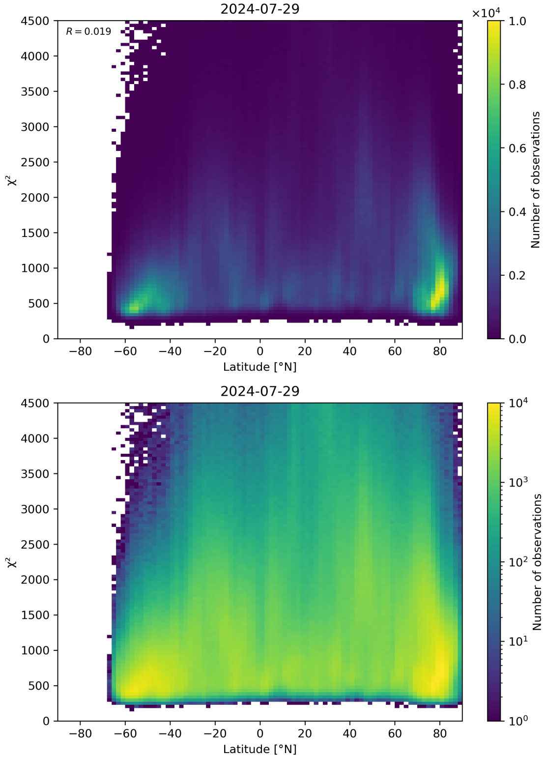
Figure 54: Scatter density plot of “Latitude” against “ \chi^2 ” for 2024-07-28 to 2024-07-30.
