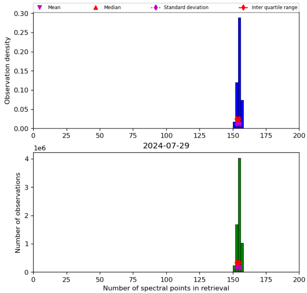
Figure 21: Histogram of “Number of spectral points in retrieval” for 2024-07-28 to 2024-07-30
