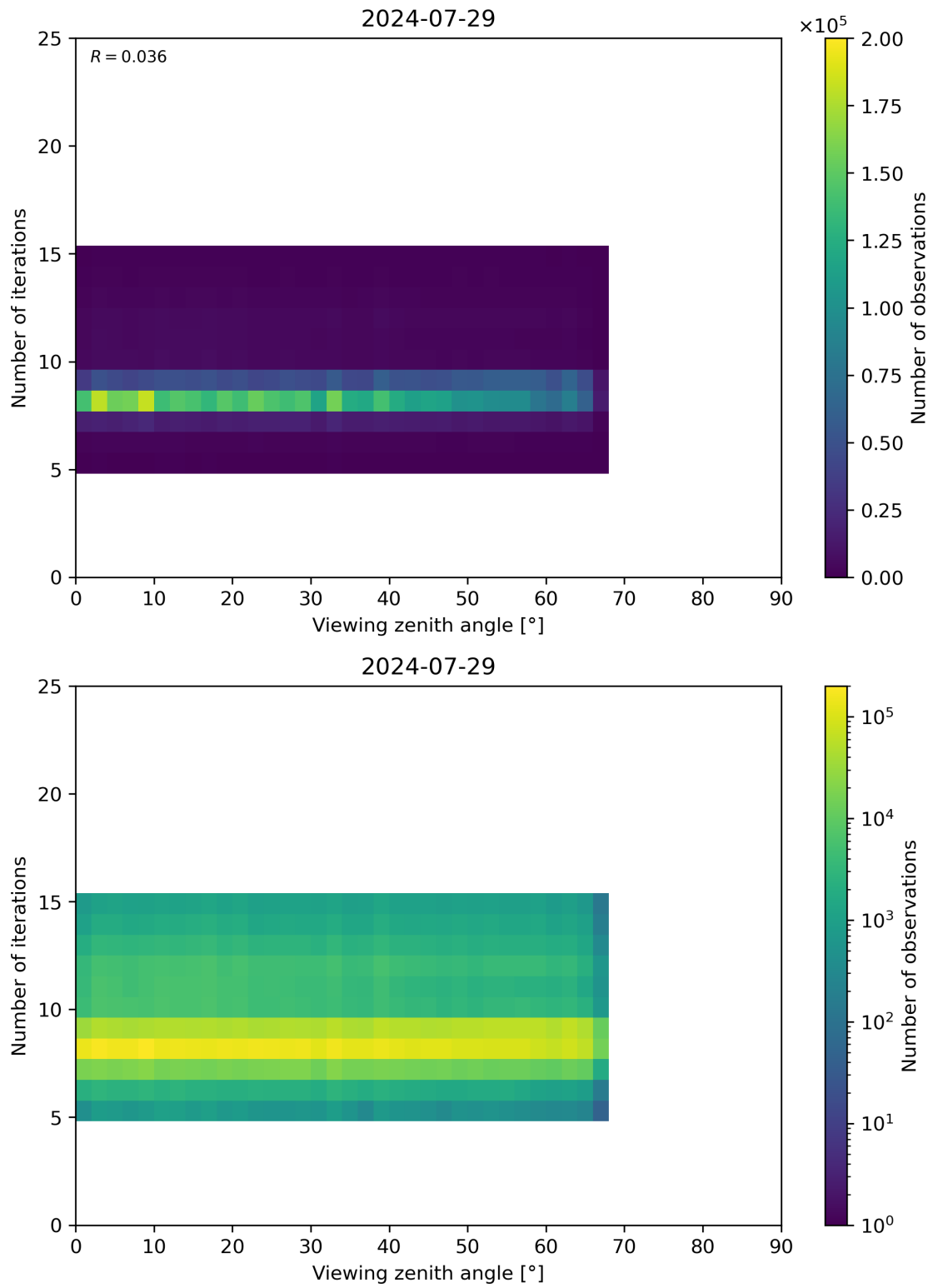
Figure 75: Scatter density plot of “Viewing zenith angle” against “Number of iterations” for 2024-07-28 to 2024-07-30.
