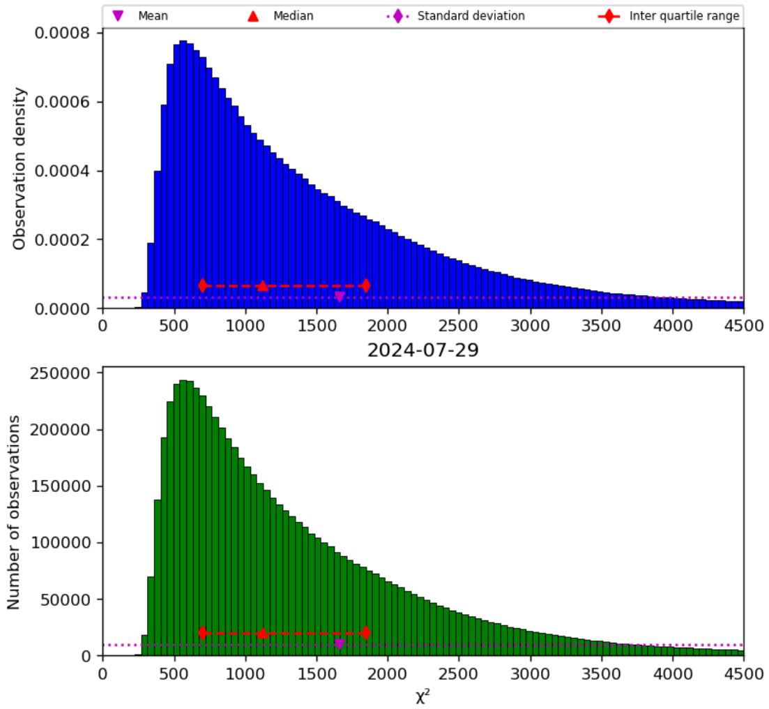
Figure 22: Histogram of “ \chi^2 ” for 2024-07-28 to 2024-07-30
