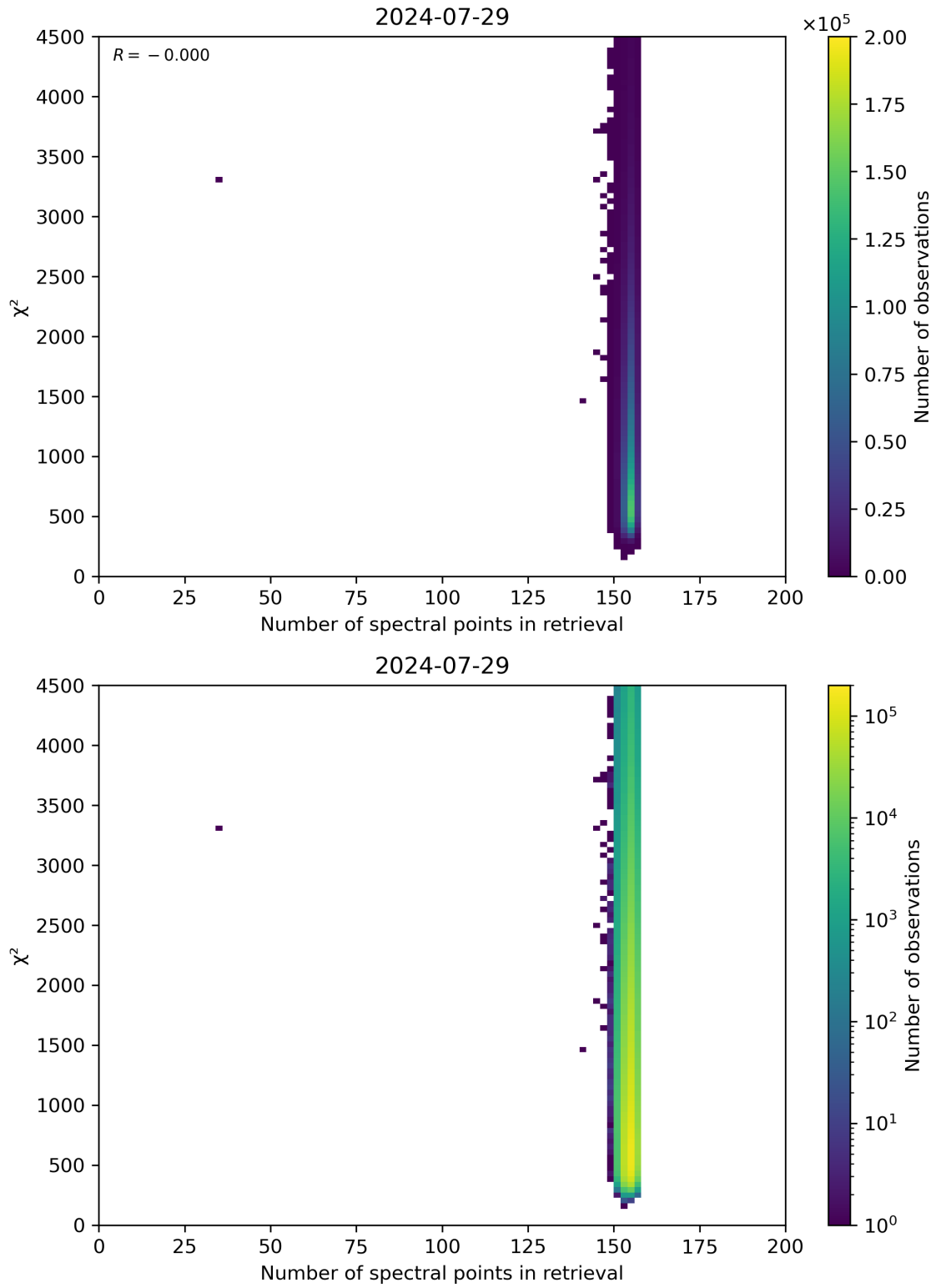
Figure 58: Scatter density plot of “Number of spectral points in retrieval” against “ \chi^2 ” for 2024-07-28 to 2024-07-30.
