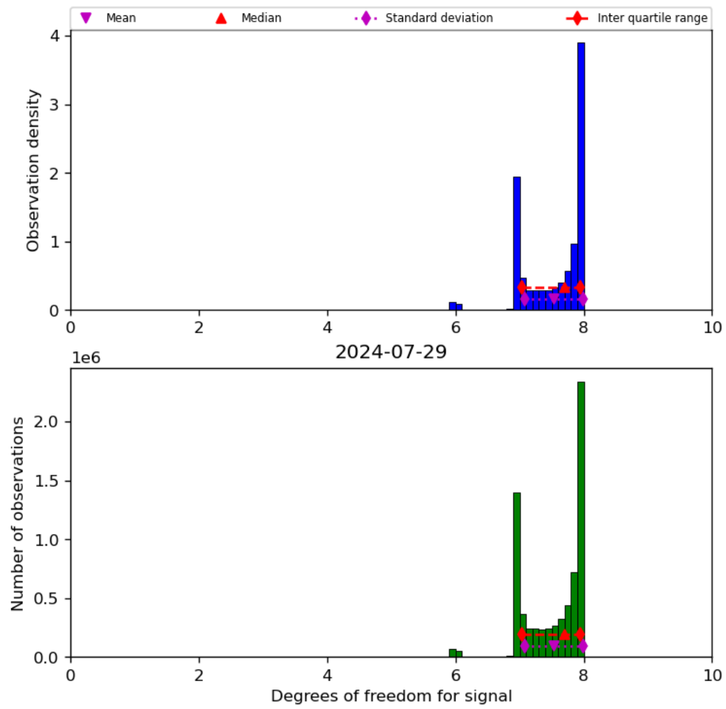
Figure 23: Histogram of “Degrees of freedom for signal” for 2024-07-28 to 2024-07-30
