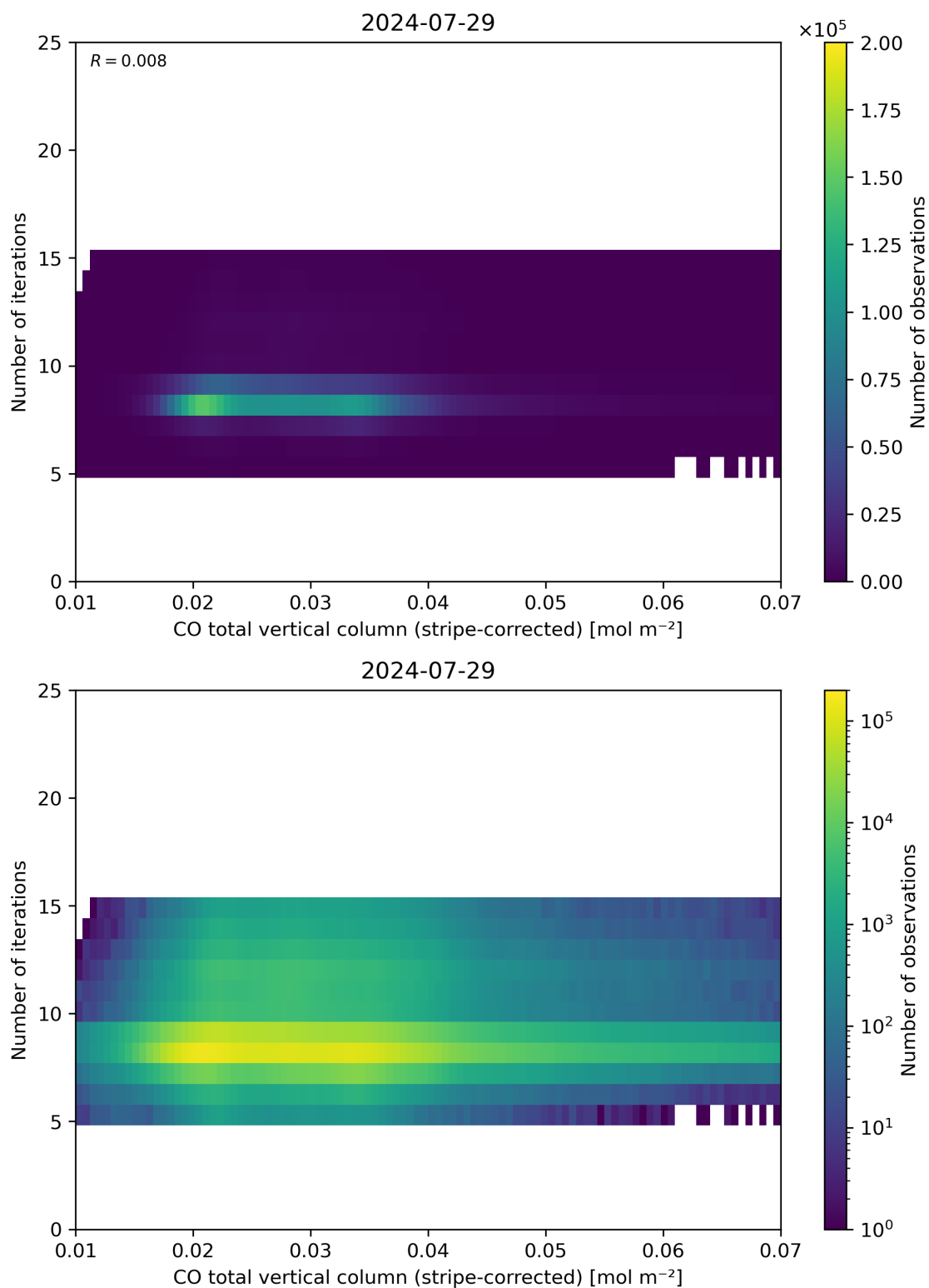
Figure 39: Scatter density plot of “CO total vertical column (stripe-corrected)” against “Number of iterations” for 2024-07-28 to 2024-07-30.
