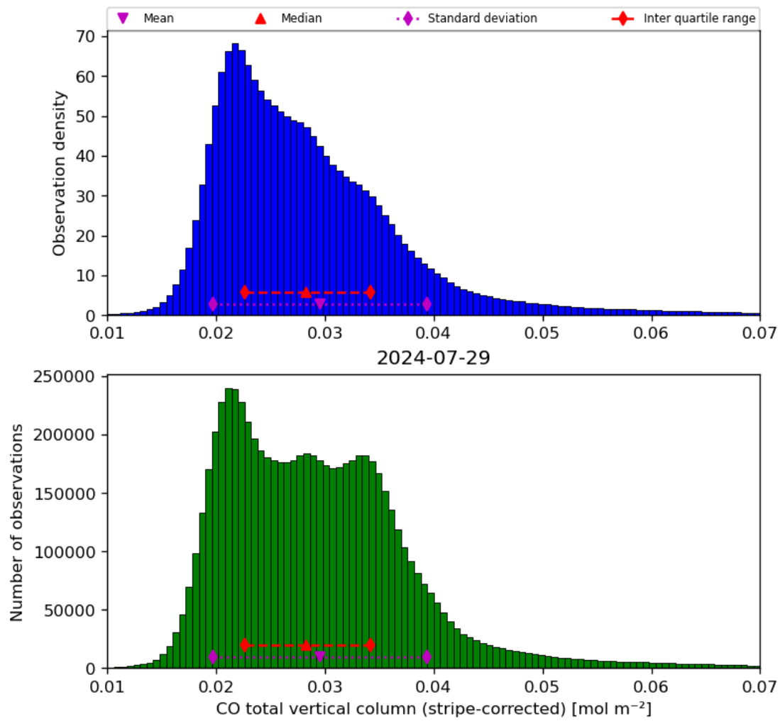
Figure 19: Histogram of “CO total vertical column (stripe-corrected)” for 2024-07-28 to 2024-07-30
