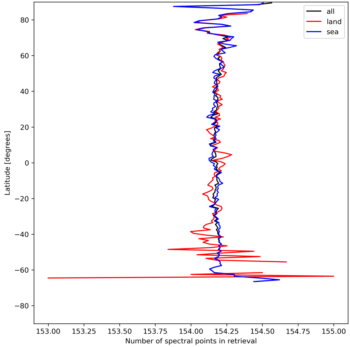
Figure 13: Zonal average of “Number of spectral points in retrieval” for 2024-07-28 to 2024-07-30.
