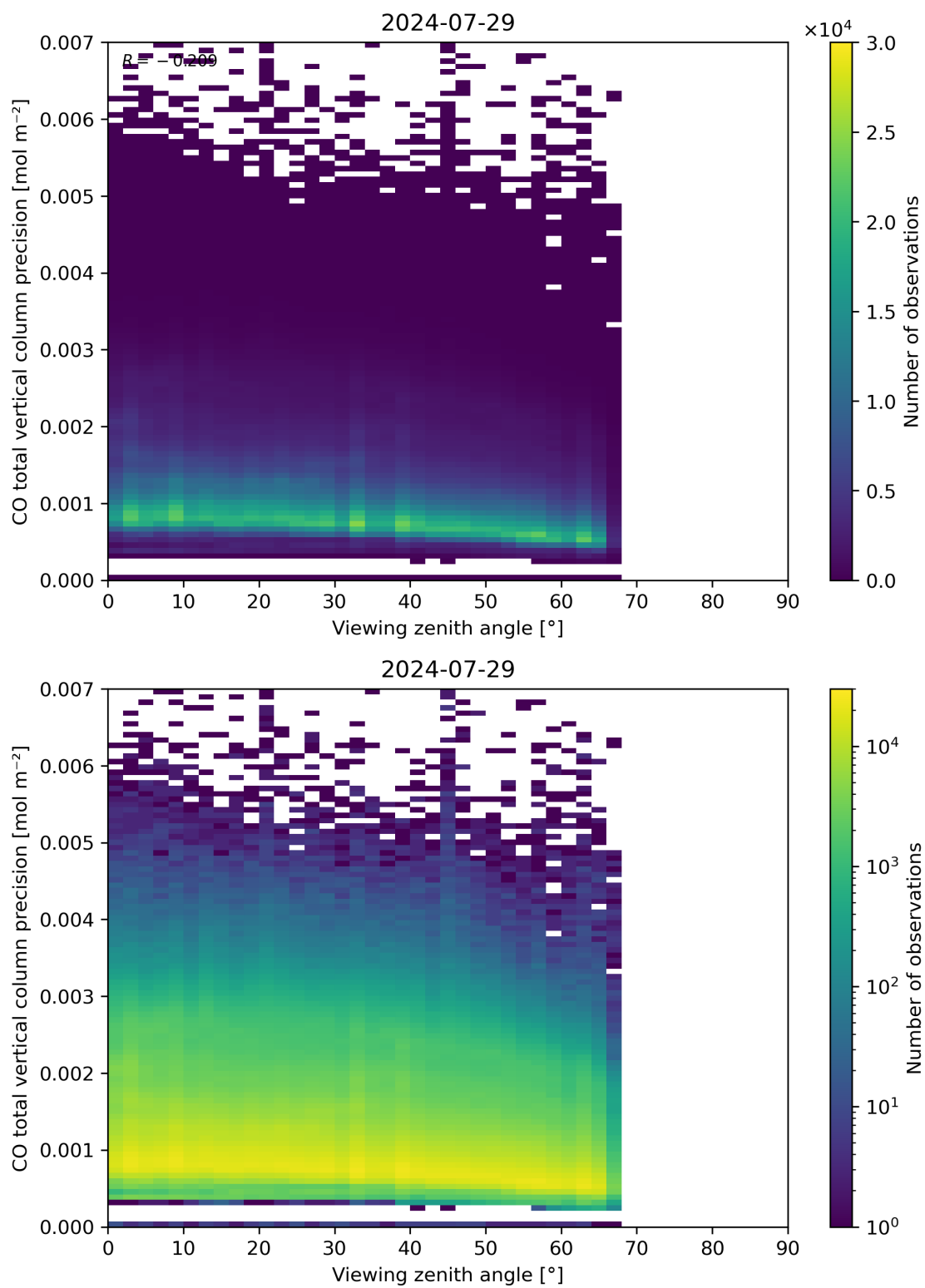
Figure 71: Scatter density plot of “Viewing zenith angle” against “CO total vertical column precision” for 2024-07-28 to 2024-07-30.
