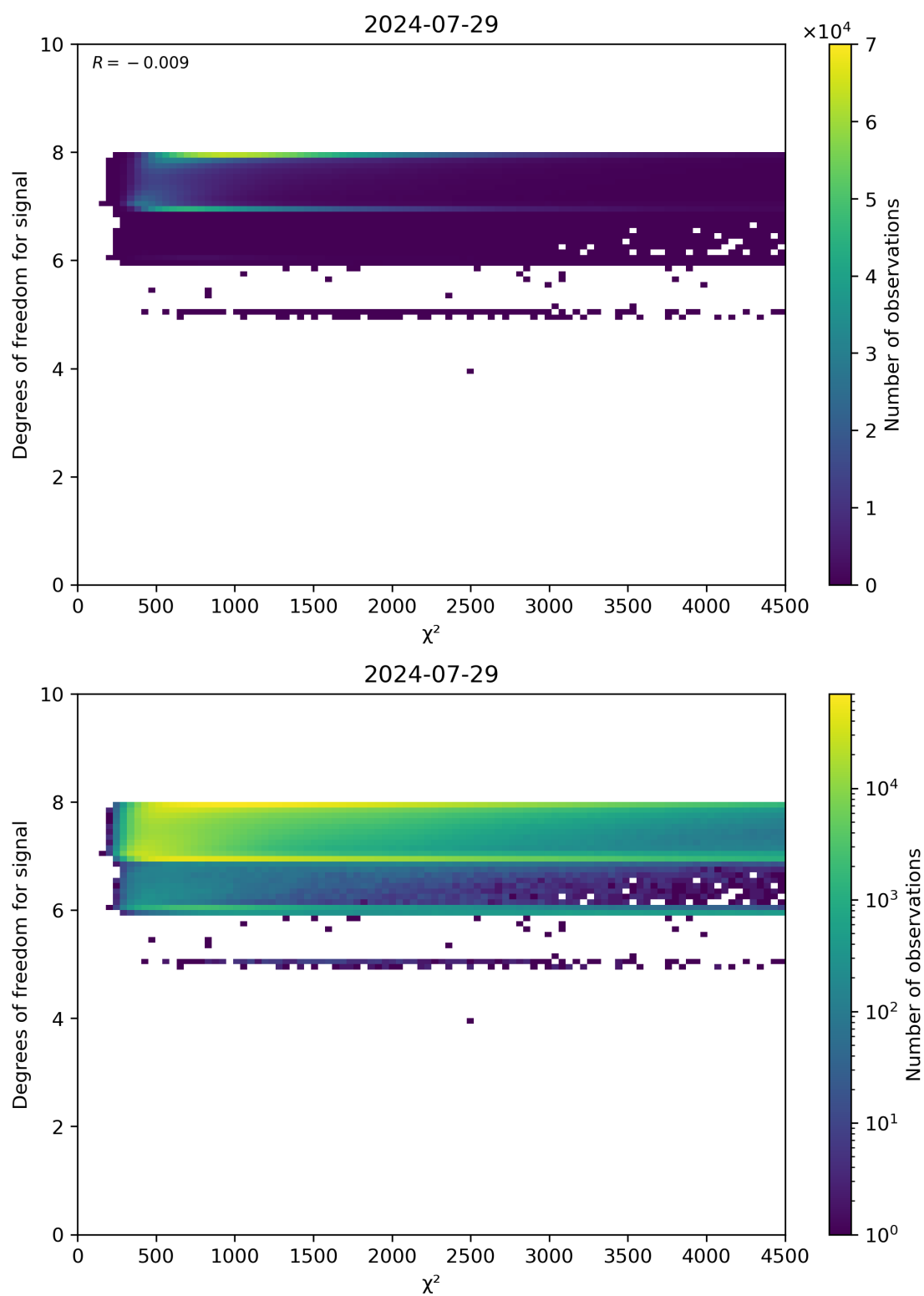
Figure 48: Scatter density plot of “ \chi^2 ” against “Degrees of freedom for signal” for 2024-07-28 to 2024-07-30.
