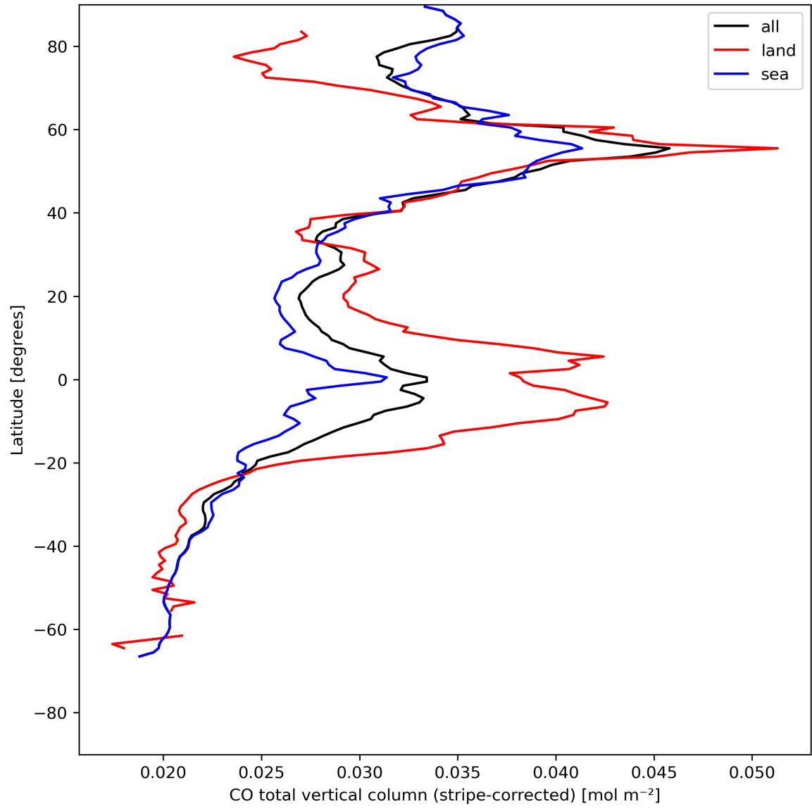
Figure 11: Zonal average of “CO total vertical column (stripe-corrected)” for 2024-07-28 to 2024-07-30.
