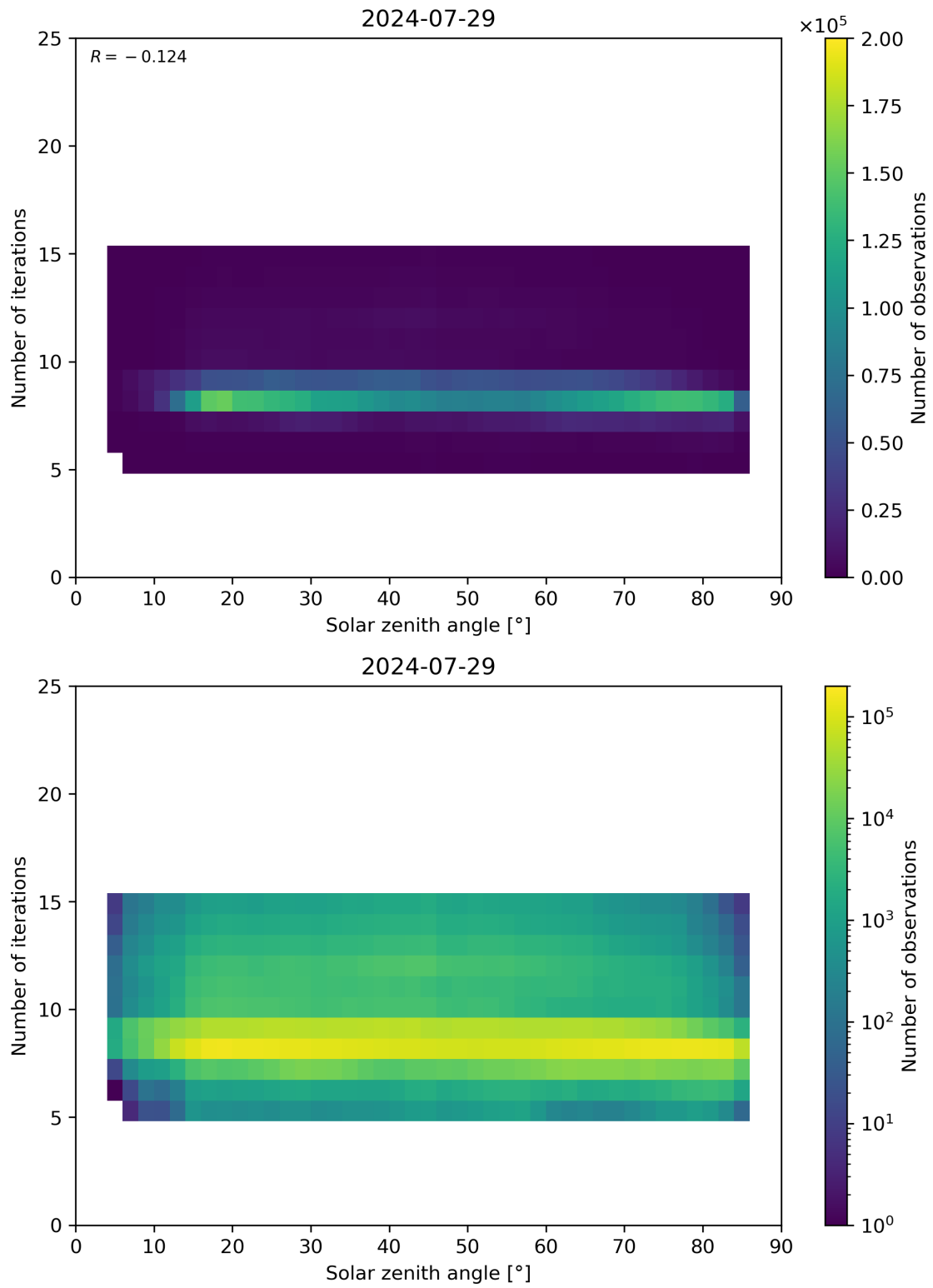
Figure 67: Scatter density plot of “Solar zenith angle” against “Number of iterations” for 2024-07-28 to 2024-07-30.
