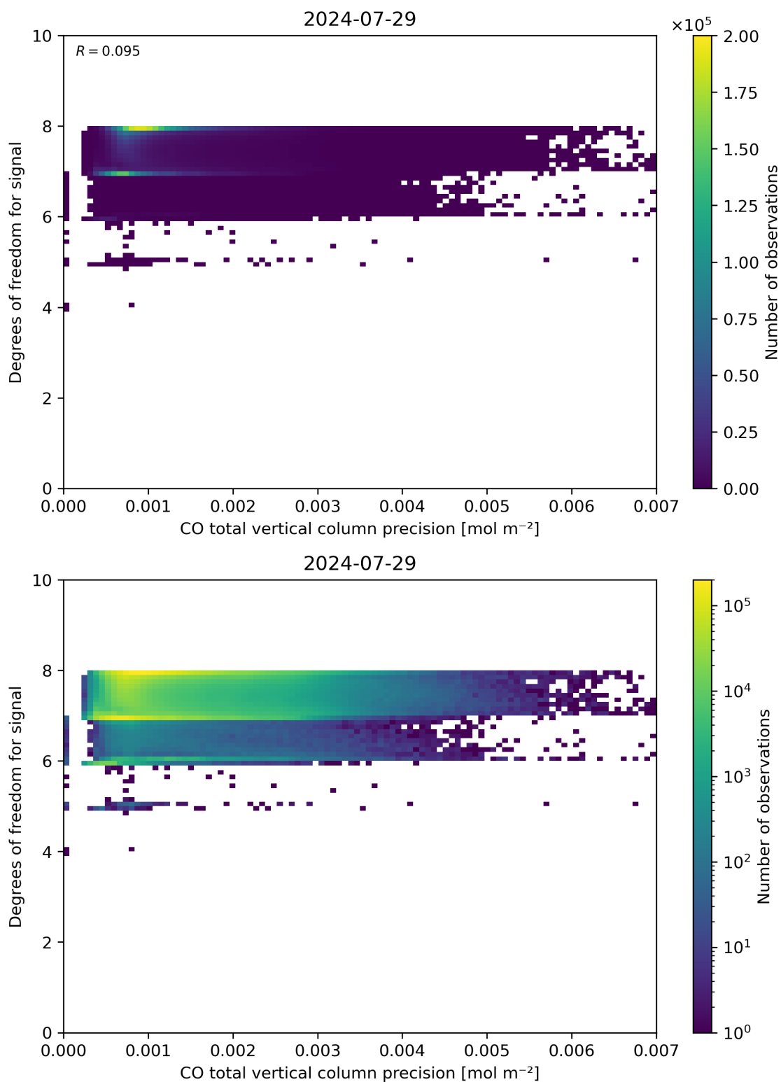
Figure 45: Scatter density plot of “CO total vertical column precision” against “Degrees of freedom for signal” for 2024-07-28 to 2024-07-30.
