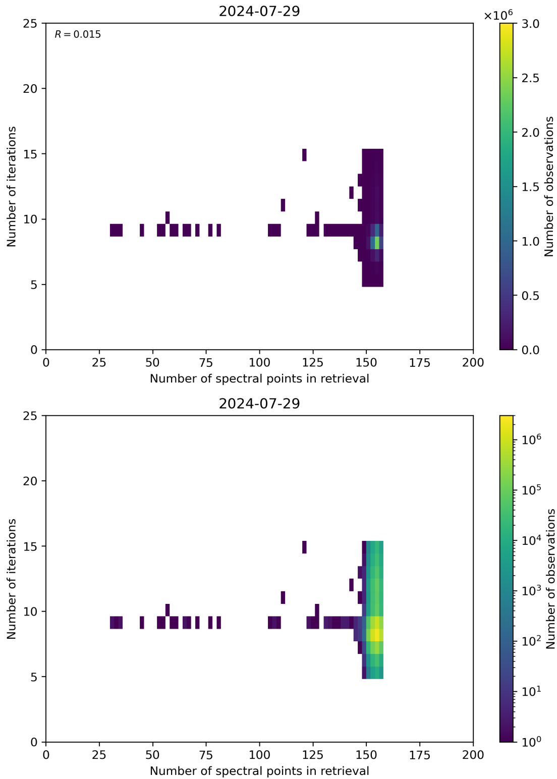
Figure 60: Scatter density plot of “Number of spectral points in retrieval” against “Number of iterations” for 2024-07-28 to 2024-07-30.
