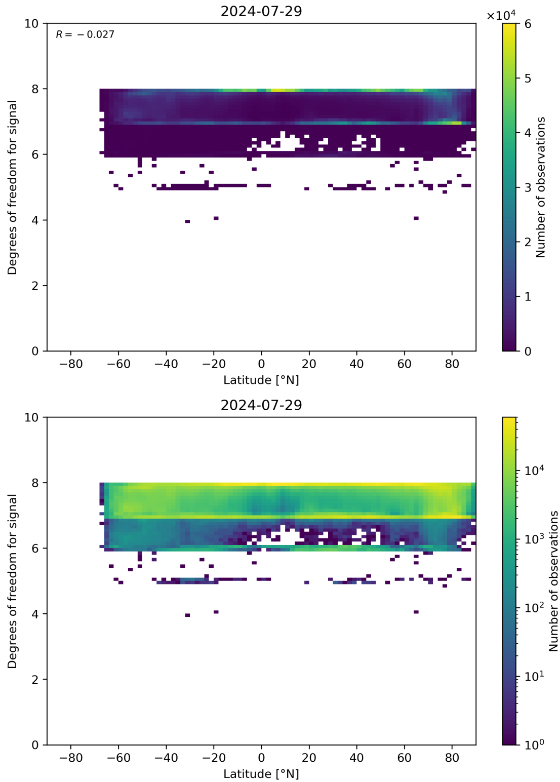
Figure 55: Scatter density plot of “Latitude” against “Degrees of freedom for signal” for 2024-07-28 to 2024-07-30.
