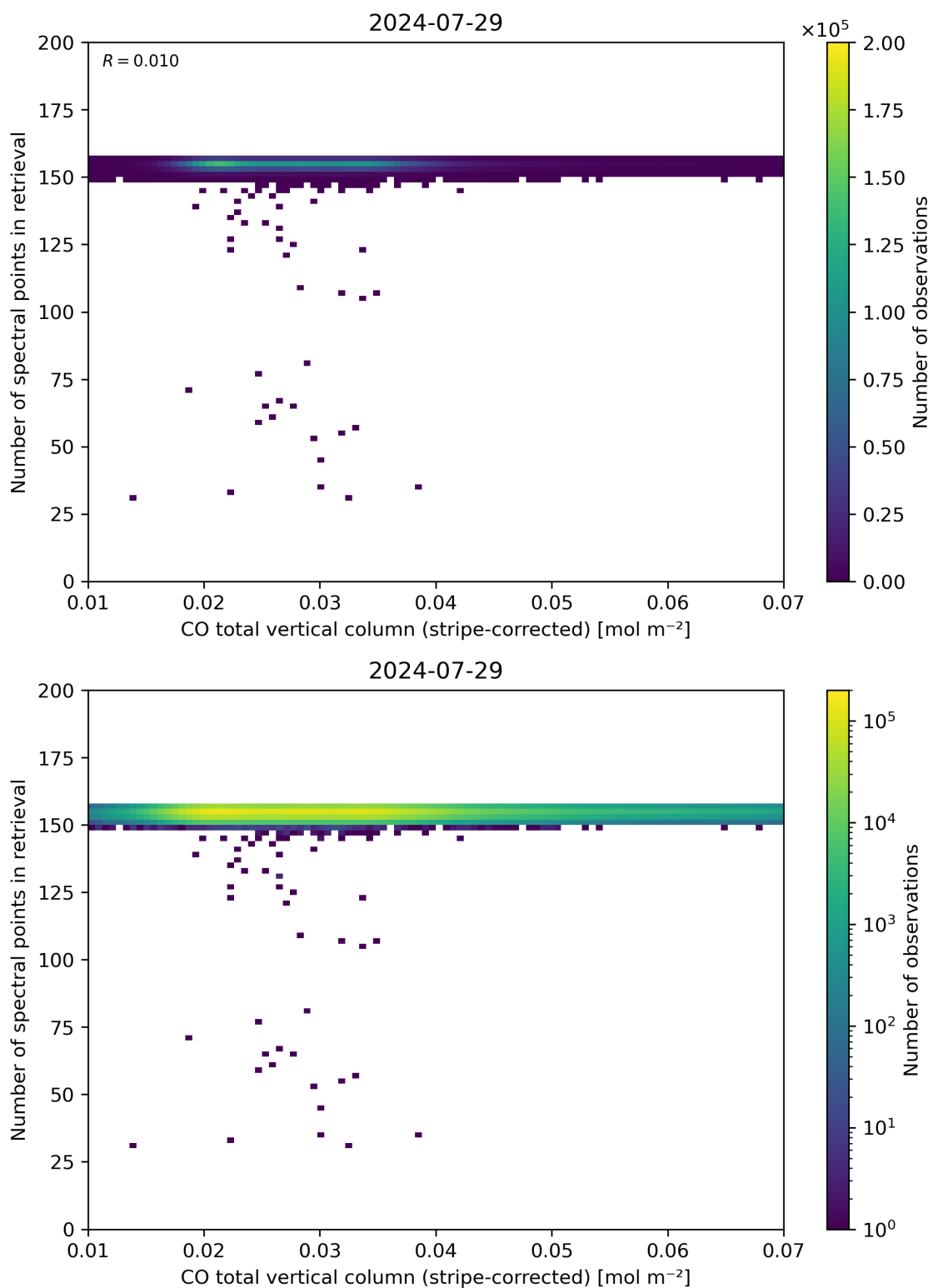
Figure 40: Scatter density plot of “CO total vertical column (stripe-corrected)” against “Number of spectral points in retrieval” for 2024-07-28 to 2024-07-30.
