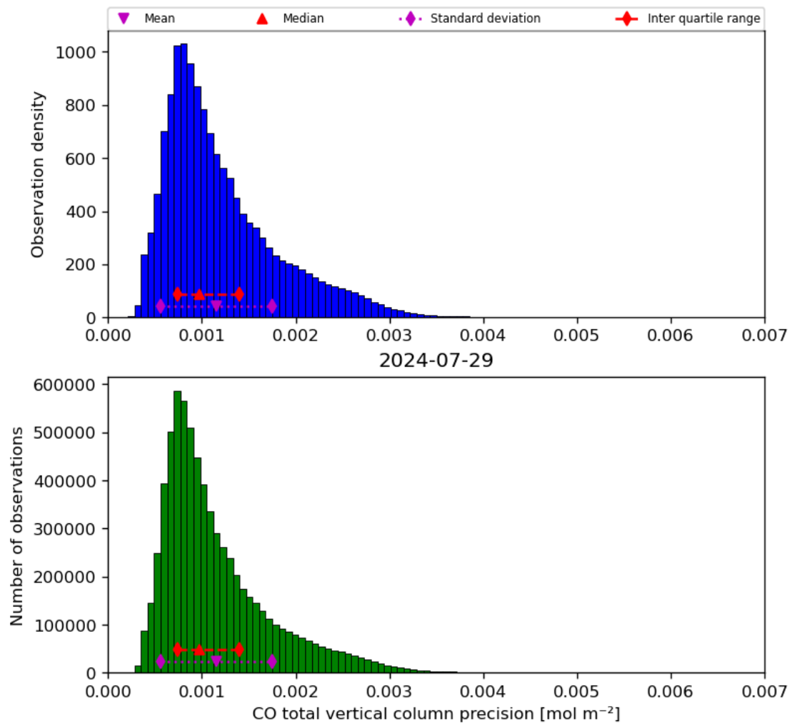
Figure 20: Histogram of “CO total vertical column precision” for 2024-07-28 to 2024-07-30
