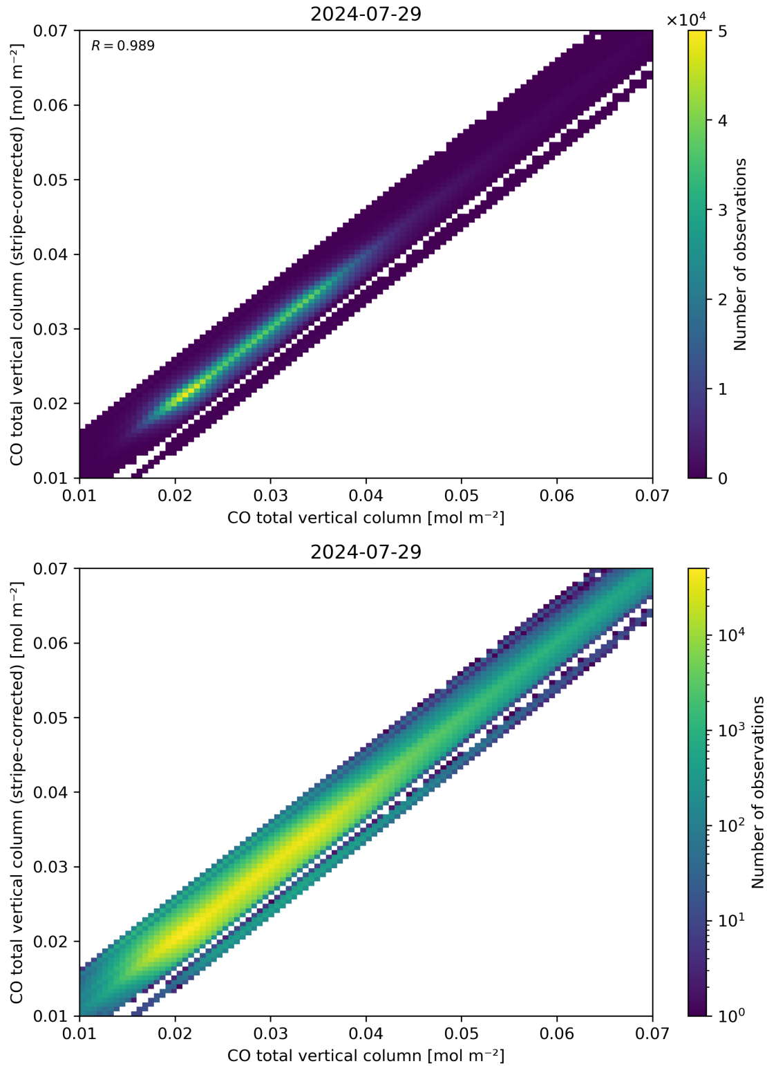
Figure 33: Scatter density plot of “CO total vertical column” against “CO total vertical column (stripe-corrected)” for 2024-07-28 to 2024-07-30.
