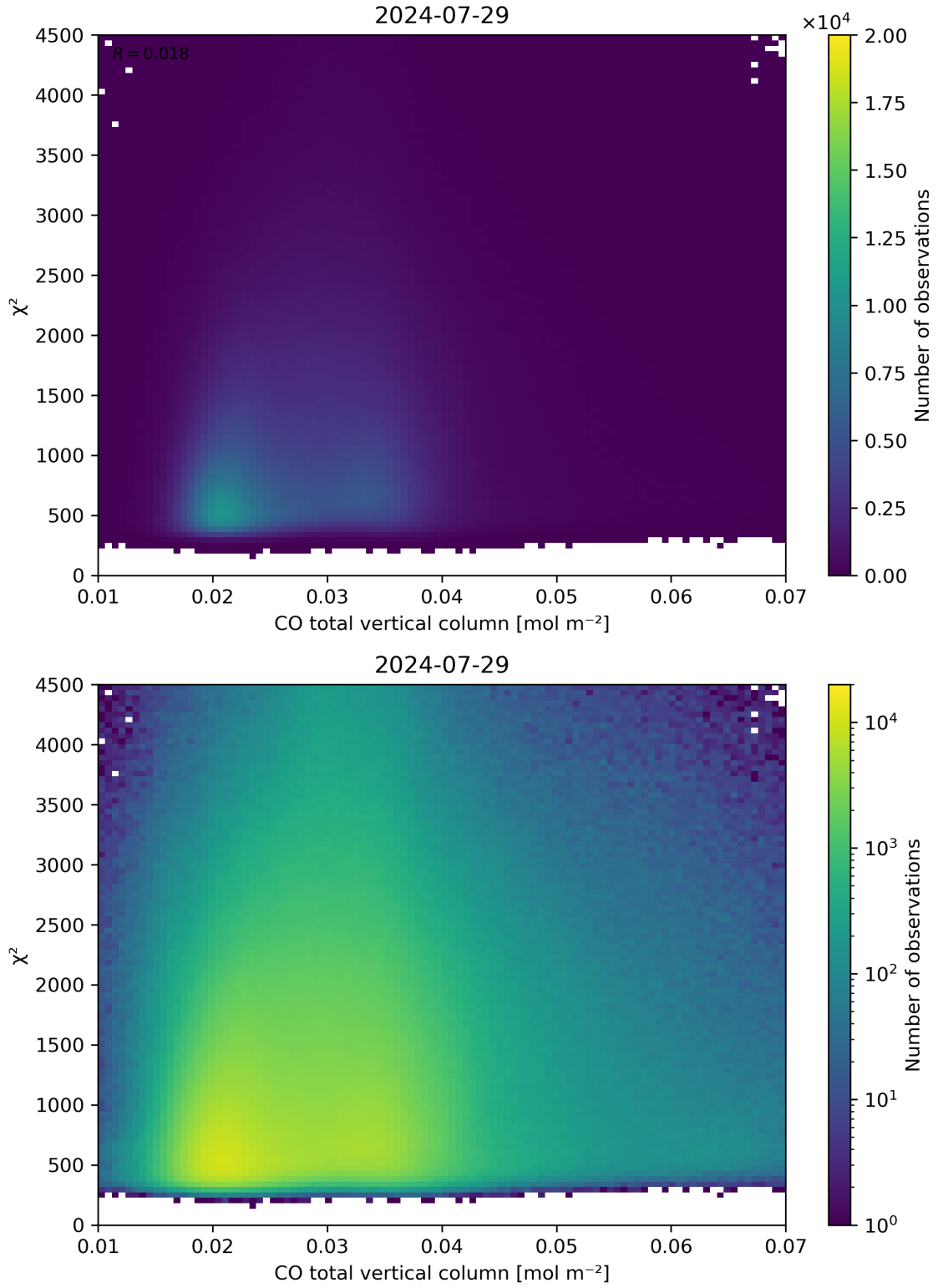
Figure 35: Scatter density plot of “CO total vertical column” against “ \chi^2 ” for 2024-07-28 to 2024-07-30.
