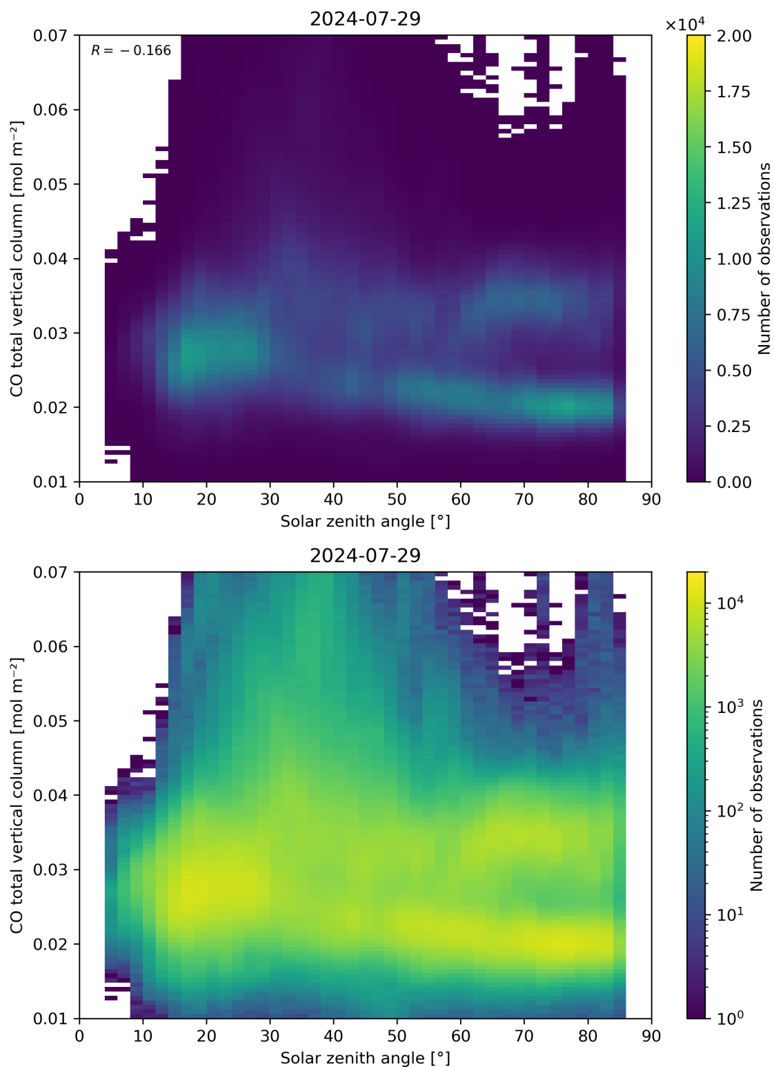
Figure 61: Scatter density plot of “Solar zenith angle” against “CO total vertical column” for 2024-07-28 to 2024-07-30.
