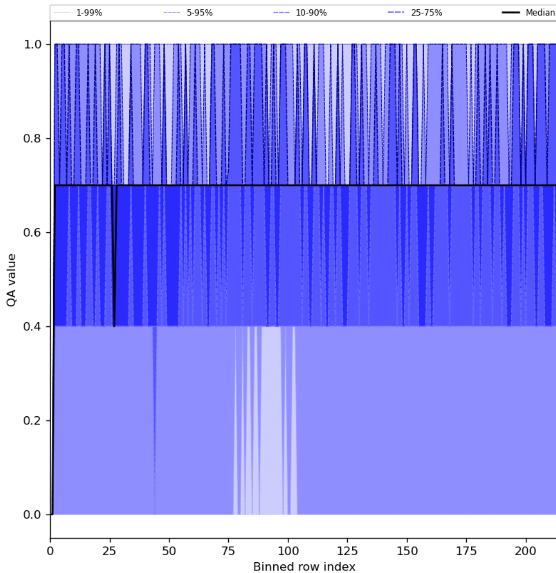
Figure 25: Along track statistics of “QA value” for 2024-07-28 to 2024-07-30
