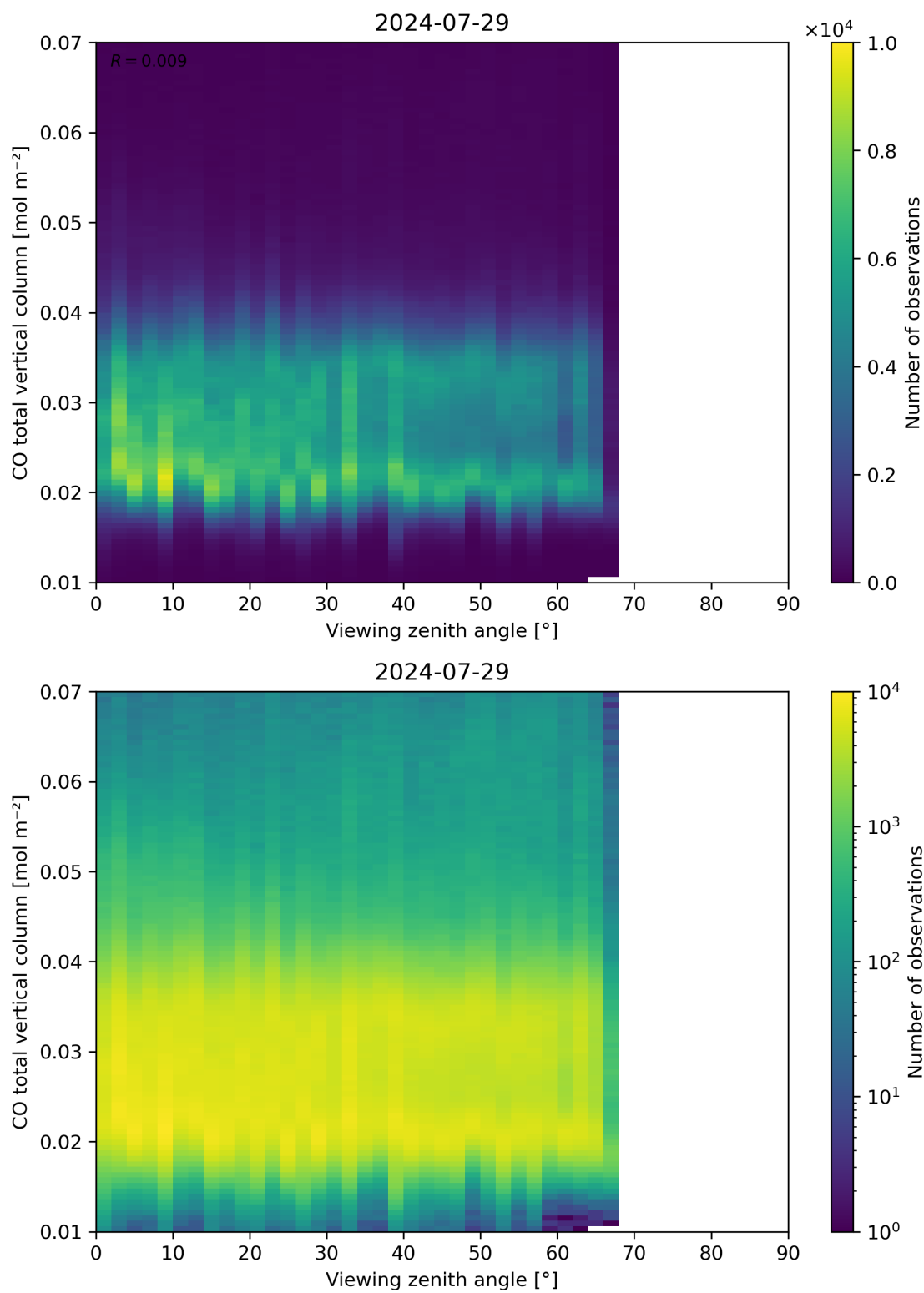
Figure 69: Scatter density plot of “Viewing zenith angle” against “CO total vertical column” for 2024-07-28 to 2024-07-30.
