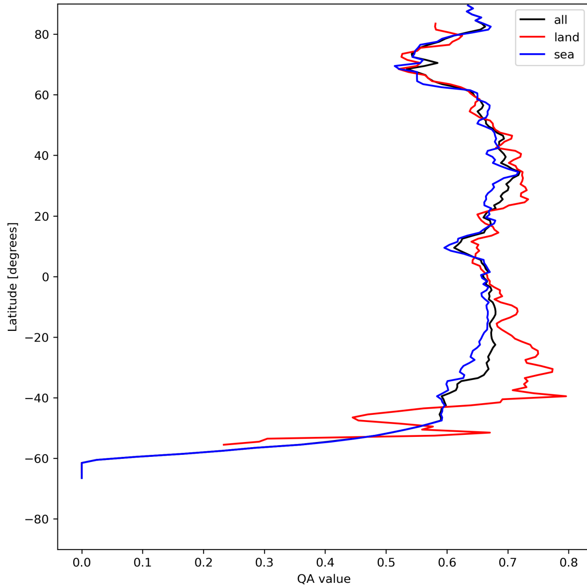
Figure 9: Zonal average of “QA value” for 2024-07-28 to 2024-07-30.
