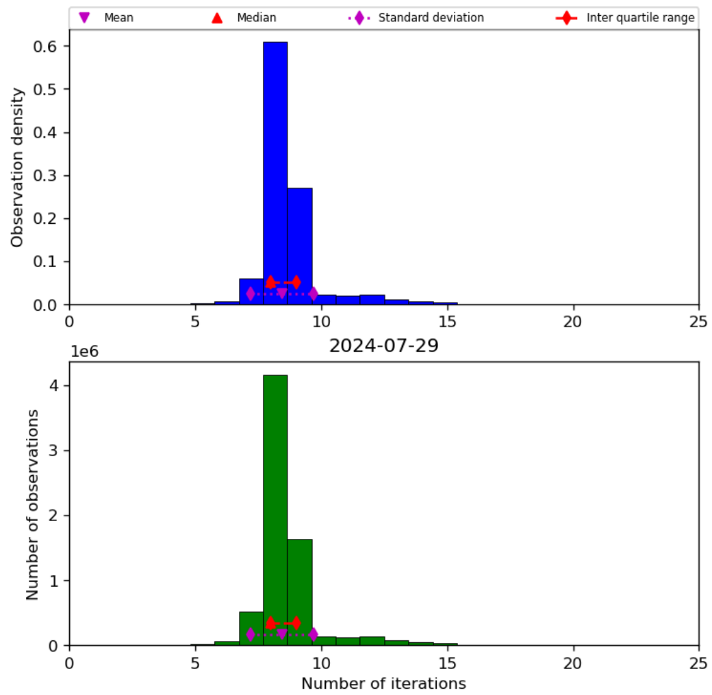
Figure 24: Histogram of “Number of iterations” for 2024-07-28 to 2024-07-30
