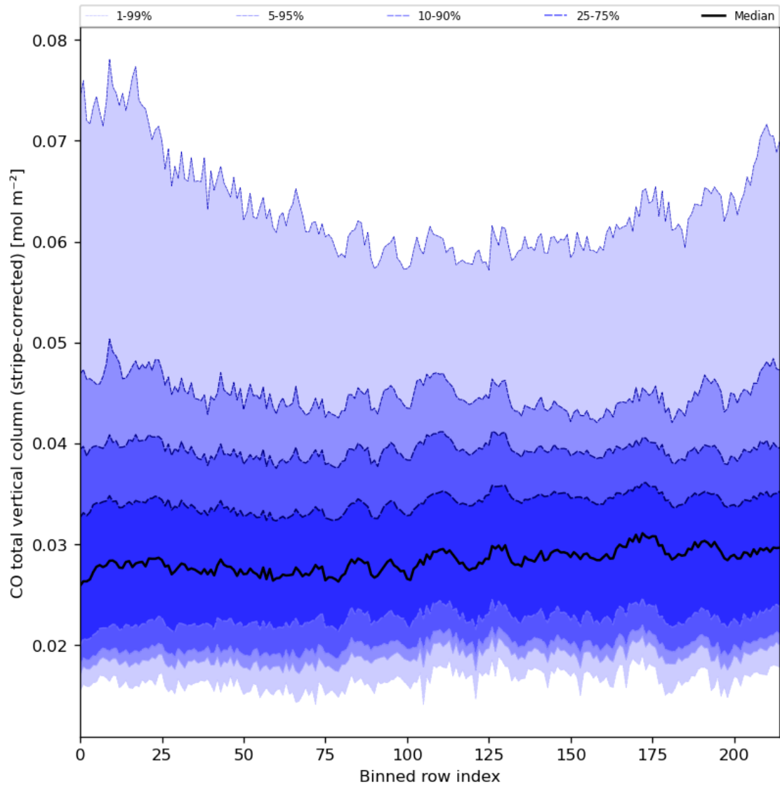
Figure 27: Along track statistics of “CO total vertical column (stripe-corrected)” for 2024-07-28 to 2024-07-30
