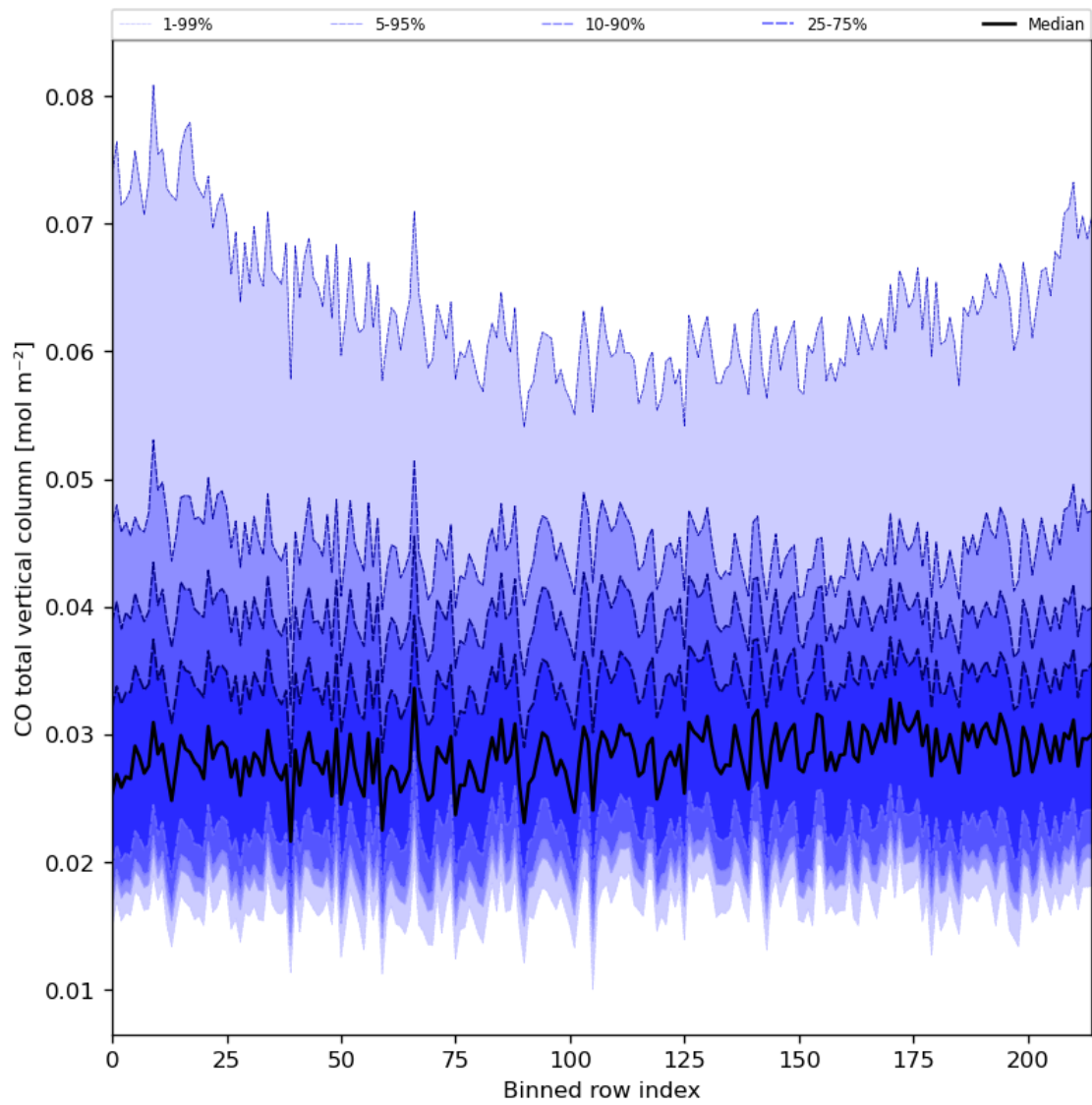
Figure 26: Along track statistics of “CO total vertical column” for 2024-07-28 to 2024-07-30
