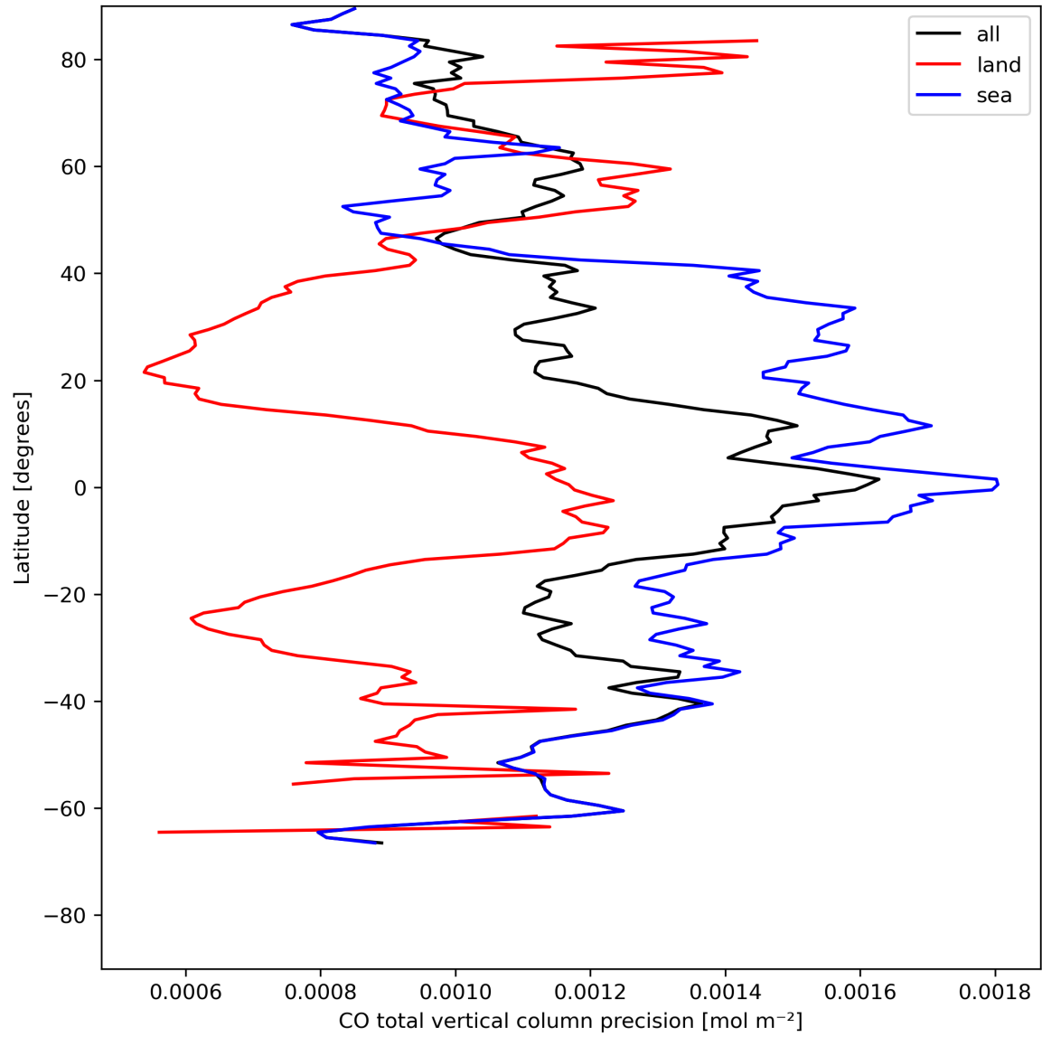
Figure 12: Zonal average of “CO total vertical column precision” for 2024-07-28 to 2024-07-30.
