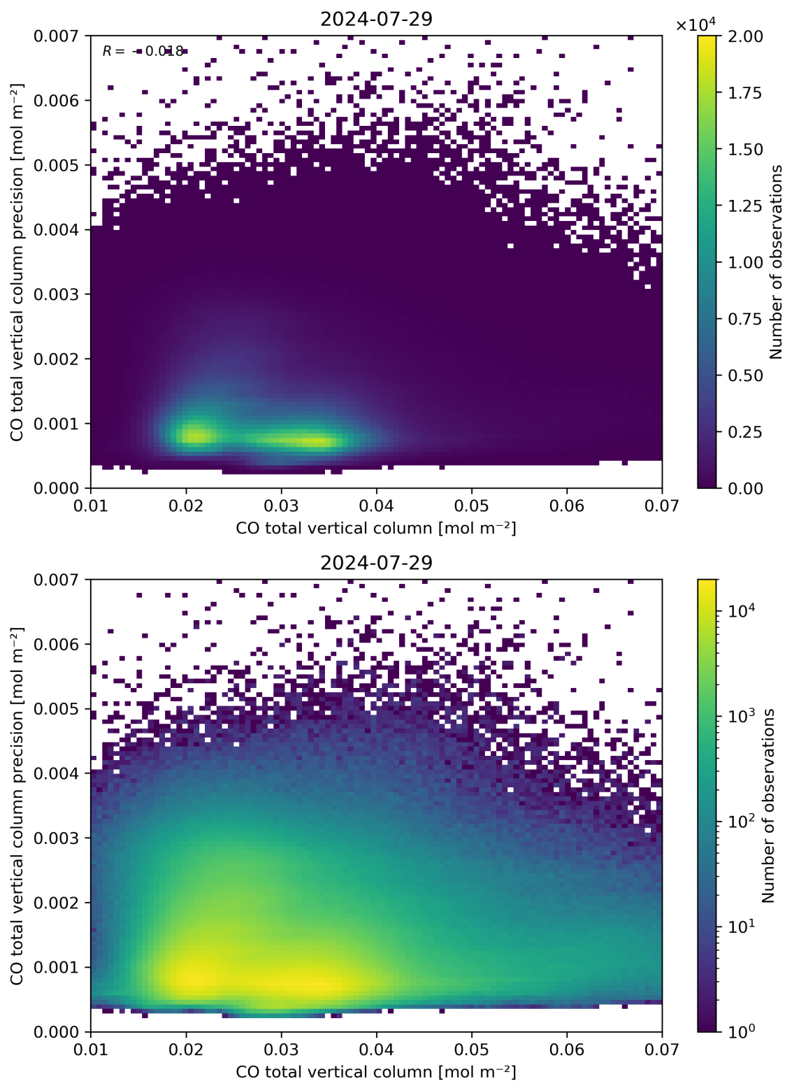
Figure 34: Scatter density plot of “CO total vertical column” against “CO total vertical column precision” for 2024-07-28 to 2024-07-30.
