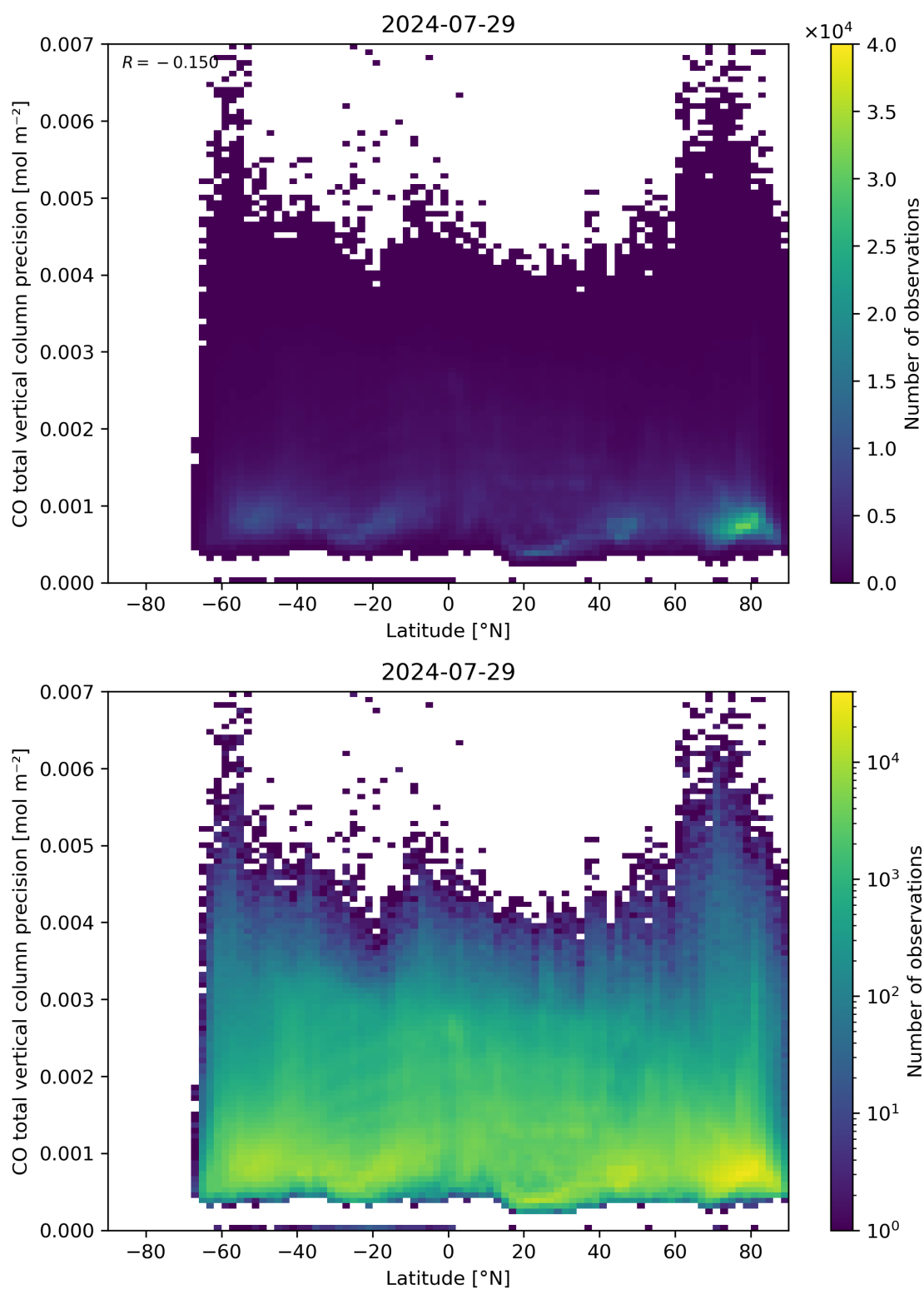
Figure 53: Scatter density plot of “Latitude” against “CO total vertical column precision” for 2024-07-28 to 2024-07-30.
