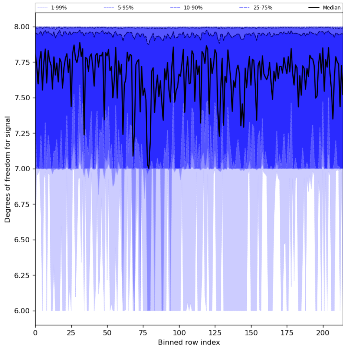
Figure 31: Along track statistics of “Degrees of freedom for signal” for 2024-07-28 to 2024-07-30
