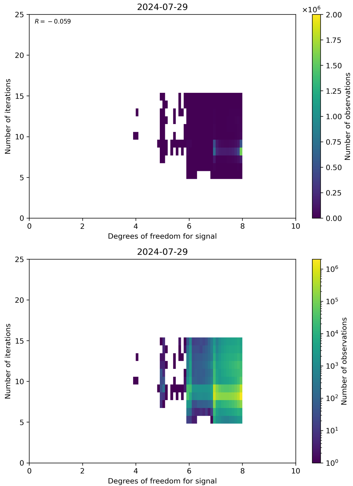
Figure 50: Scatter density plot of “Degrees of freedom for signal” against “Number of iterations” for 2024-07-28 to 2024-07-30.
