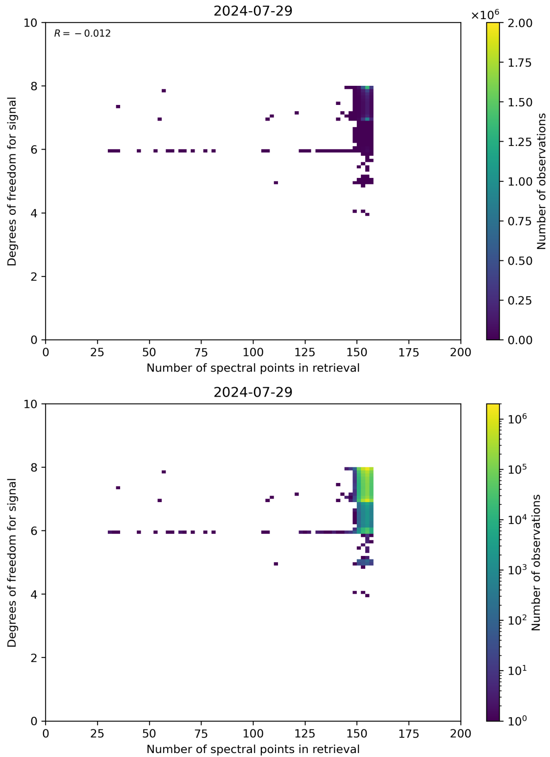
Figure 59: Scatter density plot of “Number of spectral points in retrieval” against “Degrees of freedom for signal” for 2024-07-28 to 2024-07-30.
