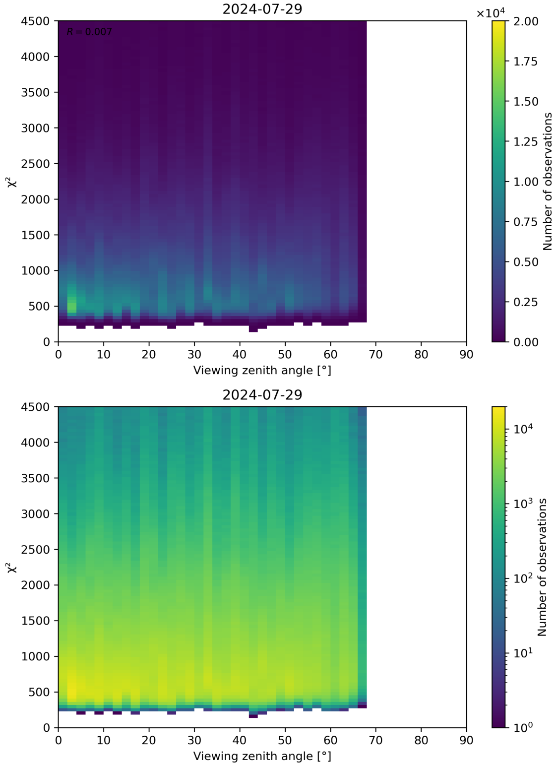
Figure 72: Scatter density plot of “Viewing zenith angle” against “ \chi^2 ” for 2024-07-28 to 2024-07-30.
