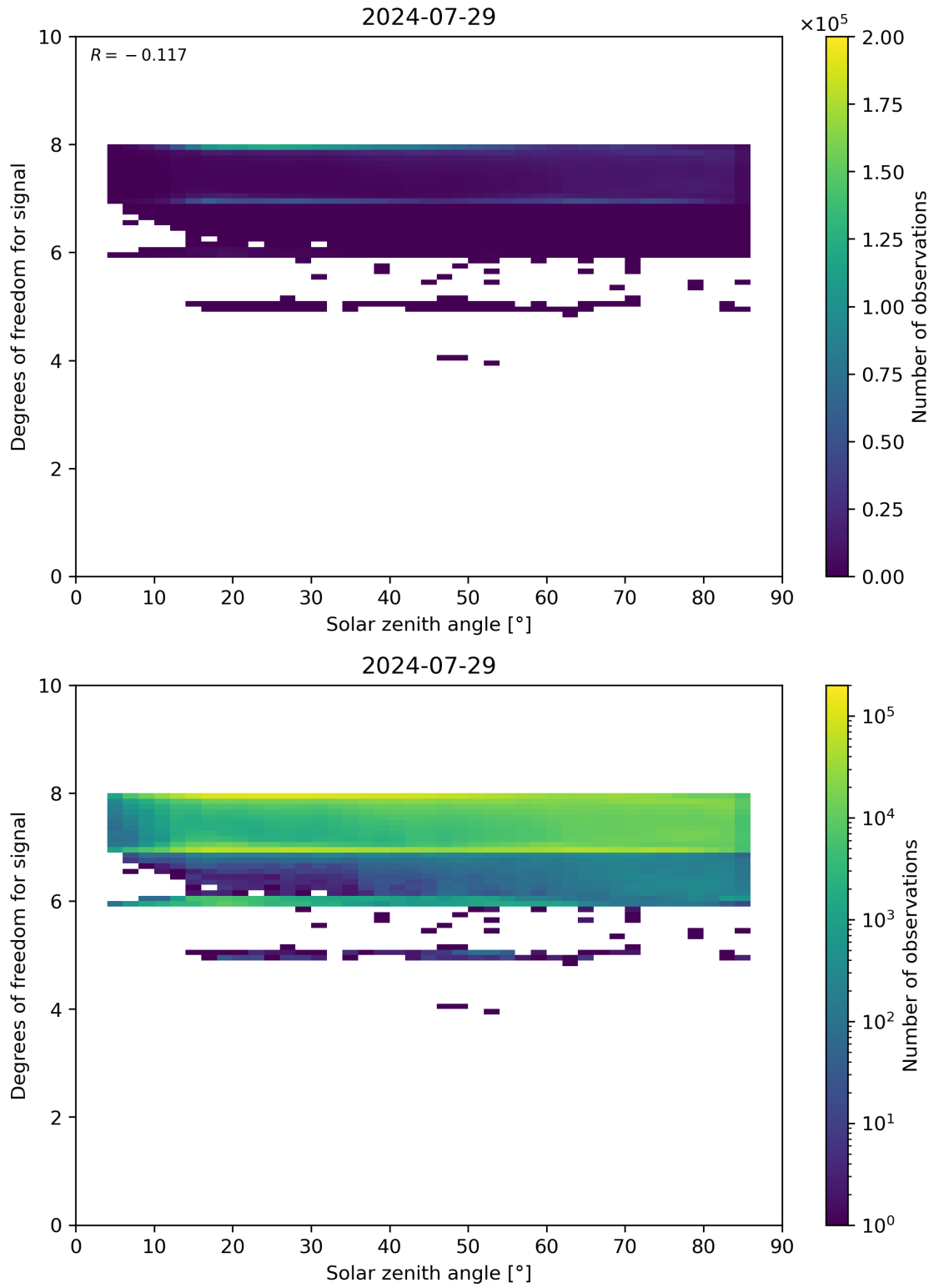
Figure 65: Scatter density plot of “Solar zenith angle” against “Degrees of freedom for signal” for 2024-07-28 to 2024-07-30.
