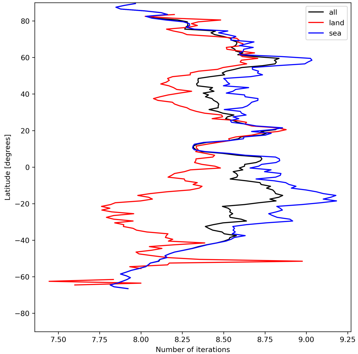
Figure 16: Zonal average of “Number of iterations” for 2024-07-28 to 2024-07-30.
