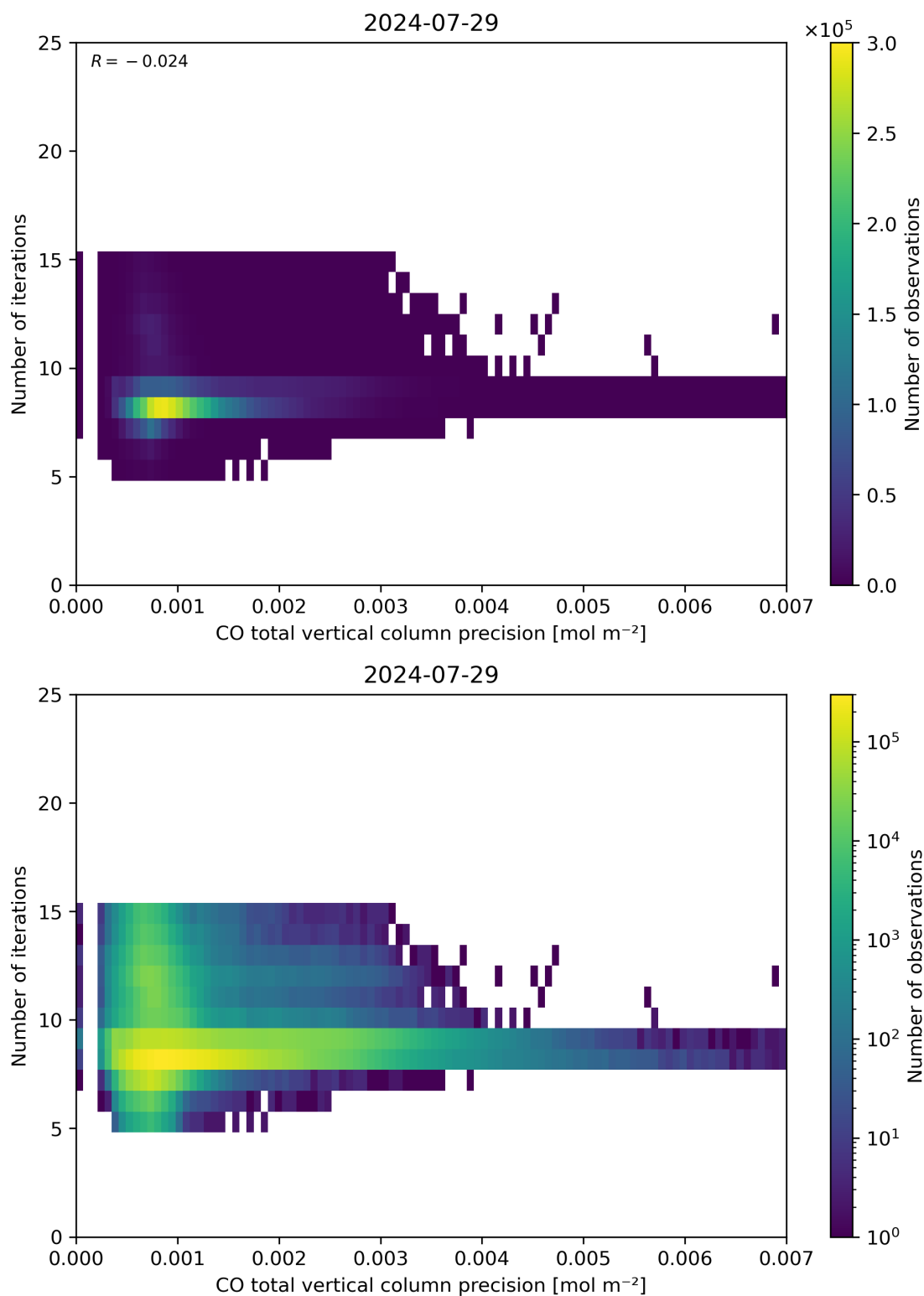
Figure 46: Scatter density plot of “CO total vertical column precision” against “Number of iterations” for 2024-07-28 to 2024-07-30.
