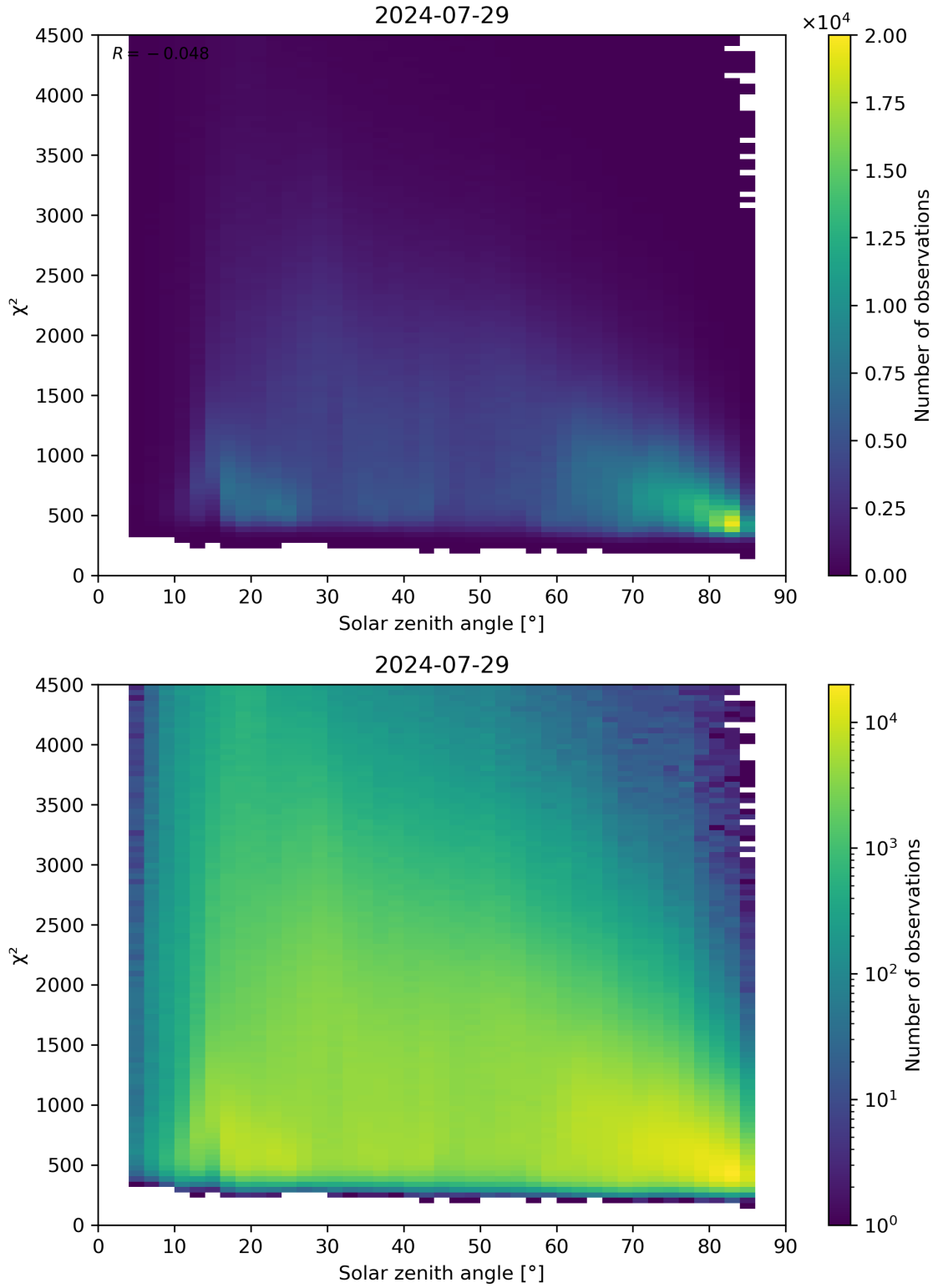
Figure 64: Scatter density plot of “Solar zenith angle” against “ \chi^2 ” for 2024-07-28 to 2024-07-30.
