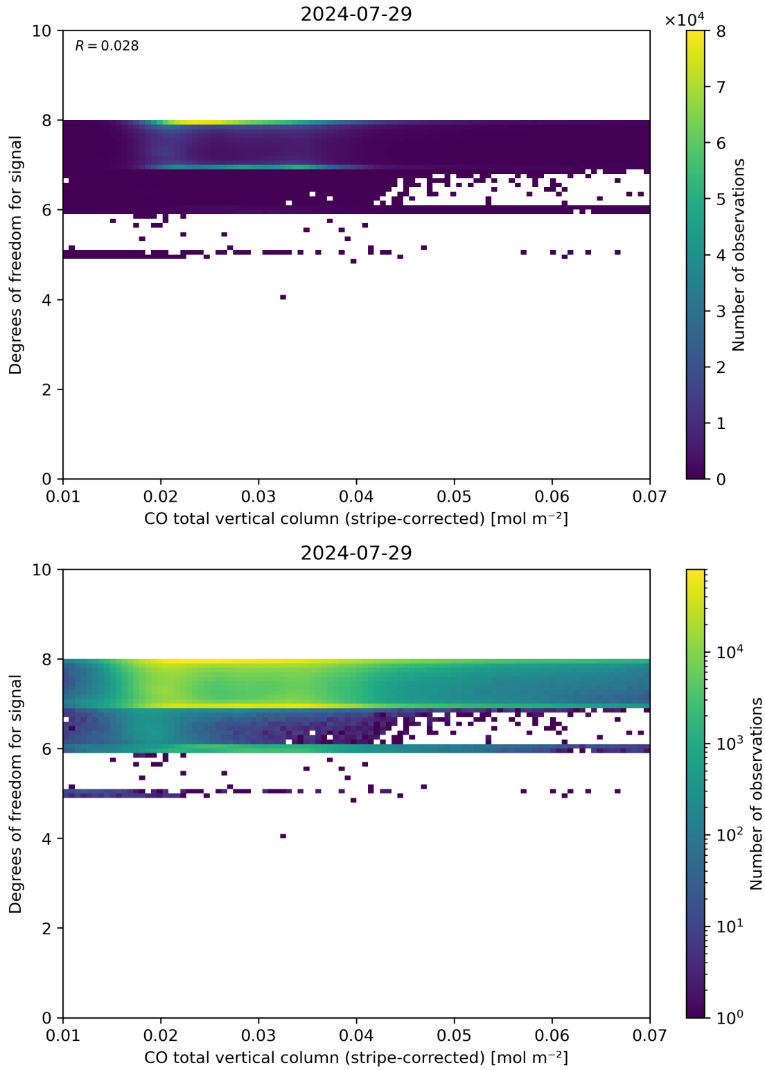
Figure 38: Scatter density plot of “CO total vertical column (stripe-corrected)” against “Degrees of freedom for signal” for 2024-07-28 to 2024-07-30.
