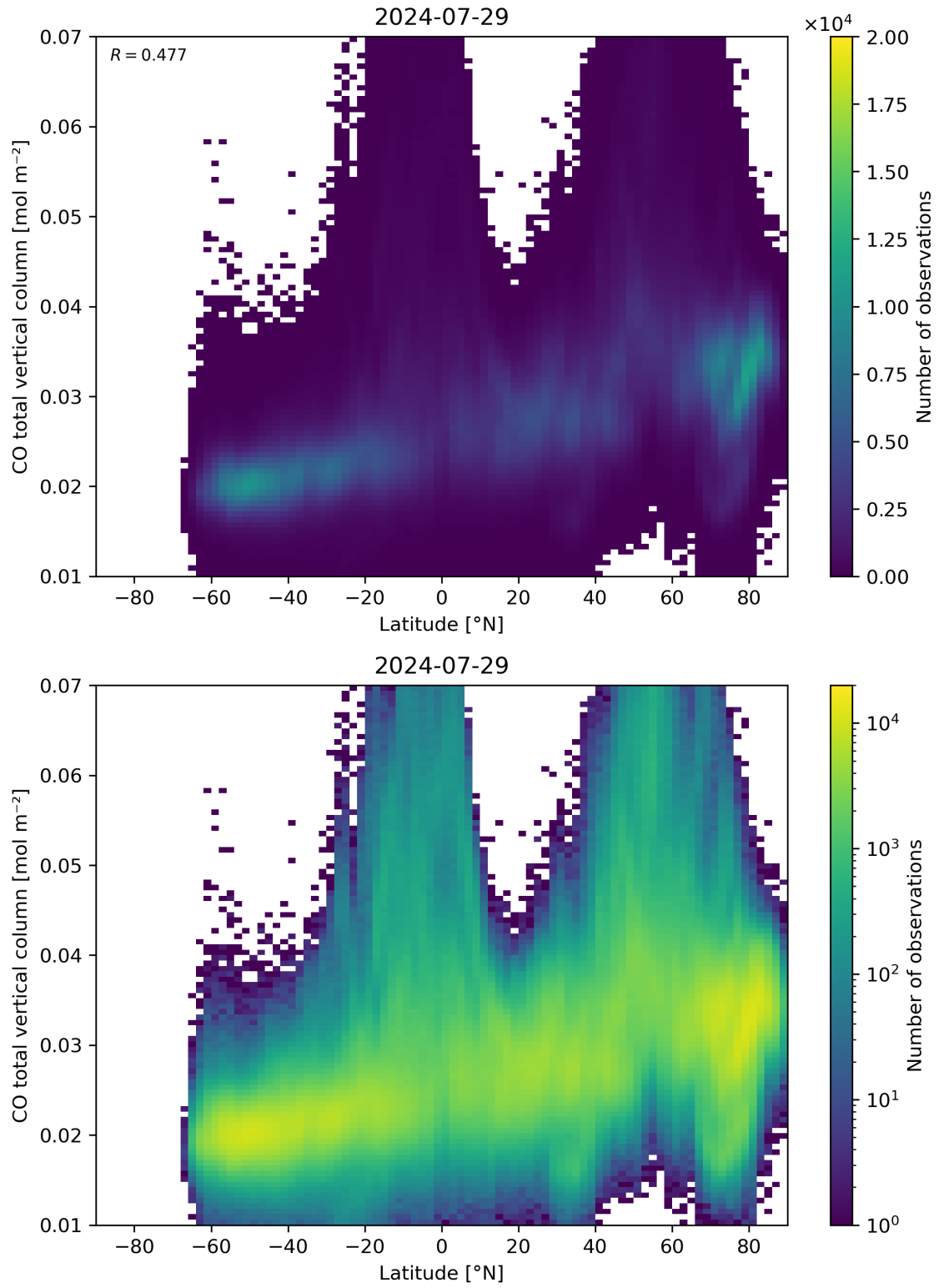
Figure 51: Scatter density plot of “Latitude” against “CO total vertical column” for 2024-07-28 to 2024-07-30.
