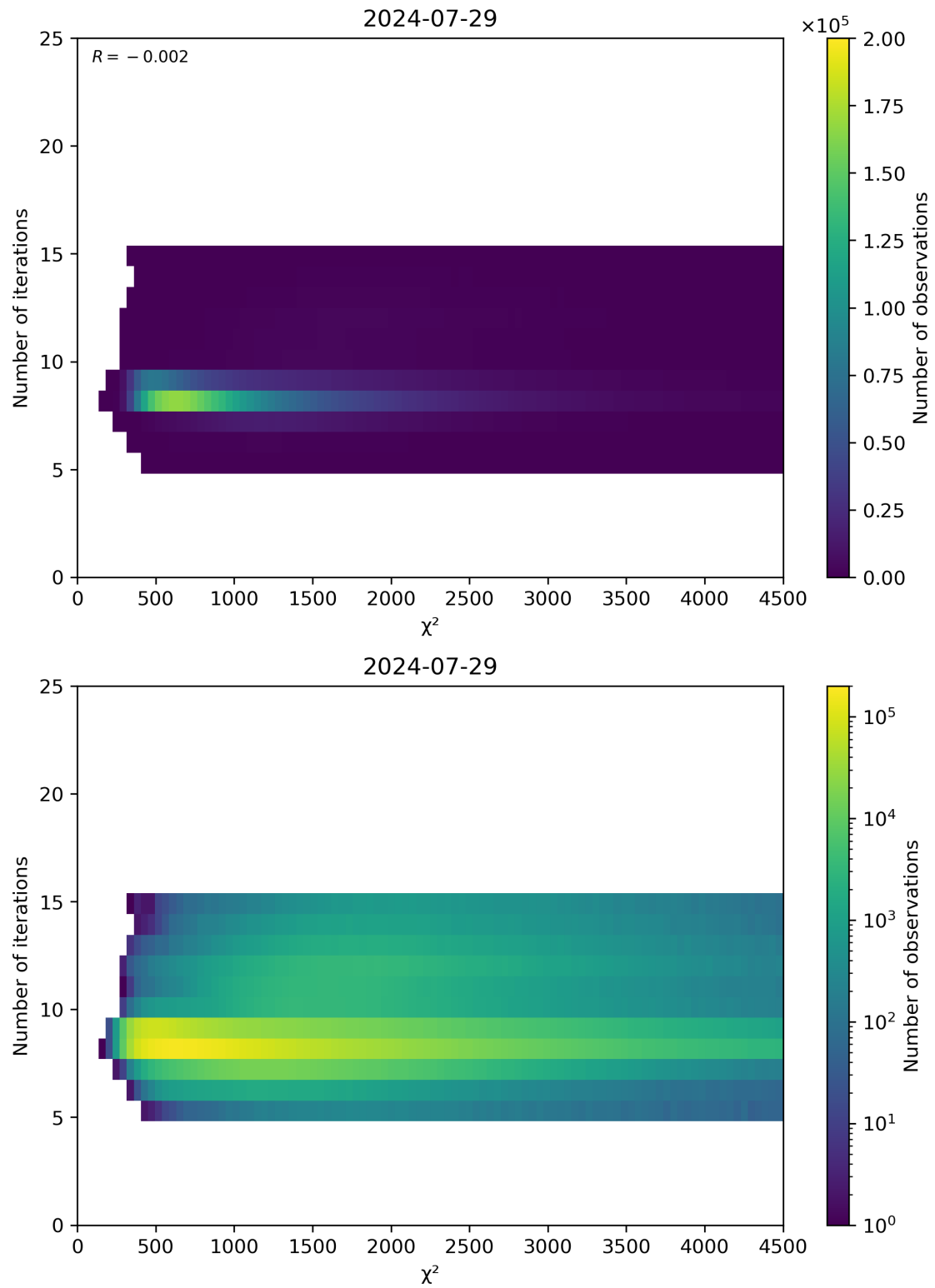
Figure 49: Scatter density plot of “ \chi^2 ” against “Number of iterations” for 2024-07-28 to 2024-07-30.
