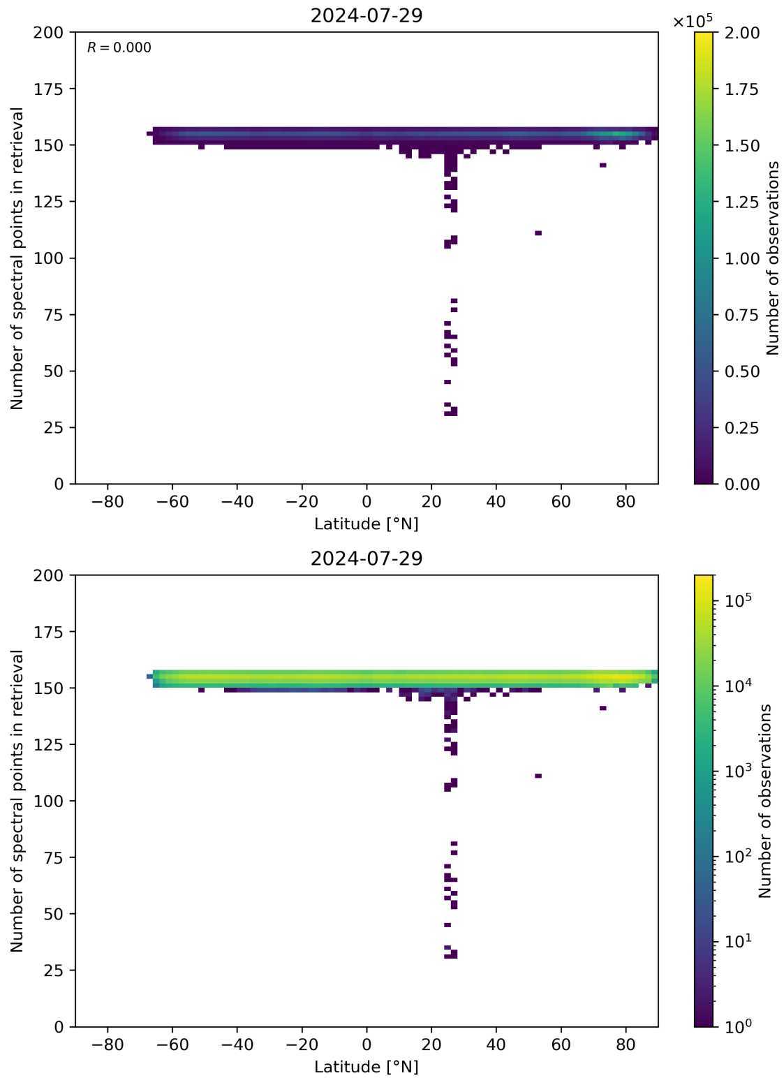
Figure 57: Scatter density plot of “Latitude” against “Number of spectral points in retrieval” for 2024-07-28 to 2024-07-30.
