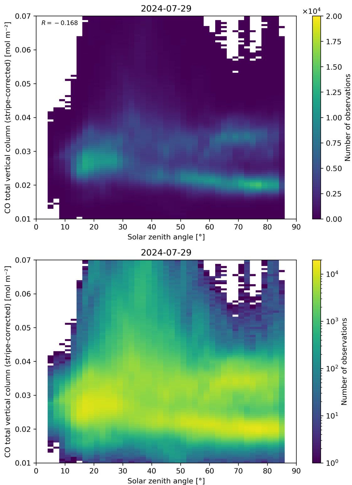
Figure 62: Scatter density plot of “Solar zenith angle” against “CO total vertical column (stripe-corrected)” for 2024-07-28 to 2024-07-30.
