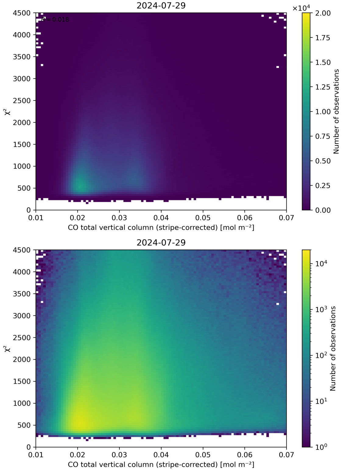
Figure 37: Scatter density plot of “CO total vertical column (stripe-corrected)” against “ \chi^2 ” for 2024-07-28 to 2024-07-30.
