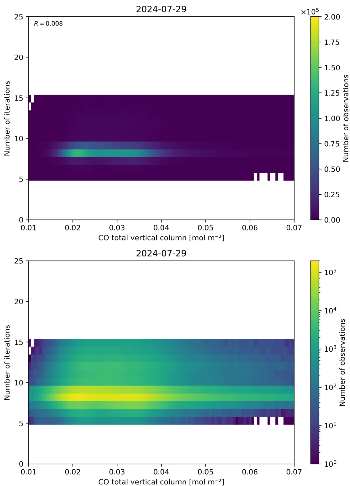
Figure 42: Scatter density plot of “CO total vertical column” against “Number of iterations” for 2024-07-28 to 2024-07-30.
