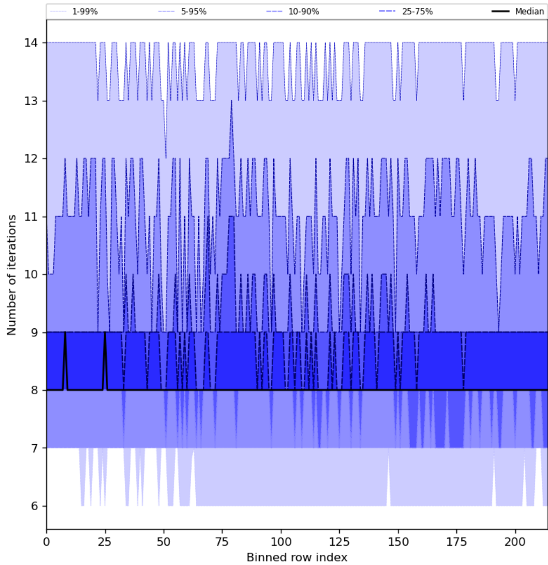
Figure 32: Along track statistics of “Number of iterations” for 2024-07-28 to 2024-07-30
