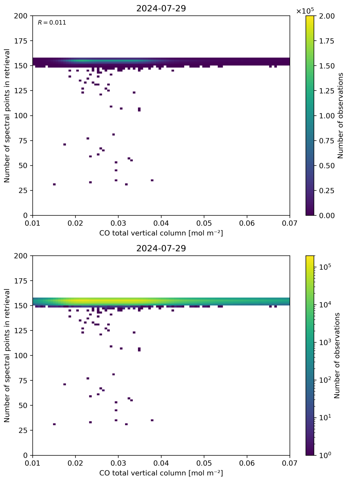
Figure 43: Scatter density plot of “CO total vertical column” against “Number of spectral points in retrieval” for 2024-07-28 to 2024-07-30.
