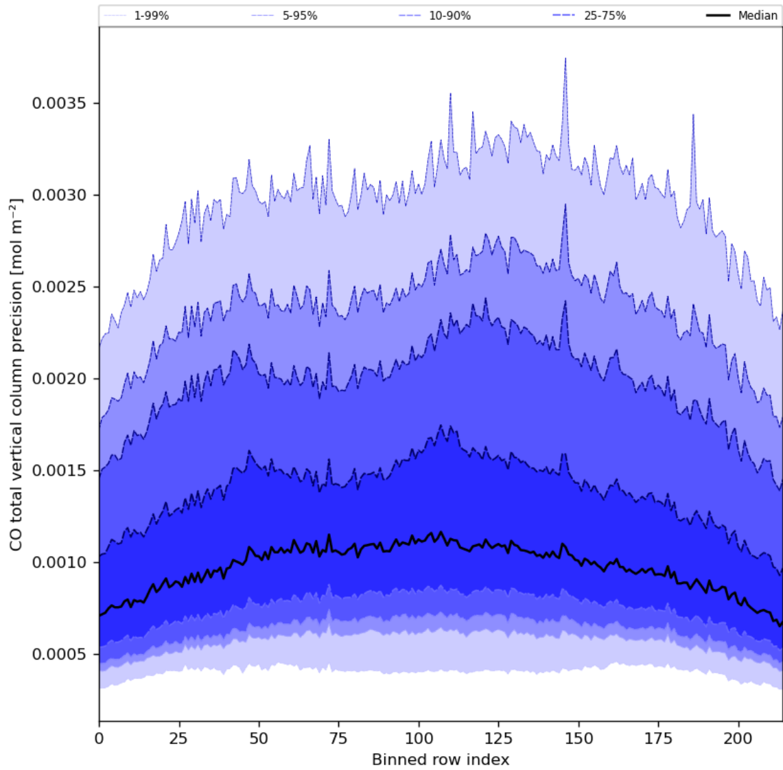
Figure 28: Along track statistics of “CO total vertical column precision” for 2024-07-28 to 2024-07-30
