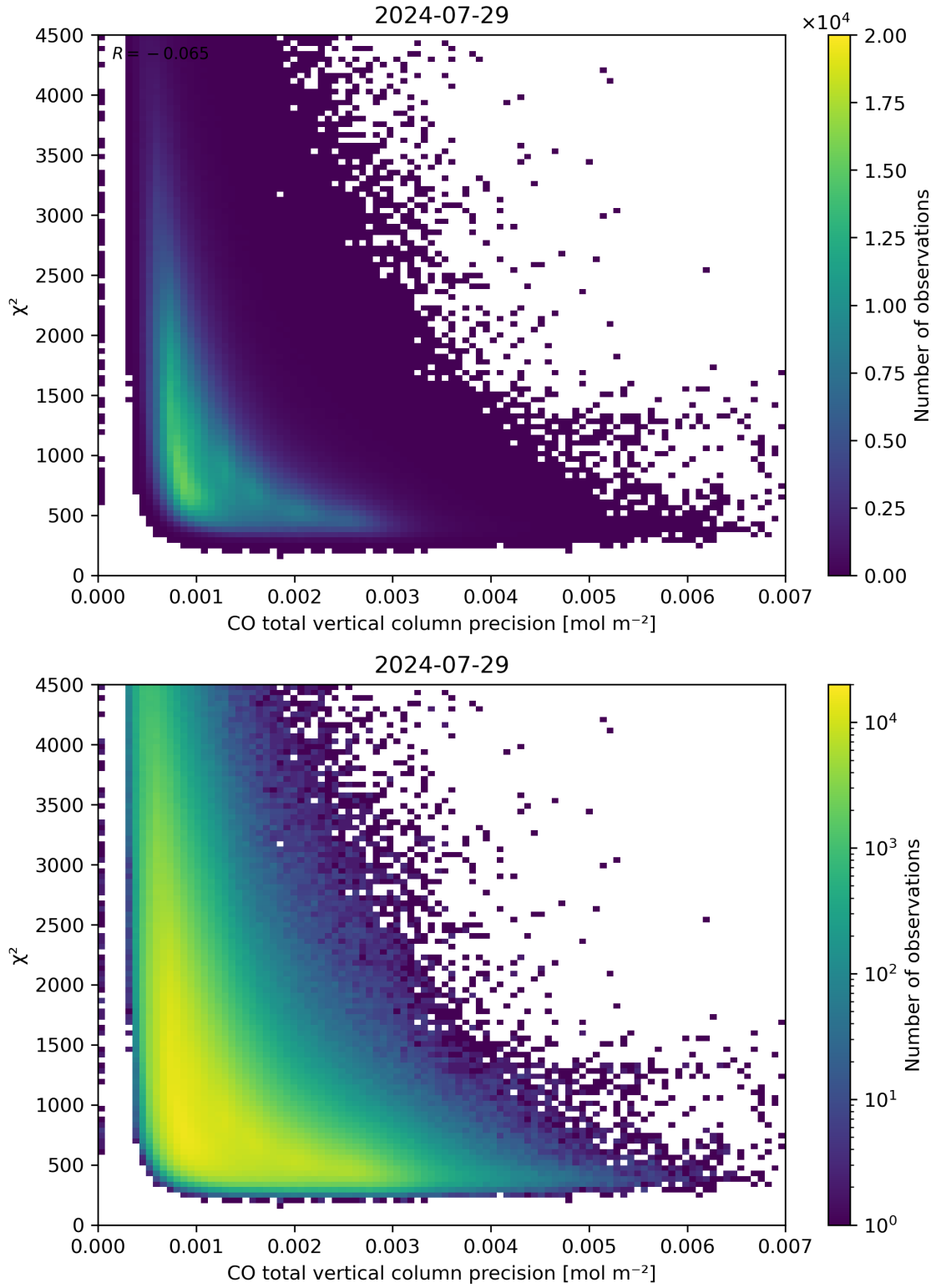
Figure 44: Scatter density plot of “CO total vertical column precision” against “ \chi^2 ” for 2024-07-28 to 2024-07-30.
