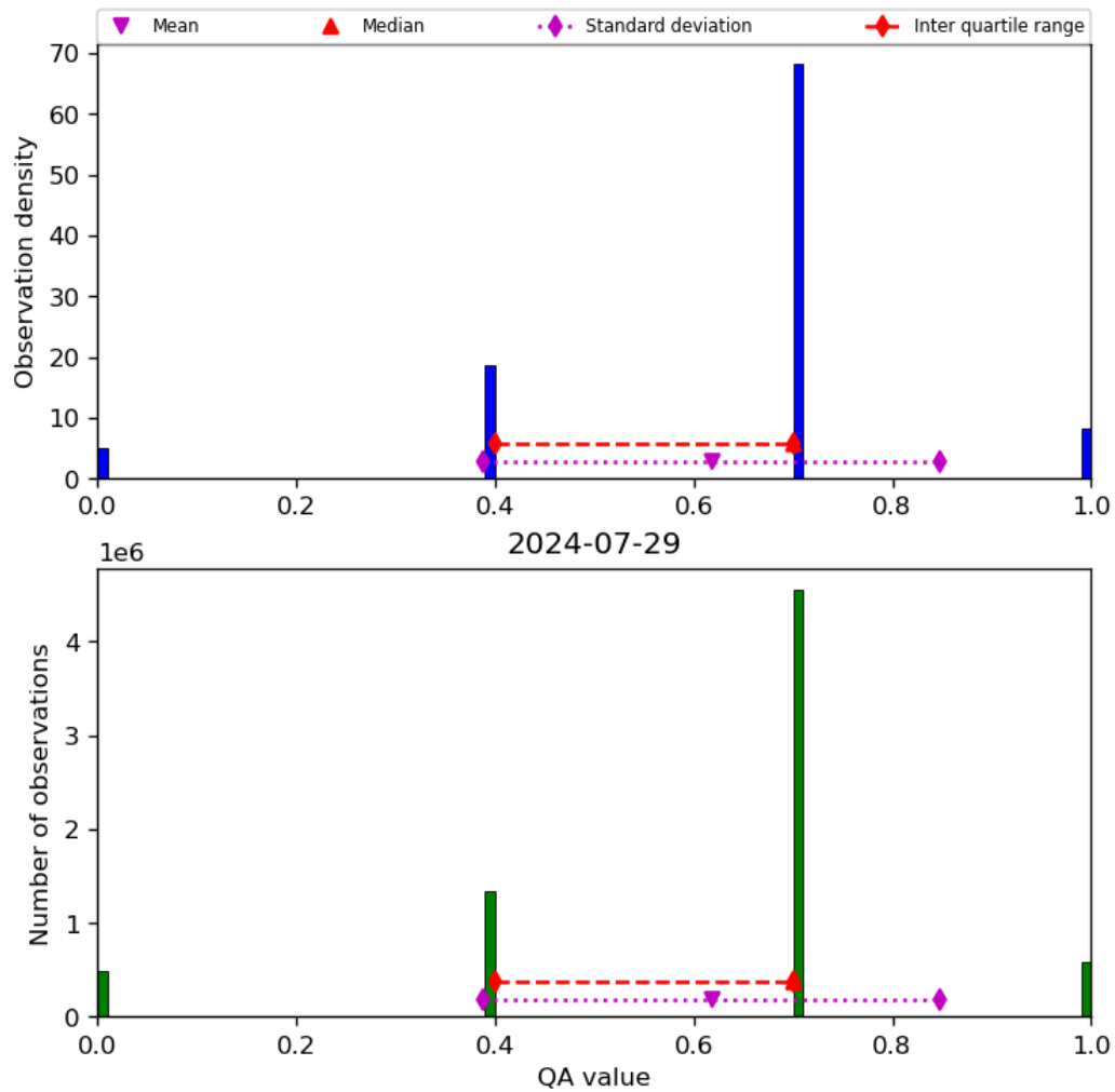
Figure 17: Histogram of “QA value” for 2024-07-28 to 2024-07-30
