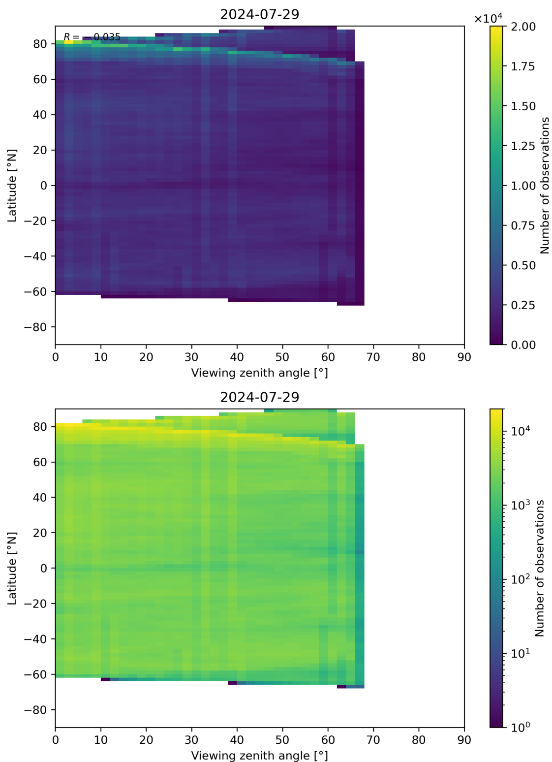
Figure 74: Scatter density plot of “Viewing zenith angle” against “Latitude” for 2024-07-28 to 2024-07-30.
