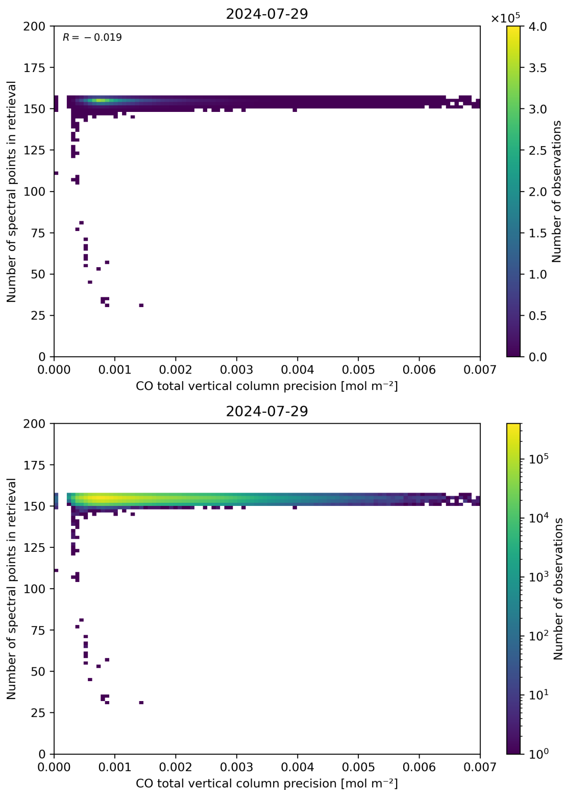
Figure 47: Scatter density plot of “CO total vertical column precision” against “Number of spectral points in retrieval” for 2024-07-28 to 2024-07-30.
