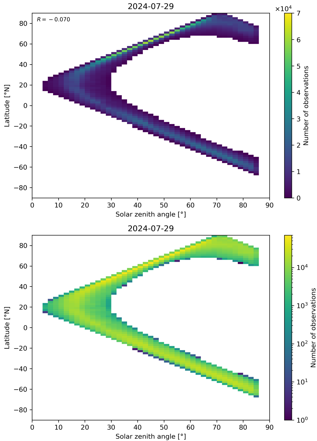
Figure 66: Scatter density plot of “Solar zenith angle” against “Latitude” for 2024-07-28 to 2024-07-30.
