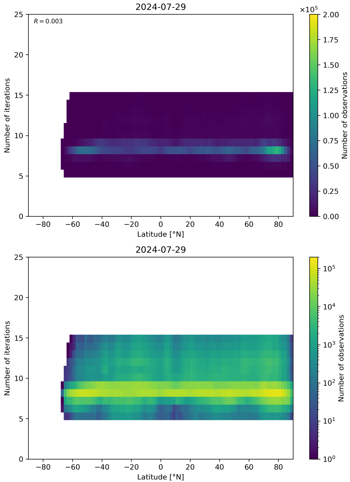
Figure 56: Scatter density plot of “Latitude” against “Number of iterations” for 2024-07-28 to 2024-07-30.
