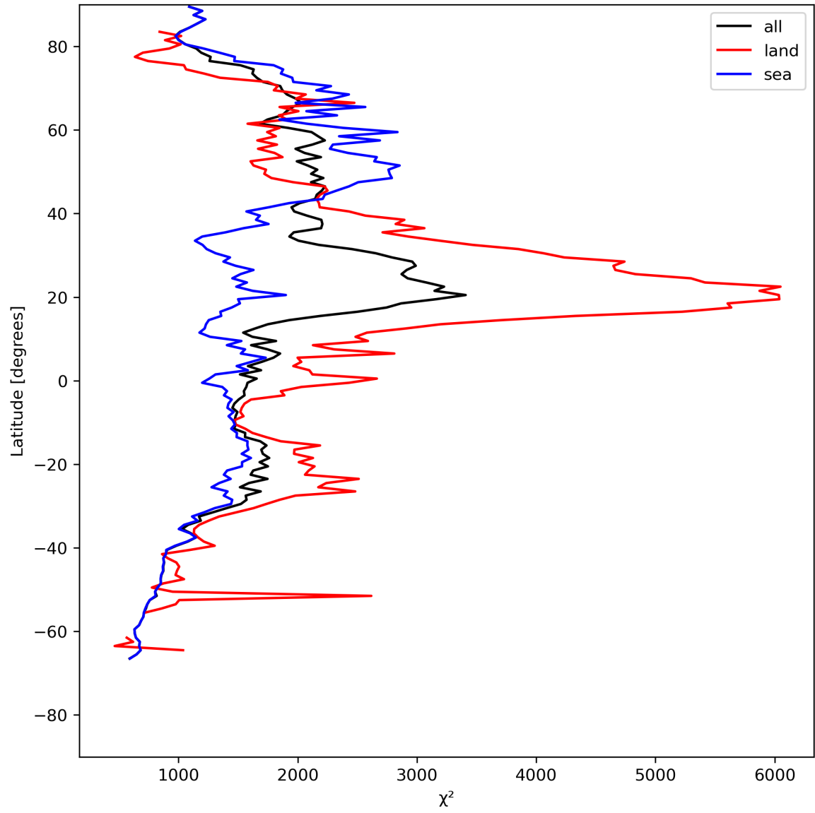
Figure 14: Zonal average of “ \chi^2 ” for 2024-07-28 to 2024-07-30.
