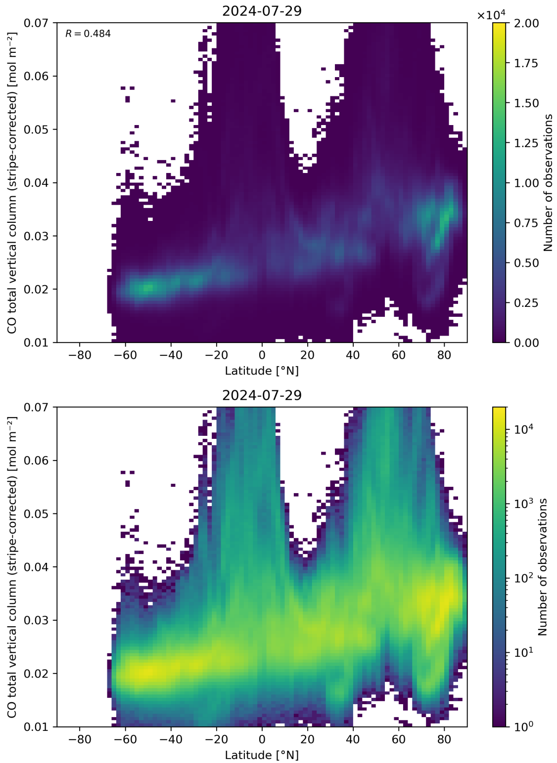
Figure 52: Scatter density plot of “Latitude” against “CO total vertical column (stripe-corrected)” for 2024-07-28 to 2024-07-30.
