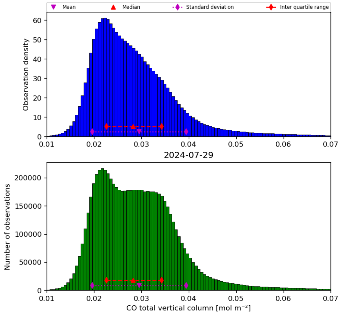
Figure 18: Histogram of “CO total vertical column” for 2024-07-28 to 2024-07-30
