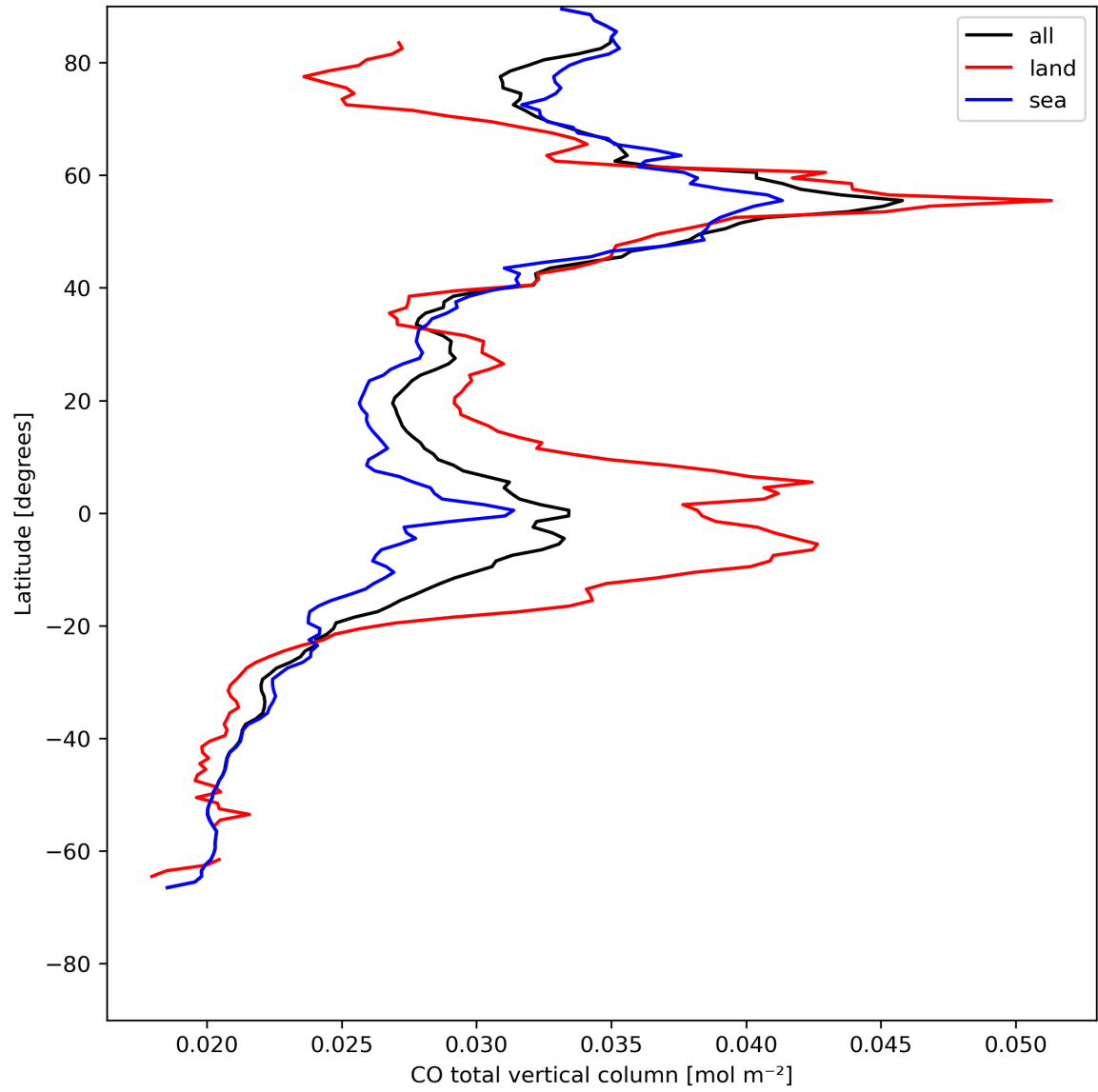
Figure 10: Zonal average of “CO total vertical column” for 2024-07-28 to 2024-07-30.
