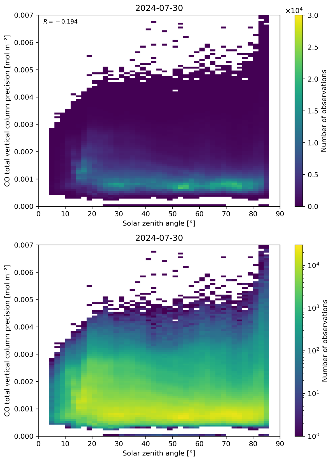
Figure 63: Scatter density plot of “Solar zenith angle” against “CO total vertical column precision” for 2024-07-29 to 2024-07-31.
