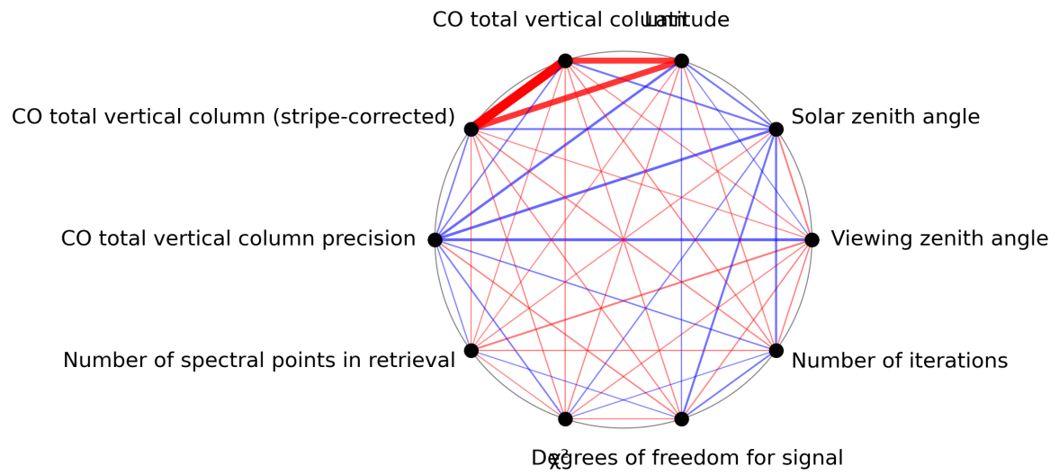
Figure 1: Map of correlation graph for 2024-07-29 to 2024-07-31.
