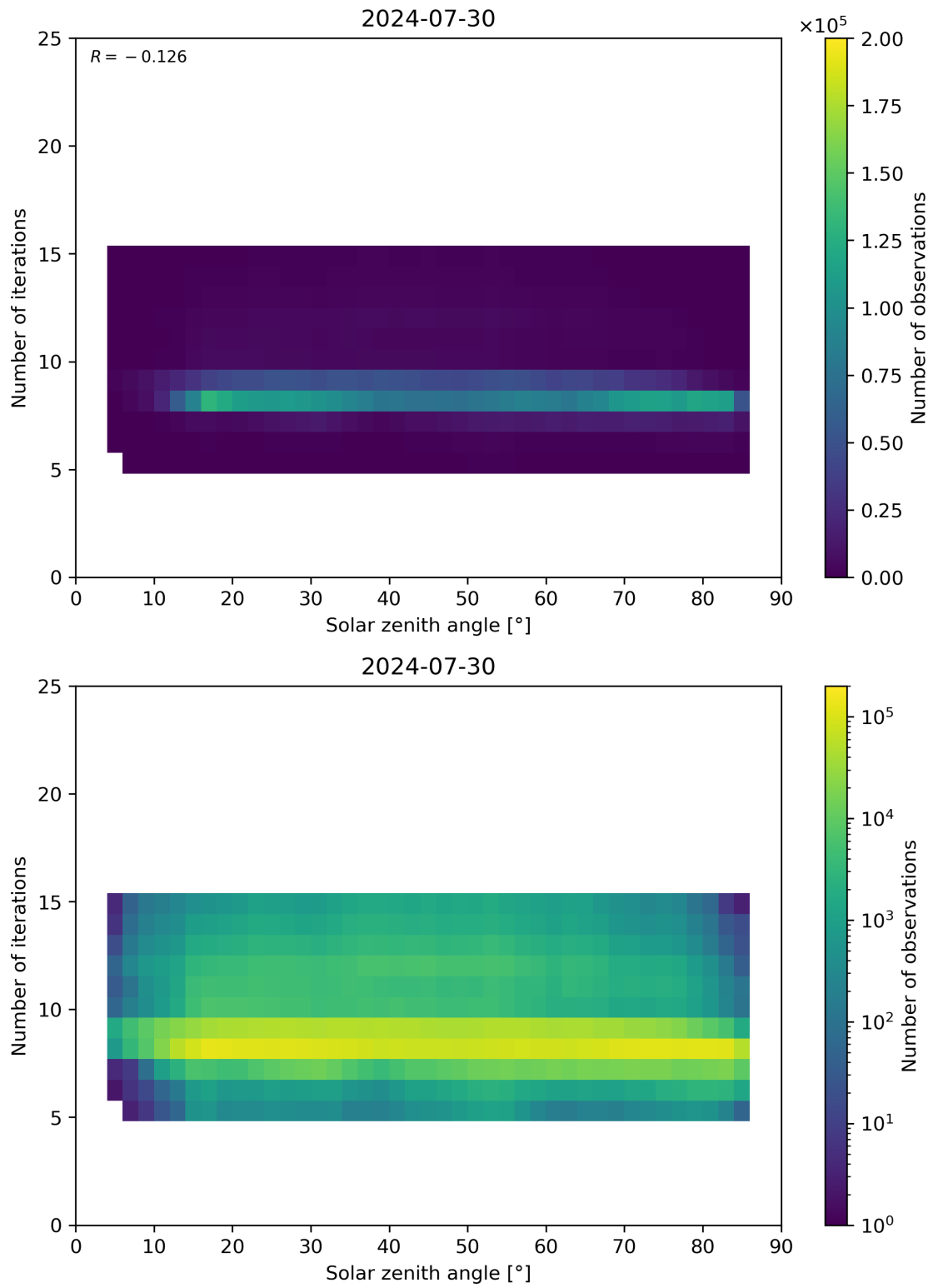
Figure 67: Scatter density plot of “Solar zenith angle” against “Number of iterations” for 2024-07-29 to 2024-07-31.
