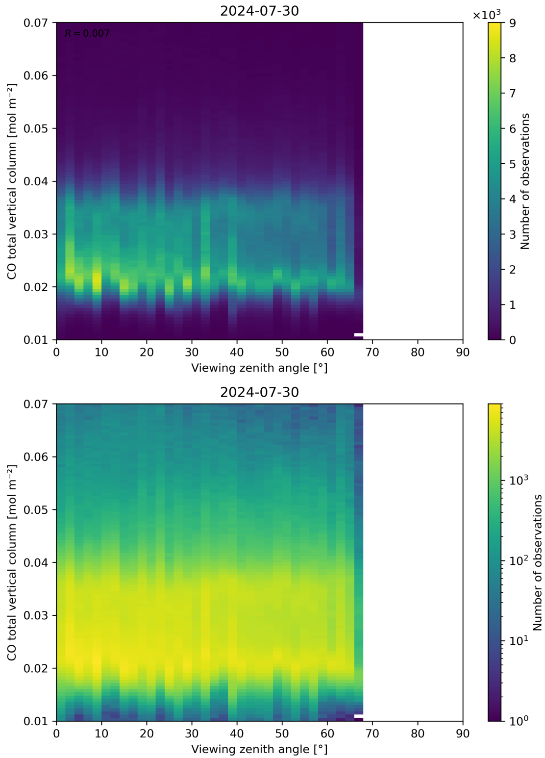
Figure 69: Scatter density plot of “Viewing zenith angle” against “CO total vertical column” for 2024-07-29 to 2024-07-31.
