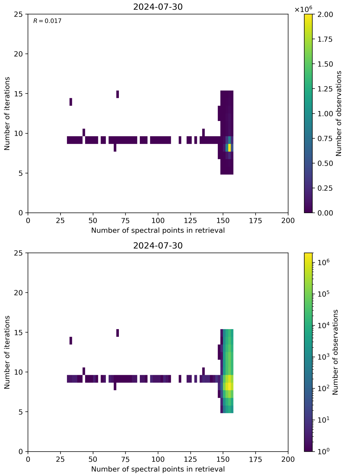
Figure 60: Scatter density plot of “Number of spectral points in retrieval” against “Number of iterations” for 2024-07-29 to 2024-07-31.
