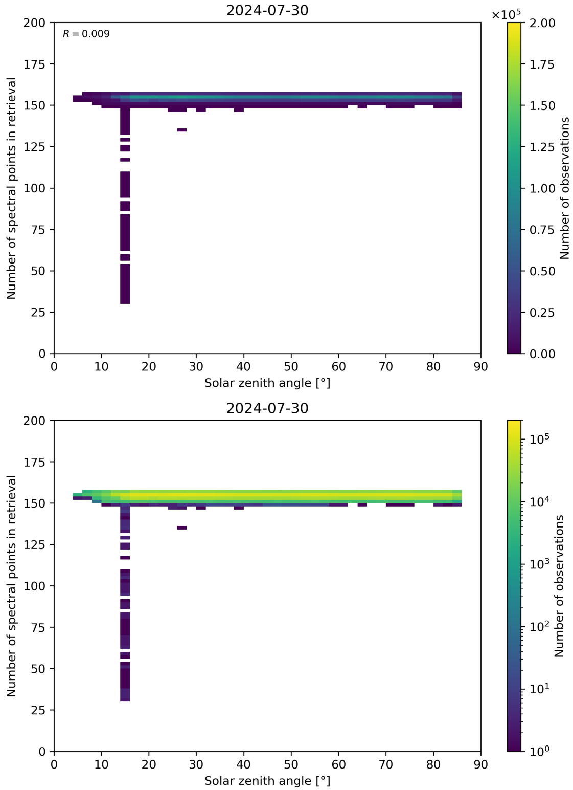
Figure 68: Scatter density plot of “Solar zenith angle” against “Number of spectral points in retrieval” for 2024-07-29 to 2024-07-31.
