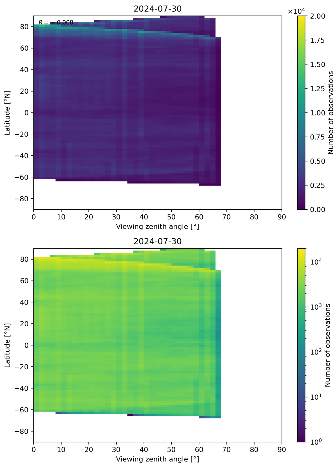
Figure 74: Scatter density plot of “Viewing zenith angle” against “Latitude” for 2024-07-29 to 2024-07-31.
