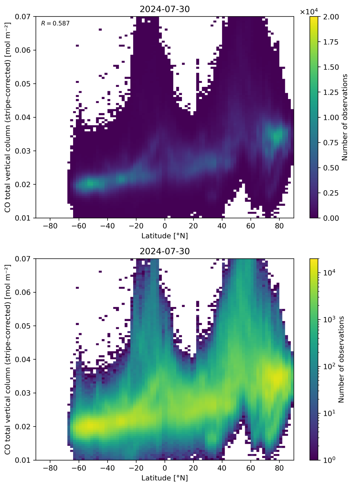
Figure 52: Scatter density plot of “Latitude” against “CO total vertical column (stripe-corrected)” for 2024-07-29 to 2024-07-31.
