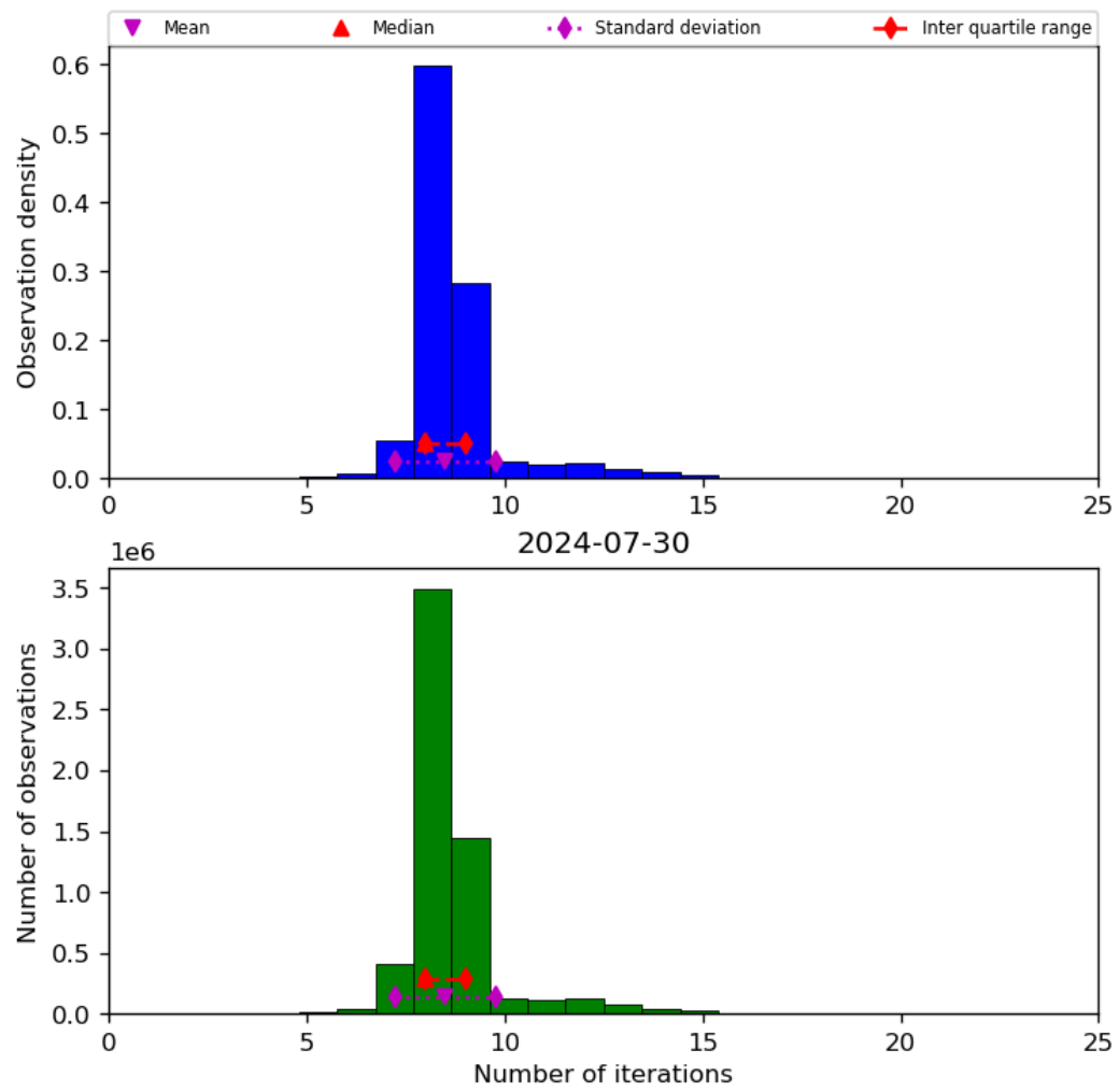
Figure 24: Histogram of “Number of iterations” for 2024-07-29 to 2024-07-31
