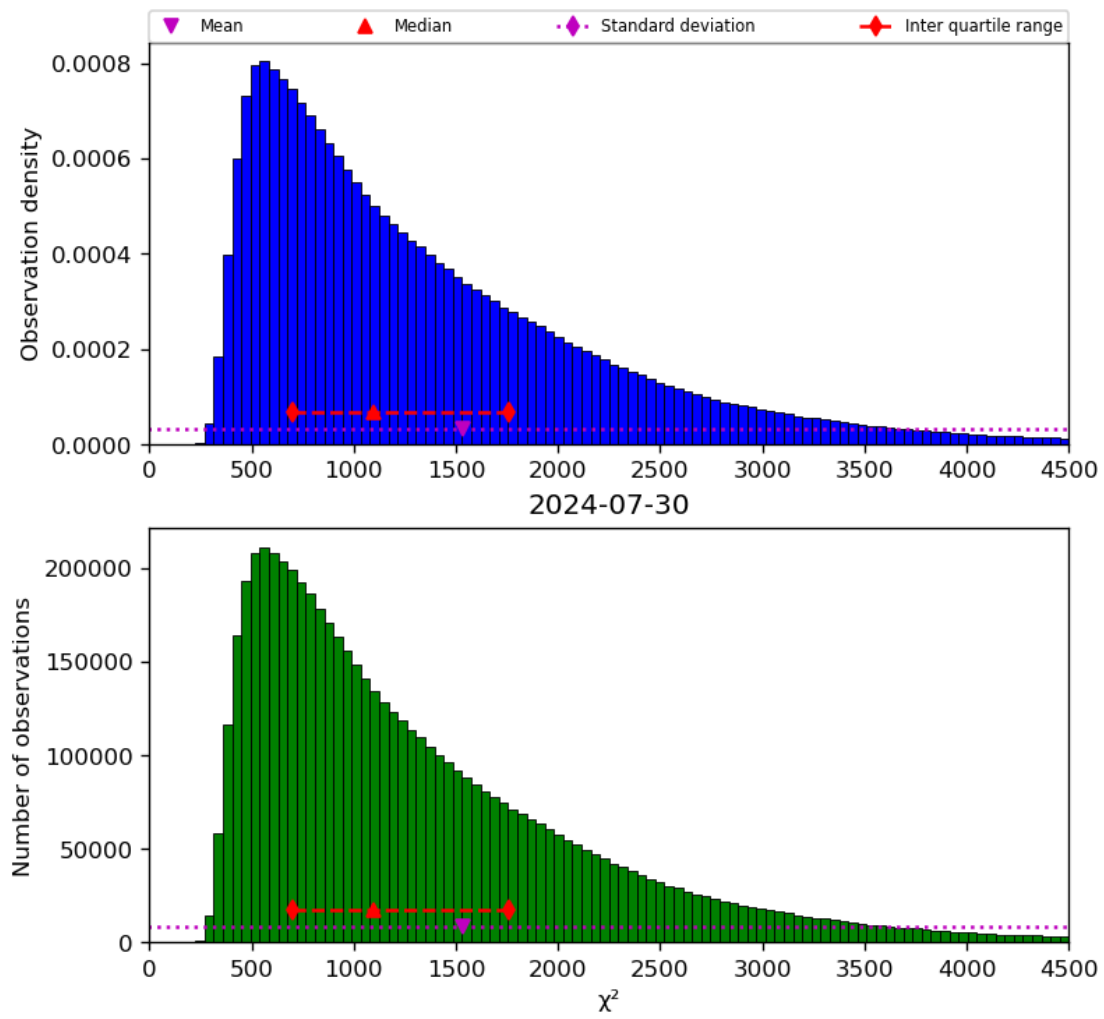
Figure 22: Histogram of “ \chi^2 ” for 2024-07-29 to 2024-07-31
