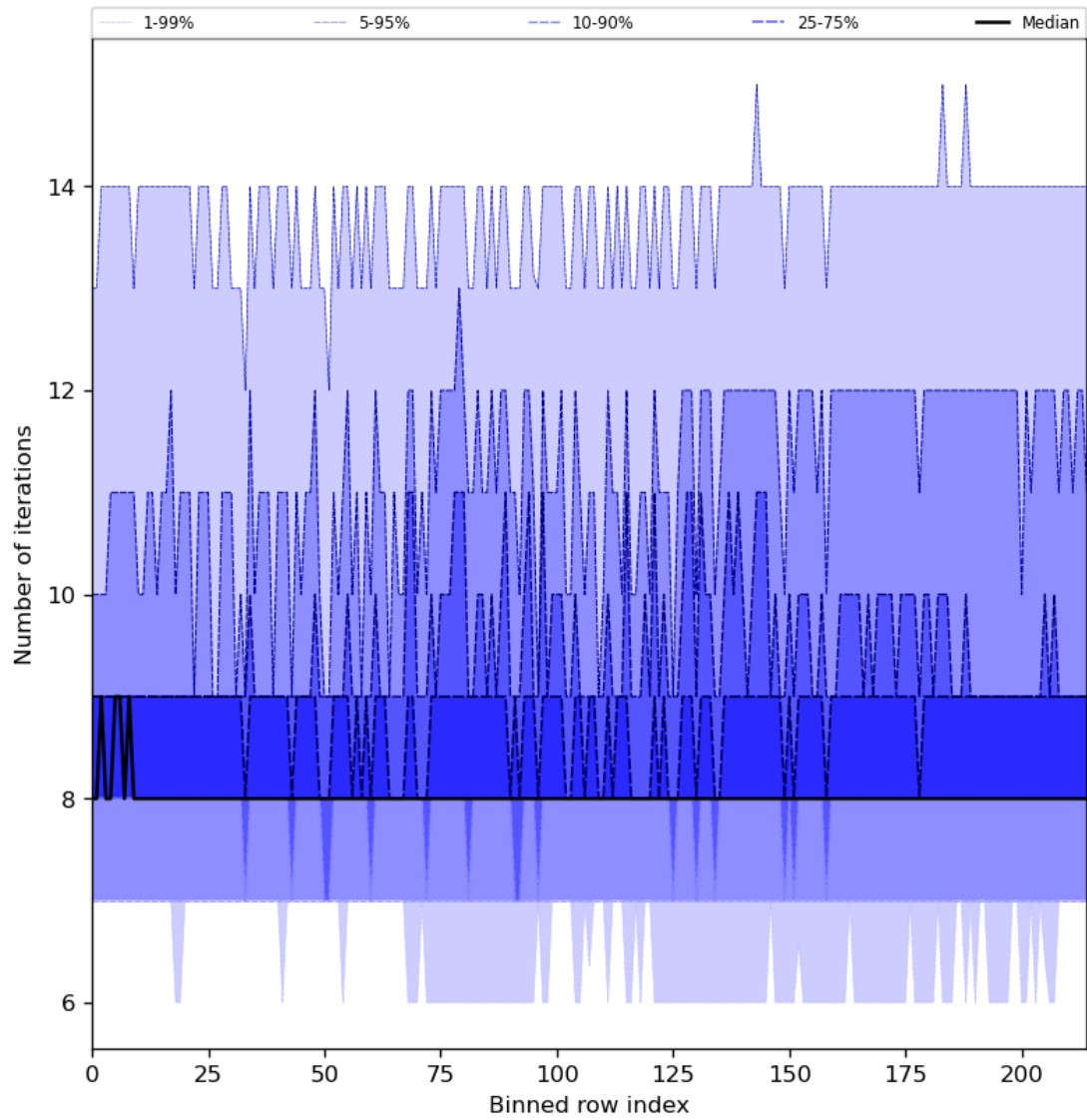
Figure 32: Along track statistics of “Number of iterations” for 2024-07-29 to 2024-07-31
