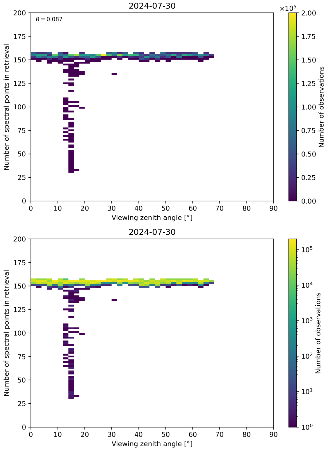
Figure 76: Scatter density plot of “Viewing zenith angle” against “Number of spectral points in retrieval” for 2024-07-29 to 2024-07-31.
