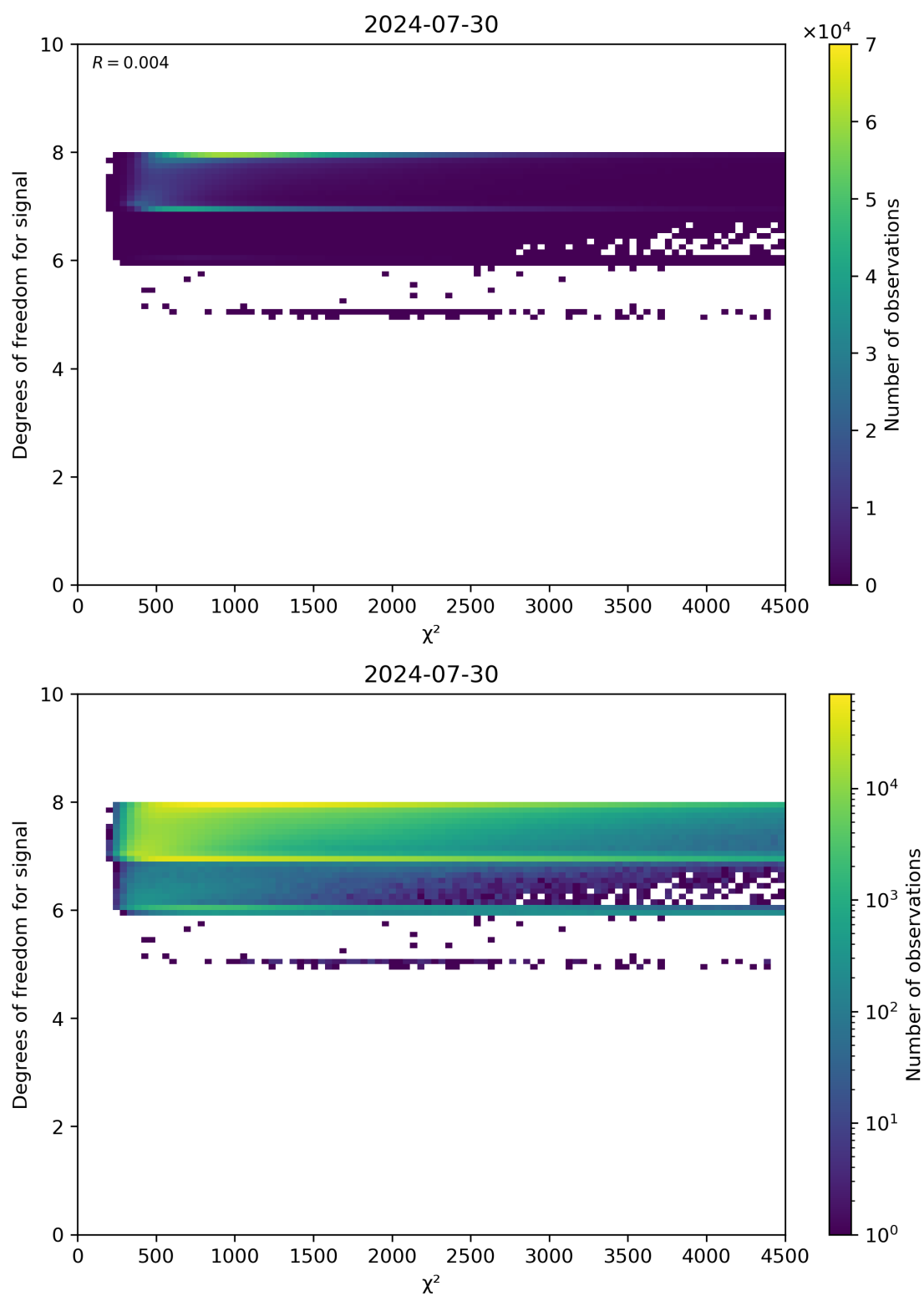
Figure 48: Scatter density plot of “ \chi^2 ” against “Degrees of freedom for signal” for 2024-07-29 to 2024-07-31.
