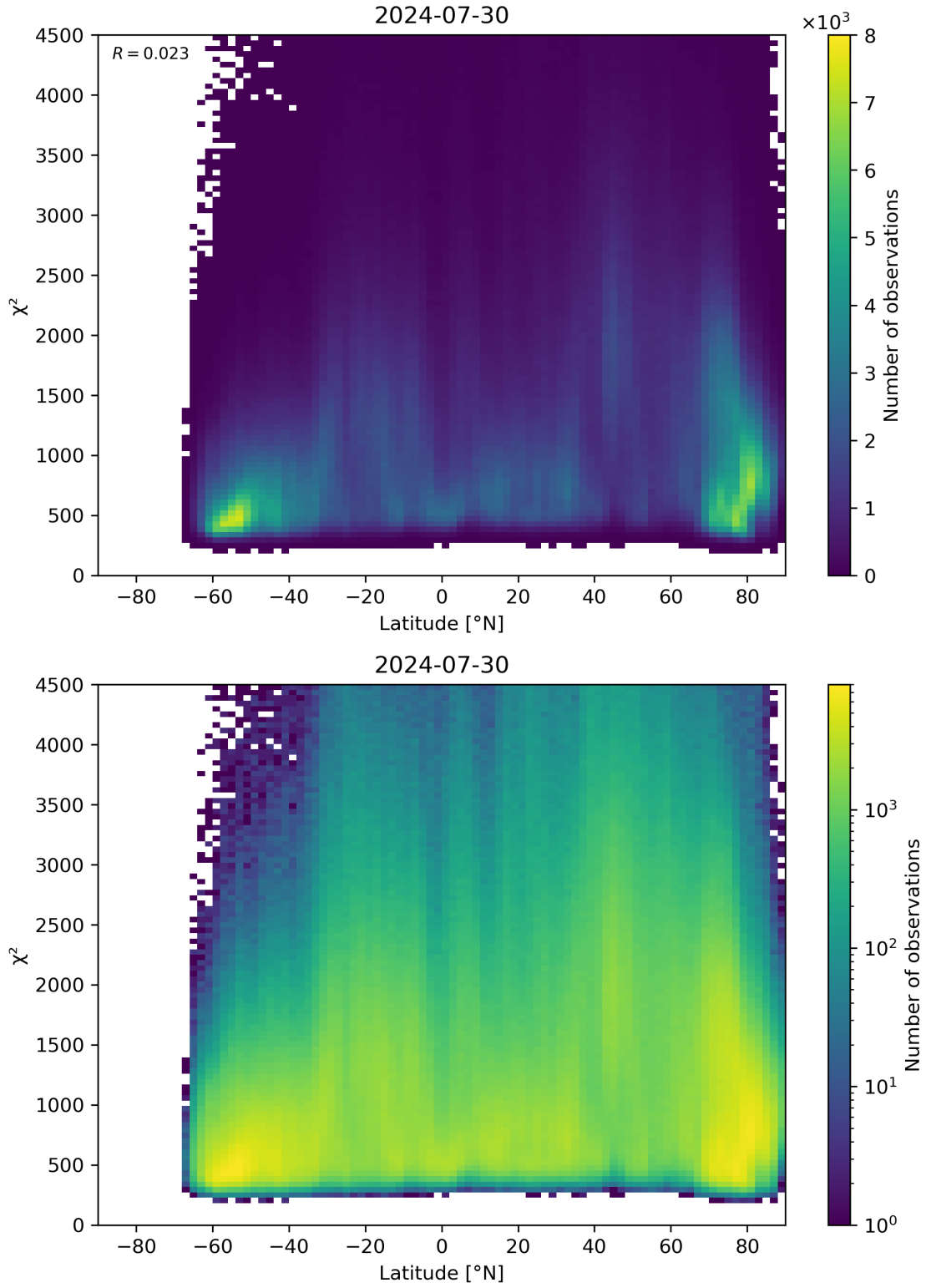
Figure 54: Scatter density plot of “Latitude” against “ \chi^2 ” for 2024-07-29 to 2024-07-31.
