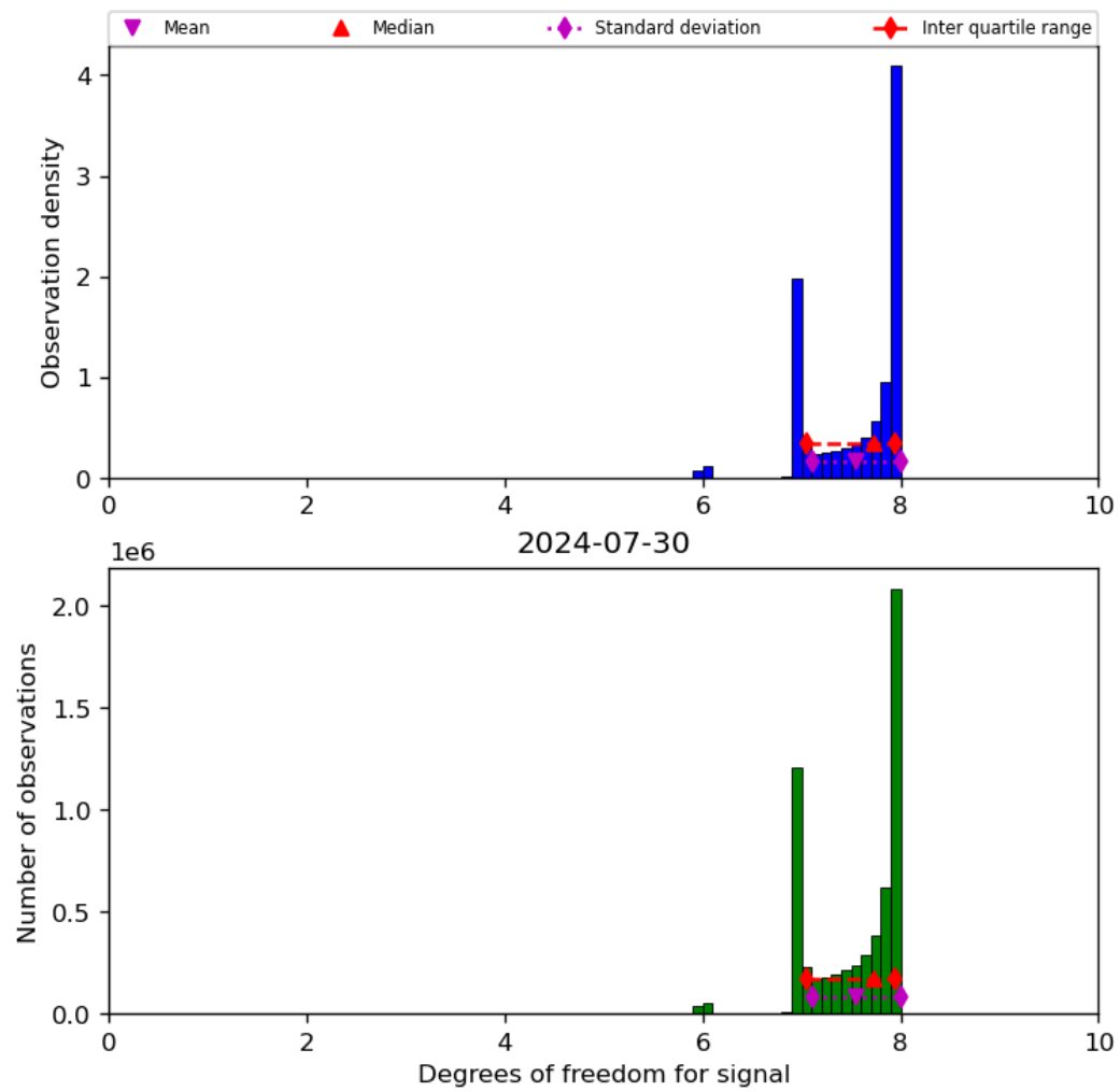
Figure 23: Histogram of “Degrees of freedom for signal” for 2024-07-29 to 2024-07-31
