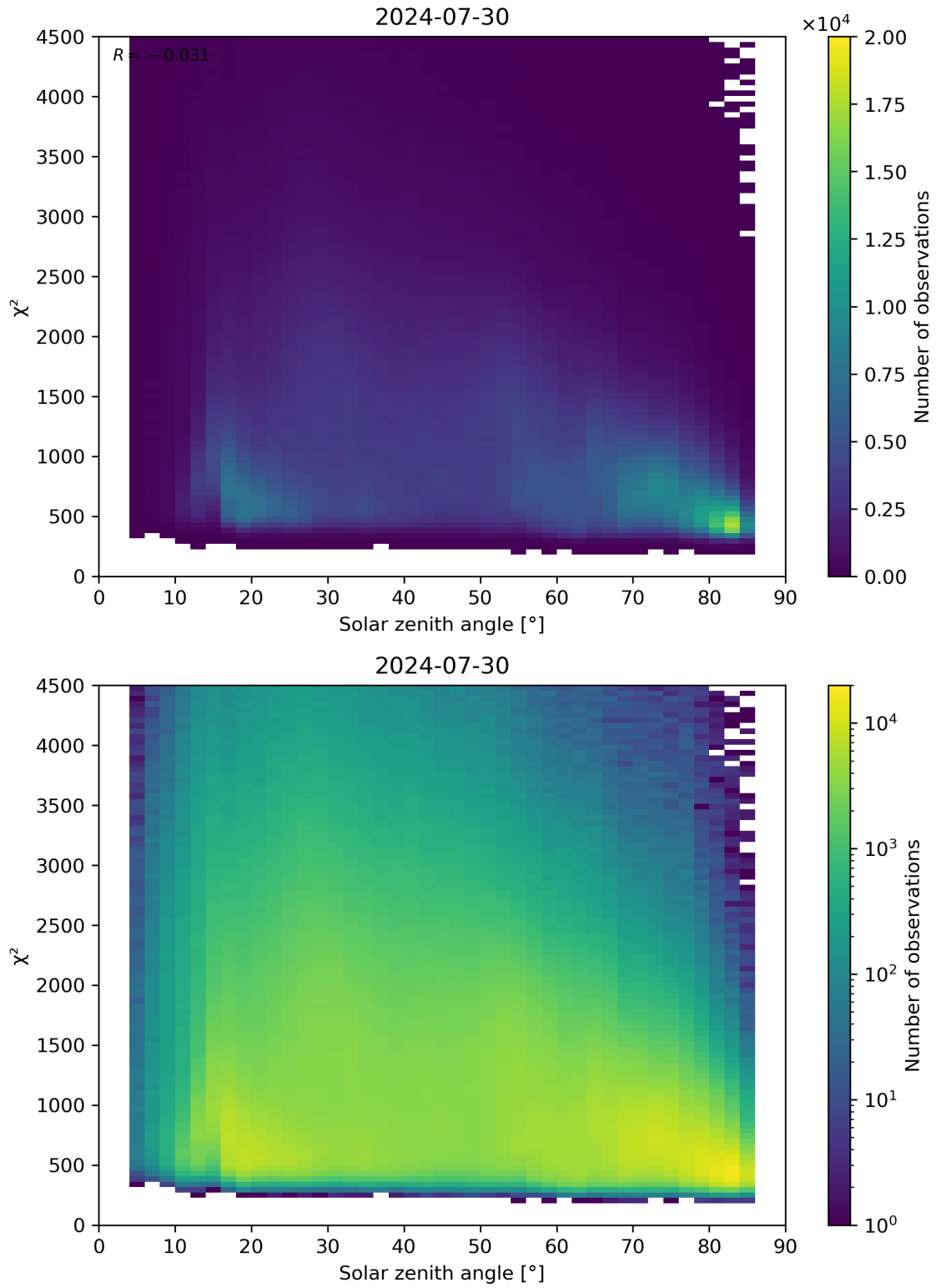
Figure 64: Scatter density plot of “Solar zenith angle” against “ \chi^2 ” for 2024-07-29 to 2024-07-31.
