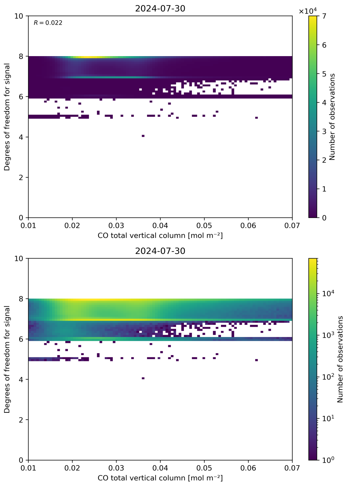
Figure 41: Scatter density plot of “CO total vertical column” against “Degrees of freedom for signal” for 2024-07-29 to 2024-07-31.
