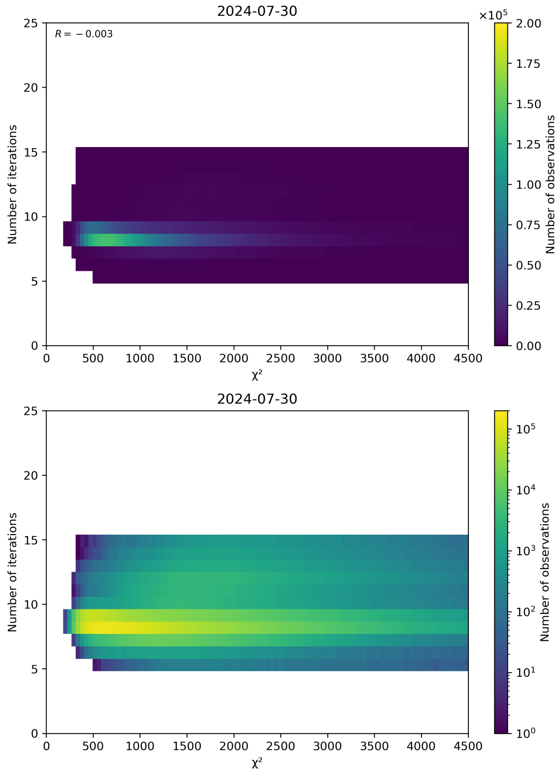
Figure 49: Scatter density plot of “ \chi^2 ” against “Number of iterations” for 2024-07-29 to 2024-07-31.
