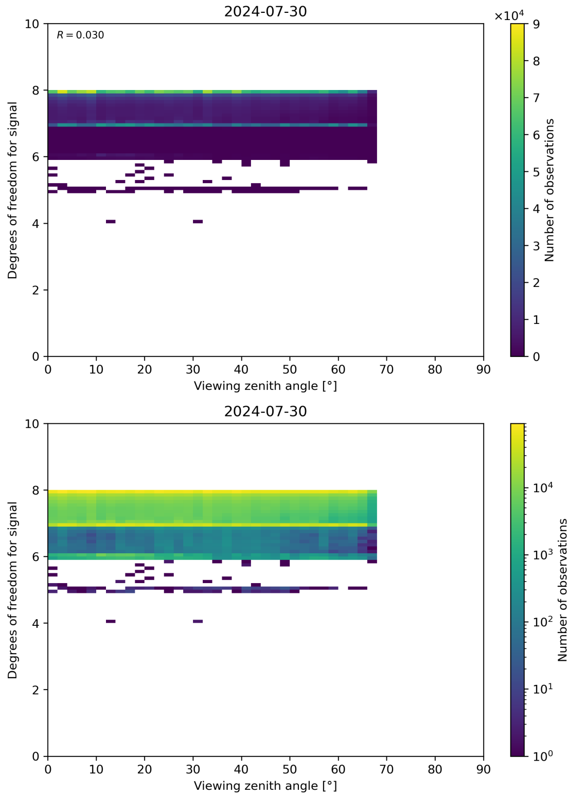
Figure 73: Scatter density plot of “Viewing zenith angle” against “Degrees of freedom for signal” for 2024-07-29 to 2024-07-31.
