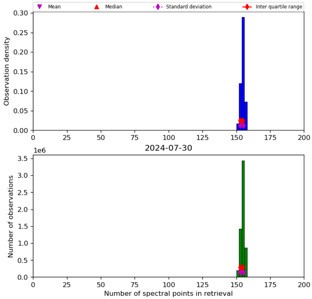
Figure 21: Histogram of “Number of spectral points in retrieval” for 2024-07-29 to 2024-07-31
