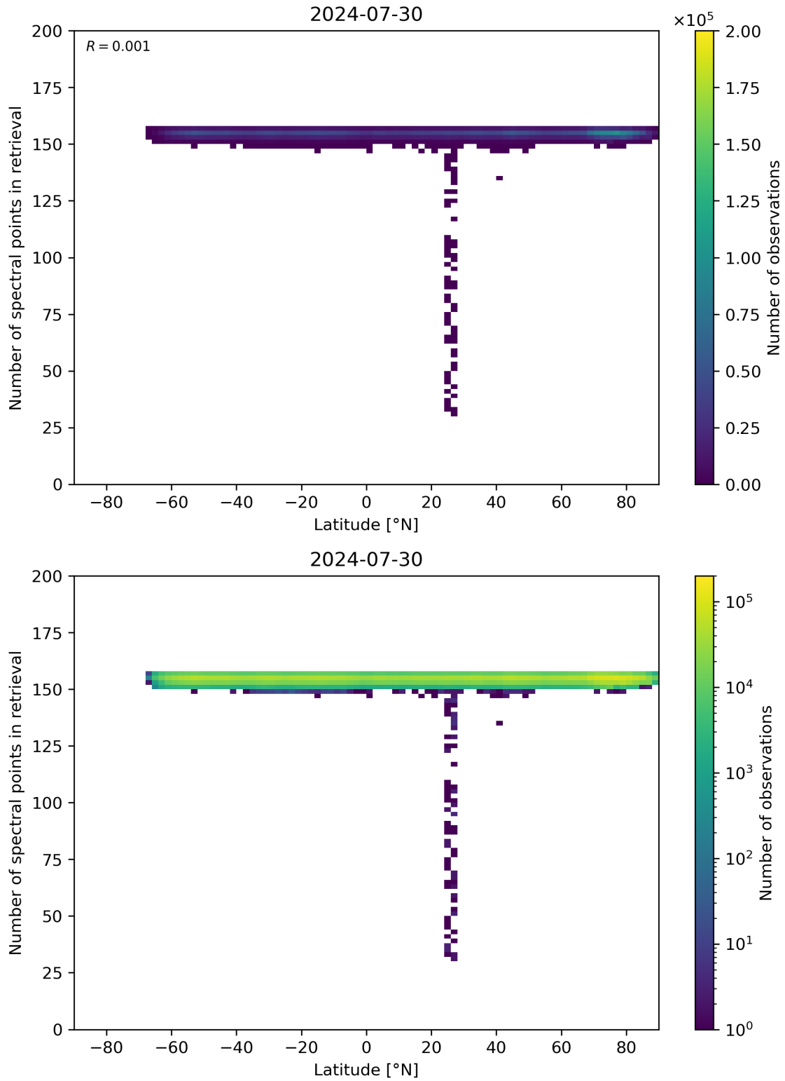
Figure 57: Scatter density plot of “Latitude” against “Number of spectral points in retrieval” for 2024-07-29 to 2024-07-31.
