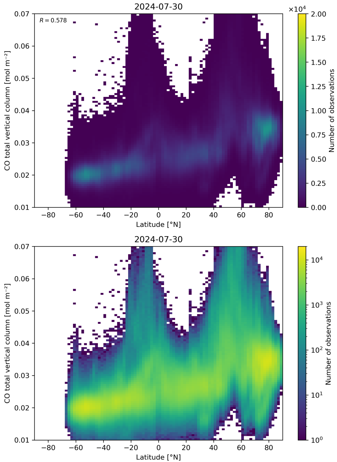
Figure 51: Scatter density plot of “Latitude” against “CO total vertical column” for 2024-07-29 to 2024-07-31.
