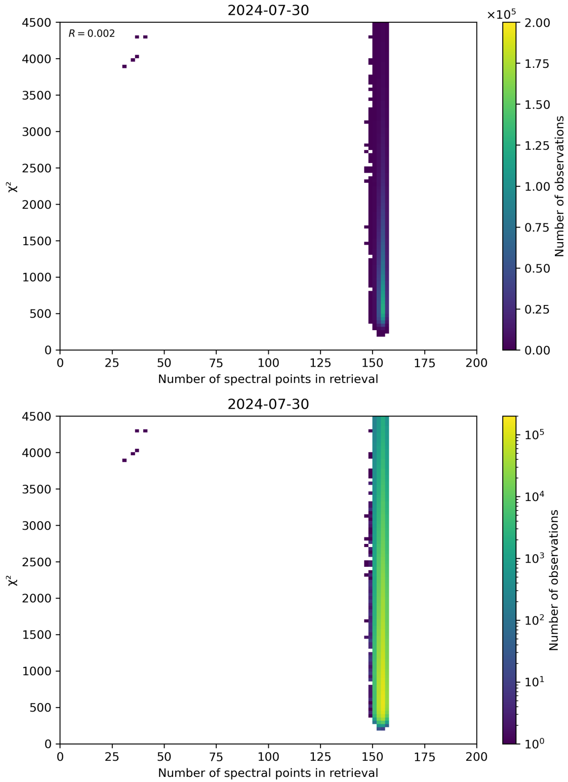
Figure 58: Scatter density plot of “Number of spectral points in retrieval” against “ \chi^2 ” for 2024-07-29 to 2024-07-31.
