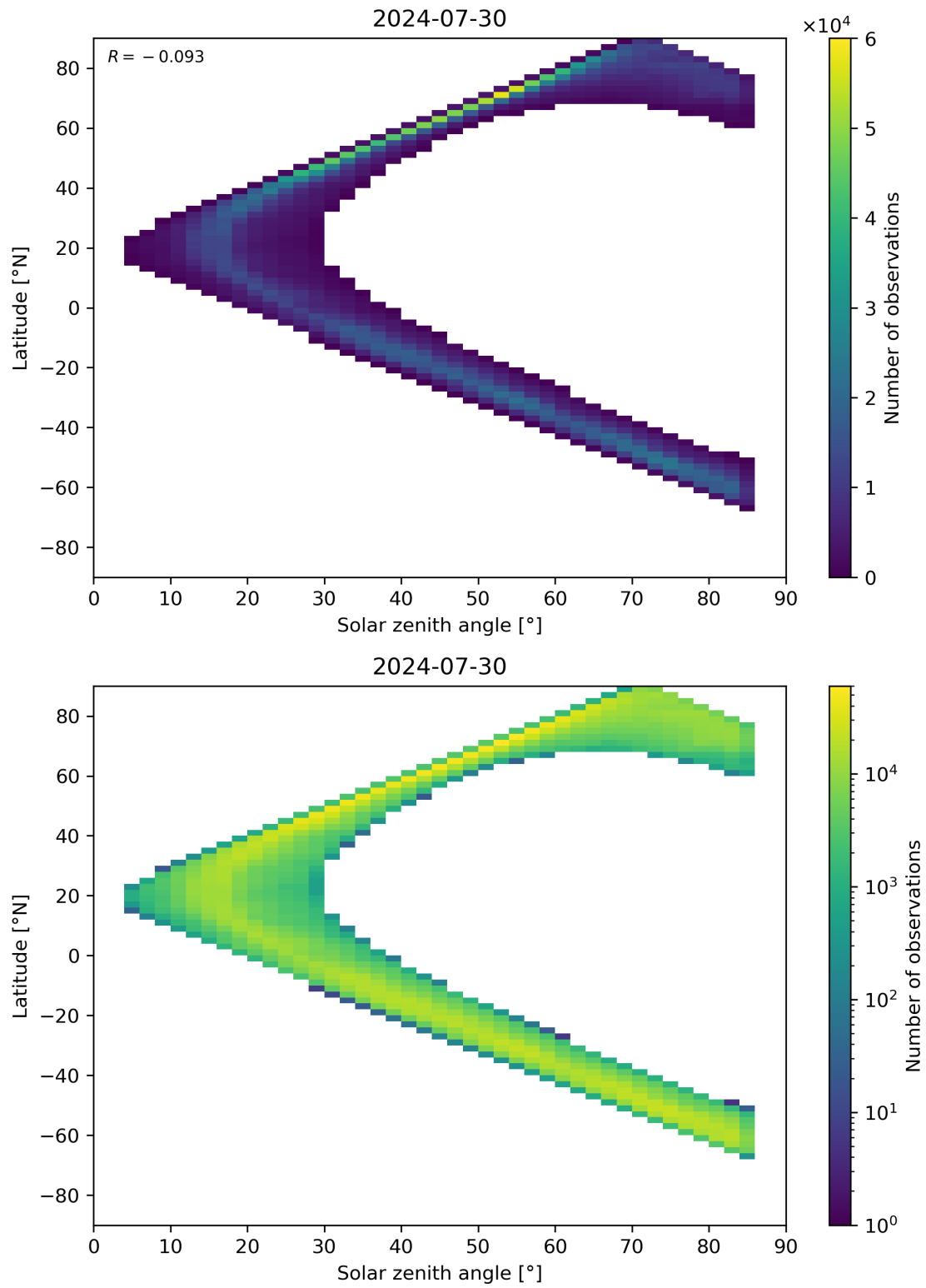
Figure 66: Scatter density plot of “Solar zenith angle” against “Latitude” for 2024-07-29 to 2024-07-31.
