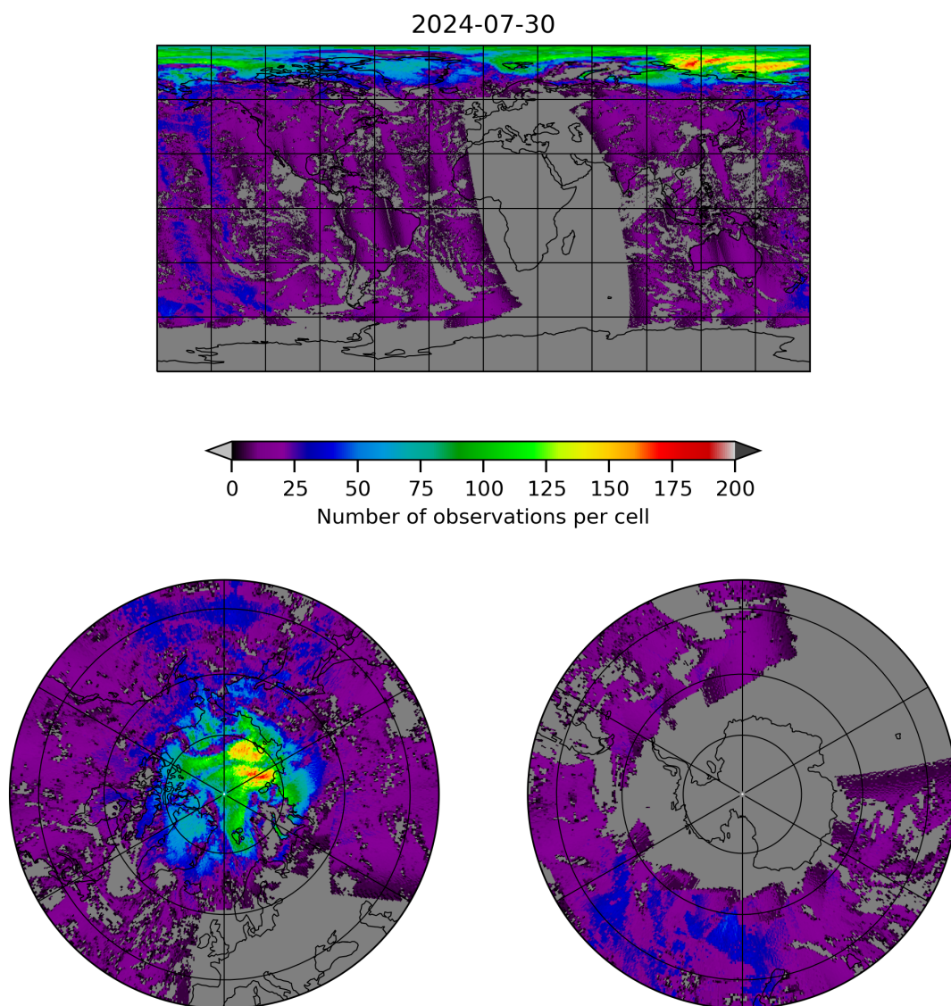
Figure 8: Map of the number of observations for 2024-07-29 to 2024-07-31
