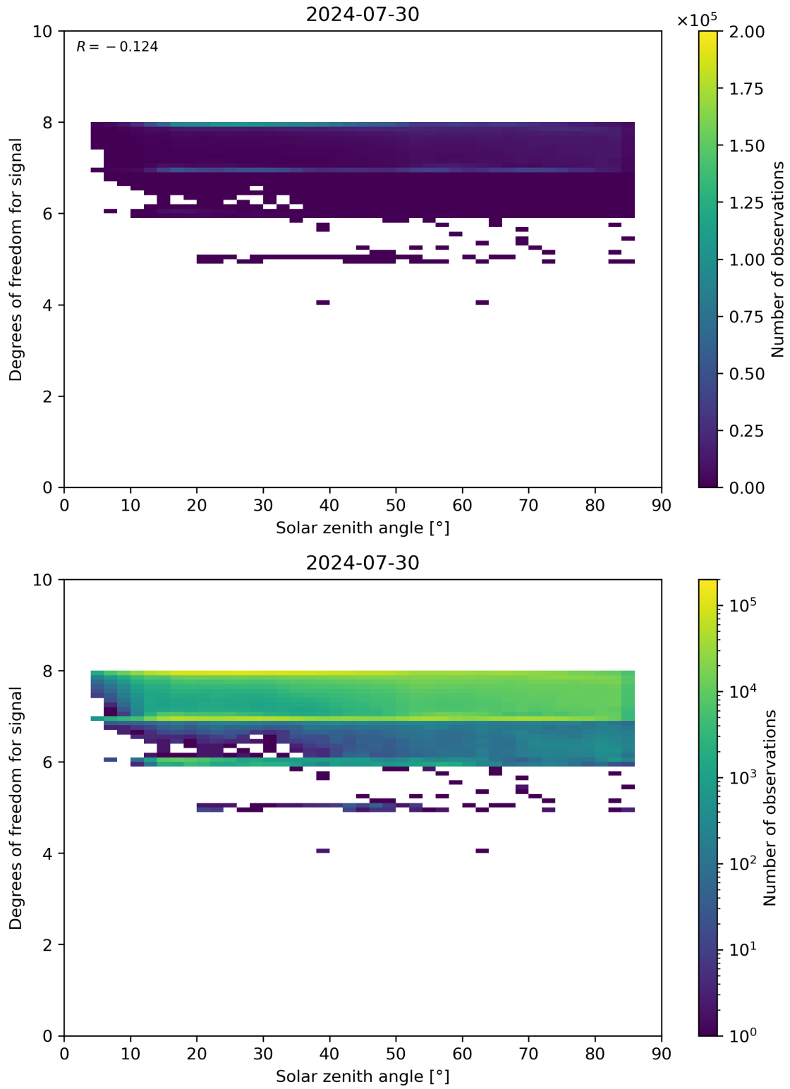
Figure 65: Scatter density plot of “Solar zenith angle” against “Degrees of freedom for signal” for 2024-07-29 to 2024-07-31.
