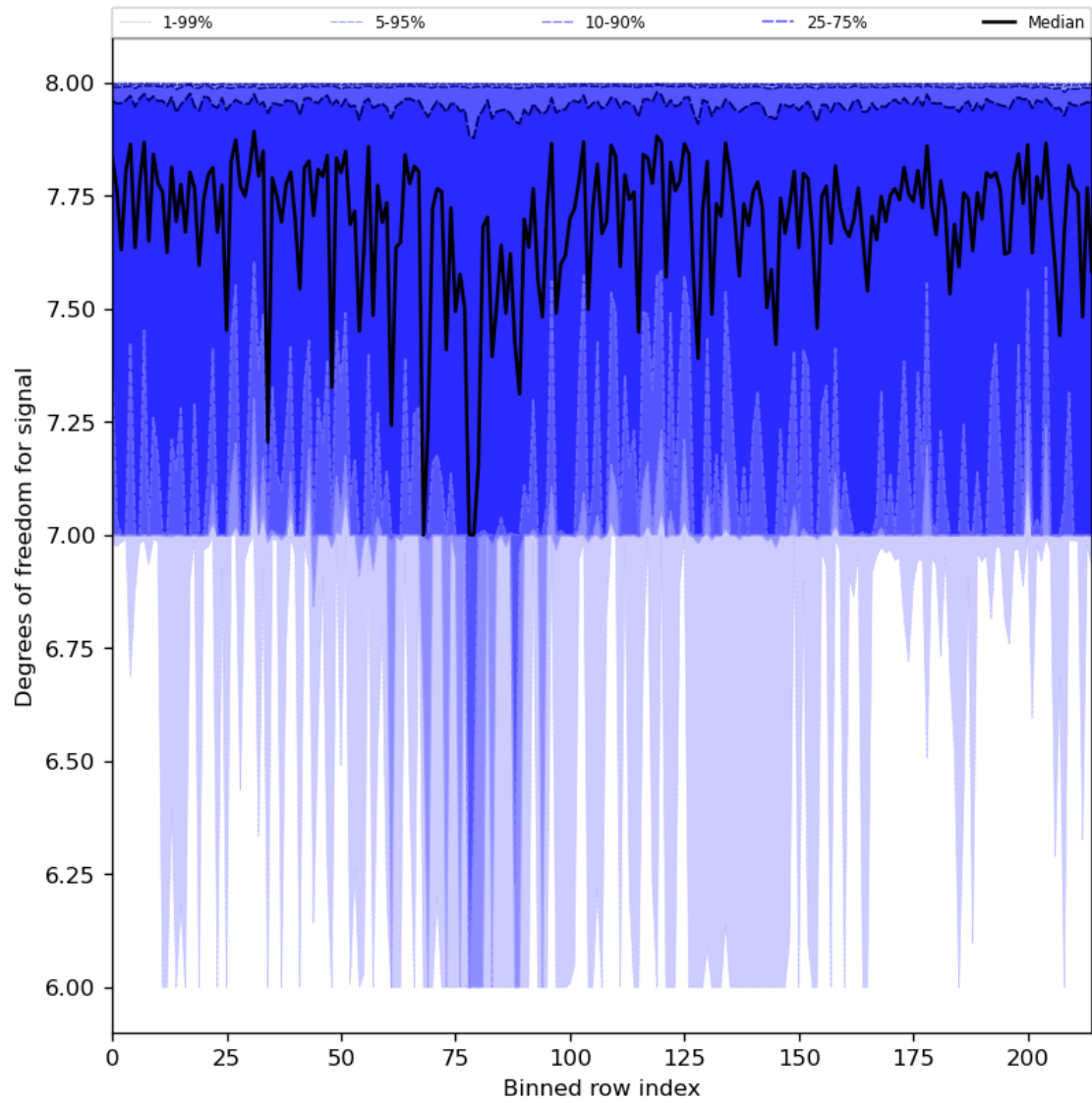
Figure 31: Along track statistics of “Degrees of freedom for signal” for 2024-07-29 to 2024-07-31
