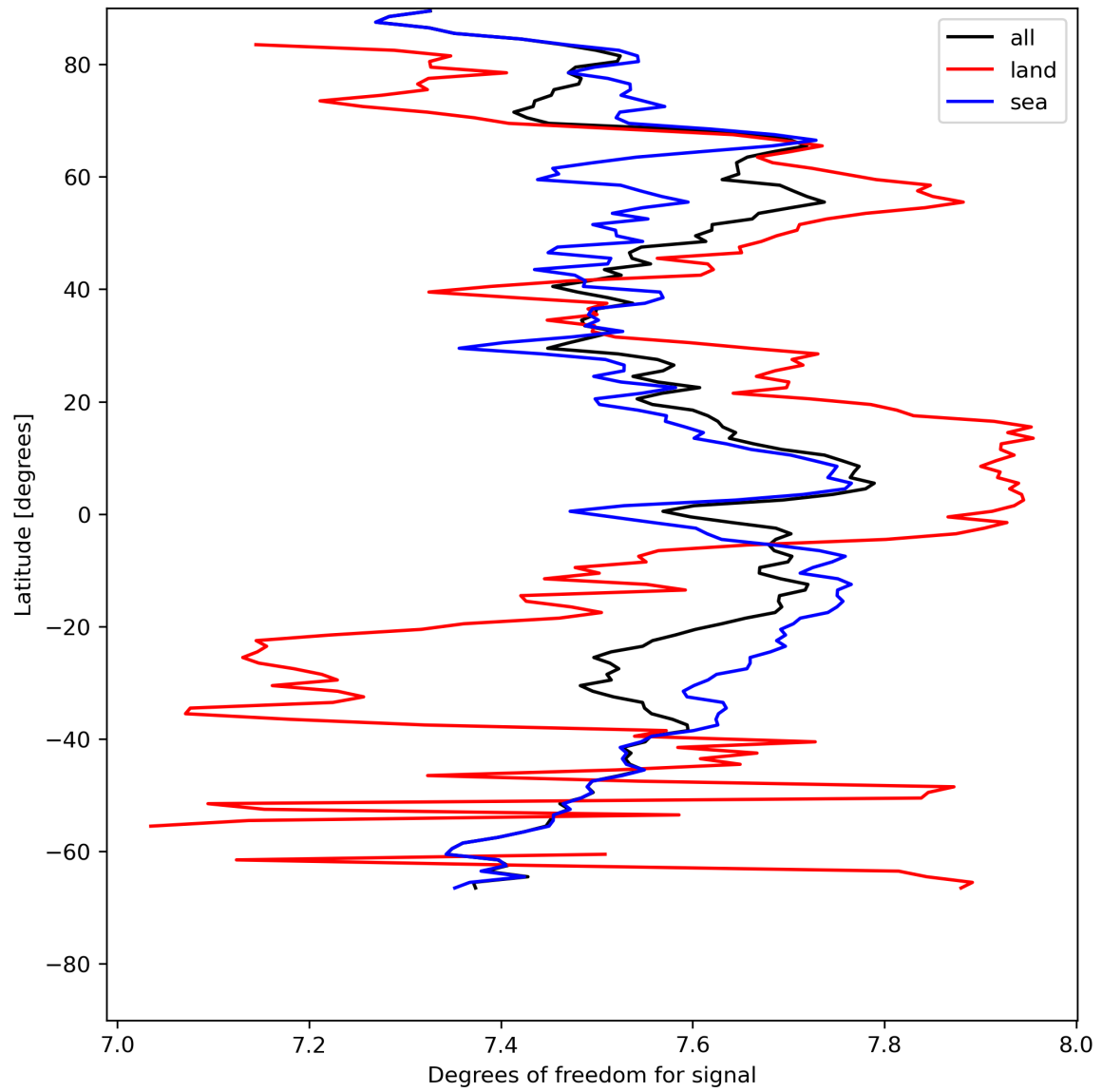
Figure 15: Zonal average of “Degrees of freedom for signal” for 2024-07-29 to 2024-07-31.
