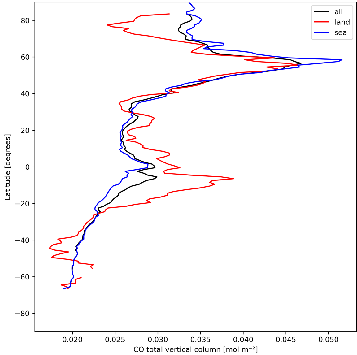
Figure 10: Zonal average of “CO total vertical column” for 2024-07-29 to 2024-07-31.
