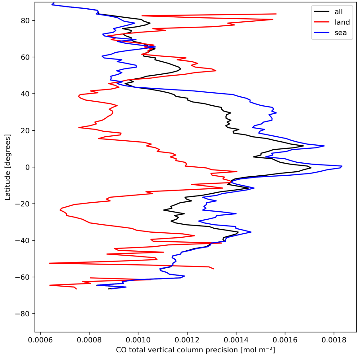
Figure 12: Zonal average of “CO total vertical column precision” for 2024-07-29 to 2024-07-31.
