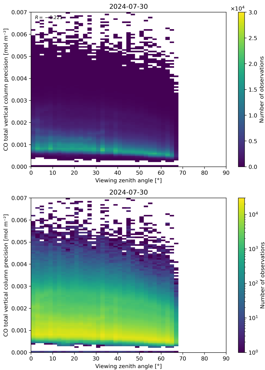
Figure 71: Scatter density plot of “Viewing zenith angle” against “CO total vertical column precision” for 2024-07-29 to 2024-07-31.
