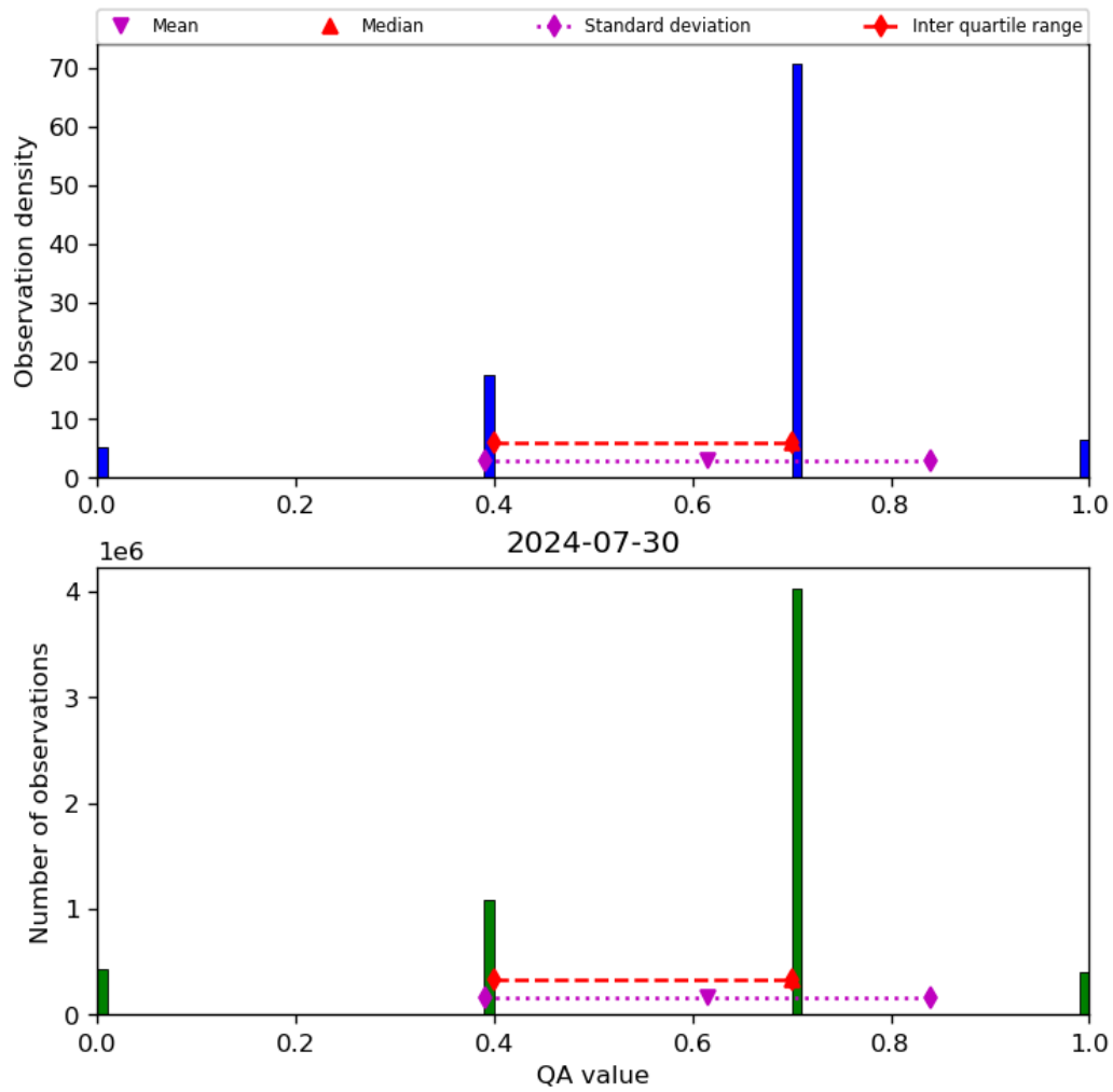
Figure 17: Histogram of “QA value” for 2024-07-29 to 2024-07-31
