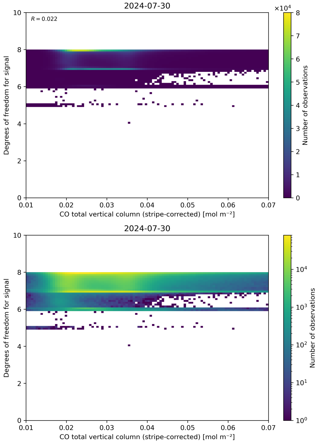
Figure 38: Scatter density plot of “CO total vertical column (stripe-corrected)” against “Degrees of freedom for signal” for 2024-07-29 to 2024-07-31.
