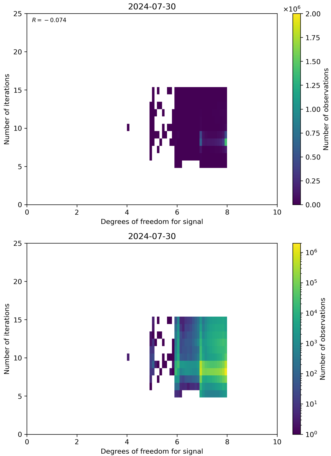
Figure 50: Scatter density plot of “Degrees of freedom for signal” against “Number of iterations” for 2024-07-29 to 2024-07-31.
