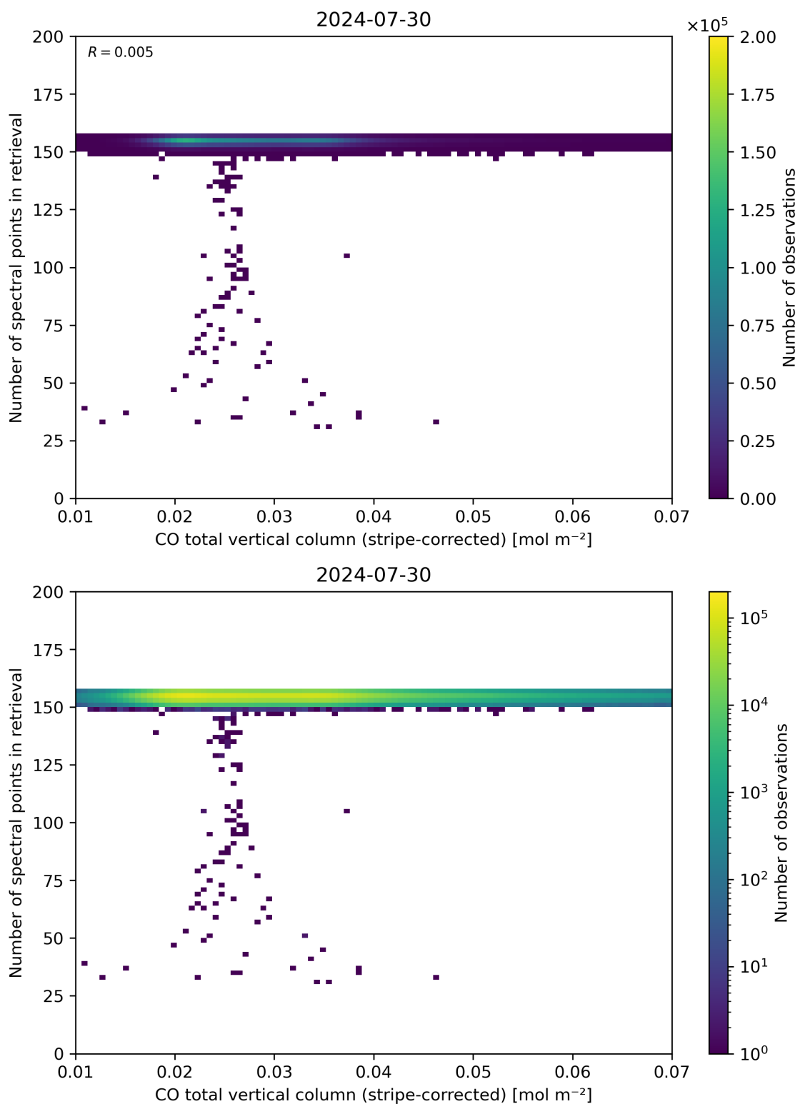
Figure 40: Scatter density plot of “CO total vertical column (stripe-corrected)” against “Number of spectral points in retrieval” for 2024-07-29 to 2024-07-31.
