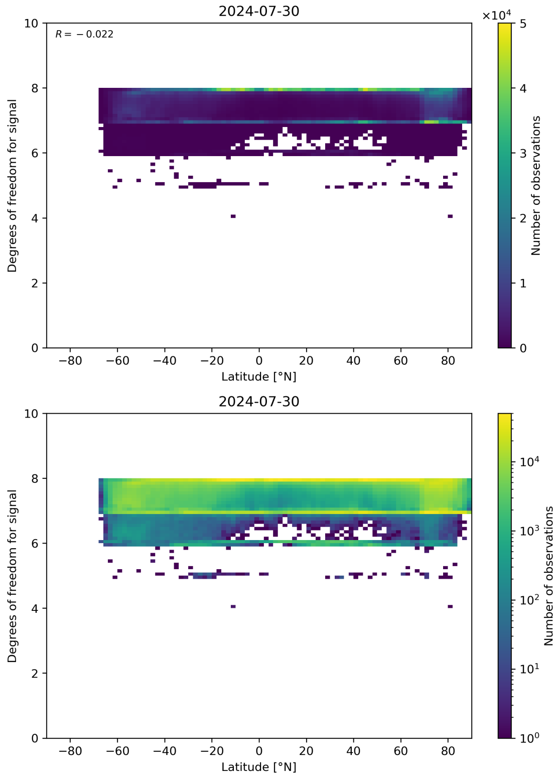
Figure 55: Scatter density plot of “Latitude” against “Degrees of freedom for signal” for 2024-07-29 to 2024-07-31.
