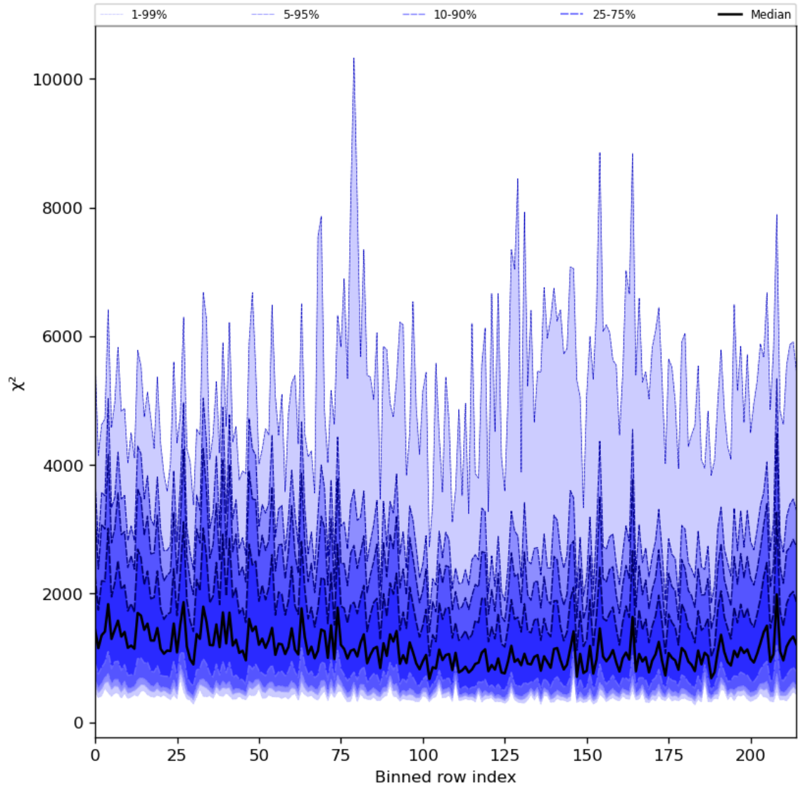
Figure 30: Along track statistics of “ \chi^2 ” for 2024-07-29 to 2024-07-31
