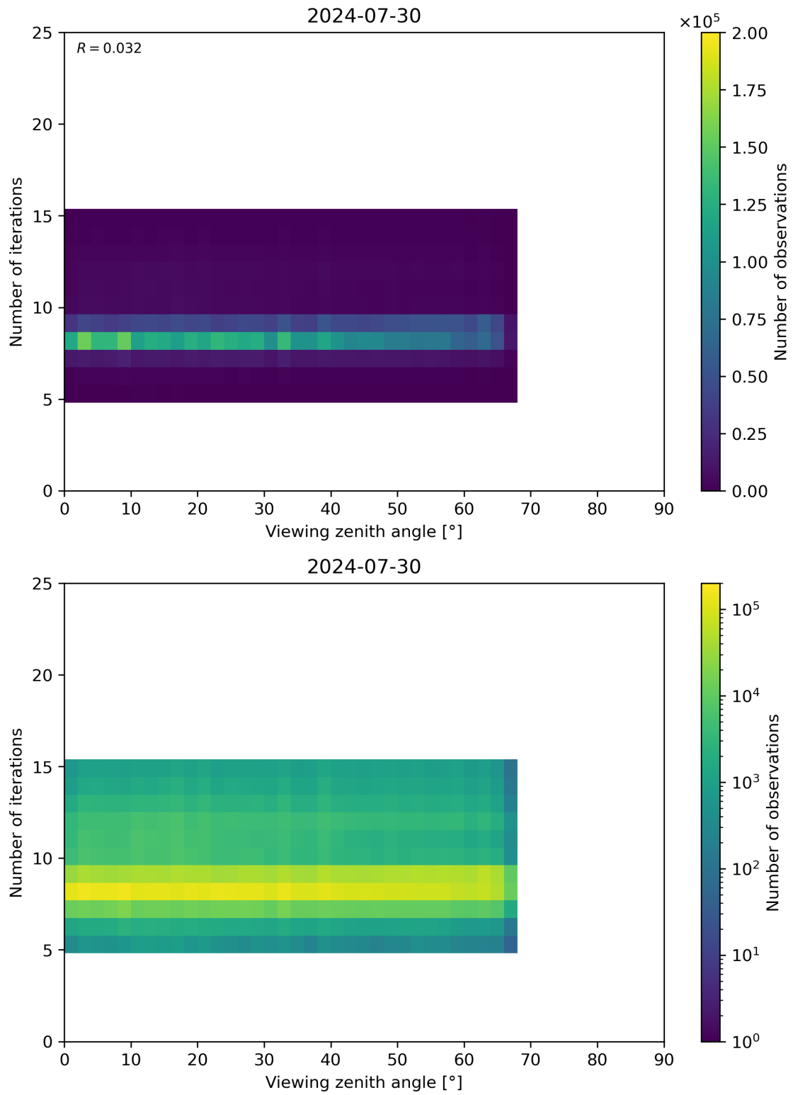
Figure 75: Scatter density plot of “Viewing zenith angle” against “Number of iterations” for 2024-07-29 to 2024-07-31.
