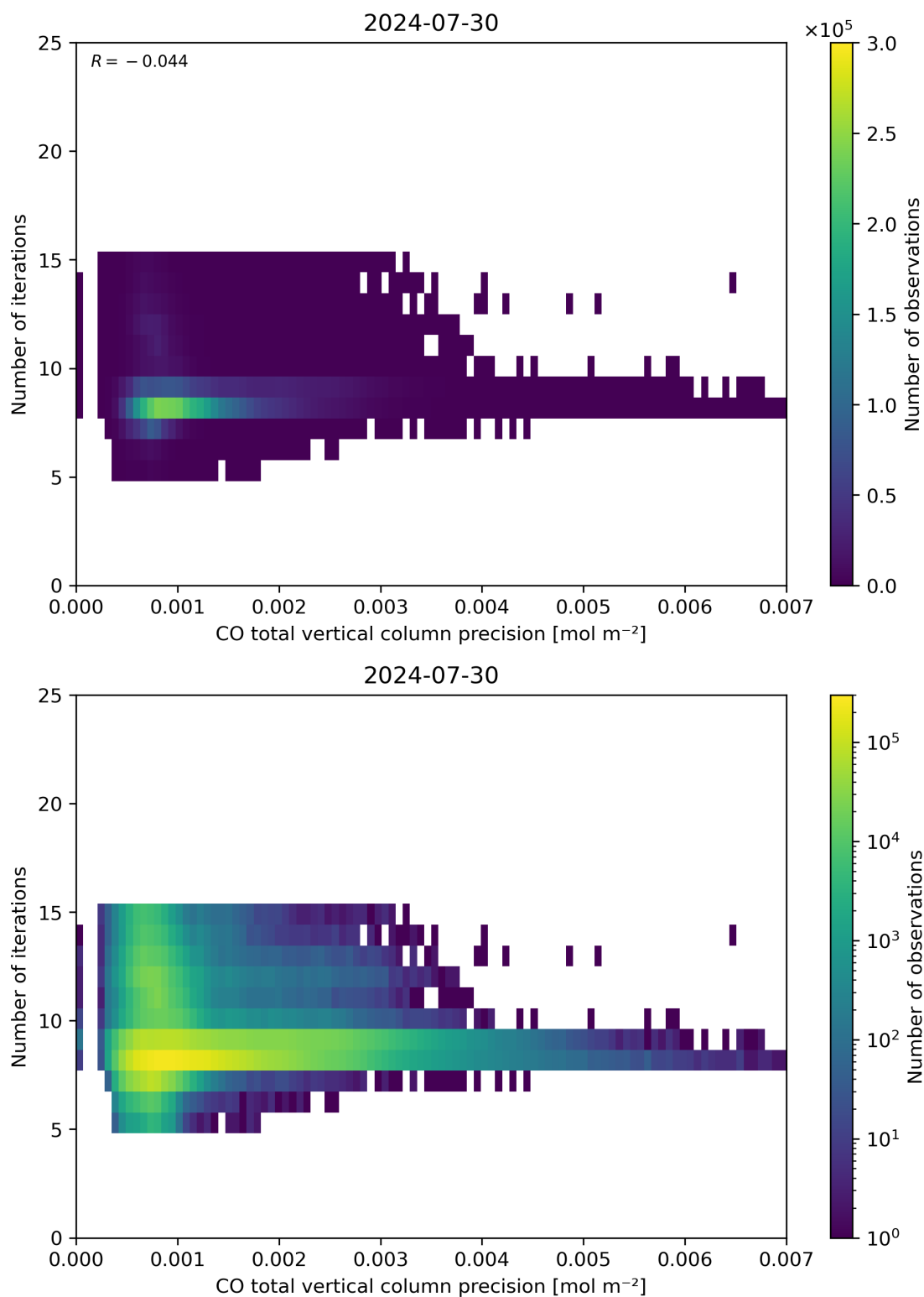
Figure 46: Scatter density plot of “CO total vertical column precision” against “Number of iterations” for 2024-07-29 to 2024-07-31.
