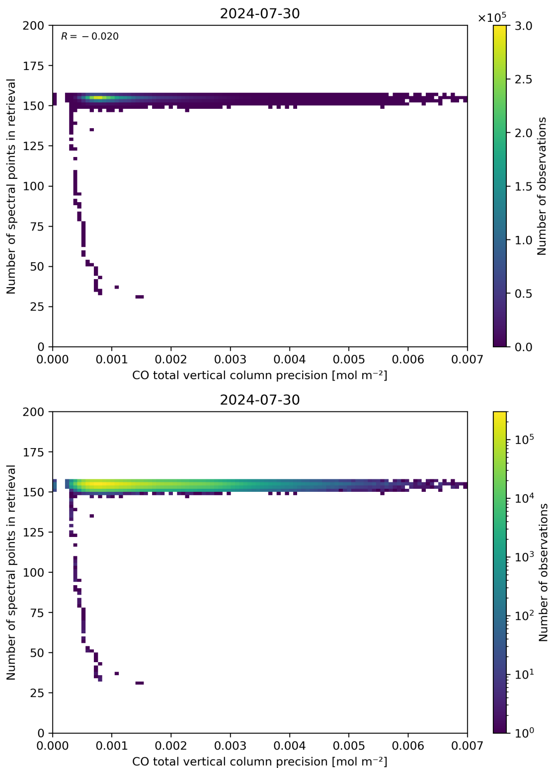
Figure 47: Scatter density plot of “CO total vertical column precision” against “Number of spectral points in retrieval” for 2024-07-29 to 2024-07-31.
