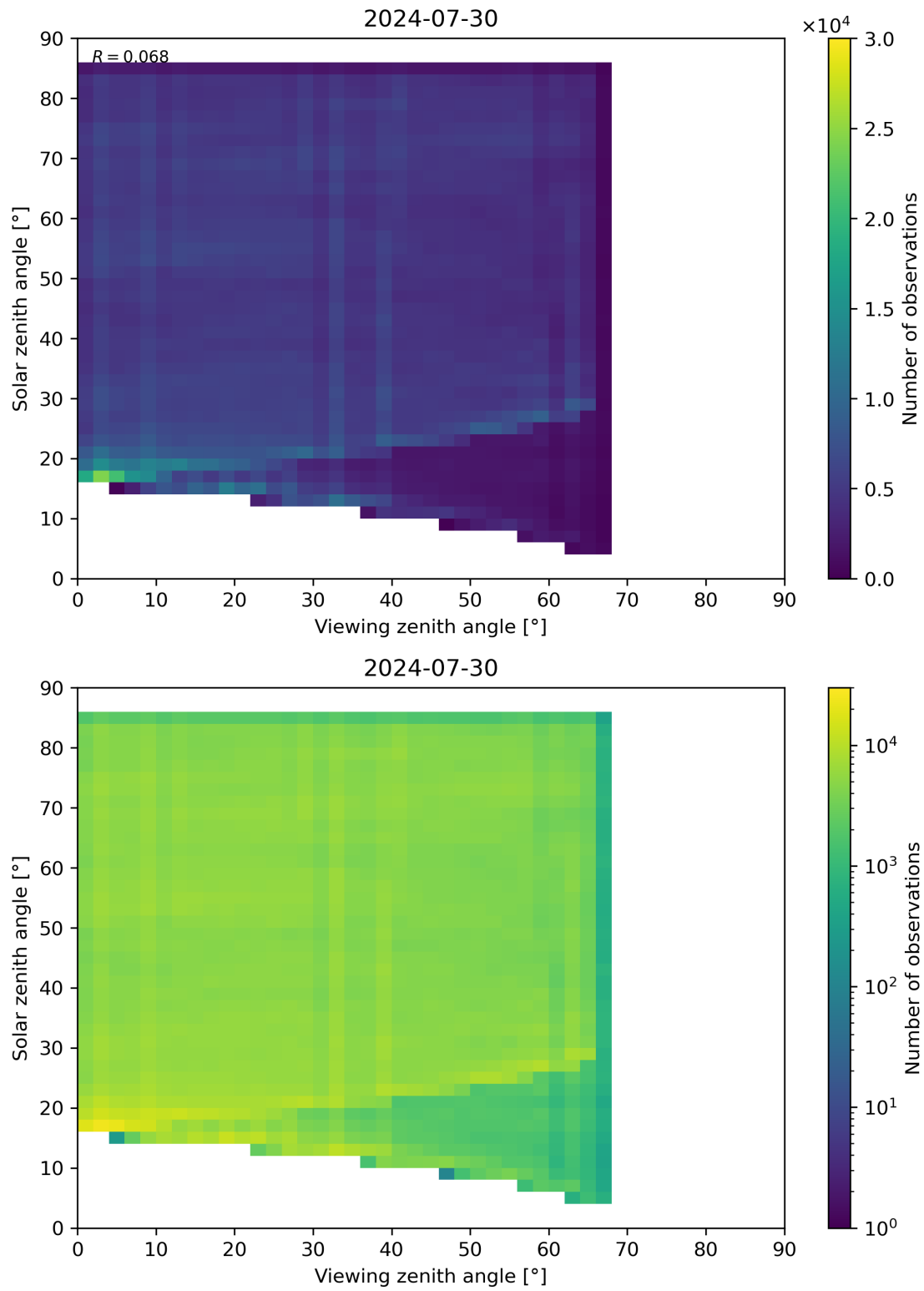
Figure 77: Scatter density plot of “Viewing zenith angle” against “Solar zenith angle” for 2024-07-29 to 2024-07-31.
