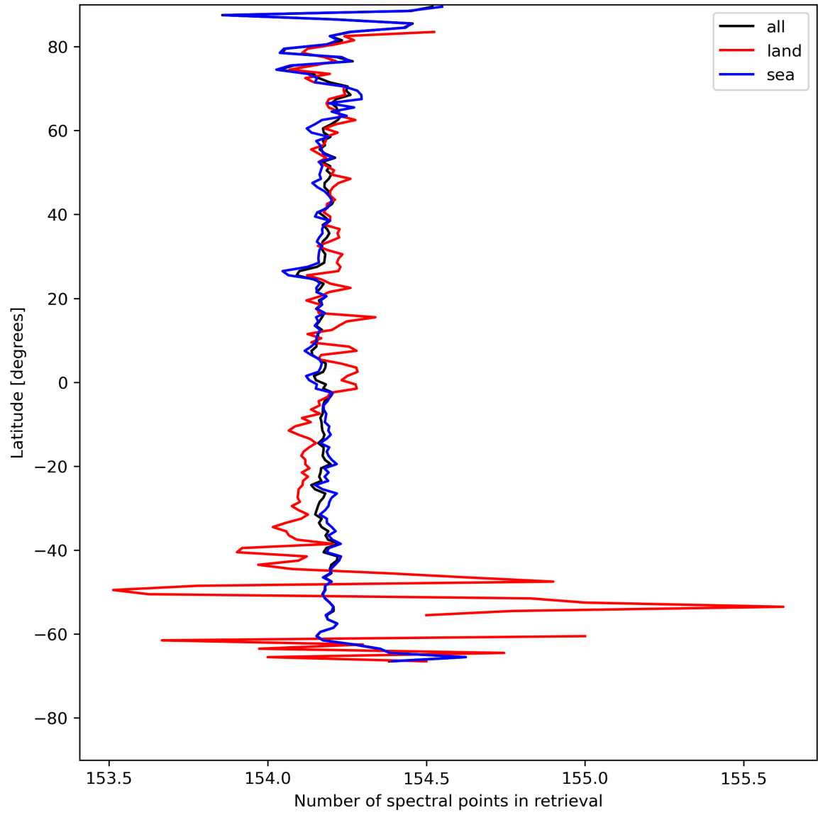
Figure 13: Zonal average of “Number of spectral points in retrieval” for 2024-07-29 to 2024-07-31.
