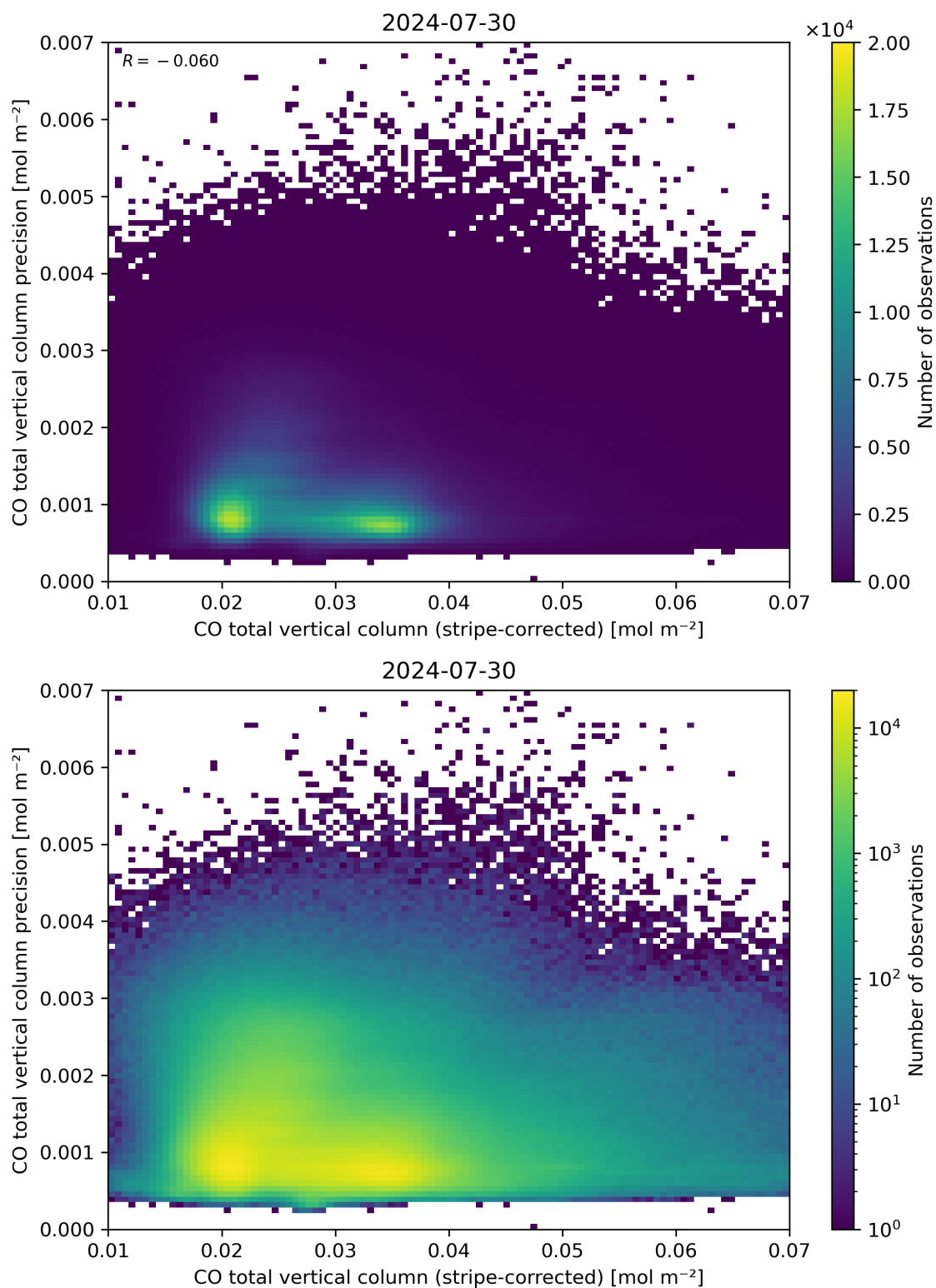
Figure 36: Scatter density plot of “CO total vertical column (stripe-corrected)” against “CO total vertical column precision” for 2024-07-29 to 2024-07-31.
