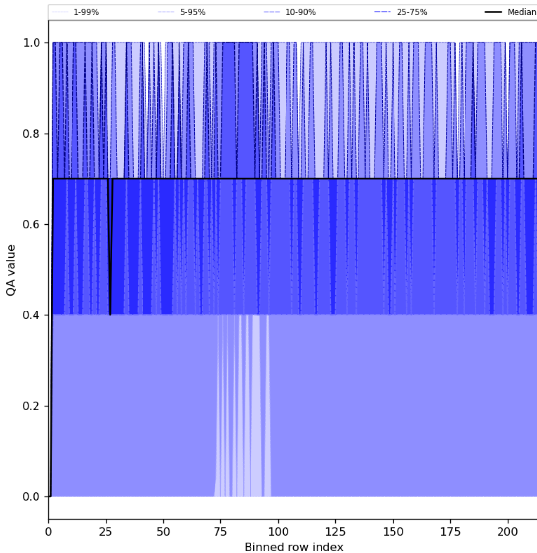
Figure 25: Along track statistics of “QA value” for 2024-07-29 to 2024-07-31
