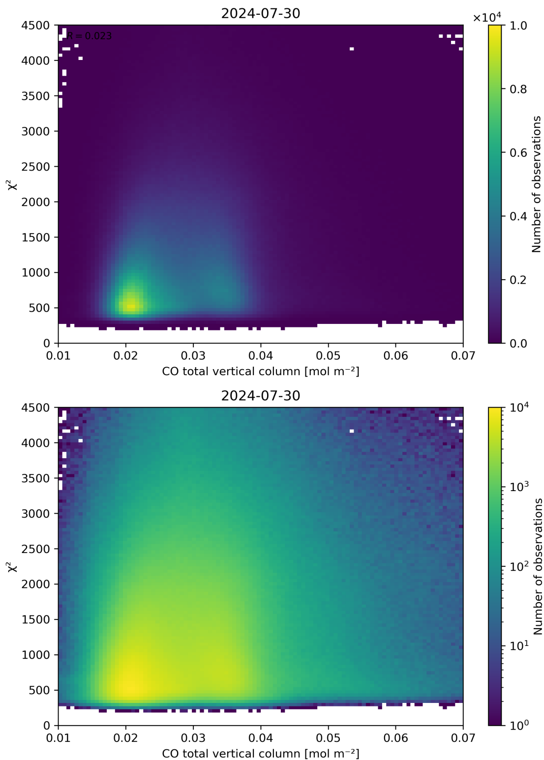
Figure 35: Scatter density plot of “CO total vertical column” against “ \chi^2 ” for 2024-07-29 to 2024-07-31.
