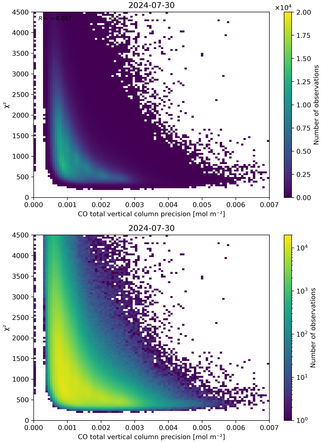
Figure 44: Scatter density plot of “CO total vertical column precision” against “ \chi^2 ” for 2024-07-29 to 2024-07-31.
