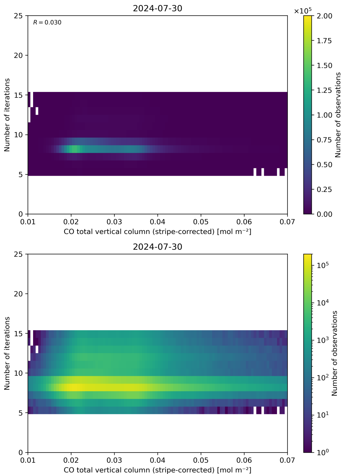
Figure 39: Scatter density plot of “CO total vertical column (stripe-corrected)” against “Number of iterations” for 2024-07-29 to 2024-07-31.
