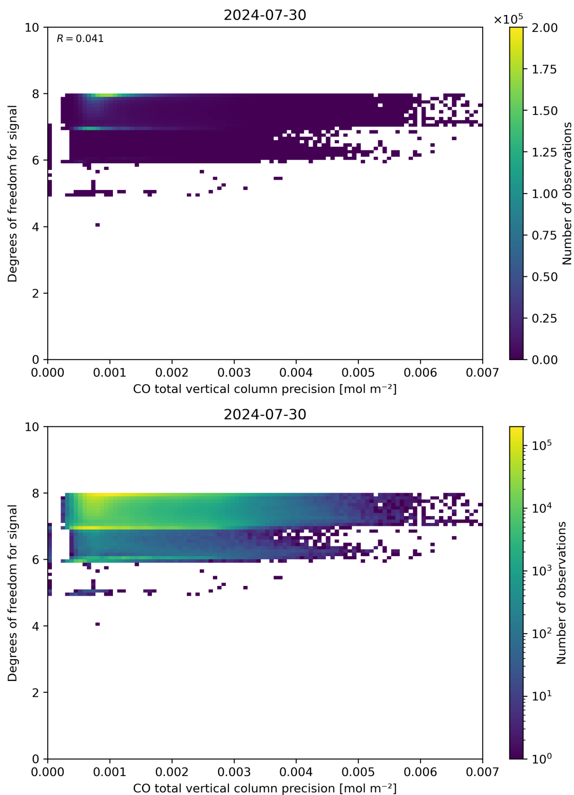
Figure 45: Scatter density plot of “CO total vertical column precision” against “Degrees of freedom for signal” for 2024-07-29 to 2024-07-31.
