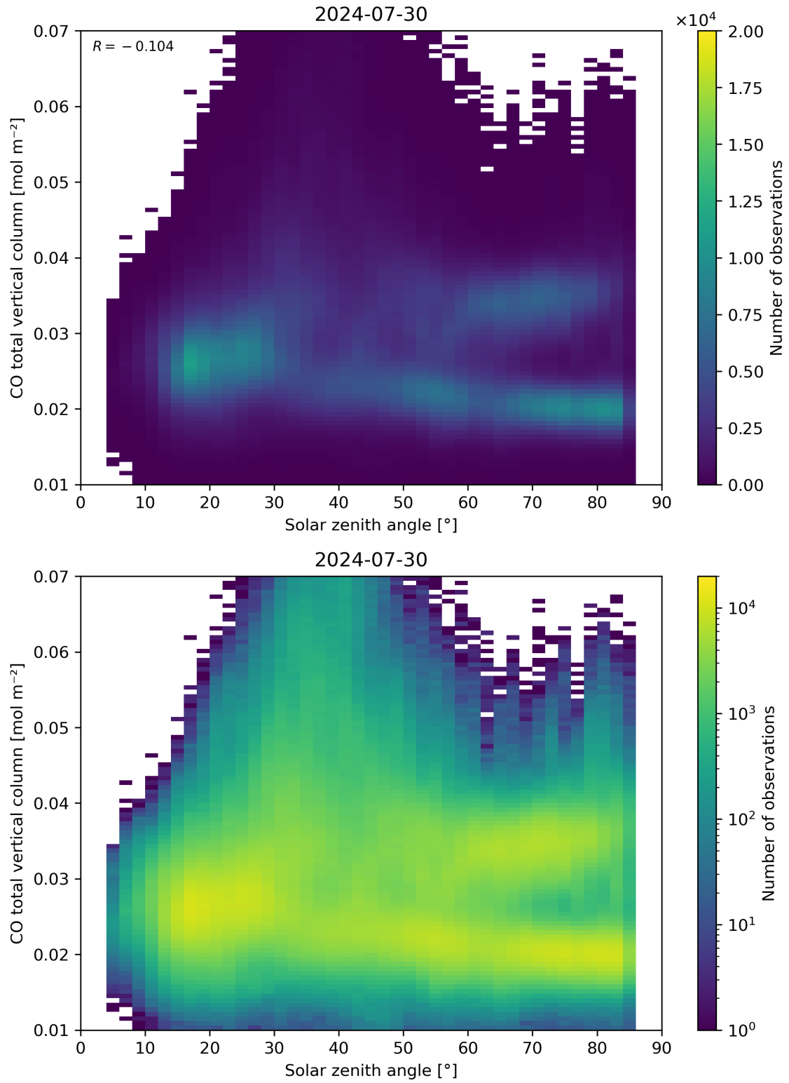
Figure 61: Scatter density plot of “Solar zenith angle” against “CO total vertical column” for 2024-07-29 to 2024-07-31.
