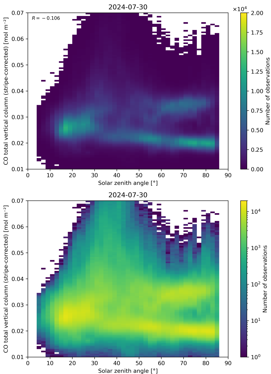
Figure 62: Scatter density plot of “Solar zenith angle” against “CO total vertical column (stripe-corrected)” for 2024-07-29 to 2024-07-31.
