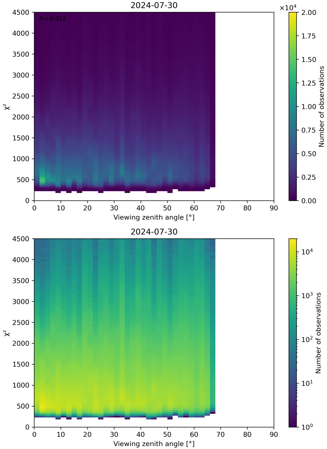
Figure 72: Scatter density plot of “Viewing zenith angle” against “ \chi^2 ” for 2024-07-29 to 2024-07-31.
