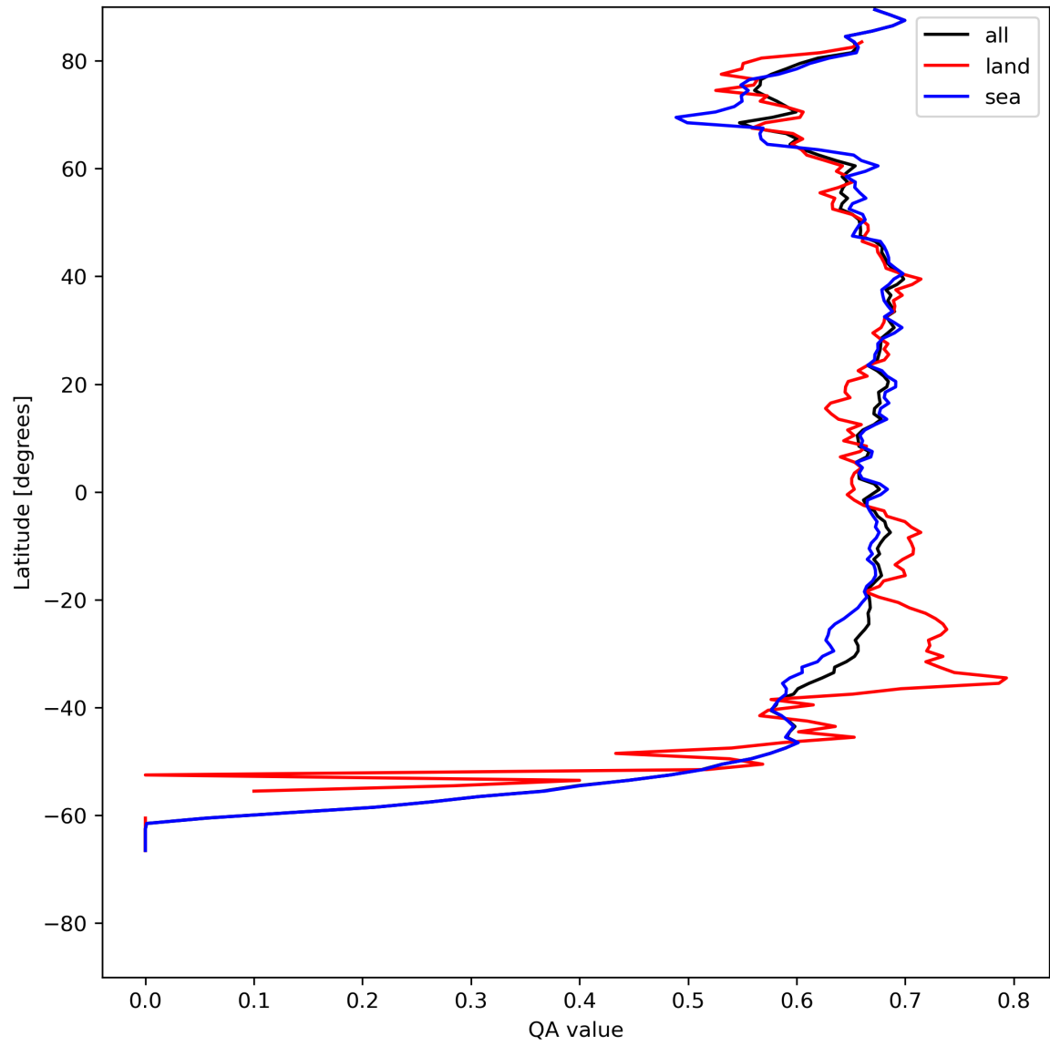
Figure 9: Zonal average of “QA value” for 2024-07-29 to 2024-07-31.
