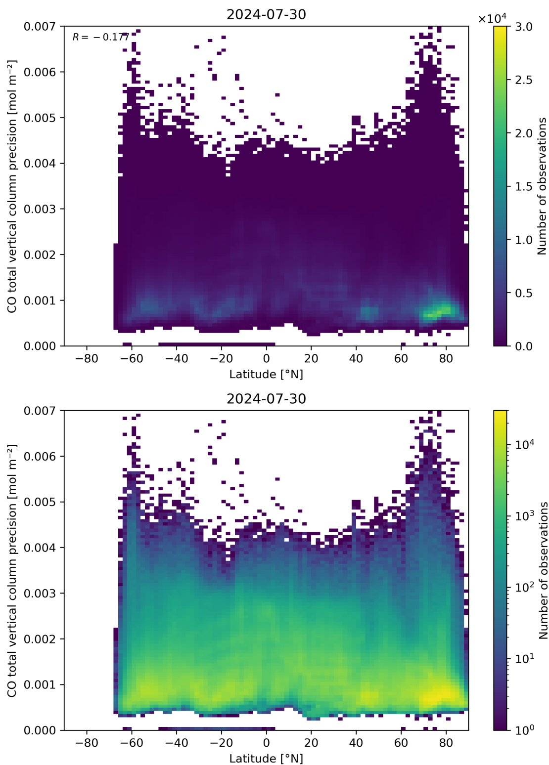
Figure 53: Scatter density plot of “Latitude” against “CO total vertical column precision” for 2024-07-29 to 2024-07-31.
