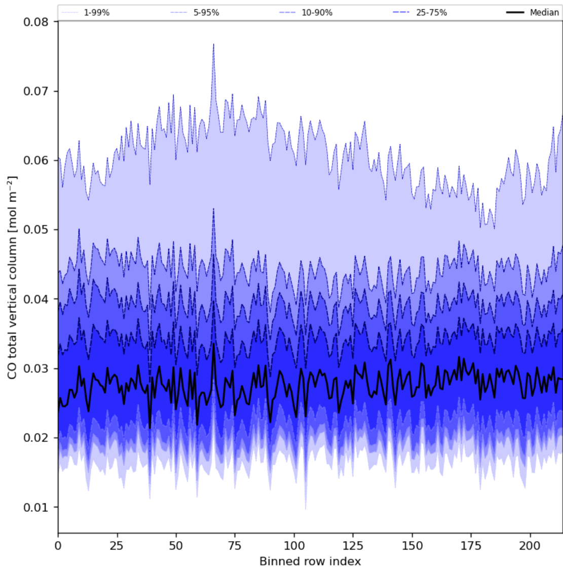
Figure 26: Along track statistics of “CO total vertical column” for 2024-07-29 to 2024-07-31
