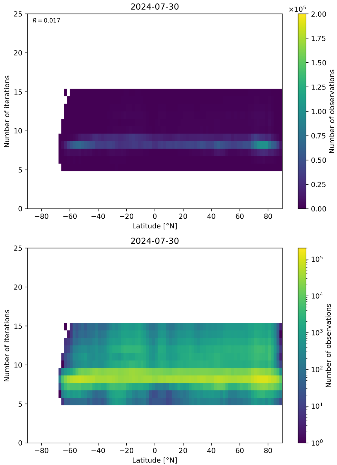
Figure 56: Scatter density plot of “Latitude” against “Number of iterations” for 2024-07-29 to 2024-07-31.
