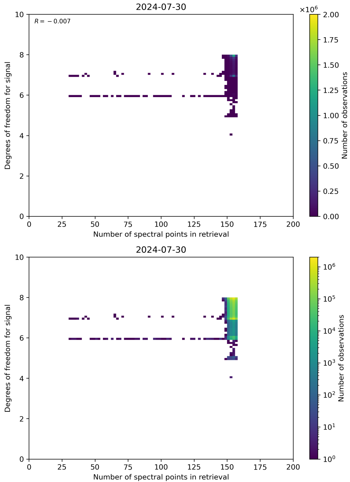
Figure 59: Scatter density plot of “Number of spectral points in retrieval” against “Degrees of freedom for signal” for 2024-07-29 to 2024-07-31.
