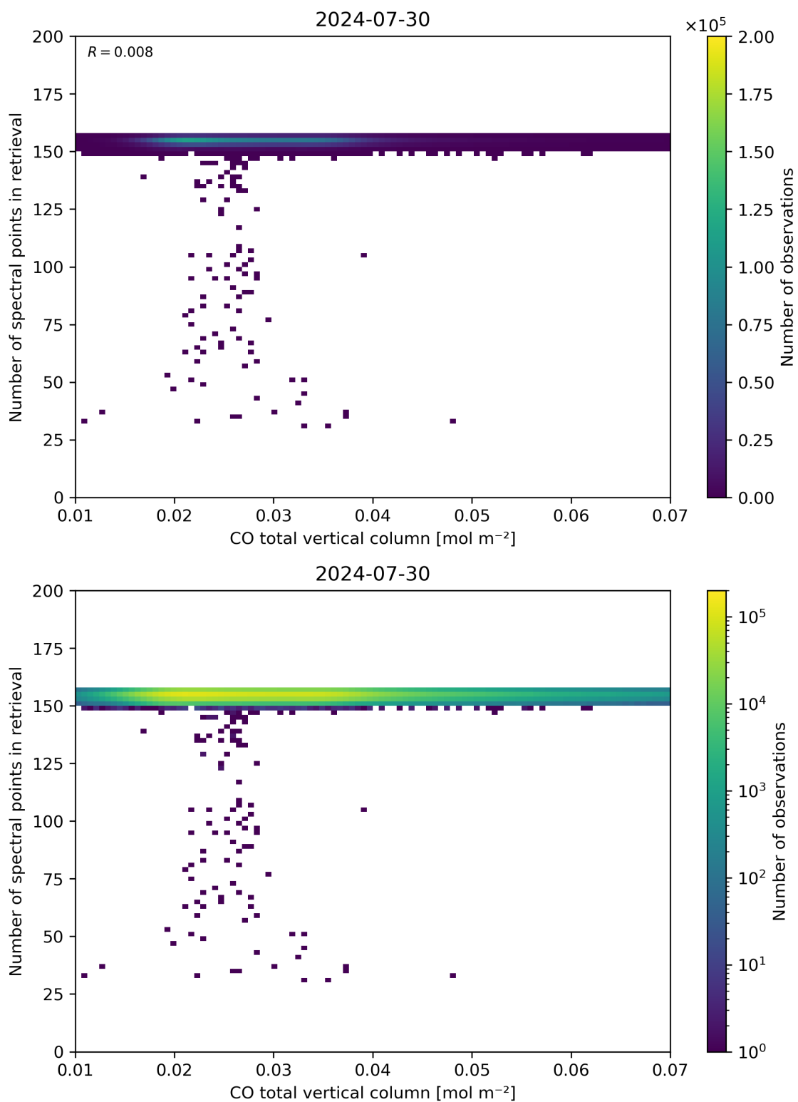
Figure 43: Scatter density plot of “CO total vertical column” against “Number of spectral points in retrieval” for 2024-07-29 to 2024-07-31.
