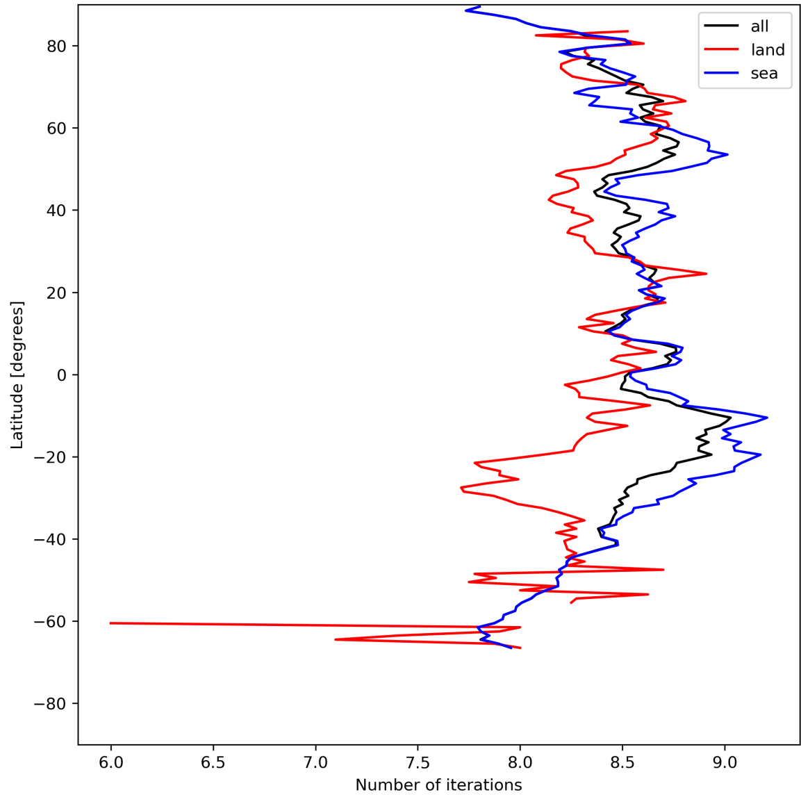
Figure 16: Zonal average of “Number of iterations” for 2024-07-29 to 2024-07-31.
