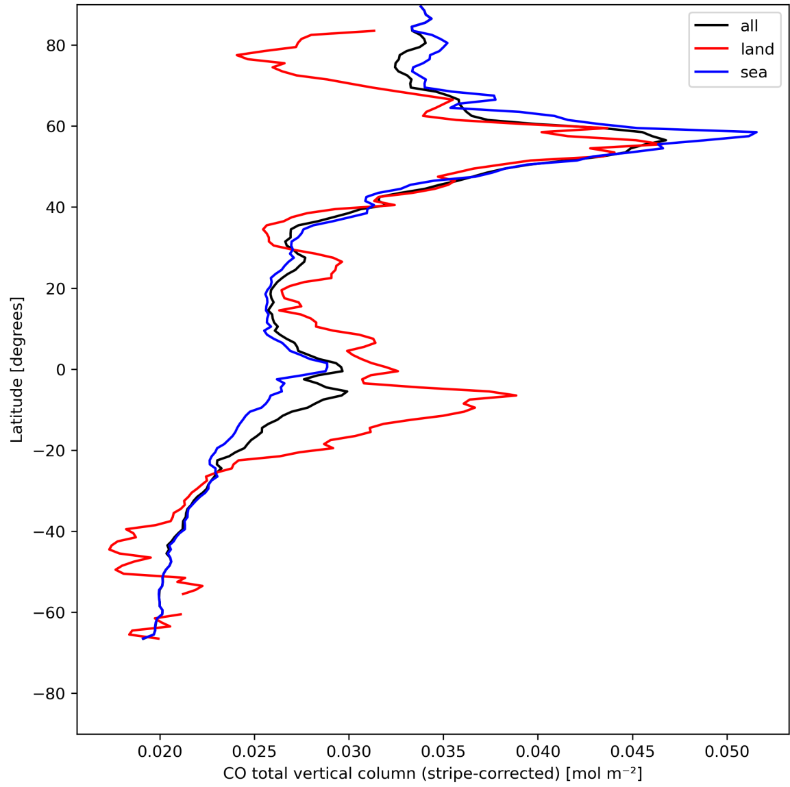
Figure 11: Zonal average of “CO total vertical column (stripe-corrected)” for 2024-07-29 to 2024-07-31.
