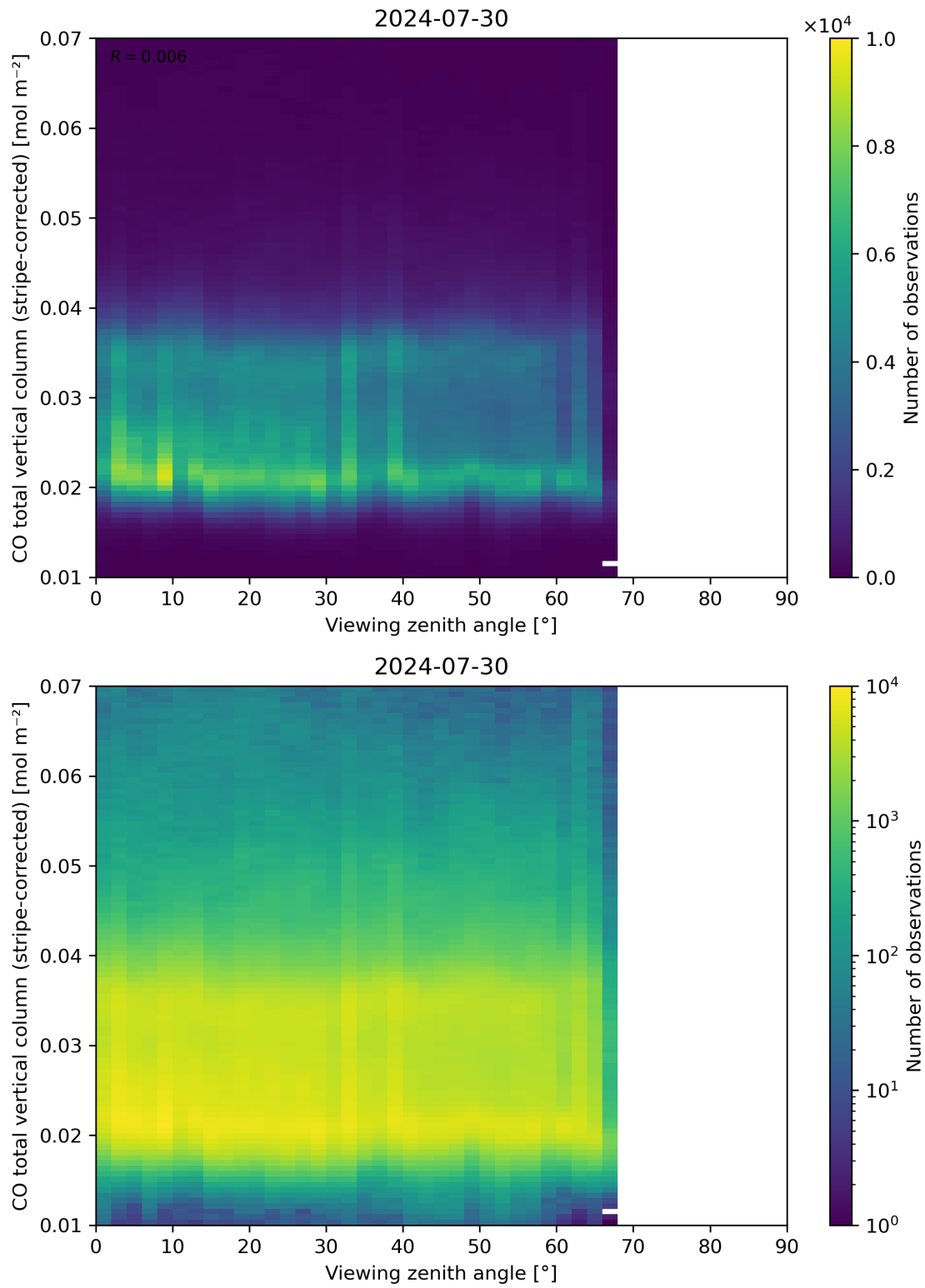
Figure 70: Scatter density plot of “Viewing zenith angle” against “CO total vertical column (stripe-corrected)” for 2024-07-29 to 2024-07-31.
