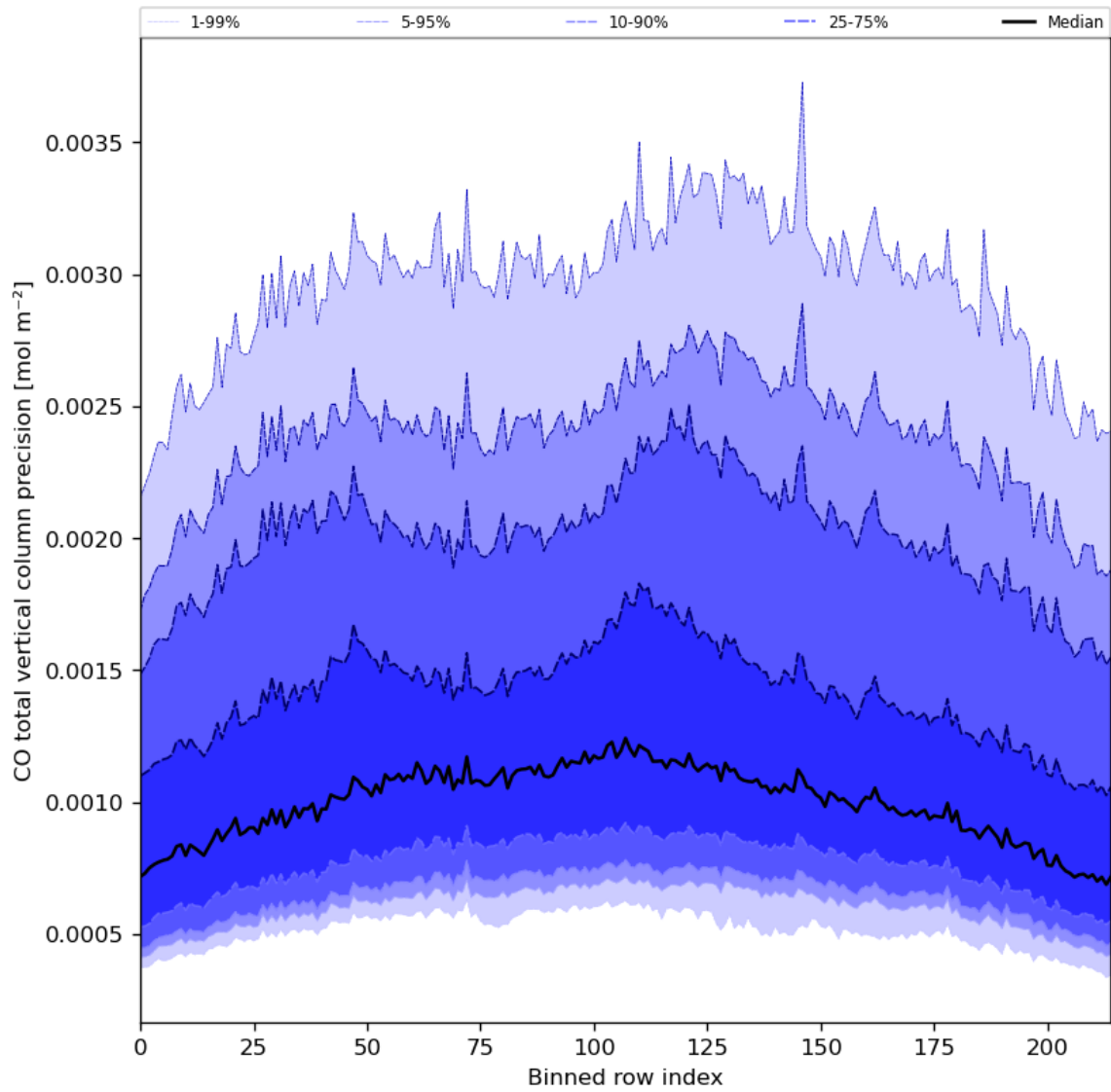
Figure 28: Along track statistics of “CO total vertical column precision” for 2024-07-29 to 2024-07-31
