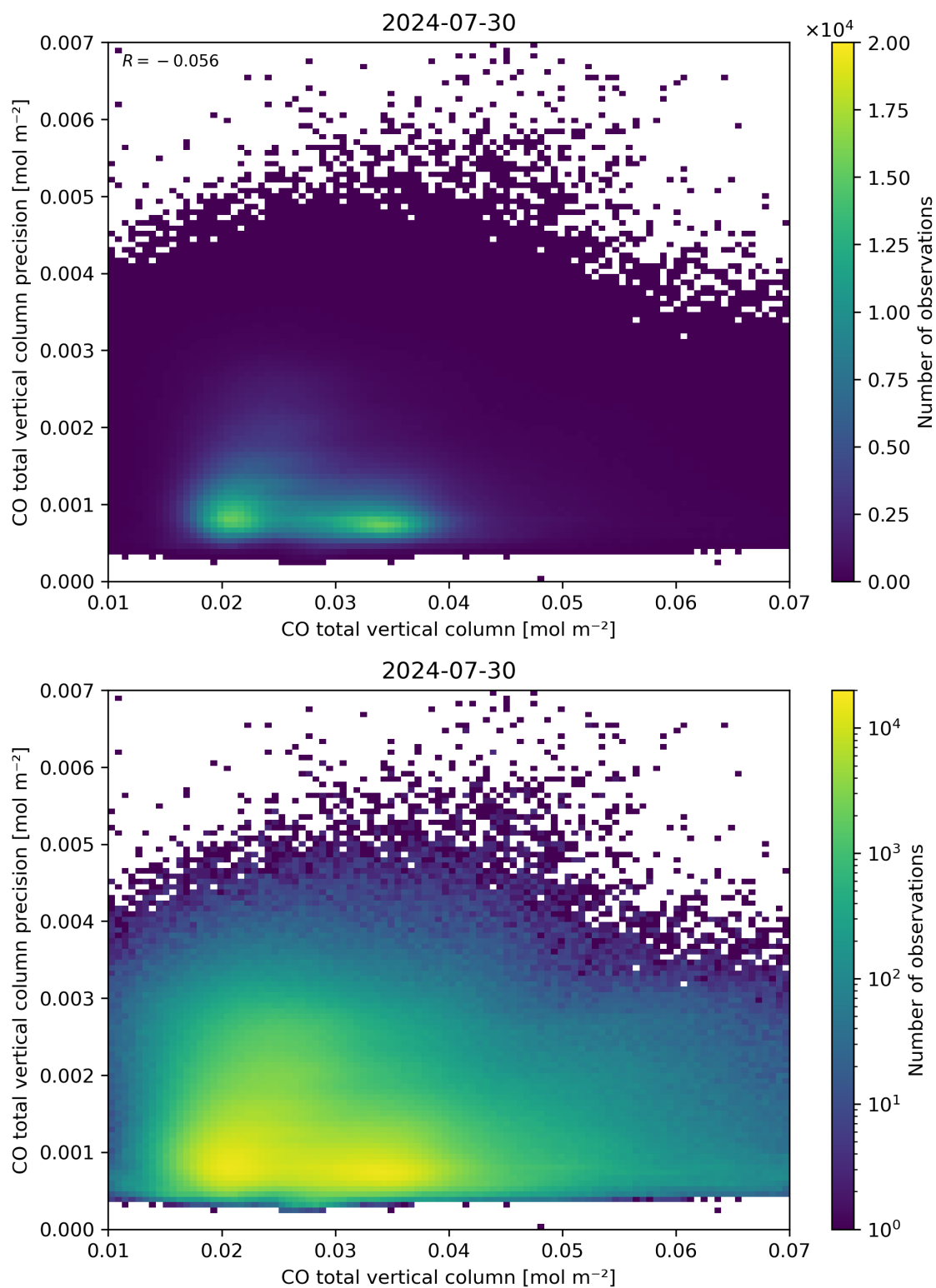
Figure 34: Scatter density plot of “CO total vertical column” against “CO total vertical column precision” for 2024-07-29 to 2024-07-31.
