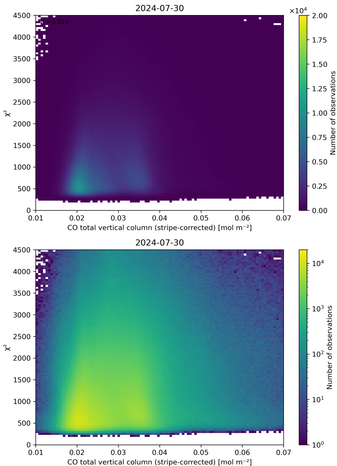
Figure 37: Scatter density plot of “CO total vertical column (stripe-corrected)” against “ \chi^2 ” for 2024-07-29 to 2024-07-31.
