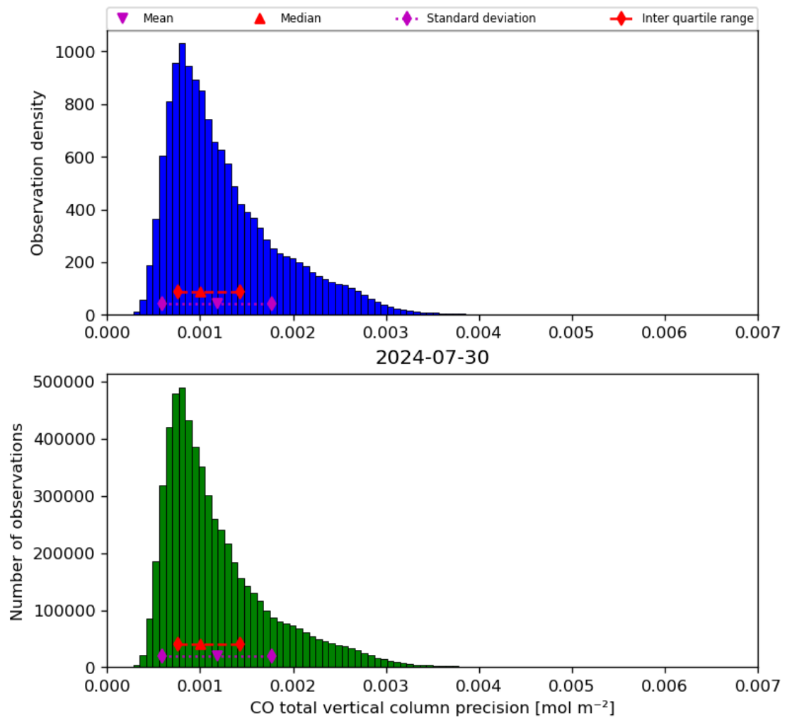
Figure 20: Histogram of “CO total vertical column precision” for 2024-07-29 to 2024-07-31
