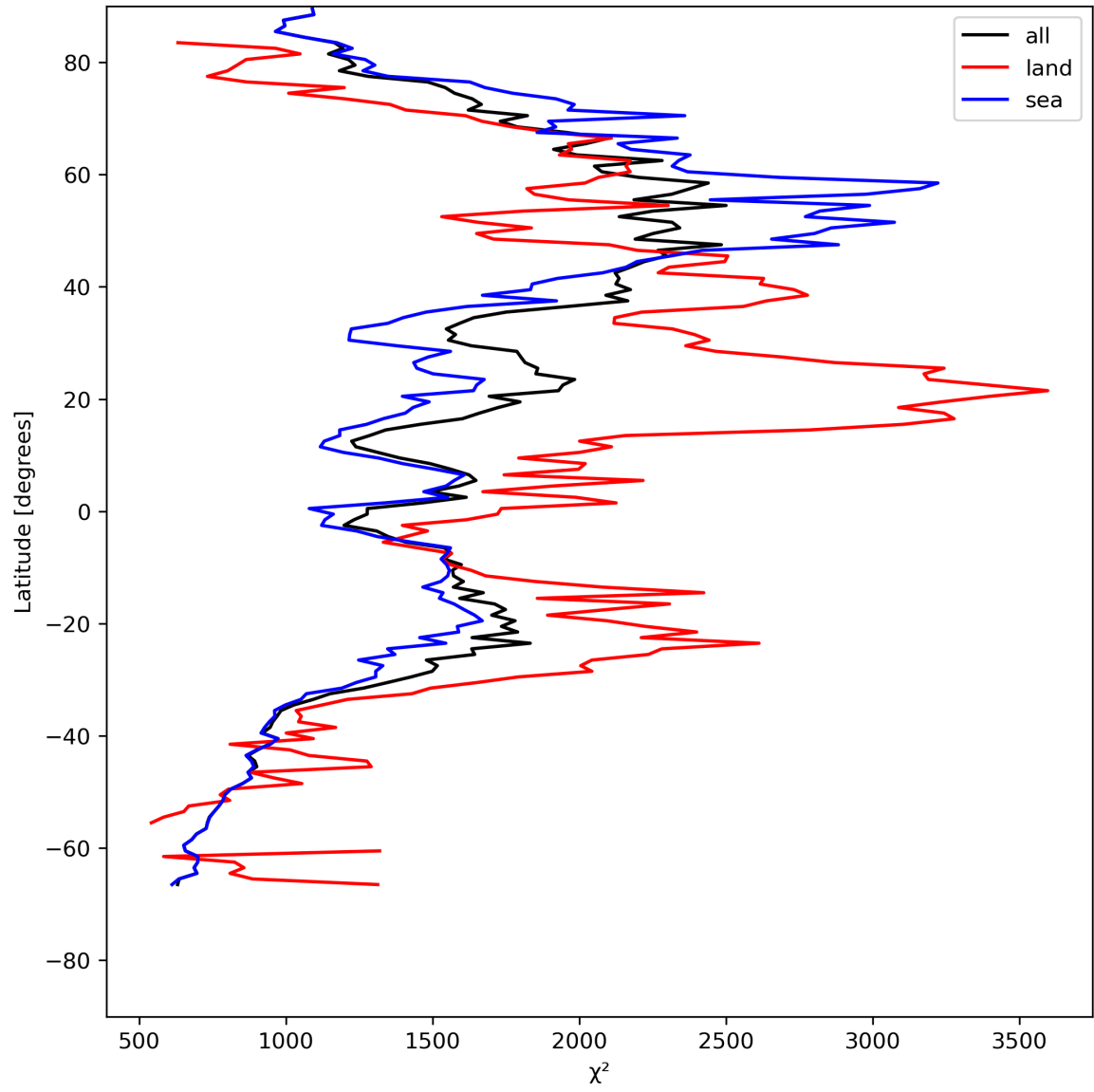
Figure 14: Zonal average of “ \chi^2 ” for 2024-07-29 to 2024-07-31.
