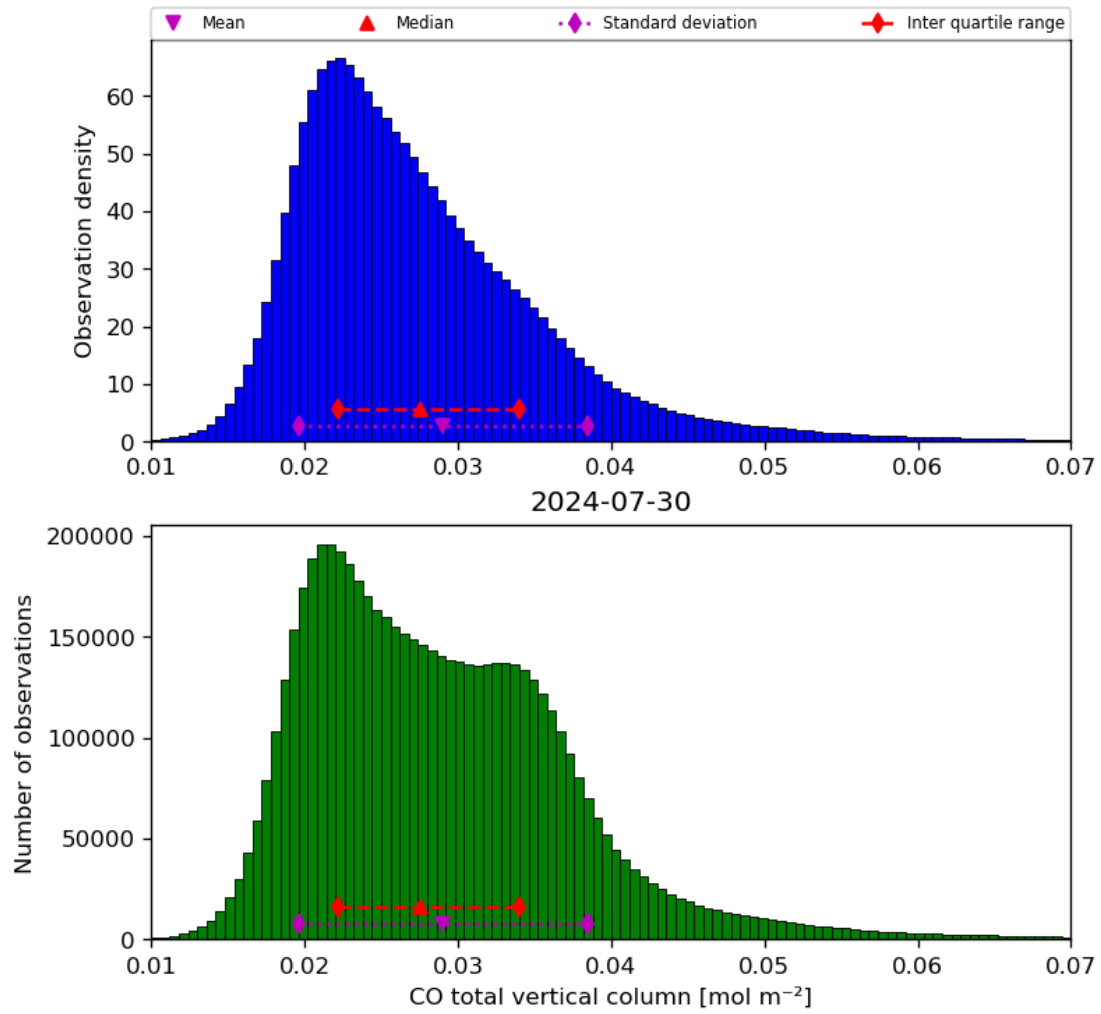
Figure 18: Histogram of “CO total vertical column” for 2024-07-29 to 2024-07-31
