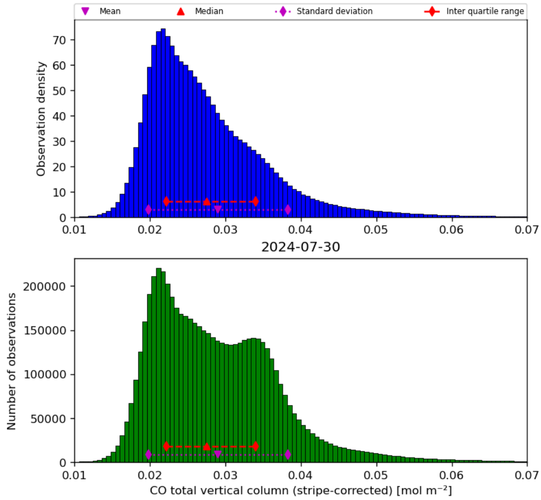
Figure 19: Histogram of “CO total vertical column (stripe-corrected)” for 2024-07-29 to 2024-07-31
