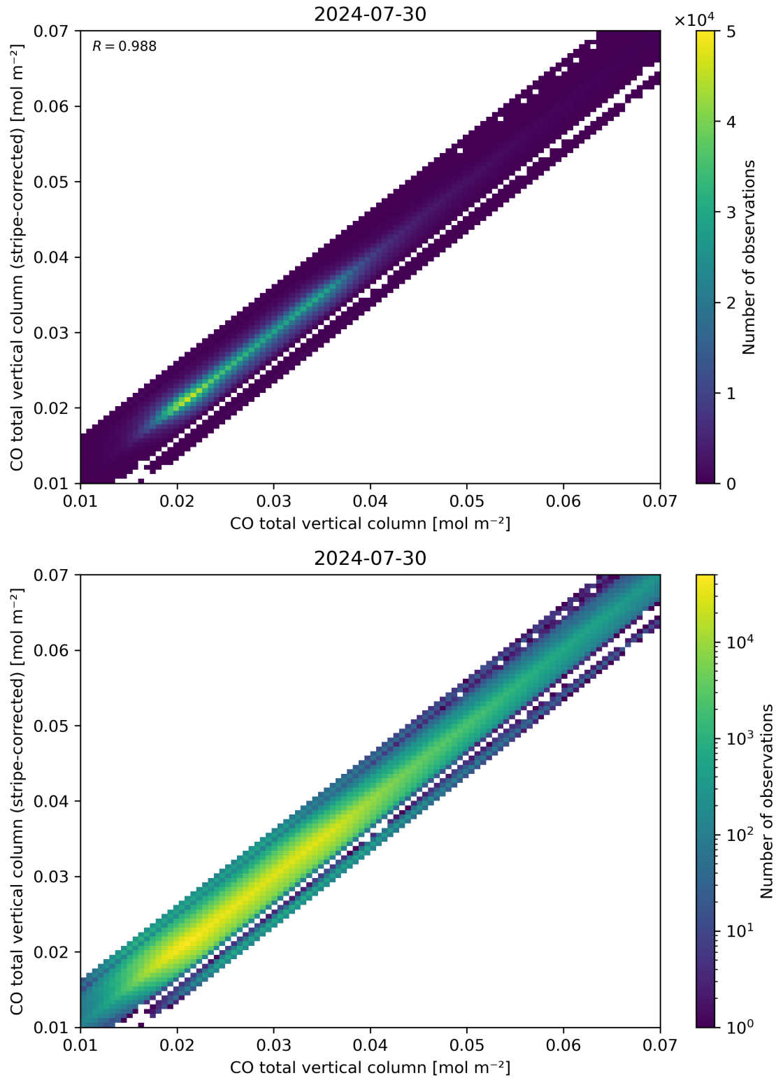
Figure 33: Scatter density plot of “CO total vertical column” against “CO total vertical column (stripe-corrected)” for 2024-07-29 to 2024-07-31.
