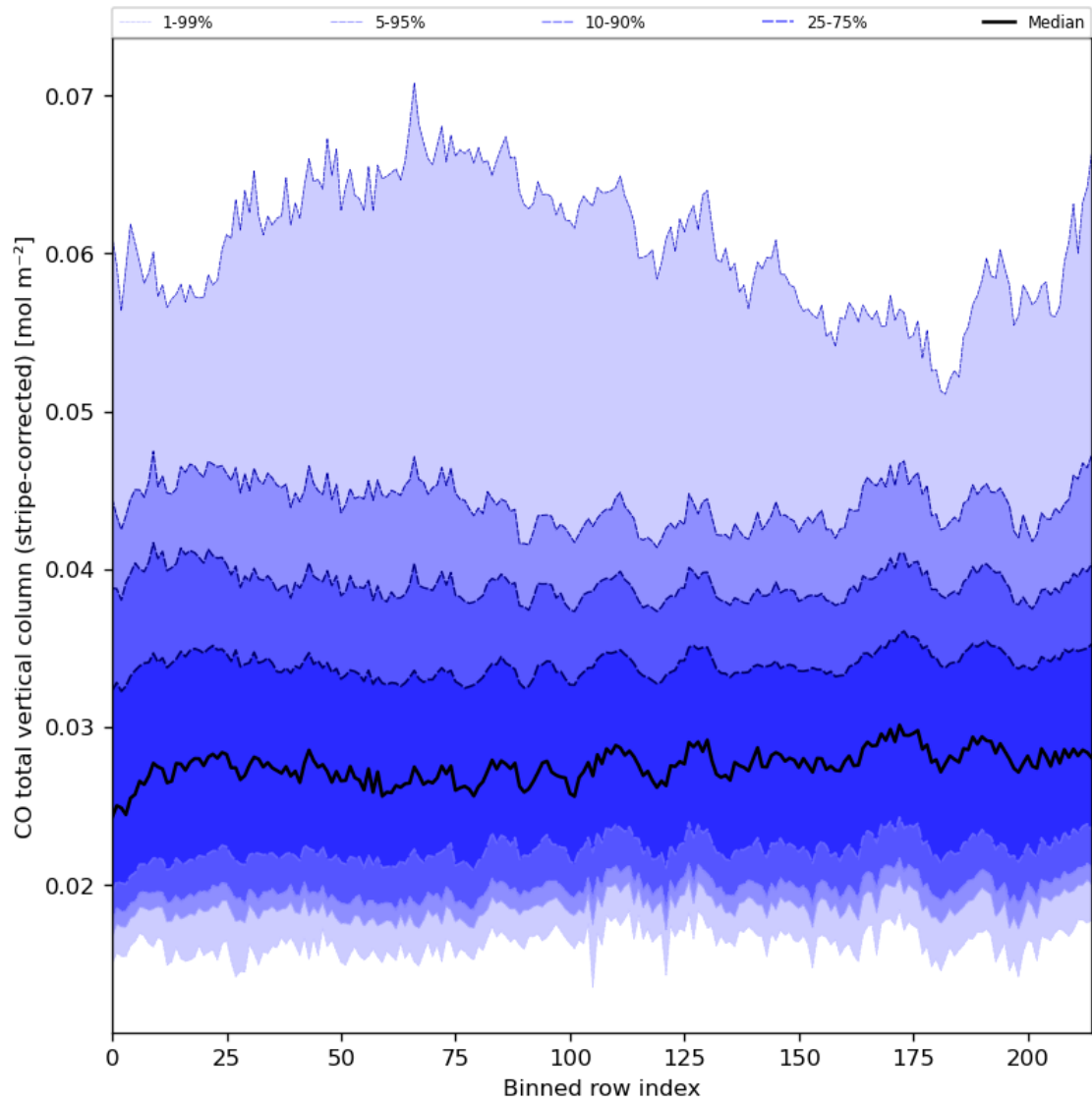
Figure 27: Along track statistics of “CO total vertical column (stripe-corrected)” for 2024-07-29 to 2024-07-31
