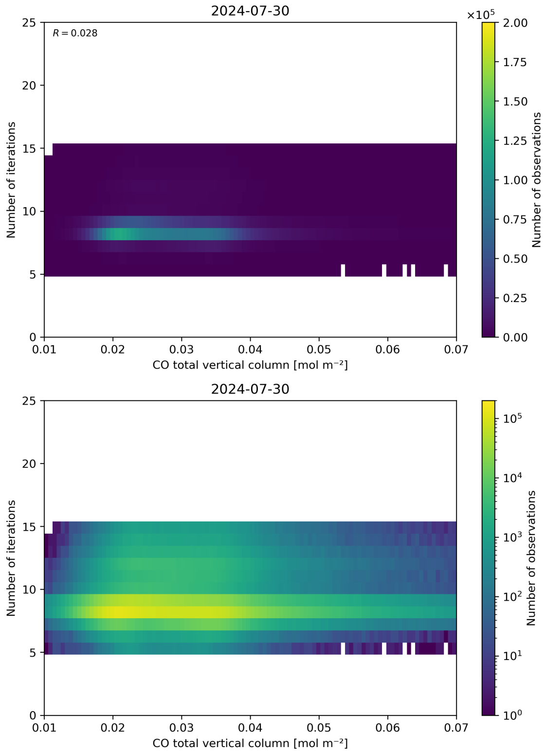
Figure 42: Scatter density plot of “CO total vertical column” against “Number of iterations” for 2024-07-29 to 2024-07-31.
