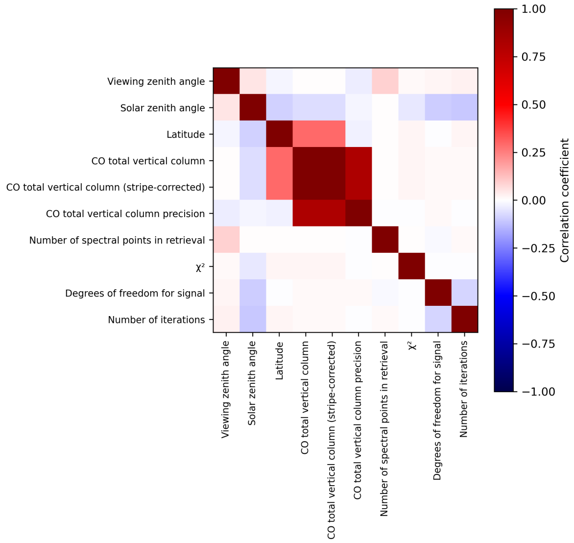
Figure 2: Map of correlation matrix for 2024-07-31 to 2024-08-01.
