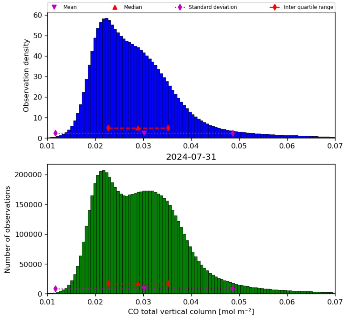
Figure 18: Histogram of “CO total vertical column” for 2024-07-31 to 2024-08-01
