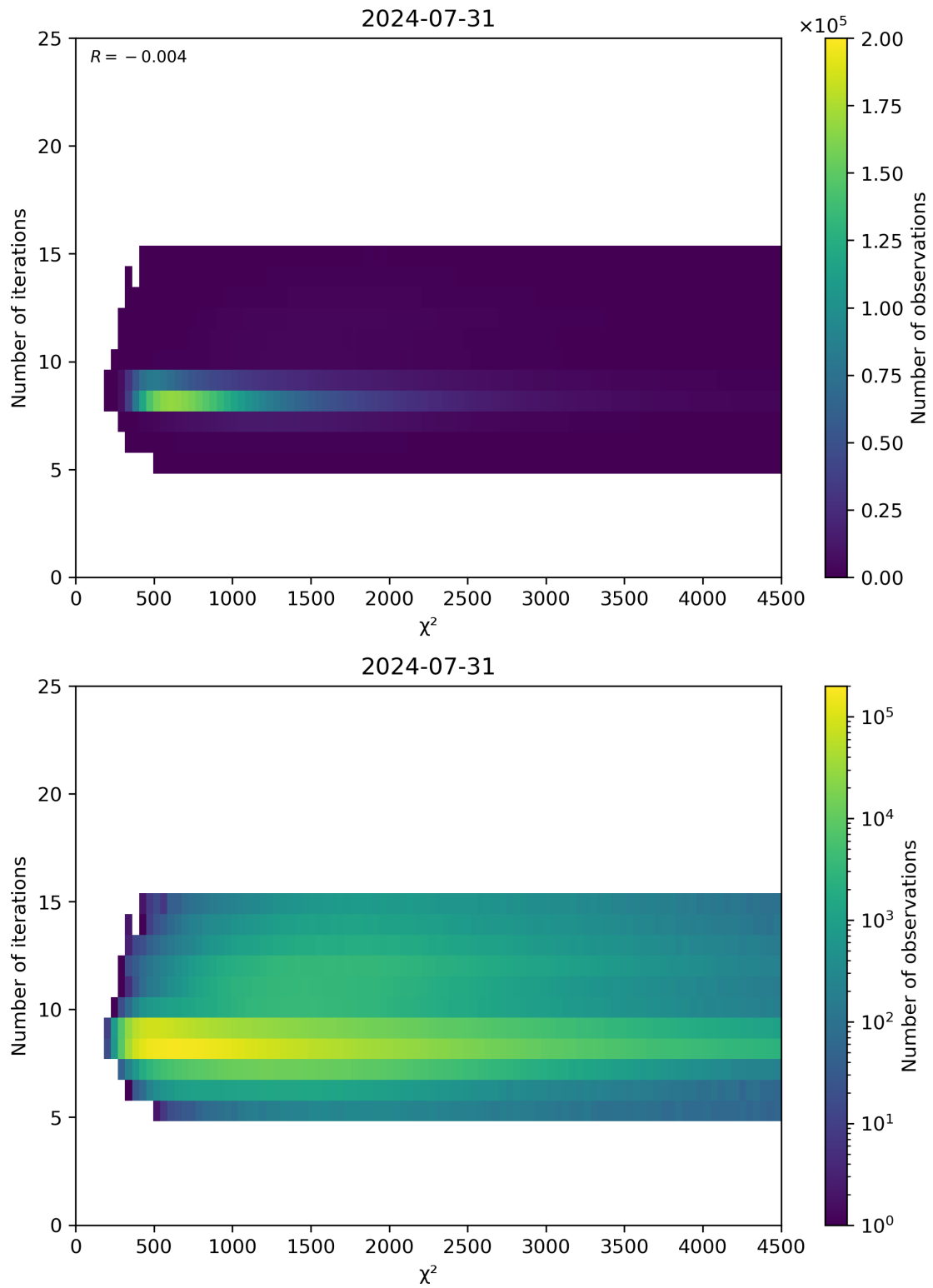
Figure 49: Scatter density plot of “ \chi^2 ” against “Number of iterations” for 2024-07-31 to 2024-08-01.
