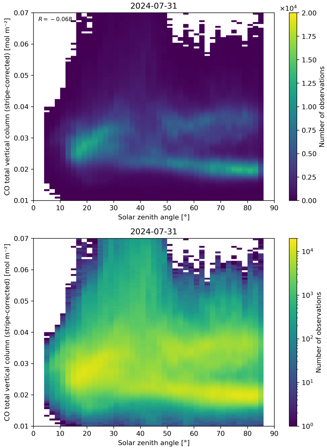
Figure 62: Scatter density plot of “Solar zenith angle” against “CO total vertical column (stripe-corrected)” for 2024-07-31 to 2024-08-01.
