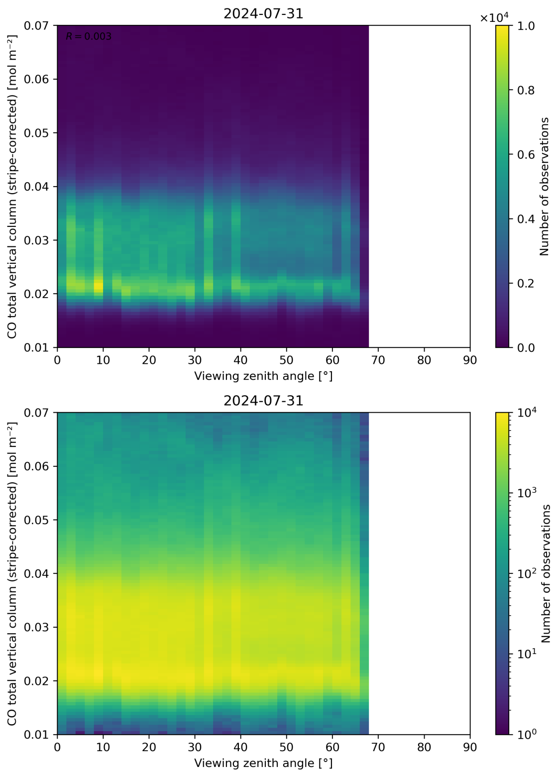
Figure 70: Scatter density plot of “Viewing zenith angle” against “CO total vertical column (stripe-corrected)” for 2024-07-31 to 2024-08-01.
