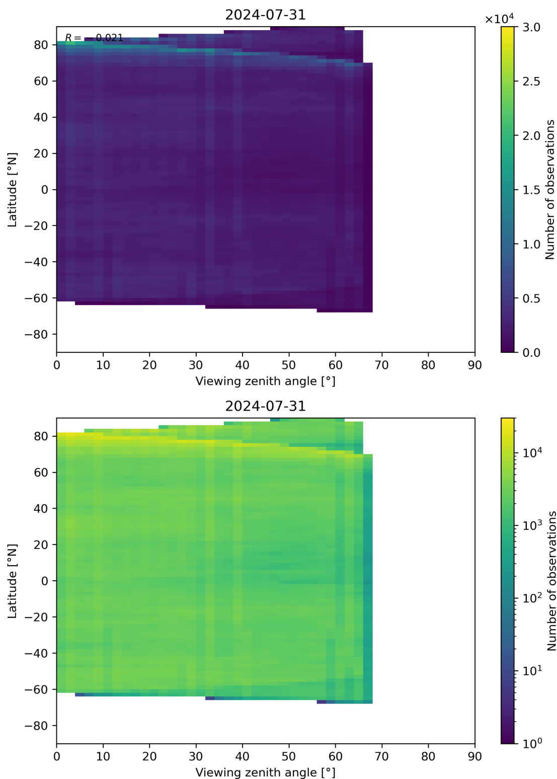
Figure 74: Scatter density plot of “Viewing zenith angle” against “Latitude” for 2024-07-31 to 2024-08-01.
