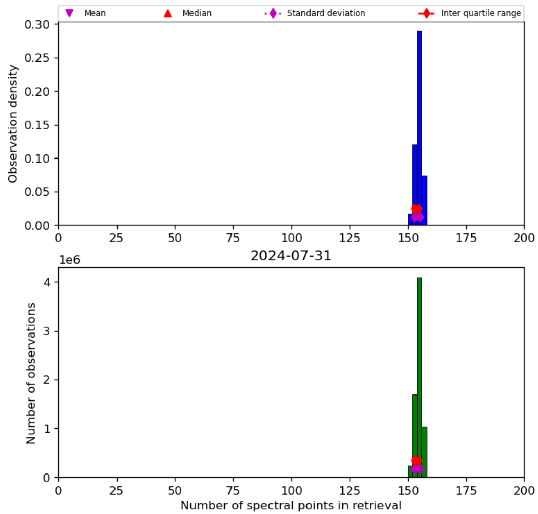
Figure 21: Histogram of “Number of spectral points in retrieval” for 2024-07-31 to 2024-08-01
