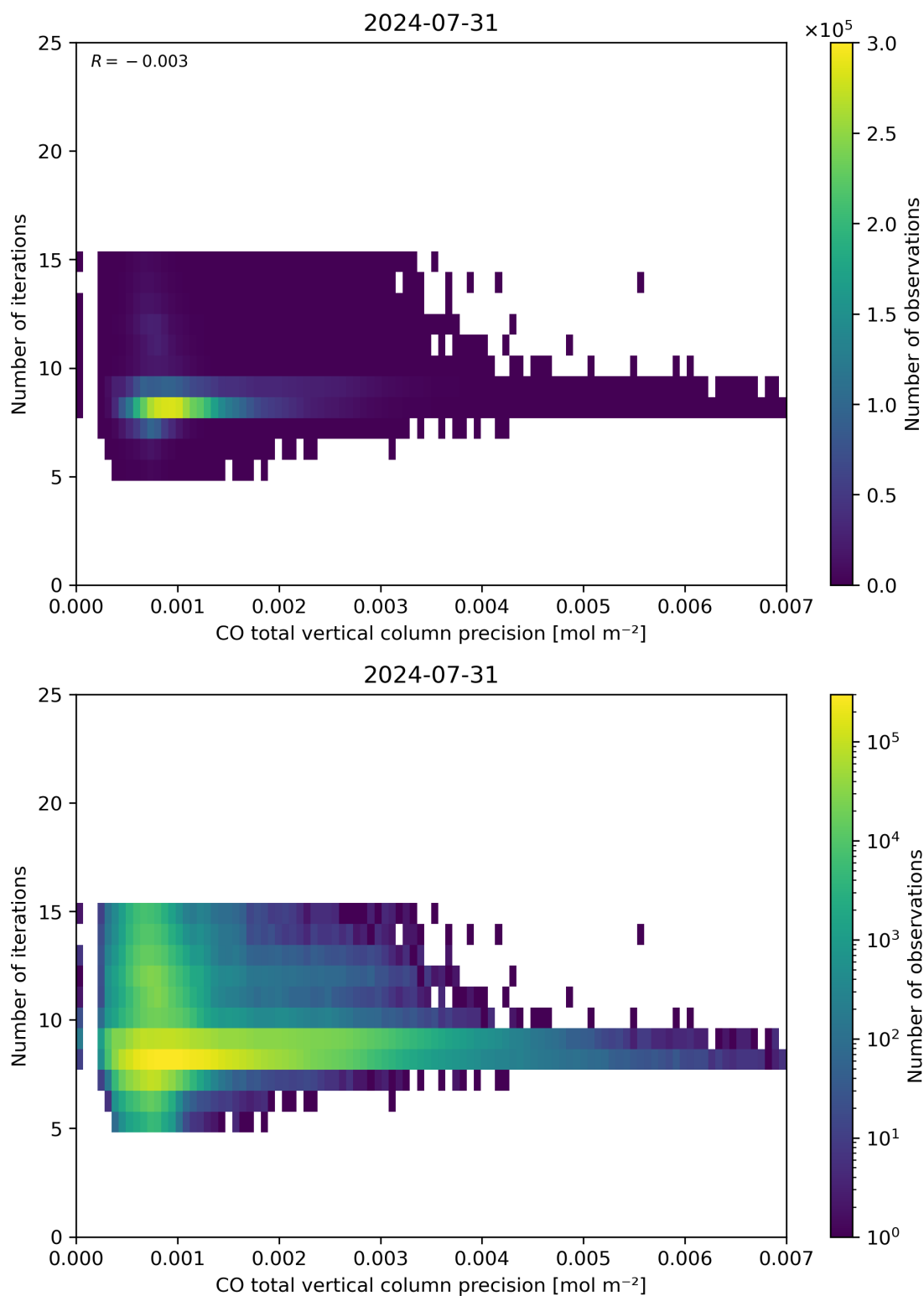
Figure 46: Scatter density plot of “CO total vertical column precision” against “Number of iterations” for 2024-07-31 to 2024-08-01.
