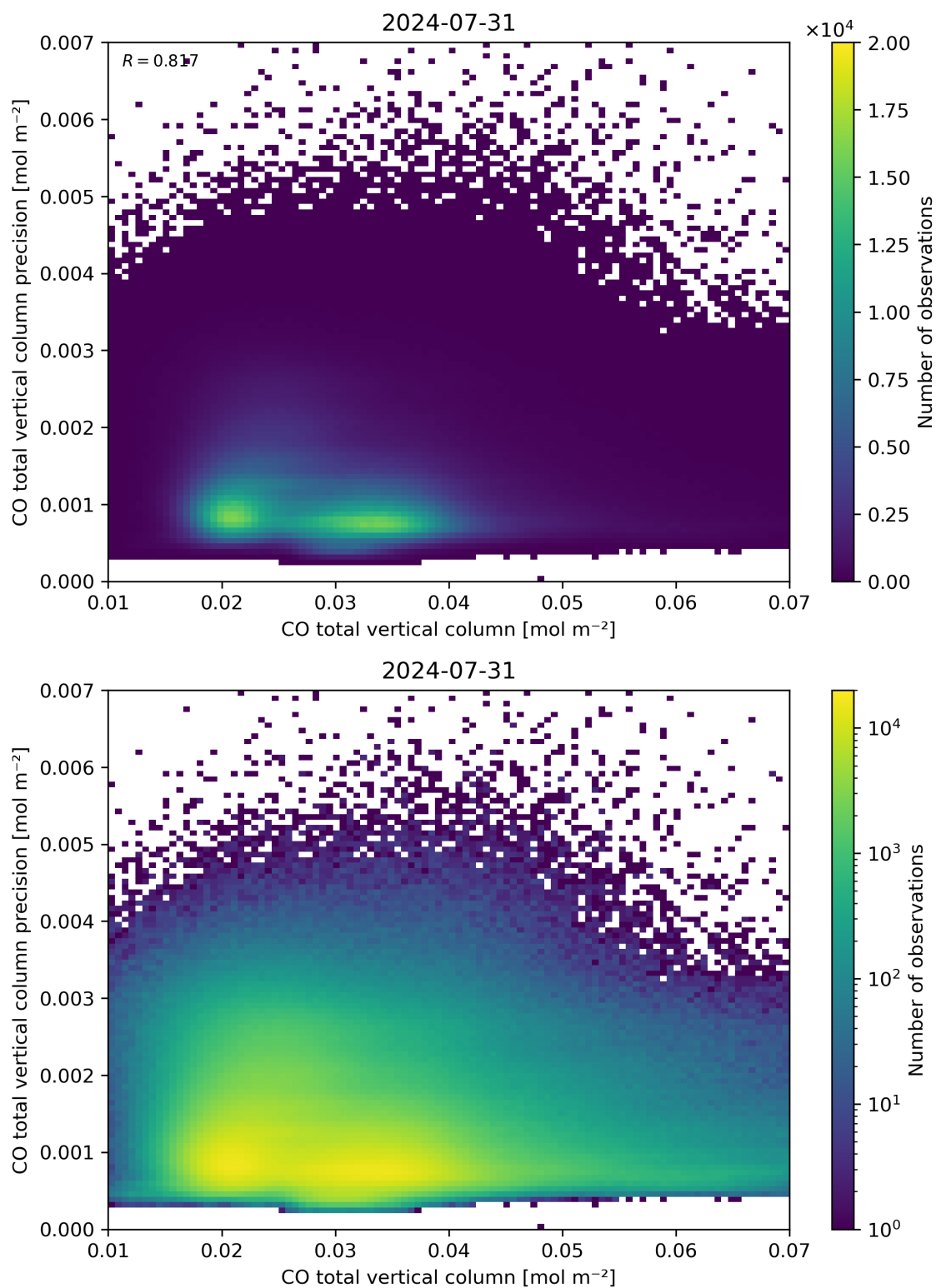
Figure 34: Scatter density plot of “CO total vertical column” against “CO total vertical column precision” for 2024-07-31 to 2024-08-01.
