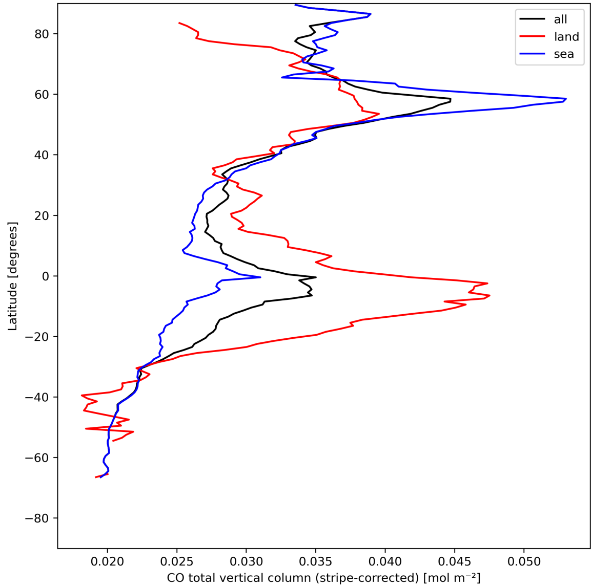
Figure 11: Zonal average of “CO total vertical column (stripe-corrected)” for 2024-07-31 to 2024-08-01.
