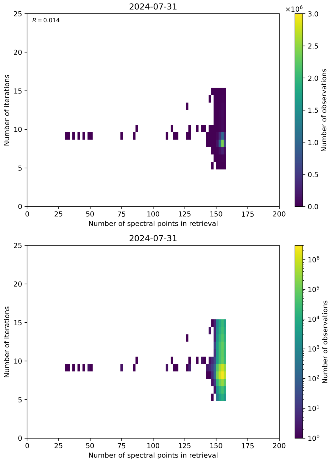
Figure 60: Scatter density plot of “Number of spectral points in retrieval” against “Number of iterations” for 2024-07-31 to 2024-08-01.
