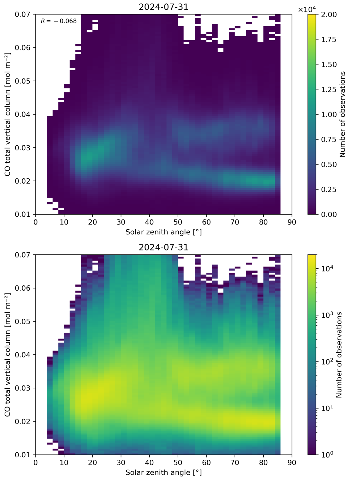
Figure 61: Scatter density plot of “Solar zenith angle” against “CO total vertical column” for 2024-07-31 to 2024-08-01.
