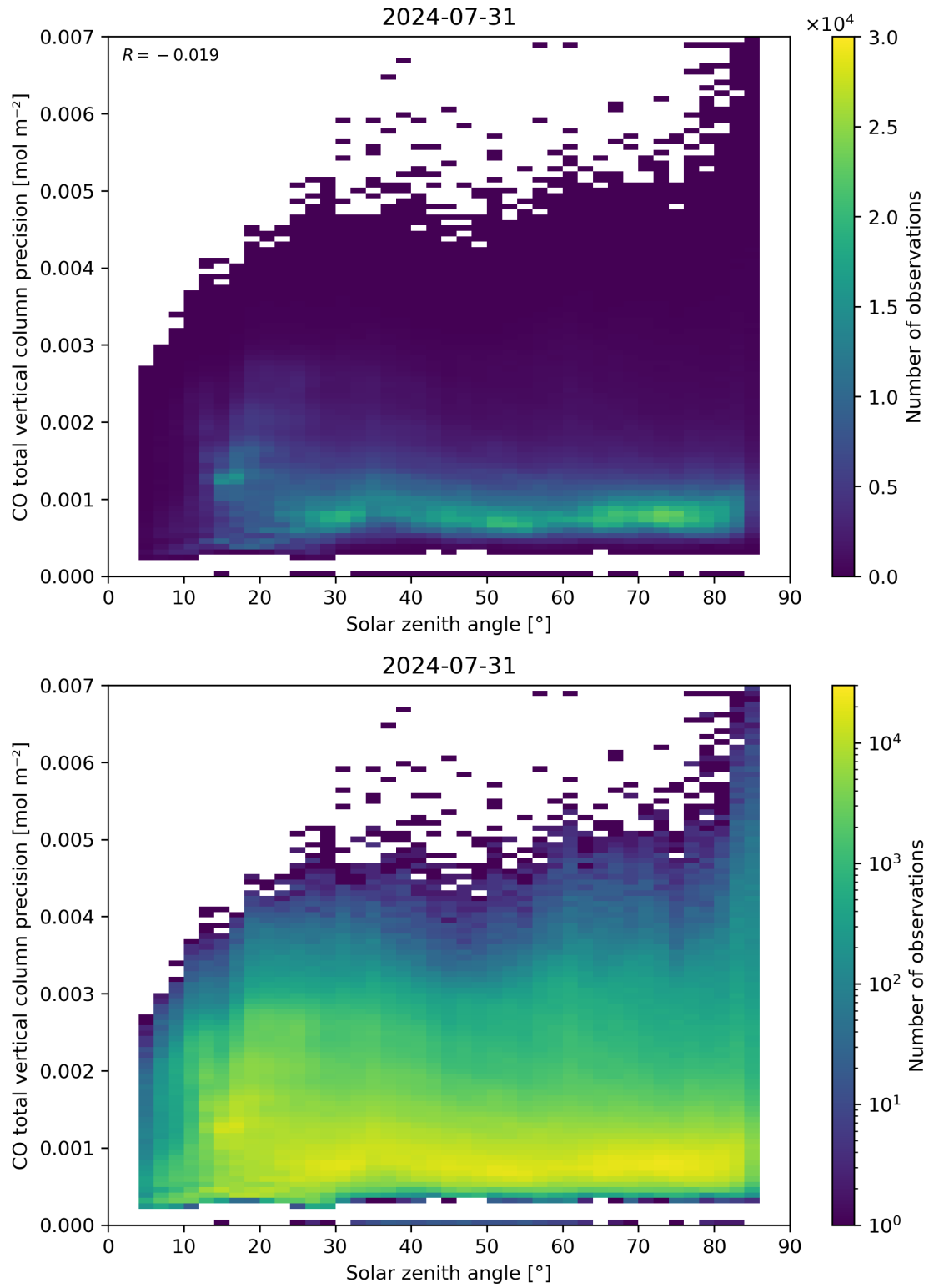
Figure 63: Scatter density plot of “Solar zenith angle” against “CO total vertical column precision” for 2024-07-31 to 2024-08-01.
