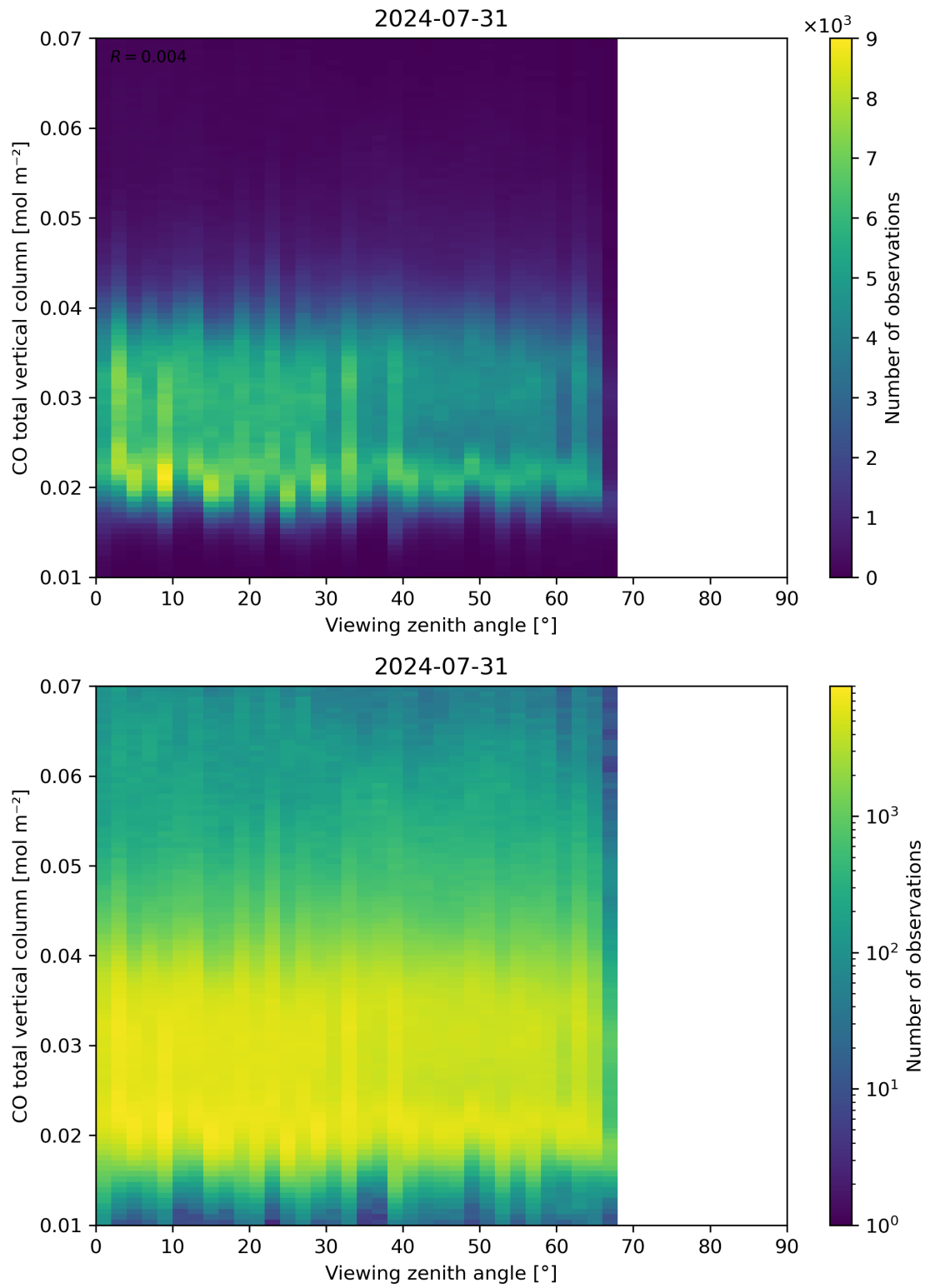
Figure 69: Scatter density plot of “Viewing zenith angle” against “CO total vertical column” for 2024-07-31 to 2024-08-01.
