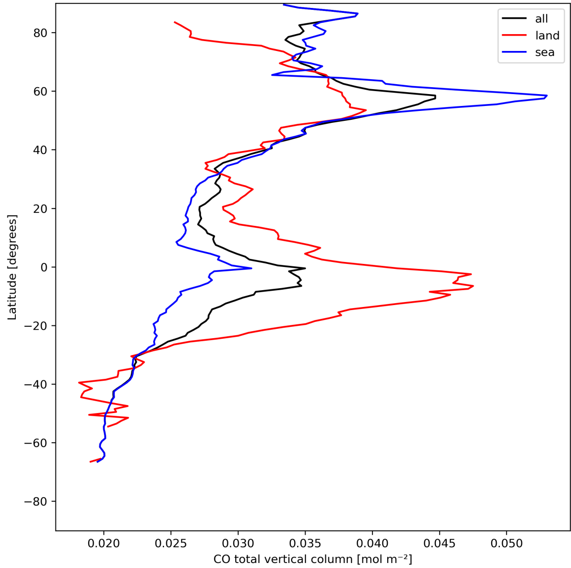
Figure 10: Zonal average of “CO total vertical column” for 2024-07-31 to 2024-08-01.
