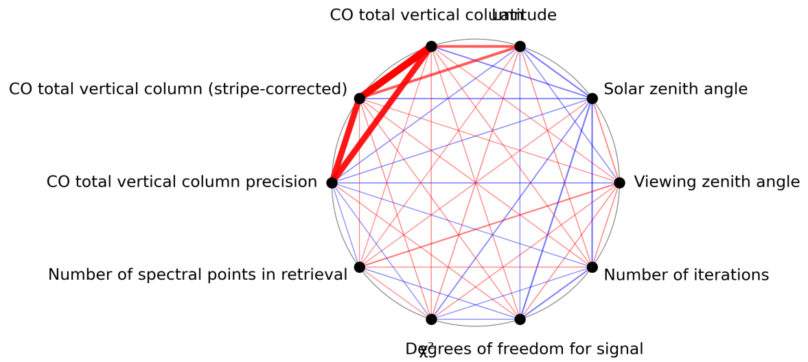
Figure 1: Map of correlation graph for 2024-07-31 to 2024-08-01.
