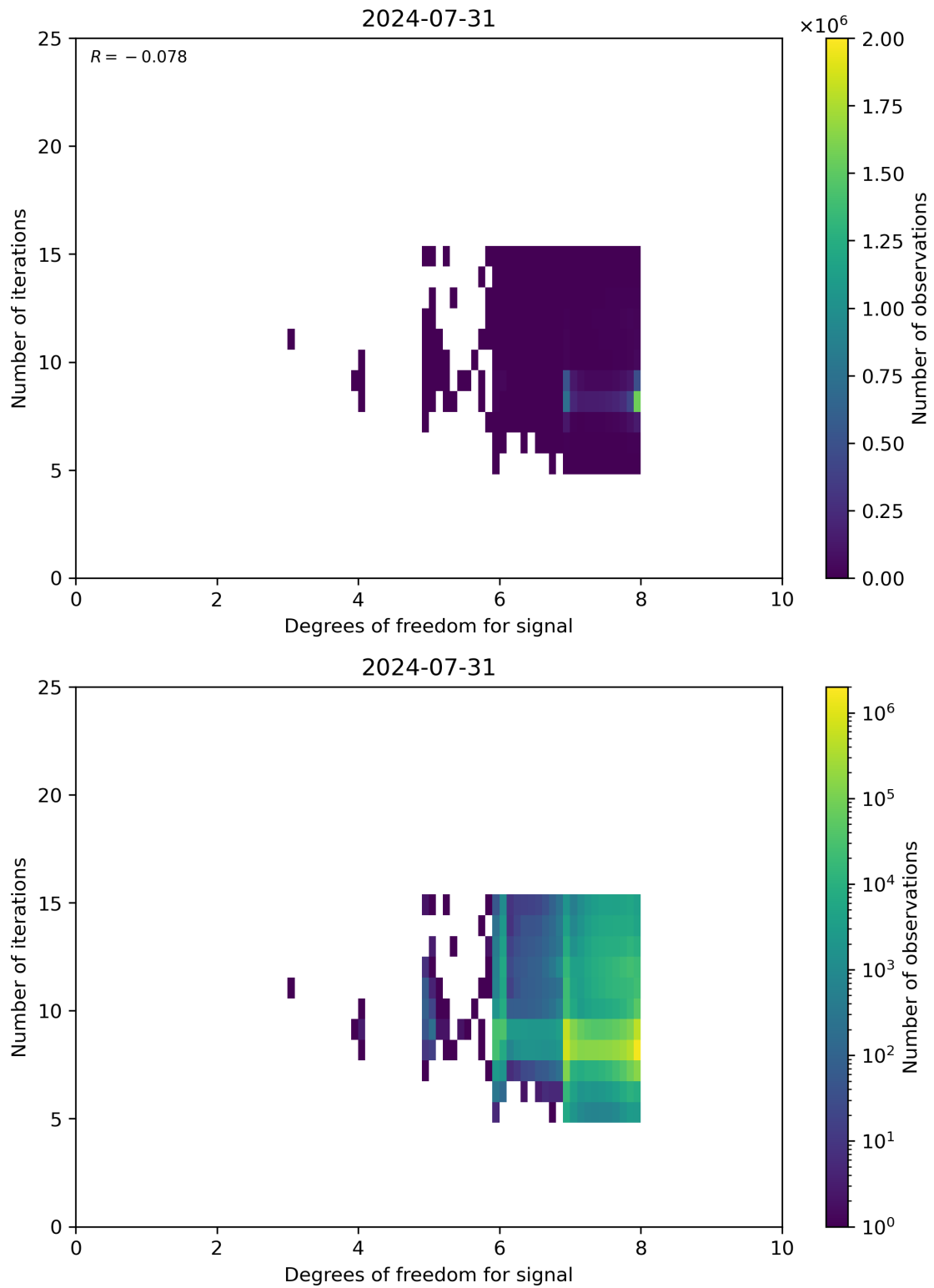
Figure 50: Scatter density plot of “Degrees of freedom for signal” against “Number of iterations” for 2024-07-31 to 2024-08-01.
