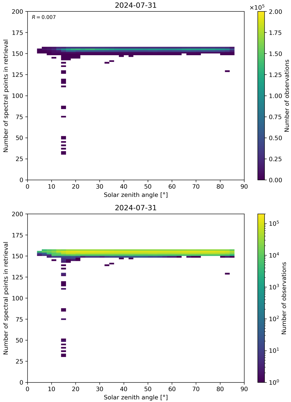
Figure 68: Scatter density plot of “Solar zenith angle” against “Number of spectral points in retrieval” for 2024-07-31 to 2024-08-01.
