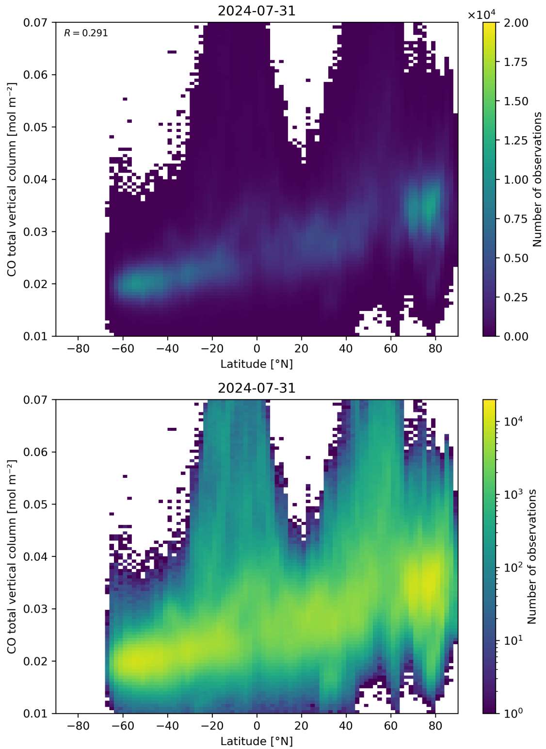
Figure 51: Scatter density plot of “Latitude” against “CO total vertical column” for 2024-07-31 to 2024-08-01.
