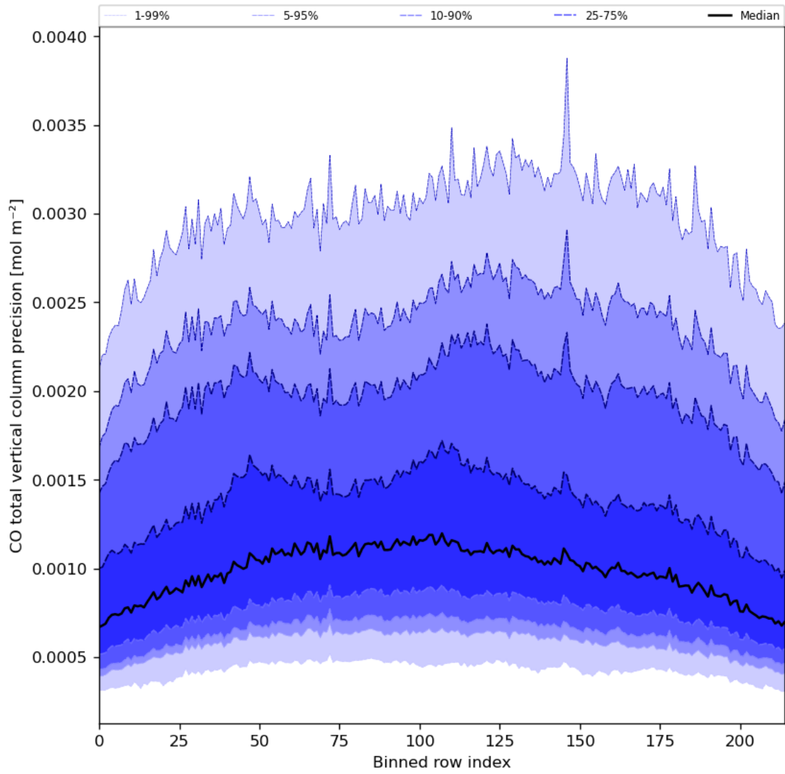
Figure 28: Along track statistics of “CO total vertical column precision” for 2024-07-31 to 2024-08-01
