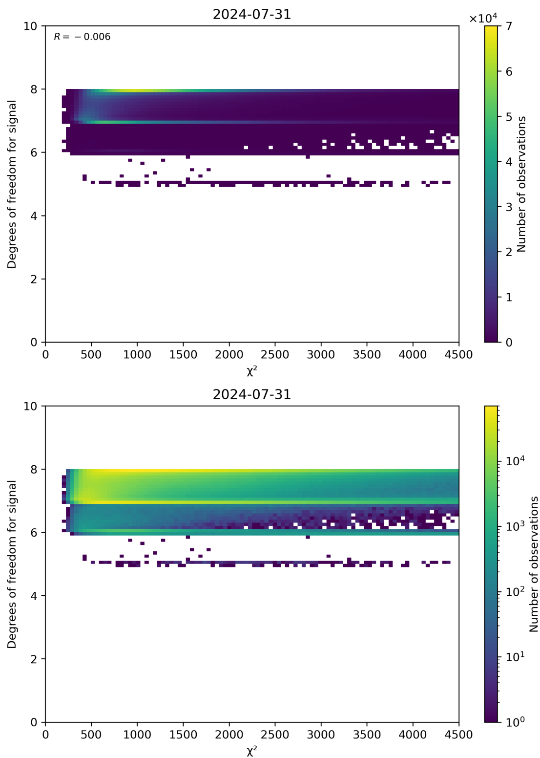
Figure 48: Scatter density plot of " \chi^2 " against "Degrees of freedom for signal" for 2024-07-31 to 2024-08-01.
