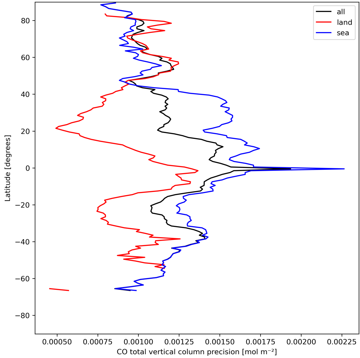
Figure 12: Zonal average of “CO total vertical column precision” for 2024-07-31 to 2024-08-01.
