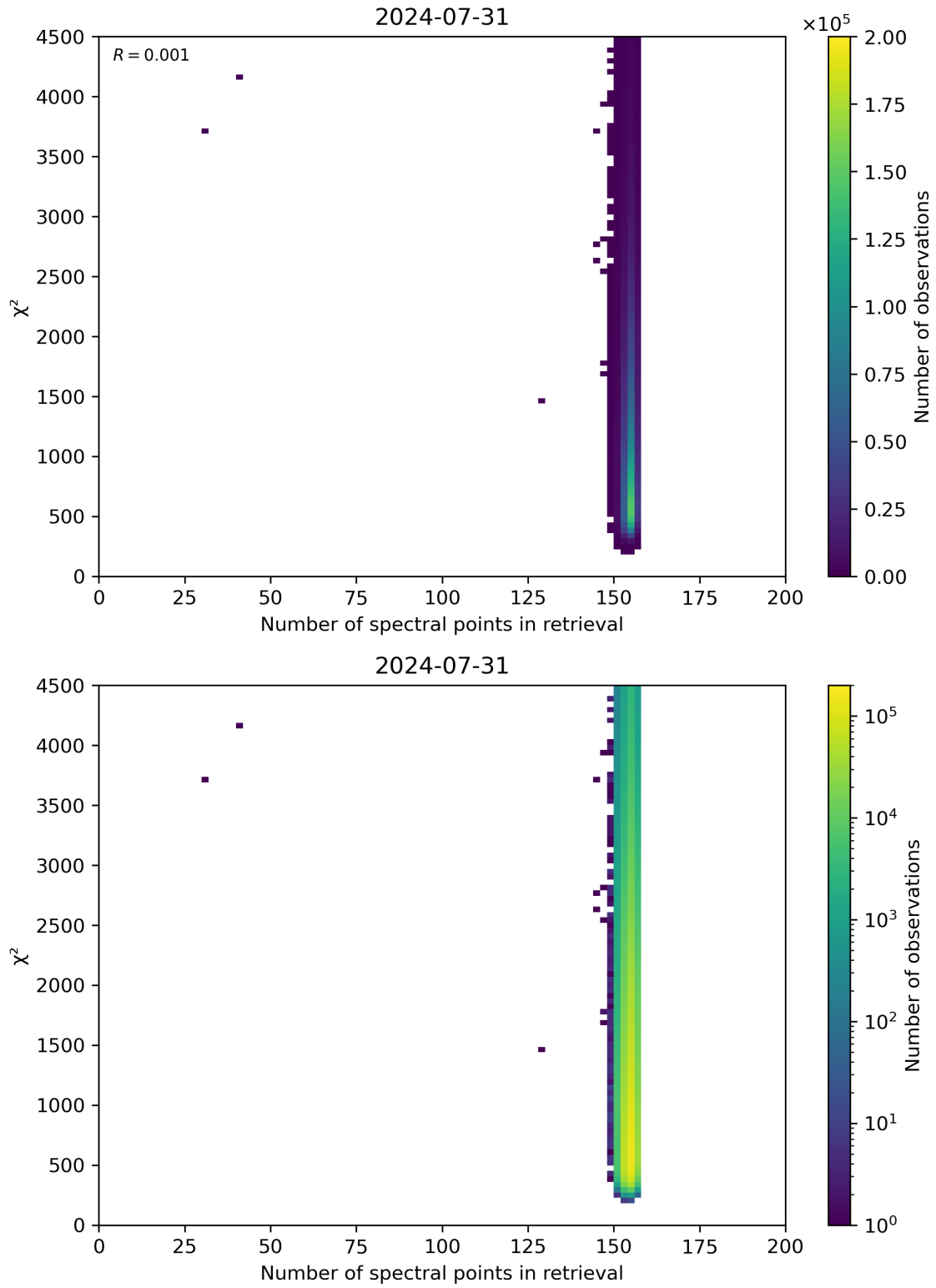
Figure 58: Scatter density plot of “Number of spectral points in retrieval” against “ \chi^2 ” for 2024-07-31 to 2024-08-01.
