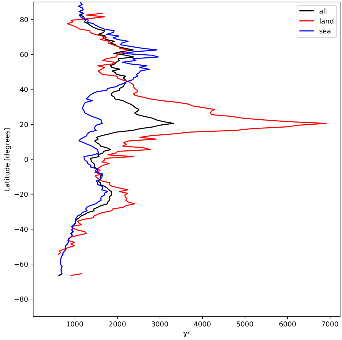
Figure 14: Zonal average of “ \chi^2 ” for 2024-07-31 to 2024-08-01.
