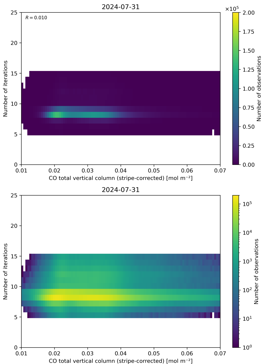
Figure 39: Scatter density plot of “CO total vertical column (stripe-corrected)” against “Number of iterations” for 2024-07-31 to 2024-08-01.
