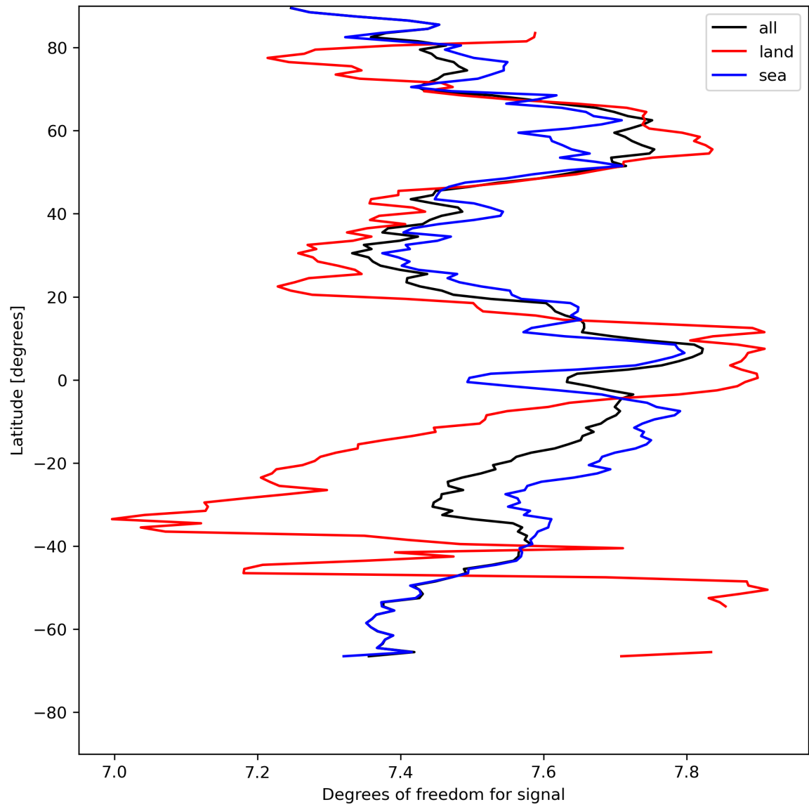
Figure 15: Zonal average of “Degrees of freedom for signal” for 2024-07-31 to 2024-08-01.
