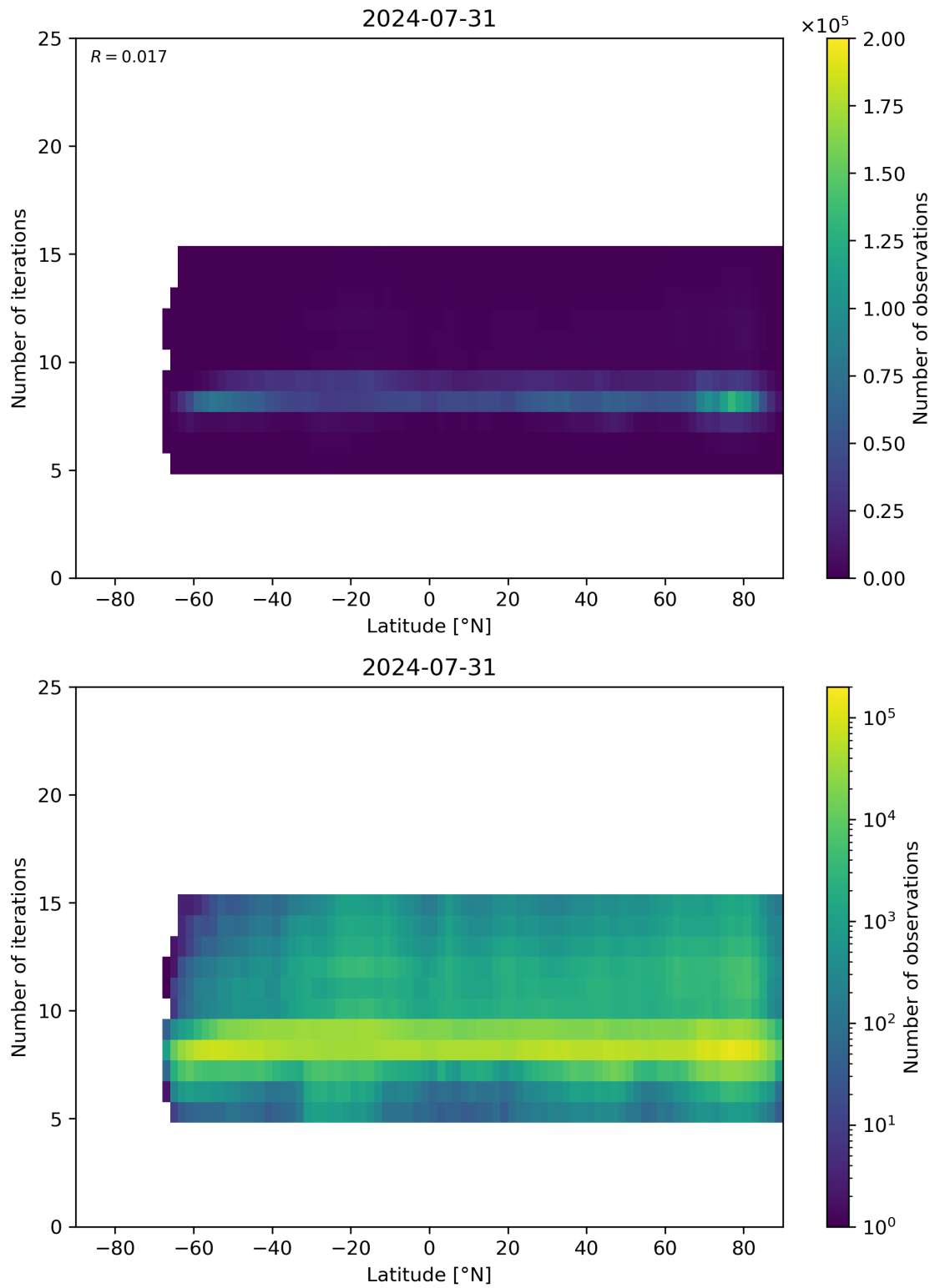
Figure 56: Scatter density plot of “Latitude” against “Number of iterations” for 2024-07-31 to 2024-08-01.
