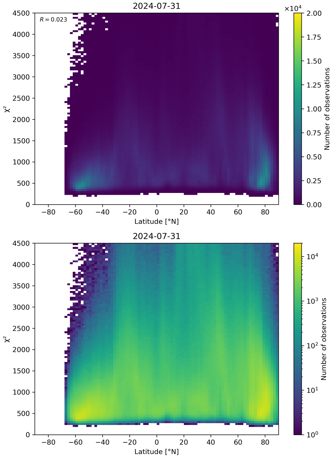
Figure 54: Scatter density plot of “Latitude” against “ \chi^2 ” for 2024-07-31 to 2024-08-01.
