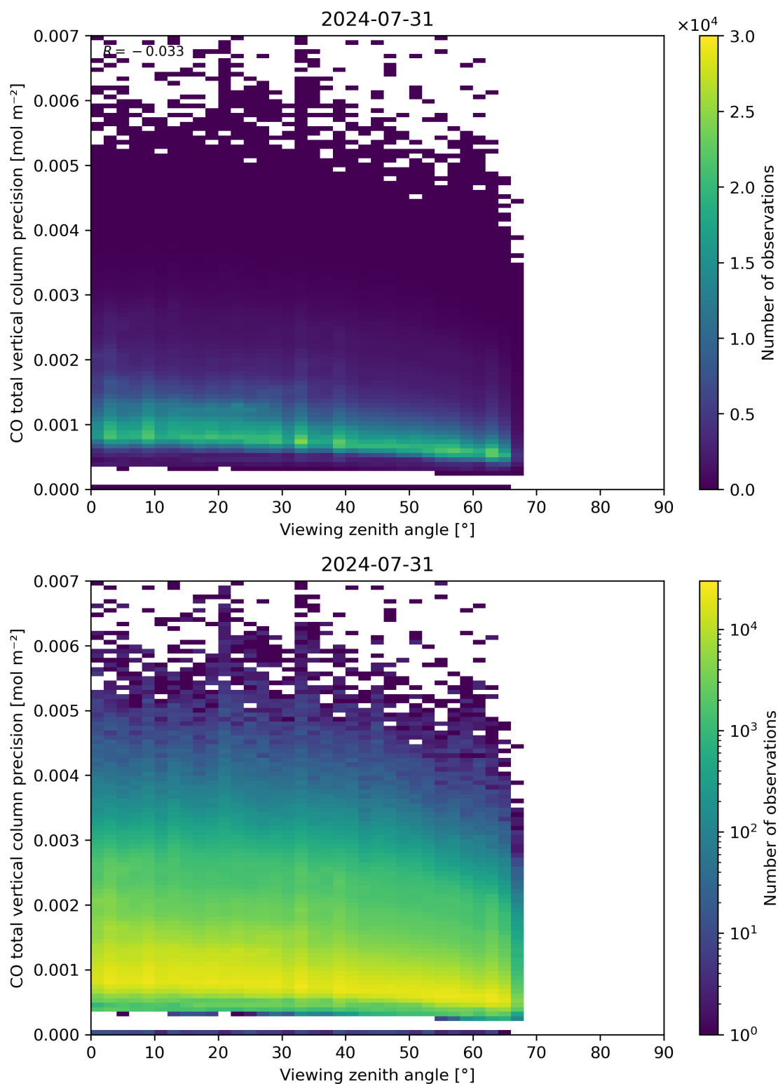
Figure 71: Scatter density plot of “Viewing zenith angle” against “CO total vertical column precision” for 2024-07-31 to 2024-08-01.
