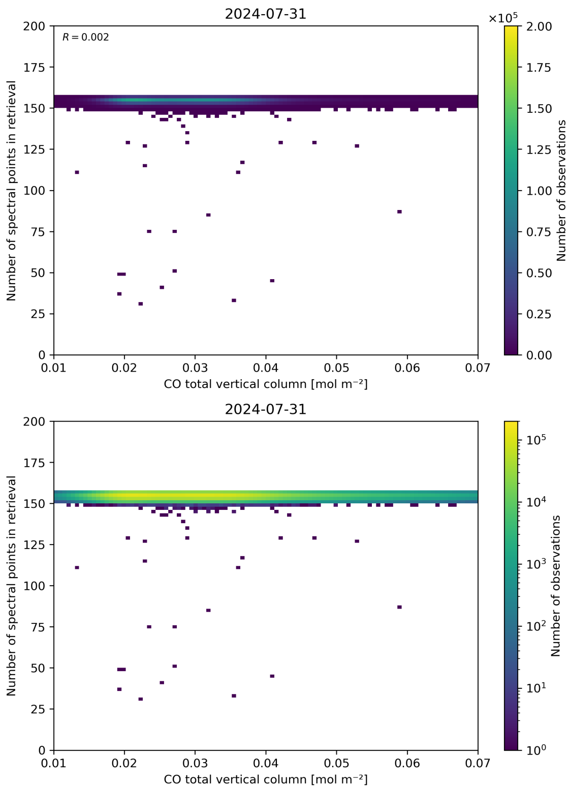
Figure 43: Scatter density plot of “CO total vertical column” against “Number of spectral points in retrieval” for 2024-07-31 to 2024-08-01.
