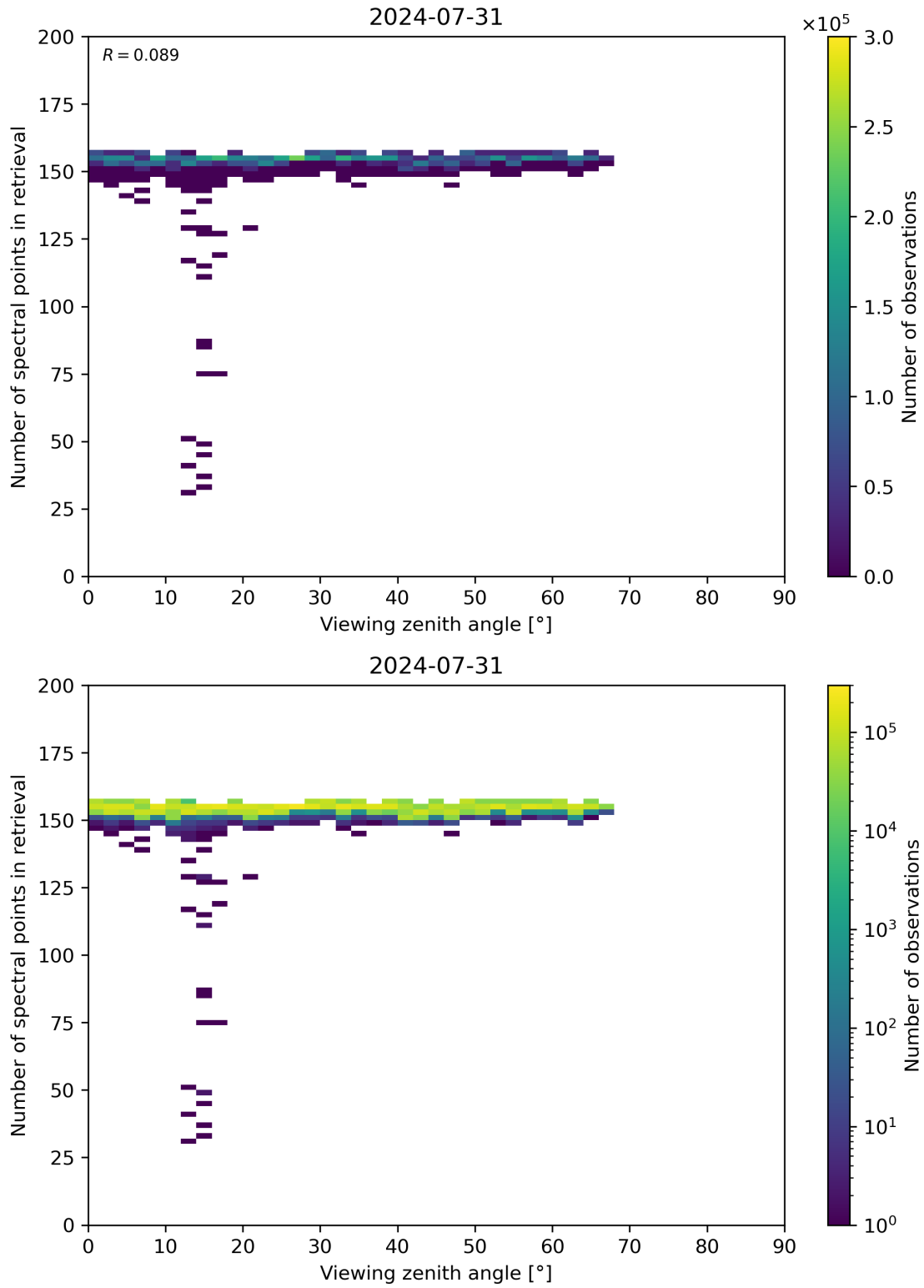
Figure 76: Scatter density plot of “Viewing zenith angle” against “Number of spectral points in retrieval” for 2024-07-31 to 2024-08-01.
