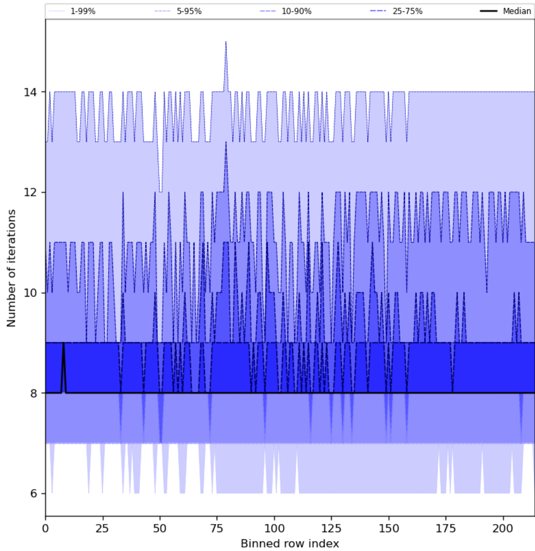
Figure 32: Along track statistics of “Number of iterations” for 2024-07-31 to 2024-08-01
