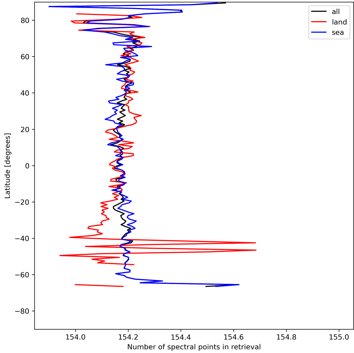
Figure 13: Zonal average of “Number of spectral points in retrieval” for 2024-07-31 to 2024-08-01.
