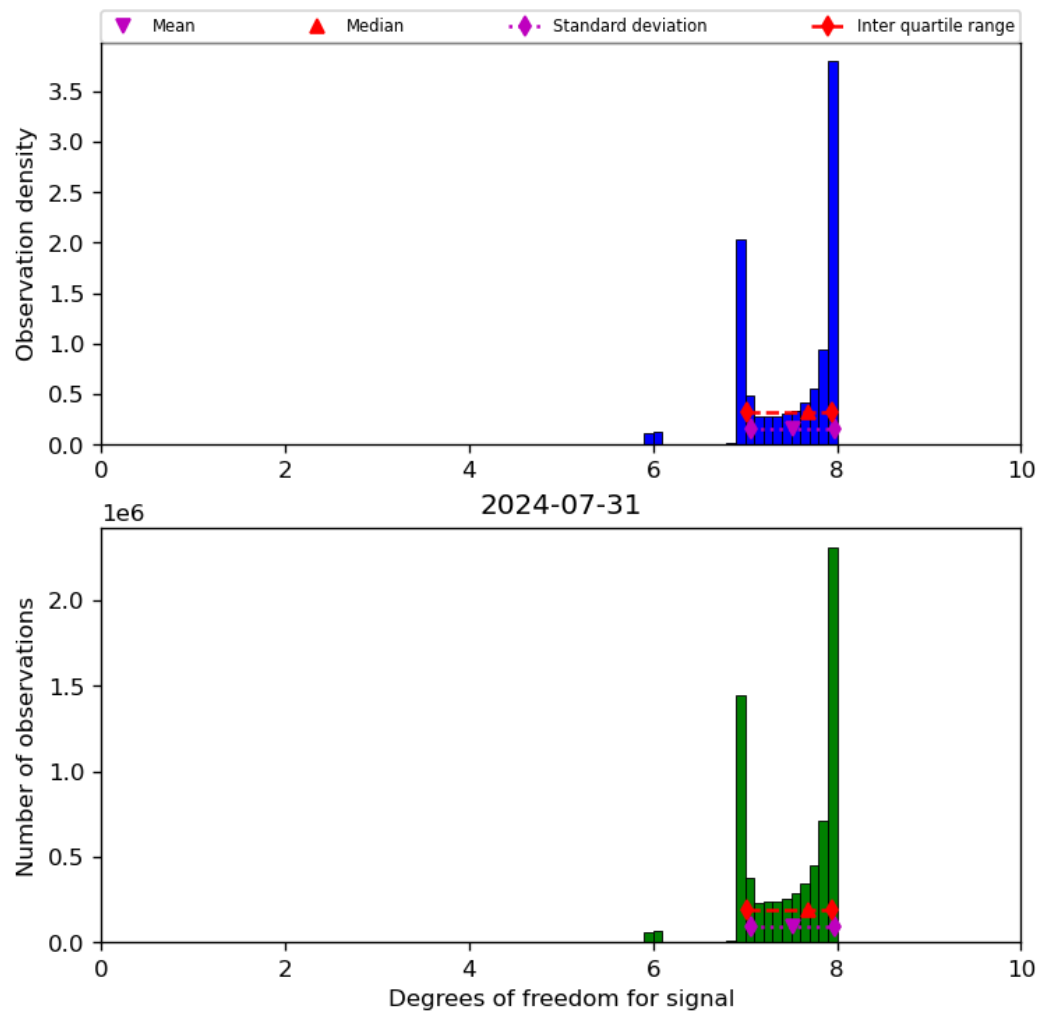
Figure 23: Histogram of “Degrees of freedom for signal” for 2024-07-31 to 2024-08-01
