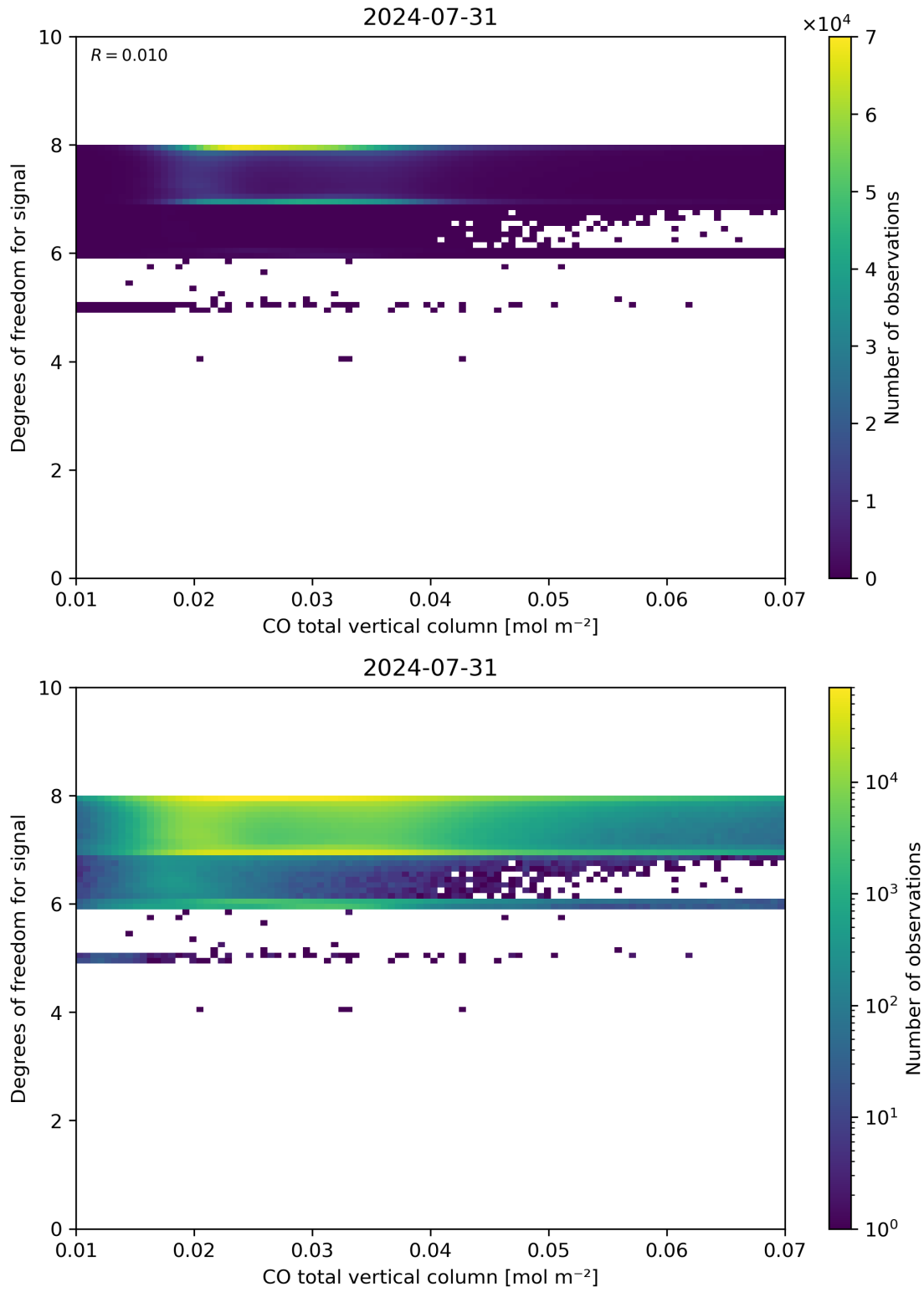
Figure 41: Scatter density plot of “CO total vertical column” against “Degrees of freedom for signal” for 2024-07-31 to 2024-08-01.
