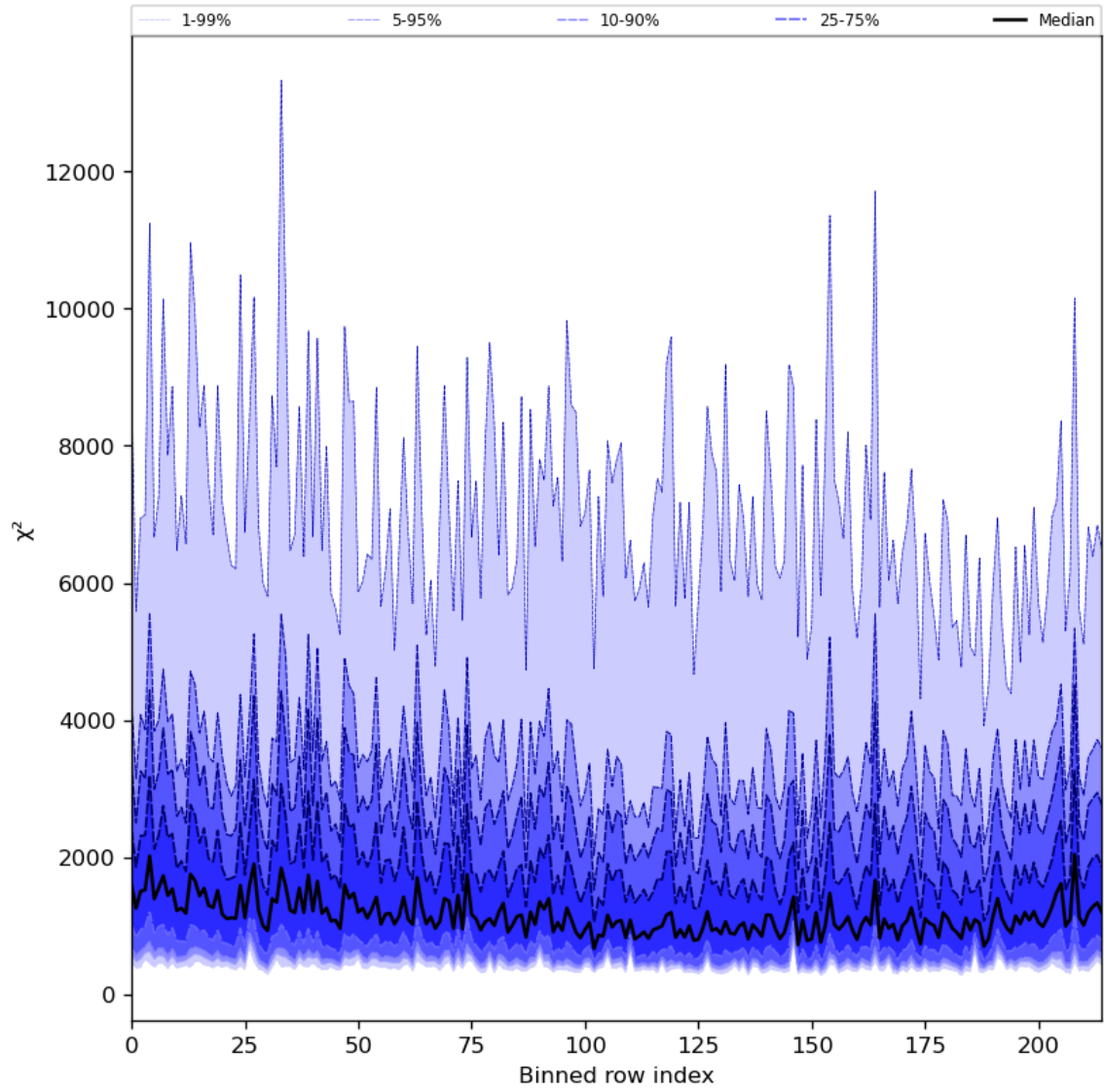
Figure 30: Along track statistics of “ \chi^2 ” for 2024-07-31 to 2024-08-01
