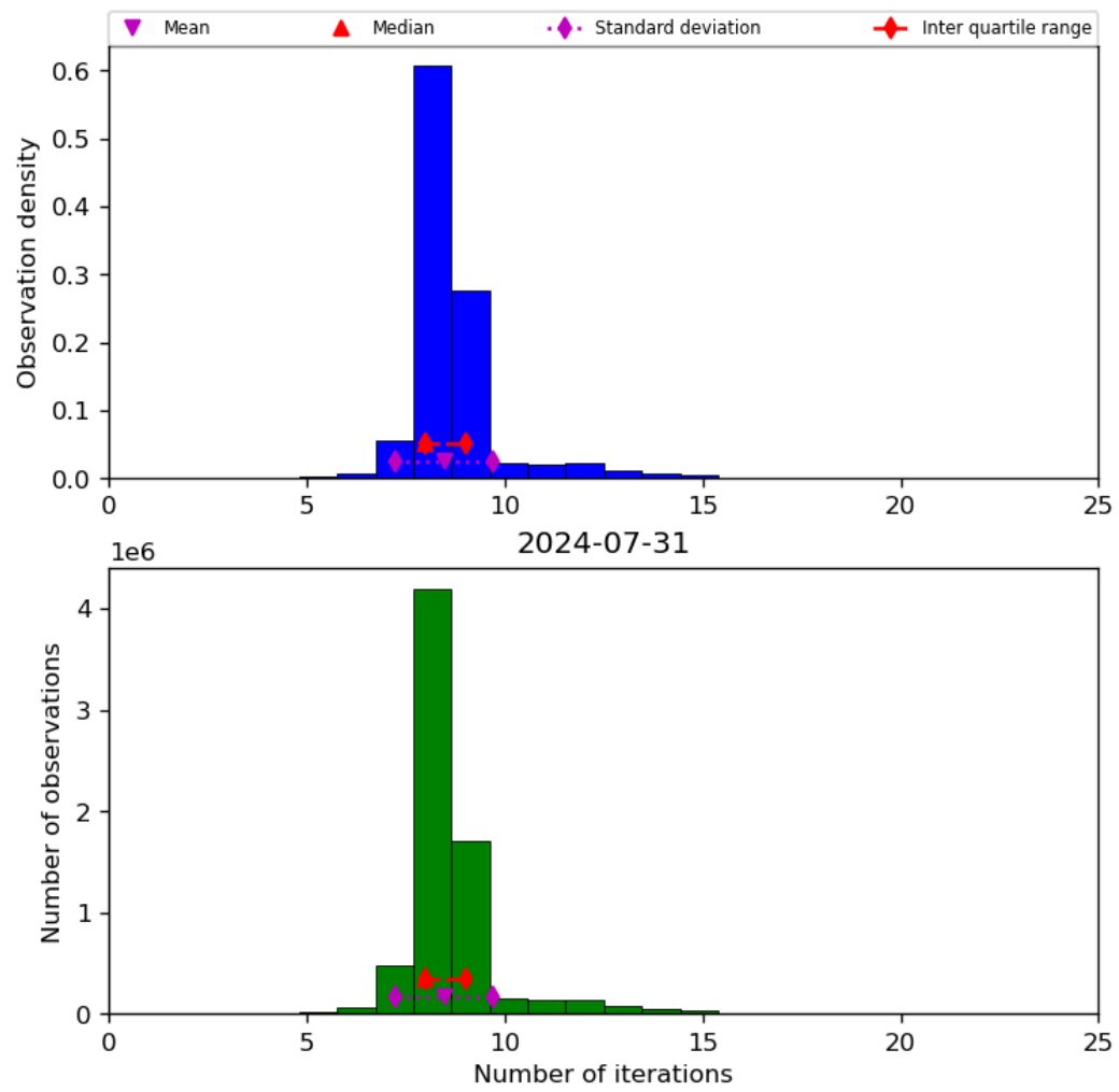
Figure 24: Histogram of “Number of iterations” for 2024-07-31 to 2024-08-01
