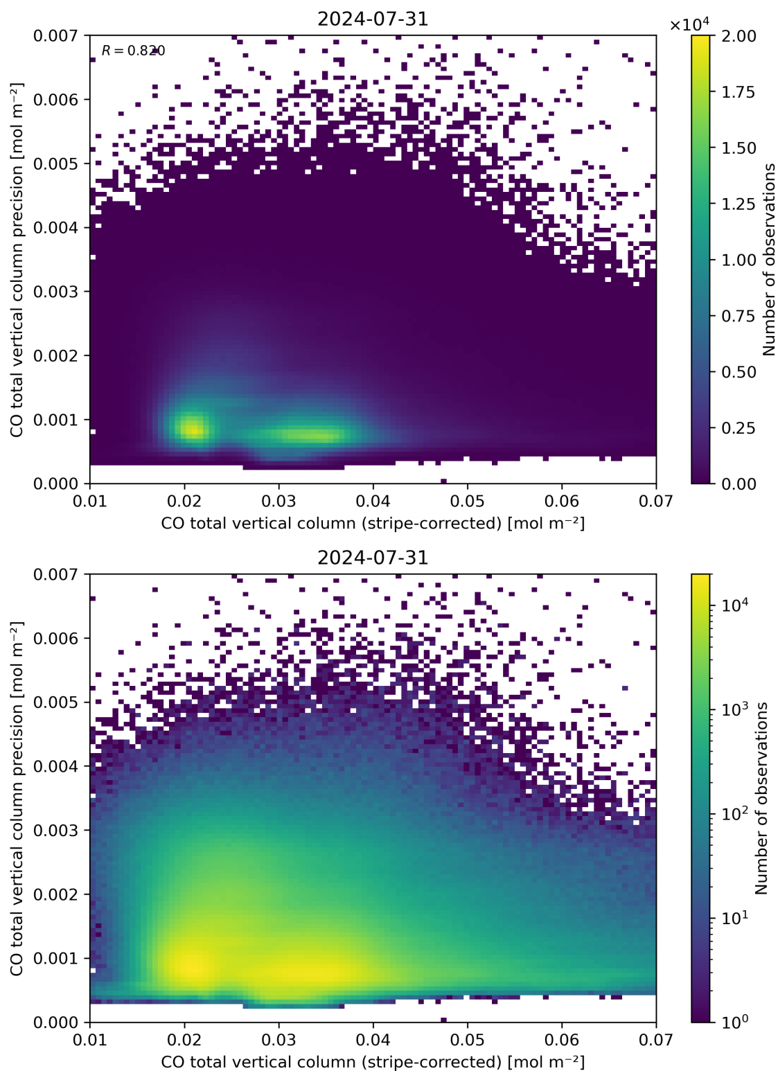
Figure 36: Scatter density plot of “CO total vertical column (stripe-corrected)” against “CO total vertical column precision” for 2024-07-31 to 2024-08-01.
