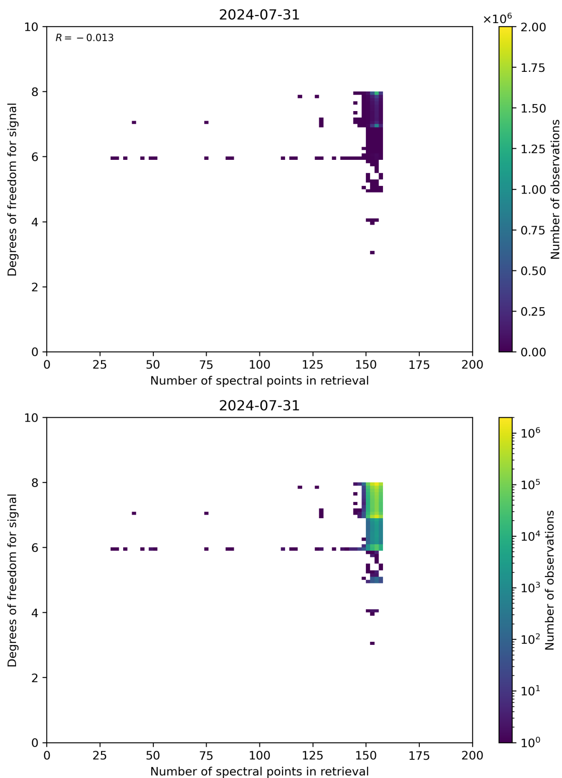
Figure 59: Scatter density plot of “Number of spectral points in retrieval” against “Degrees of freedom for signal” for 2024-07-31 to 2024-08-01.
