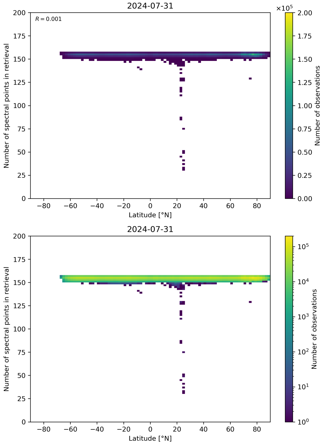
Figure 57: Scatter density plot of “Latitude” against “Number of spectral points in retrieval” for 2024-07-31 to 2024-08-01.
