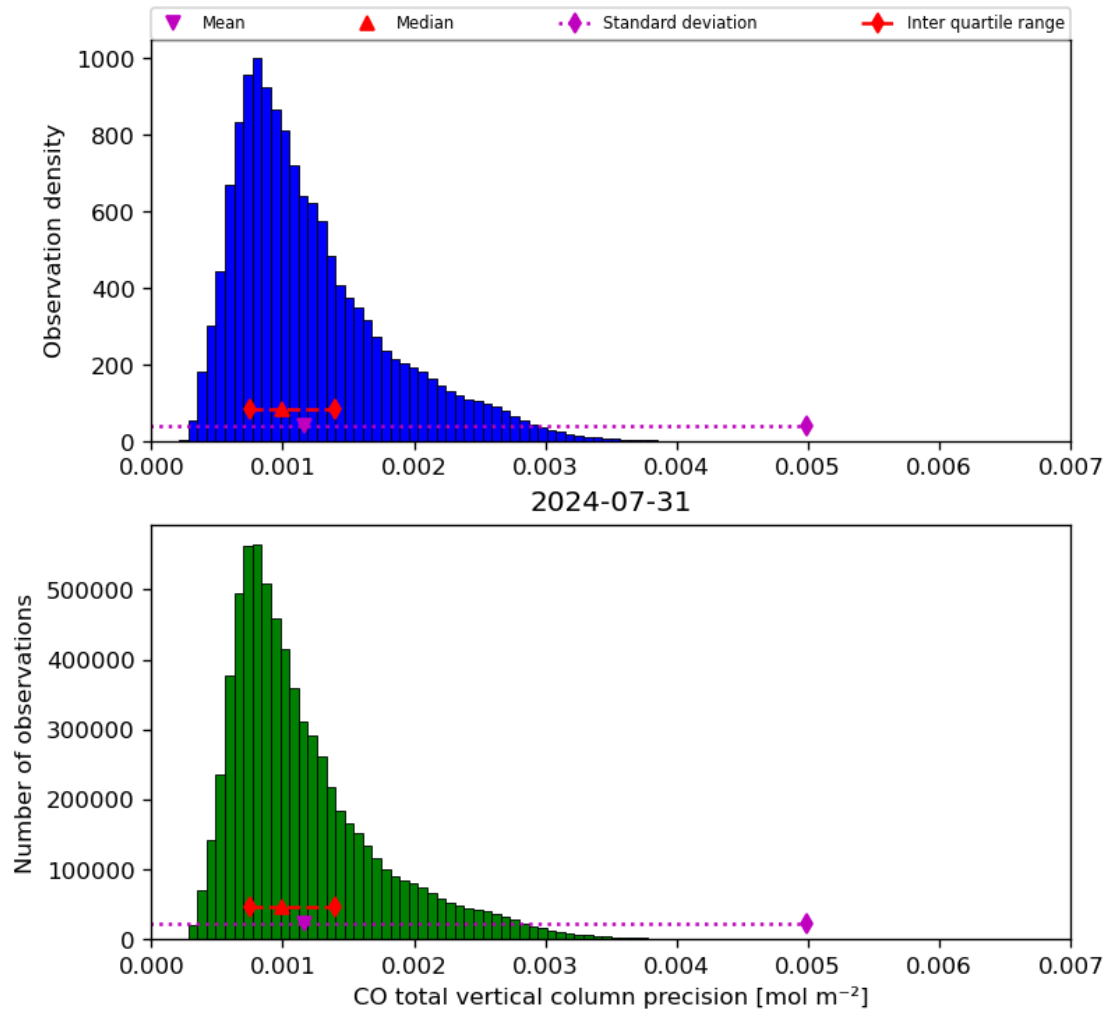
Figure 20: Histogram of “CO total vertical column precision” for 2024-07-31 to 2024-08-01
