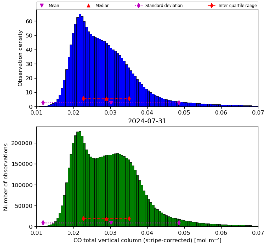
Figure 19: Histogram of “CO total vertical column (stripe-corrected)” for 2024-07-31 to 2024-08-01
