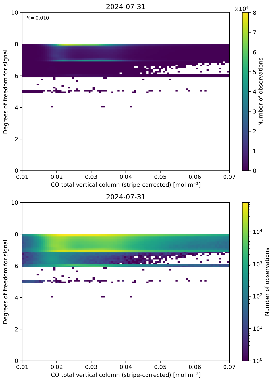
Figure 38: Scatter density plot of “CO total vertical column (stripe-corrected)” against “Degrees of freedom for signal” for 2024-07-31 to 2024-08-01.
