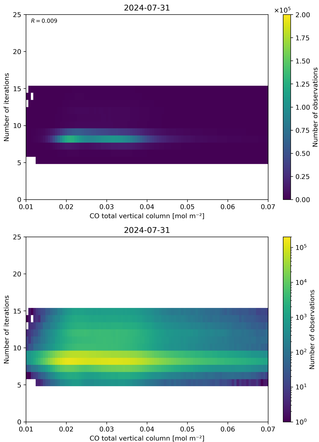
Figure 42: Scatter density plot of “CO total vertical column” against “Number of iterations” for 2024-07-31 to 2024-08-01.
