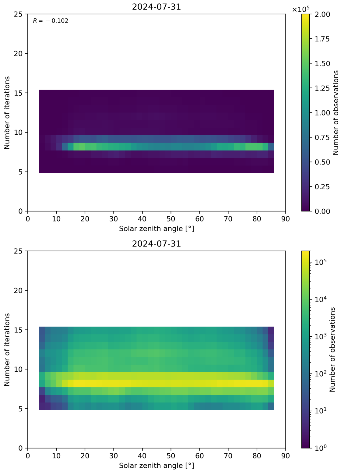
Figure 67: Scatter density plot of “Solar zenith angle” against “Number of iterations” for 2024-07-31 to 2024-08-01.
