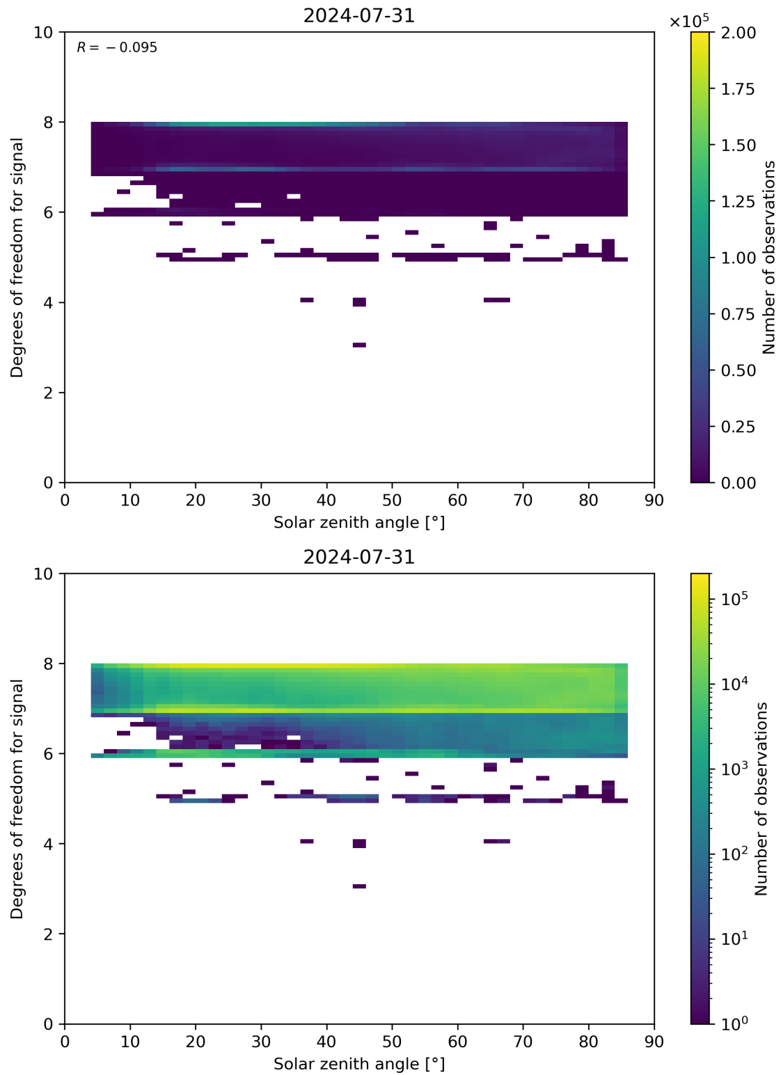
Figure 65: Scatter density plot of “Solar zenith angle” against “Degrees of freedom for signal” for 2024-07-31 to 2024-08-01.
