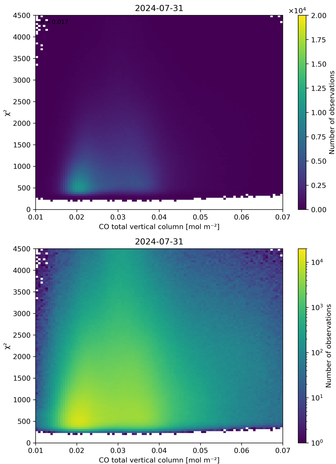
Figure 35: Scatter density plot of “CO total vertical column” against “ \chi^2 ” for 2024-07-31 to 2024-08-01.
