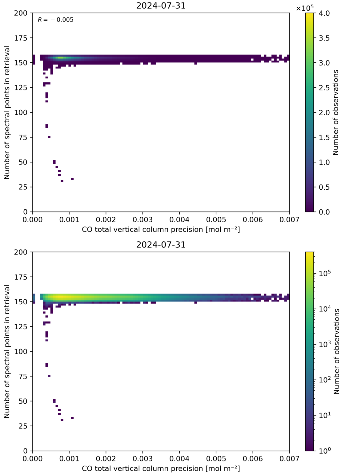
Figure 47: Scatter density plot of “CO total vertical column precision” against “Number of spectral points in retrieval” for 2024-07-31 to 2024-08-01.
