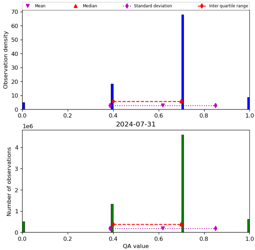
Figure 17: Histogram of “QA value” for 2024-07-31 to 2024-08-01
