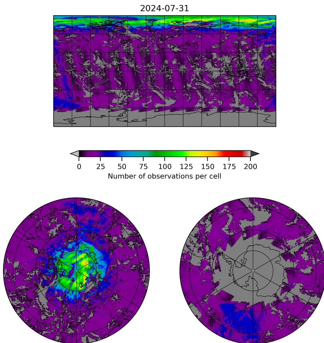
Figure 8: Map of the number of observations for 2024-07-31 to 2024-08-01
