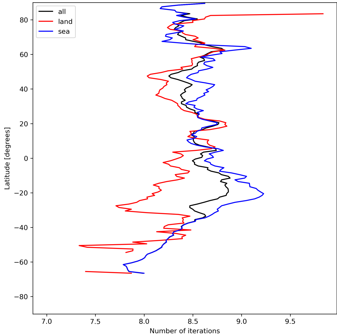
Figure 16: Zonal average of “Number of iterations” for 2024-07-31 to 2024-08-01.
