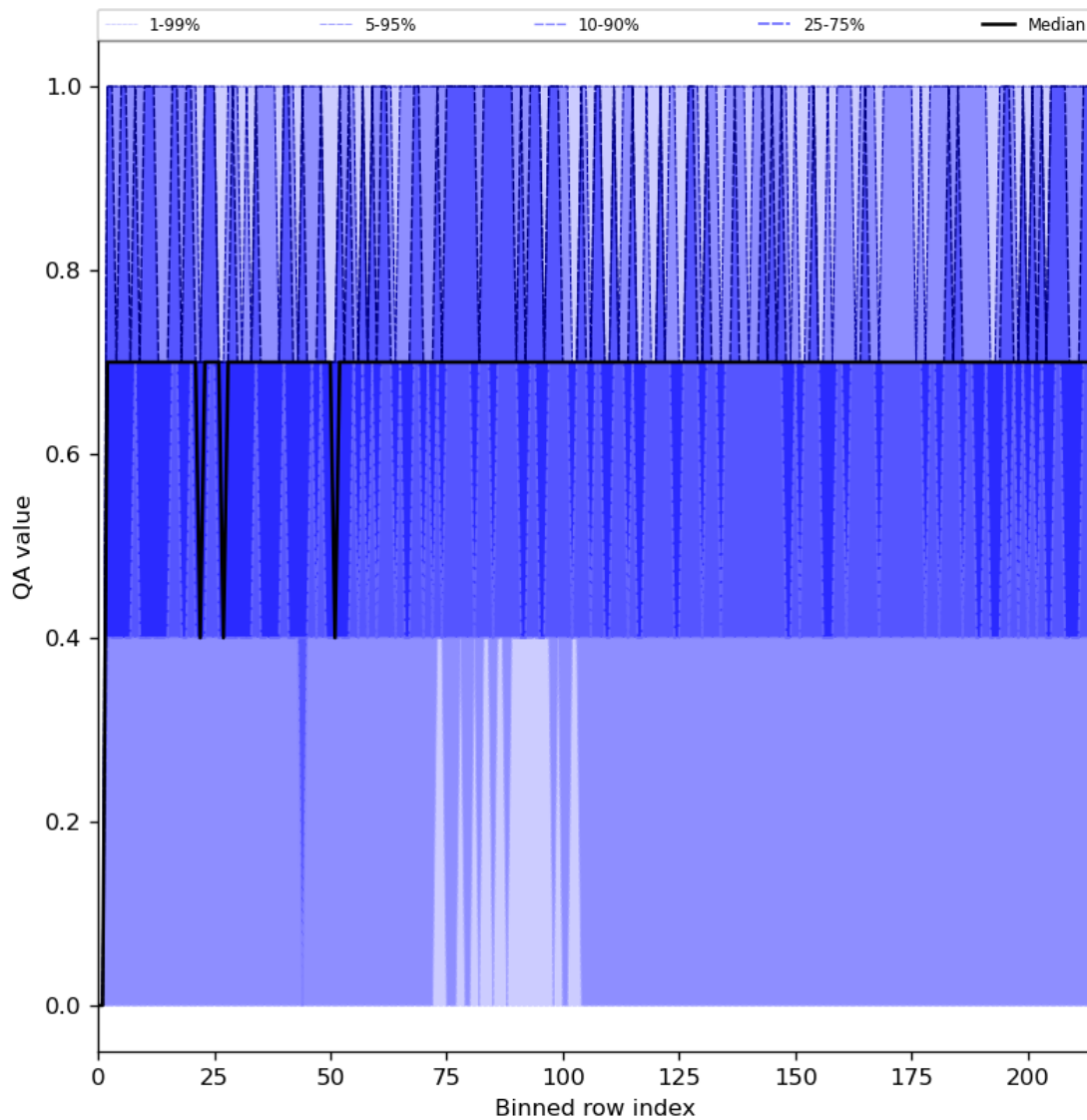
Figure 25: Along track statistics of “QA value” for 2024-07-31 to 2024-08-01
