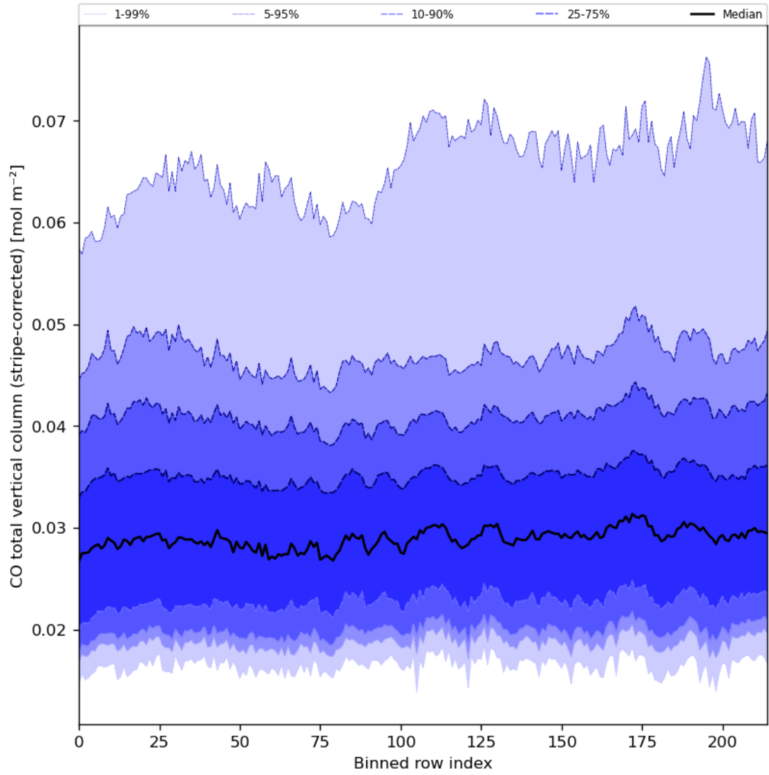
Figure 27: Along track statistics of “CO total vertical column (stripe-corrected)” for 2024-07-31 to 2024-08-01
