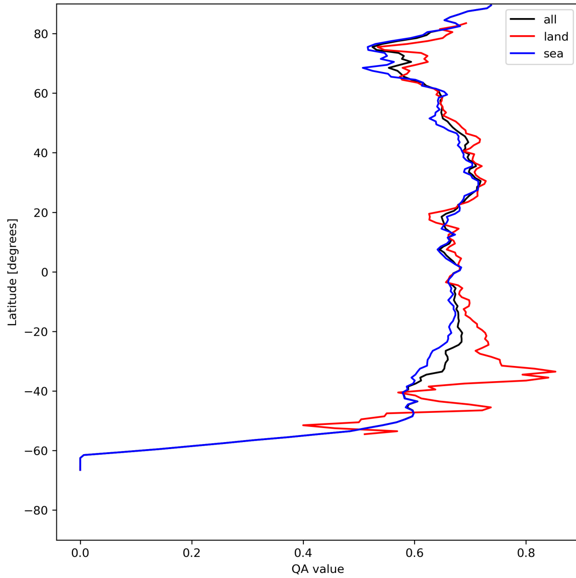
Figure 9: Zonal average of “QA value” for 2024-07-31 to 2024-08-01.
