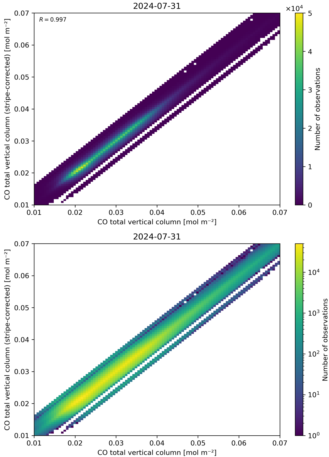
Figure 33: Scatter density plot of “CO total vertical column” against “CO total vertical column (stripe-corrected)” for 2024-07-31 to 2024-08-01.
