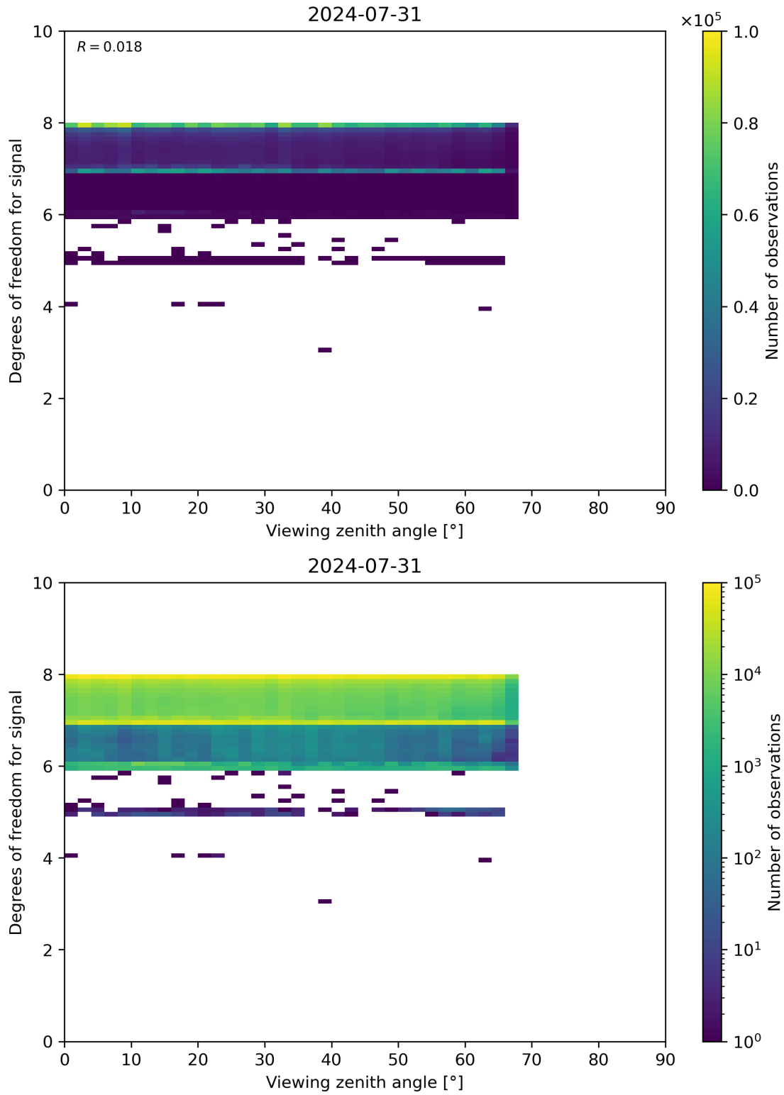
Figure 73: Scatter density plot of “Viewing zenith angle” against “Degrees of freedom for signal” for 2024-07-31 to 2024-08-01.
