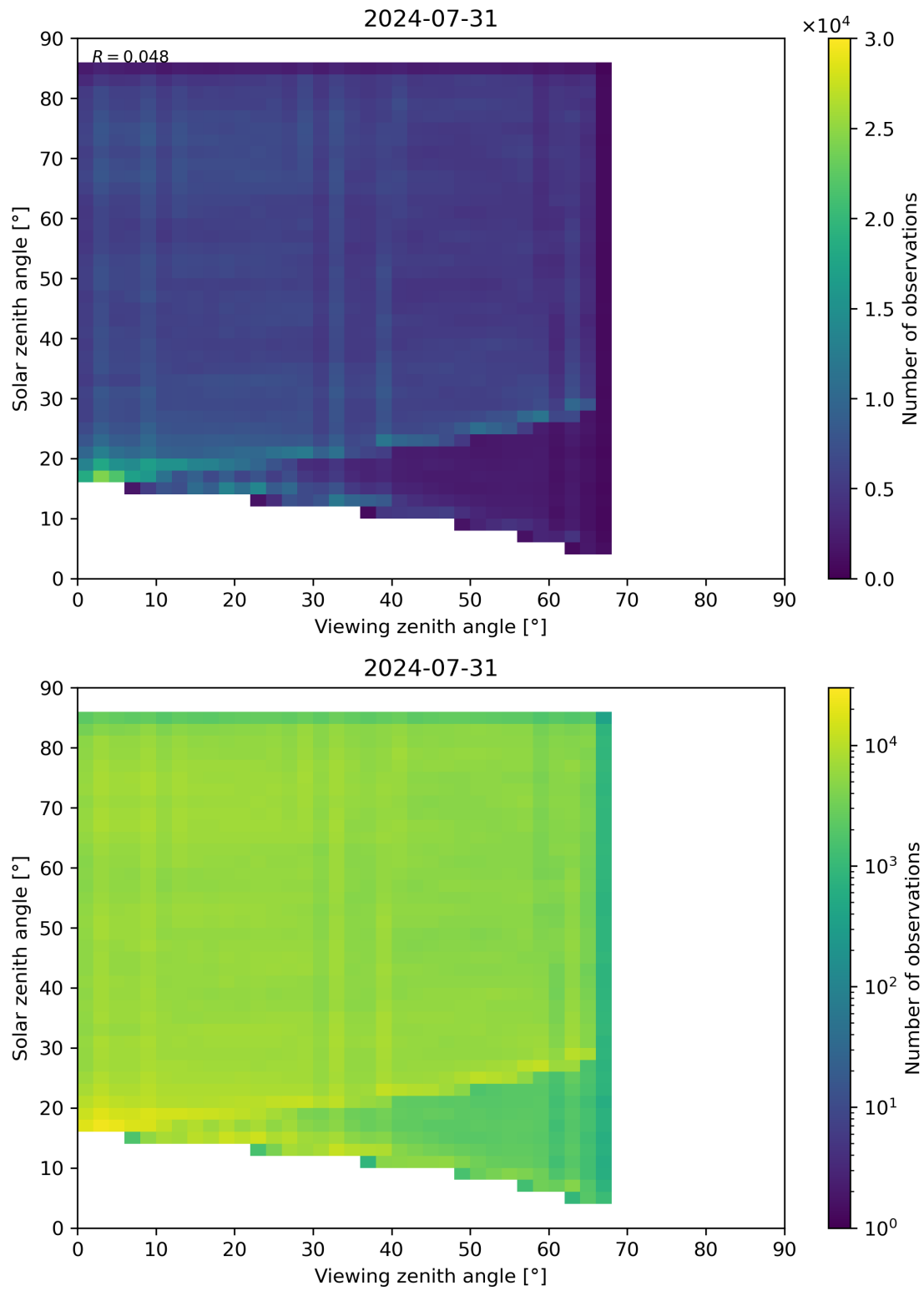
Figure 77: Scatter density plot of “Viewing zenith angle” against “Solar zenith angle” for 2024-07-31 to 2024-08-01.
