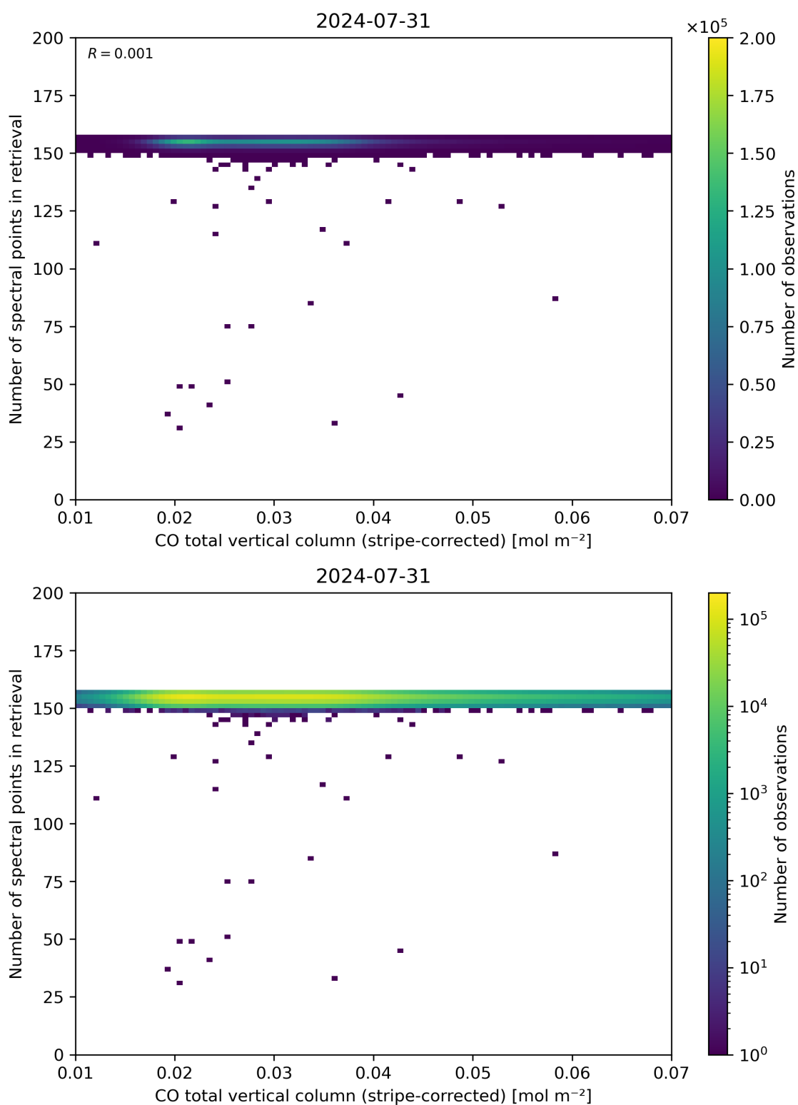
Figure 40: Scatter density plot of “CO total vertical column (stripe-corrected)” against “Number of spectral points in retrieval” for 2024-07-31 to 2024-08-01.
