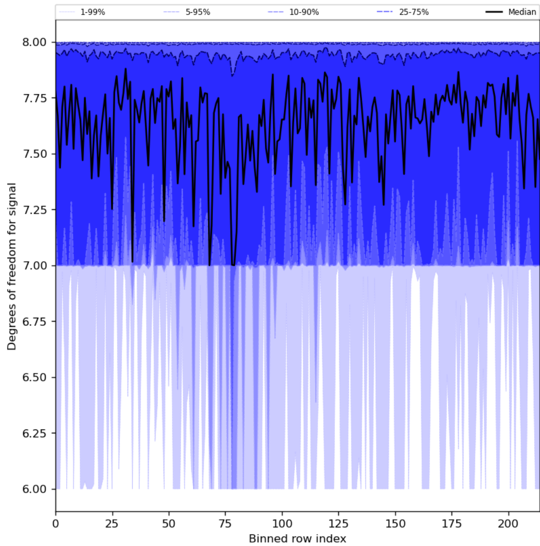
Figure 31: Along track statistics of “Degrees of freedom for signal” for 2024-07-31 to 2024-08-01
