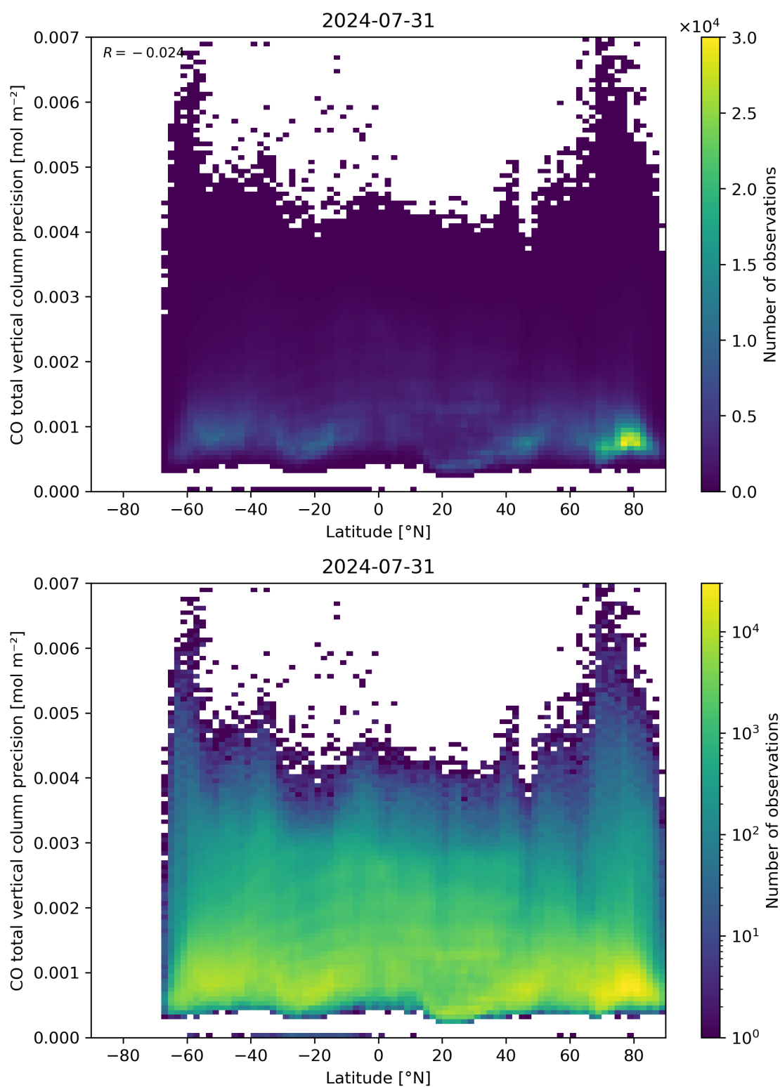
Figure 53: Scatter density plot of “Latitude” against “CO total vertical column precision” for 2024-07-31 to 2024-08-01.
