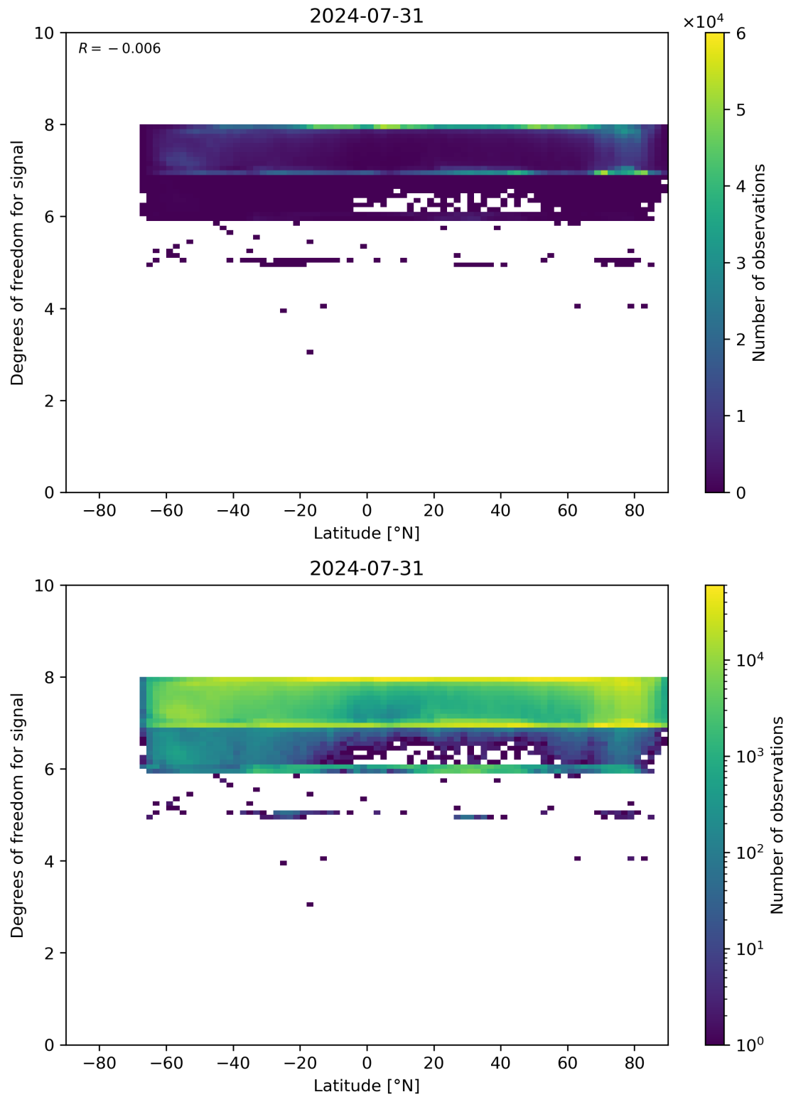
Figure 55: Scatter density plot of “Latitude” against “Degrees of freedom for signal” for 2024-07-31 to 2024-08-01.
