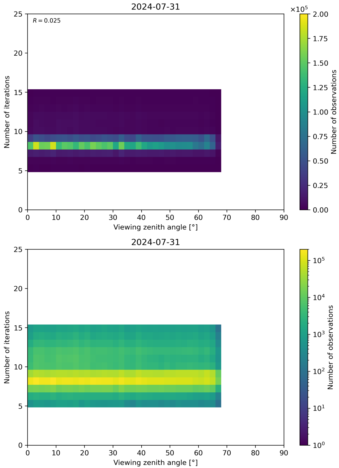
Figure 75: Scatter density plot of “Viewing zenith angle” against “Number of iterations” for 2024-07-31 to 2024-08-01.
