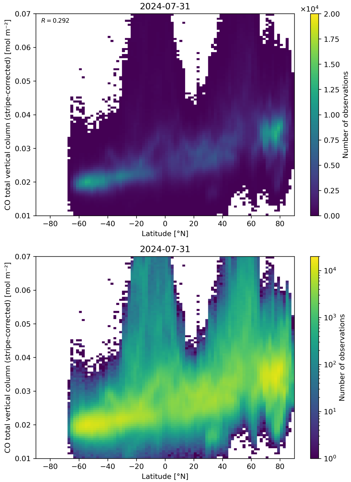
Figure 52: Scatter density plot of “Latitude” against “CO total vertical column (stripe-corrected)” for 2024-07-31 to 2024-08-01.
