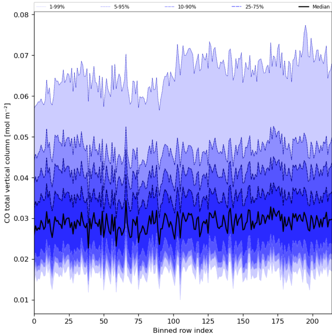
Figure 26: Along track statistics of “CO total vertical column” for 2024-07-31 to 2024-08-01
