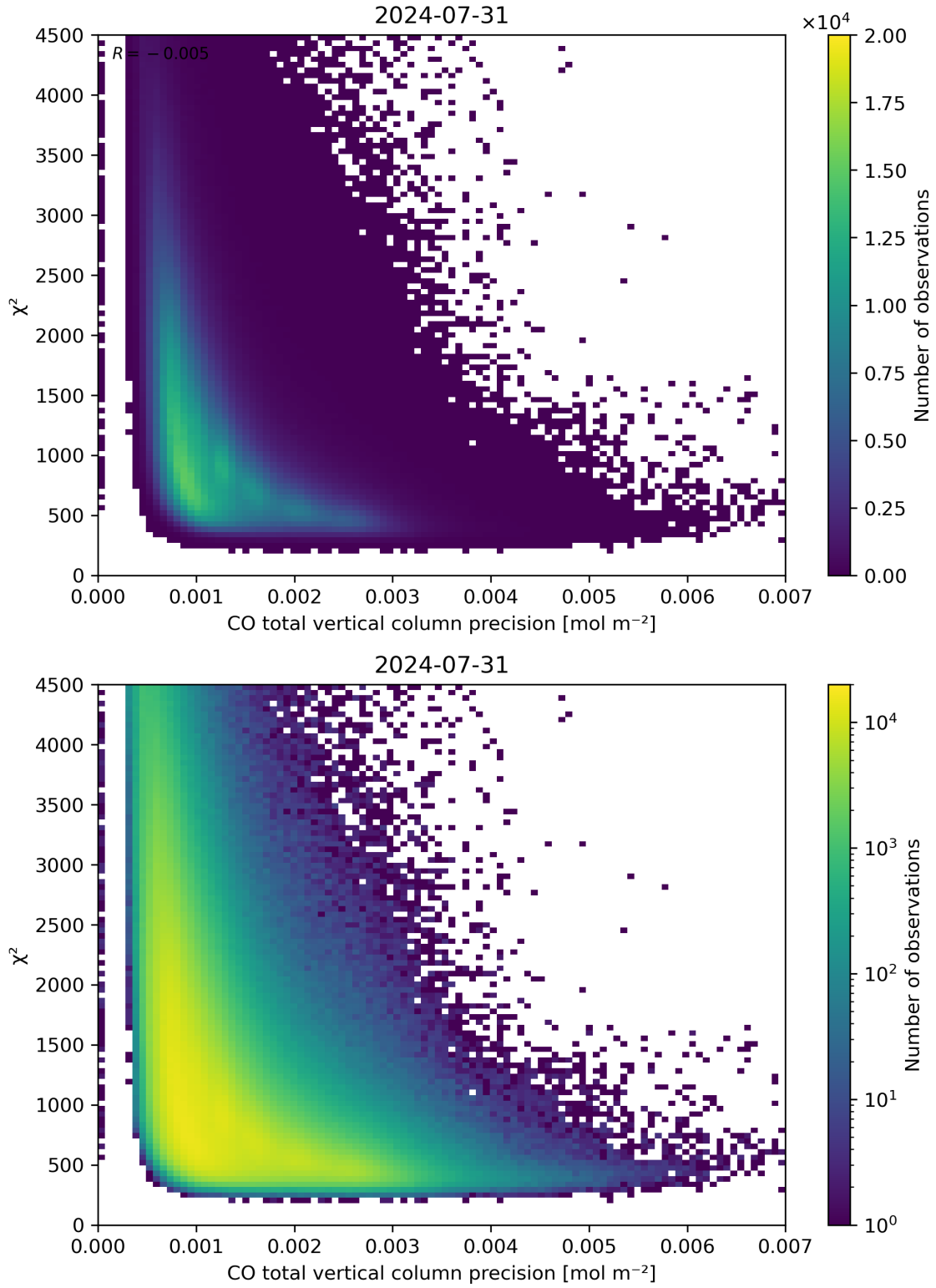
Figure 44: Scatter density plot of “CO total vertical column precision” against “ \chi^2 ” for 2024-07-31 to 2024-08-01.
