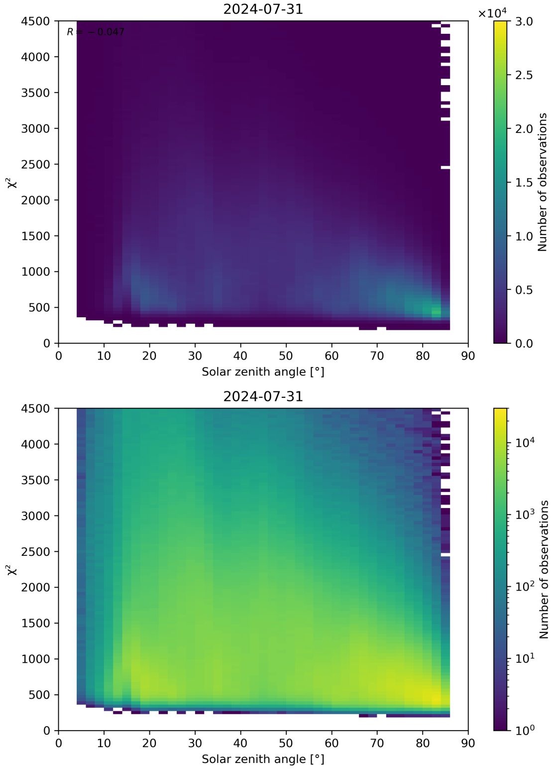
Figure 64: Scatter density plot of “Solar zenith angle” against “ \chi^2 ” for 2024-07-31 to 2024-08-01.
