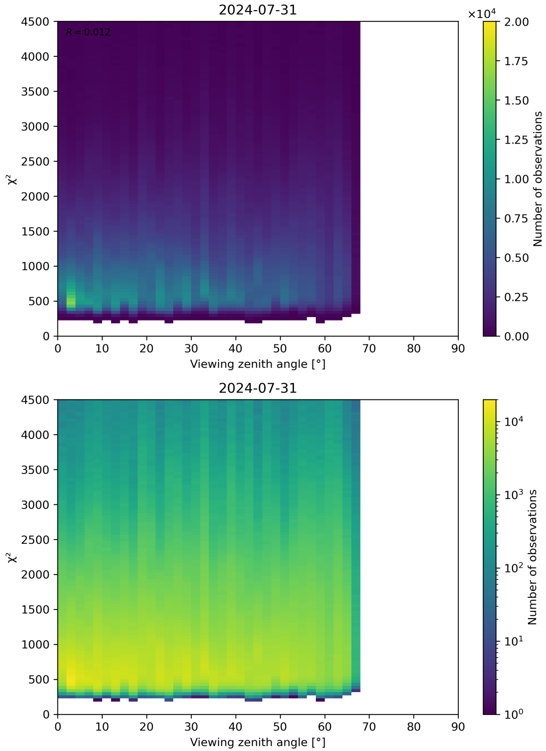
Figure 72: Scatter density plot of “Viewing zenith angle” against “ \chi^2 ” for 2024-07-31 to 2024-08-01.
