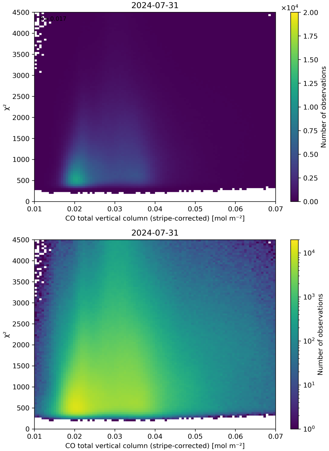
Figure 37: Scatter density plot of “CO total vertical column (stripe-corrected)” against “ \chi^2 ” for 2024-07-31 to 2024-08-01.
