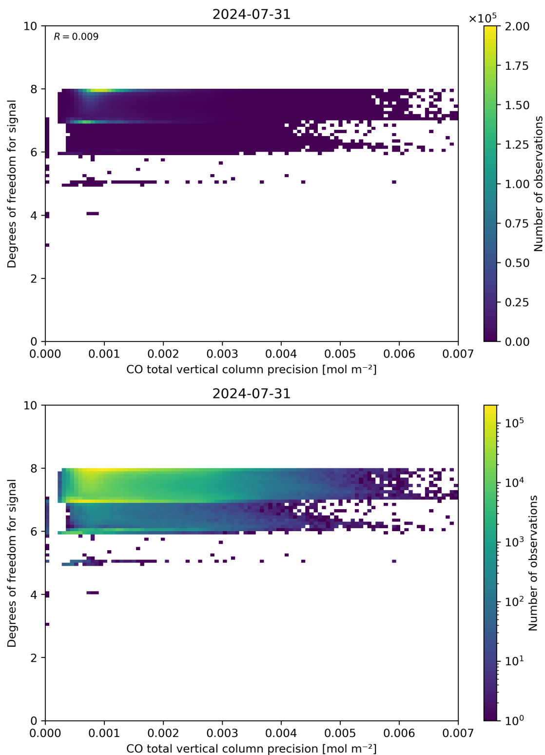
Figure 45: Scatter density plot of “CO total vertical column precision” against “Degrees of freedom for signal” for 2024-07-31 to 2024-08-01.
