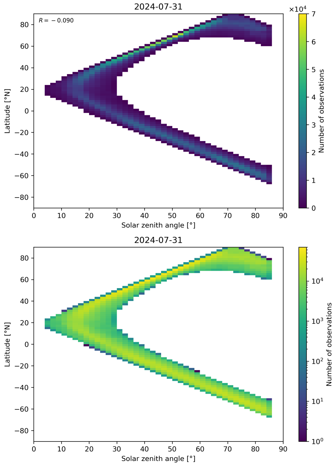
Figure 66: Scatter density plot of “Solar zenith angle” against “Latitude” for 2024-07-31 to 2024-08-01.
