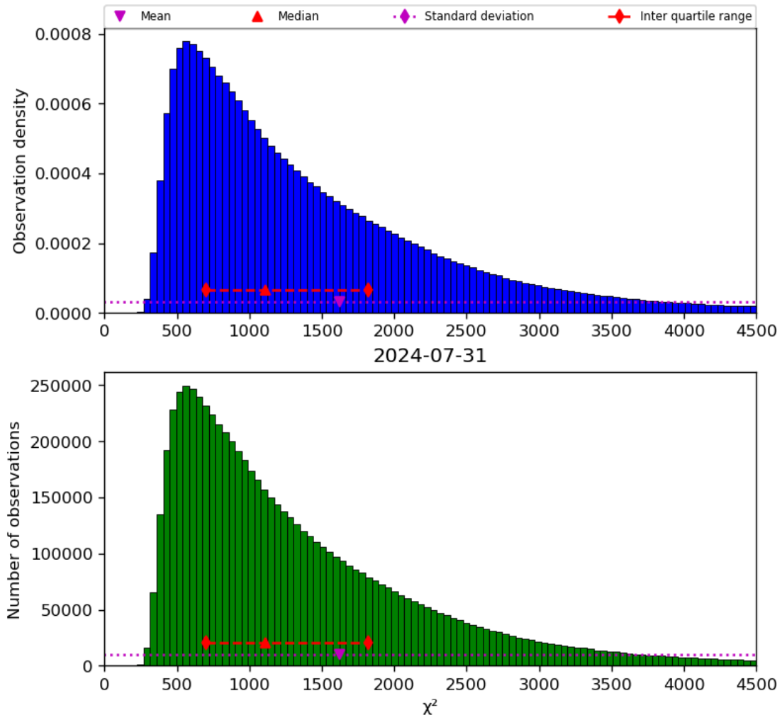
Figure 22: Histogram of " \chi^2 " for 2024-07-31 to 2024-08-01
